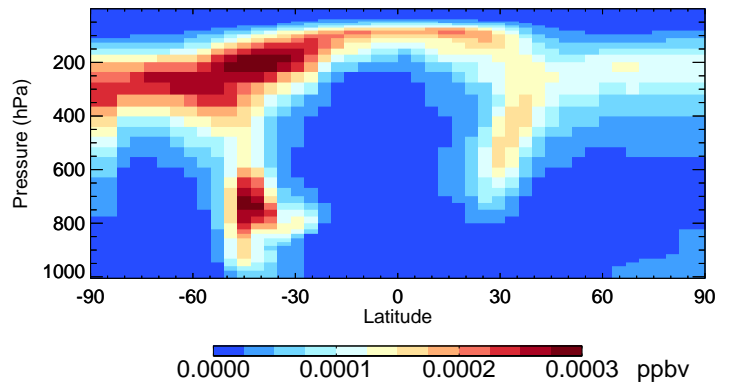
v11-02c TSOA1 - Species Curtain @ -180.000 for Jan
