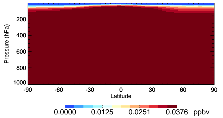
v11-02a HCFC141b - Species Curtain @ -180.000 for Jan
