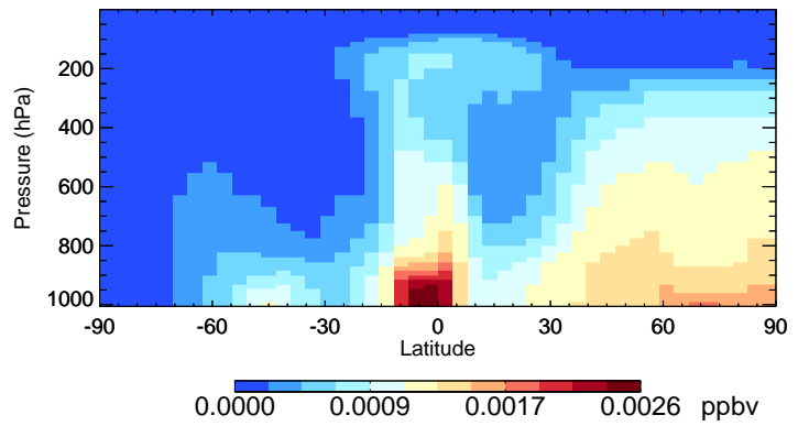
v11-02c CHBr3 - Species Curtain @ -180.000 for Jan
