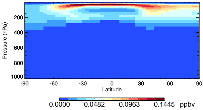
v11-01-public-Run0 MPN - Species Zonal Mean for Jan
