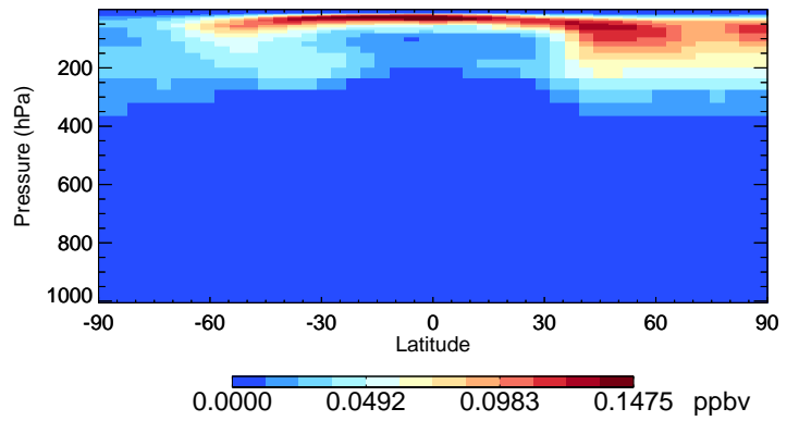
v11-02c MPN - Species Curtain @ -180.000 for Jan
