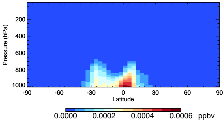
v11-01-public-Run0 MOBA - Species Zonal Mean for Jan
