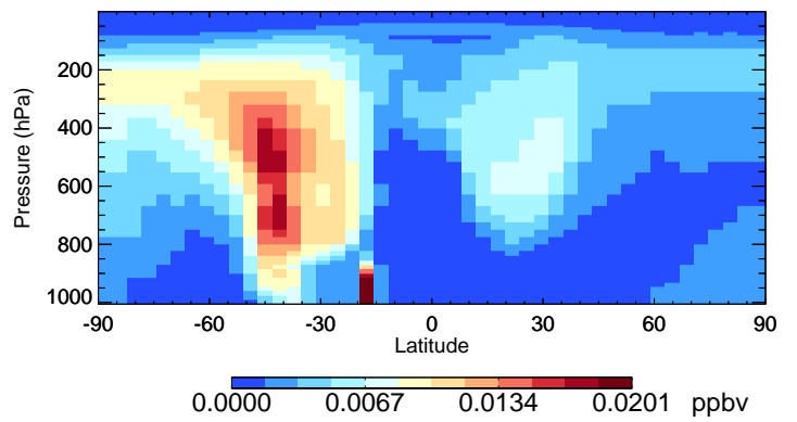
v11-02c TSOG3 - Species Curtain @ -180.000 for Jan
