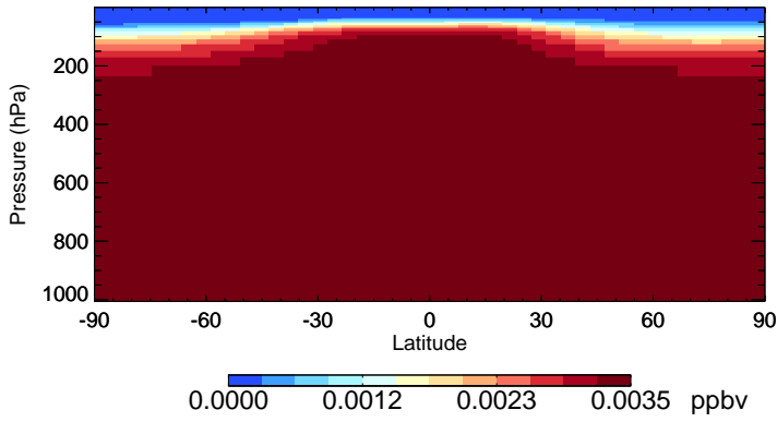
v11-02a H1211 - Species Zonal Mean for Jan
