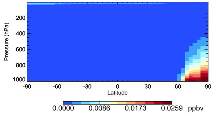
v11-02a HNO2 - Species Curtain @ -180.000 for Jan
