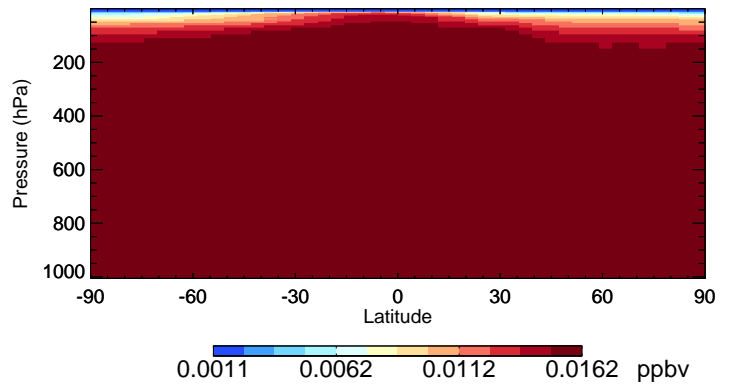
v11-02c CFC114 - Species Curtain @ -180.000 for Jan
