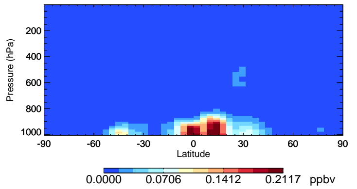
v11-01-public-Run0 NH3 - Species Curtain @ -180.000 for Jan
