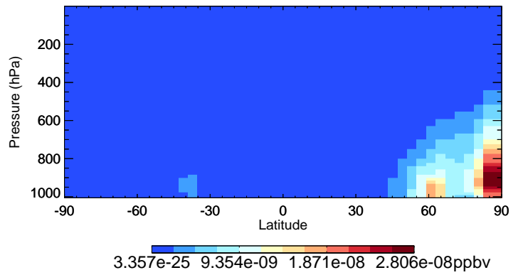
v11-02c NPMN - Species Curtain @ -180.000 for Jan
