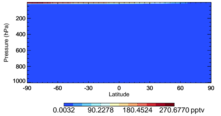
v11-01-public-Run0 HO2 - Species Curtain @ -180.000 for Jan
