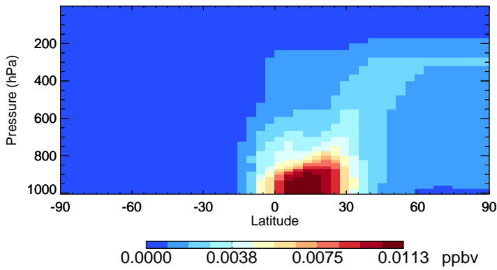
v11-02c ASOAN - Species Zonal Mean for Jan
