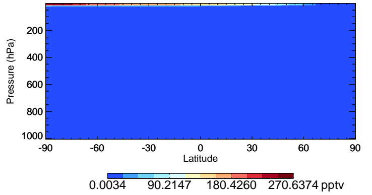
v11-02a HO2 - Species Curtain @ -180.000 for Jan
