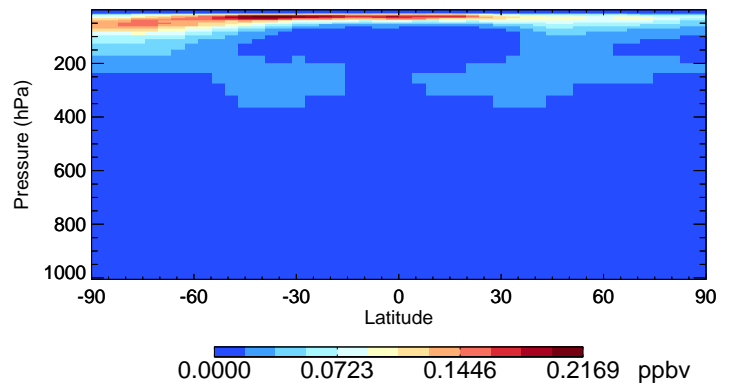
v11-02a HNO4 - Species Curtain @ -180.000 for Jan
