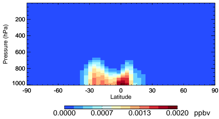
v11-02a ISOPNB - Species Zonal Mean for Jan
