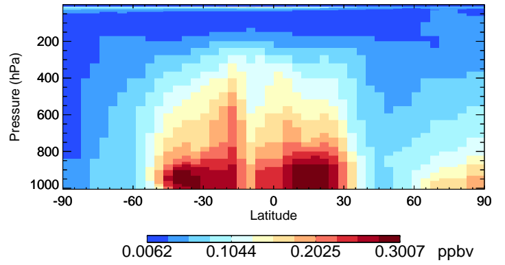
v11-02a CH2O - Species Curtain @ -180.000 for Jan
