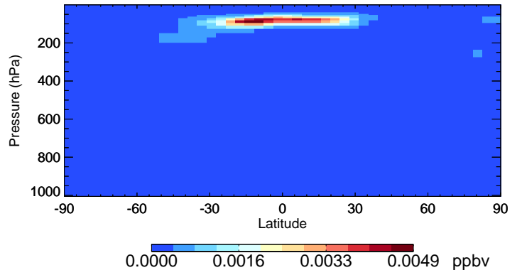
v11-02a ISOA3 - Species Curtain @ -180.000 for Jan
