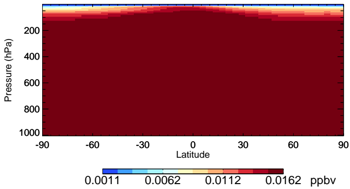
v11-02c CFC114 - Species Zonal Mean for Jan
