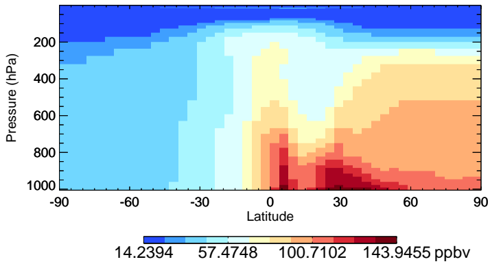
v11-01-public-Run0 CO - Species Zonal Mean for Jan
