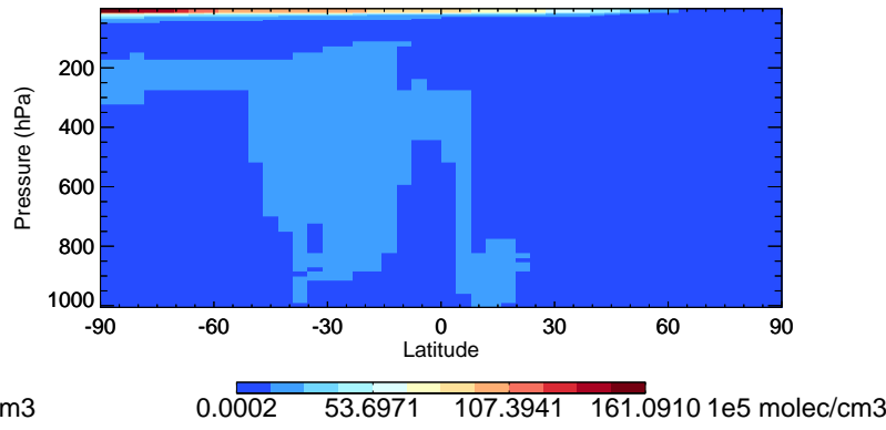
v11-01-public-Run0 OH - Species Curtain @ -180.000 for Jan
