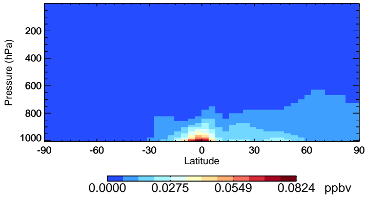
v11-02a RCHO - Species Zonal Mean for Jan
