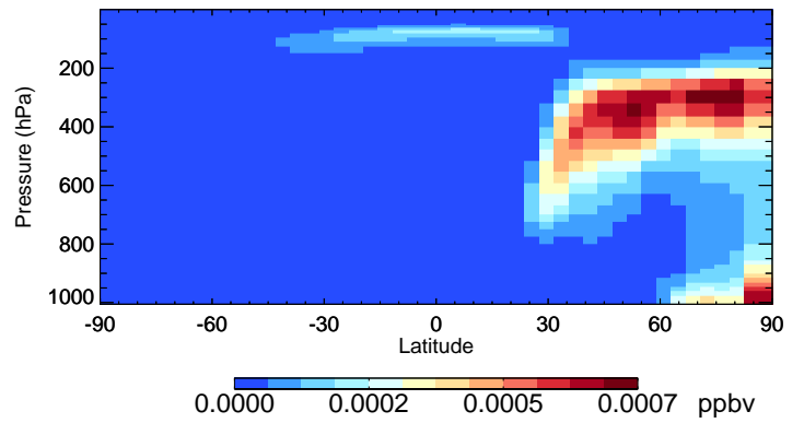
v11-02c ASOA2 - Species Curtain @ -180.000 for Jan
