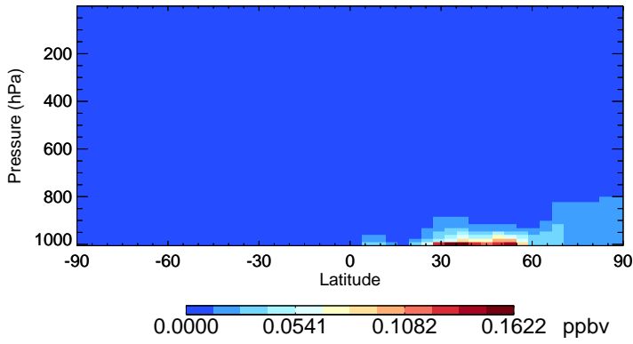
v11-02a HNO2 - Species Zonal Mean for Jan
