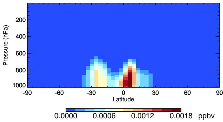
v11-01-public-Run0 MACRN - Species Zonal Mean for Jan
