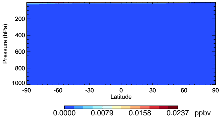
v11-01-public-Run0 Br - Species Zonal Mean for Jan
