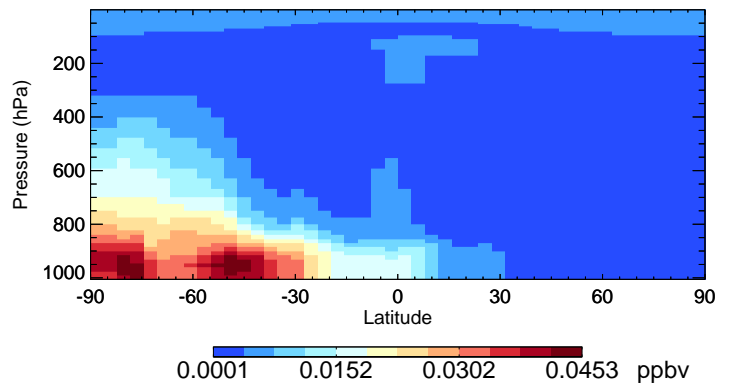
v11-01-public-Run0 MSA - Species Curtain @ -180.000 for Jan
