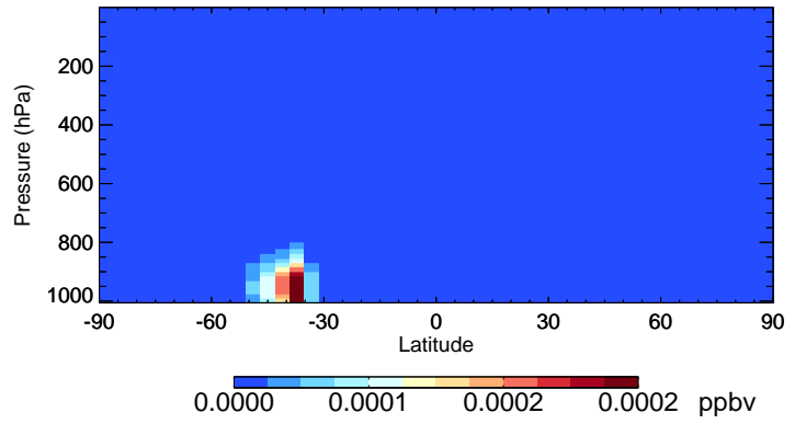
v11-02a NPMN - Species Curtain @ -180.000 for Jan
