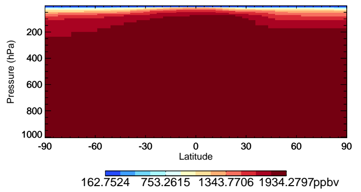
v11-02a CH4 - Species Curtain @ -180.000 for Jan
