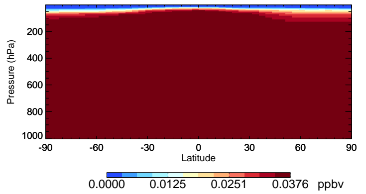
v11-01-public-Run0 HCFC141b - Species Curtain @ -180.000 for Jan
