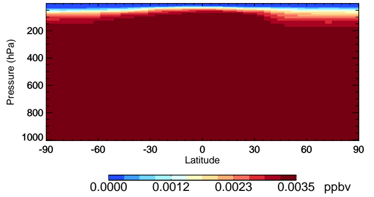
v11-02a H1301 - Species Curtain @ -180.000 for Jan
