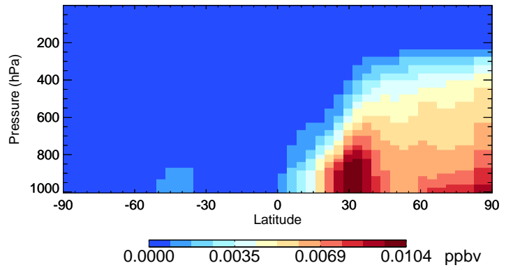
v11-01-public-Run0 RCHO - Species Curtain @ -180.000 for Jan
