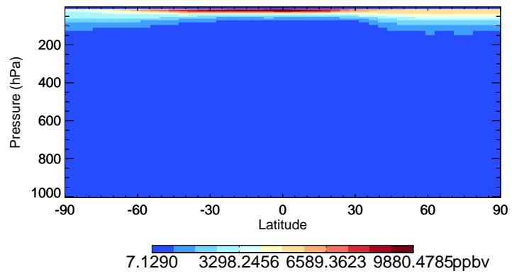
v11-01-public-Run0 O3 - Species Curtain @ -180.000 for Jan
