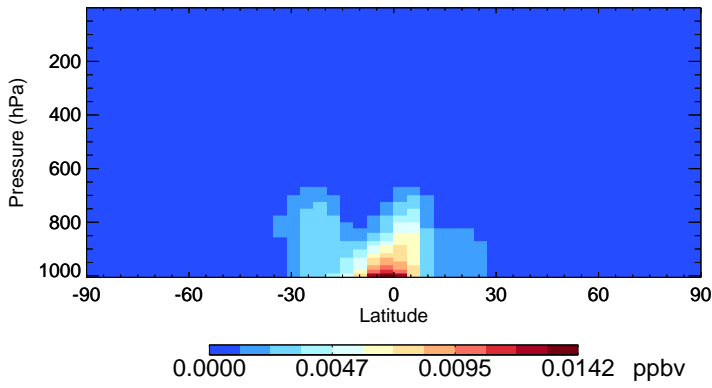
v11-01-public-Run0 TSOA1 - Species Zonal Mean for Jan
