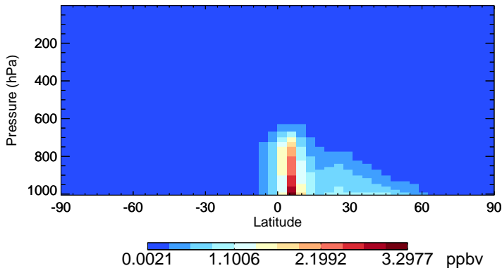
v11-01-public-Run0 OCPI - Species Zonal Mean for Jan
