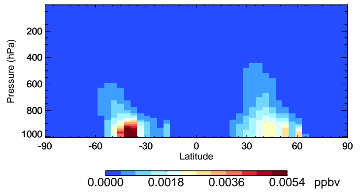
v11-02a BCPO - Species Curtain @ -180.000 for Jan
