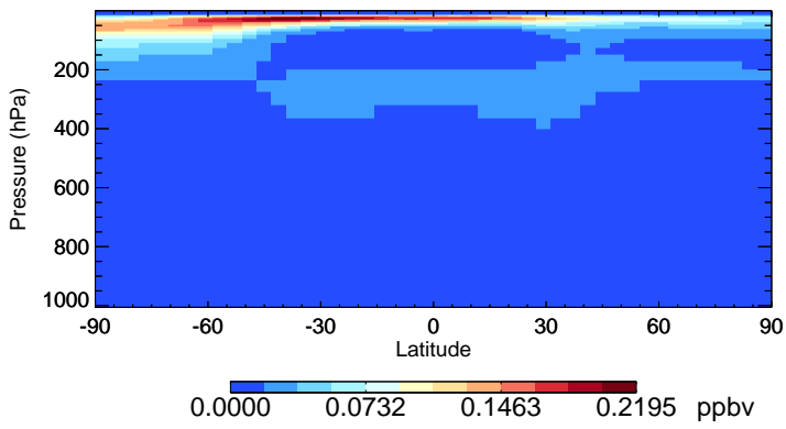
v11-02a HNO4 - Species Zonal Mean for Jan
