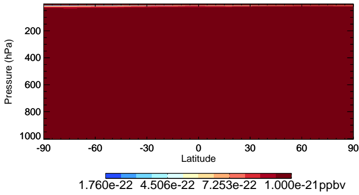
v11-01-public-Run0 HCFC123 - Species Zonal Mean for Jan
