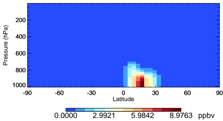
v11-02c DST1 - Species Zonal Mean for Jan
