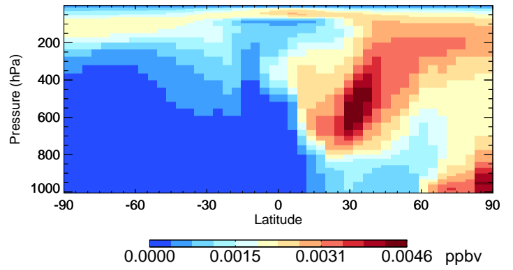
v11-01-public-Run0 ASOG3 - Species Curtain @ -180.000 for Jan
