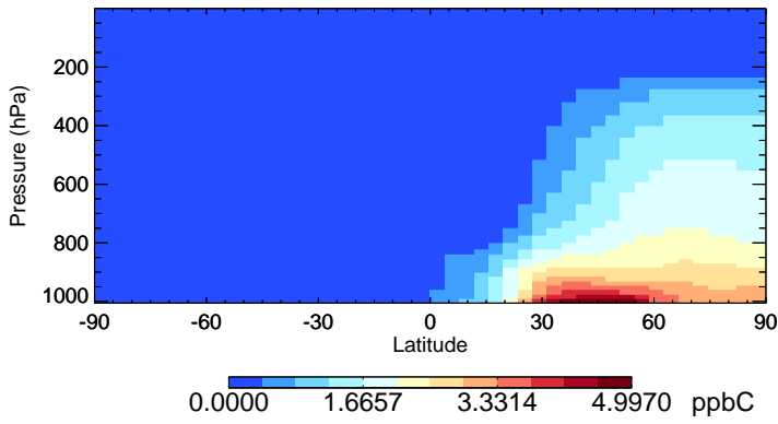
v11-01-public-Run0 ALK4 - Species Zonal Mean for Jan
