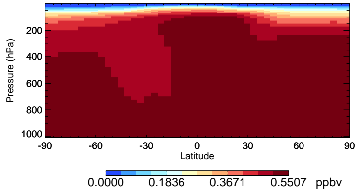
v11-01-public-Run0 CH3Cl - Species Curtain @ -180.000 for Jan
