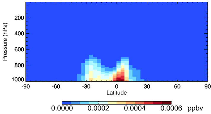
v11-02a MOBA - Species Zonal Mean for Jan
