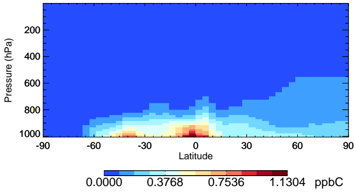
v11-02a ALD2 - Species Zonal Mean for Jan
