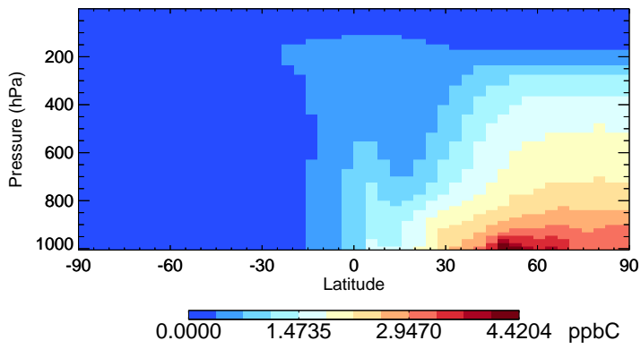
v11-01-public-Run0 C2H6 - Species Zonal Mean for Jan
