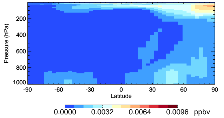
v11-01-public-Run0 HOBr - Species Curtain @ -180.000 for Jan
