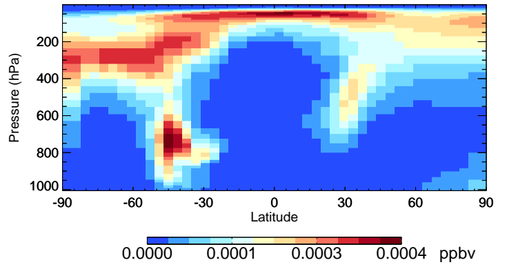
v11-02a TSOA1 - Species Curtain @ -180.000 for Jan
