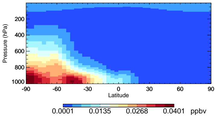
v11-01-public-Run0 MSA - Species Zonal Mean for Jan
