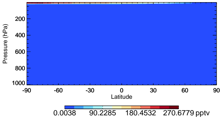
v11-01-public-Run0 HO2 - Species Zonal Mean for Jan
