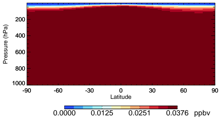
v11-02a HCFC141b - Species Zonal Mean for Jan
