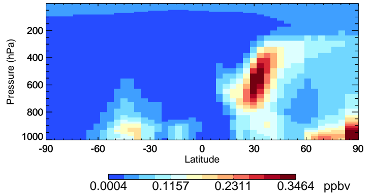
v11-02a NH4 - Species Curtain @ -180.000 for Jan
