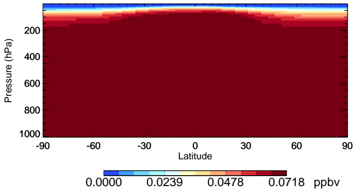
v11-01-public-Run0 CFC113 - Species Zonal Mean for Jan
