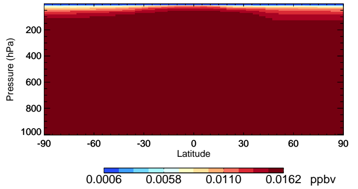
v11-01-public-Run0 CFC114 - Species Curtain @ -180.000 for Jan
