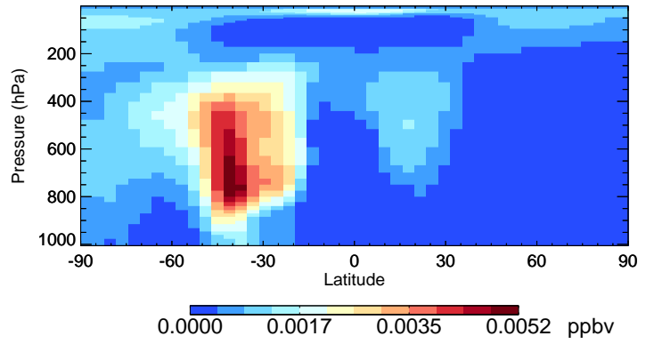
v11-02a ISOG1 - Species Curtain @ -180.000 for Jan
