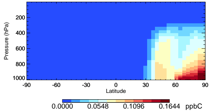
v11-02a XYLE - Species Curtain @ -180.000 for Jan
