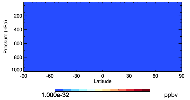
v11-01-public-Run0 SOAME - Species Curtain @ -180.000 for Jan
