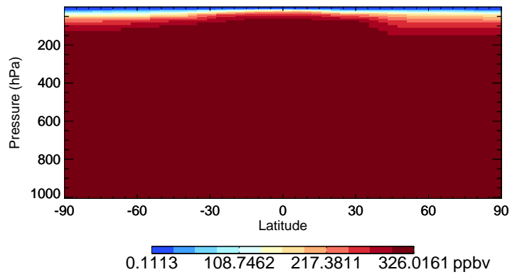
v11-02a N2O - Species Curtain @ -180.000 for Jan
