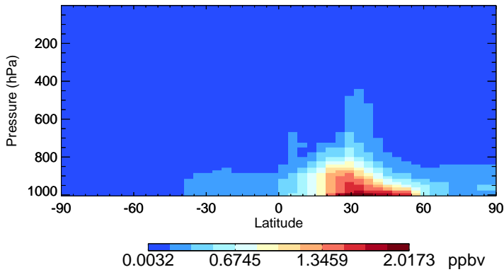
v11-01-public-Run0 NH4 - Species Zonal Mean for Jan
