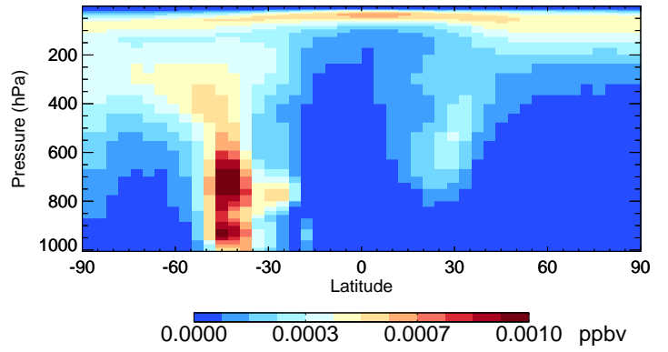
v11-02a TSOA0 - Species Curtain @ -180.000 for Jan
