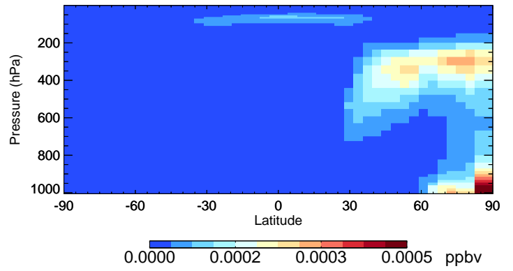
v11-01-public-Run0 ASOA2 - Species Curtain @ -180.000 for Jan
