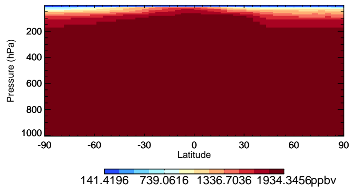
v11-02c CH4 - Species Curtain @ -180.000 for Jan
