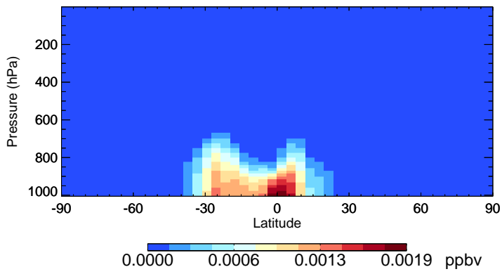
v11-01-public-Run0 ISOPNB - Species Zonal Mean for Jan
