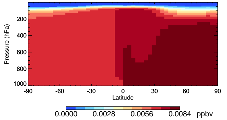
v11-01-public-Run0 CH3Br - Species Curtain @ -180.000 for Jan
