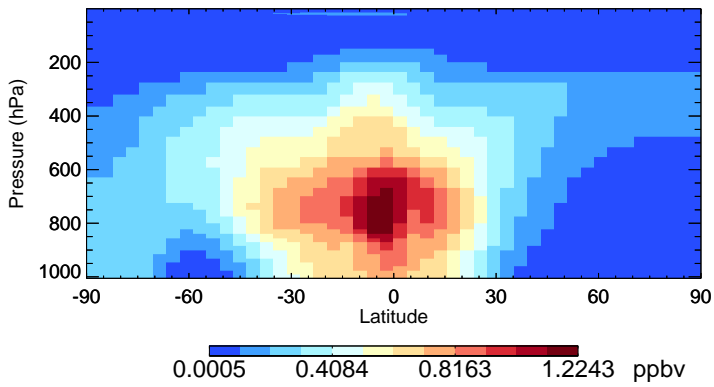
v11-02c H2O2 - Species Zonal Mean for Jan
