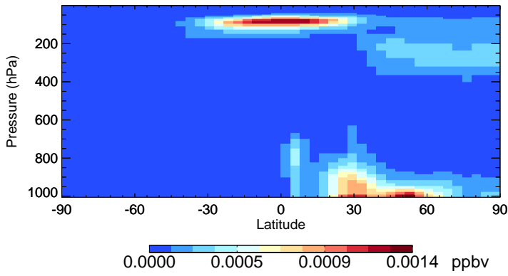
v11-01-public-Run0 ASOA3 - Species Zonal Mean for Jan
