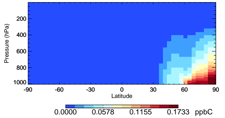
v11-01-public-Run0 XYLE - Species Curtain @ -180.000 for Jan
