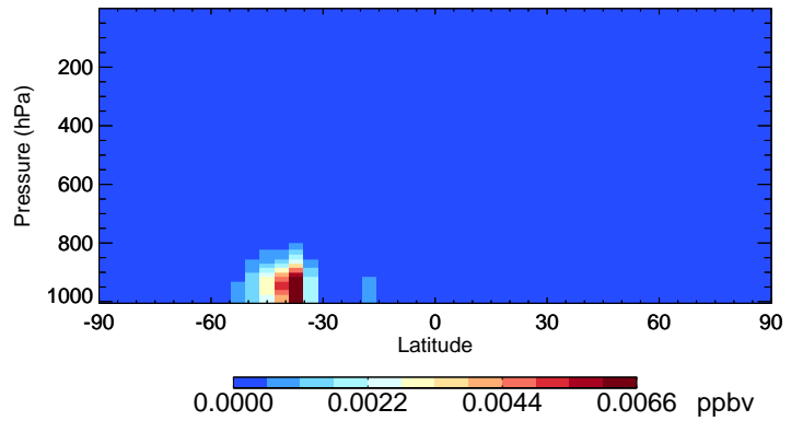
v11-01-public-Run0 MVK - Species Curtain @ -180.000 for Jan
