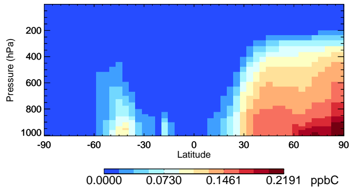
v11-02c MEK - Species Curtain @ -180.000 for Jan
