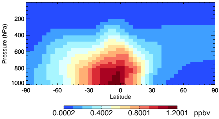
v11-01-public-Run0 MP - Species Zonal Mean for Jan
