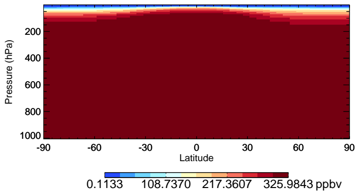
v11-01-public-Run0 N2O - Species Zonal Mean for Jan
