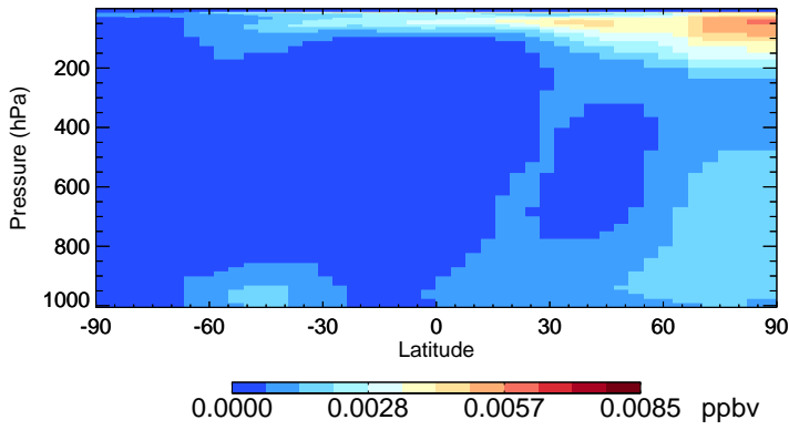
v11-01-public-Run0 HOBr - Species Zonal Mean for Jan
