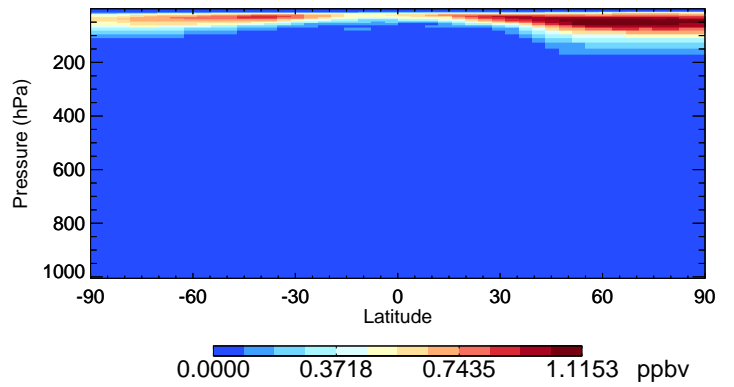
v11-02c CINO3 - Species Curtain @ -180.000 for Jan
