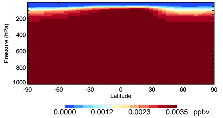
v11-01-public-Run0 H1211 - Species Curtain @ -180.000 for Jan
