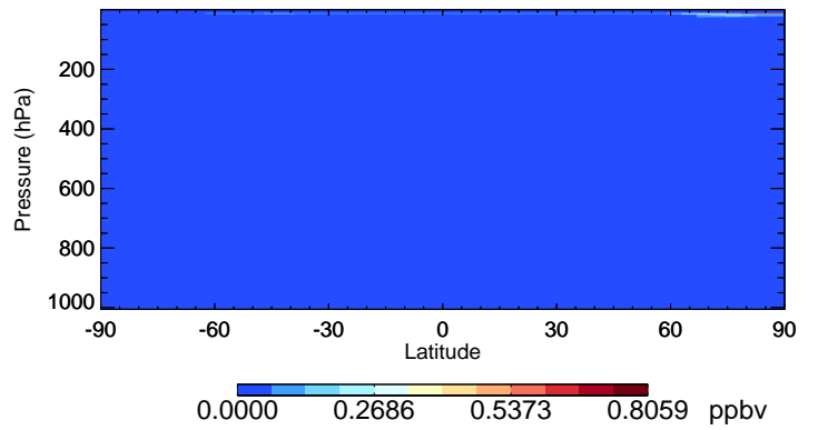
v11-02c NO3 - Species Curtain @ -180.000 for Jan
