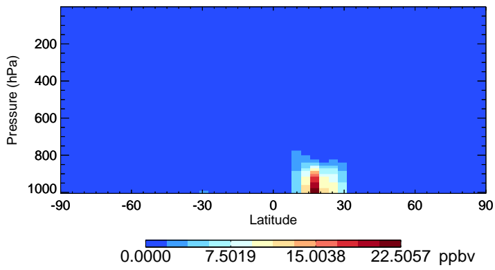
v11-02a DST4 - Species Zonal Mean for Jan
