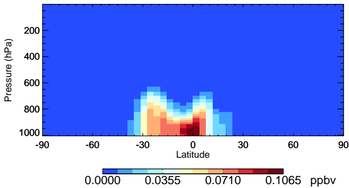
v11-02c MVK - Species Zonal Mean for Jan
