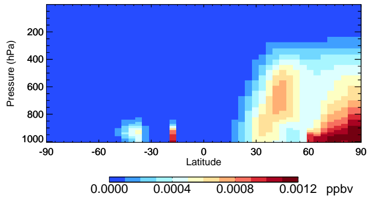
v11-02c GLYX - Species Curtain @ -180.000 for Jan
