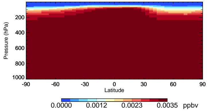
v11-02a H1211 - Species Curtain @ -180.000 for Jan
