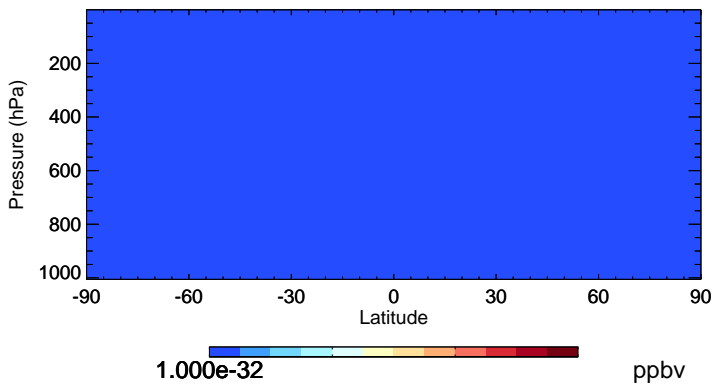
v11-01-public-Run0 MONITA - Species Zonal Mean for Jan
