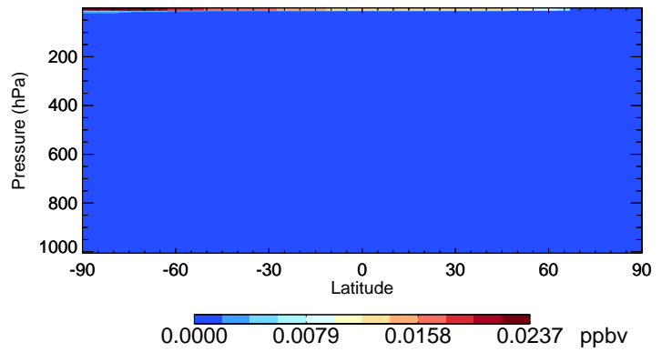
v11-02c Br - Species Curtain @ -180.000 for Jan
