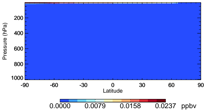
v11-02c Br - Species Zonal Mean for Jan
