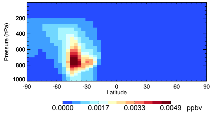
v11-02c SOAME - Species Curtain @ -180.000 for Jan
