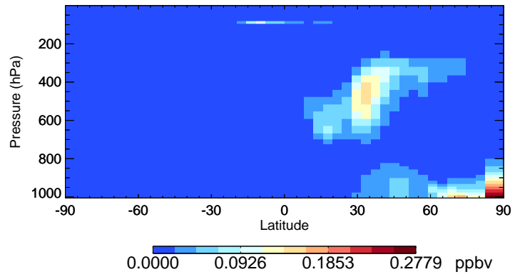
v11-01-public-Run0 NIT - Species Curtain @ -180.000 for Jan
