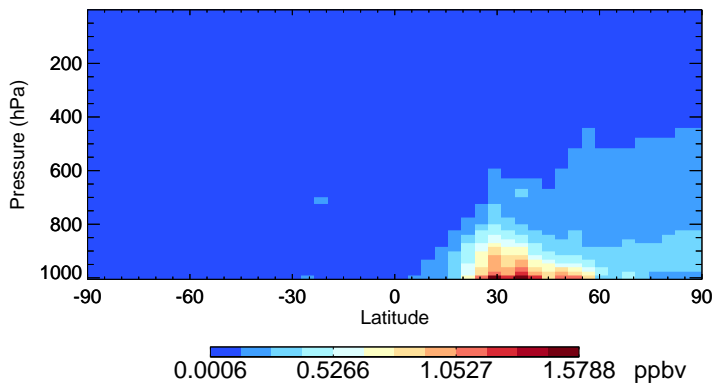
v11-01-public-Run0 SO2 - Species Zonal Mean for Jan
