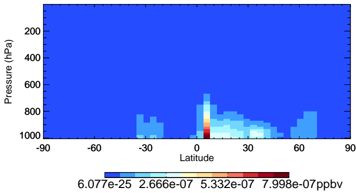
v11-02c NPMN - Species Zonal Mean for Jan
