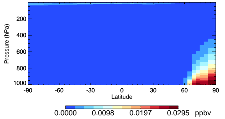
v11-01-public-Run0 HNO2 - Species Curtain @ -180.000 for Jan
