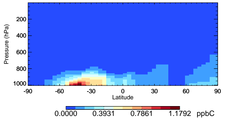
v11-02c ALD2 - Species Curtain @ -180.000 for Jan
