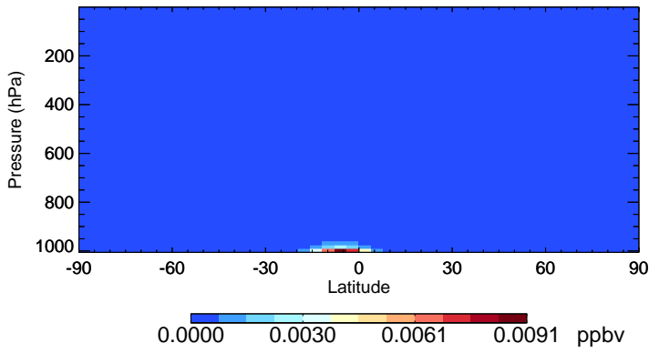
v11-01-public-Run0 LIMO - Species Zonal Mean for Jan
