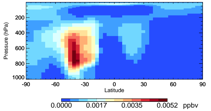
v11-01-public-Run0 ISOG1 - Species Curtain @ -180.000 for Jan
