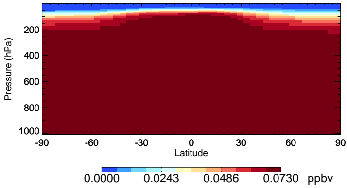
v11-01-public-Run0 CCI4 - Species Zonal Mean for Jan
