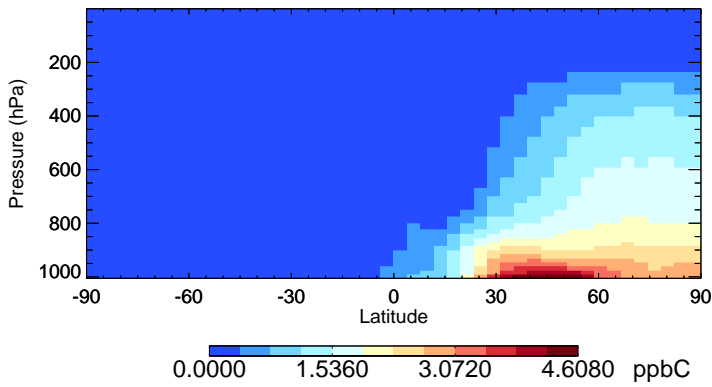
v11-02c ALK4 - Species Zonal Mean for Jan
