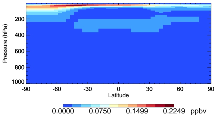
v11-01-public-Run0 HNO4 - Species Zonal Mean for Jan
