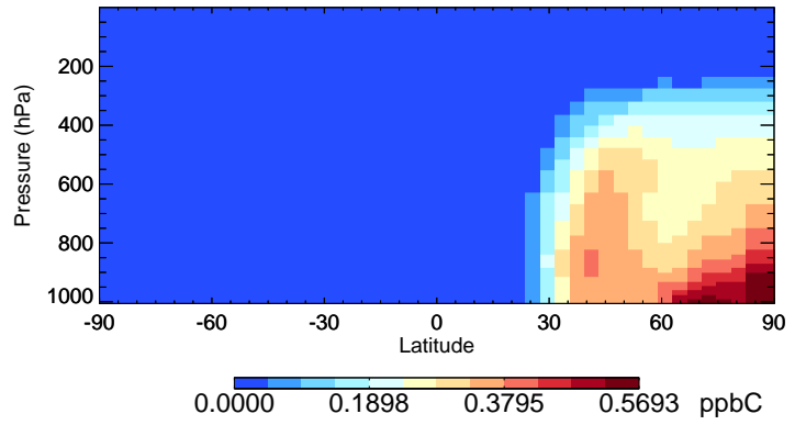
v11-02a TOLU - Species Curtain @ -180.000 for Jan
