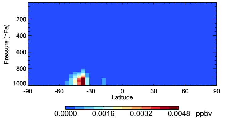
v11-02c MACR - Species Curtain @ -180.000 for Jan
