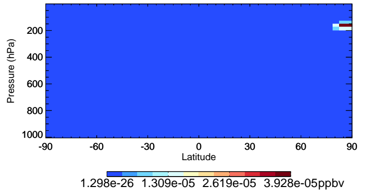
v11-01-public-Run0 CINO2 - Species Curtain @ -180.000 for Jan
