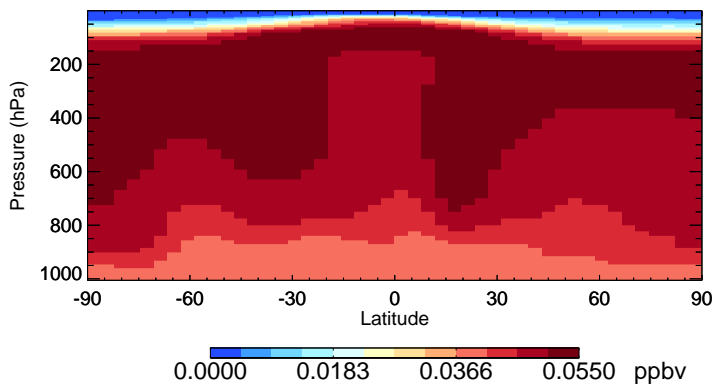
v11-02c HCFC141b - Species Zonal Mean for Jan
