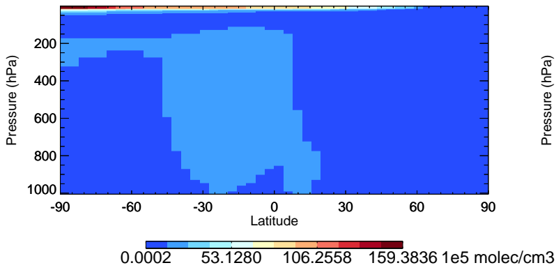
v11-02c OH - Species Zonal Mean for Jan
