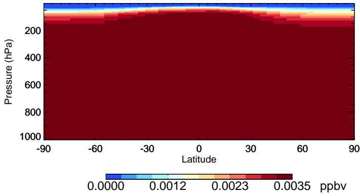
v11-02a H1301 - Species Zonal Mean for Jan
