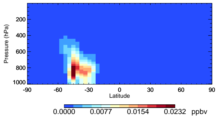
v11-02c DST4 - Species Curtain @ -180.000 for Jan
