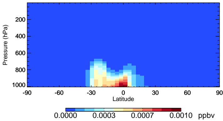
v11-02c MOBA - Species Zonal Mean for Jan
