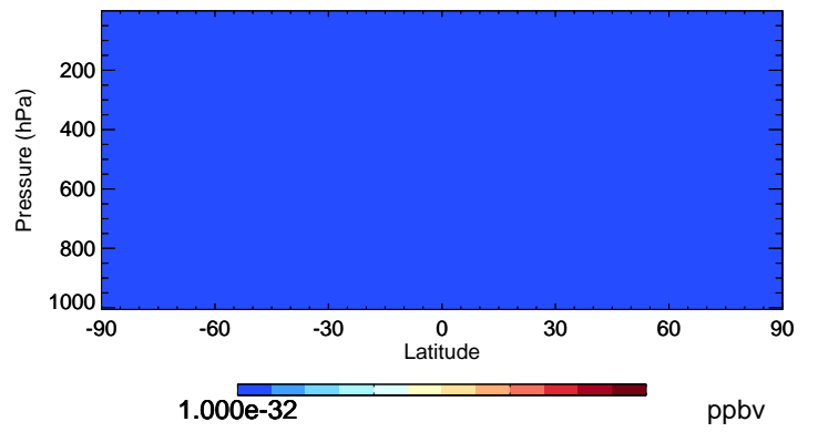
v11-02a SOAME - Species Curtain @ -180.000 for Jan
