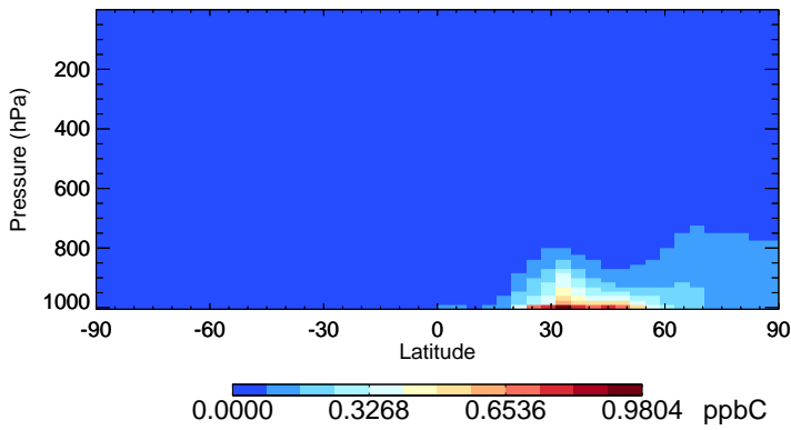
v11-02c XYLE - Species Zonal Mean for Jan
