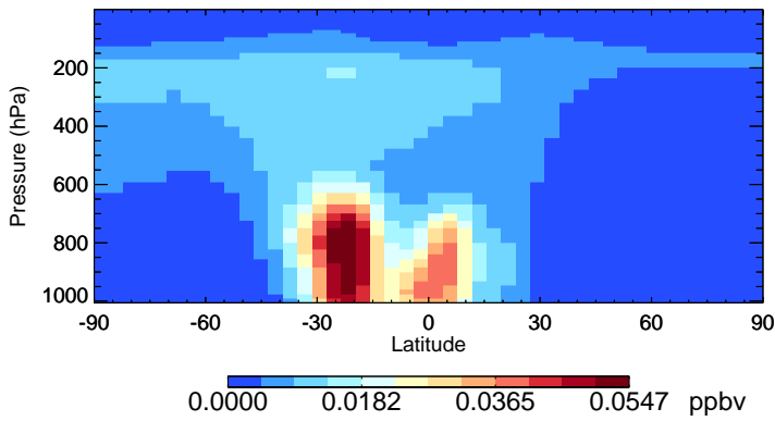
v11-02c ISO3 - Species Zonal Mean for Jan
