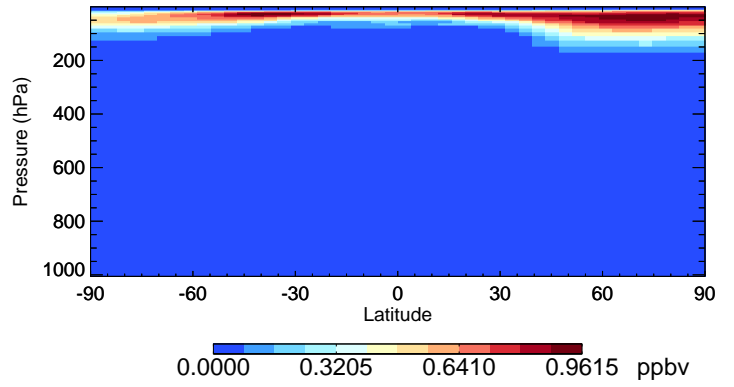
v11-02a CINO3 - Species Curtain @ -180.000 for Jan
