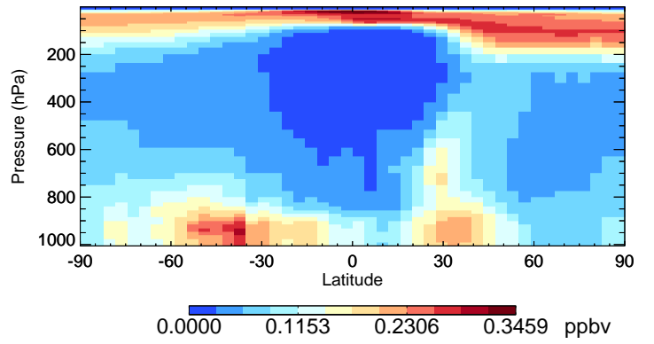
v11-01-public-Run0 SO4 - Species Curtain @ -180.000 for Jan
