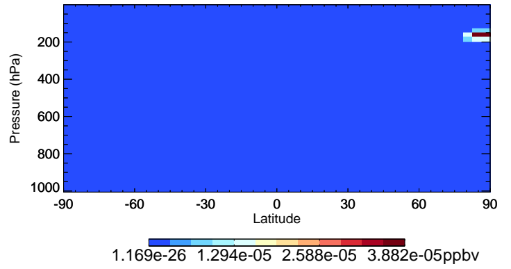
v11-02a CINO2 - Species Curtain @ -180.000 for Jan
