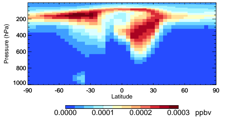
v11-02c DHDN - Species Curtain @ -180.000 for Jan
