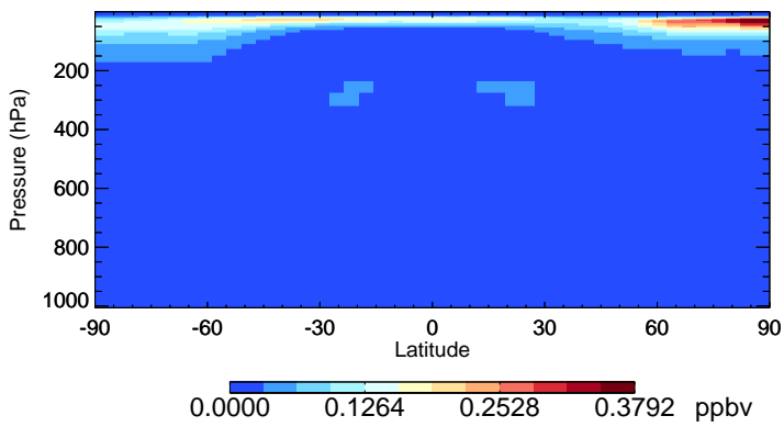
v11-02c HNO4 - Species Zonal Mean for Jan
