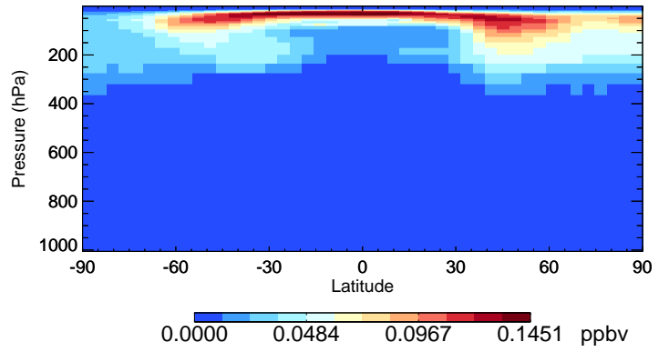
v11-02a MPN - Species Curtain @ -180.000 for Jan
