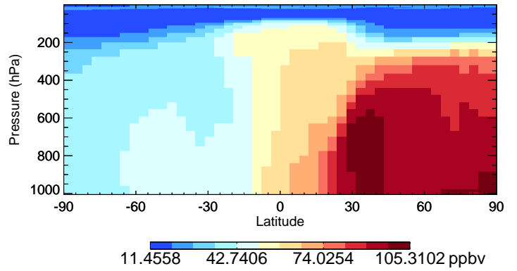
v11-02a CO - Species Curtain @ -180.000 for Jan
