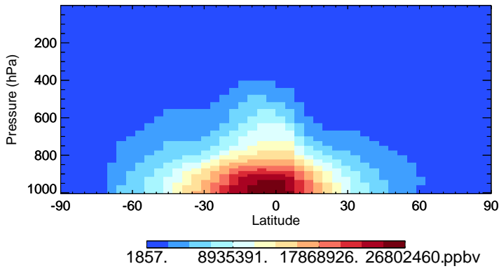
v11-01-public-Run0 H2O - Species Zonal Mean for Jan
