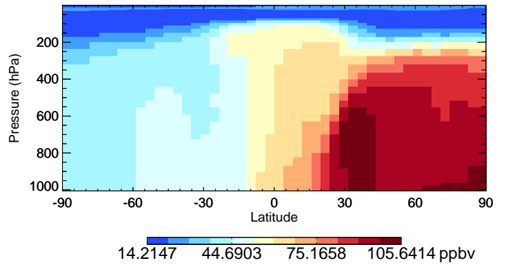
v11-01-public-Run0 CO - Species Curtain @ -180.000 for Jan
