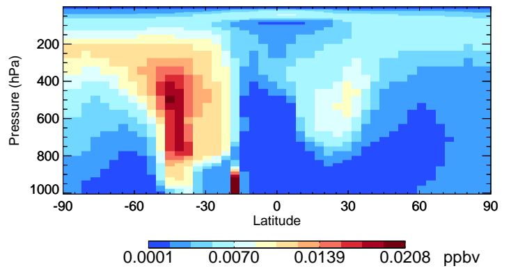
v11-01-public-Run0 TSOG3 - Species Curtain @ -180.000 for Jan
