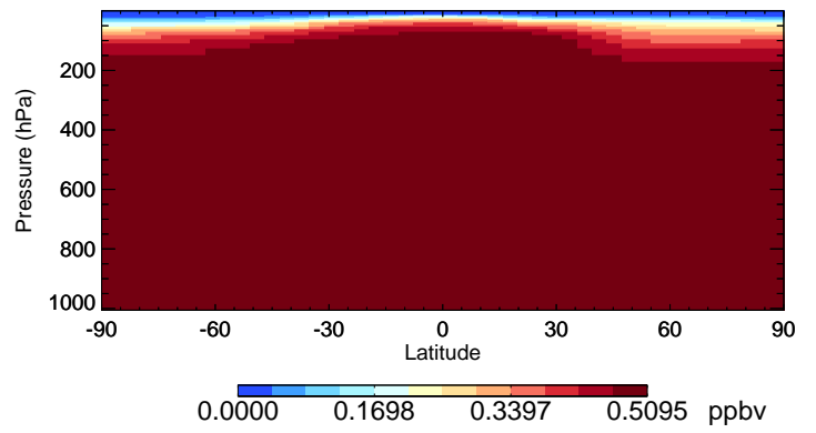
v11-02a CFC12 - Species Curtain @ -180.000 for Jan
