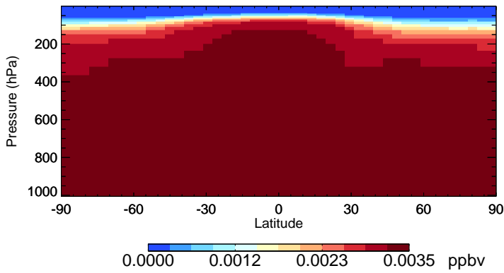
v11-02c H1211 - Species Zonal Mean for Jan
