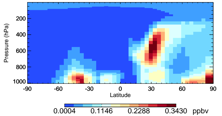
v11-01-public-Run0 NH4 - Species Curtain @ -180.000 for Jan
