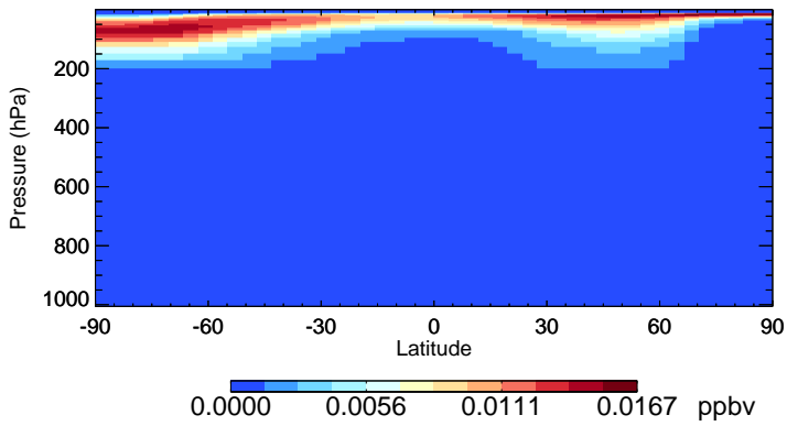
v11-02c BrNO3 - Species Zonal Mean for Jan
