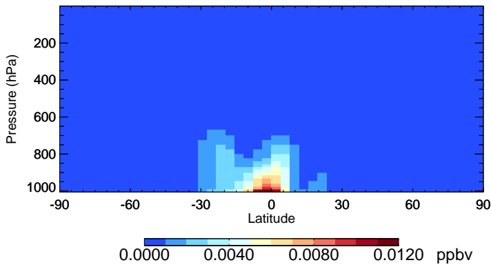
v11-02c TSOA1 - Species Zonal Mean for Jan
