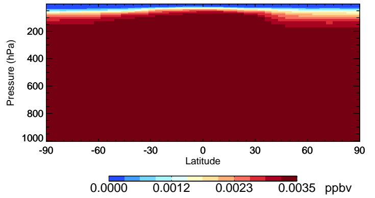
v11-01-public-Run0 H1301 - Species Curtain @ -180.000 for Jan
