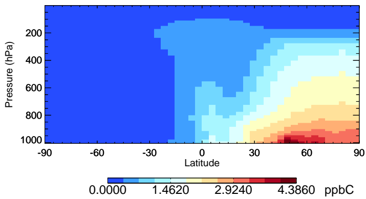
v11-02c C2H6 - Species Zonal Mean for Jan
