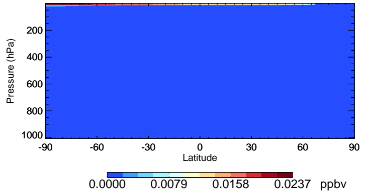
v11-02a Br - Species Curtain @ -180.000 for Jan
