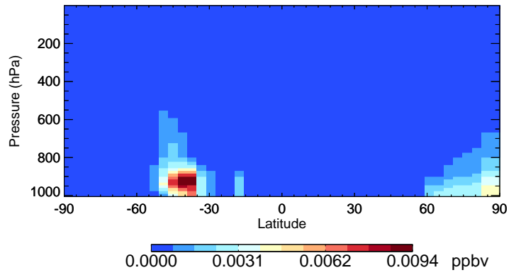
v11-01-public-Run0 GLYC - Species Curtain @ -180.000 for Jan
