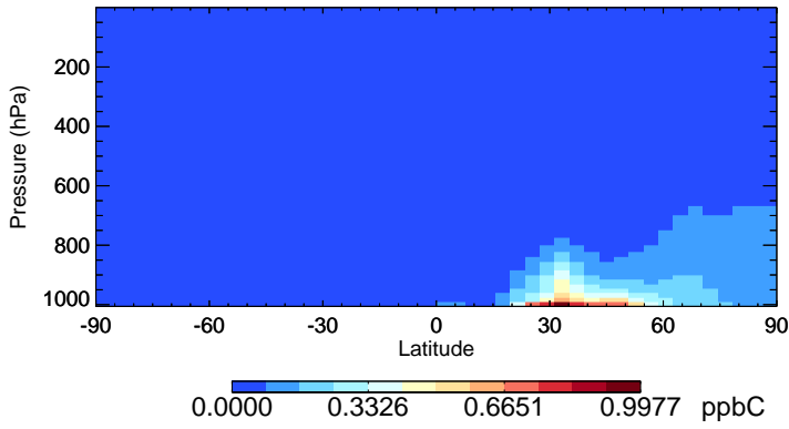
v11-02a XYLE - Species Zonal Mean for Jan
