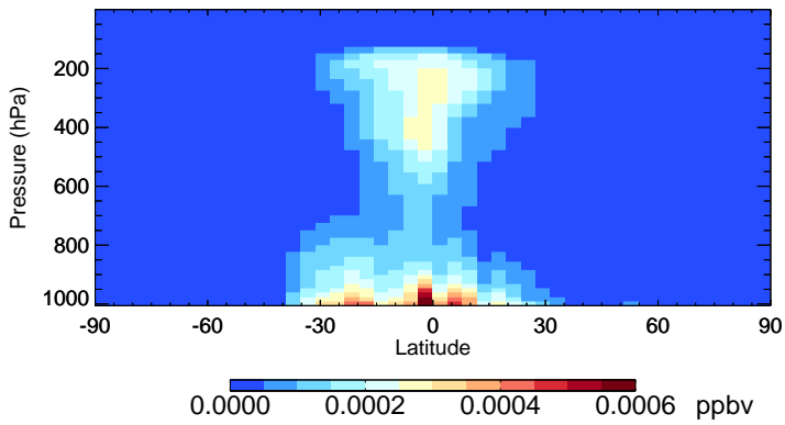
v11-02c HONIT - Species Zonal Mean for Jan
