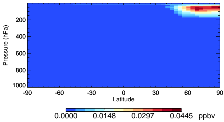
v11-02a OCIO - Species Zonal Mean for Jan
