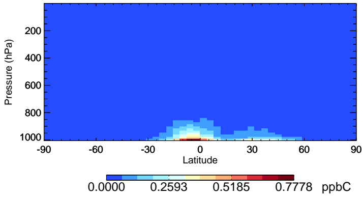
v11-02a PRPE - Species Zonal Mean for Jan
