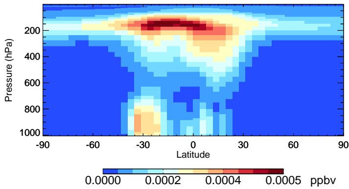
v11-02c DHDN - Species Zonal Mean for Jan
