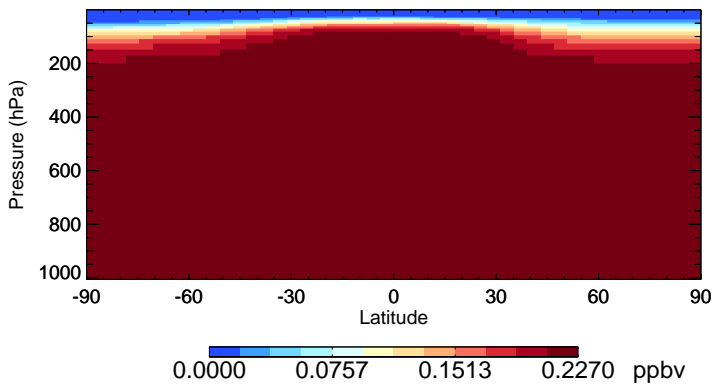
v11-02a CFC11 - Species Zonal Mean for Jan
