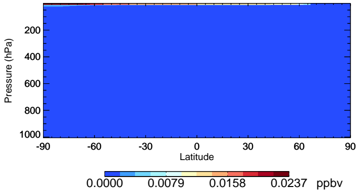
v11-02a Br - Species Zonal Mean for Jan
