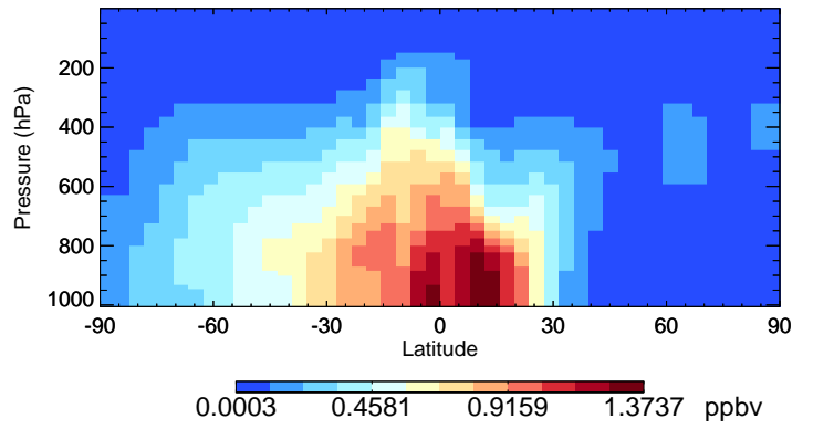
v11-01-public-Run0 MP - Species Curtain @ -180.000 for Jan
