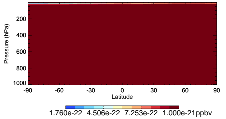
v11-01-public-Run0 HCFC123 - Species Curtain @ -180.000 for Jan
