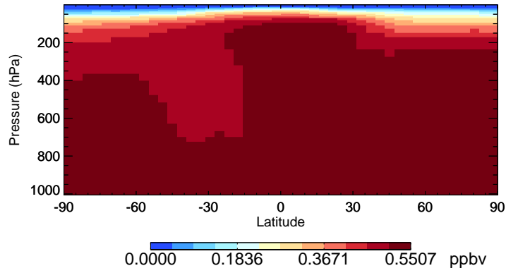
v11-02a CH3Cl - Species Curtain @ -180.000 for Jan
