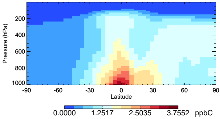
v11-02a ACET - Species Zonal Mean for Jan
