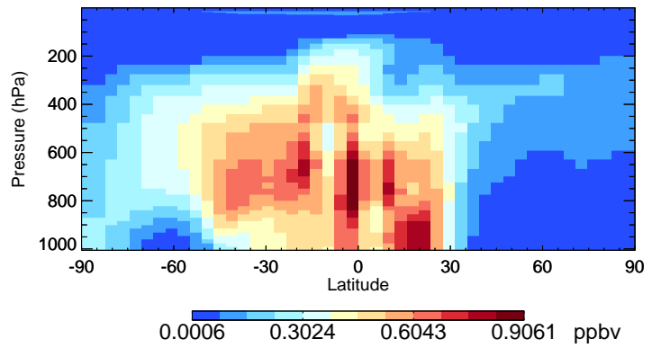
v11-02c H2O2 - Species Curtain @ -180.000 for Jan
