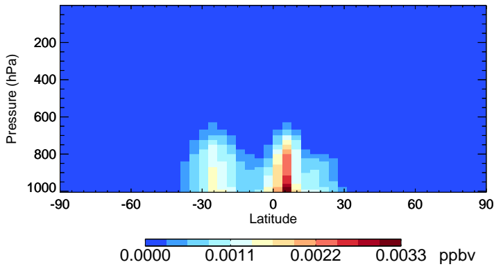
v11-01-public-Run0 NPMN - Species Zonal Mean for Jan
