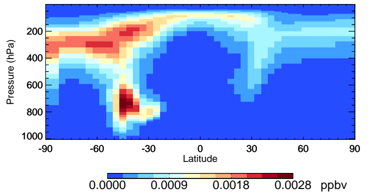
v11-02c ISOA1 - Species Curtain @ -180.000 for Jan
