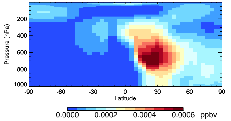
v11-02a ASOG1 - Species Curtain @ -180.000 for Jan
