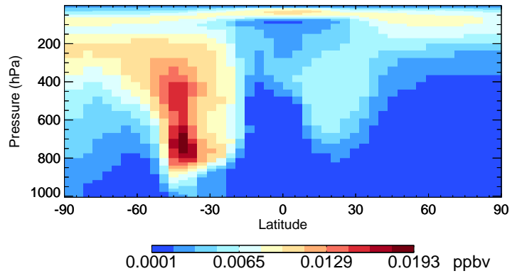
v11-01-public-Run0 ISO3 - Species Curtain @ -180.000 for Jan
