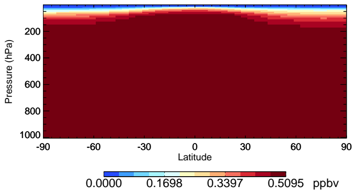
v11-01-public-Run0 CFC12 - Species Zonal Mean for Jan
