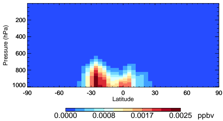
v11-02c ISOPNB - Species Zonal Mean for Jan
