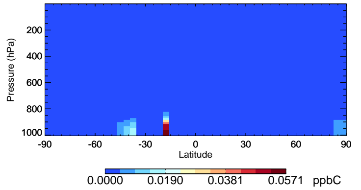
v11-01-public-Run0 PRPE - Species Curtain @ -180.000 for Jan
