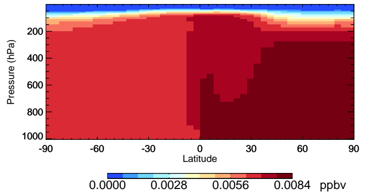
v11-02c CH3Br - Species Curtain @ -180.000 for Jan
