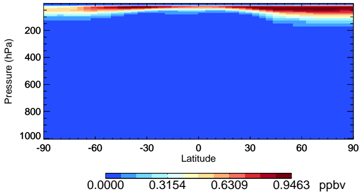
v11-02a CINO3 - Species Zonal Mean for Jan
