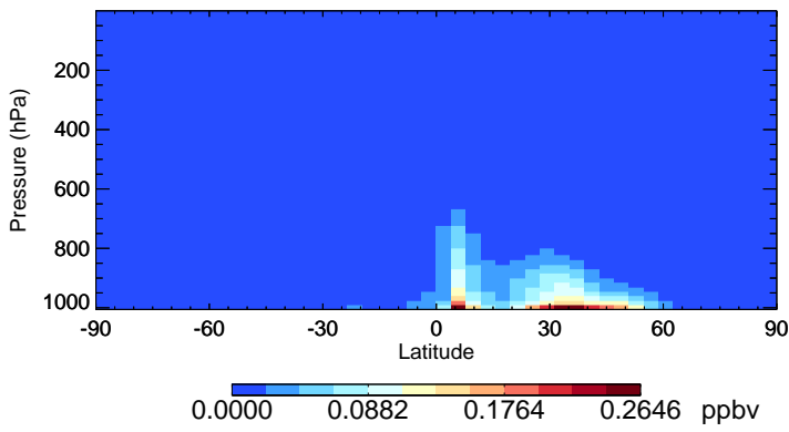
v11-02a BCPO - Species Zonal Mean for Jan
