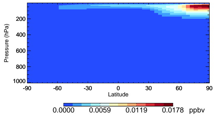
v11-01-public-Run0 BrCl - Species Curtain @ -180.000 for Jan
