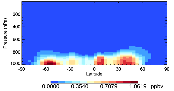
v11-02a SALA - Species Curtain @ -180.000 for Jan
