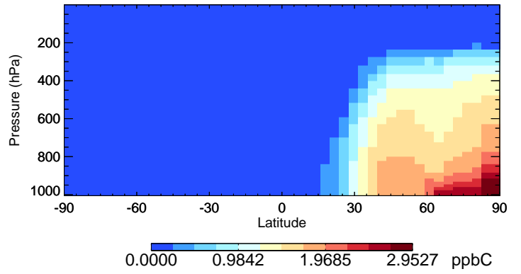
v11-02a ALK4 - Species Curtain @ -180.000 for Jan
