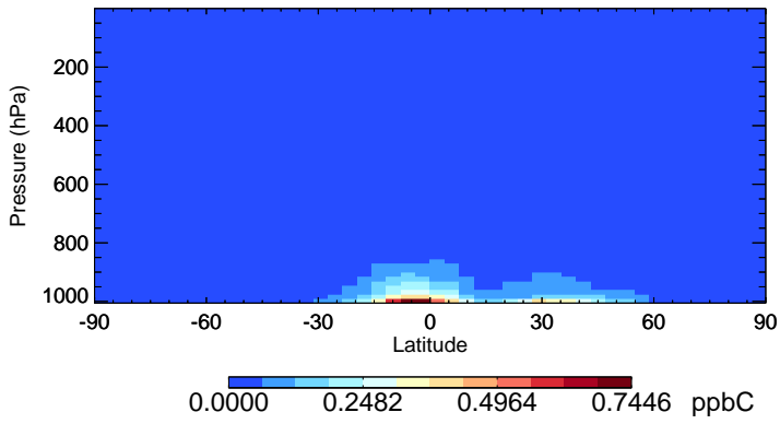
v11-01-public-Run0 PRPE - Species Zonal Mean for Jan
