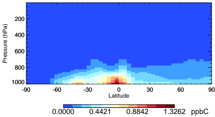
v11-02c ALD2 - Species Zonal Mean for Jan
