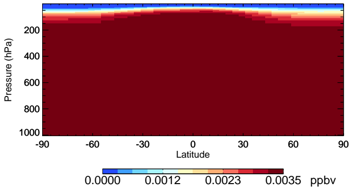
v11-01-public-Run0 H1301 - Species Zonal Mean for Jan
