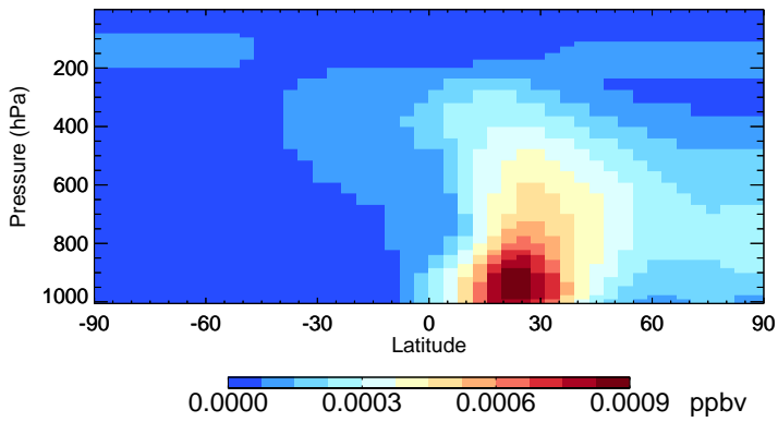
v11-02c ASOG1 - Species Zonal Mean for Jan
