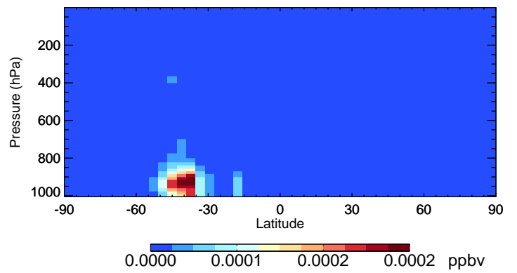
v11-02c IEPOXD - Species Curtain @ -180.000 for Jan
