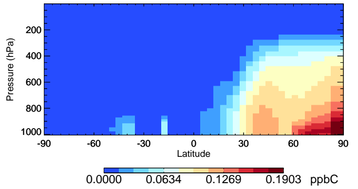
v11-01-public-Run0 ALD2 - Species Curtain @ -180.000 for Jan
