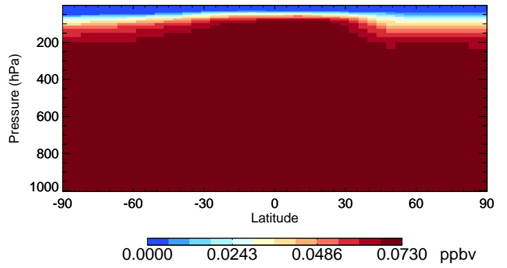
v11-01-public-Run0 CCI4 - Species Curtain @ -180.000 for Jan
