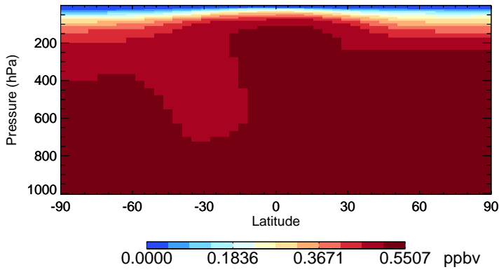
v11-01-public-Run0 CH3Cl - Species Zonal Mean for Jan
