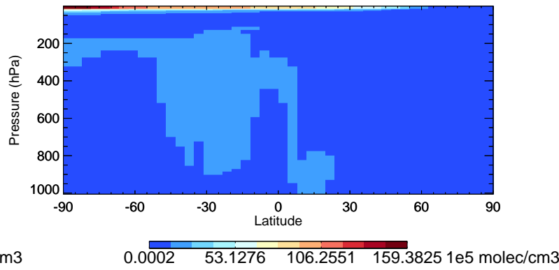
v11-02c OH - Species Curtain @ -180.000 for Jan
