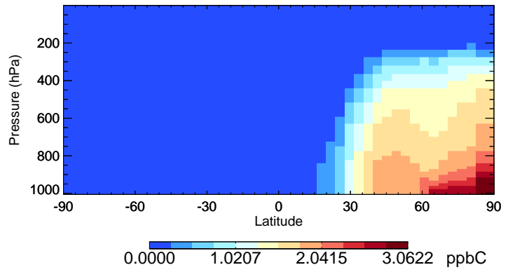
v11-01-public-Run0 ALK4 - Species Curtain @ -180.000 for Jan
