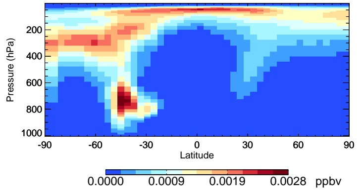
v11-02a ISOA1 - Species Curtain @ -180.000 for Jan
