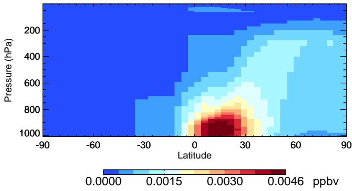
v11-01-public-Run0 ASOAN - Species Zonal Mean for Jan
