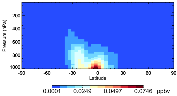
v11-01-public-Run0 TSOG2 - Species Zonal Mean for Jan
