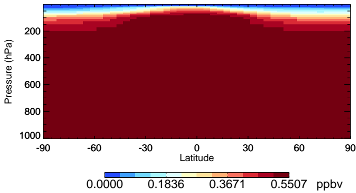
v11-02c CH3Cl - Species Zonal Mean for Jan
