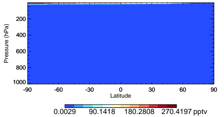
v11-02c HO2 - Species Curtain @ -180.000 for Jan
