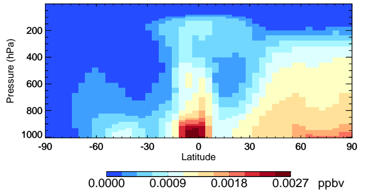
v11-01-public-Run0 CHBr3 - Species Curtain @ -180.000 for Jan
