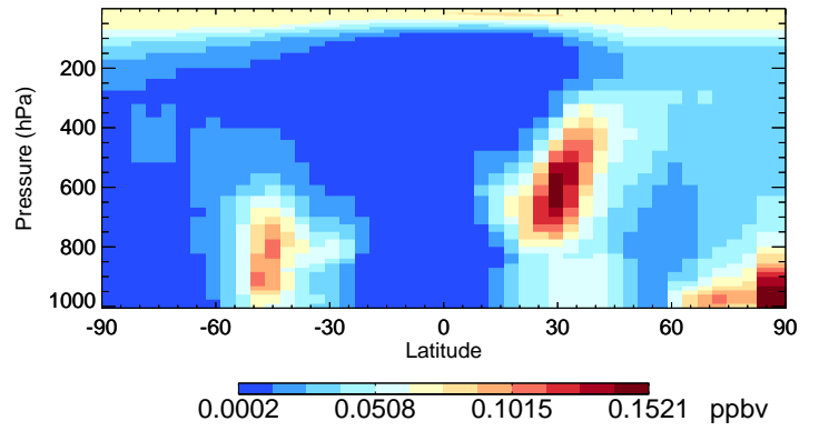
v11-01-public-Run0 OCPI - Species Curtain @ -180.000 for Jan
