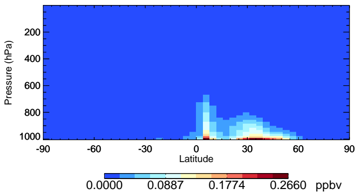
v11-02c BCPO - Species Zonal Mean for Jan
