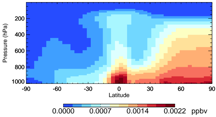
v11-01-public-Run0 CHBr3 - Species Zonal Mean for Jan
