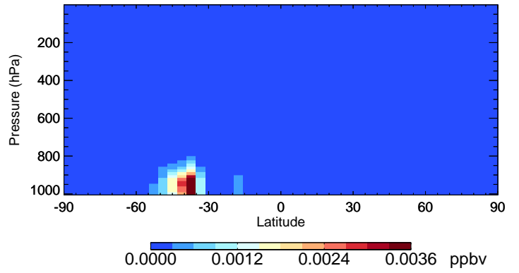
v11-02a MACR - Species Curtain @ -180.000 for Jan
