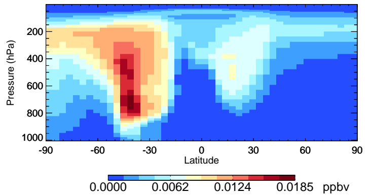
v11-02c ISO3 - Species Curtain @ -180.000 for Jan
