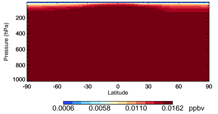
v11-02a CFC114 - Species Curtain @ -180.000 for Jan
