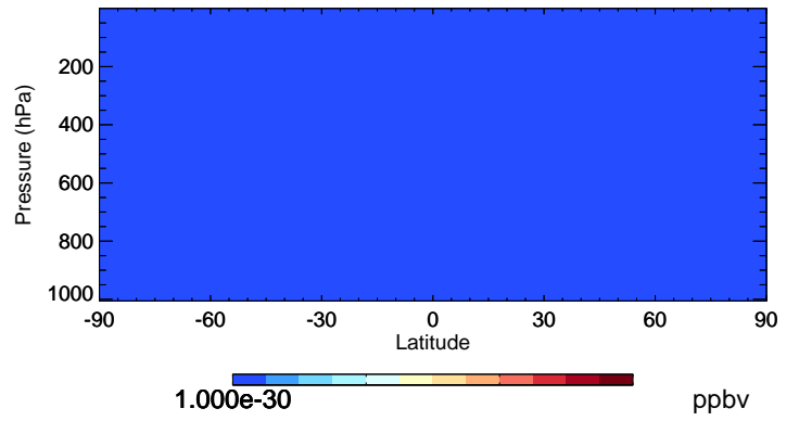
v11-01-public-Run0 MGLY - Species Curtain @ -180.000 for Jan
