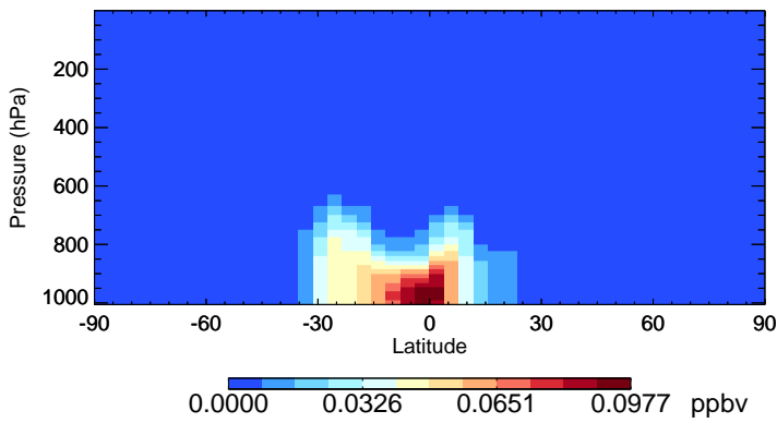
v11-02a MVK - Species Zonal Mean for Jan
