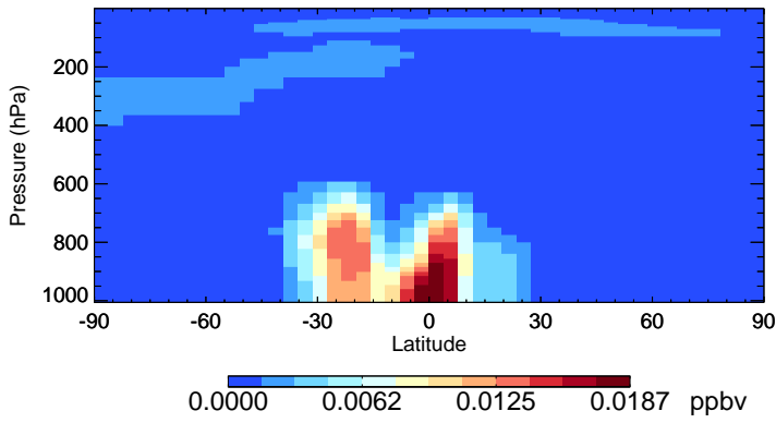
v11-01-public-Run0 ISOA1 - Species Zonal Mean for Jan
