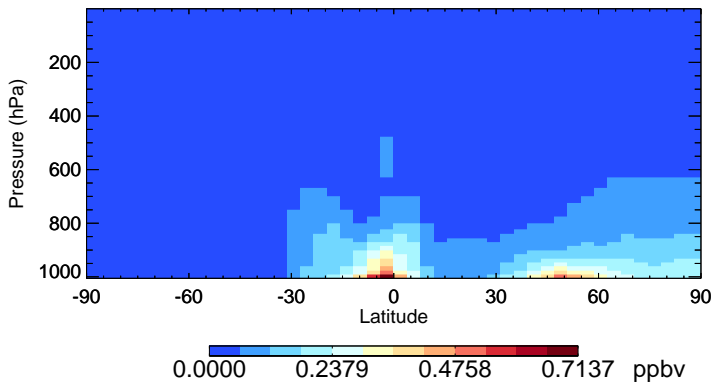
v11-02c EOH - Species Zonal Mean for Jan
