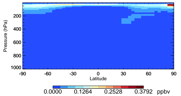
v11-02c HNO4 - Species Curtain @ -180.000 for Jan
