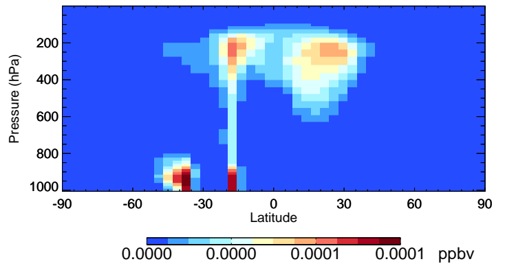
v11-02c HONIT - Species Curtain @ -180.000 for Jan
