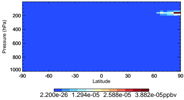
v11-02a CINO2 - Species Zonal Mean for Jan
