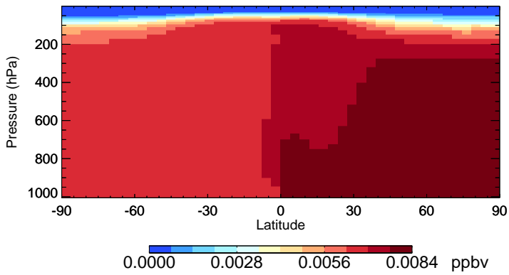
v11-02c CH3Br - Species Zonal Mean for Jan
