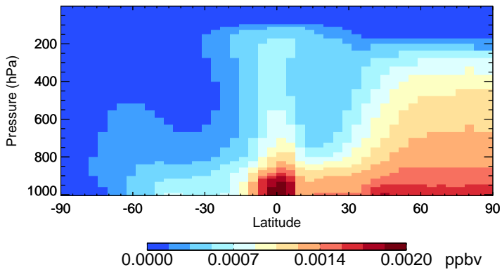
v11-02c CHBr3 - Species Zonal Mean for Jan
