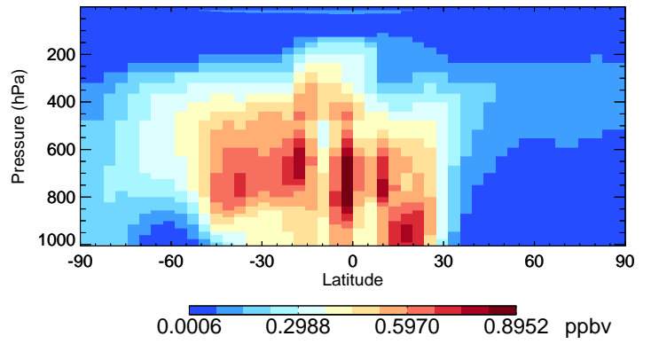
v11-01-public-Run0 H2O2 - Species Curtain @ -180.000 for Jan
