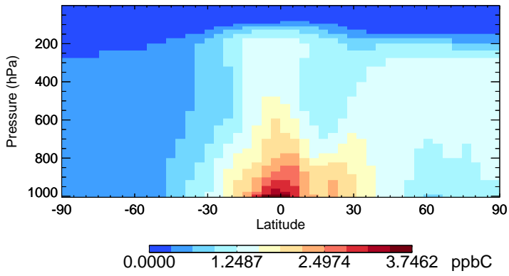
v11-01-public-Run0 ACET - Species Zonal Mean for Jan
