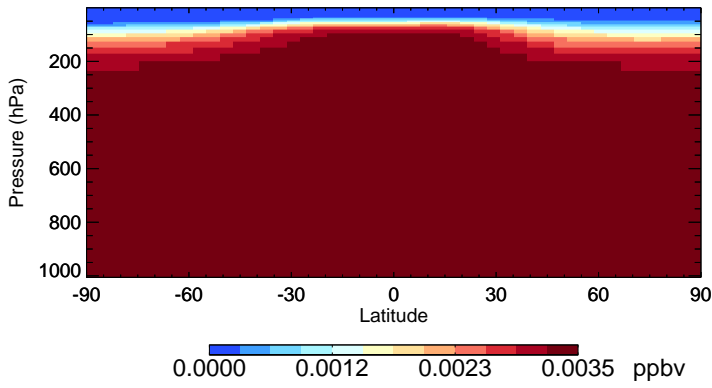
v11-01-public-Run0 H1211 - Species Zonal Mean for Jan
