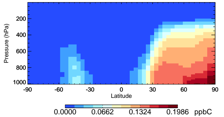
v11-01-public-Run0 MEK - Species Curtain @ -180.000 for Jan
