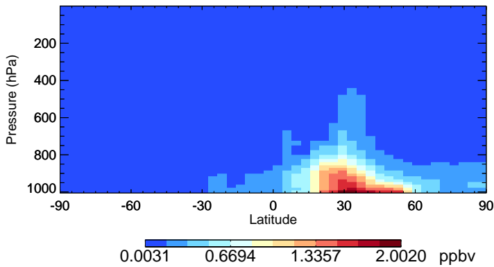
v11-02c NH4 - Species Zonal Mean for Jan
