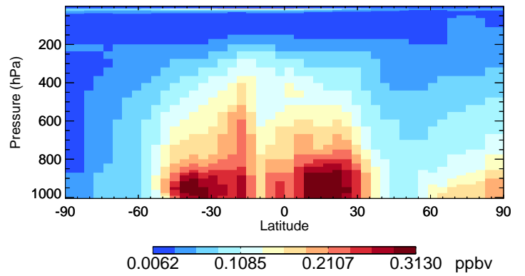
v11-02c CH2O - Species Curtain @ -180.000 for Jan
