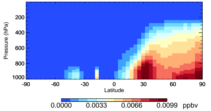
v11-02a RCHO - Species Curtain @ -180.000 for Jan
