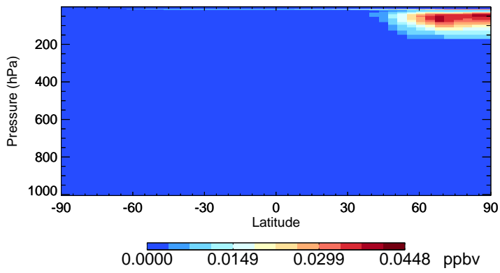
v11-01-public-Run0 OCIO - Species Zonal Mean for Jan
