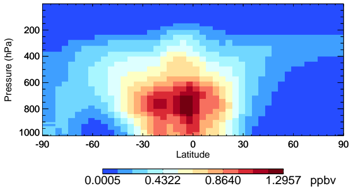
v11-01-public-Run0 H2O2 - Species Zonal Mean for Jan
