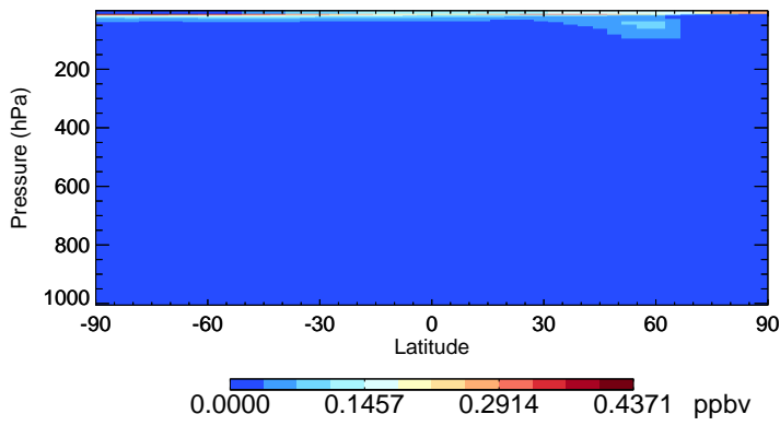
v11-01-public-Run0 CIO - Species Zonal Mean for Jan
