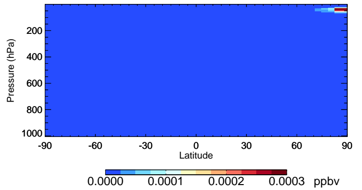
v11-02c CINO2 - Species Curtain @ -180.000 for Jan
