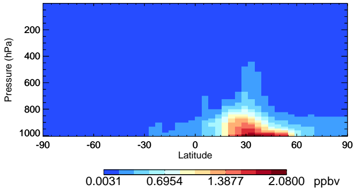
v11-02a NH4 - Species Zonal Mean for Jan
