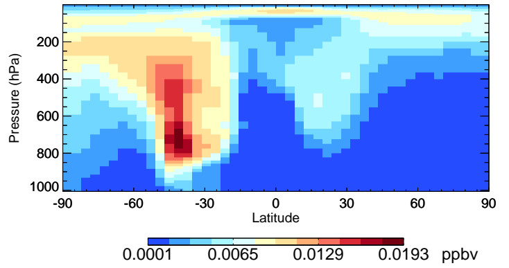
v11-02a ISO3 - Species Curtain @ -180.000 for Jan
