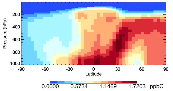
v11-01-public-Run0 ACET - Species Curtain @ -180.000 for Jan
