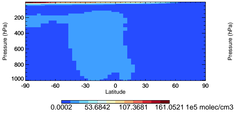
v11-02a OH - Species Zonal Mean for Jan
