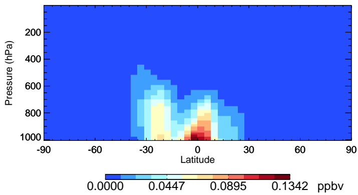
v11-02c TSOG3 - Species Zonal Mean for Jan
