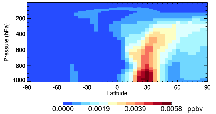
v11-02c ASOAN - Species Curtain @ -180.000 for Jan
