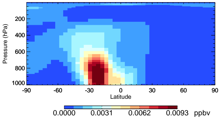
v11-01-public-Run0 ISOG1 - Species Zonal Mean for Jan
