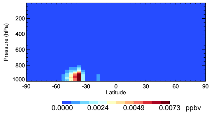
v11-02a MVK - Species Curtain @ -180.000 for Jan
