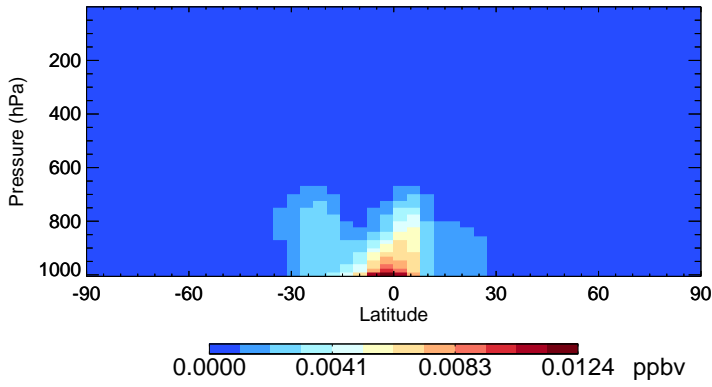
v11-02a TSOA1 - Species Zonal Mean for Jan
