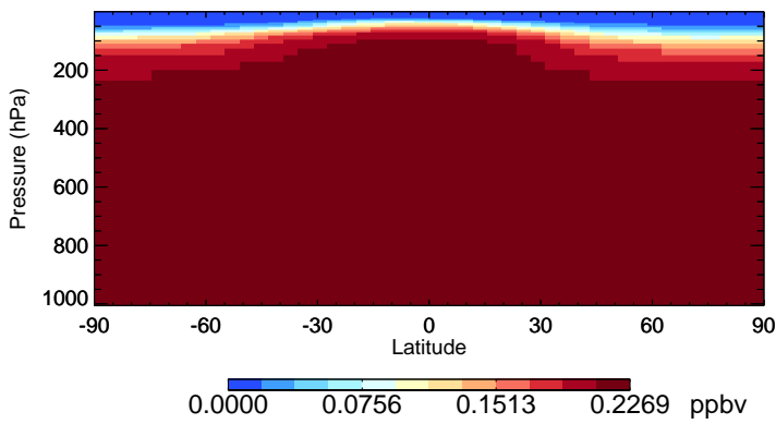
v11-02c CFC11 - Species Zonal Mean for Jan
