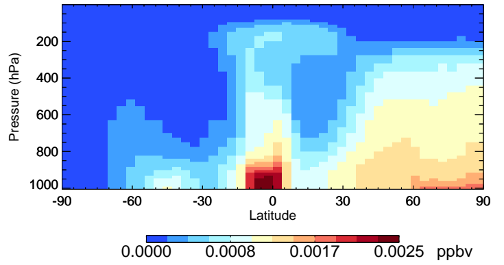
v11-02a CHBr3 - Species Curtain @ -180.000 for Jan
