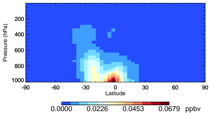
v11-02c TSOG2 - Species Zonal Mean for Jan
