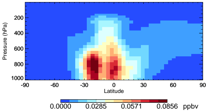
v11-01-public-Run0 MAP - Species Zonal Mean for Jan
