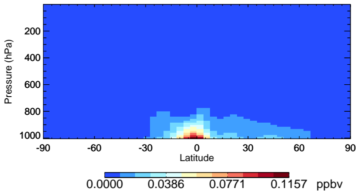
v11-02c RCHO - Species Zonal Mean for Jan
