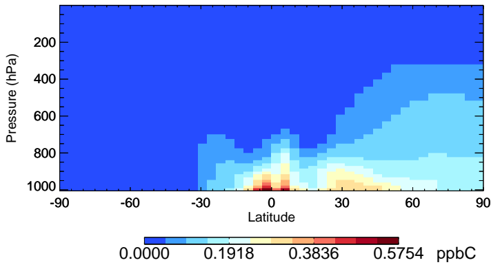
v11-01-public-Run0 ALD2 - Species Zonal Mean for Jan
