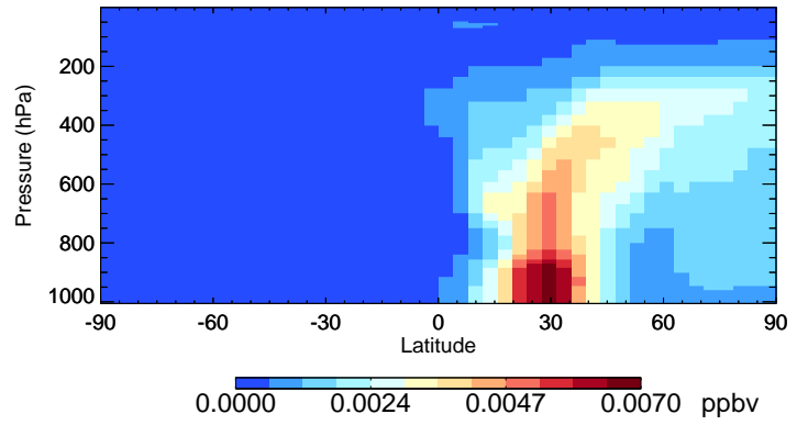
v11-02a ASOAN - Species Curtain @ -180.000 for Jan
