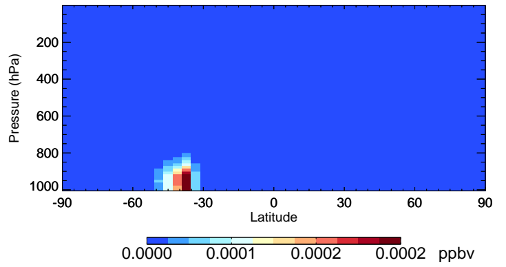
v11-01-public-Run0 NPMN - Species Curtain @ -180.000 for Jan
