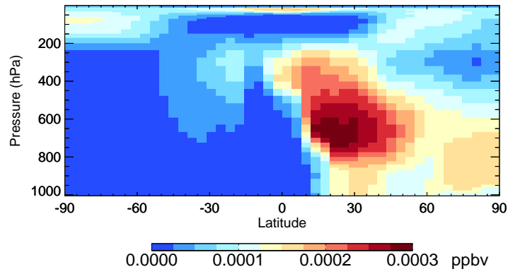
v11-01-public-Run0 ASOG1 - Species Curtain @ -180.000 for Jan
