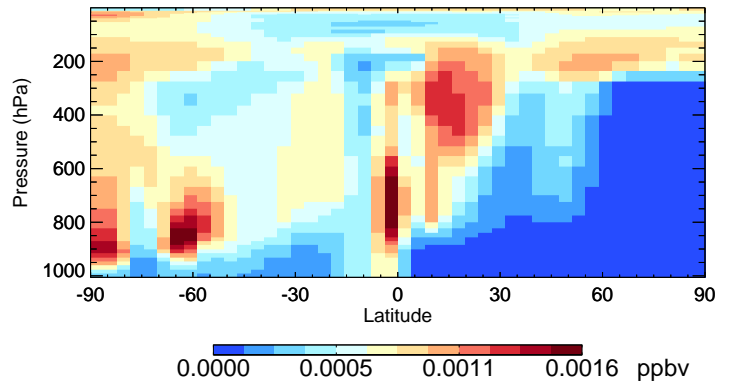
v11-01-public-Run0 HBr - Species Curtain @ -180.000 for Jan
