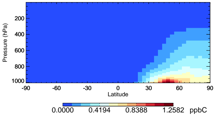
v11-01-public-Run0 TOLU - Species Zonal Mean for Jan
