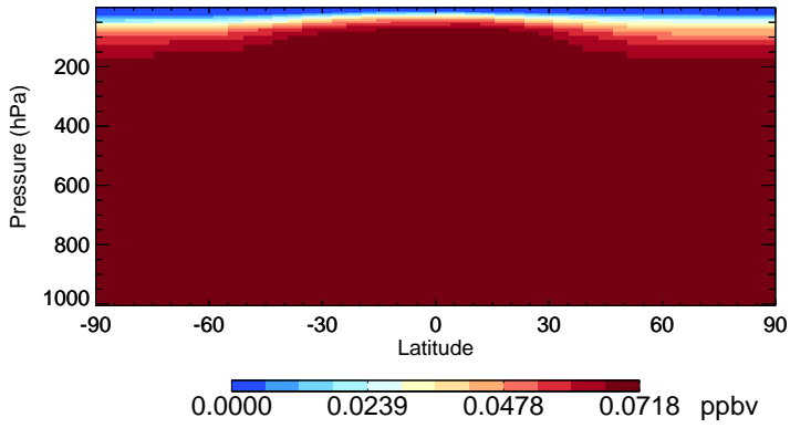
v11-02a CFC113 - Species Zonal Mean for Jan
