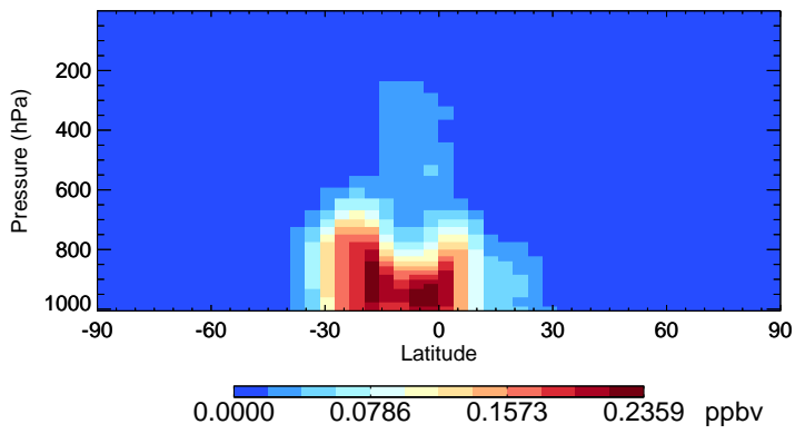
v11-01-public-Run0 HAC - Species Zonal Mean for Jan
