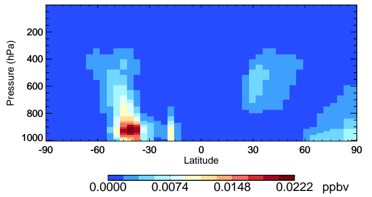
v11-02a HAC - Species Curtain @ -180.000 for Jan
