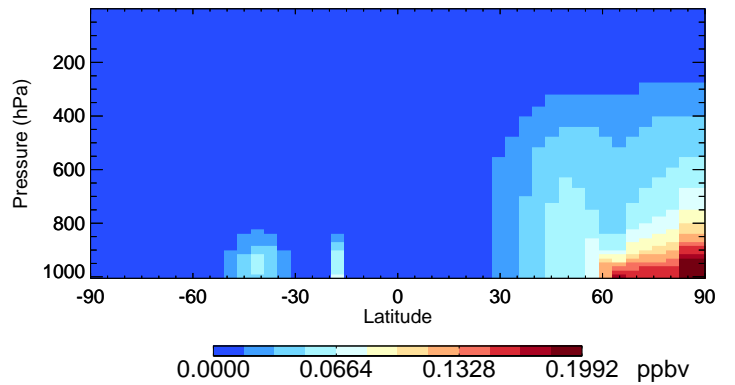
v11-02c EOH - Species Curtain @ -180.000 for Jan
