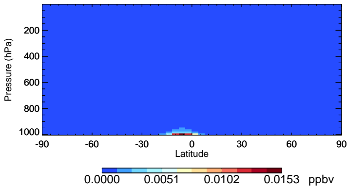
v11-02c MTPO - Species Zonal Mean for Jan
