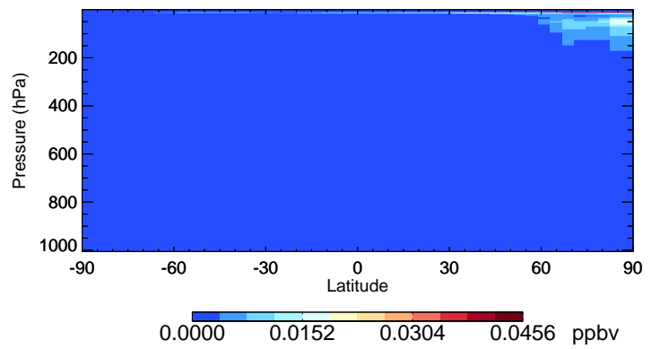
v11-02c OCIO - Species Curtain @ -180.000 for Jan
