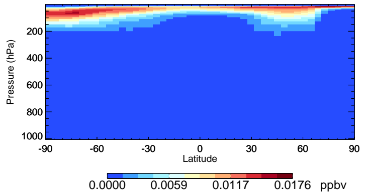
v11-02c BrNO3 - Species Curtain @ -180.000 for Jan
