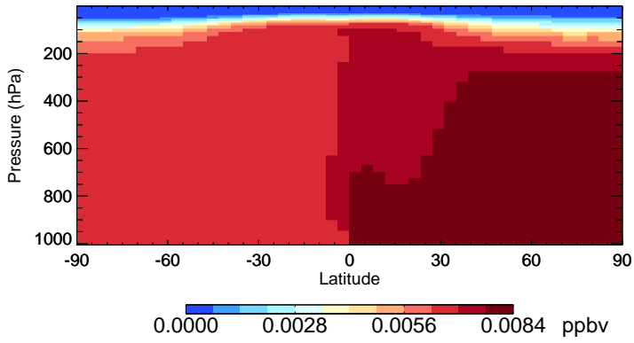
v11-02a CH3Br - Species Zonal Mean for Jan
