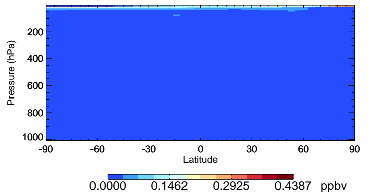
v11-01-public-Run0 CIO - Species Curtain @ -180.000 for Jan
