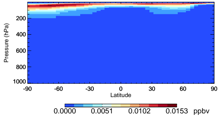
v11-02a BrNO3 - Species Curtain @ -180.000 for Jan
