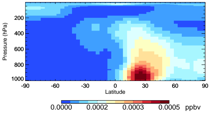
v11-01-public-Run0 ASOG1 - Species Zonal Mean for Jan
