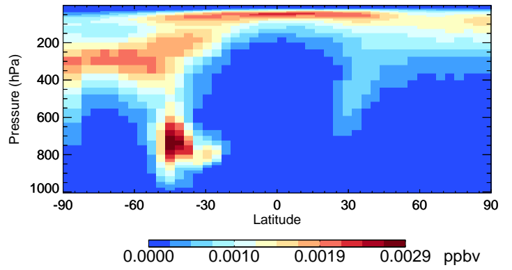
v11-01-public-Run0 ISOA1 - Species Curtain @ -180.000 for Jan
