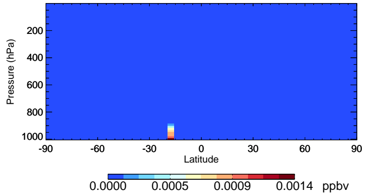
v11-02a MTPO - Species Curtain @ -180.000 for Jan
