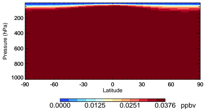
v11-01-public-Run0 HCFC141b - Species Zonal Mean for Jan
