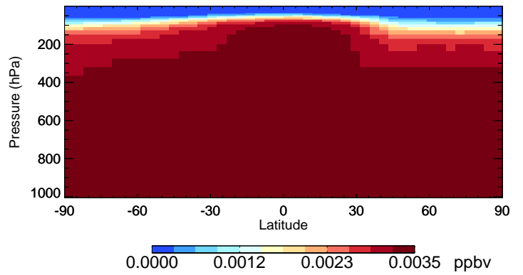
v11-02c H1211 - Species Curtain @ -180.000 for Jan
