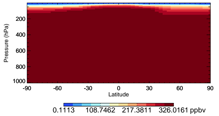
v11-01-public-Run0 N2O - Species Curtain @ -180.000 for Jan
