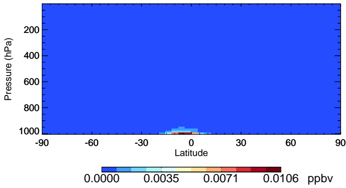
v11-01-public-Run0 MTPO - Species Zonal Mean for Jan
