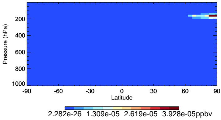
v11-01-public-Run0 CINO2 - Species Zonal Mean for Jan
