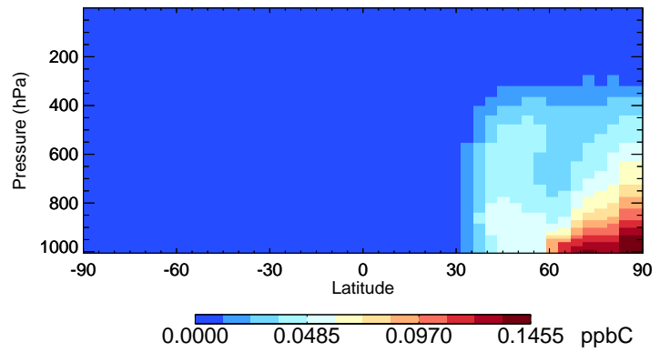
v11-02c XYLE - Species Curtain @ -180.000 for Jan
