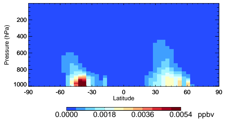
v11-02c BCPO - Species Curtain @ -180.000 for Jan
