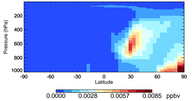
v11-02a MGLY - Species Curtain @ -180.000 for Jan
