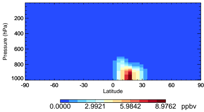
v11-01-public-Run0 DST1 - Species Zonal Mean for Jan
