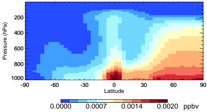
v11-02a CHBr3 - Species Zonal Mean for Jan
