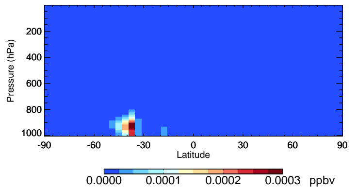
v11-02c ISOPNB - Species Curtain @ -180.000 for Jan
