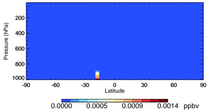
v11-02c MTPO - Species Curtain @ -180.000 for Jan
