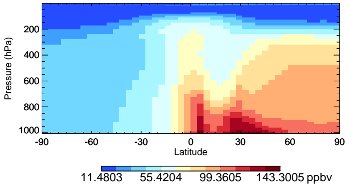
v11-02a CO - Species Zonal Mean for Jan
