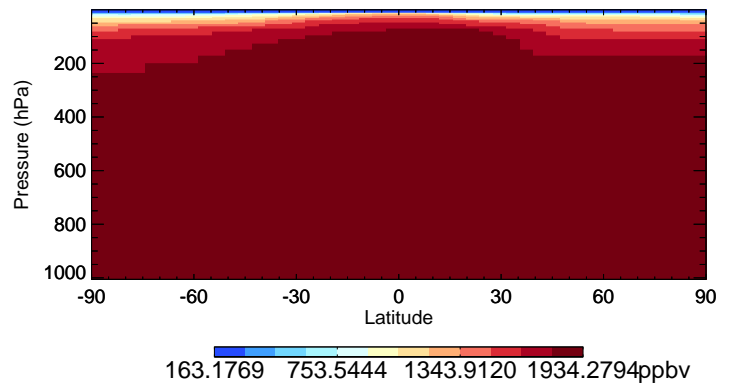
v11-01-public-Run0 CH4 - Species Curtain @ -180.000 for Jan
