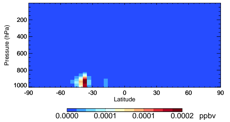
v11-01-public-Run0 ISOPNB - Species Curtain @ -180.000 for Jan
