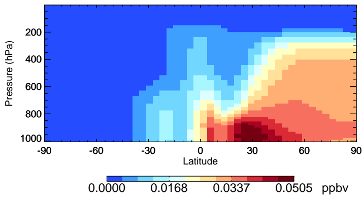
v11-01-public-Run0 R4N2 - Species Zonal Mean for Jan
