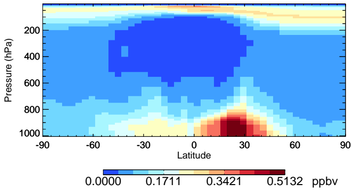
v11-01-public-Run0 SO4 - Species Zonal Mean for Jan
