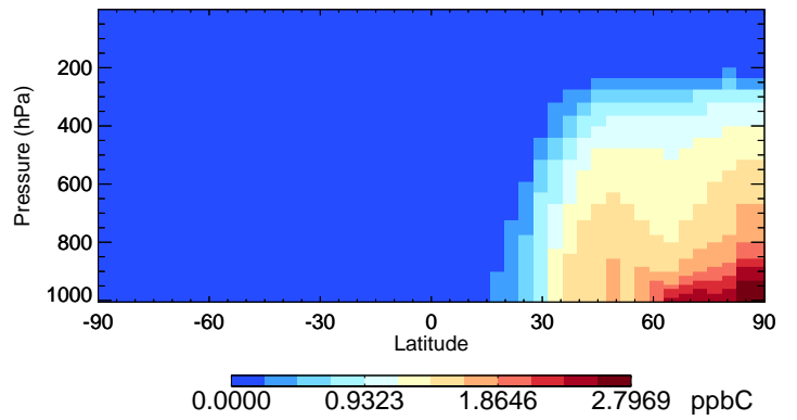
v11-02c ALK4 - Species Curtain @ -180.000 for Jan
