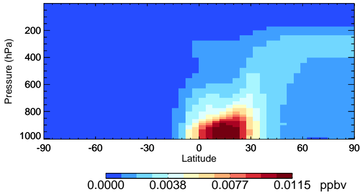
v11-02a ASOAN - Species Zonal Mean for Jan
