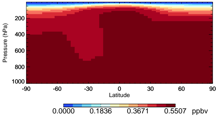
v11-02a CH3Cl - Species Zonal Mean for Jan
