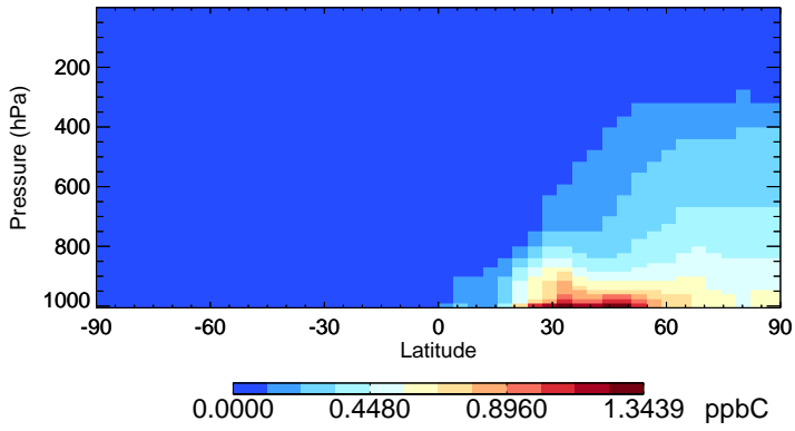
v11-02a TOLU - Species Zonal Mean for Jan
