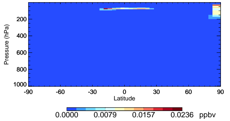
v11-01-public-Run0 Cl2 - Species Curtain @ -180.000 for Jan
