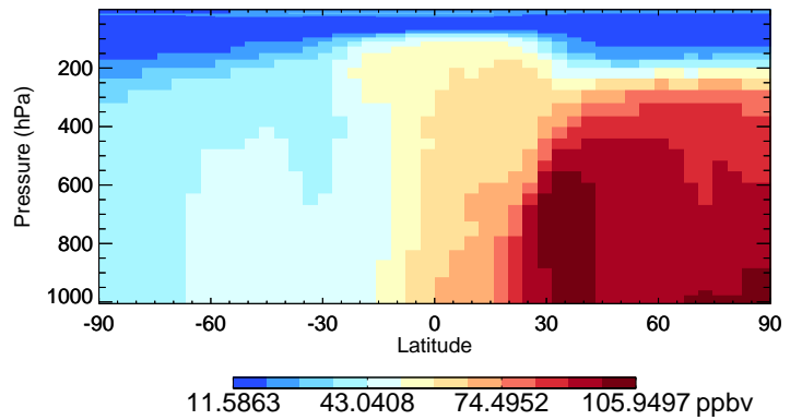
v11-02c CO - Species Curtain @ -180.000 for Jan
