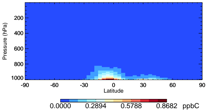
v11-02c PRPE - Species Zonal Mean for Jan
