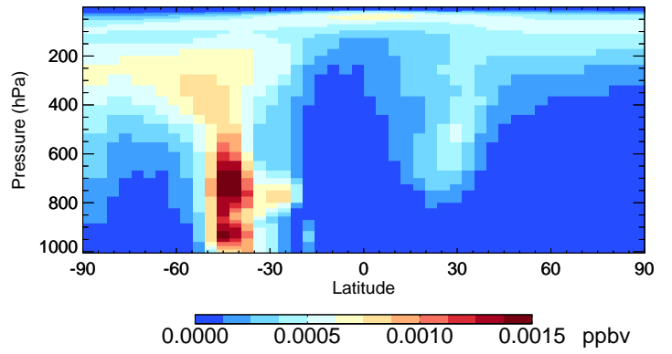
v11-01-public-Run0 TSOA0 - Species Curtain @ -180.000 for Jan
