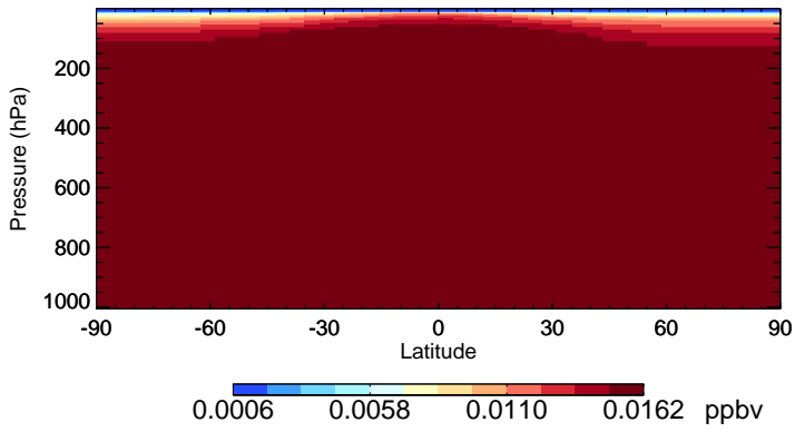
v11-01-public-Run0 CFC114 - Species Zonal Mean for Jan
