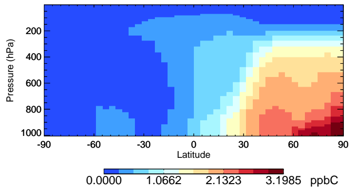
v11-02a C2H6 - Species Curtain @ -180.000 for Jan
