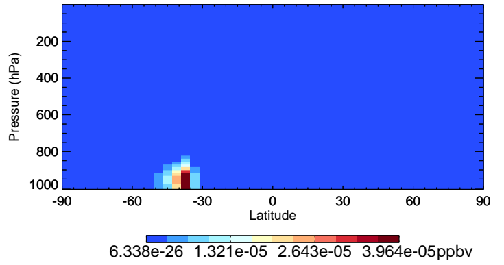
v11-02a MOBA - Species Curtain @ -180.000 for Jan
