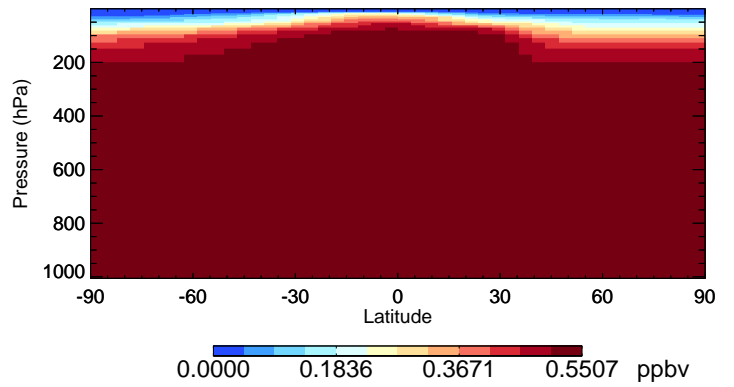
v11-02c CH3Cl - Species Curtain @ -180.000 for Jan
