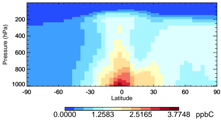
v11-02c ACET - Species Zonal Mean for Jan
