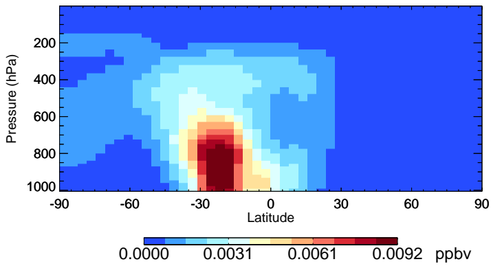
v11-02c ISOG1 - Species Zonal Mean for Jan
