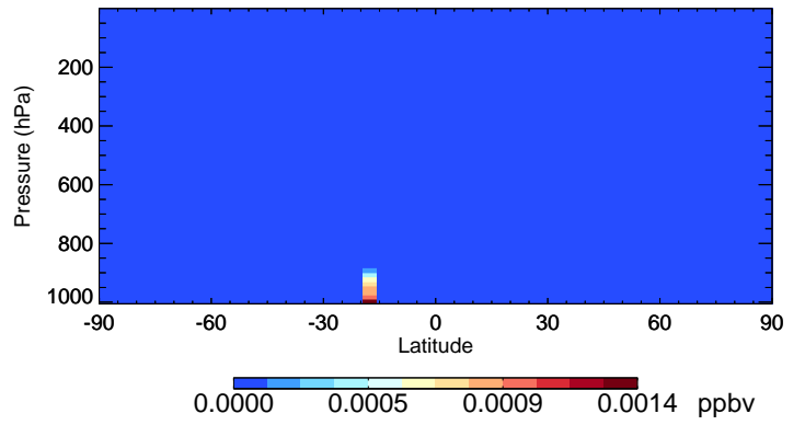
v11-01-public-Run0 MTPO - Species Curtain @ -180.000 for Jan
