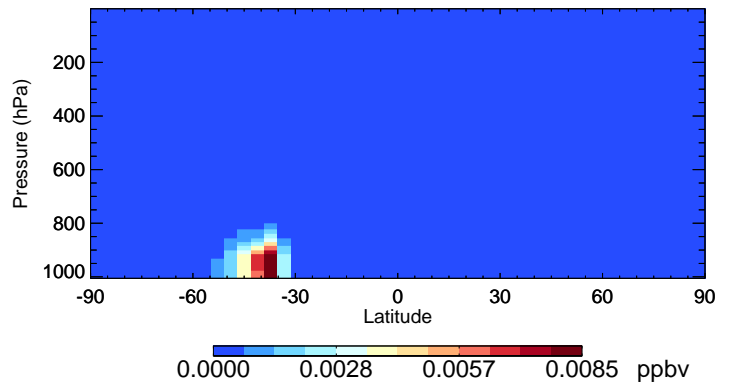
v11-02c MVK - Species Curtain @ -180.000 for Jan
