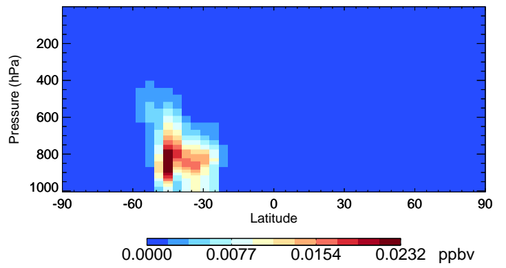
v11-01-public-Run0 DST4 - Species Curtain @ -180.000 for Jan
