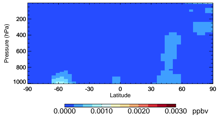
v11-01-public-Run0 Br2 - Species Curtain @ -180.000 for Jan
