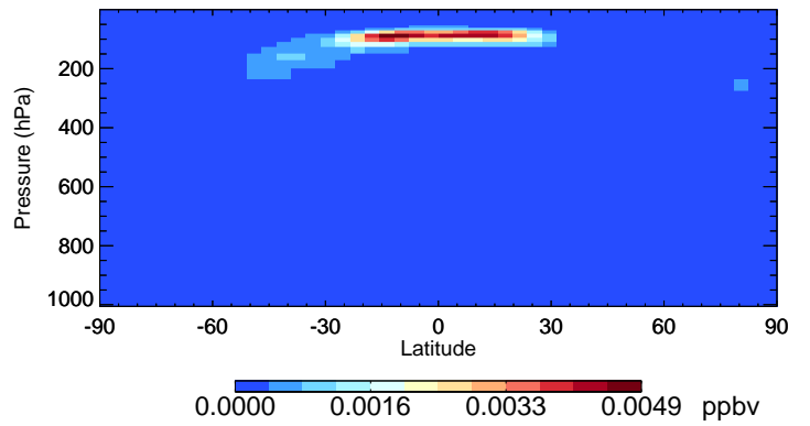
v11-02c ISOA3 - Species Curtain @ -180.000 for Jan
