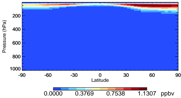
v11-02c CINO3 - Species Zonal Mean for Jan
