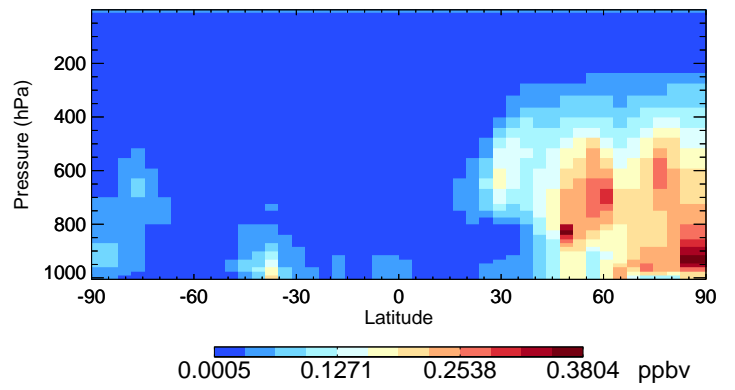
v11-01-public-Run0 SO2 - Species Curtain @ -180.000 for Jan
