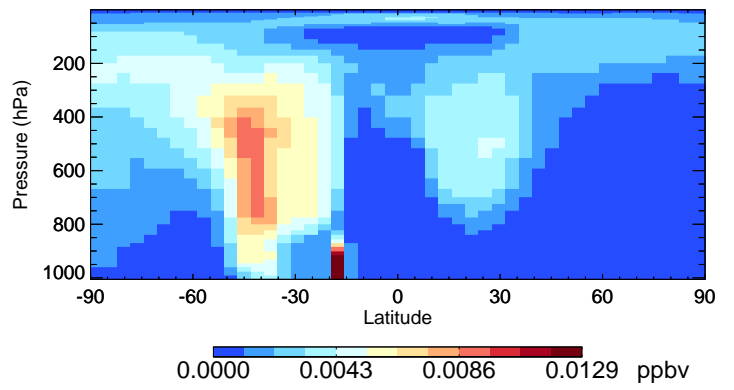
v11-01-public-Run0 TSOG2 - Species Curtain @ -180.000 for Jan
