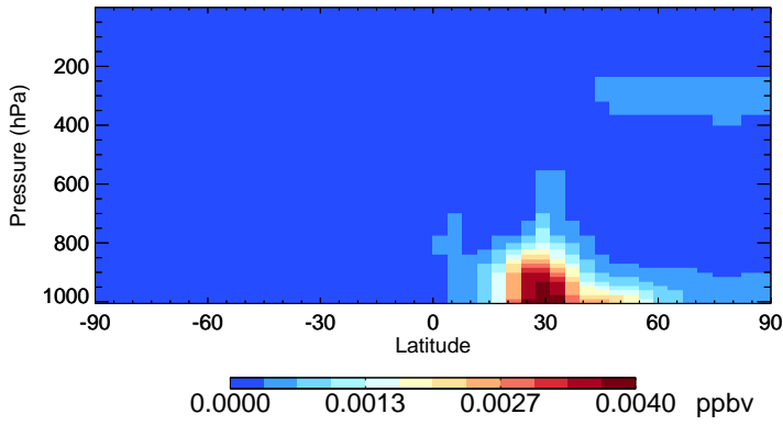
v11-02a ASOA2 - Species Zonal Mean for Jan
