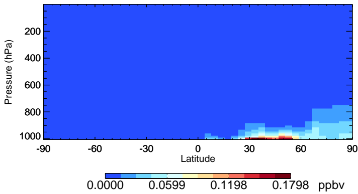
v11-02c HNO2 - Species Zonal Mean for Jan
