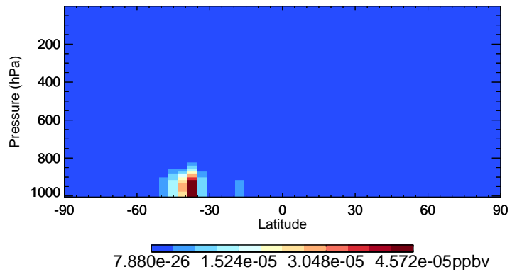
v11-02c MOBA - Species Curtain @ -180.000 for Jan
