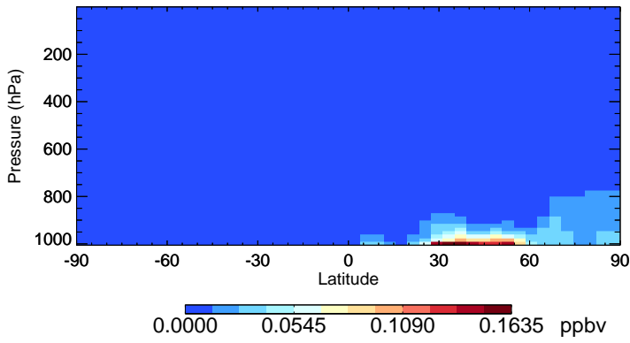
v11-01-public-Run0 HNO2 - Species Zonal Mean for Jan
