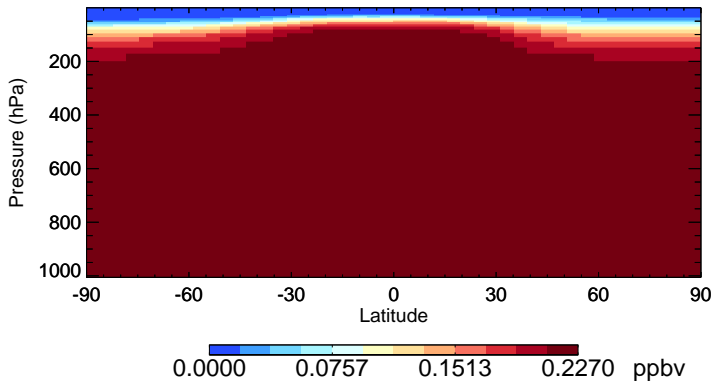
v11-01-public-Run0 CFC11 - Species Zonal Mean for Jan
