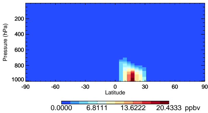
v11-02c DST2 - Species Zonal Mean for Jan
