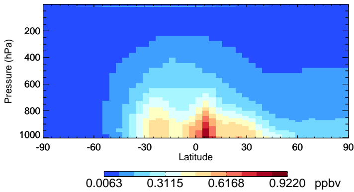
v11-02c CH2O - Species Zonal Mean for Jan
