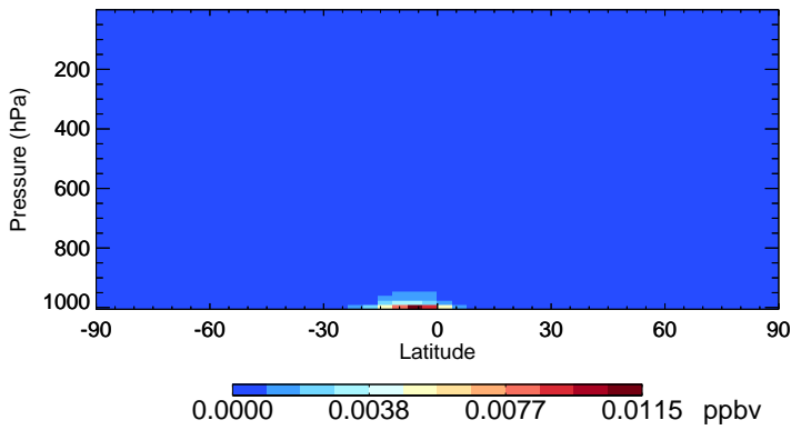
v11-02c LIMO - Species Zonal Mean for Jan
