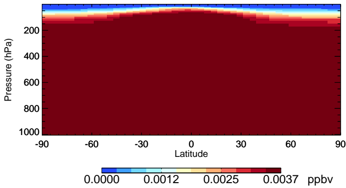
v11-02c H1301 - Species Zonal Mean for Jan
