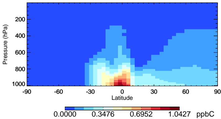
v11-02c MEK - Species Zonal Mean for Jan
