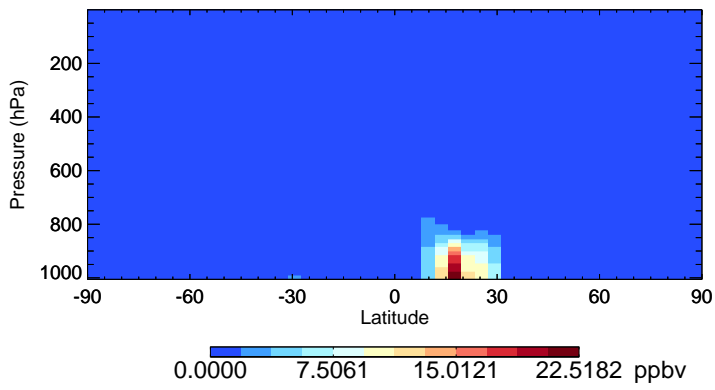
v11-01-public-Run0 DST4 - Species Zonal Mean for Jan
