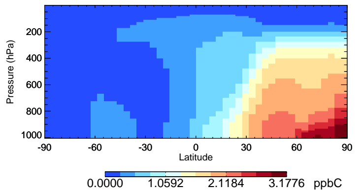
v11-02c C2H6 - Species Curtain @ -180.000 for Jan
