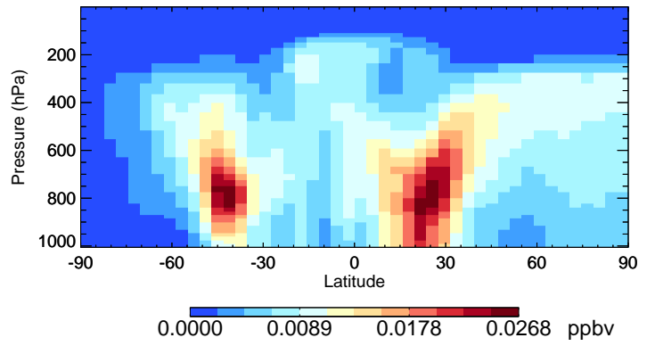
v11-01-public-Run0 MAP - Species Curtain @ -180.000 for Jan
