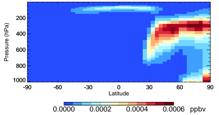
v11-02a ASOA2 - Species Curtain @ -180.000 for Jan
