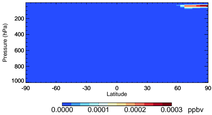
v11-02c CINO2 - Species Zonal Mean for Jan
