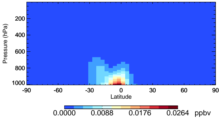
v11-02a TSOA0 - Species Zonal Mean for Jan
