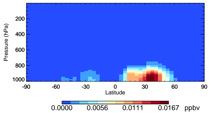
v11-02c NITs - Species Curtain @ -180.000 for Jan
