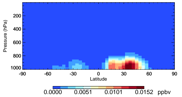
v11-02a NITs - Species Curtain @ -180.000 for Jan
