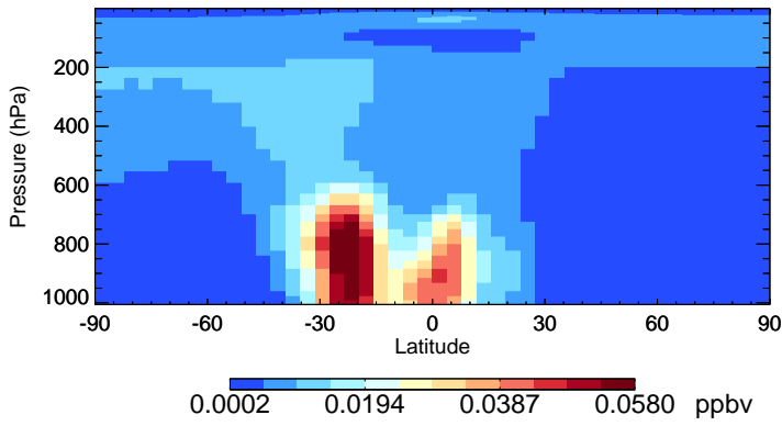
v11-01-public-Run0 ISO3 - Species Zonal Mean for Jan
