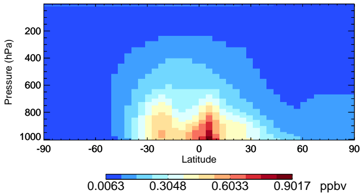
v11-01-public-Run0 CH2O - Species Zonal Mean for Jan
