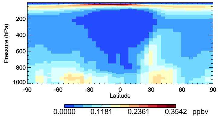
v11-02c SO4 - Species Curtain @ -180.000 for Jan
