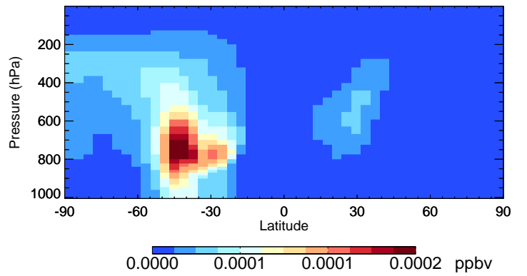
v11-02c ISN1OA - Species Curtain @ -180.000 for Jan
