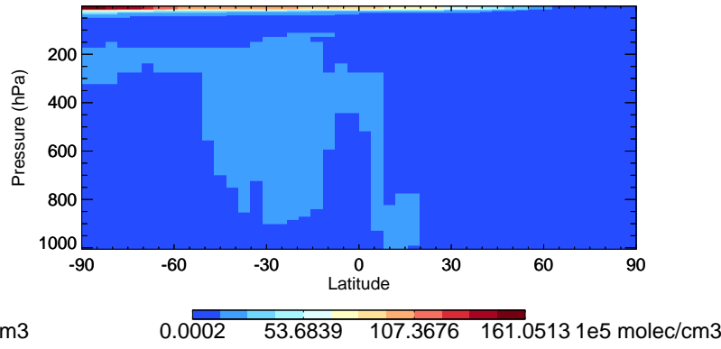
v11-02a OH - Species Curtain @ -180.000 for Jan
