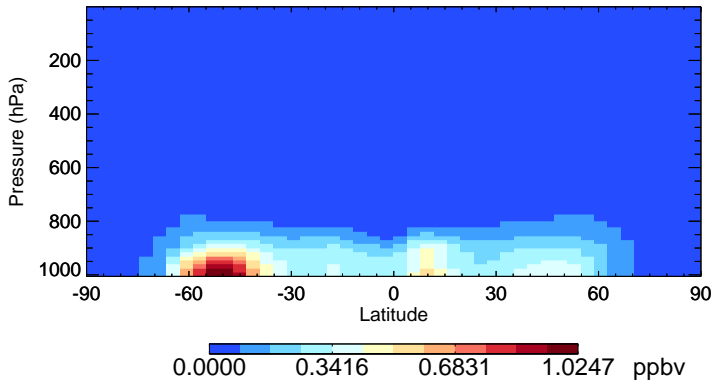
v11-02a SALA - Species Zonal Mean for Jan
