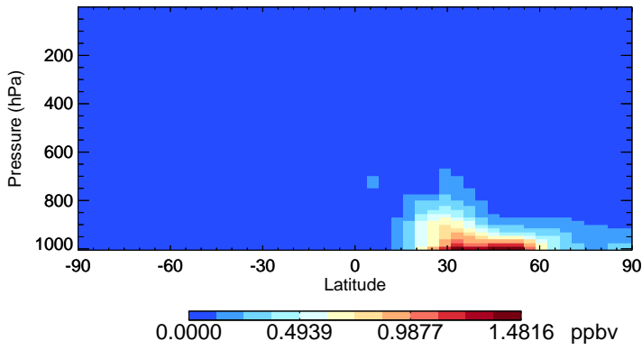
v11-01-public-Run0 NIT - Species Zonal Mean for Jan
