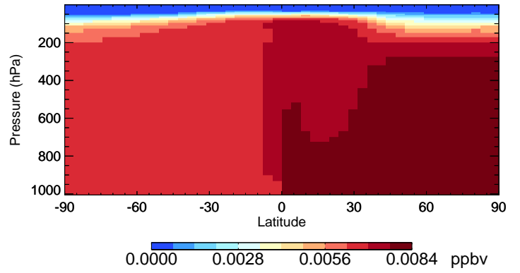
v11-02a CH3Br - Species Curtain @ -180.000 for Jan
