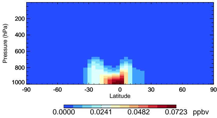
v11-01-public-Run0 MACR - Species Zonal Mean for Jan
