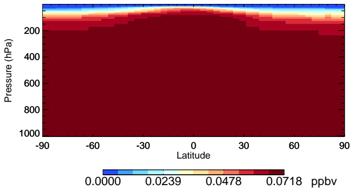
v11-02c CFC113 - Species Zonal Mean for Jan
