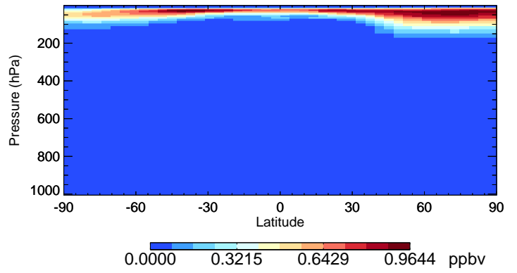
v11-01-public-Run0 CINO3 - Species Curtain @ -180.000 for Jan
