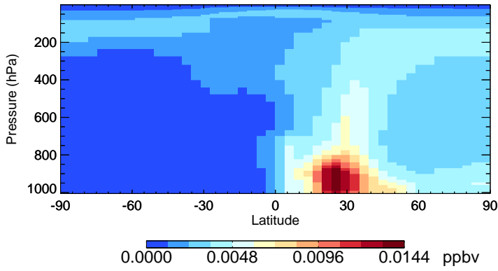
v11-02a ASOG3 - Species Zonal Mean for Jan
