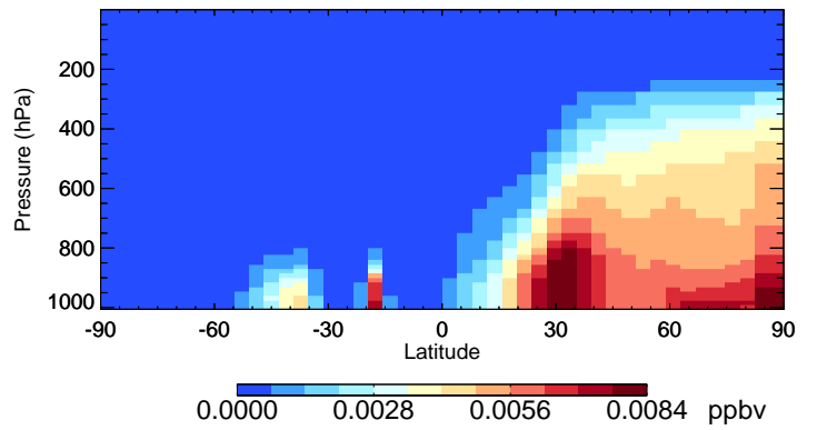
v11-02c RCHO - Species Curtain @ -180.000 for Jan
