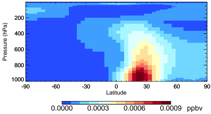
v11-02a ASOG1 - Species Zonal Mean for Jan
