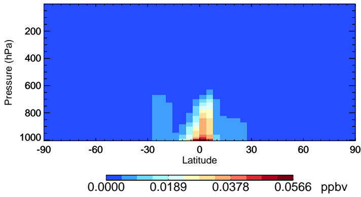
v11-01-public-Run0 TSOA2 - Species Zonal Mean for Jan
