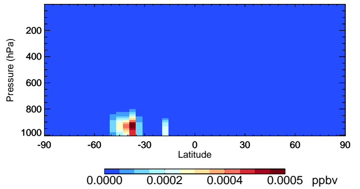
v11-02c RIPB - Species Curtain @ -180.000 for Jan
