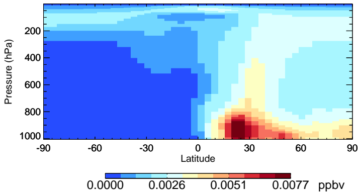
v11-01-public-Run0 ASOG3 - Species Zonal Mean for Jan
