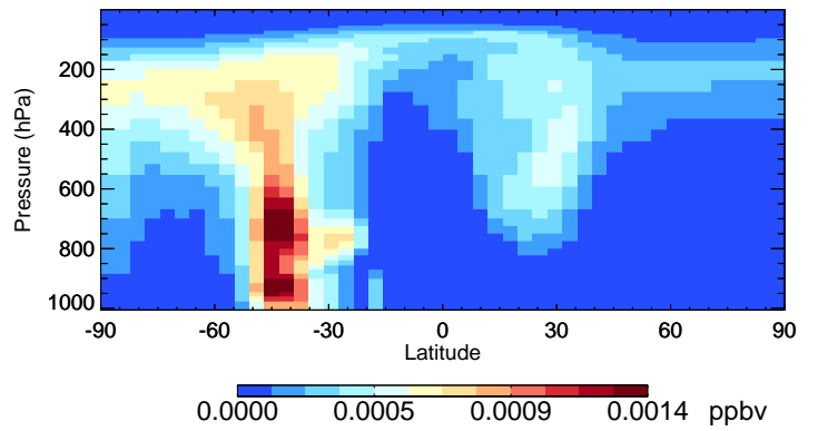
v11-02c TSOA0 - Species Curtain @ -180.000 for Jan
