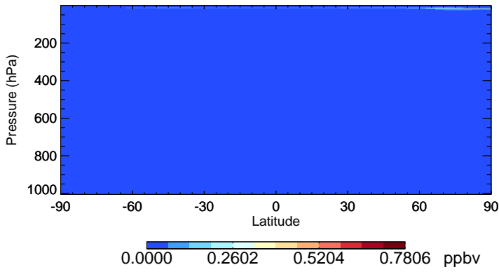
v11-01-public-Run0 NO3 - Species Zonal Mean for Jan
