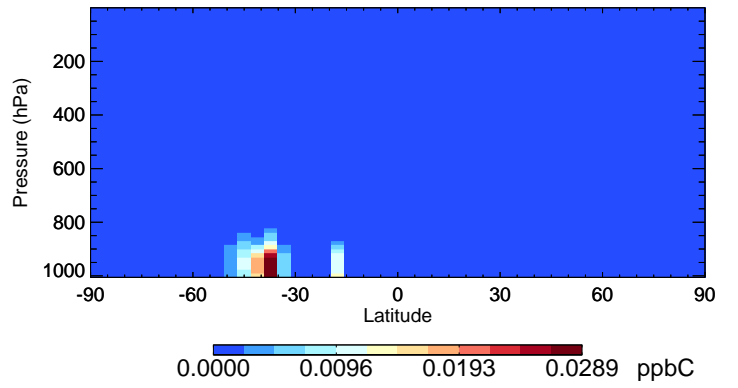
v11-01-public-Run0 ISOP - Species Curtain @ -180.000 for Jan
