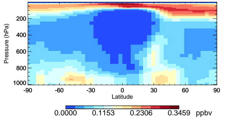
v11-02a SO4 - Species Curtain @ -180.000 for Jan
