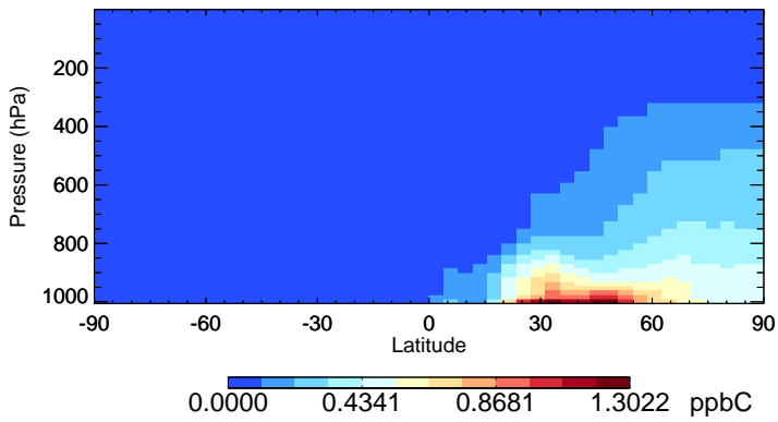
v11-02c TOLU - Species Zonal Mean for Jan
