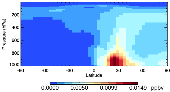
v11-02c ASOG3 - Species Zonal Mean for Jan
