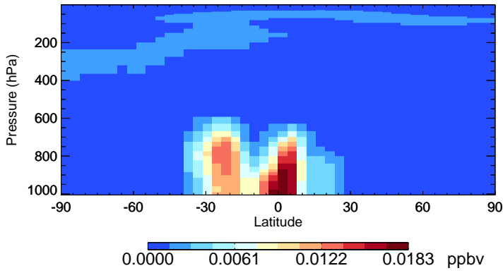
v11-02a ISOA1 - Species Zonal Mean for Jan
