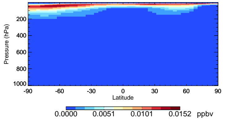
v11-01-public-Run0 BrNO3 - Species Curtain @ -180.000 for Jan
