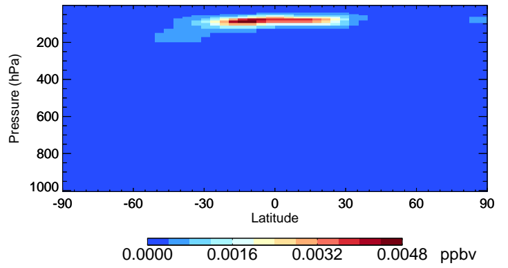
v11-01-public-Run0 ISOA3 - Species Curtain @ -180.000 for Jan
