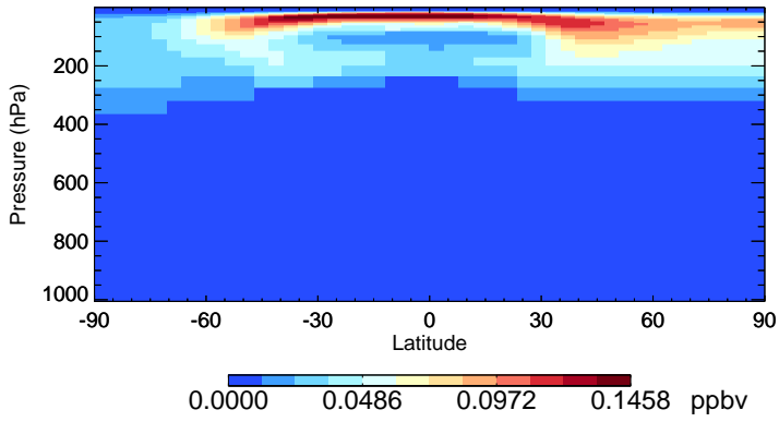
v11-02a MPN - Species Zonal Mean for Jan
