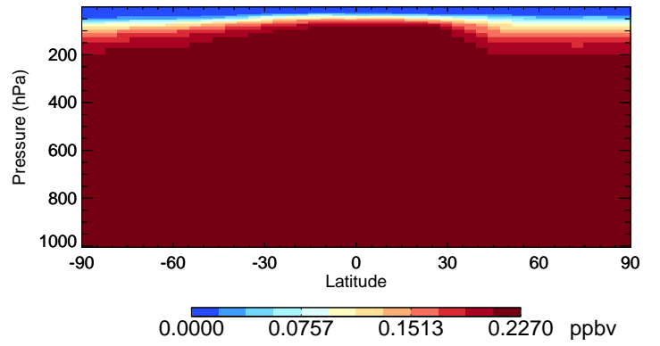
v11-01-public-Run0 CFC11 - Species Curtain @ -180.000 for Jan
