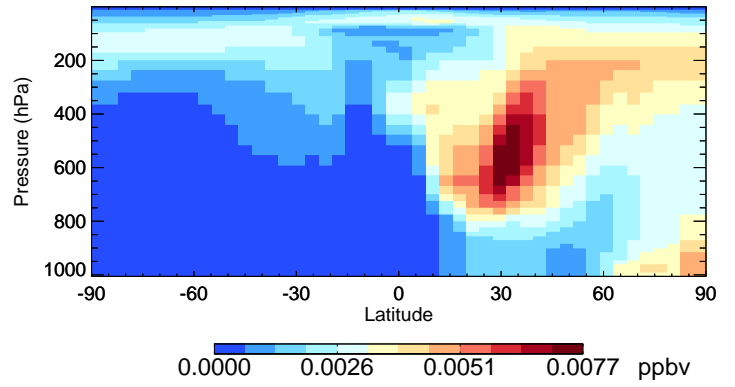
v11-02a ASOG3 - Species Curtain @ -180.000 for Jan
