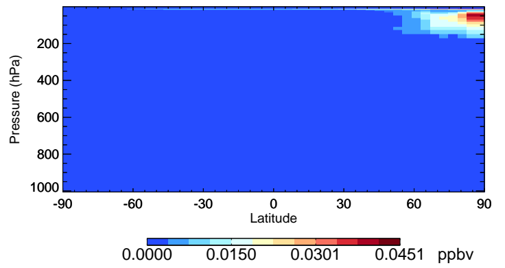
v11-01-public-Run0 OCIO - Species Curtain @ -180.000 for Jan
