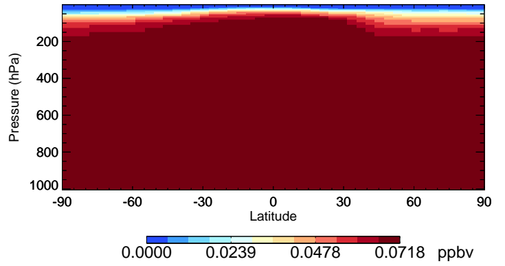
v11-02a CFC113 - Species Curtain @ -180.000 for Jan
