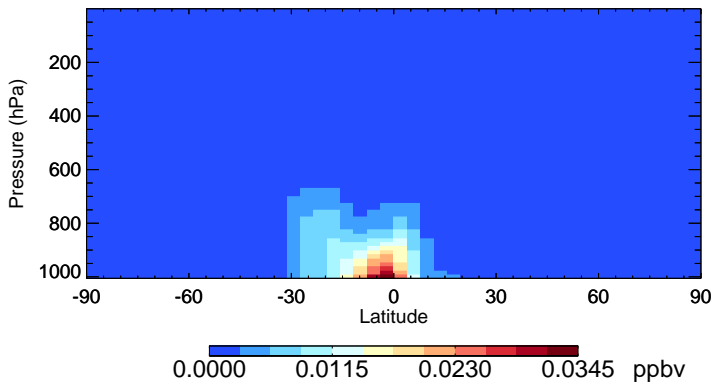
v11-02c TSOA0 - Species Zonal Mean for Jan
