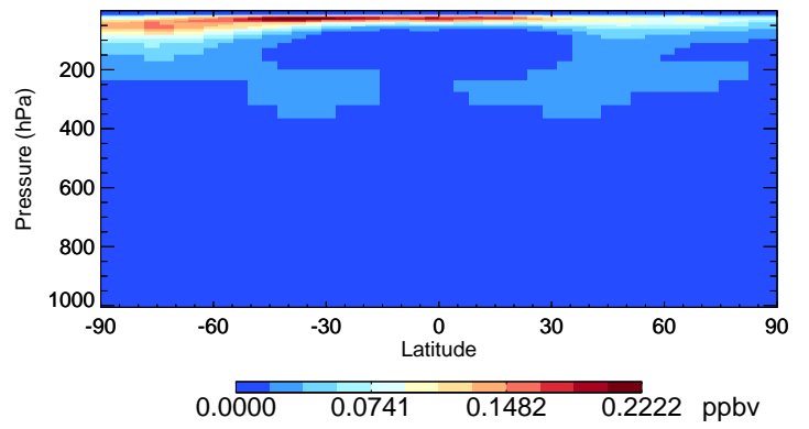
v11-01-public-Run0 HNO4 - Species Curtain @ -180.000 for Jan
