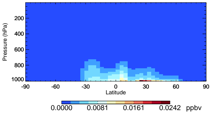
v11-02c GLYX - Species Zonal Mean for Jan
