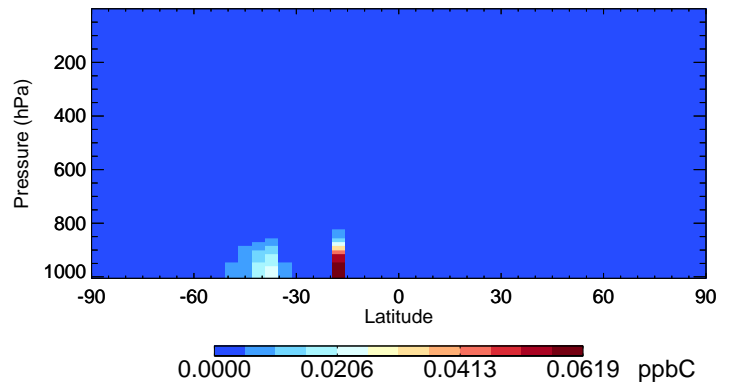
v11-02c PRPE - Species Curtain @ -180.000 for Jan
