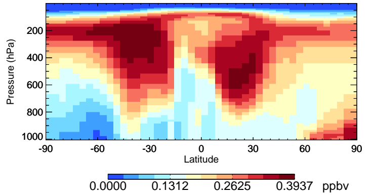
v11-02a EOH - Species Curtain @ -180.000 for Jan
