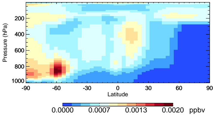
v11-01-public-Run0 HBr - Species Zonal Mean for Jan
