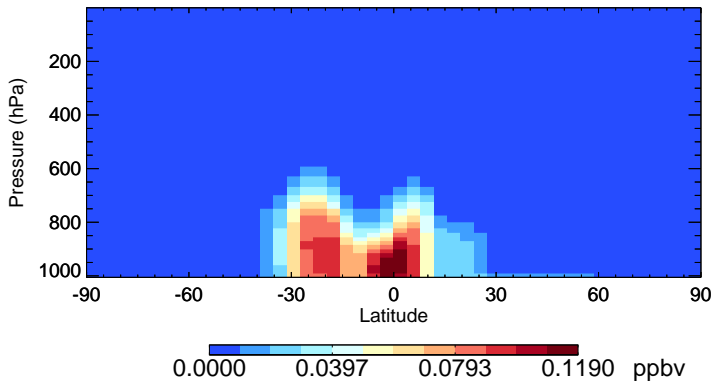
v11-01-public-Run0 GLYC - Species Zonal Mean for Jan
