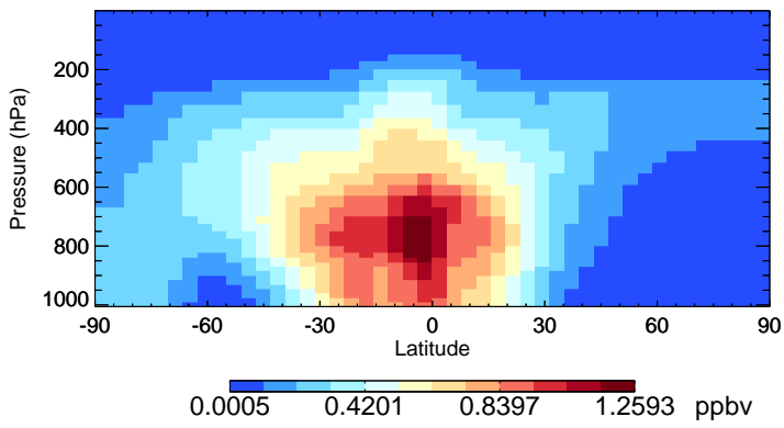
v11-02a H2O2 - Species Zonal Mean for Jan
