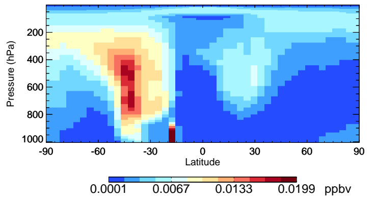
v11-02a TSOG3 - Species Curtain @ -180.000 for Jan
