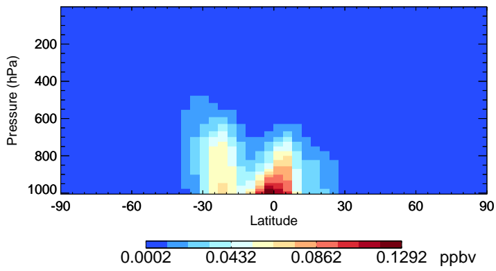
v11-02a TSOG3 - Species Zonal Mean for Jan
