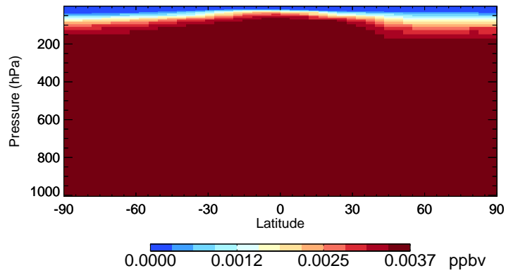
v11-02c H1301 - Species Curtain @ -180.000 for Jan
