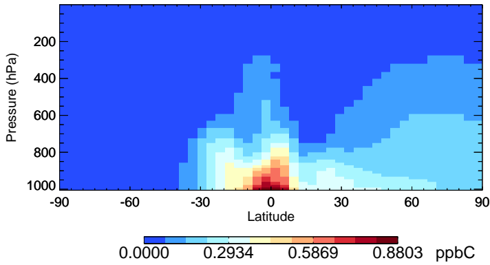
v11-02a MEK - Species Zonal Mean for Jan
