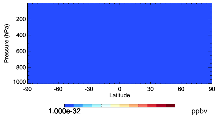
v11-02a IEPOXD - Species Curtain @ -180.000 for Jan
