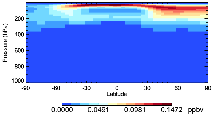
v11-02c MPN - Species Zonal Mean for Jan
