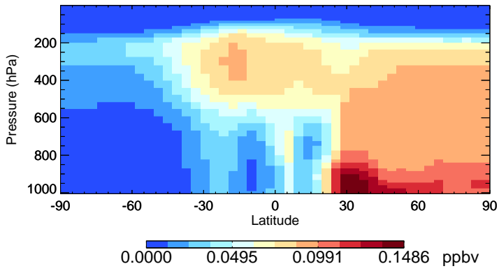
v11-01-public-Run0 PAN - Species Zonal Mean for Jan
