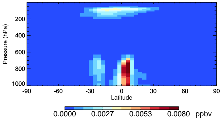
v11-01-public-Run0 ISOA3 - Species Zonal Mean for Jan
