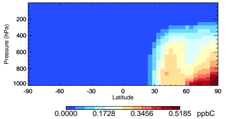
v11-02c TOLU - Species Curtain @ -180.000 for Jan
