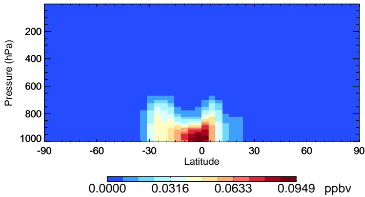
v11-01-public-Run0 MVK - Species Zonal Mean for Jan
