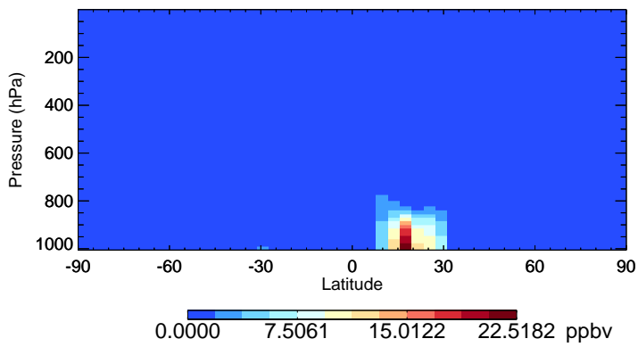
v11-02c DST4 - Species Zonal Mean for Jan
