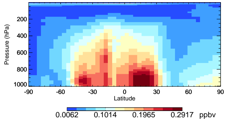
v11-01-public-Run0 CH2O - Species Curtain @ -180.000 for Jan
