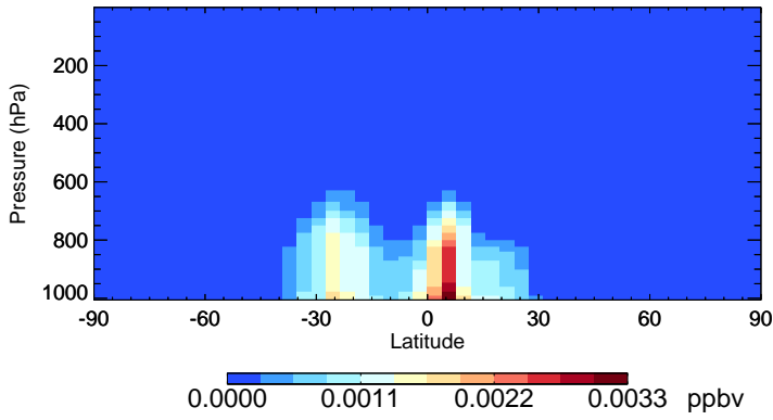
v11-02a NPMN - Species Zonal Mean for Jan
