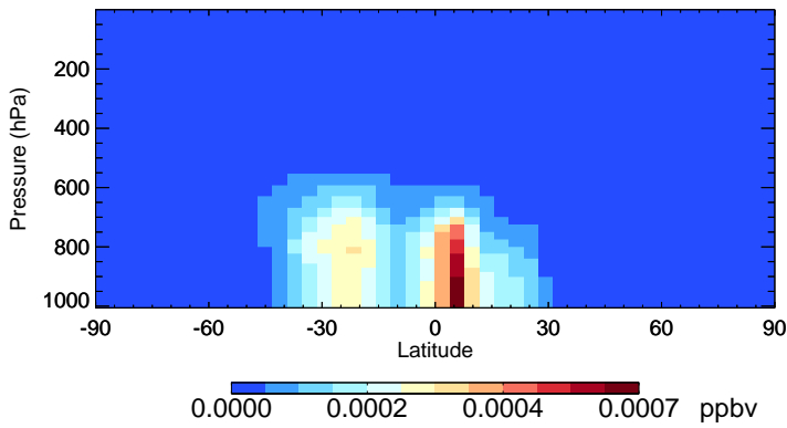
v11-02c ISN1OA - Species Zonal Mean for Jan
