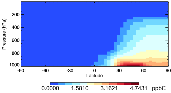
v11-02a ALK4 - Species Zonal Mean for Jan
