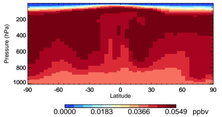
v11-02c HCFC141b - Species Curtain @ -180.000 for Jan
