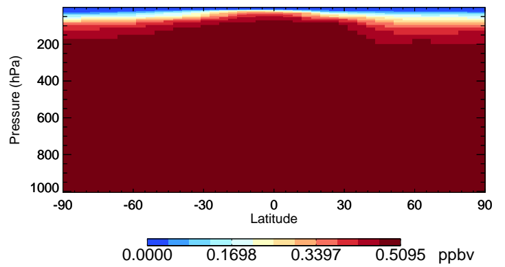
v11-02c CFC12 - Species Curtain @ -180.000 for Jan
