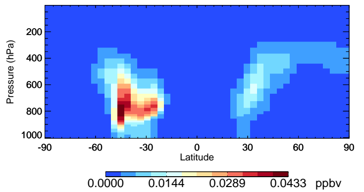
v11-02c DST2 - Species Curtain @ -180.000 for Jan
