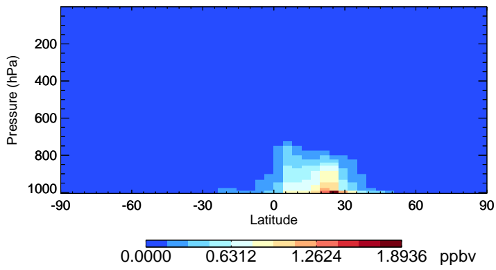
v11-01-public-Run0 NH3 - Species Zonal Mean for Jan
