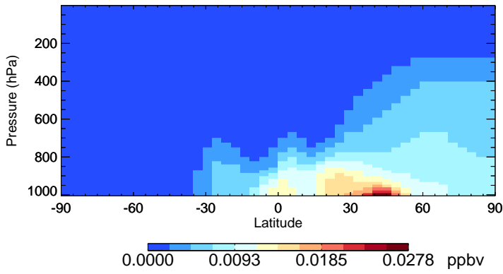
v11-01-public-Run0 RCHO - Species Zonal Mean for Jan
