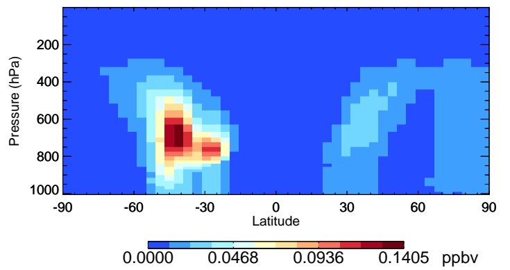
v11-02c DST1 - Species Curtain @ -180.000 for Jan
