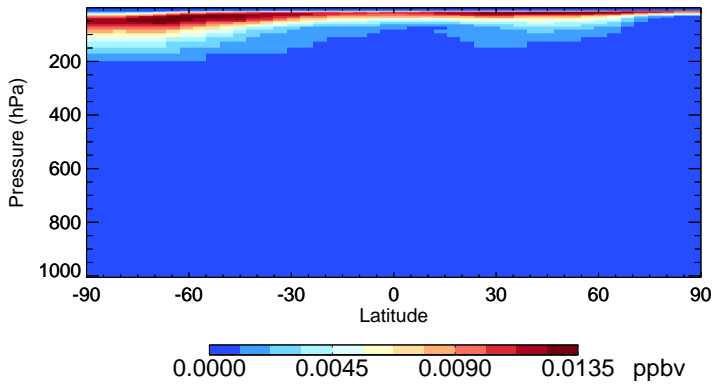
v11-01-public-Run0 BrNO3 - Species Zonal Mean for Jan
