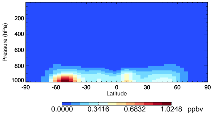
v11-01-public-Run0 SALA - Species Zonal Mean for Jan
