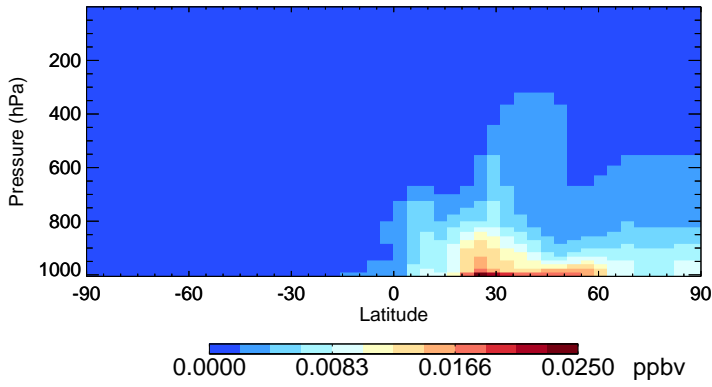
v11-02a MGLY - Species Zonal Mean for Jan
