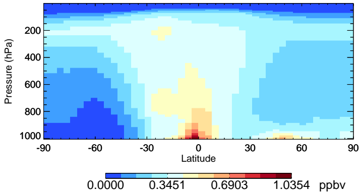
v11-02a EOH - Species Zonal Mean for Jan
