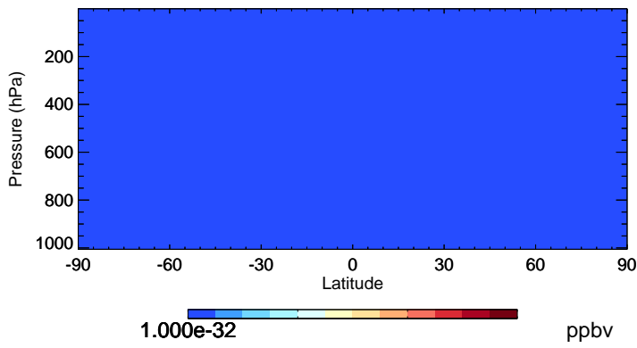
v11-02a DHDN - Species Zonal Mean for Jan
