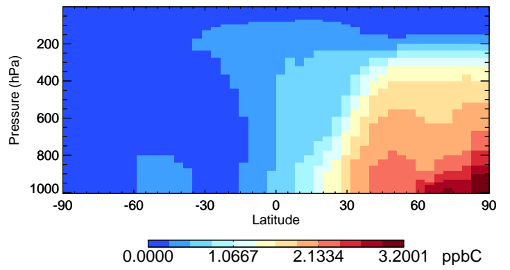
v11-01-public-Run0 C2H6 - Species Curtain @ -180.000 for Jan
