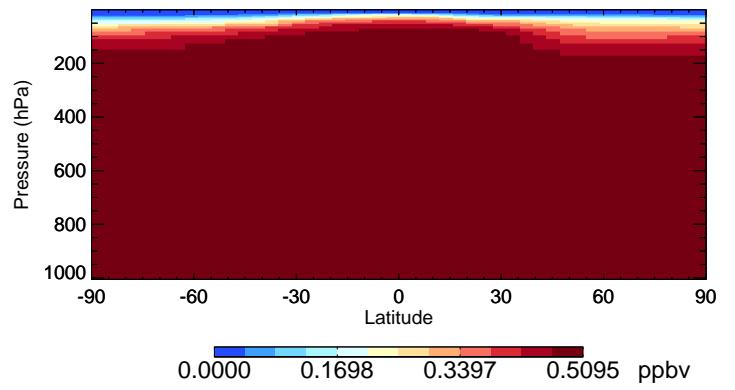
v11-01-public-Run0 CFC12 - Species Curtain @ -180.000 for Jan
