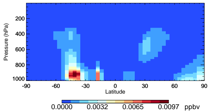
v11-02c HAC - Species Curtain @ -180.000 for Jan
