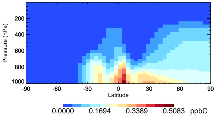
v11-01-public-Run0 MEK - Species Zonal Mean for Jan
