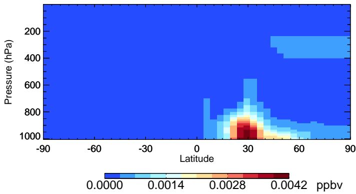
v11-02c ASOA2 - Species Zonal Mean for Jan
