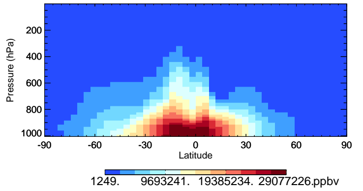
v11-01-public-Run0 H2O - Species Curtain @ -180.000 for Jan
