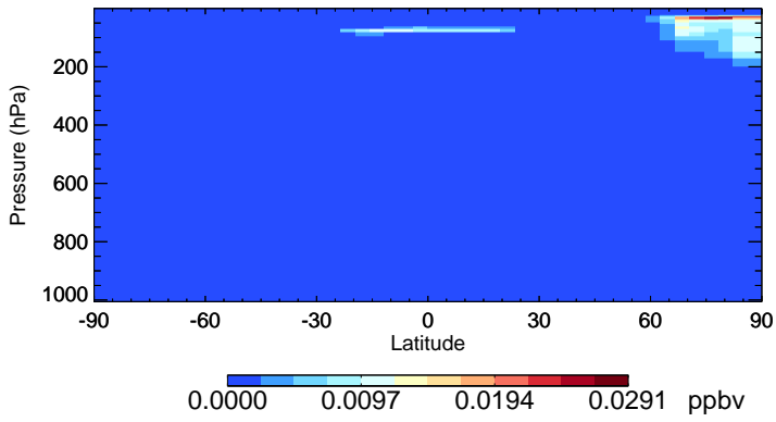
v11-01-public-Run0 Cl2 - Species Zonal Mean for Jan
