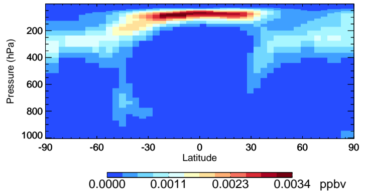
v11-01-public-Run0 TSOA2 - Species Curtain @ -180.000 for Jan
