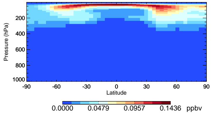
v11-01-public-Run0 MPN - Species Curtain @ -180.000 for Jan
