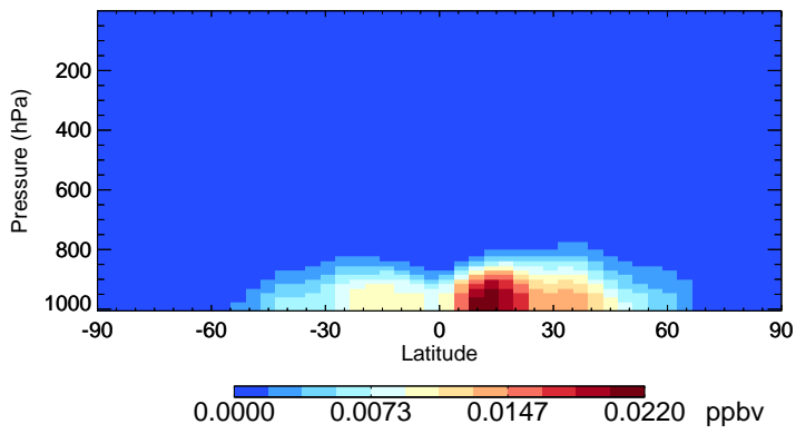
v11-01-public-Run0 NITs - Species Zonal Mean for Jan
