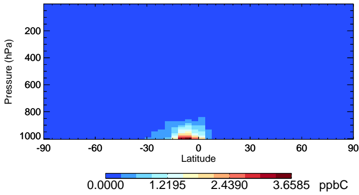
v11-01-public-Run0 ISOP - Species Zonal Mean for Jan
