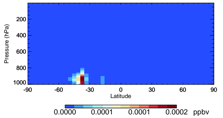
v11-02a ISOPNB - Species Curtain @ -180.000 for Jan
