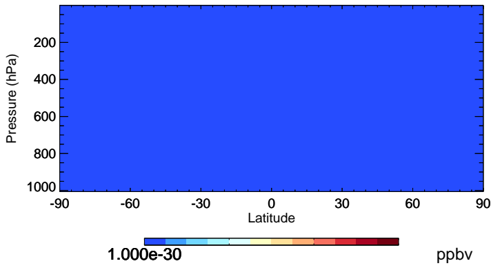
v11-01-public-Run0 MGLY - Species Zonal Mean for Jan
