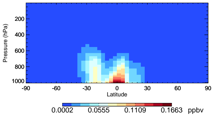
v11-01-public-Run0 TSOG3 - Species Zonal Mean for Jan
