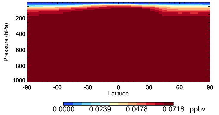
v11-01-public-Run0 CFC113 - Species Curtain @ -180.000 for Jan
