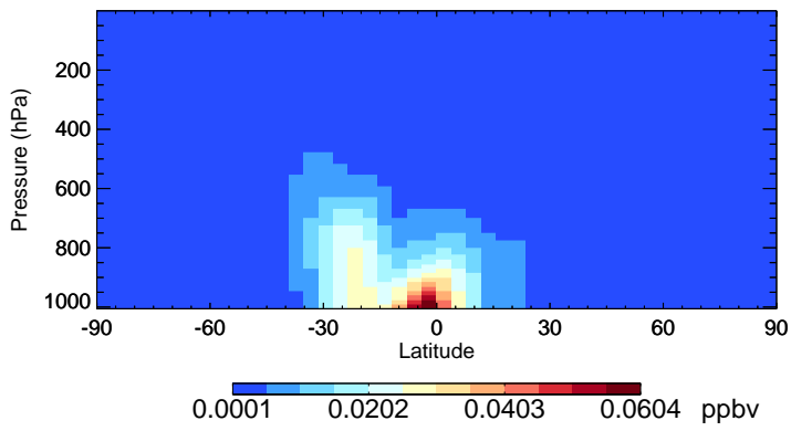
v11-02a TSOG2 - Species Zonal Mean for Jan
