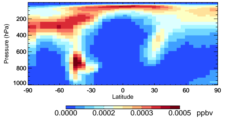
v11-01-public-Run0 TSOA1 - Species Curtain @ -180.000 for Jan
