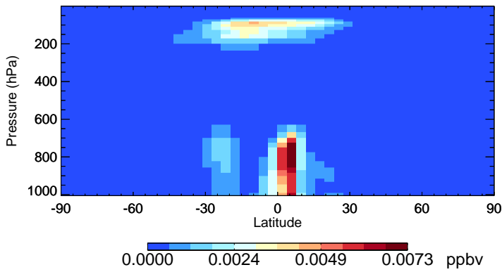
v11-02c ISOA3 - Species Zonal Mean for Jan
