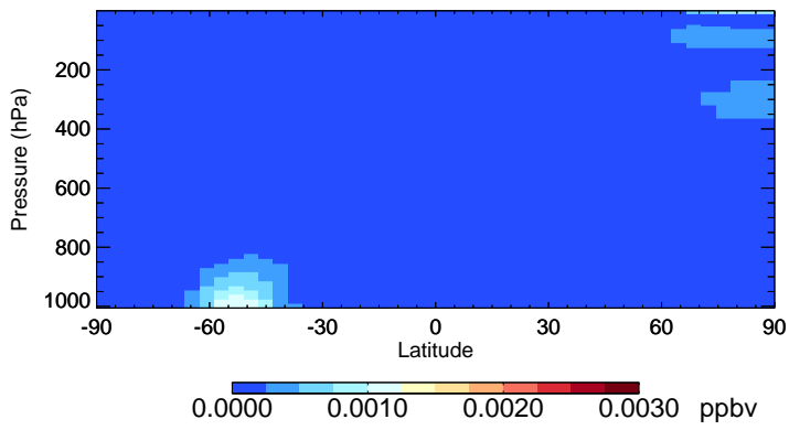
v11-01-public-Run0 Br2 - Species Zonal Mean for Jan
