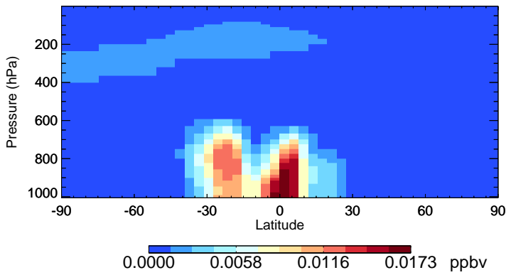
v11-02c ISOA1 - Species Zonal Mean for Jan
