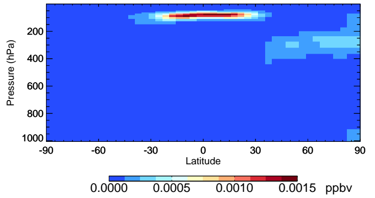
v11-01-public-Run0 ASOA3 - Species Curtain @ -180.000 for Jan
