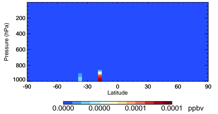
v11-01-public-Run0 LIMO - Species Curtain @ -180.000 for Jan
