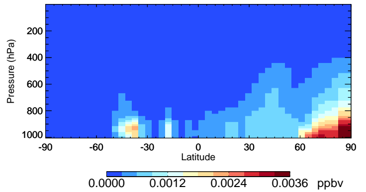
v11-02c MGLY - Species Curtain @ -180.000 for Jan
