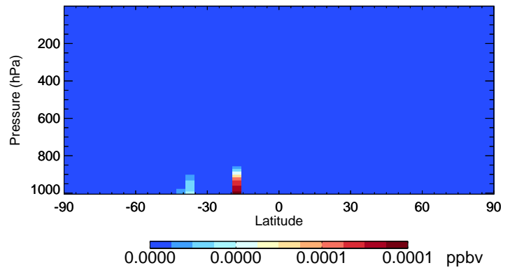
v11-02c LIMO - Species Curtain @ -180.000 for Jan
