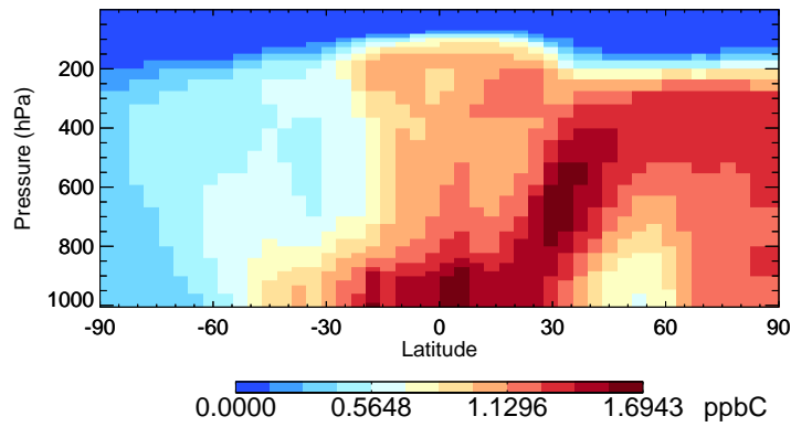
v11-02c ACET - Species Curtain @ -180.000 for Jan
