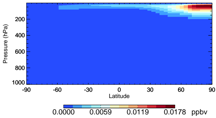
v11-01-public-Run0 BrCl - Species Zonal Mean for Jan
