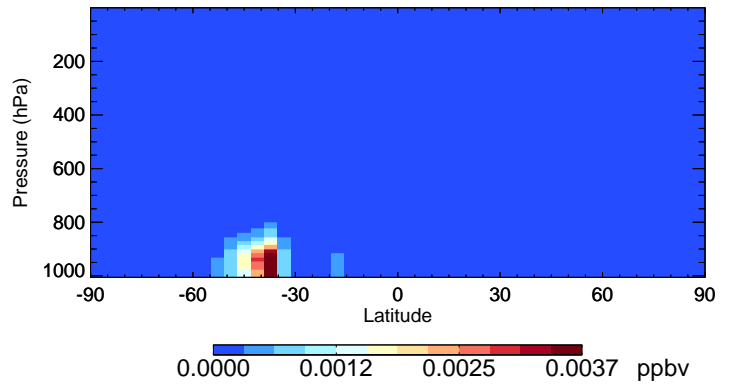
v11-01-public-Run0 MACR - Species Curtain @ -180.000 for Jan
