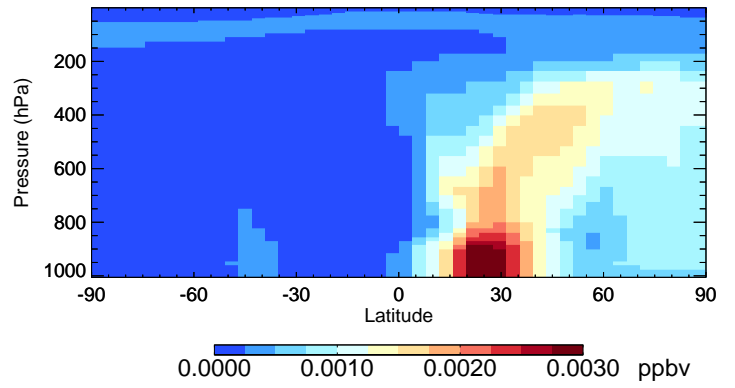
v11-01-public-Run0 ASOAN - Species Curtain @ -180.000 for Jan
