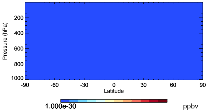
v11-01-public-Run0 EOH - Species Zonal Mean for Jan
