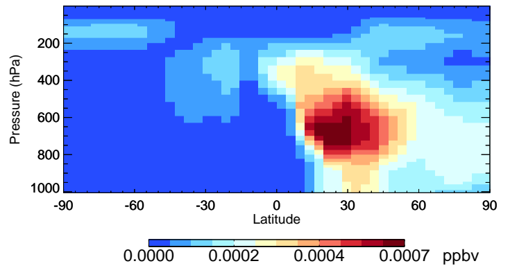
v11-02c ASOG1 - Species Curtain @ -180.000 for Jan
