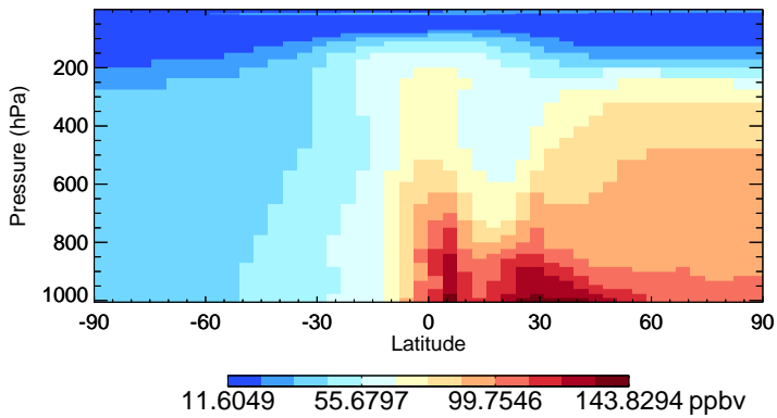
v11-02c CO - Species Zonal Mean for Jan
