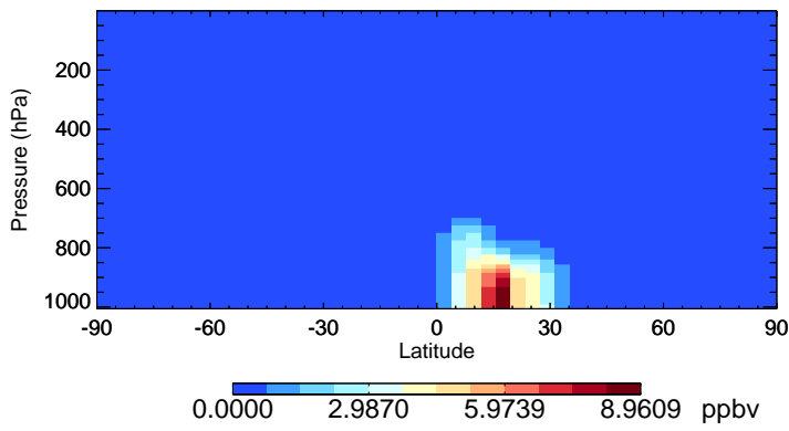
v11-02a DST1 - Species Zonal Mean for Jan
