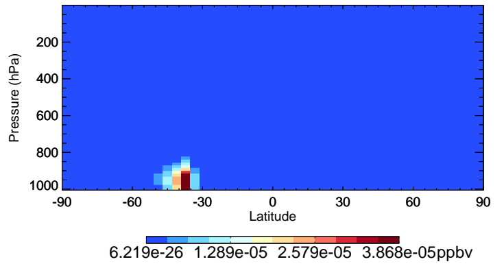
v11-01-public-Run0 MOBA - Species Curtain @ -180.000 for Jan
