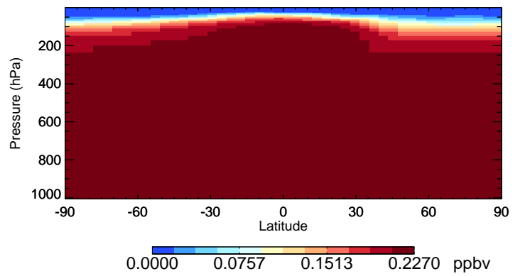
v11-02c CFC11 - Species Curtain @ -180.000 for Jan
