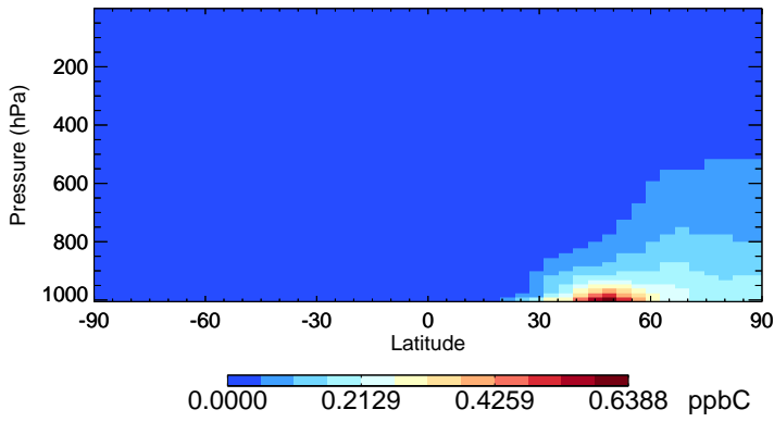
v11-01-public-Run0 XYLE - Species Zonal Mean for Jan
