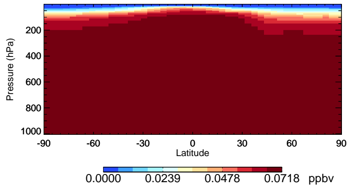
v11-02c CFC113 - Species Curtain @ -180.000 for Jan
