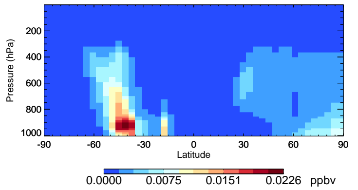
v11-01-public-Run0 HAC - Species Curtain @ -180.000 for Jan
