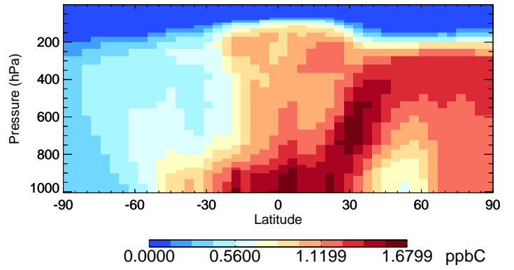
v11-02a ACET - Species Curtain @ -180.000 for Jan
