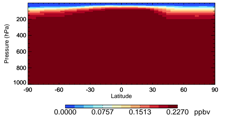
v11-02a CFC11 - Species Curtain @ -180.000 for Jan
