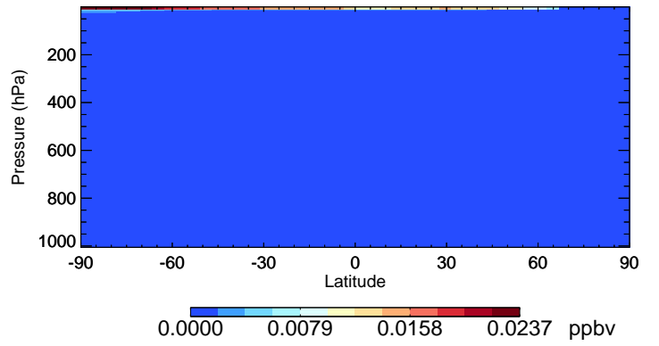
v11-01-public-Run0 Br - Species Curtain @ -180.000 for Jan
