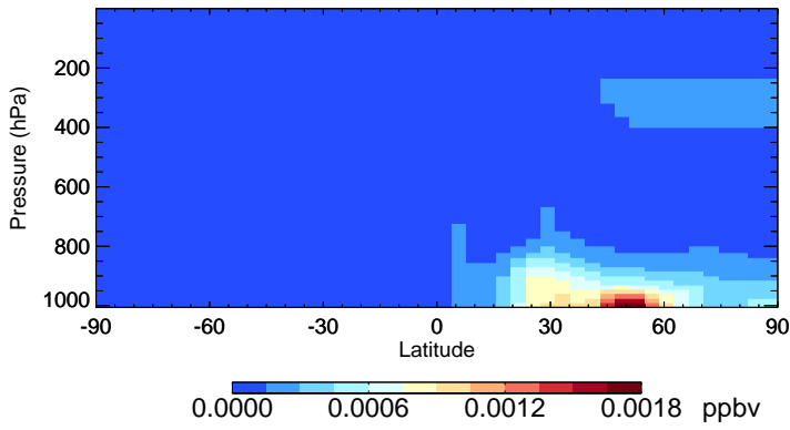
v11-01-public-Run0 ASOA2 - Species Zonal Mean for Jan
