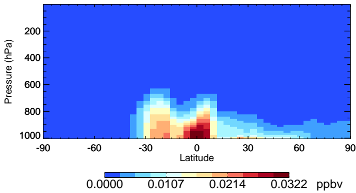
v11-02c MGLY - Species Zonal Mean for Jan
