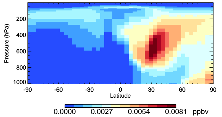
v11-02c ASOG3 - Species Curtain @ -180.000 for Jan
