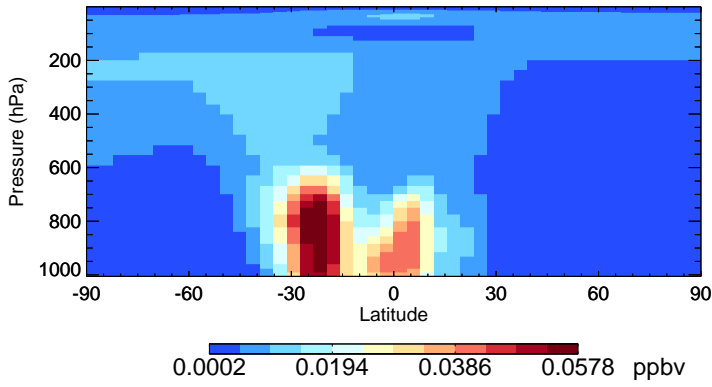
v11-02a ISO3 - Species Zonal Mean for Jan
