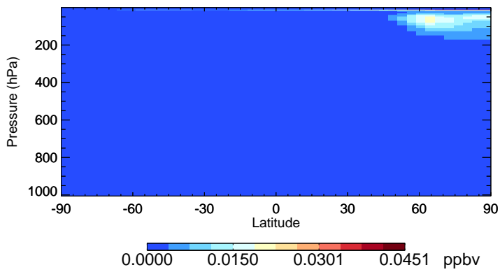
v11-02c OCIO - Species Zonal Mean for Jan
