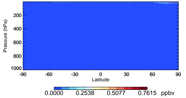
v11-02a NO3 - Species Curtain @ -180.000 for Jan
