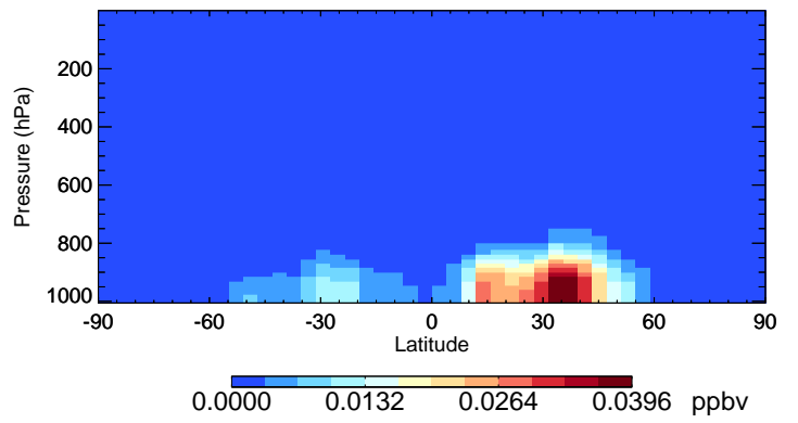
v11-01-public-Run0 NITs - Species Curtain @ -180.000 for Jan
