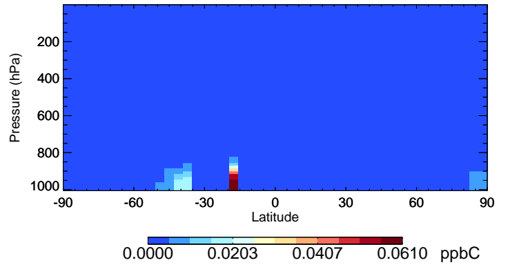
v11-02a PRPE - Species Curtain @ -180.000 for Jan
