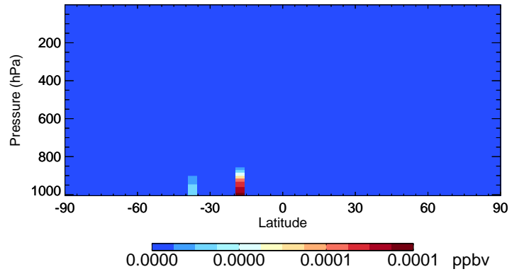
v11-02a LIMO - Species Curtain @ -180.000 for Jan
