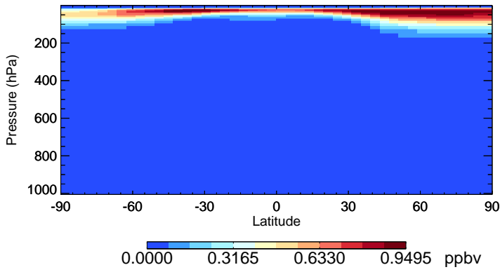
v11-01-public-Run0 CINO3 - Species Zonal Mean for Jan
