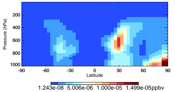
v11-02c SOAMG - Species Curtain @ -180.000 for Jan
