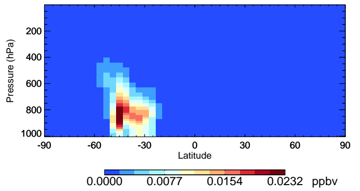
v11-02a DST4 - Species Curtain @ -180.000 for Jan
