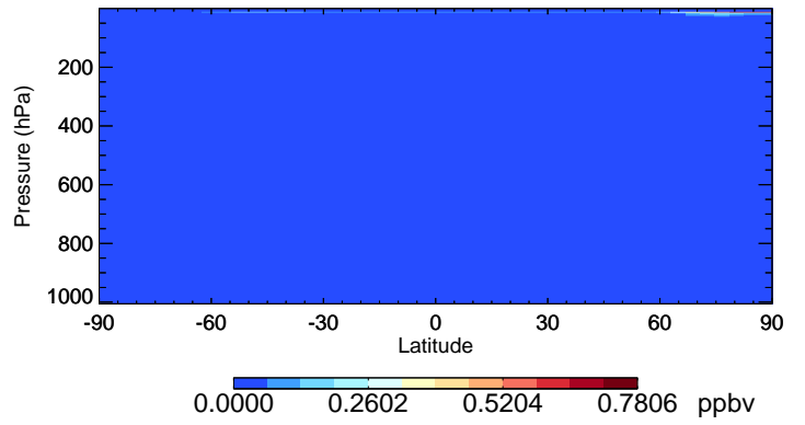
v11-01-public-Run0 NO3 - Species Curtain @ -180.000 for Jan
