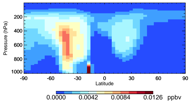
v11-02c TSOG2 - Species Curtain @ -180.000 for Jan
