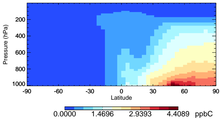
v11-02a C2H6 - Species Zonal Mean for Jan
