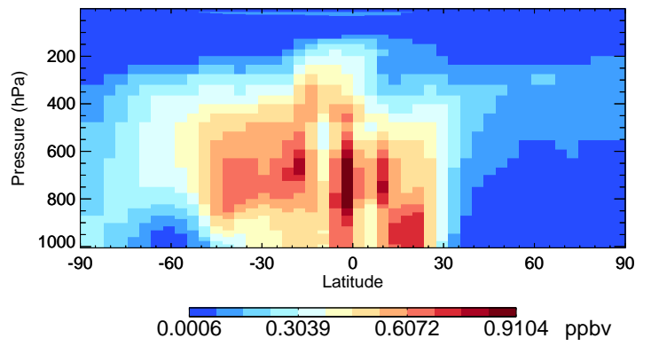
v11-02a H2O2 - Species Curtain @ -180.000 for Jan
