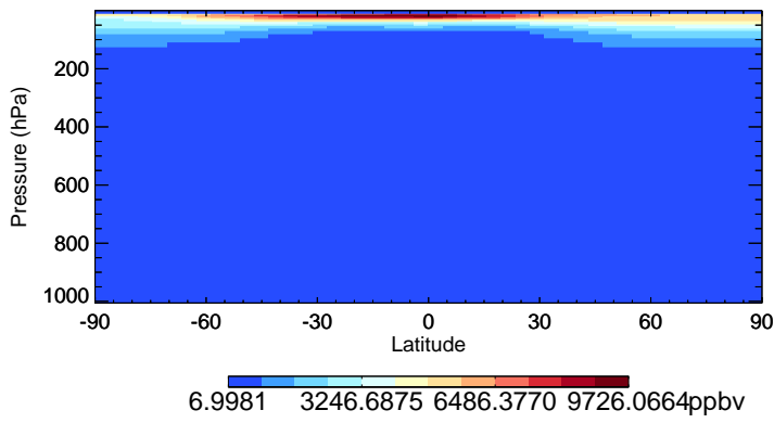
v11-01-public-Run0 O3 - Species Zonal Mean for Jan
