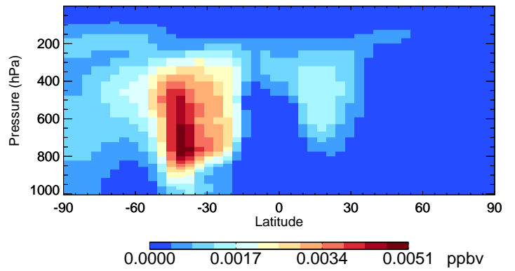
v11-02c ISOG1 - Species Curtain @ -180.000 for Jan
