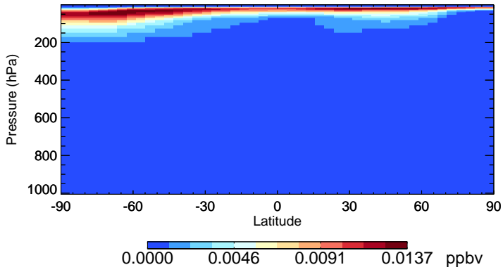
v11-02a BrNO3 - Species Zonal Mean for Jan
