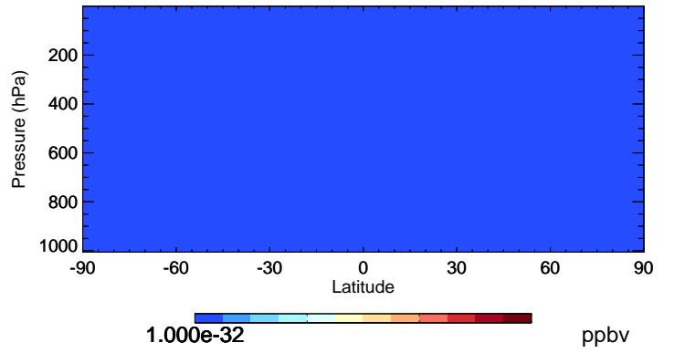
v11-02a GLYX - Species Curtain @ -180.000 for Jan
