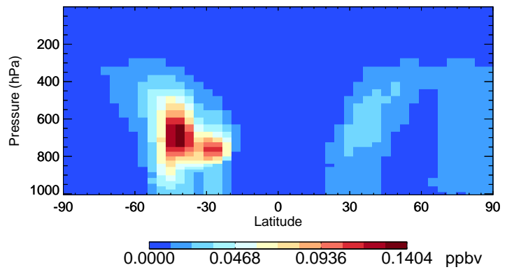
v11-02a DST1 - Species Curtain @ -180.000 for Jan
