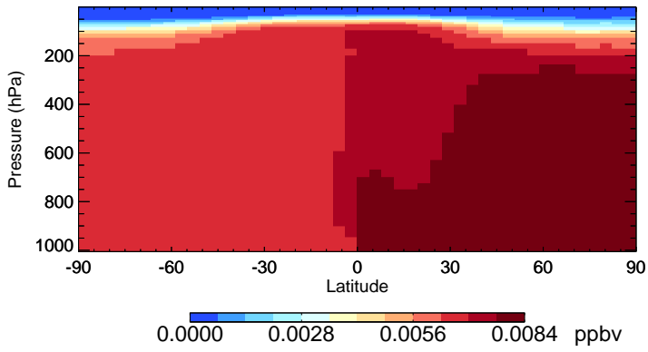
v11-01-public-Run0 CH3Br - Species Zonal Mean for Jan
