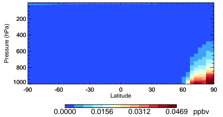
v11-02c HNO2 - Species Curtain @ -180.000 for Jan
