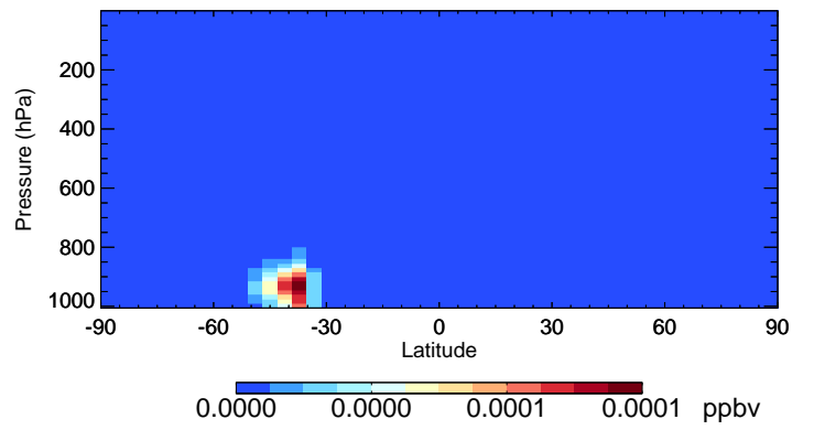
v11-01-public-Run0 MACRN - Species Curtain @ -180.000 for Jan
