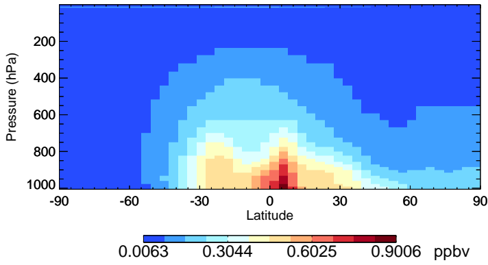
v11-02a CH2O - Species Zonal Mean for Jan
