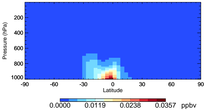
v11-01-public-Run0 TSOA0 - Species Zonal Mean for Jan
