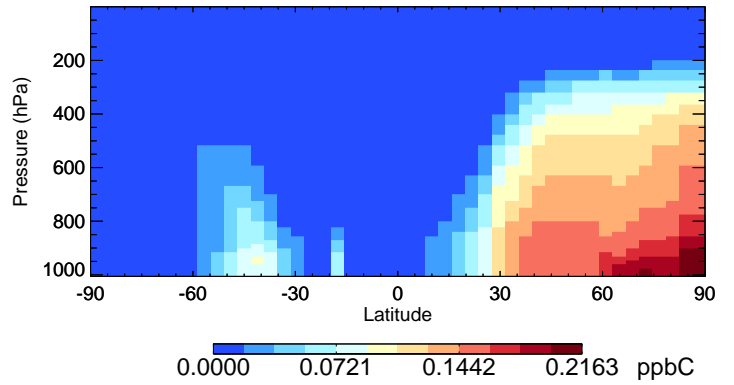
v11-02a MEK - Species Curtain @ -180.000 for Jan
