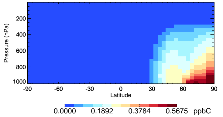
v11-01-public-Run0 TOLU - Species Curtain @ -180.000 for Jan
