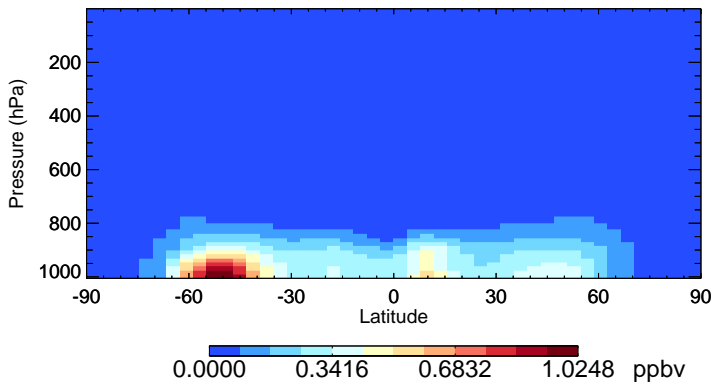
v11-02c SALA - Species Zonal Mean for Jan
