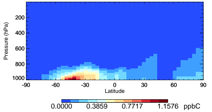
v11-02a ALD2 - Species Curtain @ -180.000 for Jan
