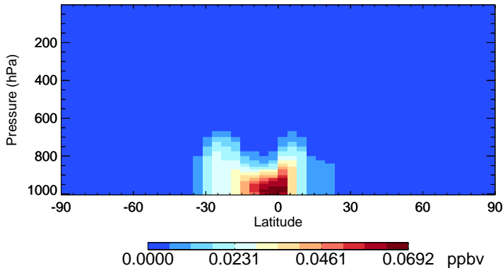
v11-02a MACR - Species Zonal Mean for Jan
