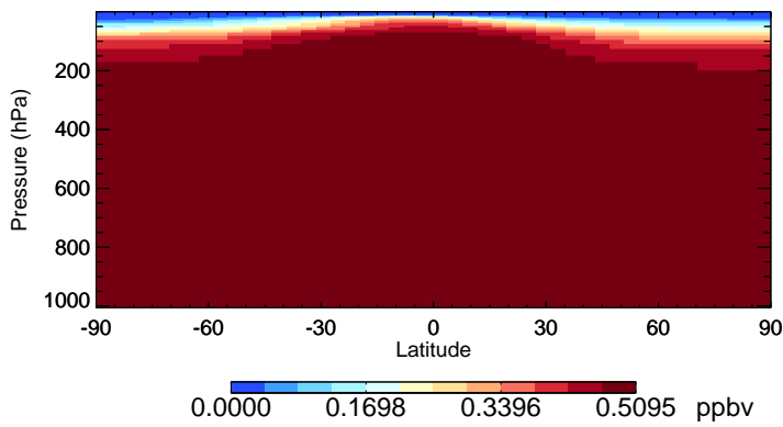
v11-02c CFC12 - Species Zonal Mean for Jan
