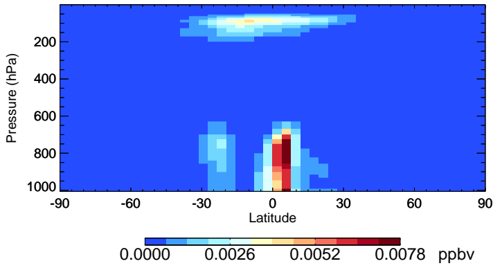
v11-02a ISOA3 - Species Zonal Mean for Jan
