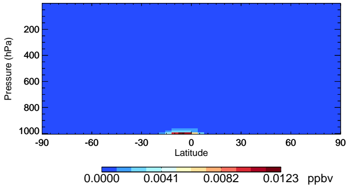
v11-02a MTPO - Species Zonal Mean for Jan
