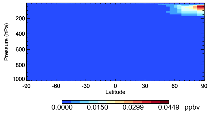
v11-02a OCIO - Species Curtain @ -180.000 for Jan
