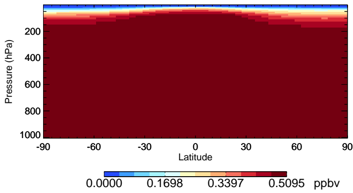
v11-02a CFC12 - Species Zonal Mean for Jan
