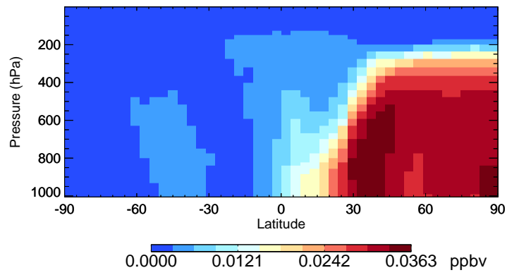
v11-01-public-Run0 R4N2 - Species Curtain @ -180.000 for Jan
