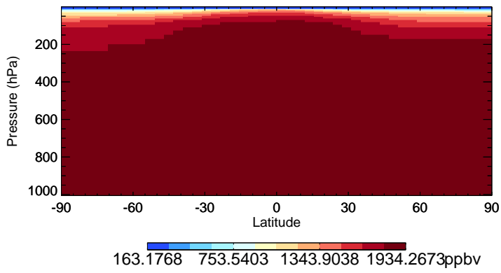
v11-01-public-Run0 CH4 - Species Zonal Mean for Jan
