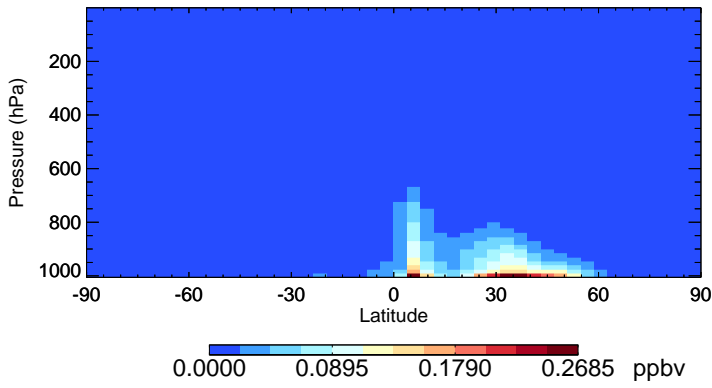
v11-01-public-Run0 BCPO - Species Zonal Mean for Jan
