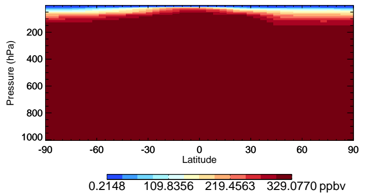
v11-02c N2O - Species Curtain @ -180.000 for Jan
