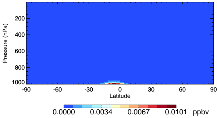
v11-02a LIMO - Species Zonal Mean for Jan
