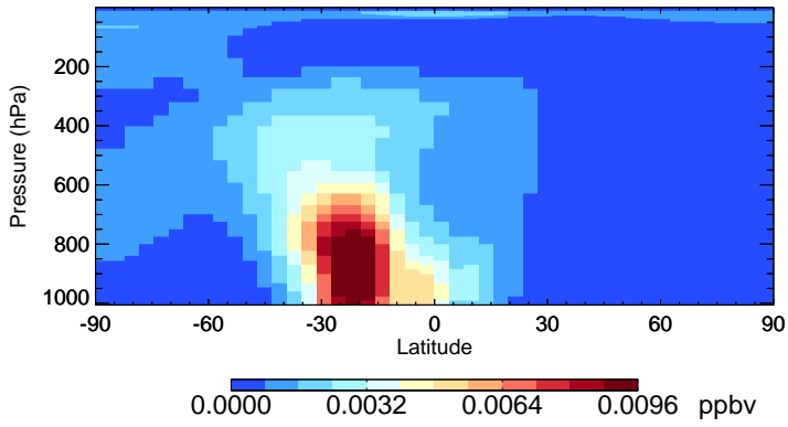
v11-02a ISOG1 - Species Zonal Mean for Jan
