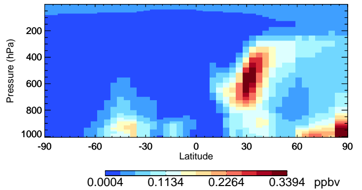
v11-02c NH4 - Species Curtain @ -180.000 for Jan
