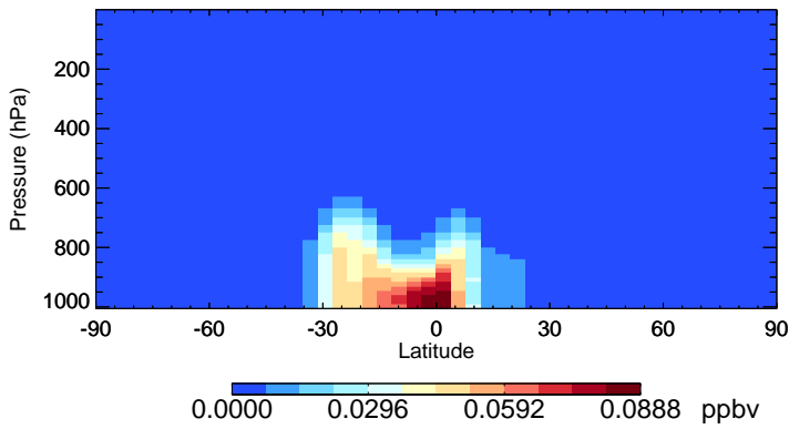
v11-02c MACR - Species Zonal Mean for Jan
