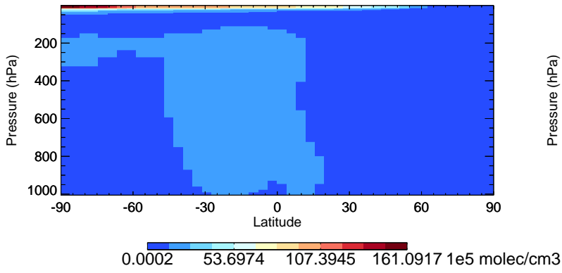
v11-01-public-Run0 OH - Species Zonal Mean for Jan
