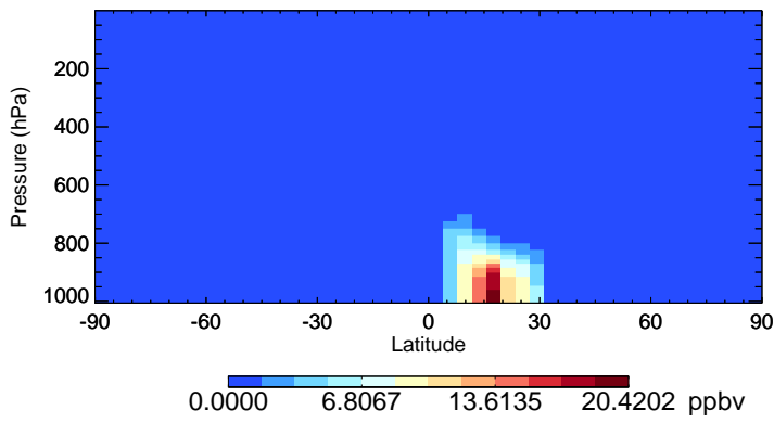
v11-02a DST2 - Species Zonal Mean for Jan
