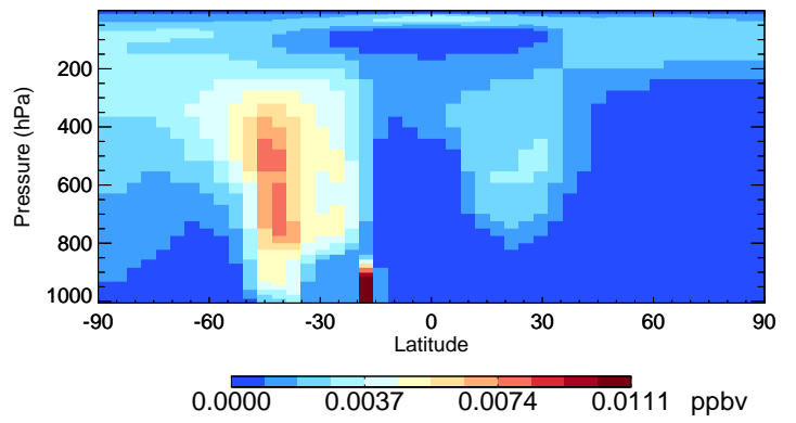
v11-02a TSOG2 - Species Curtain @ -180.000 for Jan
