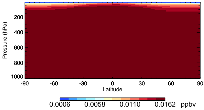
v11-02a CFC114 - Species Zonal Mean for Jan
