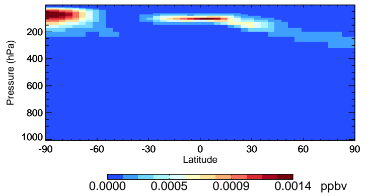
v11-01-public-Run0 ASOA3 - Species Curtain @ -180.000 for Jul
