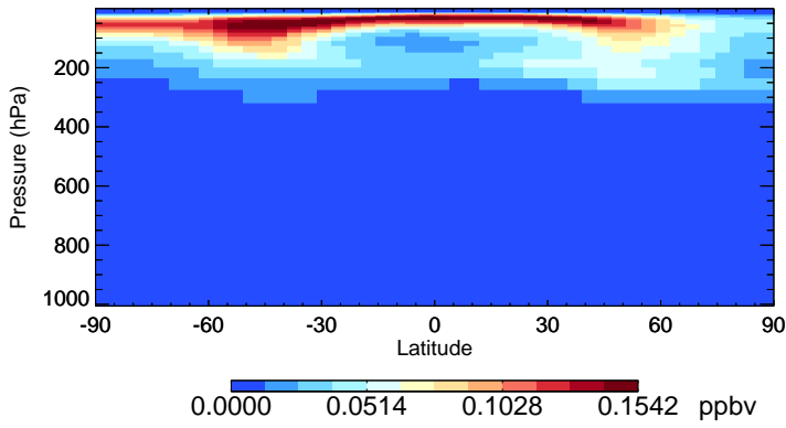
v11-01-public-Run0 MPN - Species Zonal Mean for Jul
