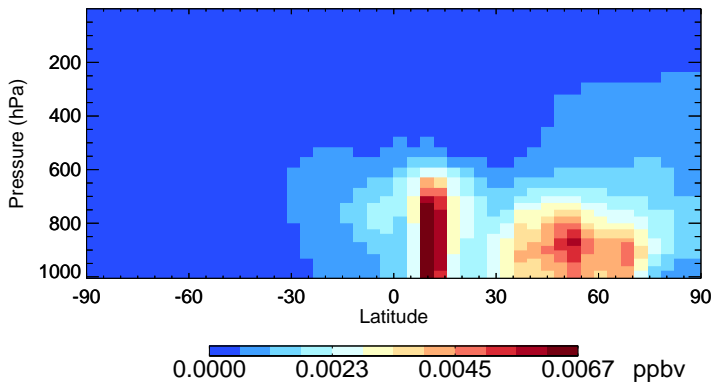
v11-02c SOAME - Species Zonal Mean for Jul
