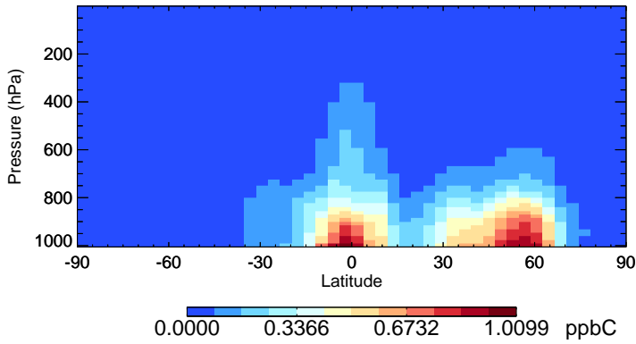
v11-02a MEK - Species Zonal Mean for Jul
