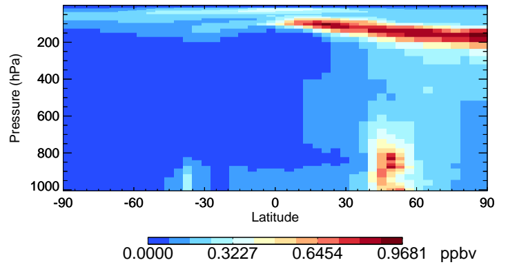
v11-01-public-Run0 SO4 - Species Curtain @ -180.000 for Jul
