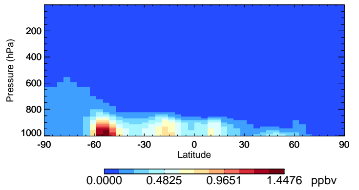
v11-02a SALA - Species Curtain @ -180.000 for Jul
