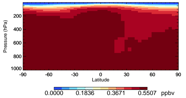
v11-01-public-Run0 CH3Cl - Species Curtain @ -180.000 for Jul
