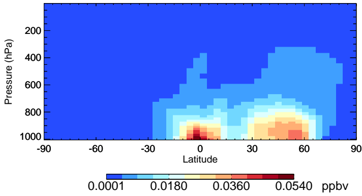
v11-02a TSOG2 - Species Zonal Mean for Jul
