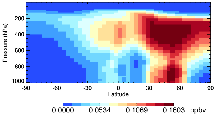
v11-01-public-Run0 PAN - Species Zonal Mean for Jul
