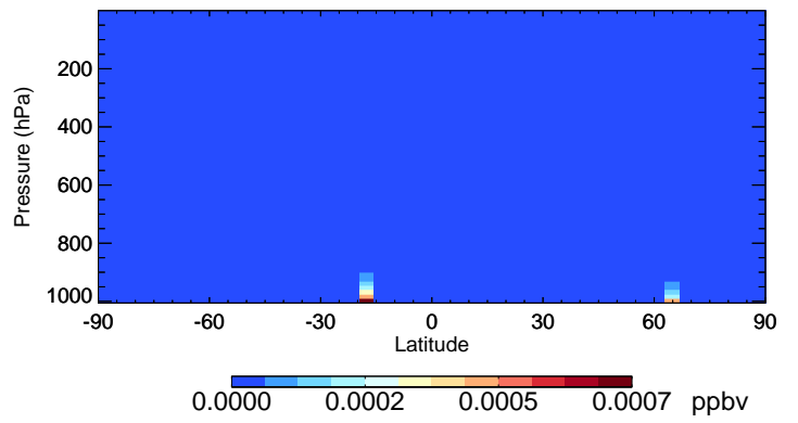
v11-01-public-Run0 MTPO - Species Curtain @ -180.000 for Jul
