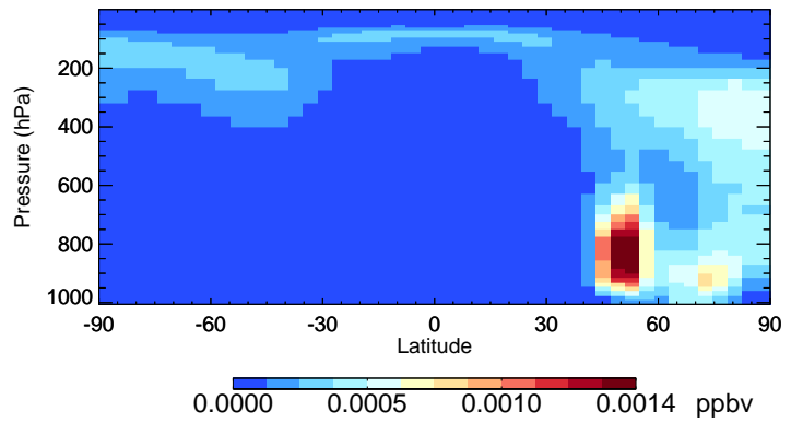
v11-02c TSOA1 - Species Curtain @ -180.000 for Jul
