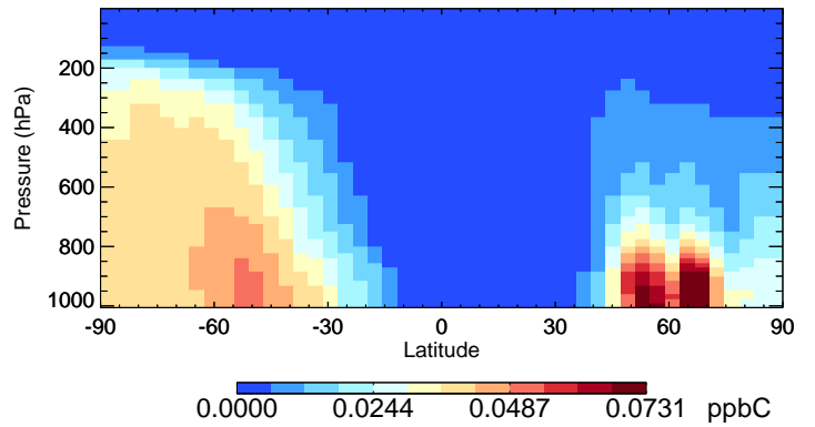
v11-01-public-Run0 MEK - Species Curtain @ -180.000 for Jul
