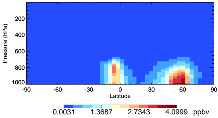
v11-01-public-Run0 OCPI - Species Zonal Mean for Jul
