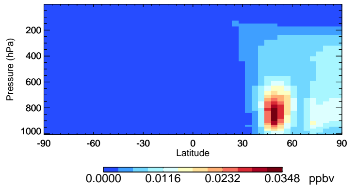
v11-02c INDIOL - Species Curtain @ -180.000 for Jul
