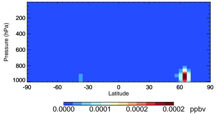
v11-02a MACRN - Species Curtain @ -180.000 for Jul
