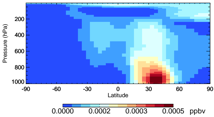
v11-01-public-Run0 ASOG1 - Species Zonal Mean for Jul
