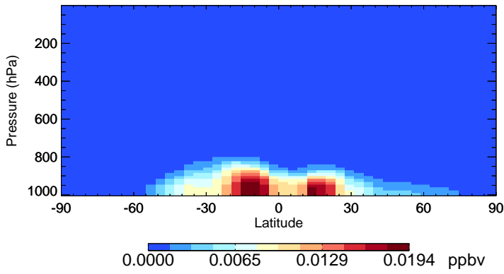
v11-01-public-Run0 NITs - Species Zonal Mean for Jul
