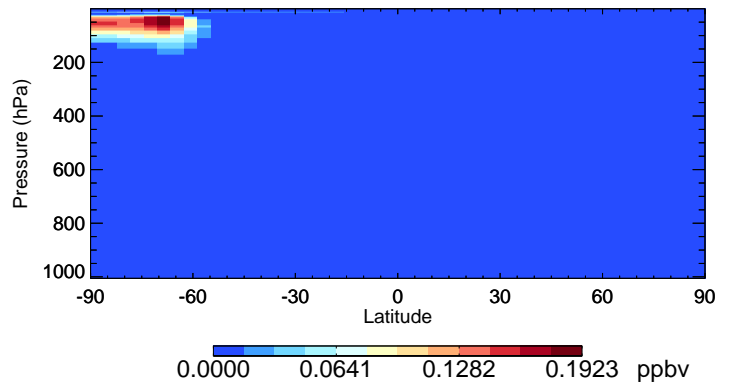
v11-02c OCIO - Species Curtain @ -180.000 for Jul
