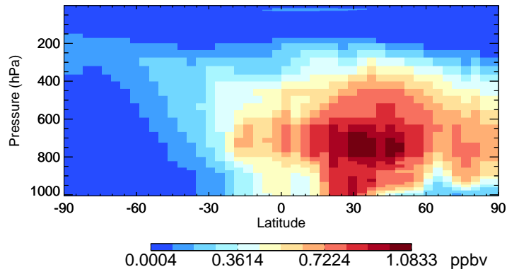
v11-01-public-Run0 H2O2 - Species Curtain @ -180.000 for Jul
