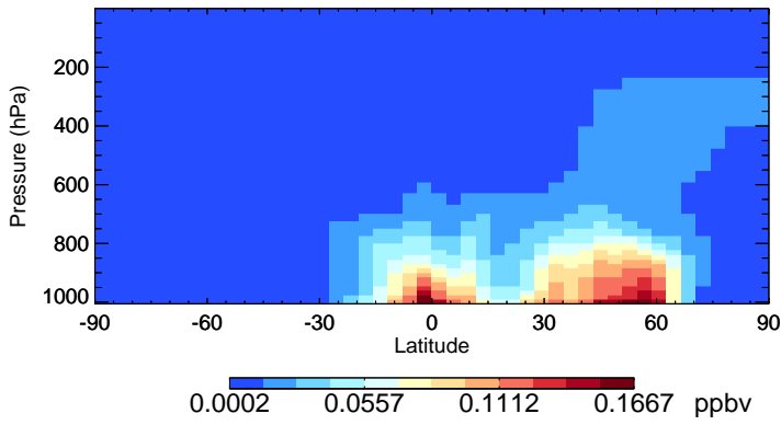
v11-01-public-Run0 TSOG3 - Species Zonal Mean for Jul
