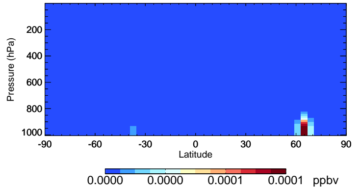
v11-02a MOBA - Species Curtain @ -180.000 for Jul
