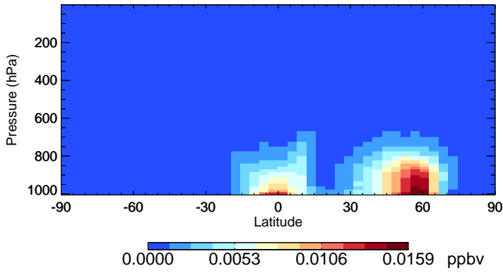
v11-02a TSOA1 - Species Zonal Mean for Jul
