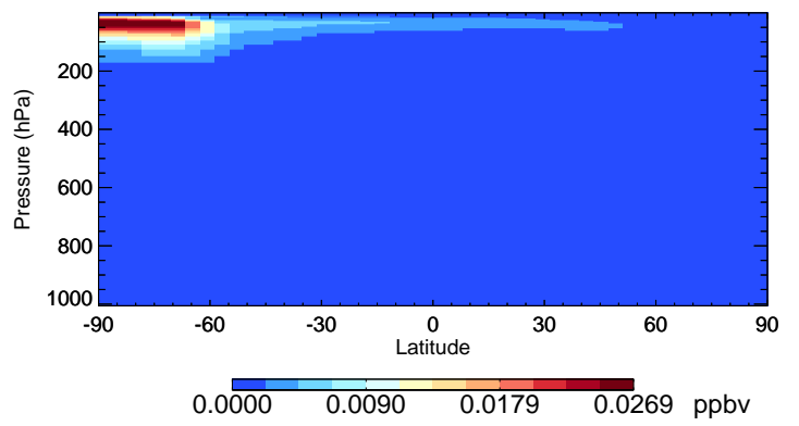
v11-02a BrCl - Species Curtain @ -180.000 for Jul
