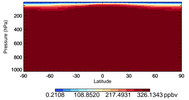
v11-01-public-Run0 N2O - Species Curtain @ -180.000 for Jul
