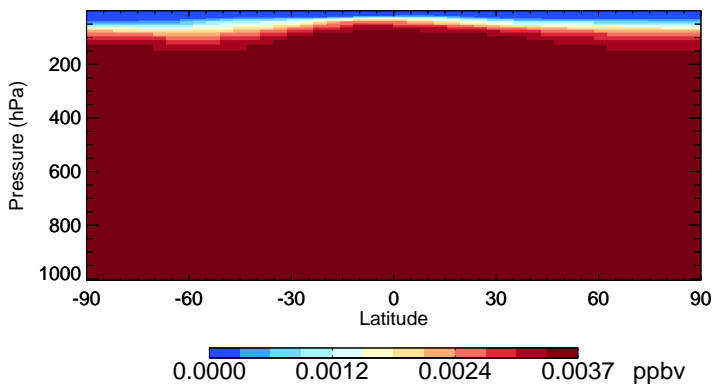
v11-02c H1301 - Species Zonal Mean for Jul
