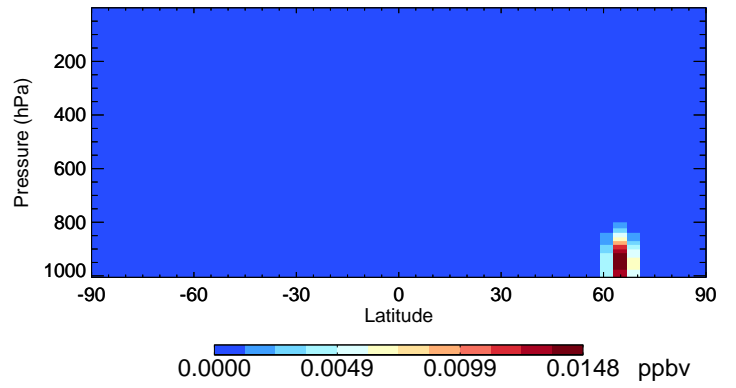
v11-01-public-Run0 MACR - Species Curtain @ -180.000 for Jul
