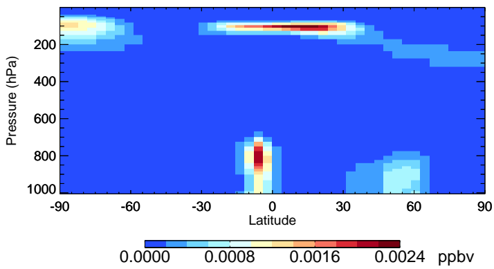
v11-02c ASOA3 - Species Zonal Mean for Jul
