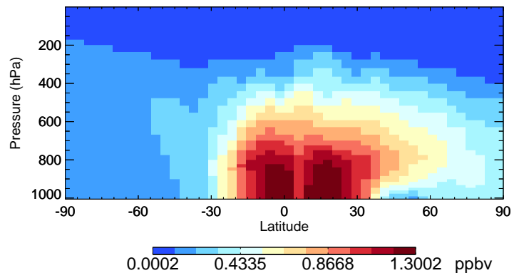
v11-01-public-Run0 MP - Species Curtain @ -180.000 for Jul
