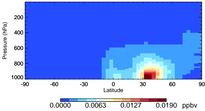
v11-02a ASOAN - Species Zonal Mean for Jul
