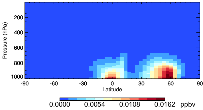
v11-01-public-Run0 TSOA1 - Species Zonal Mean for Jul
