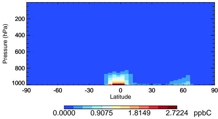
v11-01-public-Run0 ISOP - Species Zonal Mean for Jul
