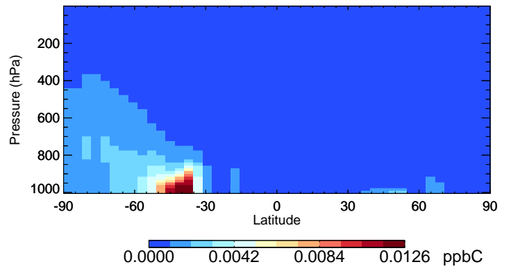
v11-02c XYLE - Species Curtain @ -180.000 for Jul
