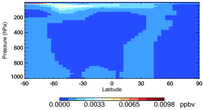
v11-01-public-Run0 HOBr - Species Zonal Mean for Jul
