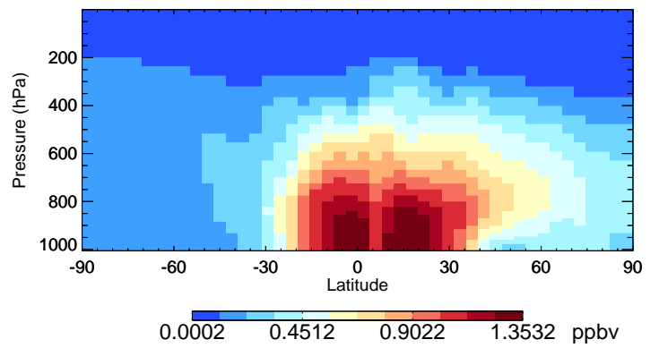
v11-02c MP - Species Curtain @ -180.000 for Jul
