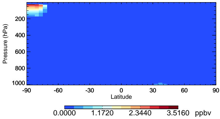
v11-01-public-Run0 NIT - Species Zonal Mean for Jul
