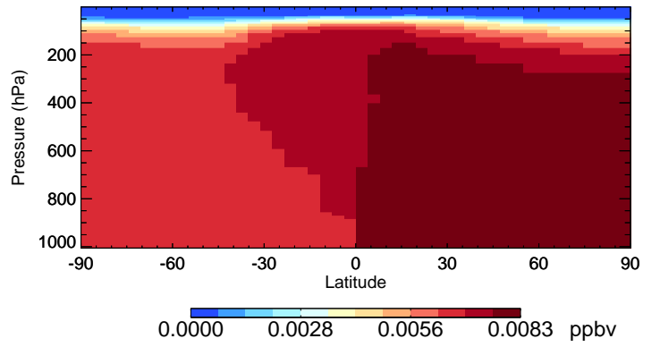
v11-01-public-Run0 CH3Br - Species Curtain @ -180.000 for Jul
