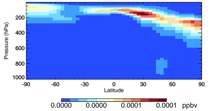
v11-01-public-Run0 ASOA2 - Species Curtain @ -180.000 for Jul
