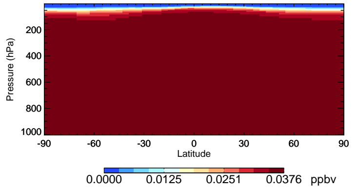
v11-01-public-Run0 HCFC141b - Species Curtain @ -180.000 for Jul
