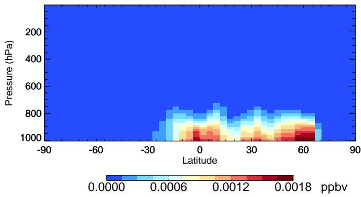
v11-01-public-Run0 ISOPNB - Species Zonal Mean for Jul
