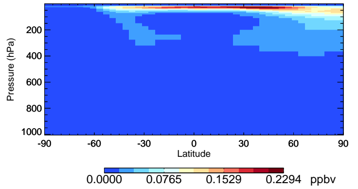
v11-01-public-Run0 HNO4 - Species Curtain @ -180.000 for Jul
