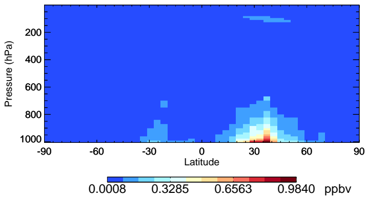
v11-01-public-Run0 SO2 - Species Zonal Mean for Jul
