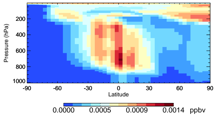
v11-01-public-Run0 HBr - Species Curtain @ -180.000 for Jul
