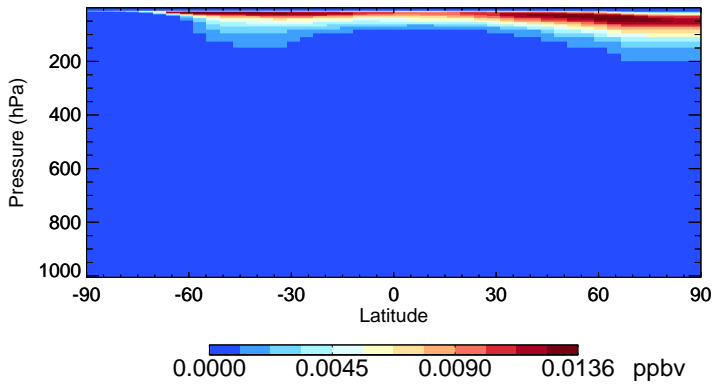
v11-01-public-Run0 BrNO3 - Species Zonal Mean for Jul
