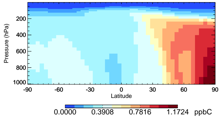
v11-01-public-Run0 C2H6 - Species Curtain @ -180.000 for Jul
