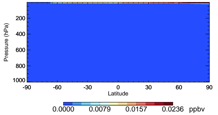
v11-01-public-Run0 Br - Species Curtain @ -180.000 for Jul
