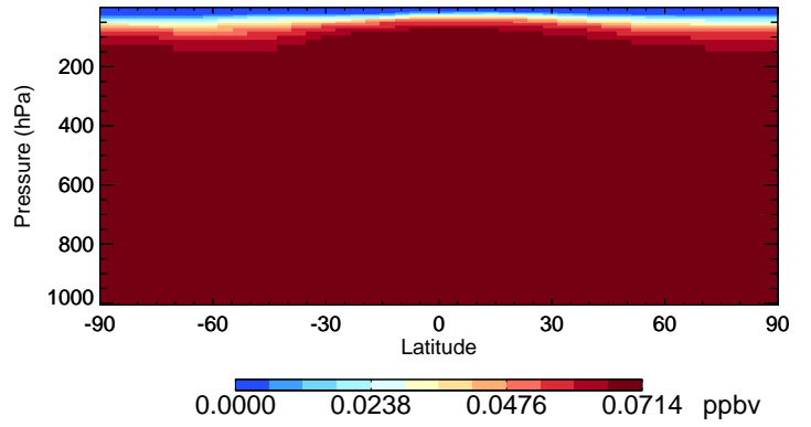
v11-02a CFC113 - Species Curtain @ -180.000 for Jul
