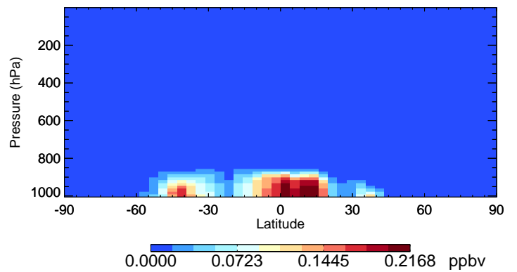
v11-02c NH3 - Species Curtain @ -180.000 for Jul
