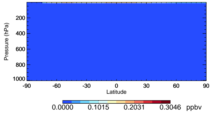
v11-01-public-Run0 CI - Species Curtain @ -180.000 for Jul
