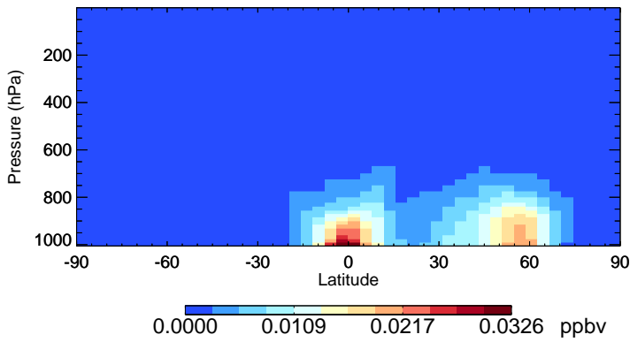
v11-02c TSOA0 - Species Zonal Mean for Jul
