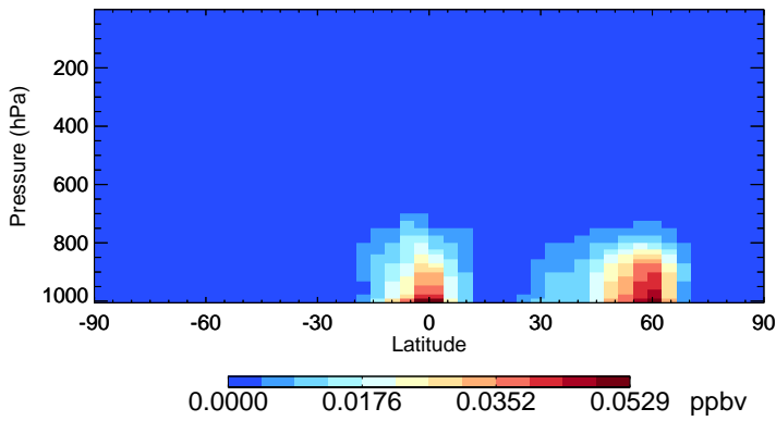
v11-02c TSOA2 - Species Zonal Mean for Jul
