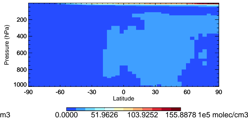
v11-01-public-Run0 OH - Species Curtain @ -180.000 for Jul
