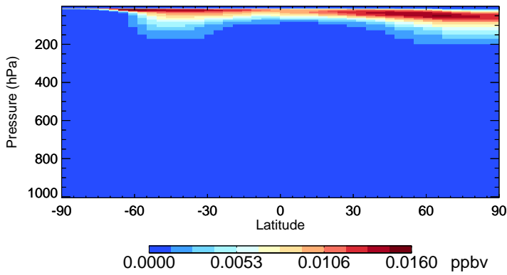
v11-02c BrNO3 - Species Zonal Mean for Jul
