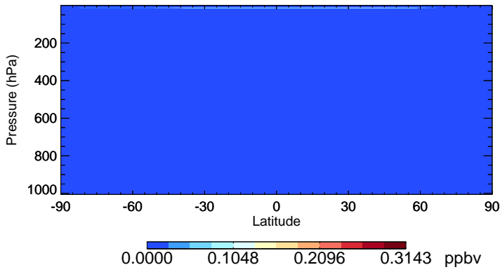
v11-01-public-Run0 NO3 - Species Zonal Mean for Jul
