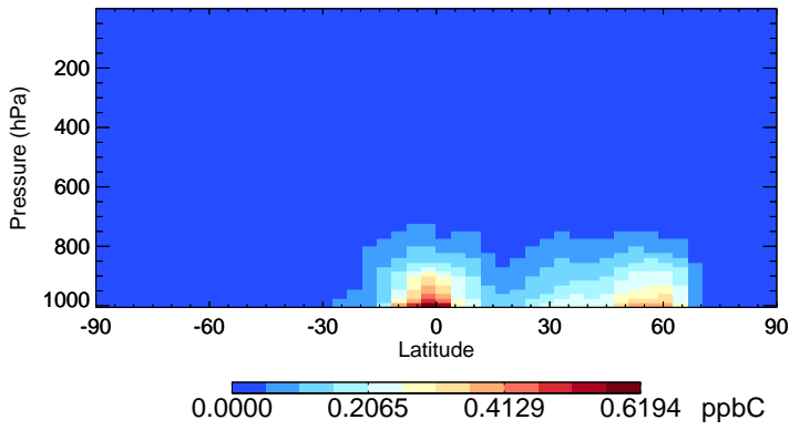
v11-01-public-Run0 ALD2 - Species Zonal Mean for Jul
