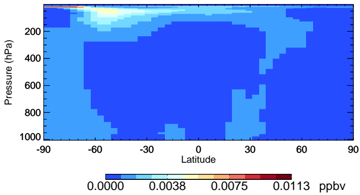
v11-02c HOBr - Species Zonal Mean for Jul
