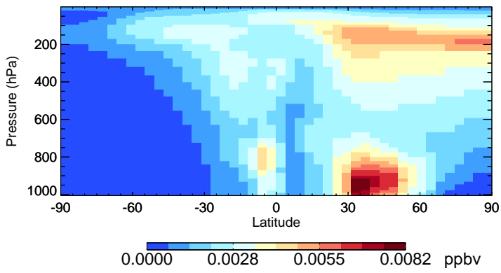
v11-02a ASOG3 - Species Zonal Mean for Jul
