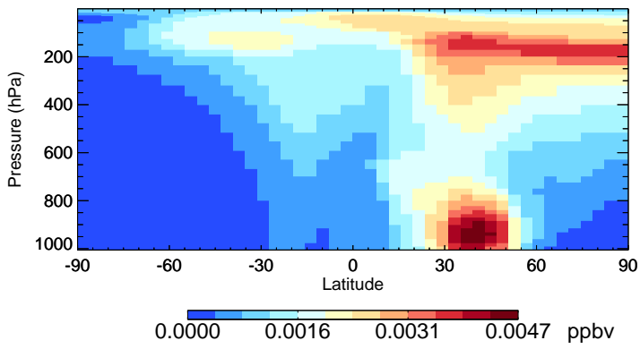
v11-01-public-Run0 ASOG3 - Species Zonal Mean for Jul
