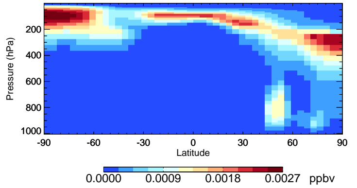
v11-02a TSOA2 - Species Curtain @ -180.000 for Jul
