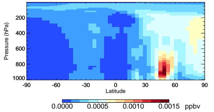
v11-01-public-Run0 ASOAN - Species Curtain @ -180.000 for Jul
