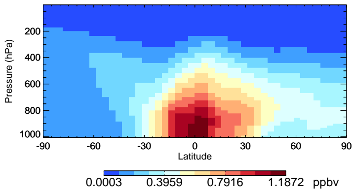
v11-01-public-Run0 MP - Species Zonal Mean for Jul
