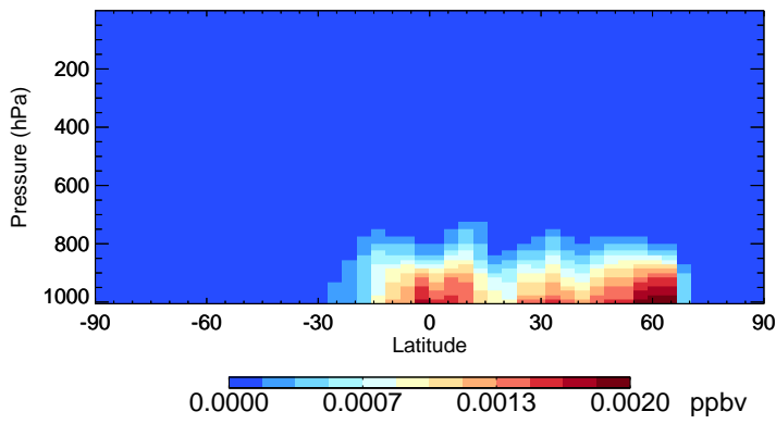
v11-02a ISOPNB - Species Zonal Mean for Jul
