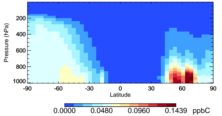
v11-02a MEK - Species Curtain @ -180.000 for Jul
