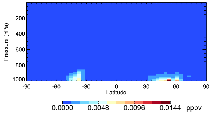
v11-02c BCPO - Species Curtain @ -180.000 for Jul
