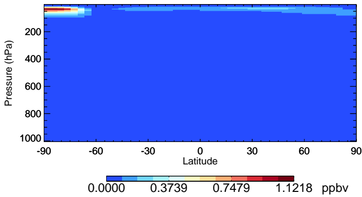
v11-02c HNO4 - Species Zonal Mean for Jul
