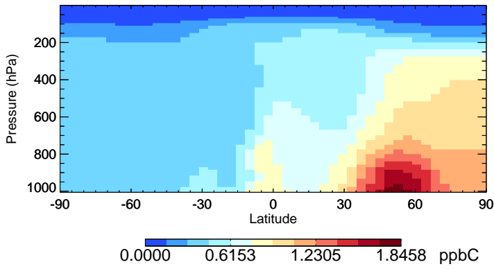
v11-01-public-Run0 C2H6 - Species Zonal Mean for Jul
