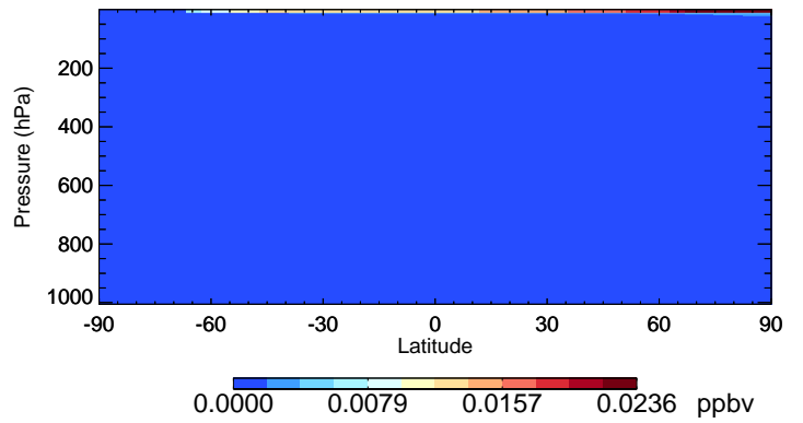
v11-02c Br - Species Curtain @ -180.000 for Jul
