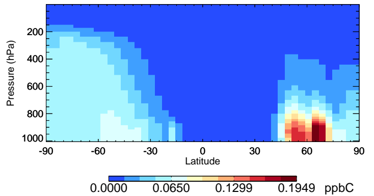
v11-02c MEK - Species Curtain @ -180.000 for Jul
