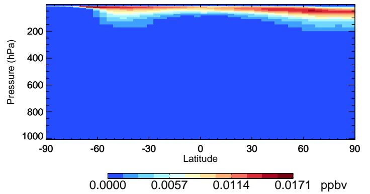
v11-02c BrNO3 - Species Curtain @ -180.000 for Jul
