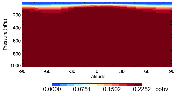
v11-01-public-Run0 CFC11 - Species Curtain @ -180.000 for Jul
