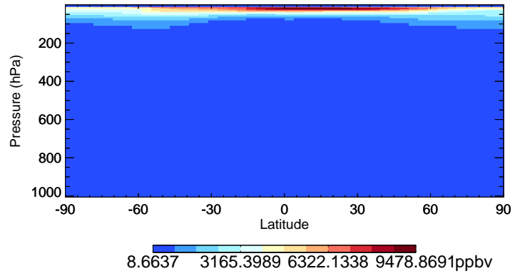
v11-02a O3 - Species Curtain @ -180.000 for Jul
