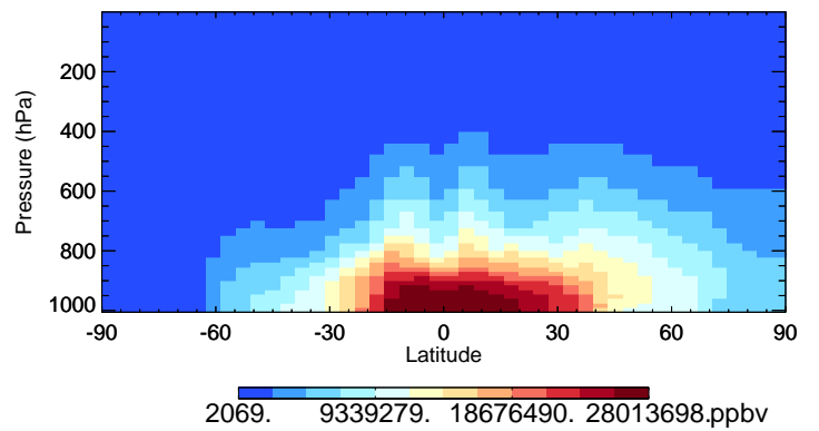
v11-02c H2O - Species Curtain @ -180.000 for Jul
