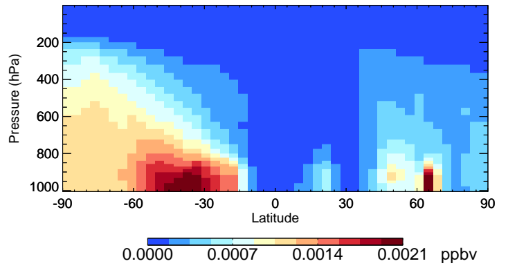
v11-01-public-Run0 RCHO - Species Curtain @ -180.000 for Jul
