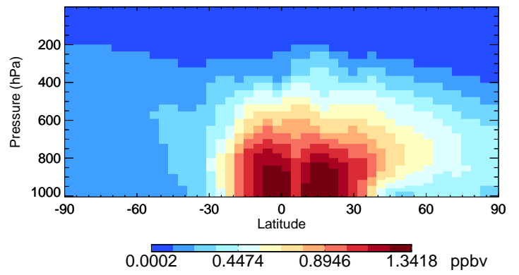
v11-02a MP - Species Curtain @ -180.000 for Jul
