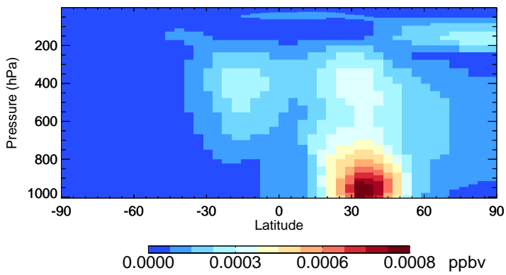
v11-02c ASOG1 - Species Zonal Mean for Jul
