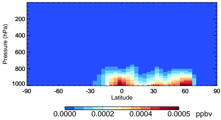
v11-01-public-Run0 MOBA - Species Zonal Mean for Jul
