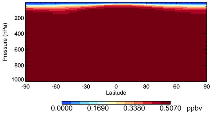
v11-01-public-Run0 CFC12 - Species Zonal Mean for Jul
