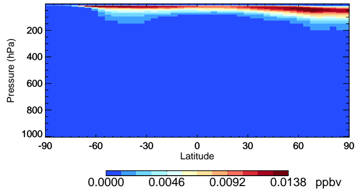
v11-01-public-Run0 BrNO3 - Species Curtain @ -180.000 for Jul
