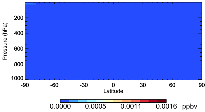
v11-01-public-Run0 ClNO2 - Species Zonal Mean for Jul
