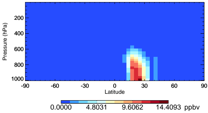
v11-01-public-Run0 DST4 - Species Zonal Mean for Jul
