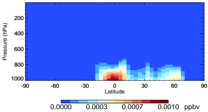
v11-02c MOBA - Species Zonal Mean for Jul
