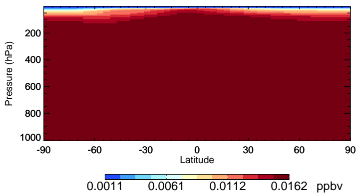
v11-02c CFC114 - Species Zonal Mean for Jul
