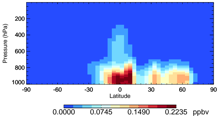
v11-01-public-Run0 HAC - Species Zonal Mean for Jul
