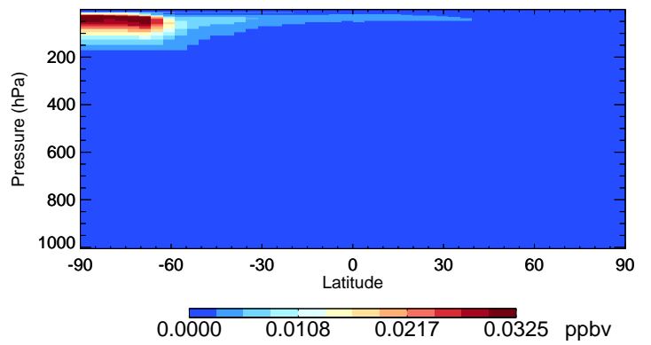
v11-02c BrCl - Species Curtain @ -180.000 for Jul
