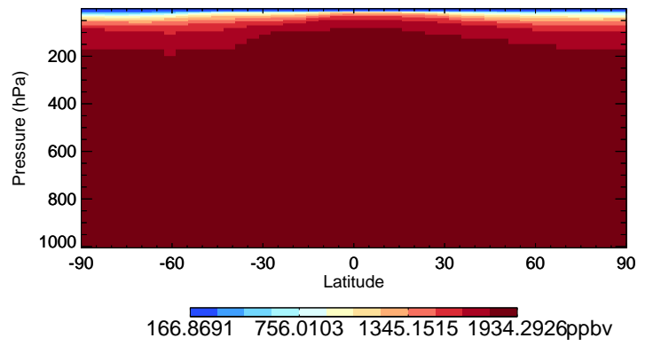
v11-01-public-Run0 CH4 - Species Curtain @ -180.000 for Jul
