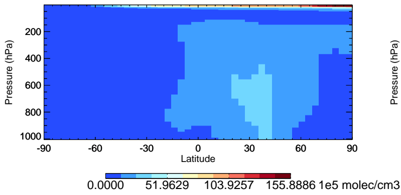
v11-01-public-Run0 OH - Species Zonal Mean for Jul
