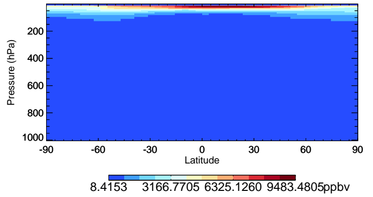
v11-01-public-Run0 O3 - Species Curtain @ -180.000 for Jul
