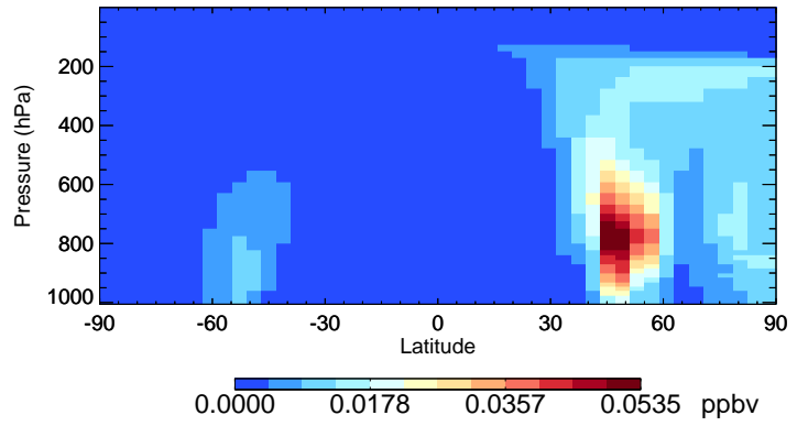
v11-02a DST1 - Species Curtain @ -180.000 for Jul
