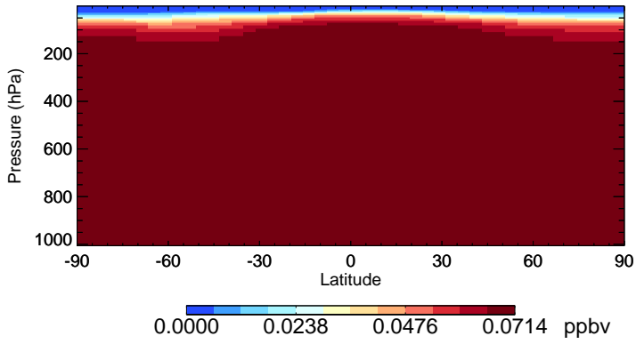
v11-02a CFC113 - Species Zonal Mean for Jul
