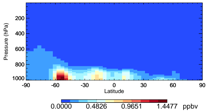
v11-01-public-Run0 SALA - Species Curtain @ -180.000 for Jul
