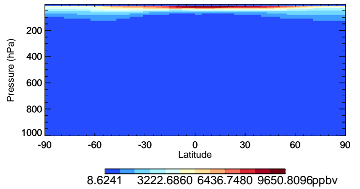
v11-02c O3 - Species Curtain @ -180.000 for Jul
