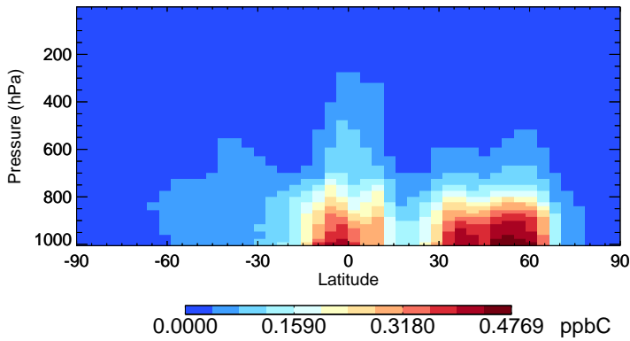
v11-01-public-Run0 MEK - Species Zonal Mean for Jul
