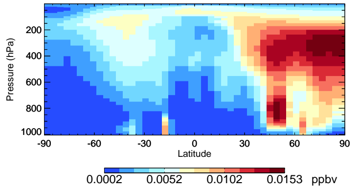
v11-01-public-Run0 TSOG3 - Species Curtain @ -180.000 for Jul
