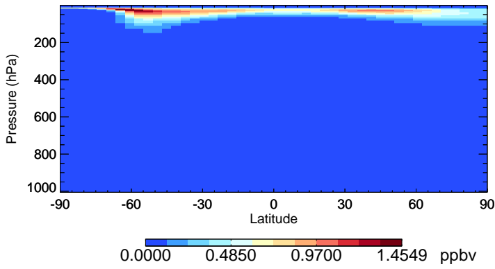
v11-01-public-Run0 ClNO3 - Species Zonal Mean for Jul
