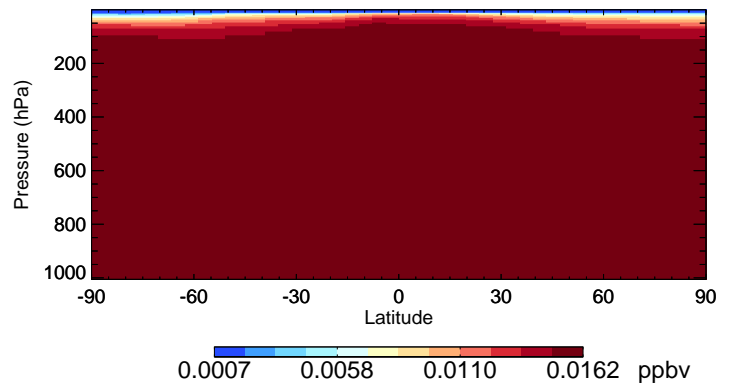
v11-01-public-Run0 CFC114 - Species Curtain @ -180.000 for Jul
