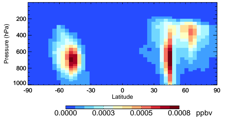
v11-01-public-Run0 DST4 - Species Curtain @ -180.000 for Jul
