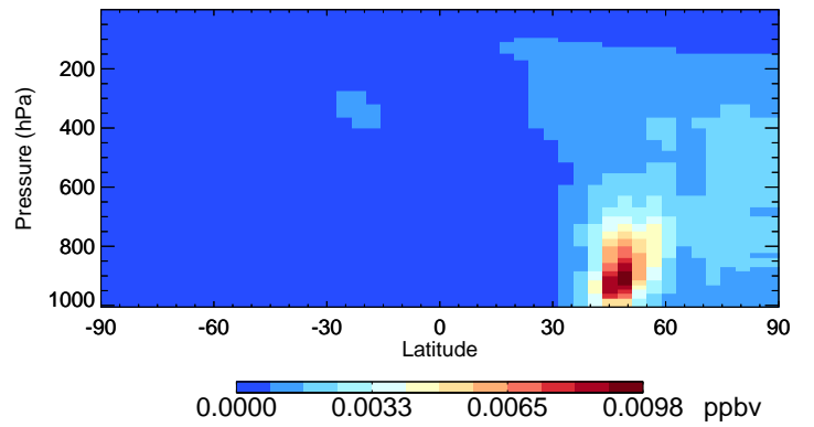
v11-02c ASOAN - Species Curtain @ -180.000 for Jul
