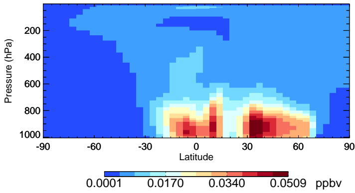
v11-01-public-Run0 ISO3 - Species Zonal Mean for Jul
