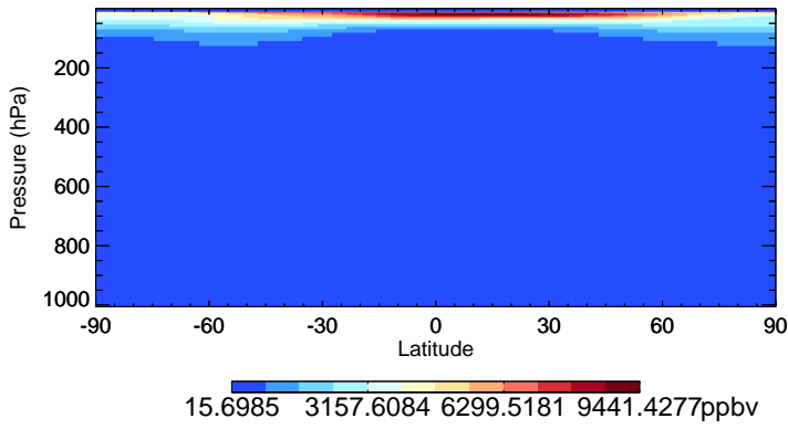
v11-01-public-Run0 O3 - Species Zonal Mean for Jul
