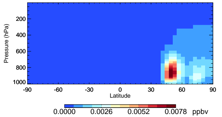
v11-02c SOAME - Species Curtain @ -180.000 for Jul
