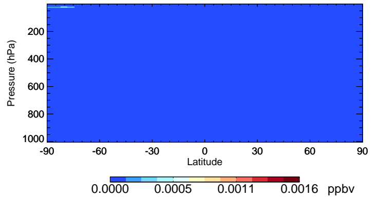
v11-01-public-Run0 ClNO2 - Species Curtain @ -180.000 for Jul
