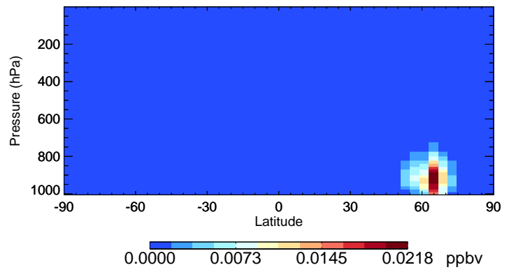
v11-02a GLYC - Species Curtain @ -180.000 for Jul
