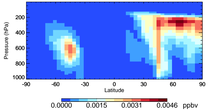
v11-02a DST2 - Species Curtain @ -180.000 for Jul
