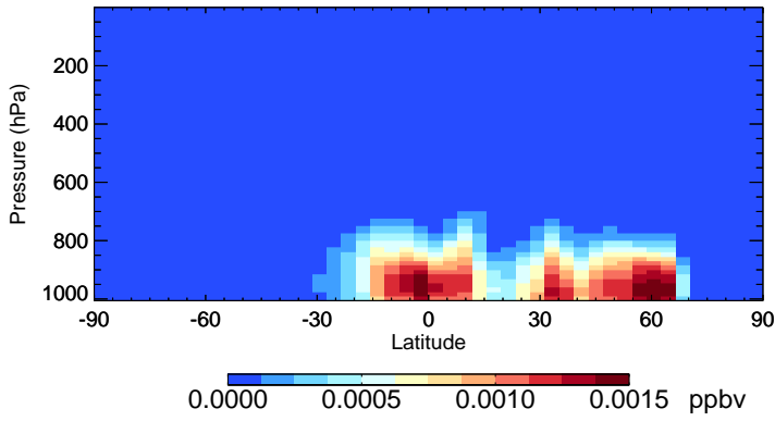
v11-02a MACRN - Species Zonal Mean for Jul
