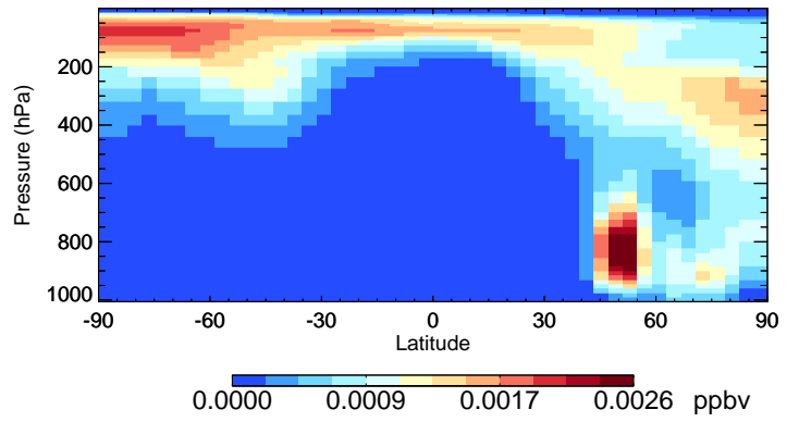
v11-01-public-Run0 ISOA1 - Species Curtain @ -180.000 for Jul
