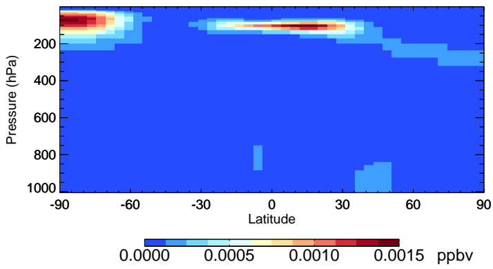
v11-01-public-Run0 ASOA3 - Species Zonal Mean for Jul
