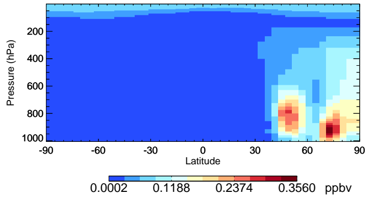
v11-01-public-Run0 OCPI - Species Curtain @ -180.000 for Jul
