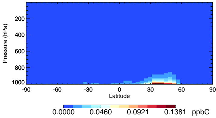
v11-01-public-Run0 XYLE - Species Zonal Mean for Jul
