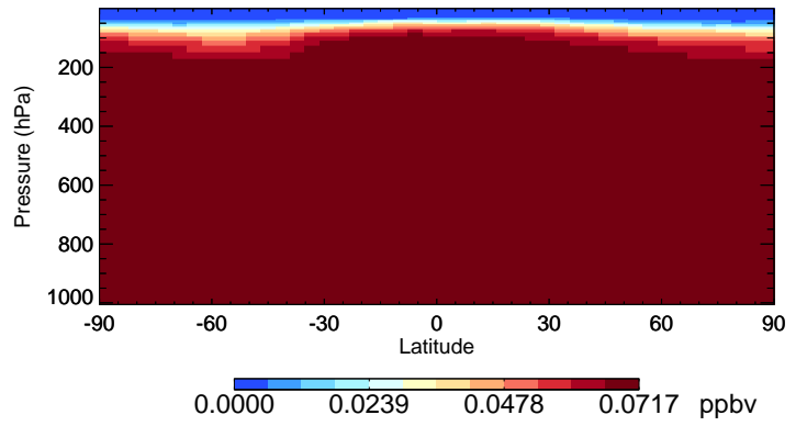
v11-01-public-Run0 CCI4 - Species Curtain @ -180.000 for Jul
