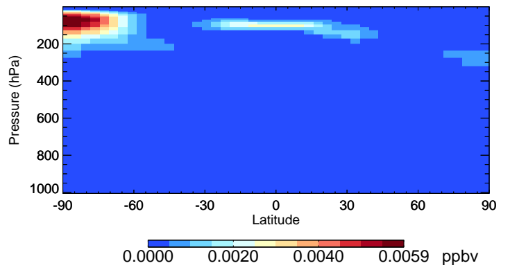
v11-01-public-Run0 ISOA3 - Species Curtain @ -180.000 for Jul
