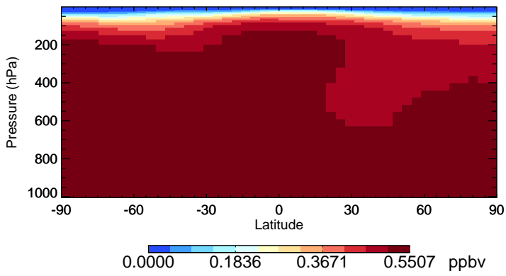
v11-01-public-Run0 CH3Cl - Species Zonal Mean for Jul
