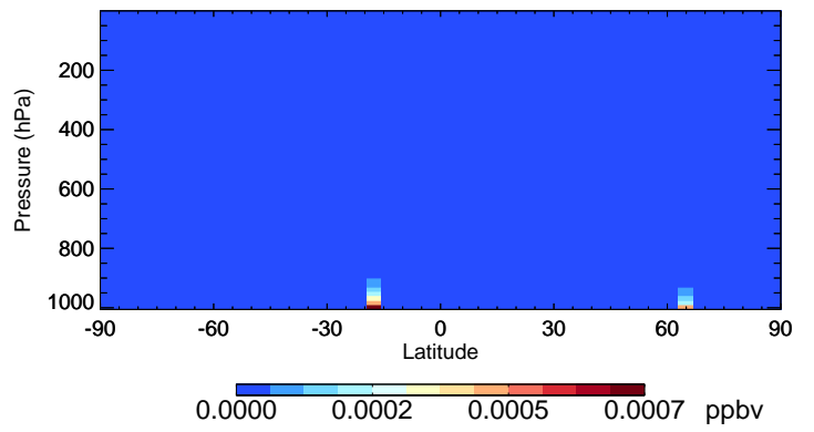
v11-02a MTPO - Species Curtain @ -180.000 for Jul
