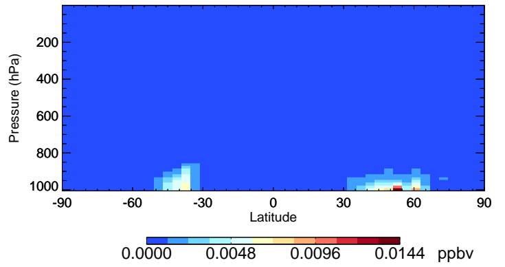
v11-01-public-Run0 BCPO - Species Curtain @ -180.000 for Jul
