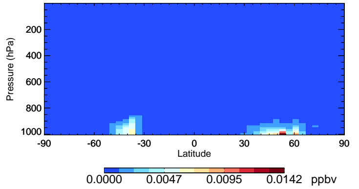
v11-02a BCPO - Species Curtain @ -180.000 for Jul
