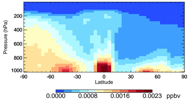
v11-01-public-Run0 CHBr3 - Species Curtain @ -180.000 for Jul
