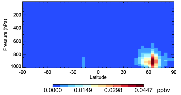
v11-02a HAC - Species Curtain @ -180.000 for Jul
