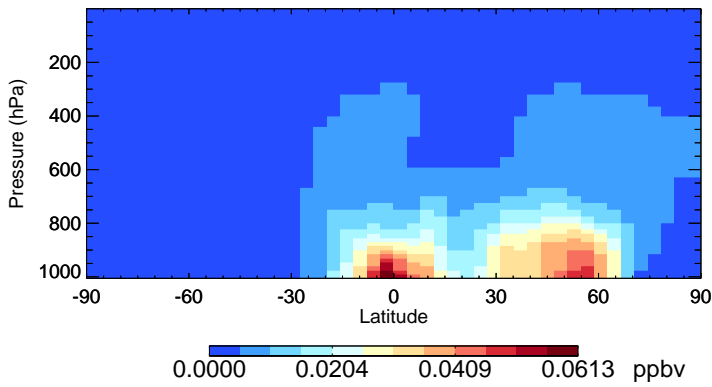
v11-02c TSOG2 - Species Zonal Mean for Jul
