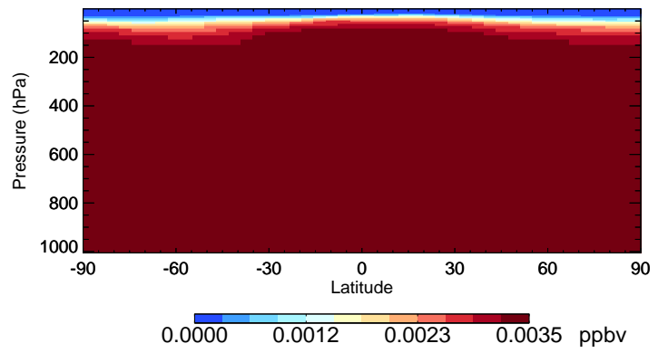
v11-01-public-Run0 H1301 - Species Curtain @ -180.000 for Jul
