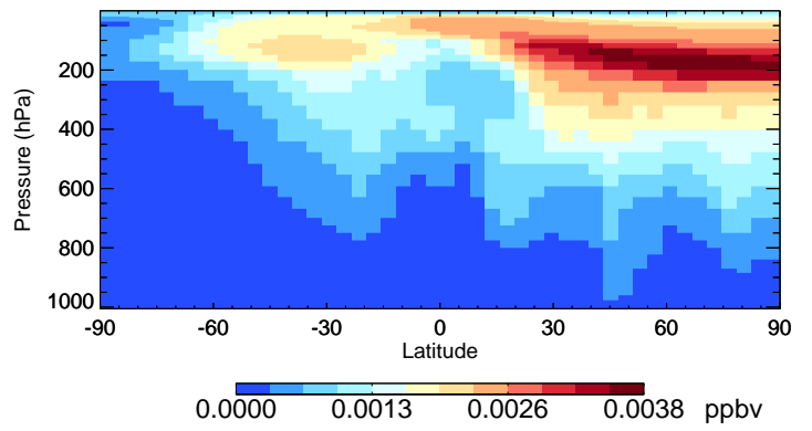
v11-01-public-Run0 ASOG3 - Species Curtain @ -180.000 for Jul
