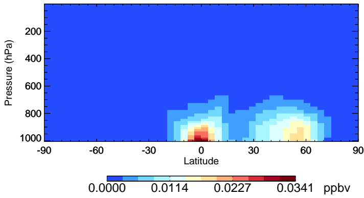
v11-01-public-Run0 TSOA0 - Species Zonal Mean for Jul
