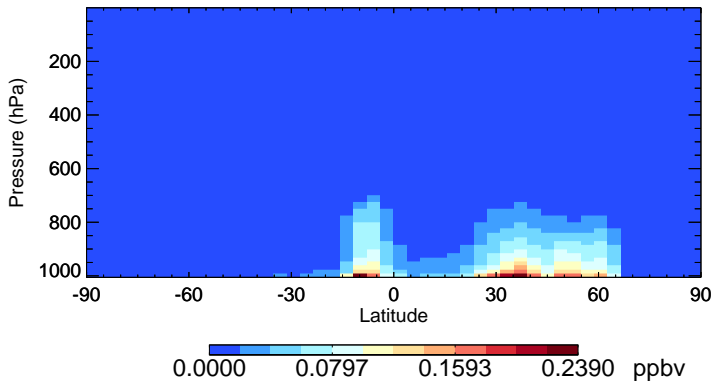
v11-01-public-Run0 BCPO - Species Zonal Mean for Jul
