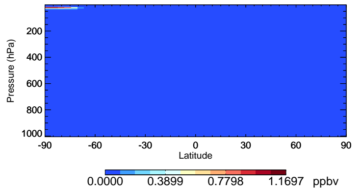
v11-01-public-Run0 Cl2 - Species Curtain @ -180.000 for Jul
