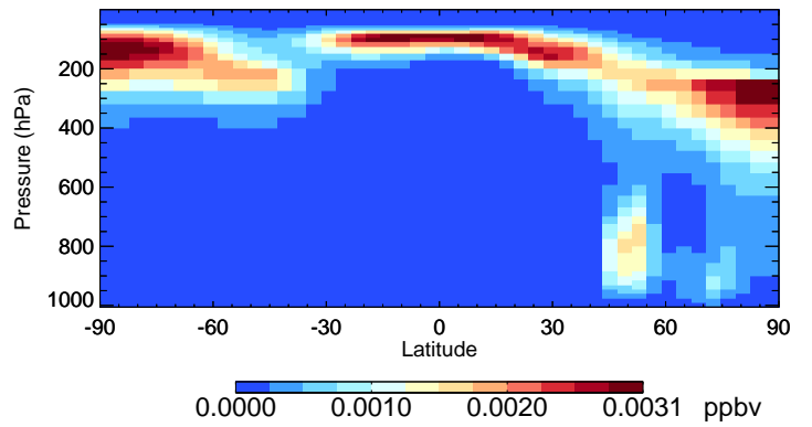
v11-02c TSOA2 - Species Curtain @ -180.000 for Jul
