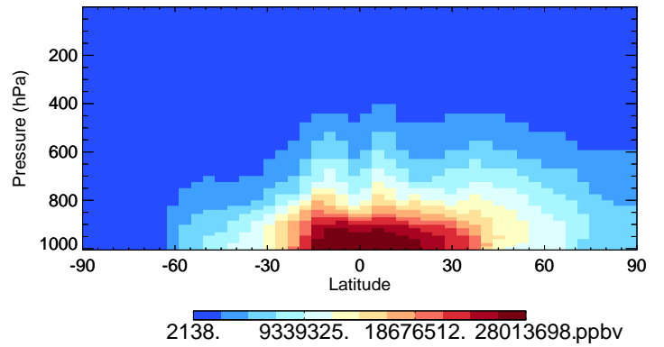
v11-01-public-Run0 H2O - Species Curtain @ -180.000 for Jul
