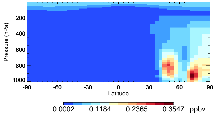
v11-02a OCPI - Species Curtain @ -180.000 for Jul
