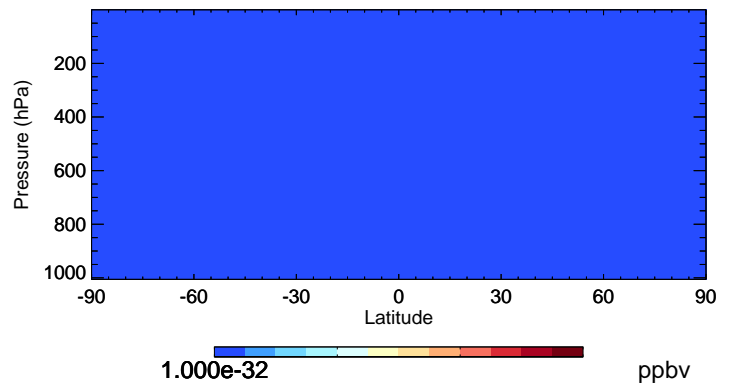
v11-01-public-Run0 MONITA - Species Curtain @ -180.000 for Jul
