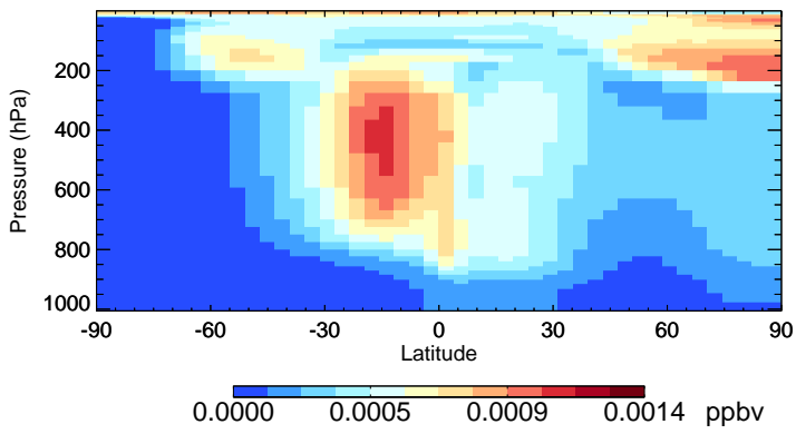
v11-01-public-Run0 HBr - Species Zonal Mean for Jul
