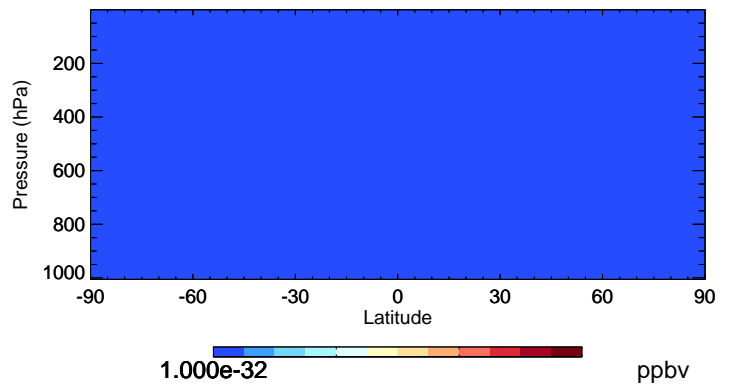
v11-01-public-Run0 DHDN - Species Curtain @ -180.000 for Jul
