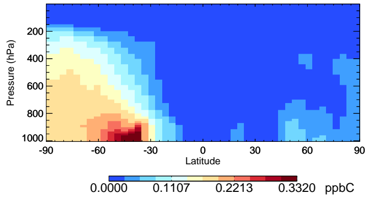
v11-01-public-Run0 ALK4 - Species Curtain @ -180.000 for Jul
