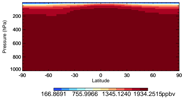
v11-01-public-Run0 CH4 - Species Zonal Mean for Jul
