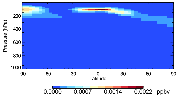
v11-02c ASOA3 - Species Curtain @ -180.000 for Jul
