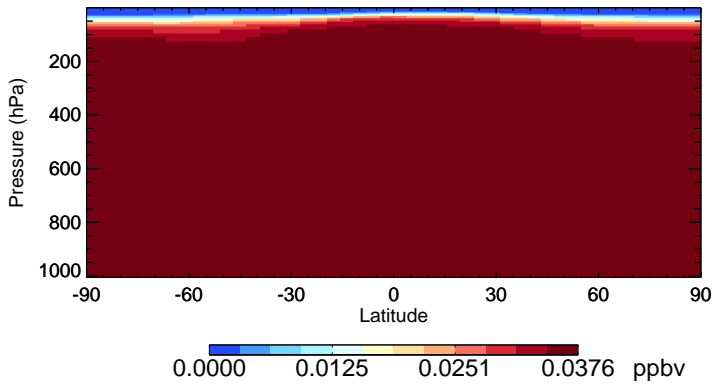
v11-01-public-Run0 HCFC141b - Species Zonal Mean for Jul
