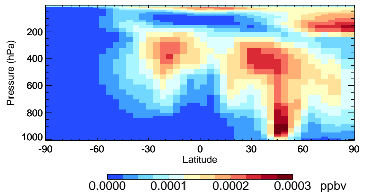
v11-02a ASOG1 - Species Curtain @ -180.000 for Jul
