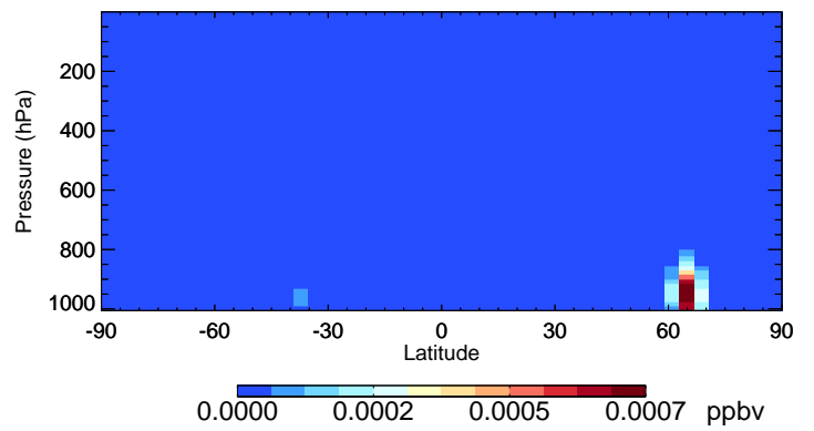
v11-02c ISOPNB - Species Curtain @ -180.000 for Jul
