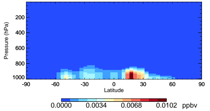
v11-02a NITs - Species Curtain @ -180.000 for Jul
