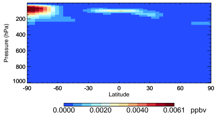
v11-02a ISOA3 - Species Curtain @ -180.000 for Jul
