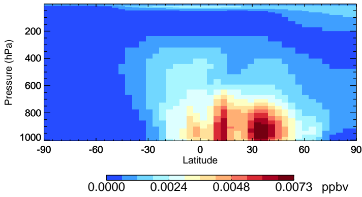
v11-01-public-Run0 ISOG1 - Species Zonal Mean for Jul
