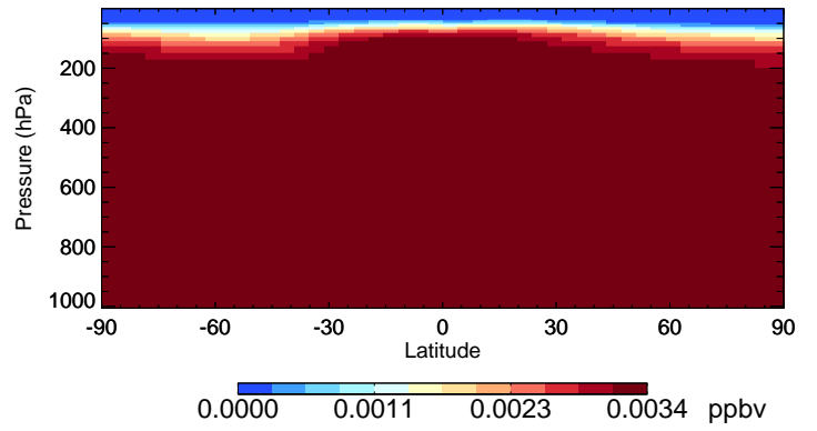
v11-01-public-Run0 H1211 - Species Curtain @ -180.000 for Jul
