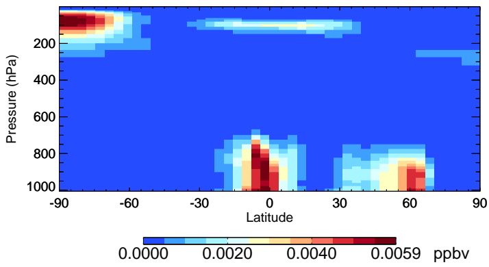
v11-01-public-Run0 ISOA3 - Species Zonal Mean for Jul
