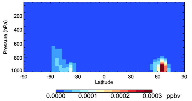
v11-01-public-Run0 NPMN - Species Curtain @ -180.000 for Jul
