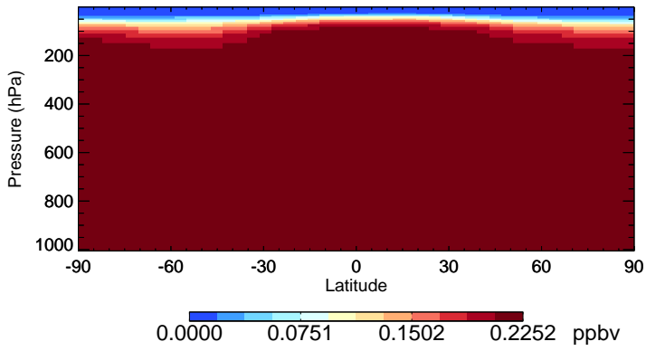
v11-01-public-Run0 CFC11 - Species Zonal Mean for Jul
