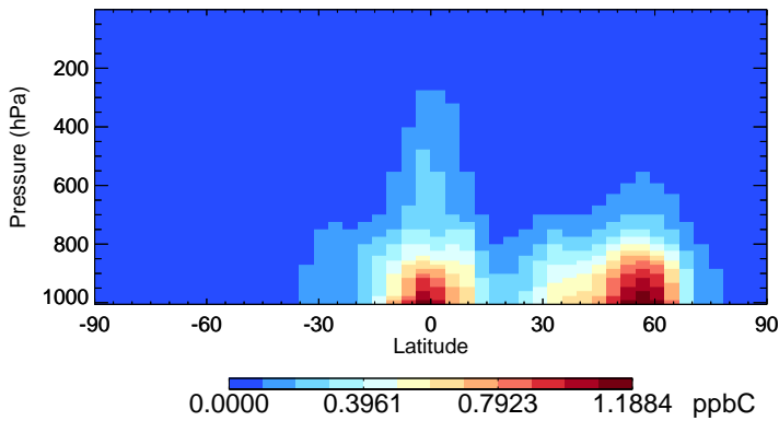
v11-02c MEK - Species Zonal Mean for Jul
