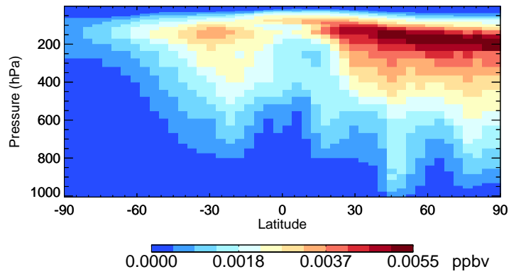
v11-02c ASOG3 - Species Curtain @ -180.000 for Jul
