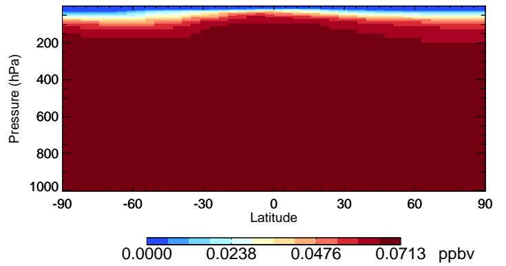
v11-02c CFC113 - Species Curtain @ -180.000 for Jul
