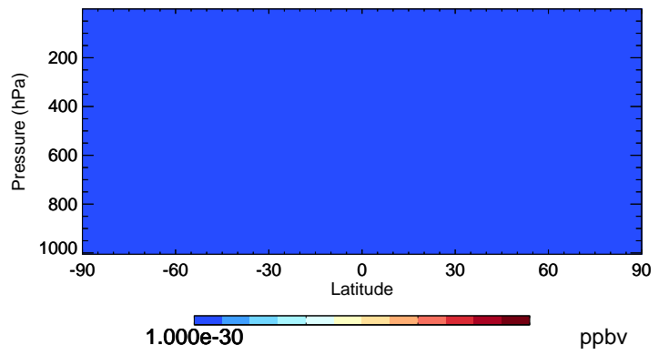
v11-01-public-Run0 MGLY - Species Curtain @ -180.000 for Jul
