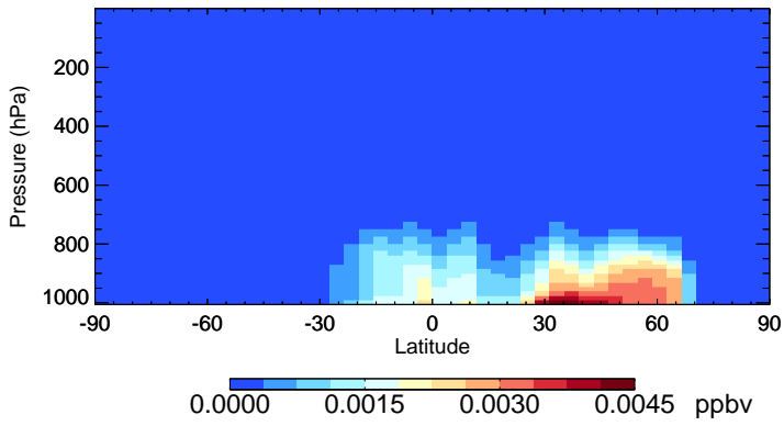
v11-01-public-Run0 NPMN - Species Zonal Mean for Jul
