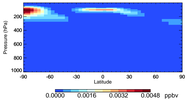
v11-02c ISOA3 - Species Curtain @ -180.000 for Jul
