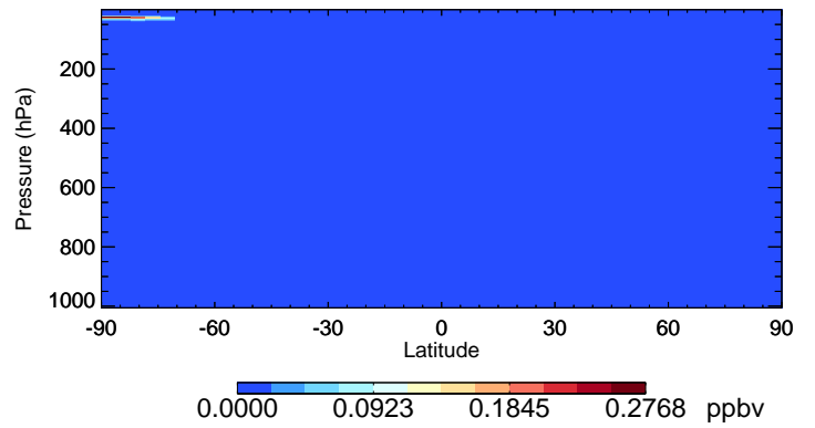
v11-02c ClNO2 - Species Curtain @ -180.000 for Jul
