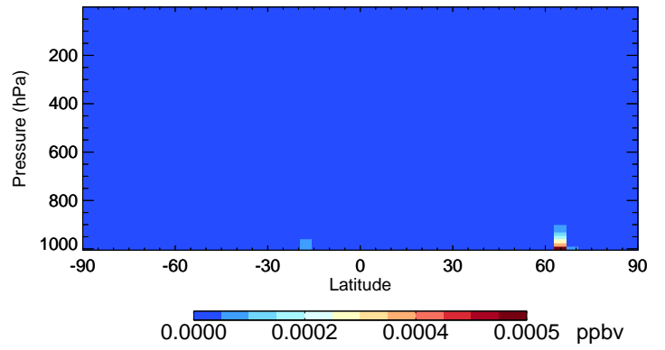
v11-01-public-Run0 LIMO - Species Curtain @ -180.000 for Jul
