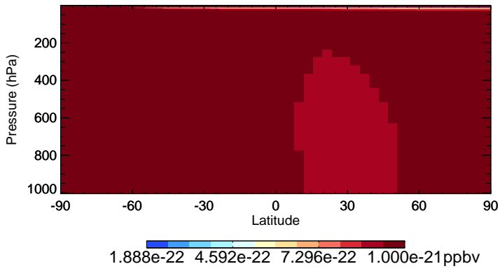
v11-01-public-Run0 HCFC123 - Species Zonal Mean for Jul
