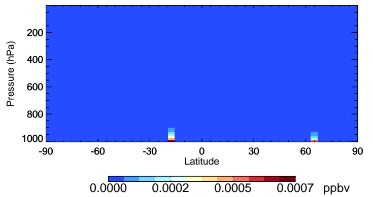
v11-02c MTPO - Species Curtain @ -180.000 for Jul
