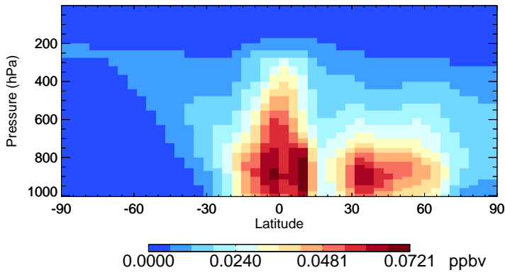
v11-01-public-Run0 MAP - Species Zonal Mean for Jul
