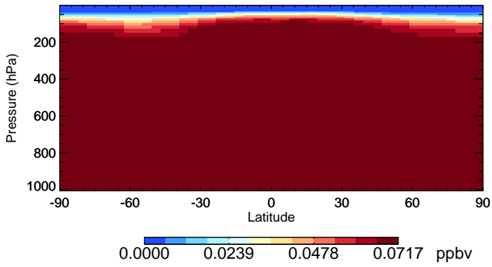
v11-01-public-Run0 CCI4 - Species Zonal Mean for Jul
