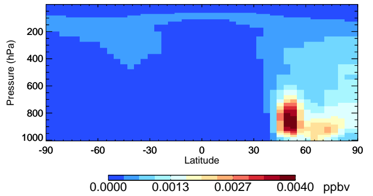
v11-02c TSOA0 - Species Curtain @ -180.000 for Jul
