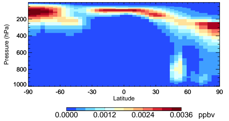
v11-01-public-Run0 TSOA2 - Species Curtain @ -180.000 for Jul
