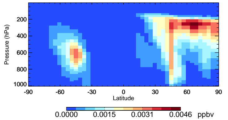
v11-02c DST2 - Species Curtain @ -180.000 for Jul
