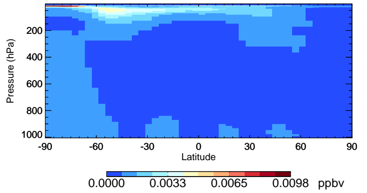
v11-01-public-Run0 HOBr - Species Curtain @ -180.000 for Jul
