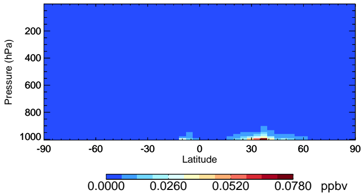
v11-01-public-Run0 HNO2 - Species Zonal Mean for Jul
