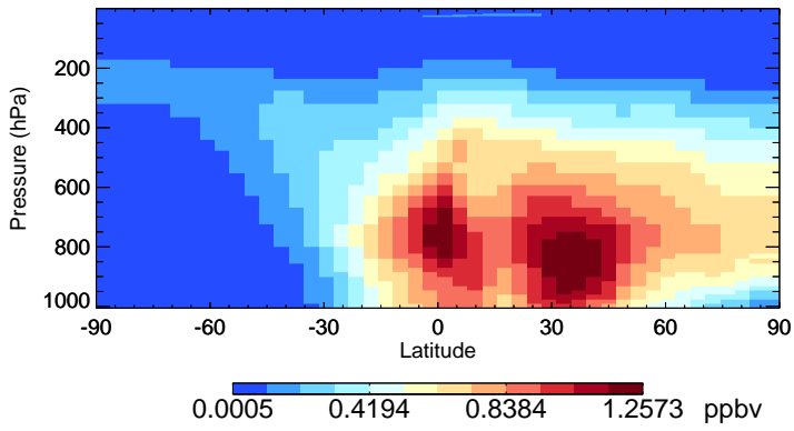
v11-01-public-Run0 H2O2 - Species Zonal Mean for Jul
