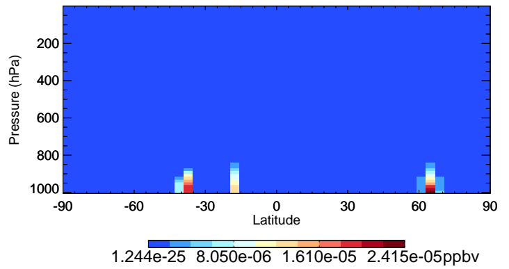
v11-02c MONITU - Species Curtain @ -180.000 for Jul
