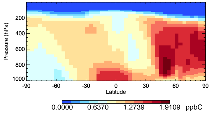
v11-01-public-Run0 ACET - Species Curtain @ -180.000 for Jul
