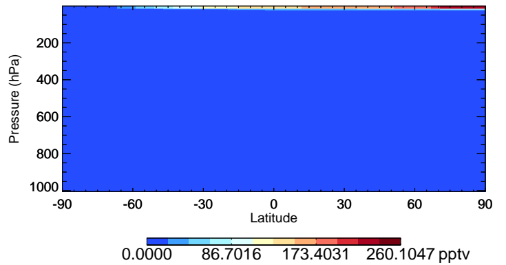
v11-02c HO2 - Species Curtain @ -180.000 for Jul
