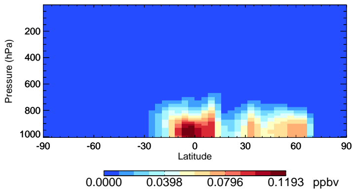
v11-01-public-Run0 GLYC - Species Zonal Mean for Jul
