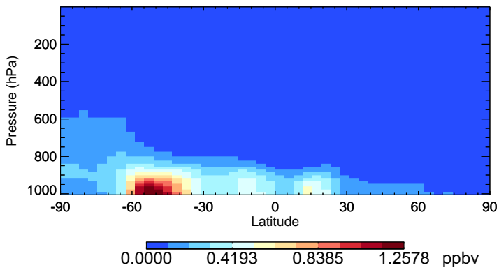
v11-01-public-Run0 SALA - Species Zonal Mean for Jul
