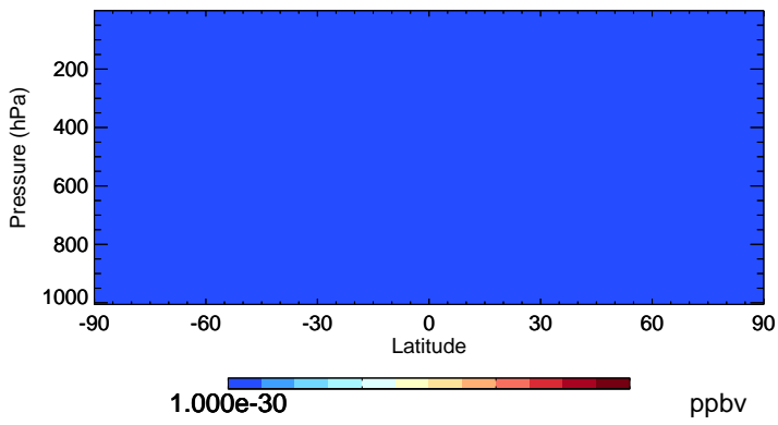
v11-01-public-Run0 MGLY - Species Zonal Mean for Jul
