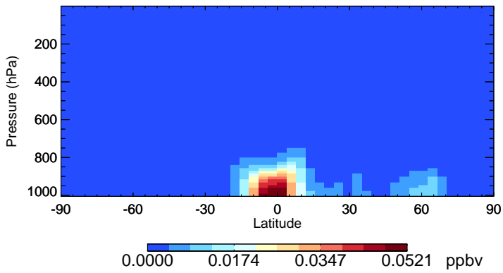
v11-02c HPALD - Species Zonal Mean for Jul
