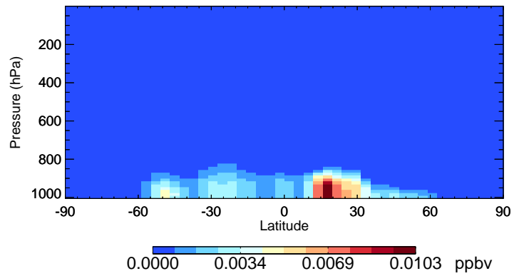
v11-02c NITs - Species Curtain @ -180.000 for Jul
