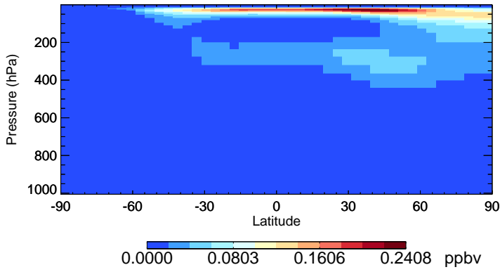
v11-02a HNO4 - Species Zonal Mean for Jul
