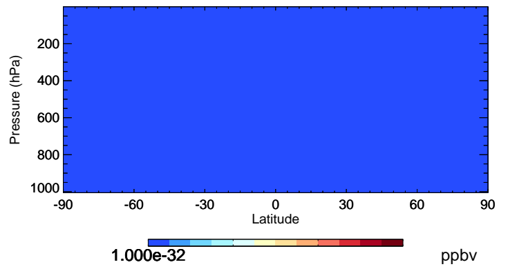
v11-01-public-Run0 HCOOH - Species Curtain @ -180.000 for Jul
