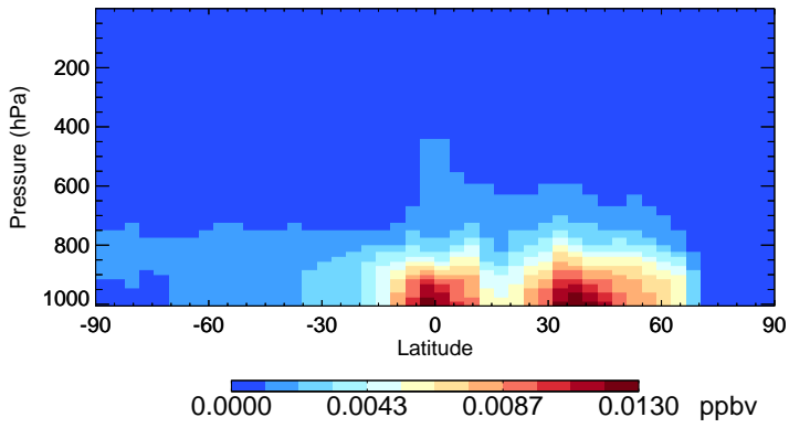
v11-01-public-Run0 RCHO - Species Zonal Mean for Jul
