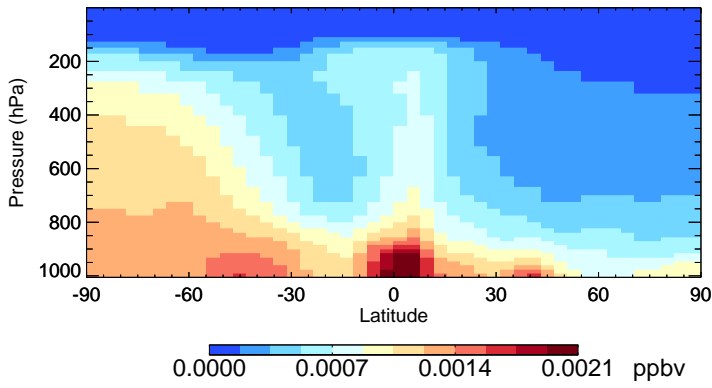
v11-01-public-Run0 CHBr3 - Species Zonal Mean for Jul
