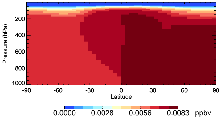
v11-01-public-Run0 CH3Br - Species Zonal Mean for Jul
