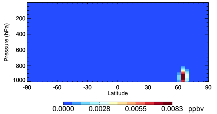
v11-02c HPALD - Species Curtain @ -180.000 for Jul
