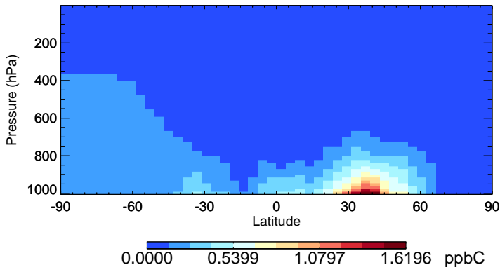
v11-01-public-Run0 ALK4 - Species Zonal Mean for Jul
