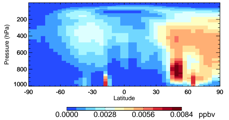
v11-02c TSOG2 - Species Curtain @ -180.000 for Jul
