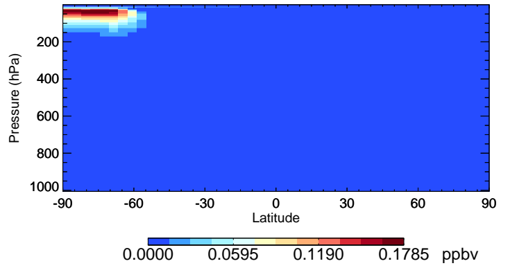
v11-02a OCIO - Species Curtain @ -180.000 for Jul
