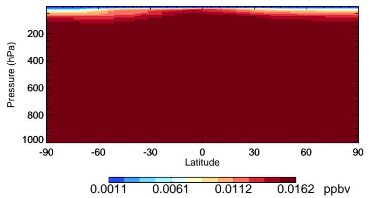
v11-02c CFC114 - Species Curtain @ -180.000 for Jul
