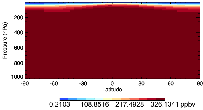
v11-01-public-Run0 N2O - Species Zonal Mean for Jul
