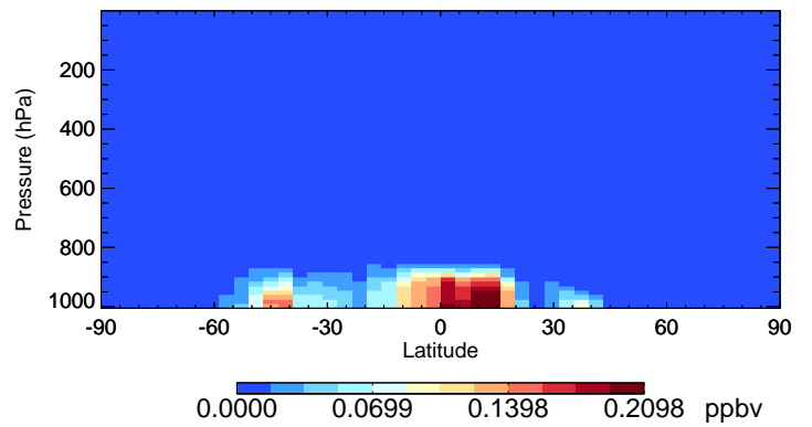
v11-01-public-Run0 NH3 - Species Curtain @ -180.000 for Jul
