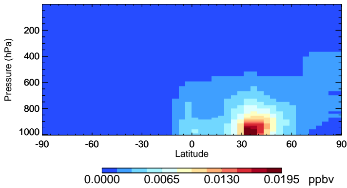
v11-02c ASOAN - Species Zonal Mean for Jul
