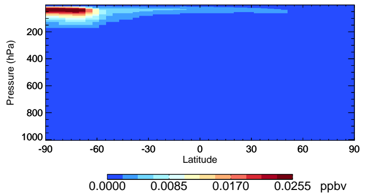
v11-01-public-Run0 BrCl - Species Curtain @ -180.000 for Jul
