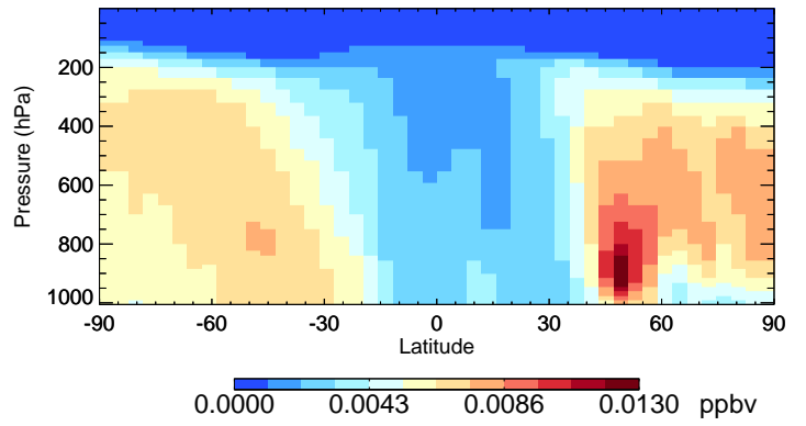
v11-01-public-Run0 R4N2 - Species Curtain @ -180.000 for Jul
