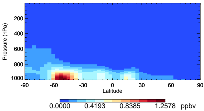
v11-02c SALA - Species Zonal Mean for Jul
