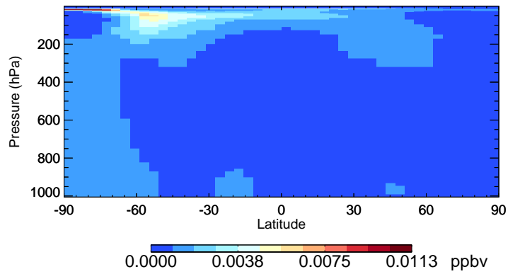
v11-02c HOBr - Species Curtain @ -180.000 for Jul
