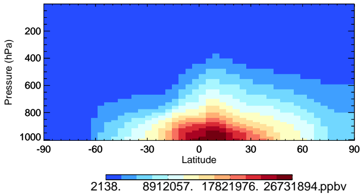
v11-01-public-Run0 H2O - Species Zonal Mean for Jul
