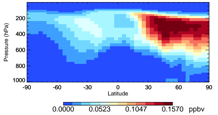
v11-01-public-Run0 PAN - Species Curtain @ -180.000 for Jul
