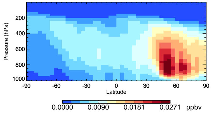
v11-01-public-Run0 MAP - Species Curtain @ -180.000 for Jul
