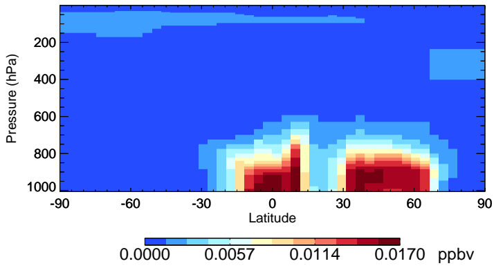
v11-01-public-Run0 ISOA1 - Species Zonal Mean for Jul
