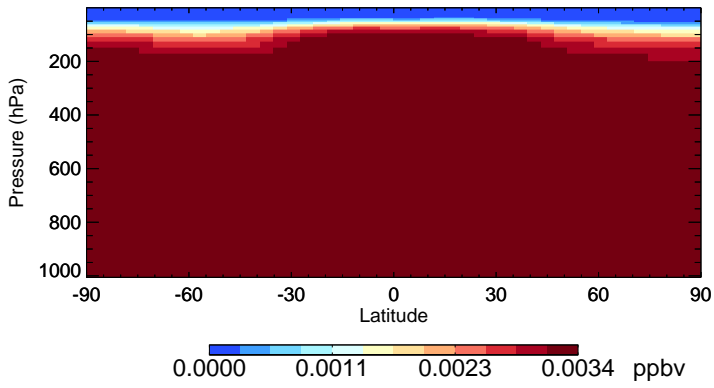
v11-01-public-Run0 H1211 - Species Zonal Mean for Jul
