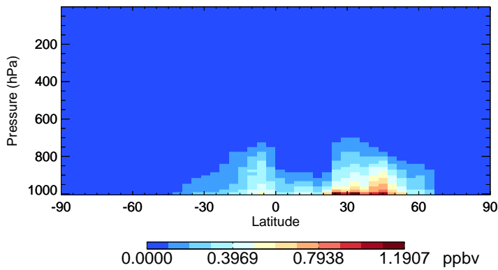
v11-01-public-Run0 NH3 - Species Zonal Mean for Jul
