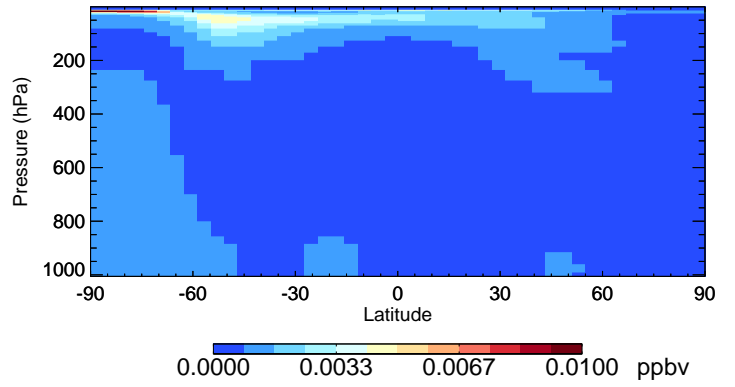
v11-02a HOBr - Species Curtain @ -180.000 for Jul
