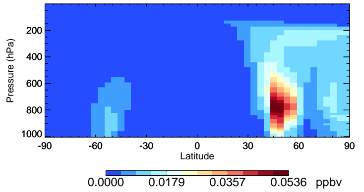
v11-01-public-Run0 DST1 - Species Curtain @ -180.000 for Jul
