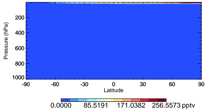
v11-01-public-Run0 HO2 - Species Curtain @ -180.000 for Jul
