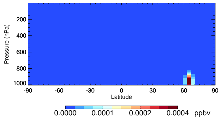
v11-01-public-Run0 ISOPNB - Species Curtain @ -180.000 for Jul
