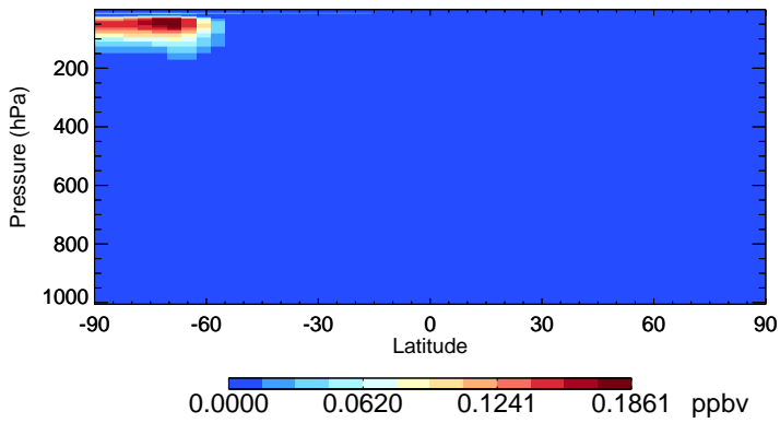
v11-02c OCIO - Species Zonal Mean for Jul
