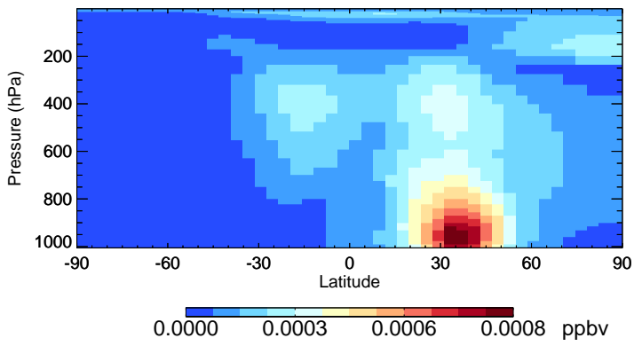
v11-02a ASOG1 - Species Zonal Mean for Jul
