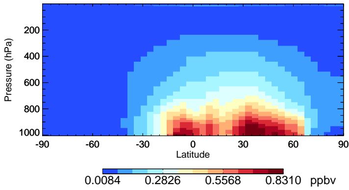
v11-01-public-Run0 CH2O - Species Zonal Mean for Jul
