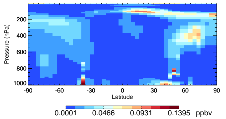
v11-01-public-Run0 SO2 - Species Curtain @ -180.000 for Jul
