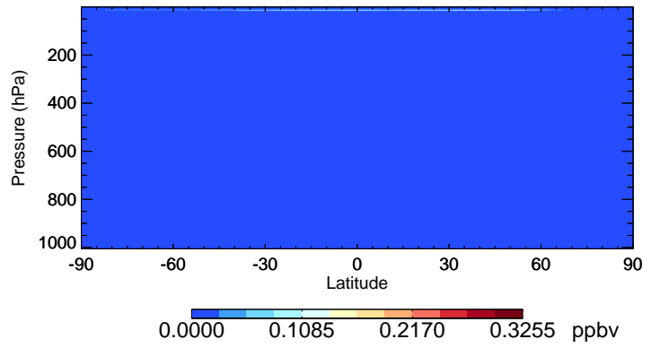
v11-01-public-Run0 NO3 - Species Curtain @ -180.000 for Jul
