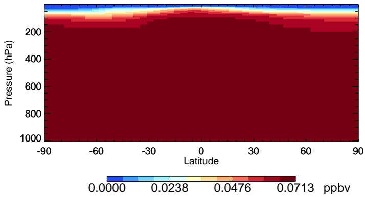
v11-02c CFC113 - Species Zonal Mean for Jul
