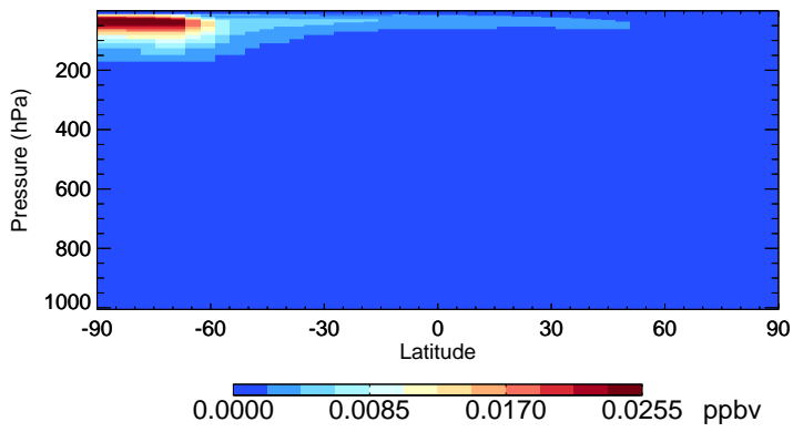
v11-01-public-Run0 BrCl - Species Zonal Mean for Jul
