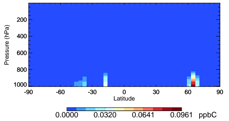
v11-01-public-Run0 PRPE - Species Curtain @ -180.000 for Jul
