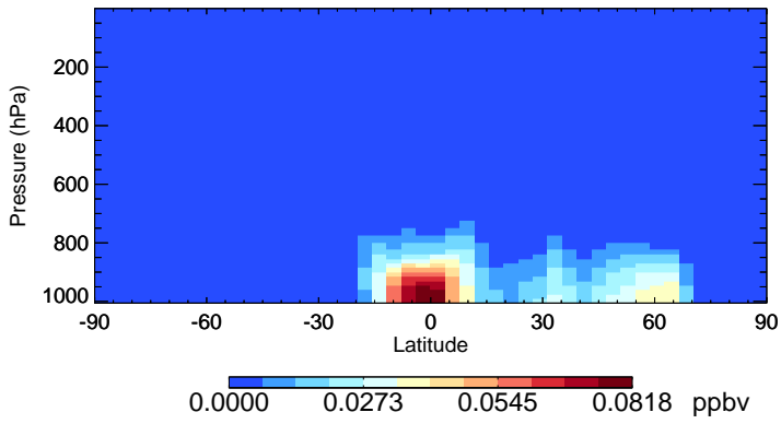
v11-01-public-Run0 MACR - Species Zonal Mean for Jul
