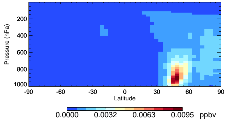
v11-02a ASOAN - Species Curtain @ -180.000 for Jul
