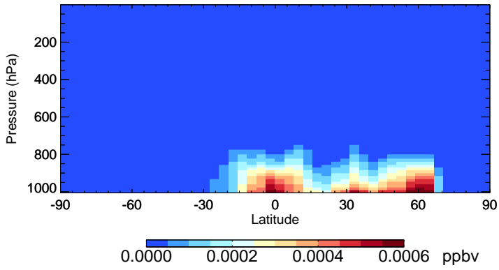
v11-02a MOBA - Species Zonal Mean for Jul
