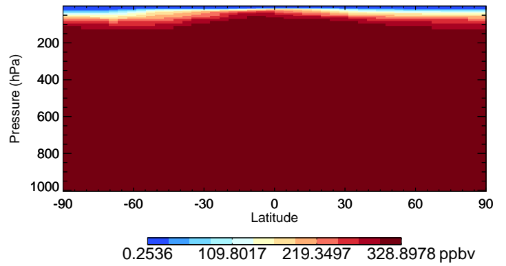
v11-02c N2O - Species Curtain @ -180.000 for Jul
