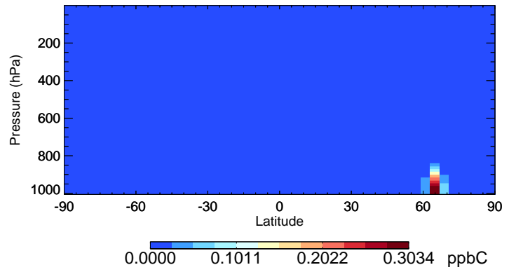
v11-01-public-Run0 ISOP - Species Curtain @ -180.000 for Jul
