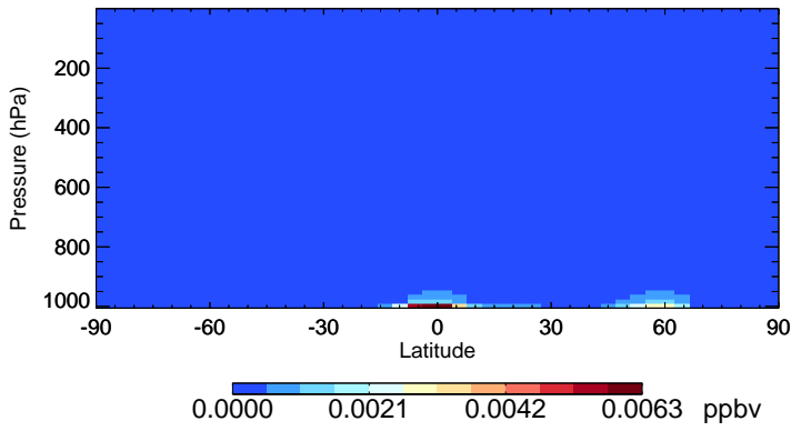
v11-01-public-Run0 LIMO - Species Zonal Mean for Jul
