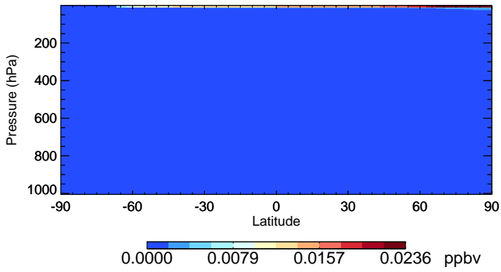
v11-01-public-Run0 Br - Species Zonal Mean for Jul
