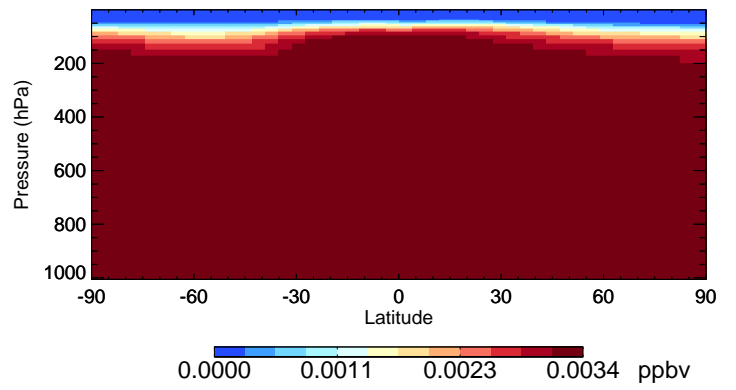
v11-02a H1211 - Species Curtain @ -180.000 for Jul
