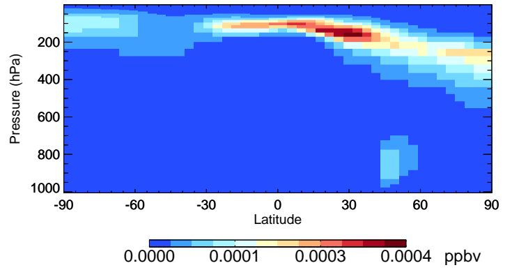
v11-02a ASOA2 - Species Curtain @ -180.000 for Jul
