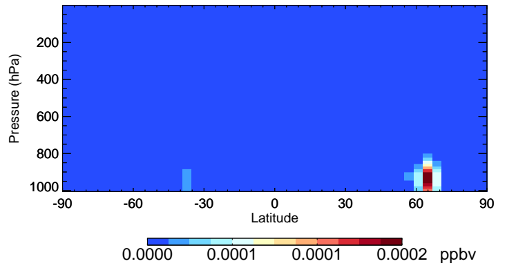
v11-01-public-Run0 MACRN - Species Curtain @ -180.000 for Jul
