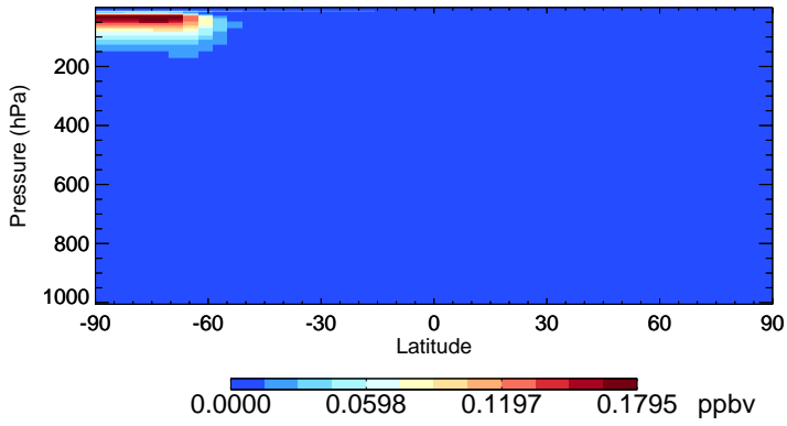
v11-02a OCIO - Species Zonal Mean for Jul
