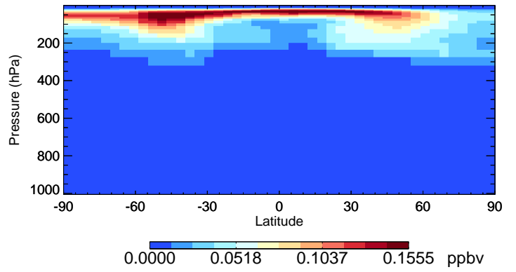
v11-01-public-Run0 MPN - Species Curtain @ -180.000 for Jul
