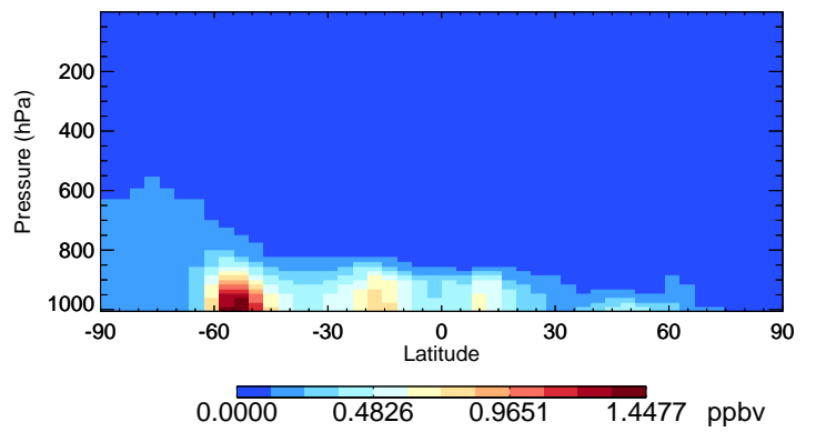
v11-02c SALA - Species Curtain @ -180.000 for Jul
