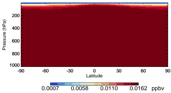
v11-02a CFC114 - Species Zonal Mean for Jul
