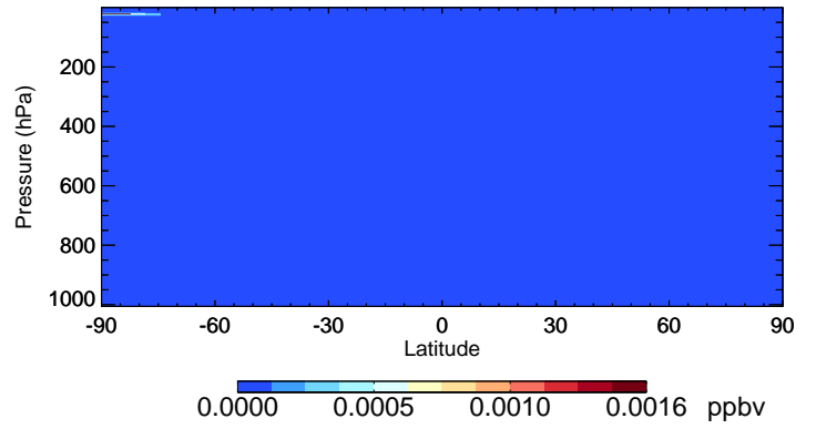
v11-02a ClNO2 - Species Curtain @ -180.000 for Jul
