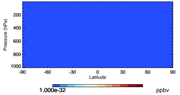
v11-02a HPALD - Species Curtain @ -180.000 for Jul
