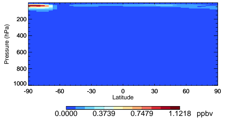
v11-02c HNO4 - Species Curtain @ -180.000 for Jul
