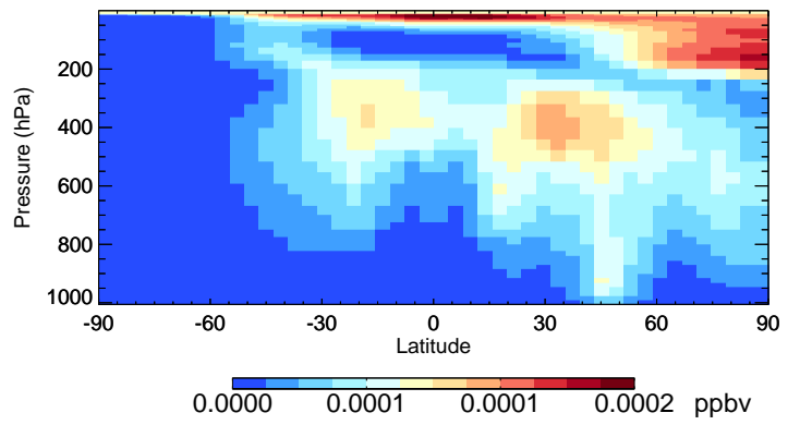
v11-01-public-Run0 ASOG1 - Species Curtain @ -180.000 for Jul
