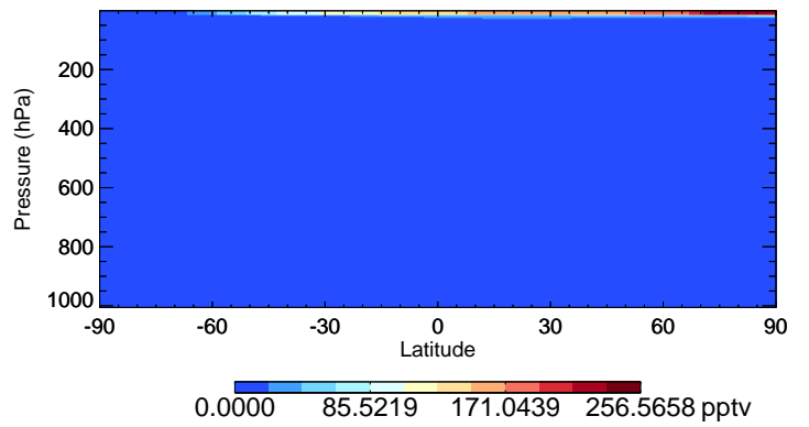
v11-02a HO2 - Species Curtain @ -180.000 for Jul
