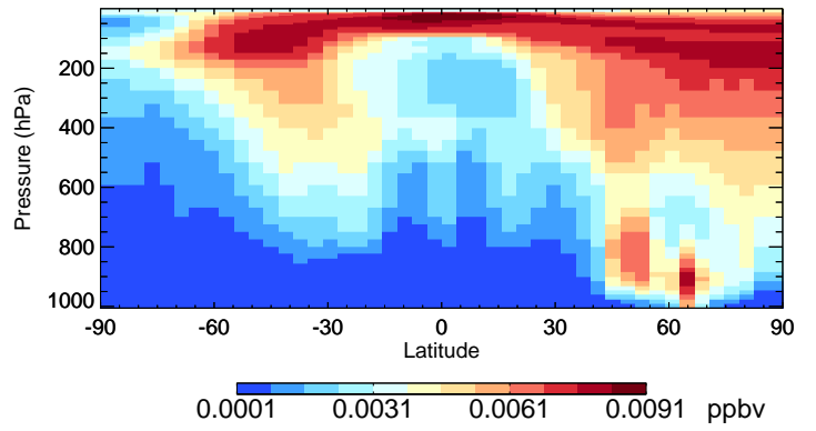
v11-01-public-Run0 ISO3 - Species Curtain @ -180.000 for Jul
