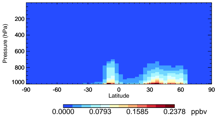
v11-02c BCPO - Species Zonal Mean for Jul
