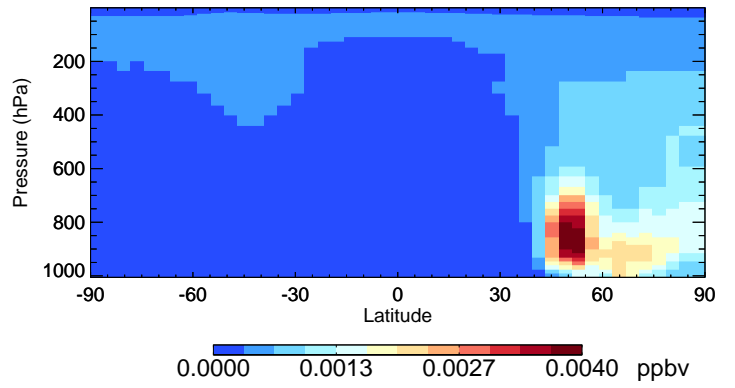
v11-01-public-Run0 TSOA0 - Species Curtain @ -180.000 for Jul
