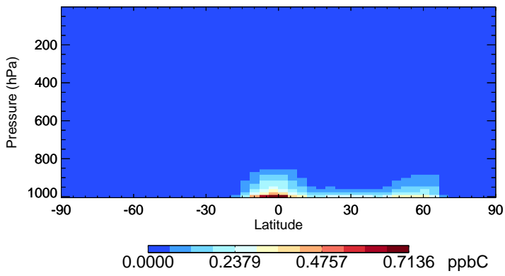
v11-01-public-Run0 PRPE - Species Zonal Mean for Jul
