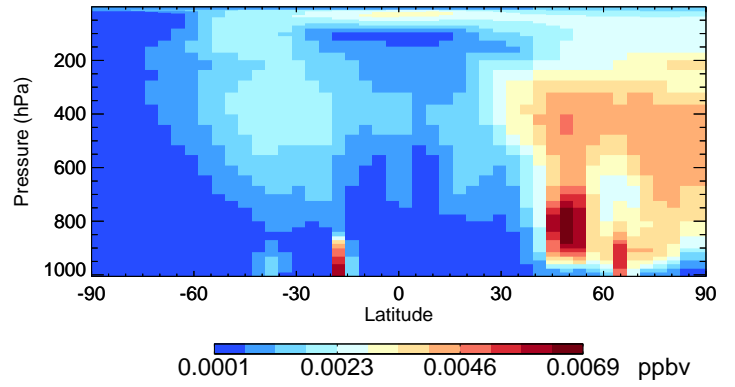
v11-02a TSOG2 - Species Curtain @ -180.000 for Jul
