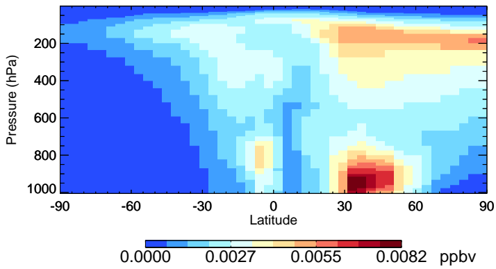
v11-02c ASOG3 - Species Zonal Mean for Jul
