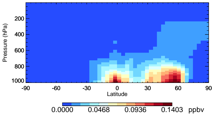
v11-02c TSOG3 - Species Zonal Mean for Jul
