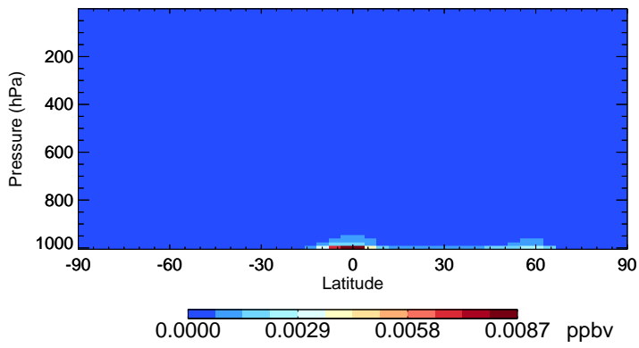
v11-02a MTPO - Species Zonal Mean for Jul
