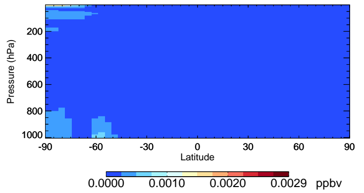
v11-01-public-Run0 Br2 - Species Curtain @ -180.000 for Jul
