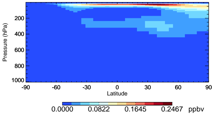
v11-01-public-Run0 HNO4 - Species Zonal Mean for Jul
