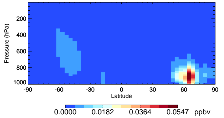
v11-01-public-Run0 HAC - Species Curtain @ -180.000 for Jul
