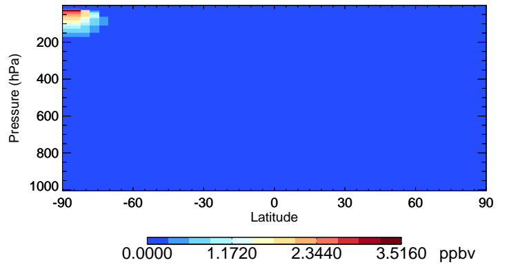
v11-01-public-Run0 NIT - Species Curtain @ -180.000 for Jul
