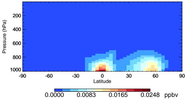
v11-02a TSOA0 - Species Zonal Mean for Jul
