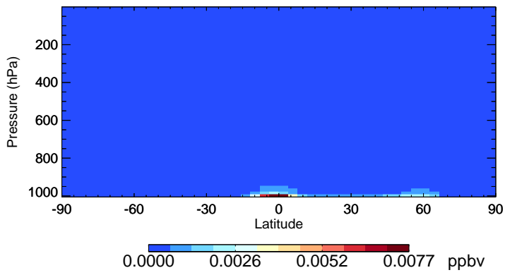
v11-01-public-Run0 MTPO - Species Zonal Mean for Jul
