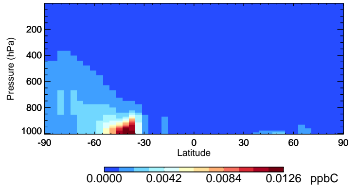
v11-02a XYLE - Species Curtain @ -180.000 for Jul
