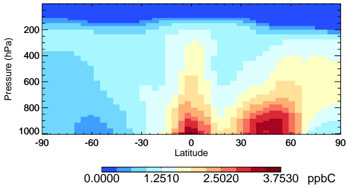
v11-01-public-Run0 ACET - Species Zonal Mean for Jul
