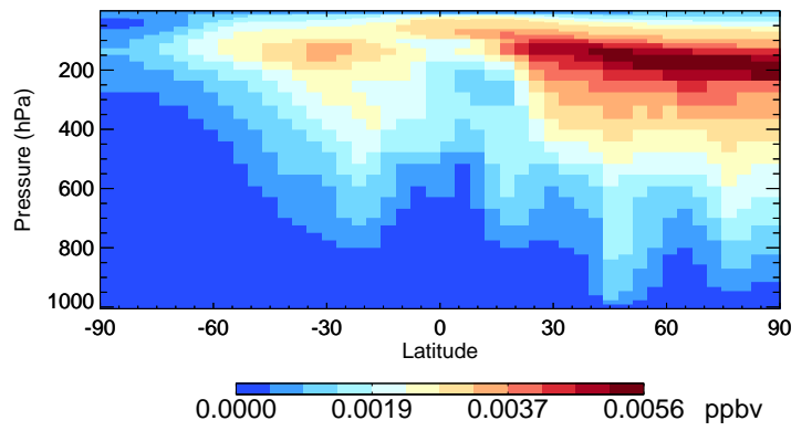
v11-02a ASOG3 - Species Curtain @ -180.000 for Jul
