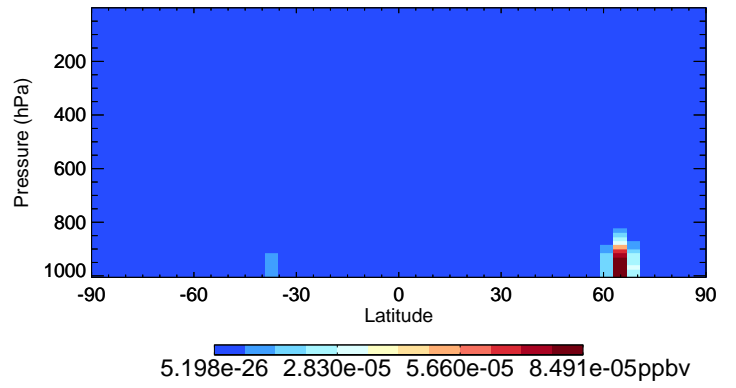
v11-01-public-Run0 MOBA - Species Curtain @ -180.000 for Jul
