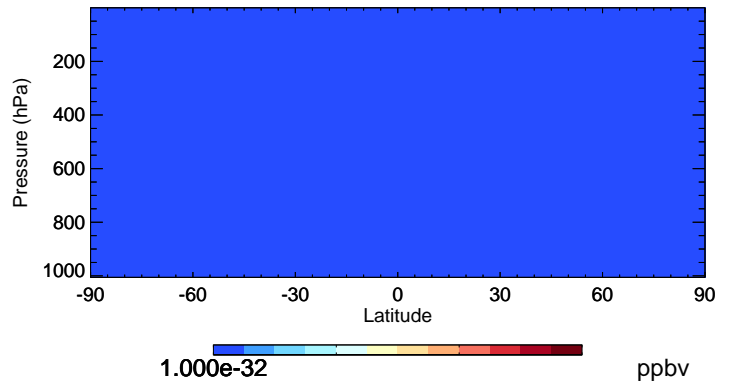
v11-01-public-Run0 MONITU - Species Curtain @ -180.000 for Jul
