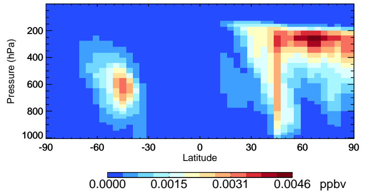
v11-01-public-Run0 DST2 - Species Curtain @ -180.000 for Jul
