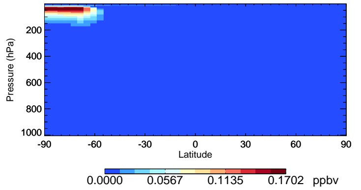
v11-01-public-Run0 OCIO - Species Curtain @ -180.000 for Jul
