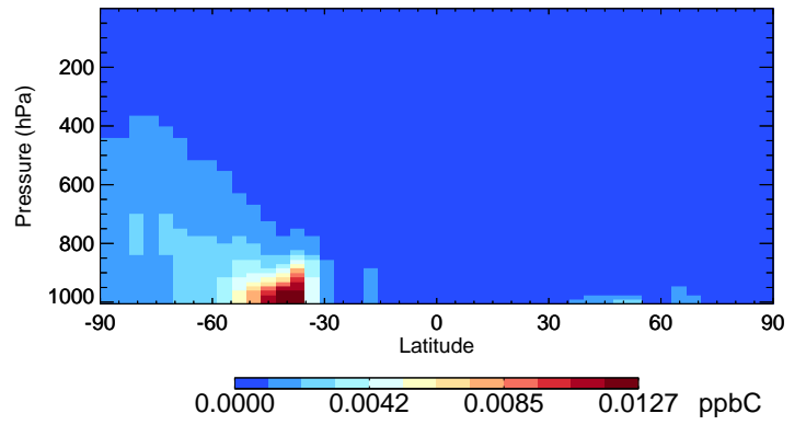
v11-01-public-Run0 XYLE - Species Curtain @ -180.000 for Jul
