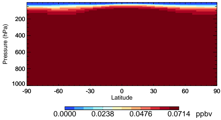
v11-01-public-Run0 CFC113 - Species Zonal Mean for Jul
