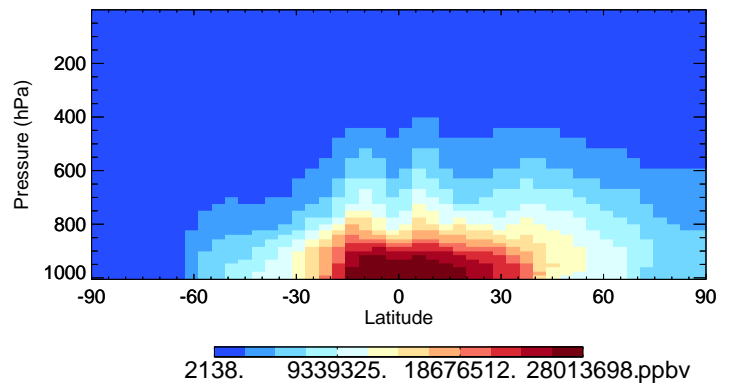
v11-02a H2O - Species Curtain @ -180.000 for Jul
