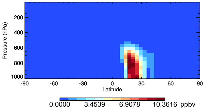
v11-01-public-Run0 DST2 - Species Zonal Mean for Jul
