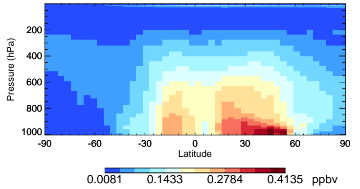
v11-01-public-Run0 CH2O - Species Curtain @ -180.000 for Jul
