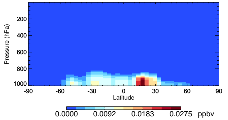
v11-01-public-Run0 NITs - Species Curtain @ -180.000 for Jul
