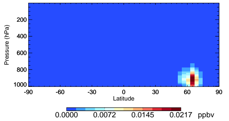
v11-01-public-Run0 GLYC - Species Curtain @ -180.000 for Jul
