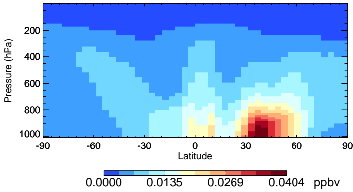
v11-01-public-Run0 R4N2 - Species Zonal Mean for Jul
