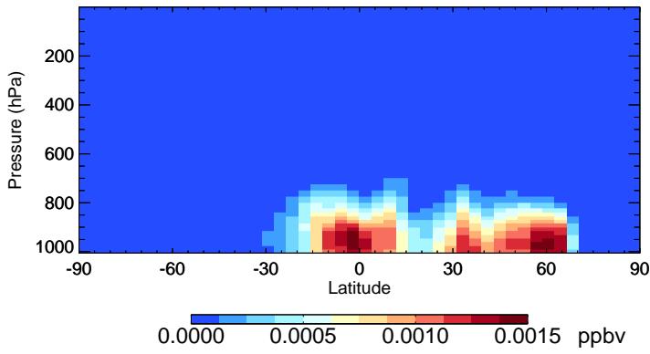
v11-01-public-Run0 MACRN - Species Zonal Mean for Jul
