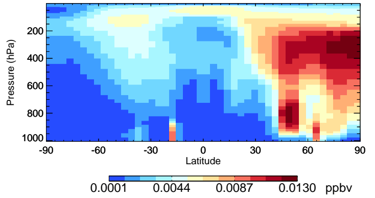
v11-02a TSOG3 - Species Curtain @ -180.000 for Jul
