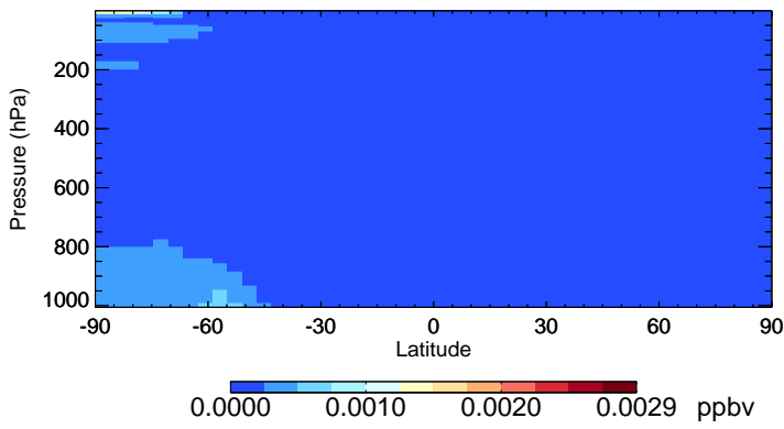
v11-01-public-Run0 Br2 - Species Zonal Mean for Jul
