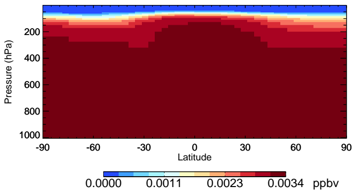
v11-02c H1211 - Species Zonal Mean for Jul
