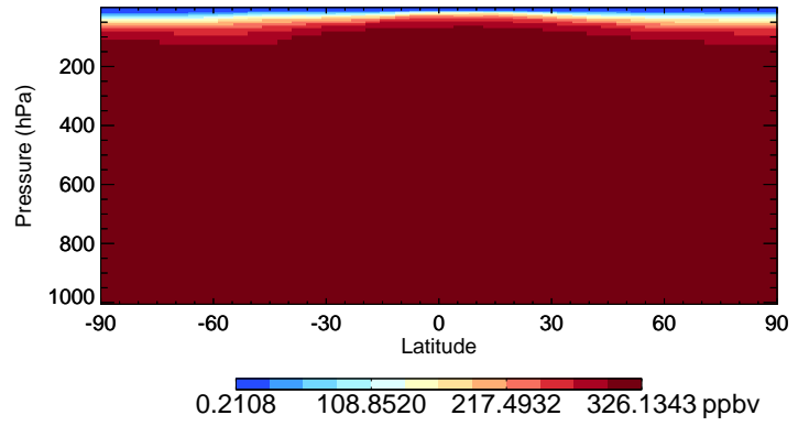
v11-02a N2O - Species Curtain @ -180.000 for Jul
