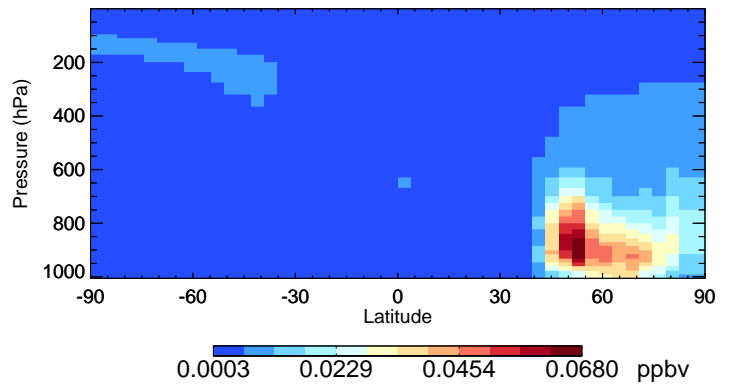
v11-02c SOAIE - Species Curtain @ -180.000 for Jul
