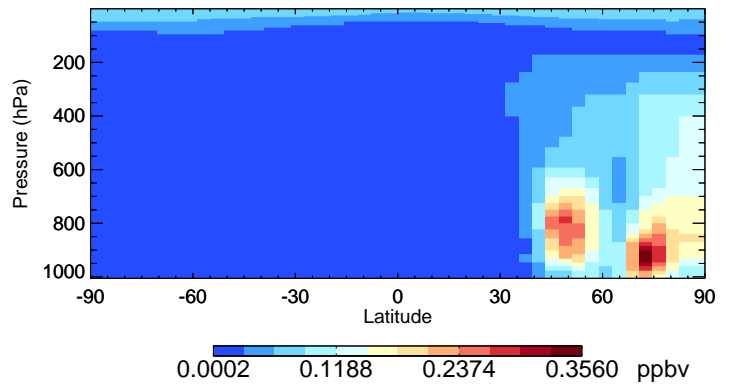
v11-02c OCPI - Species Curtain @ -180.000 for Jul
