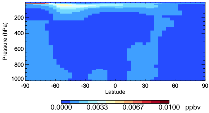
v11-02a HOBr - Species Zonal Mean for Jul
