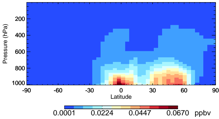
v11-01-public-Run0 TSOG2 - Species Zonal Mean for Jul
