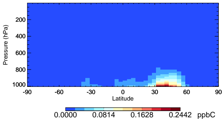
v11-01-public-Run0 TOLU - Species Zonal Mean for Jul
