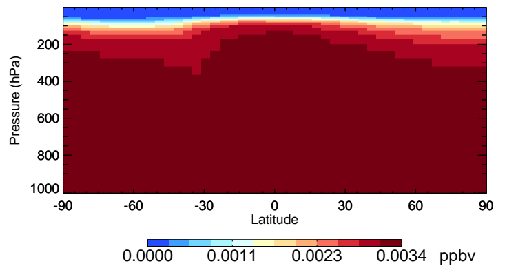
v11-02c H1211 - Species Curtain @ -180.000 for Jul
