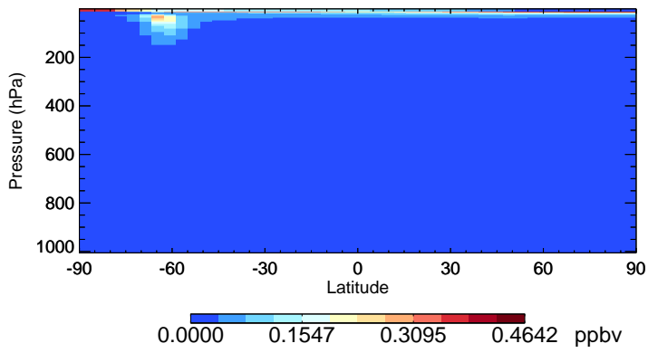
v11-01-public-Run0 CIO - Species Zonal Mean for Jul
