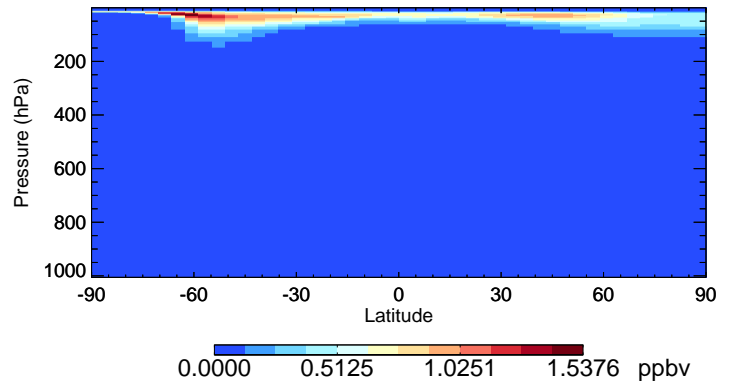
v11-01-public-Run0 ClNO3 - Species Curtain @ -180.000 for Jul
