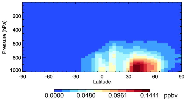
v11-02c INDIOL - Species Zonal Mean for Jul
