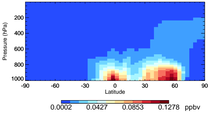
v11-02a TSOG3 - Species Zonal Mean for Jul
