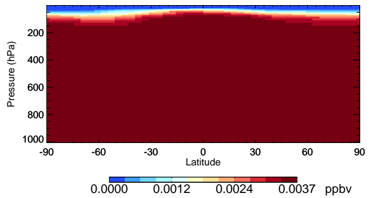
v11-02c H1301 - Species Curtain @ -180.000 for Jul
