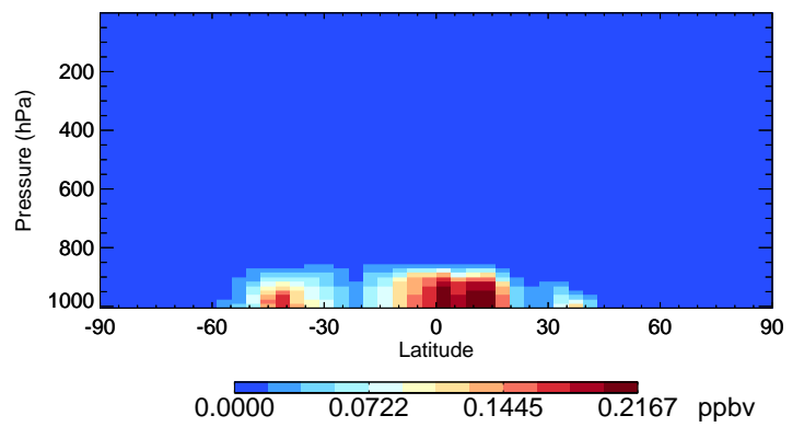
v11-02a NH3 - Species Curtain @ -180.000 for Jul
