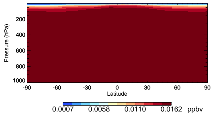
v11-02a CFC114 - Species Curtain @ -180.000 for Jul
