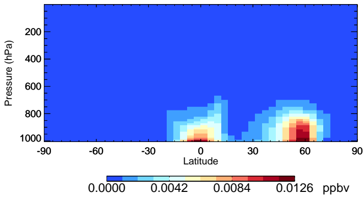
v11-02c TSOA1 - Species Zonal Mean for Jul
