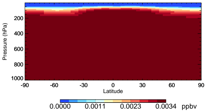
v11-02a H1211 - Species Zonal Mean for Jul
