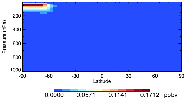
v11-01-public-Run0 OCIO - Species Zonal Mean for Jul
