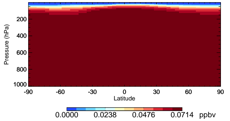
v11-01-public-Run0 CFC113 - Species Curtain @ -180.000 for Jul
