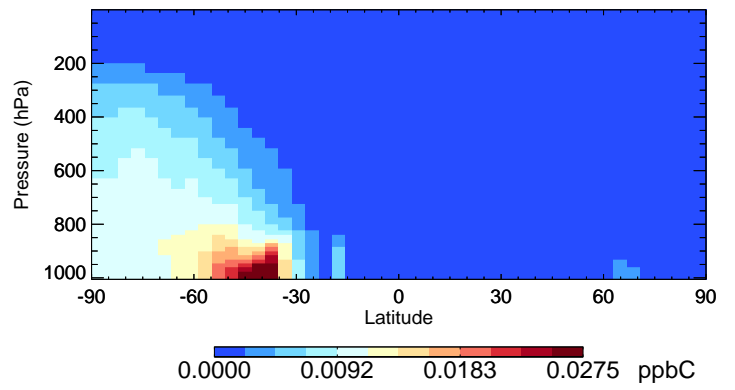
v11-01-public-Run0 TOLU - Species Curtain @ -180.000 for Jul
