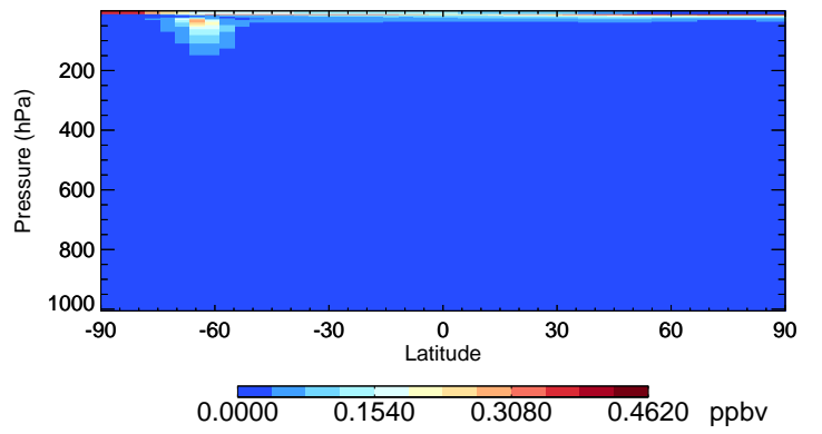
v11-01-public-Run0 CIO - Species Curtain @ -180.000 for Jul
