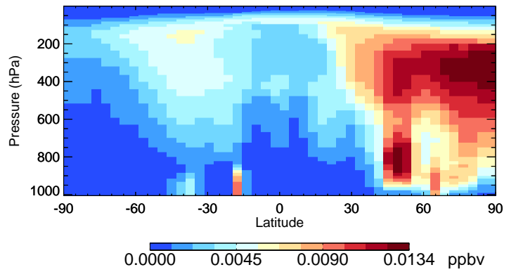
v11-02c TSOG3 - Species Curtain @ -180.000 for Jul
