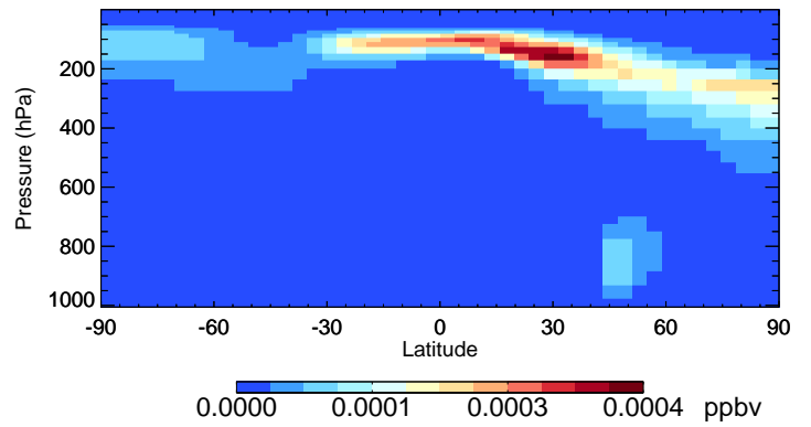
v11-02c ASOA2 - Species Curtain @ -180.000 for Jul
