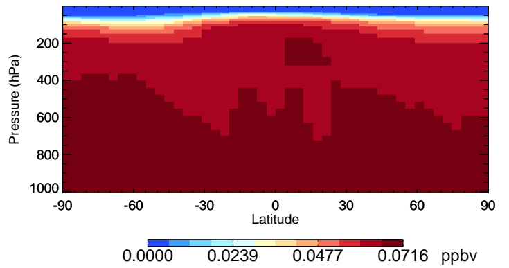
v11-02c CCI4 - Species Curtain @ -180.000 for Jul
