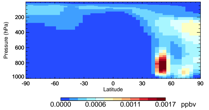
v11-02a TSOA1 - Species Curtain @ -180.000 for Jul
