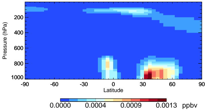
v11-02a ASOA2 - Species Zonal Mean for Jul
