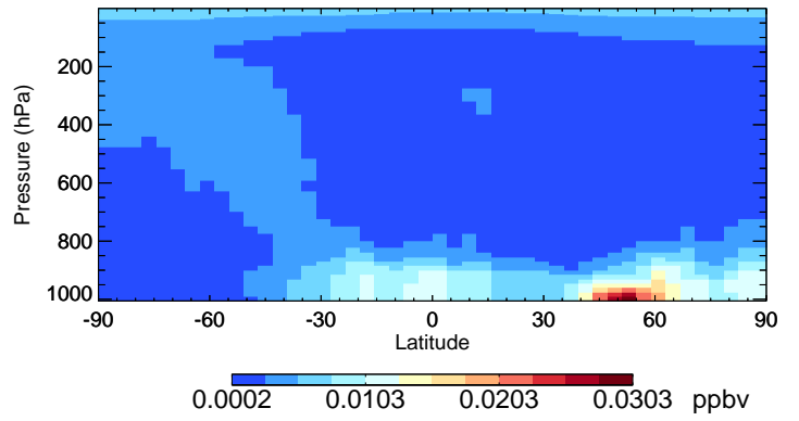
v11-01-public-Run0 MSA - Species Curtain @ -180.000 for Jul
