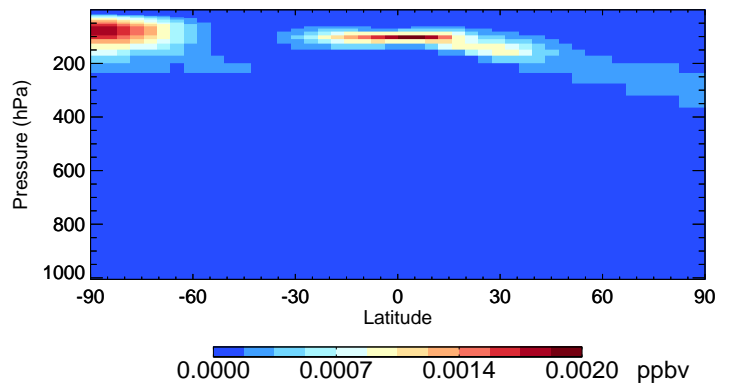
v11-02a ASOA3 - Species Curtain @ -180.000 for Jul
