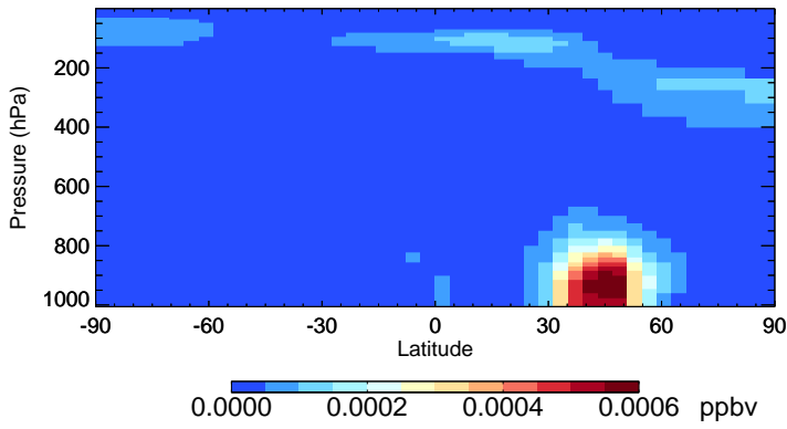
v11-01-public-Run0 ASOA2 - Species Zonal Mean for Jul
