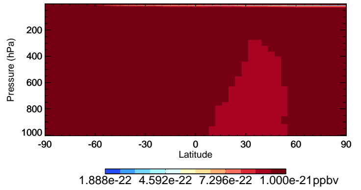
v11-01-public-Run0 HCFC123 - Species Curtain @ -180.000 for Jul
