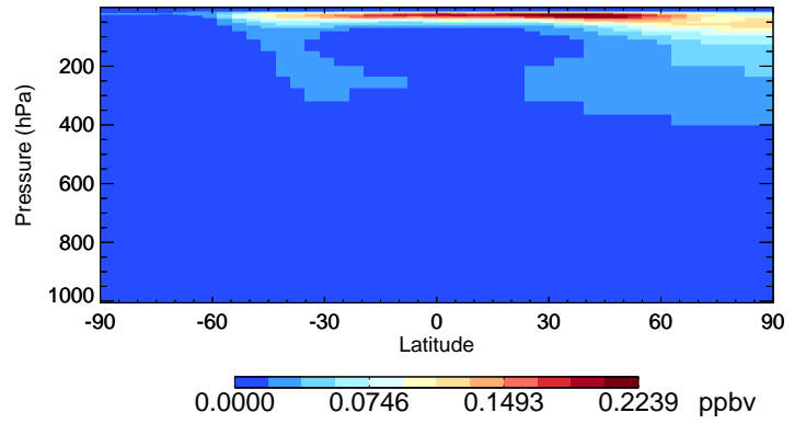
v11-02a HNO4 - Species Curtain @ -180.000 for Jul
