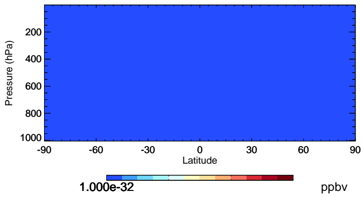
v11-01-public-Run0 ISN1OG - Species Zonal Mean for Jul
