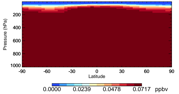
v11-02a CCI4 - Species Curtain @ -180.000 for Jul
