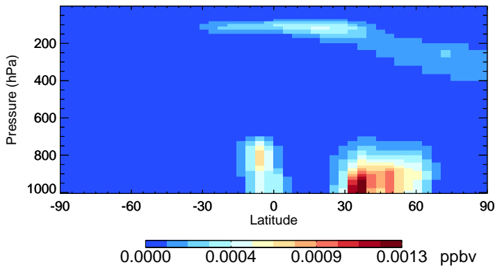
v11-02c ASOA2 - Species Zonal Mean for Jul
