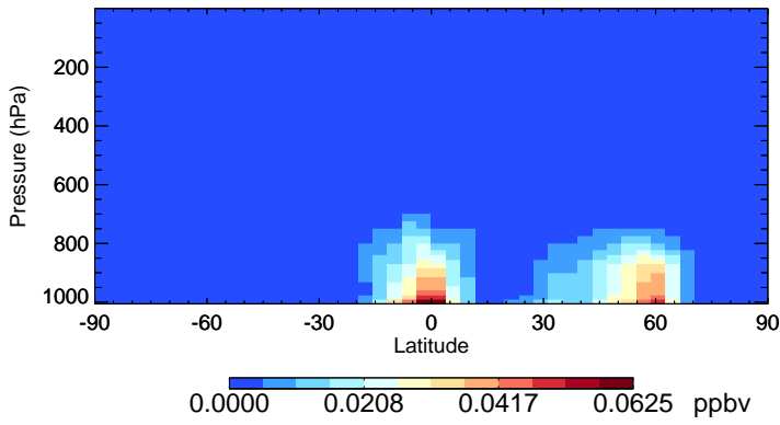
v11-01-public-Run0 TSOA2 - Species Zonal Mean for Jul
