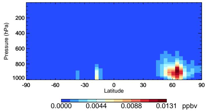
v11-02c HAC - Species Curtain @ -180.000 for Jul
