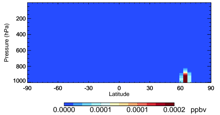
v11-02c MOBA - Species Curtain @ -180.000 for Jul
