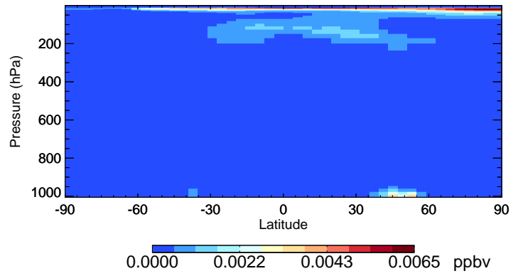
v11-01-public-Run0 HNO2 - Species Curtain @ -180.000 for Jul
