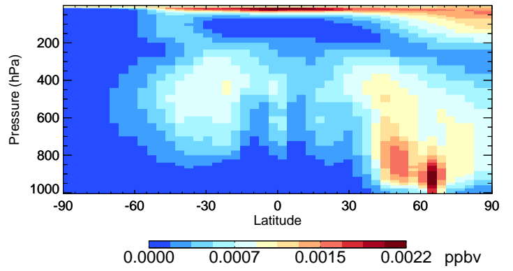
v11-01-public-Run0 ISOG1 - Species Curtain @ -180.000 for Jul
