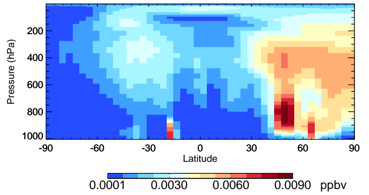
v11-01-public-Run0 TSOG2 - Species Curtain @ -180.000 for Jul
