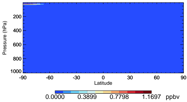
v11-01-public-Run0 Cl2 - Species Zonal Mean for Jul
