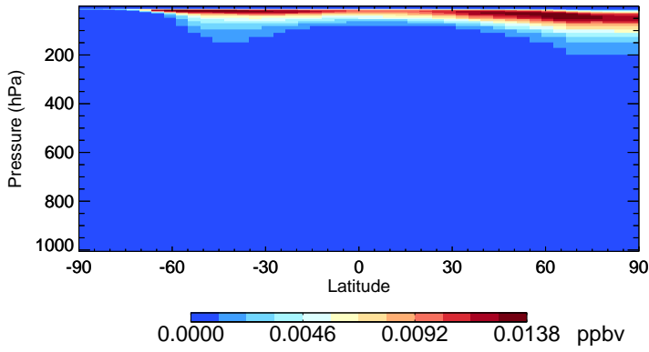
v11-02a BrNO3 - Species Zonal Mean for Jul
