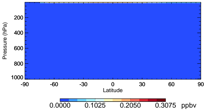
v11-01-public-Run0 CI - Species Zonal Mean for Jul
