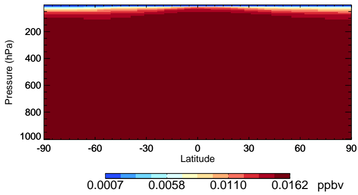
v11-01-public-Run0 CFC114 - Species Zonal Mean for Jul
