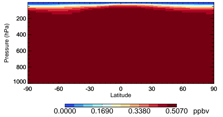
v11-01-public-Run0 CFC12 - Species Curtain @ -180.000 for Jul
