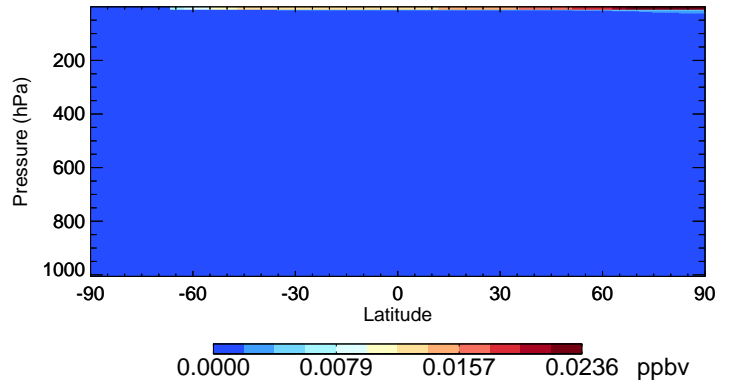
v11-02a Br - Species Curtain @ -180.000 for Jul
