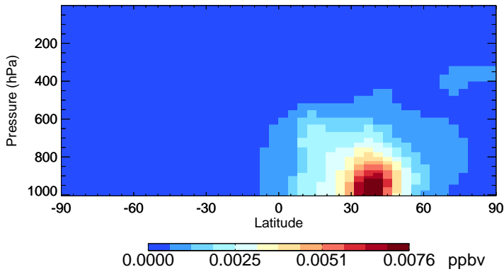
v11-01-public-Run0 ASOAN - Species Zonal Mean for Jul
