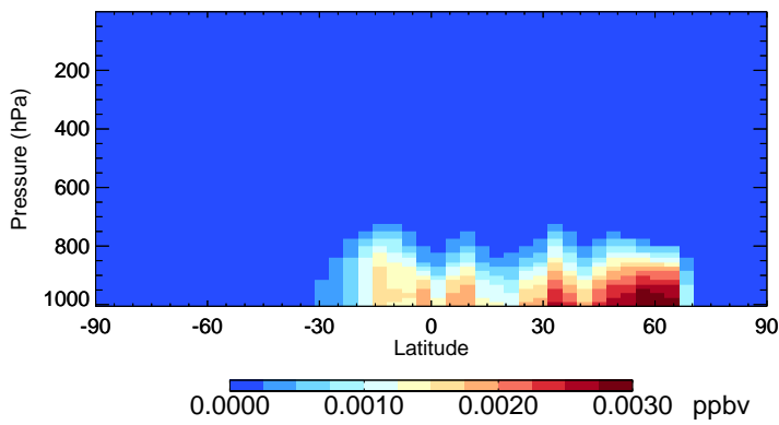
v11-02c ISOPNB - Species Zonal Mean for Jul
