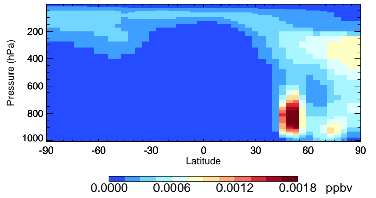
v11-01-public-Run0 TSOA1 - Species Curtain @ -180.000 for Jul
