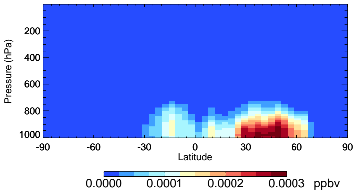
v11-02c MACRN - Species Zonal Mean for Jul
