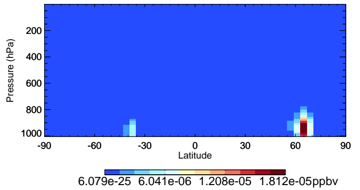
v11-02c MACRN - Species Curtain @ -180.000 for Jul
