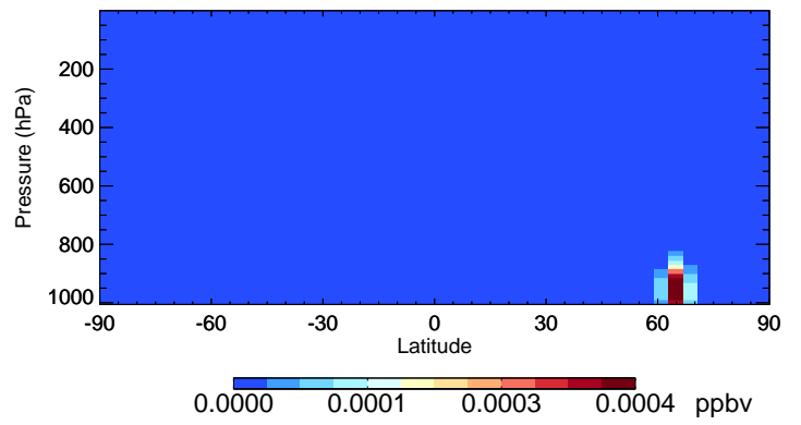
v11-02a ISOPNB - Species Curtain @ -180.000 for Jul
