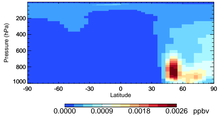
v11-02a TSOA0 - Species Curtain @ -180.000 for Jul
