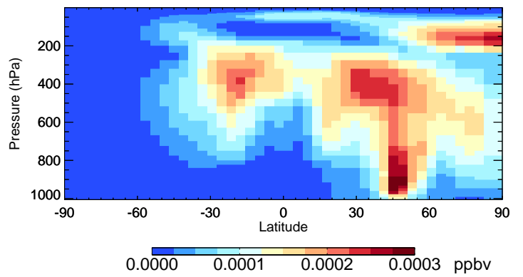
v11-02c ASOG1 - Species Curtain @ -180.000 for Jul
