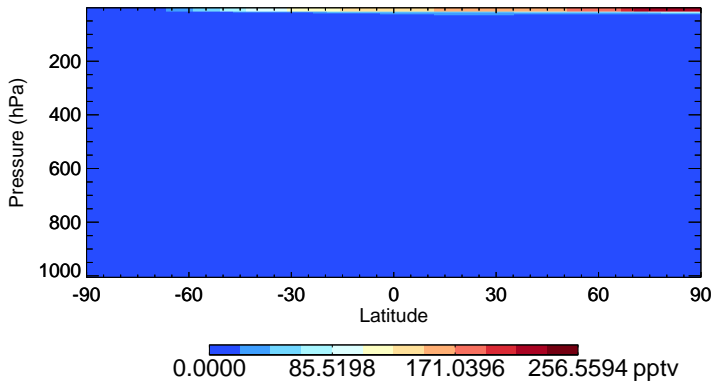
v11-01-public-Run0 HO2 - Species Zonal Mean for Jul
