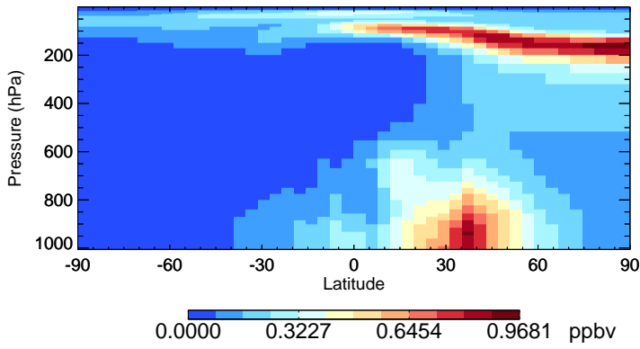
v11-01-public-Run0 SO4 - Species Zonal Mean for Jul
