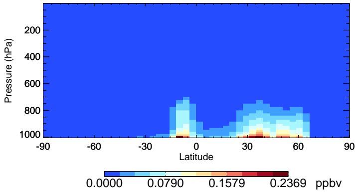
v11-02a BCPO - Species Zonal Mean for Jul
