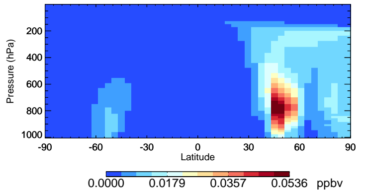
v11-02c DST1 - Species Curtain @ -180.000 for Jul
