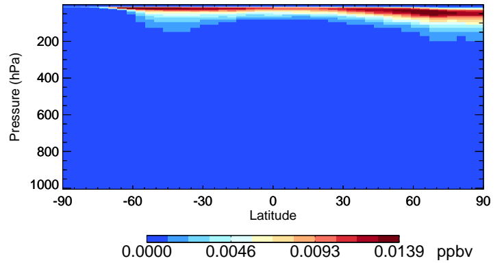
v11-02a BrNO3 - Species Curtain @ -180.000 for Jul
