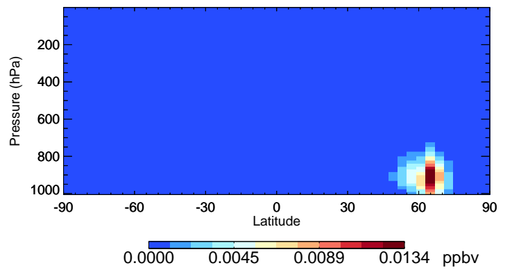
v11-02c GLYC - Species Curtain @ -180.000 for Jul
