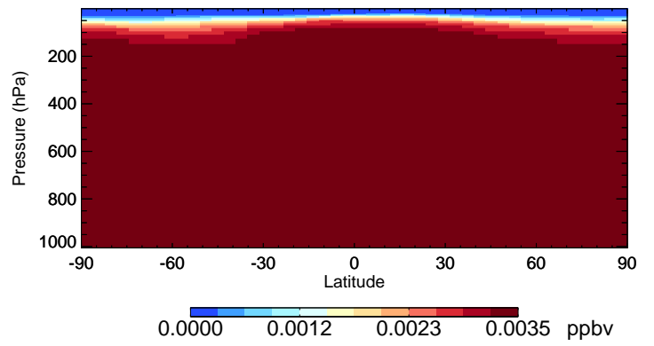
v11-02a H1301 - Species Curtain @ -180.000 for Jul
