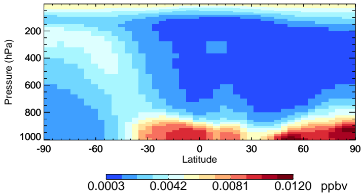
v11-01-public-Run0 MSA - Species Zonal Mean for Jul
