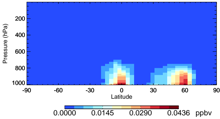
v11-02a TSOA2 - Species Zonal Mean for Jul
