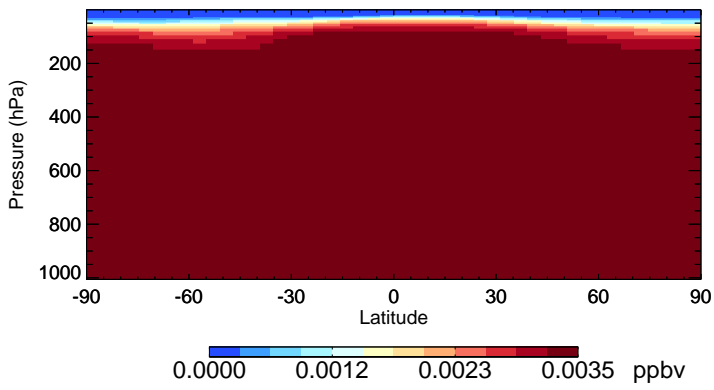
v11-02a H1301 - Species Zonal Mean for Jul
