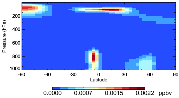
v11-02a ASOA3 - Species Zonal Mean for Jul
