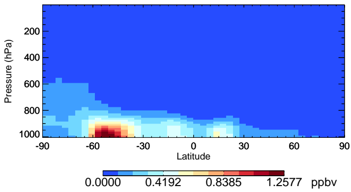
v11-02a SALA - Species Zonal Mean for Jul
