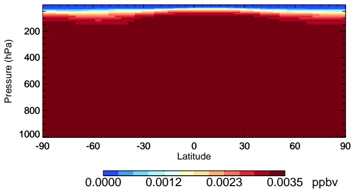
v11-01-public-Run0 H1301 - Species Zonal Mean for Jul
