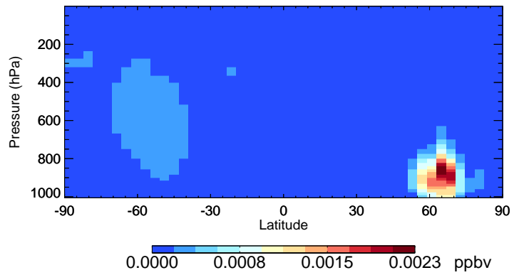
v11-02c HC187 - Species Curtain @ -180.000 for Jul
