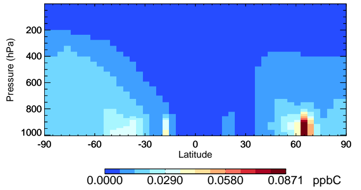
v11-01-public-Run0 ALD2 - Species Curtain @ -180.000 for Jul
