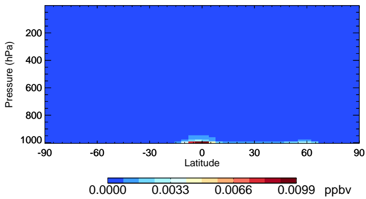
v11-02c MTPO - Species Zonal Mean for Jul
