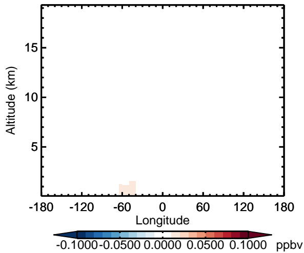
v11-02d - v11-02a IEPOXD - Diff along 15S for Apr
