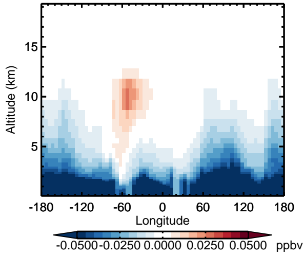
v11-02d - v11-02c MP - Diff along 15S for Apr
