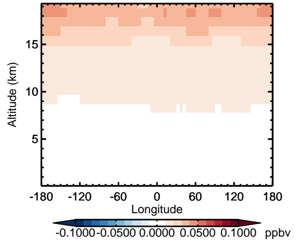
v11-02d - v11-02c CFC11 - Diff along 42N for Apr
