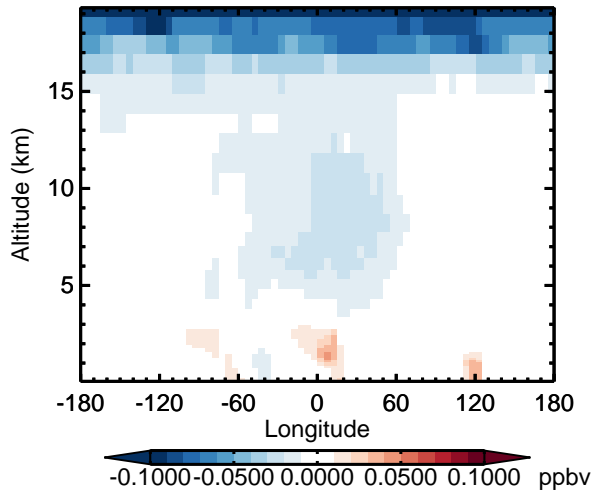
v11-02d - v11-02a HNO 3 - Diff along 15S for Apr
