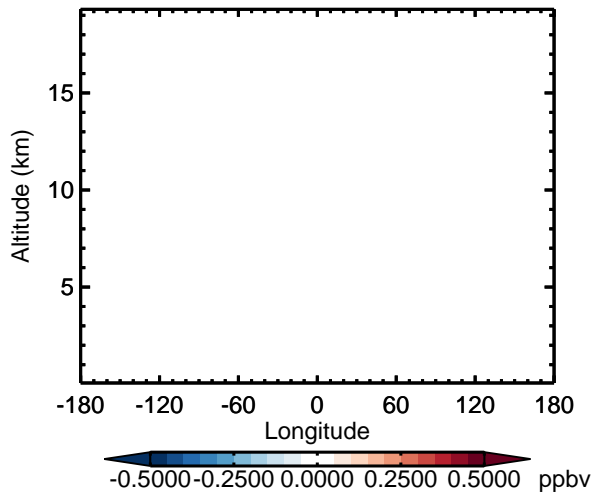
v11-02d - v11-02c CH 2 O - Diff along 15S for Apr
