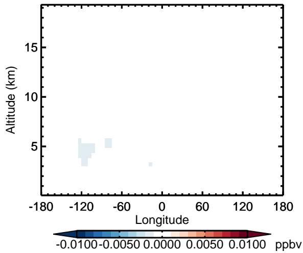
v11-02d - v11-02c HBr - Diff along 15S for Apr
