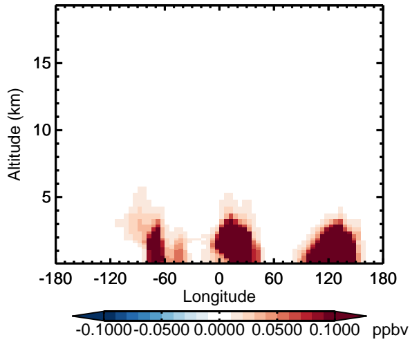
v11-02d - v11-02a SOAIE - Diff along 15S for Apr
