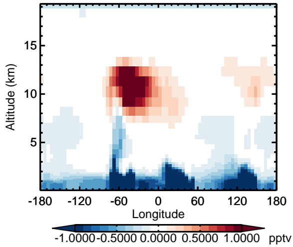
v11-02d - v11-02a HO2 - Diff along 15S for Apr
