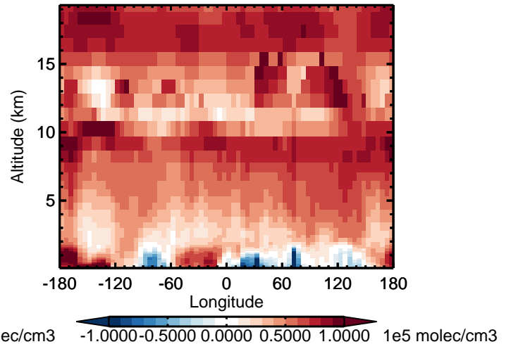
v11-02d - v11-02c OH - Diff along 42N for Apr
