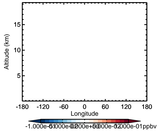
v11-02d - v11-02a MTPO - Diff along 42N for Apr
