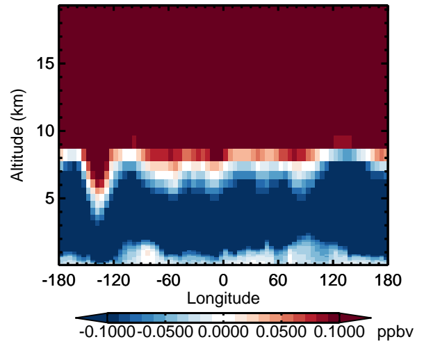
v11-02d - v11-02a CH4 - Diff along 42N for Apr
