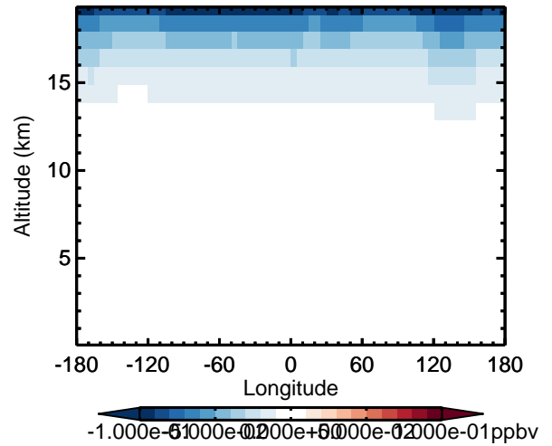
v11-02d - v11-02a N2O - Diff along 42N for Apr
