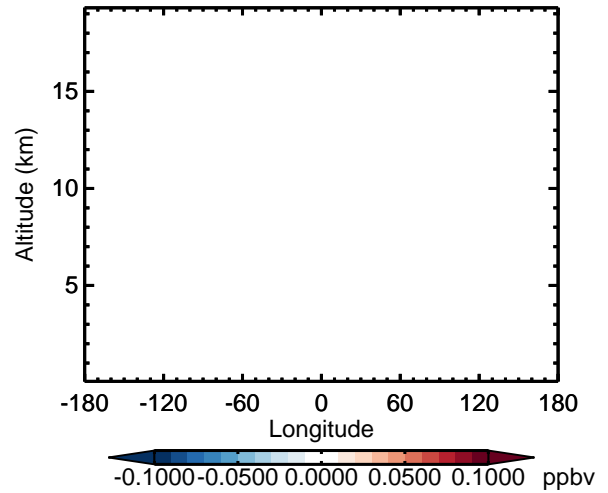
v11-02d - v11-02a HOCl - Diff along 42N for Apr
