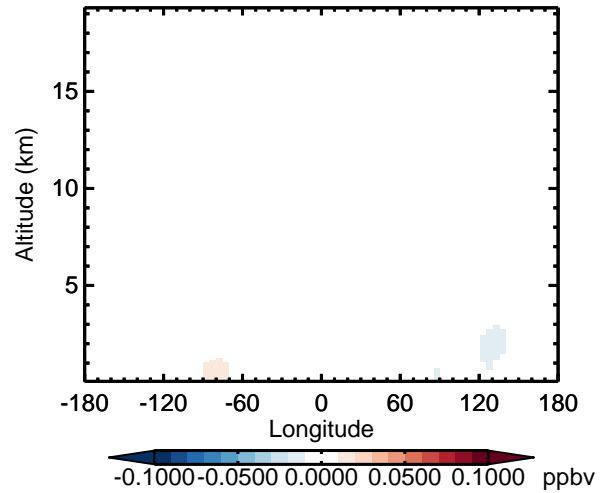
v11-02d - v11-02a MGLY - Diff along 42N for Apr
