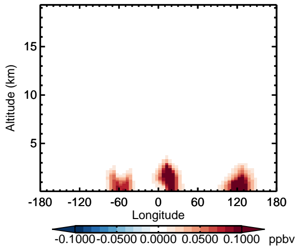
v11-02d - v11-02a INDIOL - Diff along 15S for Apr
