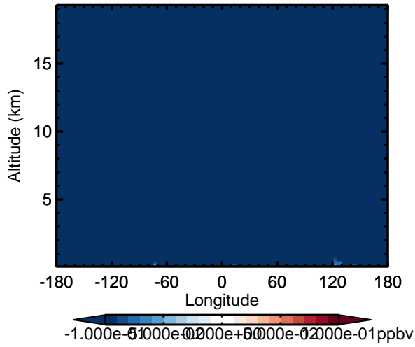
v11-02d - v11-02c CH4 - Diff along 15S for Apr
