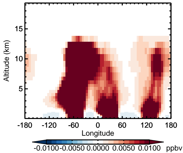
v11-02d - v11-02a MAP - Diff along 15S for Apr
