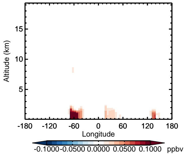
v11-02d - v11-02a RIPB - Diff along 15S for Apr
