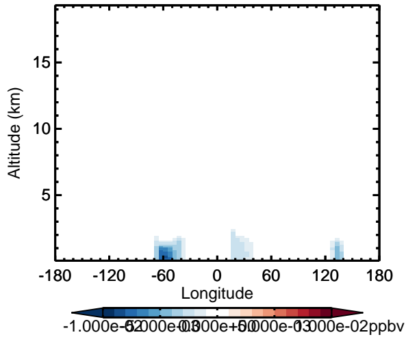
v11-02d - v11-02a MACRN - Diff along 15S for Apr
