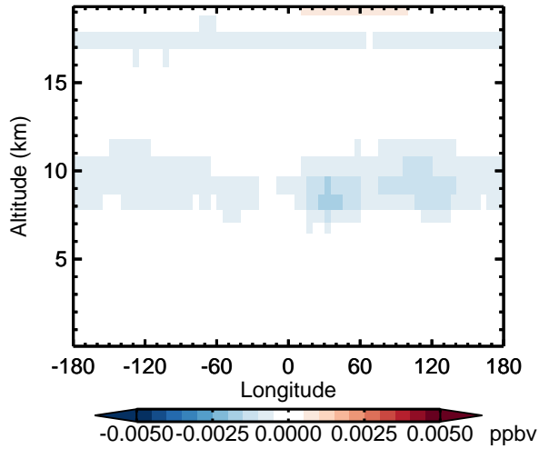
v11-02d - v11-02c HNO 4 - Diff along 15S for Apr
