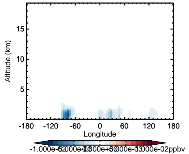
v11-02d - v11-02a MVKN - Diff along 42N for Apr
