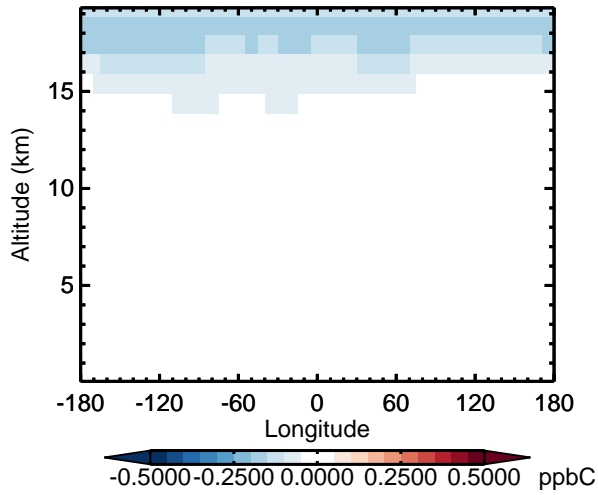
v11-02d - v11-02a C2H6 - Diff along 15S for Apr
