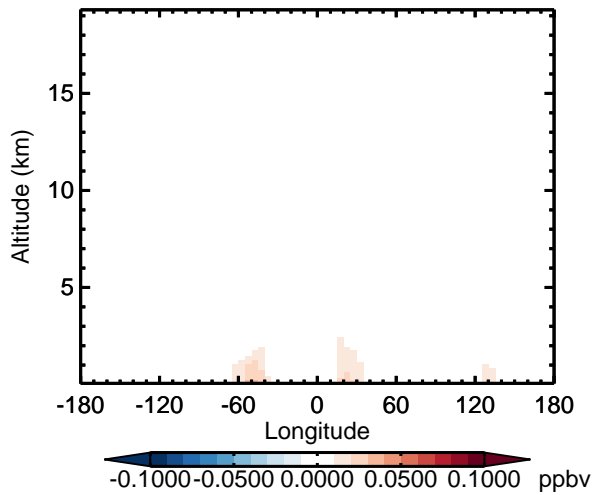
v11-02d - v11-02a MONITA - Diff along 15S for Apr
