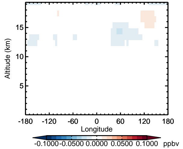
v11-02d - v11-02a CINO3 - Diff along 42N for Apr
