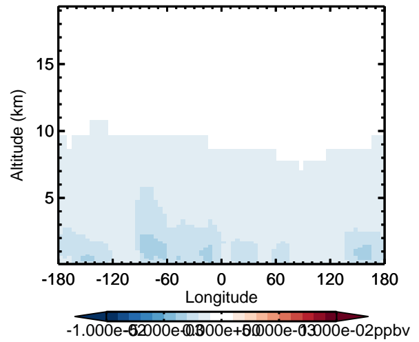
v11-02d - v11-02c MAP - Diff along 42N for Apr
