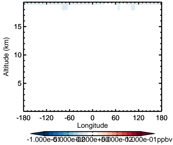
v11-02d - v11-02c CINO3 - Diff along 15S for Apr
