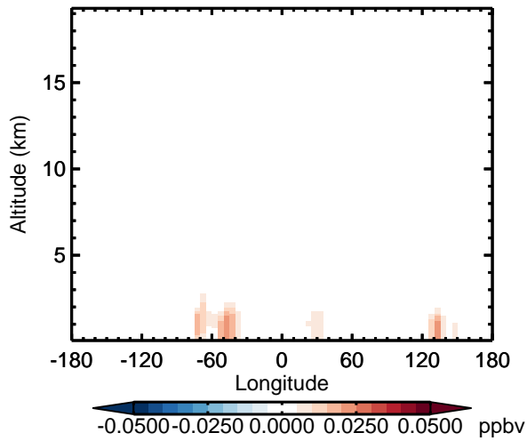
v11-02d - v11-02c MVK - Diff along 15S for Apr
