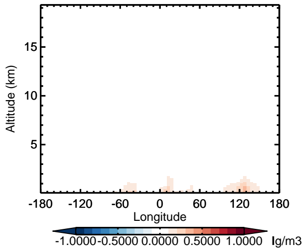
v11-02d - v11-02a NH4 - Diff along 15S for Apr
