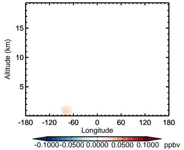
v11-02d - v11-02c INDIOL - Diff along 42N for Apr
