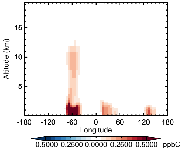
v11-02d - v11-02a ALD2 - Diff along 15S for Apr
