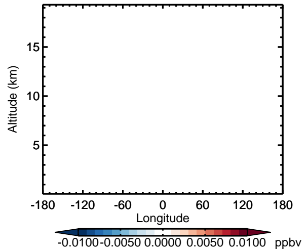
v11-02d - v11-02c Br2 - Diff along 42N for Apr
