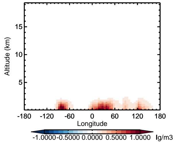
v11-02d - v11-02a NH4 - Diff along 42N for Apr
