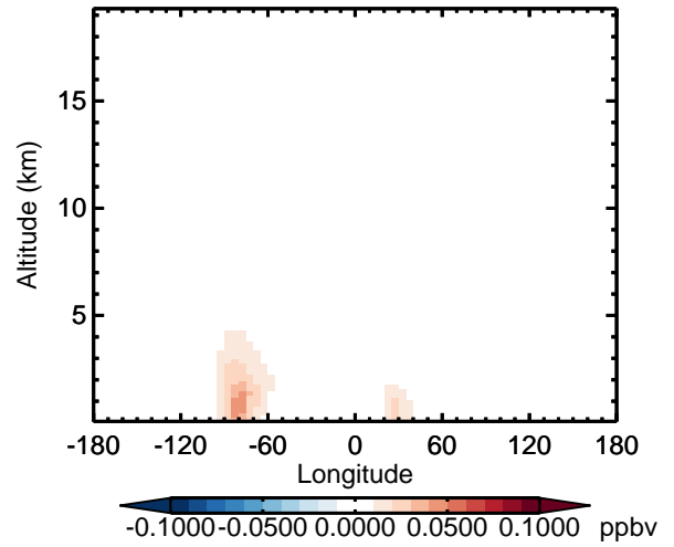
v11-02d - v11-02a SOAIE - Diff along 42N for Apr
