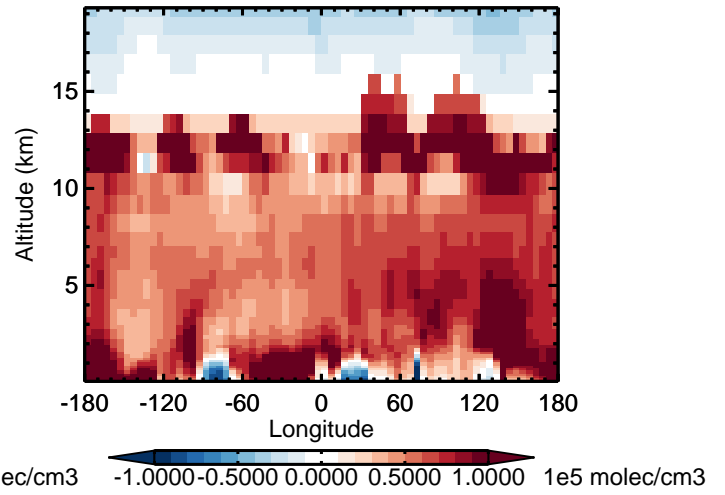
v11-02d - v11-02a OH - Diff along 42N for Apr
