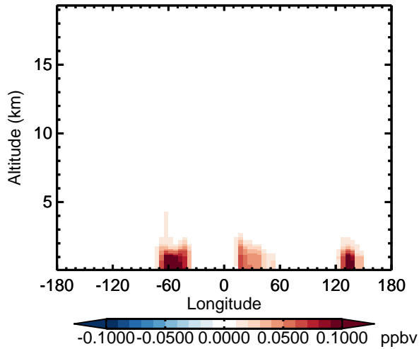
v11-02d - v11-02a MGLY - Diff along 15S for Apr
