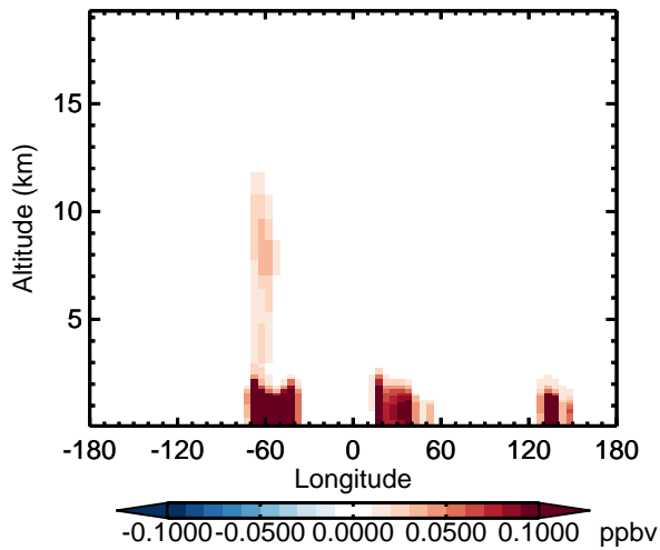
v11-02d - v11-02a RIPA - Diff along 15S for Apr
