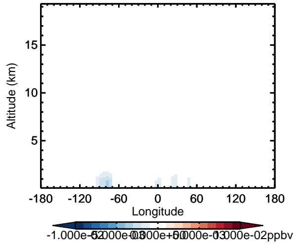
v11-02d - v11-02a NPMN - Diff along 42N for Apr
