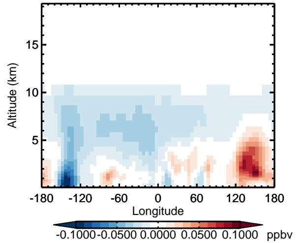
v11-02d - v11-02c H2O2 - Diff along 42N for Apr
