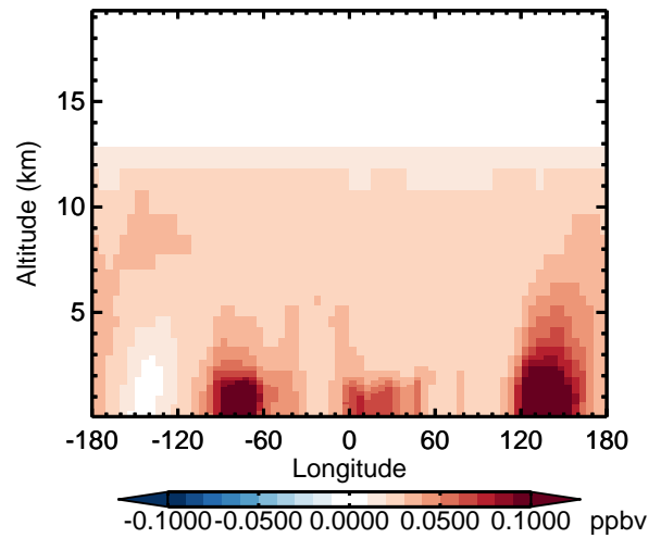
v11-02d - v11-02a PAN - Diff along 42N for Apr
