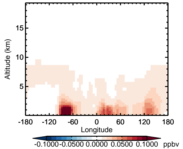
v11-02d - v11-02a INDIOL - Diff along 42N for Apr
