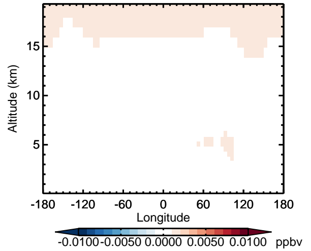
v11-02d - v11-02a BrNO 3 - Diff along 42N for Apr
