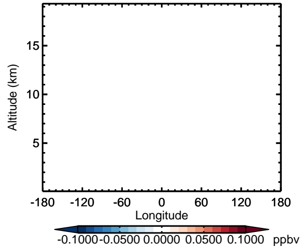
v11-02d - v11-02c ISOG3 - Diff along 42N for Apr
