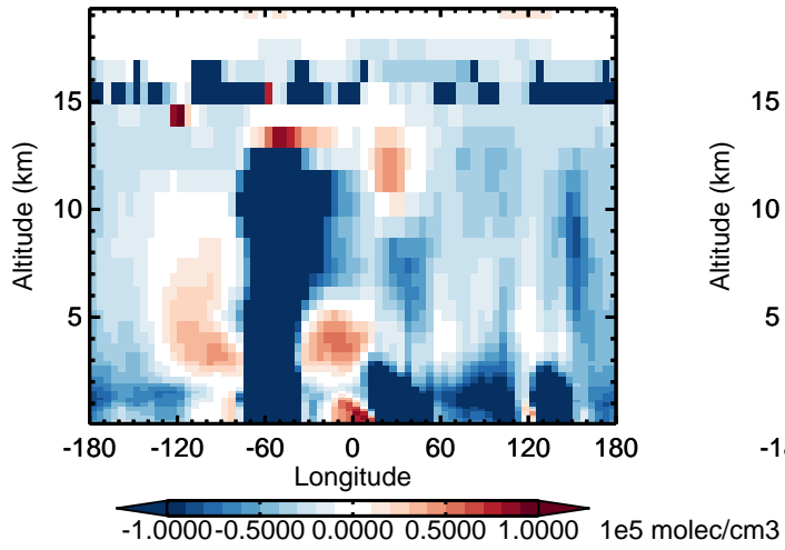
v11-02d - v11-02a OH - Diff along 15S for Apr
