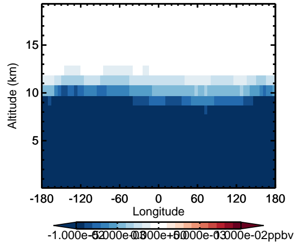
v11-02d - v11-02a R4N2 - Diff along 42N for Apr
