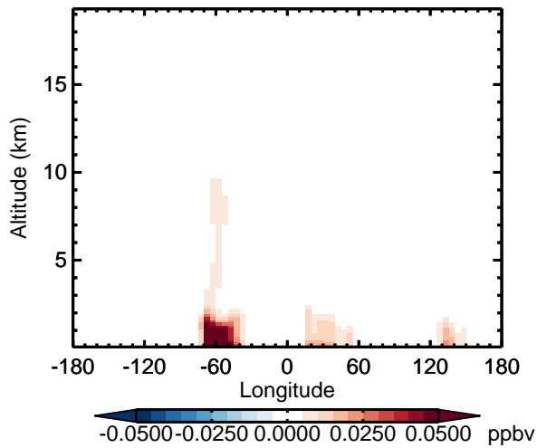
v11-02d - v11-02a RCHO - Diff along 15S for Apr
