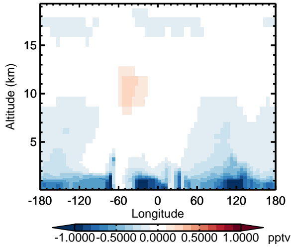
v11-02d - v11-02c HO2 - Diff along 15S for Apr
