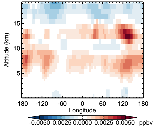
v11-02d - v11-02c HNO 4 - Diff along 42N for Apr
