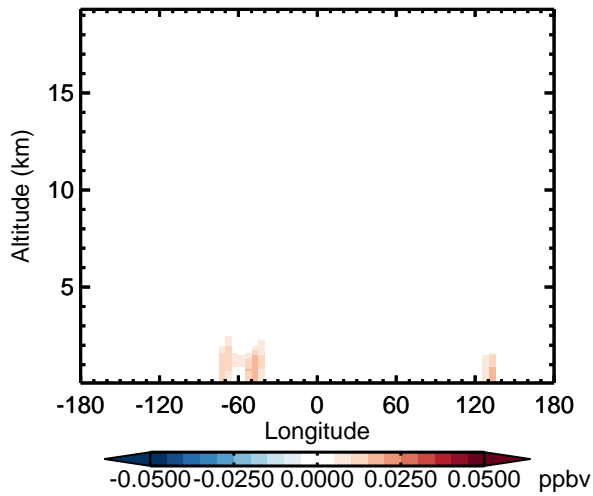
v11-02d - v11-02c MACR - Diff along 15S for Apr
