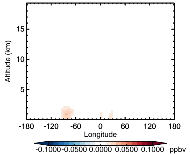
v11-02d - v11-02a IMAE - Diff along 42N for Apr
