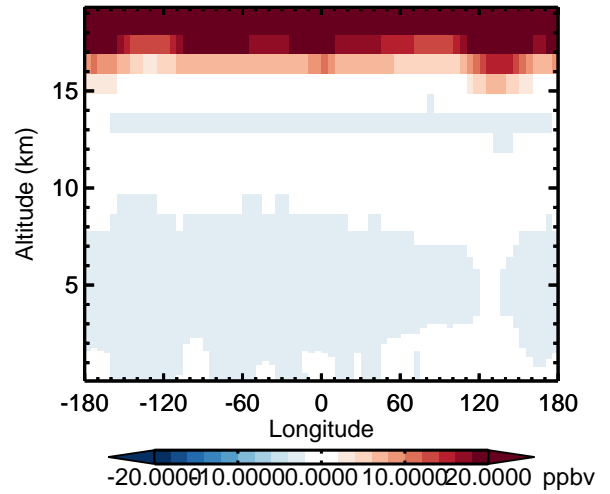
v11-02d - v11-02c O3 - Diff along 42N for Apr
