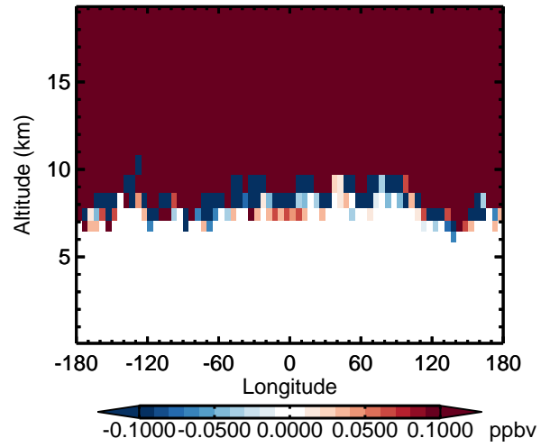
v11-02d - v11-02c H 2 O - Diff along 42N for Apr
