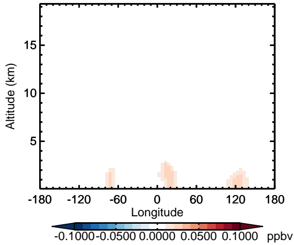
v11-02d - v11-02a SOAME - Diff along 15S for Apr
