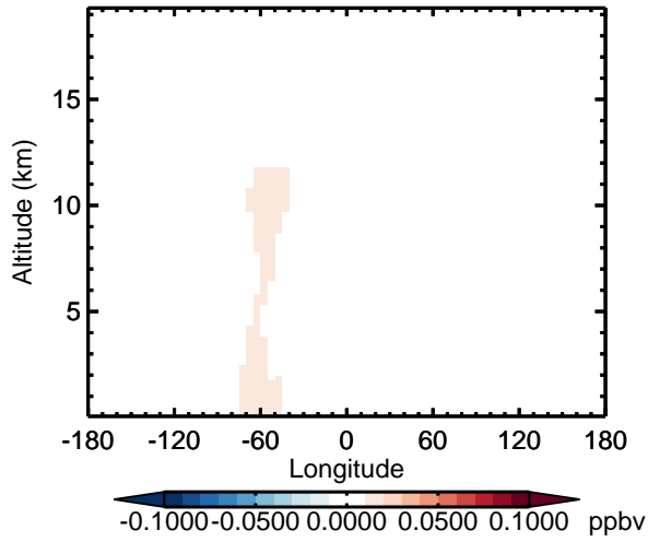
v11-02d - v11-02c EOH - Diff along 15S for Apr
