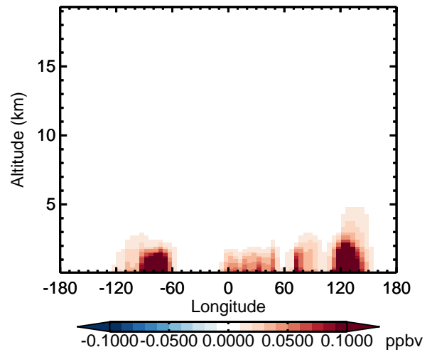
v11-02d - v11-02a SOAP - Diff along 42N for Apr
