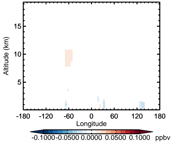
v11-02d - v11-02c IEPOXB - Diff along 15S for Apr
