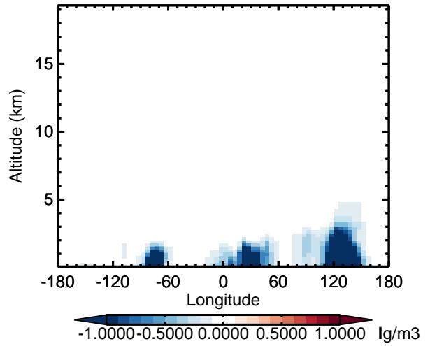
v11-02d - v11-02a NIT - Diff along 42N for Apr
