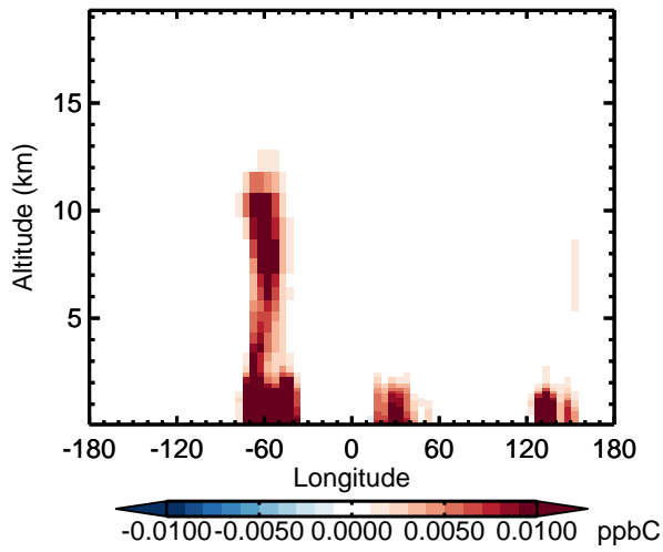
v11-02d - v11-02c PRPE - Diff along 15S for Apr
