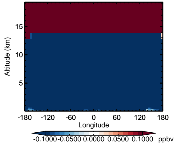
v11-02d - v11-02c N2O - Diff along 42N for Apr
