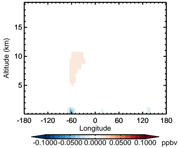
v11-02d - v11-02a ISOG3 - Diff along 15S for Apr
