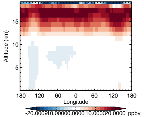
v11-02d - v11-02a O3 - Diff along 42N for Apr
