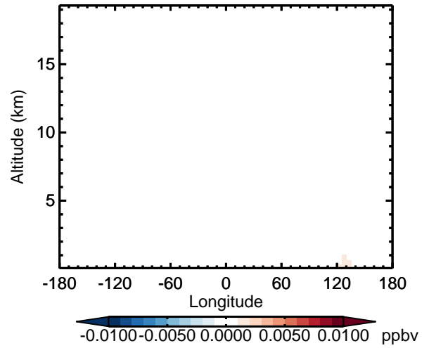
v11-02d - v11-02a NO 3 - Diff along 42N for Apr
