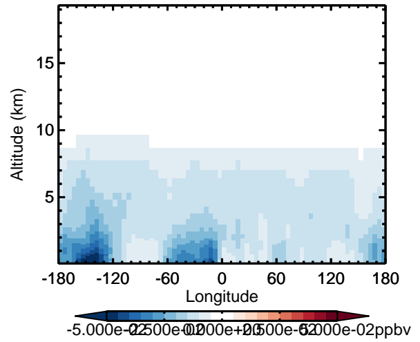
v11-02d - v11-02a MP - Diff along 42N for Apr
