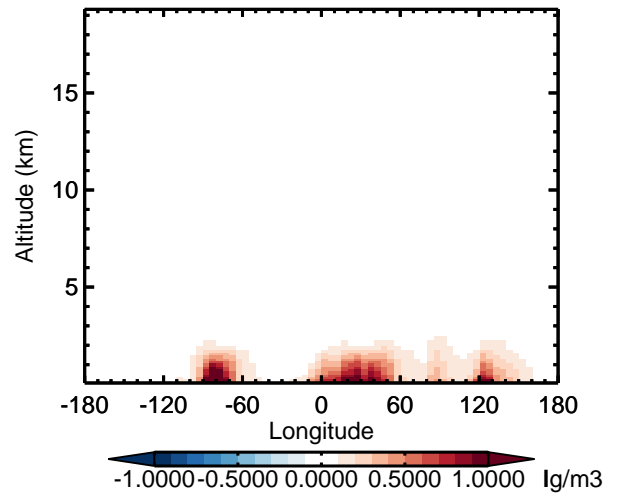
v11-02d - v11-02c NH4 - Diff along 42N for Apr
