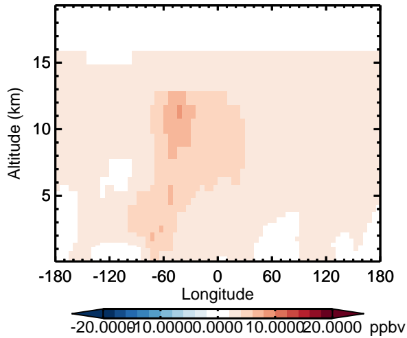
v11-02d - v11-02a CO - Diff along 15S for Apr
