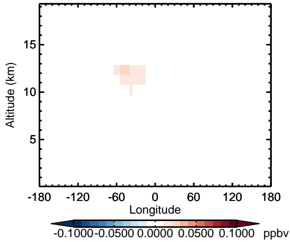
v11-02d - v11-02a MPN - Diff along 15S for Apr
