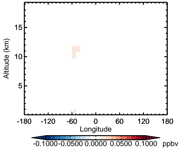
v11-02d - v11-02a TSOA2 - Diff along 15S for Apr
