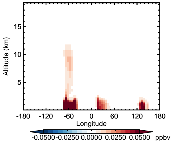
v11-02d - v11-02a MACR - Diff along 15S for Apr
