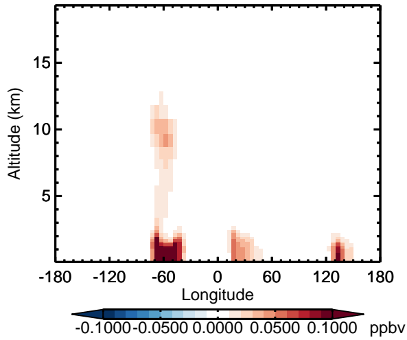
v11-02d - v11-02a IPMN - Diff along 15S for Apr
