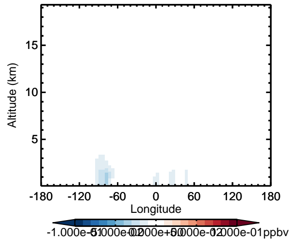
v11-02d - v11-02a HAC - Diff along 42N for Apr
