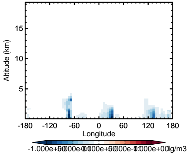
v11-02d - v11-02c SO 2 - Diff along 15S for Apr
