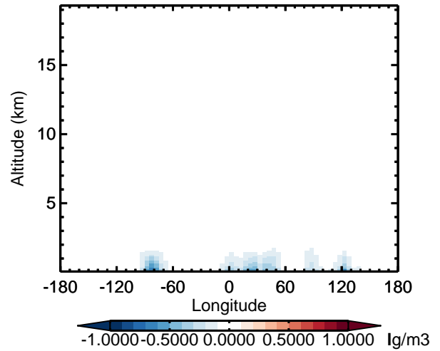
v11-02d - v11-02a NH3 - Diff along 42N for Apr
