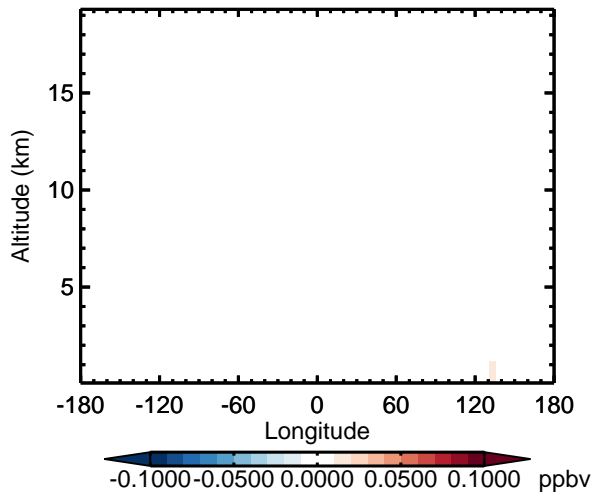
v11-02d - v11-02c HPALD - Diff along 15S for Apr
