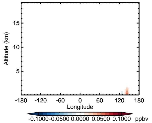
v11-02d - v11-02c XYLE - Diff along 42N for Apr
