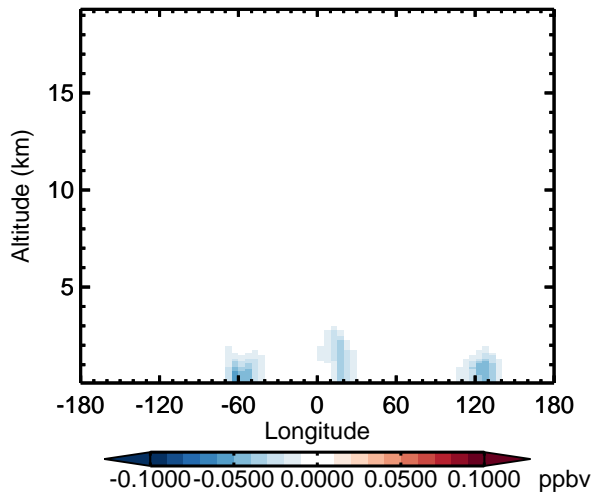
v11-02d - v11-02c SOAGX - Diff along 15S for Apr
