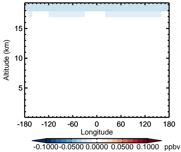
v11-02d - v11-02c PAN - Diff along 15S for Apr
