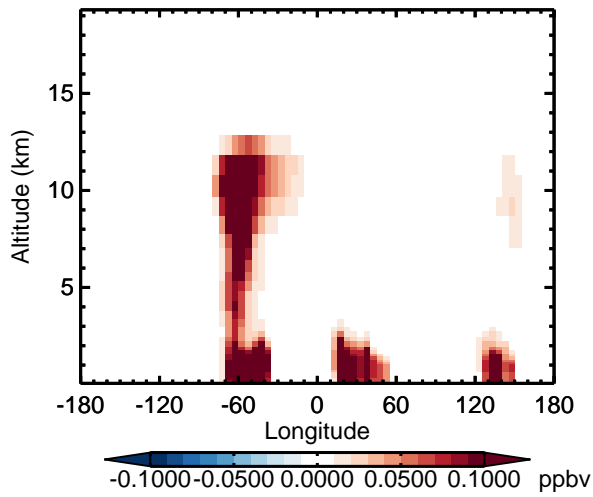
v11-02d - v11-02a IEPOXA - Diff along 15S for Apr
