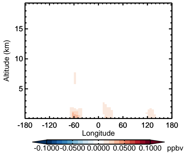
v11-02d - v11-02a TSOG2 - Diff along 15S for Apr
