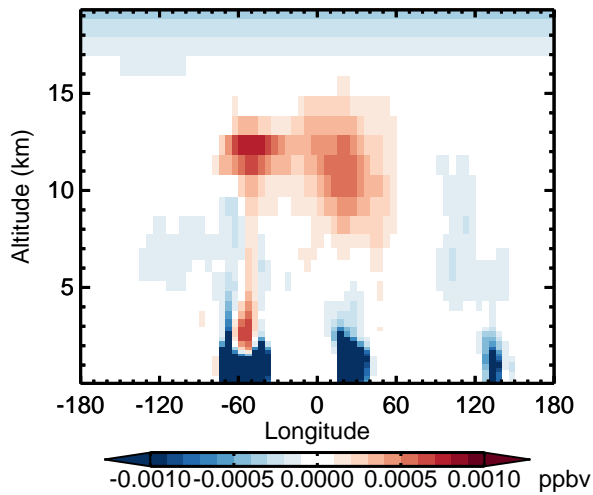
v11-02d - v11-02a PPN - Diff along 15S for Apr
