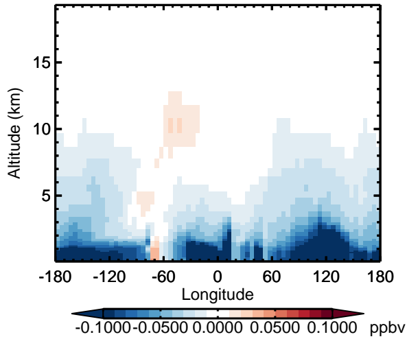
v11-02d - v11-02c H2O2 - Diff along 15S for Apr
