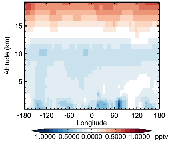
v11-02d - v11-02c HO2 - Diff along 42N for Apr
