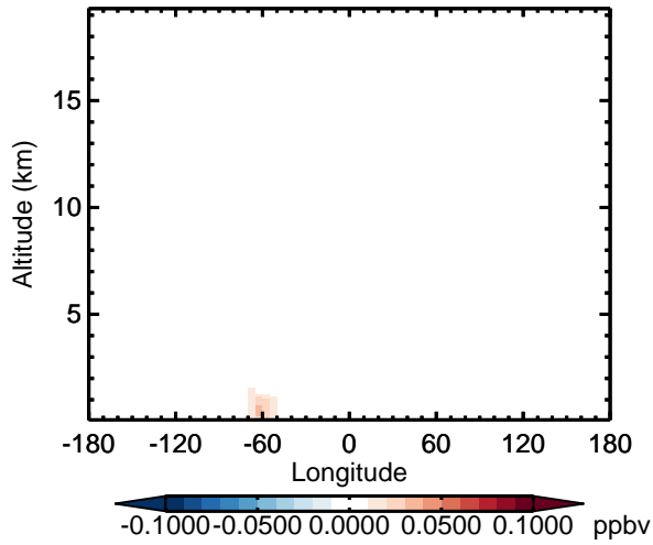
v11-02d - v11-02a RIPD - Diff along 15S for Apr
