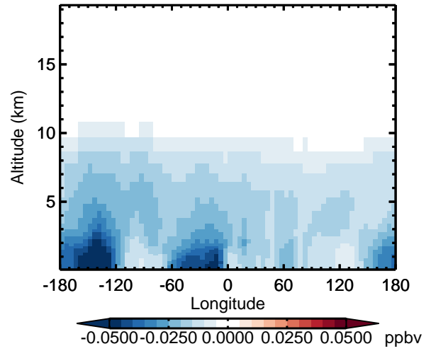
v11-02d - v11-02c MP - Diff along 42N for Apr
