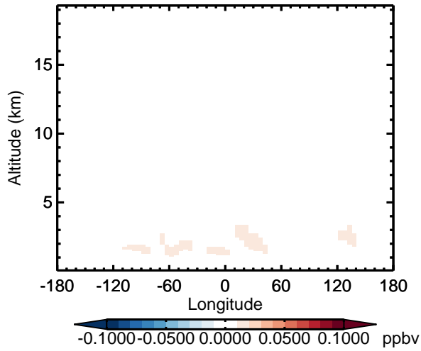
v11-02d - v11-02a CH3Cl - Diff along 15S for Apr
