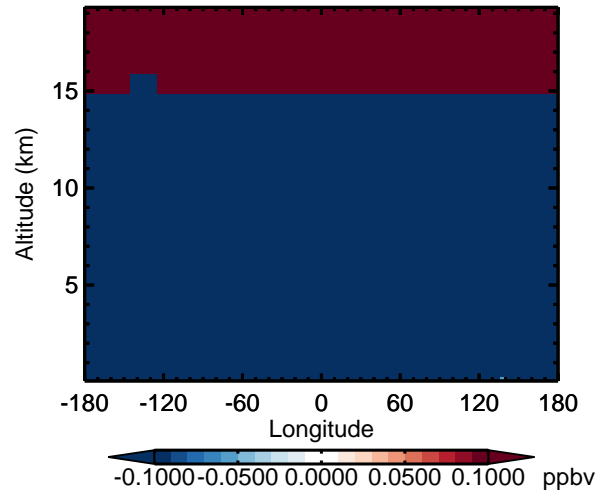
v11-02d - v11-02c CH4 - Diff along 42N for Apr
