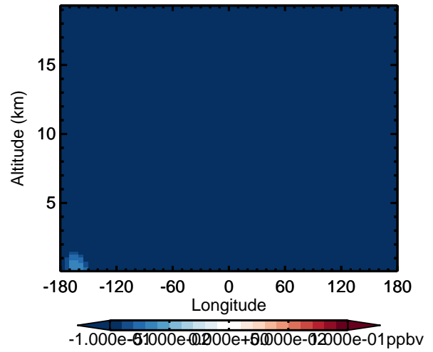
v11-02d - v11-02a EOH - Diff along 42N for Apr
