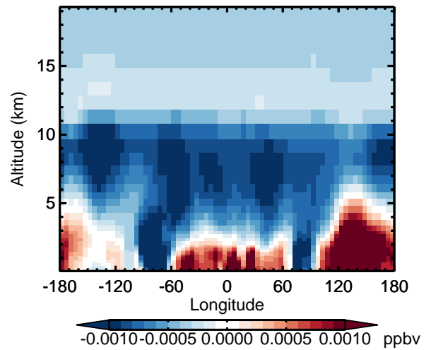
v11-02d - v11-02a PPN - Diff along 42N for Apr
