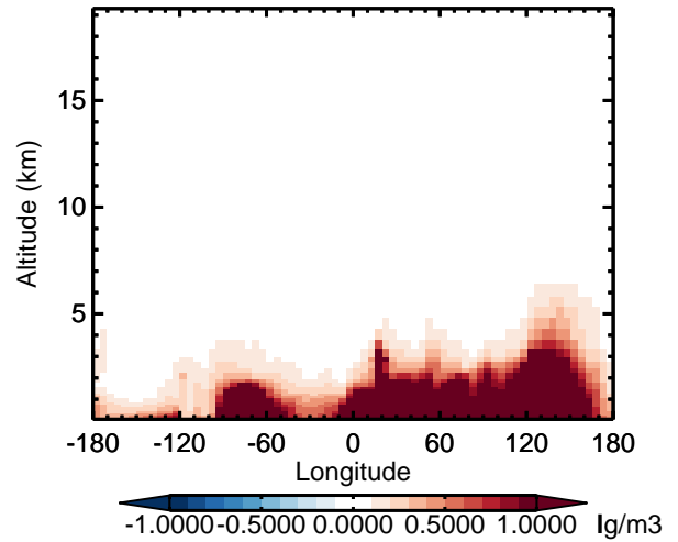
v11-02d - v11-02a SO4 - Diff along 42N for Apr
