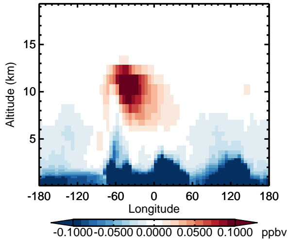
v11-02d - v11-02a H2O2 - Diff along 15S for Apr
