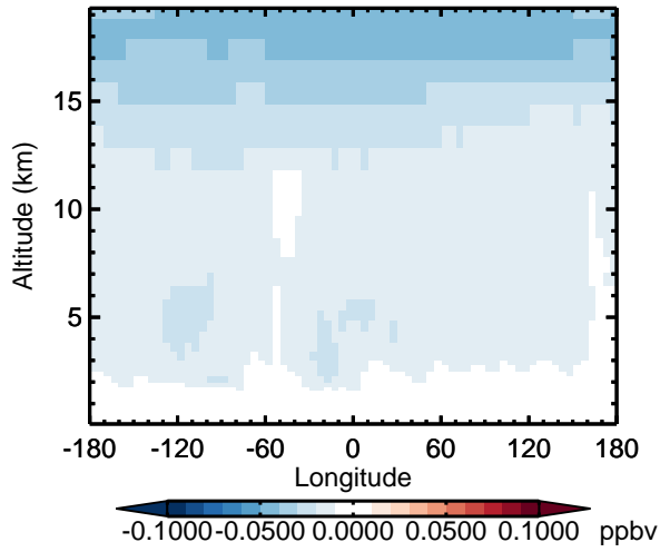
v11-02d - v11-02c CH3Cl - Diff along 15S for Apr
