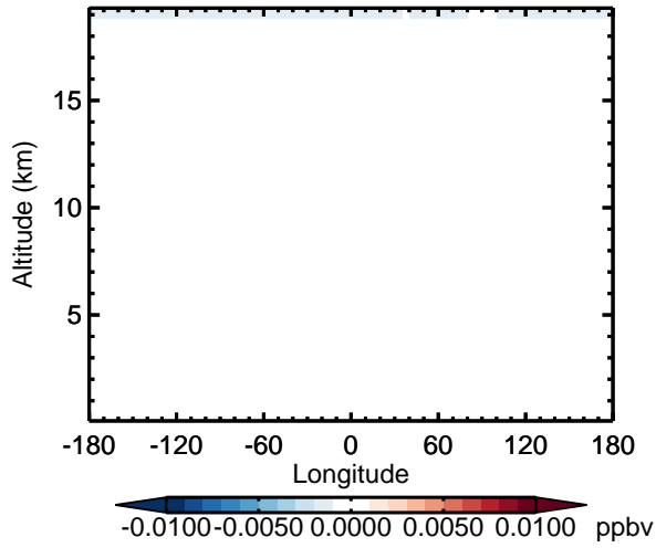
v11-02d - v11-02c BrNO 3 - Diff along 15S for Apr
