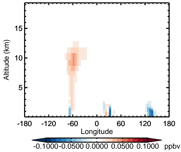
v11-02d - v11-02c IEPOXA - Diff along 15S for Apr
