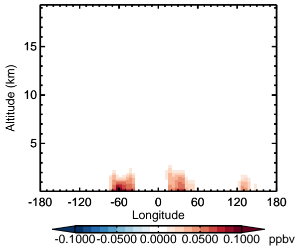
v11-02d - v11-02a SOAP - Diff along 15S for Apr
