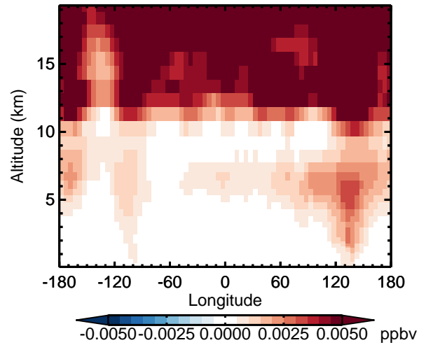
v11-02d - v11-02a HNO 4 - Diff along 42N for Apr
