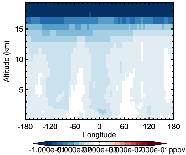
v11-02d - v11-02c HCl - Diff along 15S for Apr
