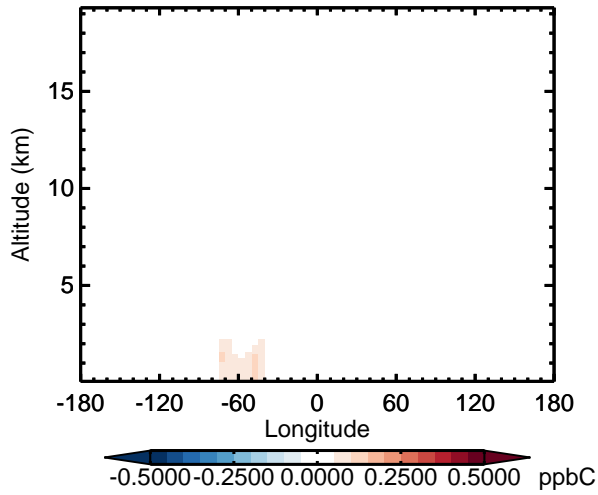
v11-02d - v11-02a ALK4 - Diff along 15S for Apr
