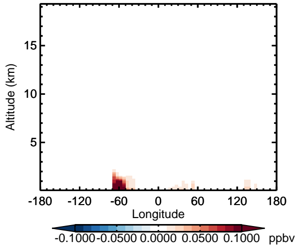
v11-02d - v11-02a MTPA - Diff along 15S for Apr
