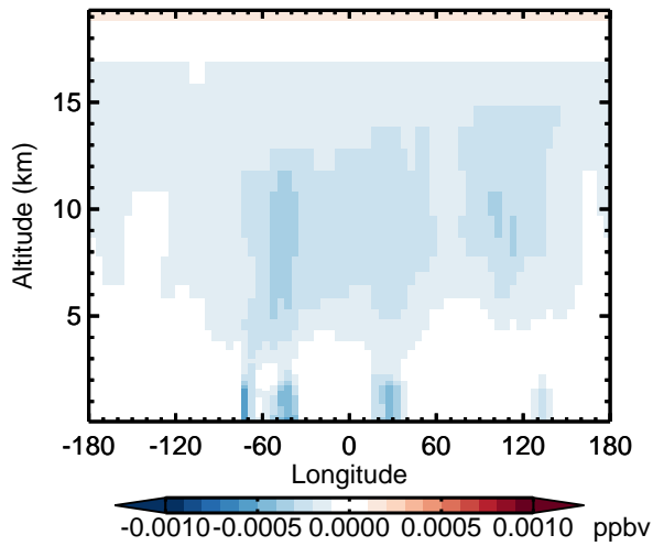
v11-02d - v11-02c PPN - Diff along 15S for Apr
