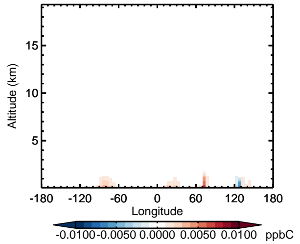
v11-02d - v11-02c PRPE - Diff along 42N for Apr
