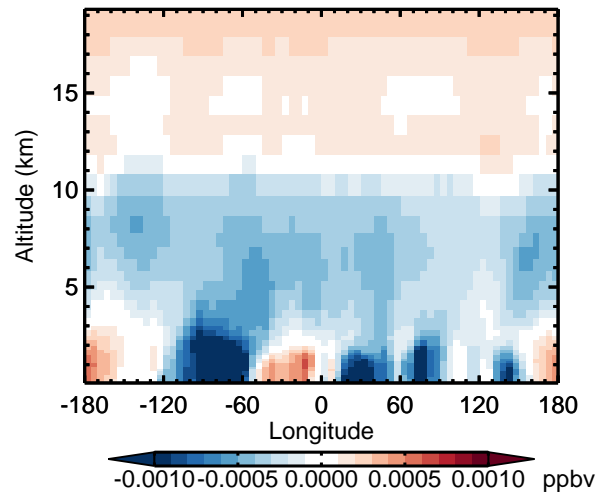
v11-02d - v11-02c PPN - Diff along 42N for Apr
