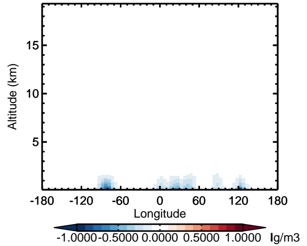
v11-02d - v11-02c NH3 - Diff along 42N for Apr
