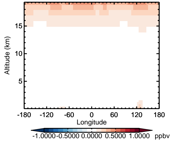
v11-02d - v11-02a NO 2 - Diff along 42N for Apr
