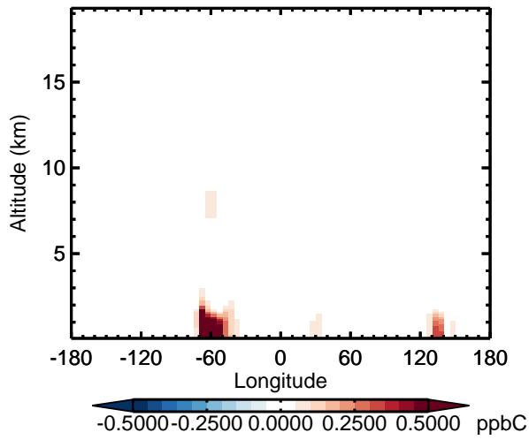
v11-02d - v11-02c ISOP - Diff along 15S for Apr
