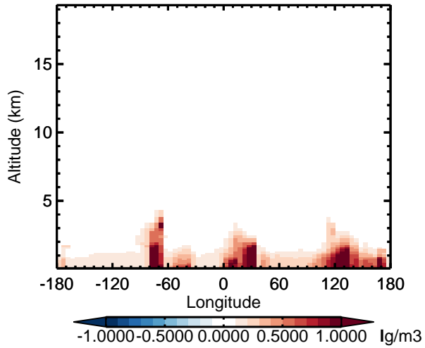
v11-02d - v11-02c SO4 - Diff along 15S for Apr
