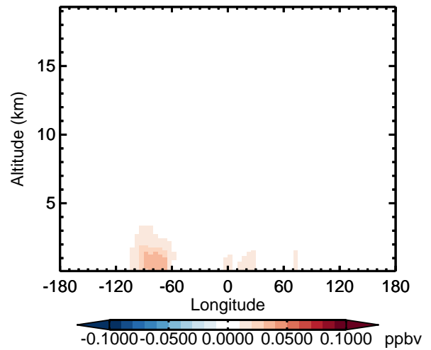
v11-02d - v11-02a IONITA - Diff along 42N for Apr
