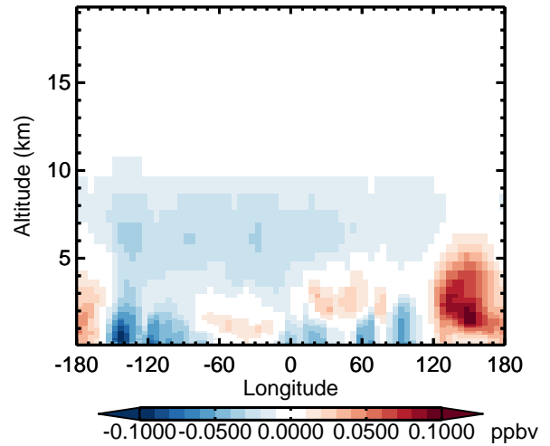
v11-02d - v11-02a H2O2 - Diff along 42N for Apr
