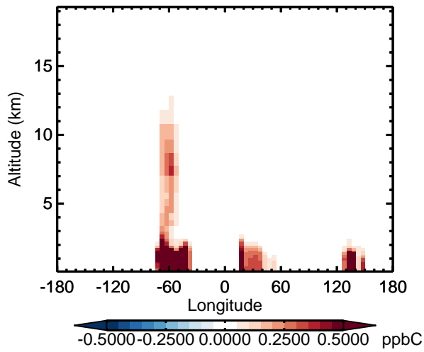
v11-02d - v11-02a ISOP - Diff along 15S for Apr
