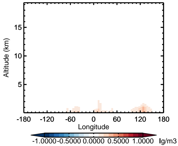
v11-02d - v11-02c NH4 - Diff along 15S for Apr
