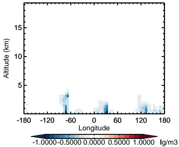
v11-02d - v11-02a SO 2 - Diff along 15S for Apr
