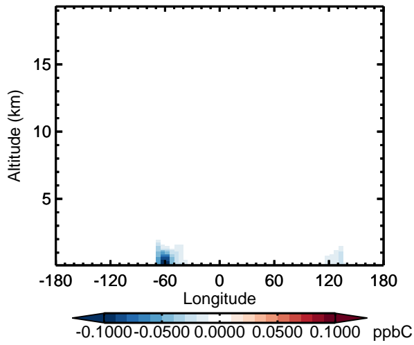
v11-02d - v11-02c MEK - Diff along 15S for Apr
