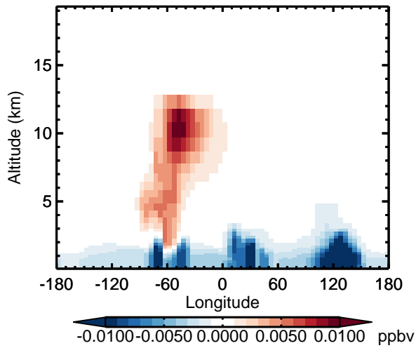
v11-02d - v11-02c MAP - Diff along 15S for Apr
