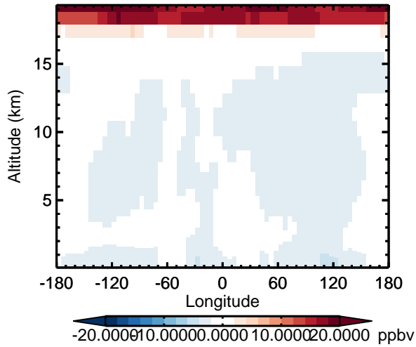
v11-02d - v11-02c O3 - Diff along 15S for Apr
