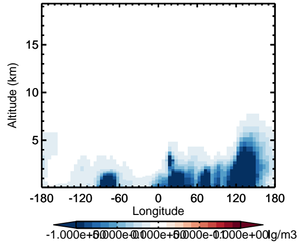
v11-02d - v11-02c SO 2 - Diff along 42N for Apr
