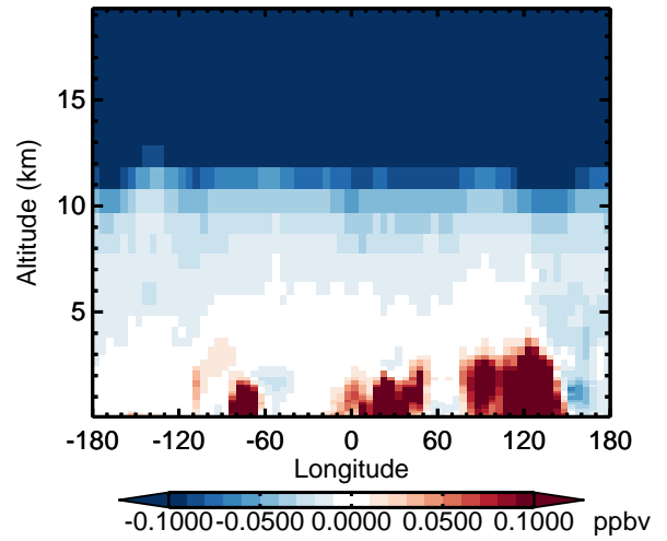
v11-02d - v11-02a HNO 3 - Diff along 42N for Apr
