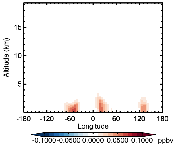
v11-02d - v11-02a IONITA - Diff along 15S for Apr
