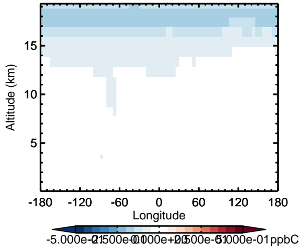
v11-02d - v11-02c C2H6 - Diff along 15S for Apr
