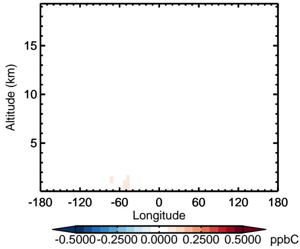
v11-02d - v11-02c ALD2 - Diff along 15S for Apr
