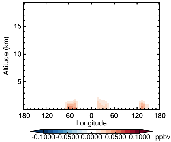
v11-02d - v11-02a GLYX - Diff along 15S for Apr
