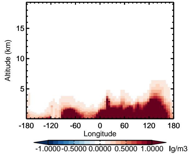
v11-02d - v11-02c SO4 - Diff along 42N for Apr
