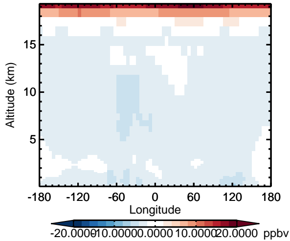
v11-02d - v11-02a O3 - Diff along 15S for Apr
