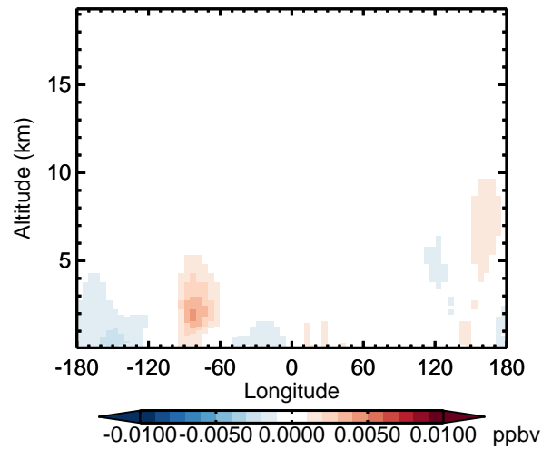
v11-02d - v11-02a MAP - Diff along 42N for Apr
