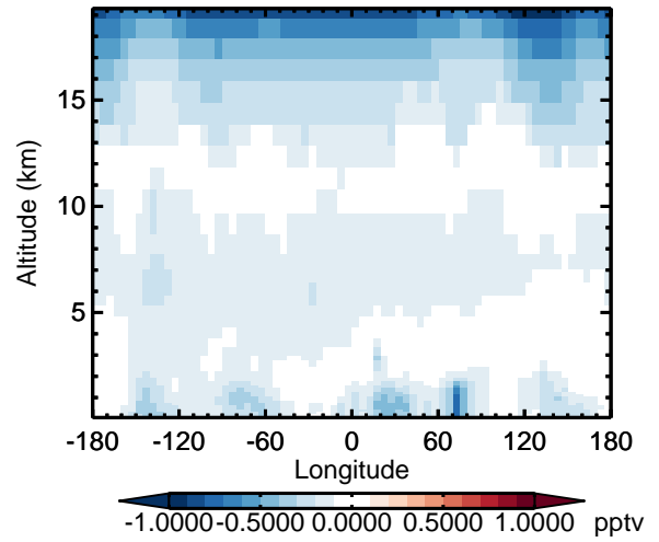
v11-02d - v11-02a HO2 - Diff along 42N for Apr
