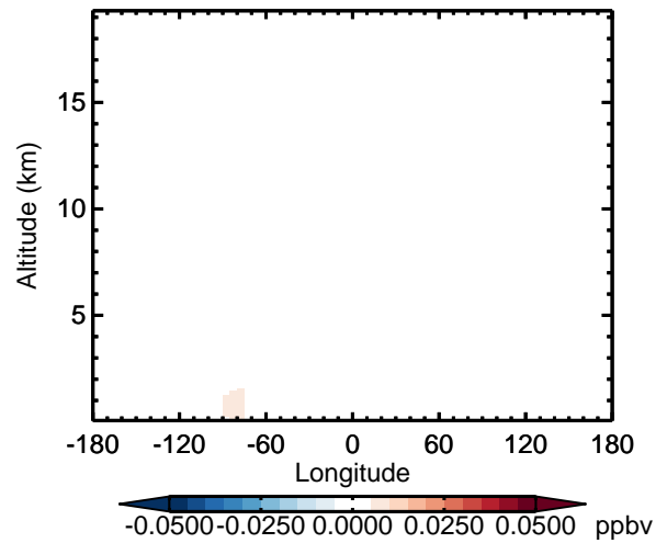
v11-02d - v11-02a MVK - Diff along 42N for Apr
