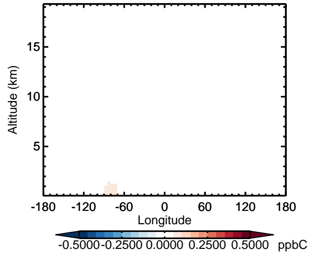
v11-02d - v11-02a ALD2 - Diff along 42N for Apr
