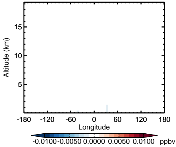
v11-02d - v11-02c R4N2 - Diff along 15S for Apr
