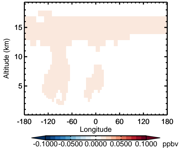
v11-02d - v11-02c CFC11 - Diff along 15S for Apr
