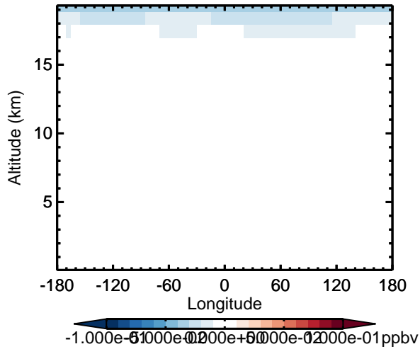
v11-02d - v11-02a N2O - Diff along 15S for Apr
