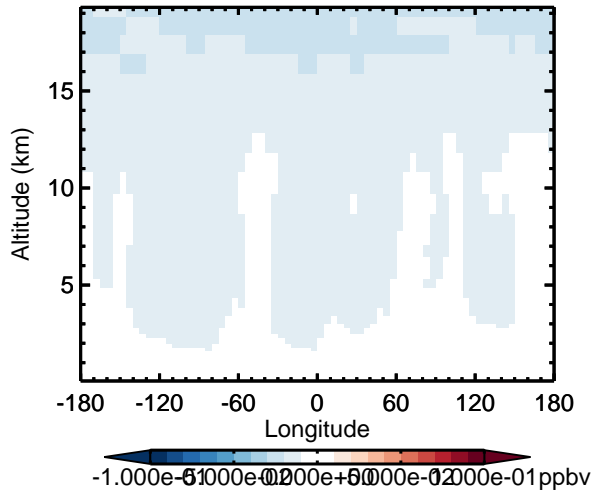
v11-02d - v11-02c OCS - Diff along 15S for Apr
