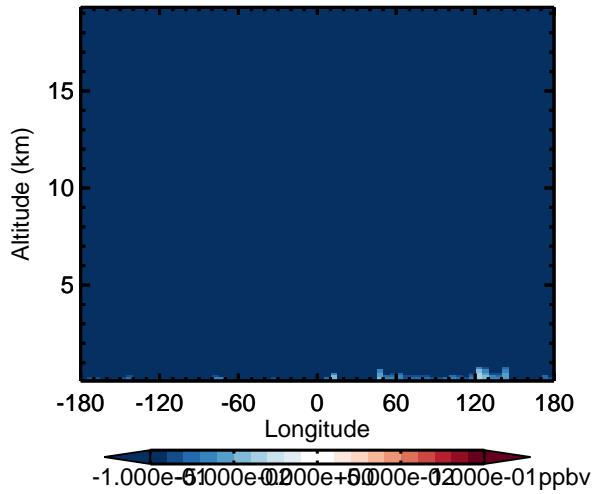
v11-02d - v11-02c N2O - Diff along 15S for Apr
