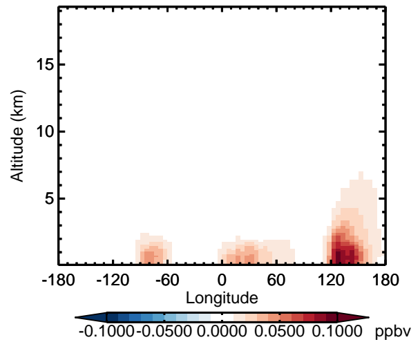
v11-02d - v11-02a SOAGX - Diff along 42N for Apr
