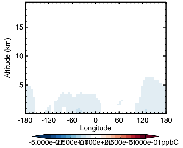
v11-02d - v11-02c ALK4 - Diff along 42N for Apr
