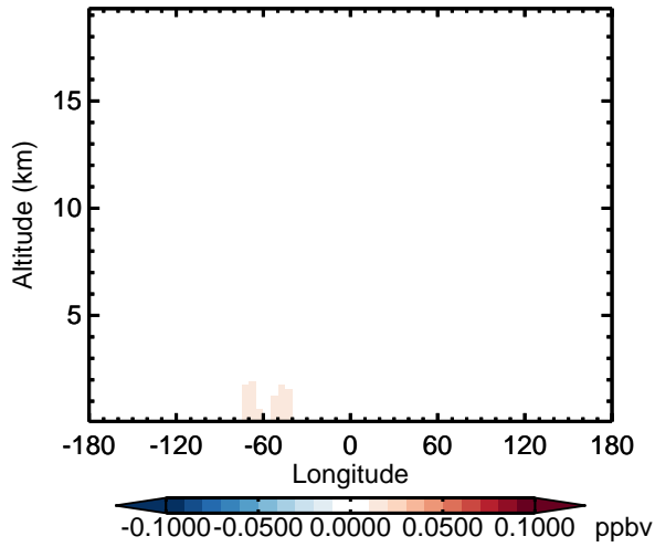
v11-02d - v11-02a TOLU - Diff along 15S for Apr
