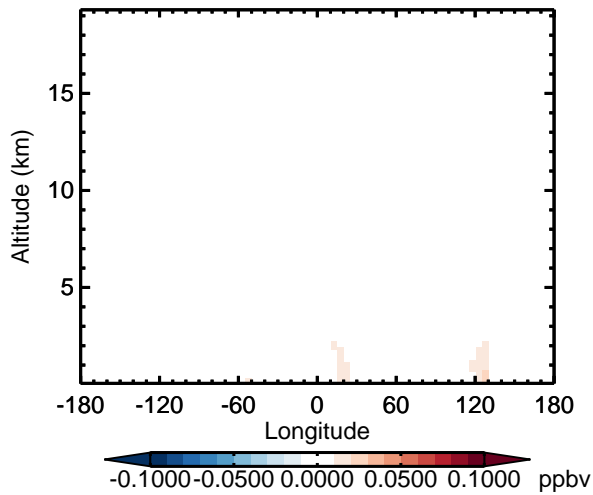
v11-02d - v11-02a TSOG3 - Diff along 15S for Apr
