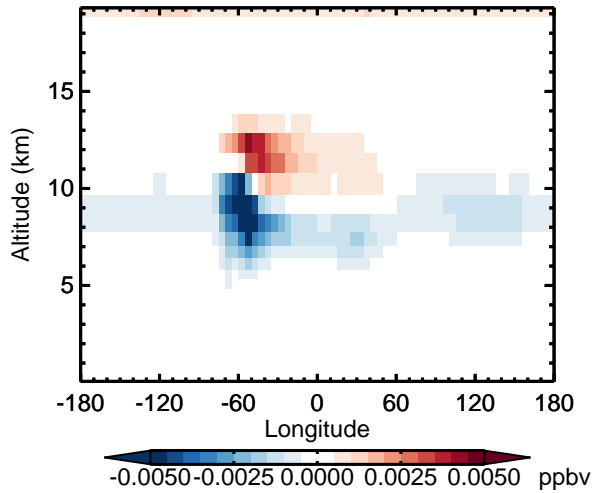
v11-02d - v11-02a HNO 4 - Diff along 15S for Apr
