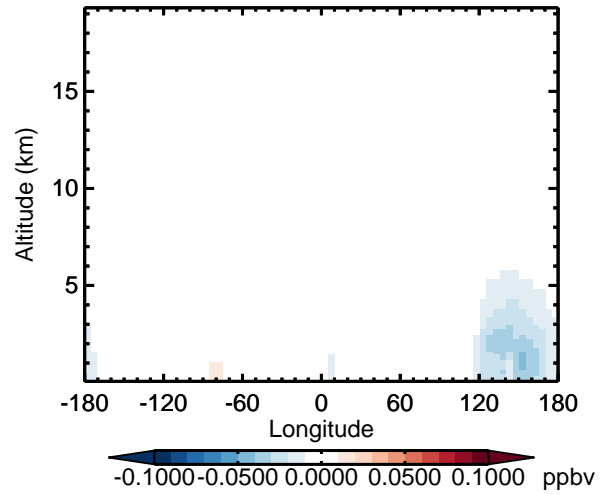
v11-02d - v11-02a TOLU - Diff along 42N for Apr
