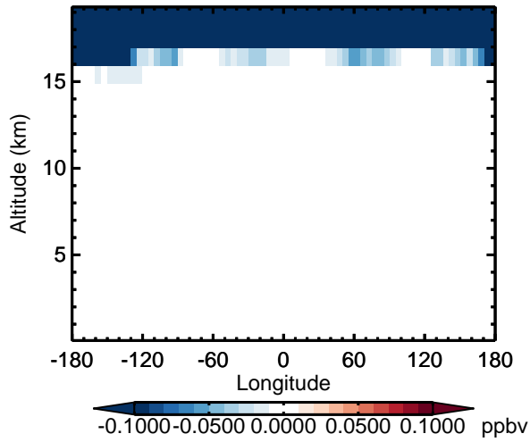
v11-02d - v11-02a H 2 O - Diff along 15S for Apr
