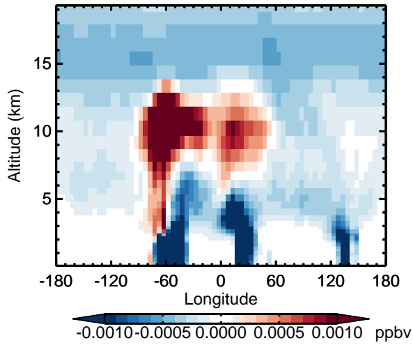
v11-02d - v11-02a PPN - Diff along 15S for Oct
