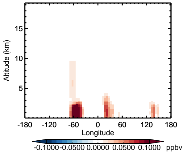
v11-02d - v11-02a IEPOXB - Diff along 15S for Oct
