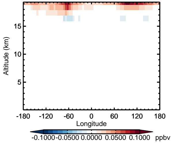
v11-02d - v11-02c CINO3 - Diff along 15S for Oct
