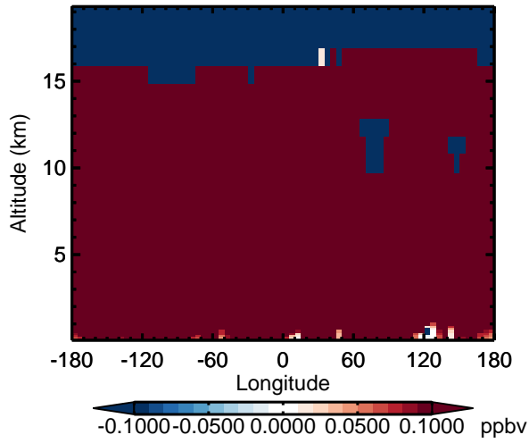
v11-02d - v11-02c CH4 - Diff along 15S for Oct
