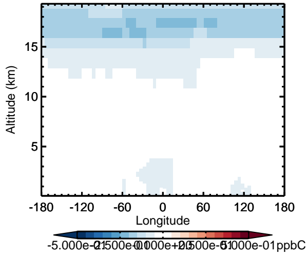
v11-02d - v11-02c C2H6 - Diff along 15S for Oct
