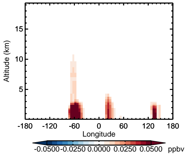
v11-02d - v11-02a MACR - Diff along 15S for Oct
