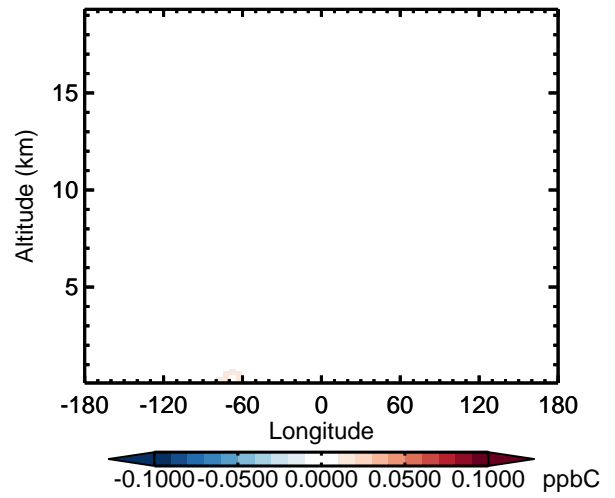
v11-02d - v11-02c MEK - Diff along 42N for Oct
