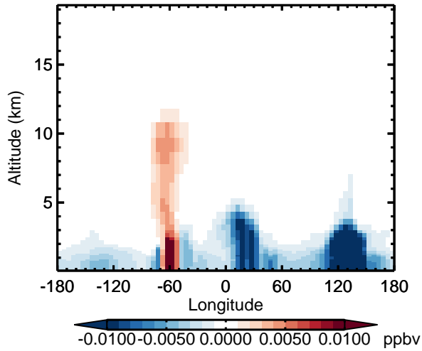
v11-02d - v11-02c MAP - Diff along 15S for Oct
