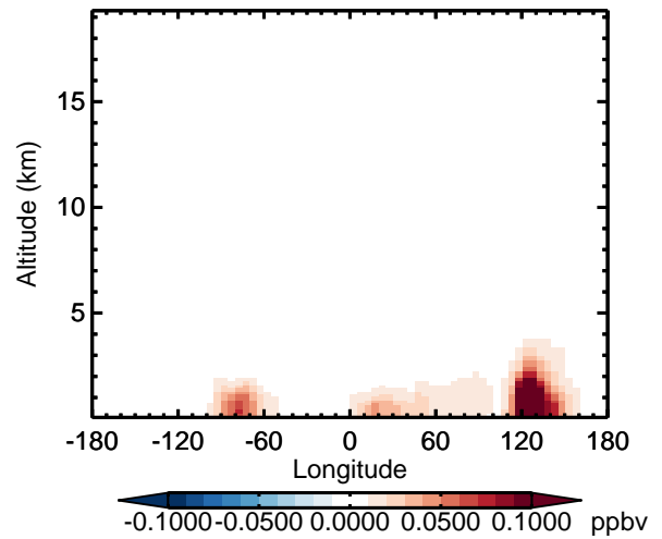
v11-02d - v11-02a SOAGX - Diff along 42N for Oct
