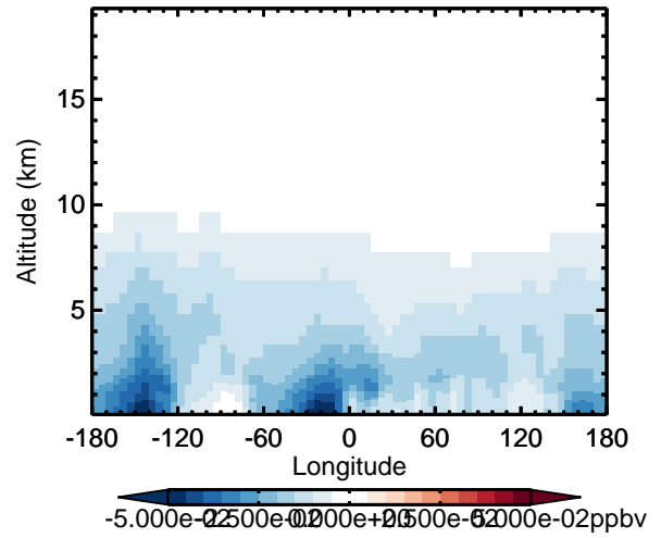
v11-02d - v11-02a MP - Diff along 42N for Oct
