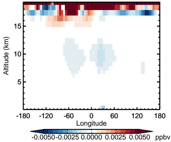
v11-02d - v11-02c N2O5 - Diff along 15S for Oct
