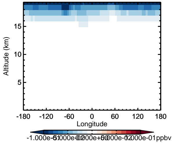
v11-02d - v11-02a N2O - Diff along 15S for Oct
