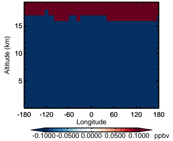
v11-02d - v11-02c CH4 - Diff along 42N for Oct
