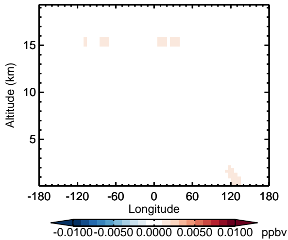
v11-02d - v11-02a BrNO 3 - Diff along 15S for Oct
