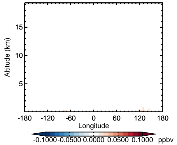
v11-02d - v11-02a GLYX - Diff along 42N for Oct
