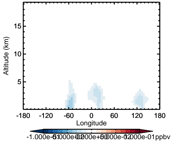
v11-02d - v11-02a PROPNN - Diff along 15S for Oct
