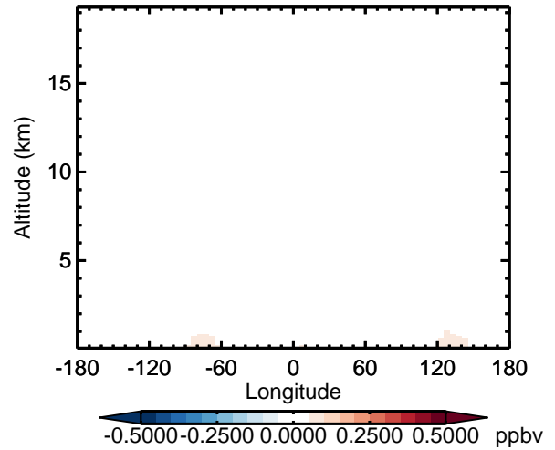
v11-02d - v11-02a CH 2 O - Diff along 42N for Oct
