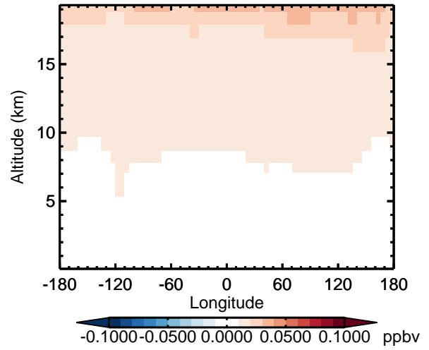
v11-02d - v11-02c CFC11 - Diff along 42N for Oct
