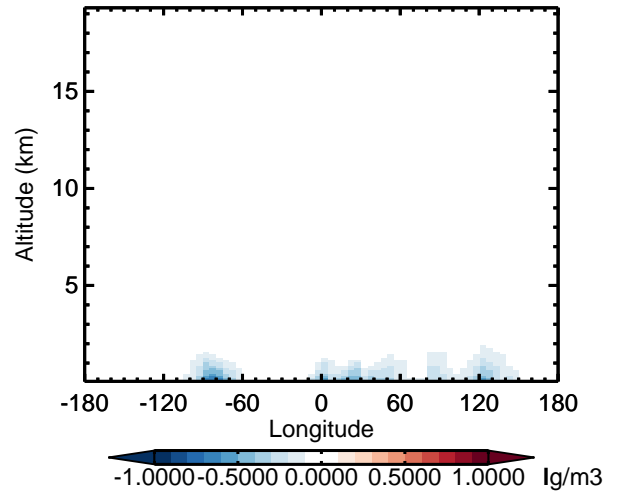
v11-02d - v11-02a NH3 - Diff along 42N for Oct
