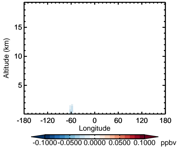
v11-02d - v11-02a ISOA1 - Diff along 15S for Oct
