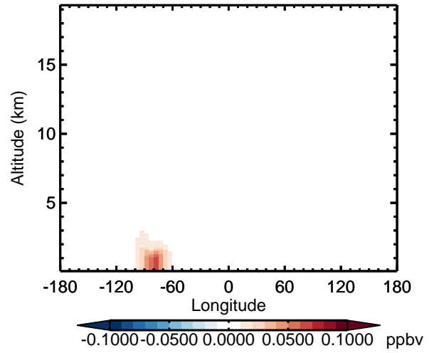
v11-02d - v11-02c SOAIE - Diff along 42N for Oct
