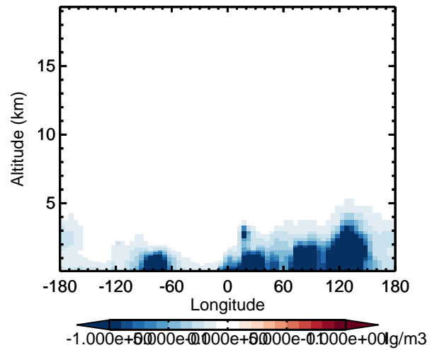
v11-02d - v11-02a SO 2 - Diff along 42N for Oct
