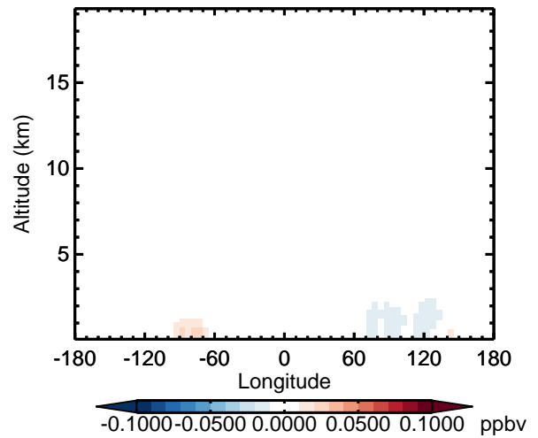
v11-02d - v11-02a MGLY - Diff along 42N for Oct
