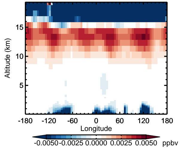
v11-02d - v11-02c N2O5 - Diff along 42N for Oct
