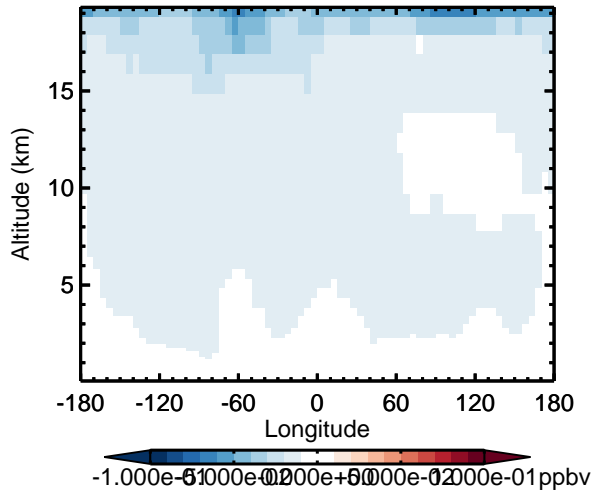
v11-02d - v11-02c OCS - Diff along 15S for Oct
