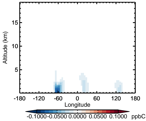
v11-02d - v11-02c MEK - Diff along 15S for Oct
