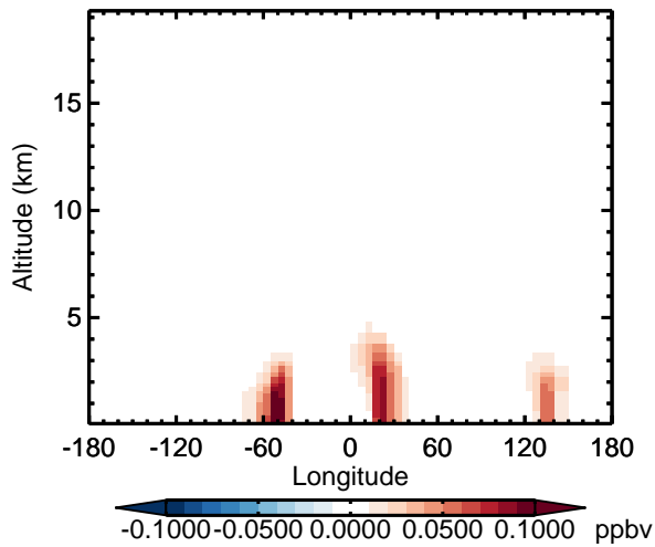
v11-02d - v11-02a IONITA - Diff along 15S for Oct
