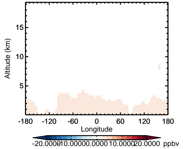
v11-02d - v11-02a CO - Diff along 42N for Oct
