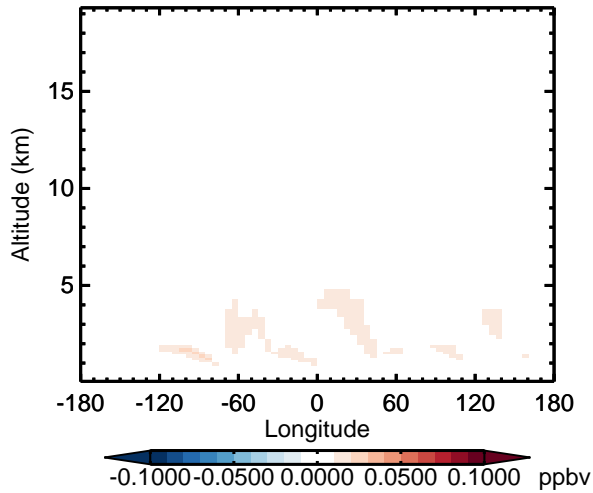
v11-02d - v11-02a CH 3 Cl - Diff along 15S for Oct
