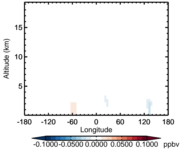
v11-02d - v11-02c HC187 - Diff along 15S for Oct
