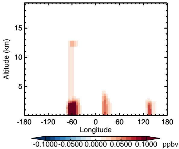
v11-02d - v11-02a IPMN - Diff along 15S for Oct
