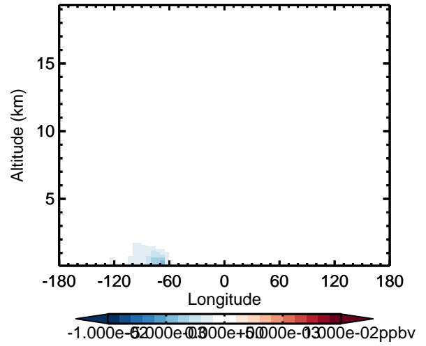
v11-02d - v11-02c R4N2 - Diff along 42N for Oct
