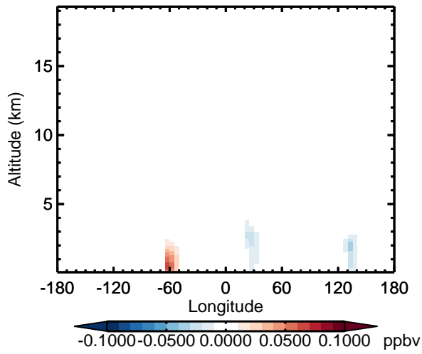
v11-02d - v11-02c IEPOXB - Diff along 15S for Oct
