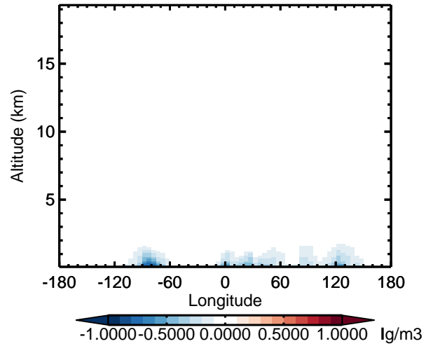
v11-02d - v11-02c NH3 - Diff along 42N for Oct
