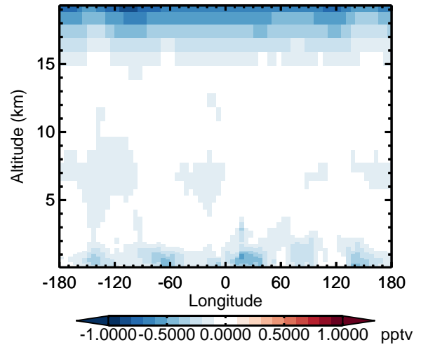
v11-02d - v11-02a HO2 - Diff along 42N for Oct
