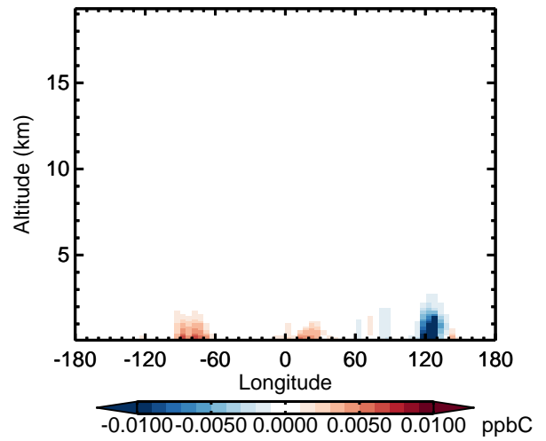
v11-02d - v11-02a PRPE - Diff along 42N for Oct
