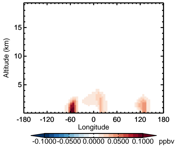
v11-02d - v11-02a SOAGX - Diff along 15S for Oct
