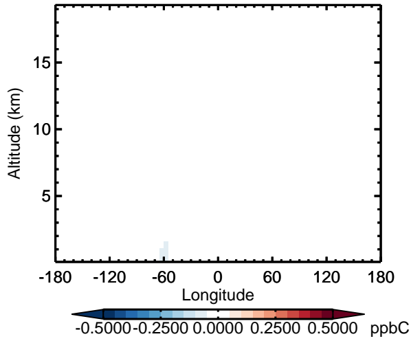
v11-02d - v11-02c ALD2 - Diff along 15S for Oct
