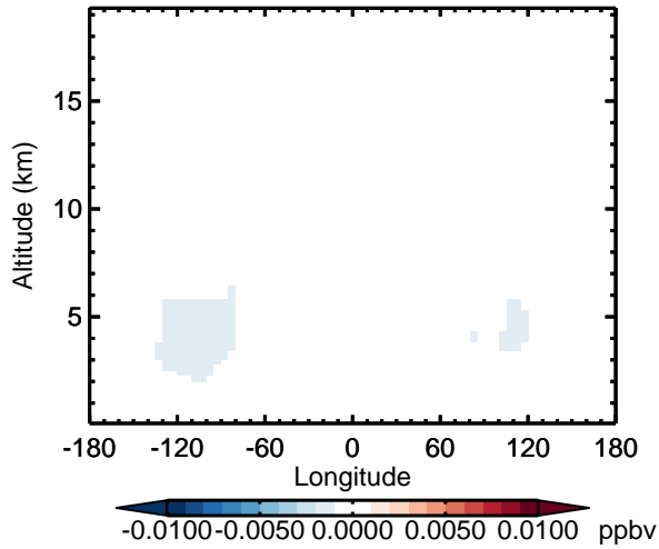
v11-02d - v11-02c HBr - Diff along 15S for Oct
