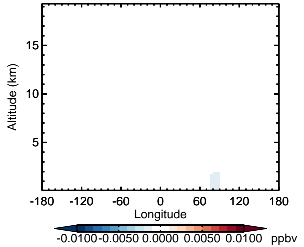
v11-02d - v11-02a HOBr - Diff along 42N for Oct
