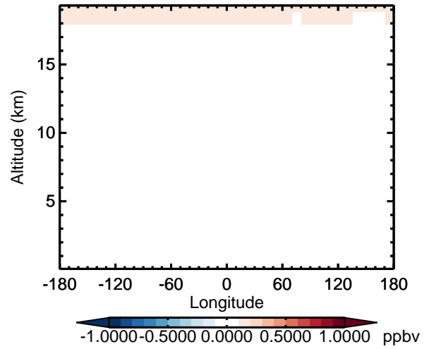
v11-02d - v11-02a NO - Diff along 42N for Oct
