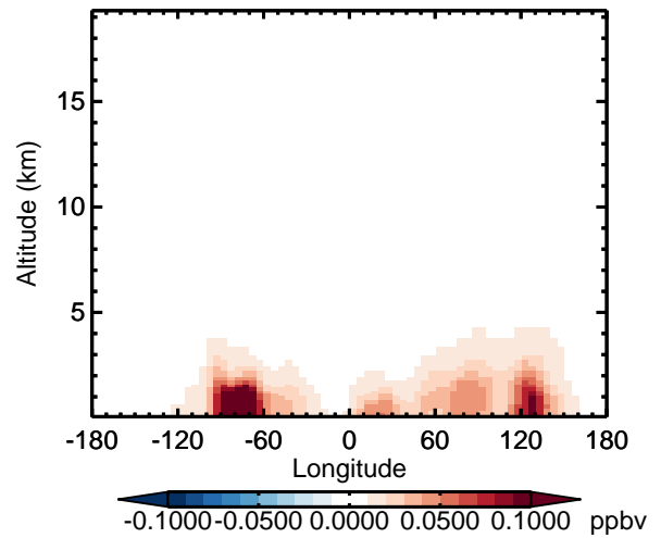
v11-02d - v11-02a INDIOL - Diff along 42N for Oct
