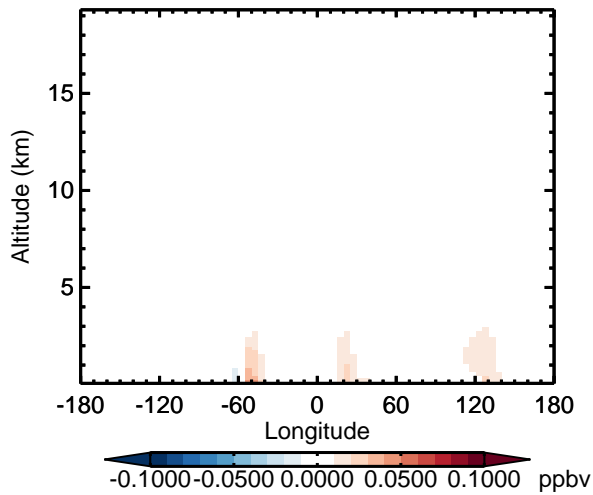
v11-02d - v11-02a TSOG3 - Diff along 15S for Oct
