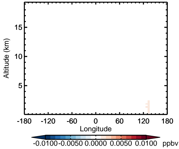
v11-02d - v11-02c HOBr - Diff along 15S for Oct
