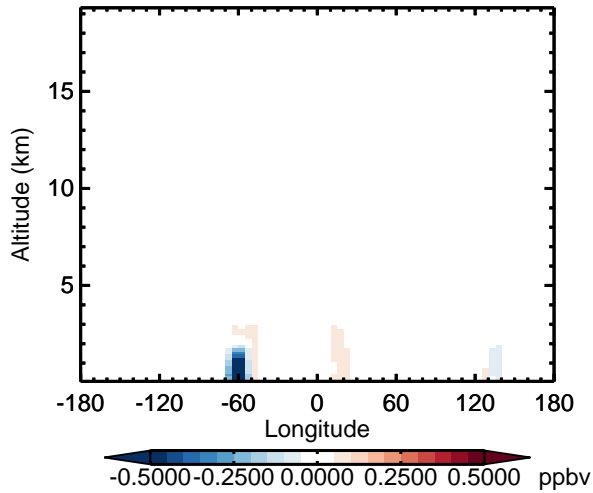
v11-02d - v11-02a CH 2 O - Diff along 15S for Oct
