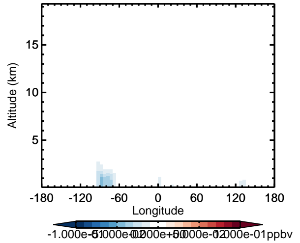
v11-02d - v11-02a HAC - Diff along 42N for Oct
