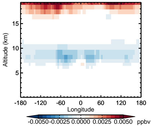
v11-02d - v11-02c HNO 4 - Diff along 15S for Oct
