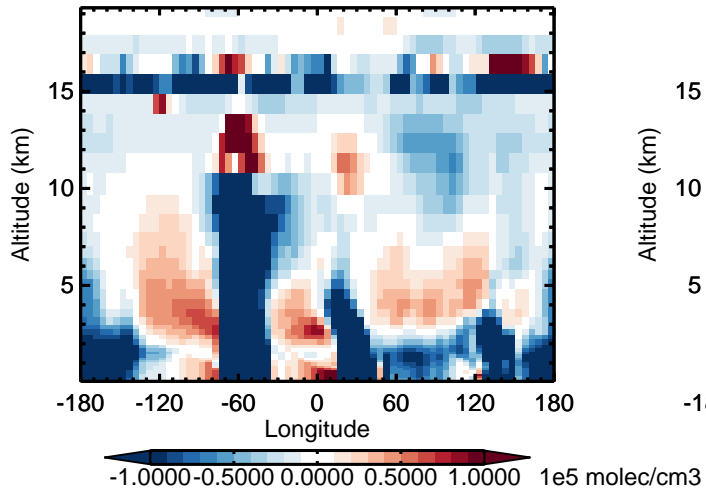
v11-02d - v11-02a OH - Diff along 15S for Oct
