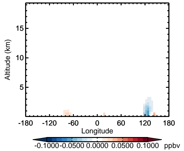
v11-02d - v11-02a TOLU - Diff along 42N for Oct
