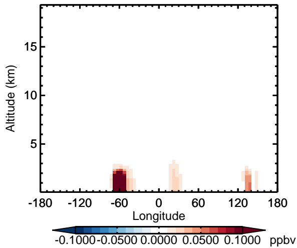
v11-02d - v11-02a HPALD - Diff along 15S for Oct
