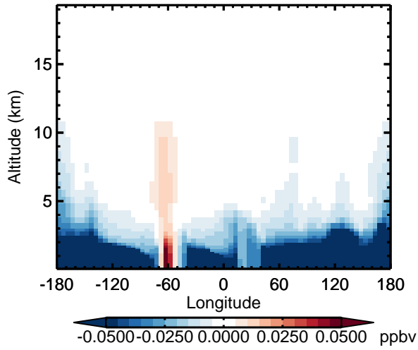
v11-02d - v11-02c MP - Diff along 15S for Oct
