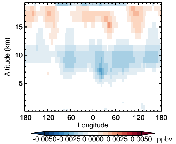
v11-02d - v11-02c HNO 4 - Diff along 42N for Oct
