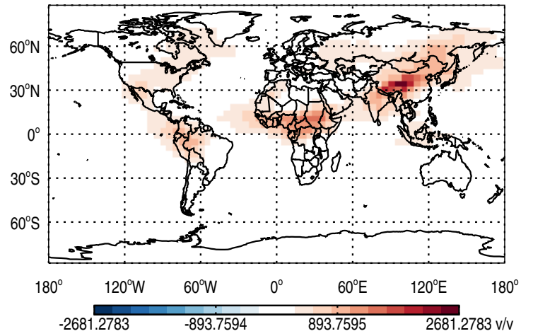
Abs Diff @ 500 hPa - Rn
