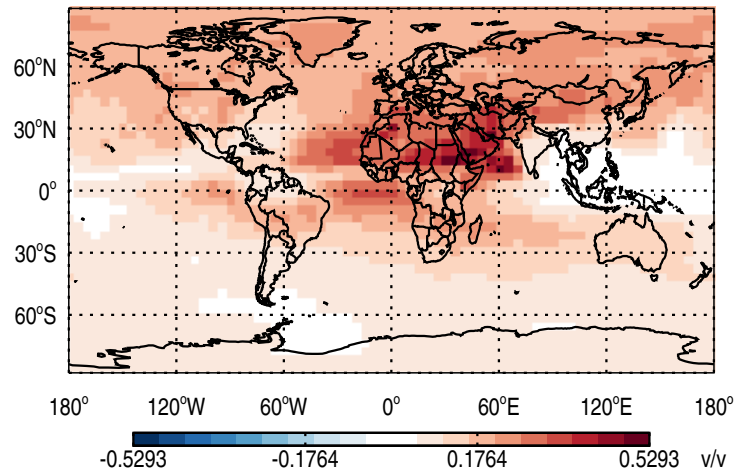
Abs Diff @ 500 hPa - Pb
