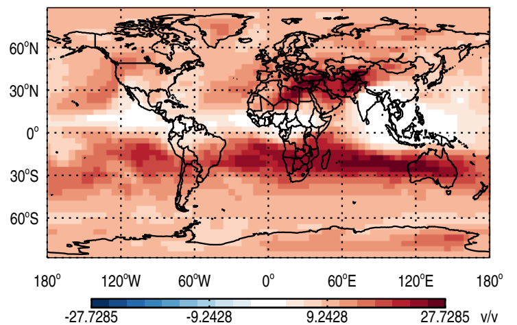
Abs Diff @ 500 hPa - Be7
