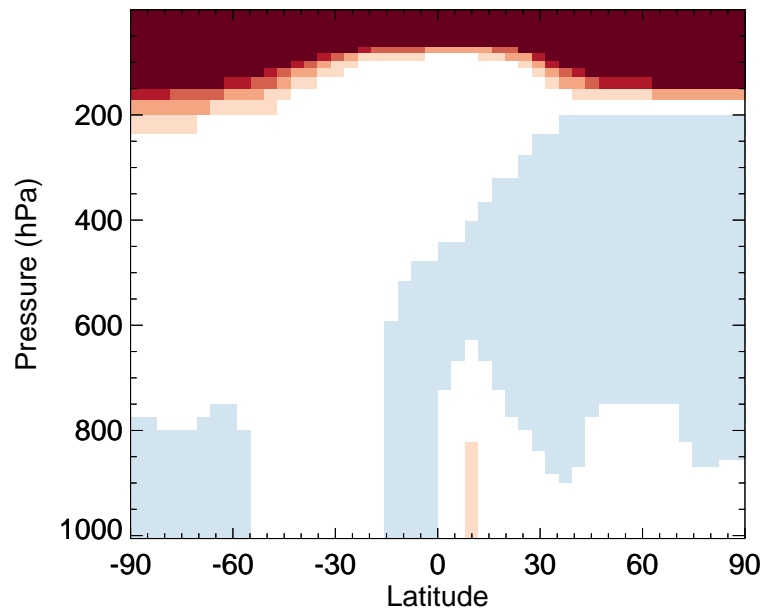
v11-02e-Run0 / v11-02c-Run0 ASOAN - Zonal mean % diff for Jan
