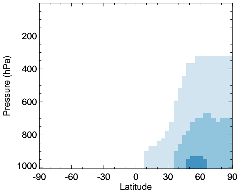
v11-02e-Run0 - v11-02c-Run0 C3H8 - Zonal mean abs diff for Jan
