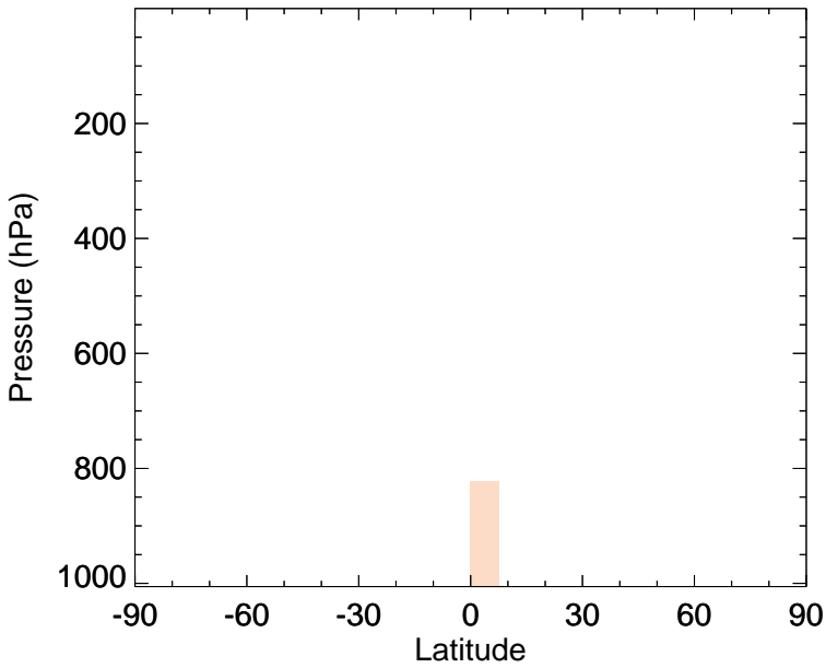
v11-02e-Run0 - v11-02c-Run0 DST1 - Zonal mean abs diff for Jan
