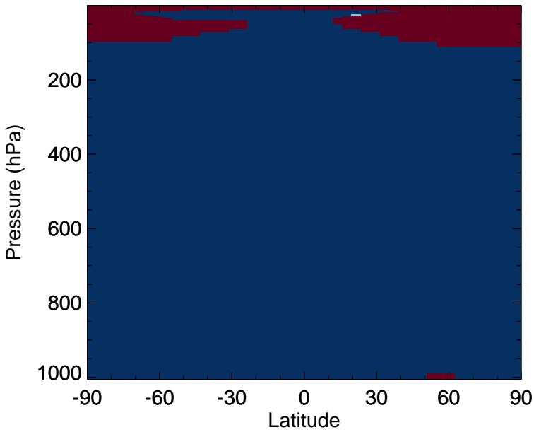
v11-02e-Run0 - v11-02c-Run0 CH4 - Zonal mean abs diff for Jan
