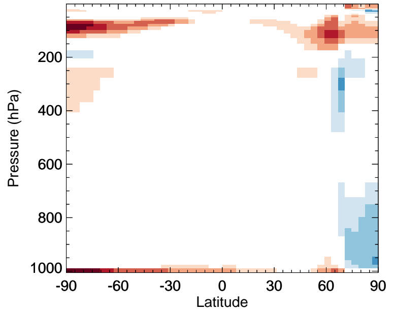
v11-02e-Run0 / v11-02d-Run1 OH - Zonal mean % diff for Jan
