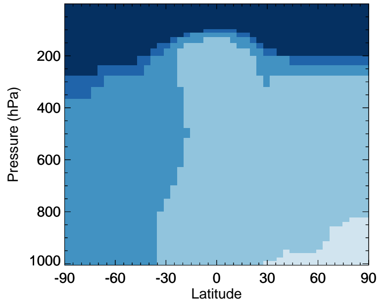
v11-02e-Run0 / v11-02c-Run0 C2H6 - Zonal mean % diff for Jan
