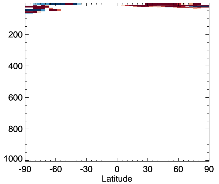
v11-02e-Run0 / v11-02d-Run1 BCPO - Zonal mean % diff for Jan
