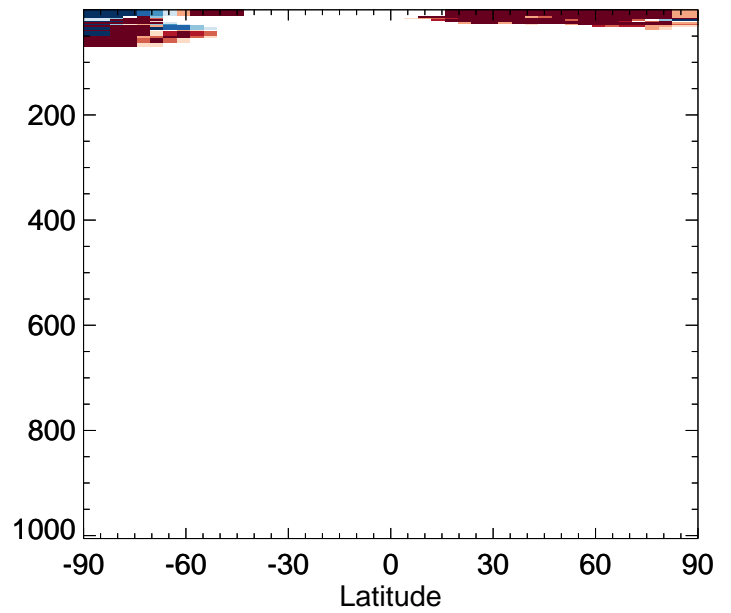
v11-02e-Run0 / v11-02c-Run0 BCPO - Zonal mean % diff for Jan
