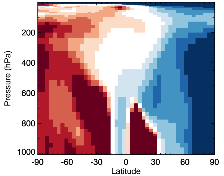
v11-02e-Run0 / v11-02c-Run0 HONIT - Zonal mean % diff for Jan
