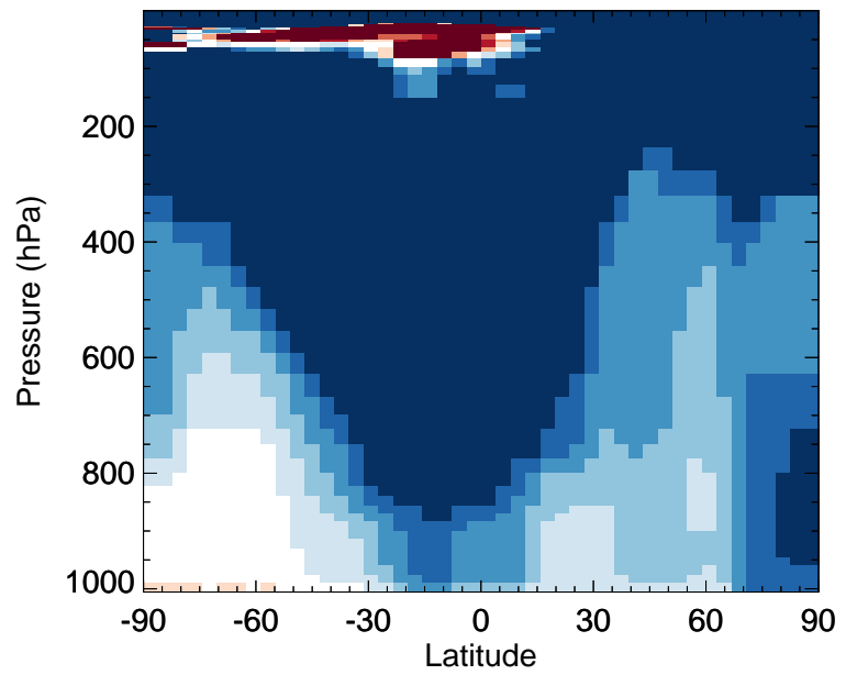
v11-02e-Run0 / v11-02d-Run1 ISN1OG - Zonal mean % diff for Jan
