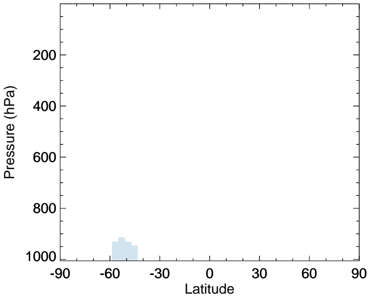
v11-02e-Run0 - v11-02c-Run0 HBr - Zonal mean abs diff for Jan
