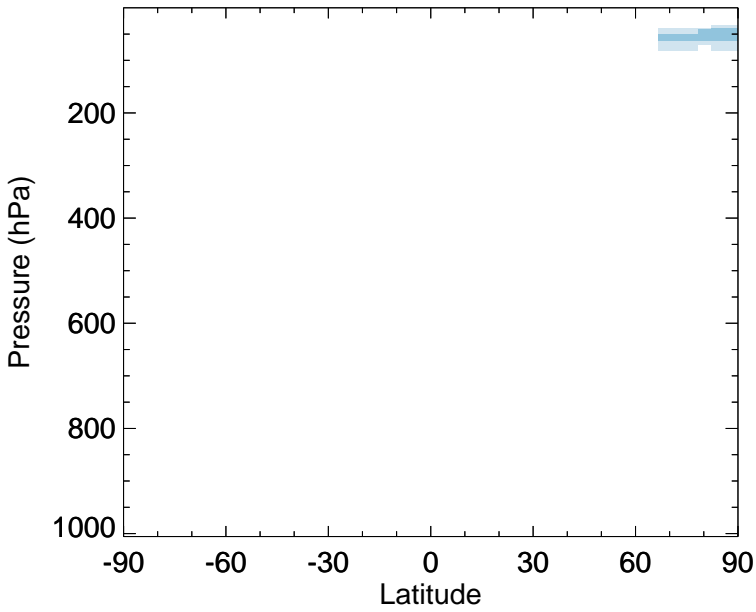
v11-02e-Run0 - v11-02d-Run1 Cl2 - Zonal mean abs diff for Jan
