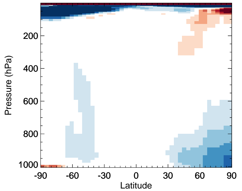
v11-02e-Run0 / v11-02d-Run1 GLYX - Zonal mean % diff for Jan
