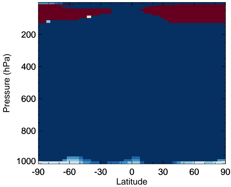
v11-02e-Run0 - v11-02d-Run1 N2O - Zonal mean abs diff for Jan
