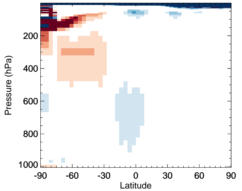
v11-02e-Run0 / v11-02d-Run1 ETHLN - Zonal mean % diff for Jan
