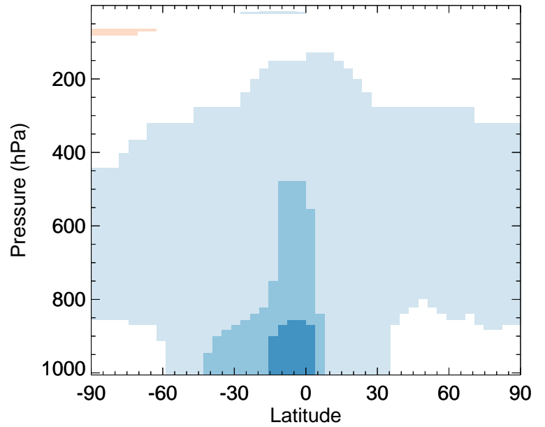
v11-02e-Run0 / v11-02c-Run0 O3 - Zonal mean % diff for Jan
