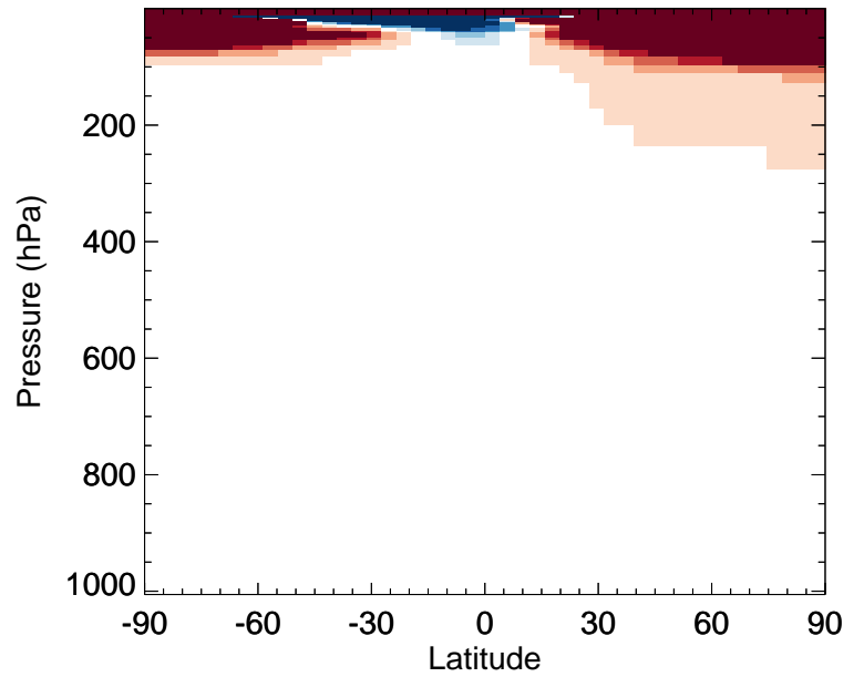
v11-02e-Run0 / v11-02c-Run0 CFC11 - Zonal mean % diff for Jan
