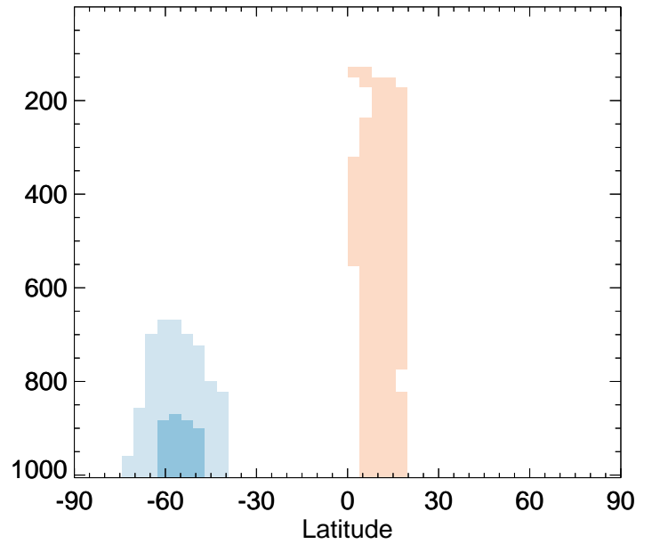
v11-02e-Run0 / v11-02c-Run0 NITs - Zonal mean % diff for Jan
