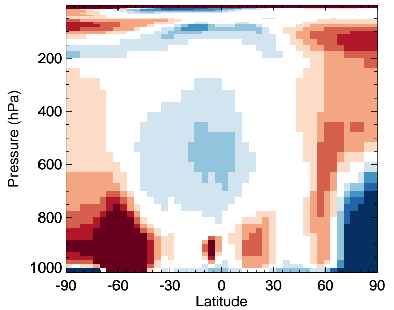
v11-02e-Run0 / v11-02c-Run0 MPN - Zonal mean % diff for Jan
