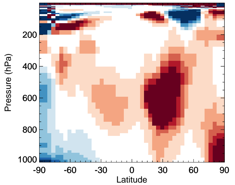
v11-02e-Run0 / v11-02d-Run1 ISOP - Zonal mean % diff for Jan
