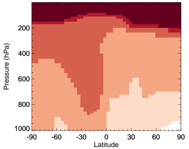
v11-02e-Run0 / v11-02d-Run1 INDIOL - Zonal mean % diff for Jan
