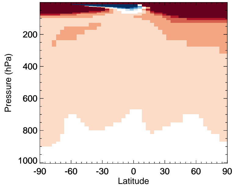
v11-02e-Run0 / v11-02d-Run1 CCI4 - Zonal mean % diff for Jan
