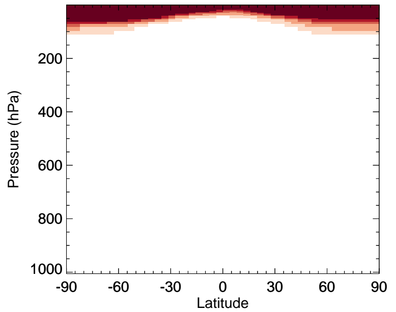
v11-02e-Run0 / v11-02d-Run1 ASOAN - Zonal mean % diff for Jan
