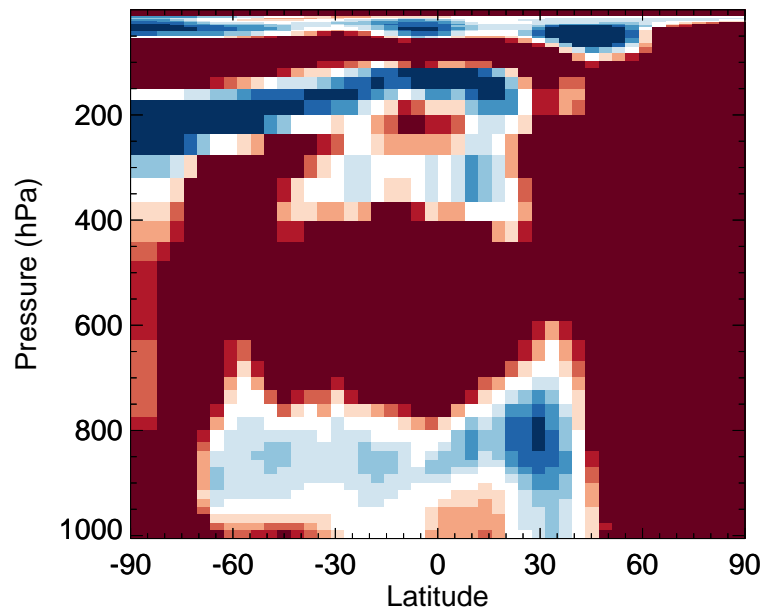
v11-02e-Run0 / v11-02d-Run1 HOCl - Zonal mean % diff for Jan
