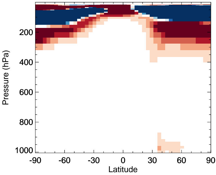
v11-02e-Run0 - v11-02d-Run1 HNO 3 - Zonal mean abs diff for Jan
