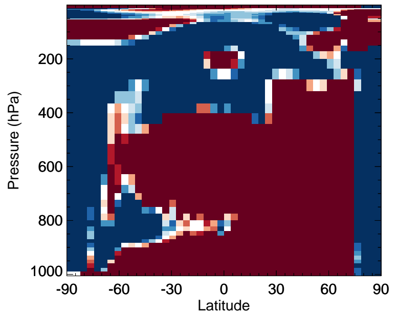
v11-02e-Run0 / v11-02c-Run0 Cl2O2 - Zonal mean % diff for Jan
