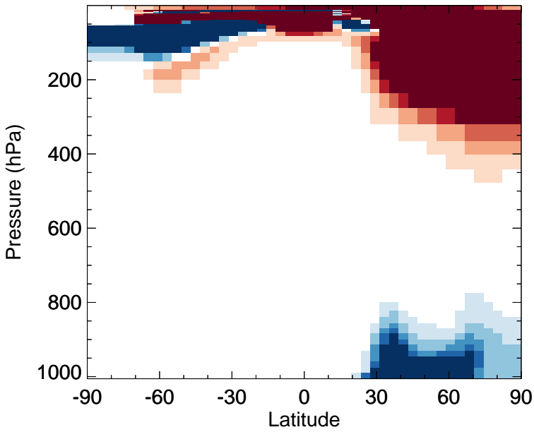
v11-02e-Run0 - v11-02d-Run1 N2O5 - Zonal mean abs diff for Jan
