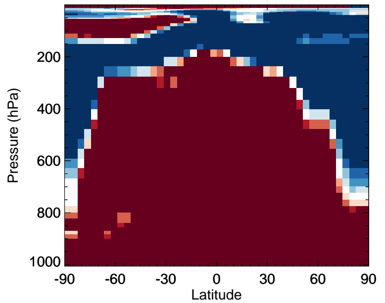
v11-02e-Run0 / v11-02c-Run0 OCIO - Zonal mean % diff for Jan
