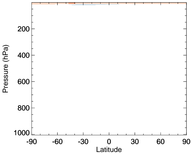
v11-02e-Run0 - v11-02d-Run1 CO - Zonal mean abs diff for Jan
