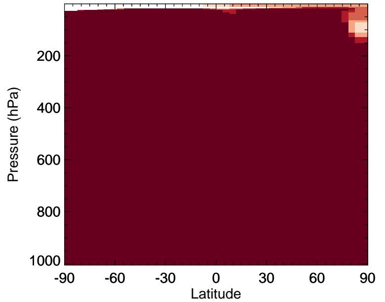
v11-02e-Run0 / v11-02c-Run0 DST3 - Zonal mean % diff for Jan
