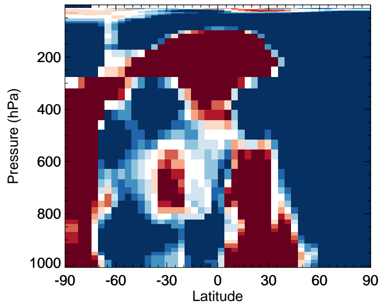
v11-02e-Run0 / v11-02d-Run1 Br2 - Zonal mean % diff for Jan
