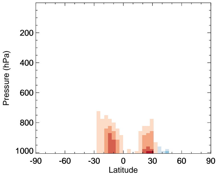
v11-02e-Run0 - v11-02d-Run1 PRPE - Zonal mean abs diff for Jan
