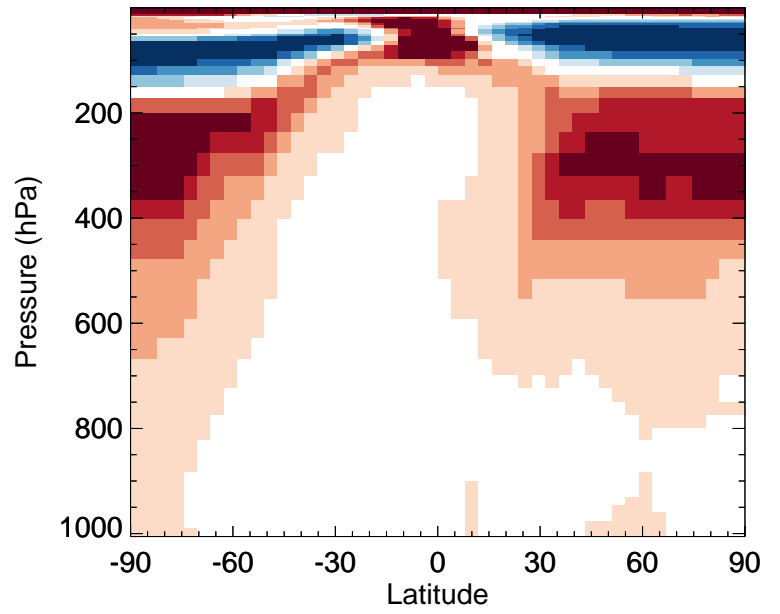
v11-02e-Run0 / v11-02d-Run1 HNO 3 - Zonal mean % diff for Jan
