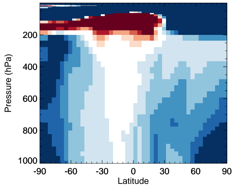
v11-02e-Run0 / v11-02c-Run0 IMAE - Zonal mean % diff for Jan
