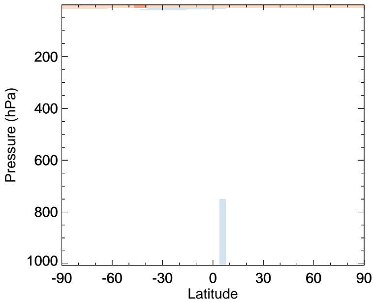
v11-02e-Run0 - v11-02c-Run0 CO - Zonal mean abs diff for Jan
