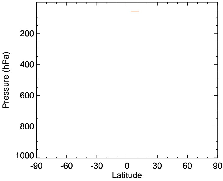
v11-02e-Run0 - v11-02d-Run1 SO4 - Zonal mean abs diff for Jan
