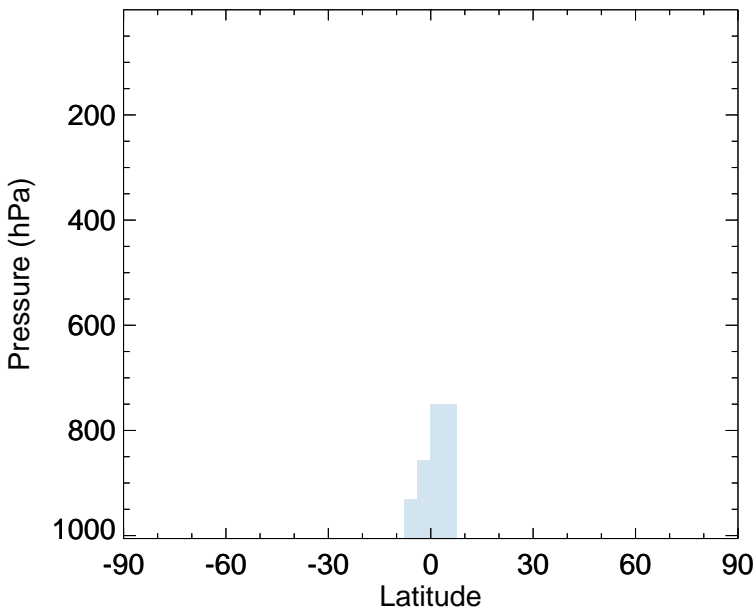
v11-02e-Run0 - v11-02c-Run0 SOAGX - Zonal mean abs diff for Jan
