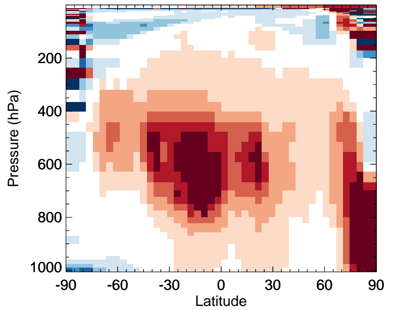
v11-02e-Run0 / v11-02d-Run1 LIMO - Zonal mean % diff for Jan
