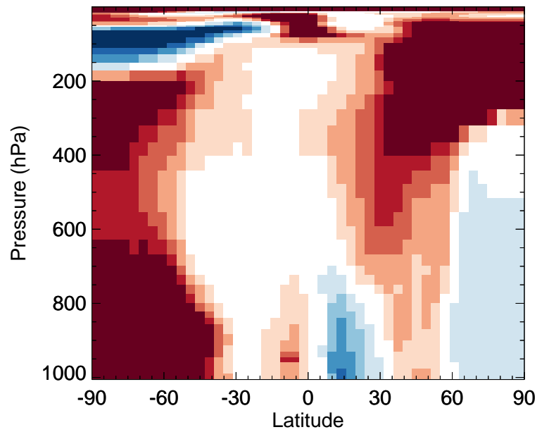
v11-02e-Run0 / v11-02c-Run0 HNO 2 - Zonal mean % diff for Jan
