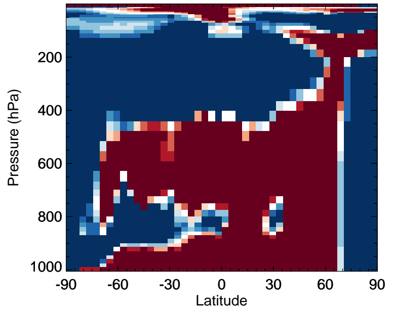
v11-02e-Run0 / v11-02c-Run0 Cl2 - Zonal mean % diff for Jan
