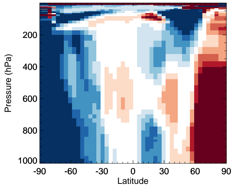
v11-02e-Run0 / v11-02c-Run0 ISOP - Zonal mean % diff for Jan
