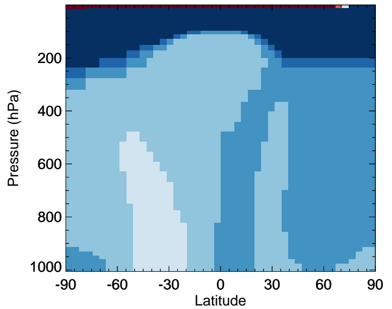
v11-02e-Run0 / v11-02c-Run0 C3H8 - Zonal mean % diff for Jan
