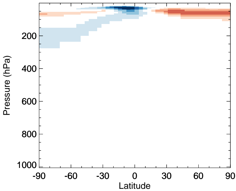
v11-02e-Run0 - v11-02c-Run0 OCS - Zonal mean abs diff for Jan
