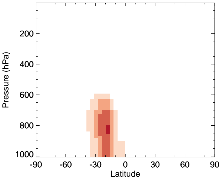
v11-02e-Run0 - v11-02d-Run1 SOAIE - Zonal mean abs diff for Jan
