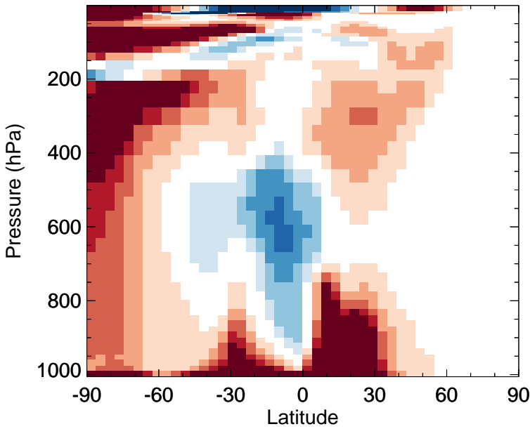
v11-02e-Run0 - v11-02c-Run0 OH - Zonal mean abs diff for Jan
