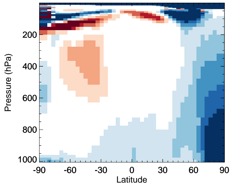
v11-02e-Run0 / v11-02d-Run1 ISOPNB - Zonal mean % diff for Jan
