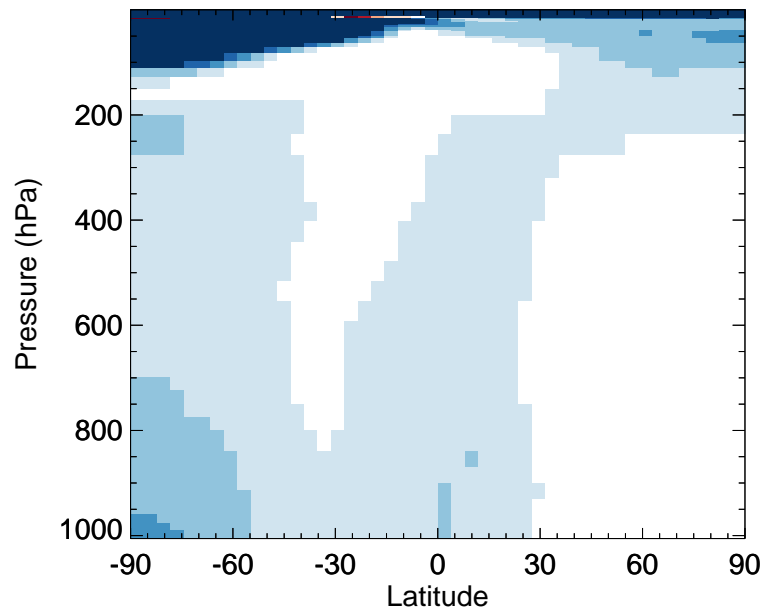
v11-02e-Run0 / v11-02c-Run0 BENZ - Zonal mean % diff for Jan
