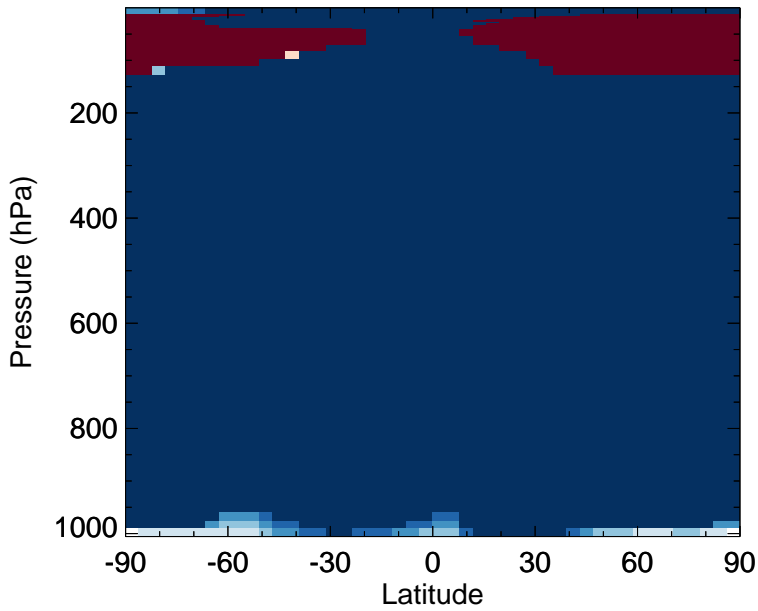
v11-02e-Run0 - v11-02c-Run0 N2O - Zonal mean abs diff for Jan
