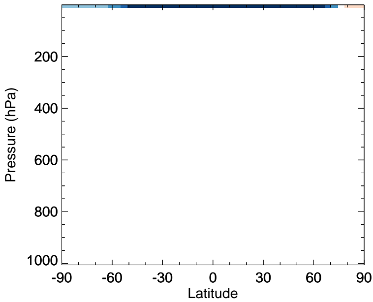
v11-02e-Run0 - v11-02d-Run1 Cl - Zonal mean abs diff for Jan
