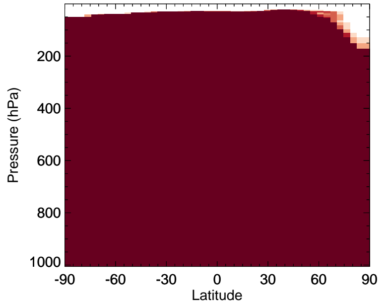
v11-02e-Run0 / v11-02d-Run1 DST4 - Zonal mean % diff for Jan
