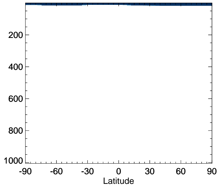
v11-02e-Run0 / v11-02c-Run0 SALC - Zonal mean % diff for Jan
