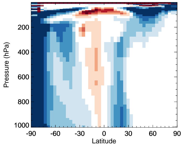
v11-02e-Run0 / v11-02c-Run0 MVK - Zonal mean % diff for Jan
