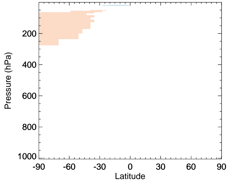
v11-02e-Run0 / v11-02d-Run1 O3 - Zonal mean % diff for Jan
