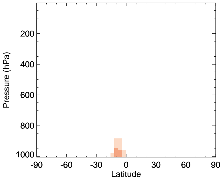
v11-02e-Run0 - v11-02c-Run0 ISOP - Zonal mean abs diff for Jan
