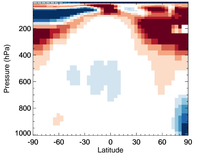
v11-02e-Run0 / v11-02d-Run1 NO - Zonal mean % diff for Jan
