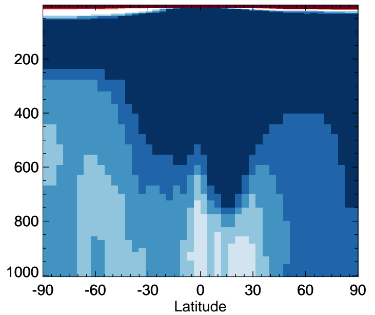
v11-02e-Run0 / v11-02c-Run0 SOAIE - Zonal mean % diff for Jan
