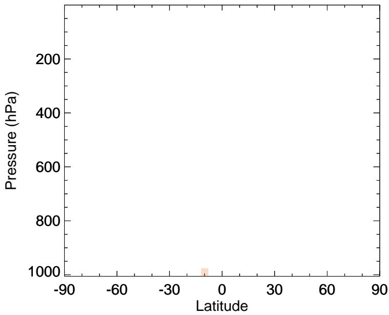
v11-02e-Run0 - v11-02d-Run1 ISOP - Zonal mean abs diff for Jan
