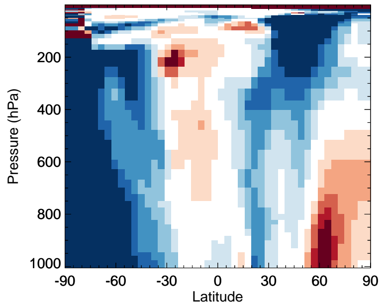
v11-02e-Run0 / v11-02c-Run0 RIPA - Zonal mean % diff for Jan
