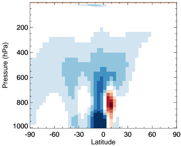
v11-02e-Run0 - v11-02c-Run0 H2O2 - Zonal mean abs diff for Jan
