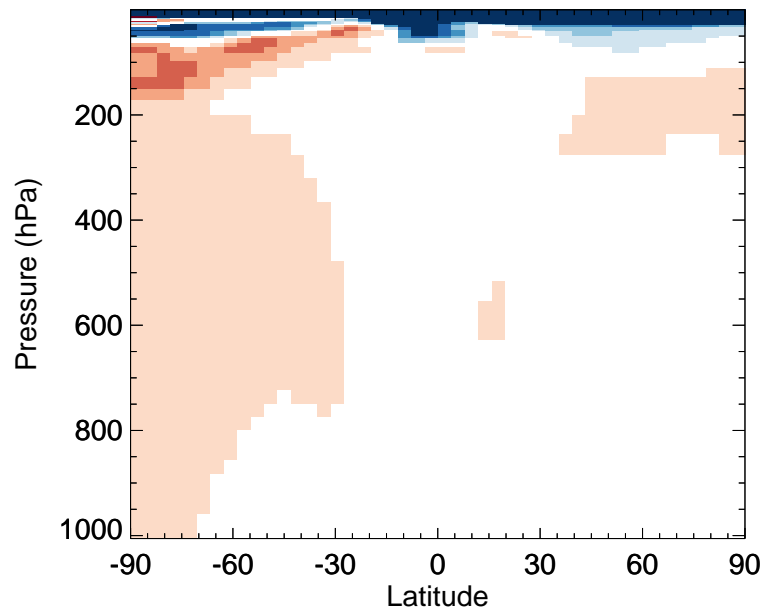
v11-02e-Run0 / v11-02d-Run1 MEK - Zonal mean % diff for Jan
