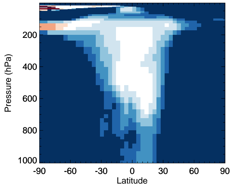
v11-02e-Run0 / v11-02d-Run1 IEPOXB - Zonal mean % diff for Jan
