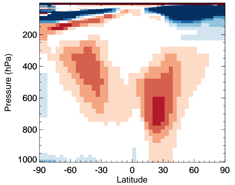
v11-02e-Run0 / v11-02d-Run1 IPMN - Zonal mean % diff for Jan
