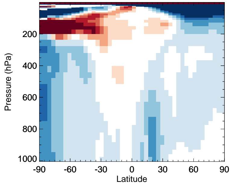
v11-02e-Run0 / v11-02c-Run0 GLYC - Zonal mean % diff for Jan
