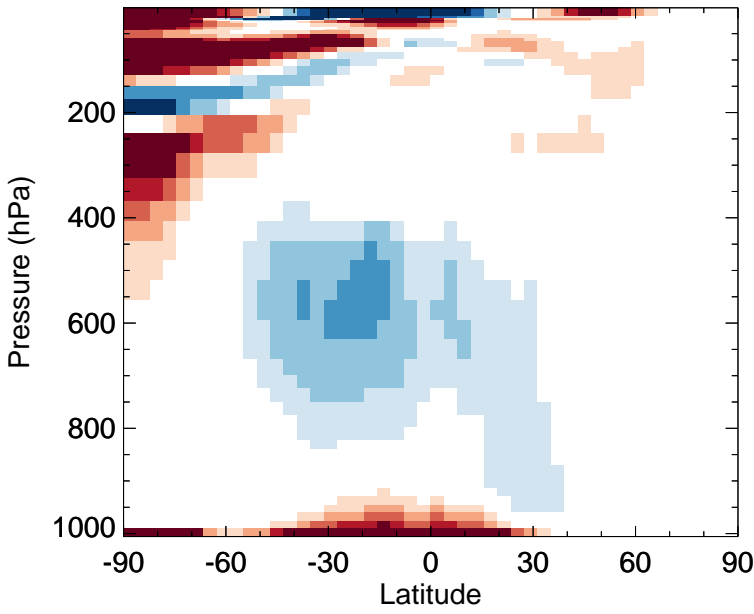
v11-02e-Run0 - v11-02d-Run1 OH - Zonal mean abs diff for Jan
