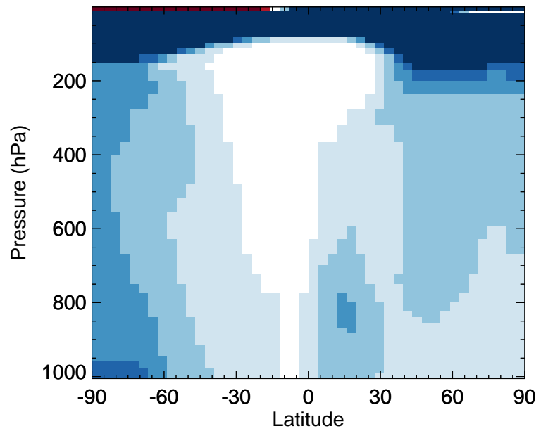
v11-02e-Run0 / v11-02c-Run0 EOH - Zonal mean % diff for Jan
