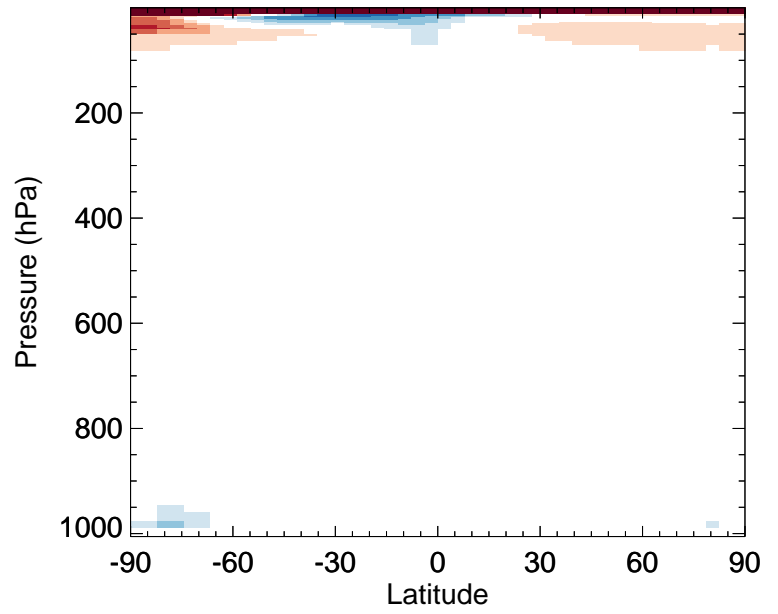
v11-02e-Run0 / v11-02d-Run1 CH4 - Zonal mean % diff for Jan
