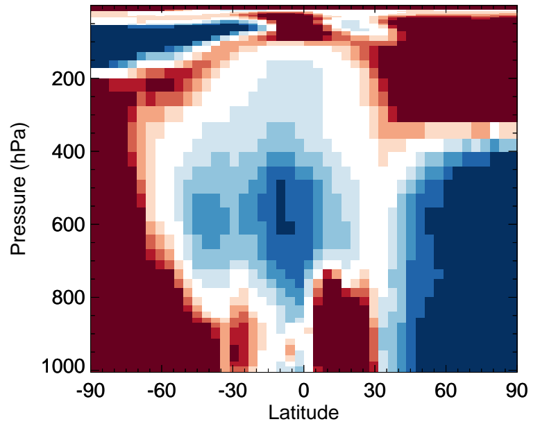
v11-02e-Run0 / v11-02c-Run0 N2O5 - Zonal mean % diff for Jan
