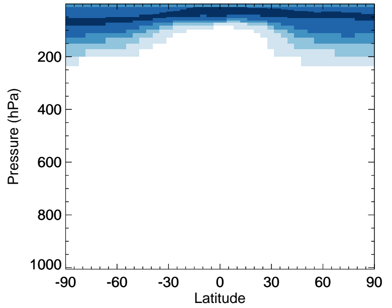
v11-02e-Run0 / v11-02d-Run1 MSA - Zonal mean % diff for Jan
