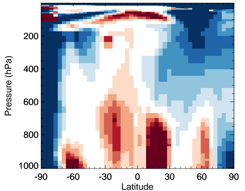
v11-02e-Run0 / v11-02c-Run0 ISOPNB - Zonal mean % diff for Jan
