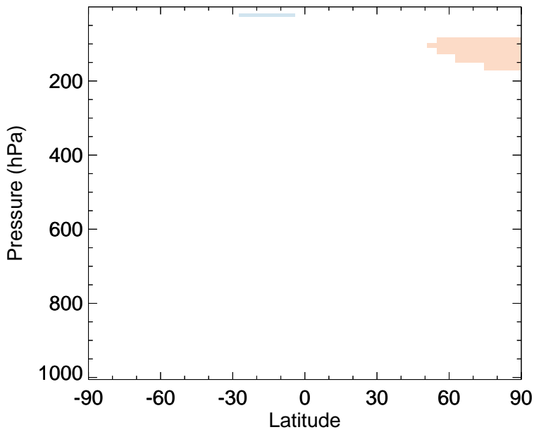
v11-02e-Run0 - v11-02c-Run0 MPN - Zonal mean abs diff for Jan
