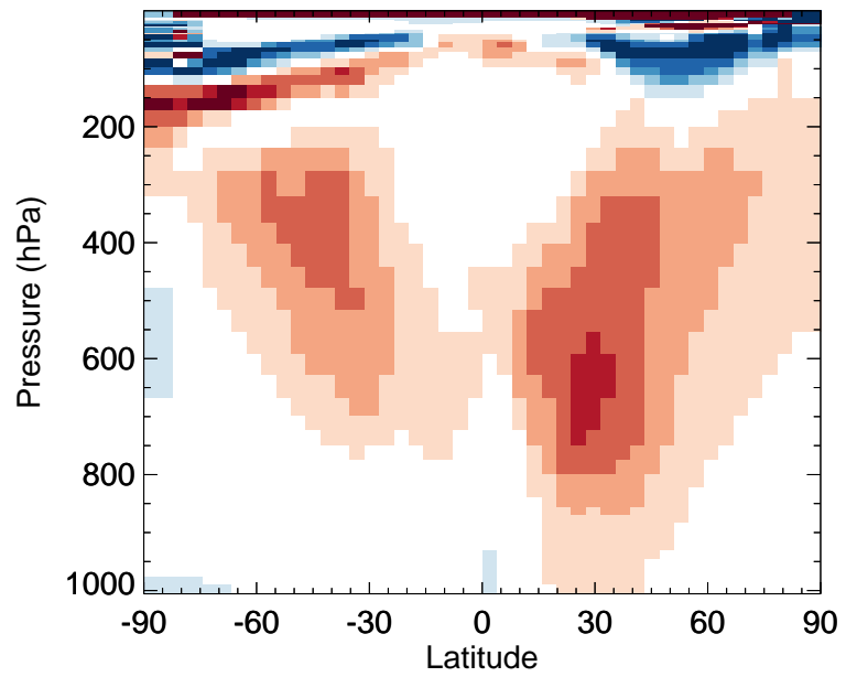
v11-02e-Run0 / v11-02d-Run1 MVK - Zonal mean % diff for Jan
