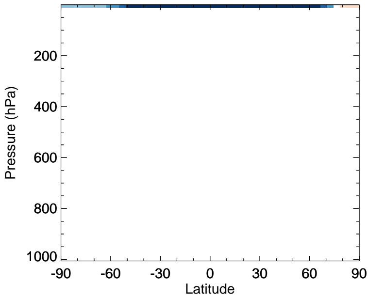
v11-02e-Run0 - v11-02c-Run0 Cl - Zonal mean abs diff for Jan
