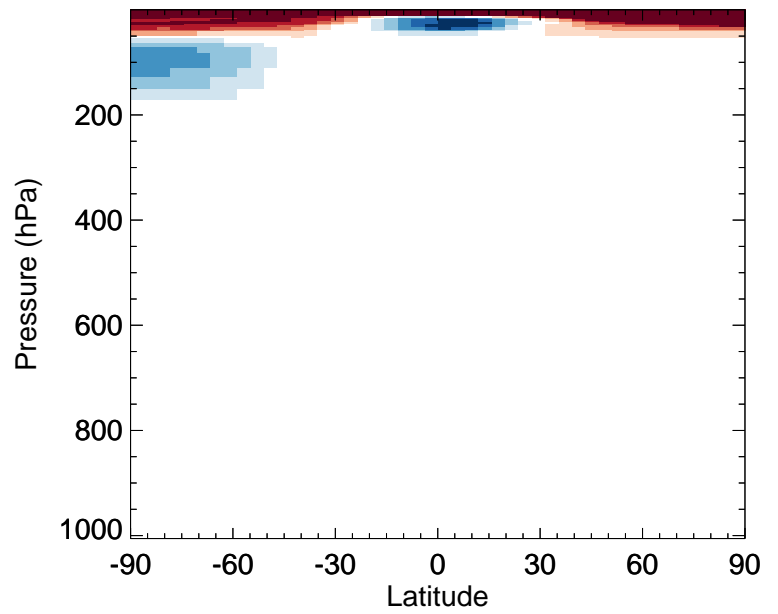
v11-02e-Run0 / v11-02d-Run1 ASOA1 - Zonal mean % diff for Jan
