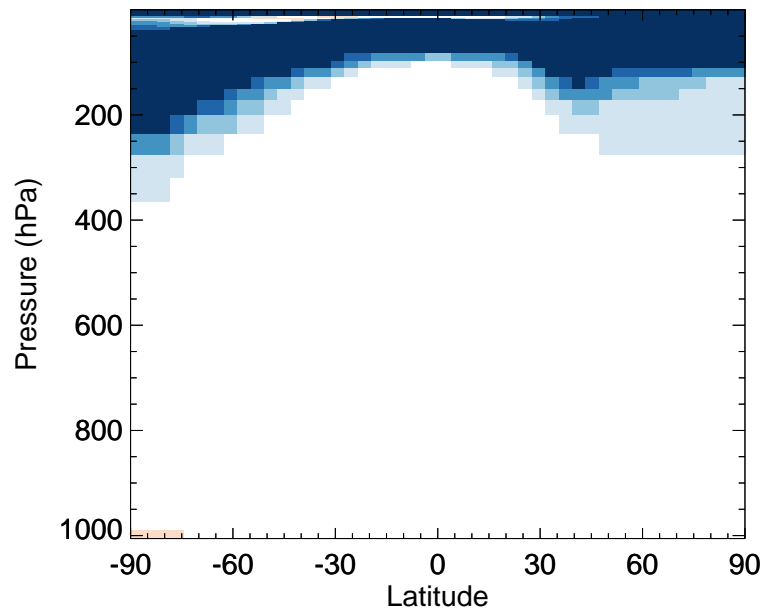
v11-02e-Run0 / v11-02d-Run1 MAP - Zonal mean % diff for Jan
