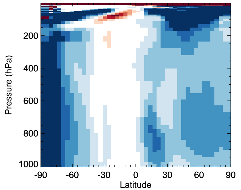
v11-02e-Run0 / v11-02c-Run0 XYLE - Zonal mean % diff for Jan
