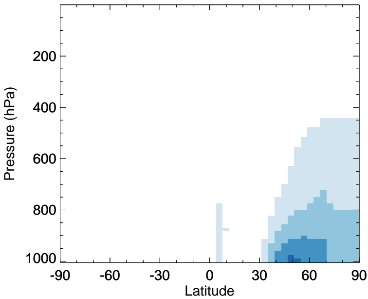
v11-02e-Run0 - v11-02c-Run0 TOLU - Zonal mean abs diff for Jan
