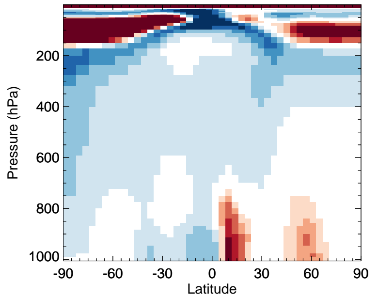
v11-02e-Run0 / v11-02c-Run0 H2O2 - Zonal mean % diff for Jan
