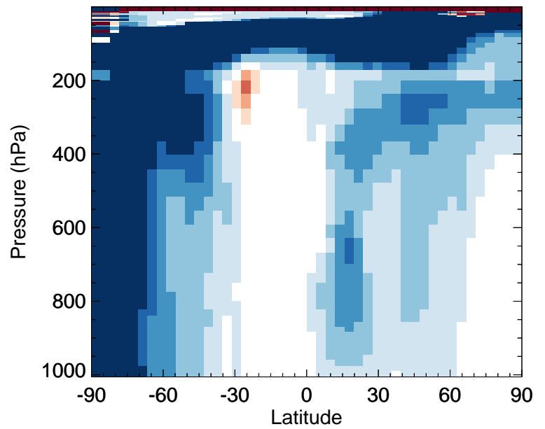
v11-02e-Run0 / v11-02c-Run0 PRPE - Zonal mean % diff for Jan
