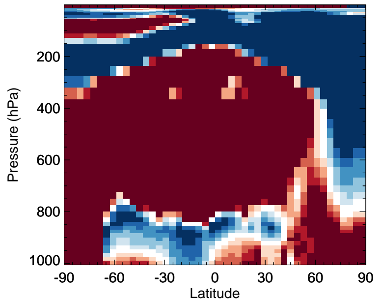
v11-02e-Run0 / v11-02d-Run1 OCIO - Zonal mean % diff for Jan
