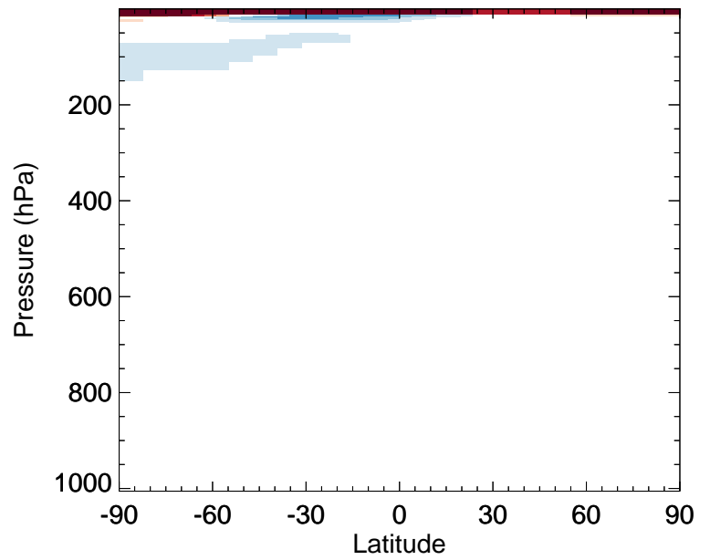
v11-02e-Run0 / v11-02d-Run1 CO - Zonal mean % diff for Jan
