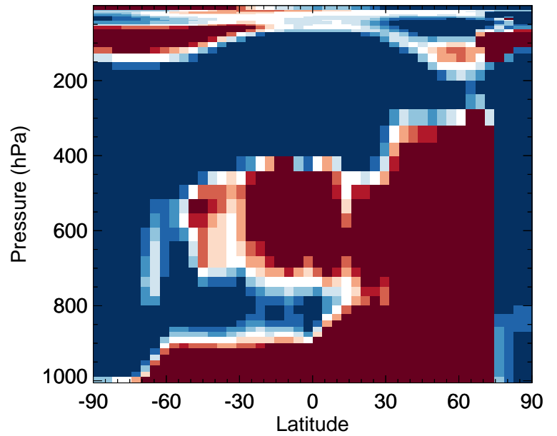
v11-02e-Run0 / v11-02c-Run0 ClO - Zonal mean % diff for Jan
