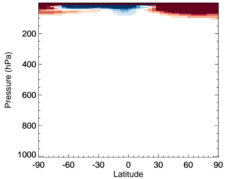
v11-02e-Run0 / v11-02c-Run0 OCS - Zonal mean % diff for Jan
