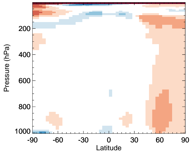
v11-02e-Run0 / v11-02c-Run0 CH 2 O - Zonal mean % diff for Jan
