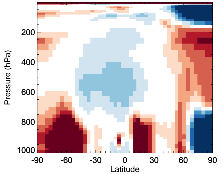
v11-02e-Run0 / v11-02c-Run0 HNO 4 - Zonal mean % diff for Jan
