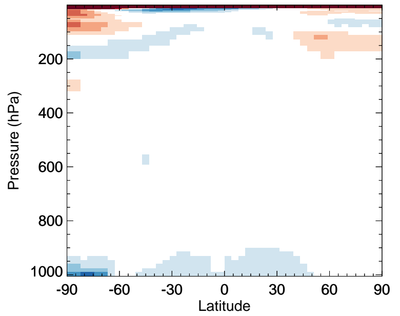
v11-02e-Run0 / v11-02d-Run1 CH 2 O - Zonal mean % diff for Jan
