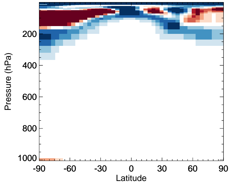
v11-02e-Run0 / v11-02d-Run1 MGLY - Zonal mean % diff for Jan
