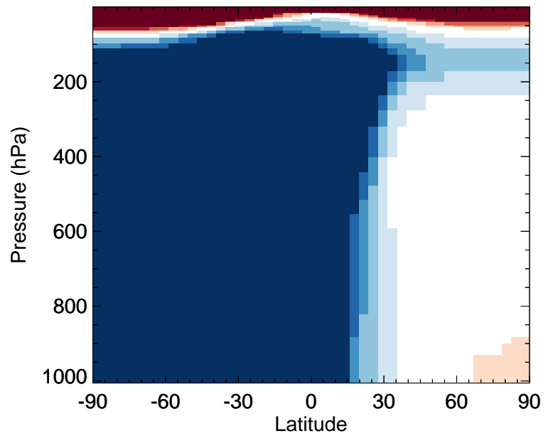
v11-02e-Run0 / v11-02c-Run0 SOAGX - Zonal mean % diff for Jan
