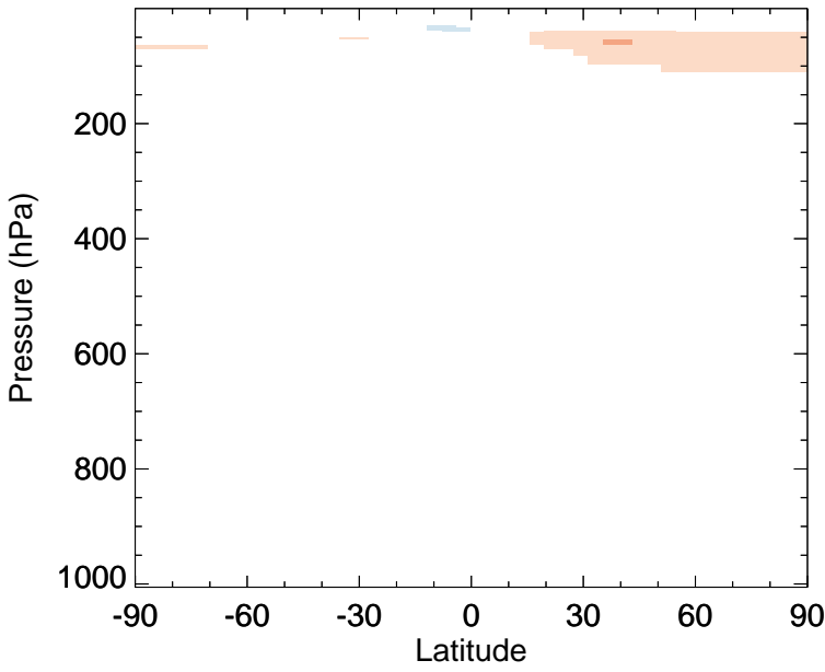
v11-02e-Run0 - v11-02d-Run1 CFC11 - Zonal mean abs diff for Jan
