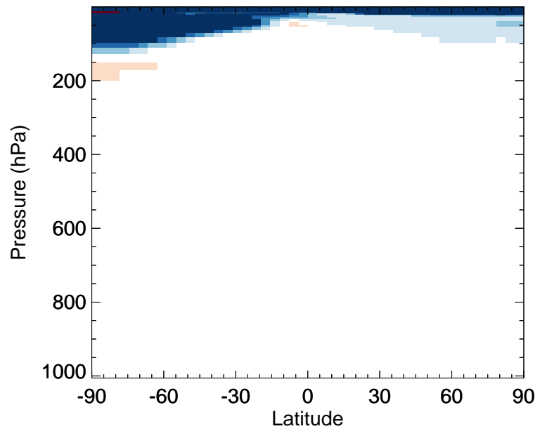
v11-02e-Run0 / v11-02d-Run1 BENZ - Zonal mean % diff for Jan
