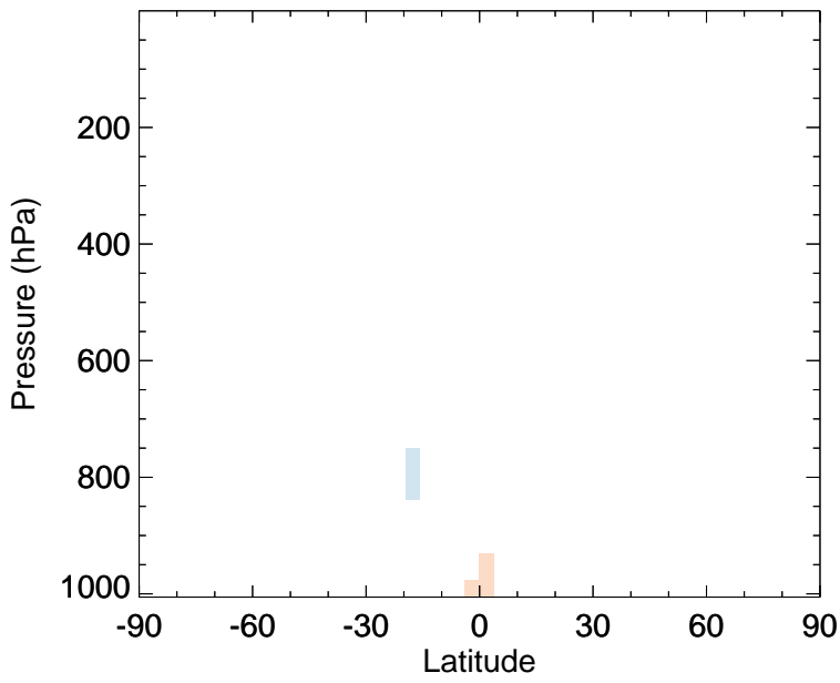
v11-02e-Run0 - v11-02d-Run1 MAP - Zonal mean abs diff for Jan
