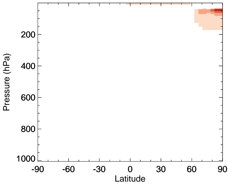
v11-02e-Run0 - v11-02d-Run1 HOCl - Zonal mean abs diff for Jan
