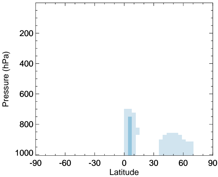
v11-02e-Run0 - v11-02c-Run0 BENZ - Zonal mean abs diff for Jan
