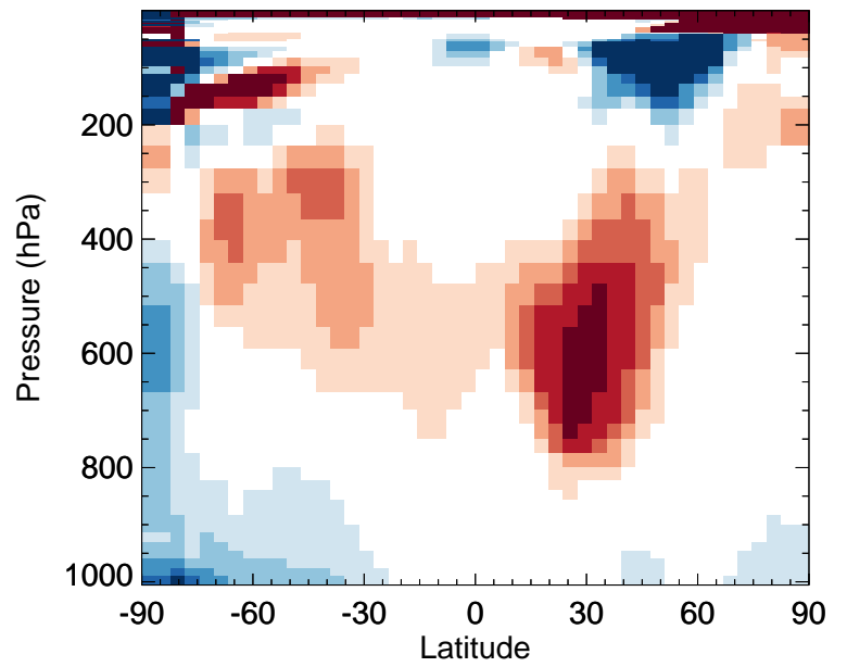
v11-02e-Run0 / v11-02d-Run1 RIPD - Zonal mean % diff for Jan
