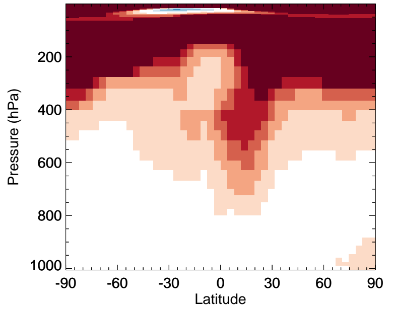
v11-02e-Run0 / v11-02d-Run1 SO4 - Zonal mean % diff for Jan
