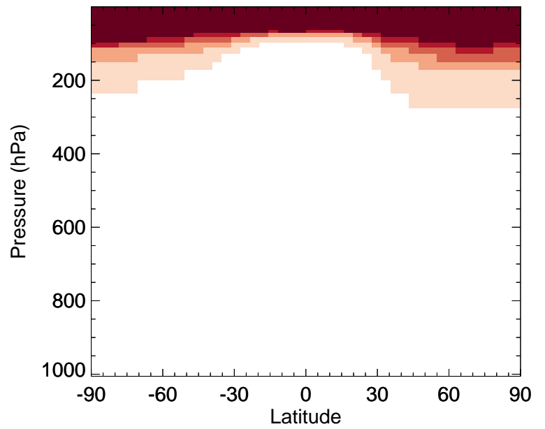
v11-02e-Run0 / v11-02d-Run1 ASOG2 - Zonal mean % diff for Jan
