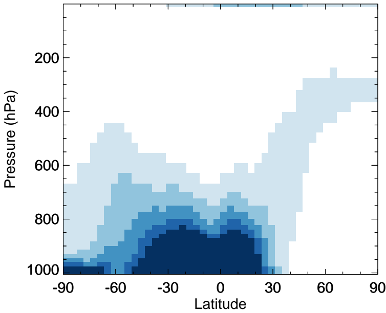
v11-02e-Run0 - v11-02d-Run1 MP - Zonal mean abs diff for Jan
