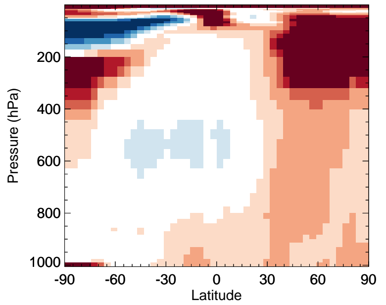
v11-02e-Run0 / v11-02d-Run1 HNO 2 - Zonal mean % diff for Jan
