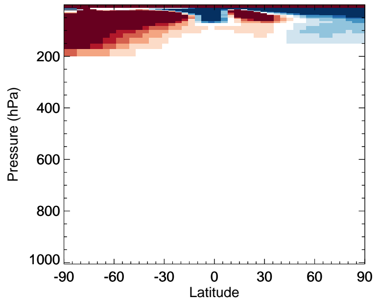
v11-02e-Run0 / v11-02d-Run1 C3H8 - Zonal mean % diff for Jan
