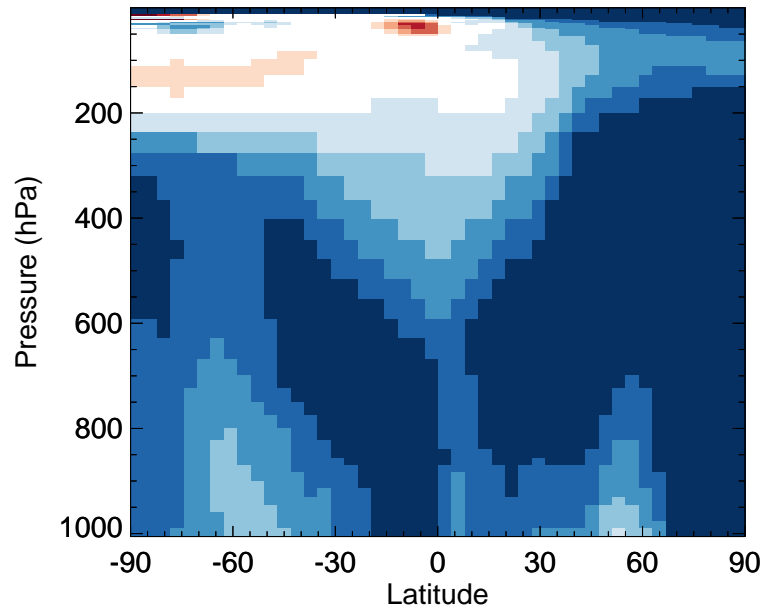
v11-02e-Run0 / v11-02d-Run1 HONIT - Zonal mean % diff for Jan
