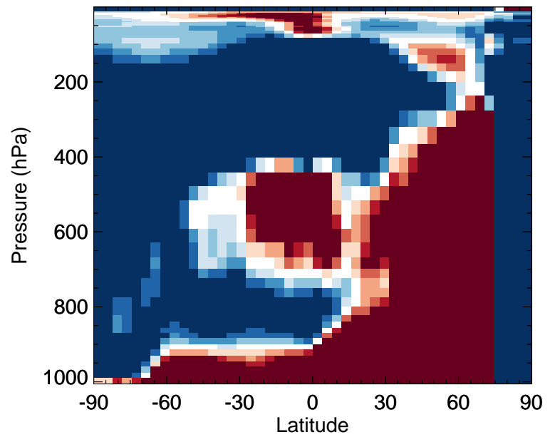
v11-02e-Run0 / v11-02c-Run0 Cl - Zonal mean % diff for Jan
