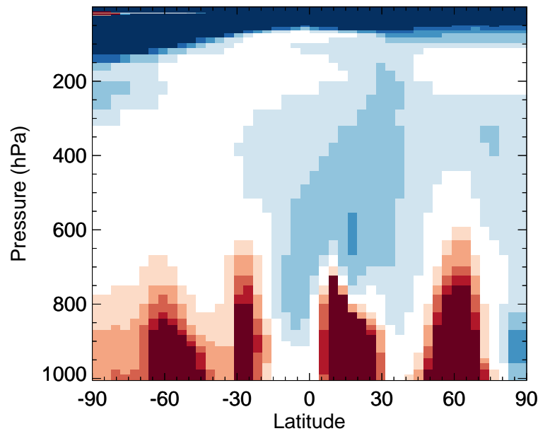
v11-02e-Run0 / v11-02c-Run0 R4N2 - Zonal mean % diff for Jan
