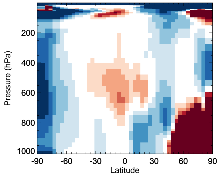
v11-02e-Run0 / v11-02c-Run0 DMS - Zonal mean % diff for Jan
