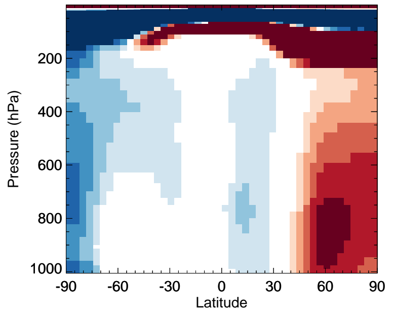
v11-02e-Run0 / v11-02c-Run0 ALD2 - Zonal mean % diff for Jan
