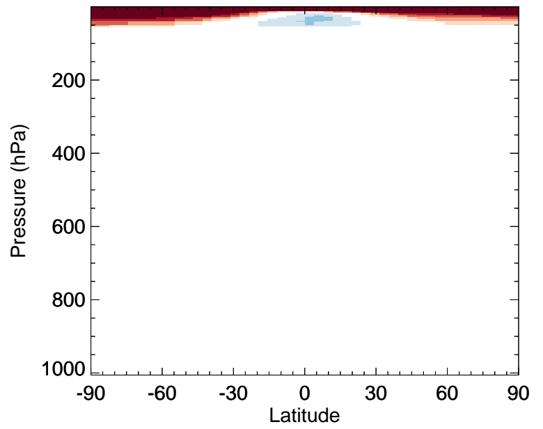
v11-02e-Run0 / v11-02d-Run1 ISO3 - Zonal mean % diff for Jan
