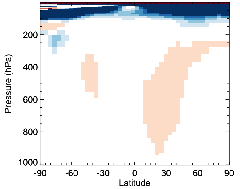
v11-02e-Run0 / v11-02d-Run1 GLYC - Zonal mean % diff for Jan
