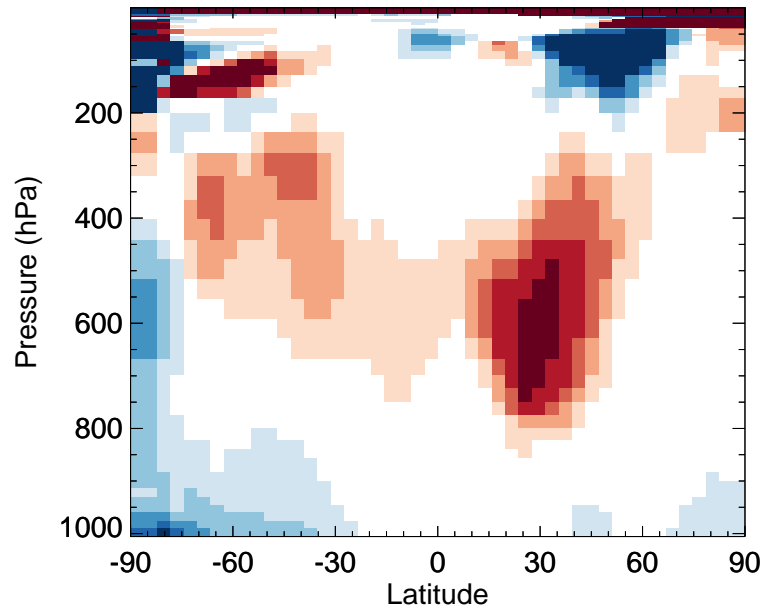
v11-02e-Run0 / v11-02d-Run1 RIPB - Zonal mean % diff for Jan
