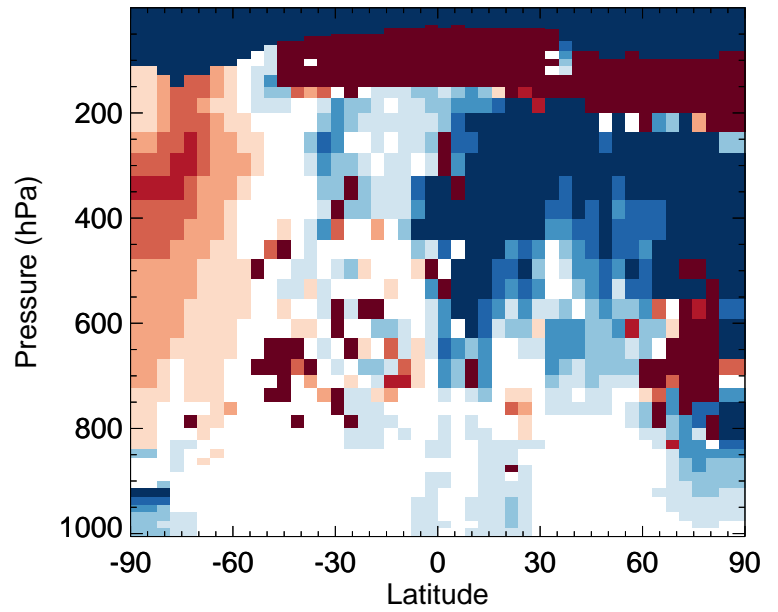
v11-02e-Run0 / v11-02d-Run1 NIT - Zonal mean % diff for Jan
