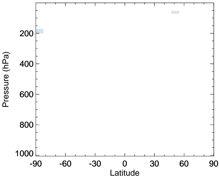
v11-02e-Run0 - v11-02d-Run1 BrO - Zonal mean abs diff for Jan
