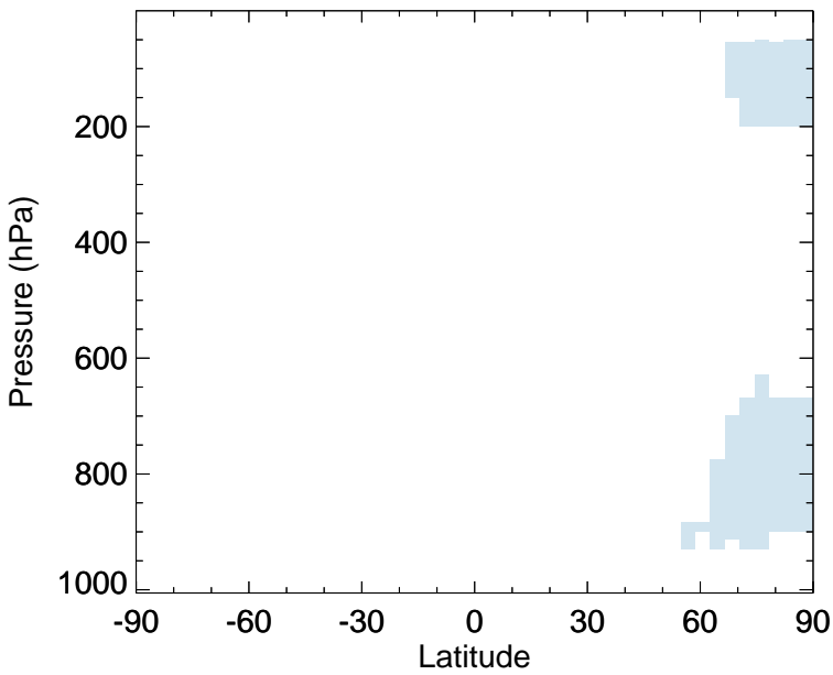
v11-02e-Run0 - v11-02c-Run0 HOBr - Zonal mean abs diff for Jan
