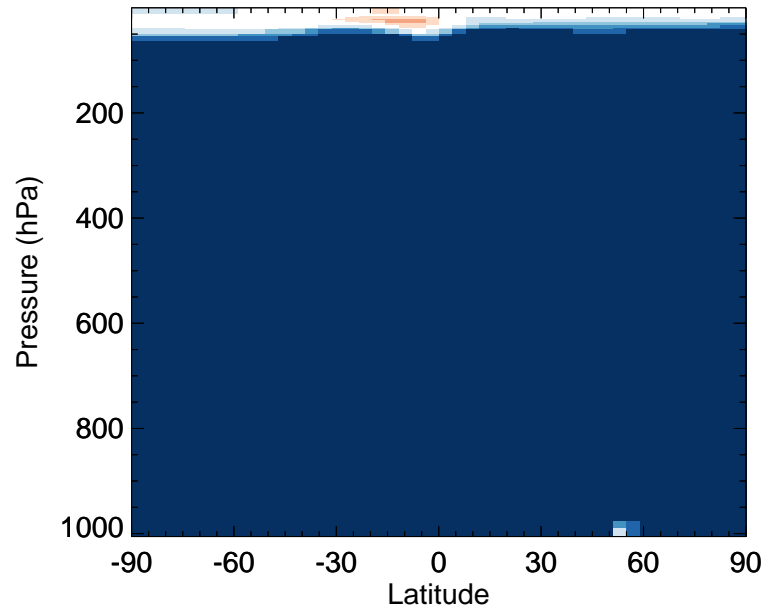
v11-02e-Run0 / v11-02c-Run0 HCl - Zonal mean % diff for Jan
