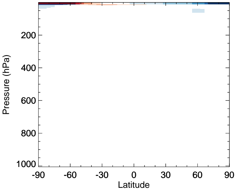
v11-02e-Run0 - v11-02c-Run0 ClO - Zonal mean abs diff for Jan
