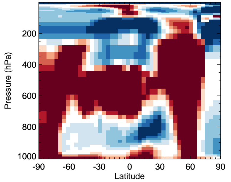
v11-02e-Run0 / v11-02d-Run1 ClOO - Zonal mean % diff for Jan
