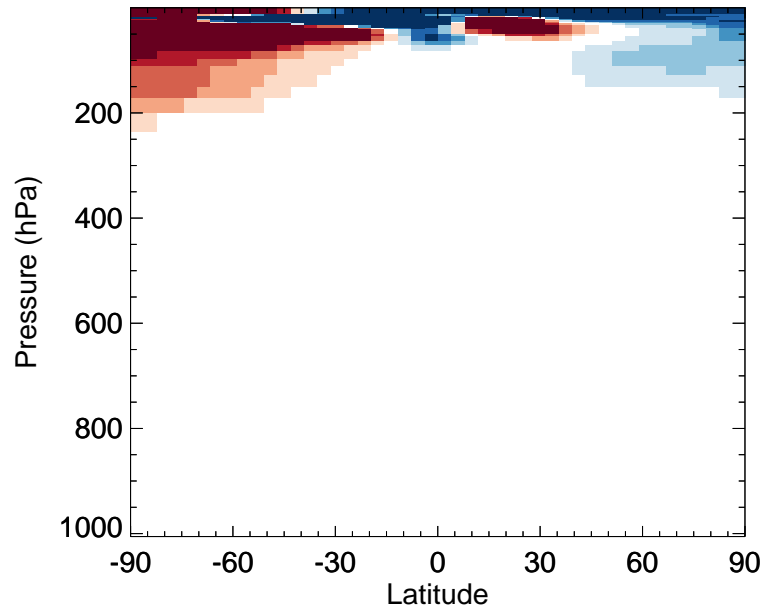
v11-02e-Run0 / v11-02d-Run1 C2H6 - Zonal mean % diff for Jan
