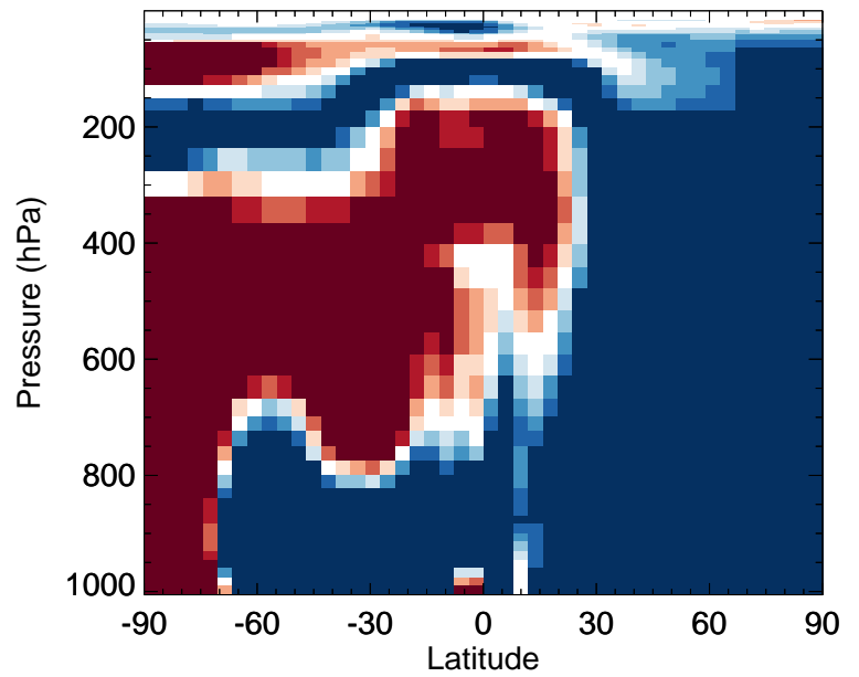
v11-02e-Run0 / v11-02c-Run0 HOBr - Zonal mean % diff for Jan
