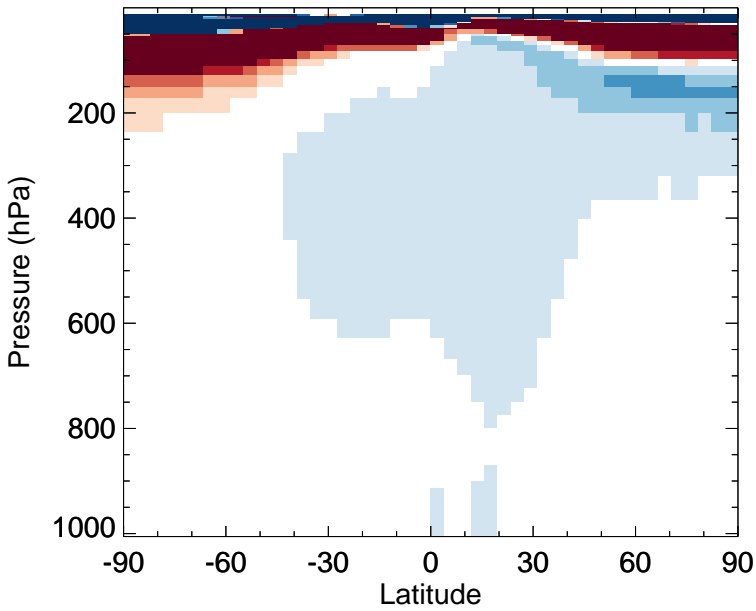
v11-02e-Run0 - v11-02c-Run0 O3 - Zonal mean abs diff for Jan
