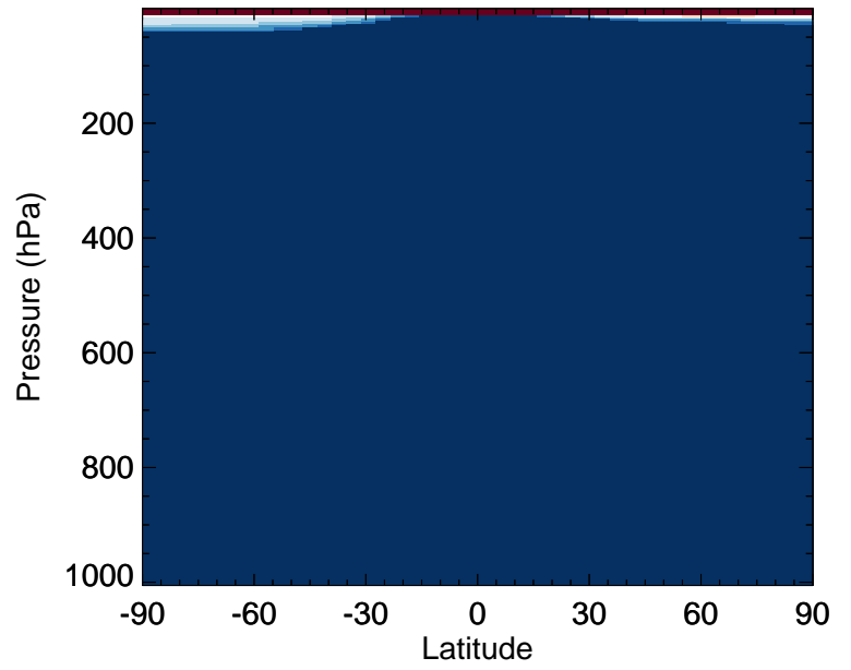
v11-02e-Run0 / v11-02d-Run1 ISO G 2 - Zonal mean % diff for Jan
