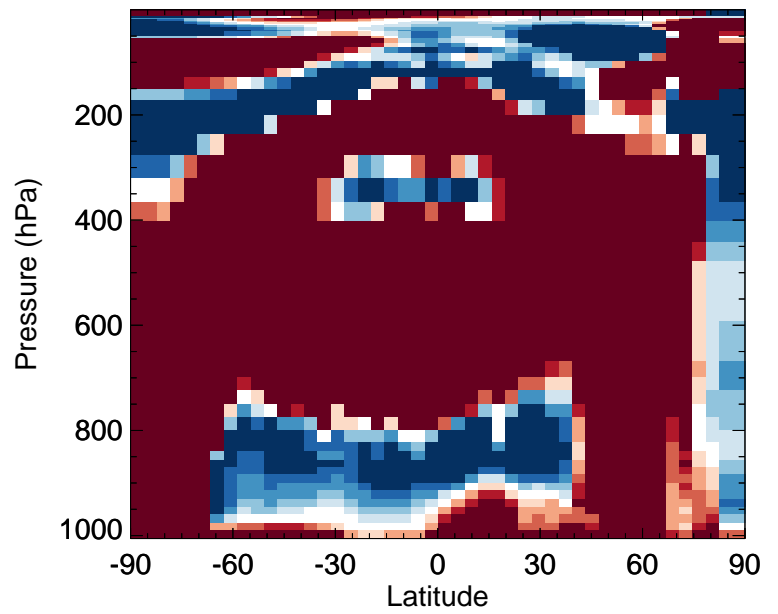
v11-02e-Run0 / v11-02d-Run1 Cl2O2 - Zonal mean % diff for Jan
