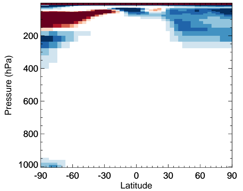
v11-02e-Run0 / v11-02d-Run1 HAC - Zonal mean % diff for Jan
