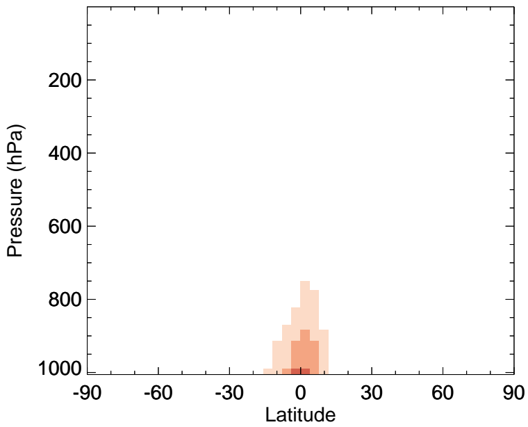
v11-02e-Run0 - v11-02d-Run1 MEK - Zonal mean abs diff for Jan
