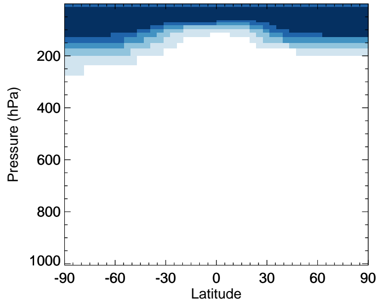
v11-02e-Run0 / v11-02c-Run0 BCPI - Zonal mean % diff for Jan
