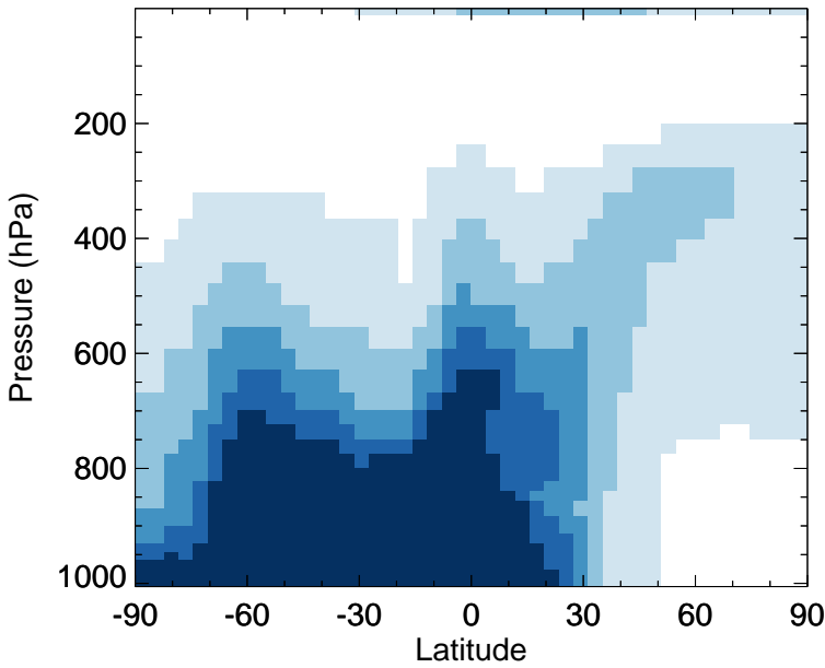
v11-02e-Run0 - v11-02c-Run0 MP - Zonal mean abs diff for Jan
