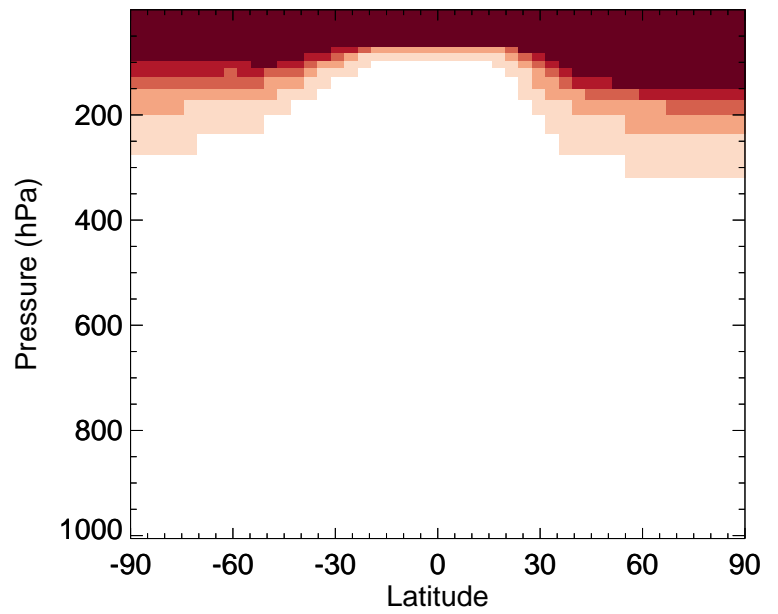
v11-02e-Run0 / v11-02d-Run1 ASOG1 - Zonal mean % diff for Jan
