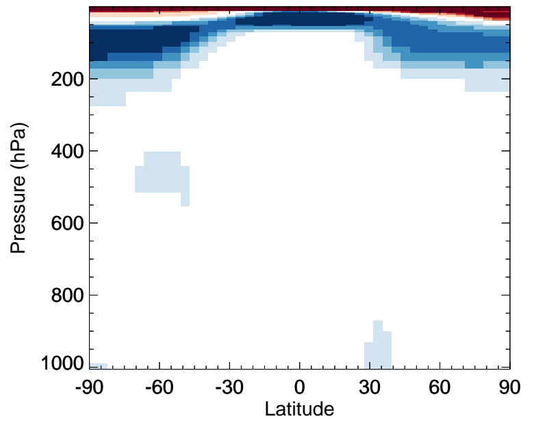
v11-02e-Run0 / v11-02d-Run1 TSOA2 - Zonal mean % diff for Jan
