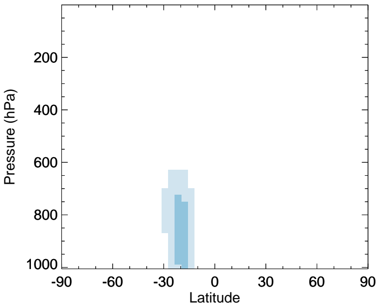
v11-02e-Run0 - v11-02c-Run0 SOAIE - Zonal mean abs diff for Jan
