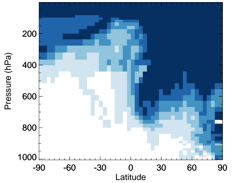
v11-02e-Run0 / v11-02d-Run1 NH3 - Zonal mean % diff for Jan
