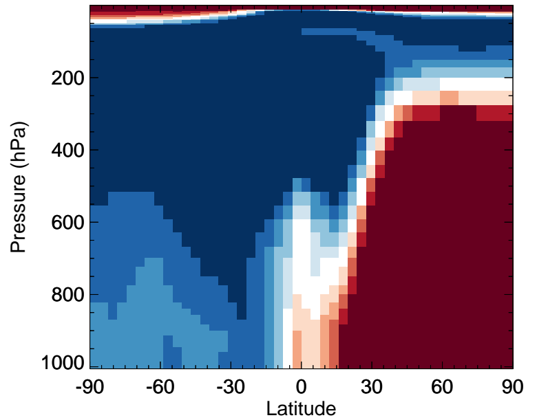
v11-02e-Run0 / v11-02c-Run0 SOAME - Zonal mean % diff for Jan
