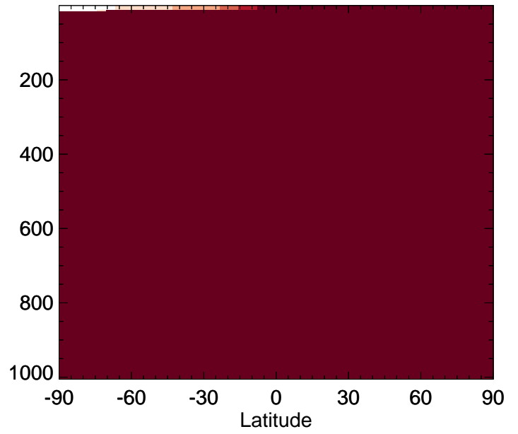
v11-02e-Run0 / v11-02d-Run1 DST1 - Zonal mean % diff for Jan
