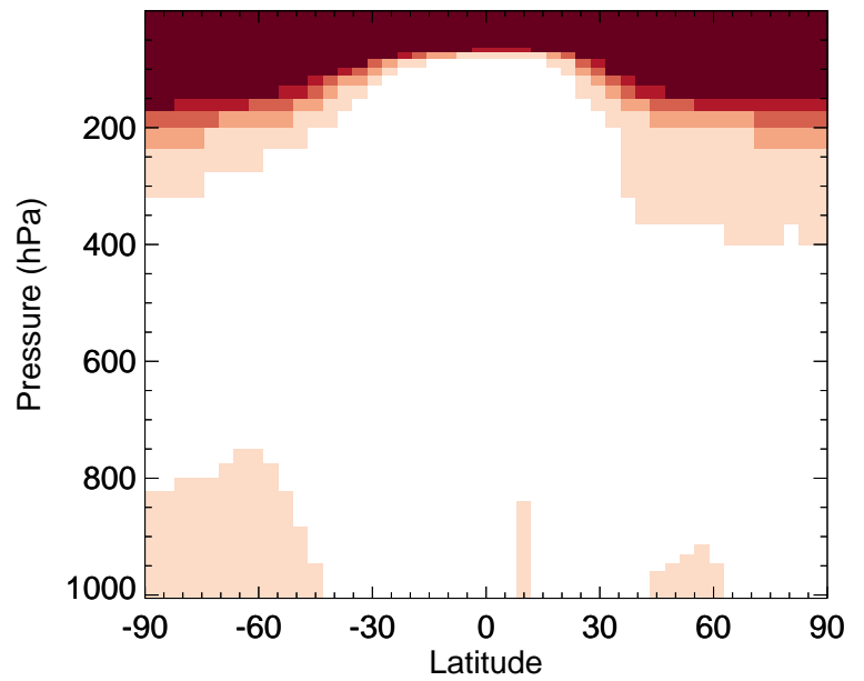
v11-02e-Run0 / v11-02c-Run0 ASOG3 - Zonal mean % diff for Jan
