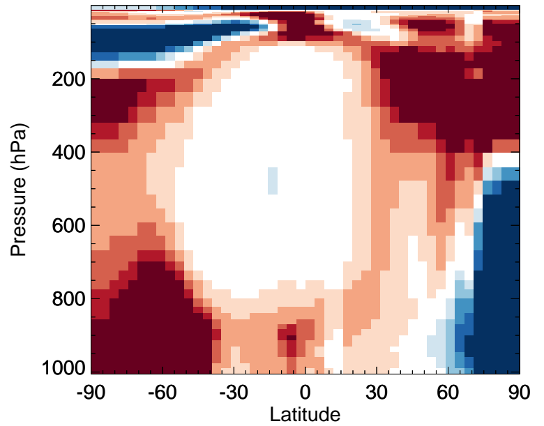
v11-02e-Run0 / v11-02c-Run0 NO - Zonal mean % diff for Jan
