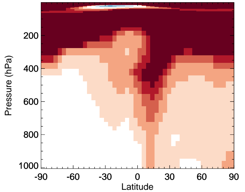
v11-02e-Run0 / v11-02c-Run0 SO4 - Zonal mean % diff for Jan
