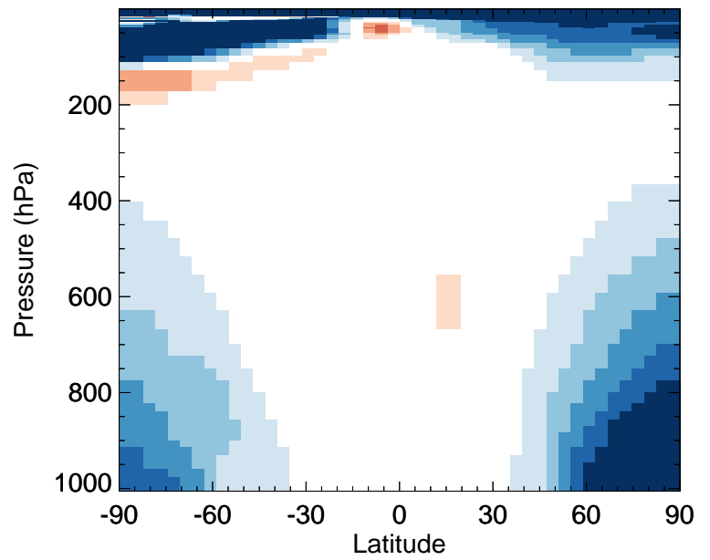
v11-02e-Run0 / v11-02d-Run1 IMAE - Zonal mean % diff for Jan
