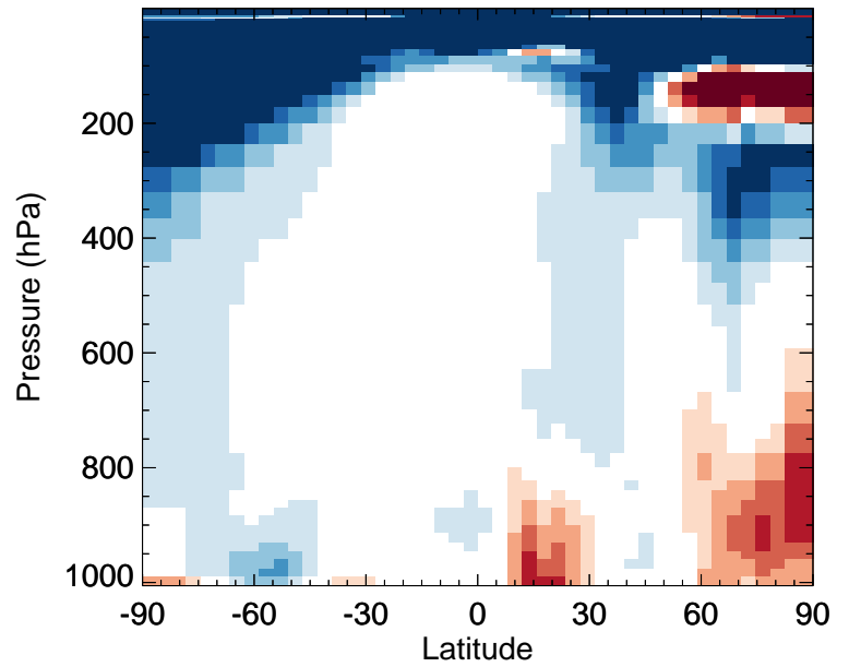
v11-02e-Run0 / v11-02c-Run0 ACTA - Zonal mean % diff for Jan
