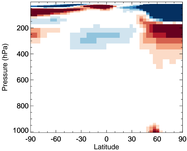
v11-02e-Run0 - v11-02c-Run0 HNO 4 - Zonal mean abs diff for Jan
