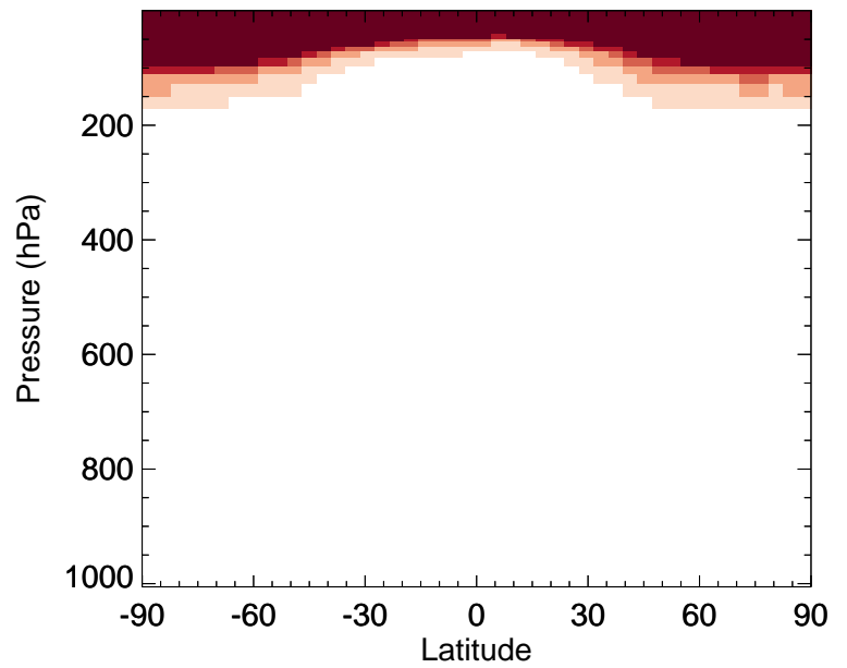
v11-02e-Run0 / v11-02c-Run0 SOAS - Zonal mean % diff for Jan
