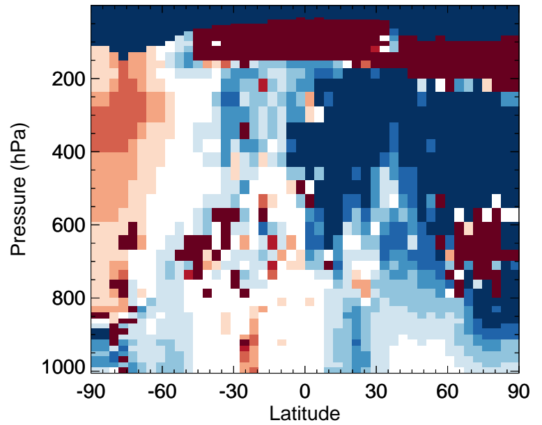
v11-02e-Run0 / v11-02c-Run0 NIT - Zonal mean % diff for Jan
