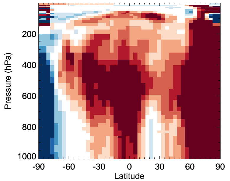
v11-02e-Run0 / v11-02c-Run0 MTPA - Zonal mean % diff for Jan
