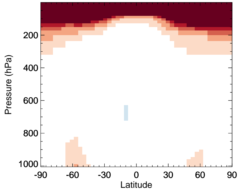
v11-02e-Run0 / v11-02c-Run0 ASOA3 - Zonal mean % diff for Jan
