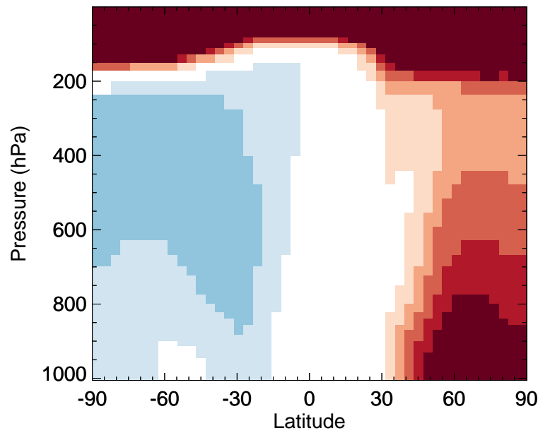
v11-02e-Run0 / v11-02c-Run0 INDIOL - Zonal mean % diff for Jan
