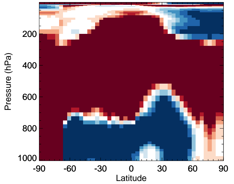
v11-02e-Run0 / v11-02d-Run1 BrCl - Zonal mean % diff for Jan
