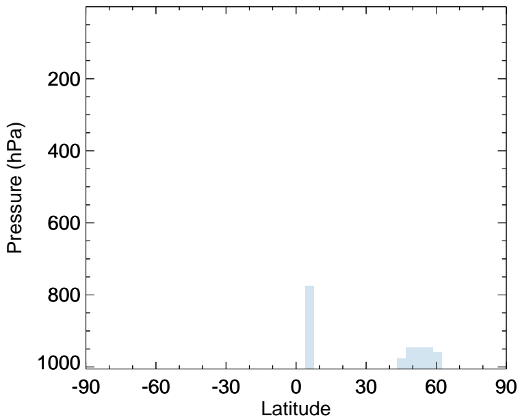
v11-02e-Run0 - v11-02c-Run0 EOH - Zonal mean abs diff for Jan
