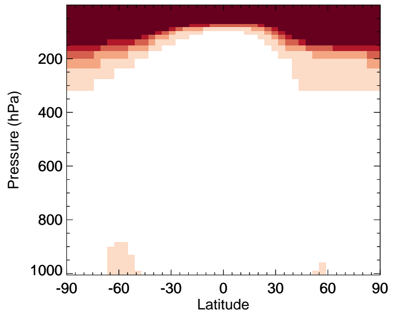
v11-02e-Run0 / v11-02c-Run0 ASOA1 - Zonal mean % diff for Jan
