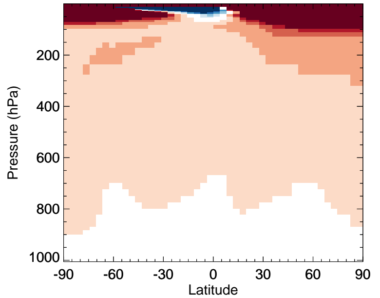
v11-02e-Run0 / v11-02c-Run0 CCI4 - Zonal mean % diff for Jan
