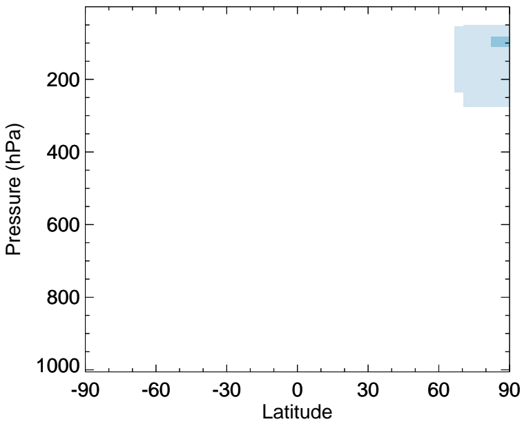
v11-02e-Run0 - v11-02d-Run1 HOBr - Zonal mean abs diff for Jan
