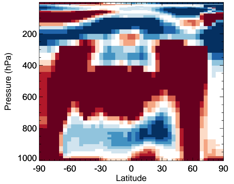
v11-02e-Run0 / v11-02d-Run1 ClO - Zonal mean % diff for Jan
