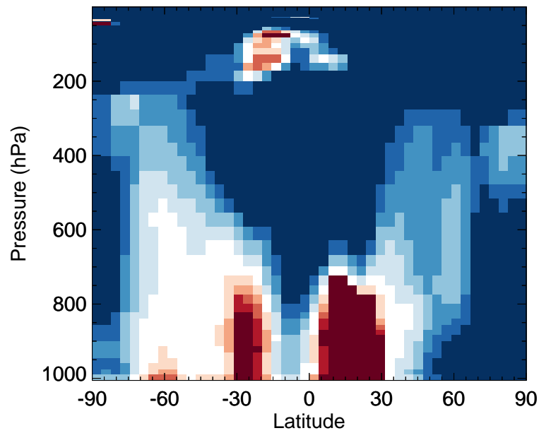
v11-02e-Run0 / v11-02c-Run0 ISN1OG - Zonal mean % diff for Jan
