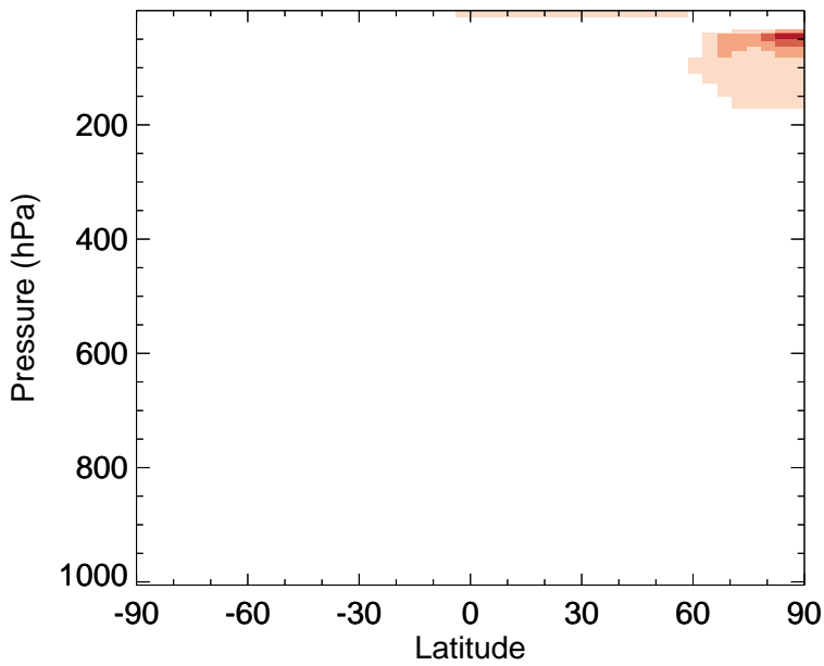
v11-02e-Run0 - v11-02c-Run0 HOCl - Zonal mean abs diff for Jan
