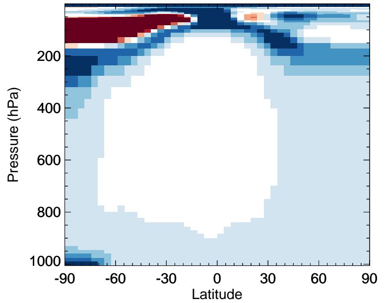
v11-02e-Run0 / v11-02d-Run1 MP - Zonal mean % diff for Jan
