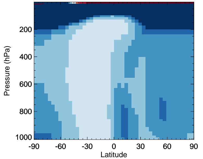
v11-02e-Run0 / v11-02c-Run0 ALK4 - Zonal mean % diff for Jan
