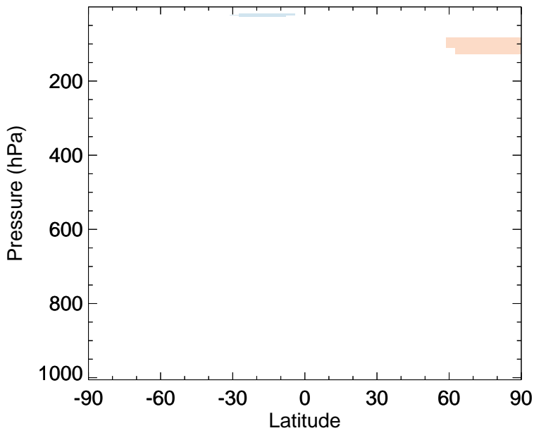
v11-02e-Run0 - v11-02d-Run1 MPN - Zonal mean abs diff for Jan
