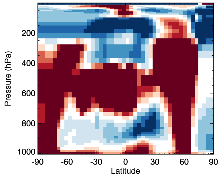
v11-02e-Run0 / v11-02d-Run1 Cl - Zonal mean % diff for Jan
