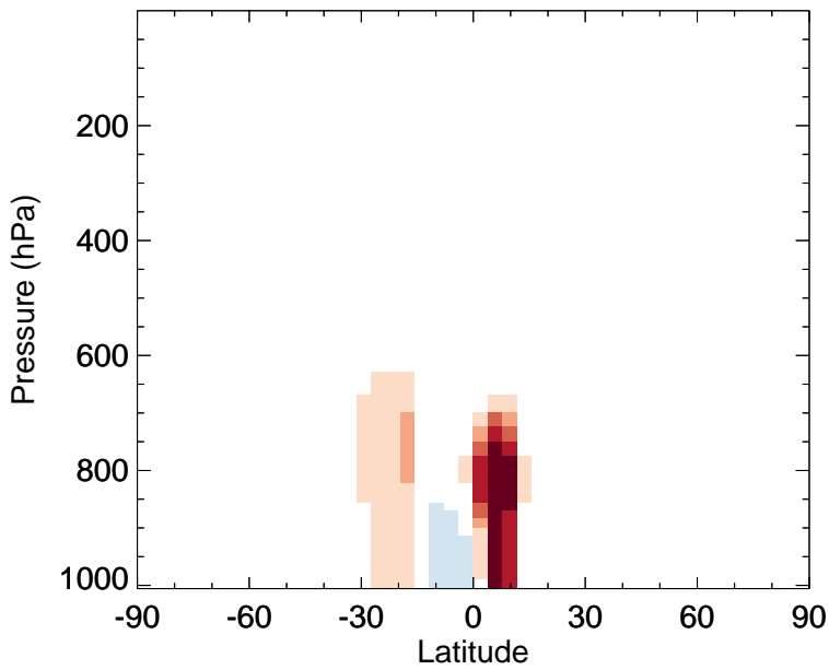
v11-02e-Run0 - v11-02c-Run0 MAP - Zonal mean abs diff for Jan
