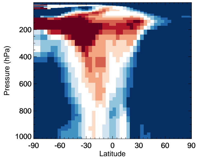
v11-02e-Run0 / v11-02c-Run0 IEPOXB - Zonal mean % diff for Jan
