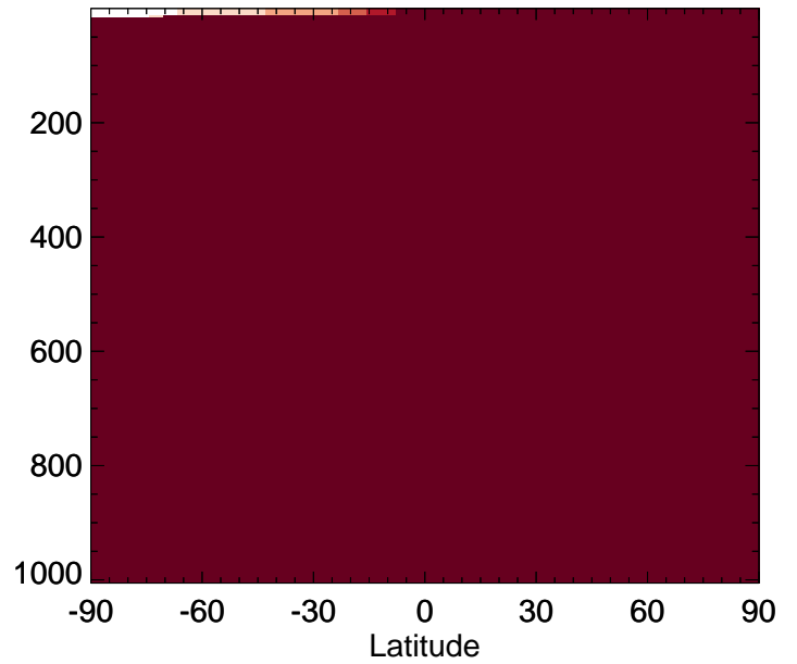
v11-02e-Run0 / v11-02c-Run0 DST1 - Zonal mean % diff for Jan
