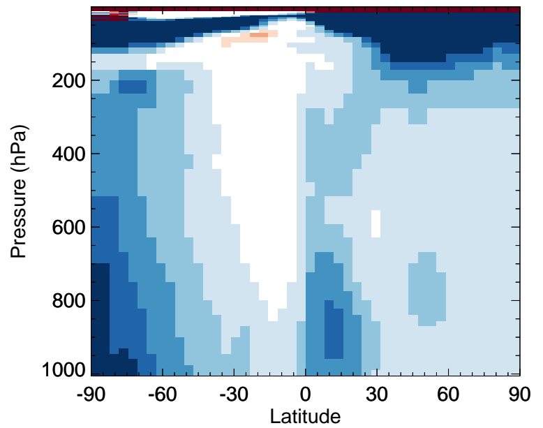
v11-02e-Run0 / v11-02c-Run0 TOLU - Zonal mean % diff for Jan
