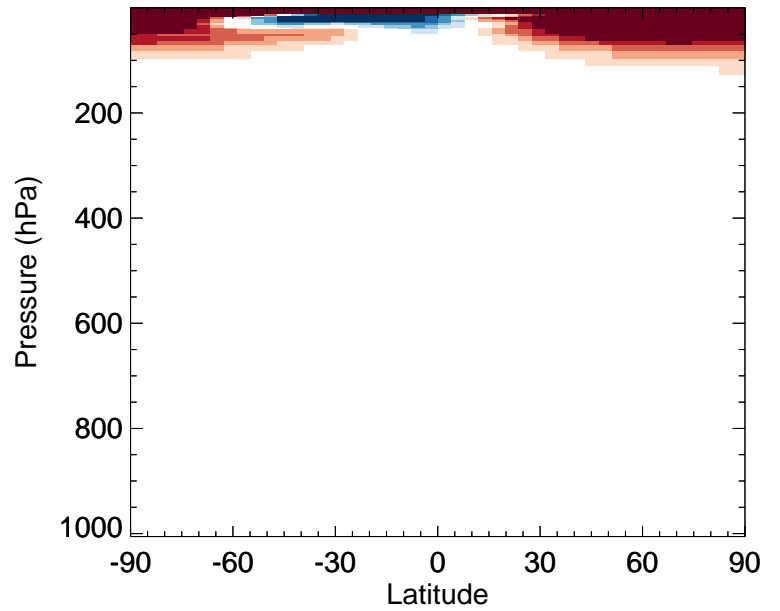
v11-02e-Run0 / v11-02c-Run0 CFC12 - Zonal mean % diff for Jan
