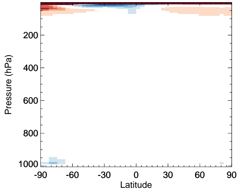
v11-02e-Run0 / v11-02c-Run0 CH4 - Zonal mean % diff for Jan
