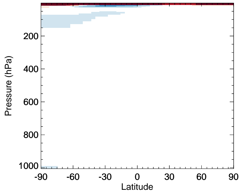
v11-02e-Run0 / v11-02c-Run0 CO - Zonal mean % diff for Jan
