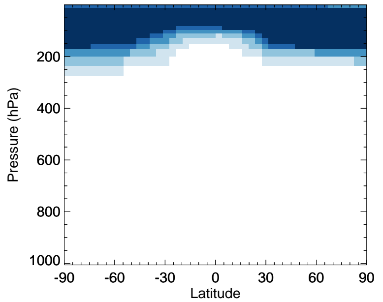
v11-02e-Run0 / v11-02d-Run1 OCPI - Zonal mean % diff for Jan
