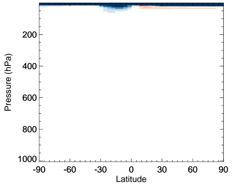
v11-02e-Run0 / v11-02d-Run1 ACET - Zonal mean % diff for Jan
