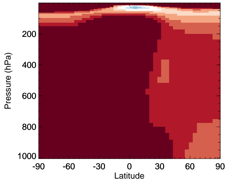
v11-02e-Run0 / v11-02d-Run1 SOAGX - Zonal mean % diff for Jan
