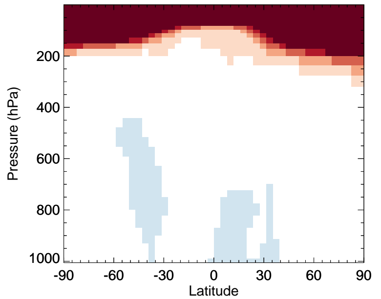
v11-02e-Run0 / v11-02c-Run0 TSOA2 - Zonal mean % diff for Jan
