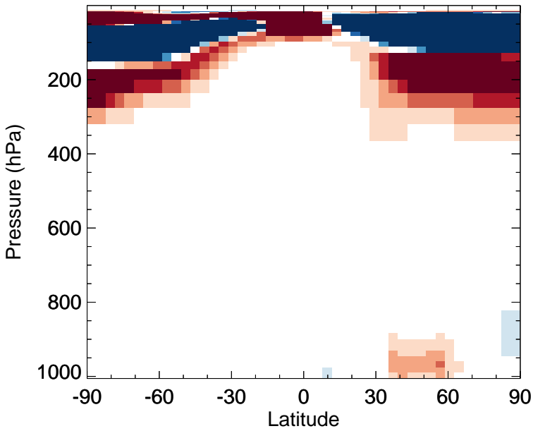
v11-02e-Run0 - v11-02c-Run0 HNO 3 - Zonal mean abs diff for Jan
