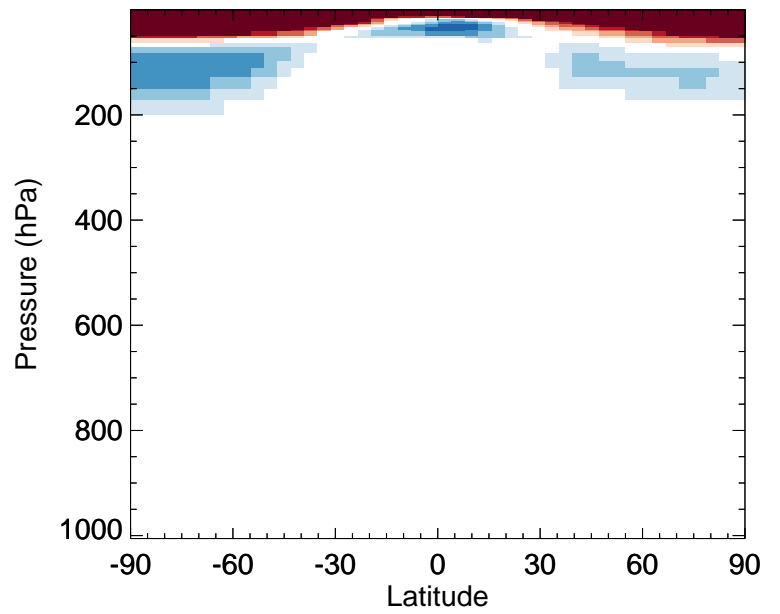
v11-02e-Run0 / v11-02d-Run1 ASOA2 - Zonal mean % diff for Jan
