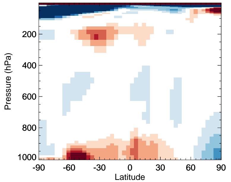
v11-02e-Run0 / v11-02c-Run0 GLYX - Zonal mean % diff for Jan
