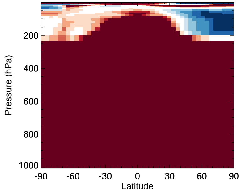
v11-02e-Run0 / v11-02c-Run0 BrCl - Zonal mean % diff for Jan
