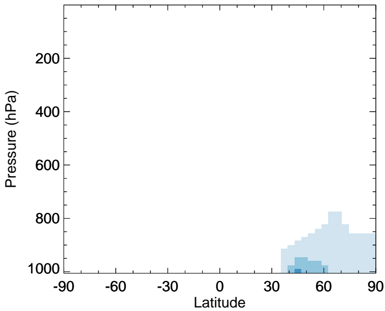
v11-02e-Run0 - v11-02c-Run0 XYLE - Zonal mean abs diff for Jan
