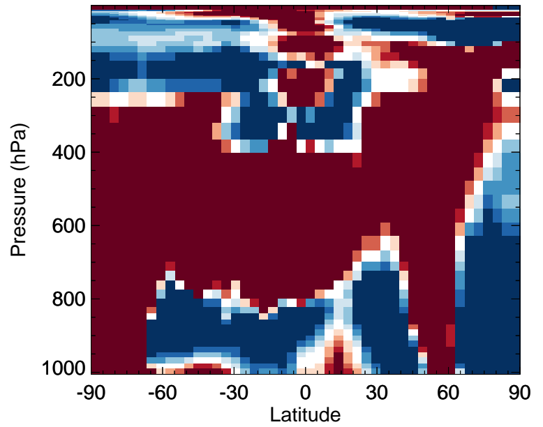
v11-02e-Run0 / v11-02d-Run1 Cl2 - Zonal mean % diff for Jan
