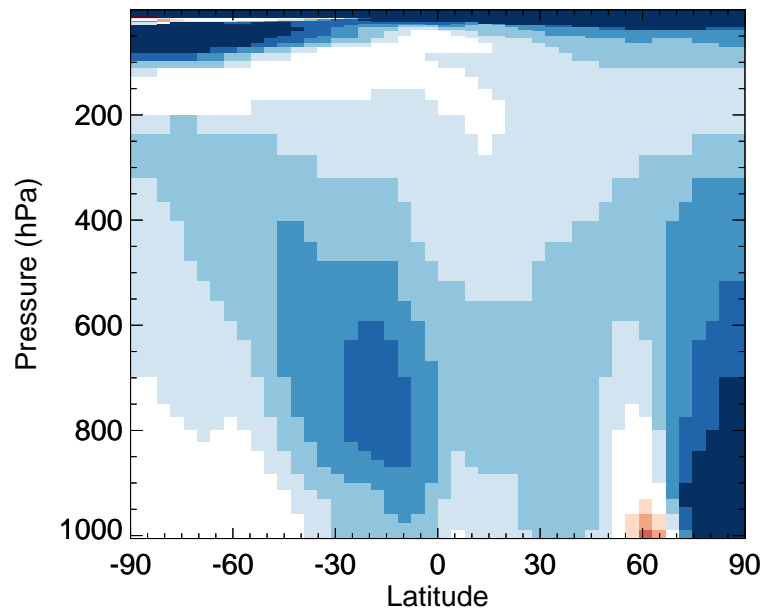
v11-02e-Run0 / v11-02d-Run1 R4N2 - Zonal mean % diff for Jan
