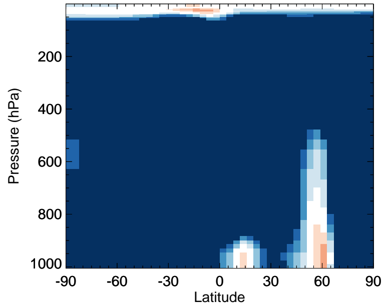
v11-02e-Run0 / v11-02d-Run1 HCl - Zonal mean % diff for Jan
