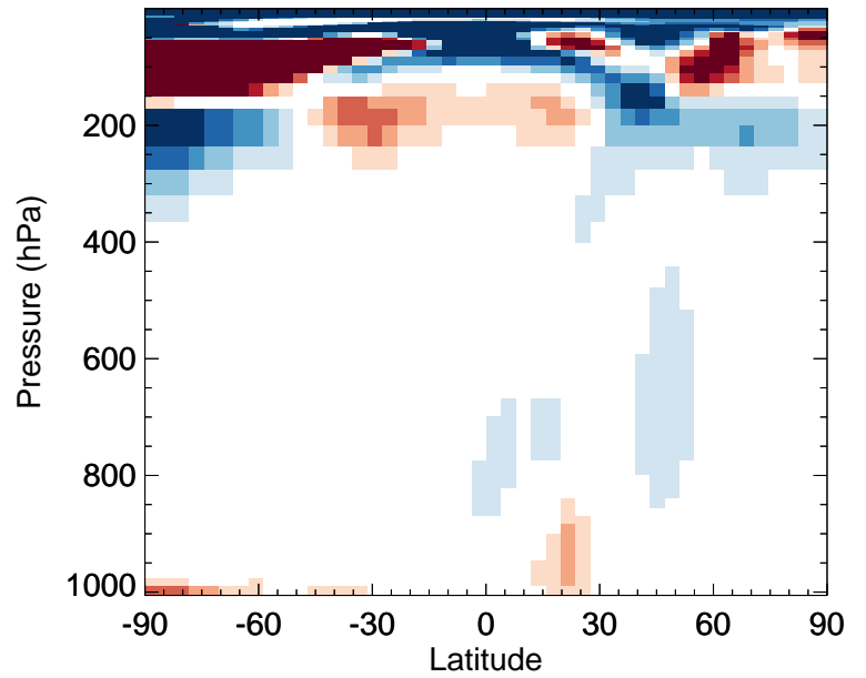
v11-02e-Run0 / v11-02c-Run0 MGLY - Zonal mean % diff for Jan
