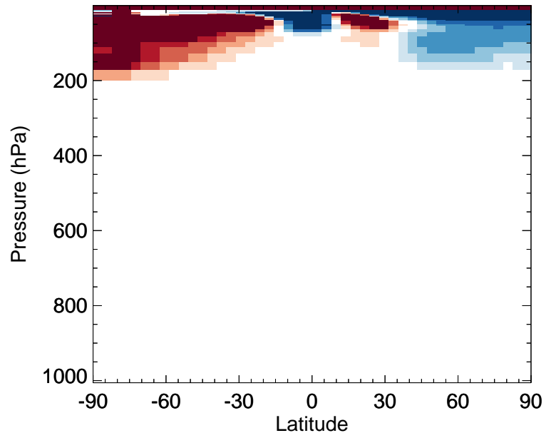
v11-02e-Run0 / v11-02d-Run1 ALK4 - Zonal mean % diff for Jan
