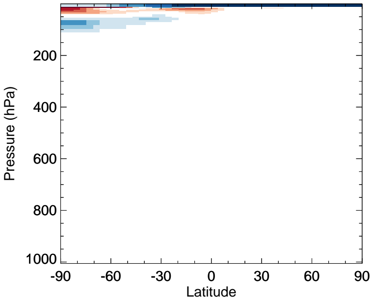
v11-02e-Run0 - v11-02c-Run0 NO - Zonal mean abs diff for Jan
