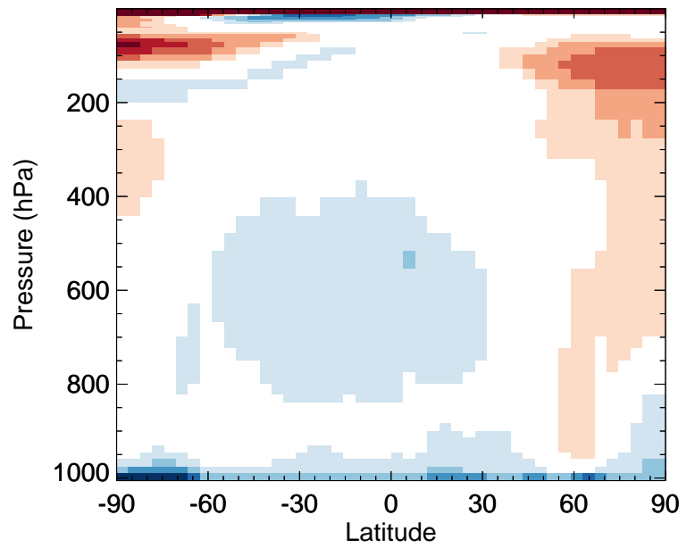
v11-02e-Run0 / v11-02d-Run1 MPN - Zonal mean % diff for Jan
