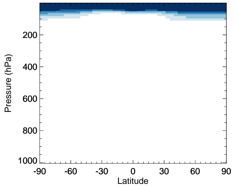
v11-02e-Run0 / v11-02c-Run0 SALA - Zonal mean % diff for Jan
