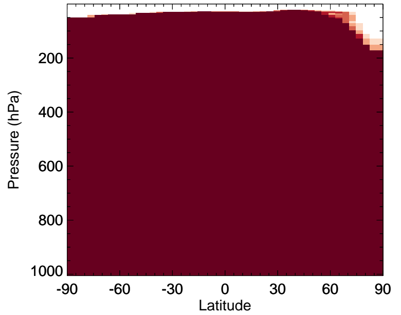
v11-02e-Run0 / v11-02c-Run0 DST4 - Zonal mean % diff for Jan
