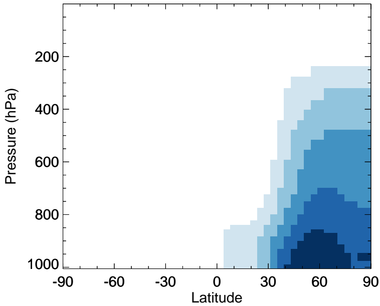
v11-02e-Run0 - v11-02c-Run0 ALK4 - Zonal mean abs diff for Jan
