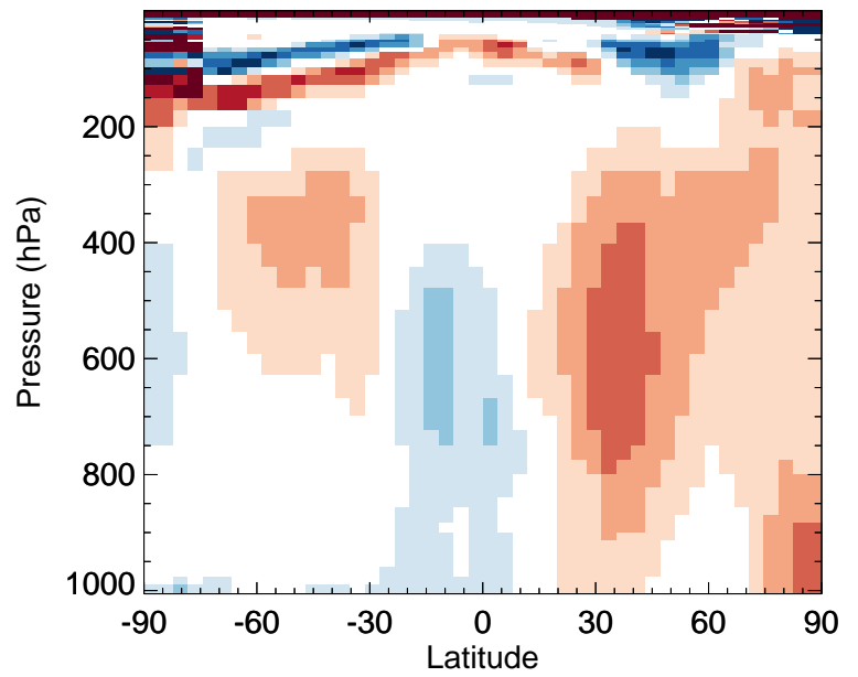
v11-02e-Run0 / v11-02d-Run1 ISN1 - Zonal mean % diff for Jan
