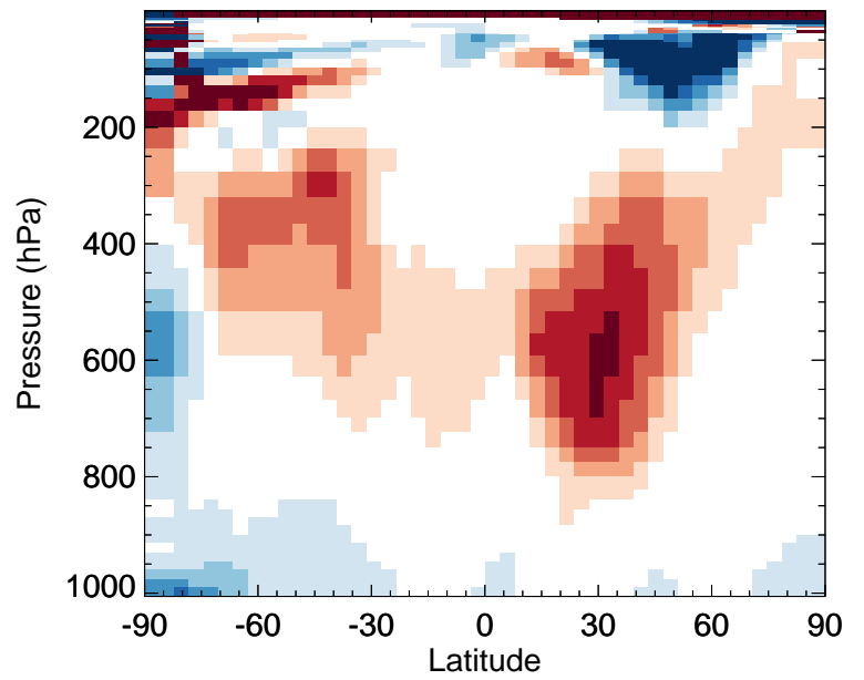
v11-02e-Run0 / v11-02d-Run1 RIPA - Zonal mean % diff for Jan
