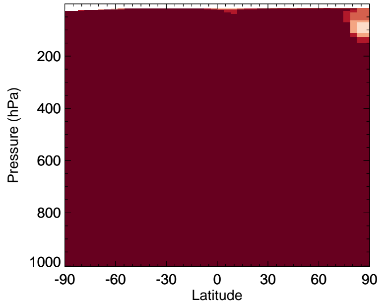
v11-02e-Run0 / v11-02d-Run1 DST3 - Zonal mean % diff for Jan
