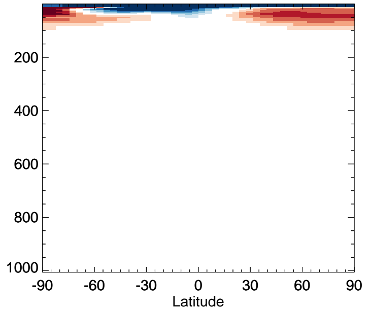
v11-02e-Run0 / v11-02c-Run0 N2O - Zonal mean % diff for Jan
