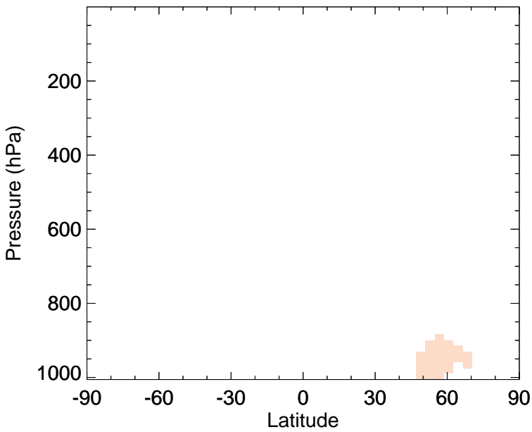
v11-02e-Run0 - v11-02c-Run0 ACET - Zonal mean abs diff for Jan
