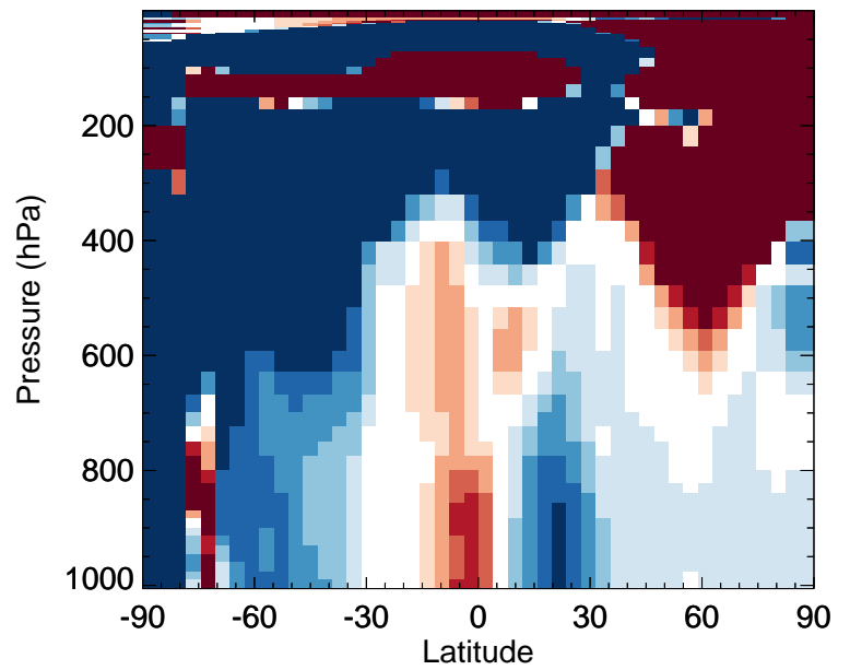
v11-02e-Run0 / v11-02c-Run0 IPMN - Zonal mean % diff for Jan
