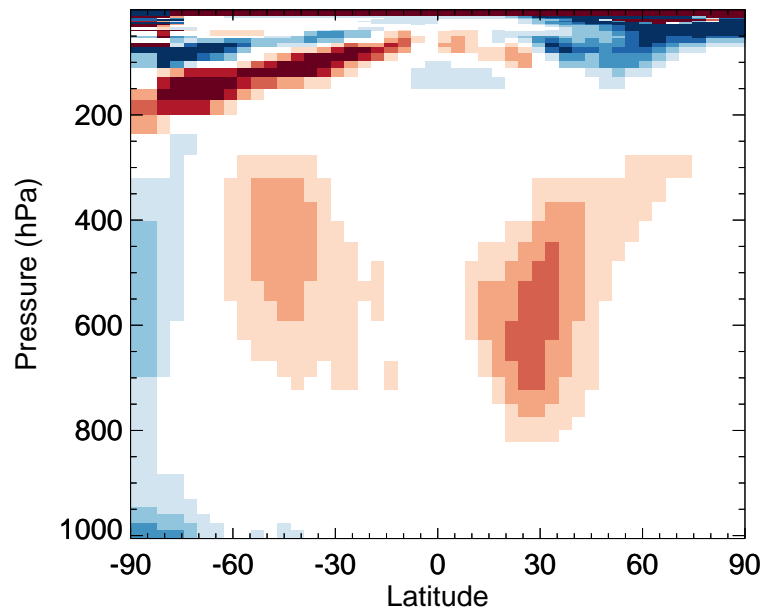
v11-02e-Run0 / v11-02d-Run1 PRPE - Zonal mean % diff for Jan
