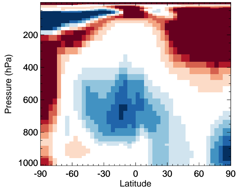
v11-02e-Run0 / v11-02d-Run1 N2O5 - Zonal mean % diff for Jan
