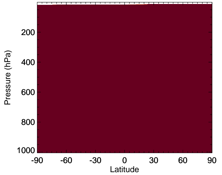
v11-02e-Run0 / v11-02d-Run1 DST2 - Zonal mean % diff for Jan
