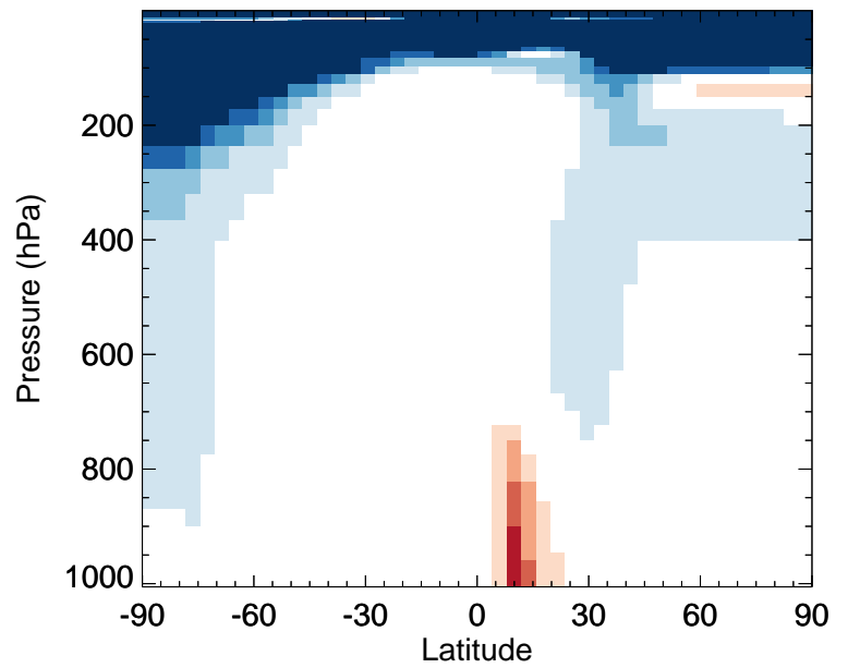
v11-02e-Run0 / v11-02c-Run0 MAP - Zonal mean % diff for Jan
