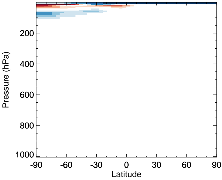
v11-02e-Run0 - v11-02d-Run1 NO - Zonal mean abs diff for Jan
