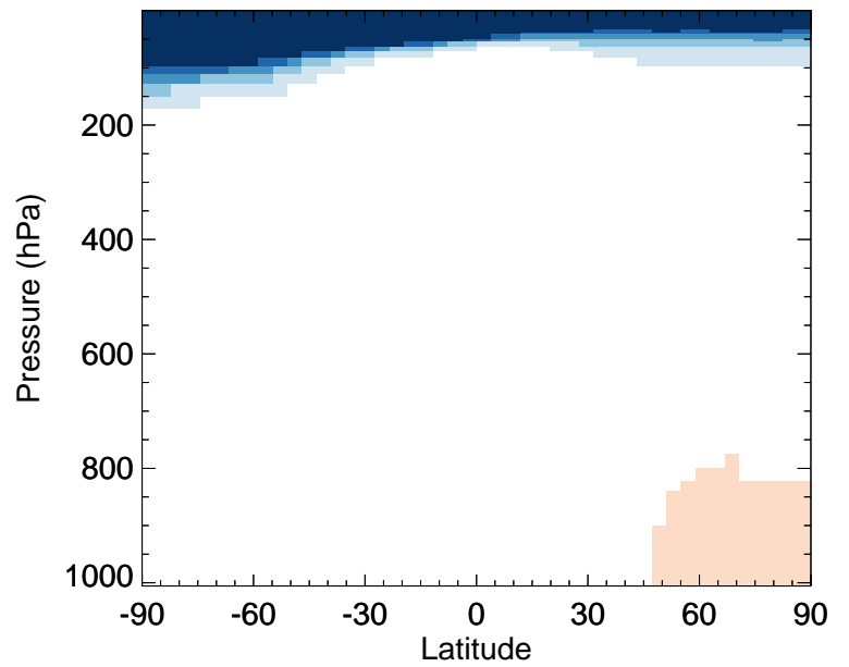
v11-02e-Run0 / v11-02c-Run0 ACET - Zonal mean % diff for Jan
