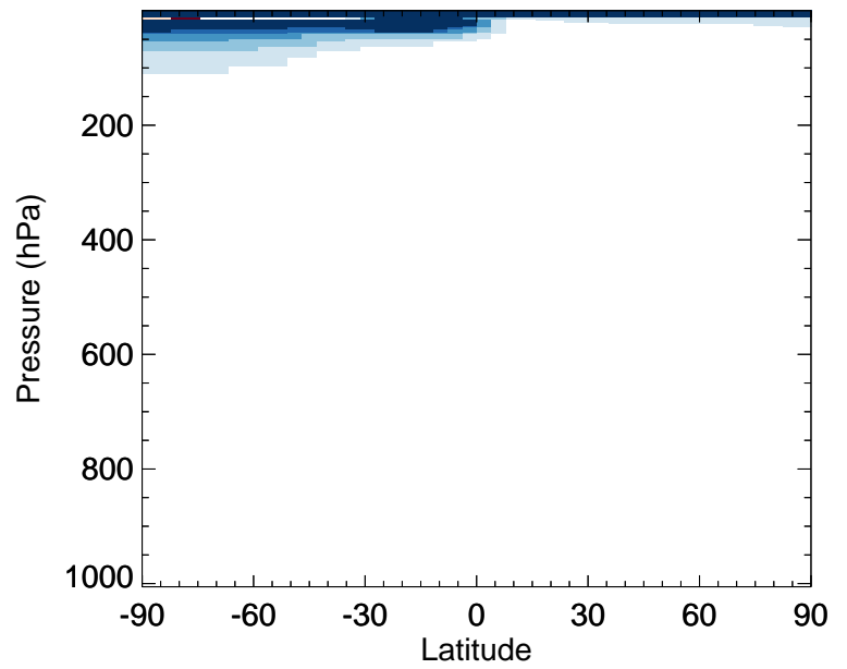
v11-02e-Run0 / v11-02d-Run1 CH 2 Br 2 - Zonal mean % diff for Jan
