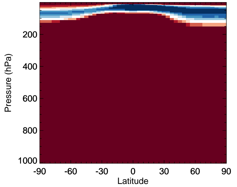
v11-02e-Run0 / v11-02d-Run1 SOAME - Zonal mean % diff for Jan
