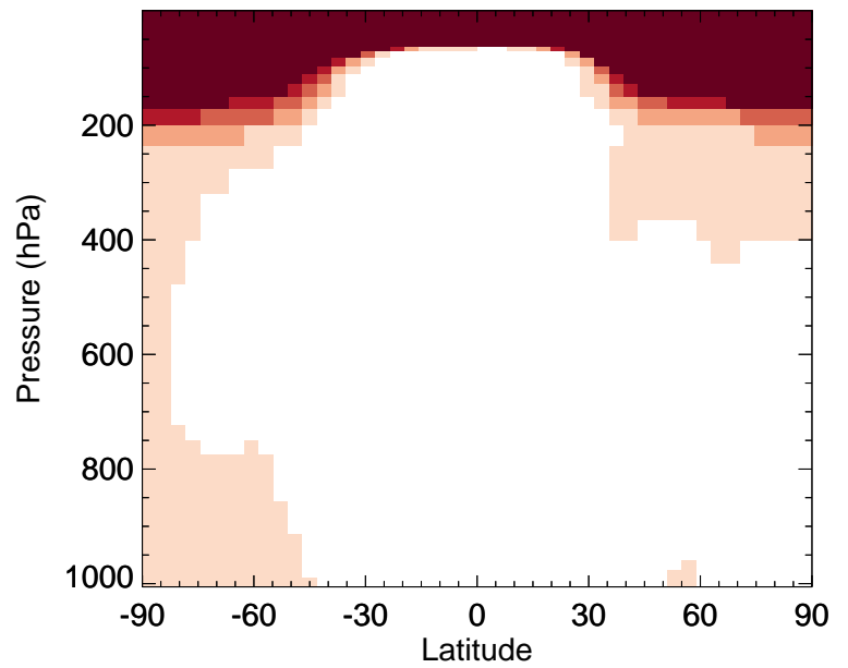
v11-02e-Run0 / v11-02c-Run0 ASOG1 - Zonal mean % diff for Jan
