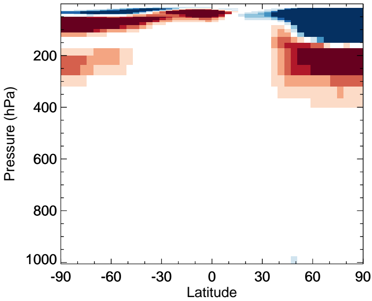
v11-02e-Run0 - v11-02d-Run1 HNO 4 - Zonal mean abs diff for Jan
