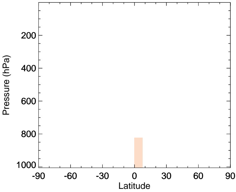
v11-02e-Run0 - v11-02d-Run1 DST1 - Zonal mean abs diff for Jan
