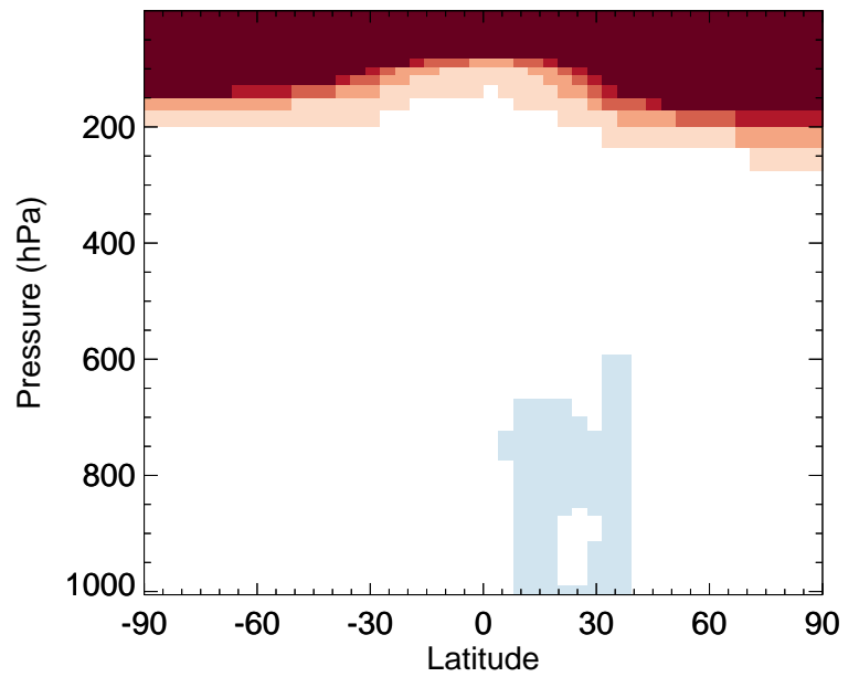
v11-02e-Run0 / v11-02c-Run0 TSOA3 - Zonal mean % diff for Jan
