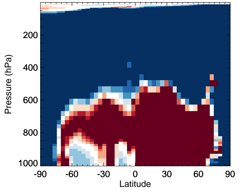
v11-02e-Run0 / v11-02d-Run1 HBr - Zonal mean % diff for Jan
