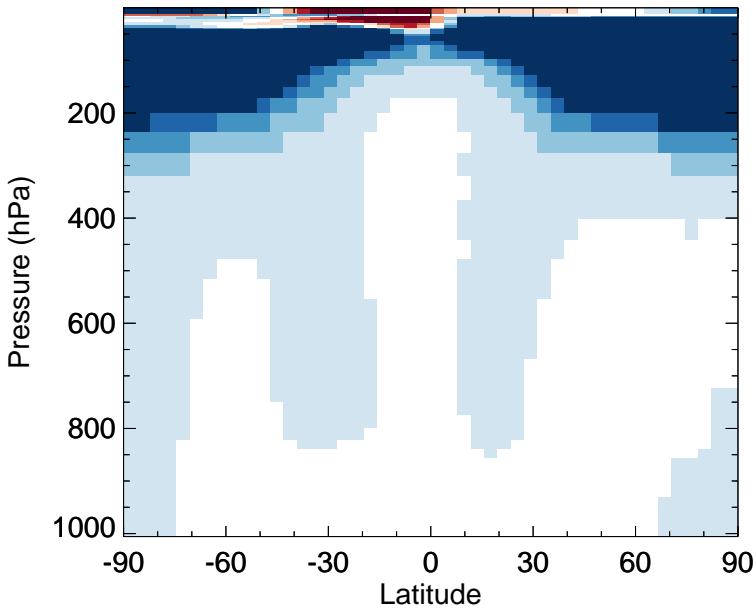
v11-02e-Run0 - v11-02c-Run0 HCl - Zonal mean abs diff for Jan
