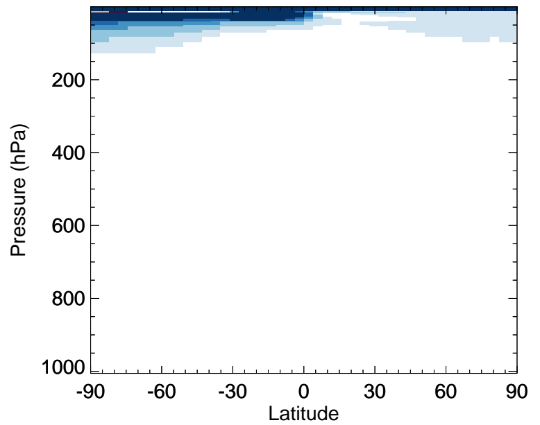
v11-02e-Run0 / v11-02c-Run0 CH 2 Br 2 - Zonal mean % diff for Jan
