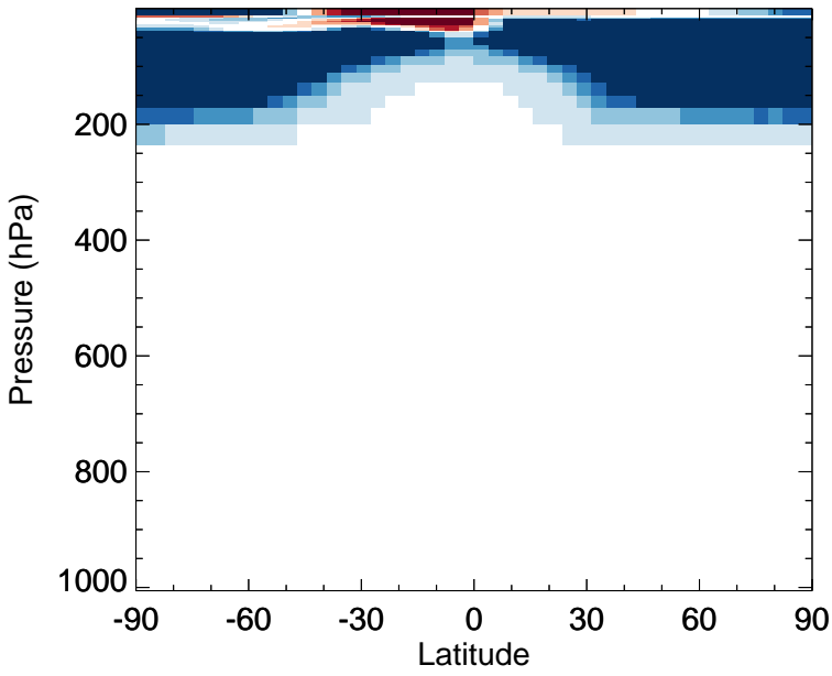
v11-02e-Run0 - v11-02d-Run1 HCl - Zonal mean abs diff for Jan
