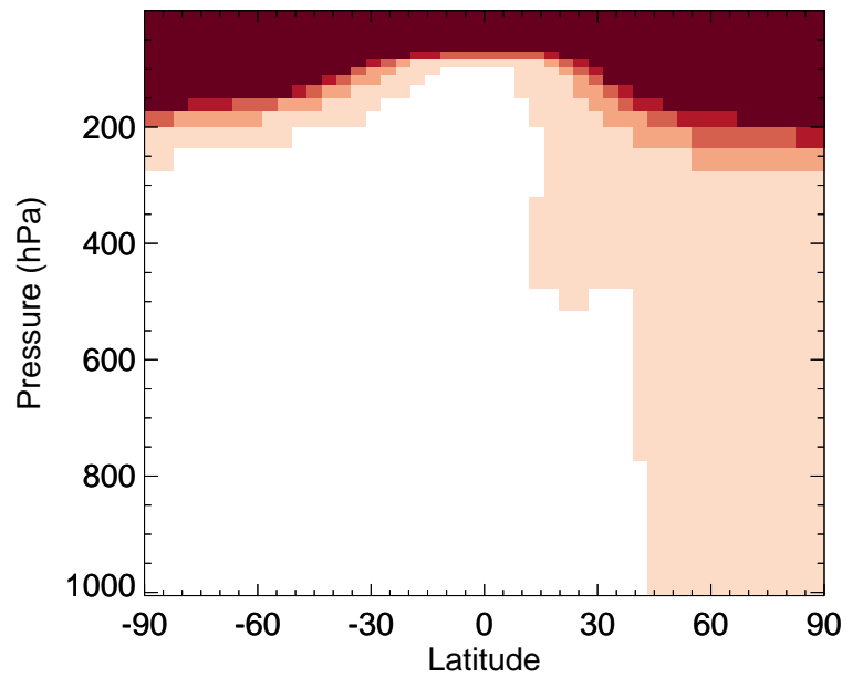
v11-02e-Run0 / v11-02c-Run0 ISO3 - Zonal mean % diff for Jan
