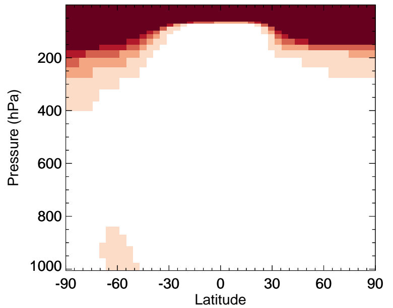
v11-02e-Run0 / v11-02c-Run0 ASOG2 - Zonal mean % diff for Jan
