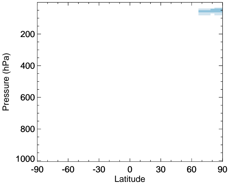
v11-02e-Run0 - v11-02c-Run0 Cl2 - Zonal mean abs diff for Jan
