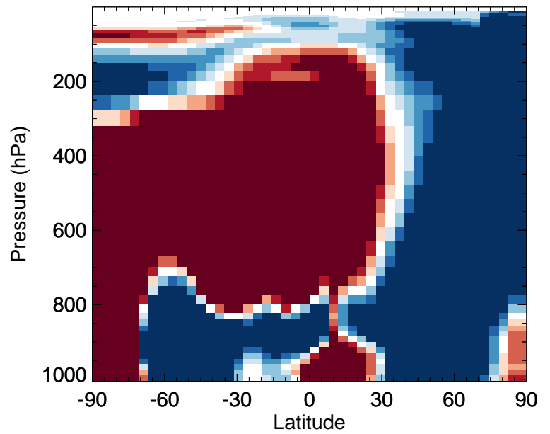
v11-02e-Run0 / v11-02c-Run0 BrO - Zonal mean % diff for Jan
