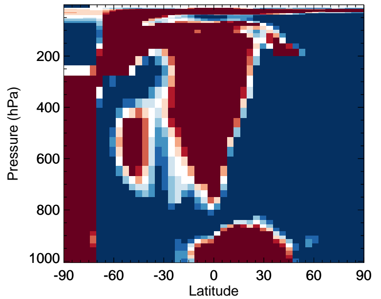
v11-02e-Run0 / v11-02c-Run0 Br2 - Zonal mean % diff for Jan
