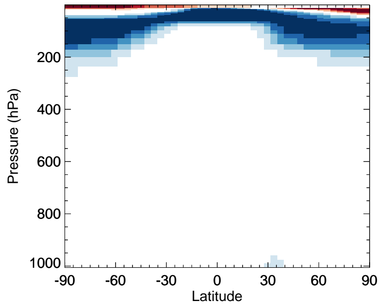
v11-02e-Run0 / v11-02d-Run1 TSOA3 - Zonal mean % diff for Jan
