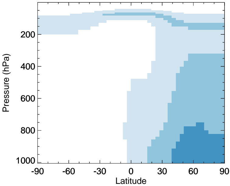
v11-02e-Run0 - v11-02c-Run0 C2H6 - Zonal mean abs diff for Jan
