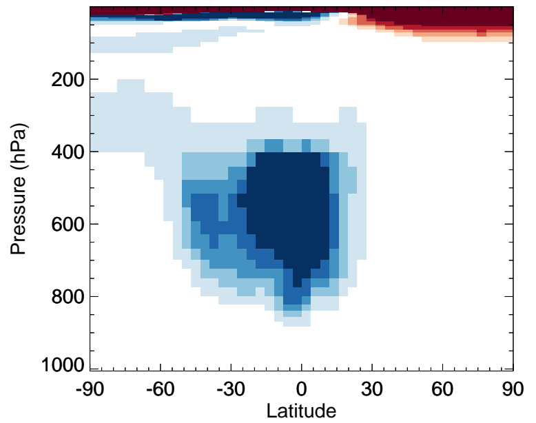
v11-02e-Run0 / v11-02d-Run1 SO 2 - Zonal mean % diff for Jan
