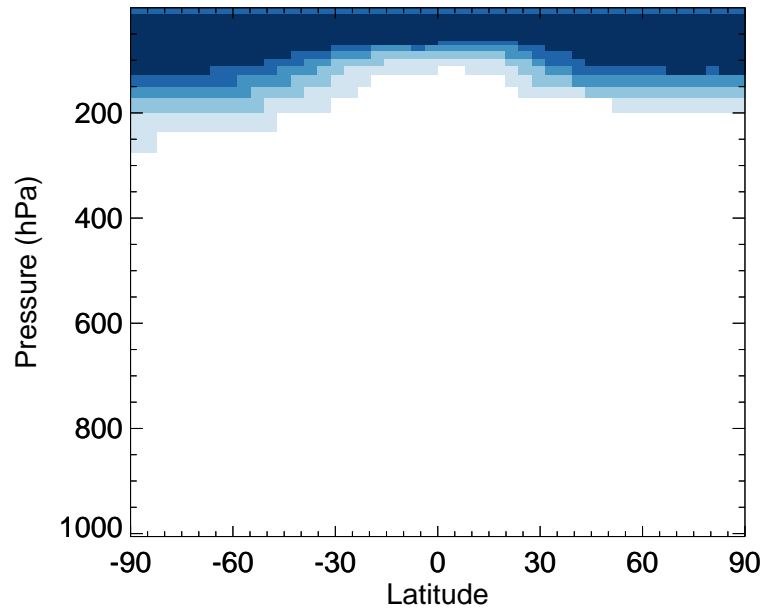
v11-02e-Run0 / v11-02d-Run1 BCPI - Zonal mean % diff for Jan
