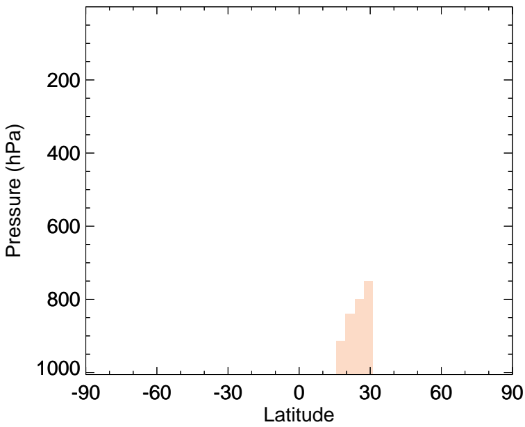
v11-02e-Run0 - v11-02d-Run1 TOLU - Zonal mean abs diff for Jan
