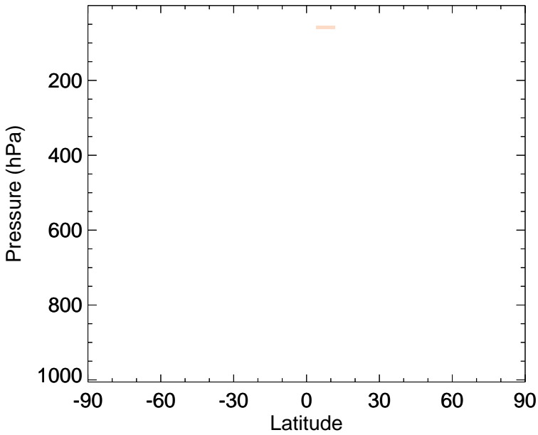
v11-02e-Run0 - v11-02c-Run0 SO4 - Zonal mean abs diff for Jan
