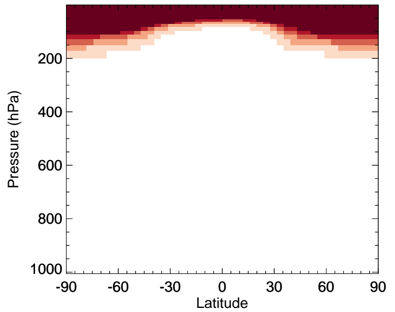
v11-02e-Run0 / v11-02d-Run1 SOAS - Zonal mean % diff for Jan
