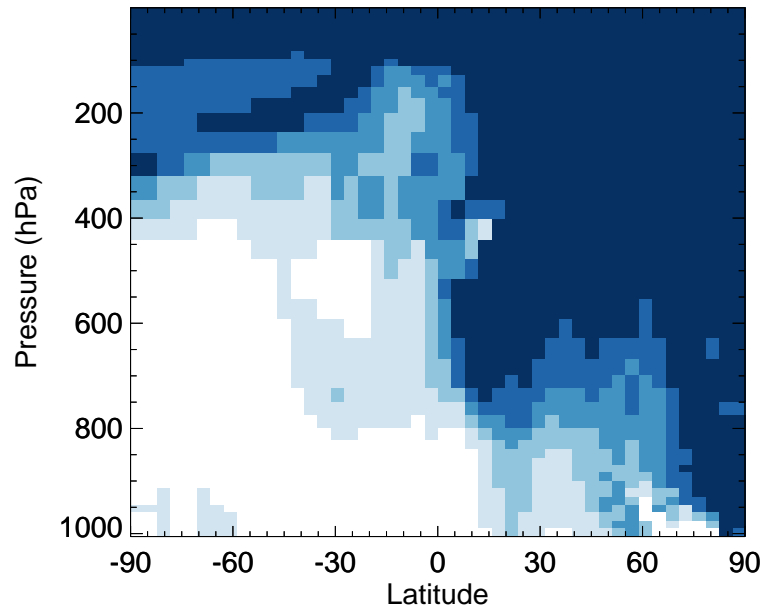
v11-02e-Run0 / v11-02c-Run0 NH3 - Zonal mean % diff for Jan
