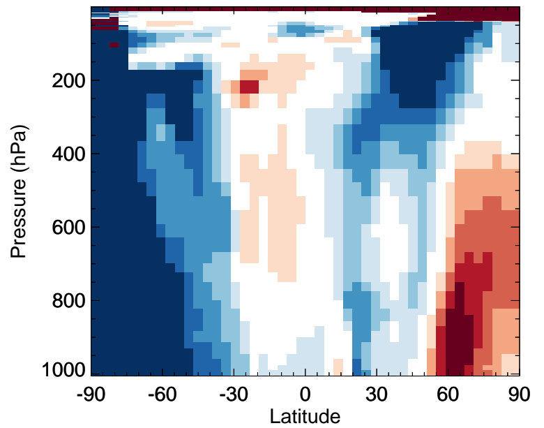
v11-02e-Run0 / v11-02c-Run0 RIPD - Zonal mean % diff for Jan
