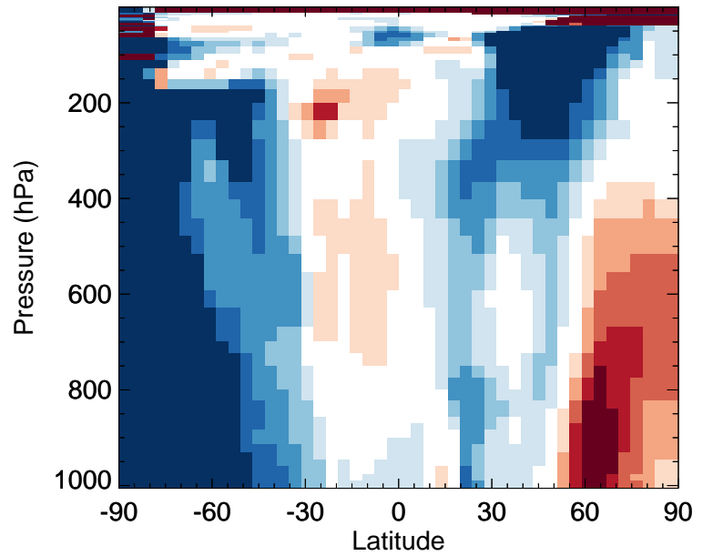
v11-02e-Run0 / v11-02c-Run0 RIPB - Zonal mean % diff for Jan
