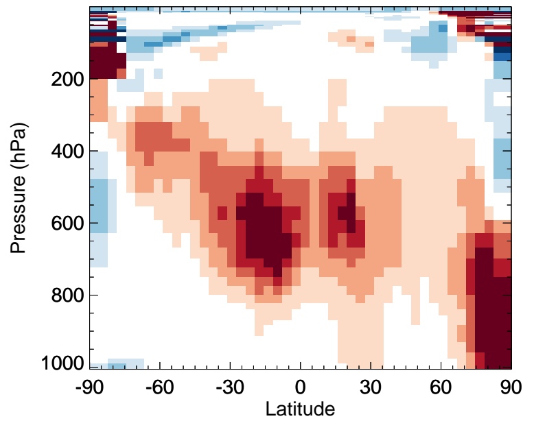
v11-02e-Run0 / v11-02d-Run1 MTPA - Zonal mean % diff for Jan
