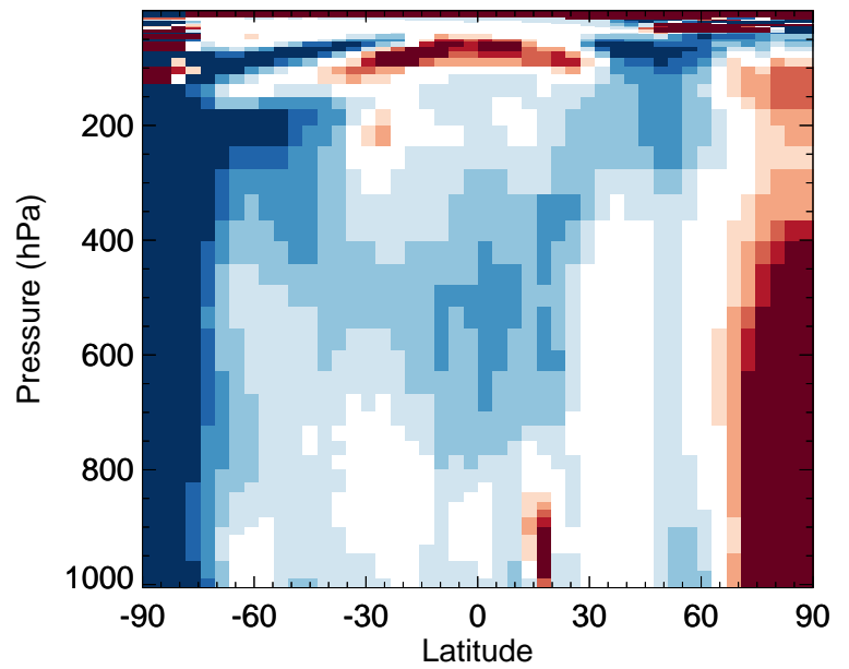
v11-02e-Run0 / v11-02c-Run0 ISN1 - Zonal mean % diff for Jan
