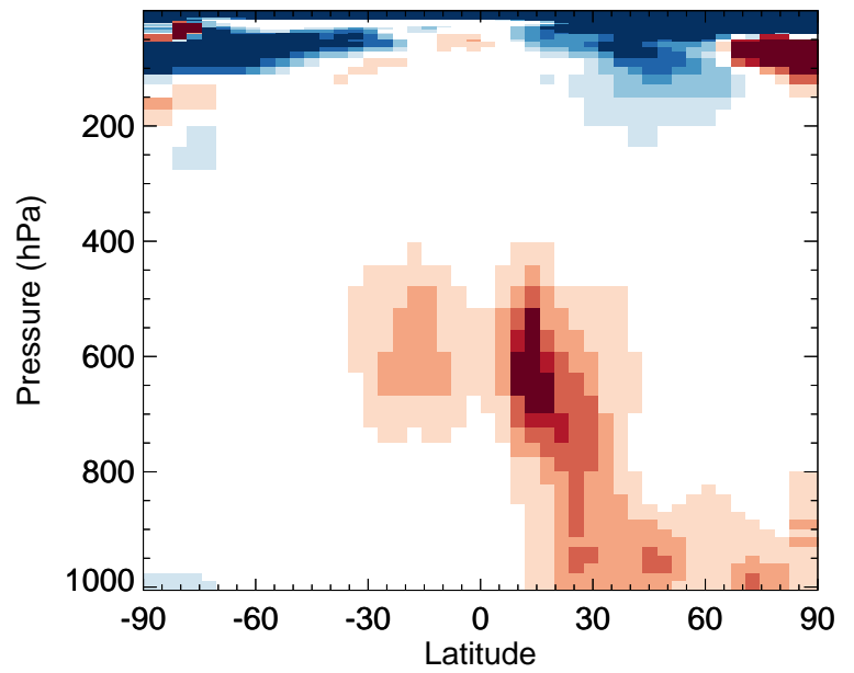
v11-02e-Run0 / v11-02d-Run1 DMS - Zonal mean % diff for Jan
