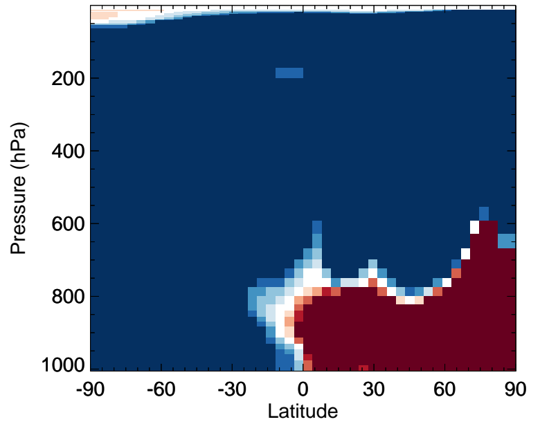
v11-02e-Run0 / v11-02c-Run0 HBr - Zonal mean % diff for Jan
