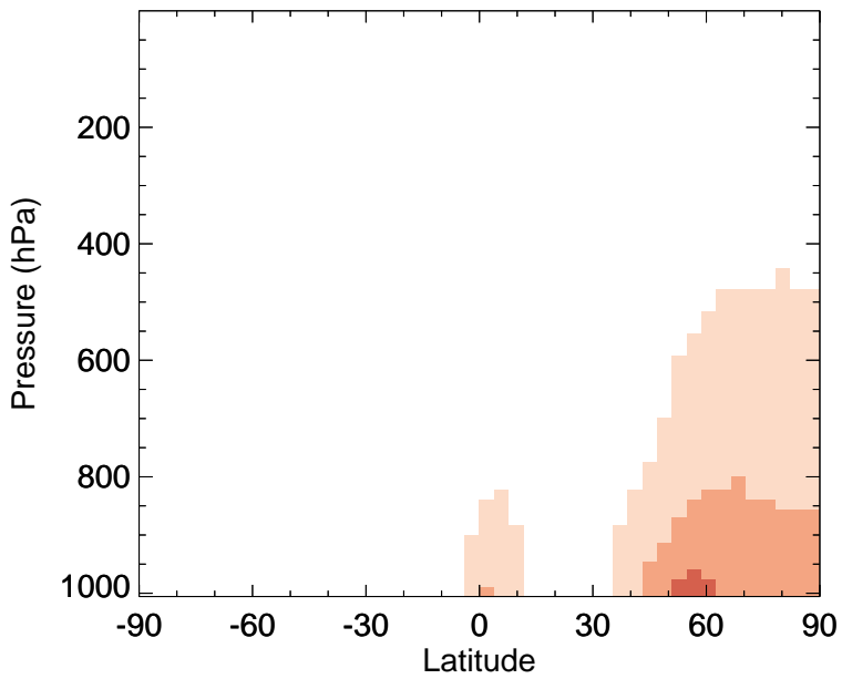
v11-02e-Run0 - v11-02c-Run0 MEK - Zonal mean abs diff for Jan
