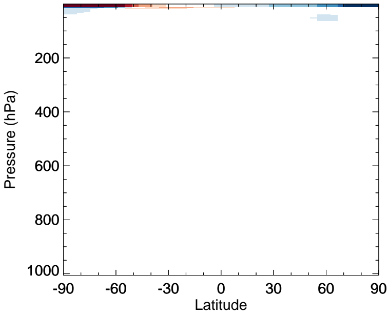
v11-02e-Run0 - v11-02d-Run1 ClO - Zonal mean abs diff for Jan
