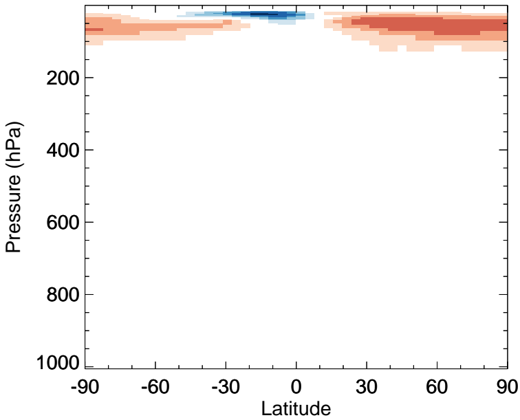
v11-02e-Run0 - v11-02c-Run0 CFC12 - Zonal mean abs diff for Jan
