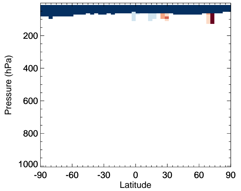
v11-02e-Run0 / v11-02d-Run1 SO4s - Zonal mean % diff for Jan
