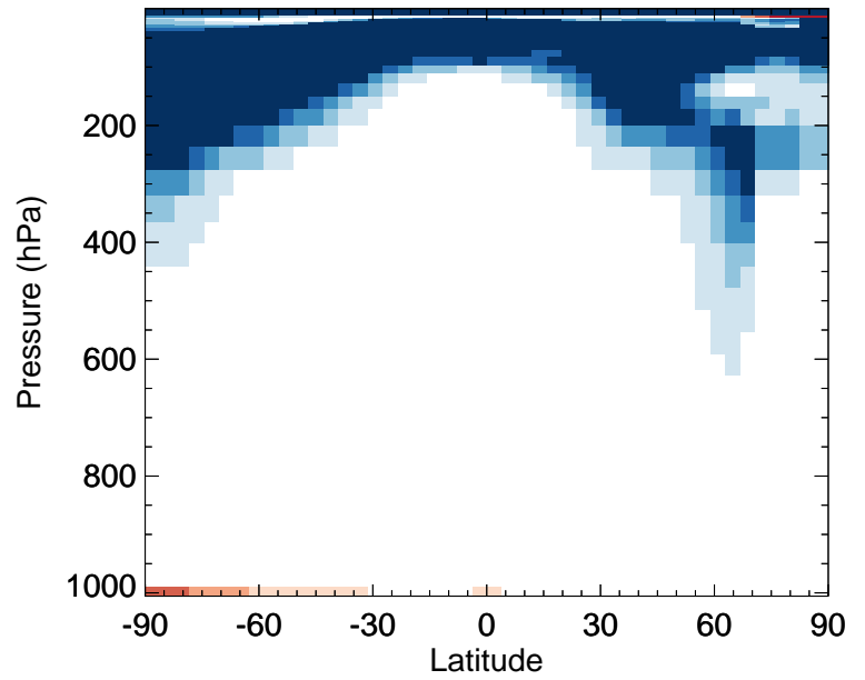
v11-02e-Run0 / v11-02d-Run1 ACTA - Zonal mean % diff for Jan
