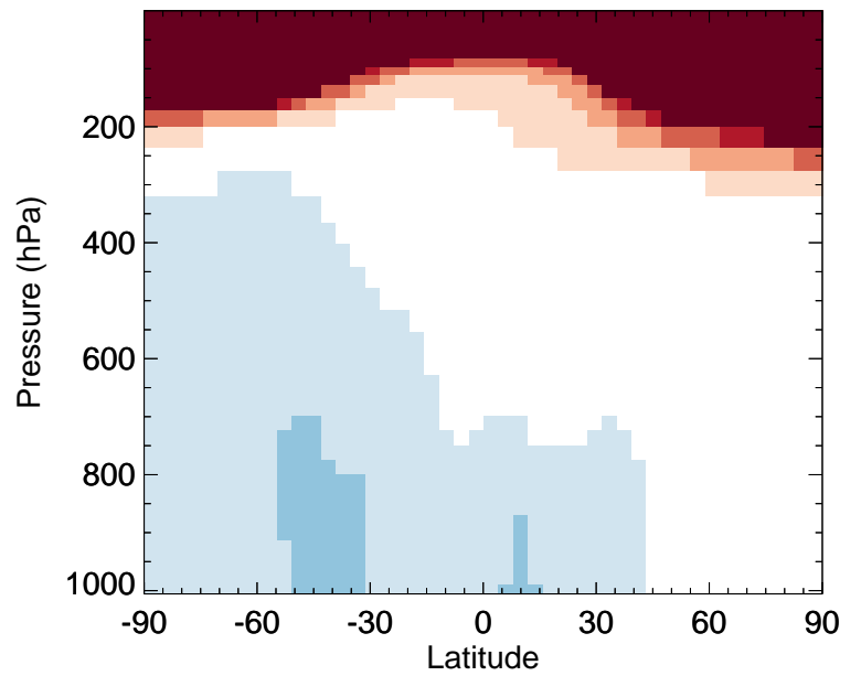
v11-02e-Run0 / v11-02c-Run0 TSOA0 - Zonal mean % diff for Jan
