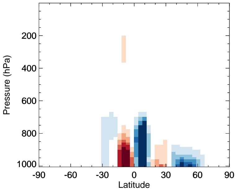
v11-02e-Run0 - v11-02c-Run0 PRPE - Zonal mean abs diff for Jan
