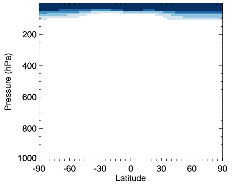
v11-02e-Run0 / v11-02d-Run1 SALA - Zonal mean % diff for Jan
