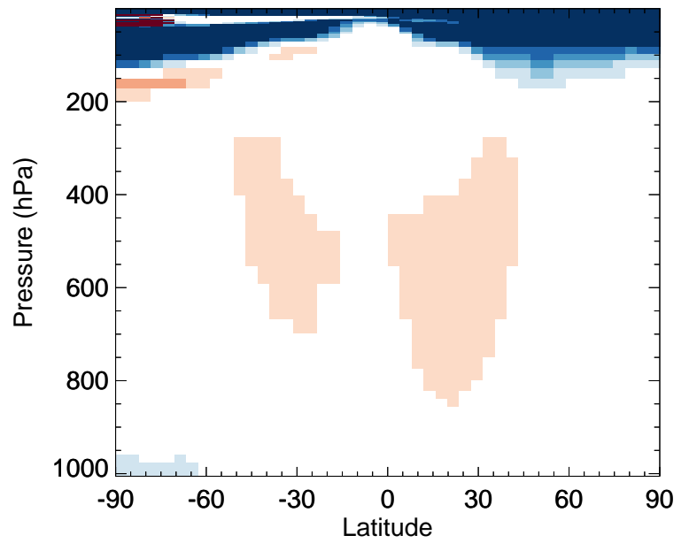
v11-02e-Run0 / v11-02d-Run1 TOLU - Zonal mean % diff for Jan
