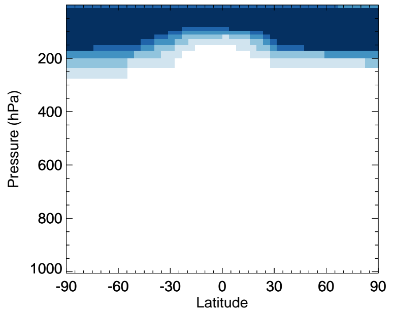
v11-02e-Run0 / v11-02c-Run0 OCPI - Zonal mean % diff for Jan
