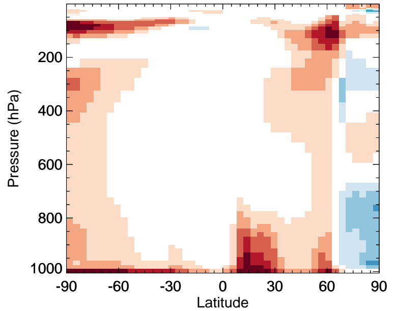
v11-02e-Run0 / v11-02c-Run0 OH - Zonal mean % diff for Jan
