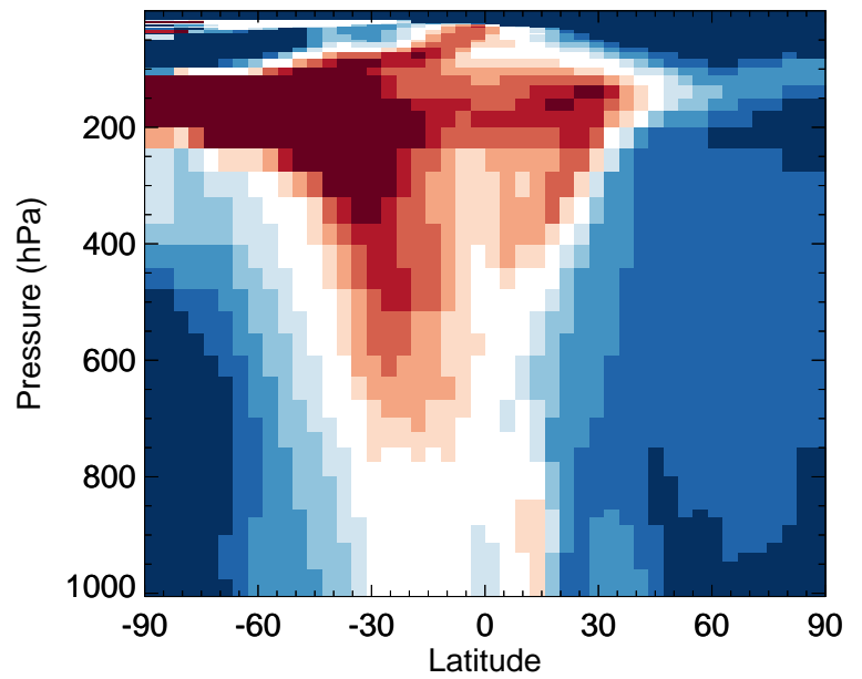
v11-02e-Run0 / v11-02c-Run0 HC187 - Zonal mean % diff for Jan
