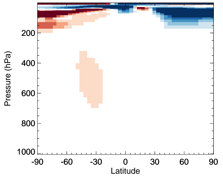
v11-02e-Run0 / v11-02d-Run1 EOH - Zonal mean % diff for Jan
