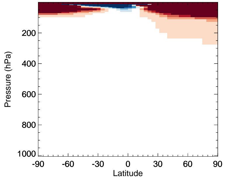
v11-02e-Run0 / v11-02d-Run1 CFC11 - Zonal mean % diff for Jan
