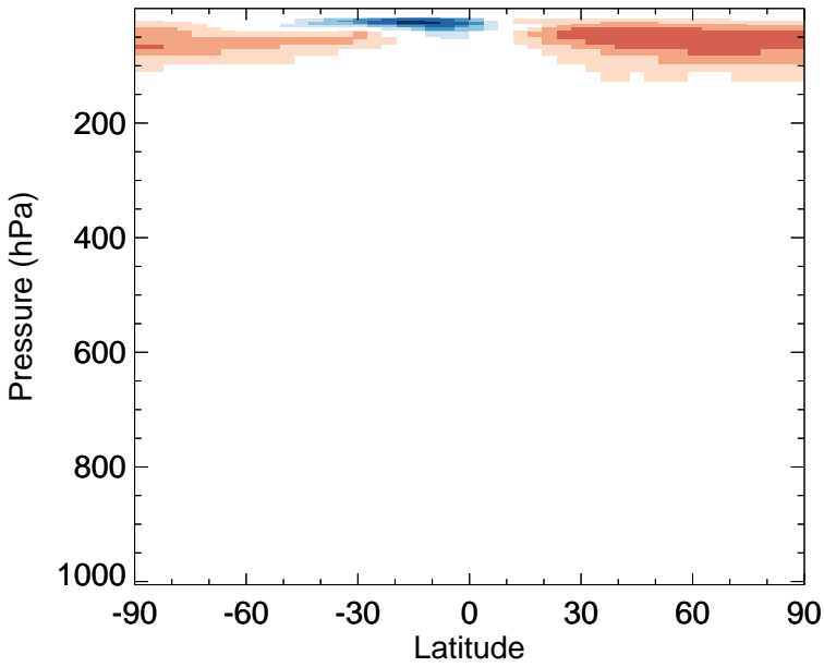
v11-02e-Run0 - v11-02d-Run1 CFC12 - Zonal mean abs diff for Jan
