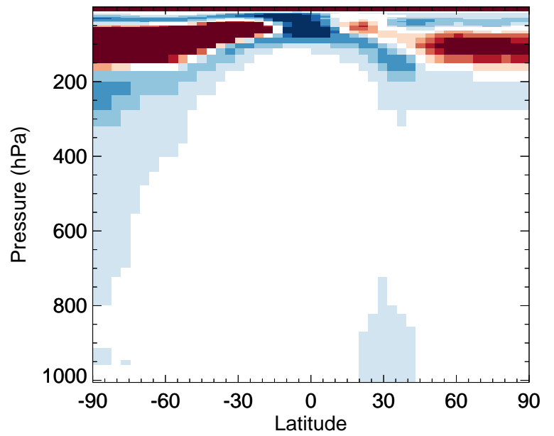
v11-02e-Run0 / v11-02d-Run1 H2O2 - Zonal mean % diff for Jan
