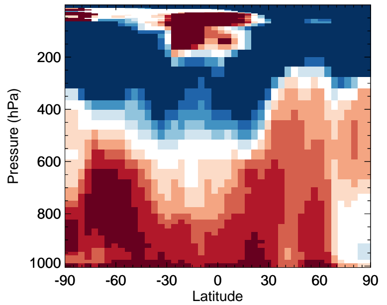
v11-02e-Run0 / v11-02d-Run1 LVOC - Zonal mean % diff for Jan
