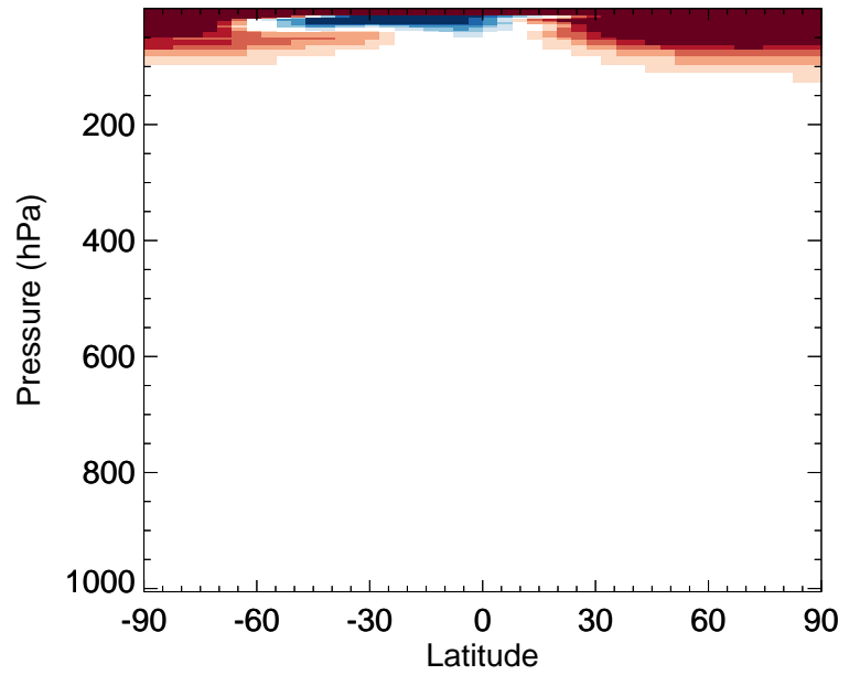
v11-02e-Run0 / v11-02d-Run1 CFC12 - Zonal mean % diff for Jan
