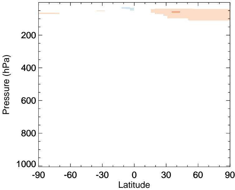
v11-02e-Run0 - v11-02c-Run0 CFC11 - Zonal mean abs diff for Jan
