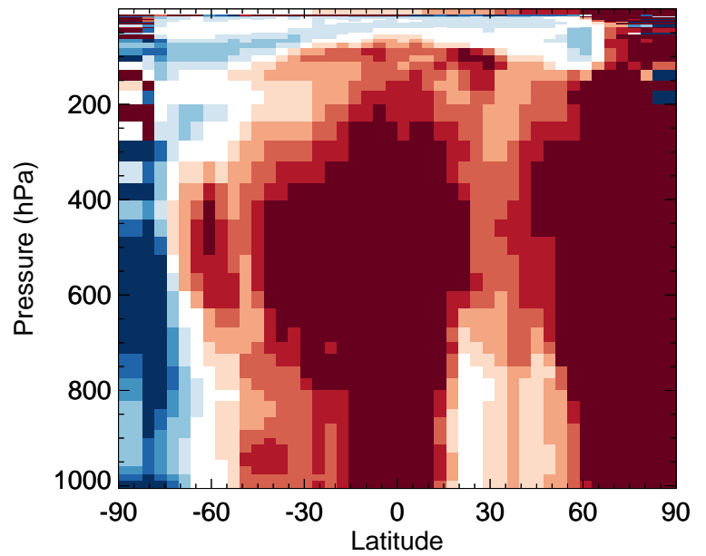
v11-02e-Run0 / v11-02c-Run0 LIMO - Zonal mean % diff for Jan
