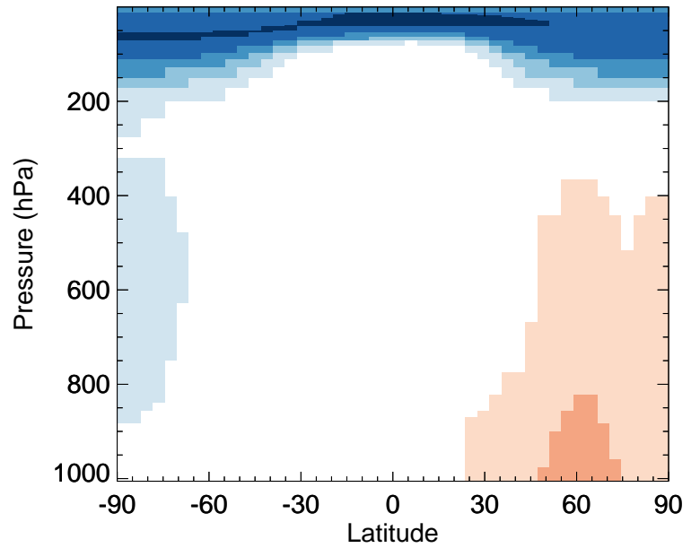
v11-02e-Run0 / v11-02c-Run0 MSA - Zonal mean % diff for Jan
