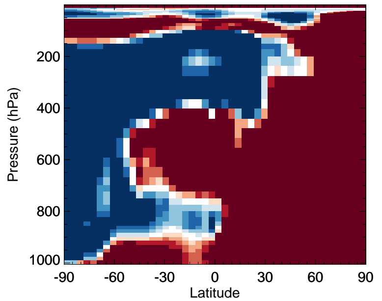
v11-02e-Run0 / v11-02c-Run0 HOCl - Zonal mean % diff for Jan
