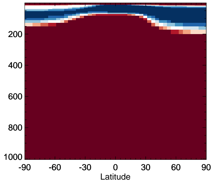
v11-02e-Run0 / v11-02d-Run1 SOAIE - Zonal mean % diff for Jan
