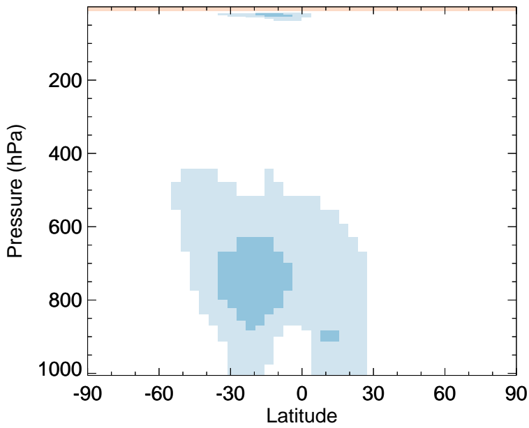
v11-02e-Run0 - v11-02d-Run1 H2O2 - Zonal mean abs diff for Jan
