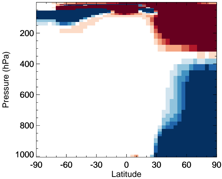
v11-02e-Run0 - v11-02c-Run0 N2O5 - Zonal mean abs diff for Jan
