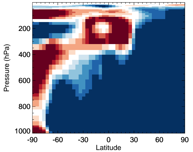
v11-02e-Run0 / v11-02d-Run1 HOBr - Zonal mean % diff for Jan
