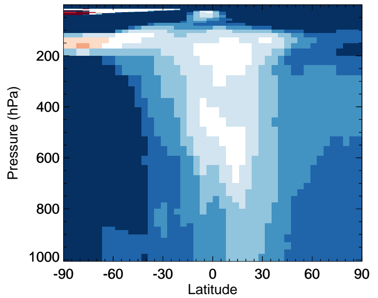
v11-02e-Run0 / v11-02d-Run1 HC187 - Zonal mean % diff for Jan
