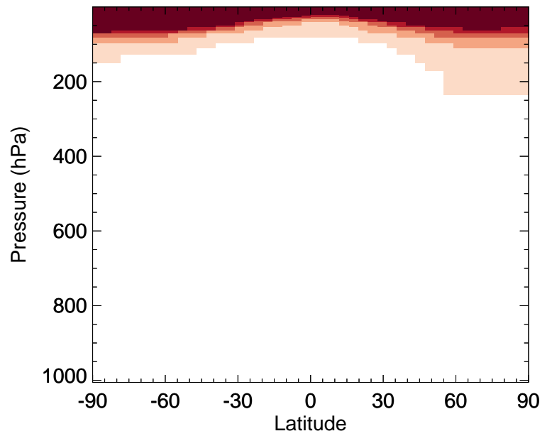
v11-02e-Run0 / v11-02d-Run1 ASOG3 - Zonal mean % diff for Jan
