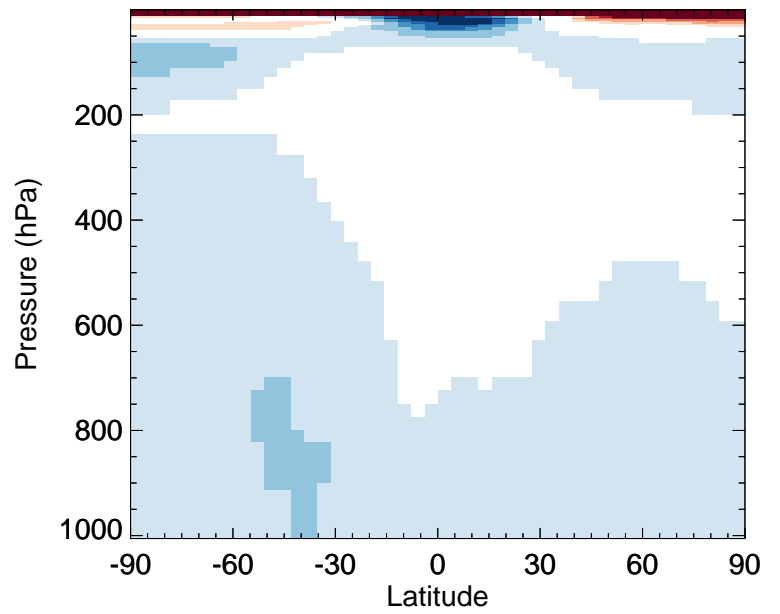
v11-02e-Run0 / v11-02d-Run1 TSOA0 - Zonal mean % diff for Jan
