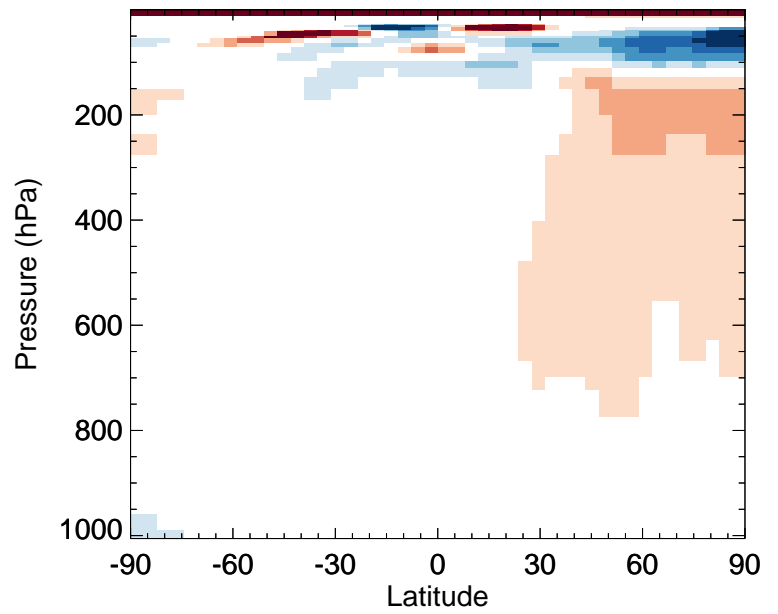
v11-02e-Run0 / v11-02d-Run1 ALD2 - Zonal mean % diff for Jan
