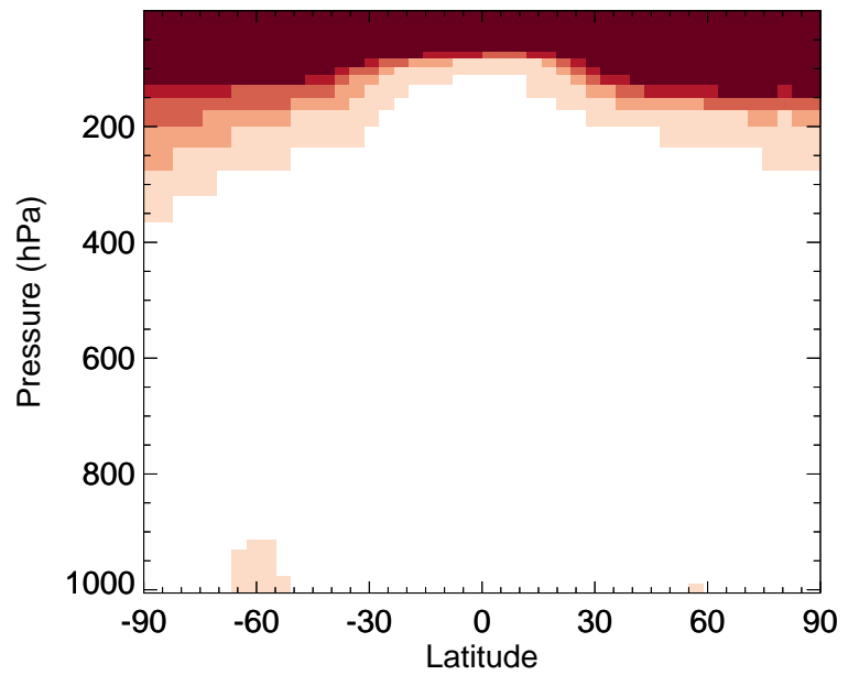
v11-02e-Run0 / v11-02c-Run0 ASOA2 - Zonal mean % diff for Jan
