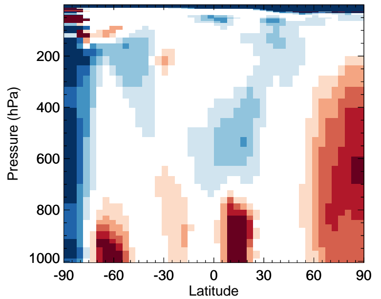
v11-02e-Run0 / v11-02c-Run0 ETHLN - Zonal mean % diff for Jan
