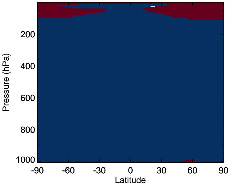
v11-02e-Run0 - v11-02d-Run1 CH4 - Zonal mean abs diff for Jan
