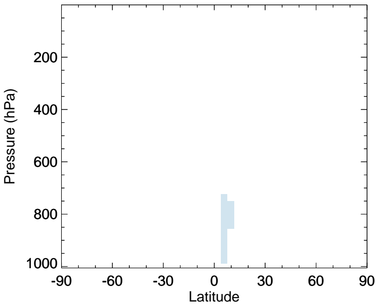
v11-02e-Run0 - v11-02c-Run0 INDIOL - Zonal mean abs diff for Jan
