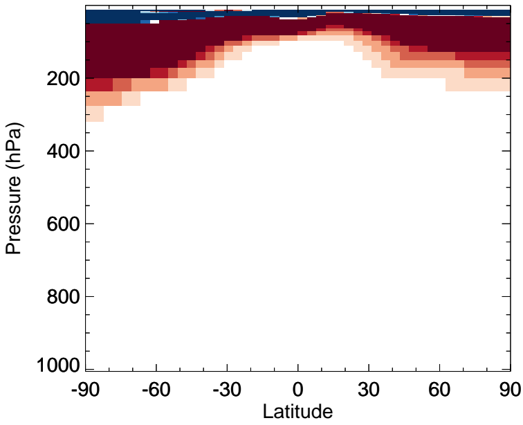
v11-02e-Run0 - v11-02d-Run1 O3 - Zonal mean abs diff for Jan
