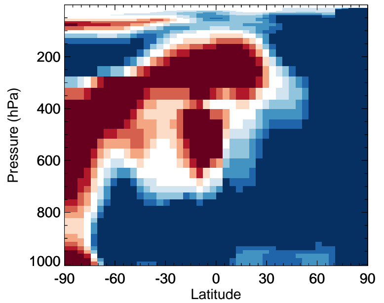
v11-02e-Run0 / v11-02d-Run1 BrO - Zonal mean % diff for Jan
