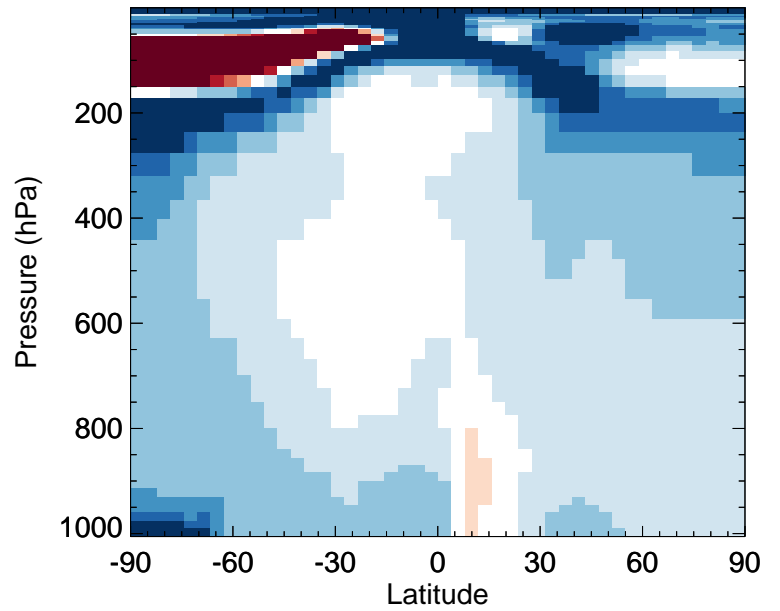
v11-02e-Run0 / v11-02c-Run0 MP - Zonal mean % diff for Jan
