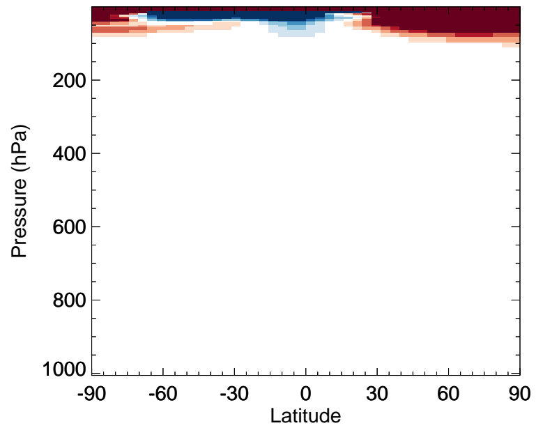
v11-02e-Run0 / v11-02d-Run1 OCS - Zonal mean % diff for Jan
