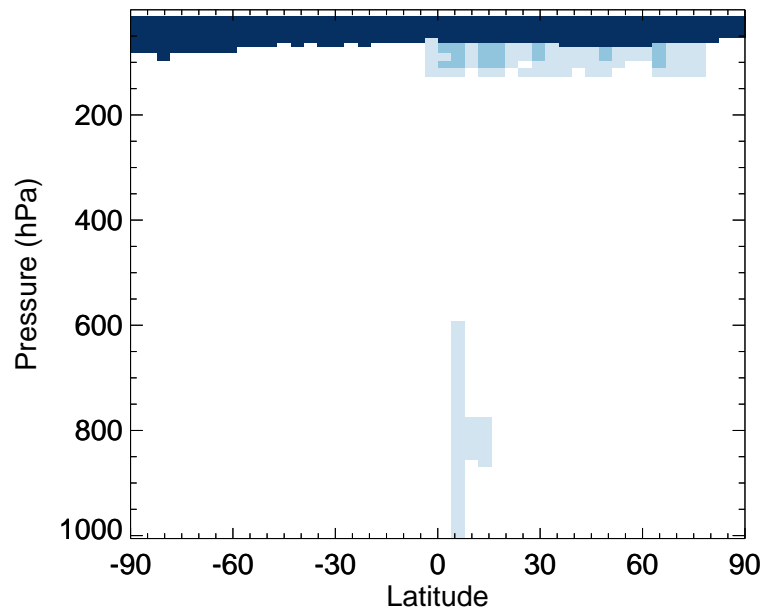
v11-02e-Run0 / v11-02c-Run0 SO4s - Zonal mean % diff for Jan
