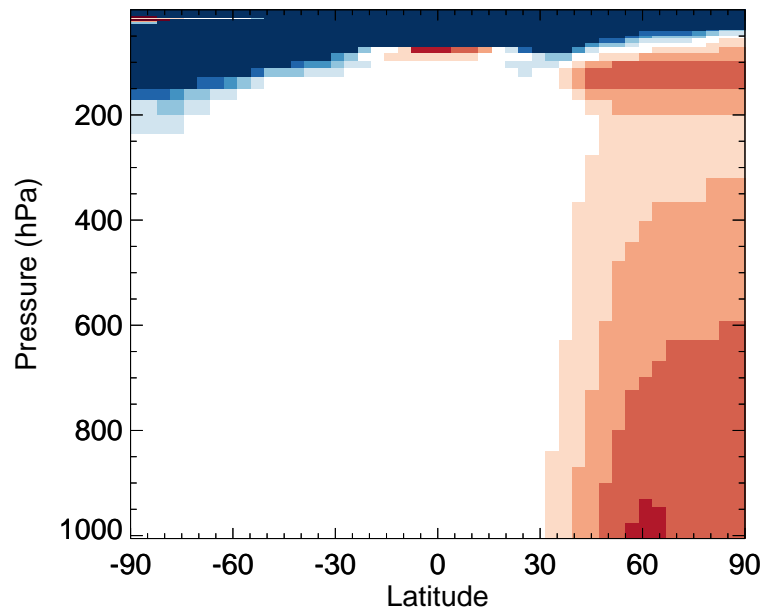
v11-02e-Run0 / v11-02c-Run0 MEK - Zonal mean % diff for Jan
