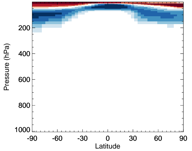
v11-02e-Run0 / v11-02d-Run1 ASOA3 - Zonal mean % diff for Jan
