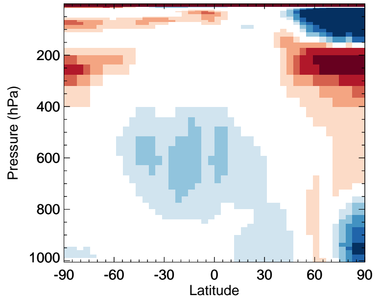
v11-02e-Run0 / v11-02d-Run1 HNO 4 - Zonal mean % diff for Jan
