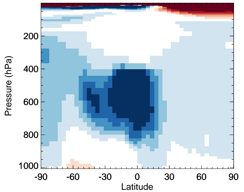
v11-02e-Run0 / v11-02c-Run0 SO 2 - Zonal mean % diff for Jan
