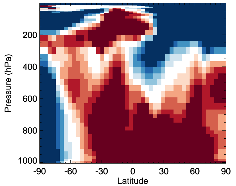
v11-02e-Run0 / v11-02c-Run0 LVOC - Zonal mean % diff for Jan
