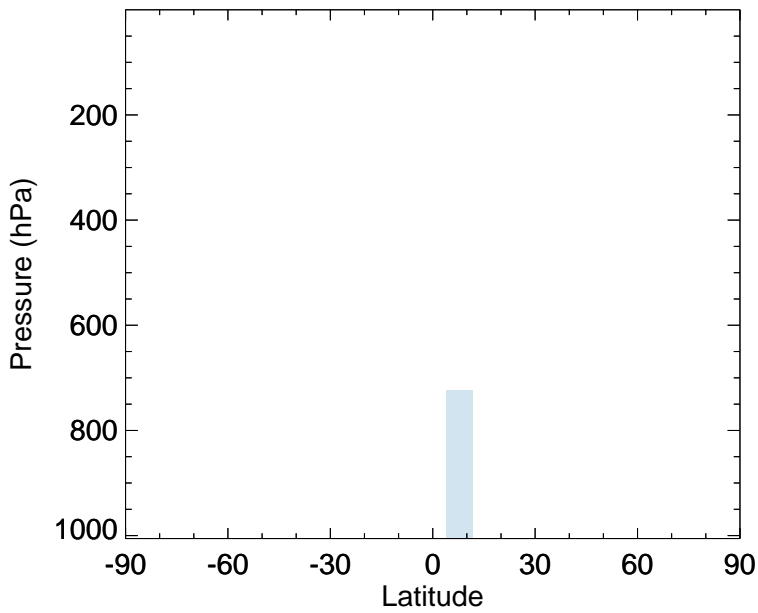
v11-02e-Run0 - v11-02c-Run0 MVK - Zonal mean abs diff for Jan
