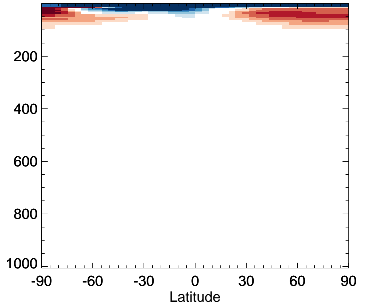
v11-02e-Run0 / v11-02d-Run1 N2O - Zonal mean % diff for Jan
