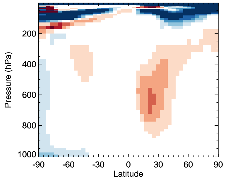
v11-02e-Run0 / v11-02d-Run1 XYLE - Zonal mean % diff for Jan
