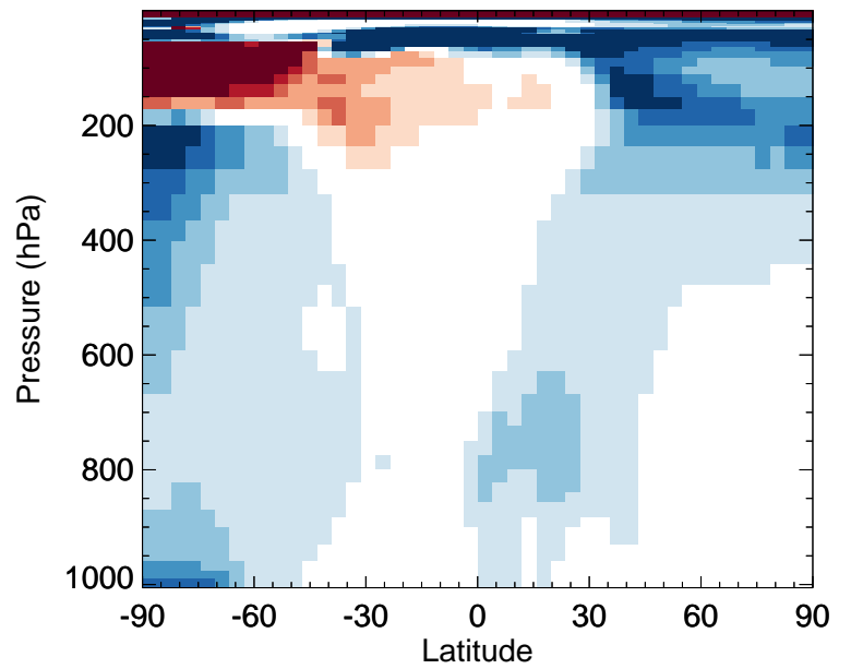
v11-02e-Run0 / v11-02c-Run0 HAC - Zonal mean % diff for Jan
