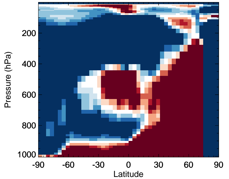
v11-02e-Run0 / v11-02c-Run0 ClOO - Zonal mean % diff for Jan
