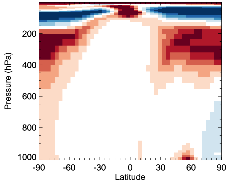
v11-02e-Run0 / v11-02c-Run0 HNO 3 - Zonal mean % diff for Jan
