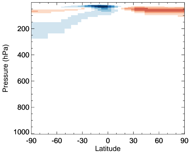
v11-02e-Run0 - v11-02d-Run1 OCS - Zonal mean abs diff for Jan
