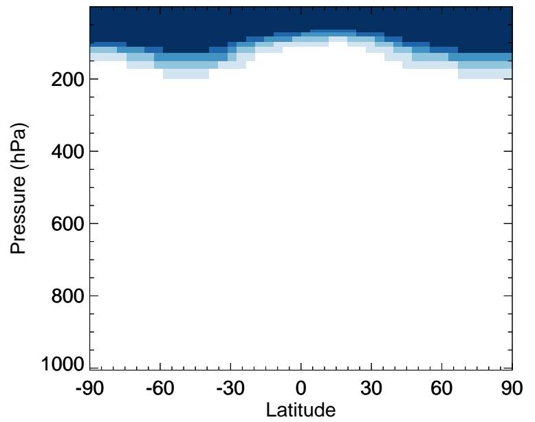
v11-02e-Run0 / v11-02d-Run1 OCPI - Zonal mean % diff for Oct
