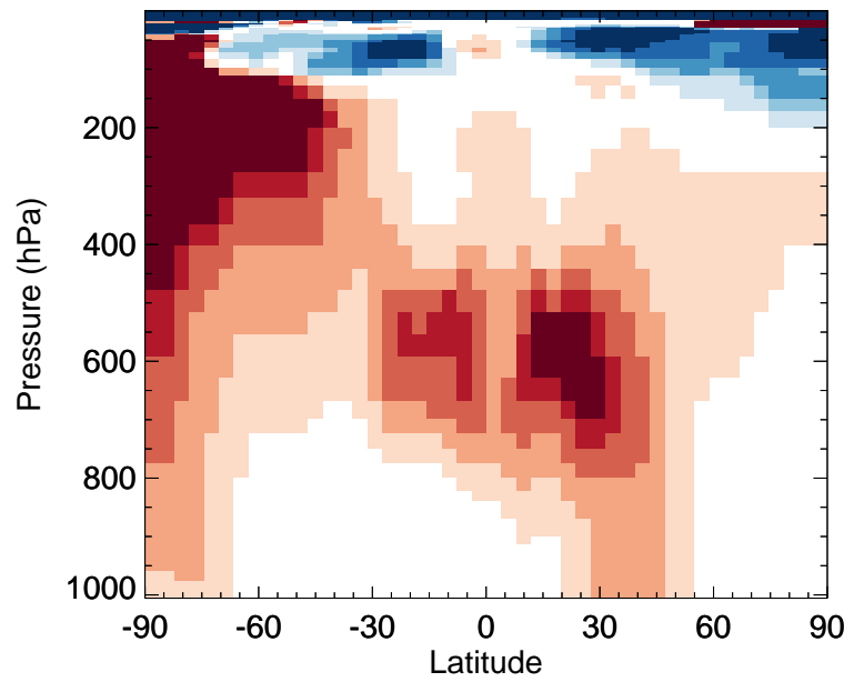
v11-02e-Run0 / v11-02d-Run1 DMS - Zonal mean % diff for Oct
