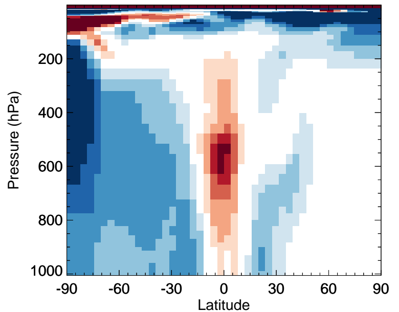
v11-02e-Run0 / v11-02c-Run0 GLYC - Zonal mean % diff for Oct
