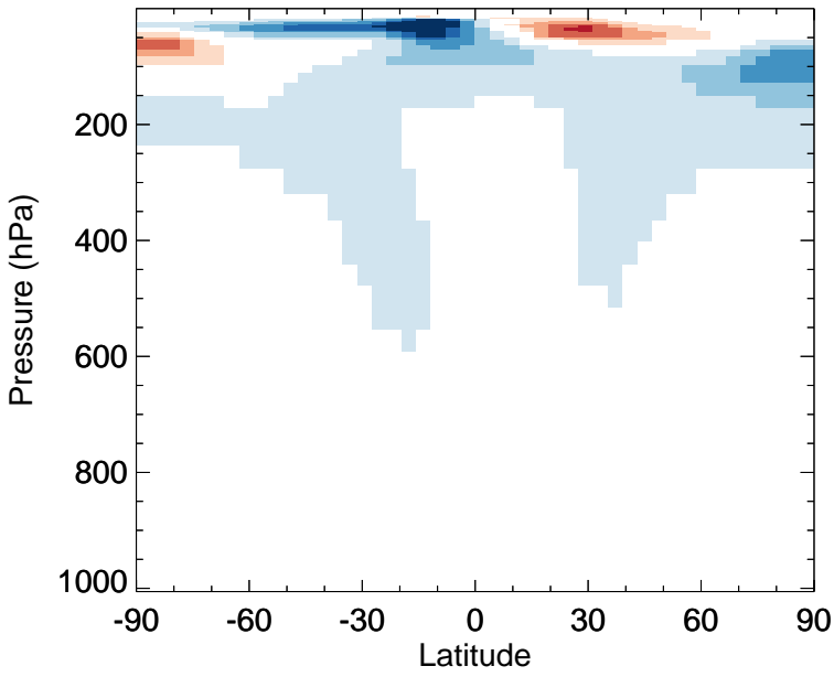
v11-02e-Run0 - v11-02d-Run1 CH3Cl - Zonal mean abs diff for Oct
