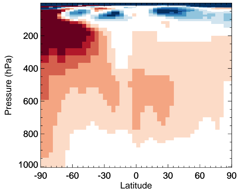
v11-02e-Run0 / v11-02d-Run1 TOLU - Zonal mean % diff for Oct
