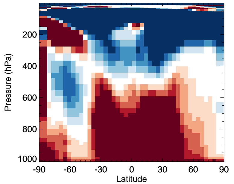
v11-02e-Run0 / v11-02c-Run0 LVOC - Zonal mean % diff for Oct
