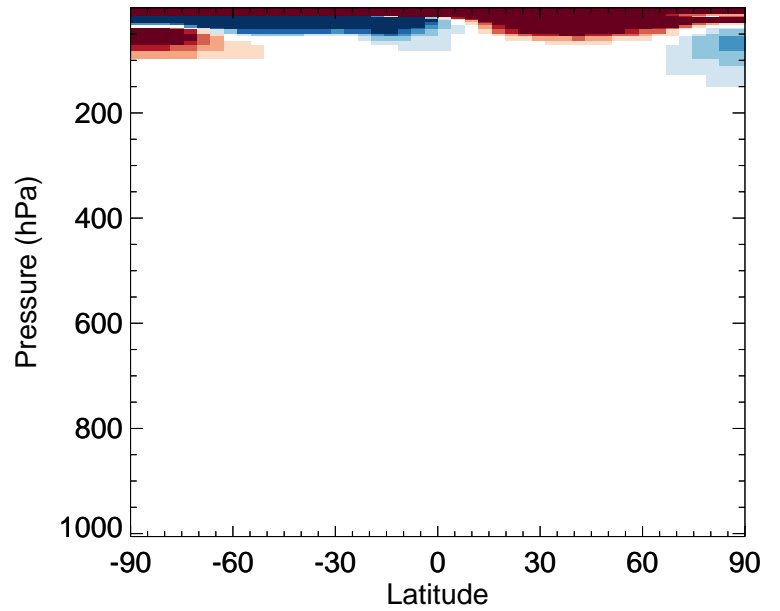
v11-02e-Run0 / v11-02c-Run0 OCS - Zonal mean % diff for Oct
