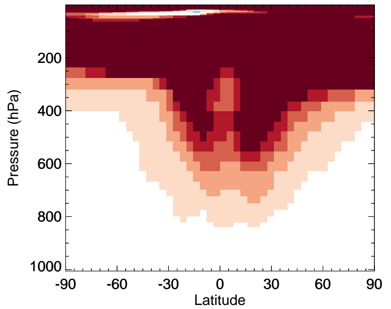
v11-02e-Run0 / v11-02d-Run1 SO4 - Zonal mean % diff for Oct
