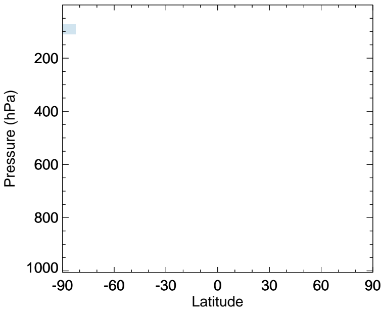
v11-02e-Run0 - v11-02c-Run0 Cl2O2 - Zonal mean abs diff for Oct
