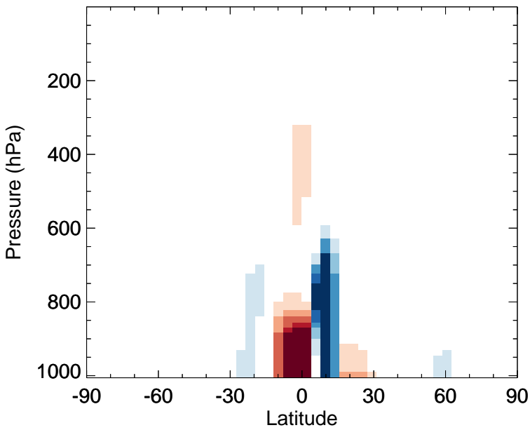
v11-02e-Run0 - v11-02c-Run0 PRPE - Zonal mean abs diff for Oct
