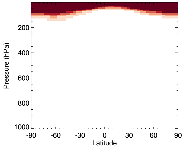
v11-02e-Run0 / v11-02c-Run0 SOAS - Zonal mean % diff for Oct
