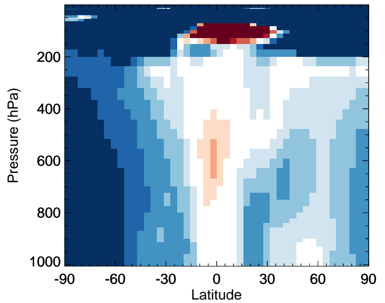
v11-02e-Run0 / v11-02c-Run0 IMAE - Zonal mean % diff for Oct
