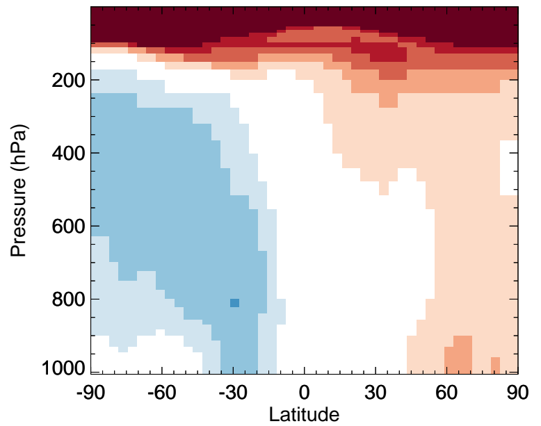
v11-02e-Run0 / v11-02c-Run0 INDIOL - Zonal mean % diff for Oct
