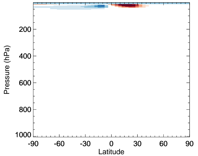
v11-02e-Run0 / v11-02c-Run0 CH 2 Br 2 - Zonal mean % diff for Oct
