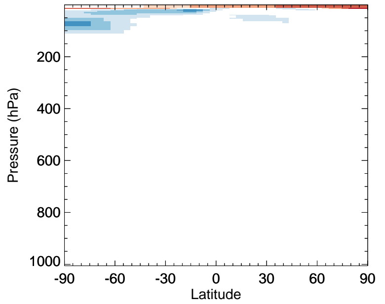
v11-02e-Run0 / v11-02d-Run1 CO - Zonal mean % diff for Oct
