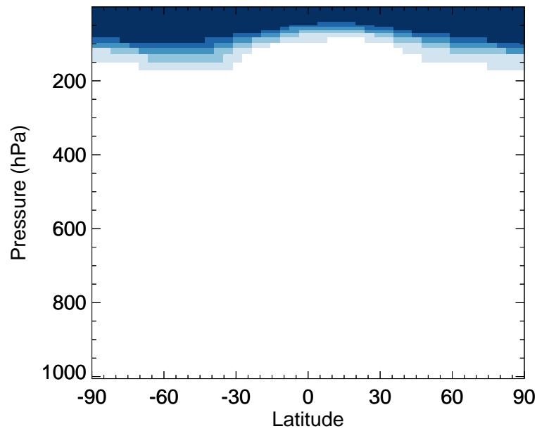
v11-02e-Run0 / v11-02c-Run0 BCPI - Zonal mean % diff for Oct
