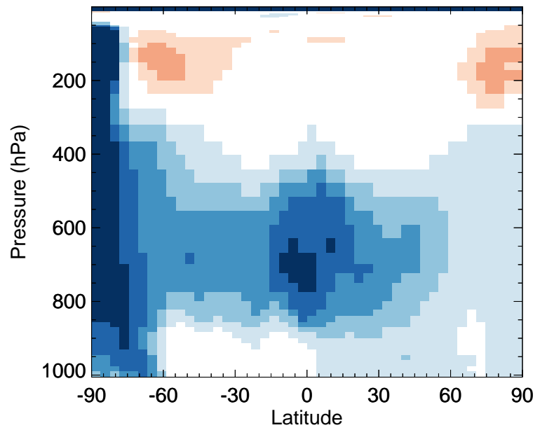
v11-02e-Run0 / v11-02d-Run1 NO3 - Zonal mean % diff for Oct
