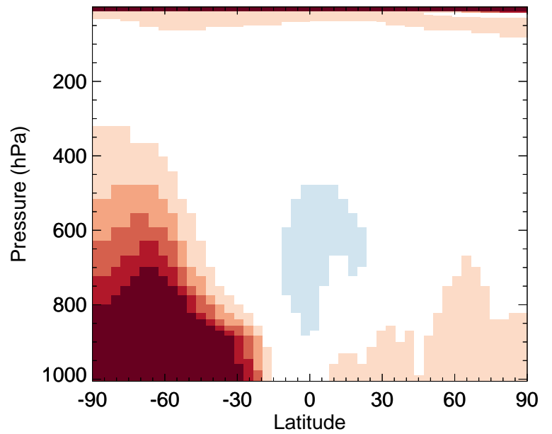
v11-02e-Run0 / v11-02c-Run0 PPN - Zonal mean % diff for Oct
