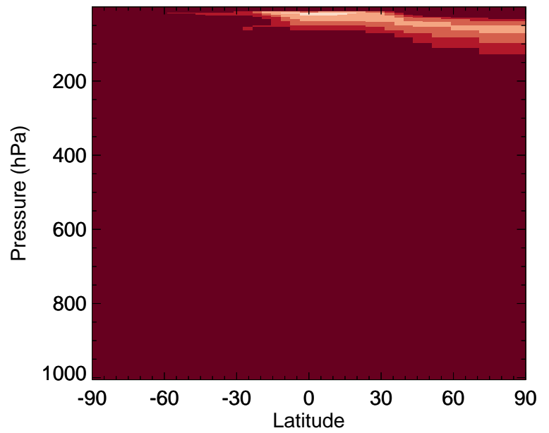
v11-02e-Run0 / v11-02d-Run1 SOAGX - Zonal mean % diff for Oct
