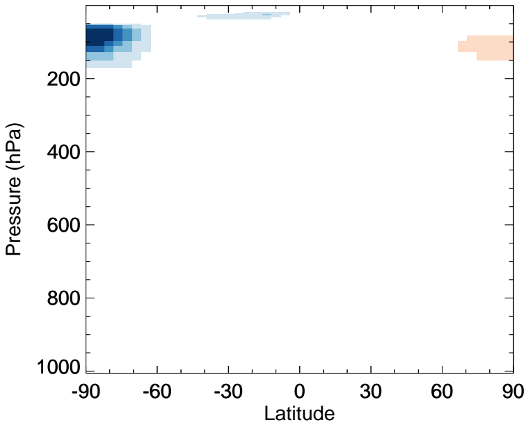
v11-02e-Run0 - v11-02c-Run0 MPN - Zonal mean abs diff for Oct
