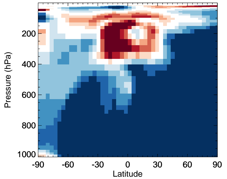
v11-02e-Run0 / v11-02d-Run1 HOBr - Zonal mean % diff for Oct
