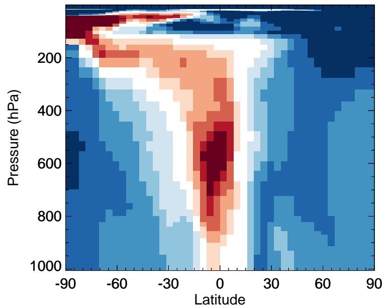
v11-02e-Run0 / v11-02c-Run0 HC187 - Zonal mean % diff for Oct
