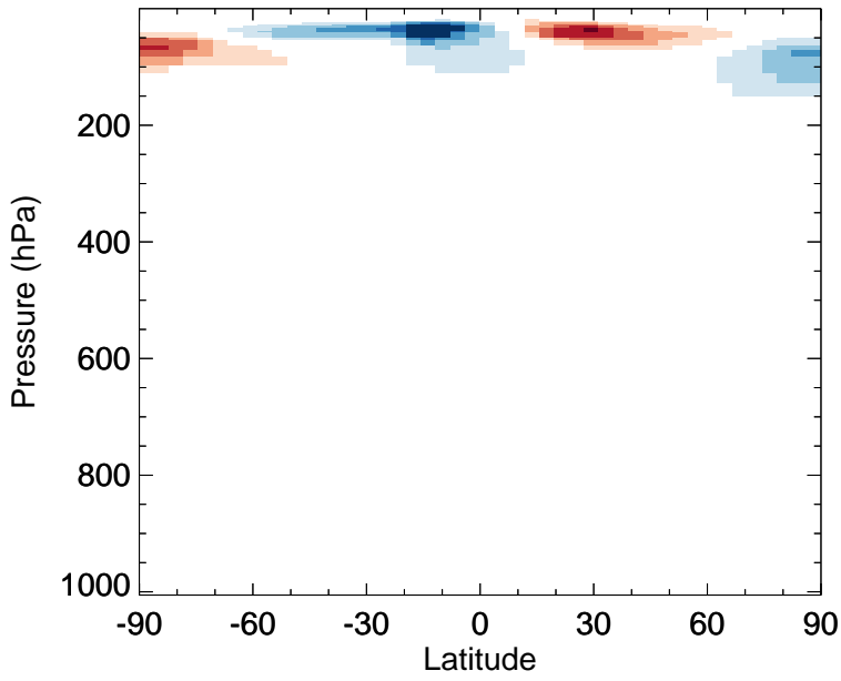
v11-02e-Run0 - v11-02d-Run1 OCS - Zonal mean abs diff for Oct
