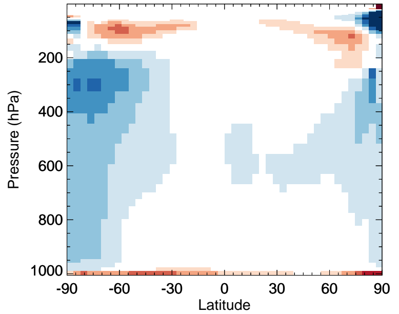
v11-02e-Run0 / v11-02d-Run1 OH - Zonal mean % diff for Oct
