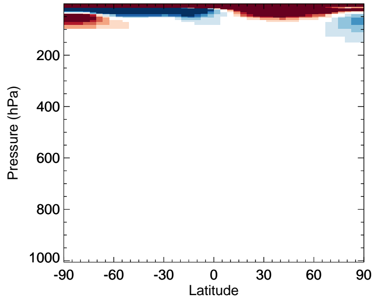
v11-02e-Run0 / v11-02d-Run1 OCS - Zonal mean % diff for Oct
