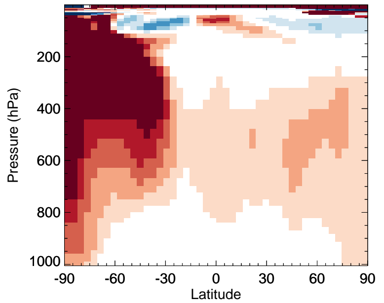
v11-02e-Run0 / v11-02d-Run1 PRPE - Zonal mean % diff for Oct
