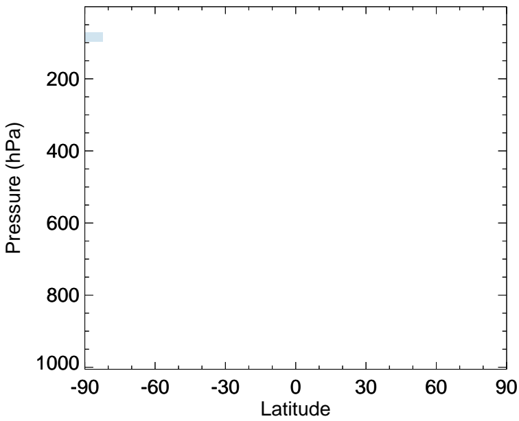
v11-02e-Run0 - v11-02d-Run1 Cl2O2 - Zonal mean abs diff for Oct
