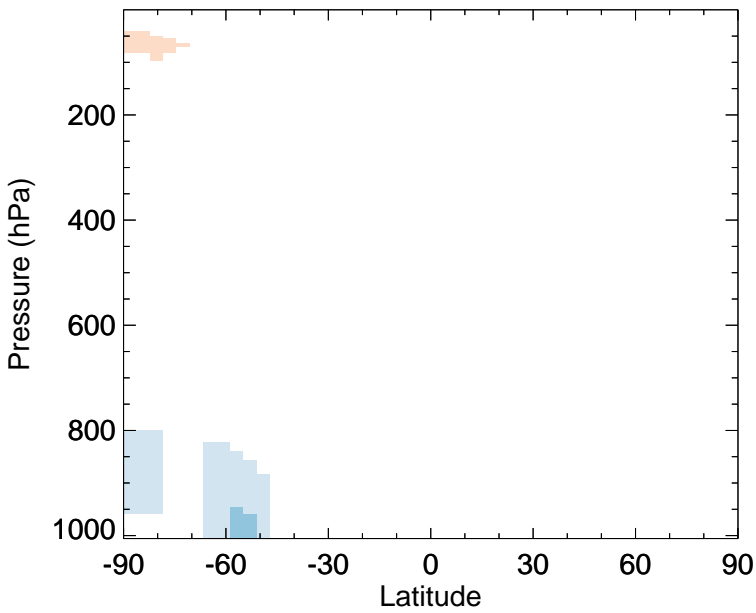
v11-02e-Run0 - v11-02c-Run0 BrO - Zonal mean abs diff for Oct
