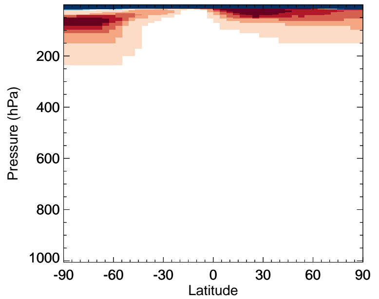
v11-02e-Run0 / v11-02d-Run1 ACET - Zonal mean % diff for Oct
