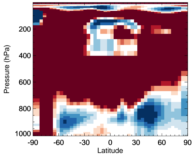
v11-02e-Run0 / v11-02d-Run1 HOCl - Zonal mean % diff for Oct
