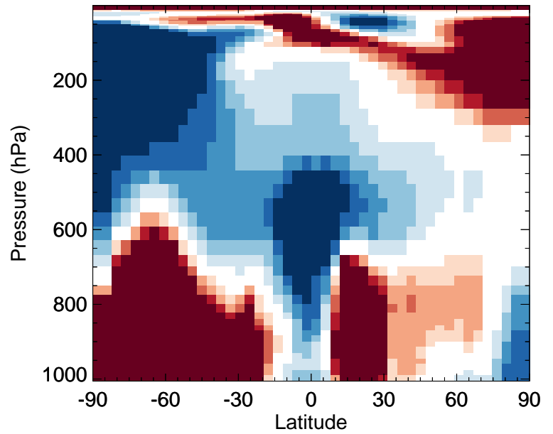
v11-02e-Run0 / v11-02c-Run0 N2O5 - Zonal mean % diff for Oct
