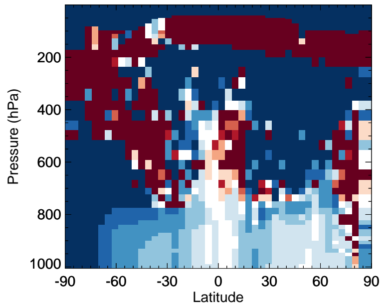
v11-02e-Run0 / v11-02c-Run0 NIT - Zonal mean % diff for Oct
