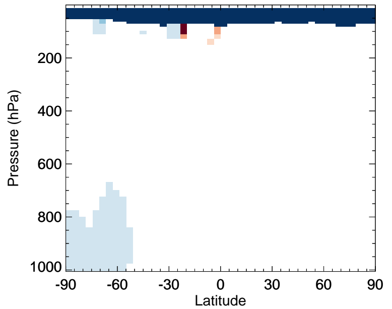
v11-02e-Run0 / v11-02c-Run0 SO4s - Zonal mean % diff for Oct
