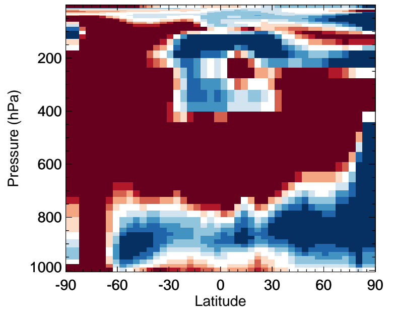
v11-02e-Run0 / v11-02d-Run1 ClO - Zonal mean % diff for Oct
