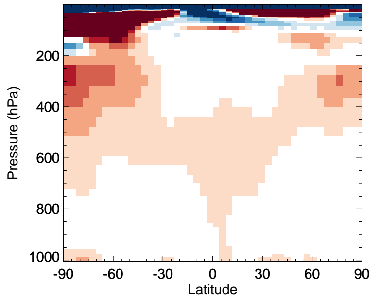
v11-02e-Run0 / v11-02d-Run1 RCHO - Zonal mean % diff for Oct
