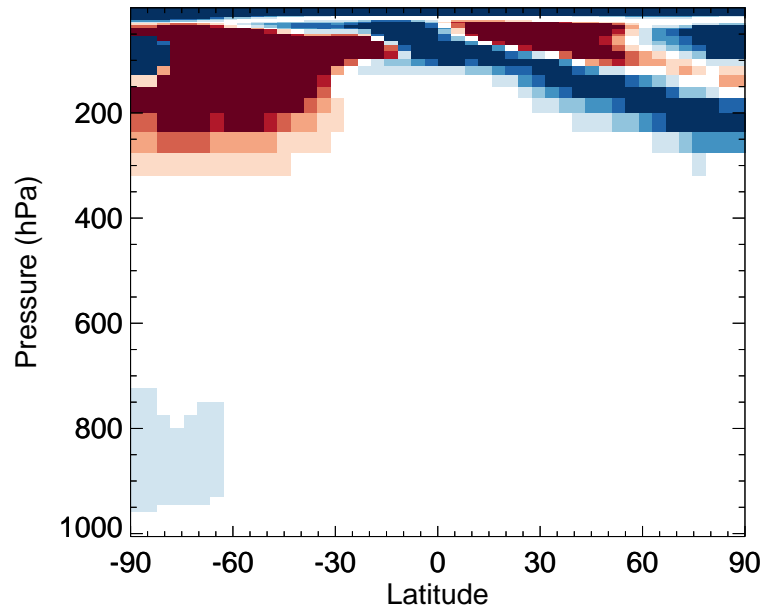
v11-02e-Run0 / v11-02d-Run1 MGLY - Zonal mean % diff for Oct
