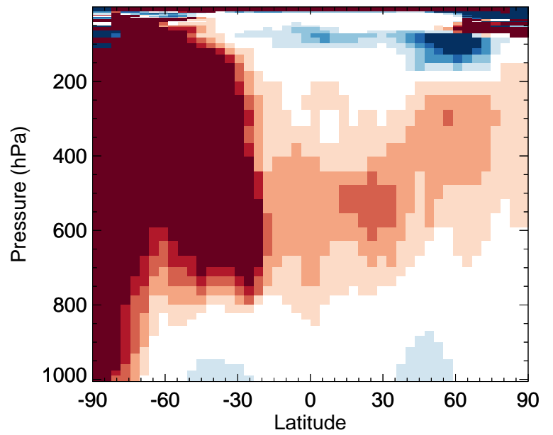
v11-02e-Run0 / v11-02d-Run1 RIPB - Zonal mean % diff for Oct
