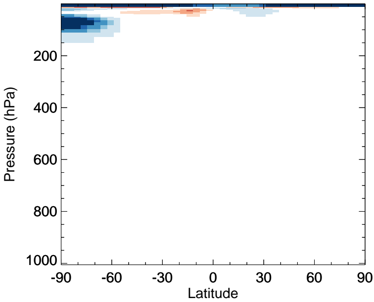
v11-02e-Run0 - v11-02d-Run1 NO - Zonal mean abs diff for Oct
