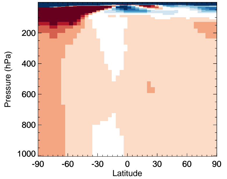
v11-02e-Run0 / v11-02d-Run1 MEK - Zonal mean % diff for Oct
