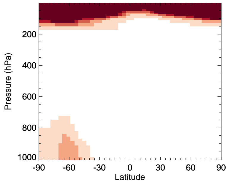
v11-02e-Run0 / v11-02c-Run0 ASOA3 - Zonal mean % diff for Oct
