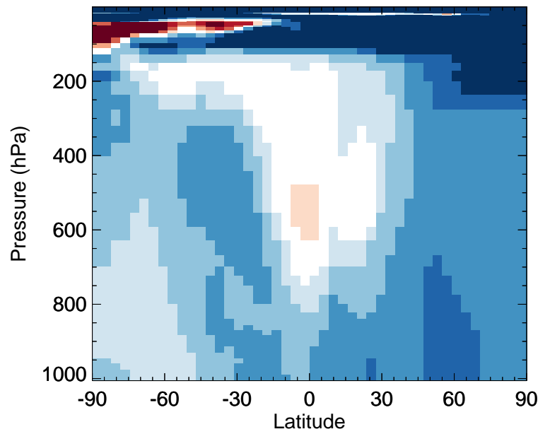
v11-02e-Run0 / v11-02d-Run1 HC187 - Zonal mean % diff for Oct
