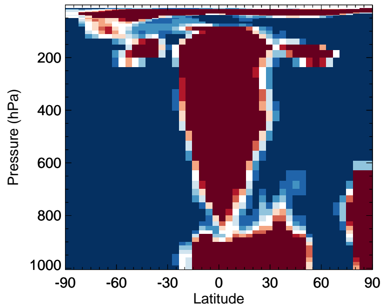
v11-02e-Run0 / v11-02c-Run0 Br2 - Zonal mean % diff for Oct
