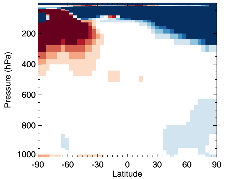
v11-02e-Run0 / v11-02d-Run1 ACTA - Zonal mean % diff for Oct
