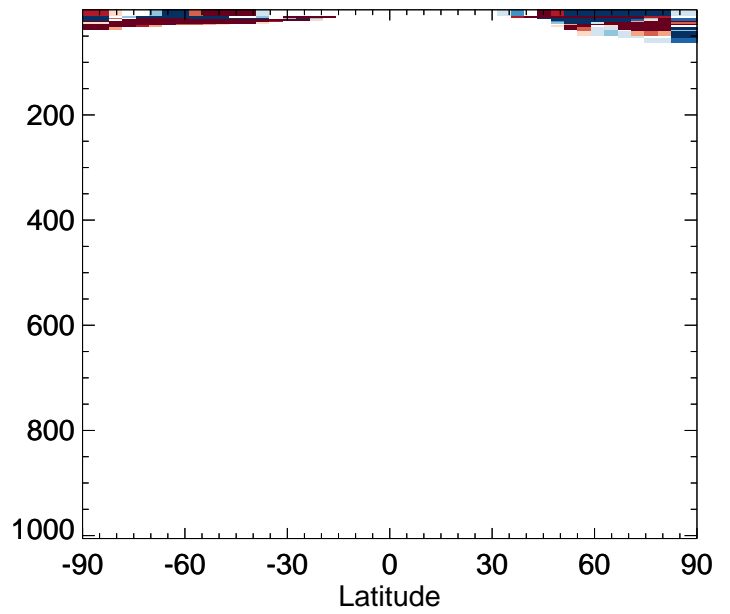
v11-02e-Run0 / v11-02d-Run1 BCPO - Zonal mean % diff for Oct
