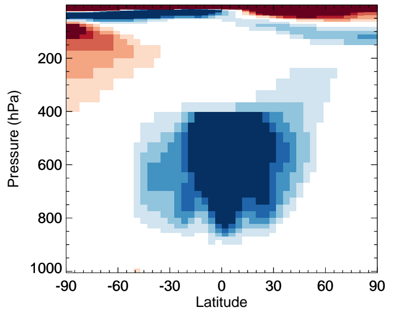
v11-02e-Run0 / v11-02d-Run1 SO 2 - Zonal mean % diff for Oct
