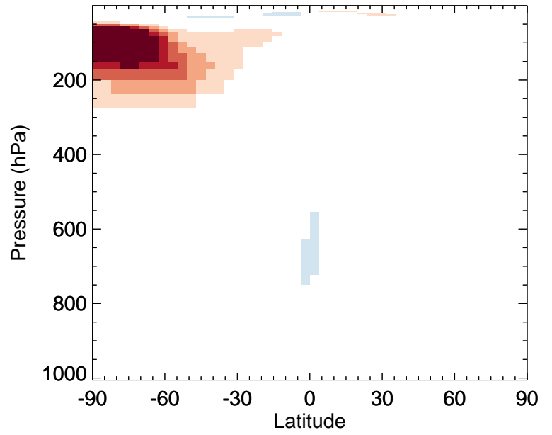
v11-02e-Run0 / v11-02d-Run1 O3 - Zonal mean % diff for Oct
