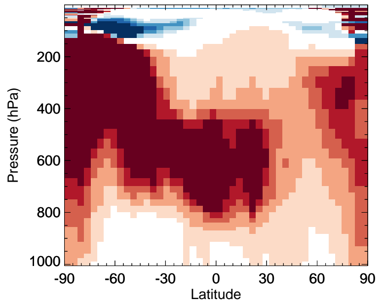
v11-02e-Run0 / v11-02d-Run1 MTPA - Zonal mean % diff for Oct
