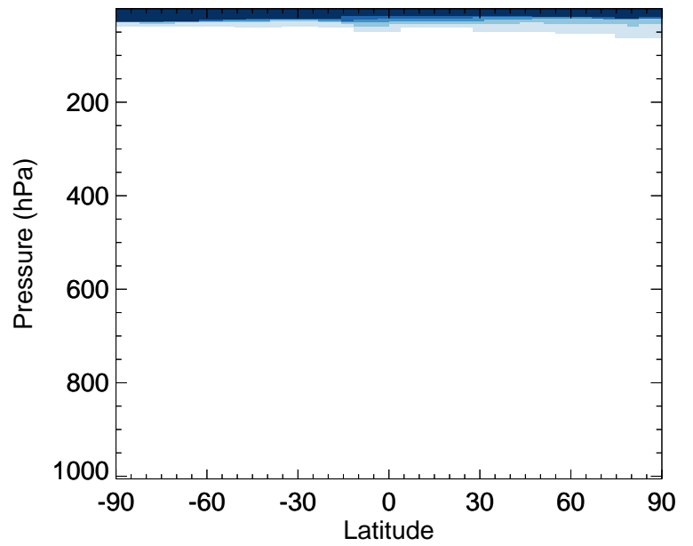
v11-02e-Run0 / v11-02d-Run1 SALA - Zonal mean % diff for Oct
