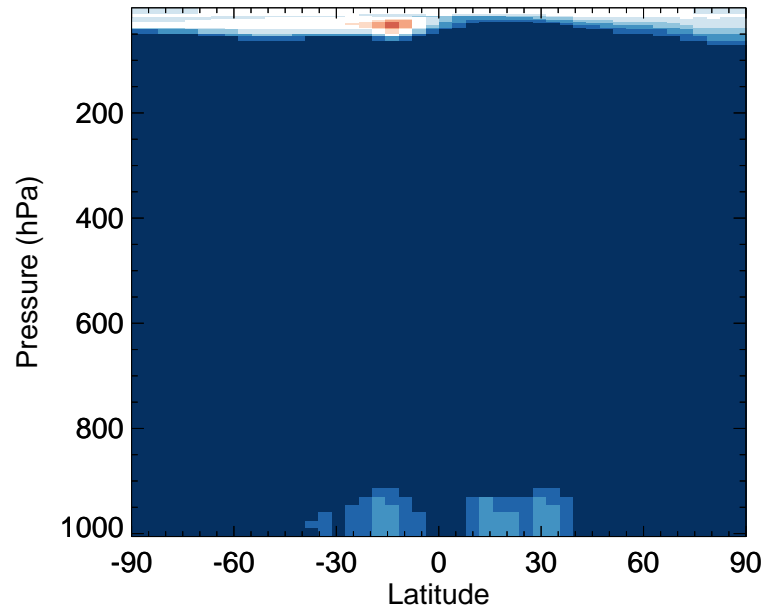
v11-02e-Run0 / v11-02d-Run1 HCl - Zonal mean % diff for Oct
