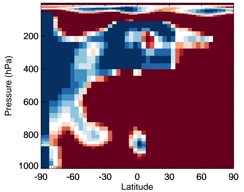
v11-02e-Run0 / v11-02c-Run0 HOCl - Zonal mean % diff for Oct
