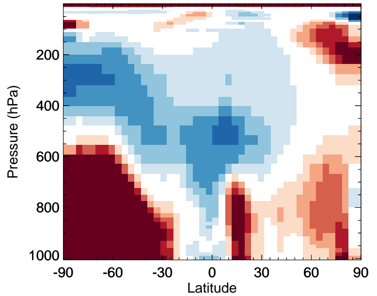
v11-02e-Run0 / v11-02c-Run0 HNO 4 - Zonal mean % diff for Oct
