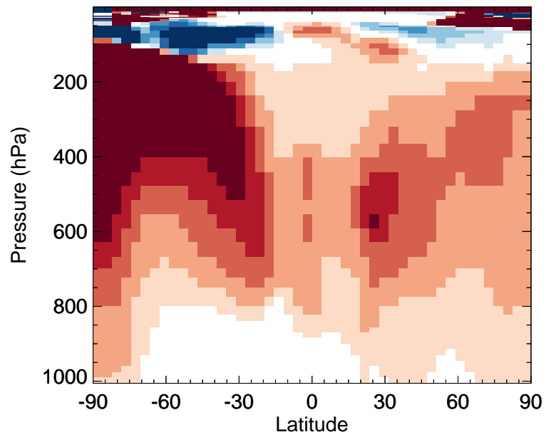
v11-02e-Run0 / v11-02d-Run1 MVK - Zonal mean % diff for Oct
