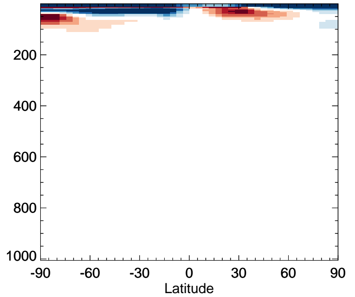
v11-02e-Run0 / v11-02d-Run1 N2O - Zonal mean % diff for Oct
