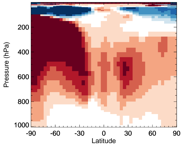
v11-02e-Run0 / v11-02d-Run1 IPMN - Zonal mean % diff for Oct
