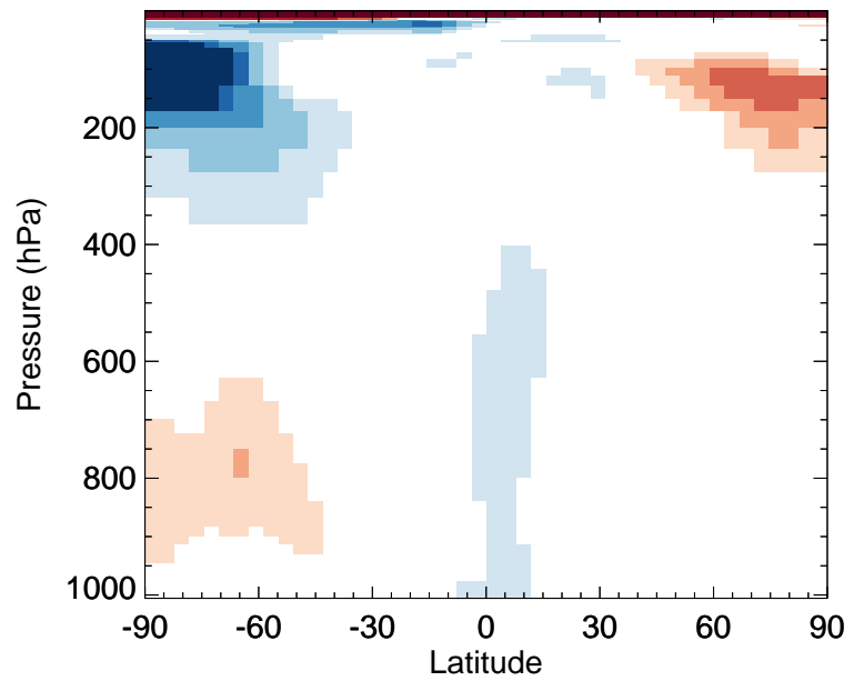
v11-02e-Run0 / v11-02c-Run0 CH 2 O - Zonal mean % diff for Oct
