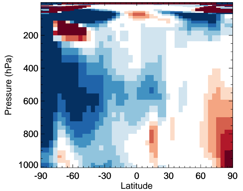
v11-02e-Run0 / v11-02c-Run0 ISN1 - Zonal mean % diff for Oct
