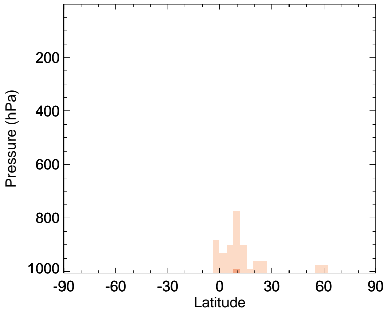
v11-02e-Run0 - v11-02c-Run0 MEK - Zonal mean abs diff for Oct
