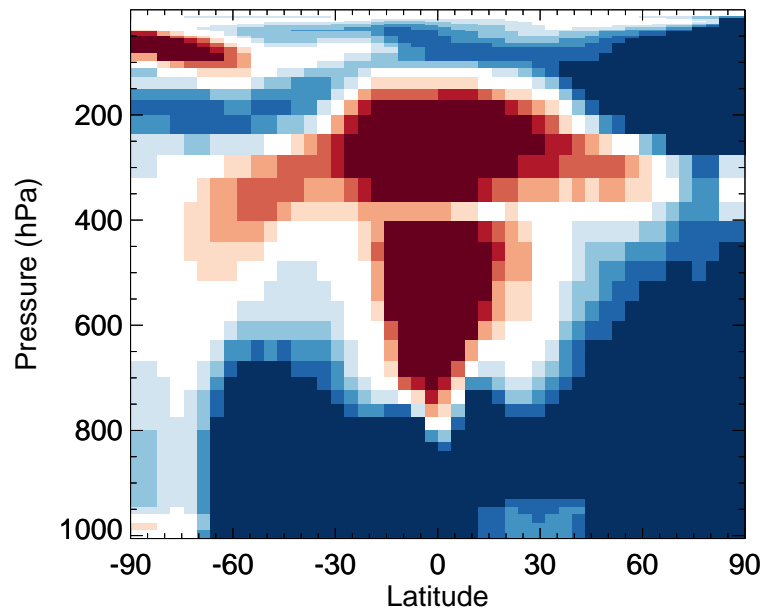
v11-02e-Run0 / v11-02d-Run1 BrO - Zonal mean % diff for Oct
