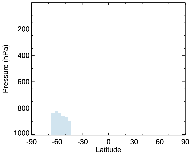
v11-02e-Run0 - v11-02c-Run0 HOBr - Zonal mean abs diff for Oct
