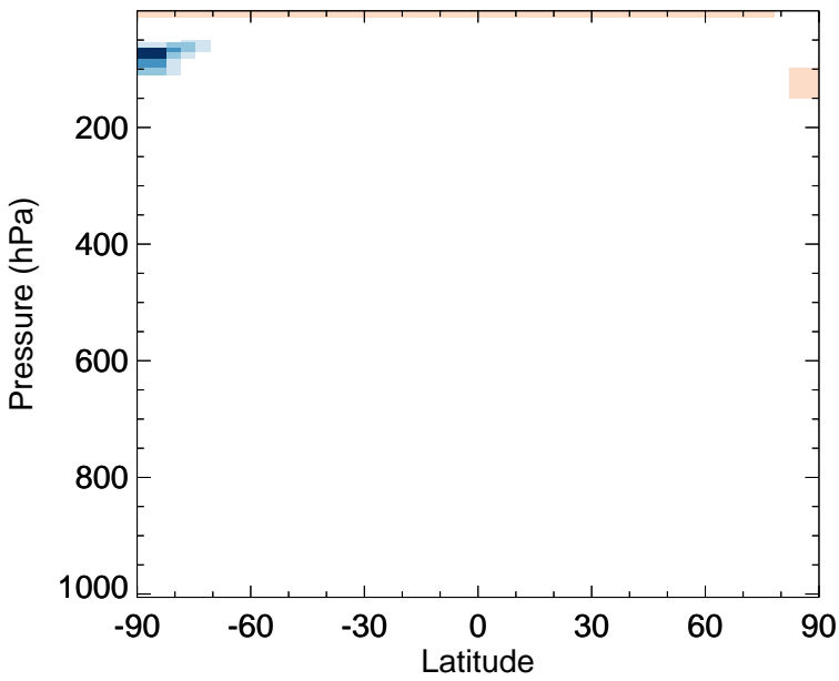
v11-02e-Run0 - v11-02d-Run1 HOCl - Zonal mean abs diff for Oct
