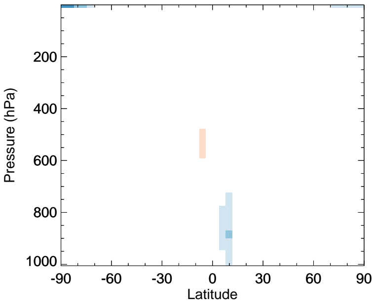
v11-02e-Run0 - v11-02d-Run1 MAP - Zonal mean abs diff for Oct
