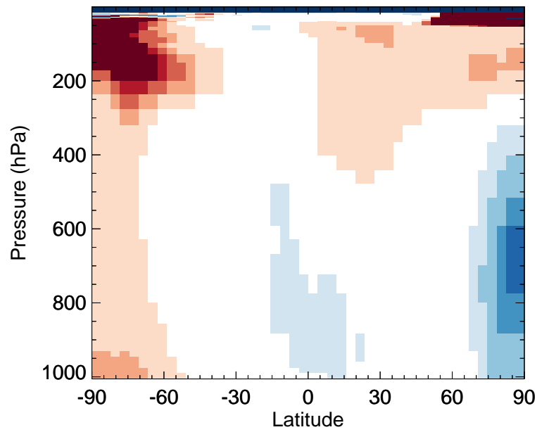
v11-02e-Run0 / v11-02d-Run1 MVKN - Zonal mean % diff for Oct
