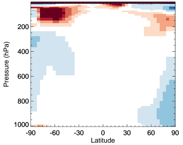
v11-02e-Run0 / v11-02d-Run1 GLYX - Zonal mean % diff for Oct
