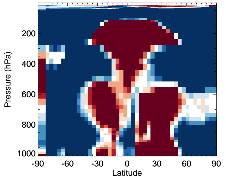
v11-02e-Run0 / v11-02d-Run1 Br2 - Zonal mean % diff for Oct
