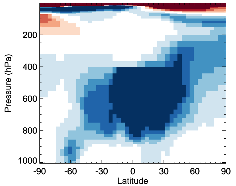
v11-02e-Run0 / v11-02c-Run0 SO 2 - Zonal mean % diff for Oct
