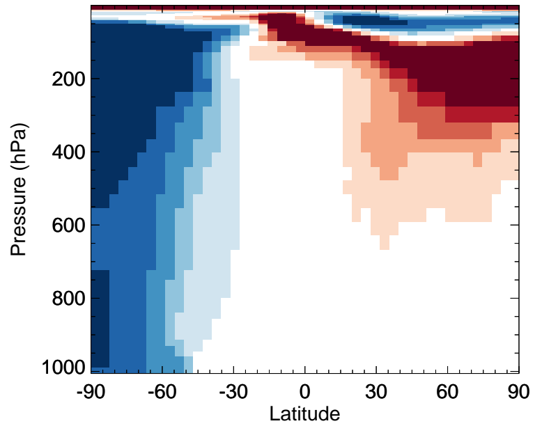
v11-02e-Run0 / v11-02d-Run1 HNO 3 - Zonal mean % diff for Oct
