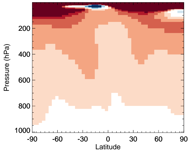
v11-02e-Run0 / v11-02c-Run0 CCI4 - Zonal mean % diff for Oct
