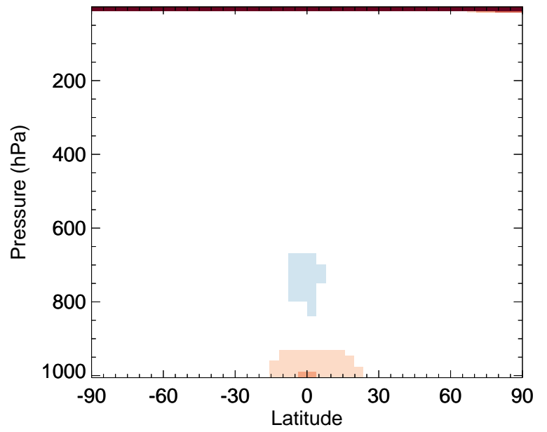
v11-02e-Run0 / v11-02d-Run1 PPN - Zonal mean % diff for Oct
