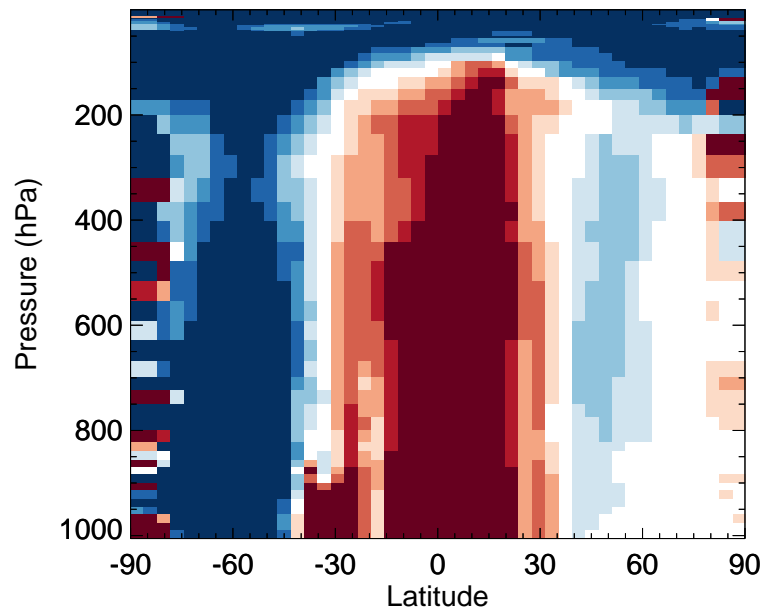
v11-02e-Run0 / v11-02c-Run0 MTPO - Zonal mean % diff for Oct
