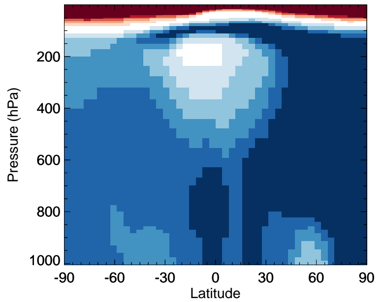
v11-02e-Run0 / v11-02d-Run1 DHDN - Zonal mean % diff for Oct
