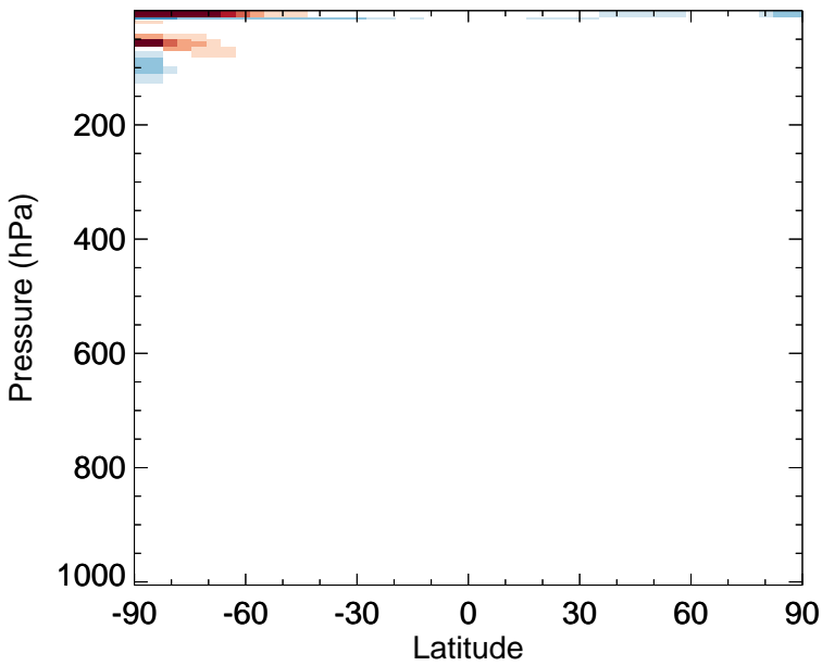
v11-02e-Run0 - v11-02c-Run0 ClO - Zonal mean abs diff for Oct
