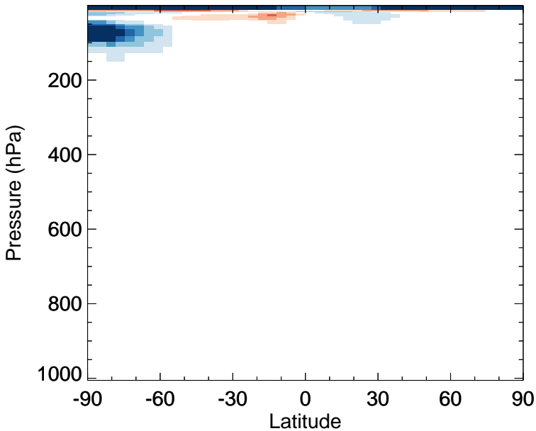
v11-02e-Run0 - v11-02c-Run0 NO - Zonal mean abs diff for Oct
