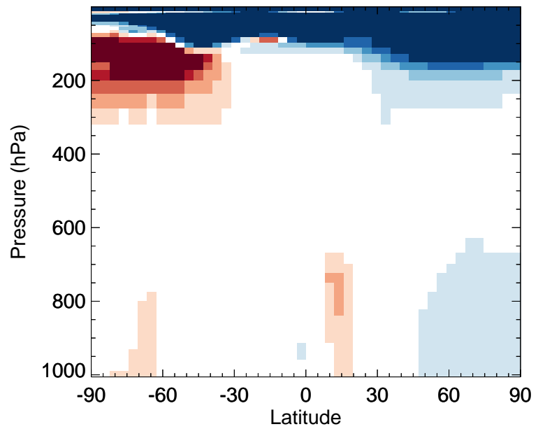
v11-02e-Run0 / v11-02c-Run0 MAP - Zonal mean % diff for Oct
