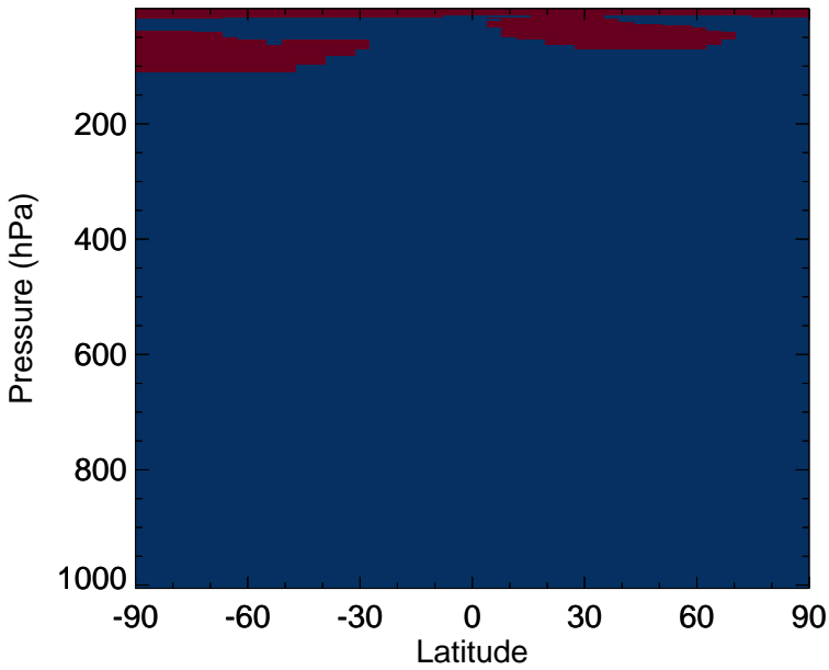
v11-02e-Run0 - v11-02c-Run0 CH4 - Zonal mean abs diff for Oct
