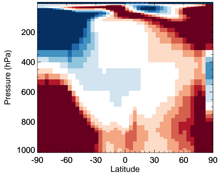
v11-02e-Run0 / v11-02c-Run0 NO - Zonal mean % diff for Oct
