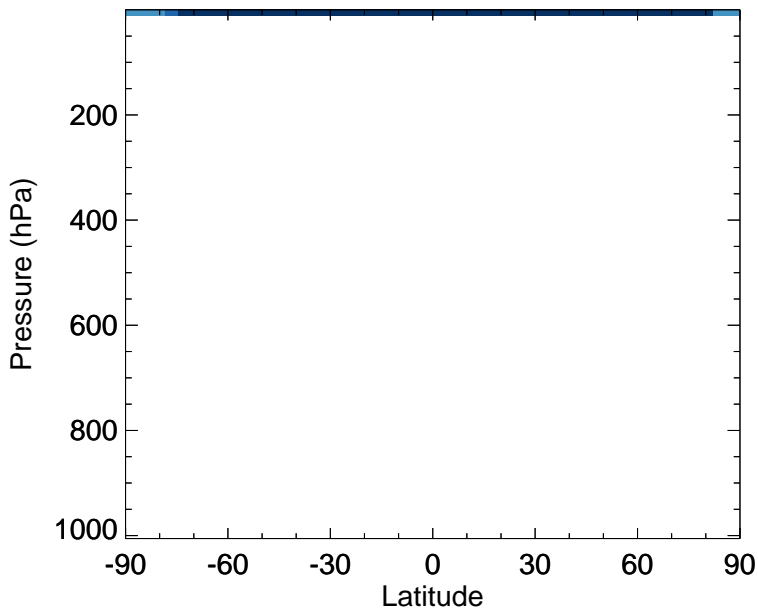
v11-02e-Run0 - v11-02c-Run0 Cl - Zonal mean abs diff for Oct
