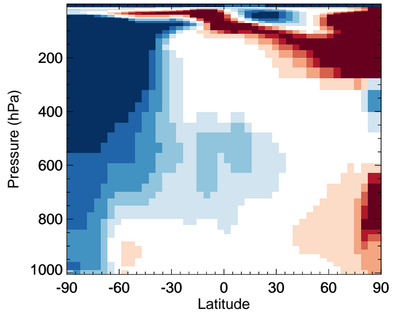
v11-02e-Run0 / v11-02d-Run1 NO - Zonal mean % diff for Oct
