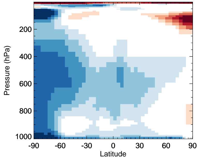
v11-02e-Run0 / v11-02d-Run1 MPN - Zonal mean % diff for Oct
