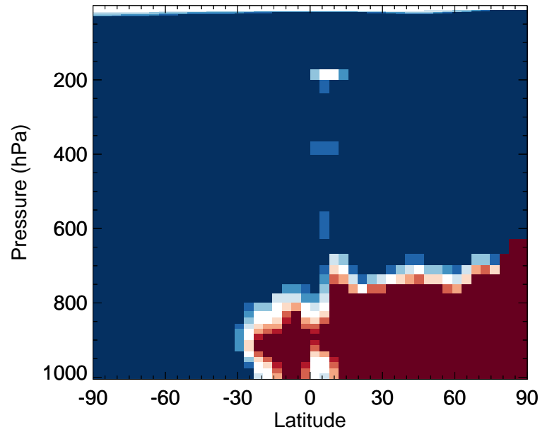
v11-02e-Run0 / v11-02c-Run0 HBr - Zonal mean % diff for Oct
