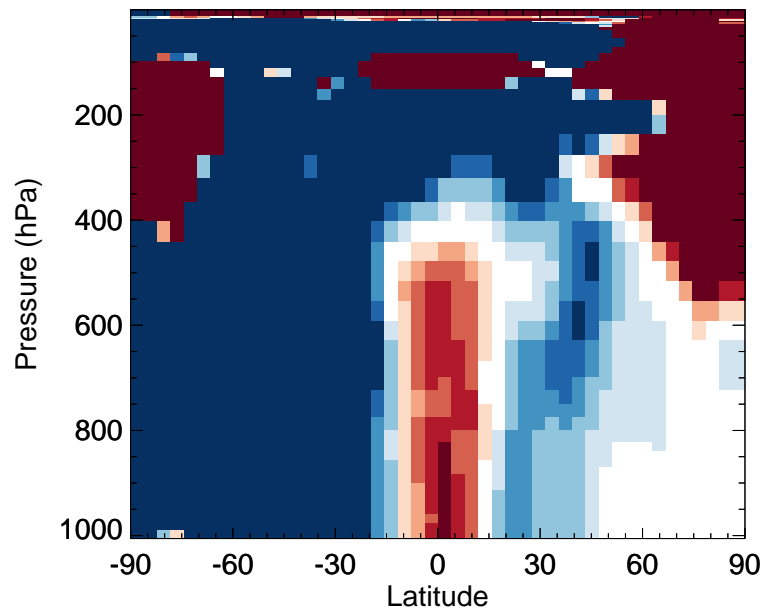
v11-02e-Run0 / v11-02c-Run0 IPMN - Zonal mean % diff for Oct
