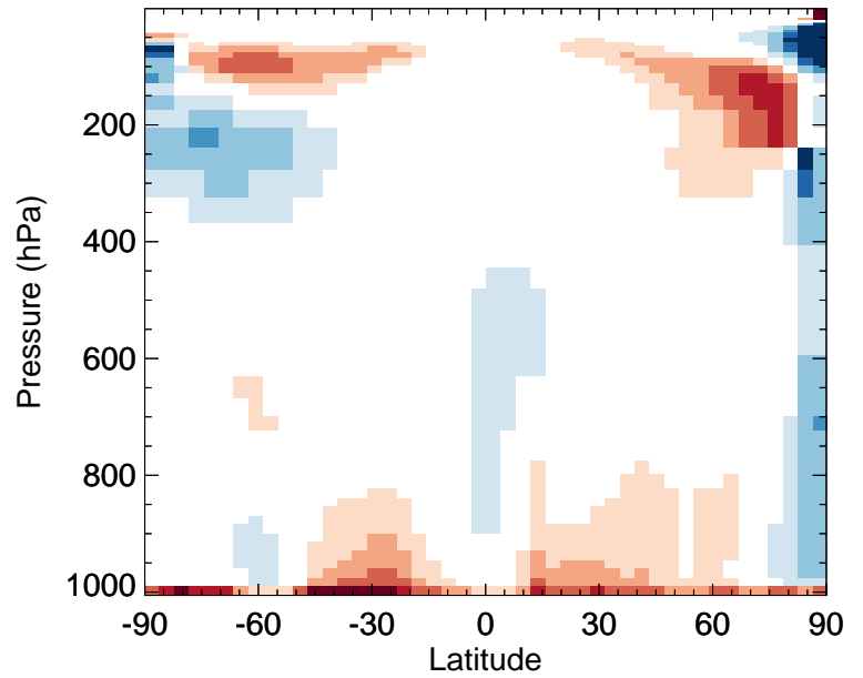
v11-02e-Run0 / v11-02c-Run0 OH - Zonal mean % diff for Oct
