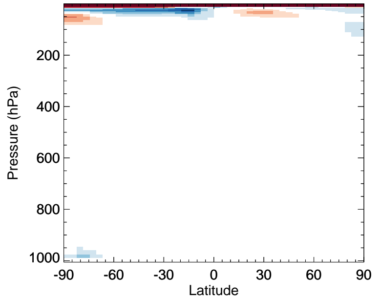
v11-02e-Run0 / v11-02d-Run1 CH4 - Zonal mean % diff for Oct
