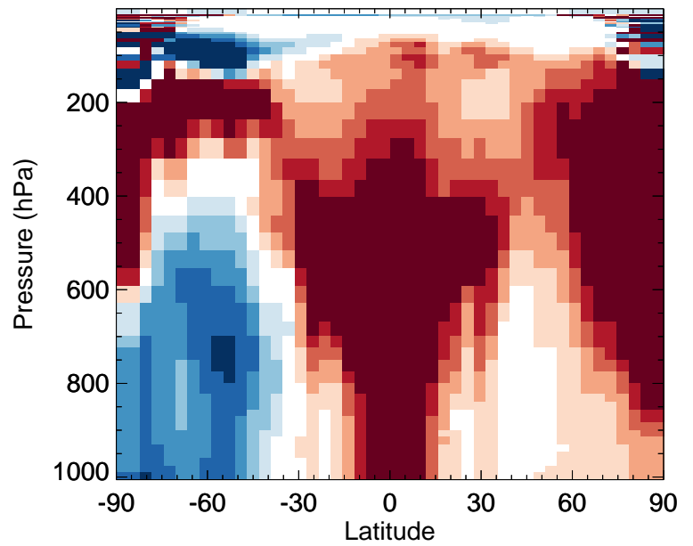
v11-02e-Run0 / v11-02c-Run0 MTPA - Zonal mean % diff for Oct
