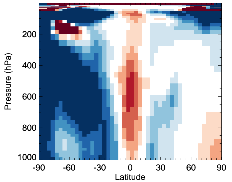
v11-02e-Run0 / v11-02c-Run0 MVK - Zonal mean % diff for Oct
