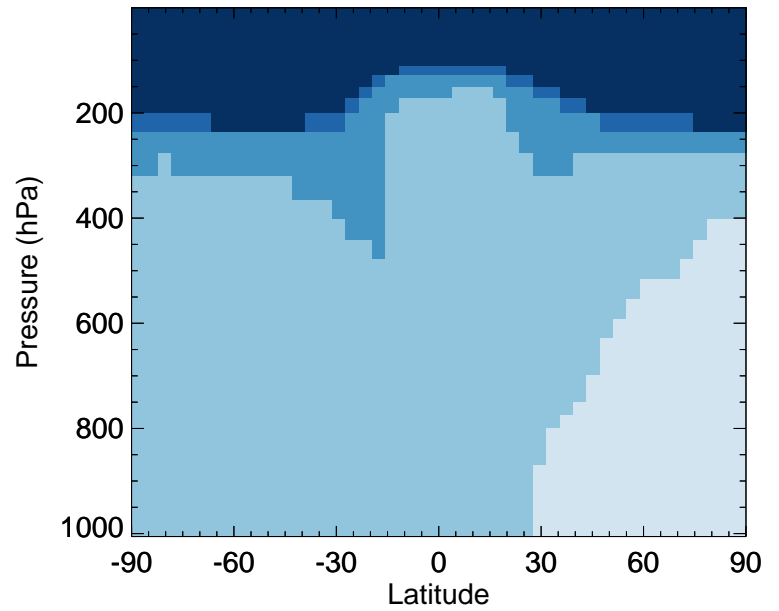
v11-02e-Run0 / v11-02c-Run0 C2H6 - Zonal mean % diff for Oct
