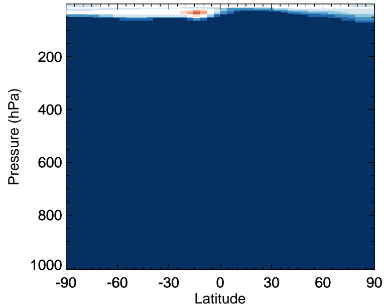
v11-02e-Run0 / v11-02c-Run0 HCl - Zonal mean % diff for Oct
