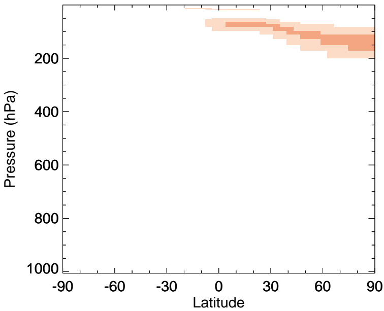
v11-02e-Run0 - v11-02c-Run0 SO4 - Zonal mean abs diff for Oct
