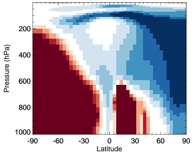
v11-02e-Run0 / v11-02c-Run0 DHDN - Zonal mean % diff for Oct
