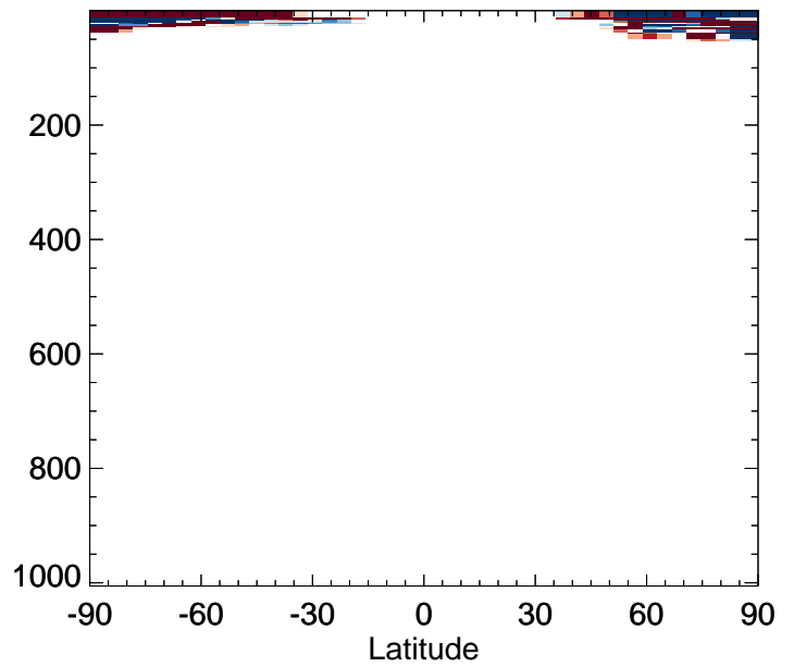
v11-02e-Run0 / v11-02c-Run0 BCPO - Zonal mean % diff for Oct
