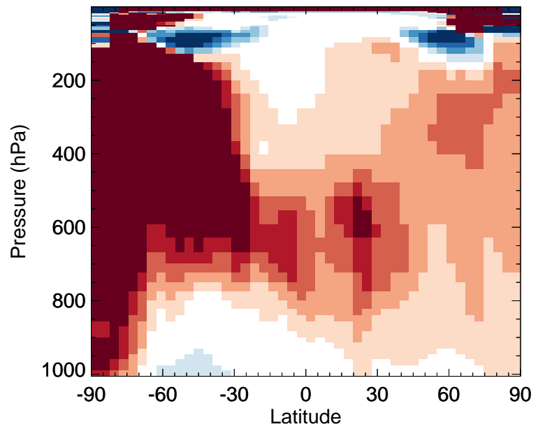
v11-02e-Run0 / v11-02d-Run1 ISOP - Zonal mean % diff for Oct
