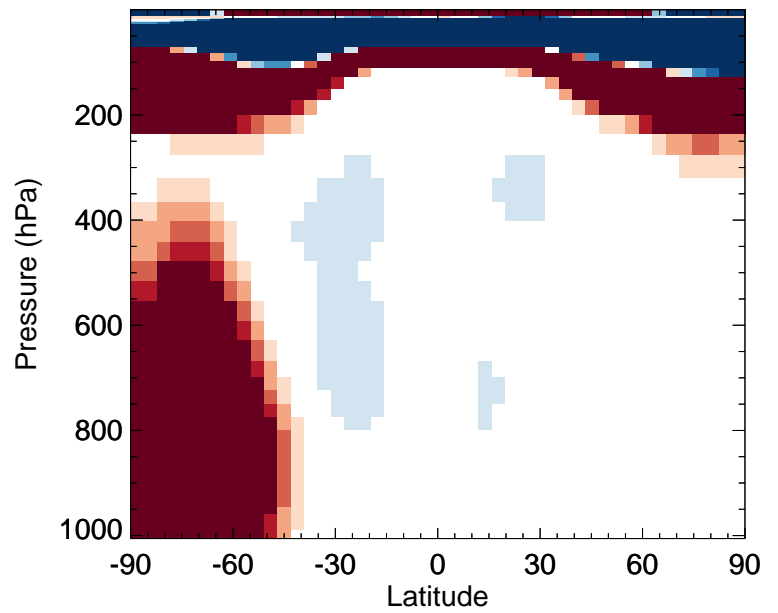
v11-02e-Run0 / v11-02c-Run0 ALD2 - Zonal mean % diff for Oct
