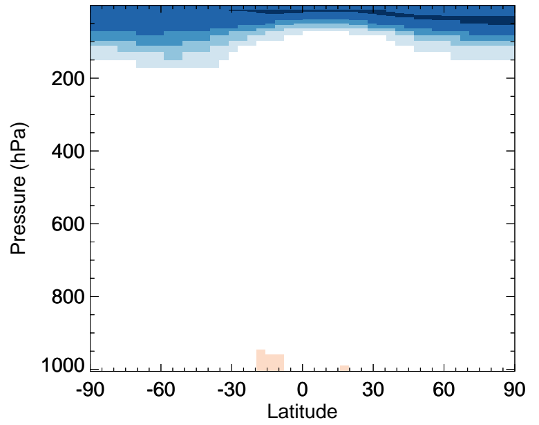
v11-02e-Run0 / v11-02d-Run1 NH4 - Zonal mean % diff for Oct
