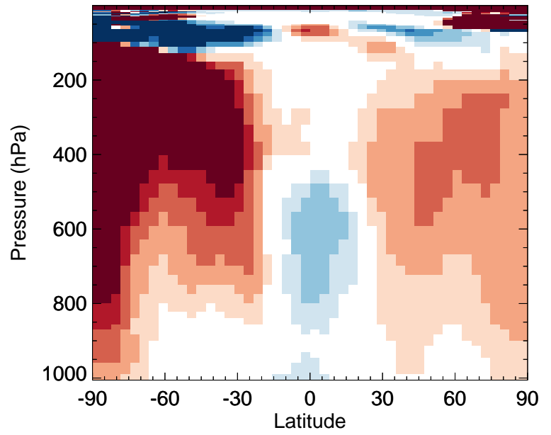
v11-02e-Run0 / v11-02d-Run1 ISN1 - Zonal mean % diff for Oct
