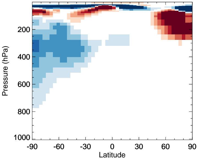
v11-02e-Run0 - v11-02d-Run1 HNO 4 - Zonal mean abs diff for Oct
