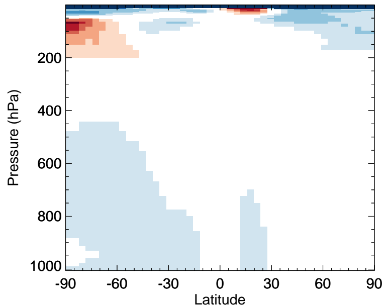
v11-02e-Run0 / v11-02c-Run0 BENZ - Zonal mean % diff for Oct
