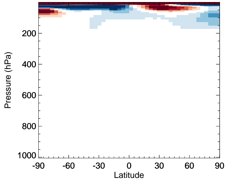
v11-02e-Run0 / v11-02c-Run0 CH3Cl - Zonal mean % diff for Oct
