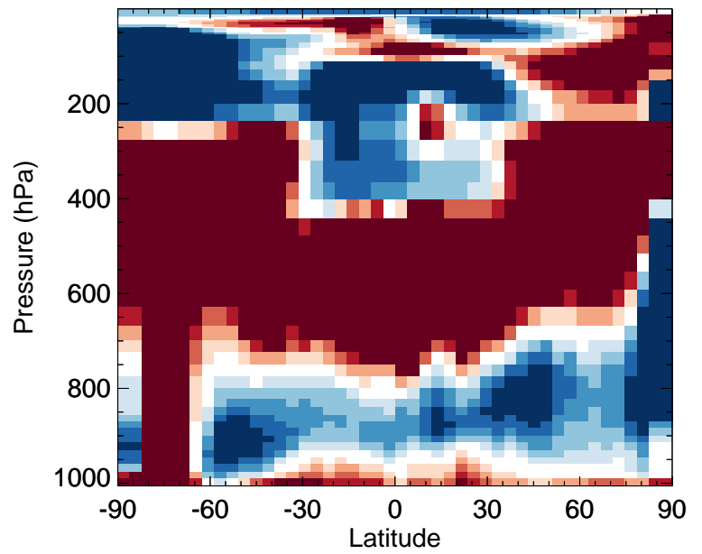
v11-02e-Run0 / v11-02d-Run1 ClOO - Zonal mean % diff for Oct
