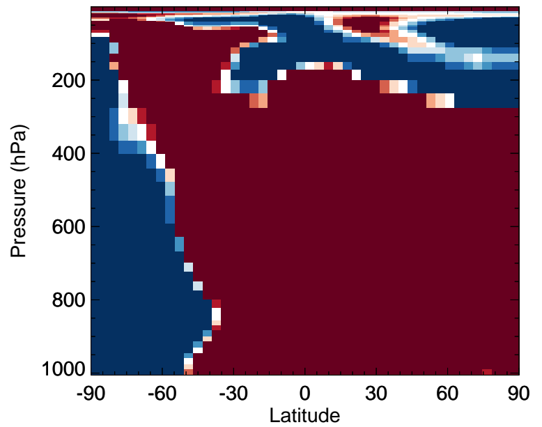
v11-02e-Run0 / v11-02c-Run0 OCIO - Zonal mean % diff for Oct
