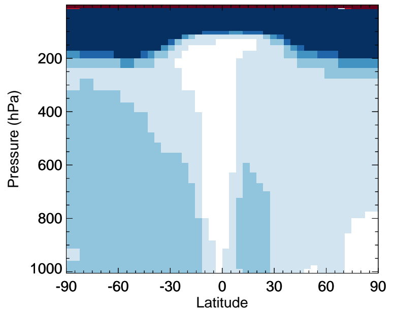
v11-02e-Run0 / v11-02c-Run0 ALK4 - Zonal mean % diff for Oct
