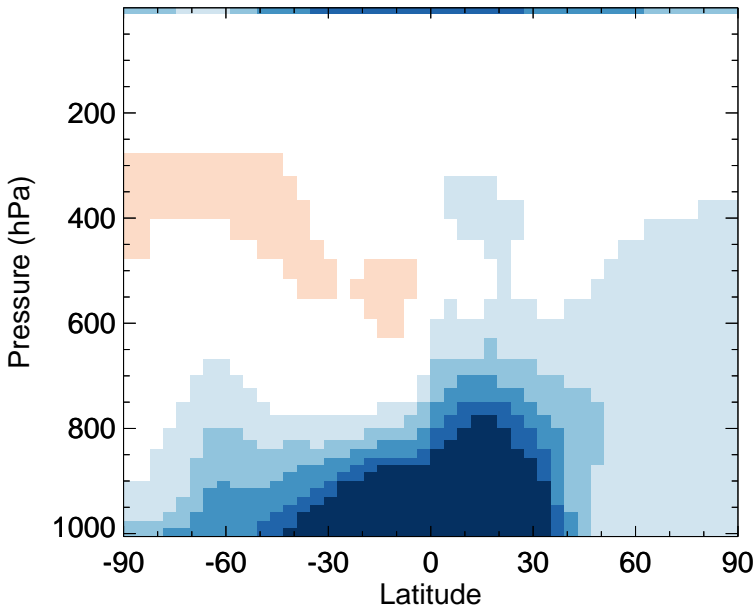
v11-02e-Run0 - v11-02d-Run1 MP - Zonal mean abs diff for Oct
