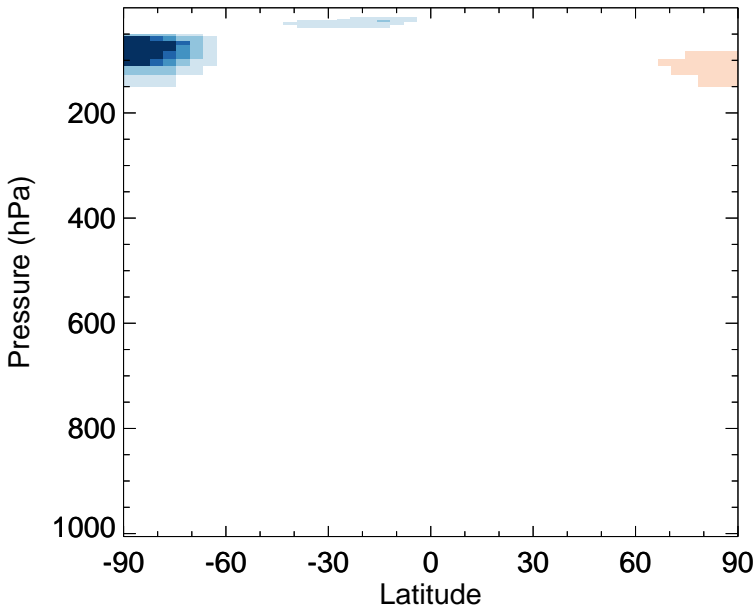
v11-02e-Run0 - v11-02d-Run1 MPN - Zonal mean abs diff for Oct
