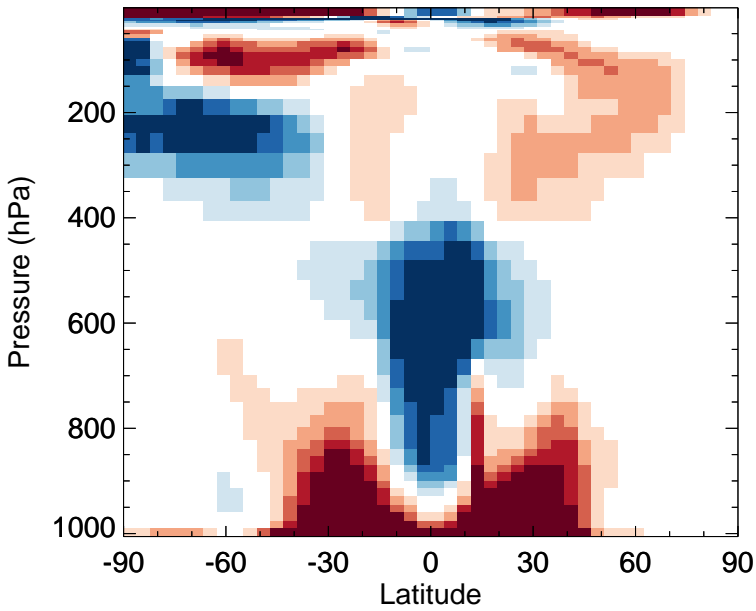
v11-02e-Run0 - v11-02c-Run0 OH - Zonal mean abs diff for Oct
