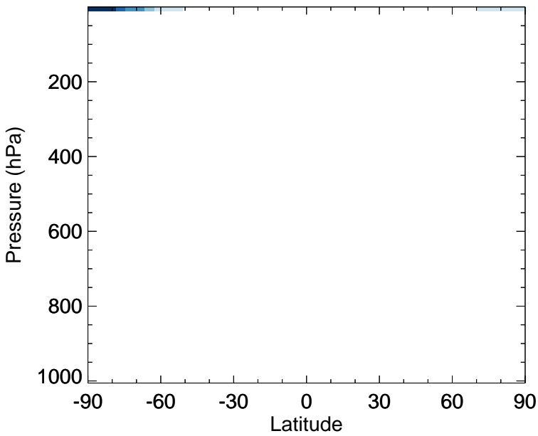
v11-02e-Run0 - v11-02c-Run0 ACTA - Zonal mean abs diff for Oct
