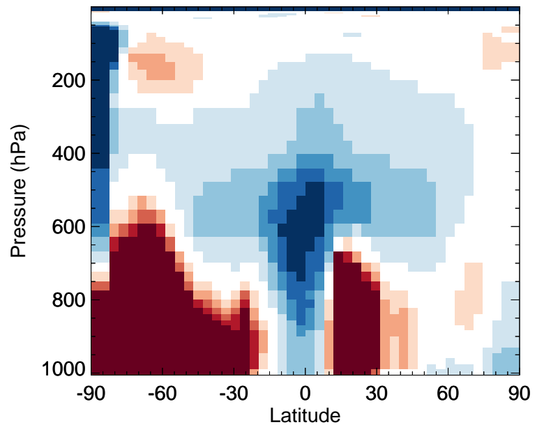
v11-02e-Run0 / v11-02c-Run0 NO3 - Zonal mean % diff for Oct
