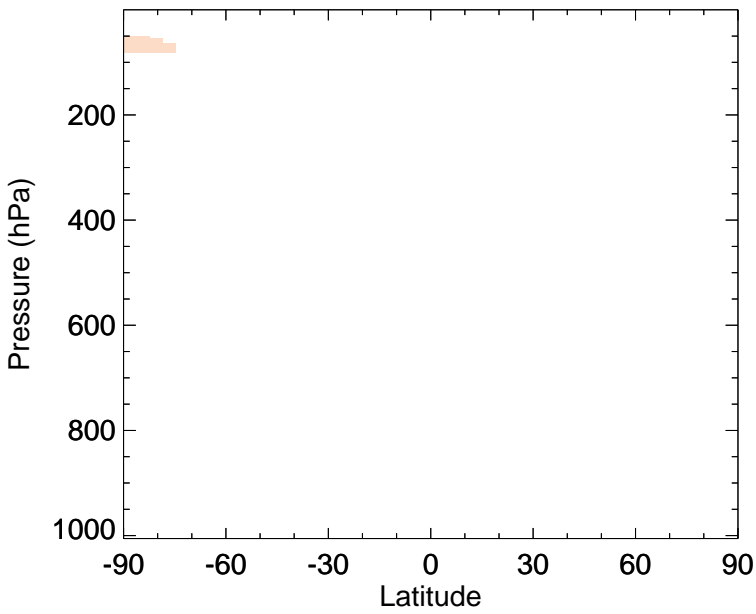
v11-02e-Run0 - v11-02d-Run1 BrO - Zonal mean abs diff for Oct
