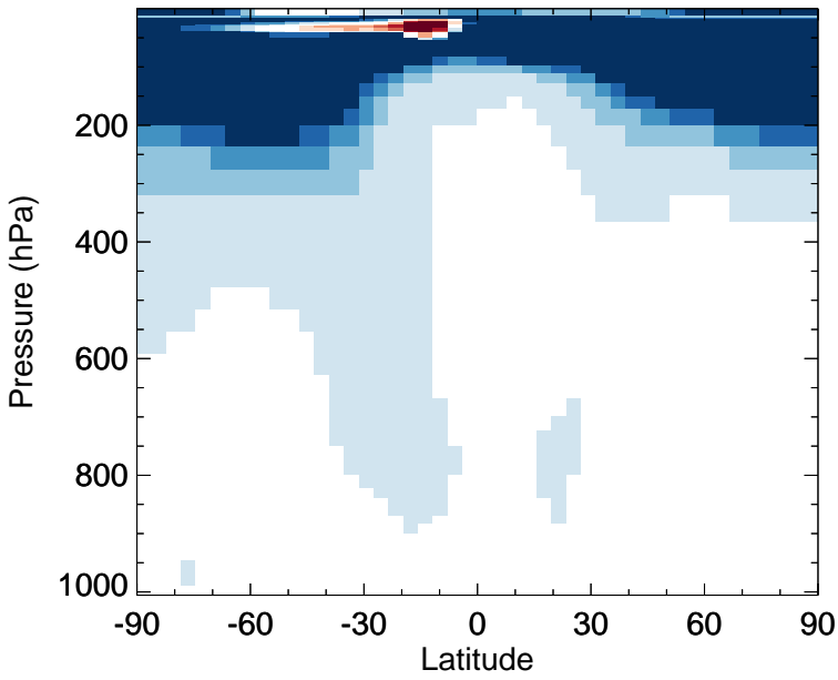
v11-02e-Run0 - v11-02c-Run0 HCl - Zonal mean abs diff for Oct
