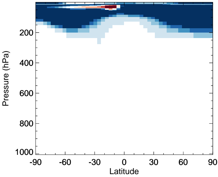
v11-02e-Run0 - v11-02d-Run1 HCl - Zonal mean abs diff for Oct
