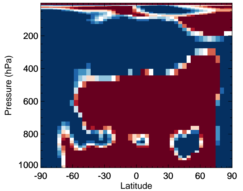
v11-02e-Run0 / v11-02c-Run0 Cl2 - Zonal mean % diff for Oct
