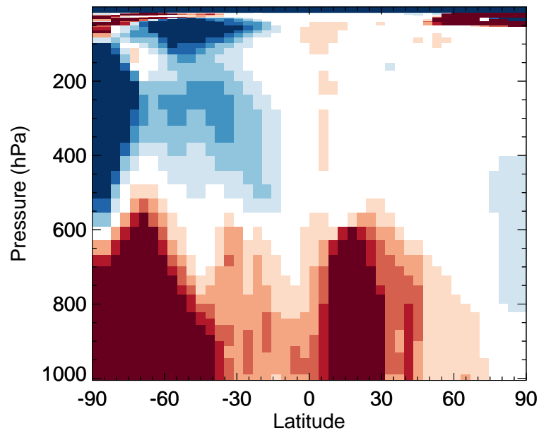
v11-02e-Run0 / v11-02c-Run0 MVKN - Zonal mean % diff for Oct
