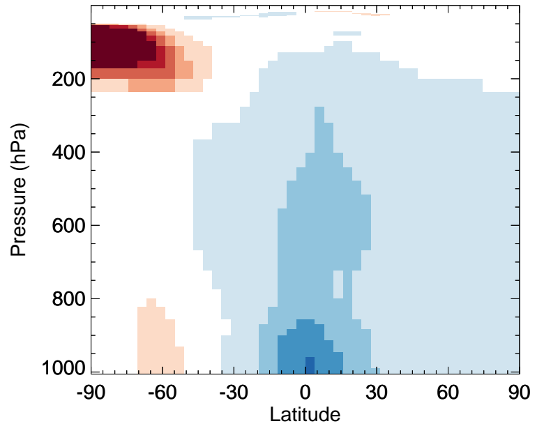
v11-02e-Run0 / v11-02c-Run0 O3 - Zonal mean % diff for Oct
