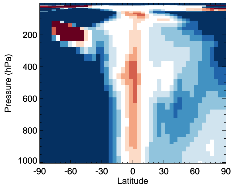
v11-02e-Run0 / v11-02c-Run0 HPALD - Zonal mean % diff for Oct
