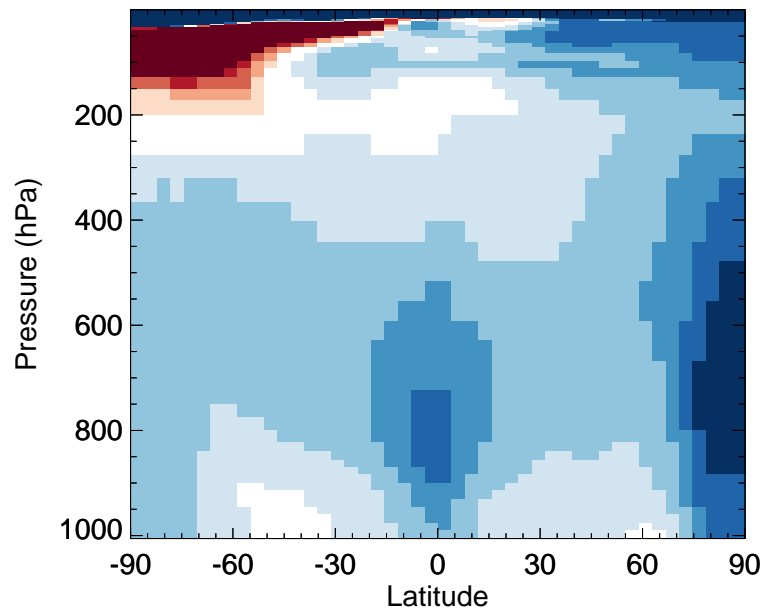
v11-02e-Run0 / v11-02d-Run1 R4N2 - Zonal mean % diff for Oct
