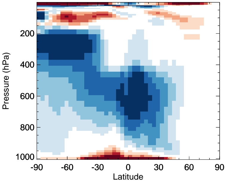
v11-02e-Run0 - v11-02d-Run1 OH - Zonal mean abs diff for Oct
