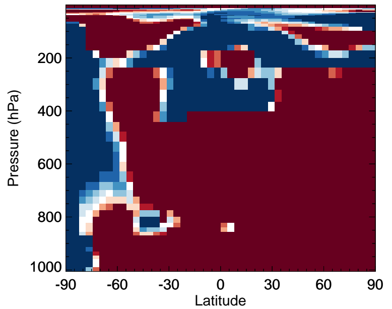
v11-02e-Run0 / v11-02c-Run0 Cl2O2 - Zonal mean % diff for Oct
