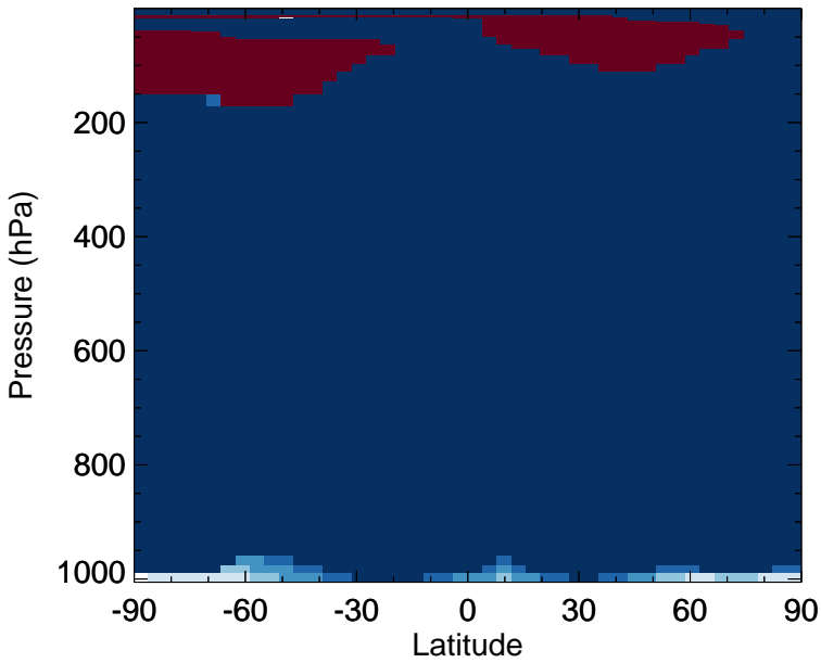
v11-02e-Run0 - v11-02c-Run0 N2O - Zonal mean abs diff for Oct
