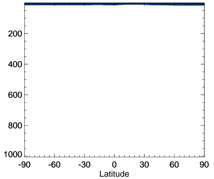
v11-02e-Run0 / v11-02d-Run1 SALC - Zonal mean % diff for Oct
