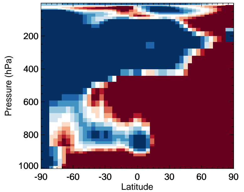
v11-02e-Run0 / v11-02c-Run0 ClOO - Zonal mean % diff for Oct
