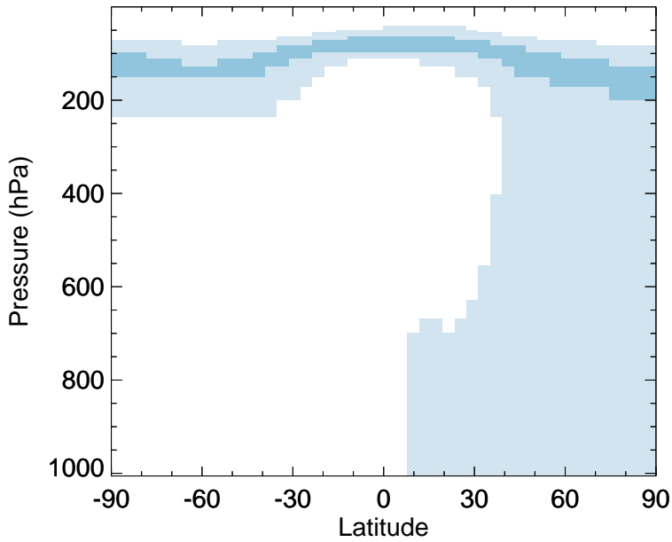
v11-02e-Run0 - v11-02c-Run0 C2H6 - Zonal mean abs diff for Oct
