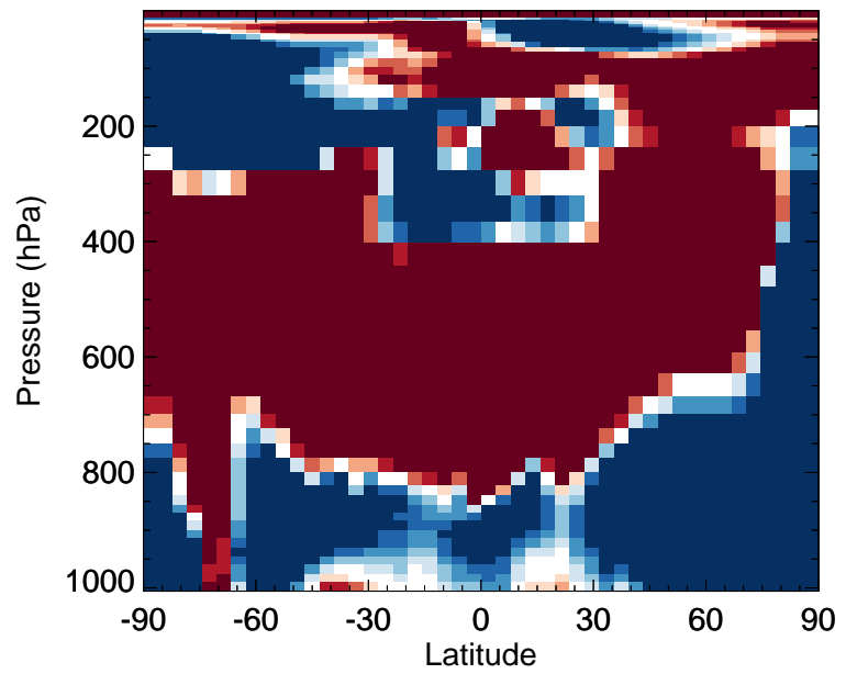
v11-02e-Run0 / v11-02d-Run1 Cl2 - Zonal mean % diff for Oct
