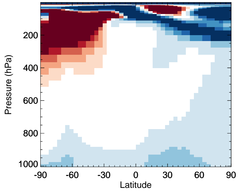
v11-02e-Run0 / v11-02d-Run1 MP - Zonal mean % diff for Oct
