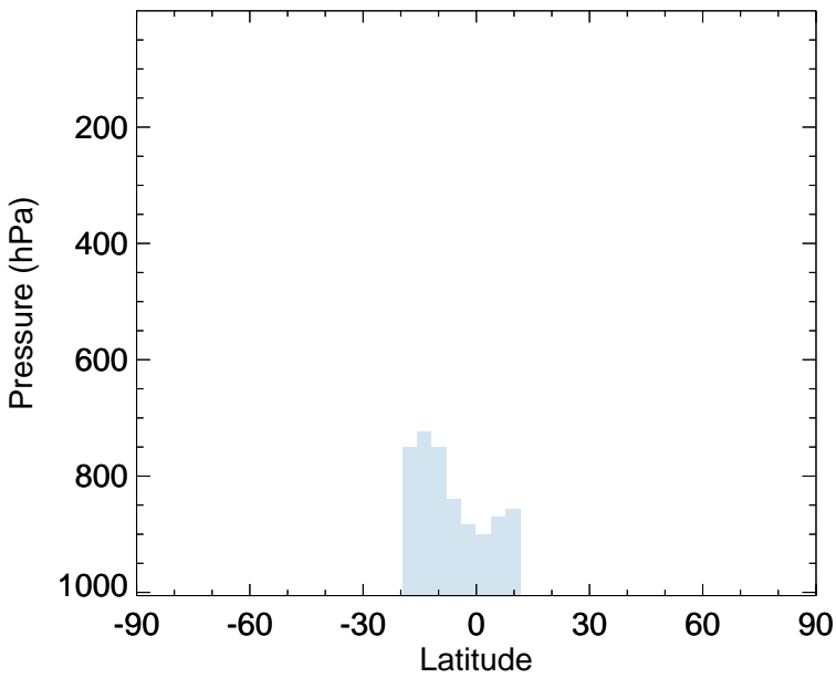
v11-02e-Run0 - v11-02c-Run0 SOAGX - Zonal mean abs diff for Oct
