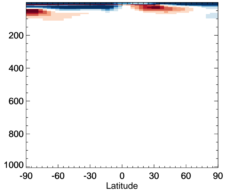
v11-02e-Run0 / v11-02c-Run0 N2O - Zonal mean % diff for Oct
