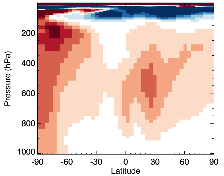
v11-02e-Run0 / v11-02d-Run1 GLYC - Zonal mean % diff for Oct
