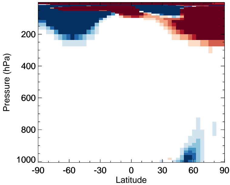
v11-02e-Run0 - v11-02c-Run0 N2O5 - Zonal mean abs diff for Oct
