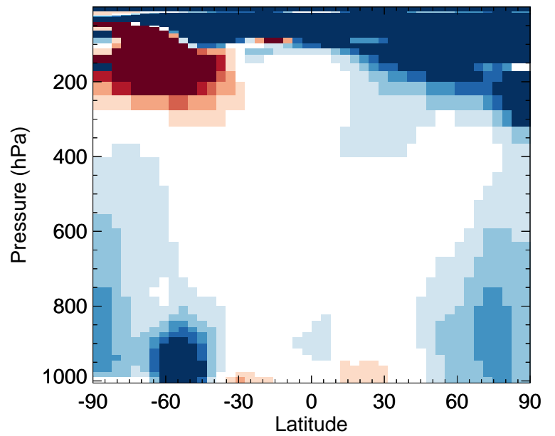
v11-02e-Run0 / v11-02c-Run0 ACTA - Zonal mean % diff for Oct
