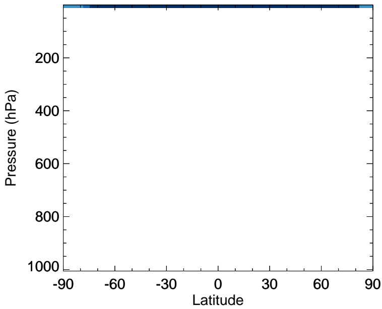
v11-02e-Run0 - v11-02d-Run1 Cl - Zonal mean abs diff for Oct
