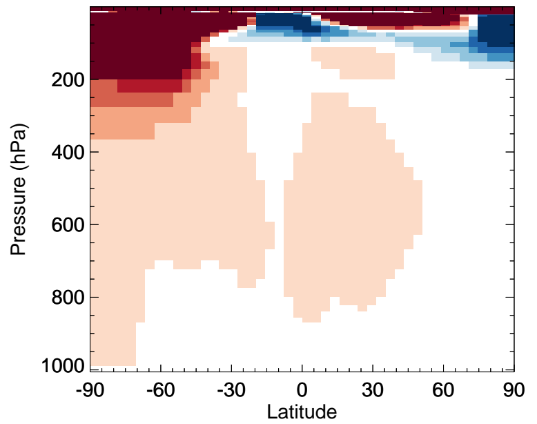
v11-02e-Run0 / v11-02d-Run1 ALK4 - Zonal mean % diff for Oct
