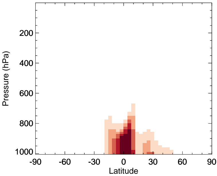
v11-02e-Run0 - v11-02d-Run1 PRPE - Zonal mean abs diff for Oct
