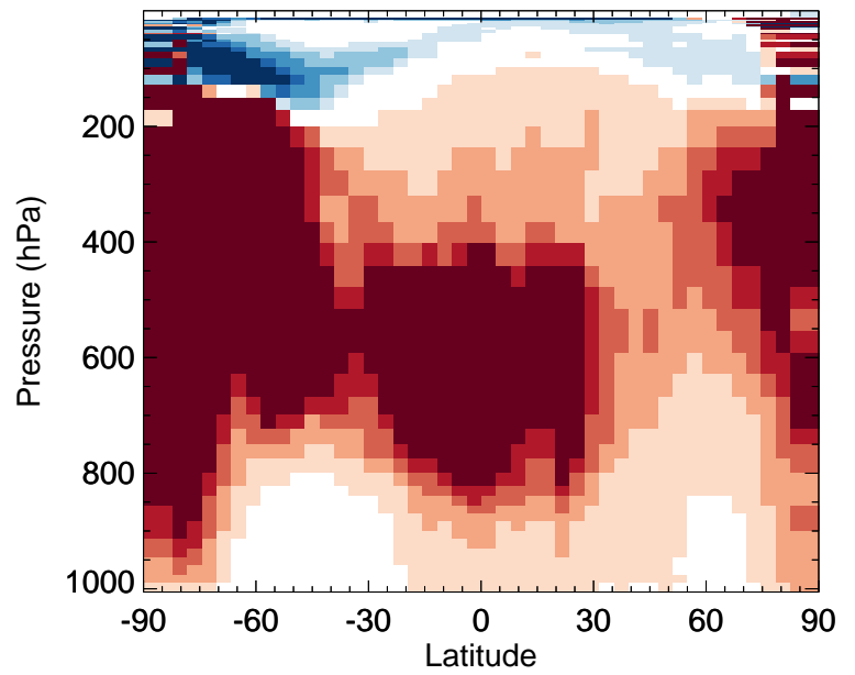
v11-02e-Run0 / v11-02d-Run1 LIMO - Zonal mean % diff for Oct
