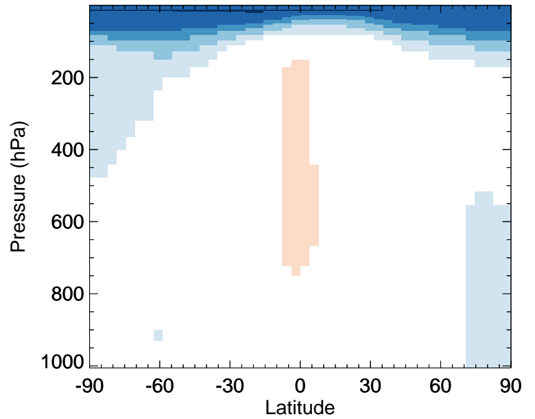
v11-02e-Run0 / v11-02c-Run0 MSA - Zonal mean % diff for Oct
