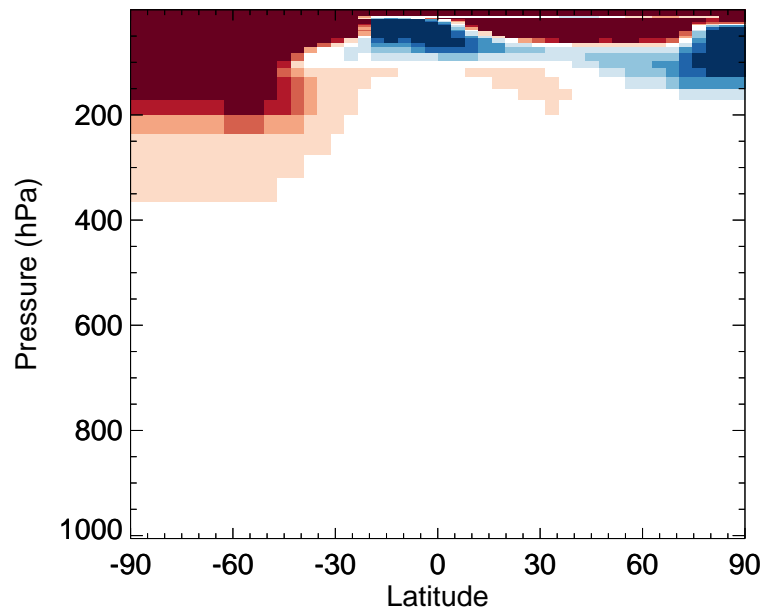
v11-02e-Run0 / v11-02d-Run1 C3H8 - Zonal mean % diff for Oct
