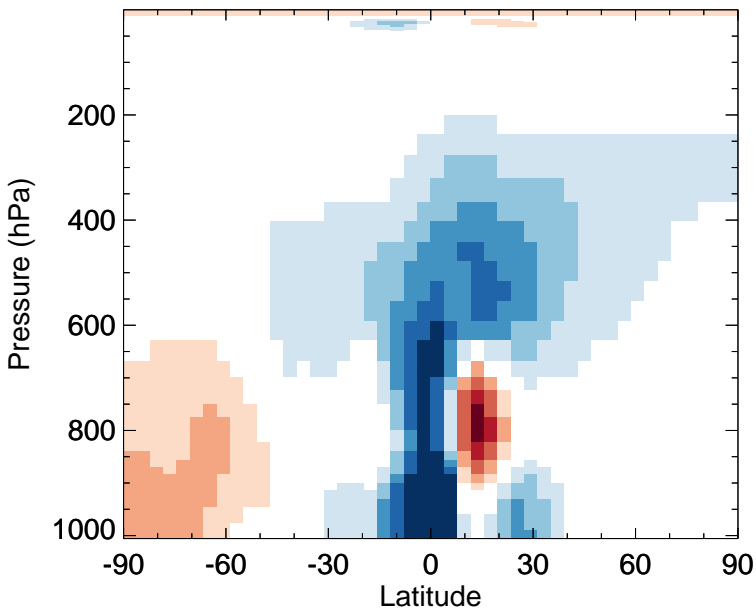
v11-02e-Run0 - v11-02c-Run0 H2O2 - Zonal mean abs diff for Oct
