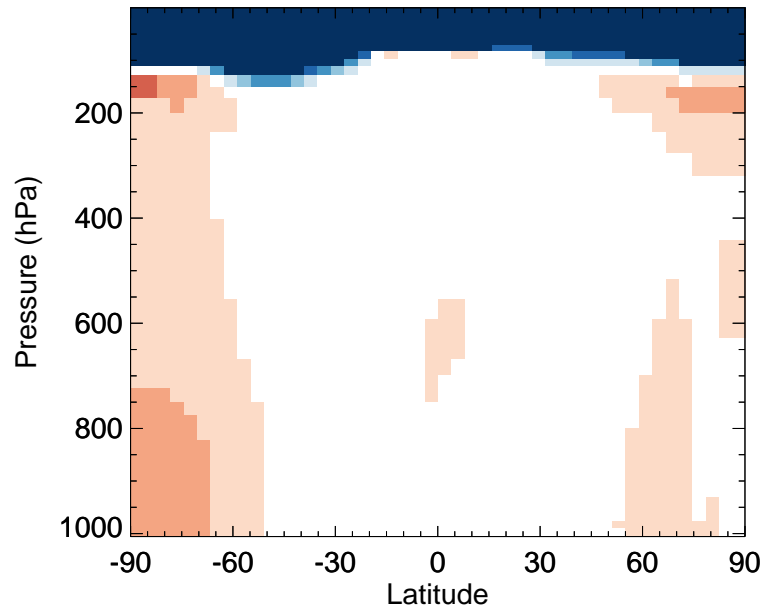
v11-02e-Run0 / v11-02c-Run0 MEK - Zonal mean % diff for Oct
