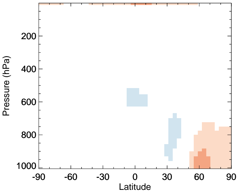
v11-02e-Run0 - v11-02d-Run1 PPN - Zonal mean abs diff for Oct
