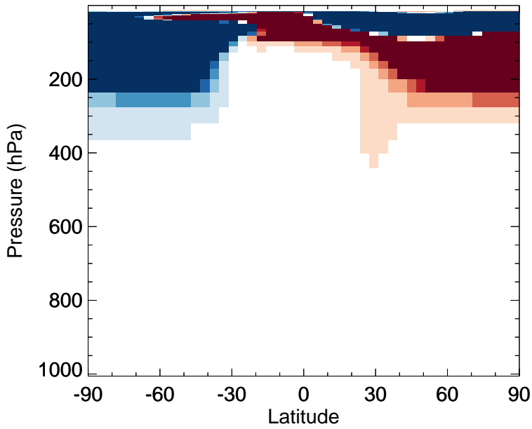
v11-02e-Run0 - v11-02d-Run1 HNO 3 - Zonal mean abs diff for Oct
