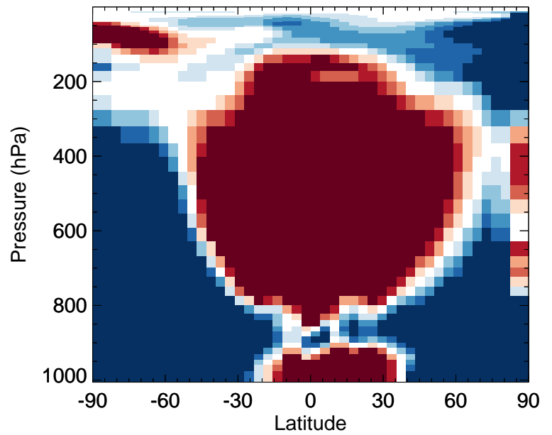
v11-02e-Run0 / v11-02c-Run0 BrO - Zonal mean % diff for Oct
