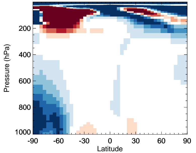
v11-02e-Run0 / v11-02c-Run0 MGLY - Zonal mean % diff for Oct
