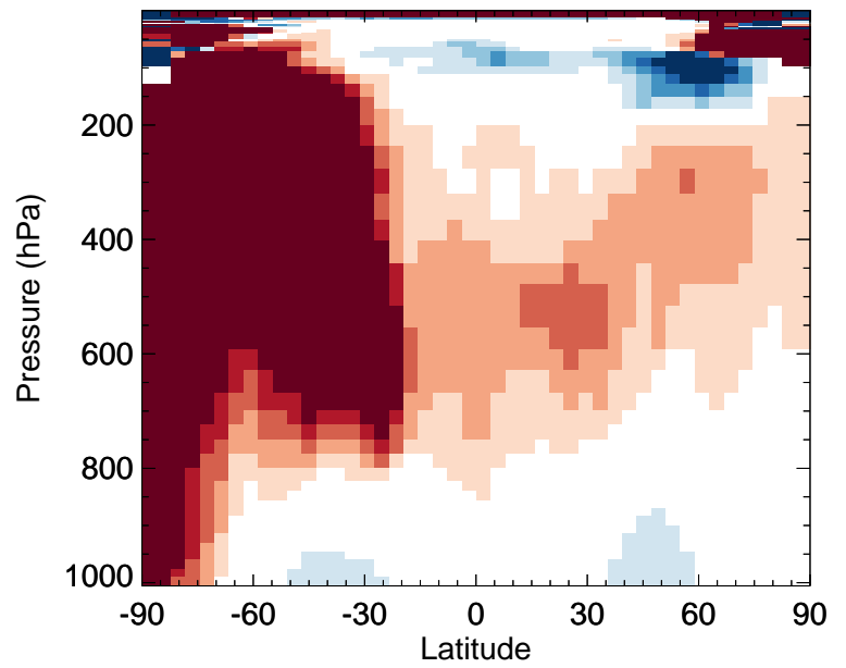
v11-02e-Run0 / v11-02d-Run1 RIPD - Zonal mean % diff for Oct
