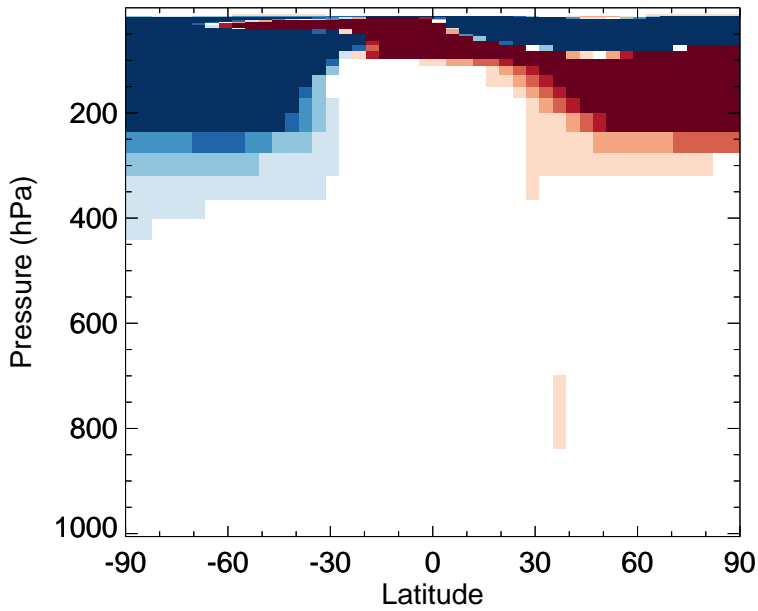
v11-02e-Run0 - v11-02c-Run0 HNO 3 - Zonal mean abs diff for Oct
