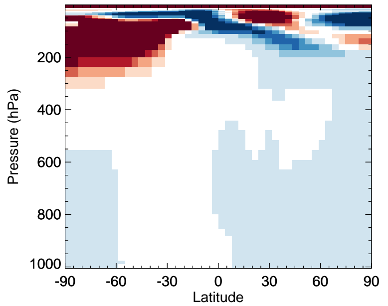
v11-02e-Run0 / v11-02d-Run1 H2O2 - Zonal mean % diff for Oct
