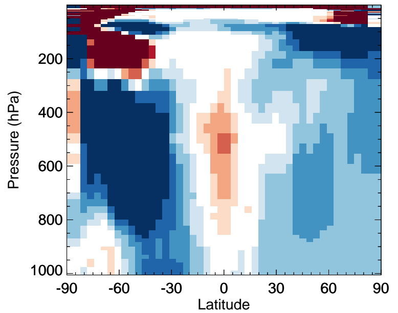
v11-02e-Run0 / v11-02c-Run0 RIPD - Zonal mean % diff for Oct
