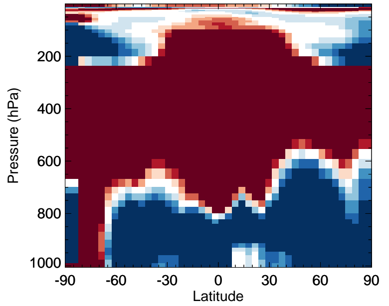
v11-02e-Run0 / v11-02d-Run1 BrCl - Zonal mean % diff for Oct
