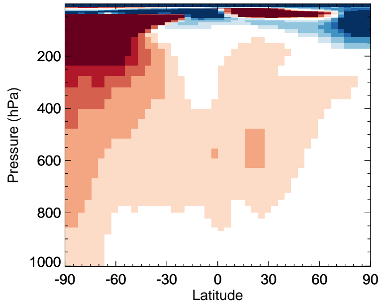
v11-02e-Run0 / v11-02d-Run1 EOH - Zonal mean % diff for Oct
