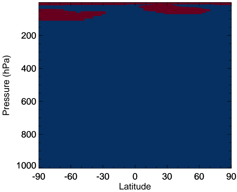
v11-02e-Run0 - v11-02d-Run1 CH4 - Zonal mean abs diff for Oct
