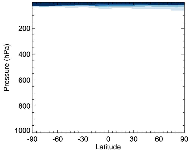
v11-02e-Run0 / v11-02c-Run0 SALA - Zonal mean % diff for Oct
