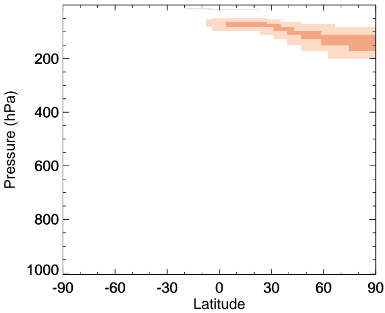
v11-02e-Run0 - v11-02d-Run1 SO4 - Zonal mean abs diff for Oct
