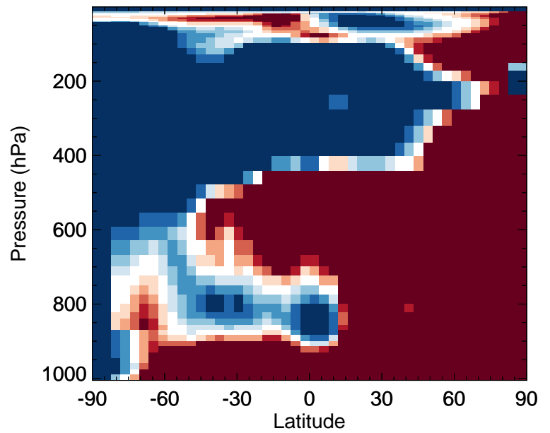
v11-02e-Run0 / v11-02c-Run0 Cl - Zonal mean % diff for Oct
