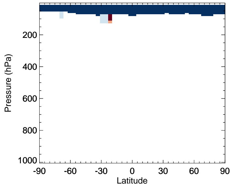
v11-02e-Run0 / v11-02d-Run1 SO4s - Zonal mean % diff for Oct
