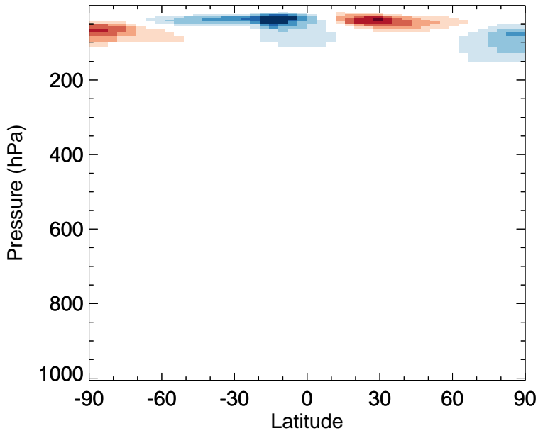
v11-02e-Run0 - v11-02c-Run0 OCS - Zonal mean abs diff for Oct
