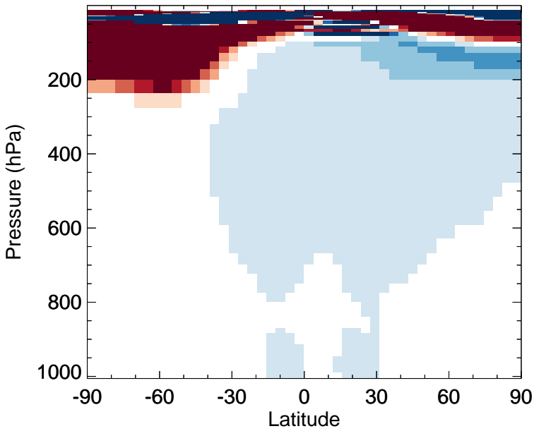
v11-02e-Run0 - v11-02c-Run0 O3 - Zonal mean abs diff for Oct
