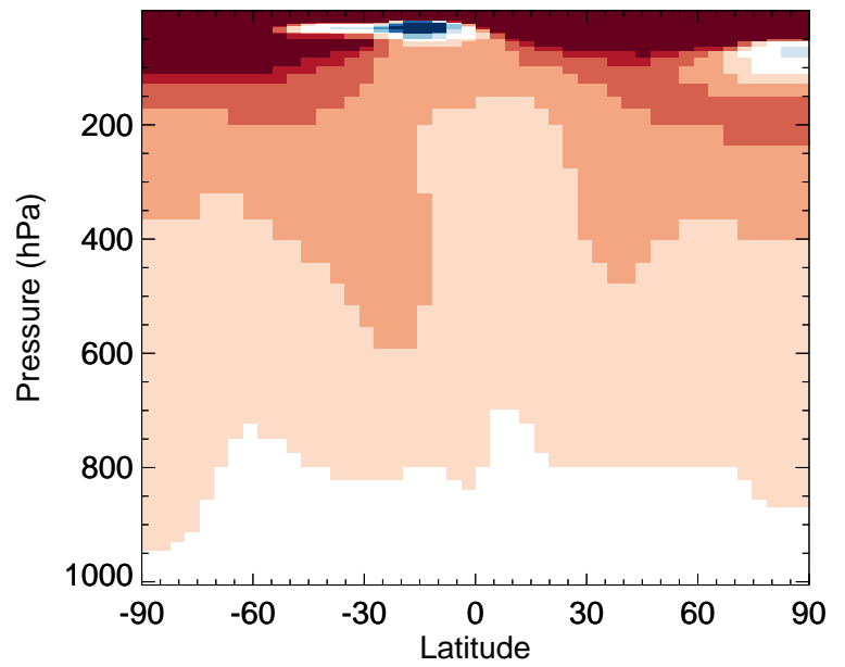
v11-02e-Run0 / v11-02d-Run1 CCI4 - Zonal mean % diff for Oct
