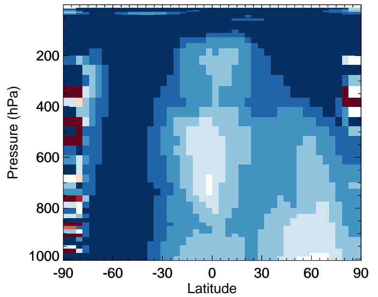
v11-02e-Run0 / v11-02d-Run1 MTPO - Zonal mean % diff for Oct
