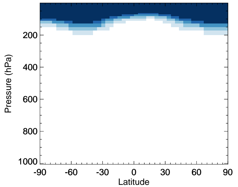
v11-02e-Run0 / v11-02c-Run0 OCPI - Zonal mean % diff for Oct
