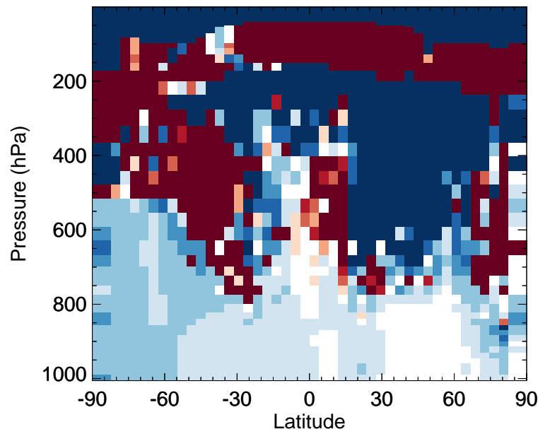
v11-02e-Run0 / v11-02d-Run1 NIT - Zonal mean % diff for Oct
