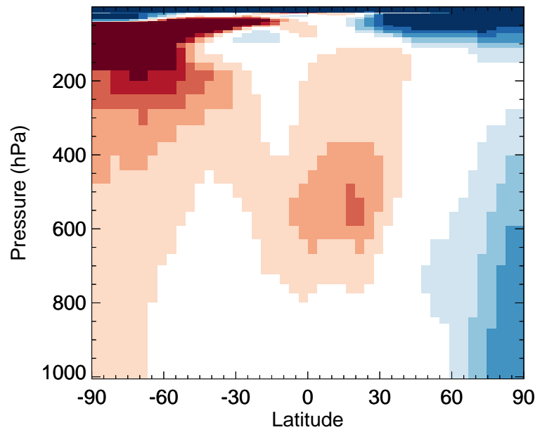
v11-02e-Run0 / v11-02d-Run1 IMAE - Zonal mean % diff for Oct
