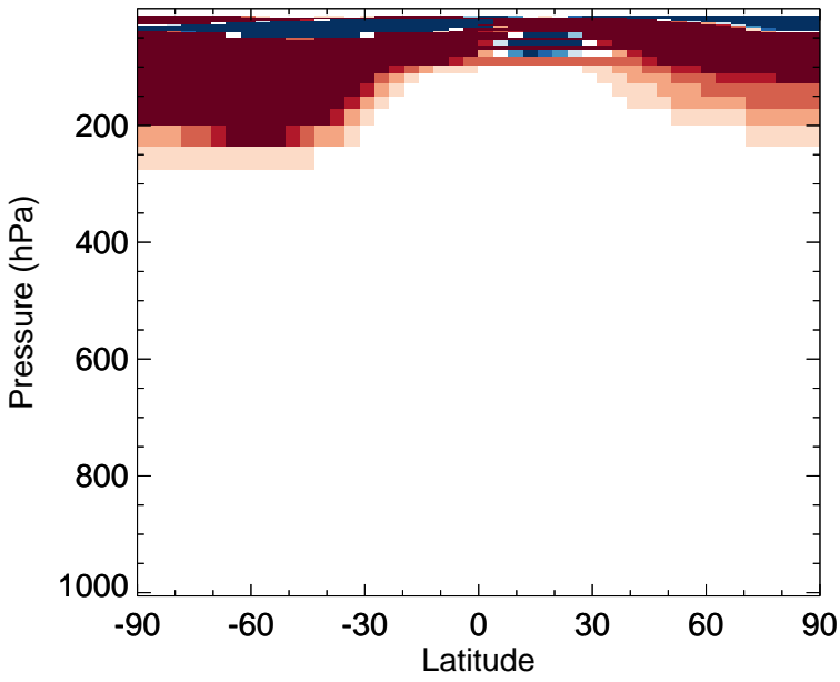
v11-02e-Run0 - v11-02d-Run1 O3 - Zonal mean abs diff for Oct
