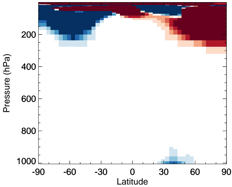
v11-02e-Run0 - v11-02d-Run1 N2O5 - Zonal mean abs diff for Oct
