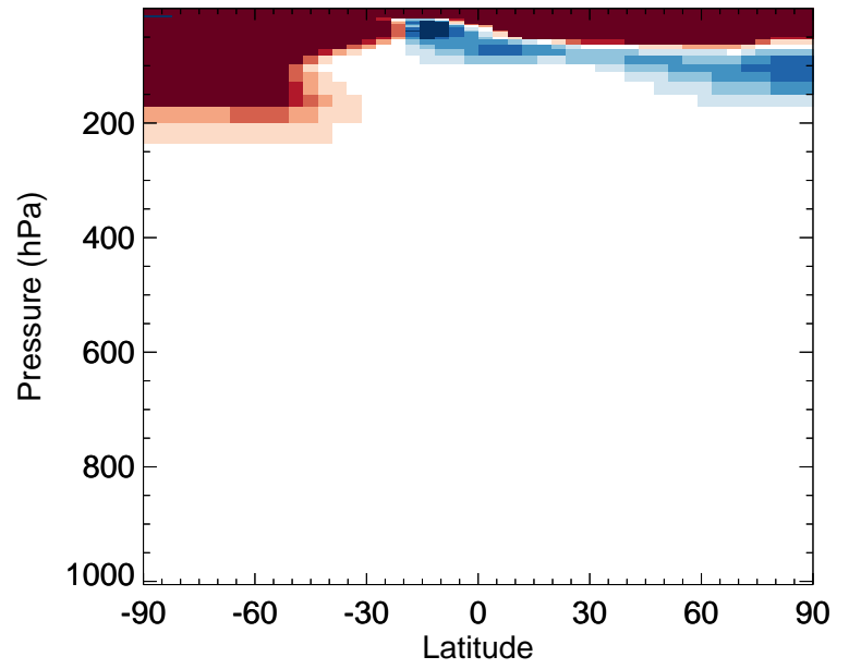
v11-02e-Run0 / v11-02d-Run1 C2H6 - Zonal mean % diff for Oct
