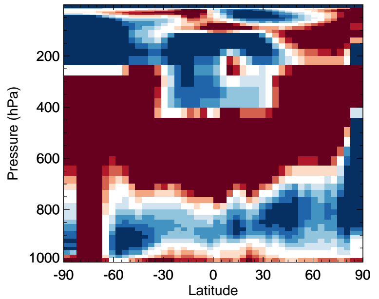
v11-02e-Run0 / v11-02d-Run1 Cl - Zonal mean % diff for Oct
