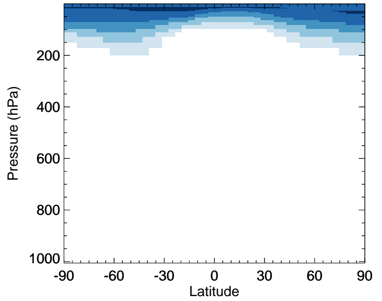
v11-02e-Run0 / v11-02d-Run1 MSA - Zonal mean % diff for Oct
