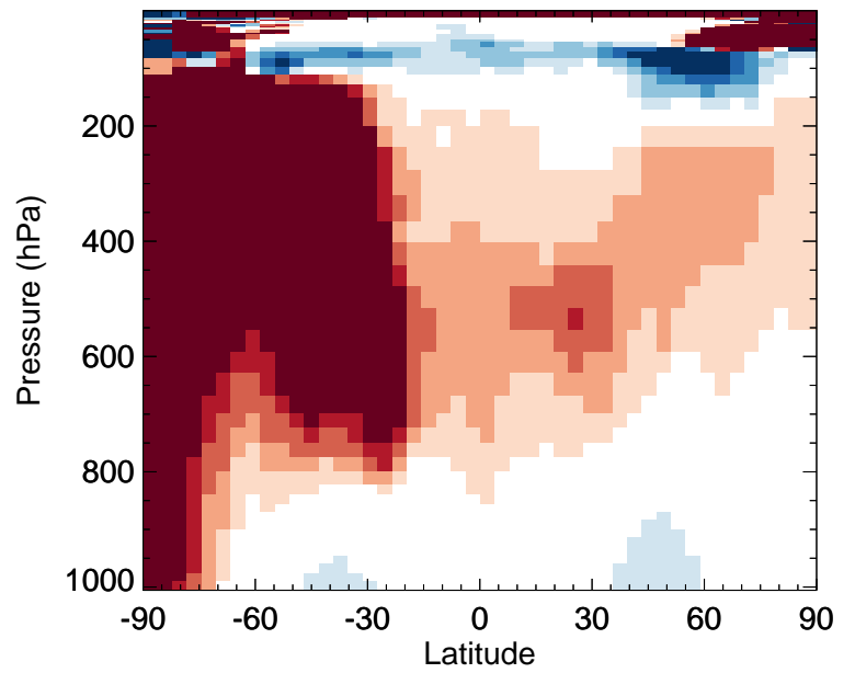
v11-02e-Run0 / v11-02d-Run1 RIPA - Zonal mean % diff for Oct
