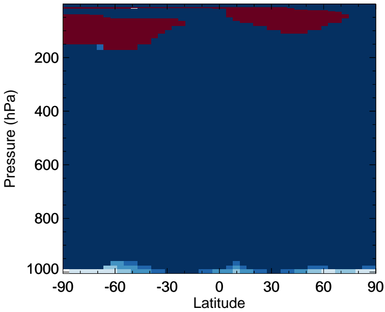
v11-02e-Run0 - v11-02d-Run1 N2O - Zonal mean abs diff for Oct
