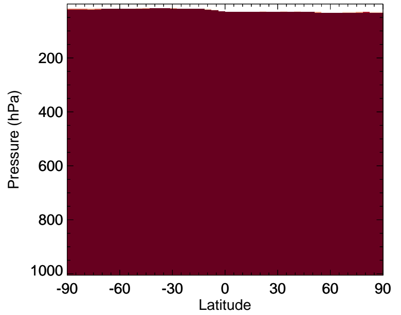
v11-02e-Run0 / v11-02d-Run1 DST4 - Zonal mean % diff for Oct
