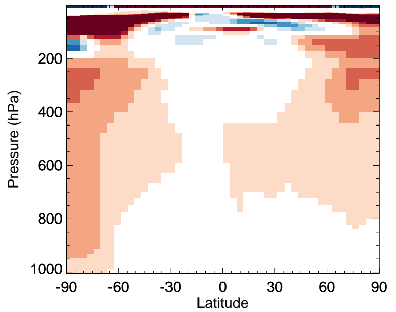
v11-02e-Run0 / v11-02d-Run1 ALD2 - Zonal mean % diff for Oct
