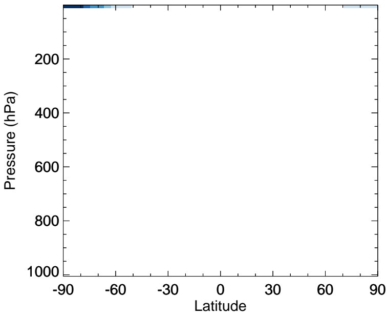
v11-02e-Run0 - v11-02d-Run1 ACTA - Zonal mean abs diff for Oct
