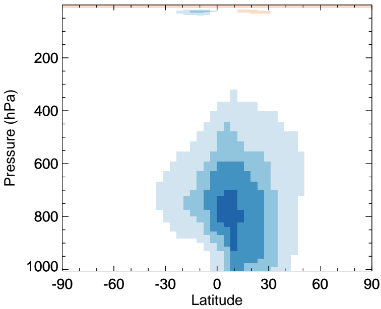
v11-02e-Run0 - v11-02d-Run1 H2O2 - Zonal mean abs diff for Oct
