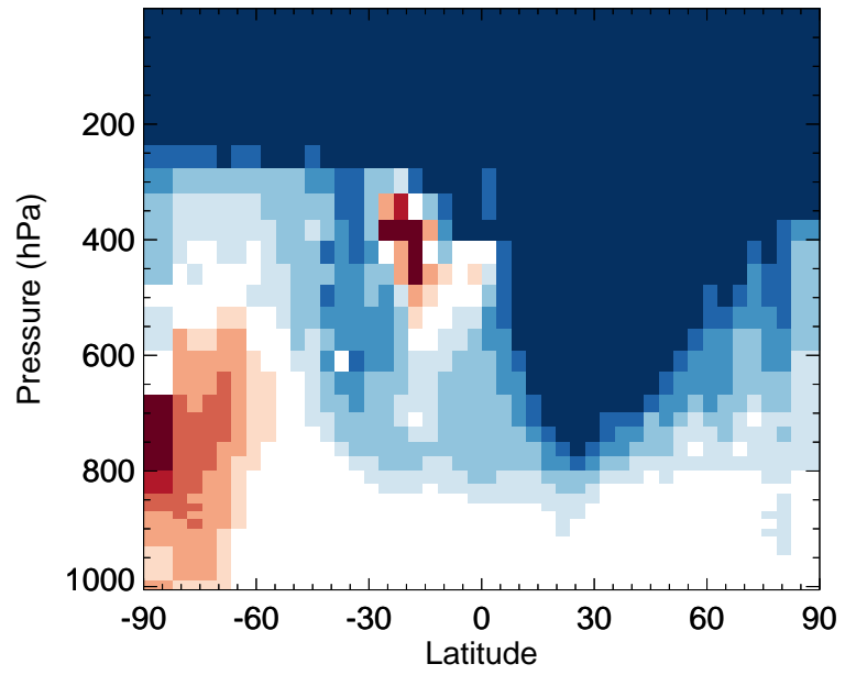
v11-02e-Run0 / v11-02d-Run1 NH3 - Zonal mean % diff for Oct
