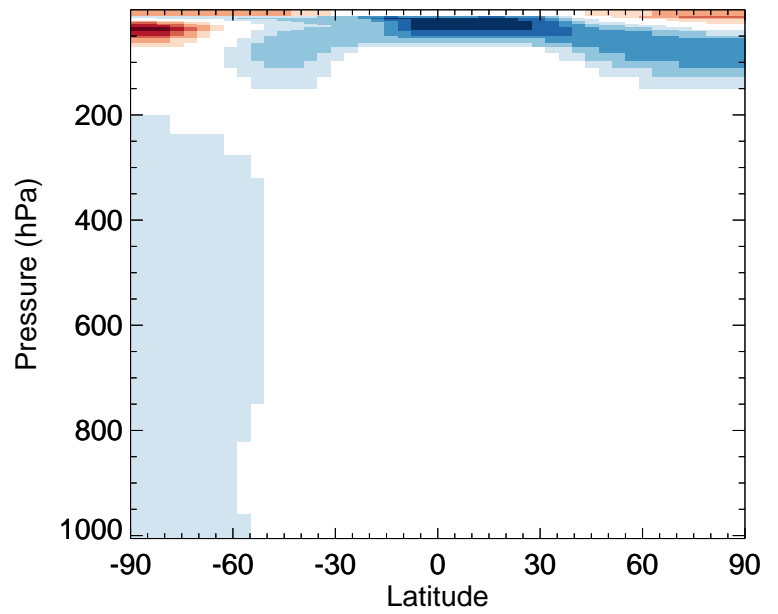
v11-02e-Run0 / v11-02d-Run1 ASOA3 - Zonal mean % diff for Oct
