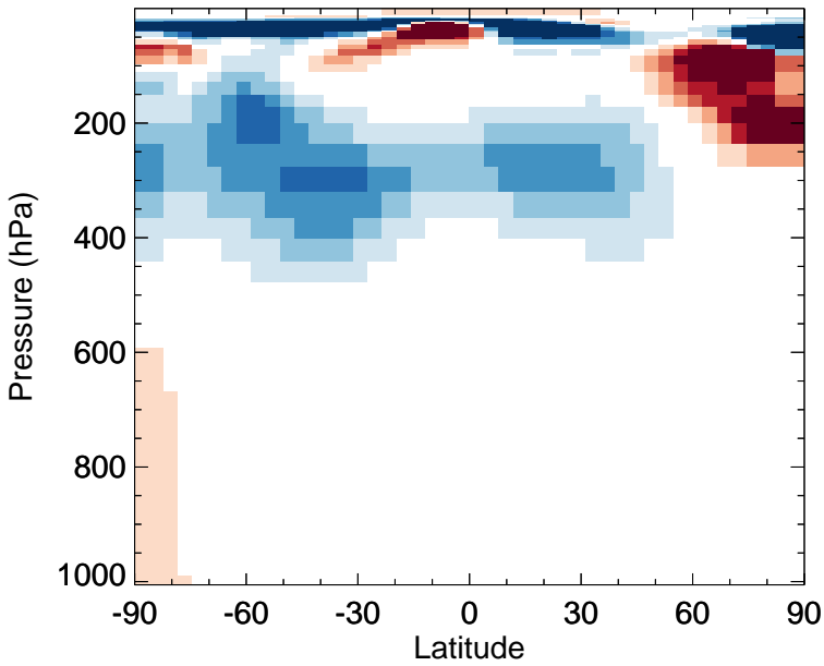
v11-02e-Run0 - v11-02c-Run0 HNO 4 - Zonal mean abs diff for Oct
