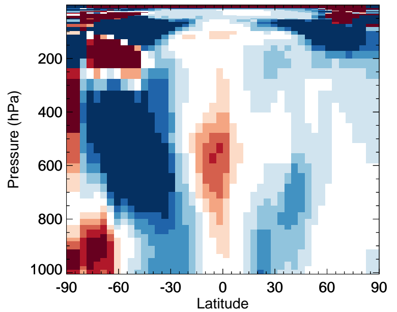
v11-02e-Run0 / v11-02c-Run0 ISOP - Zonal mean % diff for Oct
