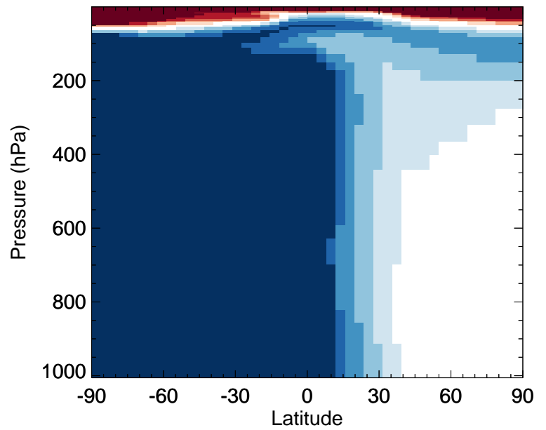
v11-02e-Run0 / v11-02c-Run0 SOAGX - Zonal mean % diff for Oct
