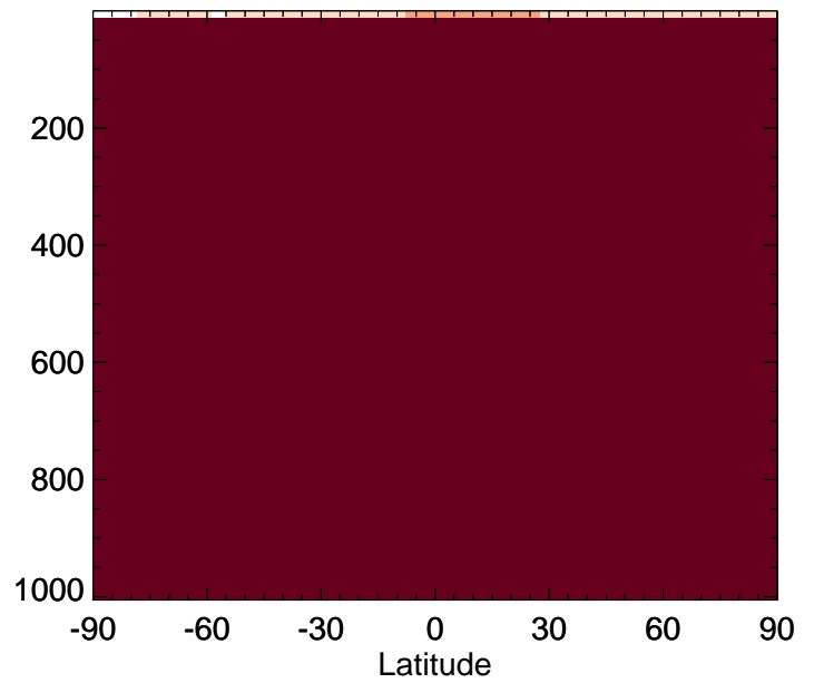
v11-02e-Run0 / v11-02c-Run0 DST1 - Zonal mean % diff for Oct
