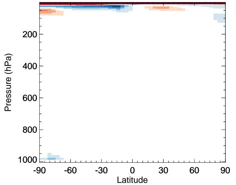
v11-02e-Run0 / v11-02c-Run0 CH4 - Zonal mean % diff for Oct
