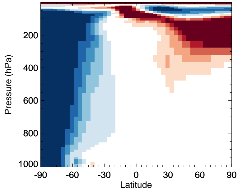
v11-02e-Run0 / v11-02c-Run0 HNO 3 - Zonal mean % diff for Oct
