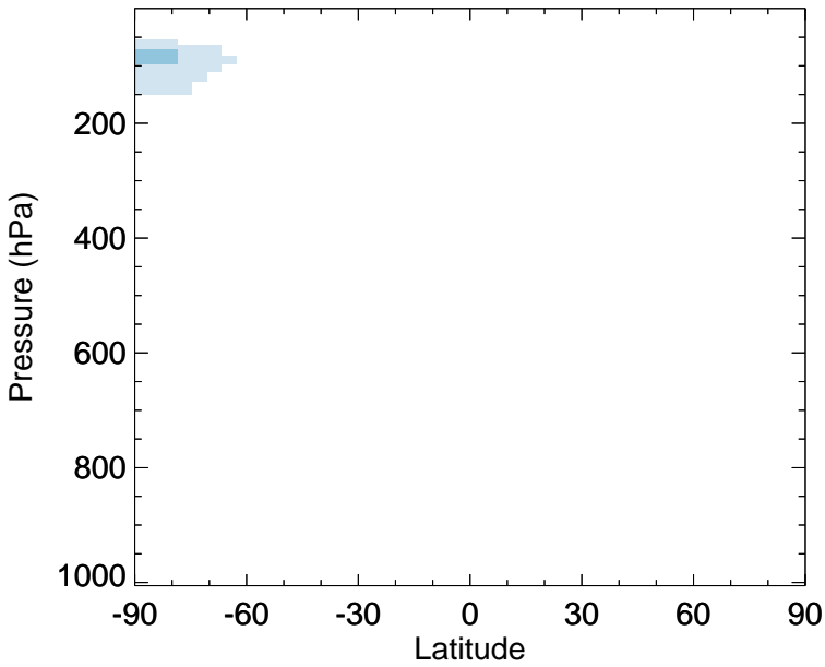
v11-02e-Run0 - v11-02c-Run0 HBr - Zonal mean abs diff for Oct
