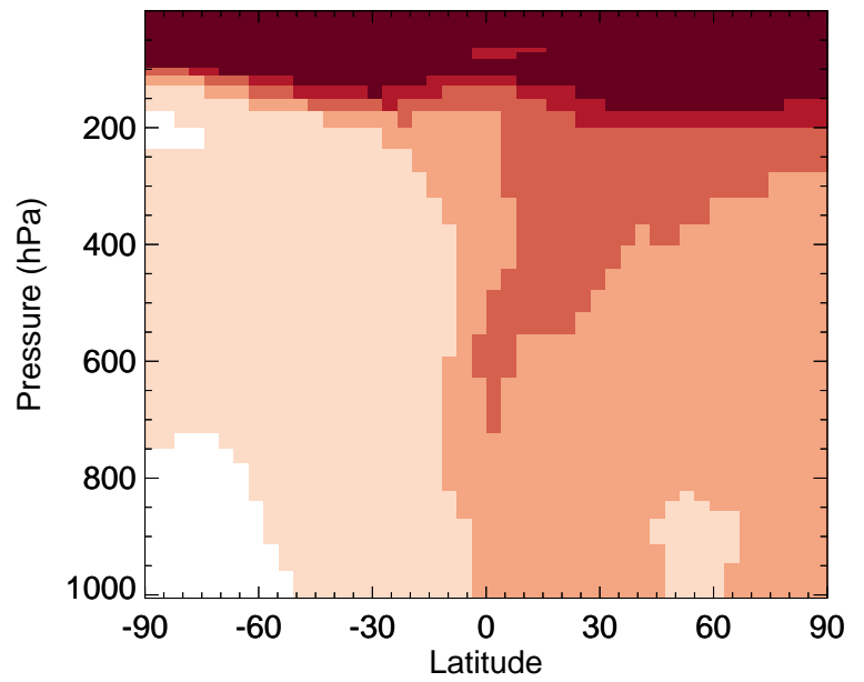
v11-02e-Run0 / v11-02d-Run1 INDIOL - Zonal mean % diff for Oct
