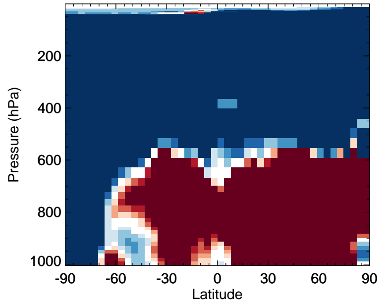
v11-02e-Run0 / v11-02d-Run1 HBr - Zonal mean % diff for Oct
