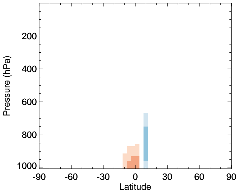
v11-02e-Run0 - v11-02c-Run0 ISOP - Zonal mean abs diff for Oct
