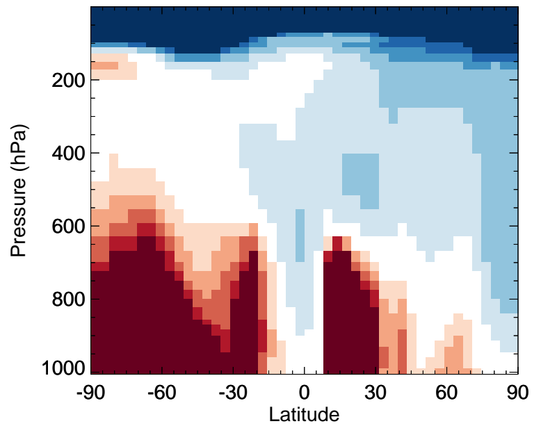
v11-02e-Run0 / v11-02c-Run0 R4N2 - Zonal mean % diff for Oct
