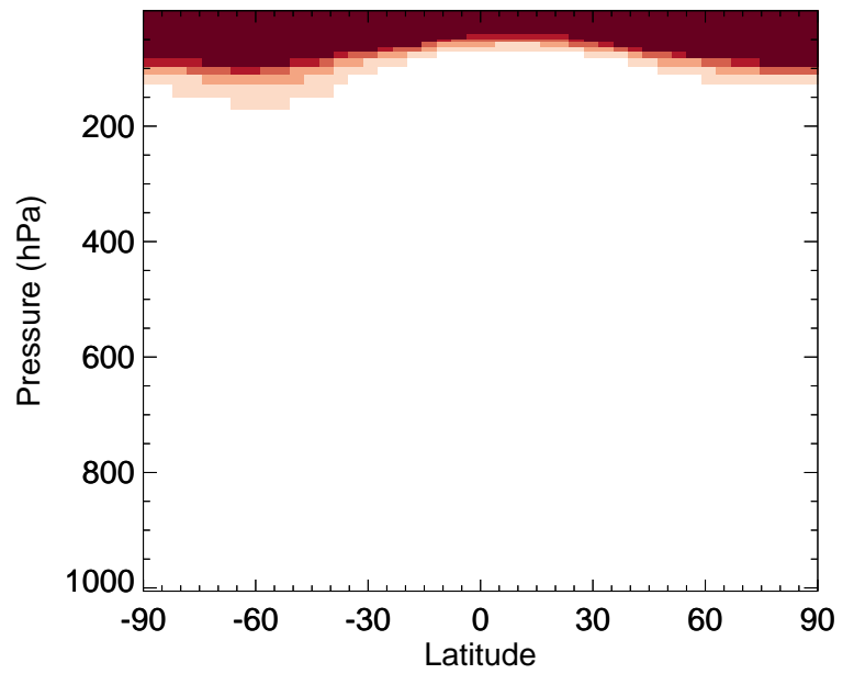
v11-02e-Run0 / v11-02d-Run1 SOAS - Zonal mean % diff for Oct
