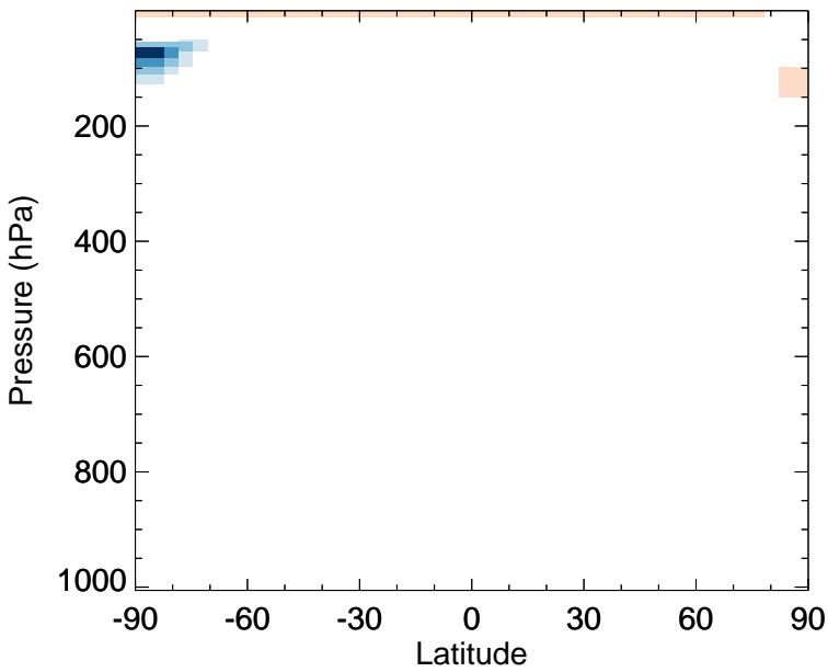
v11-02e-Run0 - v11-02c-Run0 HOCl - Zonal mean abs diff for Oct
