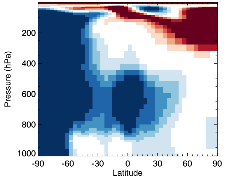
v11-02e-Run0 / v11-02d-Run1 N2O5 - Zonal mean % diff for Oct
