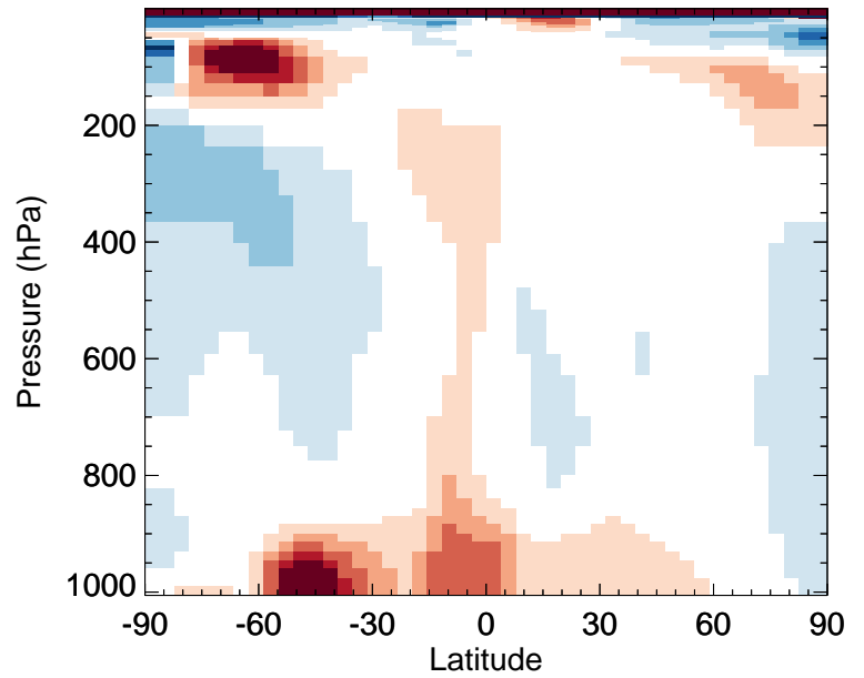
v11-02e-Run0 / v11-02c-Run0 GLYX - Zonal mean % diff for Oct
