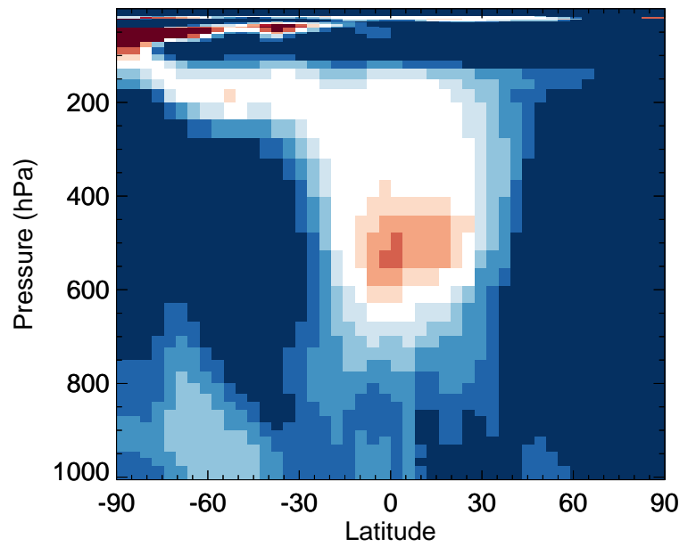
v11-02e-Run0 / v11-02d-Run1 IEPOXB - Zonal mean % diff for Oct
