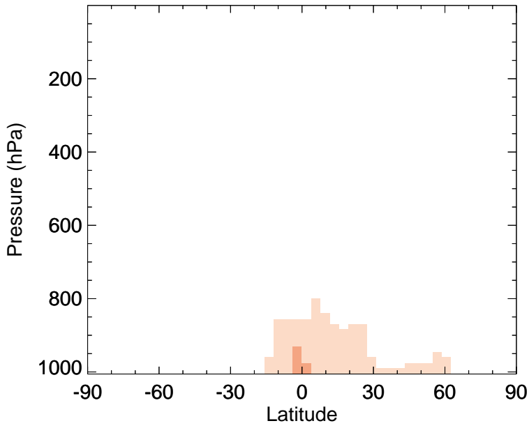
v11-02e-Run0 - v11-02d-Run1 MEK - Zonal mean abs diff for Oct
