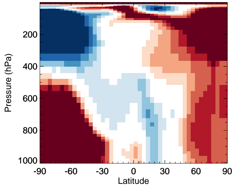
v11-02e-Run0 / v11-02c-Run0 HNO 2 - Zonal mean % diff for Oct
