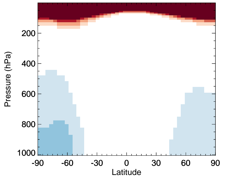
v11-02e-Run0 / v11-02c-Run0 ASOAN - Zonal mean % diff for Oct
