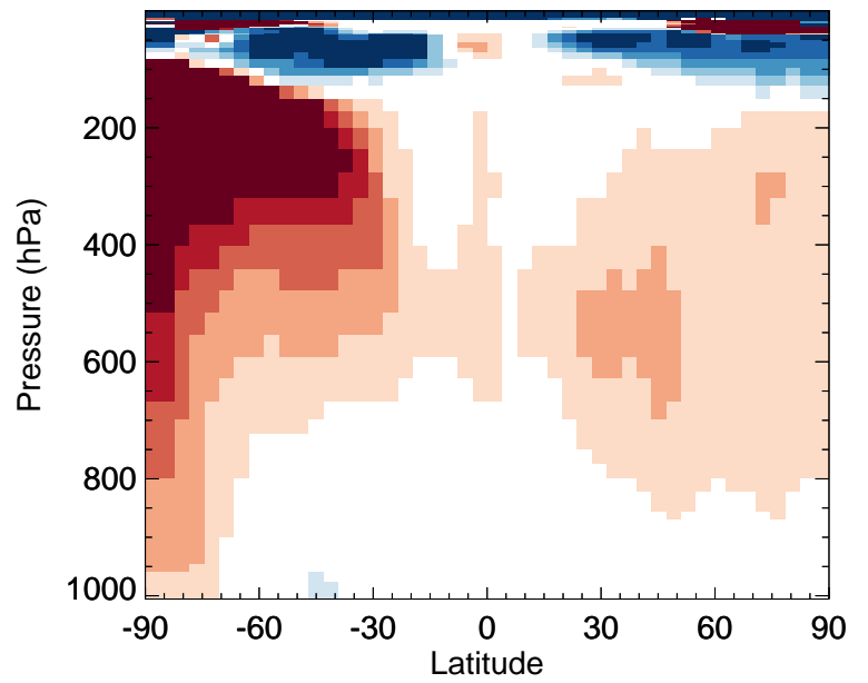
v11-02e-Run0 / v11-02d-Run1 XYLE - Zonal mean % diff for Oct
