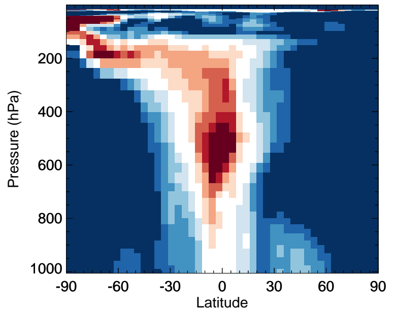
v11-02e-Run0 / v11-02c-Run0 IEPOXB - Zonal mean % diff for Oct
