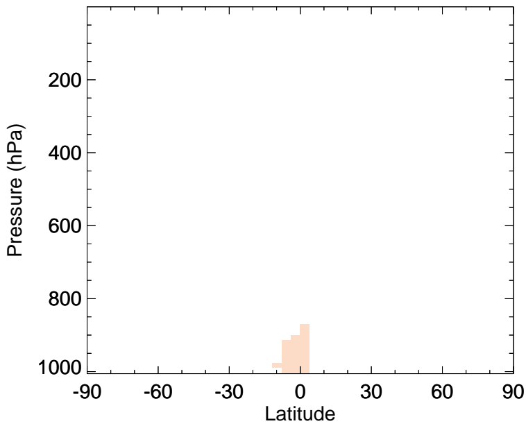
v11-02e-Run0 - v11-02d-Run1 ISOP - Zonal mean abs diff for Oct
