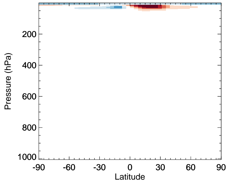
v11-02e-Run0 / v11-02d-Run1 CH 2 Br 2 - Zonal mean % diff for Oct
