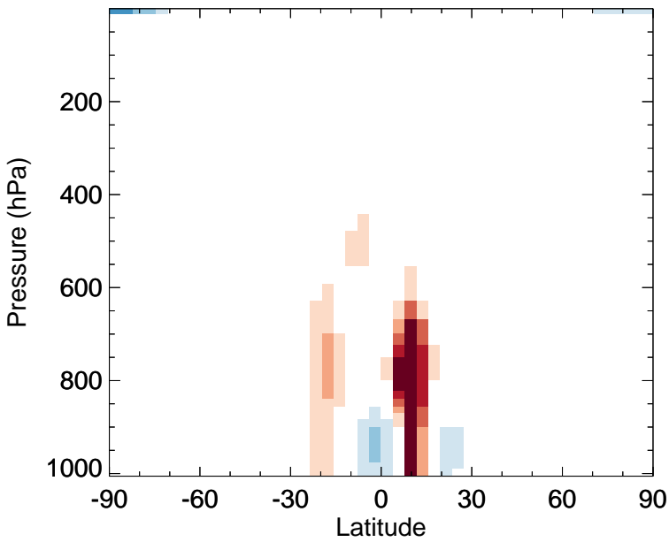
v11-02e-Run0 - v11-02c-Run0 MAP - Zonal mean abs diff for Oct
