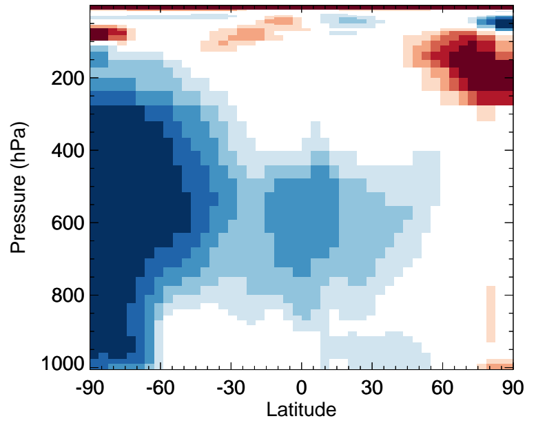
v11-02e-Run0 / v11-02d-Run1 HNO 4 - Zonal mean % diff for Oct
