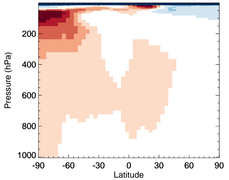
v11-02e-Run0 / v11-02d-Run1 BENZ - Zonal mean % diff for Oct
