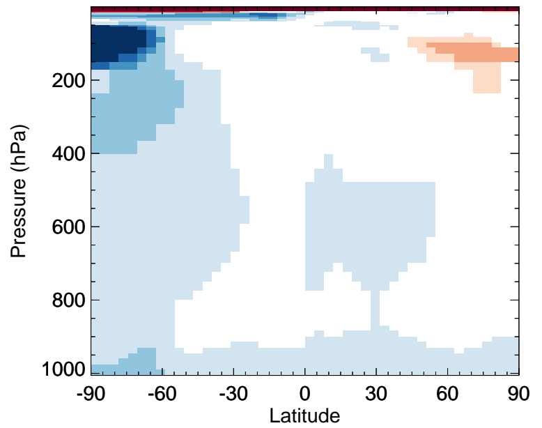
v11-02e-Run0 / v11-02d-Run1 CH 2 O - Zonal mean % diff for Oct
