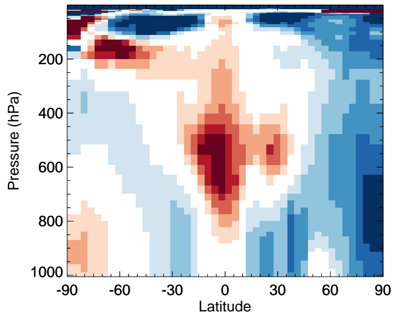
v11-02e-Run0 / v11-02c-Run0 DMS - Zonal mean % diff for Oct
