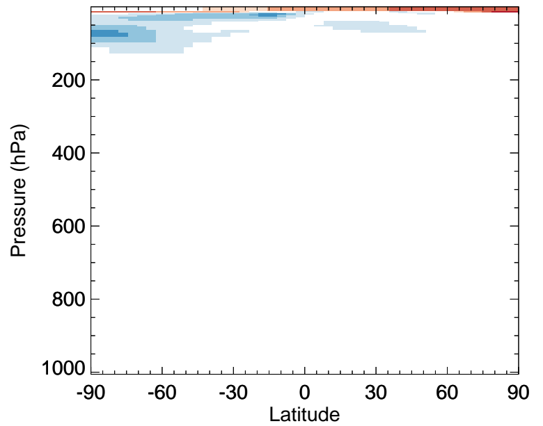
v11-02e-Run0 / v11-02c-Run0 CO - Zonal mean % diff for Oct
