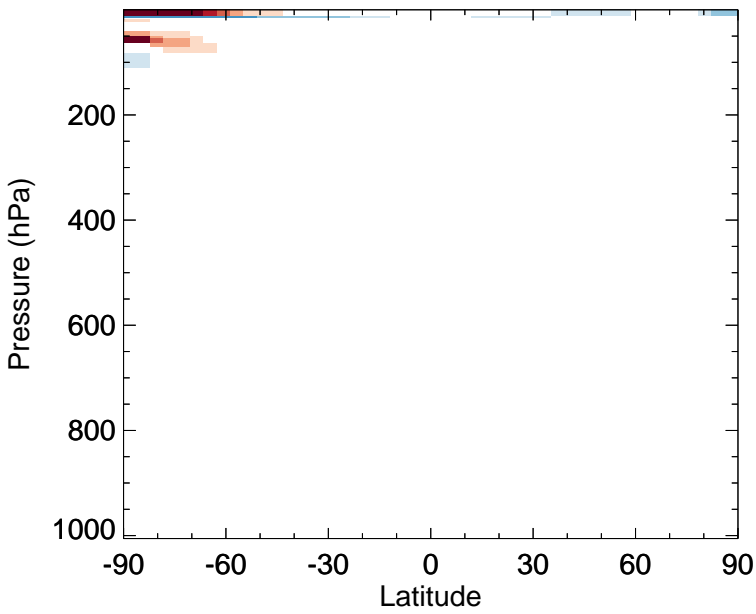
v11-02e-Run0 - v11-02d-Run1 ClO - Zonal mean abs diff for Oct
