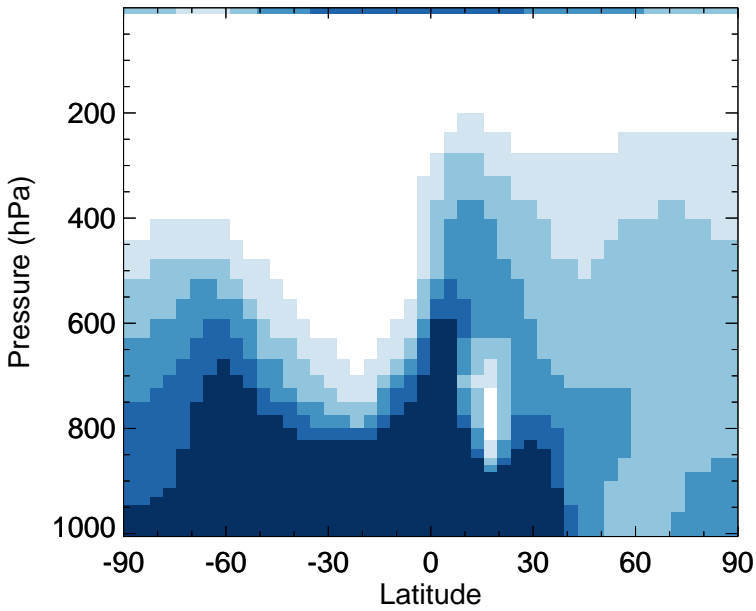
v11-02e-Run0 - v11-02c-Run0 MP - Zonal mean abs diff for Oct
