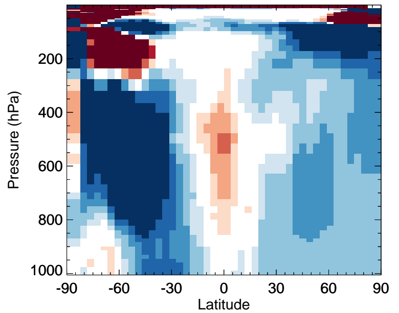
v11-02e-Run0 / v11-02c-Run0 RIPB - Zonal mean % diff for Oct
