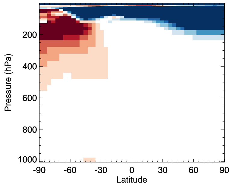
v11-02e-Run0 / v11-02d-Run1 MAP - Zonal mean % diff for Oct
