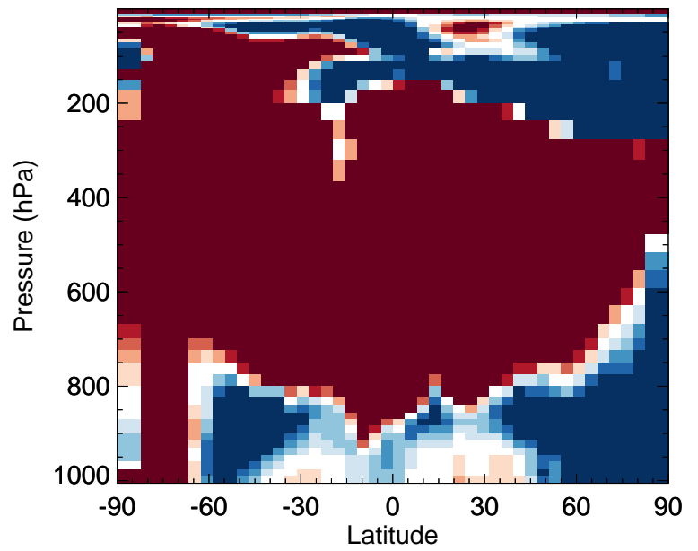
v11-02e-Run0 / v11-02d-Run1 OCIO - Zonal mean % diff for Oct
