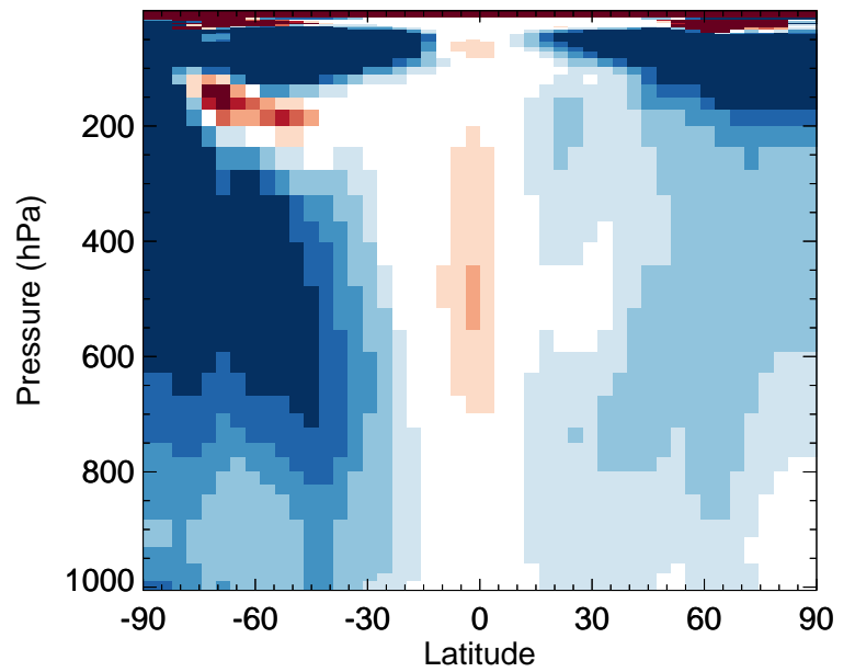
v11-02e-Run0 / v11-02c-Run0 XYLE - Zonal mean % diff for Oct
