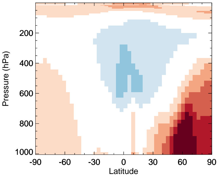
v11-02e-Run0 - v11-02c-Run0 PPN - Zonal mean abs diff for Oct
