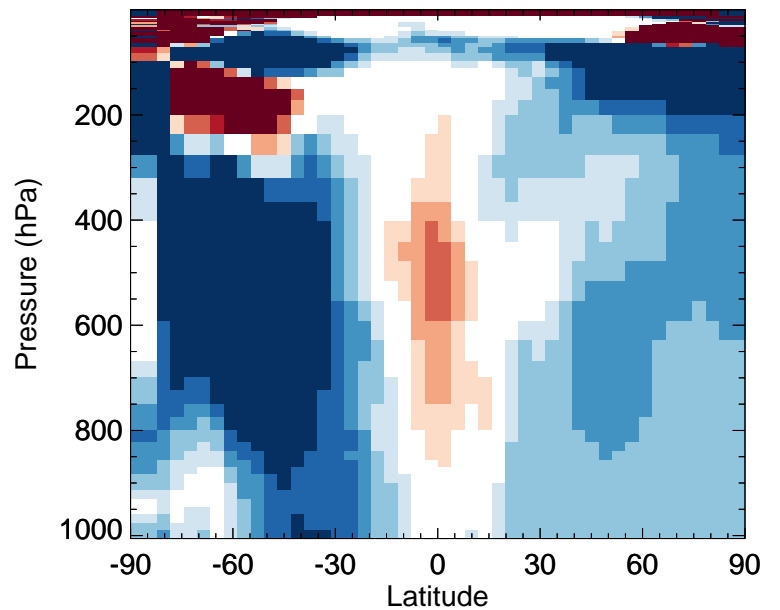
v11-02e-Run0 / v11-02c-Run0 RIPA - Zonal mean % diff for Oct
