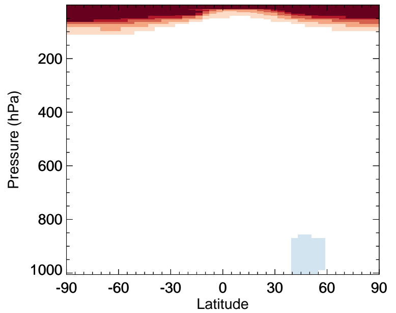
v11-02e-Run0 / v11-02d-Run1 ASOAN - Zonal mean % diff for Oct
