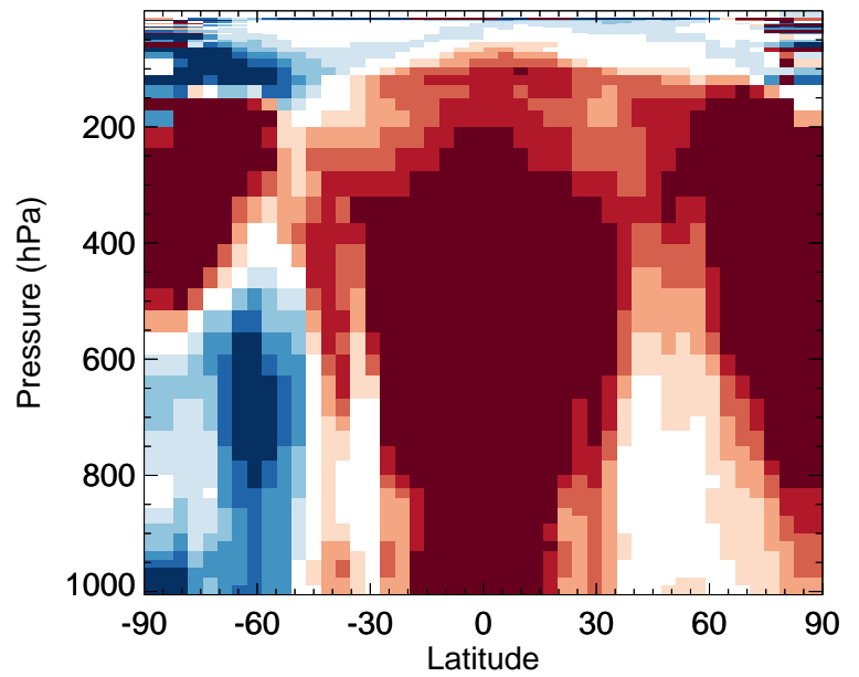
v11-02e-Run0 / v11-02c-Run0 LIMO - Zonal mean % diff for Oct
