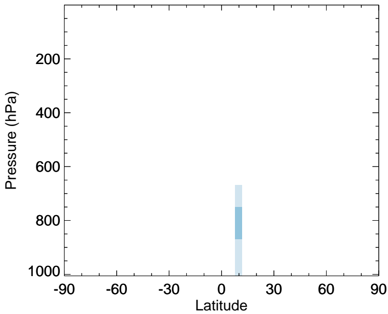
v11-02e-Run0 - v11-02c-Run0 MVK - Zonal mean abs diff for Oct
