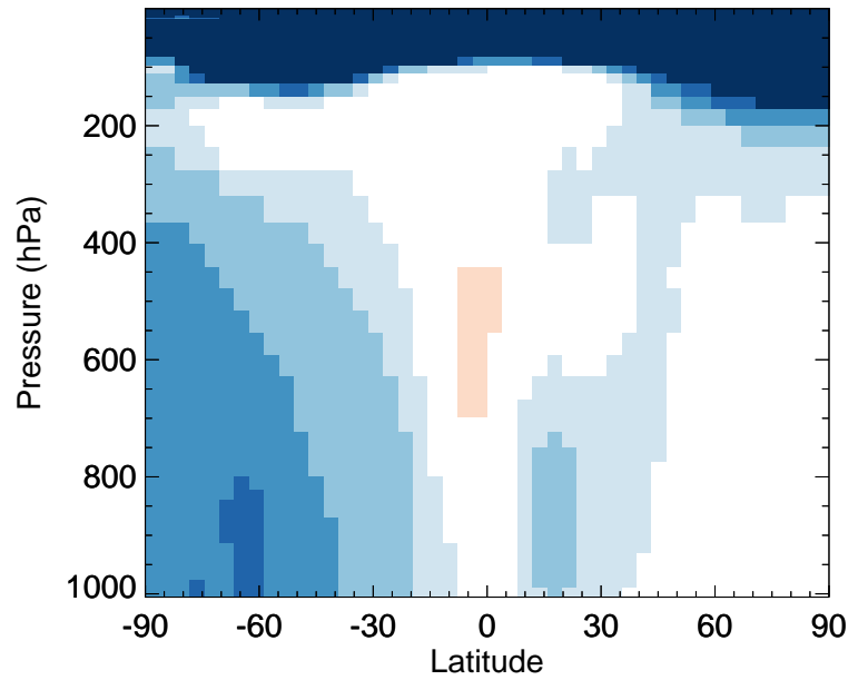
v11-02e-Run0 / v11-02c-Run0 EOH - Zonal mean % diff for Oct
