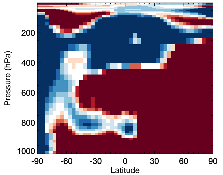
v11-02e-Run0 / v11-02c-Run0 ClO - Zonal mean % diff for Oct
