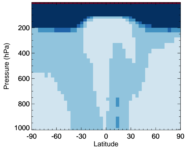
v11-02e-Run0 / v11-02c-Run0 C3H8 - Zonal mean % diff for Oct
