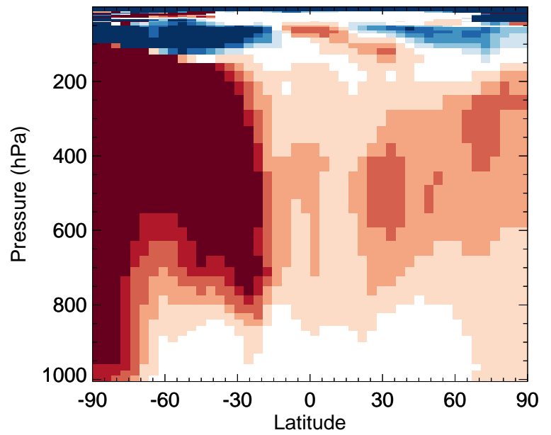
v11-02e-Run0 / v11-02d-Run1 HPALD - Zonal mean % diff for Oct
