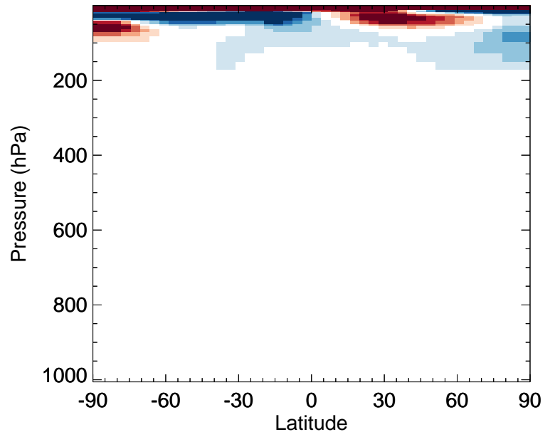
v11-02e-Run0 / v11-02d-Run1 CH3Cl - Zonal mean % diff for Oct
