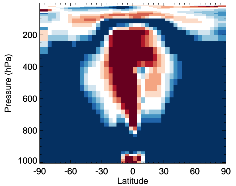
v11-02e-Run0 / v11-02c-Run0 HOBr - Zonal mean % diff for Oct
