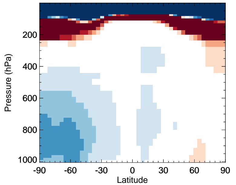
v11-02e-Run0 / v11-02c-Run0 RCHO - Zonal mean % diff for Oct
