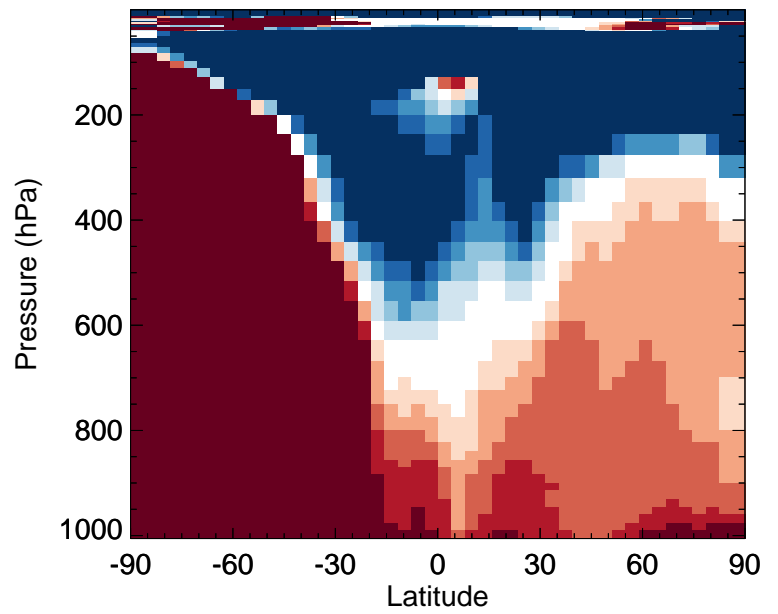
v11-02e-Run0 / v11-02d-Run1 LVOC - Zonal mean % diff for Oct
