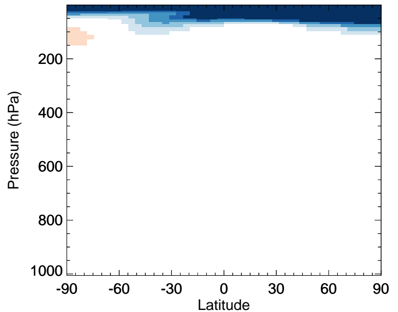
v11-02e-Run0 / v11-02c-Run0 ACET - Zonal mean % diff for Oct
