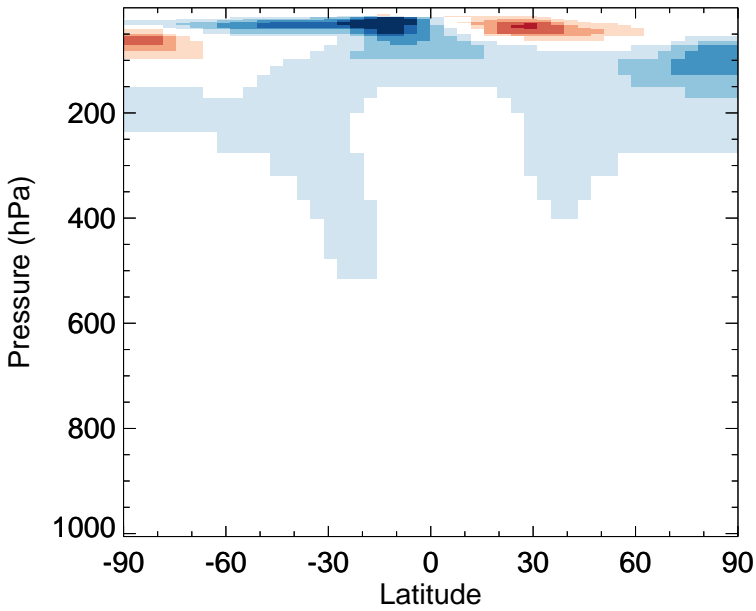
v11-02e-Run0 - v11-02c-Run0 CH3Cl - Zonal mean abs diff for Oct
