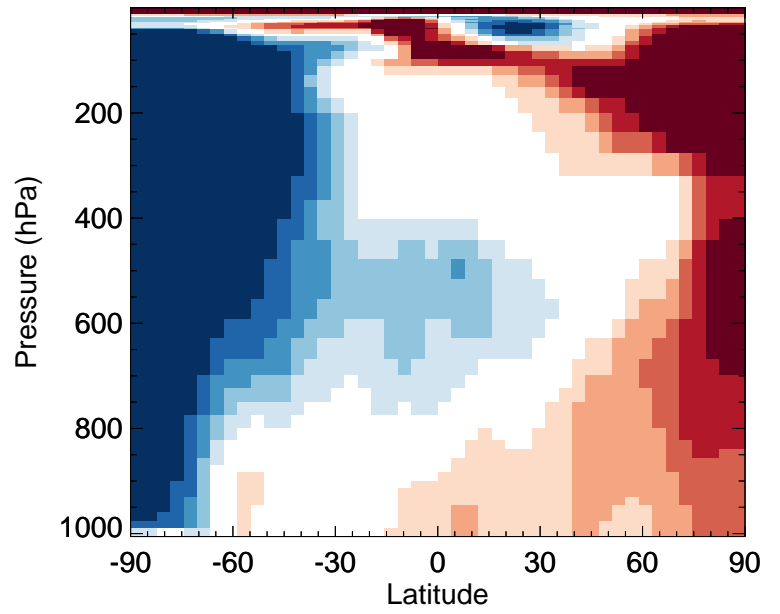
v11-02e-Run0 / v11-02d-Run1 HNO 2 - Zonal mean % diff for Oct
