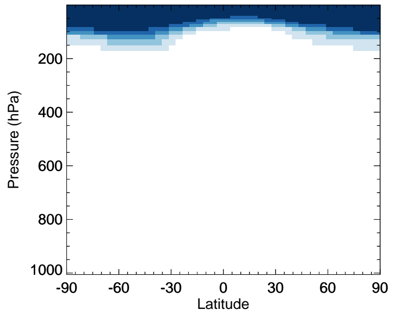
v11-02e-Run0 / v11-02d-Run1 BCPI - Zonal mean % diff for Oct
