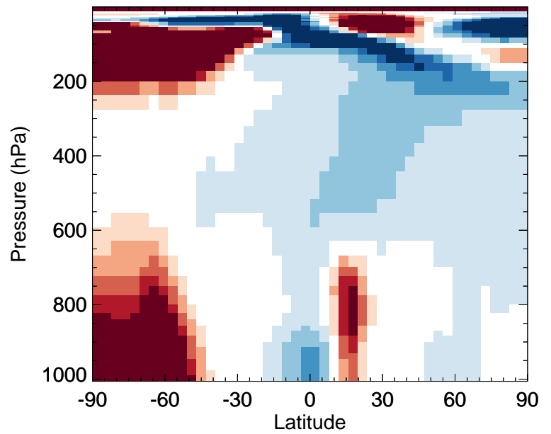
v11-02e-Run0 / v11-02c-Run0 H2O2 - Zonal mean % diff for Oct
