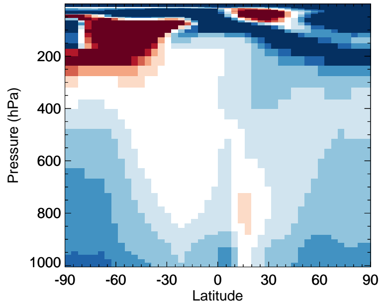
v11-02e-Run0 / v11-02c-Run0 MP - Zonal mean % diff for Oct
