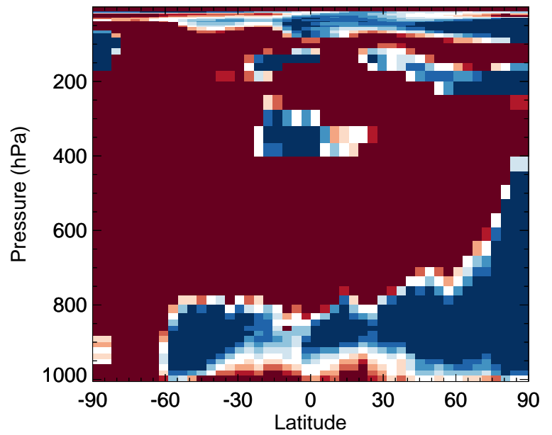
v11-02e-Run0 / v11-02d-Run1 Cl2O2 - Zonal mean % diff for Oct
