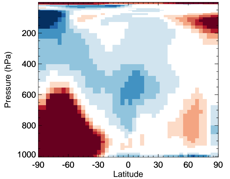
v11-02e-Run0 / v11-02c-Run0 MPN - Zonal mean % diff for Oct
