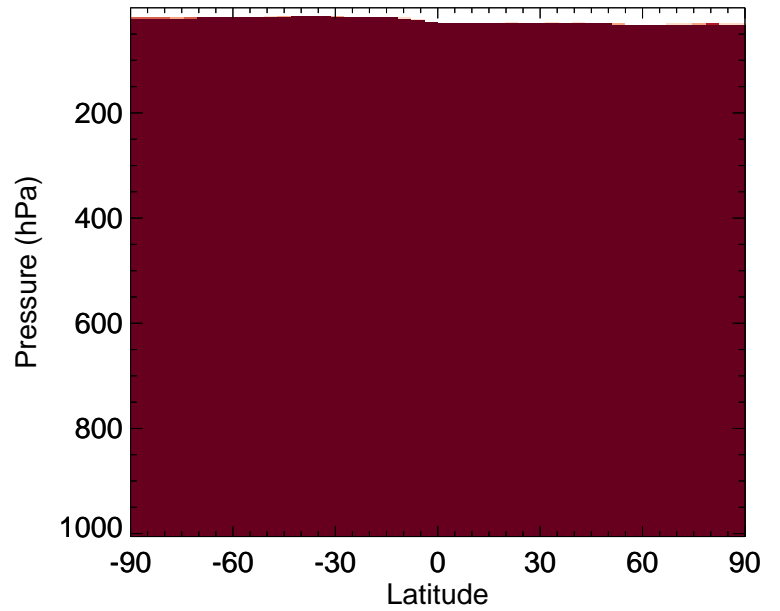
v11-02e-Run0 / v11-02c-Run0 DST4 - Zonal mean % diff for Oct
