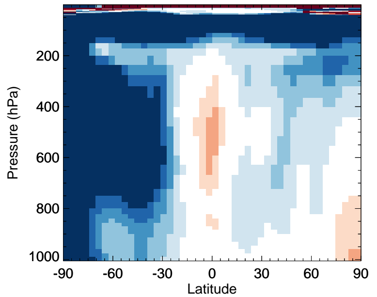
v11-02e-Run0 / v11-02c-Run0 PRPE - Zonal mean % diff for Oct
