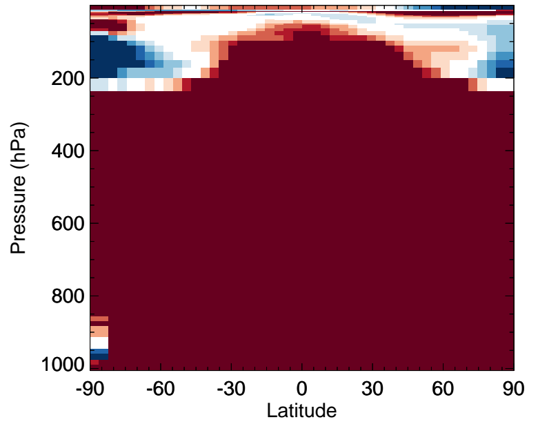
v11-02e-Run0 / v11-02c-Run0 BrCl - Zonal mean % diff for Oct
