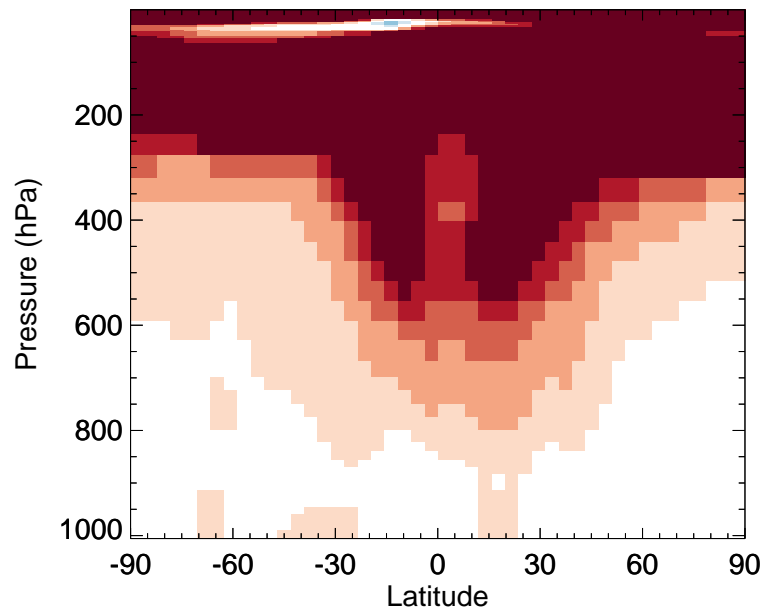
v11-02e-Run0 / v11-02c-Run0 SO4 - Zonal mean % diff for Oct
