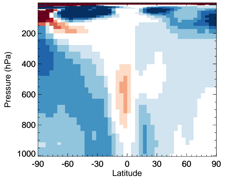
v11-02e-Run0 / v11-02c-Run0 TOLU - Zonal mean % diff for Oct
