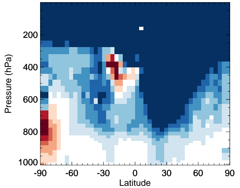
v11-02e-Run0 / v11-02c-Run0 NH3 - Zonal mean % diff for Oct
