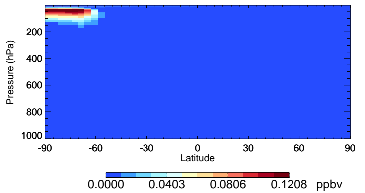
v11-02e-Run0 OCIO - Species Curtain @ -180.000 for Jul
