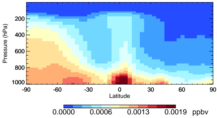
v11-02c-Run0 CHBr3 - Species Zonal Mean for Jul
