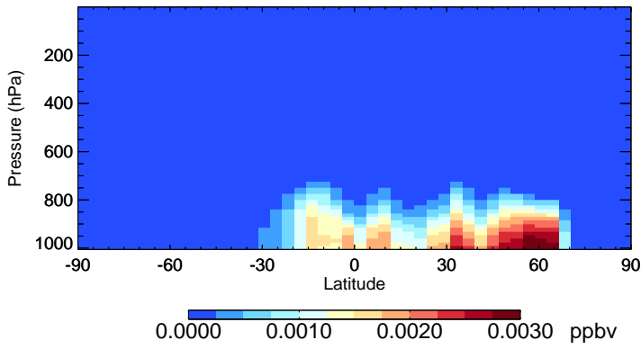
v11-02c-Run0 ISOPNB - Species Zonal Mean for Jul
