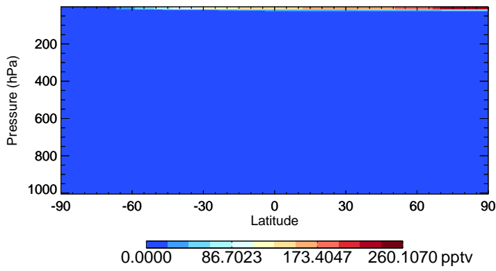
v11-02d-Run1 HO2 - Species Zonal Mean for Jul
