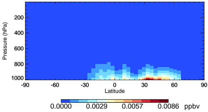
v11-02d-Run1 ISN1 - Species Zonal Mean for Jul
