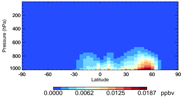
v11-02d-Run1 MONITA - Species Zonal Mean for Jul
