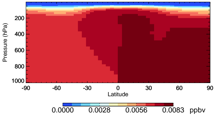
v11-02d-Run1 CH3Br - Species Zonal Mean for Jul
