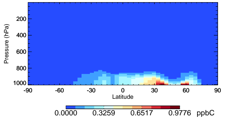
v11-02c-Run0 ALD2 - Species Curtain @ -180.000 for Jul
