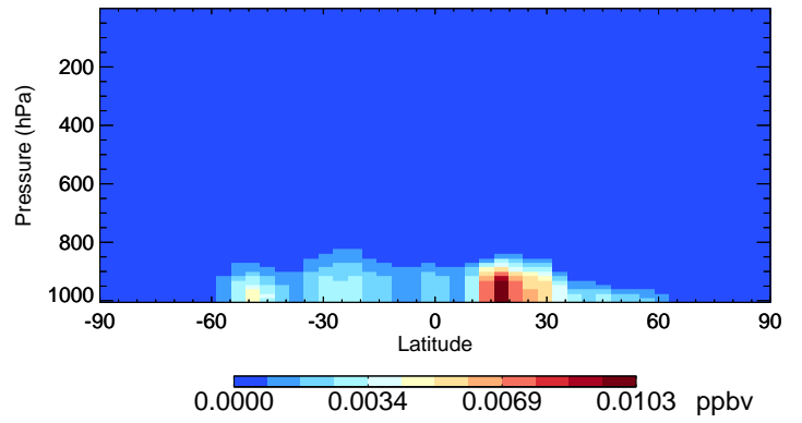
v11-02c-Run0 NITs - Species Curtain @ -180.000 for Jul
