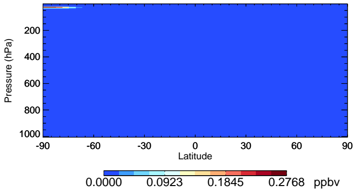
v11-02c-Run0 ClNO2 - Species Zonal Mean for Jul
