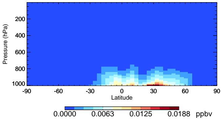
v11-02c-Run0 GLYX - Species Zonal Mean for Jul
