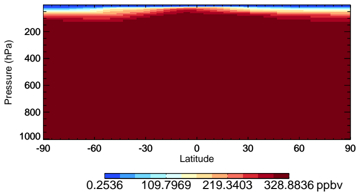
v11-02d-Run1 N2O - Species Zonal Mean for Jul
