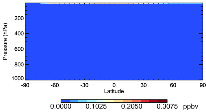
v11-02c-Run0 CI - Species Zonal Mean for Jul
