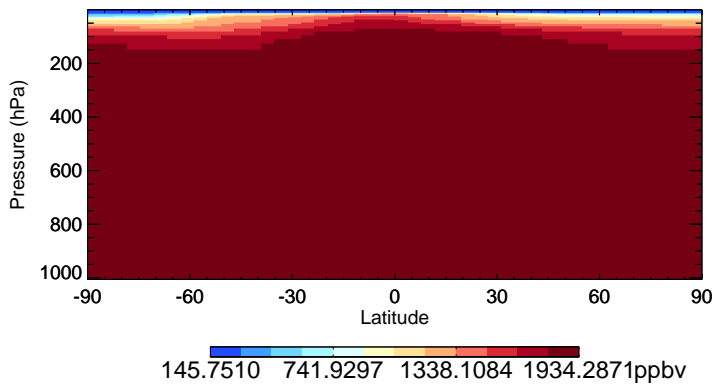
v11-02d-Run1 CH4 - Species Zonal Mean for Jul
