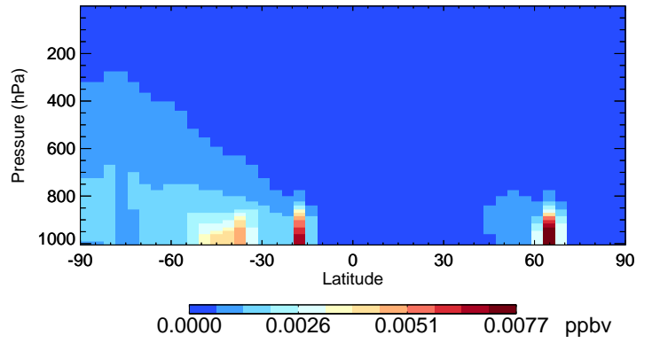
v11-02d-Run1 RCHO - Species Curtain @ -180.000 for Jul
