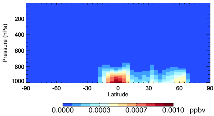
v11-02d-Run1 MOBA - Species Zonal Mean for Jul
