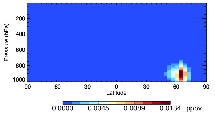
v11-02c-Run0 GLYC - Species Curtain @ -180.000 for Jul
