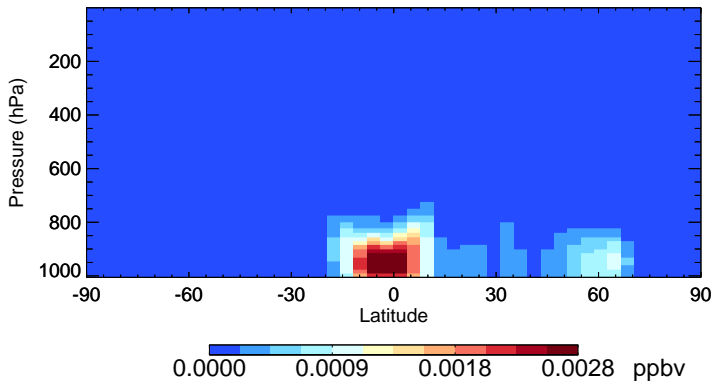
v11-02c-Run0 RIPD - Species Zonal Mean for Jul
