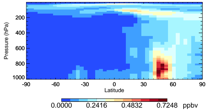
v11-02c-Run0 SO4 - Species Curtain @ -180.000 for Jul
