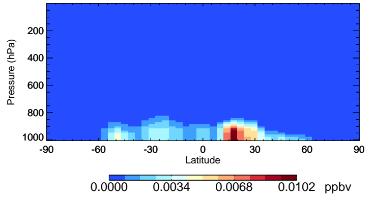
v11-02d-Run1 NITs - Species Curtain @ -180.000 for Jul
