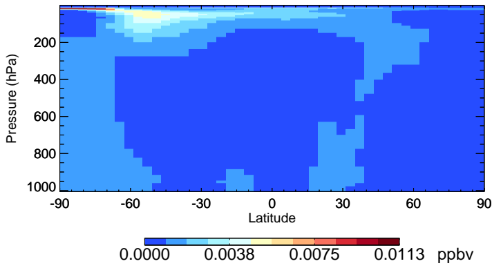
v11-02c-Run0 HOBr - Species Zonal Mean for Jul
