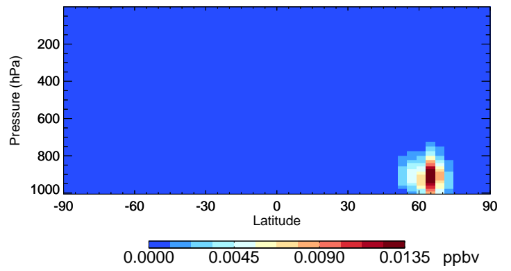
v11-02d-Run1 GLYC - Species Curtain @ -180.000 for Jul
