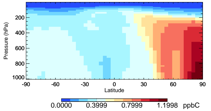
v11-02c-Run0 C2H6 - Species Curtain @ -180.000 for Jul
