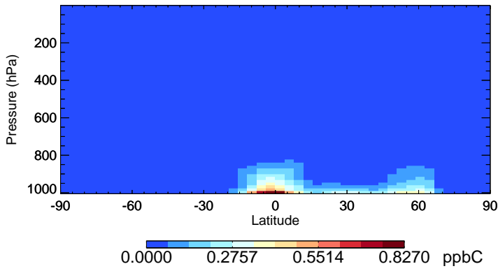
v11-02c-Run0 PRPE - Species Zonal Mean for Jul
