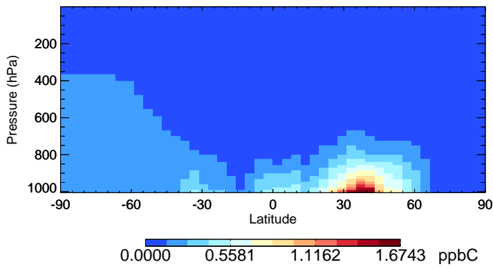
v11-02c-Run0 ALK4 - Species Zonal Mean for Jul
