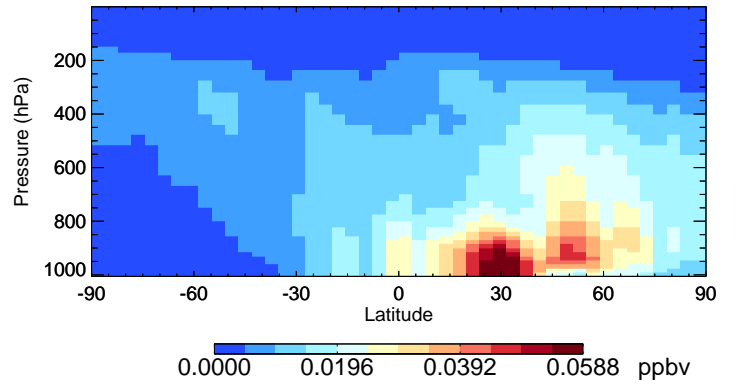
v11-02d-Run1 MAP - Species Curtain @ -180.000 for Jul
