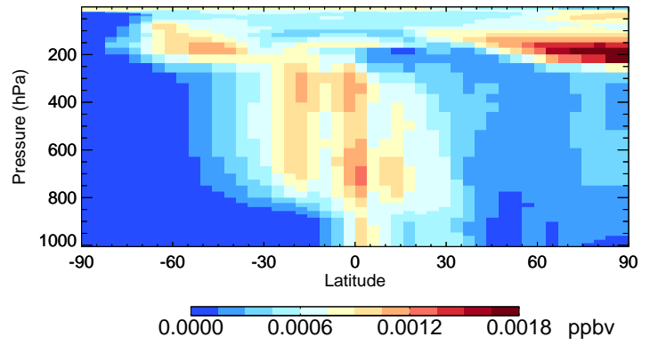
v11-02c-Run0 HBr - Species Curtain @ -180.000 for Jul
