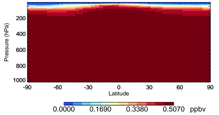
v11-02c-Run0 CFC12 - Species Curtain @ -180.000 for Jul
