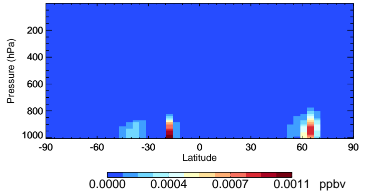
v11-02d-Run1 GLYX - Species Curtain @ -180.000 for Jul
