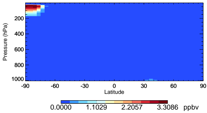
v11-02d-Run1 NIT - Species Zonal Mean for Jul
