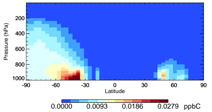
v11-02c-Run0 TOLU - Species Curtain @ -180.000 for Jul
