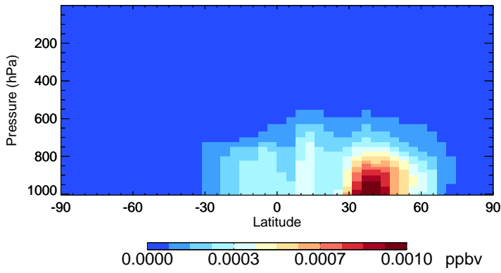
v11-02c-Run0 ISN10A - Species Zonal Mean for Jul
