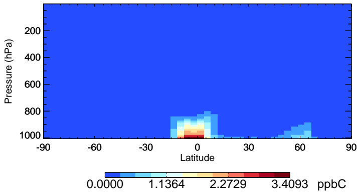
v11-02c-Run0 ISOP - Species Zonal Mean for Jul
