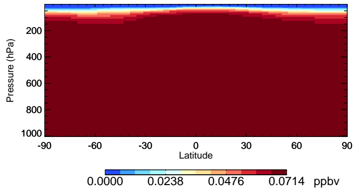
v11-02e-Run0 CFC113 - Species Curtain @ -180.000 for Jul
