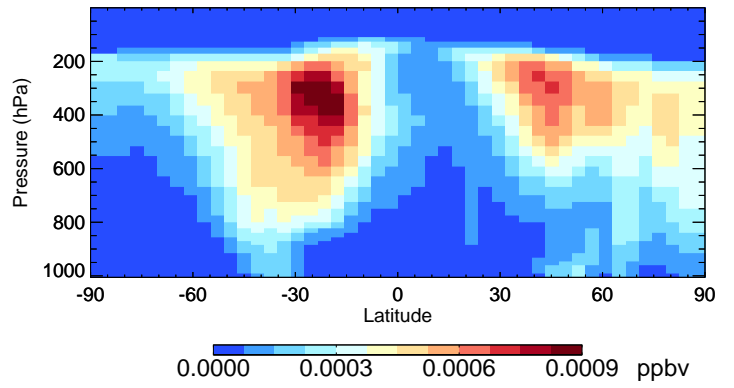
v11-02c-Run0 R4N2 - Species Curtain @ -180.000 for Jul
