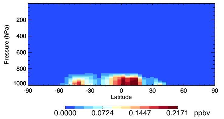
v11-02d-Run1 NH3 - Species Curtain @ -180.000 for Jul
