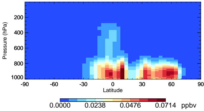
v11-02d-Run1 HAC - Species Zonal Mean for Jul
