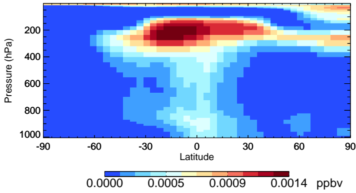
v11-02d-Run1 HBr - Species Zonal Mean for Jul
