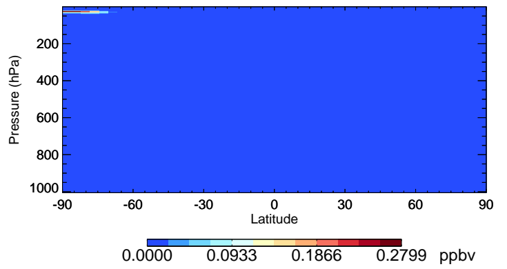
v11-02d-Run1 ClNO2 - Species Curtain @ -180.000 for Jul
