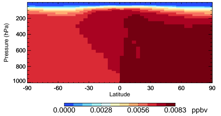
v11-02c-Run0 CH3Br - Species Curtain @ -180.000 for Jul
