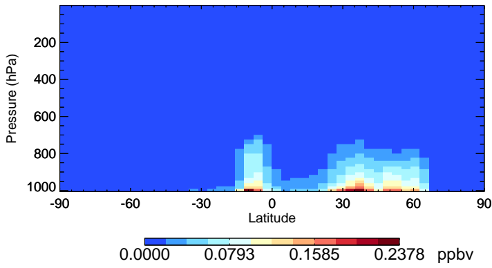
v11-02c-Run0 BCPO - Species Zonal Mean for Jul
