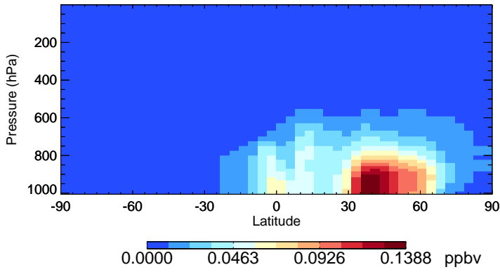
v11-02d-Run1 INDIOL - Species Zonal Mean for Jul
