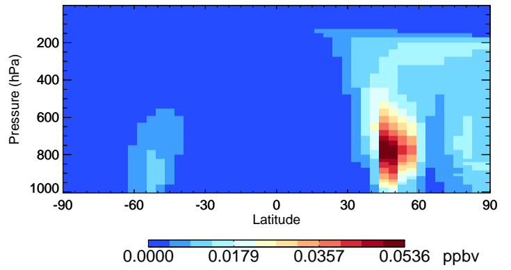
v11-02c-Run0 DST1 - Species Curtain @ -180.000 for Jul
