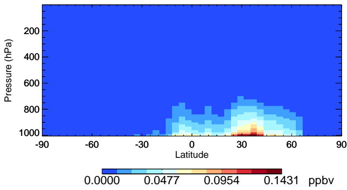
v11-02d-Run1 SOAP - Species Zonal Mean for Jul
