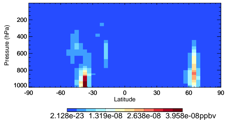
v11-02c-Run0 ISN1OG - Species Curtain @ -180.000 for Jul
