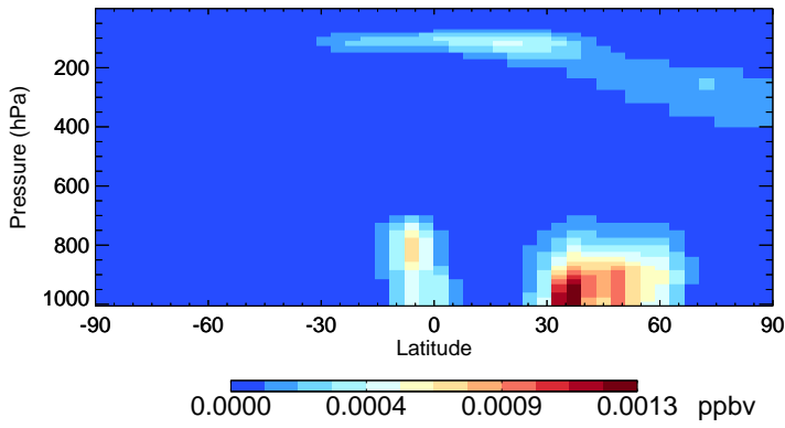
v11-02c-Run0 ASOA2 - Species Zonal Mean for Jul
