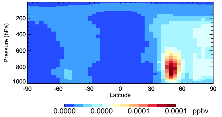
v11-02d-Run1 ISN10A - Species Curtain @ -180.000 for Jul
