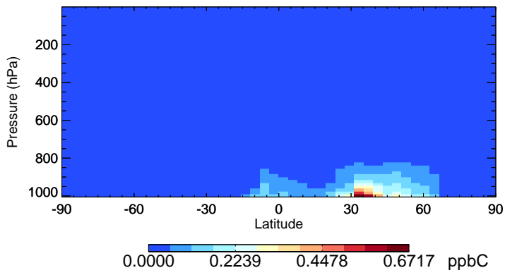
v11-02d-Run1 TOLU - Species Zonal Mean for Jul
