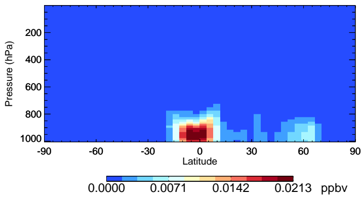
v11-02e-Run0 RIPB - Species Zonal Mean for Jul
