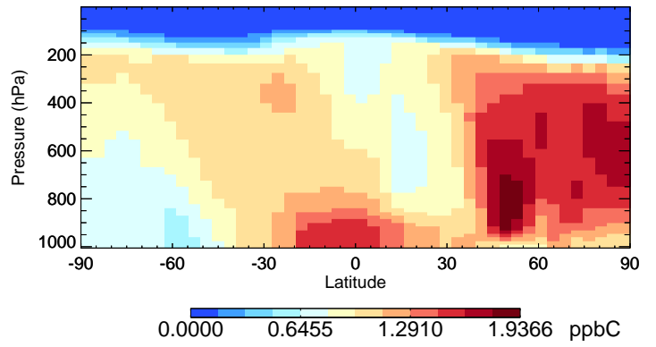
v11-02c-Run0 ACET - Species Curtain @ -180.000 for Jul
