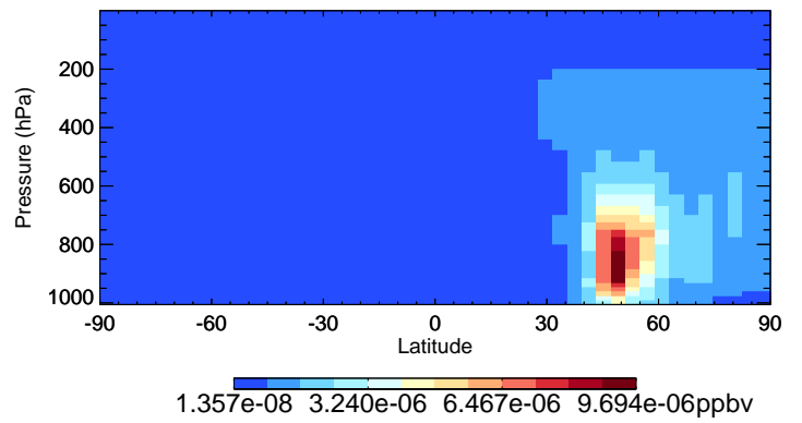
v11-02d-Run1 SOAMG - Species Curtain @ -180.000 for Jul
