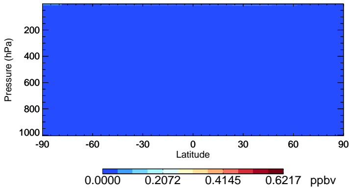
v11-02c-Run0 NO3 - Species Zonal Mean for Jul
