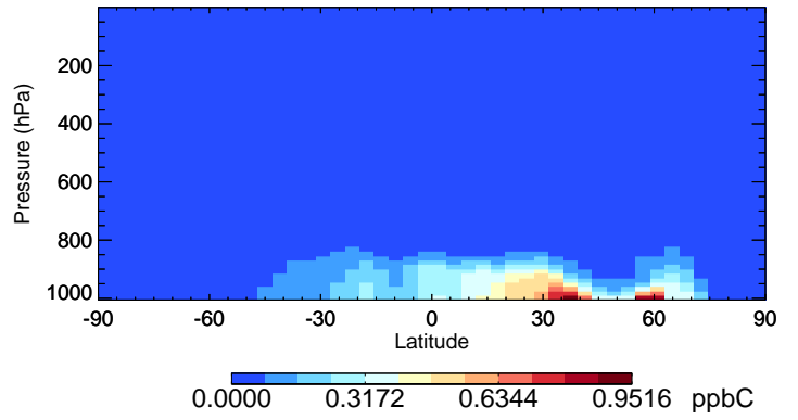
v11-02d-Run1 ALD2 - Species Curtain @ -180.000 for Jul
