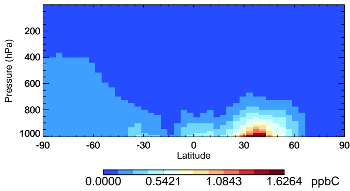
v11-02d-Run1 ALK4 - Species Zonal Mean for Jul
