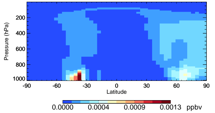
v11-02d-Run1 MONITA - Species Curtain @ -180.000 for Jul
