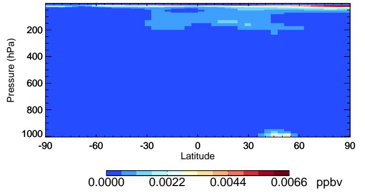
v11-02d-Run1 HNO2 - Species Curtain @ -180.000 for Jul
