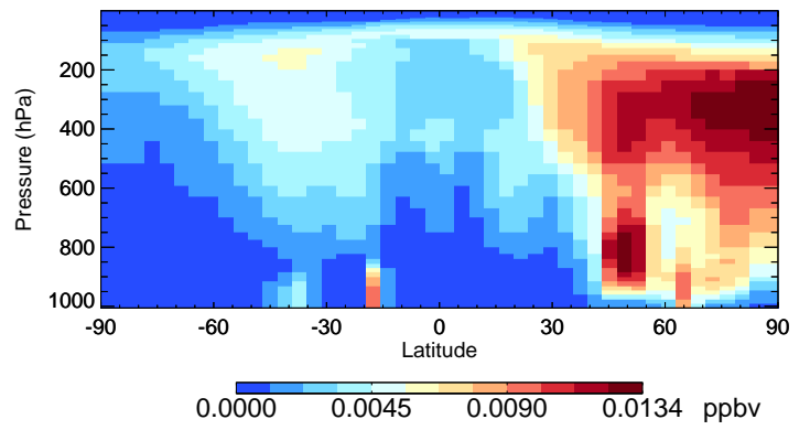
v11-02c-Run0 TSOG3 - Species Curtain @ -180.000 for Jul
