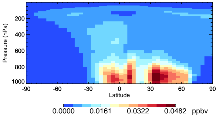
v11-02c-Run0 ISO3 - Species Zonal Mean for Jul
