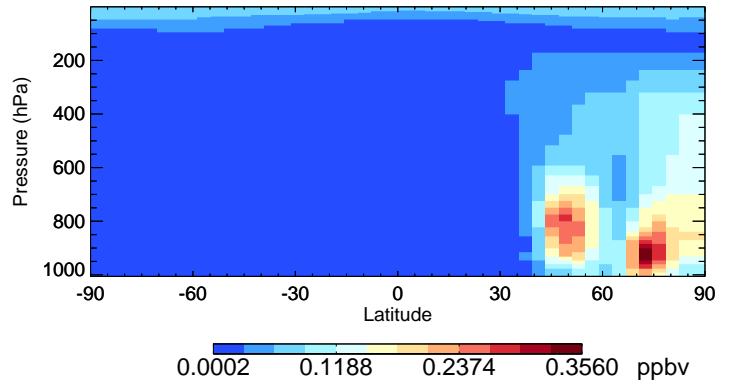
v11-02d-Run1 OCPI - Species Curtain @ -180.000 for Jul
