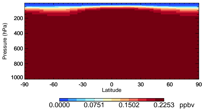
v11-02e-Run0 CFC11 - Species Zonal Mean for Jul
