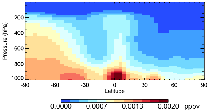
v11-02d-Run1 CHBr3 - Species Zonal Mean for Jul
