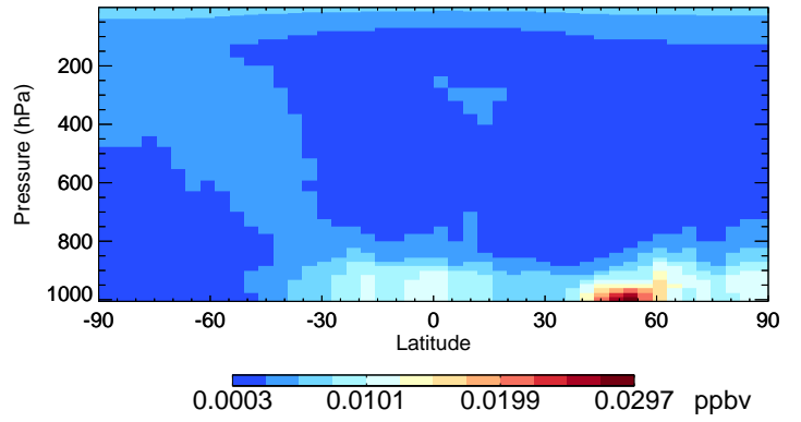
v11-02d-Run1 MSA - Species Curtain @ -180.000 for Jul
