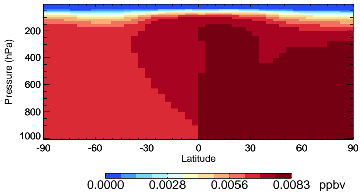
v11-02c-Run0 CH3Br - Species Zonal Mean for Jul
