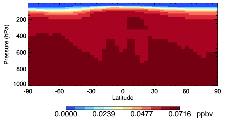
v11-02d-Run1 CCI4 - Species Curtain @ -180.000 for Jul
