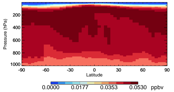
v11-02d-Run1 HCFC141b - Species Curtain @ -180.000 for Jul
