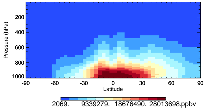
v11-02d-Run1 H2O - Species Curtain @ -180.000 for Jul
