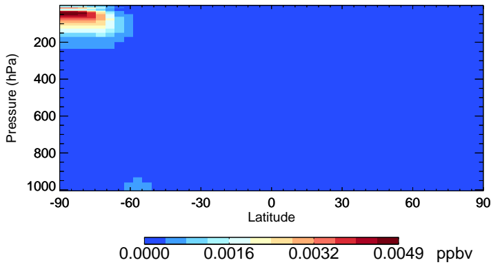
v11-02c-Run0 Br2 - Species Zonal Mean for Jul
