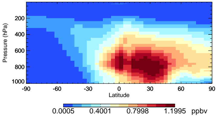
v11-02d-Run1 H2O2 - Species Zonal Mean for Jul
