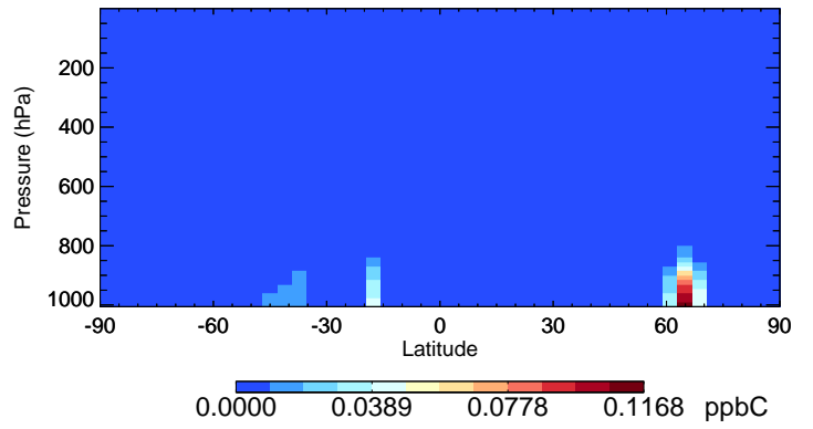
v11-02c-Run0 PRPE - Species Curtain @ -180.000 for Jul
