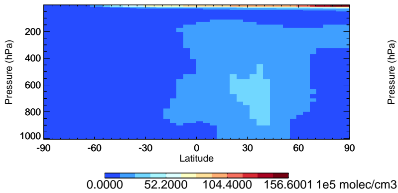
v11-02c-Run0 OH - Species Zonal Mean for Jul
