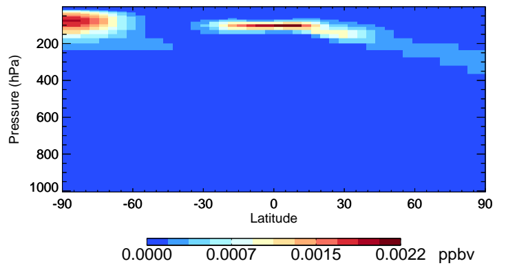
v11-02d-Run1 ASOA3 - Species Curtain @ -180.000 for Jul
