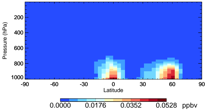
v11-02d-Run1 TSOA2 - Species Zonal Mean for Jul
