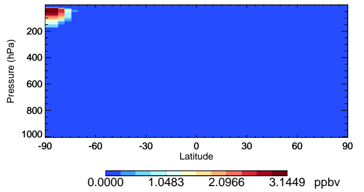
v11-02d-Run1 NIT - Species Curtain @ -180.000 for Jul
