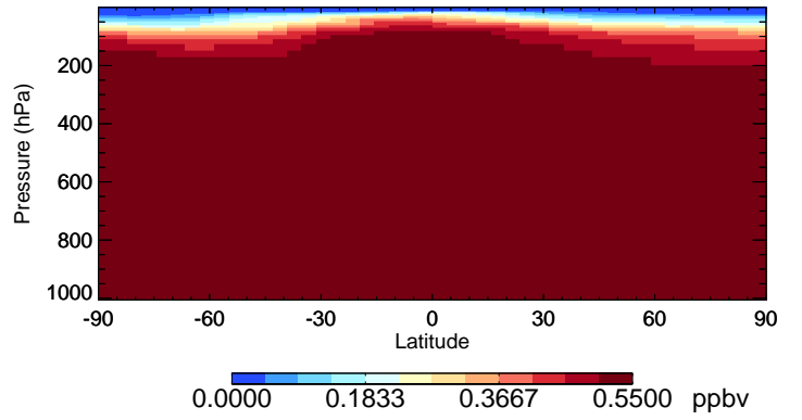
v11-02d-Run1 CH3Cl - Species Curtain @ -180.000 for Jul
