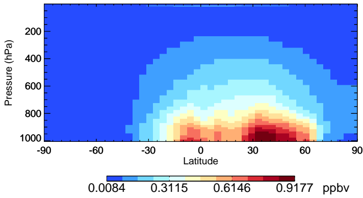
v11-02c-Run0 CH2O - Species Zonal Mean for Jul
