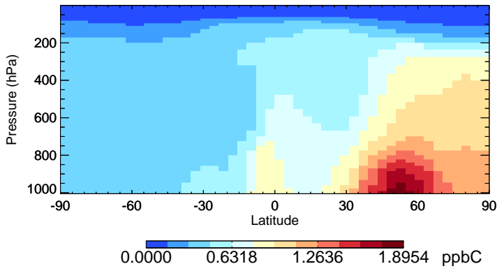
v11-02c-Run0 C2H6 - Species Zonal Mean for Jul
