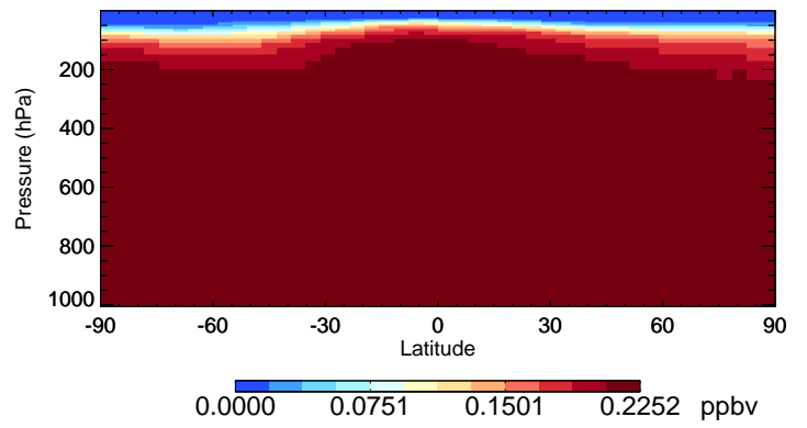
v11-02d-Run1 CFC11 - Species Curtain @ -180.000 for Jul
