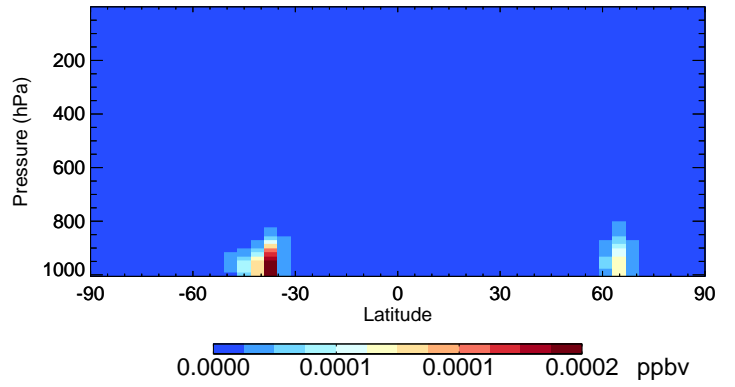
v11-02d-Run1 ISN1 - Species Curtain @ -180.000 for Jul
