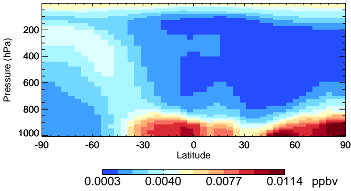
v11-02d-Run1 MSA - Species Zonal Mean for Jul
