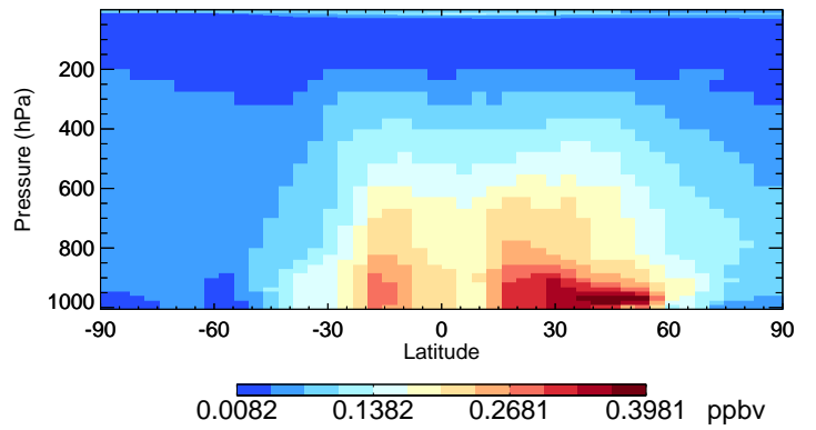
v11-02e-Run0 CH2O - Species Curtain @ -180.000 for Jul
