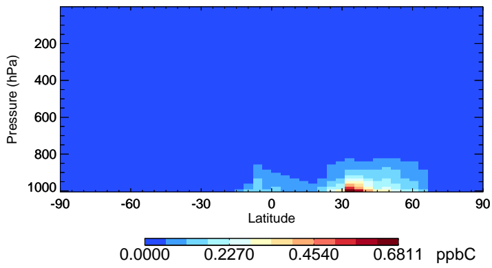
v11-02c-Run0 TOLU - Species Zonal Mean for Jul
