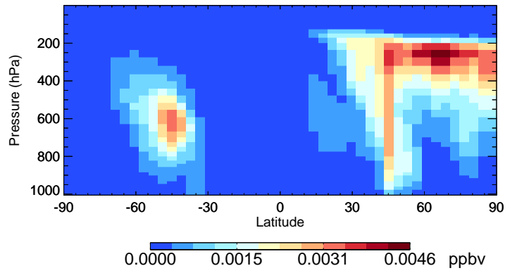
v11-02c-Run0 DST2 - Species Curtain @ -180.000 for Jul
