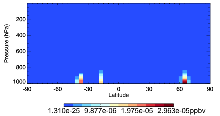
v11-02e-Run0 MONITU - Species Curtain @ -180.000 for Jul
