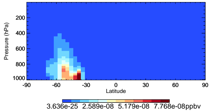
v11-02c-Run0 NPMN - Species Curtain @ -180.000 for Jul
