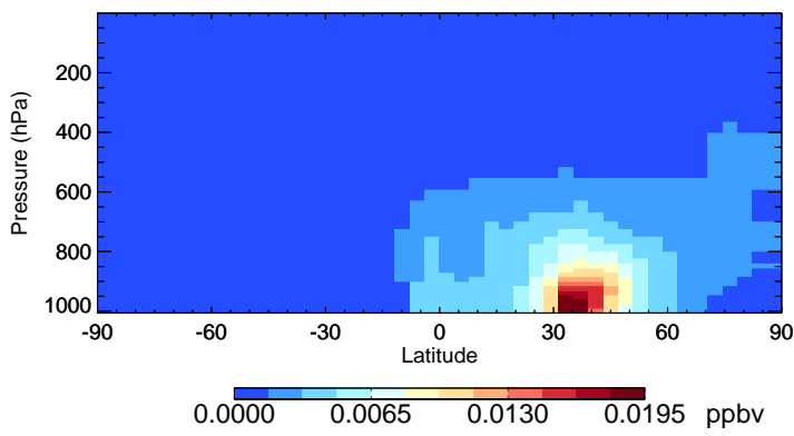
v11-02d-Run1 ASOAN - Species Zonal Mean for Jul
