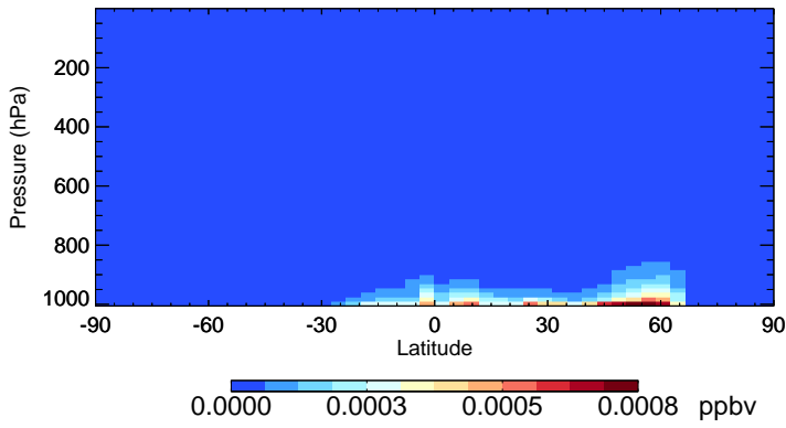
v11-02c-Run0 MONITU - Species Zonal Mean for Jul
