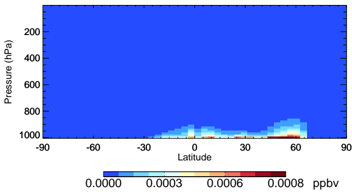
v11-02e-Run0 MONITU - Species Zonal Mean for Jul
