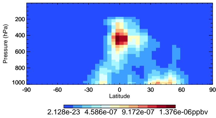
v11-02c-Run0 ISN1OG - Species Zonal Mean for Jul
