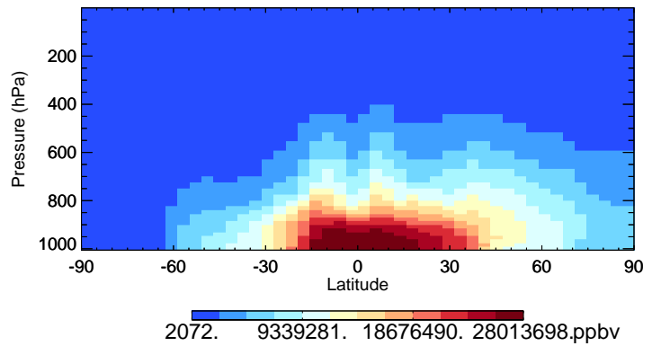
v11-02e-Run0 H2O - Species Curtain @ -180.000 for Jul
