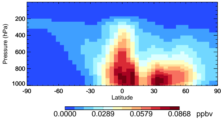
v11-02d-Run1 MAP - Species Zonal Mean for Jul
