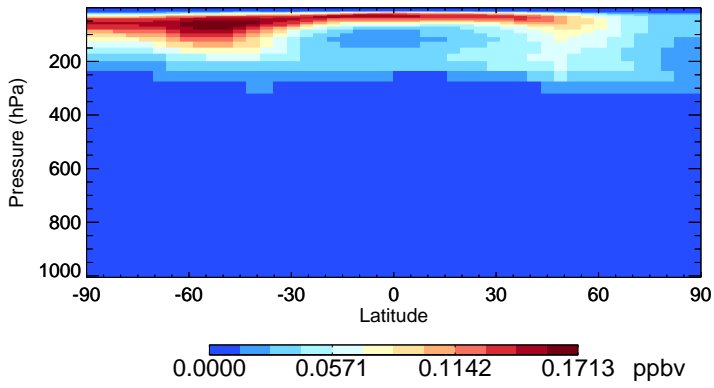
v11-02c-Run0 MPN - Species Zonal Mean for Jul
