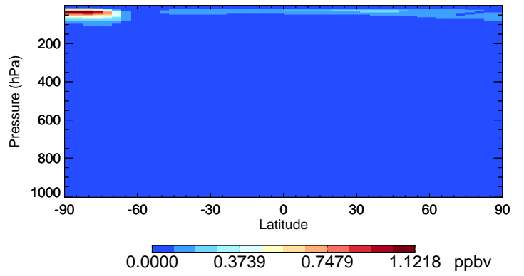
v11-02c-Run0 HNO4 - Species Curtain @ -180.000 for Jul
