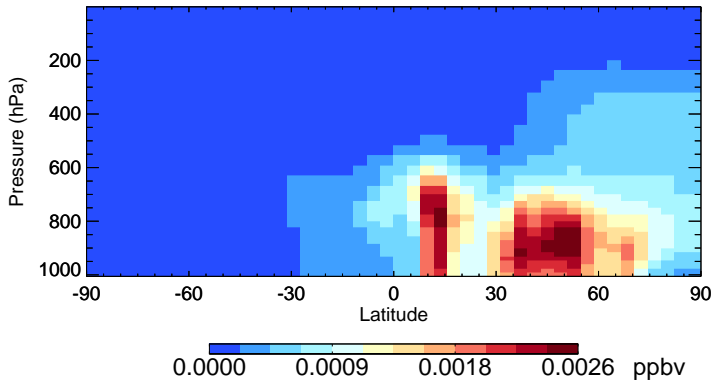
v11-02d-Run1 SOAME - Species Zonal Mean for Jul
