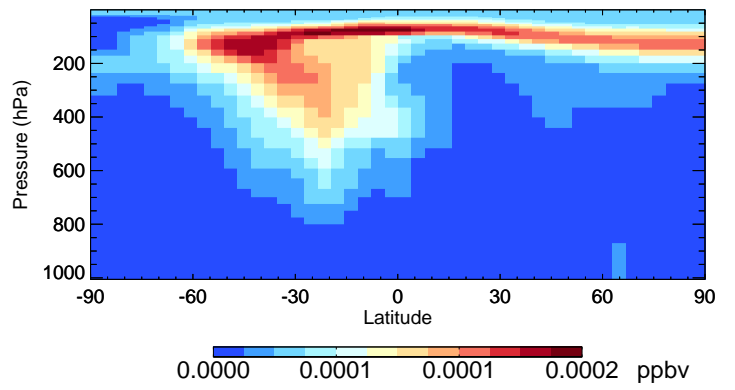
v11-02d-Run1 DHDN - Species Curtain @ -180.000 for Jul
