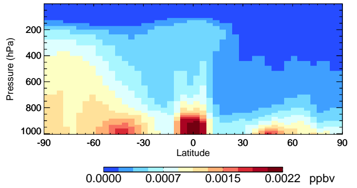
v11-02c-Run0 CHBr3 - Species Curtain @ -180.000 for Jul
