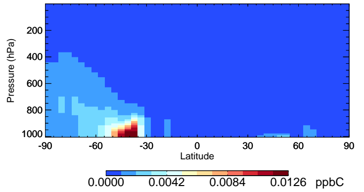
v11-02c-Run0 XYLE - Species Curtain @ -180.000 for Jul
