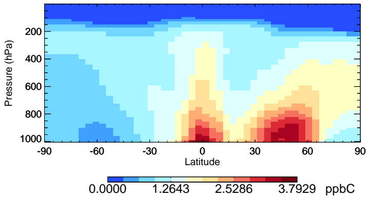
v11-02c-Run0 ACET - Species Zonal Mean for Jul
