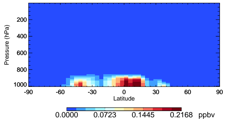
v11-02c-Run0 NH3 - Species Curtain @ -180.000 for Jul
