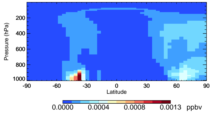
v11-02c-Run0 MONITA - Species Curtain @ -180.000 for Jul
