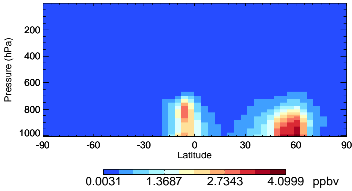
v11-02d-Run1 OCPI - Species Zonal Mean for Jul
