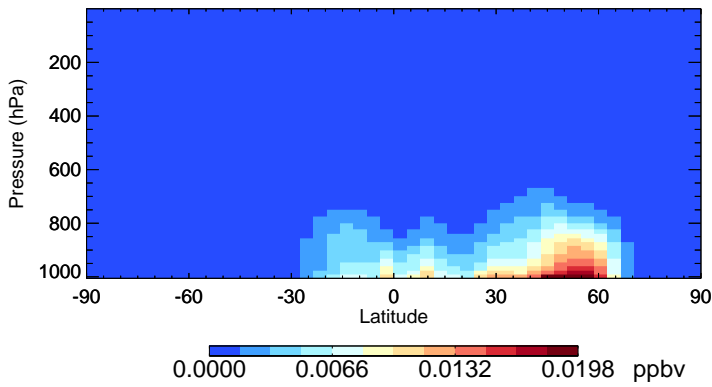
v11-02e-Run0 MONITA - Species Zonal Mean for Jul
