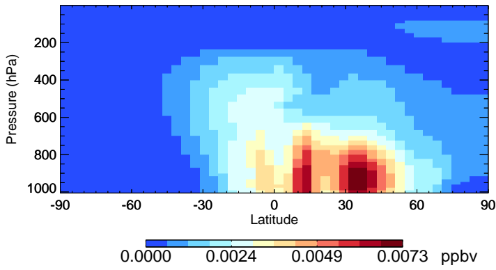
v11-02c-Run0 ISOG1 - Species Zonal Mean for Jul
