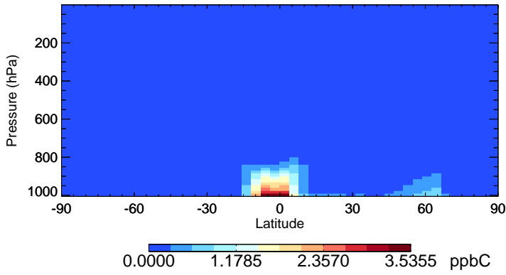
v11-02d-Run1 ISOP - Species Zonal Mean for Jul
