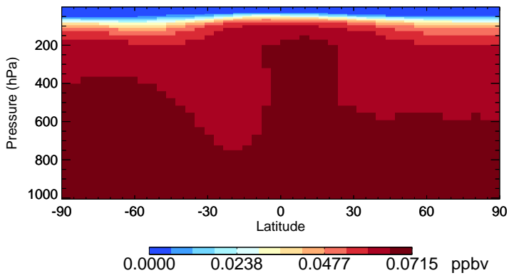
v11-02d-Run1 CCI4 - Species Zonal Mean for Jul
