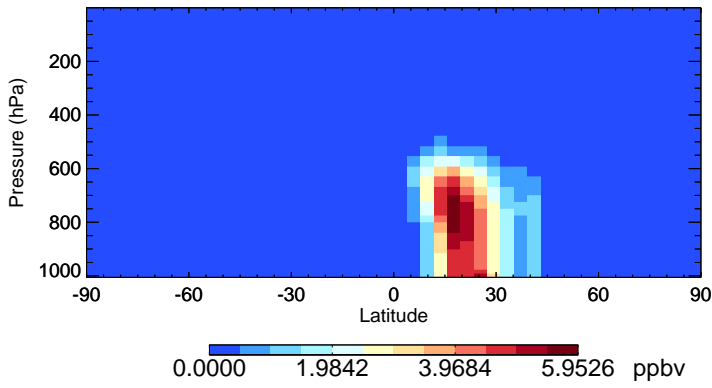
v11-02c-Run0 DST1 - Species Zonal Mean for Jul
