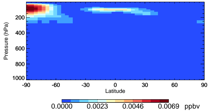
v11-02d-Run1 ISOA3 - Species Curtain @ -180.000 for Jul
