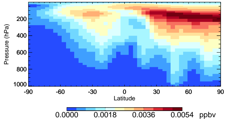
v11-02d-Run1 ASOG3 - Species Curtain @ -180.000 for Jul
