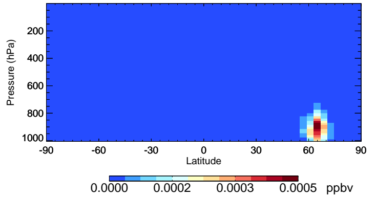
v11-02d-Run1 IEPOXD - Species Curtain @ -180.000 for Jul
