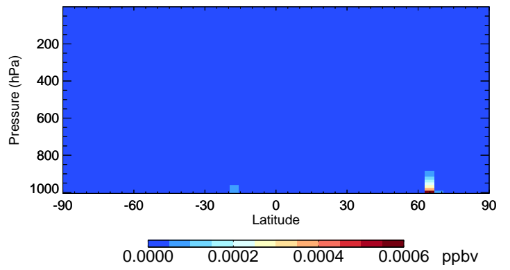
v11-02d-Run1 LIMO - Species Curtain @ -180.000 for Jul
