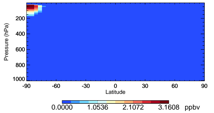
v11-02c-Run0 NIT - Species Curtain @ -180.000 for Jul
