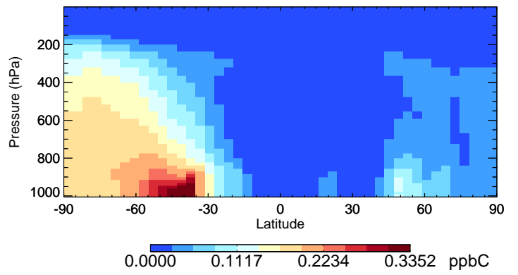
v11-02c-Run0 ALK4 - Species Curtain @ -180.000 for Jul
