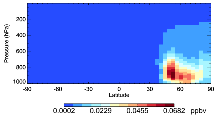
v11-02e-Run0 SOAIE - Species Curtain @ -180.000 for Jul
