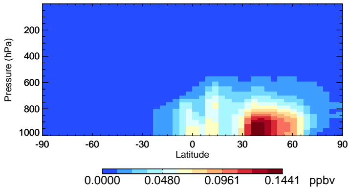
v11-02c-Run0 INDIOL - Species Zonal Mean for Jul
