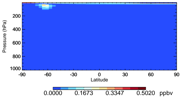
v11-02c-Run0 CIO - Species Zonal Mean for Jul
