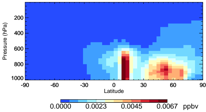
v11-02c-Run0 SOAME - Species Zonal Mean for Jul
