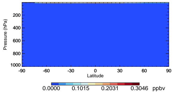
v11-02c-Run0 CI - Species Curtain @ -180.000 for Jul
