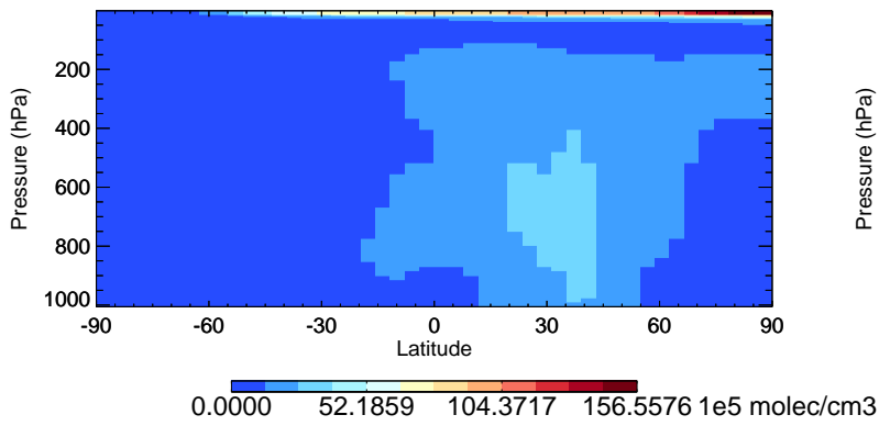
v11-02d-Run1 OH - Species Zonal Mean for Jul
