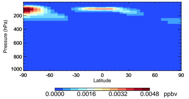
v11-02c-Run0 ISOA3 - Species Curtain @ -180.000 for Jul
