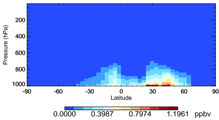
v11-02d-Run1 NH3 - Species Zonal Mean for Jul
