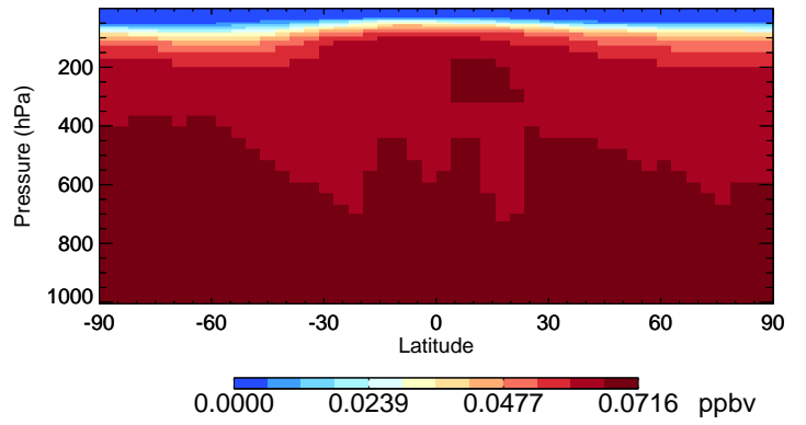
v11-02c-Run0 CCI4 - Species Curtain @ -180.000 for Jul
