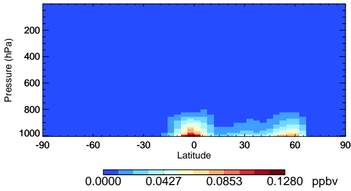
v11-02c-Run0 RCHO - Species Zonal Mean for Jul
