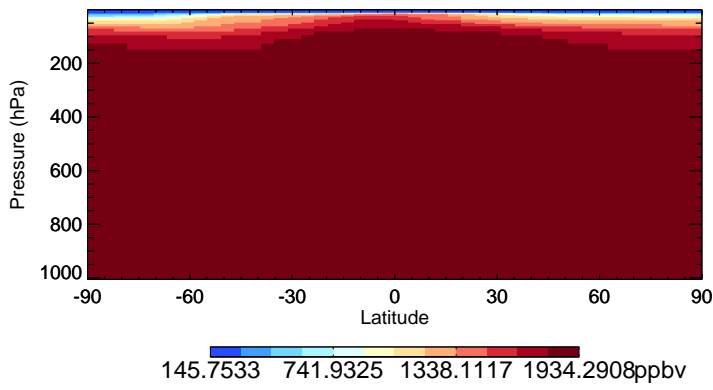
v11-02c-Run0 CH4 - Species Zonal Mean for Jul
