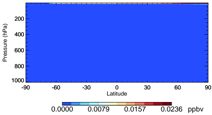
v11-02d-Run1 Br - Species Zonal Mean for Jul
