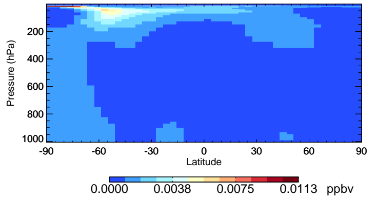
v11-02c-Run0 HOBr - Species Curtain @ -180.000 for Jul
