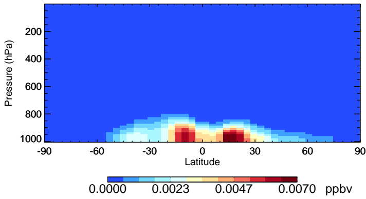
v11-02c-Run0 NITs - Species Zonal Mean for Jul
