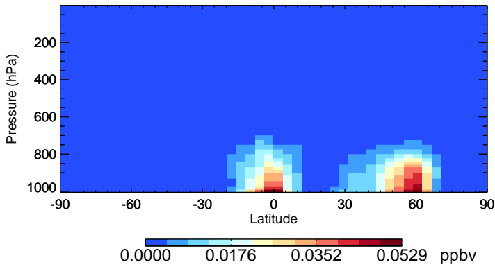
v11-02c-Run0 TSOA2 - Species Zonal Mean for Jul
