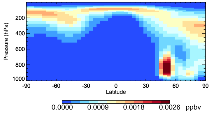
v11-02c-Run0 ISOA1 - Species Curtain @ -180.000 for Jul
