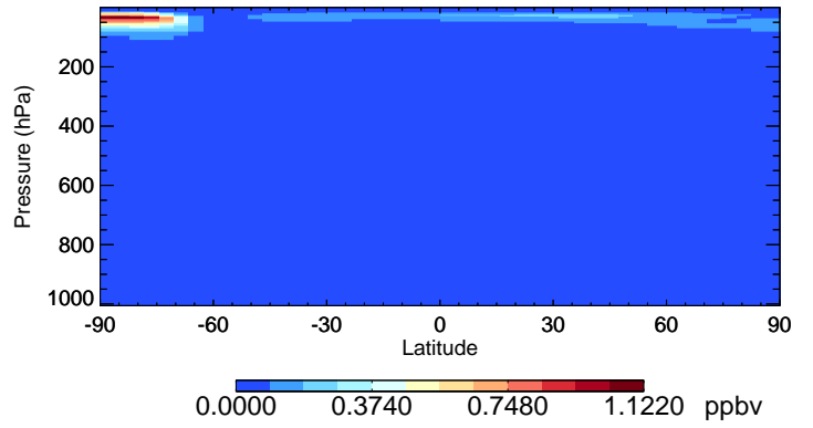
v11-02d-Run1 HNO4 - Species Curtain @ -180.000 for Jul
