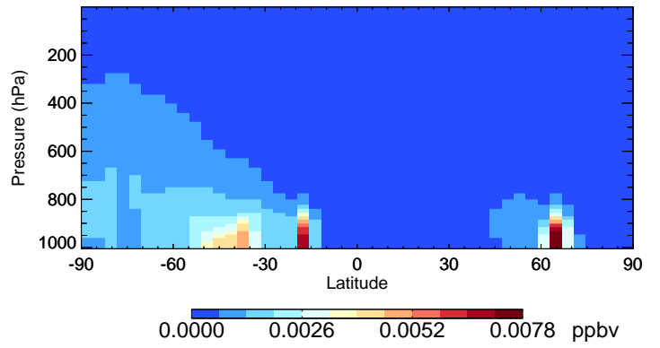
v11-02c-Run0 RCHO - Species Curtain @ -180.000 for Jul
