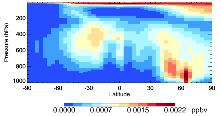
v11-02d-Run1 ISOG1 - Species Curtain @ -180.000 for Jul
