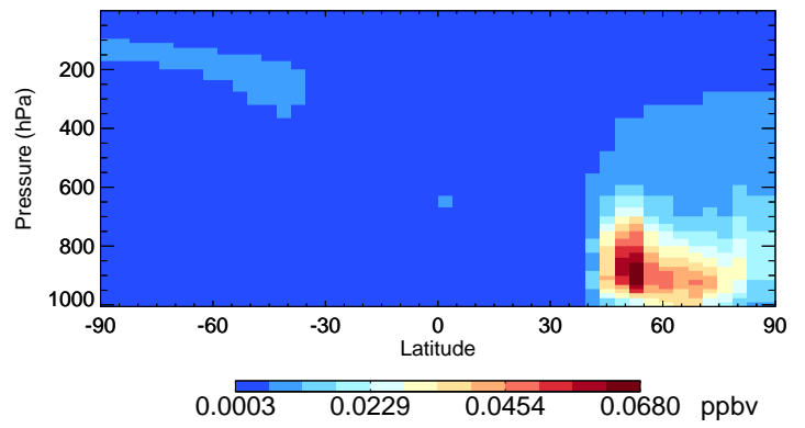
v11-02c-Run0 SOAIE - Species Curtain @ -180.000 for Jul
