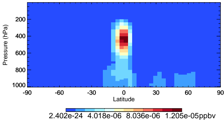
v11-02c-Run0 LVOC - Species Zonal Mean for Jul
