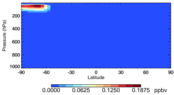
v11-02d-Run1 OCIO - Species Zonal Mean for Jul
