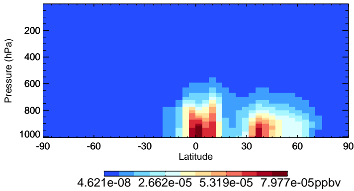
v11-02c-Run0 SOAMG - Species Zonal Mean for Jul
