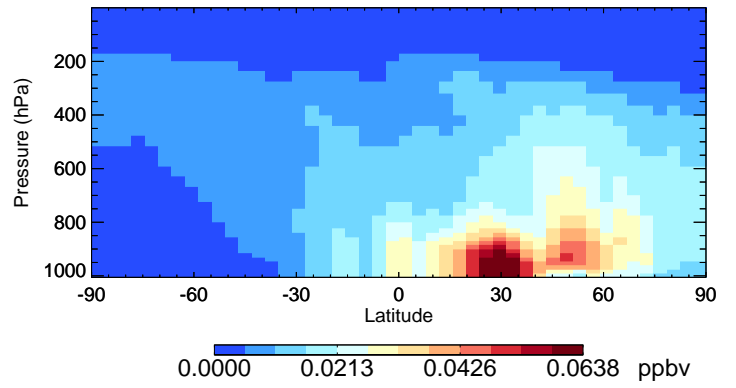
v11-02c-Run0 MAP - Species Curtain @ -180.000 for Jul
