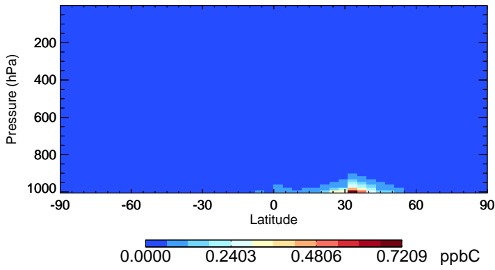
v11-02c-Run0 XYLE - Species Zonal Mean for Jul
