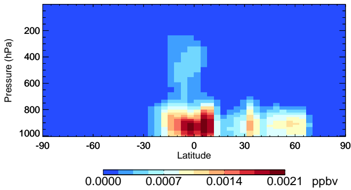
v11-02e-Run0 IEPOXD - Species Zonal Mean for Jul
