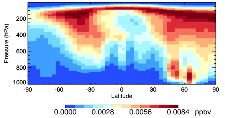
v11-02c-Run0 ISO3 - Species Curtain @ -180.000 for Jul
