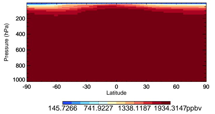
v11-02c-Run0 CH4 - Species Curtain @ -180.000 for Jul
