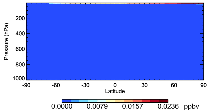
v11-02d-Run1 Br - Species Curtain @ -180.000 for Jul
