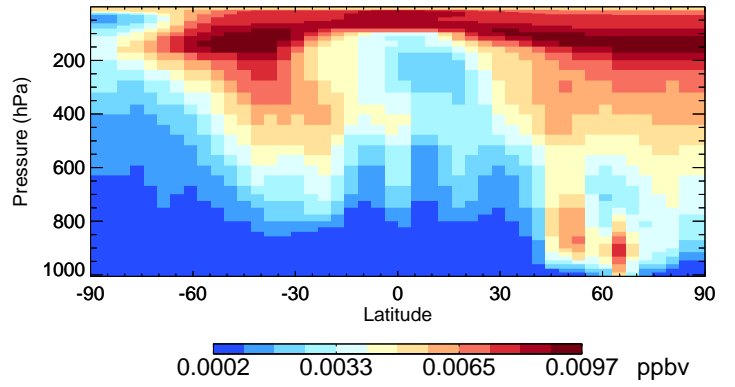
v11-02d-Run1 ISO3 - Species Curtain @ -180.000 for Jul
