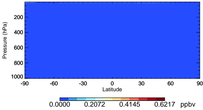
v11-02d-Run1 NO3 - Species Zonal Mean for Jul
