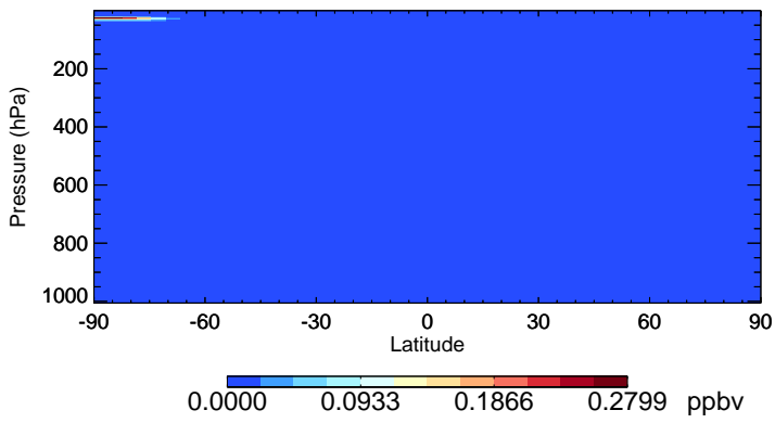
v11-02d-Run1 ClNO2 - Species Zonal Mean for Jul
