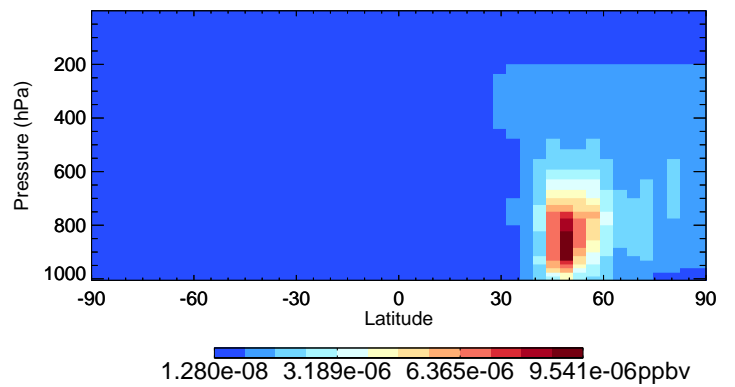
v11-02e-Run0 SOAMG - Species Curtain @ -180.000 for Jul
