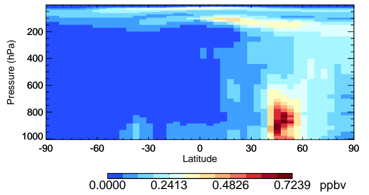
v11-02d-Run1 SO4 - Species Curtain @ -180.000 for Jul
