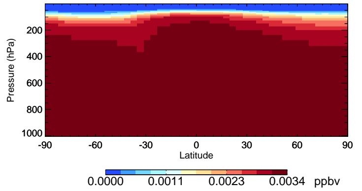
v11-02c-Run0 H1211 - Species Curtain @ -180.000 for Jul
