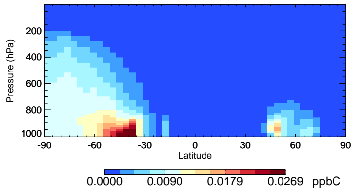
v11-02d-Run1 TOLU - Species Curtain @ -180.000 for Jul
