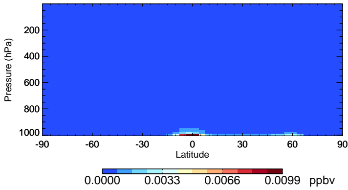
v11-02c-Run0 MTPO - Species Zonal Mean for Jul
