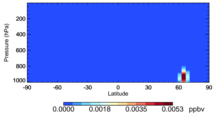
v11-02c-Run0 RIPB - Species Curtain @ -180.000 for Jul
