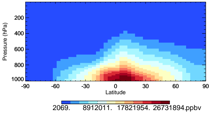
v11-02d-Run1 H2O - Species Zonal Mean for Jul
