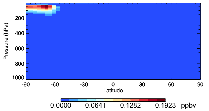
v11-02c-Run0 OCIO - Species Curtain @ -180.000 for Jul
