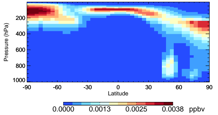
v11-02d-Run1 TSOA2 - Species Curtain @ -180.000 for Jul
