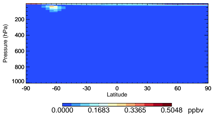
v11-02d-Run1 CIO - Species Zonal Mean for Jul
