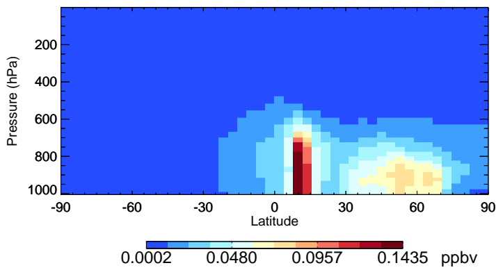
v11-02e-Run0 SOAIE - Species Zonal Mean for Jul
