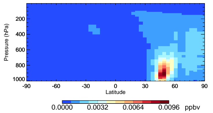
v11-02d-Run1 ASOAN - Species Curtain @ -180.000 for Jul
