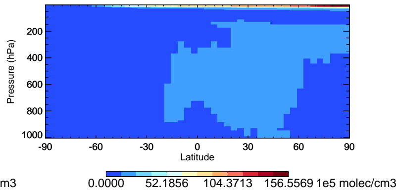
v11-02d-Run1 OH - Species Curtain @ -180.000 for Jul
