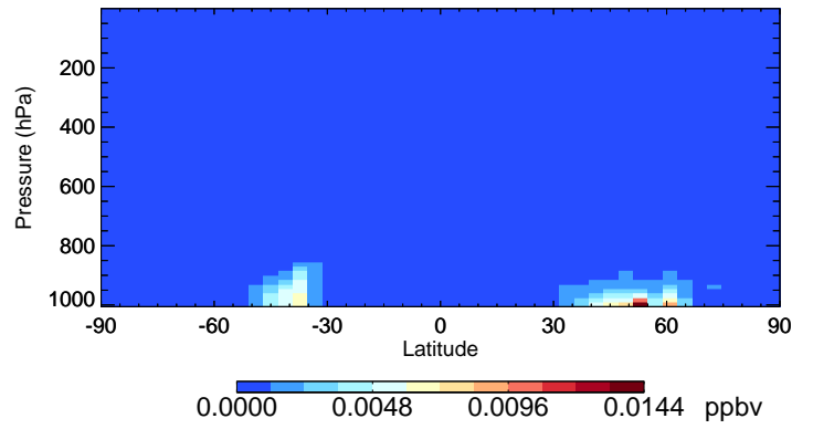
v11-02c-Run0 BCPO - Species Curtain @ -180.000 for Jul
