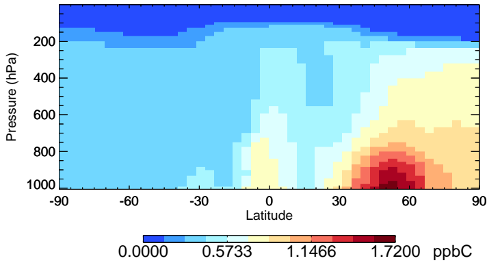
v11-02d-Run1 C2H6 - Species Zonal Mean for Jul
