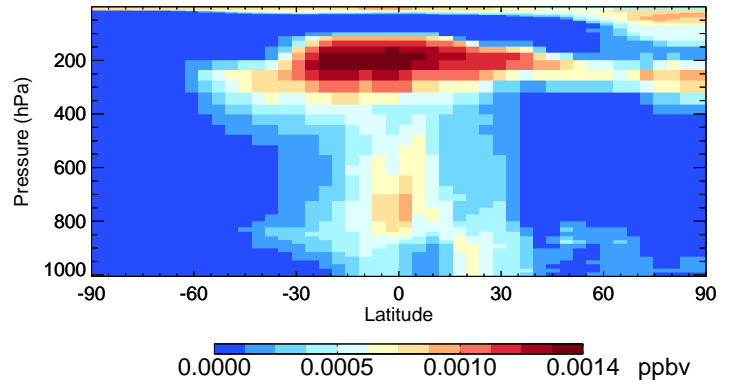
v11-02d-Run1 HBr - Species Curtain @ -180.000 for Jul
