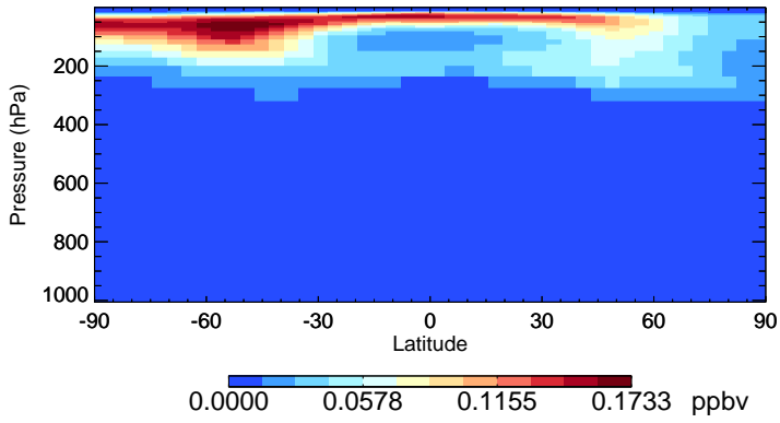
v11-02d-Run1 MPN - Species Zonal Mean for Jul
