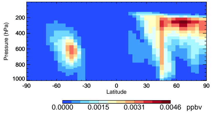
v11-02d-Run1 DST2 - Species Curtain @ -180.000 for Jul
