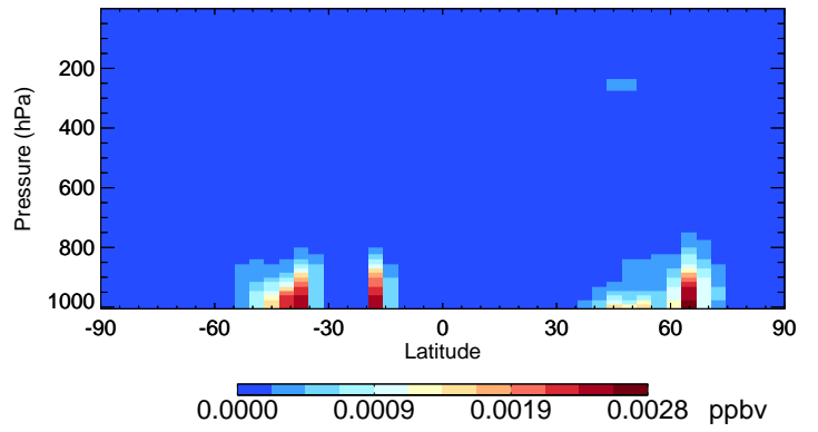
v11-02c-Run0 SOAP - Species Curtain @ -180.000 for Jul
