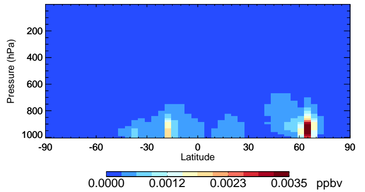
v11-02e-Run0 MGLY - Species Curtain @ -180.000 for Jul
