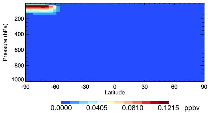
v11-02e-Run0 OCIO - Species Zonal Mean for Jul
