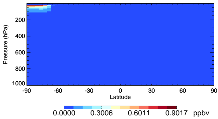
v11-02d-Run1 Cl2 - Species Zonal Mean for Jul
