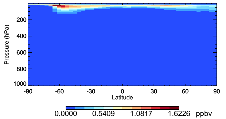
v11-02e-Run0 ClNO3 - Species Curtain @ -180.000 for Jul
