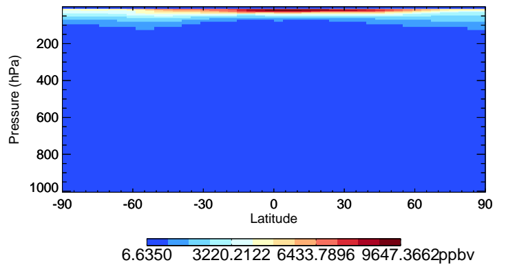
v11-02d-Run1 O3 - Species Curtain @ -180.000 for Jul
