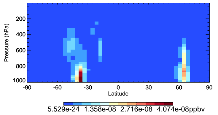
v11-02d-Run1 ISN1OG - Species Curtain @ -180.000 for Jul
