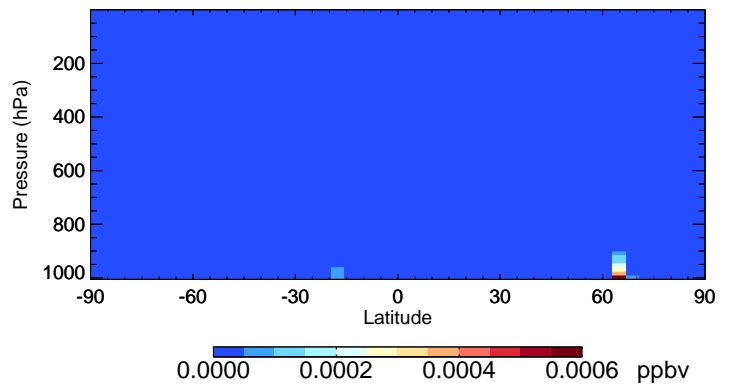
v11-02c-Run0 LIMO - Species Curtain @ -180.000 for Jul
