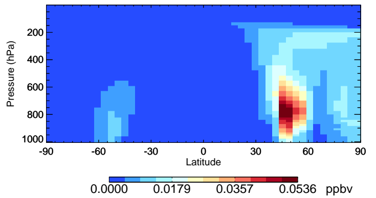
v11-02d-Run1 DST1 - Species Curtain @ -180.000 for Jul
