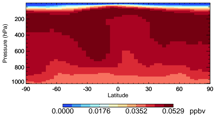
v11-02c-Run0 HCFC141b - Species Zonal Mean for Jul
