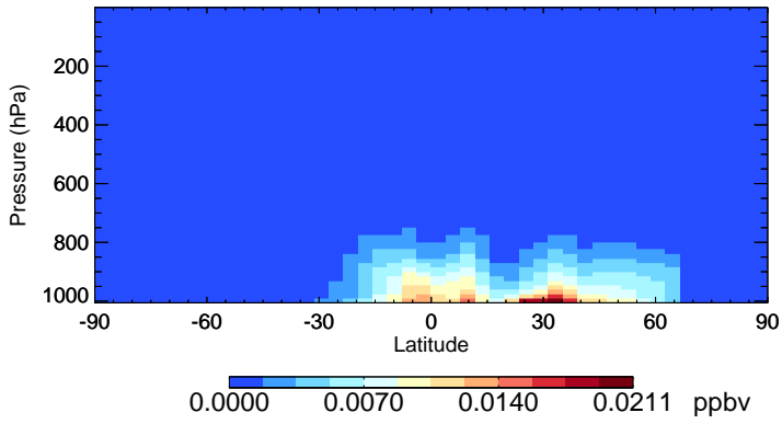
v11-02d-Run1 GLYX - Species Zonal Mean for Jul
