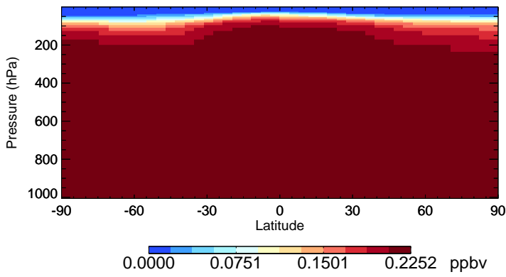
v11-02d-Run1 CFC11 - Species Zonal Mean for Jul
