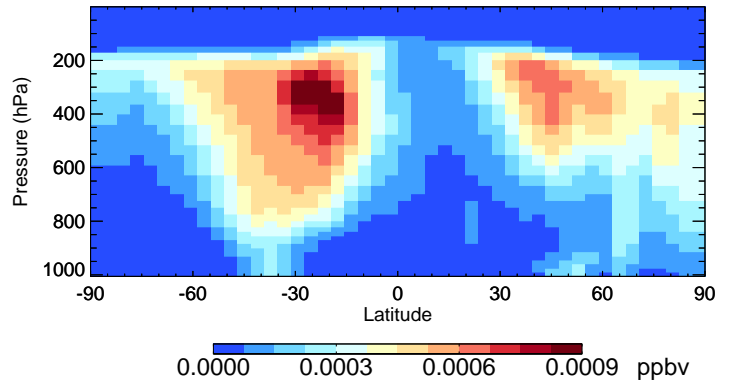
v11-02d-Run1 R4N2 - Species Curtain @ -180.000 for Jul
