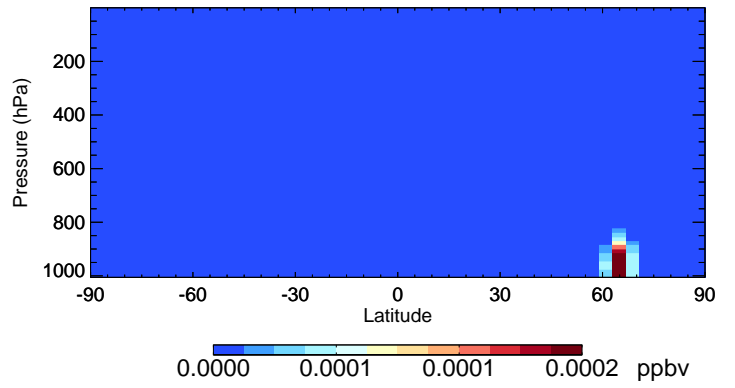
v11-02c-Run0 MOBA - Species Curtain @ -180.000 for Jul
