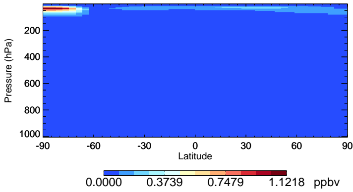
v11-02c-Run0 HNO4 - Species Zonal Mean for Jul
