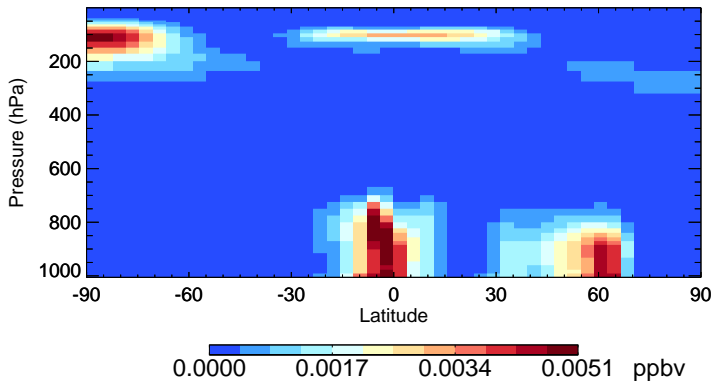
v11-02c-Run0 ISOA3 - Species Zonal Mean for Jul
