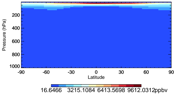
v11-02c-Run0 O3 - Species Zonal Mean for Jul
