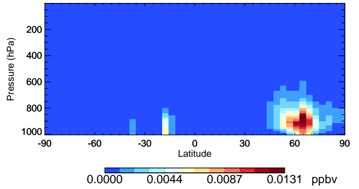
v11-02d-Run1 HAC - Species Curtain @ -180.000 for Jul
