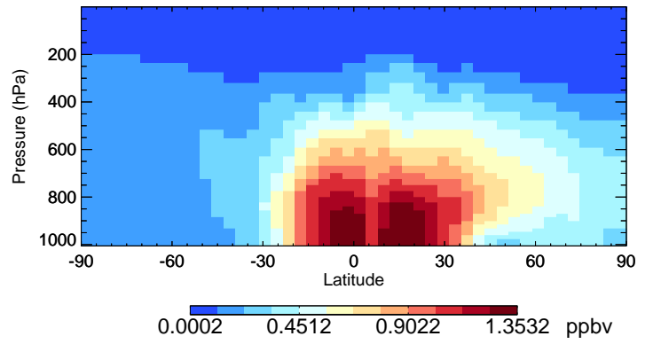
v11-02c-Run0 MP - Species Curtain @ -180.000 for Jul
