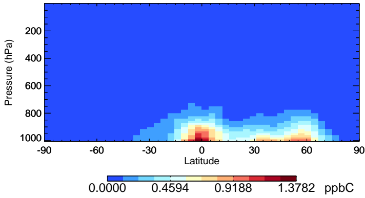
v11-02d-Run1 ALD2 - Species Zonal Mean for Jul
