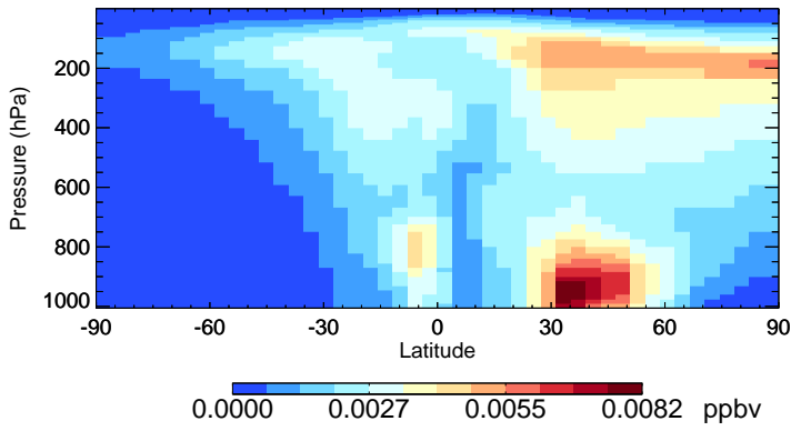
v11-02c-Run0 ASOG3 - Species Zonal Mean for Jul
