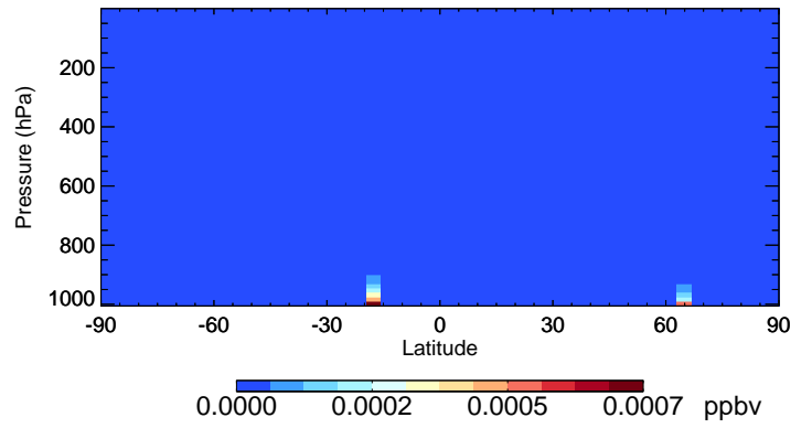
v11-02c-Run0 MTPO - Species Curtain @ -180.000 for Jul
