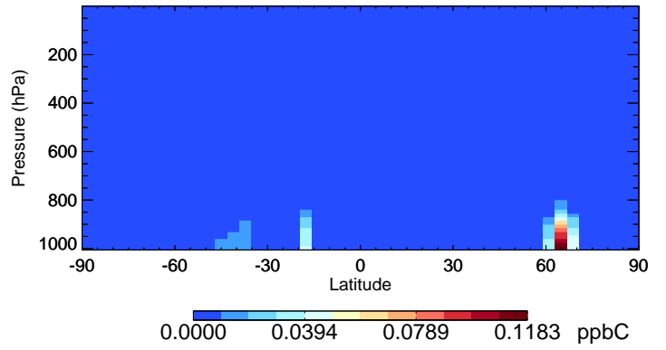
v11-02d-Run1 PRPE - Species Curtain @ -180.000 for Jul
