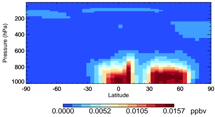
v11-02c-Run0 ISOA1 - Species Zonal Mean for Jul
