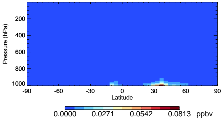
v11-02d-Run1 HNO2 - Species Zonal Mean for Jul
