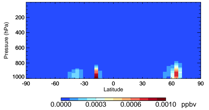
v11-02c-Run0 GLYX - Species Curtain @ -180.000 for Jul
