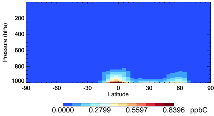
v11-02d-Run1 PRPE - Species Zonal Mean for Jul
