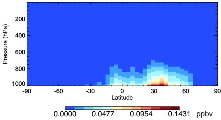
v11-02c-Run0 SOAP - Species Zonal Mean for Jul
