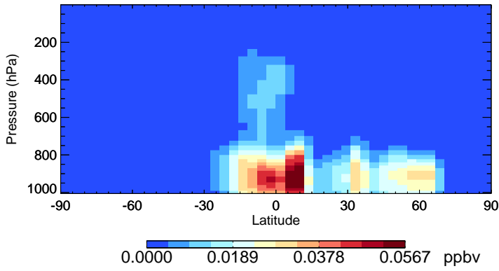
v11-02d-Run1 IEPOXA - Species Zonal Mean for Jul
