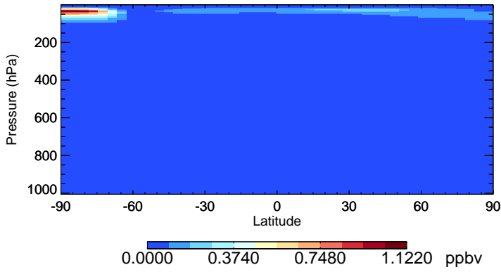
v11-02d-Run1 HNO4 - Species Zonal Mean for Jul
