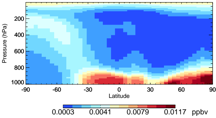
v11-02c-Run0 MSA - Species Zonal Mean for Jul
