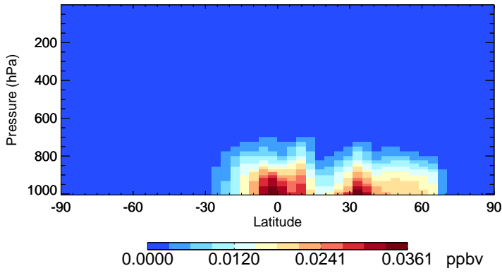
v11-02d-Run1 MGLY - Species Zonal Mean for Jul
