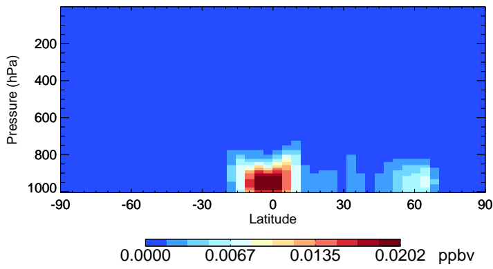
v11-02c-Run0 RIPB - Species Zonal Mean for Jul
