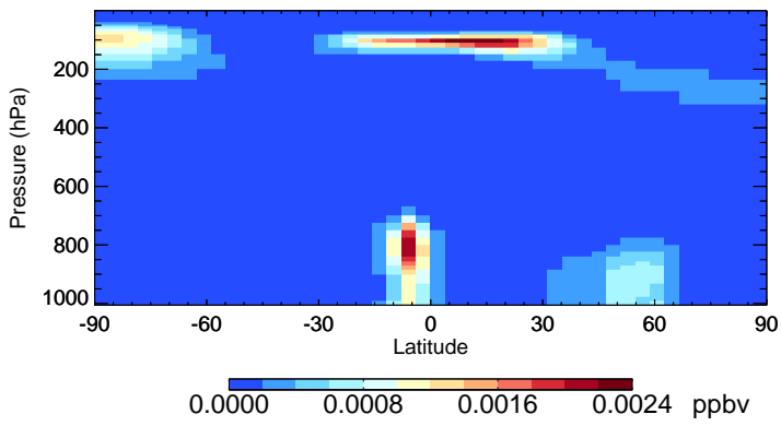
v11-02c-Run0 ASOA3 - Species Zonal Mean for Jul
