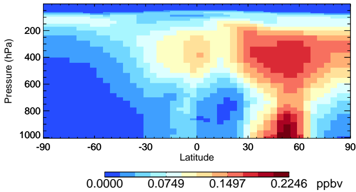
v11-02c-Run0 PAN - Species Zonal Mean for Jul
