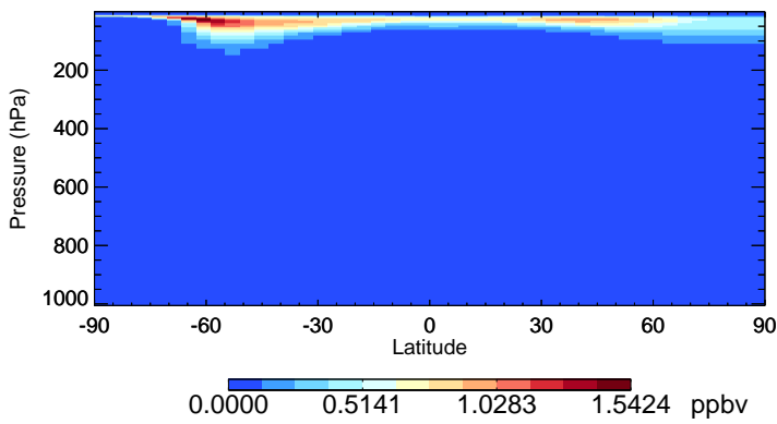
v11-02e-Run0 ClNO3 - Species Zonal Mean for Jul
