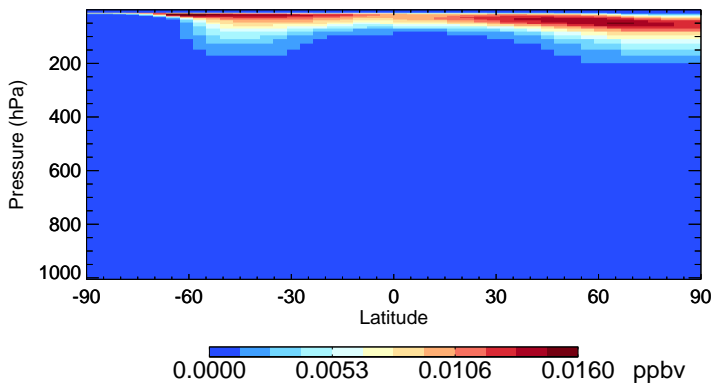
v11-02c-Run0 BrNO3 - Species Zonal Mean for Jul
