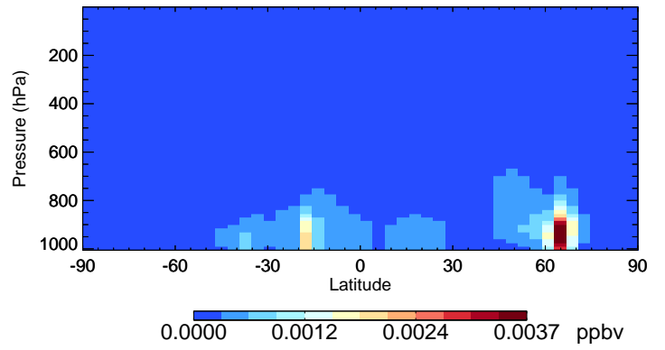
v11-02c-Run0 MGLY - Species Curtain @ -180.000 for Jul
