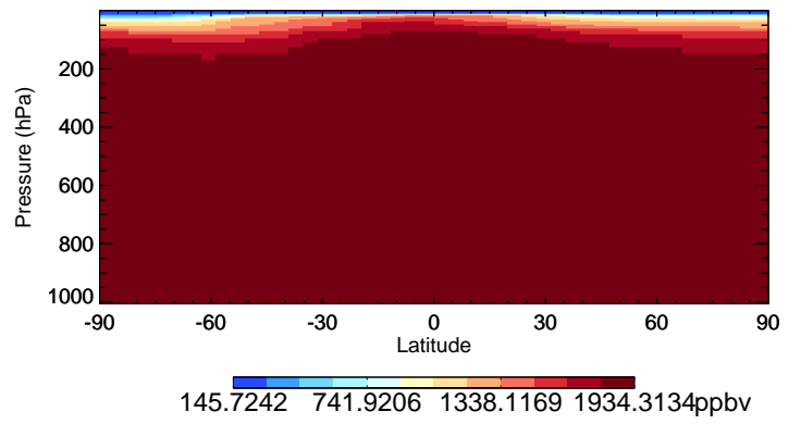
v11-02d-Run1 CH4 - Species Curtain @ -180.000 for Jul
