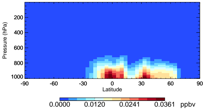
v11-02c-Run0 MGLY - Species Zonal Mean for Jul
