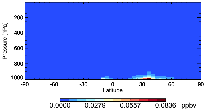
v11-02c-Run0 HNO2 - Species Zonal Mean for Jul
