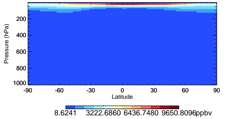
v11-02c-Run0 O3 - Species Curtain @ -180.000 for Jul
