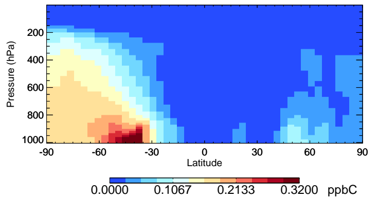
v11-02d-Run1 ALK4 - Species Curtain @ -180.000 for Jul
