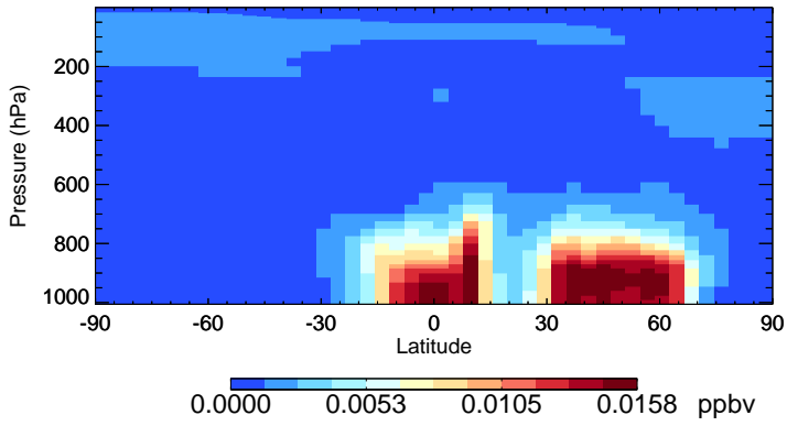
v11-02d-Run1 ISOA1 - Species Zonal Mean for Jul
