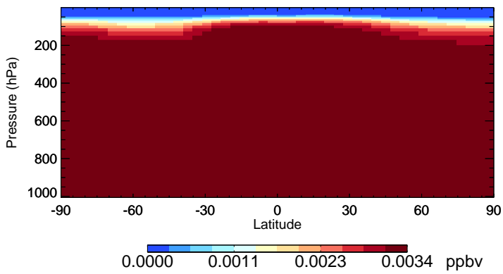
v11-02e-Run0 H1211 - Species Zonal Mean for Jul
