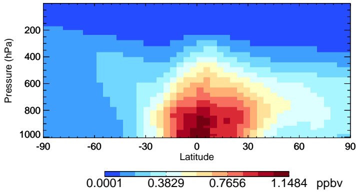
v11-02d-Run1 MP - Species Zonal Mean for Jul
