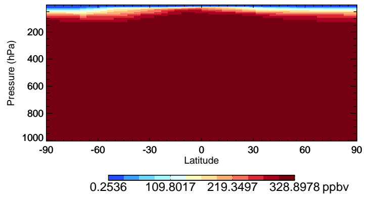
v11-02d-Run1 N2O - Species Curtain @ -180.000 for Jul
