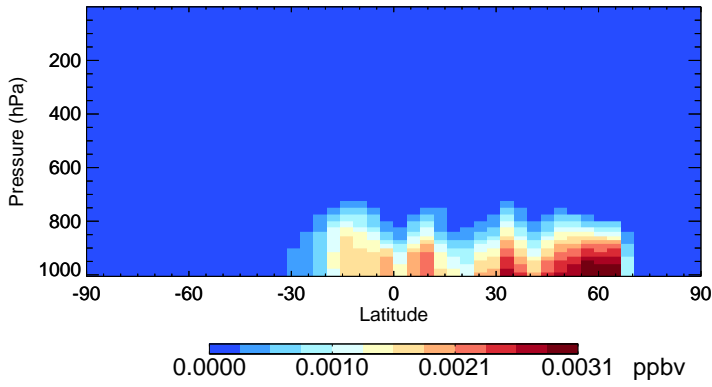
v11-02d-Run1 ISOPNB - Species Zonal Mean for Jul
