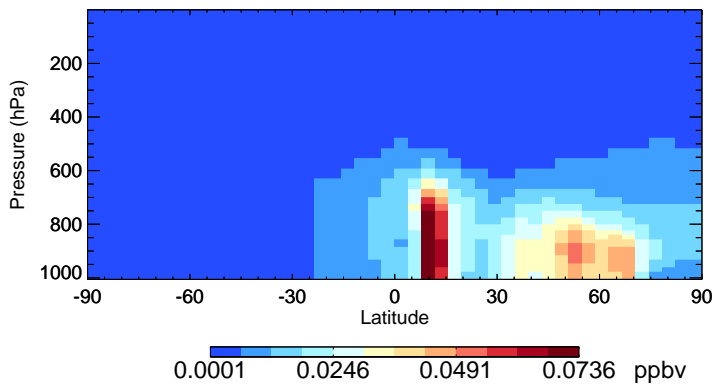
v11-02d-Run1 SOAIE - Species Zonal Mean for Jul
