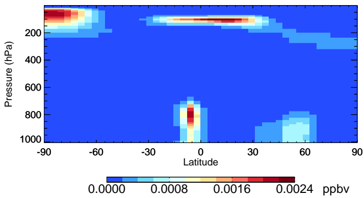
v11-02e-Run0 ASOA3 - Species Zonal Mean for Jul
