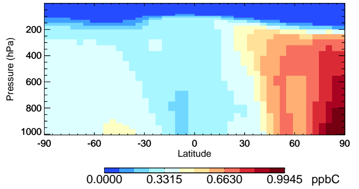
v11-02d-Run1 C2H6 - Species Curtain @ -180.000 for Jul
