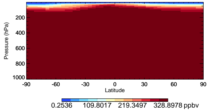
v11-02c-Run0 N2O - Species Curtain @ -180.000 for Jul
