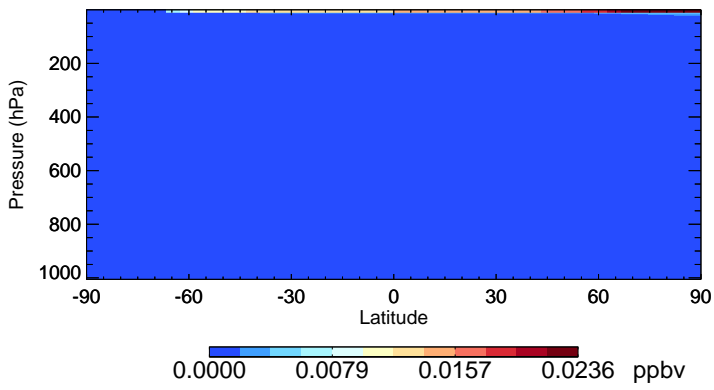
v11-02c-Run0 Br - Species Zonal Mean for Jul
