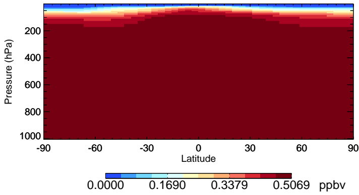
v11-02c-Run0 CFC12 - Species Zonal Mean for Jul
