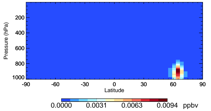
v11-02c-Run0 IEPOXA - Species Curtain @ -180.000 for Jul
