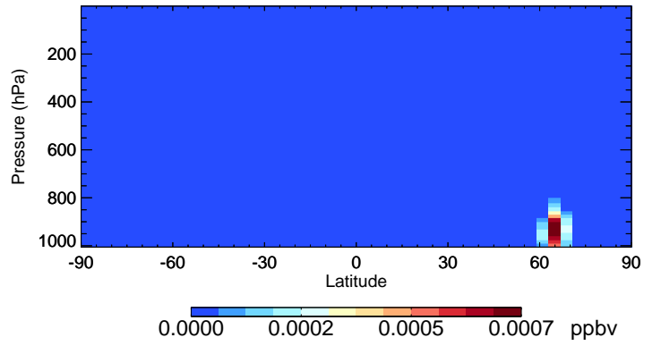
v11-02d-Run1 RIPD - Species Curtain @ -180.000 for Jul
