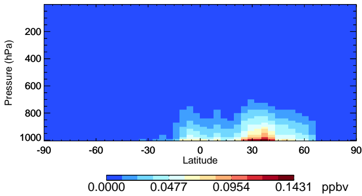
v11-02e-Run0 SOAP - Species Zonal Mean for Jul
