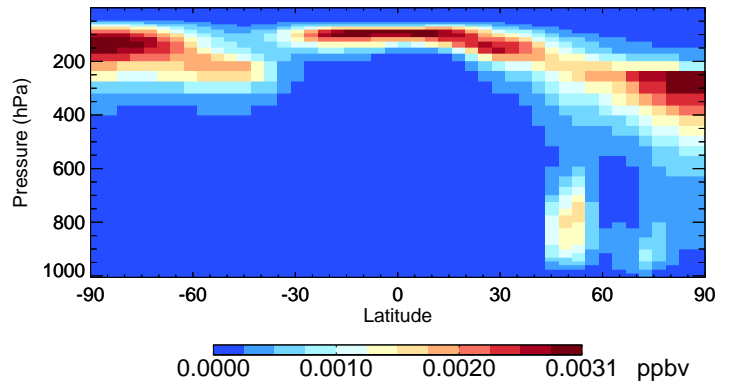
v11-02c-Run0 TSOA2 - Species Curtain @ -180.000 for Jul
