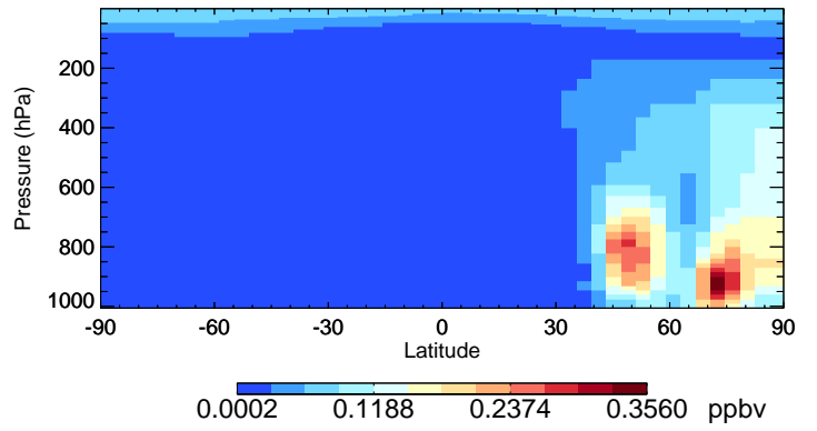
v11-02c-Run0 OCPI - Species Curtain @ -180.000 for Jul
