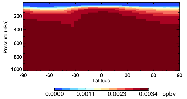
v11-02d-Run1 H1211 - Species Curtain @ -180.000 for Jul
