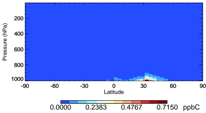
v11-02d-Run1 XYLE - Species Zonal Mean for Jul
