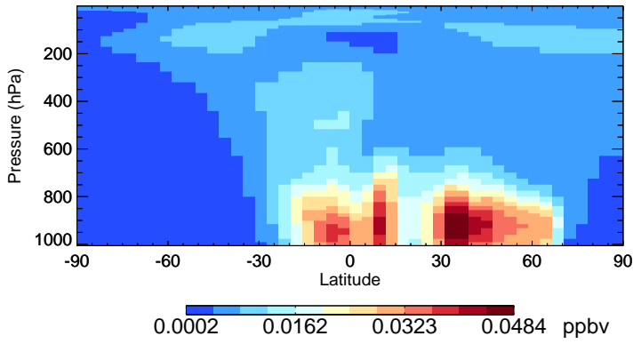
v11-02d-Run1 ISO3 - Species Zonal Mean for Jul
