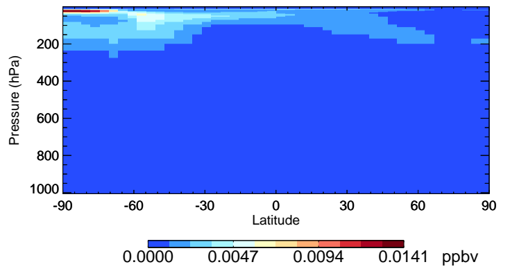
v11-02d-Run1 HOBr - Species Curtain @ -180.000 for Jul
