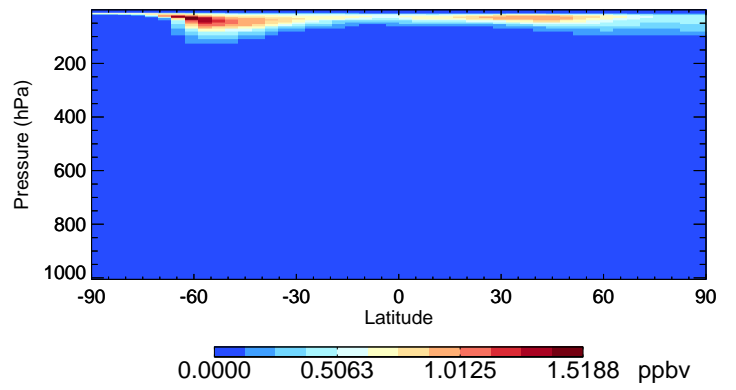
v11-02d-Run1 ClNO3 - Species Curtain @ -180.000 for Jul
