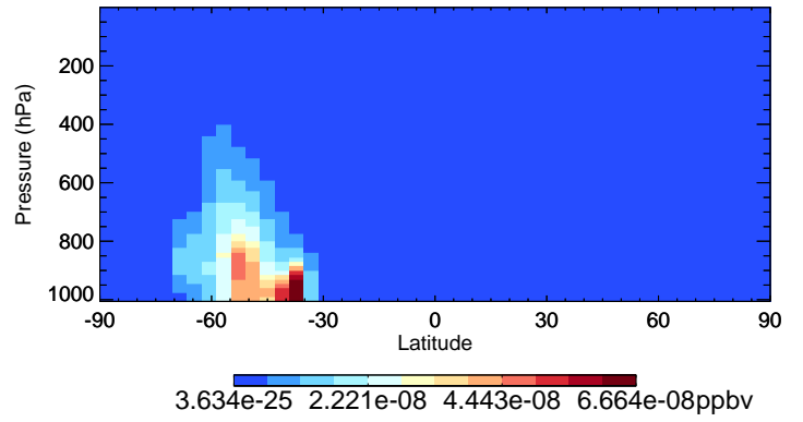
v11-02d-Run1 NPMN - Species Curtain @ -180.000 for Jul
