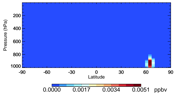
v11-02e-Run0 RIPB - Species Curtain @ -180.000 for Jul
