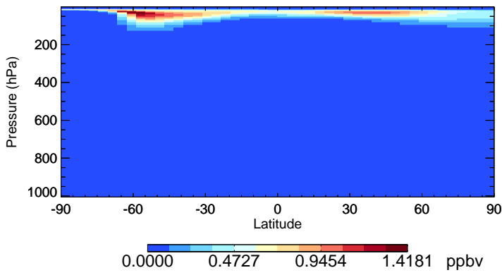
v11-02d-Run1 ClNO3 - Species Zonal Mean for Jul
