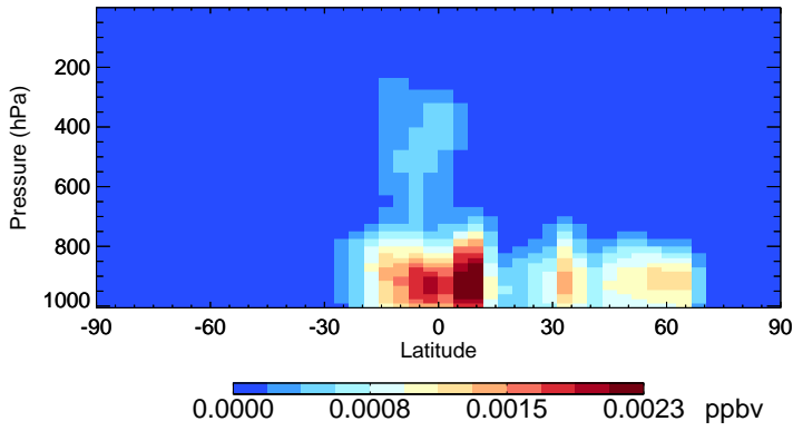
v11-02d-Run1 IEPOXD - Species Zonal Mean for Jul
