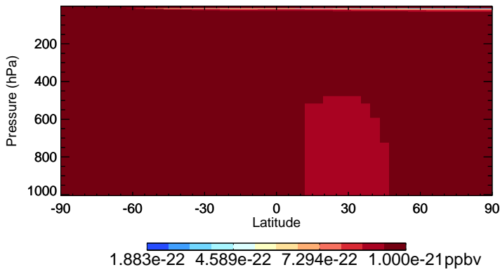
v11-02e-Run0 HCFC123 - Species Zonal Mean for Jul
