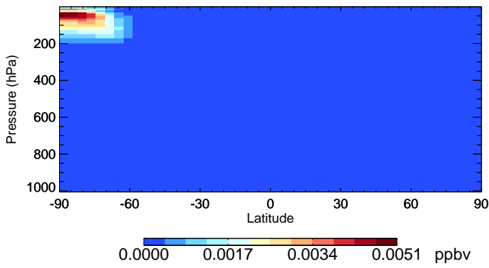
v11-02d-Run1 Br2 - Species Zonal Mean for Jul
