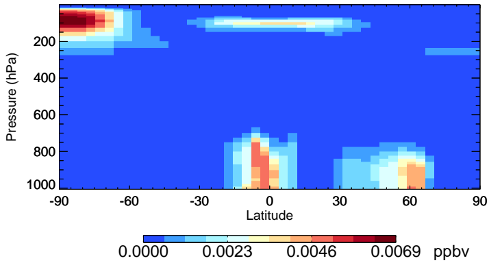
v11-02d-Run1 ISOA3 - Species Zonal Mean for Jul
