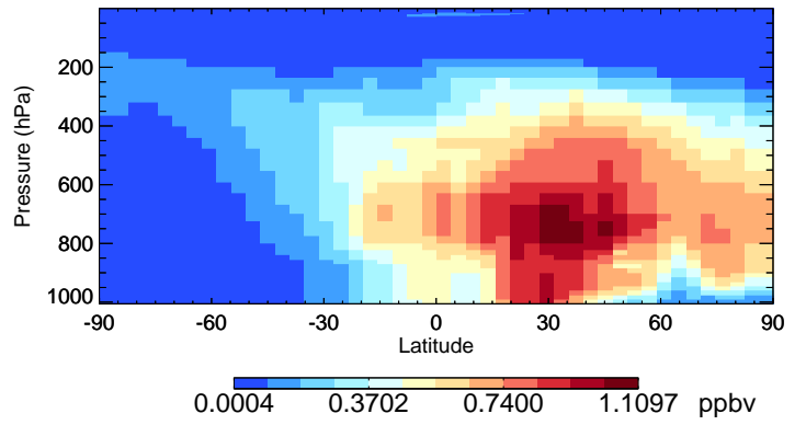
v11-02c-Run0 H2O2 - Species Curtain @ -180.000 for Jul
