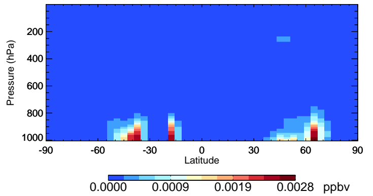
v11-02e-Run0 SOAP - Species Curtain @ -180.000 for Jul
