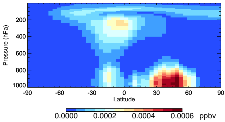
v11-02c-Run0 DHDN - Species Zonal Mean for Jul
