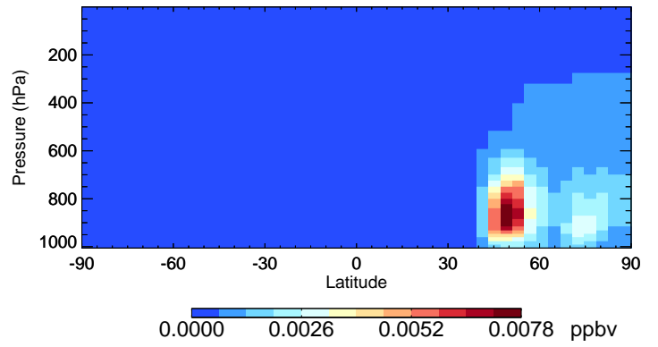
v11-02c-Run0 SOAME - Species Curtain @ -180.000 for Jul
