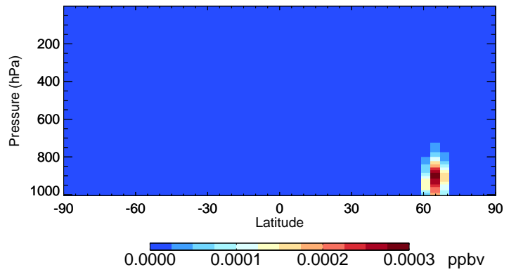
v11-02e-Run0 IEPOXD - Species Curtain @ -180.000 for Jul
