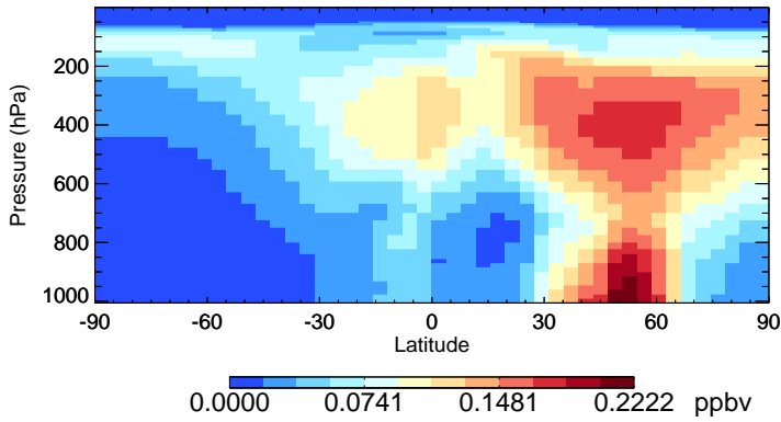
v11-02d-Run1 PAN - Species Zonal Mean for Jul
