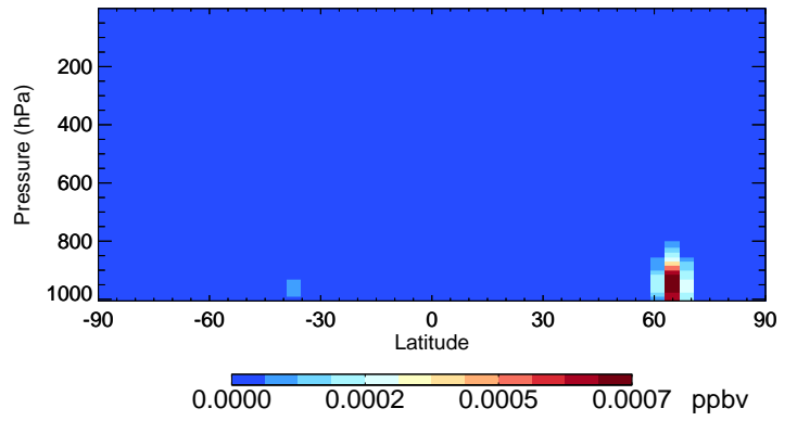
v11-02c-Run0 ISOPNB - Species Curtain @ -180.000 for Jul
