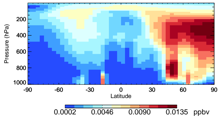
v11-02d-Run1 TSOG3 - Species Curtain @ -180.000 for Jul
