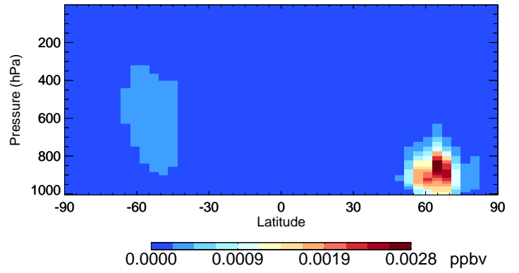
v11-02d-Run1 HC187 - Species Curtain @ -180.000 for Jul
