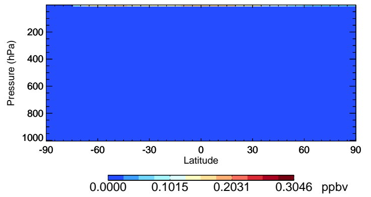
v11-02d-Run1 CI - Species Curtain @ -180.000 for Jul
