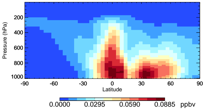
v11-02c-Run0 MAP - Species Zonal Mean for Jul
