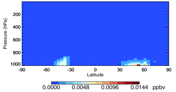
v11-02d-Run1 BCPO - Species Curtain @ -180.000 for Jul
