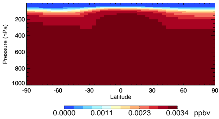
v11-02d-Run1 H1211 - Species Zonal Mean for Jul
