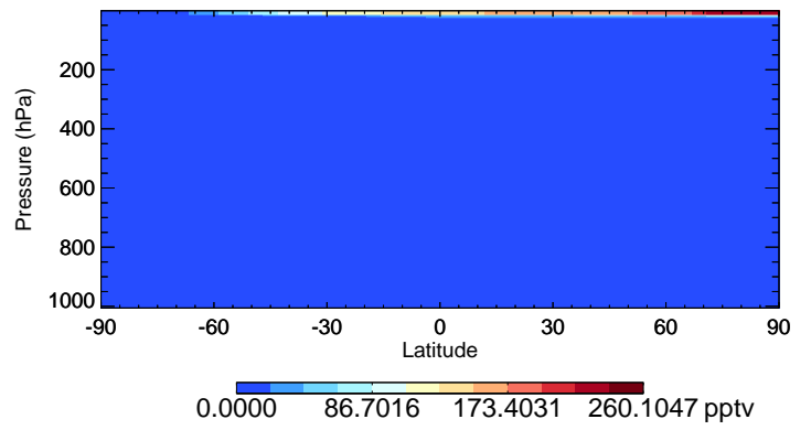
v11-02c-Run0 HO2 - Species Curtain @ -180.000 for Jul
