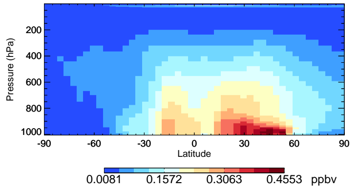
v11-02c-Run0 CH2O - Species Curtain @ -180.000 for Jul
