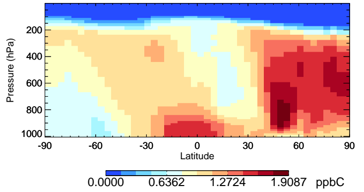
v11-02d-Run1 ACET - Species Curtain @ -180.000 for Jul
