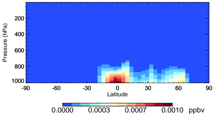
v11-02c-Run0 MOBA - Species Zonal Mean for Jul
