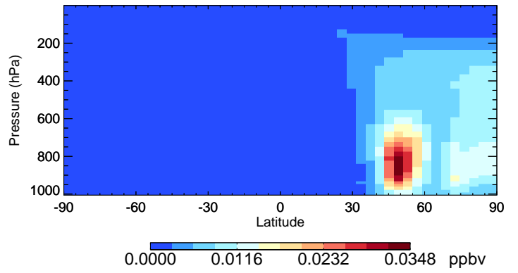
v11-02c-Run0 INDIOL - Species Curtain @ -180.000 for Jul
