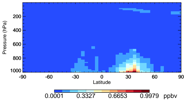
v11-02c-Run0 SO2 - Species Zonal Mean for Jul
