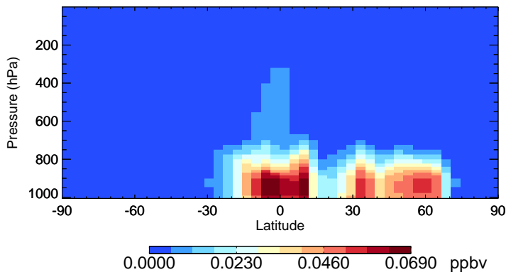
v11-02d-Run1 GLYC - Species Zonal Mean for Jul
