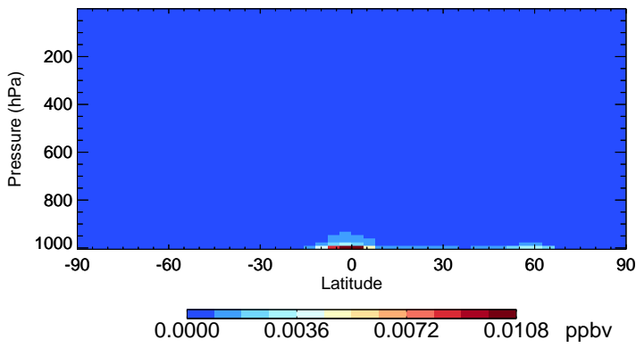
v11-02d-Run1 MTPO - Species Zonal Mean for Jul
