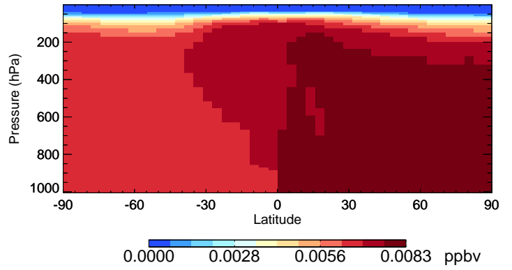
v11-02d-Run1 CH3Br - Species Curtain @ -180.000 for Jul
