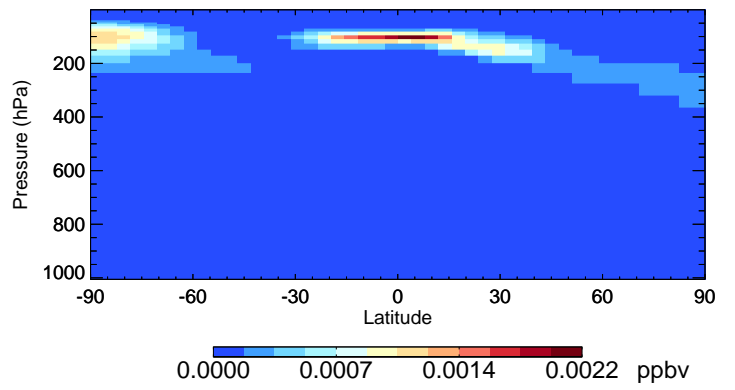
v11-02c-Run0 ASOA3 - Species Curtain @ -180.000 for Jul
