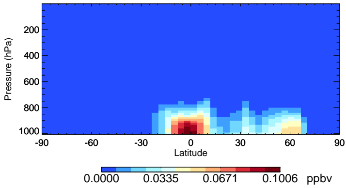
v11-02c-Run0 MACR - Species Zonal Mean for Jul
