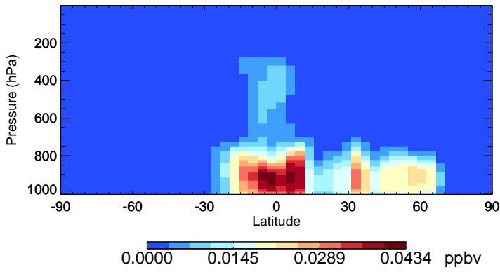
v11-02c-Run0 IEPOXA - Species Zonal Mean for Jul
