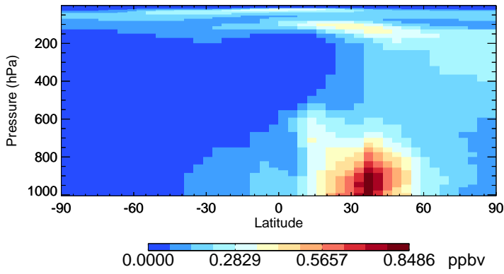
v11-02c-Run0 SO4 - Species Zonal Mean for Jul
