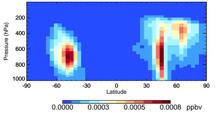
v11-02d-Run1 DST4 - Species Curtain @ -180.000 for Jul
