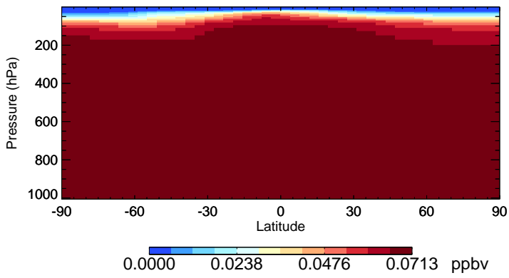
v11-02d-Run1 CFC113 - Species Zonal Mean for Jul
