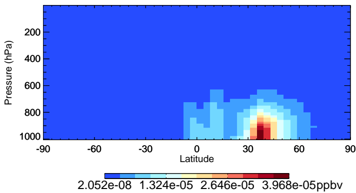
v11-02e-Run0 SOAMG - Species Zonal Mean for Jul
