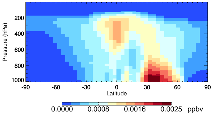
v11-02d-Run1 R4N2 - Species Zonal Mean for Jul
