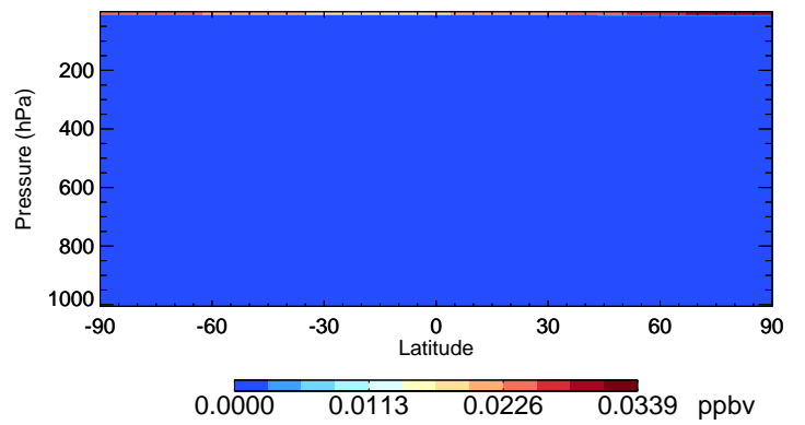
v11-02e-Run0 CI - Species Curtain @ -180.000 for Jul
