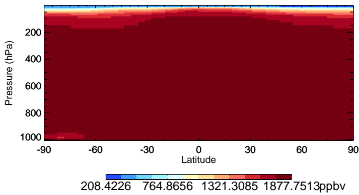
v11-02e-Run0 CH4 - Species Zonal Mean for Jul
