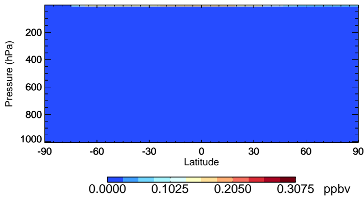
v11-02d-Run1 CI - Species Zonal Mean for Jul
