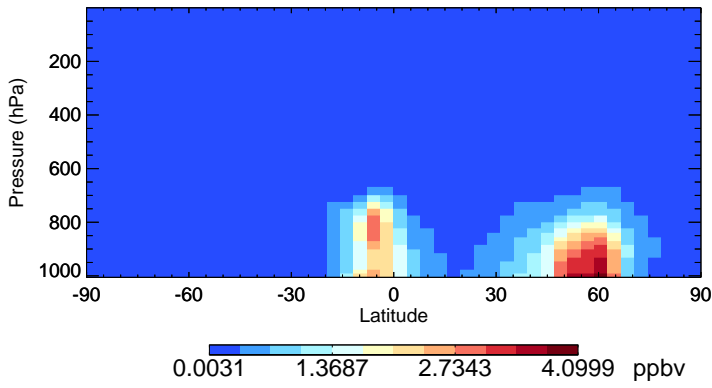
v11-02c-Run0 OCPI - Species Zonal Mean for Jul
