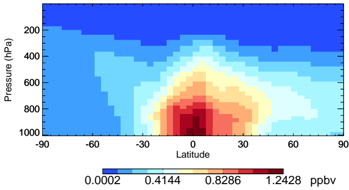
v11-02c-Run0 MP - Species Zonal Mean for Jul
