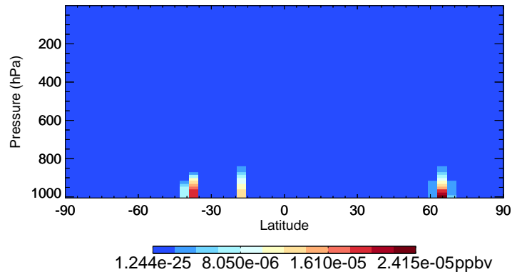
v11-02c-Run0 MONITU - Species Curtain @ -180.000 for Jul
