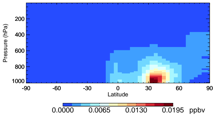
v11-02c-Run0 ASOAN - Species Zonal Mean for Jul
