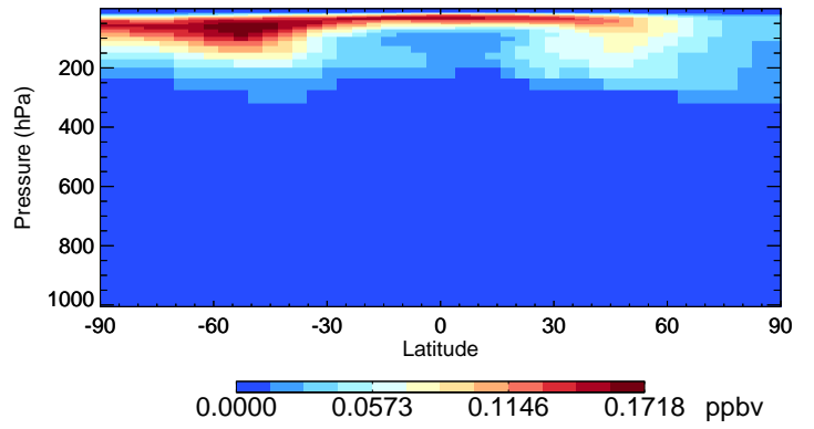
v11-02c-Run0 MPN - Species Curtain @ -180.000 for Jul
