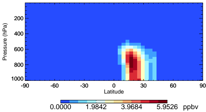
v11-02d-Run1 DST1 - Species Zonal Mean for Jul
