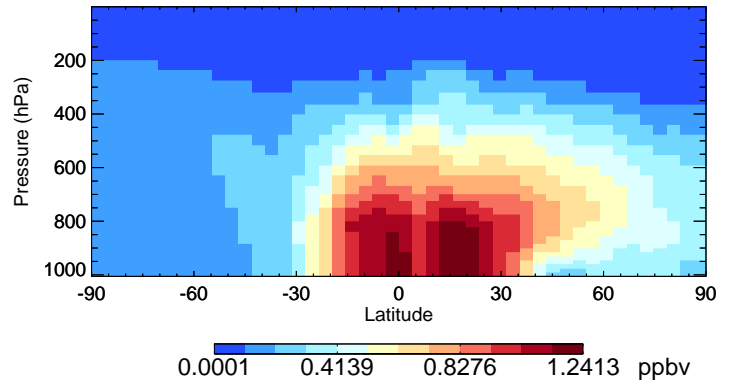
v11-02d-Run1 MP - Species Curtain @ -180.000 for Jul
