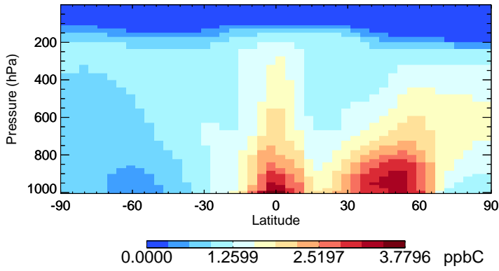
v11-02d-Run1 ACET - Species Zonal Mean for Jul
