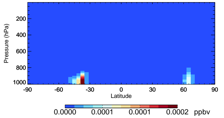
v11-02c-Run0 ISN1 - Species Curtain @ -180.000 for Jul
