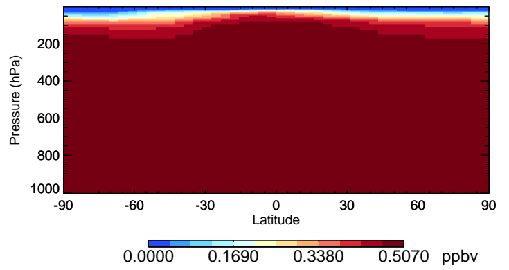
v11-02d-Run1 CFC12 - Species Curtain @ -180.000 for Jul
