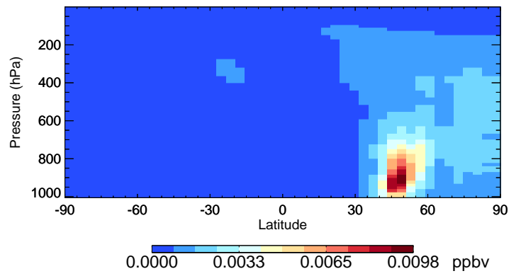
v11-02c-Run0 ASOAN - Species Curtain @ -180.000 for Jul
