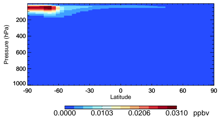
v11-02d-Run1 BrCl - Species Curtain @ -180.000 for Jul
