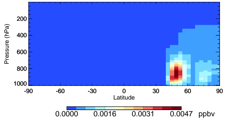
v11-02d-Run1 SOAME - Species Curtain @ -180.000 for Jul
