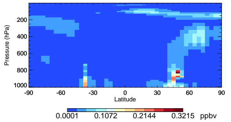
v11-02d-Run1 SO2 - Species Curtain @ -180.000 for Jul
