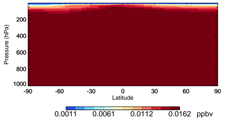
v11-02d-Run1 CFC114 - Species Curtain @ -180.000 for Jul
