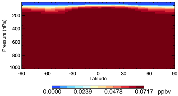
v11-02e-Run0 CCI4 - Species Zonal Mean for Jul
