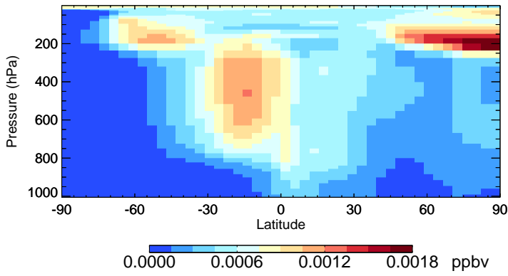
v11-02c-Run0 HBr - Species Zonal Mean for Jul
