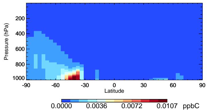
v11-02e-Run0 XYLE - Species Curtain @ -180.000 for Jul
