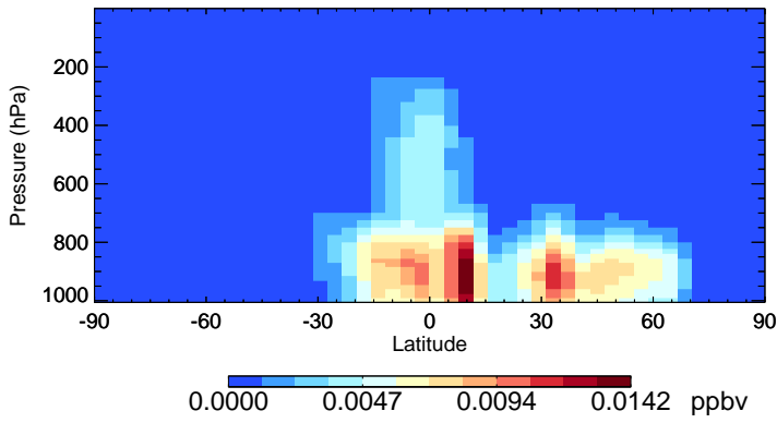
v11-02c-Run0 HC187 - Species Zonal Mean for Jul
