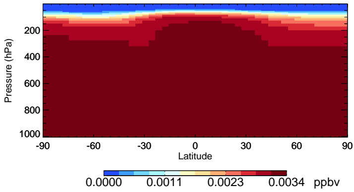
v11-02c-Run0 H1211 - Species Zonal Mean for Jul
