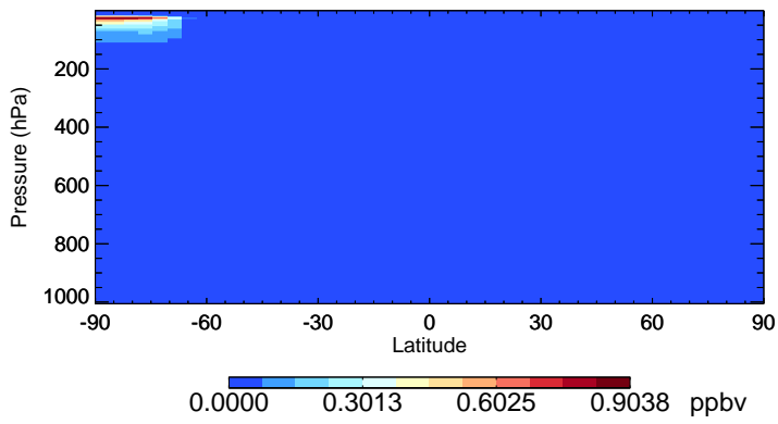
v11-02c-Run0 Cl2 - Species Zonal Mean for Jul
