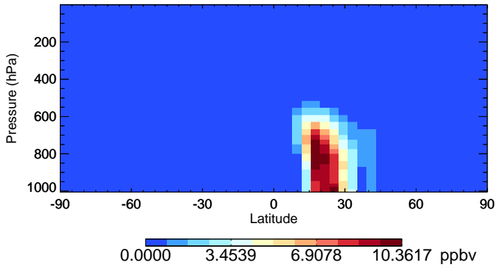
v11-02d-Run1 DST2 - Species Zonal Mean for Jul
