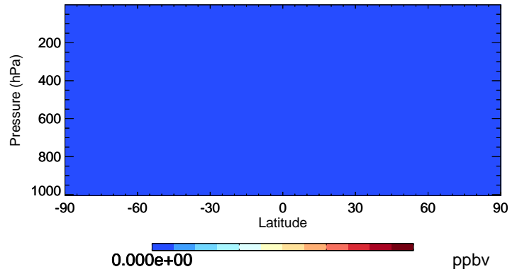
v11-02d-Run1 HCFC123 - Species Curtain @ -180.000 for Jul
