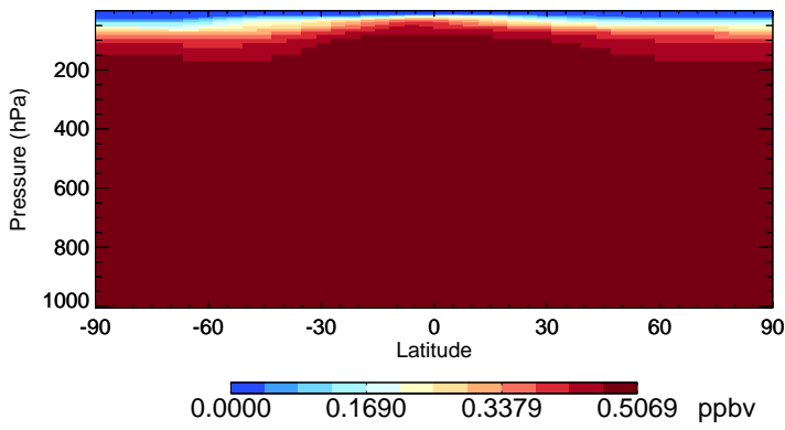
v11-02d-Run1 CFC12 - Species Zonal Mean for Jul
