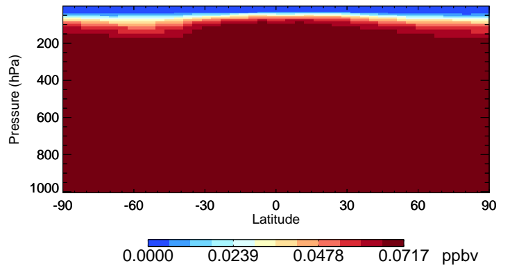
v11-02e-Run0 CCI4 - Species Curtain @ -180.000 for Jul
