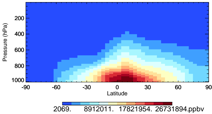
v11-02c-Run0 H2O - Species Zonal Mean for Jul
