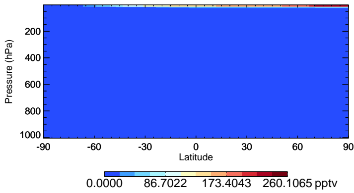
v11-02c-Run0 HO2 - Species Zonal Mean for Jul
