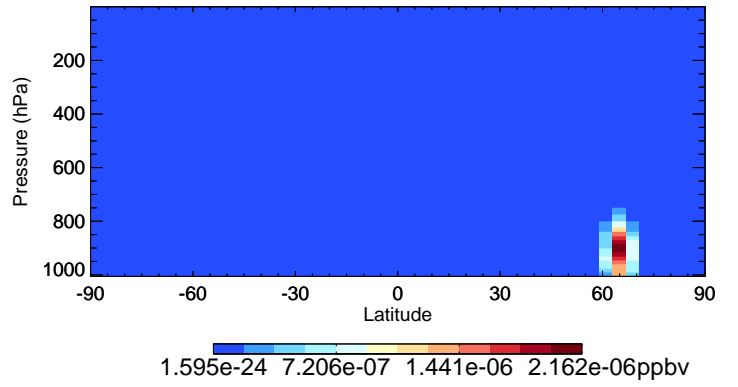
v11-02d-Run1 LVOC - Species Curtain @ -180.000 for Jul
