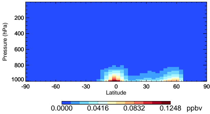
v11-02d-Run1 RCHO - Species Zonal Mean for Jul
