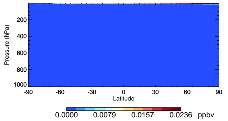
v11-02c-Run0 Br - Species Curtain @ -180.000 for Jul
