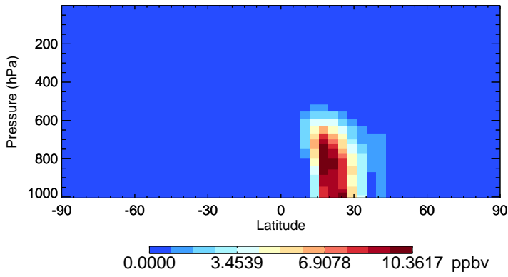
v11-02c-Run0 DST2 - Species Zonal Mean for Jul
