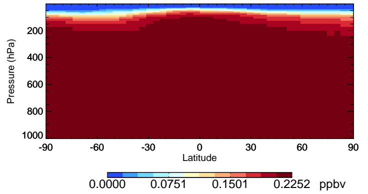
v11-02c-Run0 CFC11 - Species Curtain @ -180.000 for Jul
