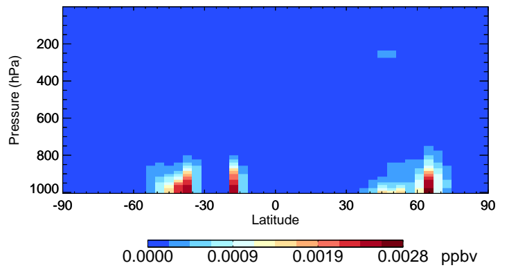
v11-02d-Run1 SOAP - Species Curtain @ -180.000 for Jul
