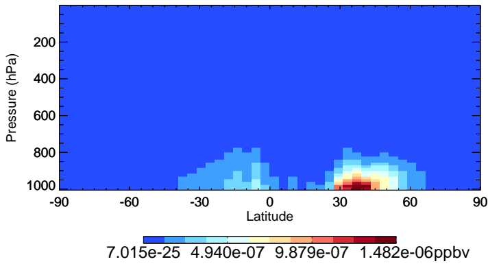
v11-02c-Run0 NPMN - Species Zonal Mean for Jul
