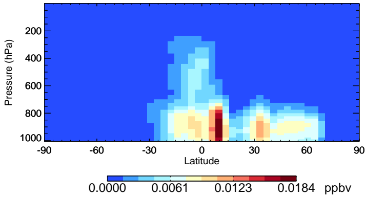
v11-02d-Run1 HC187 - Species Zonal Mean for Jul
