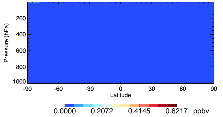
v11-02d-Run1 NO3 - Species Curtain @ -180.000 for Jul
