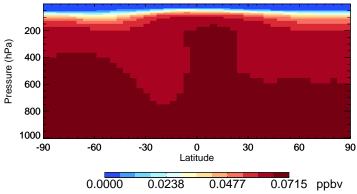
v11-02c-Run0 CCI4 - Species Zonal Mean for Jul
