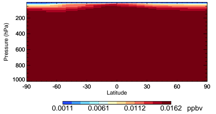
v11-02c-Run0 CFC114 - Species Curtain @ -180.000 for Jul
