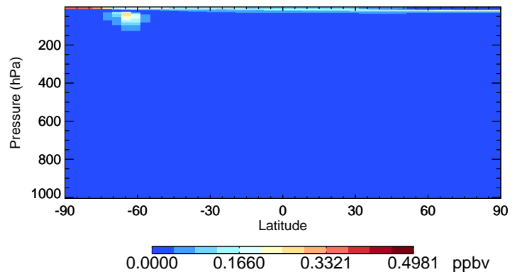
v11-02c-Run0 CIO - Species Curtain @ -180.000 for Jul
