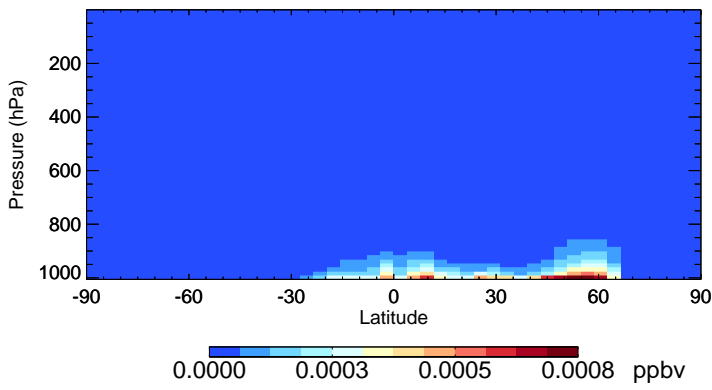
v11-02d-Run1 MONITU - Species Zonal Mean for Jul
