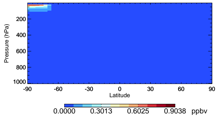
v11-02c-Run0 Cl2 - Species Curtain @ -180.000 for Jul
