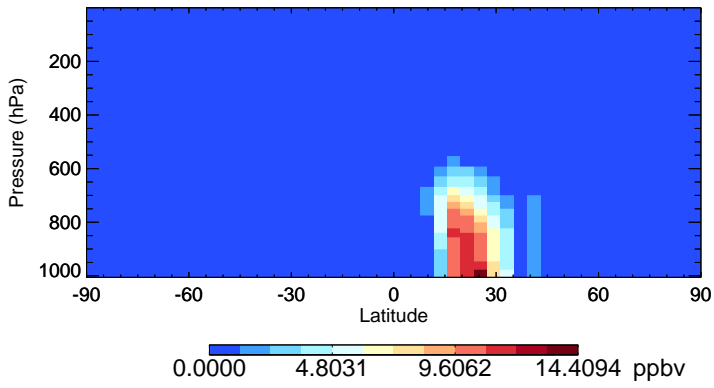
v11-02c-Run0 DST4 - Species Zonal Mean for Jul
