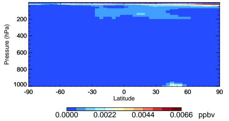
v11-02c-Run0 HNO2 - Species Curtain @ -180.000 for Jul
