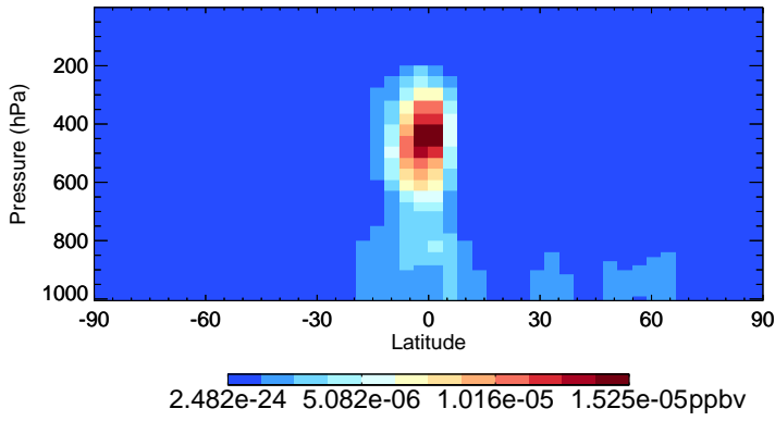
v11-02d-Run1 LVOC - Species Zonal Mean for Jul
