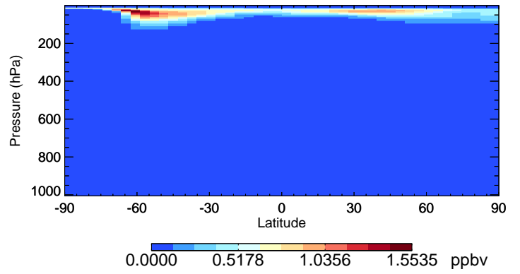
v11-02c-Run0 ClNO3 - Species Curtain @ -180.000 for Jul
