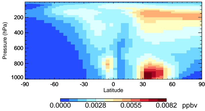
v11-02d-Run1 ASOG3 - Species Zonal Mean for Jul
