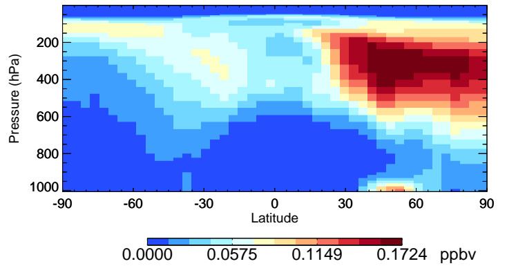
v11-02c-Run0 PAN - Species Curtain @ -180.000 for Jul
