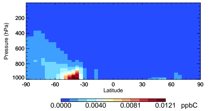
v11-02d-Run1 XYLE - Species Curtain @ -180.000 for Jul
