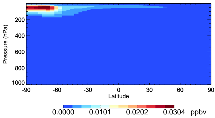
v11-02d-Run1 BrCl - Species Zonal Mean for Jul
