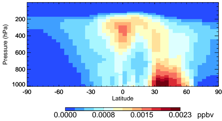
v11-02c-Run0 R4N2 - Species Zonal Mean for Jul
