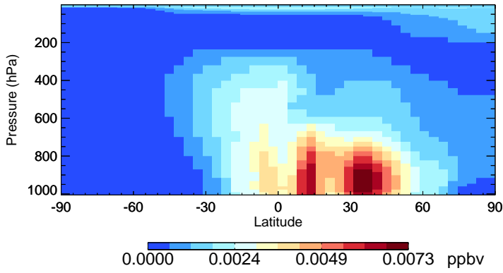
v11-02d-Run1 ISOG1 - Species Zonal Mean for Jul
