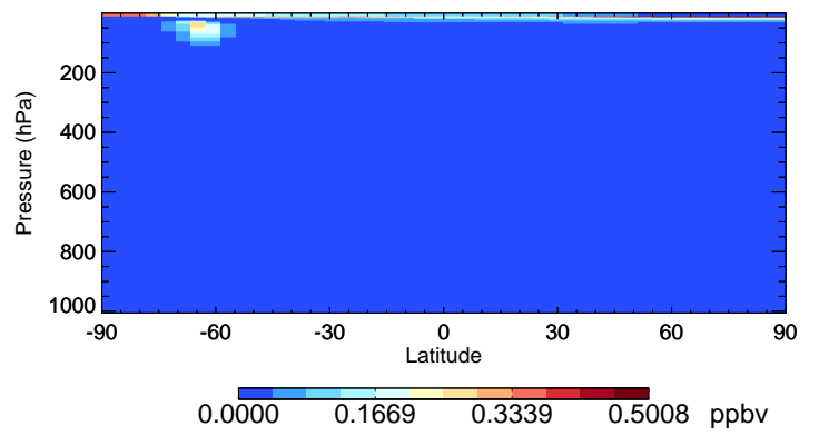
v11-02d-Run1 CIO - Species Curtain @ -180.000 for Jul
