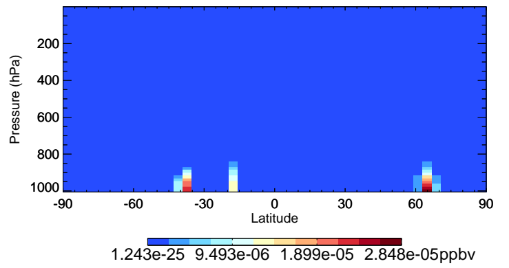
v11-02d-Run1 MONITU - Species Curtain @ -180.000 for Jul
