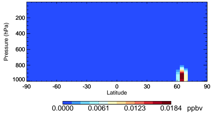
v11-02d-Run1 MACR - Species Curtain @ -180.000 for Jul
