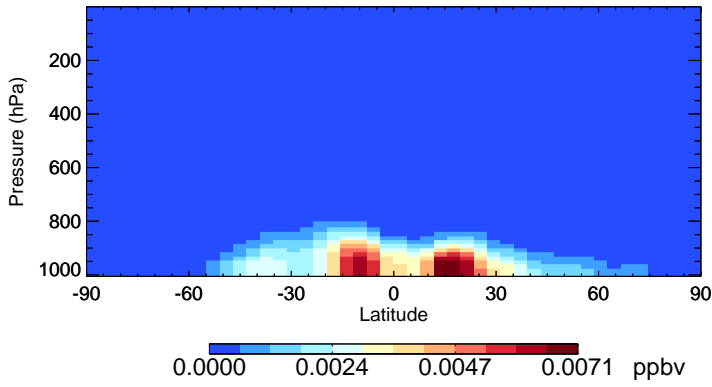
v11-02d-Run1 NITs - Species Zonal Mean for Jul
