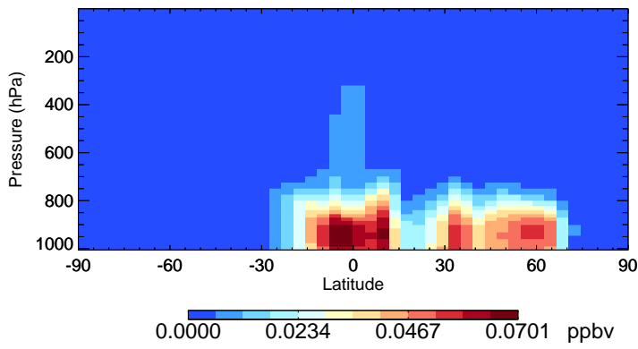
v11-02c-Run0 GLYC - Species Zonal Mean for Jul
