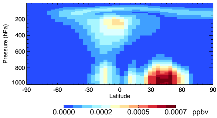
v11-02d-Run1 DHDN - Species Zonal Mean for Jul
