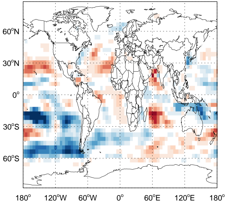
v11-02f-Run0 - v11-02e-Run0 SALC: Column AOD diff for Jul
