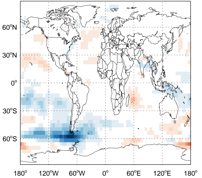
v11-02f-Run0 - v11-02e-Run0 SALA: Column AOD diff for Jul
