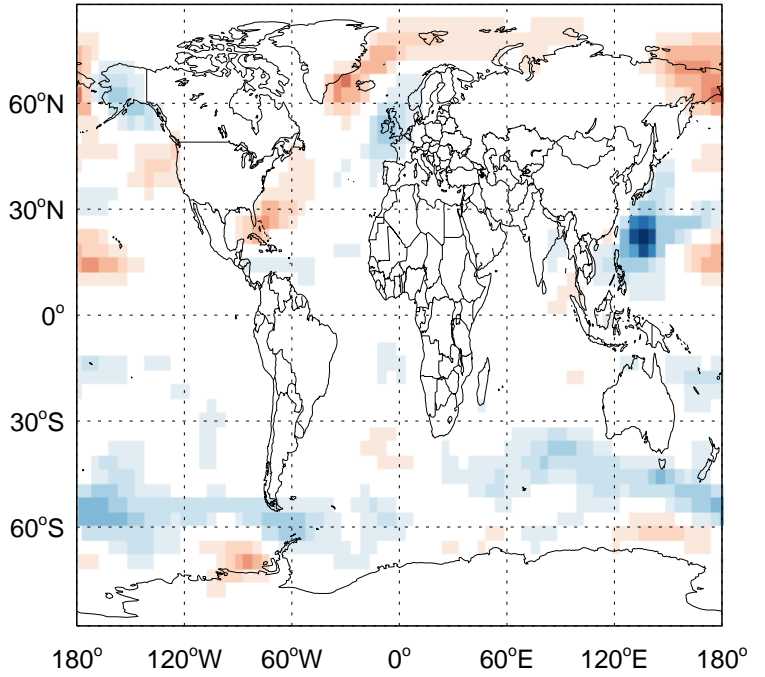
v11-02f-Run0 - v11-02e-Run0 SALA: Column AOD diff for Oct
