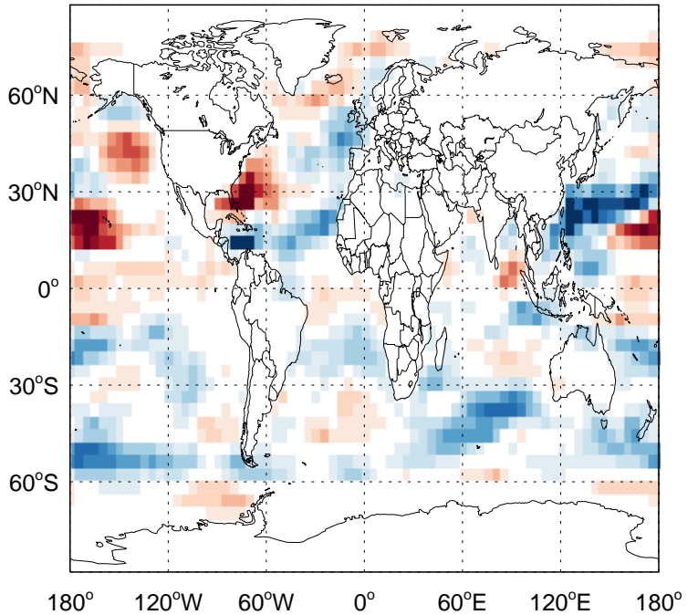
v11-02f-Run0 - v11-02e-Run0 SALC: Column AOD diff for Oct
