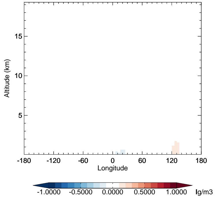
v11-02f-Run0 - v11-02e-Run1 BCPI - Diff along 42N for Apr
