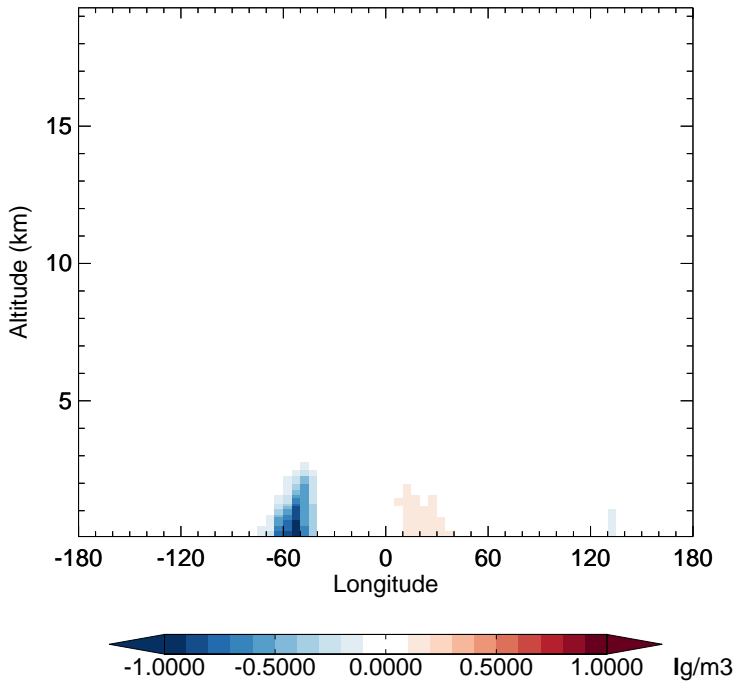
v11-02f-Run0 - v11-02e-Run1 SOAS - Diff along 15S for Apr
