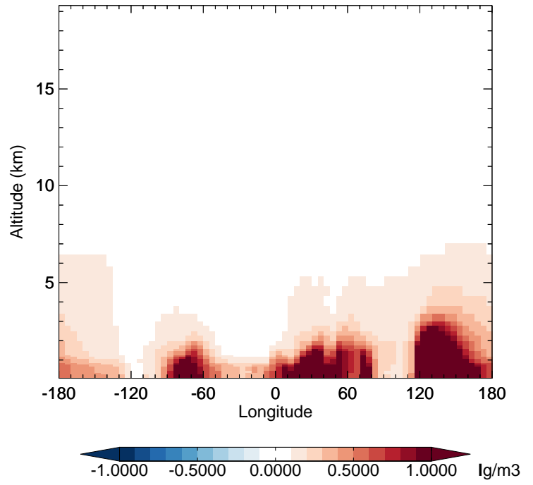
v11-02f-Run0 - v11-02e-Run1 NH4 - Diff along 42N for Apr
