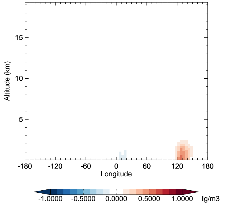
v11-02f-Run0 - v11-02e-Run0 BCPI - Diff along 42N for Apr
