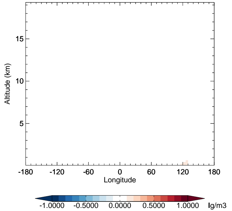
v11-02f-Run0 - v11-02e-Run0 BCPO - Diff along 42N for Apr
