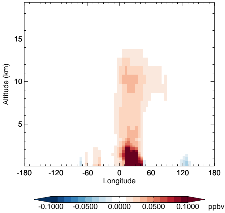
v11-02f-Run0 - v11-02e-Run1 BENZ - Diff along 15S for Apr
