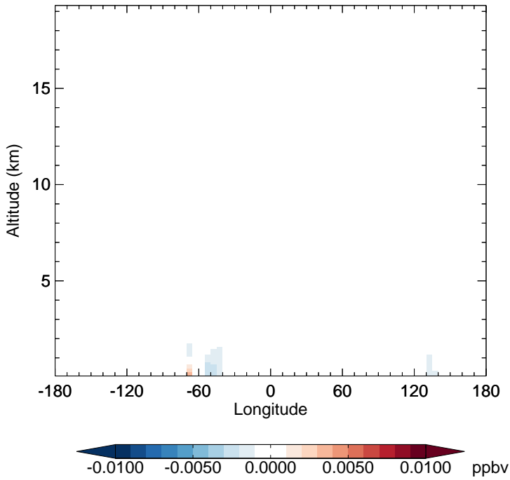
v11-02f-Run0 - v11-02e-Run0 MOBA - Diff along 15S for Apr
