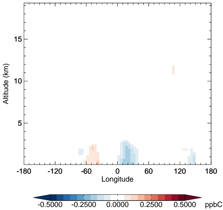
v11-02f-Run0 - v11-02e-Run0 C3H8 - Diff along 15S for Apr
