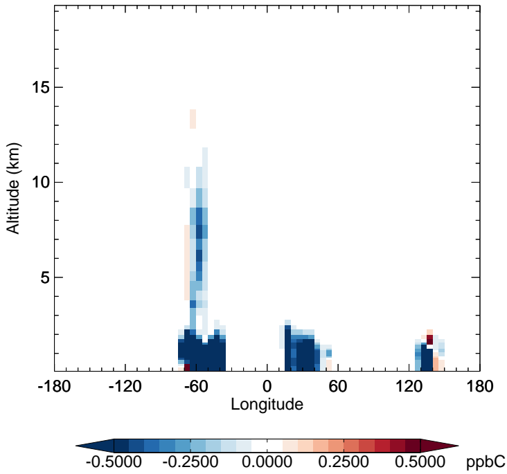
v11-02f-Run0 - v11-02e-Run0 ISOP - Diff along 15S for Apr
