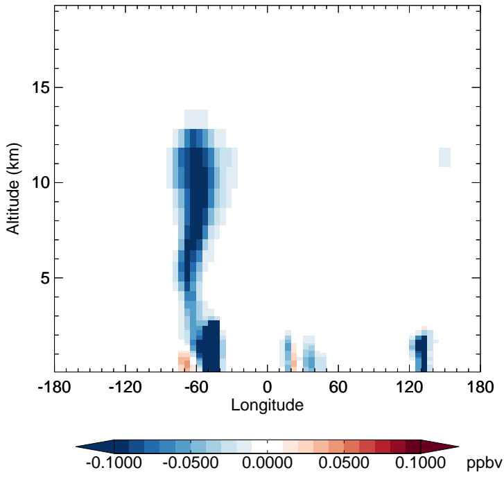
v11-02f-Run0 - v11-02e-Run1 IEPOXA - Diff along 15S for Apr
