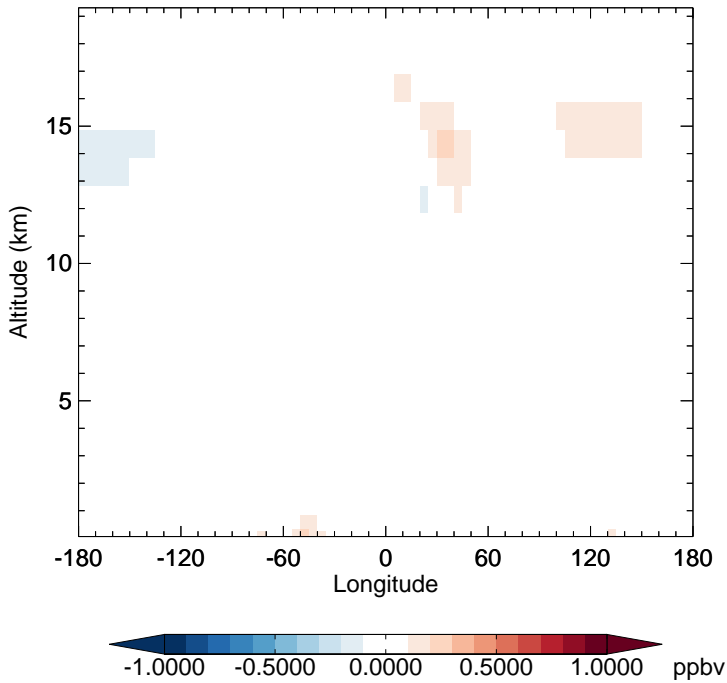
v11-02f-Run0 - v11-02e-Run0 NO 2 - Diff along 15S for Apr
