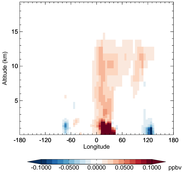
v11-02f-Run0 - v11-02e-Run0 BENZ - Diff along 15S for Apr
