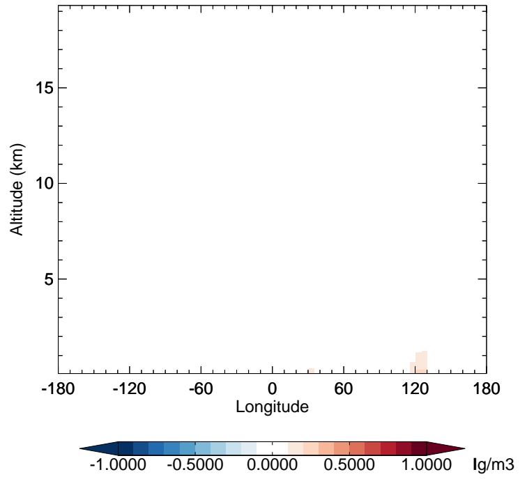
v11-02f-Run0 - v11-02e-Run1 OCPO - Diff along 42N for Apr
