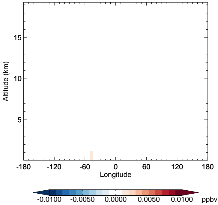
v11-02f-Run0 - v11-02e-Run1 NO3 - Diff along 15S for Apr
