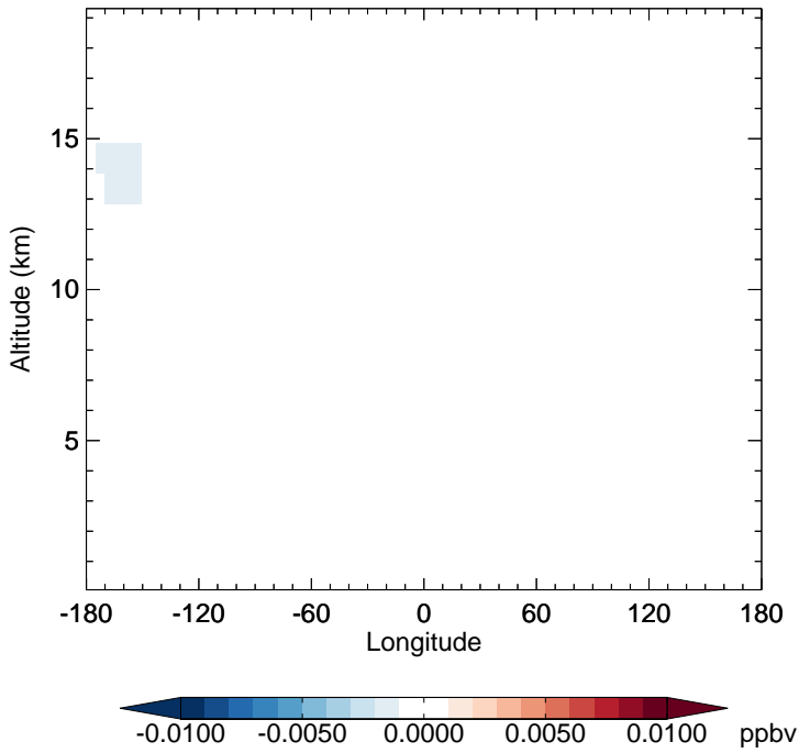
v11-02f-Run0 - v11-02e-Run0 BrNO3 - Diff along 15S for Apr
