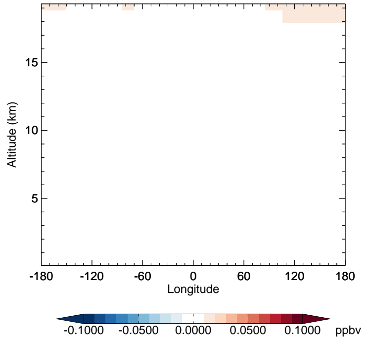
v11-02f-Run0 - v11-02e-Run0 ClO - Diff along 42N for Apr
