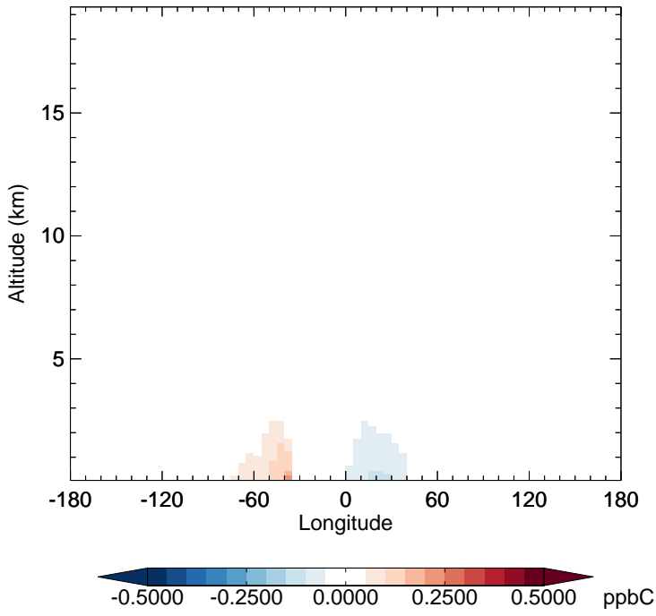
v11-02f-Run0 - v11-02e-Run1 C3H8 - Diff along 15S for Apr
