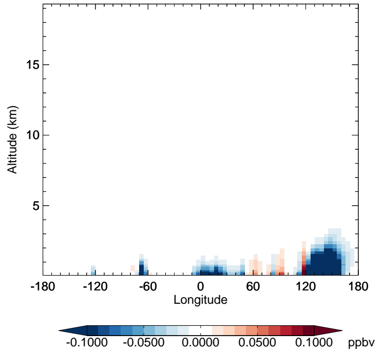
v11-02f-Run0 - v11-02e-Run1 XYLE - Diff along 42N for Apr
