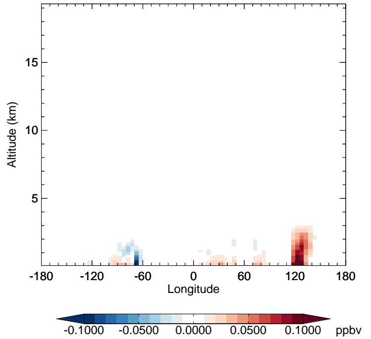
v11-02f-Run0 - v11-02e-Run0 SOAP - Diff along 42N for Apr
