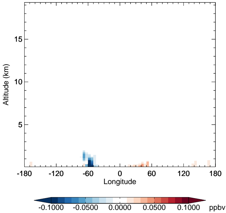
v11-02f-Run0 - v11-02e-Run0 MTPA - Diff along 15S for Apr
