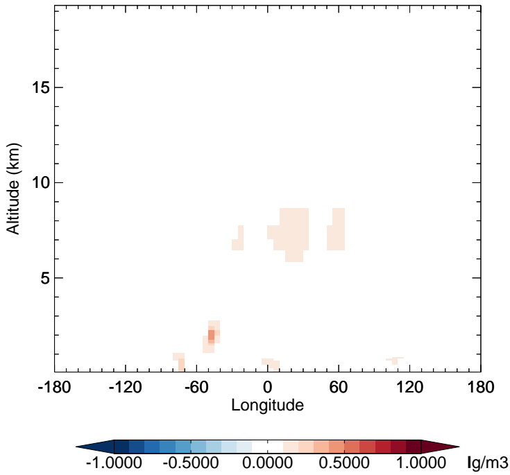
v11-02f-Run0 - v11-02e-Run0 NIT - Diff along 15S for Apr
