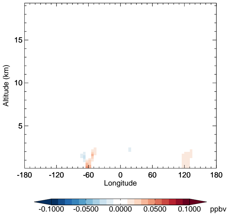
v11-02f-Run0 - v11-02e-Run0 TSOA0 - Diff along 15S for Apr
