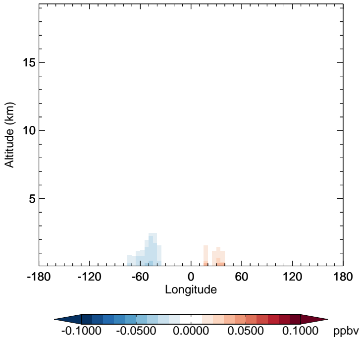
v11-02f-Run0 - v11-02e-Run1 SOAP - Diff along 15S for Apr
