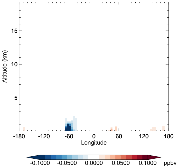
v11-02f-Run0 - v11-02e-Run1 MTPA - Diff along 15S for Apr
