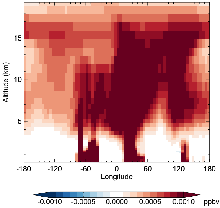
v11-02f-Run0 - v11-02e-Run1 PPN - Diff along 15S for Apr
