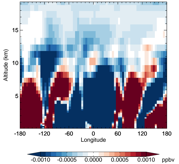
v11-02f-Run0 - v11-02e-Run0 PPN - Diff along 42N for Apr
