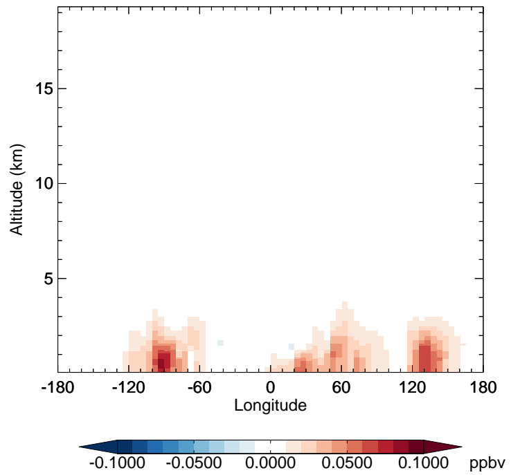
v11-02f-Run0 - v11-02e-Run0 INDIOL - Diff along 42N for Apr
