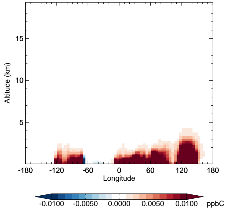
v11-02f-Run0 - v11-02e-Run1 PRPE - Diff along 42N for Apr
