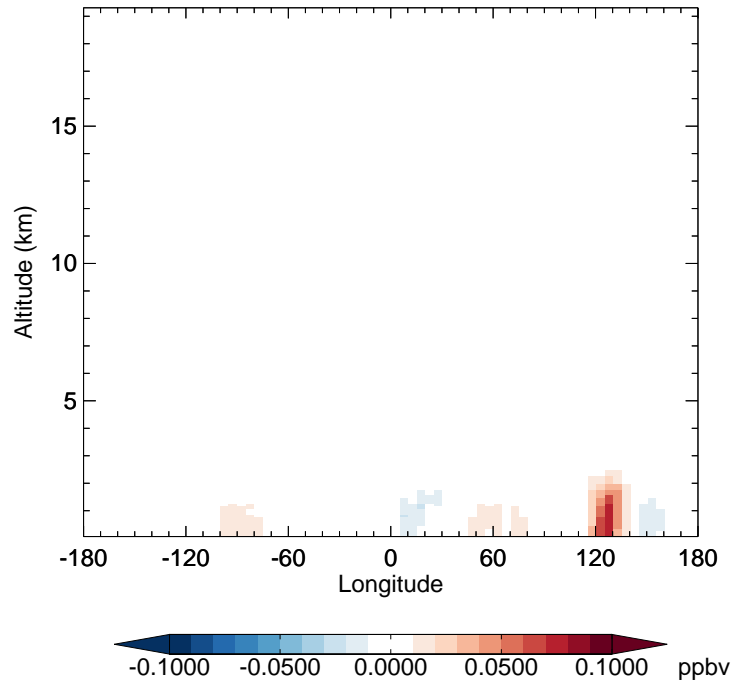
v11-02f-Run0 - v11-02e-Run0 SOAGX - Diff along 42N for Apr
