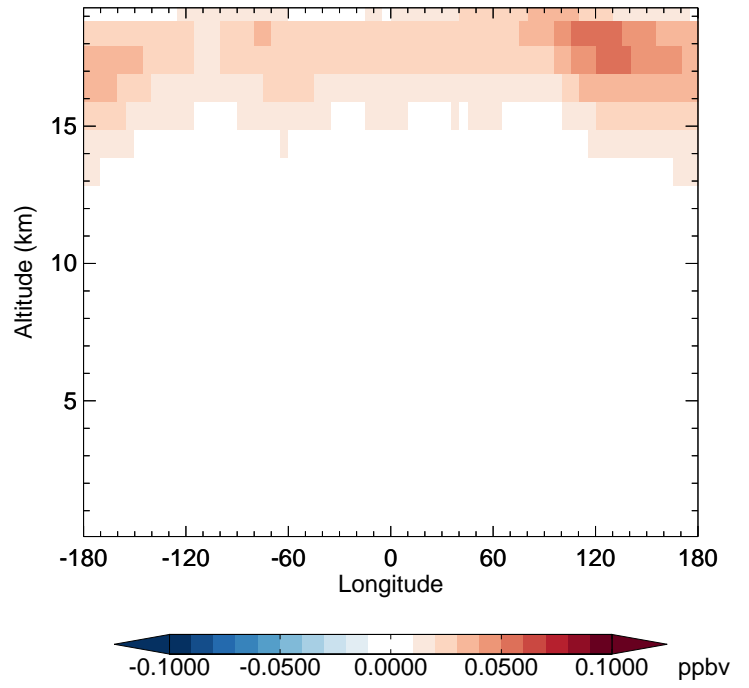
v11-02f-Run0 - v11-02e-Run1 HCl - Diff along 42N for Apr
