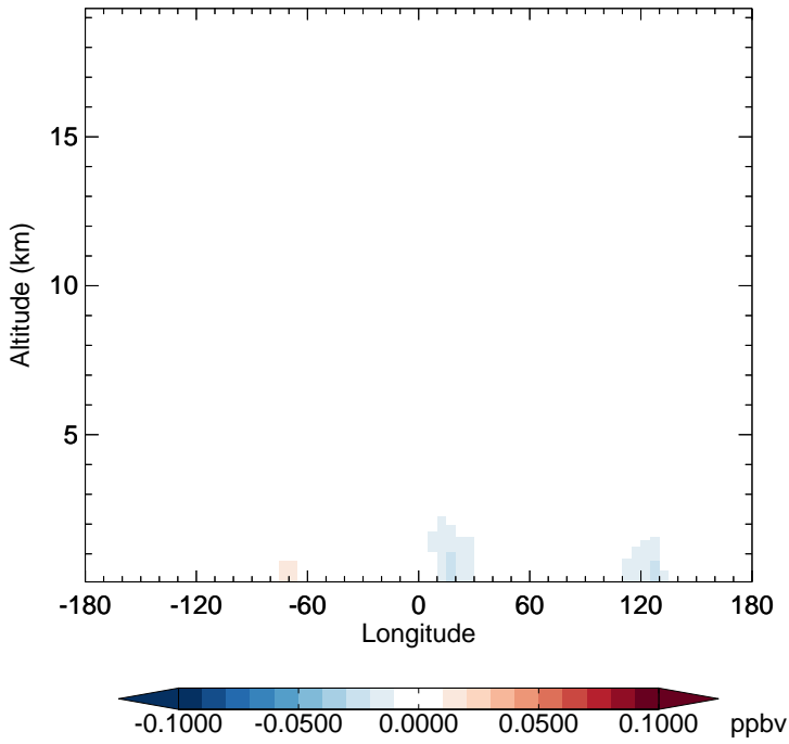
v11-02f-Run0 - v11-02e-Run1 SOAGX - Diff along 15S for Apr
