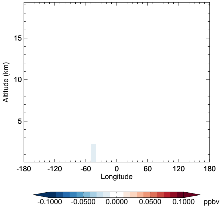
v11-02f-Run0 - v11-02e-Run1 ISOPNB - Diff along 15S for Apr
