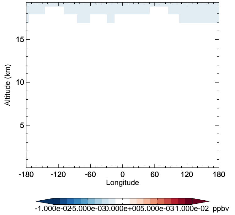
v11-02f-Run0 - v11-02e-Run1 BrNO3 - Diff along 42N for Apr
