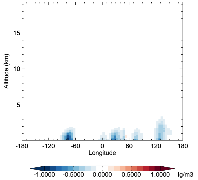
v11-02f-Run0 - v11-02e-Run1 SO 2 - Diff along 42N for Apr
