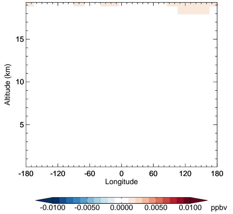
v11-02f-Run0 - v11-02e-Run1 BrO - Diff along 42N for Apr
