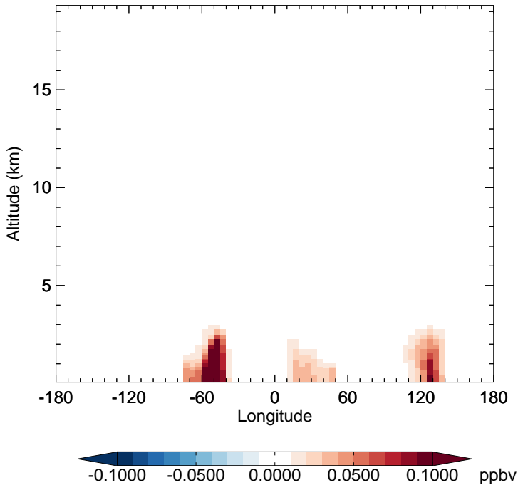
v11-02f-Run0 - v11-02e-Run1 INDIOL - Diff along 15S for Apr
