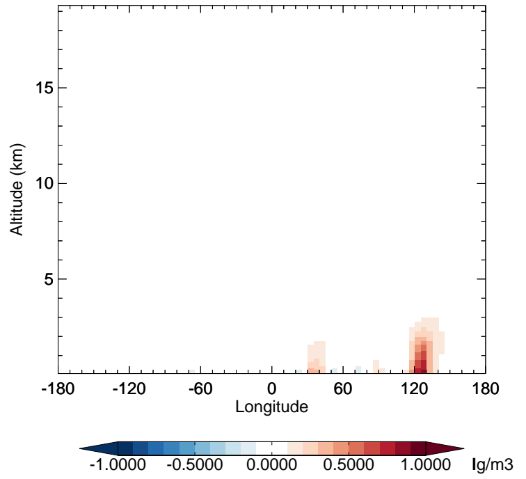
v11-02f-Run0 - v11-02e-Run1 OCPI - Diff along 42N for Apr
