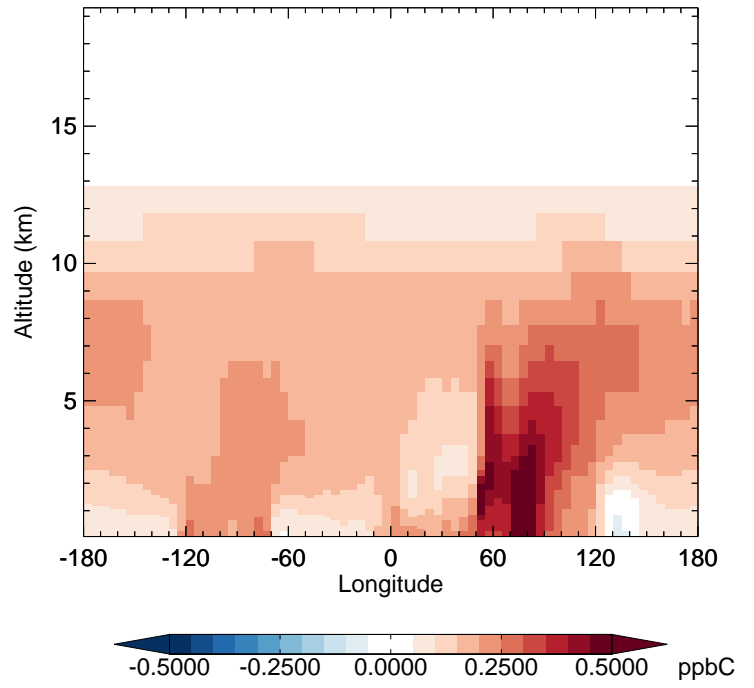
v11-02f-Run0 - v11-02e-Run1 ACET - Diff along 42N for Apr
