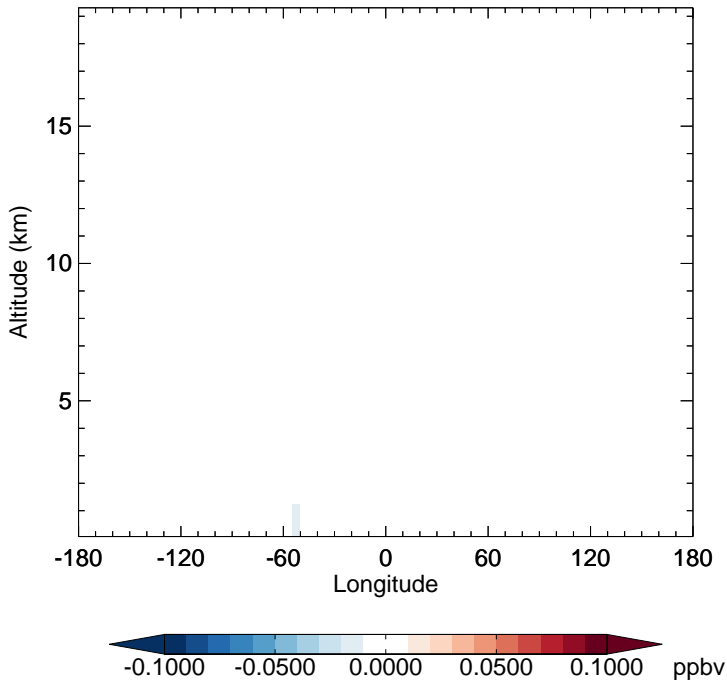
v11-02f-Run0 - v11-02e-Run1 TSOA1 - Diff along 15S for Apr
