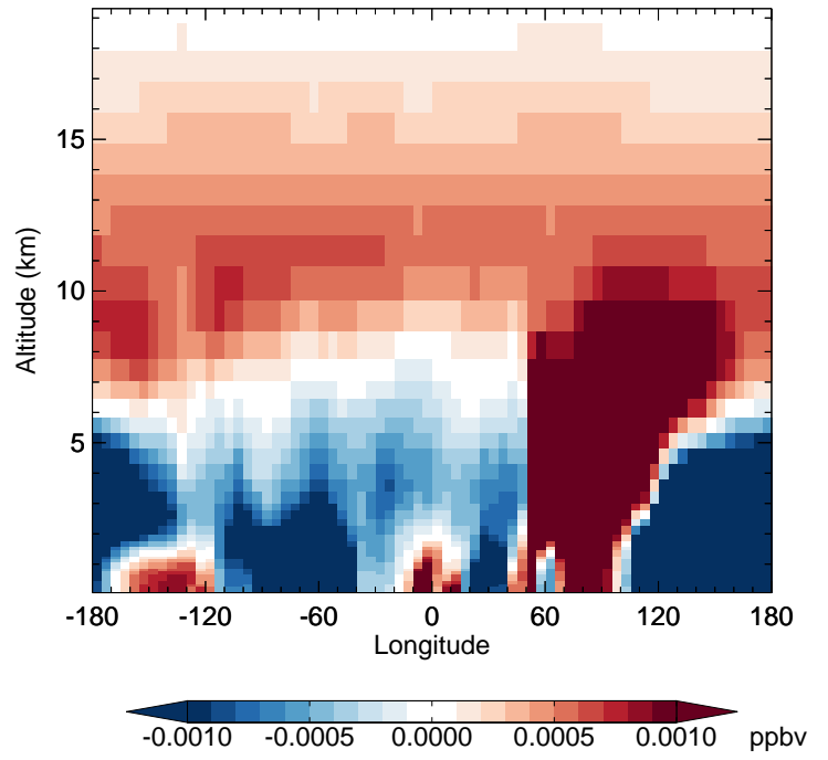
v11-02f-Run0 - v11-02e-Run1 PPN - Diff along 42N for Apr
