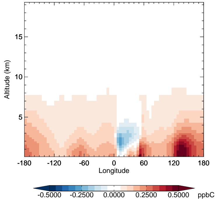
v11-02f-Run0 - v11-02e-Run1 C3H8 - Diff along 42N for Apr
