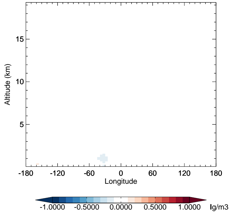
v11-02f-Run0 - v11-02e-Run0 DMS - Diff along 42N for Apr
