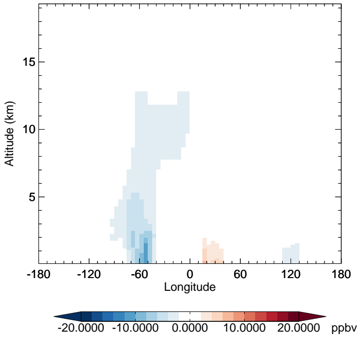
v11-02f-Run0 - v11-02e-Run1 CO - Diff along 15S for Apr
