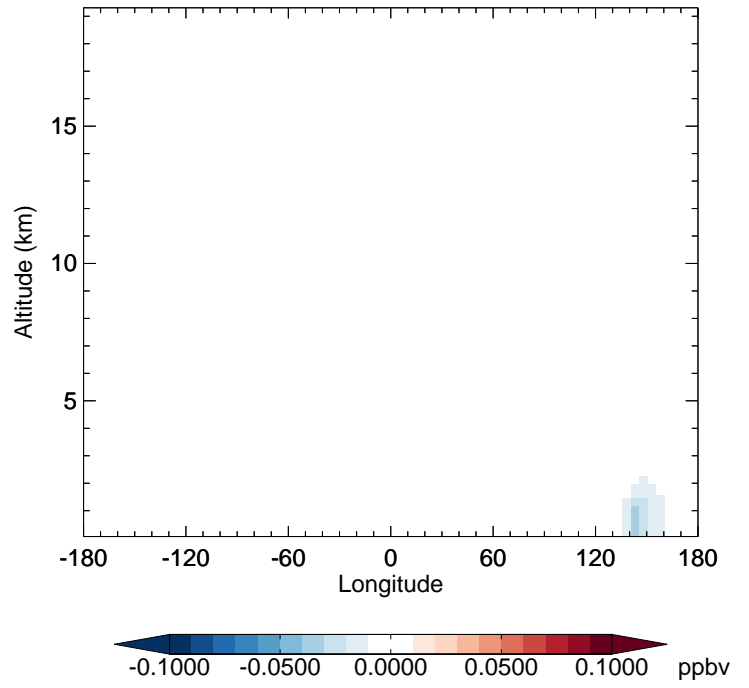
v11-02f-Run0 - v11-02e-Run1 ASOAN - Diff along 42N for Apr
