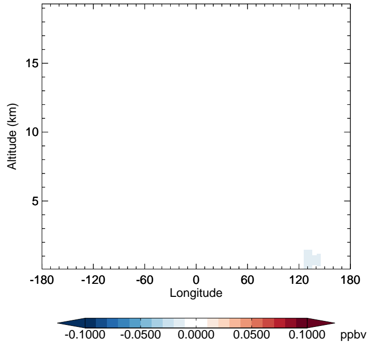
v11-02f-Run0 - v11-02e-Run1 ASOG3 - Diff along 42N for Apr
