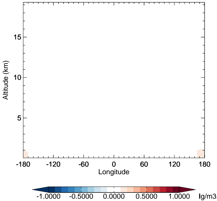
v11-02f-Run0 - v11-02e-Run0 DMS - Diff along 15S for Apr
