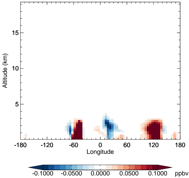
v11-02f-Run0 - v11-02e-Run0 TSOG3 - Diff along 15S for Apr
