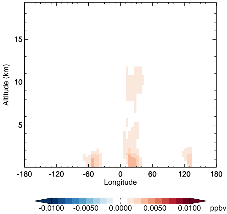
v11-02f-Run0 - v11-02e-Run1 R4N2 - Diff along 15S for Apr
