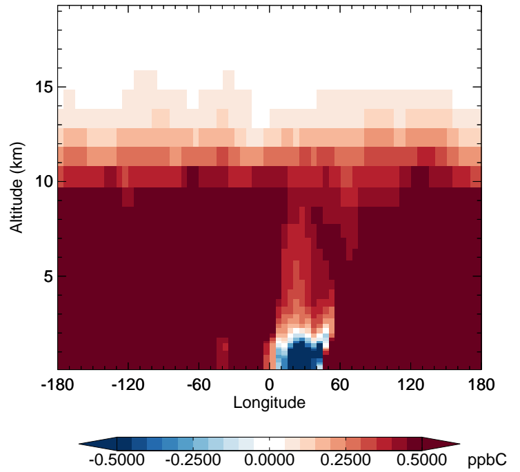
v11-02f-Run0 - v11-02e-Run0 C2H6 - Diff along 42N for Apr
