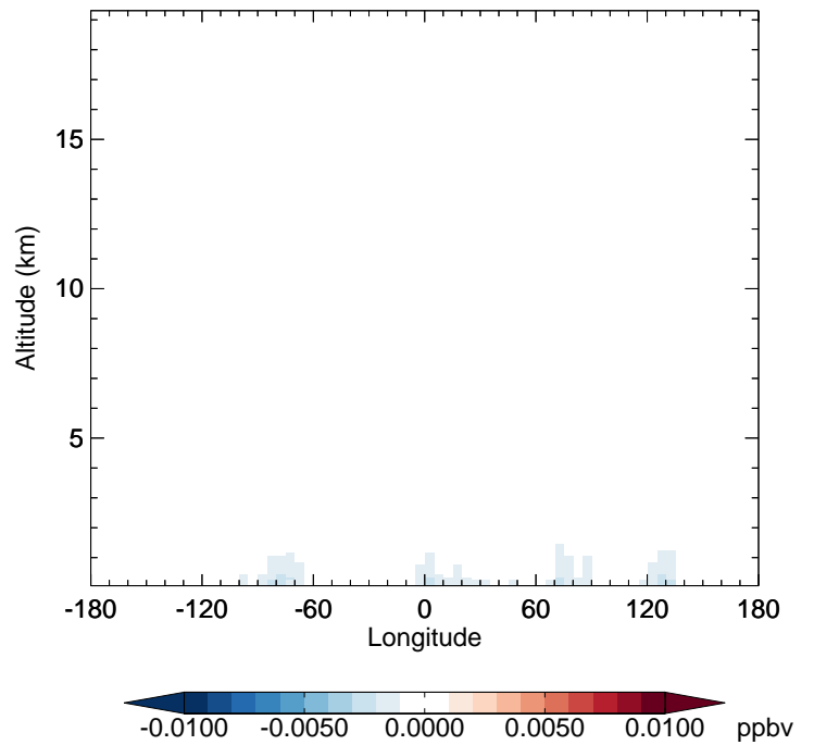
v11-02f-Run0 - v11-02e-Run0 NO3 - Diff along 42N for Apr
