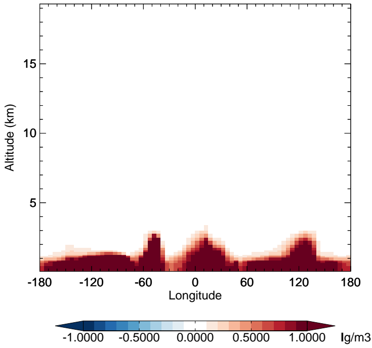
v11-02f-Run0 - v11-02e-Run1 NH3 - Diff along 15S for Apr
