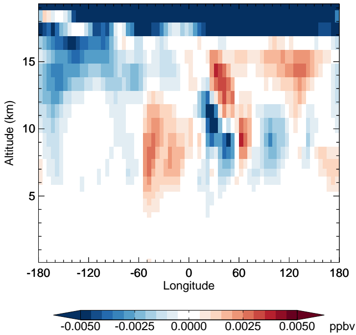
v11-02f-Run0 - v11-02e-Run0 N2O5 - Diff along 15S for Apr
