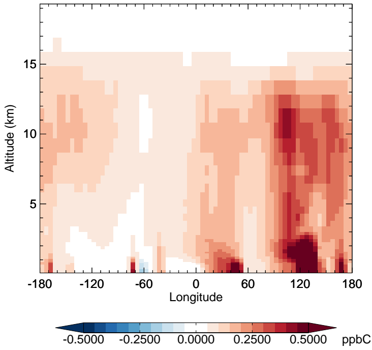
v11-02f-Run0 - v11-02e-Run1 ACET - Diff along 15S for Apr
