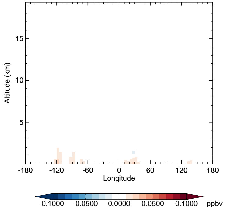
v11-02f-Run0 - v11-02e-Run0 TSOG3 - Diff along 42N for Apr
