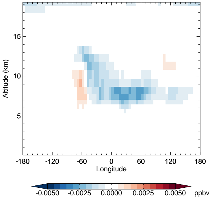
v11-02f-Run0 - v11-02e-Run1 HNO 4 - Diff along 15S for Apr
