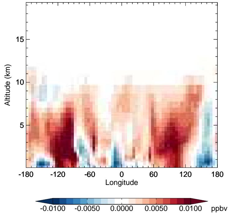
v11-02f-Run0 - v11-02e-Run0 MAP - Diff along 42N for Apr
