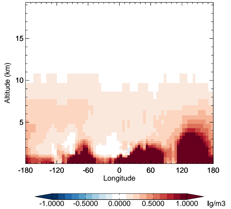
v11-02f-Run0 - v11-02e-Run0 NIT - Diff along 42N for Apr
