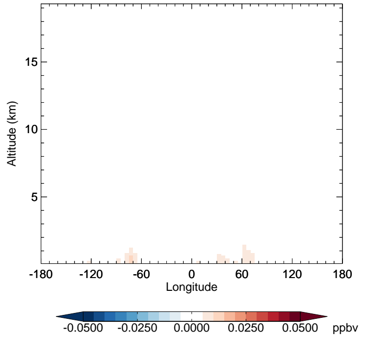
v11-02f-Run0 - v11-02e-Run1 MVK - Diff along 42N for Apr
