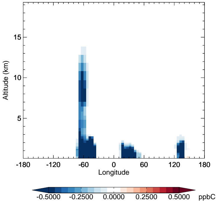
v11-02f-Run0 - v11-02e-Run1 ISOP - Diff along 15S for Apr
