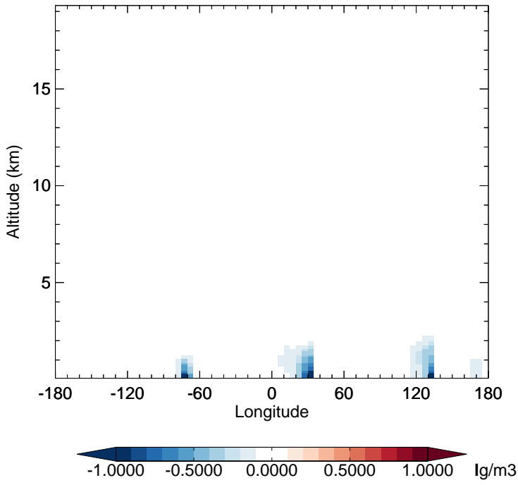
v11-02f-Run0 - v11-02e-Run1 SO 2 - Diff along 15S for Apr
