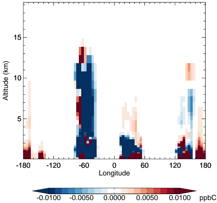
v11-02f-Run0 - v11-02e-Run0 PRPE - Diff along 15S for Apr
