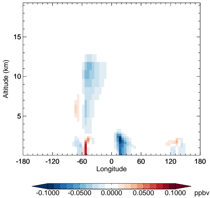
v11-02f-Run0 - v11-02e-Run0 IMAE - Diff along 15S for Apr
