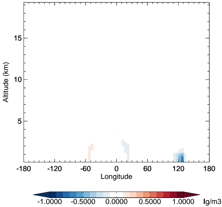
v11-02f-Run0 - v11-02e-Run0 OCPI - Diff along 15S for Apr
