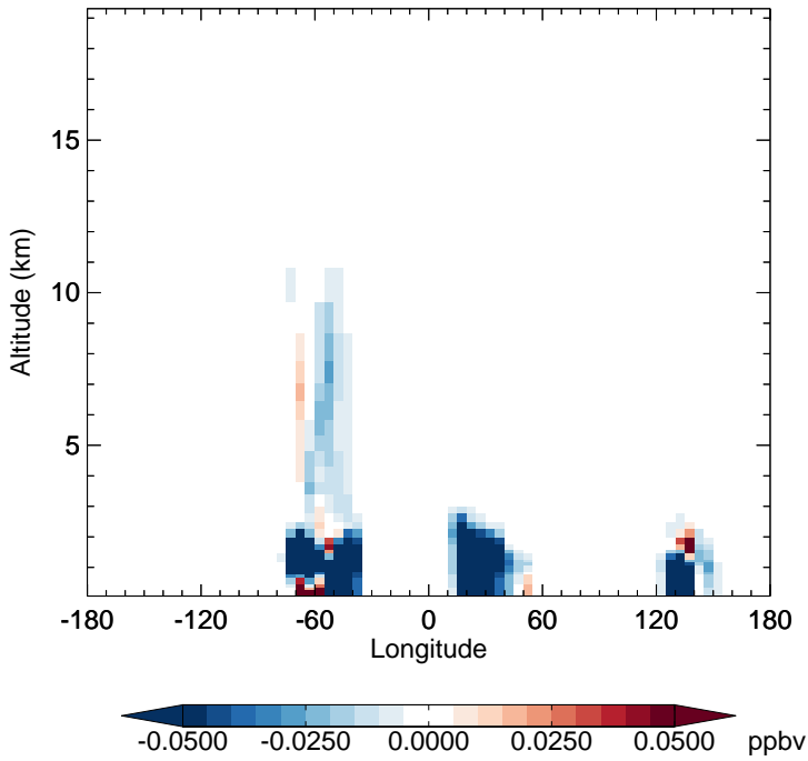
v11-02f-Run0 - v11-02e-Run0 MVK - Diff along 15S for Apr
