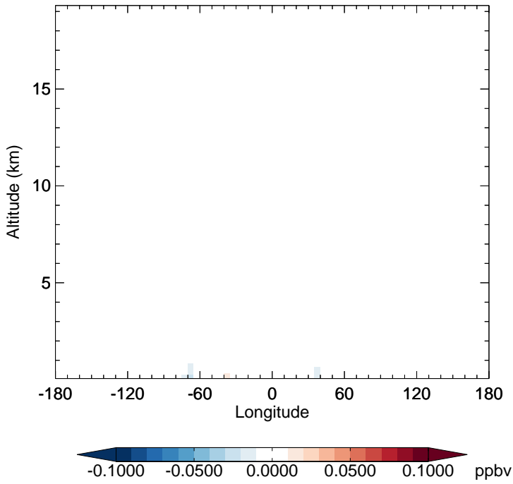
v11-02f-Run0 - v11-02e-Run1 XYLE - Diff along 15S for Apr
