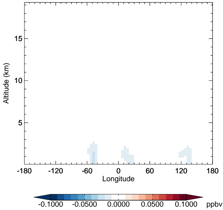
v11-02f-Run0 - v11-02e-Run1 ISOG1 - Diff along 15S for Apr
