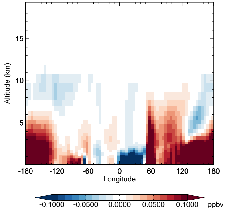
v11-02f-Run0 - v11-02e-Run0 BENZ - Diff along 42N for Apr
