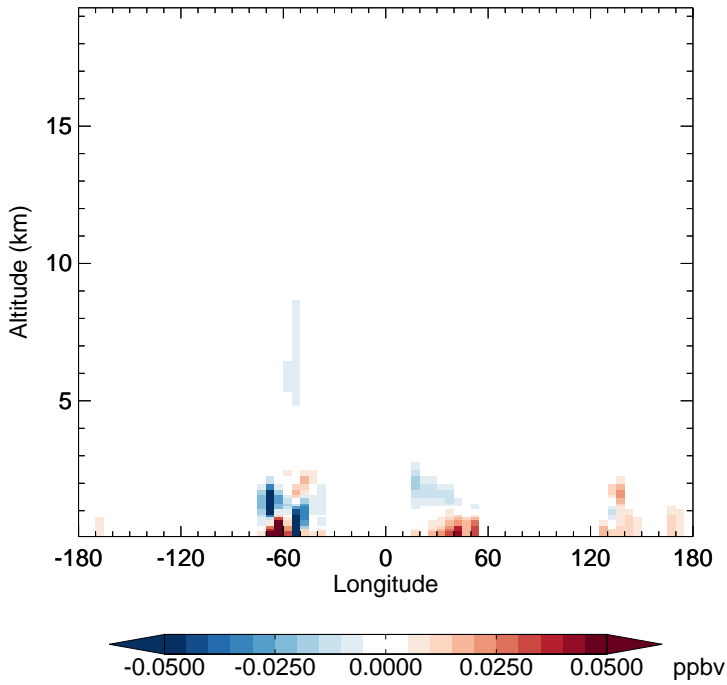
v11-02f-Run0 - v11-02e-Run0 RCHO - Diff along 15S for Apr
