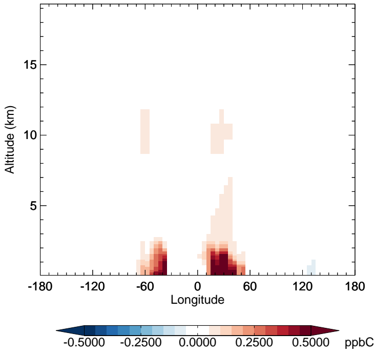
v11-02f-Run0 - v11-02e-Run1 ALK4 - Diff along 15S for Apr
