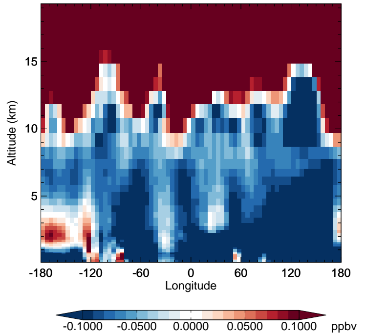
v11-02f-Run0 - v11-02e-Run0 HNO 3 - Diff along 42N for Apr
