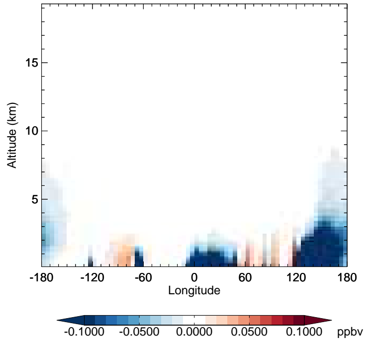
v11-02f-Run0 - v11-02e-Run1 TOLU - Diff along 42N for Apr
