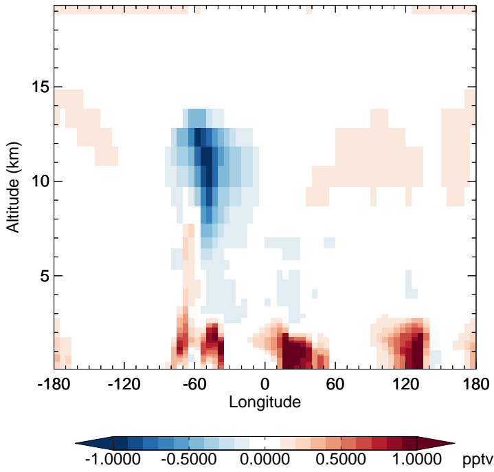
v11-02f-Run0 - v11-02e-Run1 HO2 - Diff along 15S for Apr
