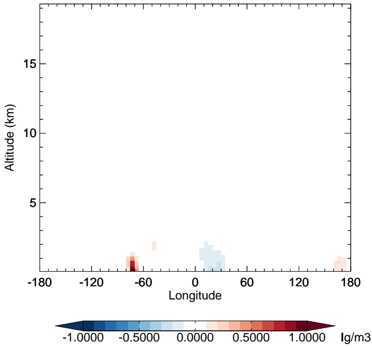
v11-02f-Run0 - v11-02e-Run1 NH4 - Diff along 15S for Apr
