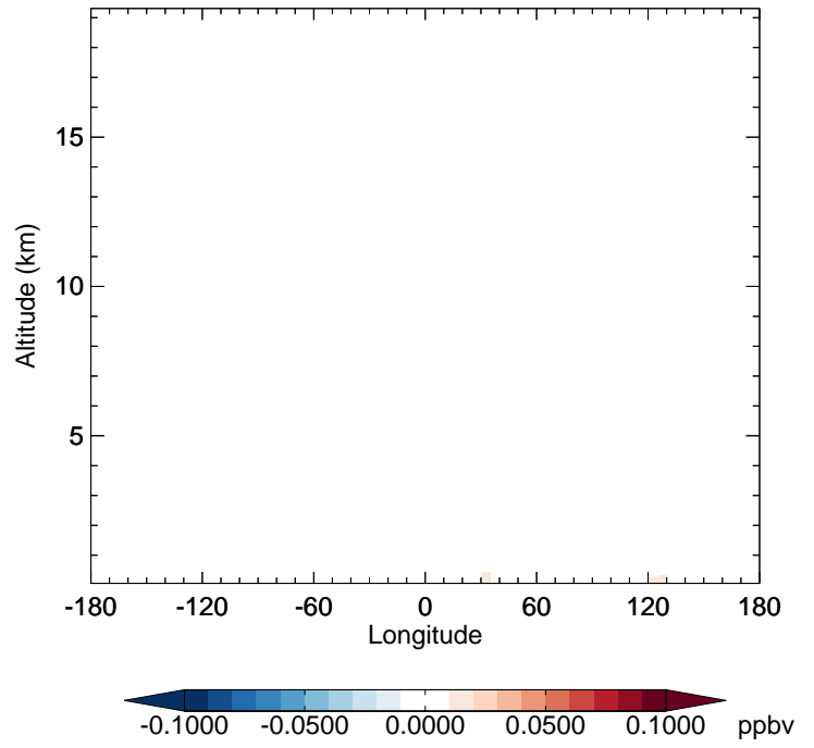
v11-02f-Run0 - v11-02e-Run1 GLYC - Diff along 42N for Apr
