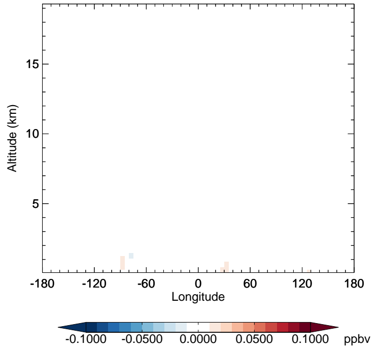
v11-02f-Run0 - v11-02e-Run0 HAC - Diff along 42N for Apr
