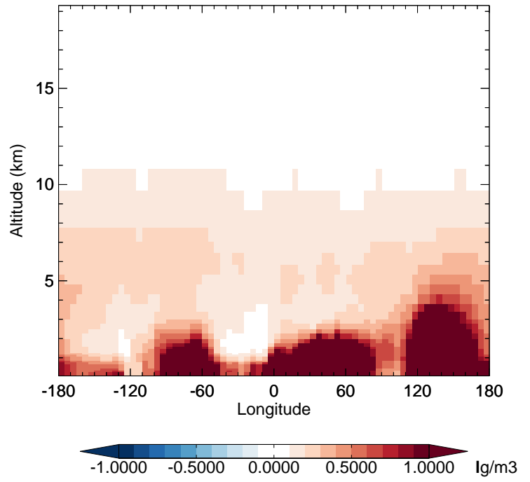
v11-02f-Run0 - v11-02e-Run1 NIT - Diff along 42N for Apr
