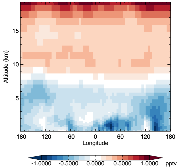
v11-02f-Run0 - v11-02e-Run1 HO2 - Diff along 42N for Apr
