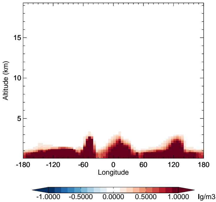
v11-02f-Run0 - v11-02e-Run0 NH3 - Diff along 15S for Apr
