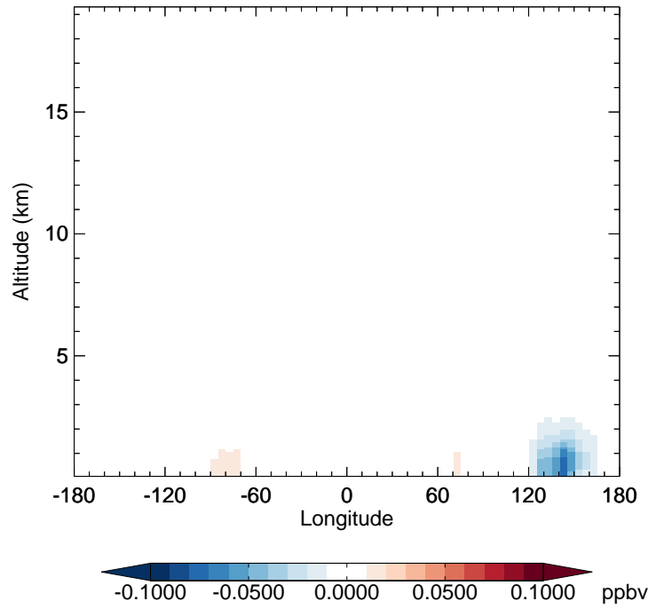
v11-02f-Run0 - v11-02e-Run1 SOAGX - Diff along 42N for Apr
