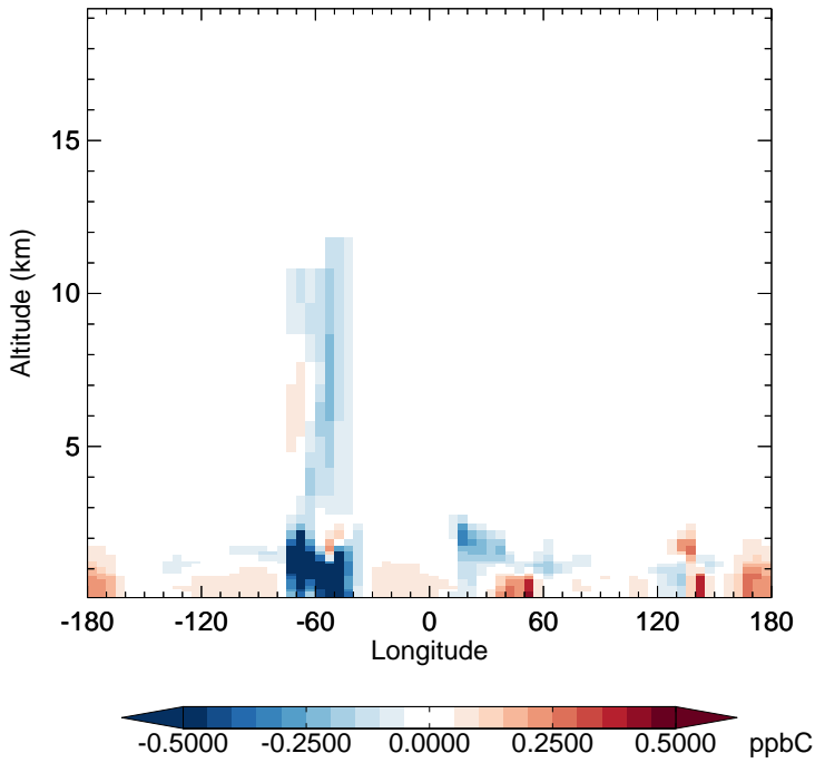
v11-02f-Run0 - v11-02e-Run0 ALD2 - Diff along 15S for Apr
