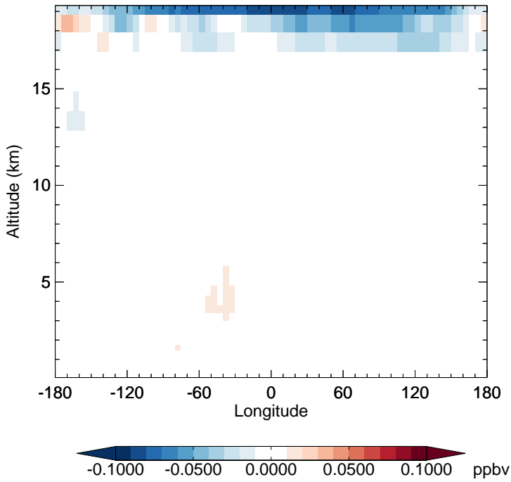
v11-02f-Run0 - v11-02e-Run0 HCl - Diff along 15S for Apr
