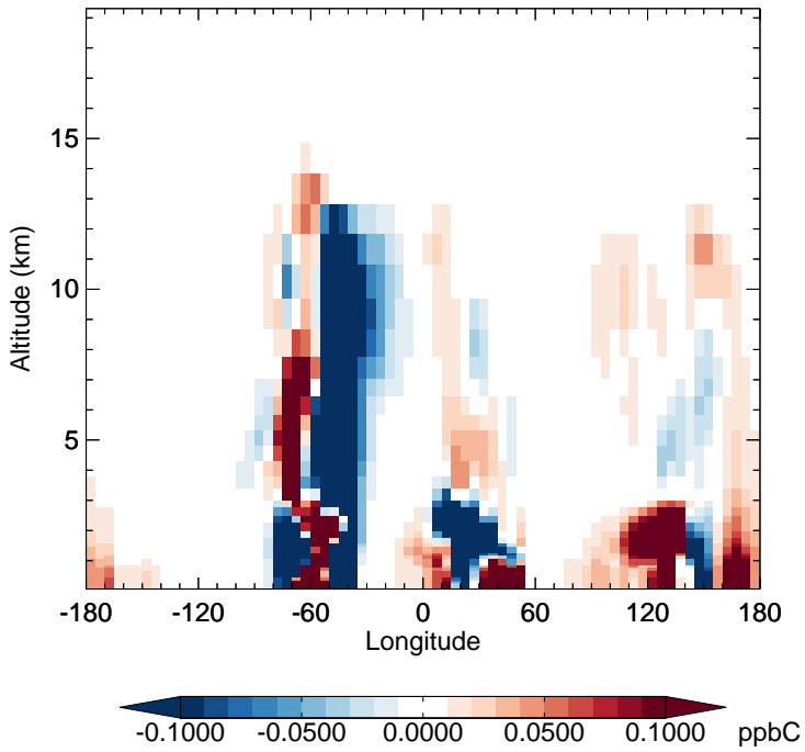
v11-02f-Run0 - v11-02e-Run0 MEK - Diff along 15S for Apr
