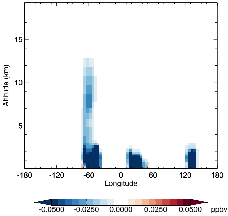
v11-02f-Run0 - v11-02e-Run1 MVK - Diff along 15S for Apr
