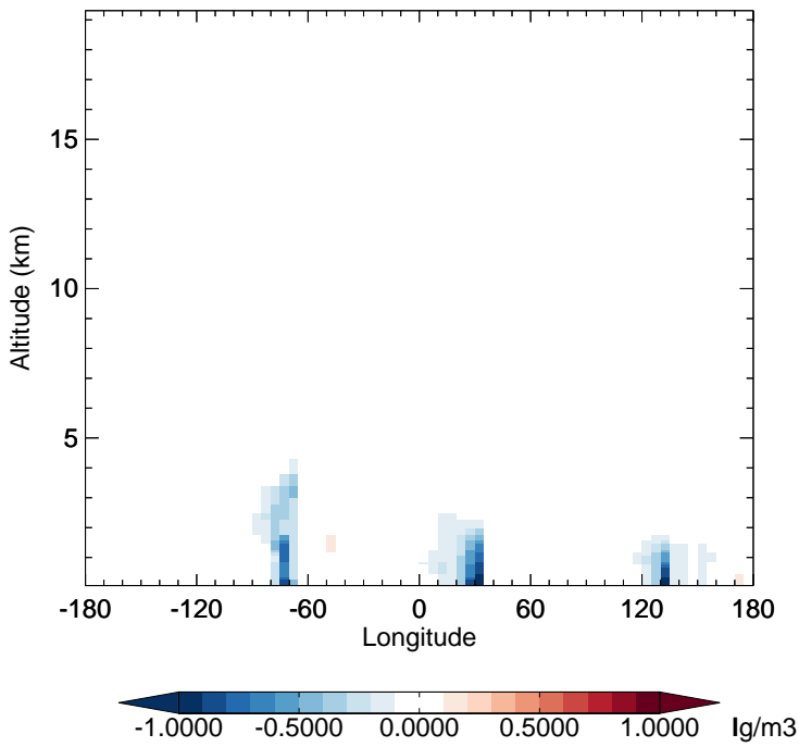
v11-02f-Run0 - v11-02e-Run0 SO 2 - Diff along 15S for Apr
