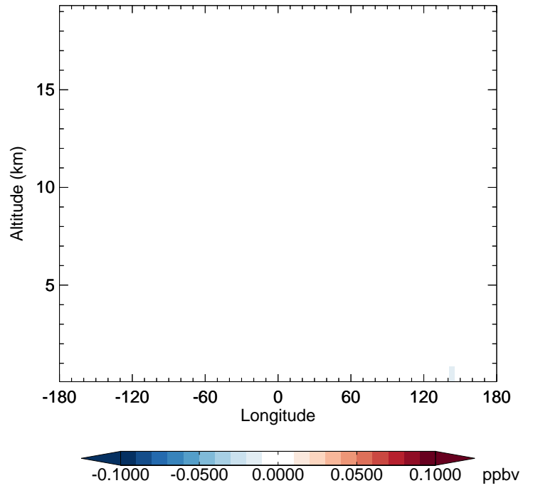
v11-02f-Run0 - v11-02e-Run1 MGLY - Diff along 42N for Apr
