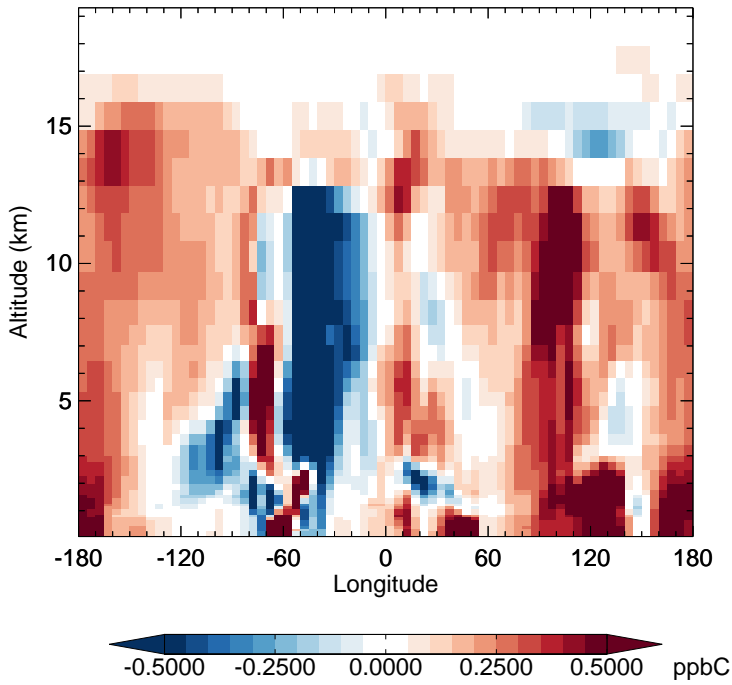
v11-02f-Run0 - v11-02e-Run0 ACET - Diff along 15S for Apr
