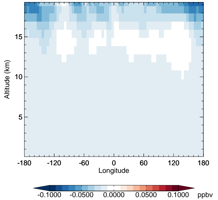
v11-02f-Run0 - v11-02e-Run0 CFC12 - Diff along 42N for Apr
