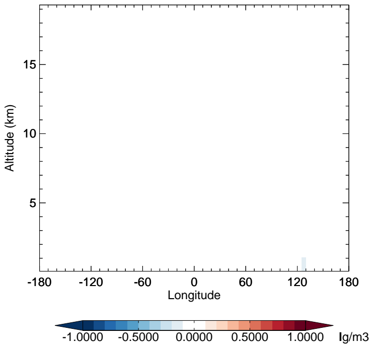
v11-02f-Run0 - v11-02e-Run0 OCPO - Diff along 15S for Apr
