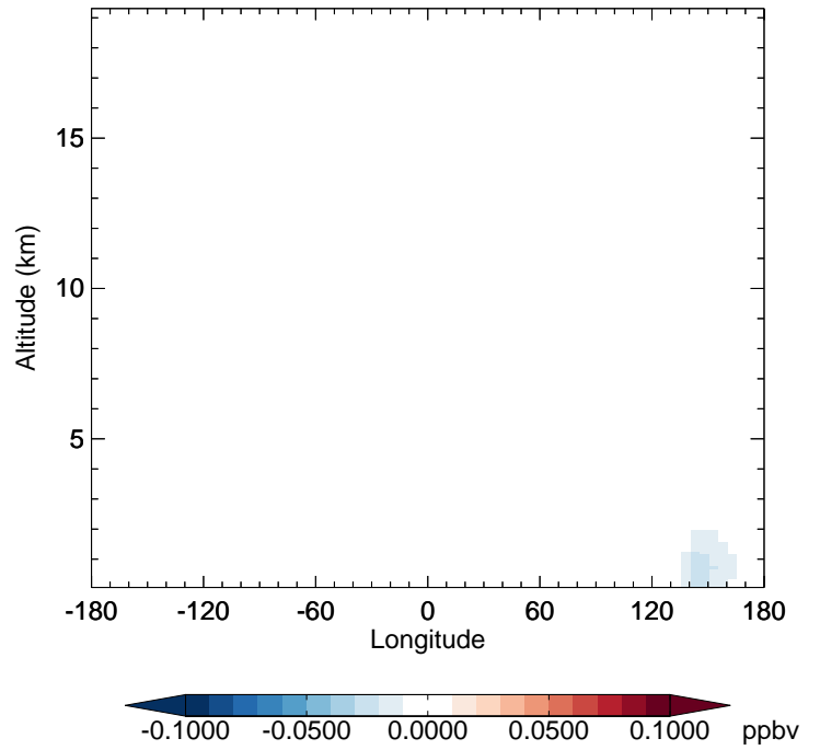
v11-02f-Run0 - v11-02e-Run0 ASOAN - Diff along 42N for Apr
