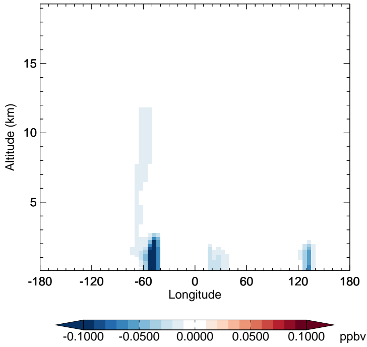
v11-02f-Run0 - v11-02e-Run1 IPMN - Diff along 15S for Apr
