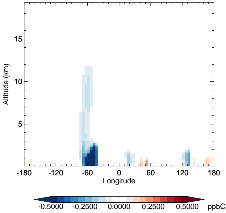
v11-02f-Run0 - v11-02e-Run1 ALD2 - Diff along 15S for Apr
