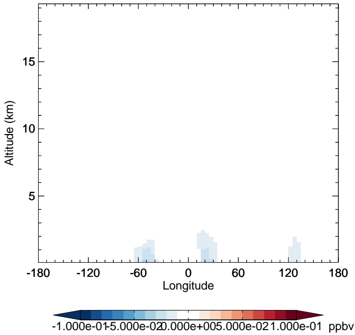
v11-02f-Run0 - v11-02e-Run0 MONITA - Diff along 15S for Apr
