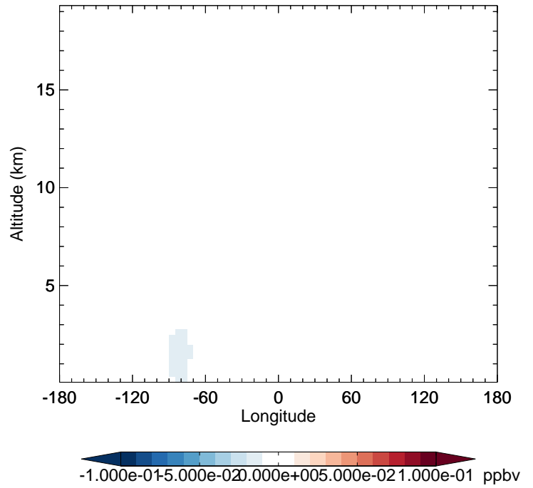
v11-02f-Run0 - v11-02e-Run0 SOAIE - Diff along 42N for Apr
