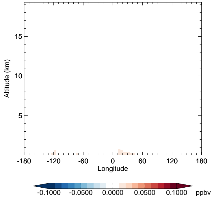
v11-02f-Run0 - v11-02e-Run1 TSOG3 - Diff along 42N for Apr
