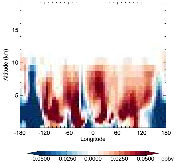
v11-02f-Run0 - v11-02e-Run0 MP - Diff along 42N for Apr
