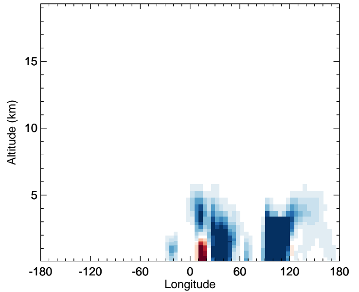
v11-02f-Run0 - v11-02e-Run0 DST4 - Diff along 42N for Apr
