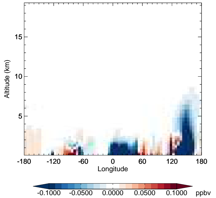
v11-02f-Run0 - v11-02e-Run0 TOLU - Diff along 42N for Apr
