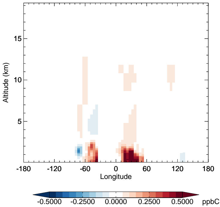
v11-02f-Run0 - v11-02e-Run0 ALK4 - Diff along 15S for Apr
