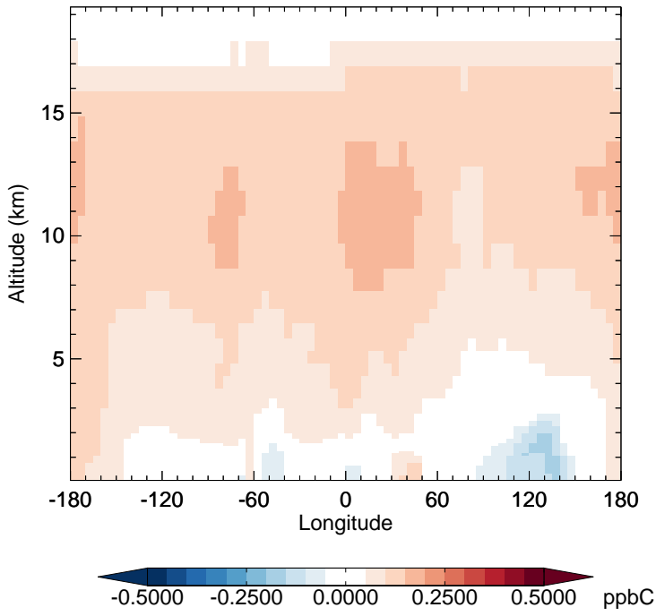
v11-02f-Run0 - v11-02e-Run1 C2H6 - Diff along 15S for Apr
