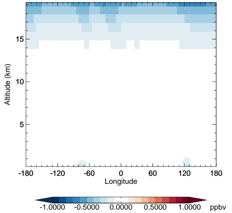
v11-02f-Run0 - v11-02e-Run1 NO 2 - Diff along 42N for Apr
