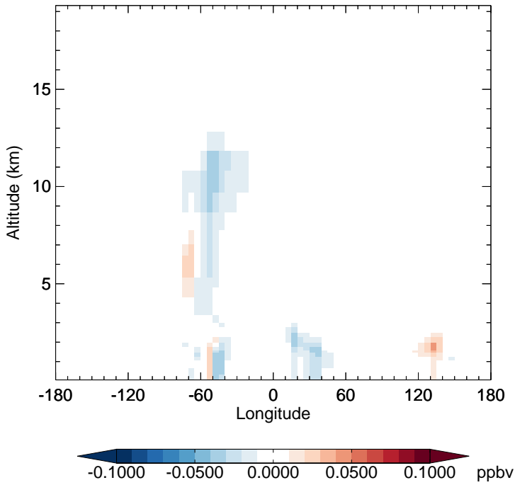
v11-02f-Run0 - v11-02e-Run0 HC187 - Diff along 15S for Apr
