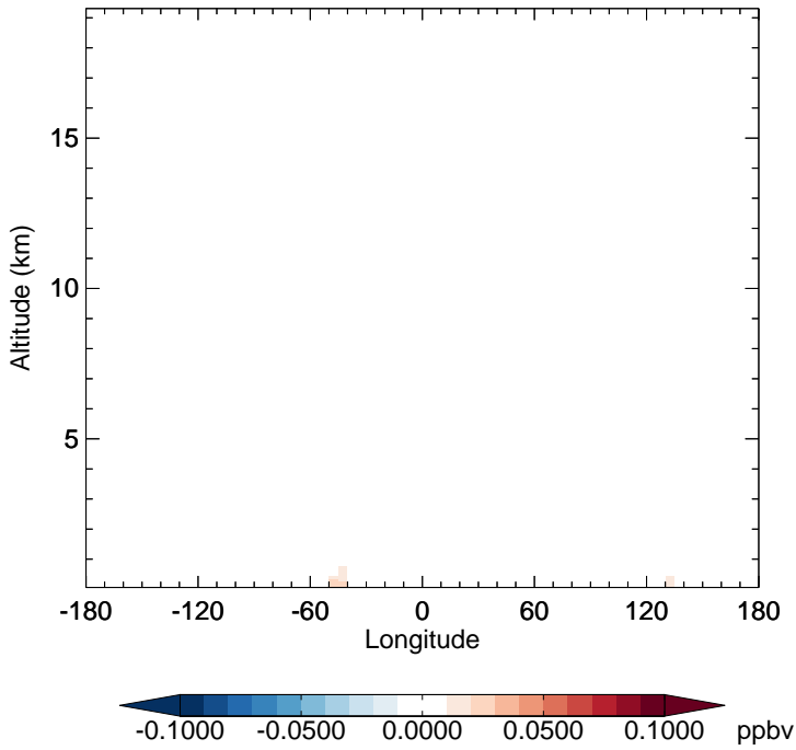
v11-02f-Run0 - v11-02e-Run0 MONITS - Diff along 15S for Apr
