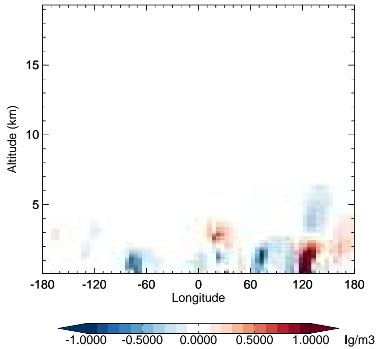
v11-02f-Run0 - v11-02e-Run0 SO 2 - Diff along 42N for Apr
