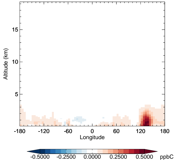
v11-02f-Run0 - v11-02e-Run0 ALD2 - Diff along 42N for Apr
