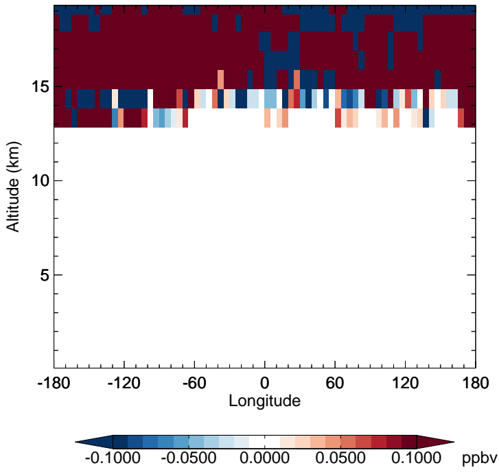
v11-02f-Run0 - v11-02e-Run1 H2O - Diff along 15S for Apr
