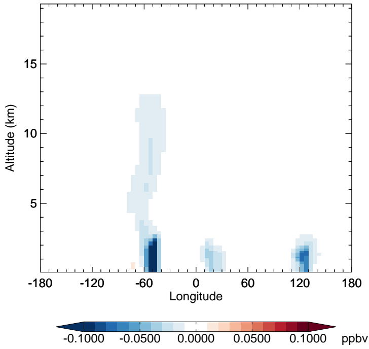
v11-02f-Run0 - v11-02e-Run1 IMAE - Diff along 15S for Apr
