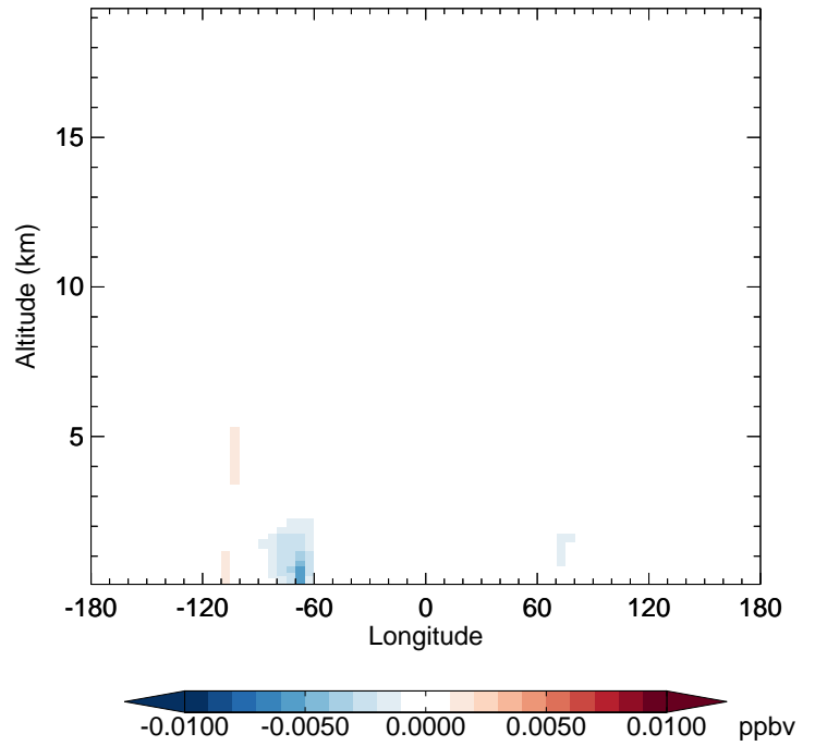
v11-02f-Run0 - v11-02e-Run0 R4N2 - Diff along 42N for Apr
