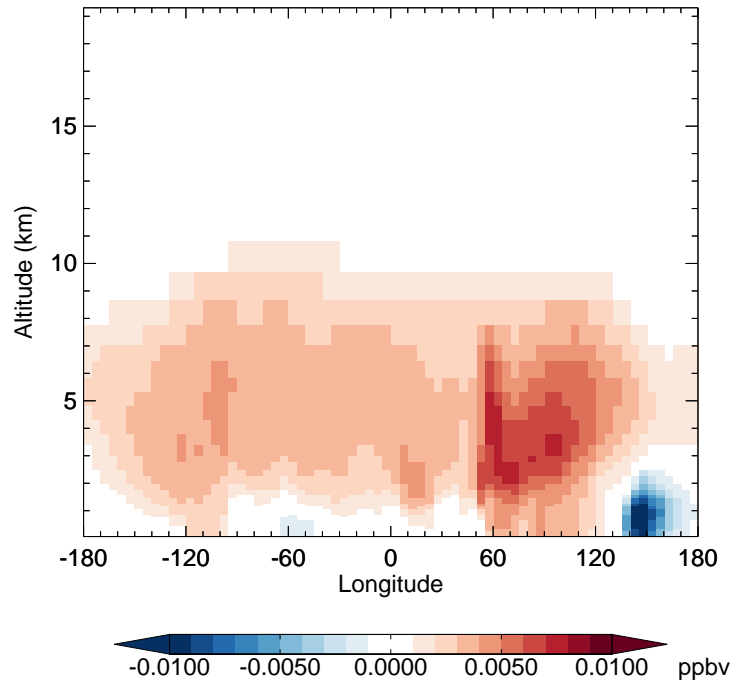
v11-02f-Run0 - v11-02e-Run1 MAP - Diff along 42N for Apr
