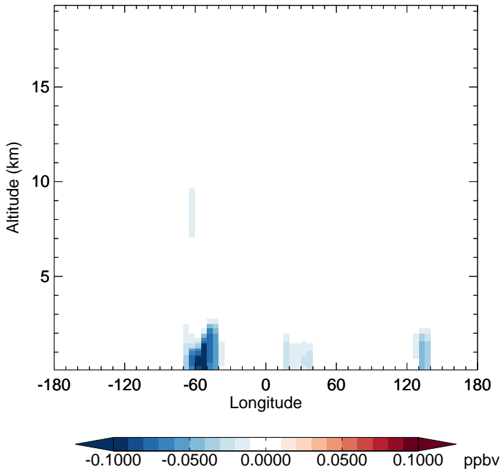
v11-02f-Run0 - v11-02e-Run1 RIPB - Diff along 15S for Apr
