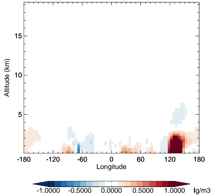
v11-02f-Run0 - v11-02e-Run0 SOAS - Diff along 42N for Apr
