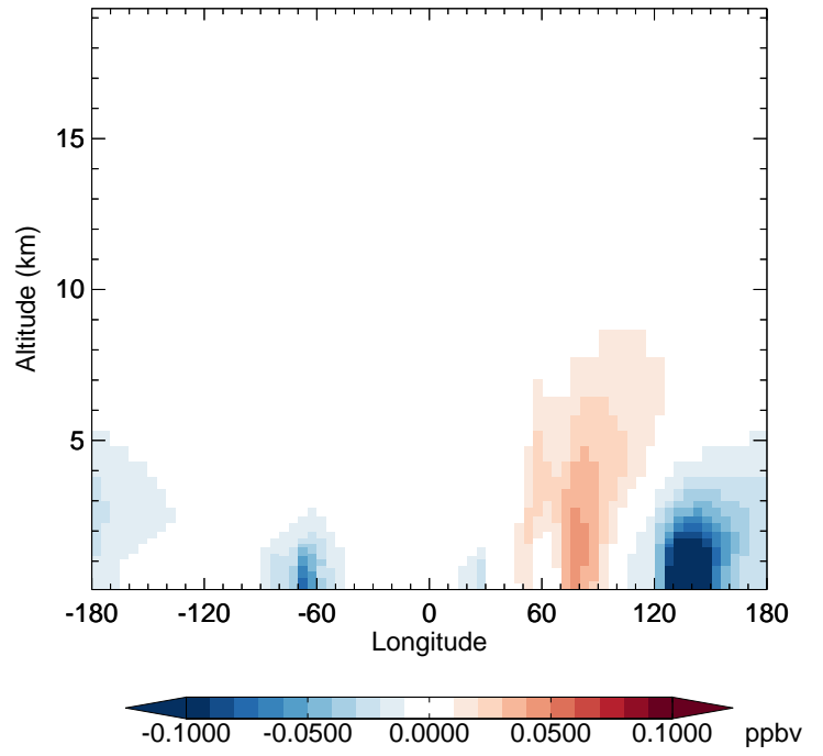
v11-02f-Run0 - v11-02e-Run1 PAN - Diff along 42N for Apr
