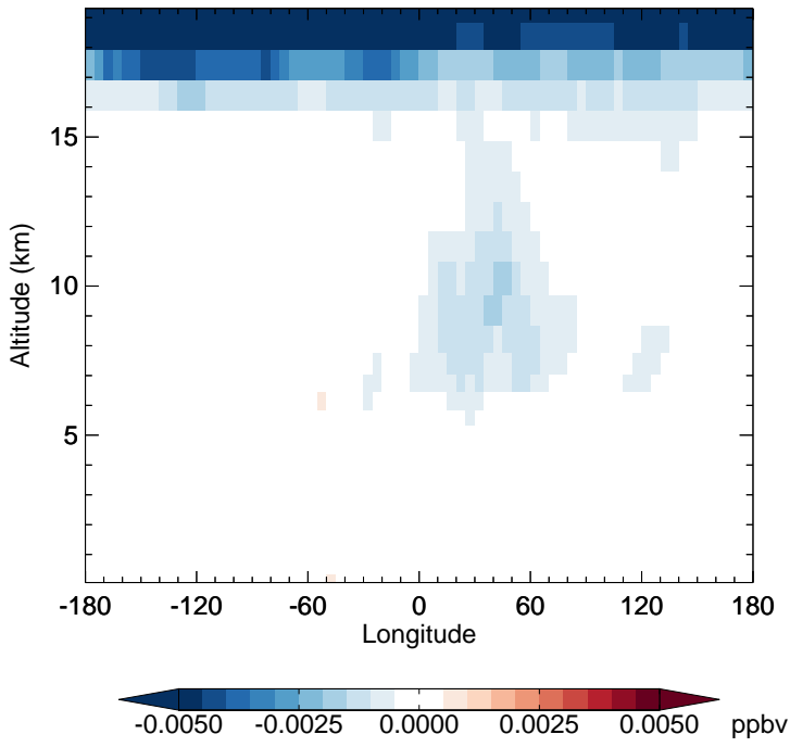
v11-02f-Run0 - v11-02e-Run1 N2O5 - Diff along 15S for Apr
