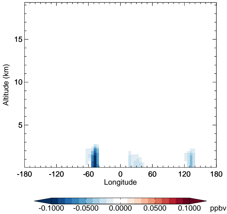
v11-02f-Run0 - v11-02e-Run1 MGLY - Diff along 15S for Apr
