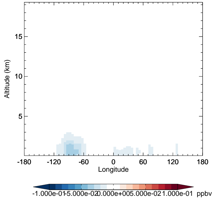
v11-02f-Run0 - v11-02e-Run1 IONITA - Diff along 42N for Apr
