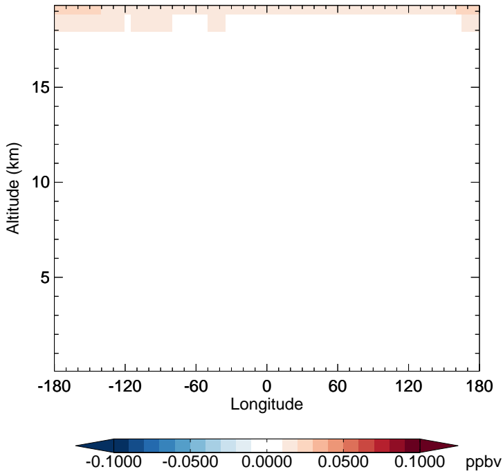
v11-02f-Run0 - v11-02e-Run1 N2O - Diff along 15S for Apr
