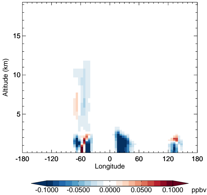
v11-02f-Run0 - v11-02e-Run0 GLYC - Diff along 15S for Apr
