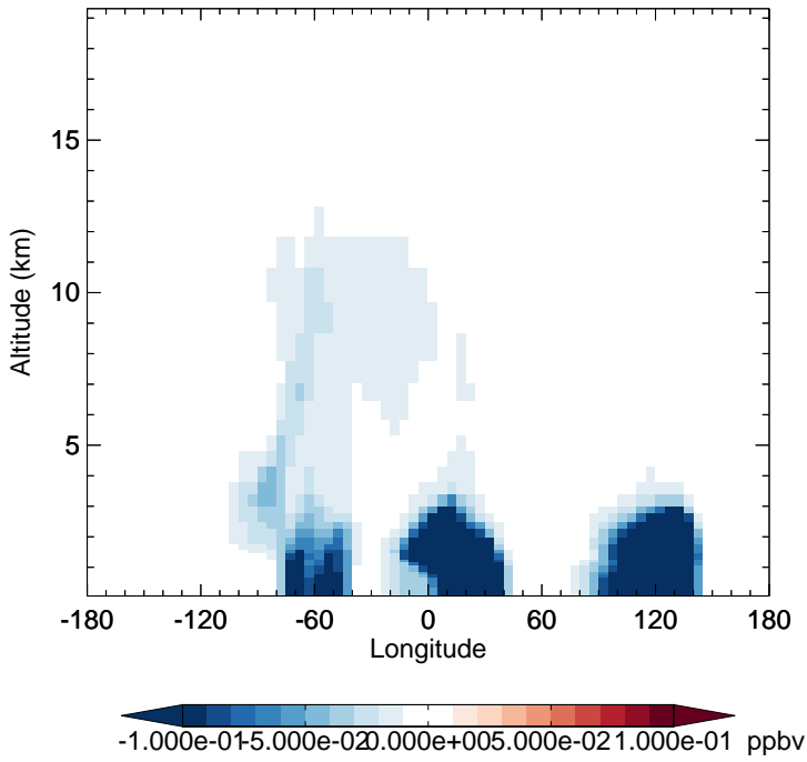
v11-02f-Run0 - v11-02e-Run1 SOAIE - Diff along 15S for Apr
