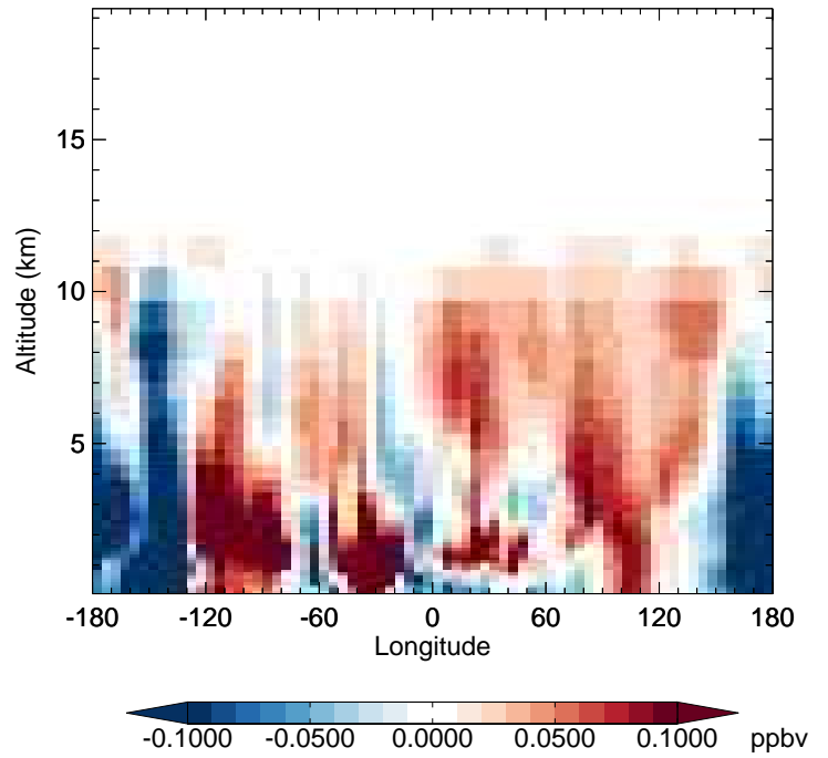
v11-02f-Run0 - v11-02e-Run0 H2O2 - Diff along 42N for Apr
