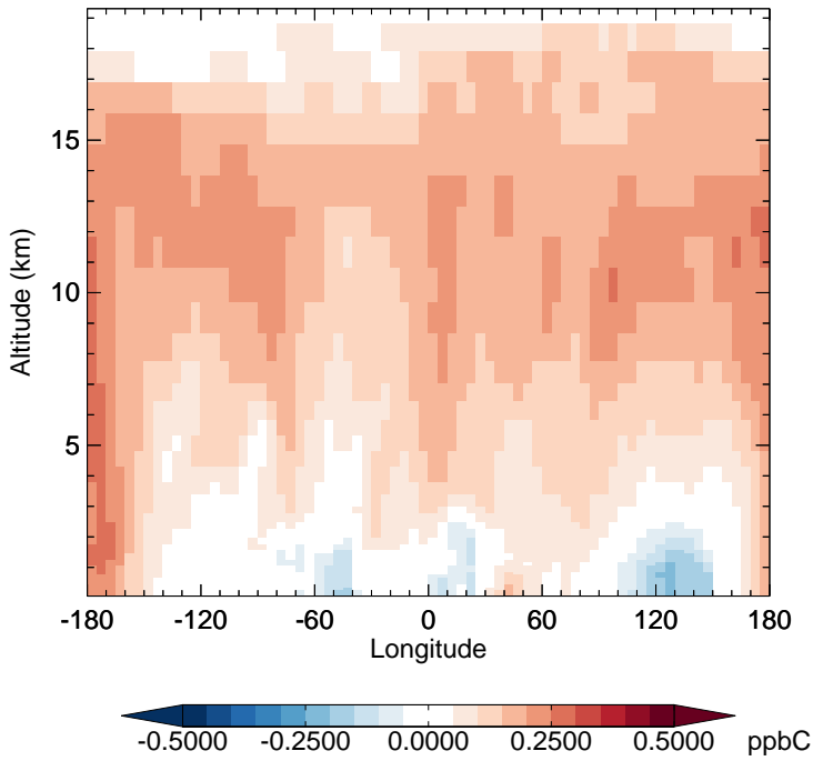
v11-02f-Run0 - v11-02e-Run0 C2H6 - Diff along 15S for Apr
