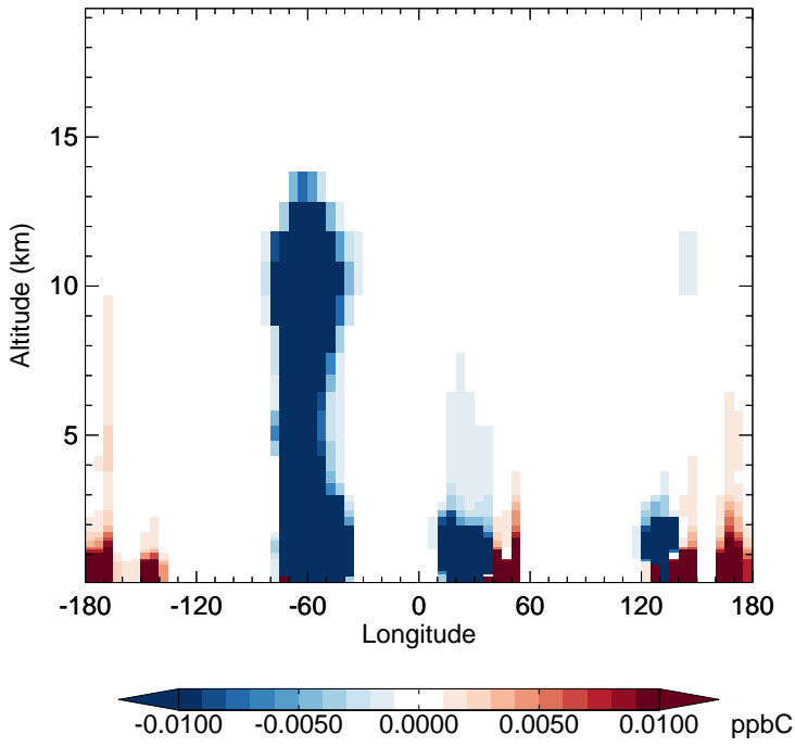
v11-02f-Run0 - v11-02e-Run1 PRPE - Diff along 15S for Apr
