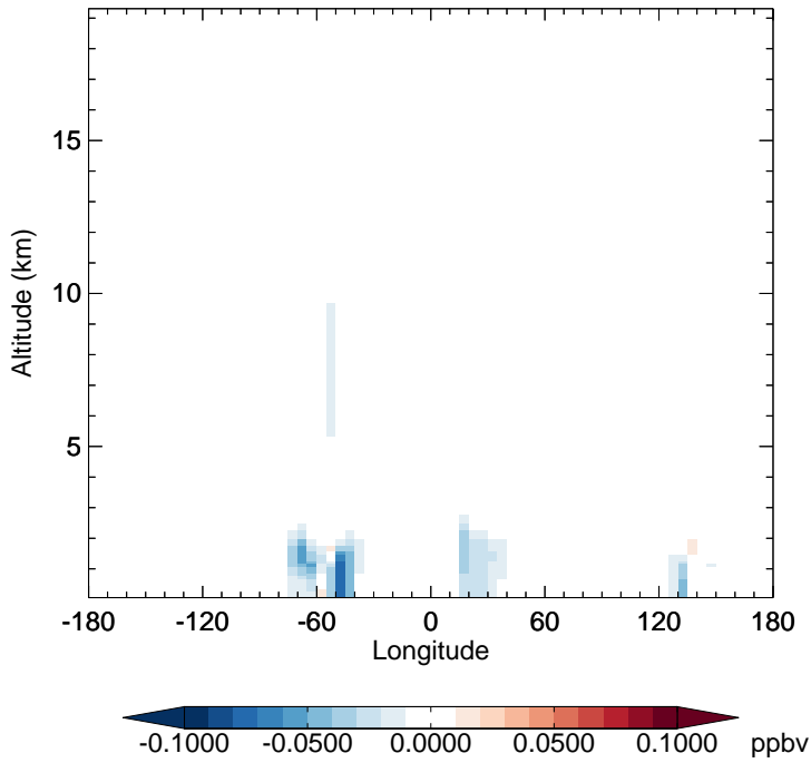
v11-02f-Run0 - v11-02e-Run0 IPMN - Diff along 15S for Apr
