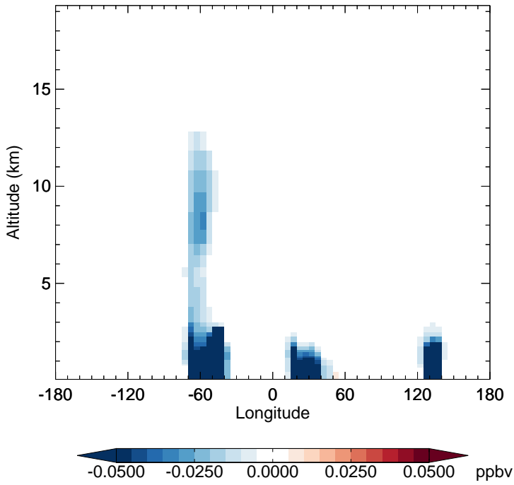
v11-02f-Run0 - v11-02e-Run1 MACR - Diff along 15S for Apr
