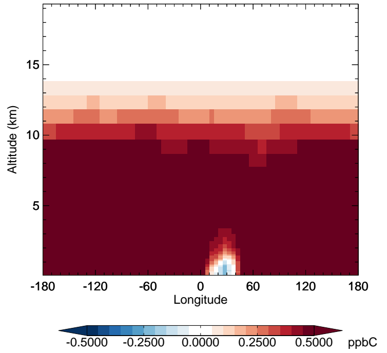
v11-02f-Run0 - v11-02e-Run1 C2H6 - Diff along 42N for Apr
