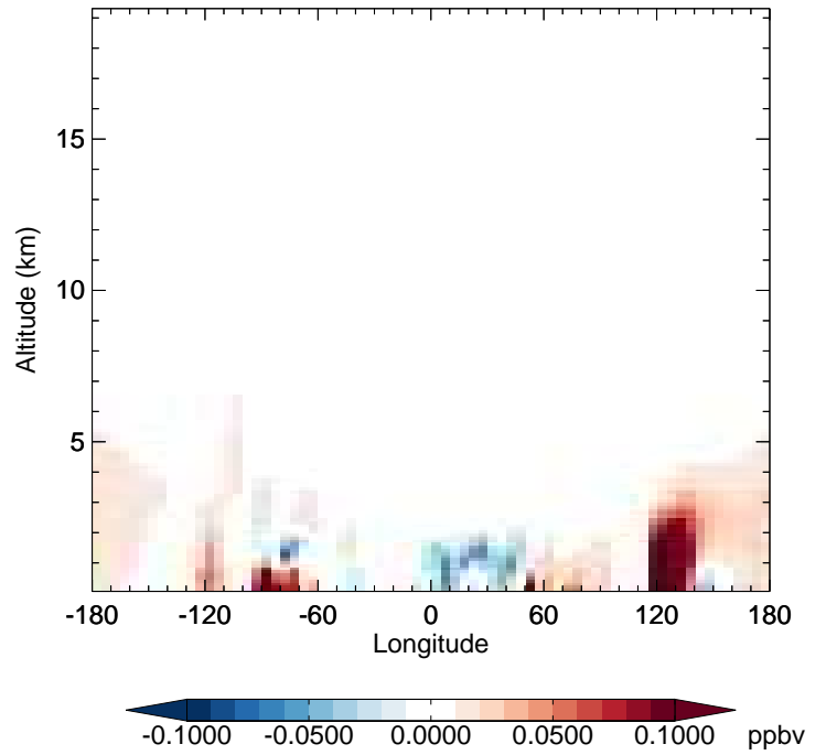
v11-02f-Run0 - v11-02e-Run0 EOH - Diff along 42N for Apr
