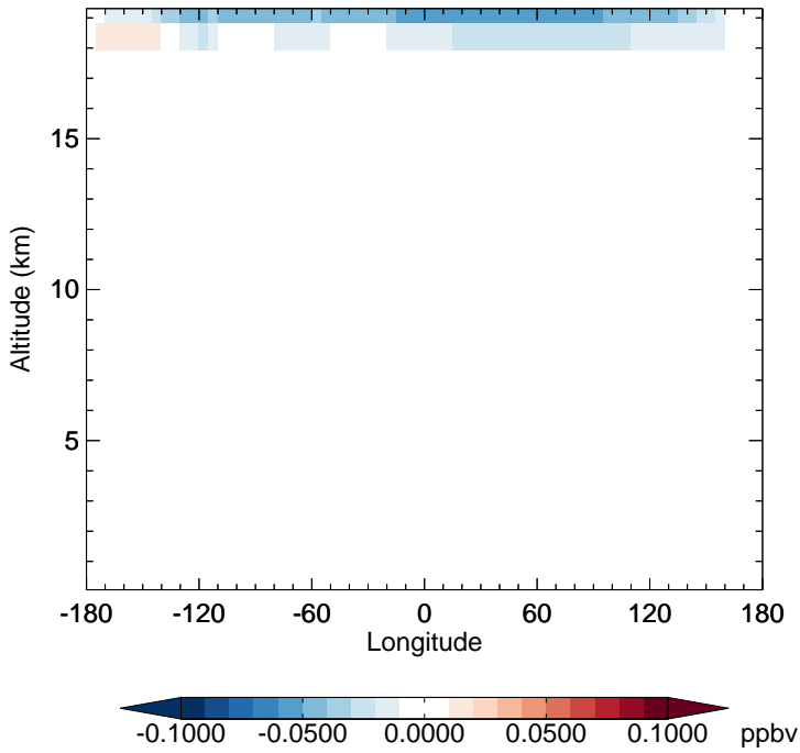
v11-02f-Run0 - v11-02e-Run0 CINO3 - Diff along 15S for Apr
