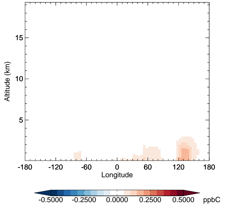
v11-02f-Run0 - v11-02e-Run1 ALD2 - Diff along 42N for Apr
