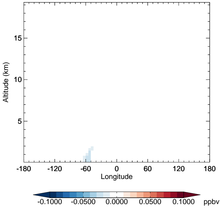
v11-02f-Run0 - v11-02e-Run1 TSOA2 - Diff along 15S for Apr
