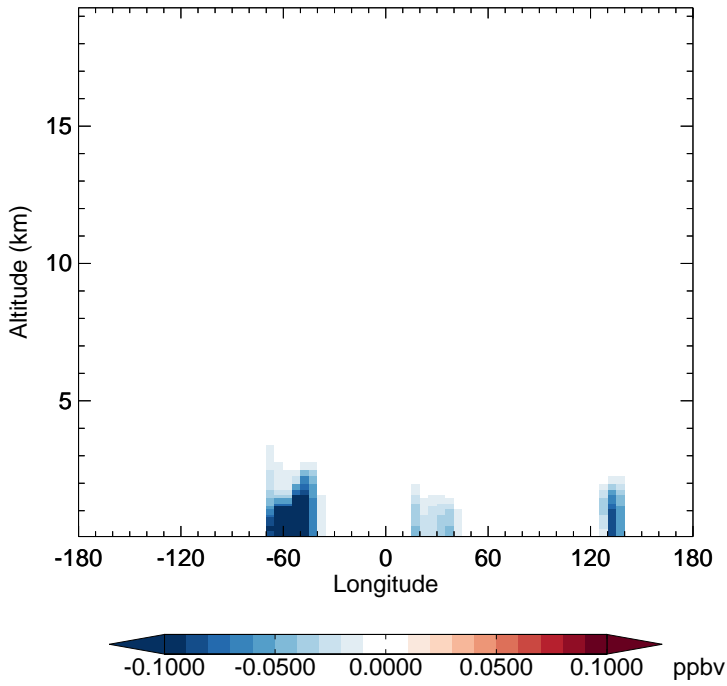
v11-02f-Run0 - v11-02e-Run1 HPALD - Diff along 15S for Apr
