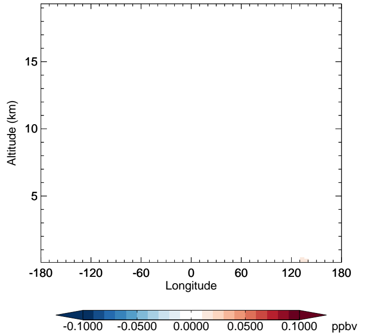
v11-02f-Run0 - v11-02e-Run0 TSOA2 - Diff along 42N for Apr
