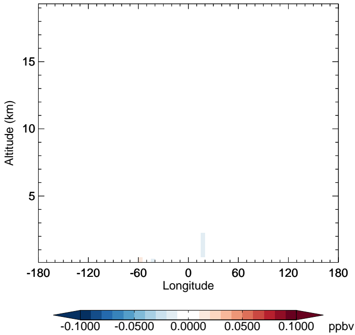
v11-02f-Run0 - v11-02e-Run0 GLYX - Diff along 15S for Apr
