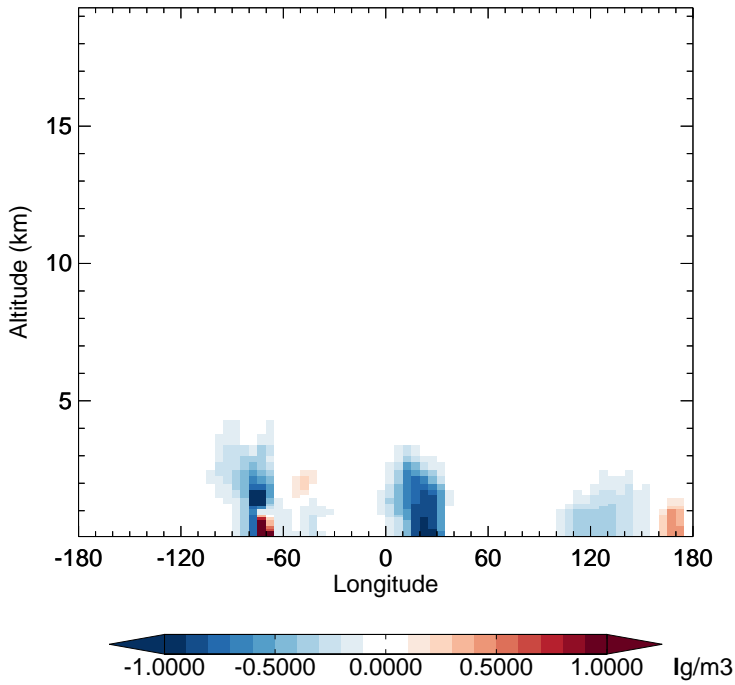
v11-02f-Run0 - v11-02e-Run0 SO4 - Diff along 15S for Apr
