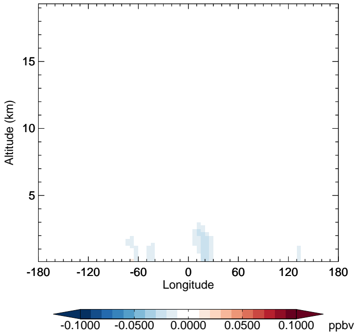
v11-02f-Run0 - v11-02e-Run0 SOAGX - Diff along 15S for Apr
