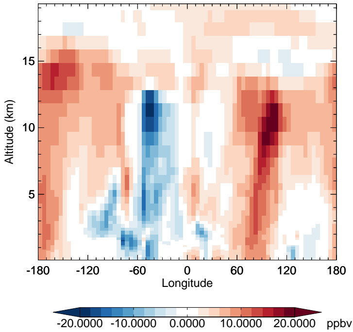
v11-02f-Run0 - v11-02e-Run0 CO - Diff along 15S for Apr
