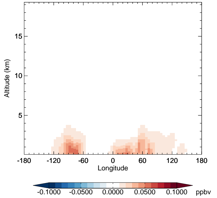
v11-02f-Run0 - v11-02e-Run1 INDIOL - Diff along 42N for Apr
