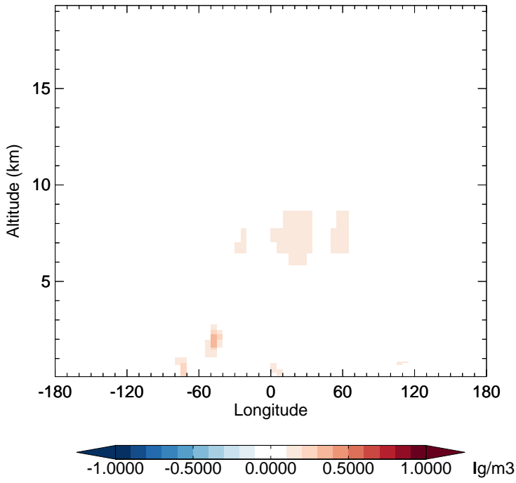
v11-02f-Run0 - v11-02e-Run1 NIT - Diff along 15S for Apr
