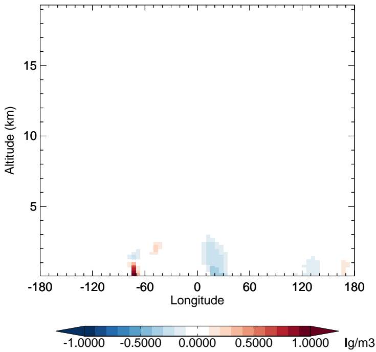
v11-02f-Run0 - v11-02e-Run0 NH4 - Diff along 15S for Apr
