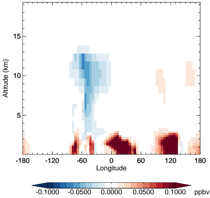
v11-02f-Run0 - v11-02e-Run1 H2O2 - Diff along 15S for Apr
