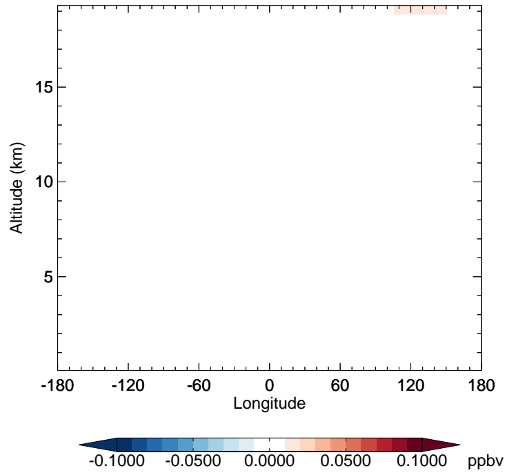
v11-02f-Run0 - v11-02e-Run1 ClO - Diff along 42N for Apr
