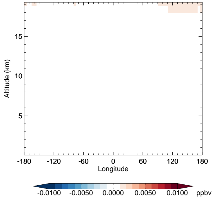
v11-02f-Run0 - v11-02e-Run0 BrO - Diff along 42N for Apr
