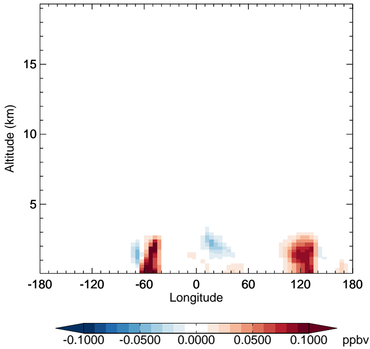
v11-02f-Run0 - v11-02e-Run0 TSOG2 - Diff along 15S for Apr
