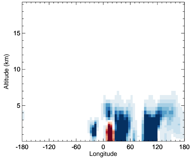
v11-02f-Run0 - v11-02e-Run0 DST3 - Diff along 42N for Apr
