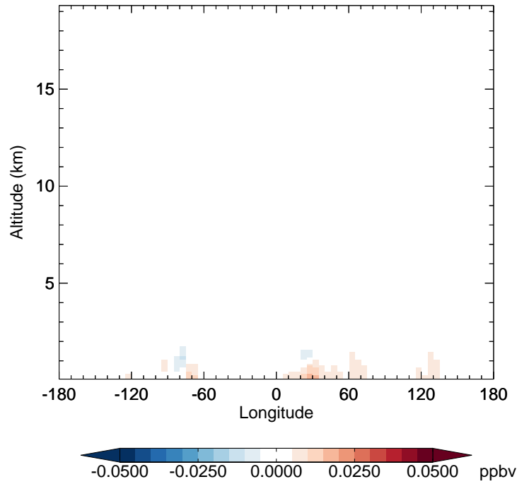
v11-02f-Run0 - v11-02e-Run0 MVK - Diff along 42N for Apr
