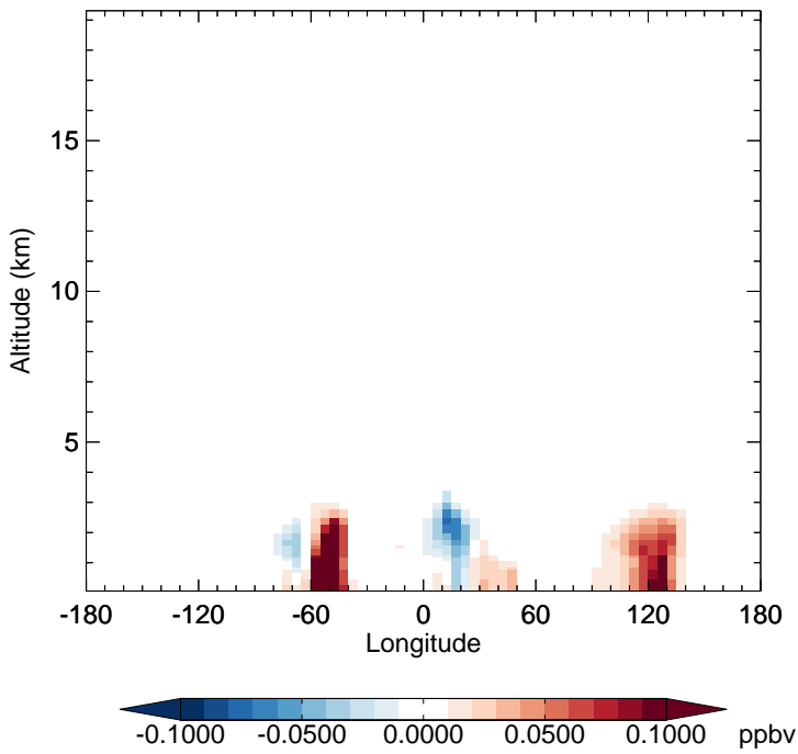
v11-02f-Run0 - v11-02e-Run0 INDIOL - Diff along 15S for Apr
