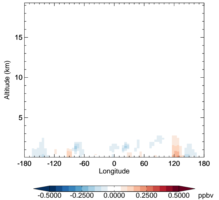
v11-02f-Run0 - v11-02e-Run0 CH 2 O - Diff along 42N for Apr
