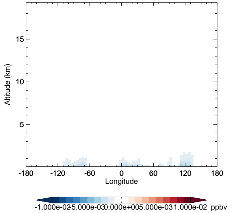
v11-02f-Run0 - v11-02e-Run1 NO3 - Diff along 42N for Apr
