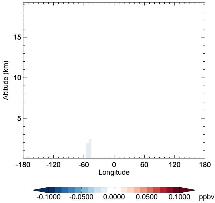
v11-02f-Run0 - v11-02e-Run1 IEPOXD - Diff along 15S for Apr
