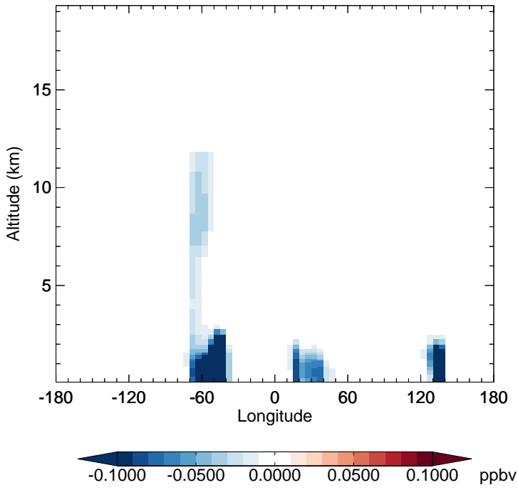
v11-02f-Run0 - v11-02e-Run1 RIPA - Diff along 15S for Apr
