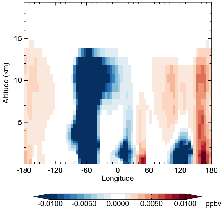
v11-02f-Run0 - v11-02e-Run1 MAP - Diff along 15S for Apr
