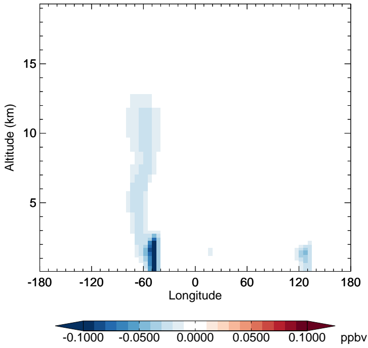
v11-02f-Run0 - v11-02e-Run1 HC187 - Diff along 15S for Apr
