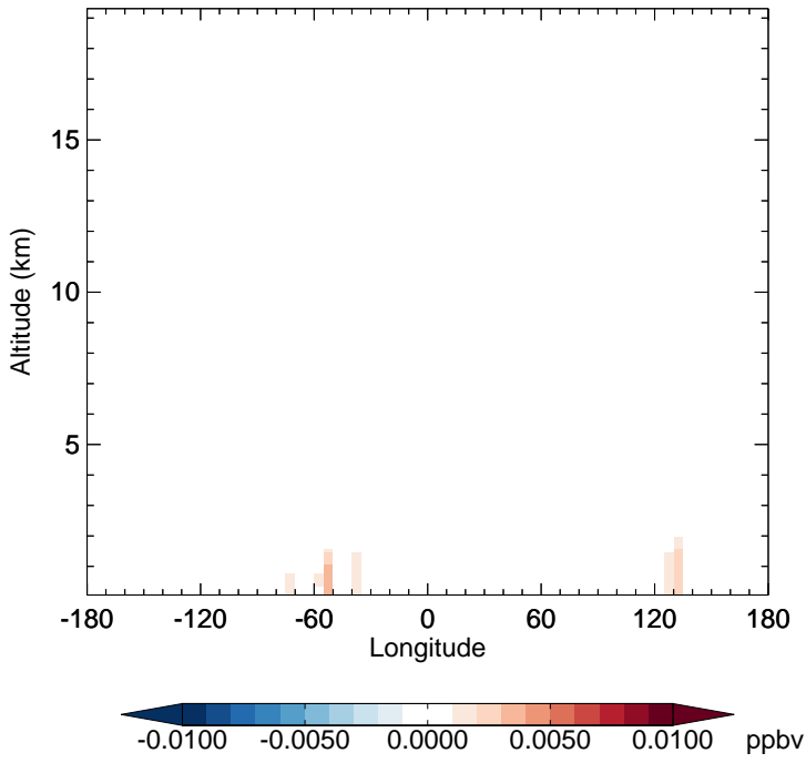
v11-02f-Run0 - v11-02e-Run1 MVKN - Diff along 15S for Apr
