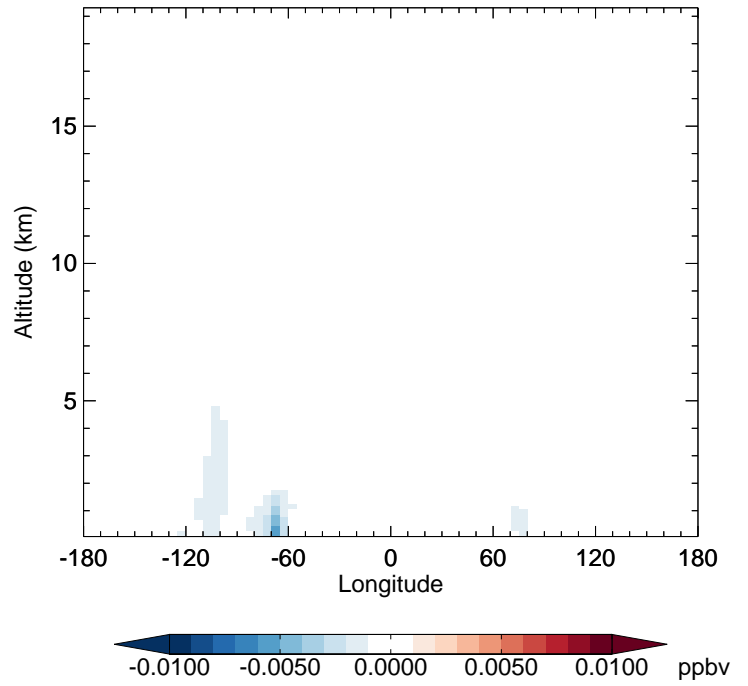
v11-02f-Run0 - v11-02e-Run1 R4N2 - Diff along 42N for Apr
