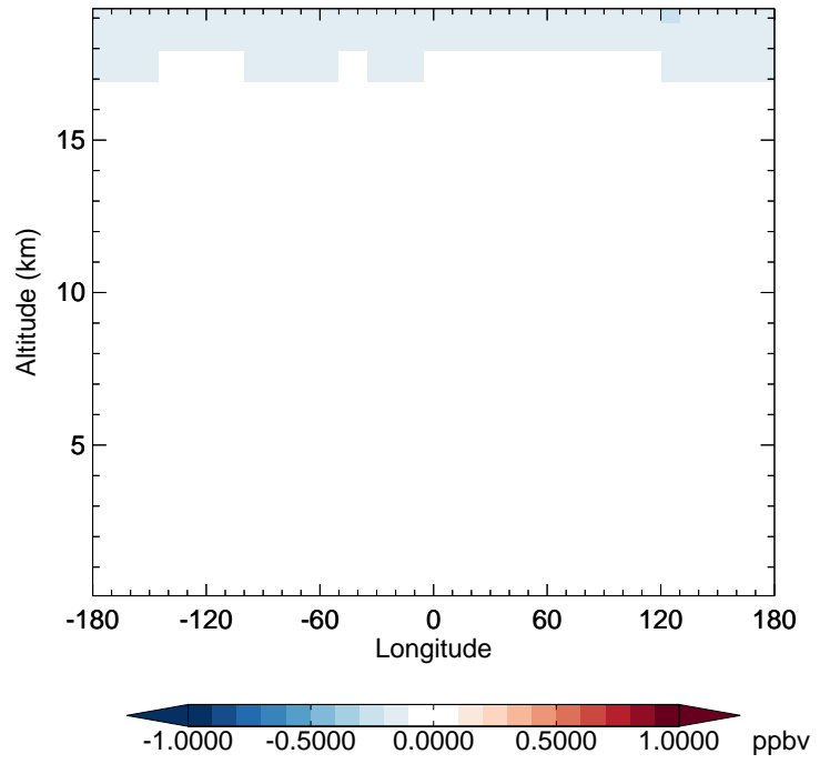
v11-02f-Run0 - v11-02e-Run1 NO - Diff along 42N for Apr
