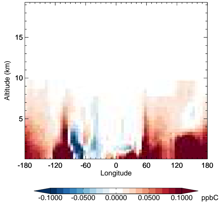
v11-02f-Run0 - v11-02e-Run0 MEK - Diff along 42N for Apr
