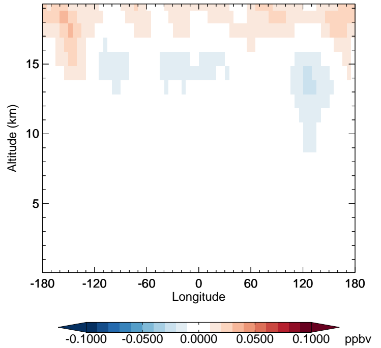
v11-02f-Run0 - v11-02e-Run0 MPN - Diff along 42N for Apr
