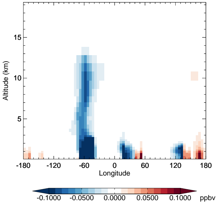
v11-02f-Run0 - v11-02e-Run1 EOH - Diff along 15S for Apr
