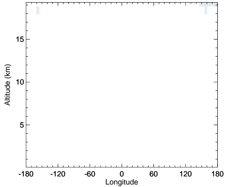
v11-02f-Run0 - v11-02e-Run0 HCFC22 - Diff along 42N for Apr
