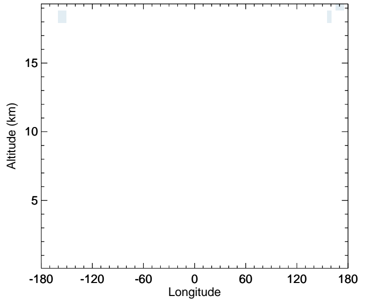
v11-02f-Run0 - v11-02e-Run0 CH3Br - Diff along 42N for Apr
