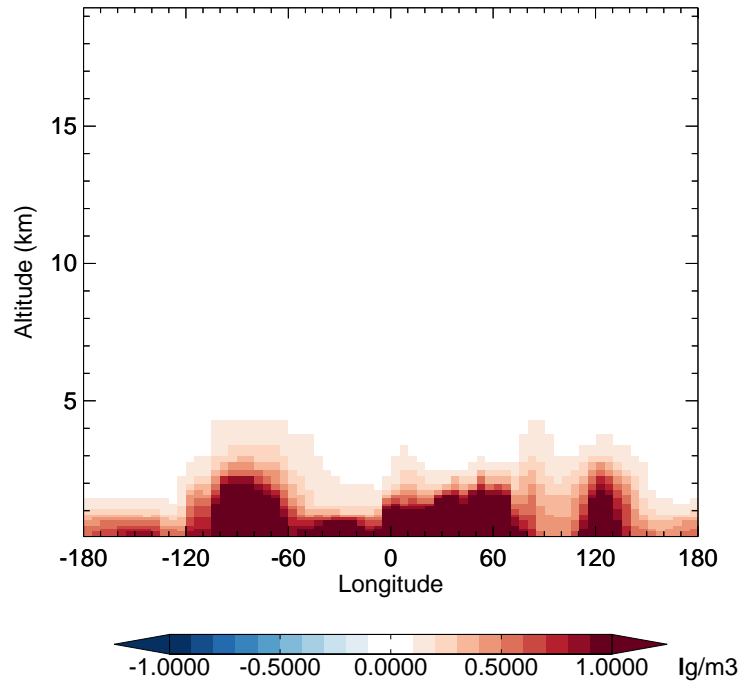
v11-02f-Run0 - v11-02e-Run1 NH3 - Diff along 42N for Apr
