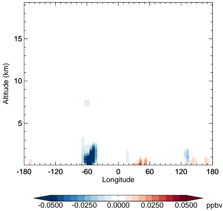
v11-02f-Run0 - v11-02e-Run1 RCHO - Diff along 15S for Apr
