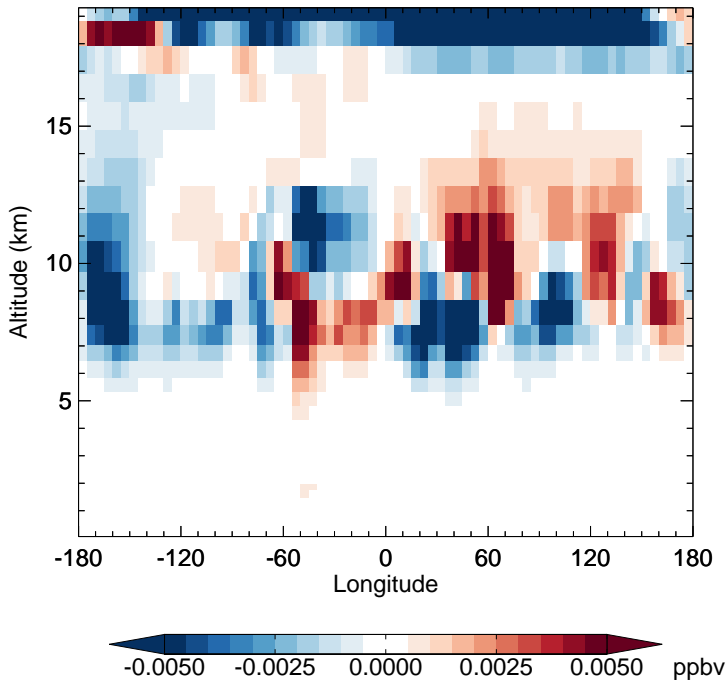
v11-02f-Run0 - v11-02e-Run0 HNO 4 - Diff along 15S for Apr
