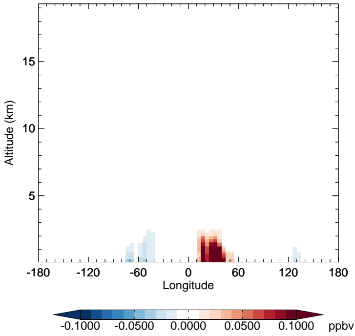
v11-02f-Run0 - v11-02e-Run1 TOLU - Diff along 15S for Apr
