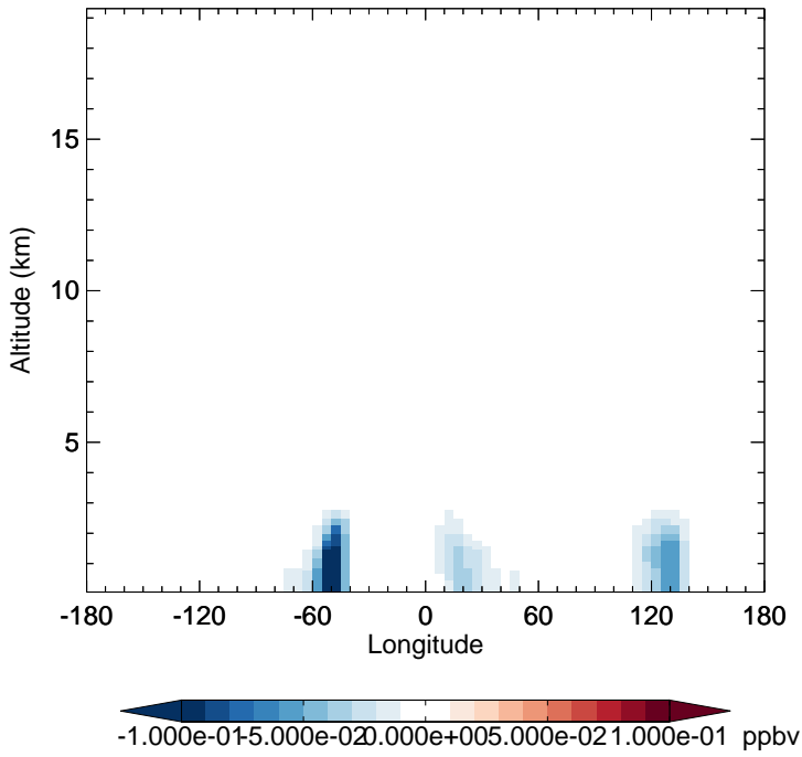
v11-02f-Run0 - v11-02e-Run1 IONITA - Diff along 15S for Apr
