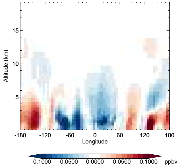
v11-02f-Run0 - v11-02e-Run0 PAN - Diff along 42N for Apr
