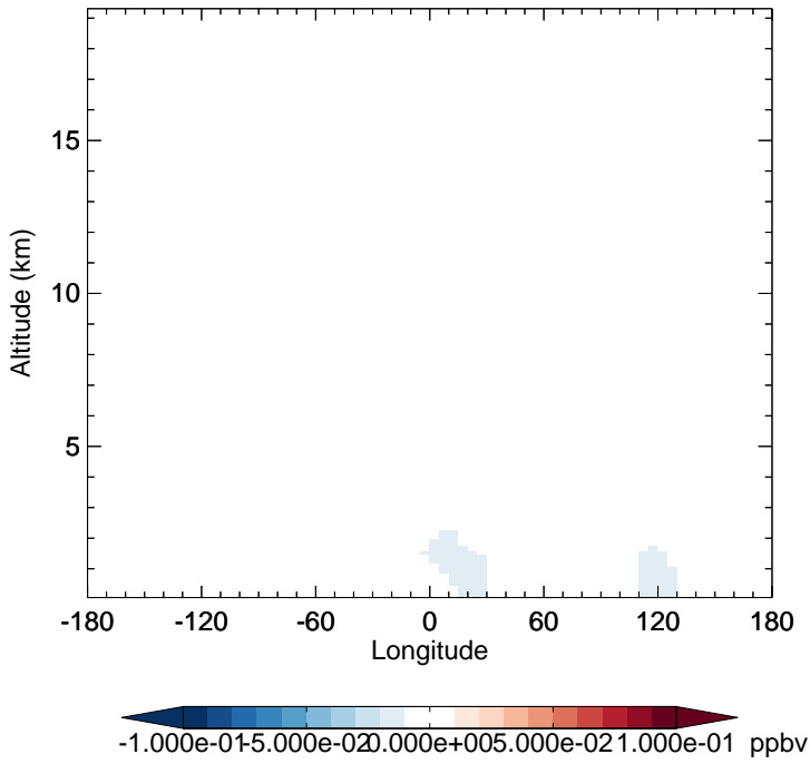
v11-02f-Run0 - v11-02e-Run1 SOAME - Diff along 15S for Apr
