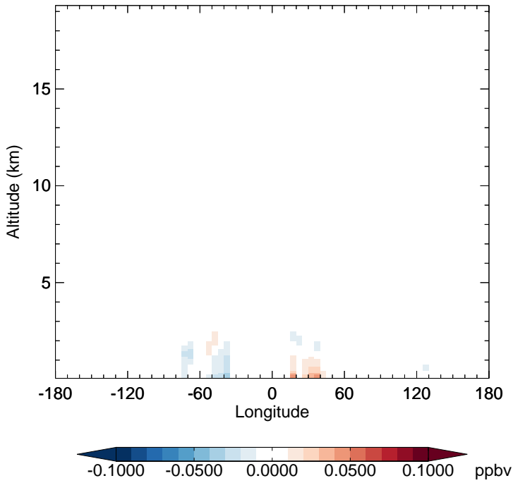
v11-02f-Run0 - v11-02e-Run0 SOAP - Diff along 15S for Apr
