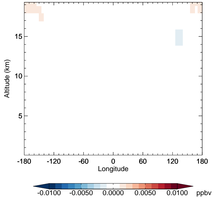
v11-02f-Run0 - v11-02e-Run0 BrNO3 - Diff along 42N for Apr
