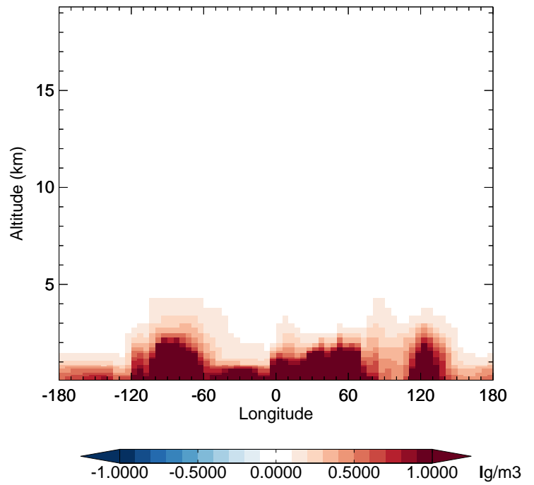
v11-02f-Run0 - v11-02e-Run0 NH3 - Diff along 42N for Apr
