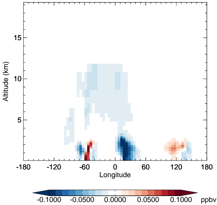
v11-02f-Run0 - v11-02e-Run0 ISO3 - Diff along 15S for Apr
