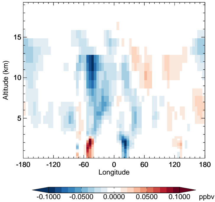
v11-02f-Run0 - v11-02e-Run0 PAN - Diff along 15S for Apr
