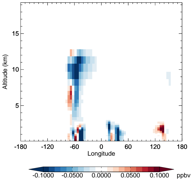
v11-02f-Run0 - v11-02e-Run0 IEPOXA - Diff along 15S for Apr
