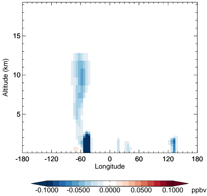
v11-02f-Run0 - v11-02e-Run1 IEPOXB - Diff along 15S for Apr
