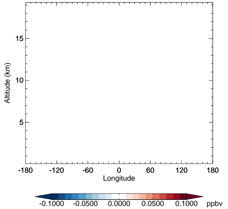
v11-02f-Run0 - v11-02e-Run0 TSOG2 - Diff along 42N for Apr
