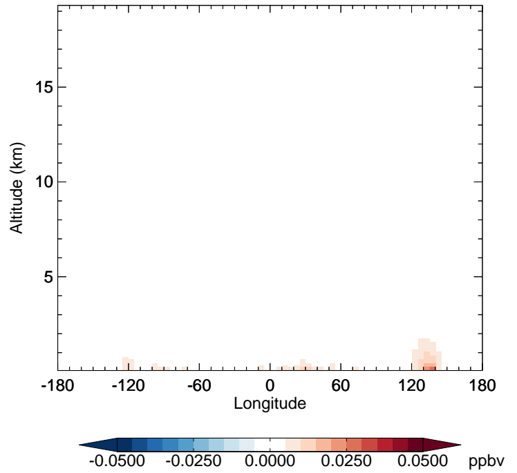
v11-02f-Run0 - v11-02e-Run0 RCHO - Diff along 42N for Apr
