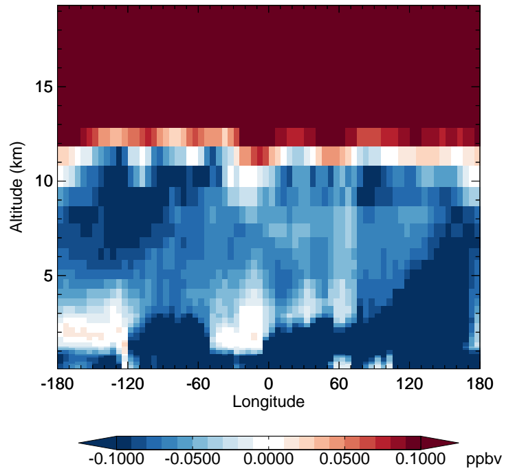
v11-02f-Run0 - v11-02e-Run1 HNO 3 - Diff along 42N for Apr
