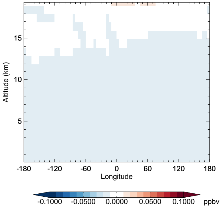
v11-02f-Run0 - v11-02e-Run0 CFC11 - Diff along 15S for Apr
