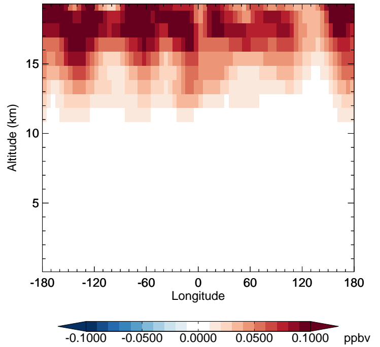
v11-02f-Run0 - v11-02e-Run0 HCl - Diff along 42N for Apr
