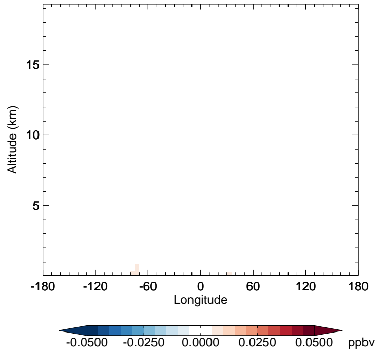
v11-02f-Run0 - v11-02e-Run1 MACR - Diff along 42N for Apr
