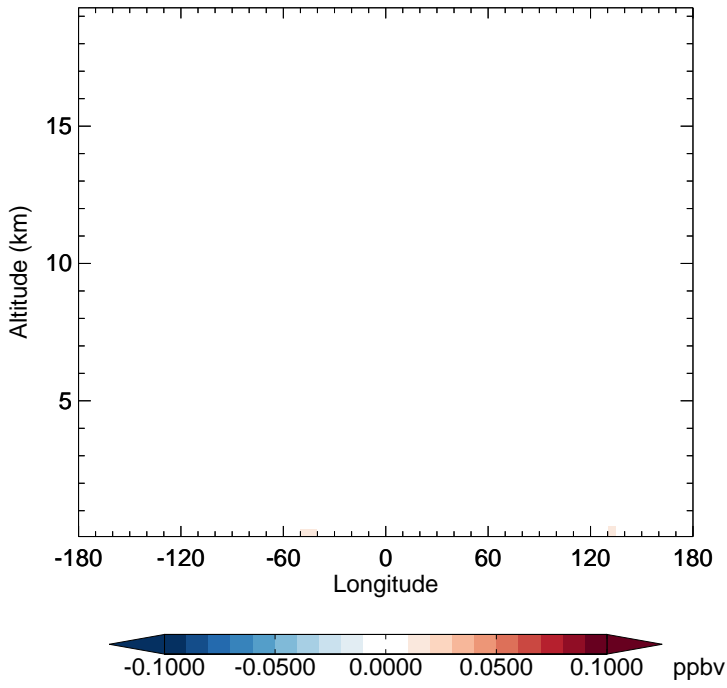
v11-02f-Run0 - v11-02e-Run1 MONITS - Diff along 15S for Apr
