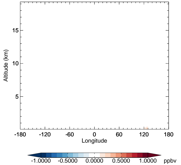
v11-02f-Run0 - v11-02e-Run0 HNO 2 - Diff along 42N for Apr
