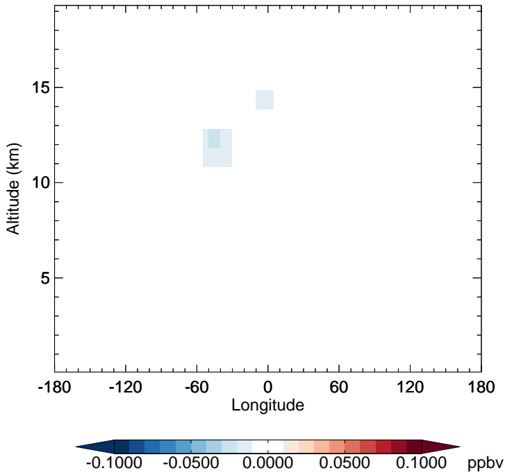
v11-02f-Run0 - v11-02e-Run0 ISOA3 - Diff along 15S for Apr
