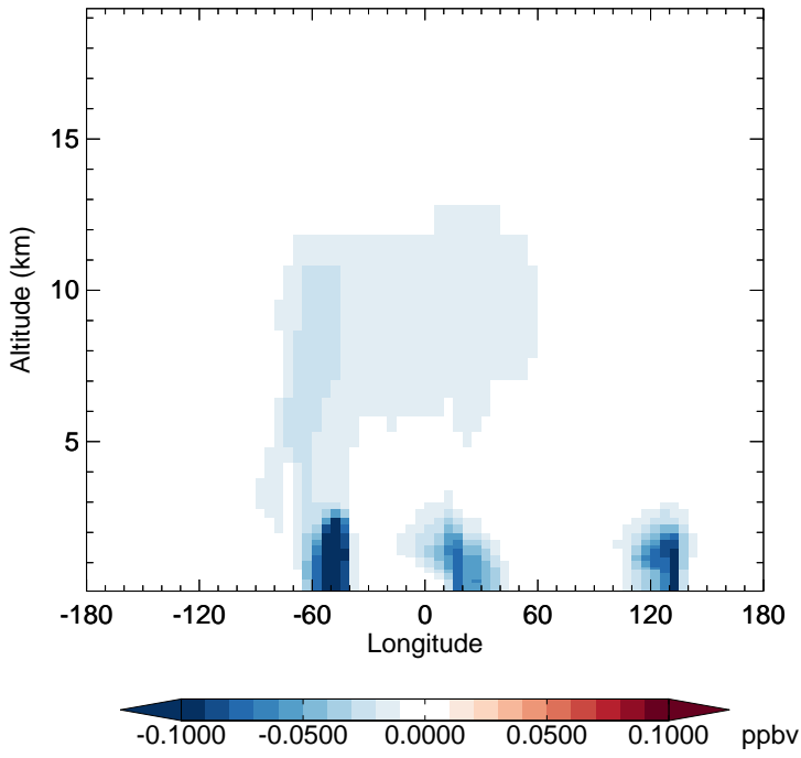
v11-02f-Run0 - v11-02e-Run1 ISO3 - Diff along 15S for Apr
