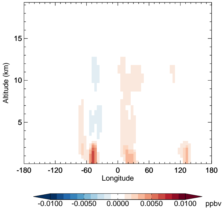
v11-02f-Run0 - v11-02e-Run0 R4N2 - Diff along 15S for Apr
