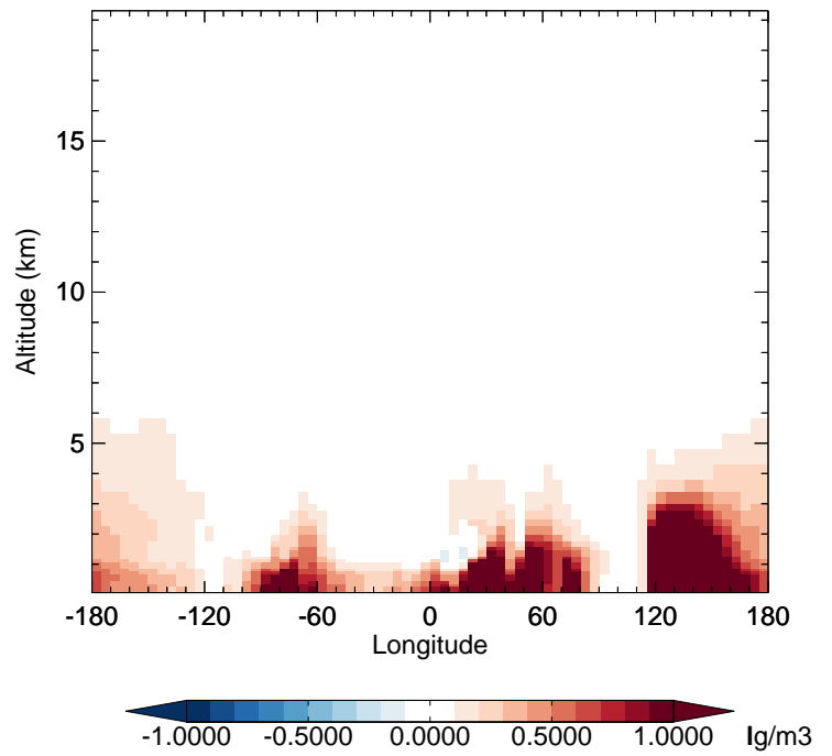
v11-02f-Run0 - v11-02e-Run0 NH4 - Diff along 42N for Apr
