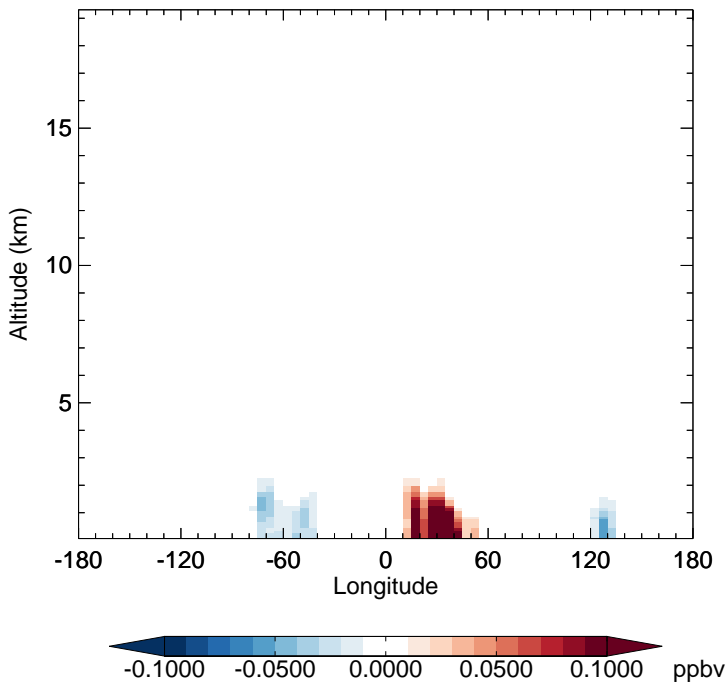
v11-02f-Run0 - v11-02e-Run0 TOLU - Diff along 15S for Apr
