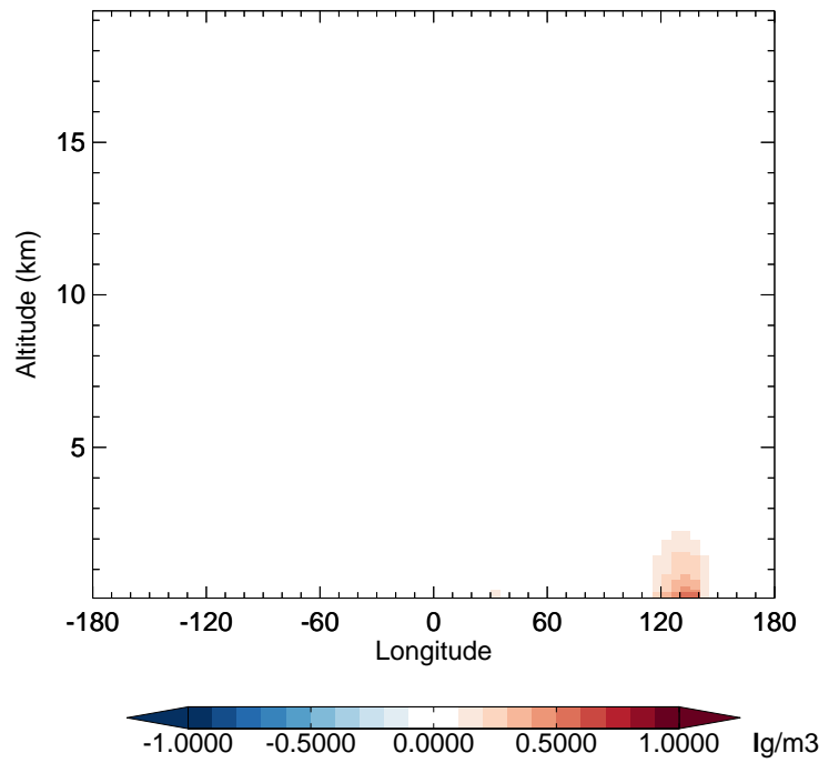
v11-02f-Run0 - v11-02e-Run0 OCPO - Diff along 42N for Apr
