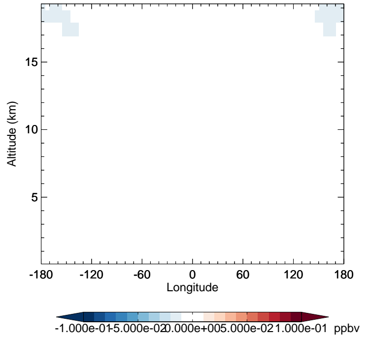
v11-02f-Run0 - v11-02e-Run0 CCI4 - Diff along 42N for Apr
