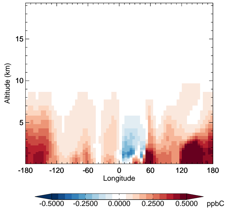
v11-02f-Run0 - v11-02e-Run0 C3H8 - Diff along 42N for Apr
