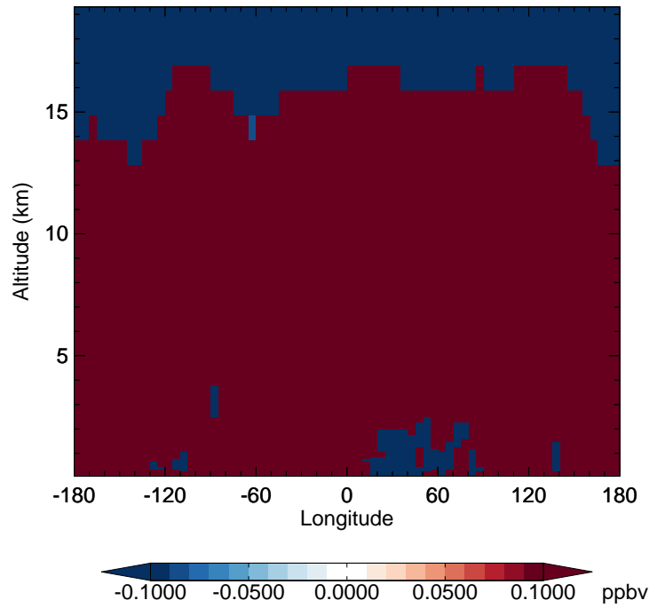
v11-02f-Run0 - v11-02e-Run0 CH4 - Diff along 42N for Apr
