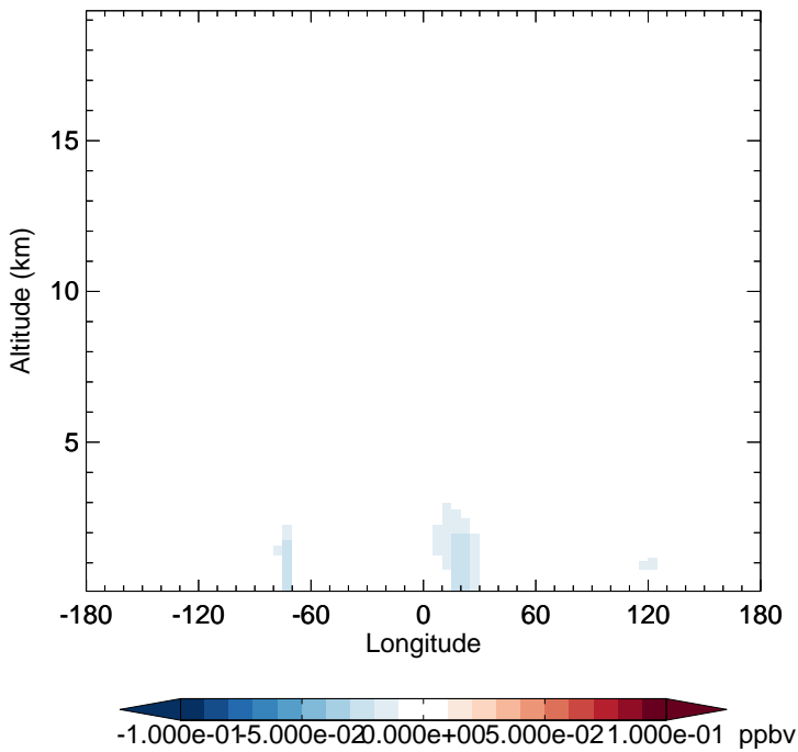
v11-02f-Run0 - v11-02e-Run0 SOAME - Diff along 15S for Apr
