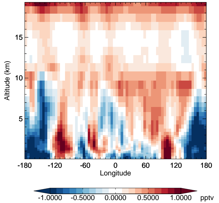
v11-02f-Run0 - v11-02e-Run0 HO2 - Diff along 42N for Apr
