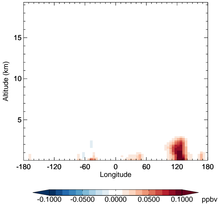
v11-02f-Run0 - v11-02e-Run1 TSOG3 - Diff along 15S for Apr
