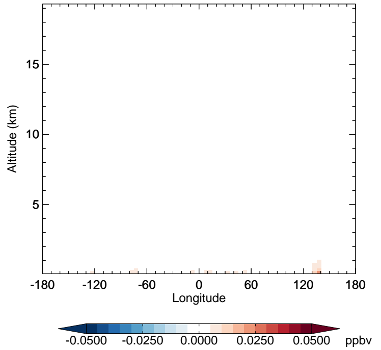
v11-02f-Run0 - v11-02e-Run1 RCHO - Diff along 42N for Apr
