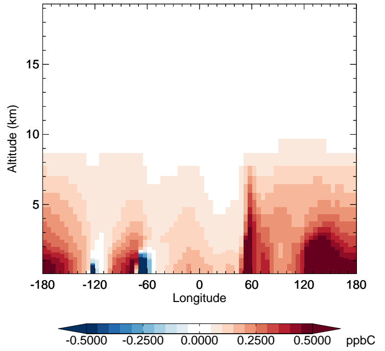
v11-02f-Run0 - v11-02e-Run1 ALK4 - Diff along 42N for Apr
