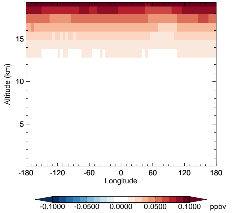
v11-02f-Run0 - v11-02e-Run1 N2O - Diff along 42N for Apr
