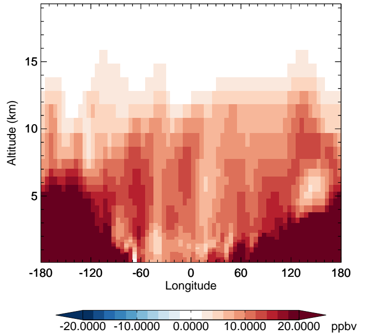
v11-02f-Run0 - v11-02e-Run0 CO - Diff along 42N for Apr
