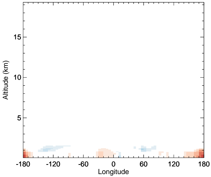
v11-02f-Run0 - v11-02e-Run0 SALA - Diff along 15S for Apr
