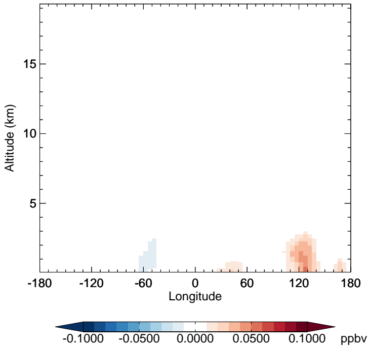
v11-02f-Run0 - v11-02e-Run1 TSOG2 - Diff along 15S for Apr
