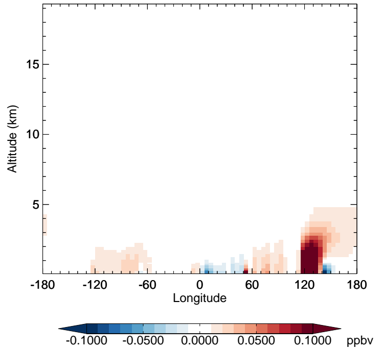
v11-02f-Run0 - v11-02e-Run1 EOH - Diff along 42N for Apr
