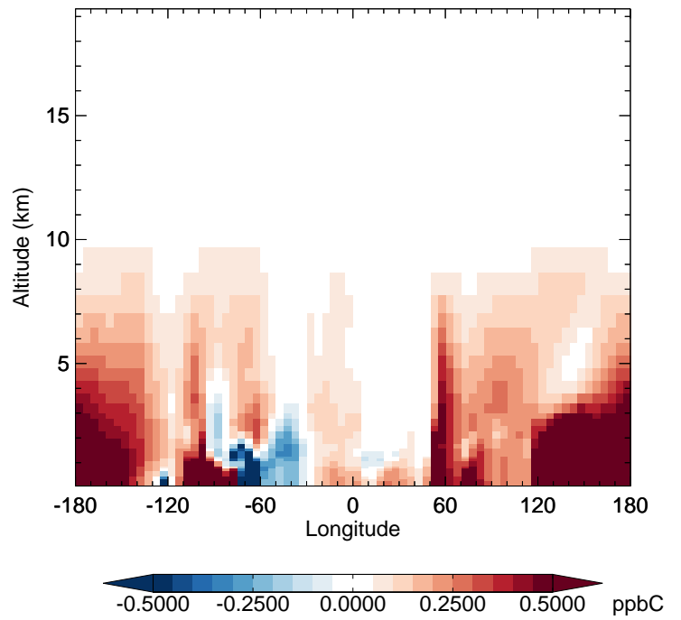
v11-02f-Run0 - v11-02e-Run0 ALK4 - Diff along 42N for Apr
