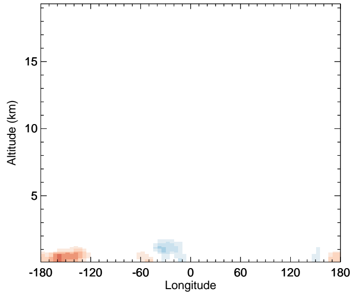
v11-02f-Run0 - v11-02e-Run0 SALA - Diff along 42N for Apr
