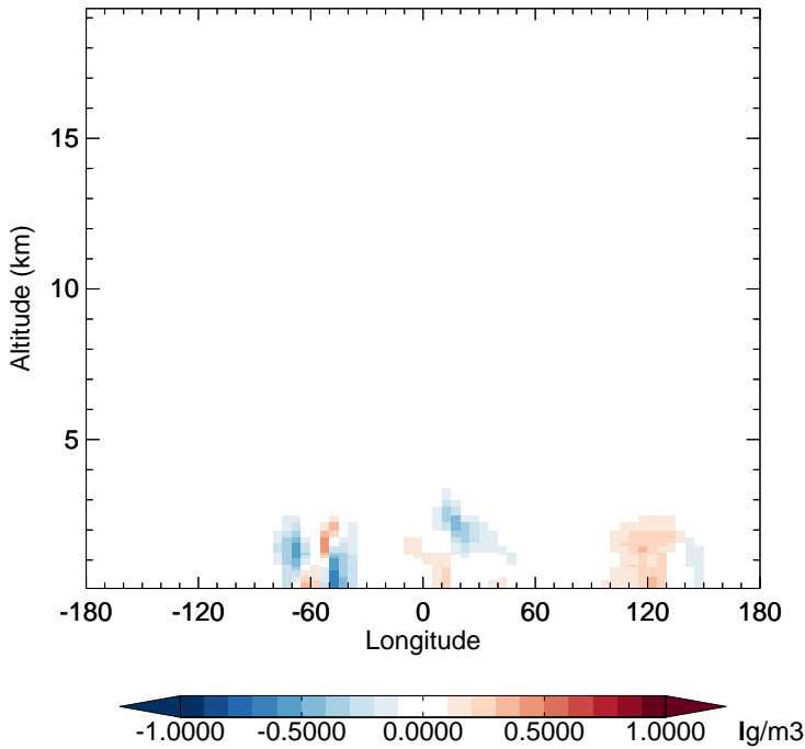
v11-02f-Run0 - v11-02e-Run0 SOAS - Diff along 15S for Apr
