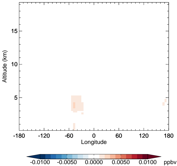
v11-02f-Run0 - v11-02e-Run0 NO3 - Diff along 15S for Apr
