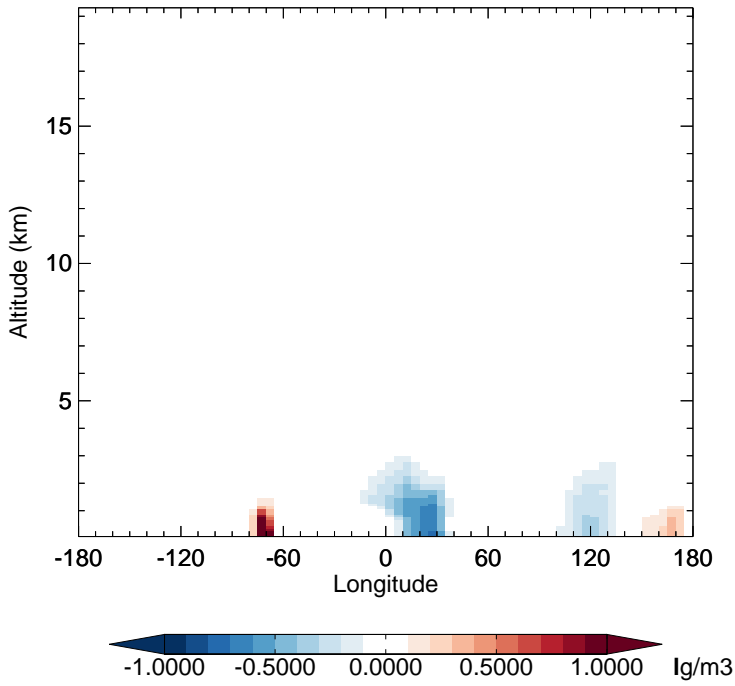
v11-02f-Run0 - v11-02e-Run1 SO4 - Diff along 15S for Apr
