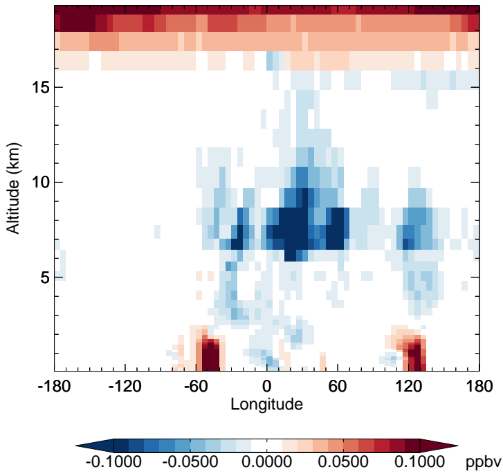
v11-02f-Run0 - v11-02e-Run1 HNO 3 - Diff along 15S for Apr
