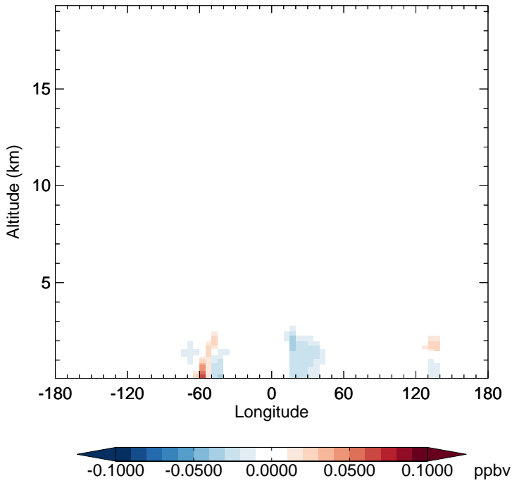
v11-02f-Run0 - v11-02e-Run0 MGLY - Diff along 15S for Apr
