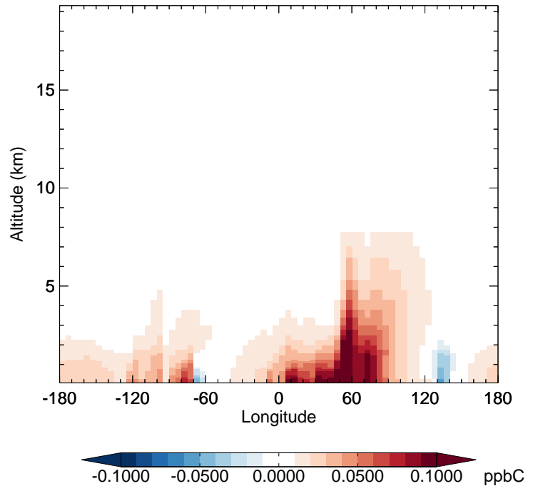
v11-02f-Run0 - v11-02e-Run1 MEK - Diff along 42N for Apr
