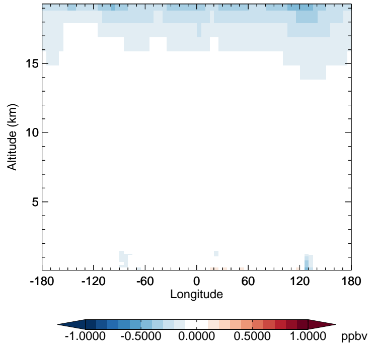
v11-02f-Run0 - v11-02e-Run0 NO 2 - Diff along 42N for Apr
