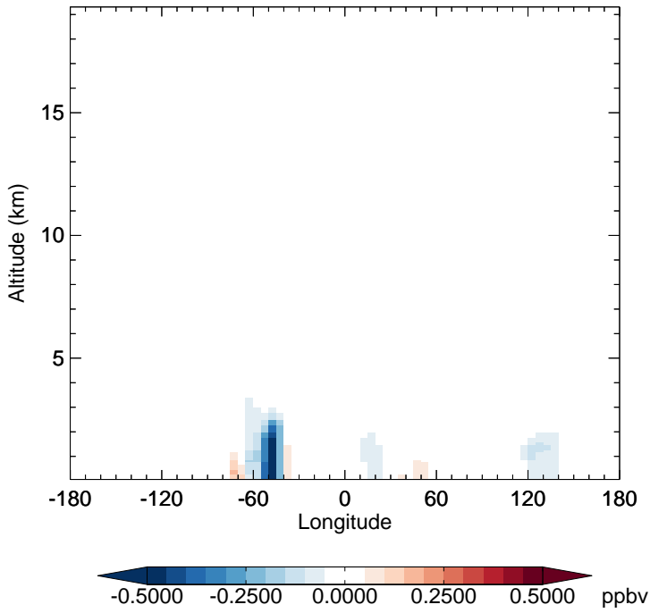
v11-02f-Run0 - v11-02e-Run1 CH 2 O - Diff along 15S for Apr
