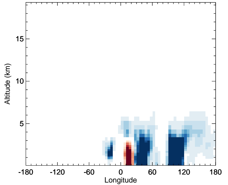
v11-02f-Run0 - v11-02e-Run0 DST2 - Diff along 42N for Apr
