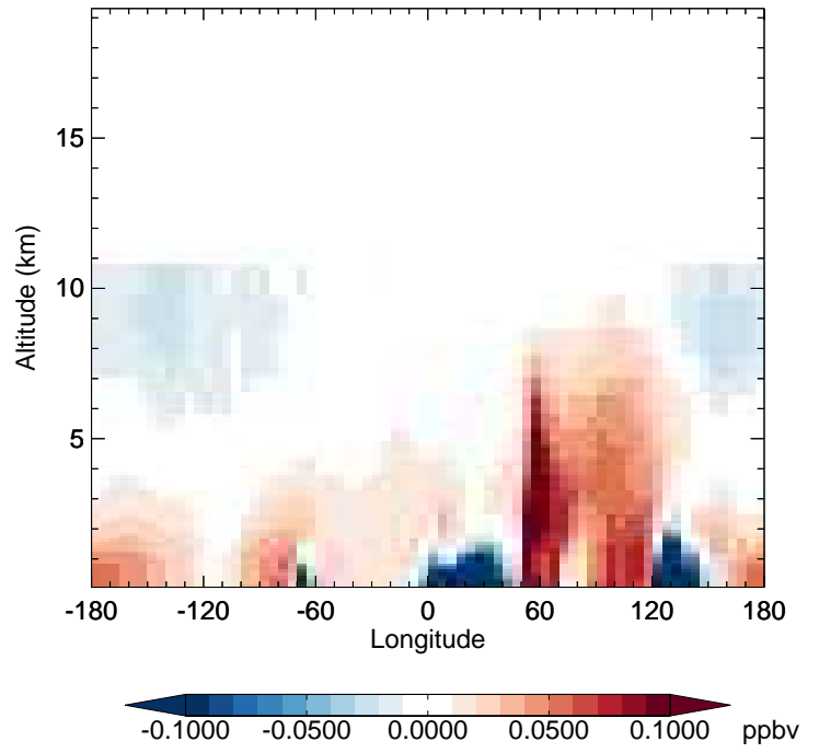
v11-02f-Run0 - v11-02e-Run1 BENZ - Diff along 42N for Apr
