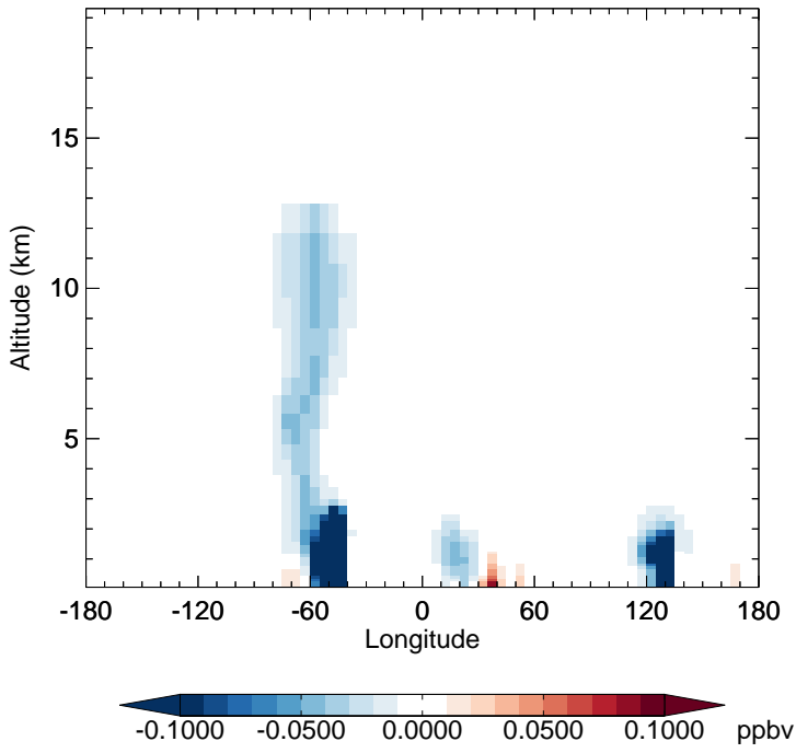
v11-02f-Run0 - v11-02e-Run1 HAC - Diff along 15S for Apr
