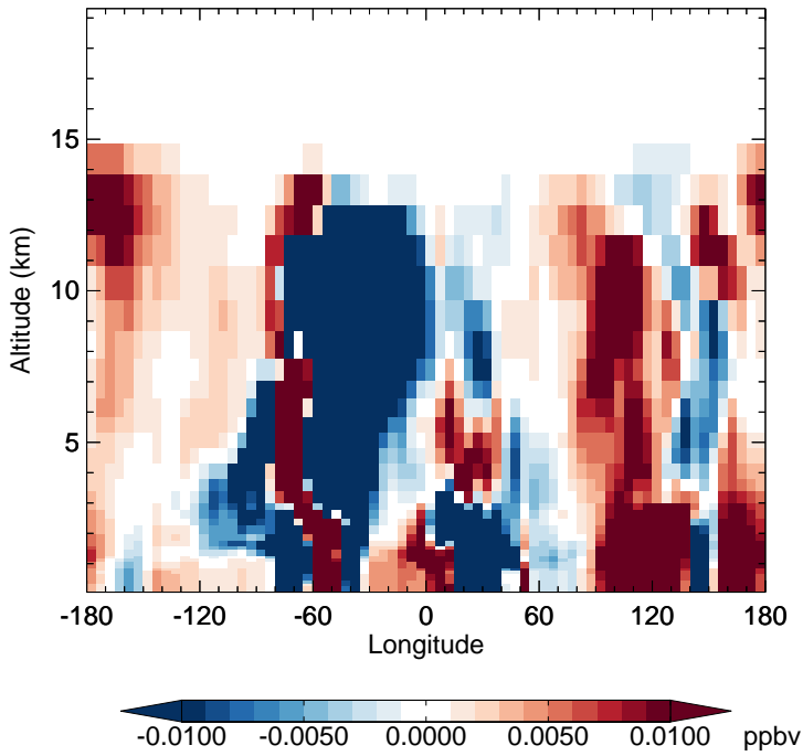
v11-02f-Run0 - v11-02e-Run0 MAP - Diff along 15S for Apr
