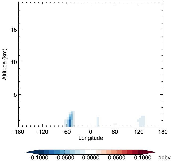
v11-02f-Run0 - v11-02e-Run1 ISOA1 - Diff along 15S for Apr
