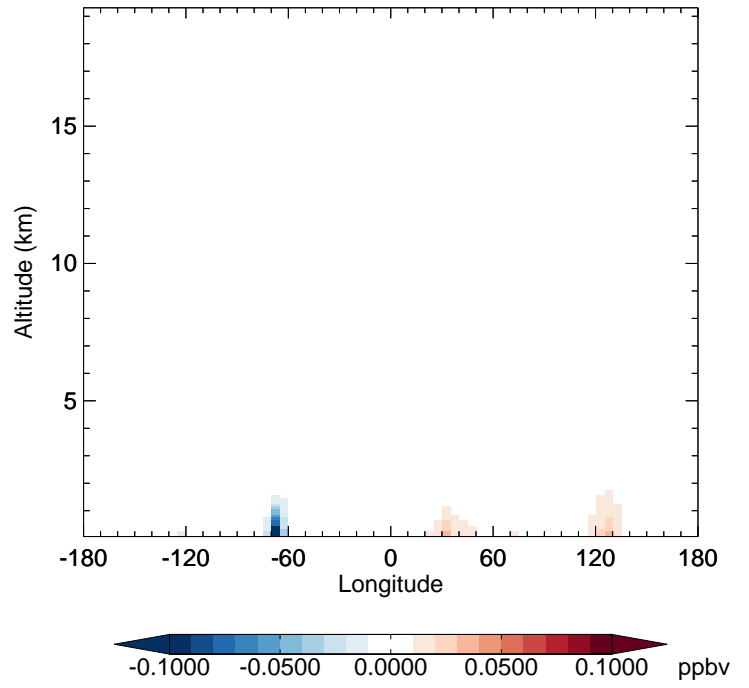
v11-02f-Run0 - v11-02e-Run1 SOAP - Diff along 42N for Apr
