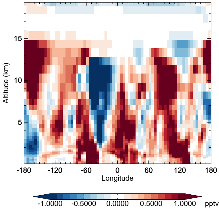
v11-02f-Run0 - v11-02e-Run0 HO2 - Diff along 15S for Apr
