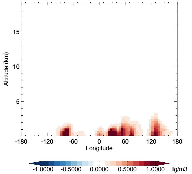
v11-02f-Run0 - v11-02e-Run1 SO4 - Diff along 42N for Apr
