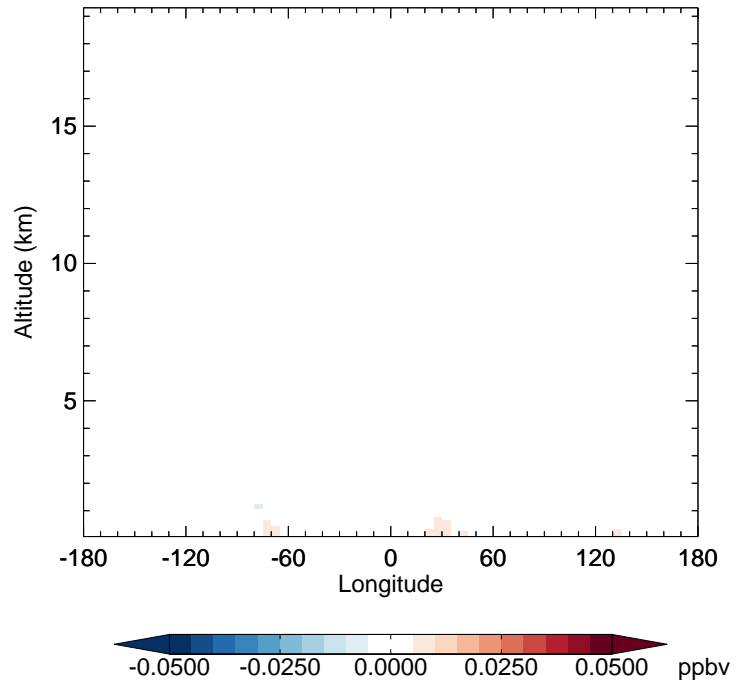
v11-02f-Run0 - v11-02e-Run0 MACR - Diff along 42N for Apr
