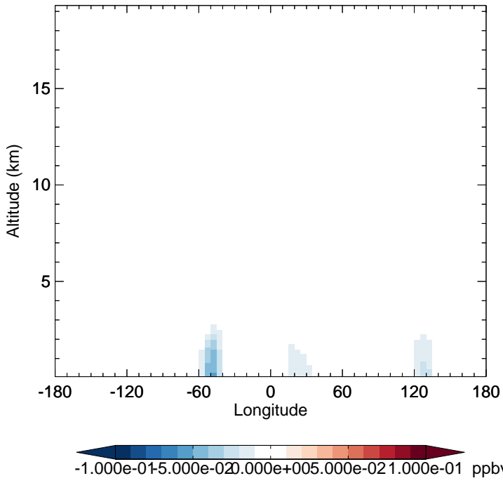
v11-02f-Run0 - v11-02e-Run1 MONITA - Diff along 15S for Apr
