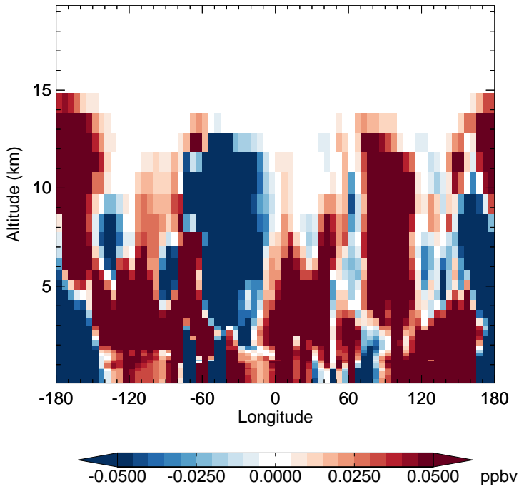
v11-02f-Run0 - v11-02e-Run0 MP - Diff along 15S for Apr
