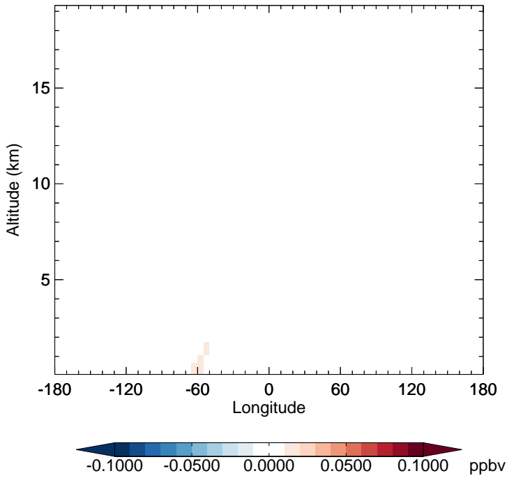
v11-02f-Run0 - v11-02e-Run0 TSOA1 - Diff along 15S for Apr
