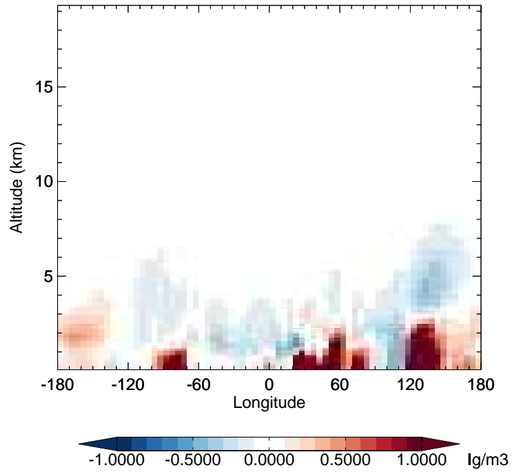
v11-02f-Run0 - v11-02e-Run0 SO4 - Diff along 42N for Apr
