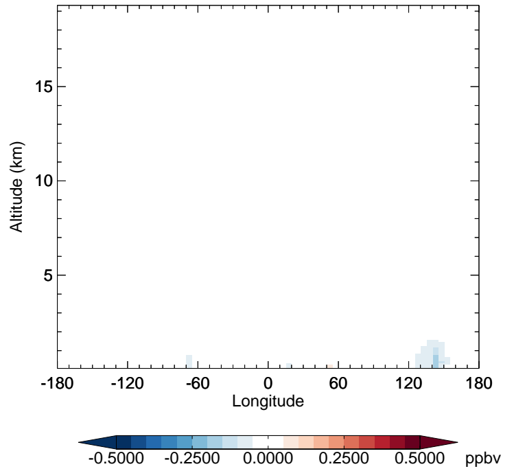
v11-02f-Run0 - v11-02e-Run1 CH 2 O - Diff along 42N for Apr
