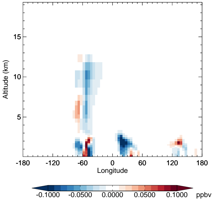
v11-02f-Run0 - v11-02e-Run0 HAC - Diff along 15S for Apr
