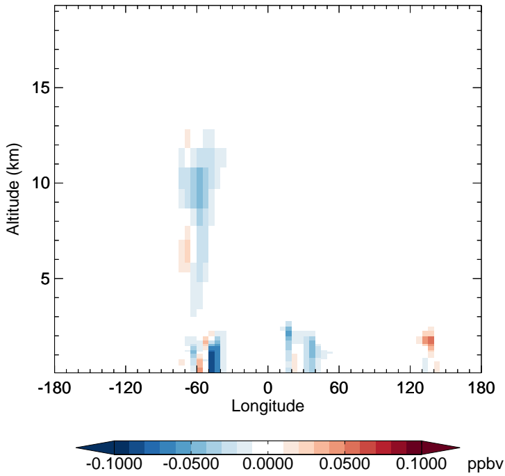
v11-02f-Run0 - v11-02e-Run0 IEPOXB - Diff along 15S for Apr
