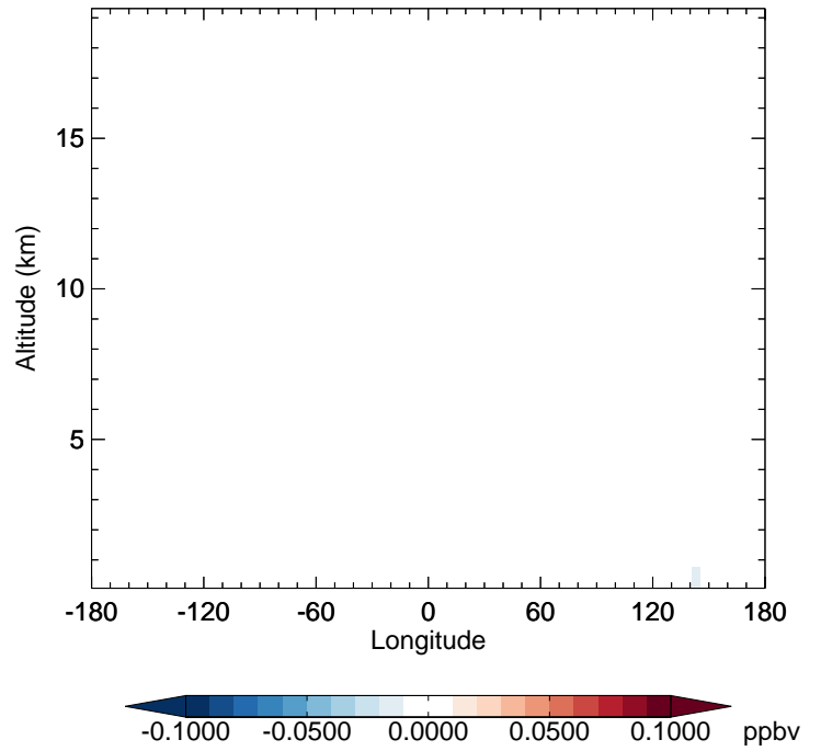
v11-02f-Run0 - v11-02e-Run0 MGLY - Diff along 42N for Apr
