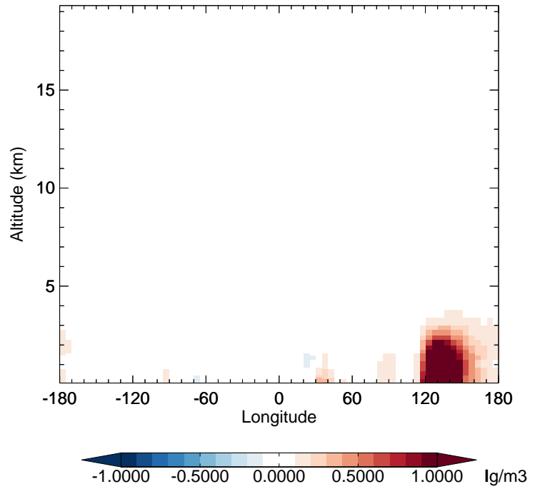
v11-02f-Run0 - v11-02e-Run0 OCPI - Diff along 42N for Apr
