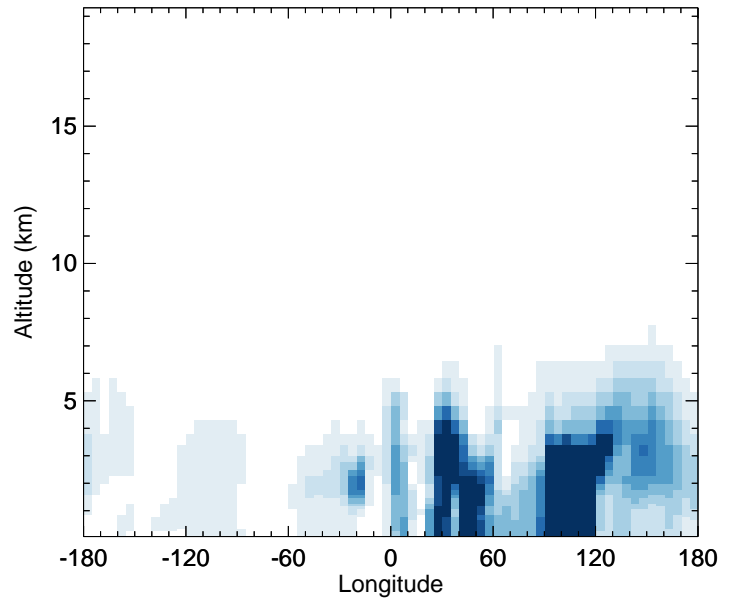
v11-02f-Run0 - v11-02e-Run0 DST1 - Diff along 42N for Apr
