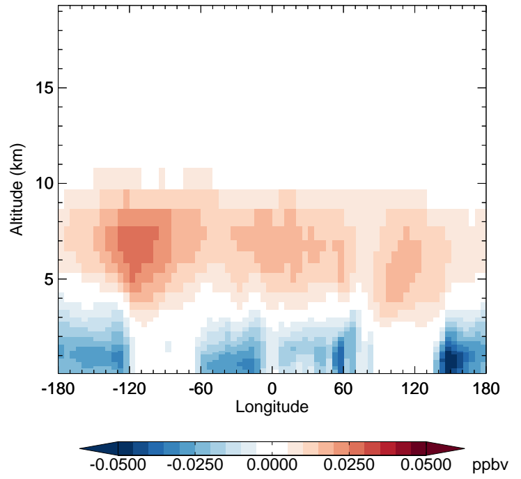
v11-02f-Run0 - v11-02e-Run1 MP - Diff along 42N for Apr
