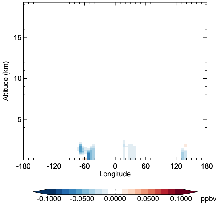
v11-02f-Run0 - v11-02e-Run0 RIPB - Diff along 15S for Apr
