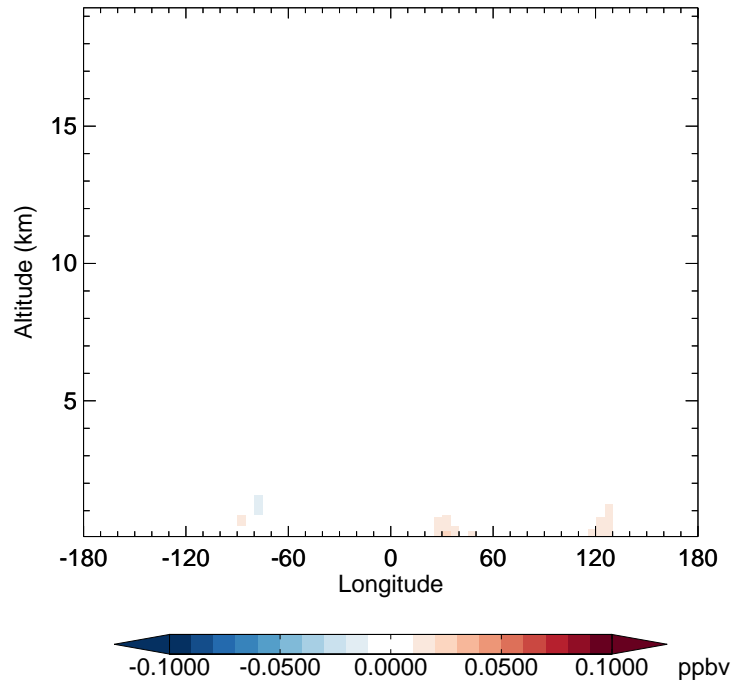
v11-02f-Run0 - v11-02e-Run0 GLYC - Diff along 42N for Apr
