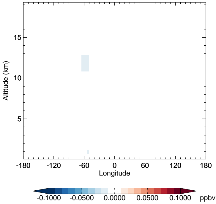
v11-02f-Run0 - v11-02e-Run1 ISOA3 - Diff along 15S for Apr
