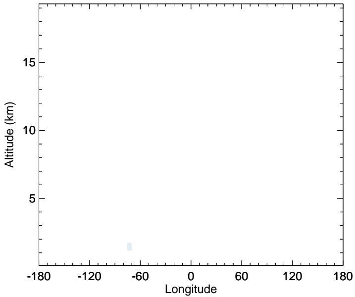
v11-02f-Run0 - v11-02e-Run0 HCFC22 - Diff along 15S for Apr
