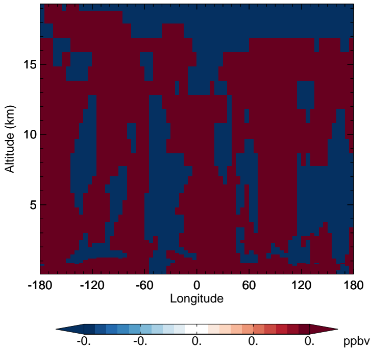
v11-02f-Run0 - v11-02e-Run0 H2O - Diff along 15S for Apr
