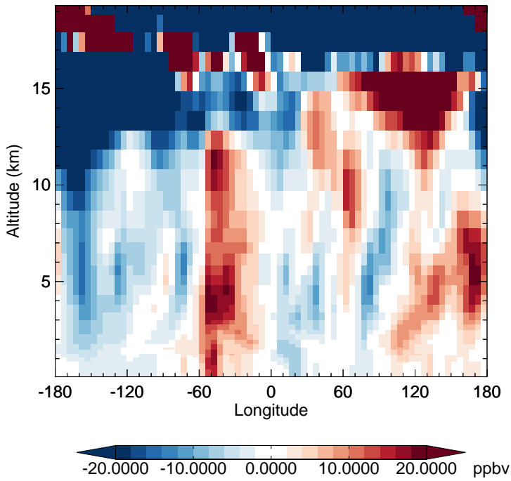
v11-02f-Run0 - v11-02e-Run0 O3 - Diff along 15S for Apr
