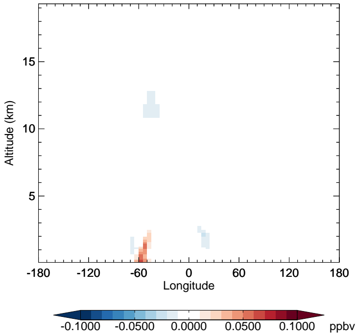
v11-02f-Run0 - v11-02e-Run0 TSOA2 - Diff along 15S for Apr
