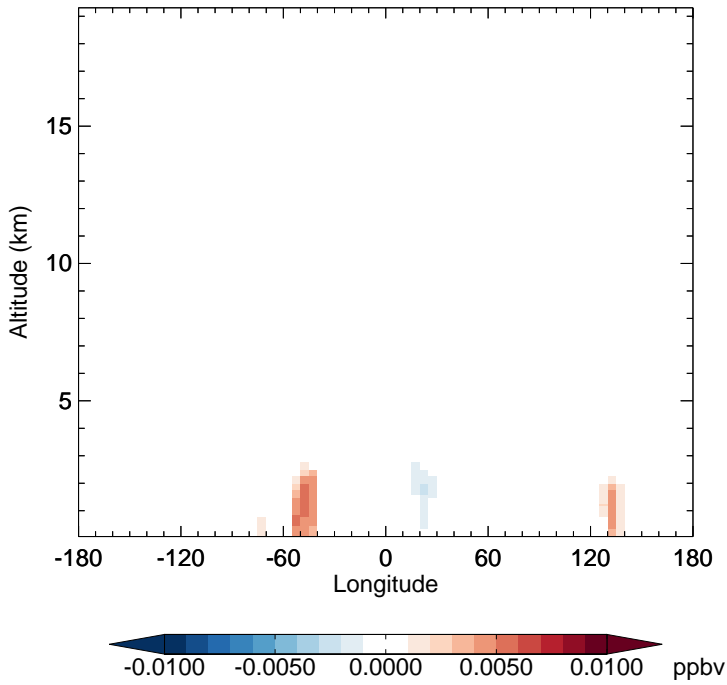
v11-02f-Run0 - v11-02e-Run0 MVKN - Diff along 15S for Apr
