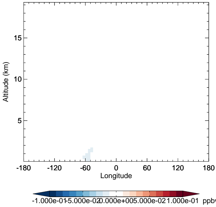
v11-02f-Run0 - v11-02e-Run1 RIPD - Diff along 15S for Apr
