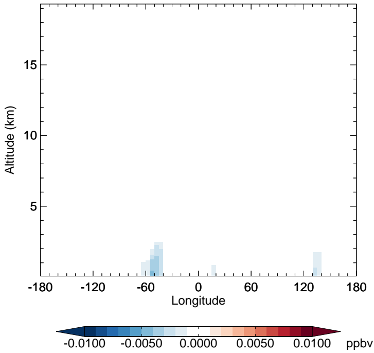
v11-02f-Run0 - v11-02e-Run1 MOBA - Diff along 15S for Apr
