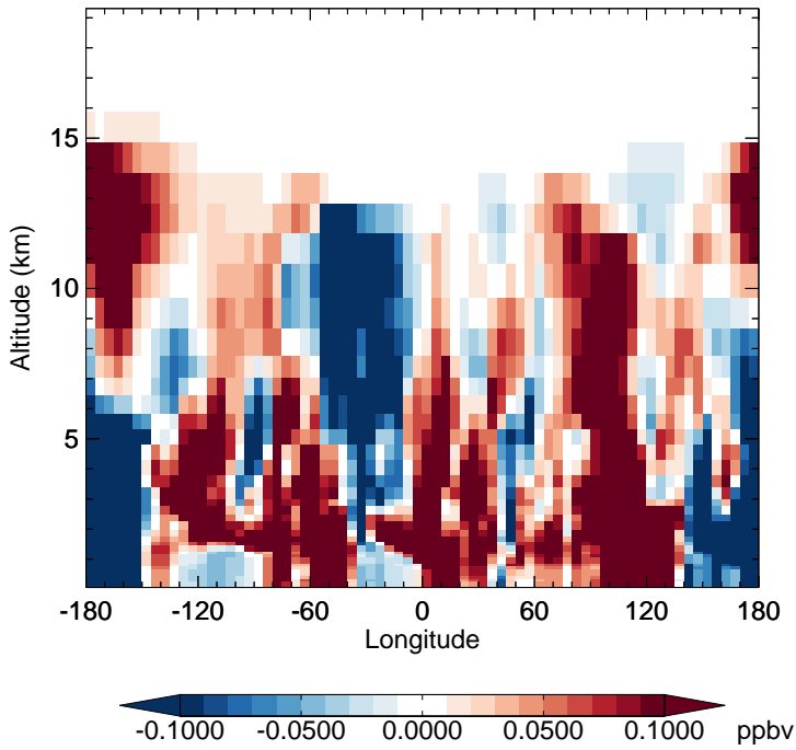
v11-02f-Run0 - v11-02e-Run0 H2O2 - Diff along 15S for Apr
