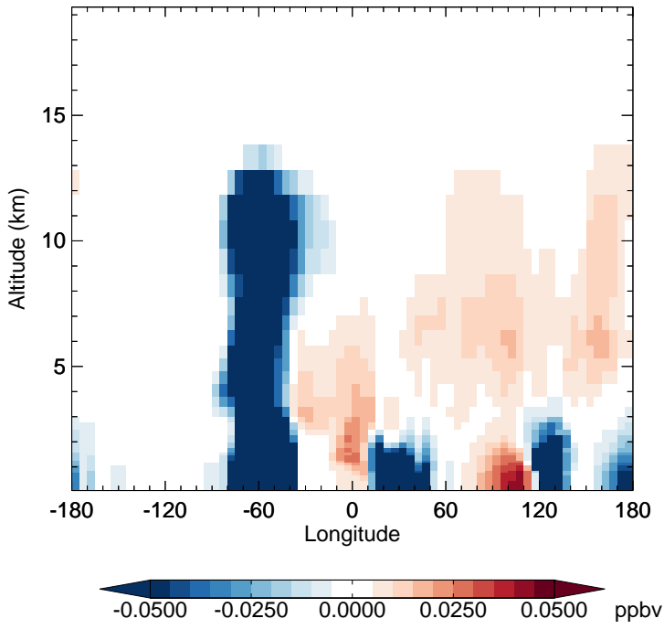
v11-02f-Run0 - v11-02e-Run1 MP - Diff along 15S for Apr
