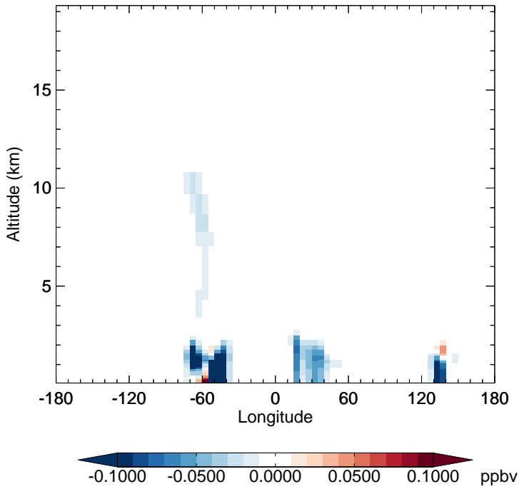
v11-02f-Run0 - v11-02e-Run0 RIPA - Diff along 15S for Apr
