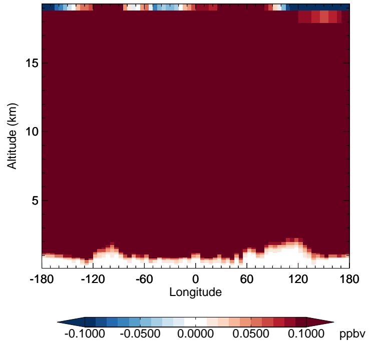
v11-02f-Run0 - v11-02e-Run1 CH4 - Diff along 42N for Apr
