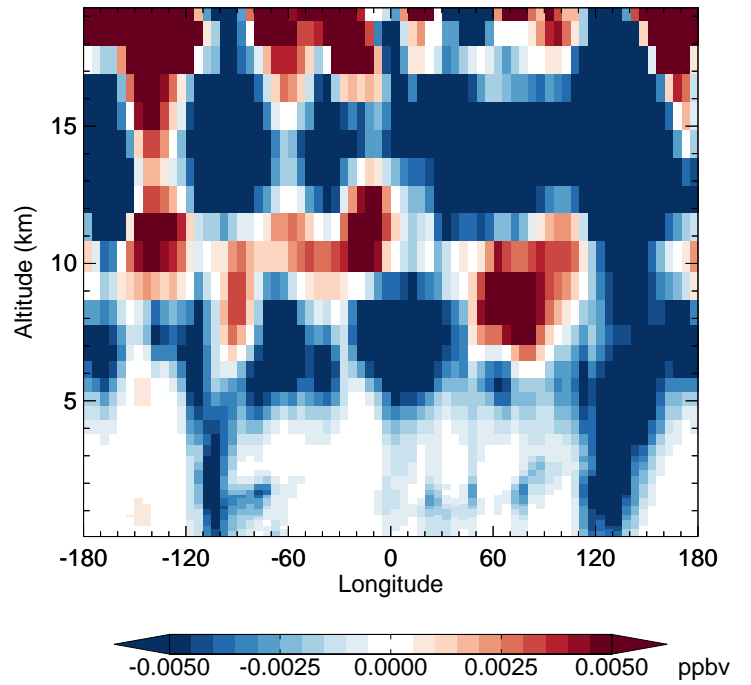
v11-02f-Run0 - v11-02e-Run0 HNO 4 - Diff along 42N for Apr
