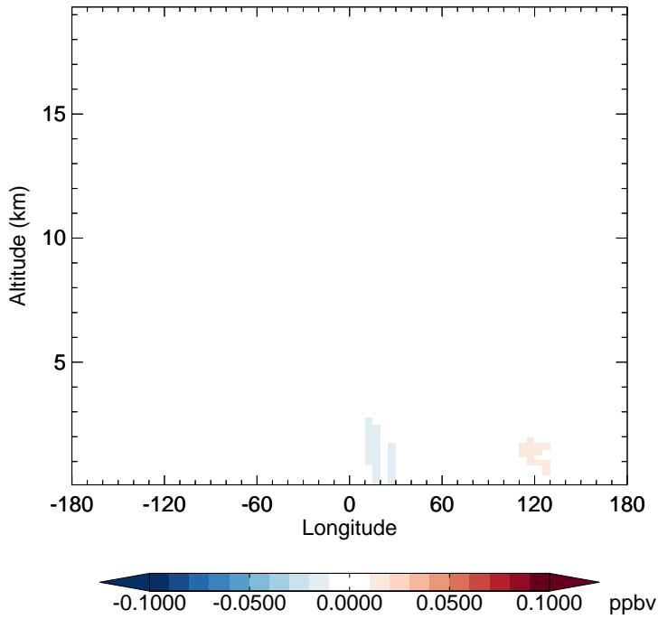
v11-02f-Run0 - v11-02e-Run0 ISOG1 - Diff along 15S for Apr
