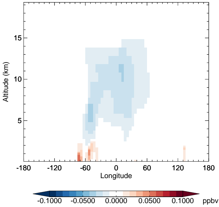
v11-02f-Run0 - v11-02e-Run1 PAN - Diff along 15S for Apr
