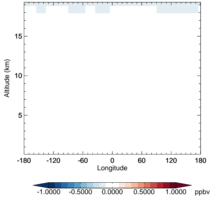
v11-02f-Run0 - v11-02e-Run0 NO - Diff along 42N for Apr
