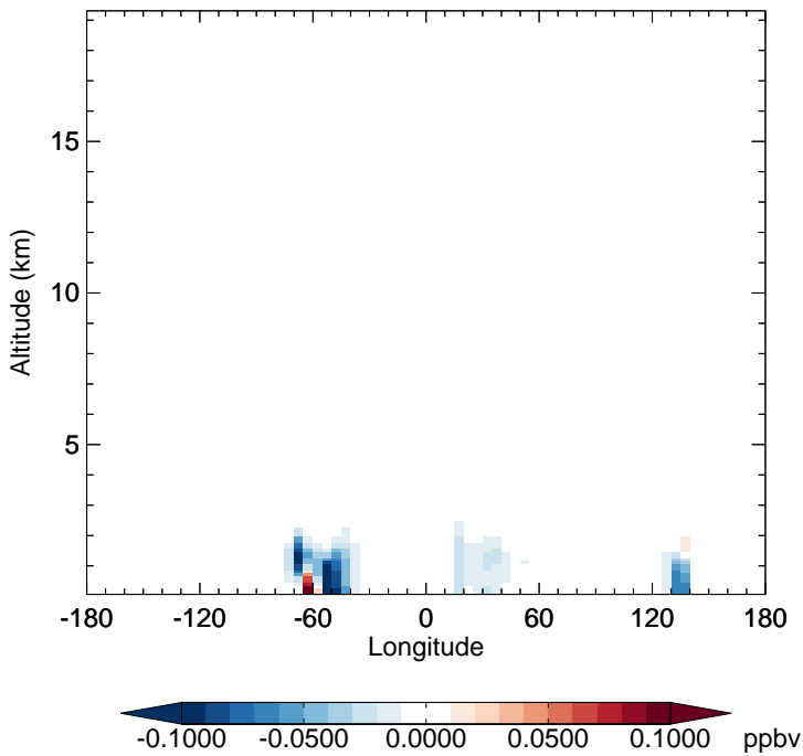
v11-02f-Run0 - v11-02e-Run0 HPALD - Diff along 15S for Apr
