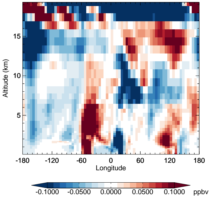
v11-02f-Run0 - v11-02e-Run0 HNO 3 - Diff along 15S for Apr
