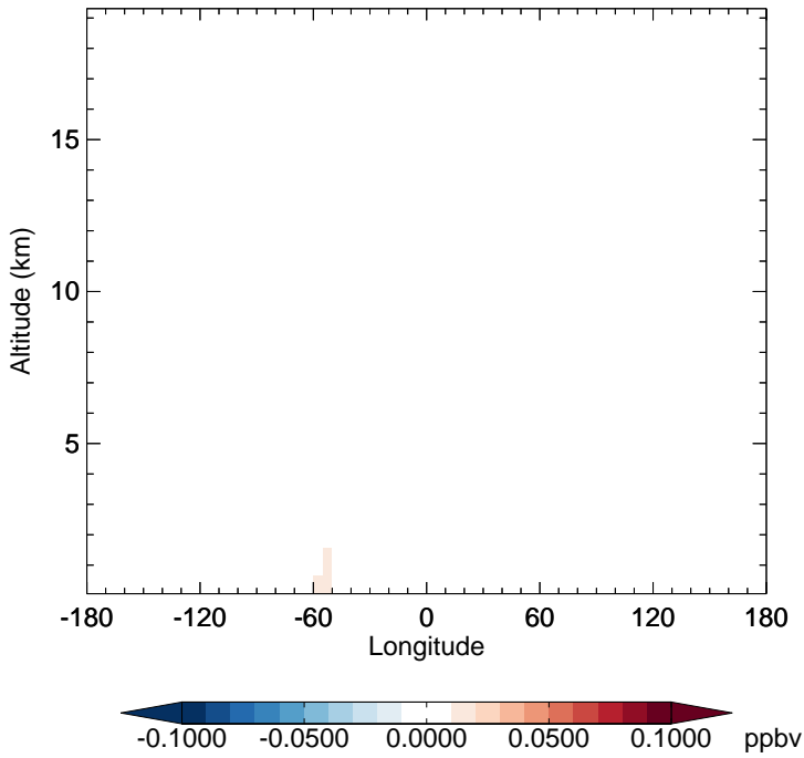
v11-02f-Run0 - v11-02e-Run0 TSOA3 - Diff along 15S for Apr
