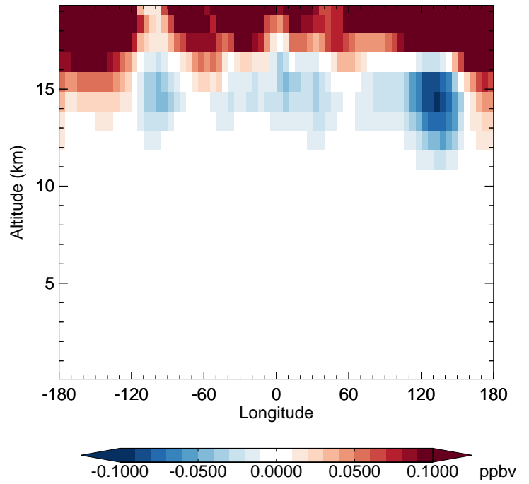
v11-02f-Run0 - v11-02e-Run0 CINO3 - Diff along 42N for Apr
