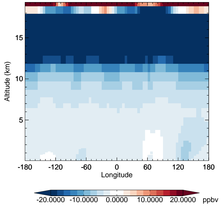
v11-02f-Run0 - v11-02e-Run1 O3 - Diff along 42N for Apr
