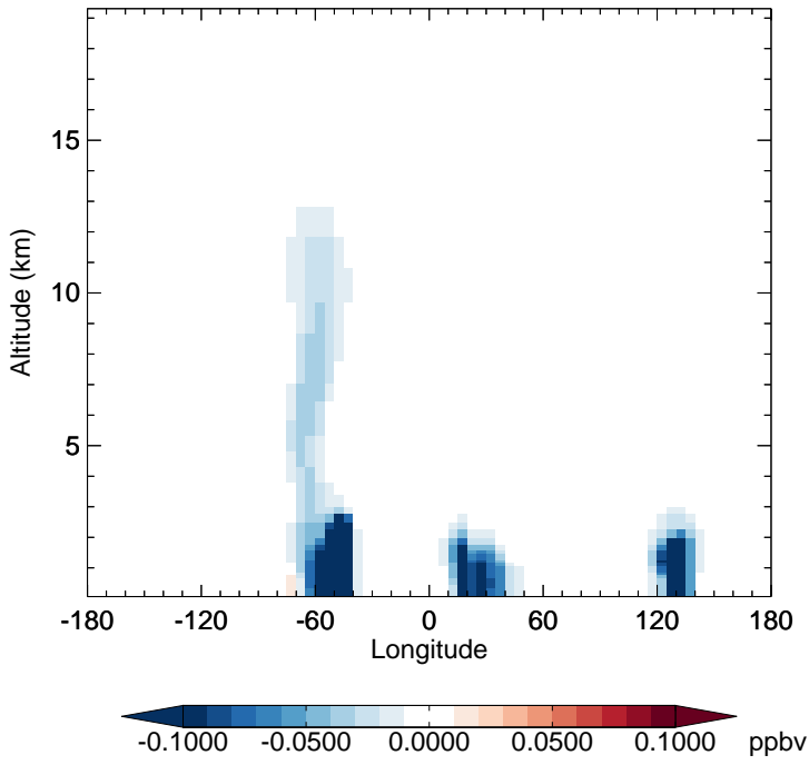
v11-02f-Run0 - v11-02e-Run1 GLYC - Diff along 15S for Apr
