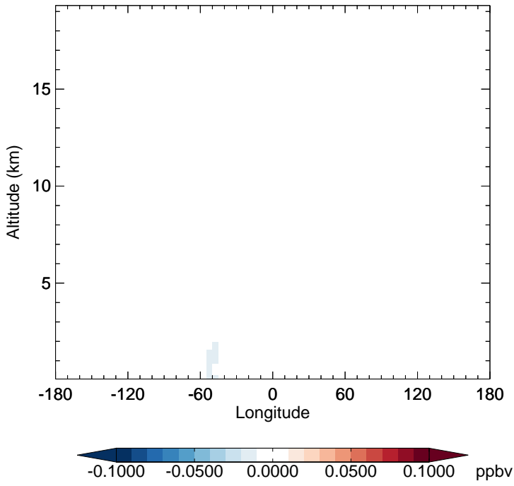
v11-02f-Run0 - v11-02e-Run1 LVOCOA - Diff along 15S for Apr
