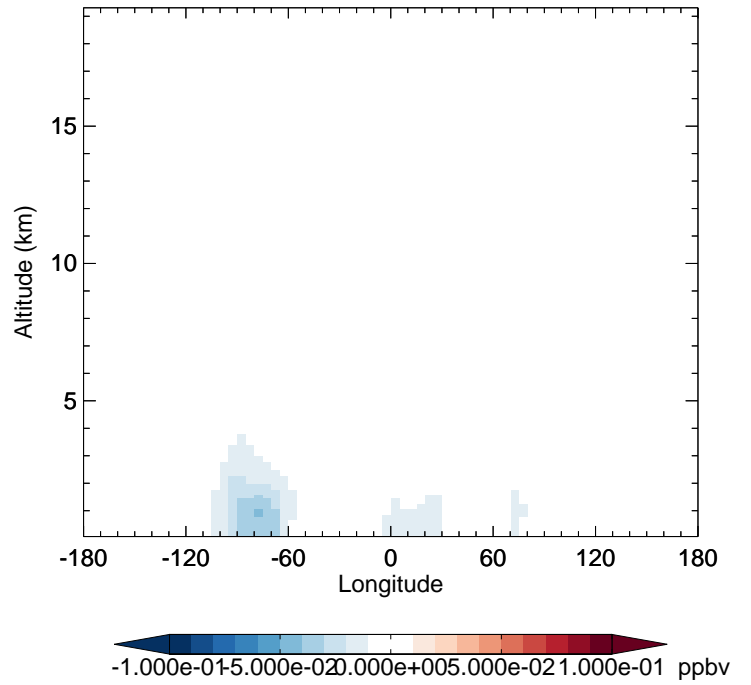
v11-02f-Run0 - v11-02e-Run0 IONITA - Diff along 42N for Apr
