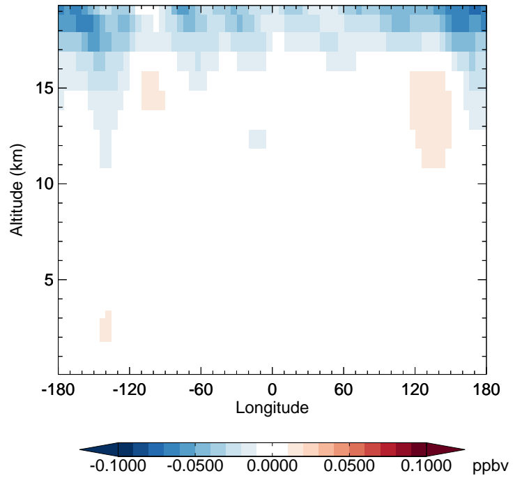
v11-02f-Run0 - v11-02e-Run0 CH3Cl - Diff along 42N for Apr
