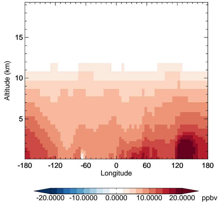
v11-02f-Run0 - v11-02e-Run1 CO - Diff along 42N for Apr
