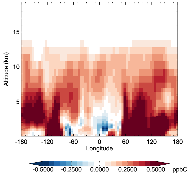
v11-02f-Run0 - v11-02e-Run0 ACET - Diff along 42N for Apr
