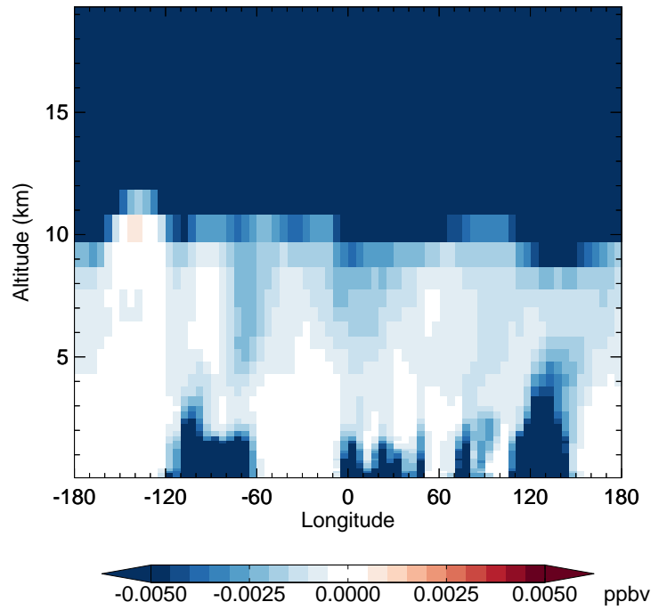
v11-02f-Run0 - v11-02e-Run0 N2O5 - Diff along 42N for Apr
