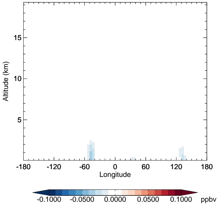
v11-02f-Run0 - v11-02e-Run1 GLYX - Diff along 15S for Apr
