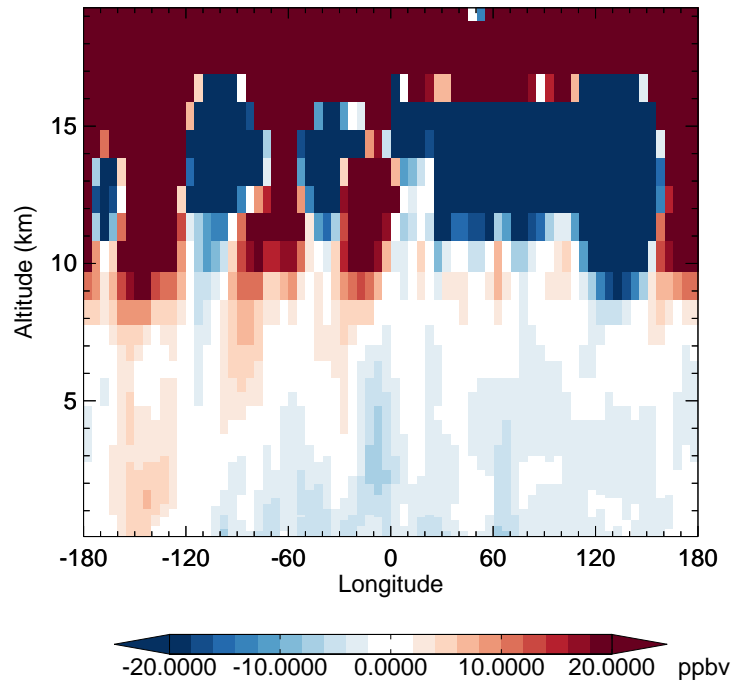
v11-02f-Run0 - v11-02e-Run0 O3 - Diff along 42N for Apr
