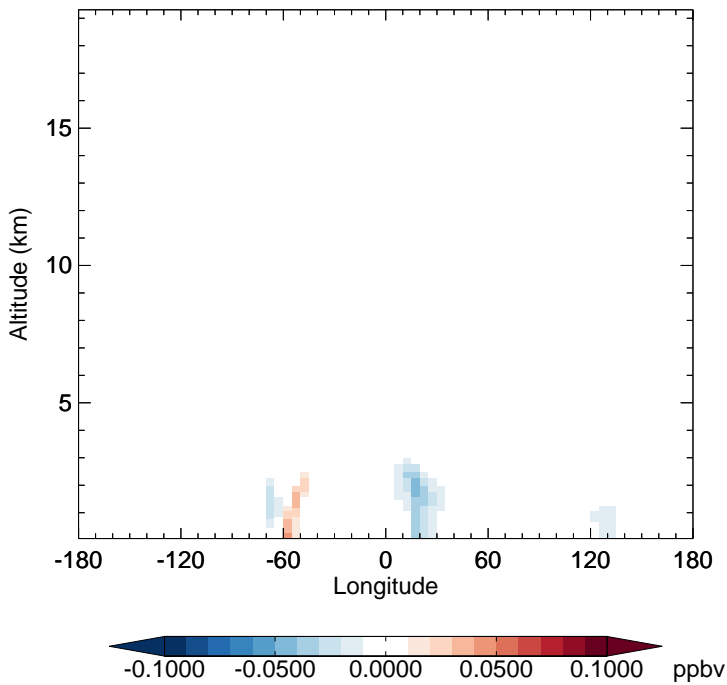
v11-02f-Run0 - v11-02e-Run0 ISOA1 - Diff along 15S for Apr
