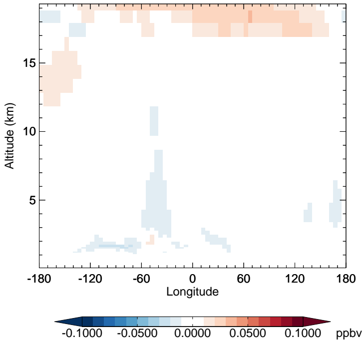
v11-02f-Run0 - v11-02e-Run0 CH3Cl - Diff along 15S for Apr
