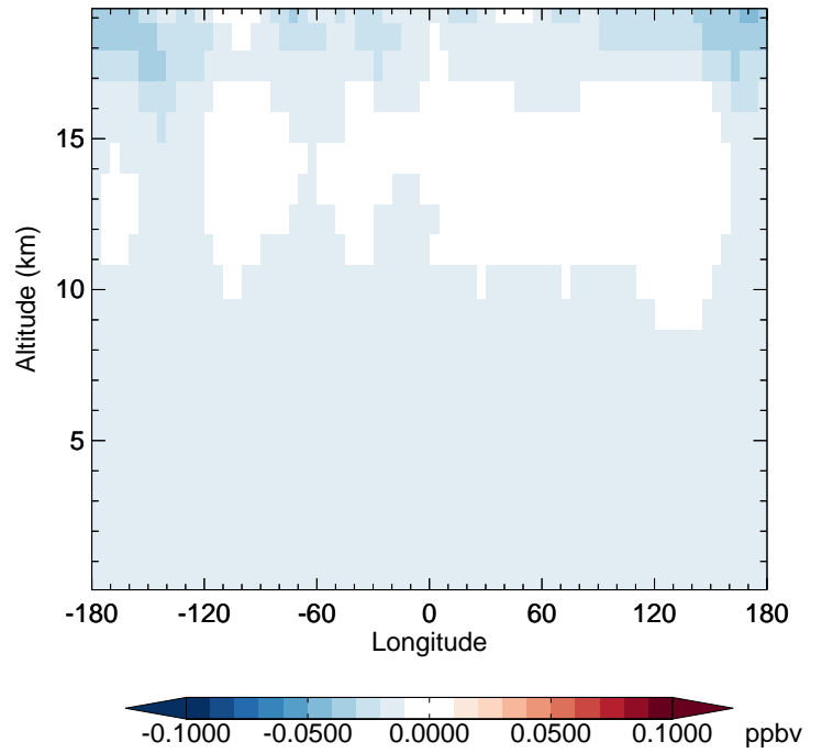
v11-02f-Run0 - v11-02e-Run0 CFC11 - Diff along 42N for Apr
