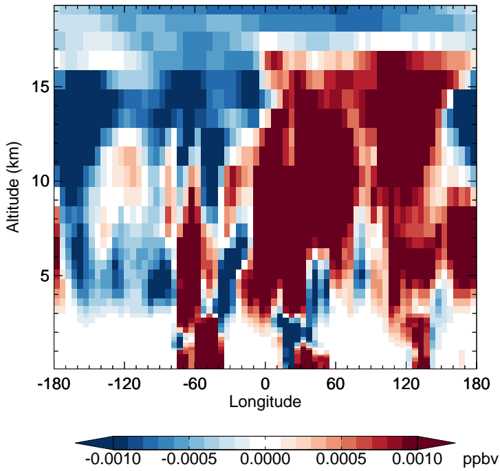
v11-02f-Run0 - v11-02e-Run0 PPN - Diff along 15S for Apr
