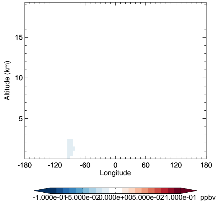
v11-02f-Run0 - v11-02e-Run1 SOAIE - Diff along 42N for Apr
