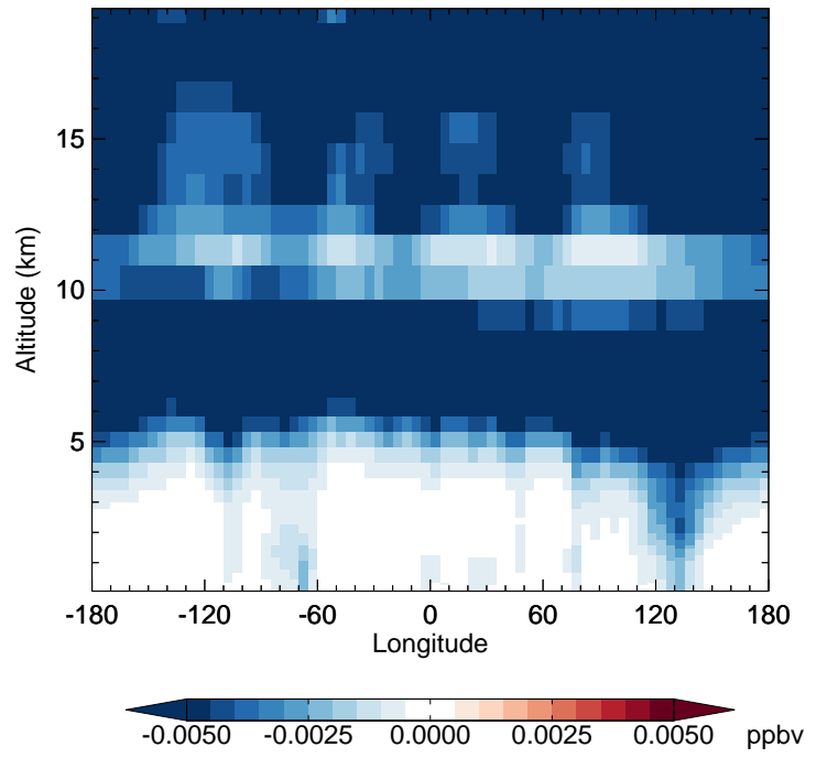
v11-02f-Run0 - v11-02e-Run1 HNO 4 - Diff along 42N for Apr
