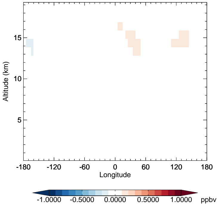
v11-02f-Run0 - v11-02e-Run0 NO - Diff along 15S for Apr
