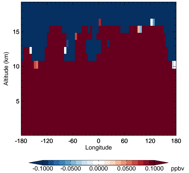
v11-02f-Run0 - v11-02e-Run0 N2O - Diff along 42N for Apr
