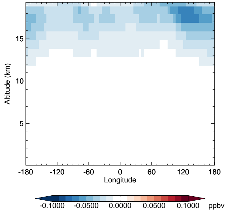
v11-02f-Run0 - v11-02e-Run1 CINO3 - Diff along 42N for Apr
