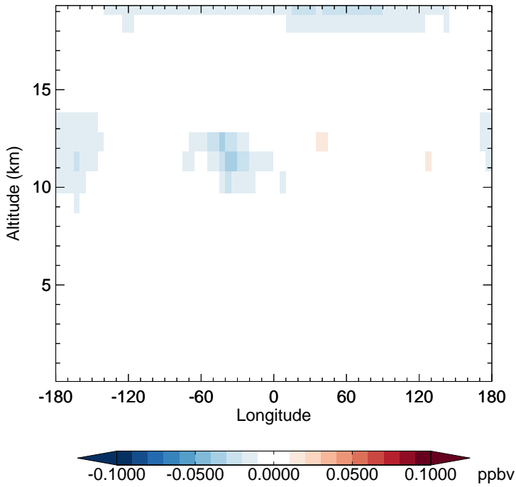
v11-02f-Run0 - v11-02e-Run0 MPN - Diff along 15S for Apr
