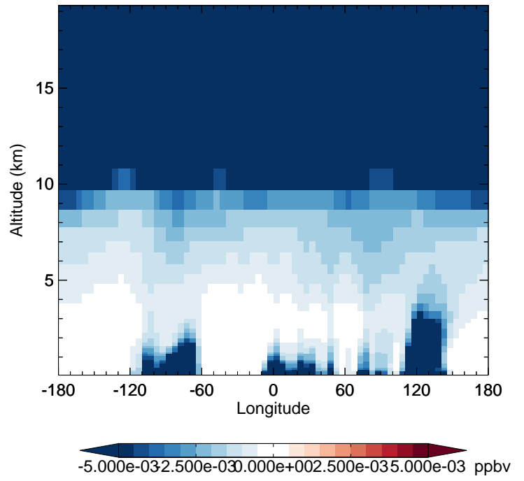
v11-02f-Run0 - v11-02e-Run1 N2O5 - Diff along 42N for Apr
