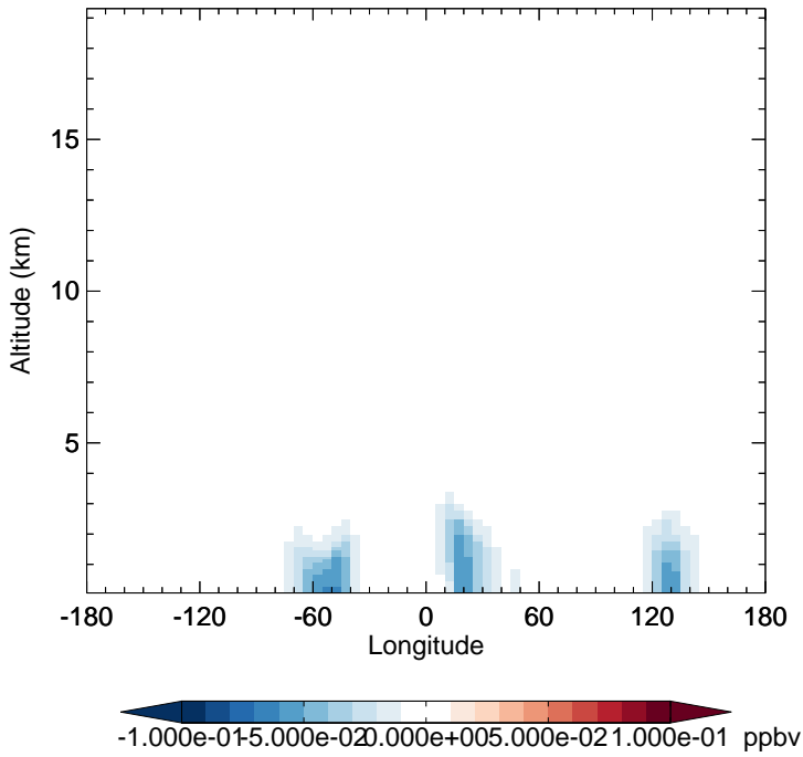
v11-02f-Run0 - v11-02e-Run0 IONITA - Diff along 15S for Apr
