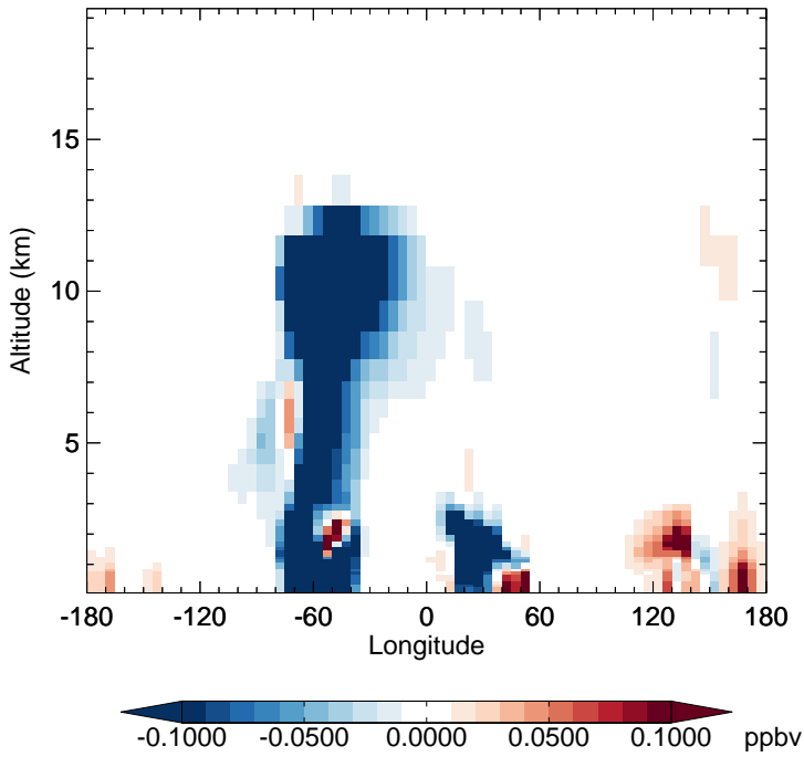
v11-02f-Run0 - v11-02e-Run0 EOH - Diff along 15S for Apr
