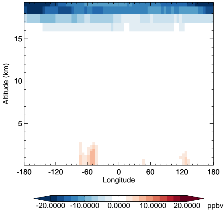
v11-02f-Run0 - v11-02e-Run1 O3 - Diff along 15S for Apr
