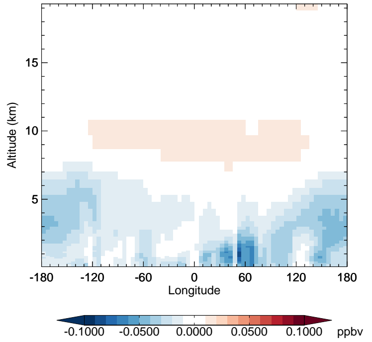
v11-02f-Run0 - v11-02e-Run1 H2O2 - Diff along 42N for Apr
