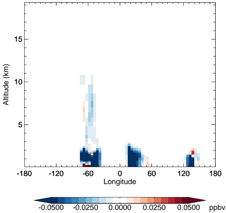
v11-02f-Run0 - v11-02e-Run0 MACR - Diff along 15S for Apr
