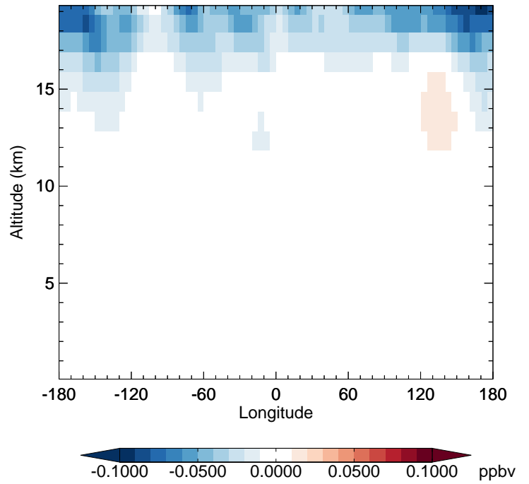
v11-02f-Run0 - v11-02e-Run0 OCS - Diff along 42N for Apr
