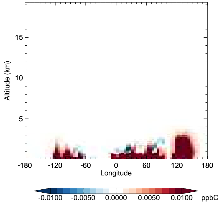
v11-02f-Run0 - v11-02e-Run0 PRPE - Diff along 42N for Apr
