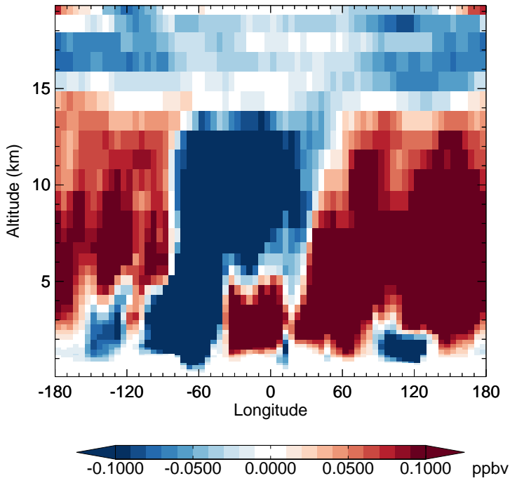
v11-02f-Run0 - v11-02e-Run1 CH4 - Diff along 15S for Apr
