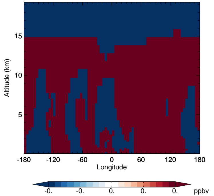
v11-02f-Run0 - v11-02e-Run0 H2O - Diff along 42N for Apr
