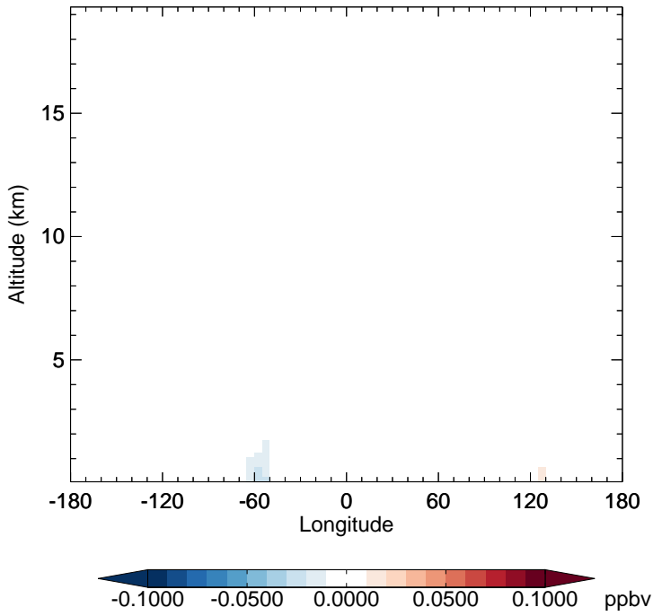
v11-02f-Run0 - v11-02e-Run1 TSOA0 - Diff along 15S for Apr
