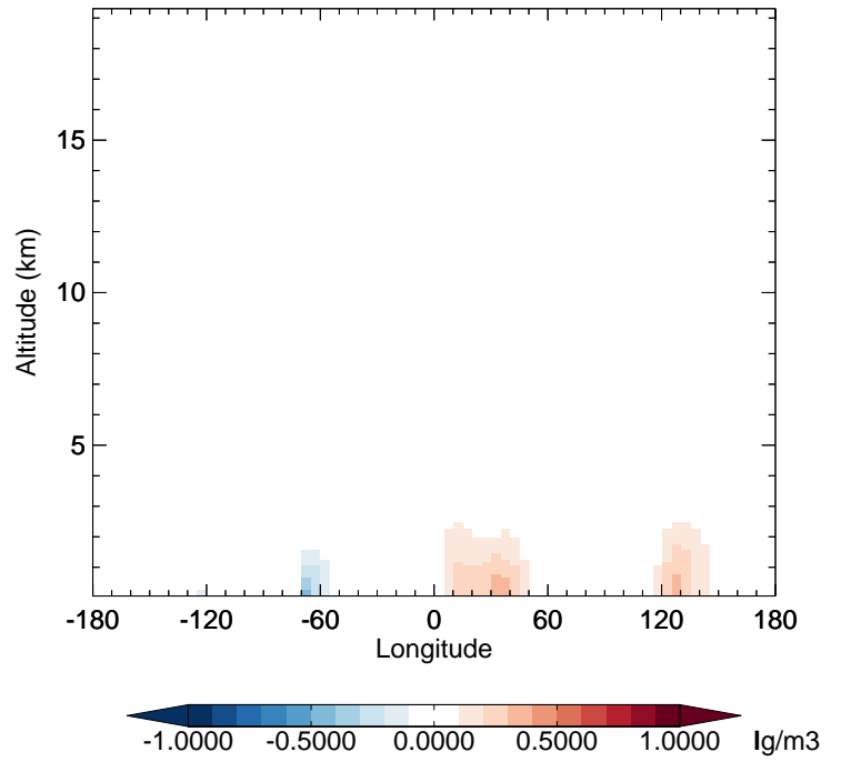
v11-02f-Run0 - v11-02e-Run1 SOAS - Diff along 42N for Apr
