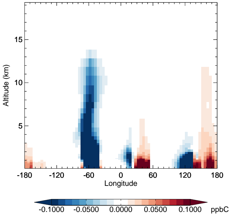
v11-02f-Run0 - v11-02e-Run1 MEK - Diff along 15S for Apr
