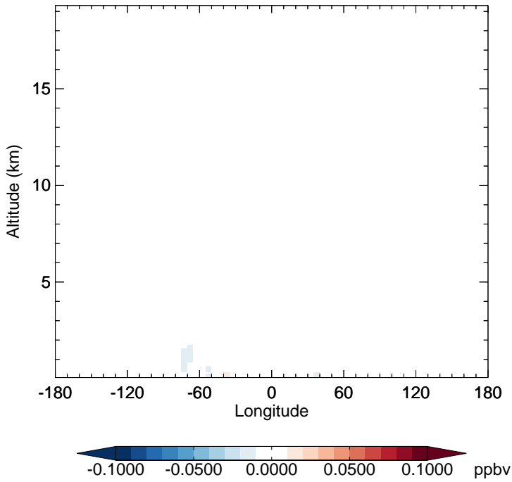
v11-02f-Run0 - v11-02e-Run0 XYLE - Diff along 15S for Apr
