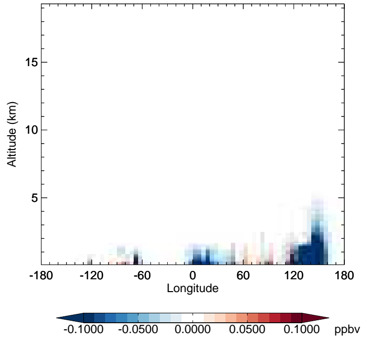
v11-02f-Run0 - v11-02e-Run0 XYLE - Diff along 42N for Apr
