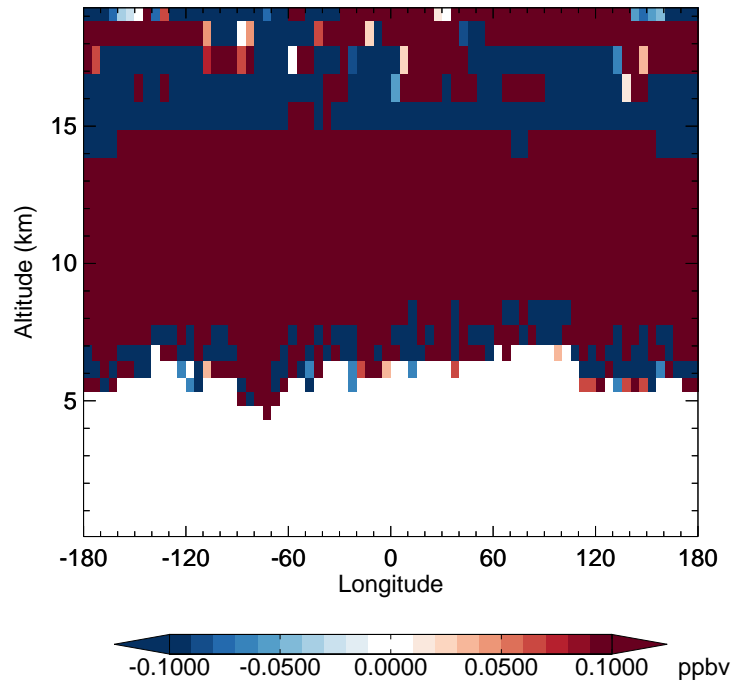
v11-02f-Run0 - v11-02e-Run1 H2O - Diff along 42N for Apr
