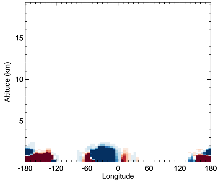
v11-02f-Run0 - v11-02e-Run0 SALC - Diff along 42N for Apr
