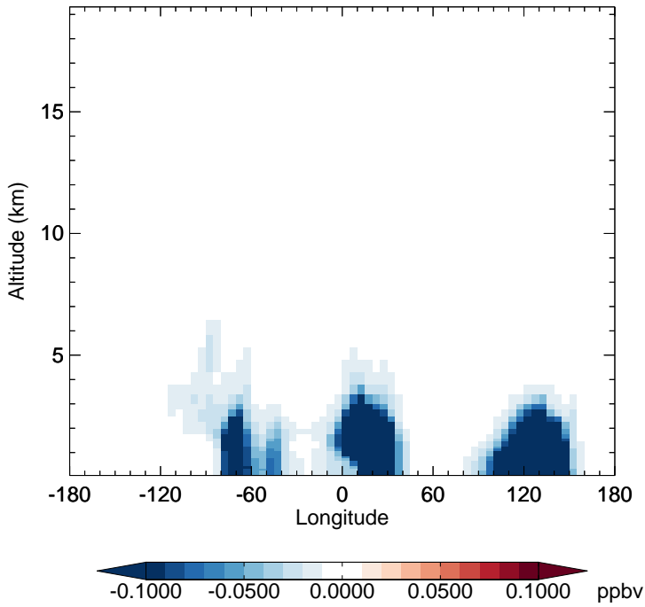
v11-02f-Run0 - v11-02e-Run0 SOAIE - Diff along 15S for Apr
