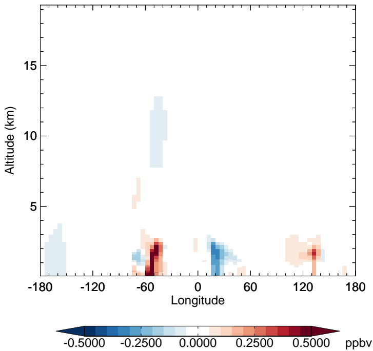
v11-02f-Run0 - v11-02e-Run0 CH 2 O - Diff along 15S for Apr
