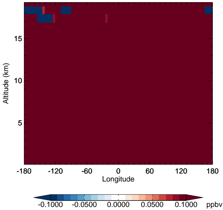
v11-02f-Run0 - v11-02e-Run0 N2O - Diff along 15S for Apr
