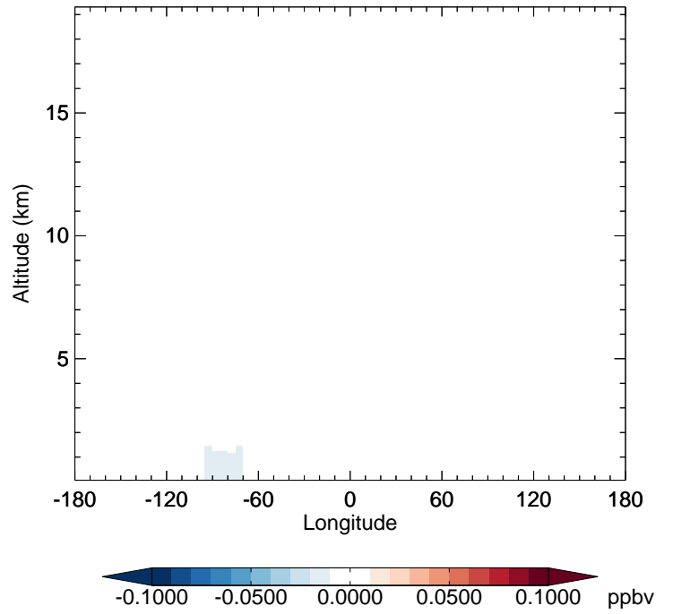
v11-02f-Run0 - v11-02e-Run1 HC187 - Diff along 42N for Jul
