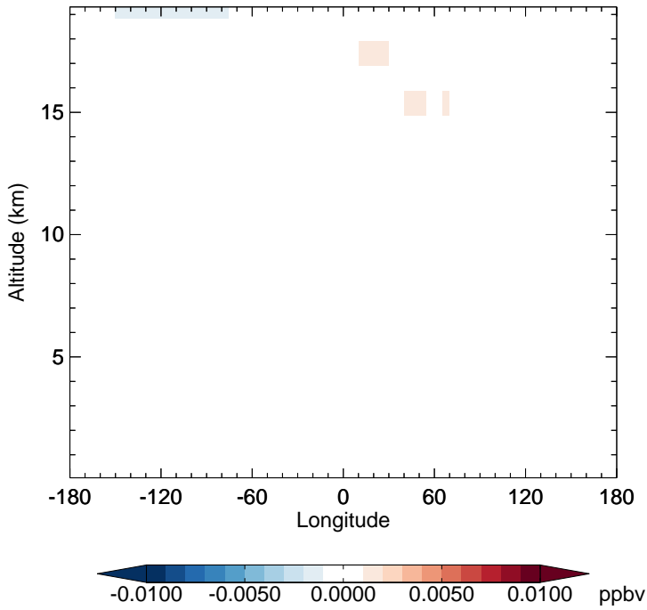
v11-02f-Run0 - v11-02e-Run0 BrNO 3 - Diff along 15S for Jul
