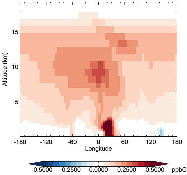
v11-02f-Run0 - v11-02e-Run1 C2H6 - Diff along 15S for Jul
