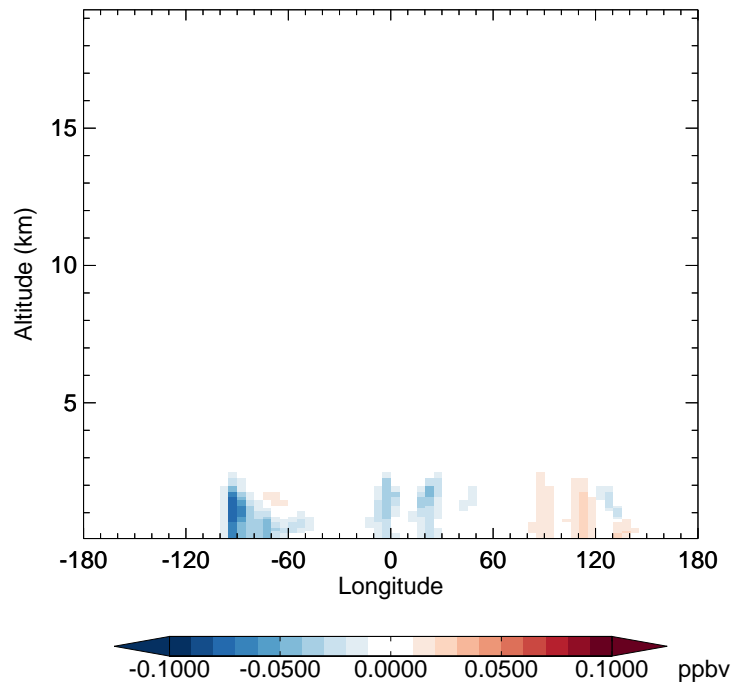
v11-02f-Run0 - v11-02e-Run0 IMAE - Diff along 42N for Jul
