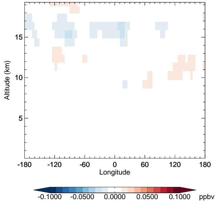
v11-02f-Run0 - v11-02e-Run0 MPN - Diff along 42N for Jul
