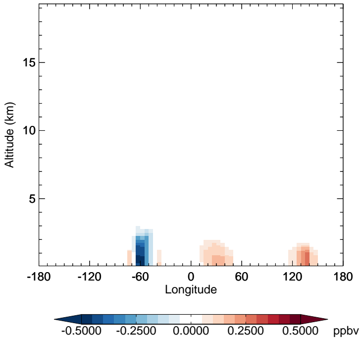
v11-02f-Run0 - v11-02e-Run1 CH 2 O - Diff along 15S for Jul
