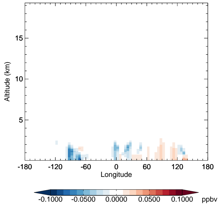
v11-02f-Run0 - v11-02e-Run0 GLYC - Diff along 42N for Jul
