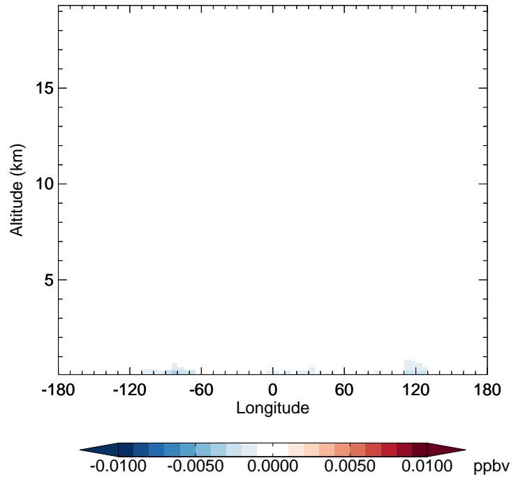
v11-02f-Run0 - v11-02e-Run1 NO3 - Diff along 42N for Jul
