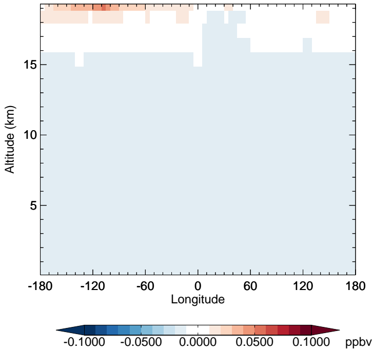
v11-02f-Run0 - v11-02e-Run0 CFC12 - Diff along 15S for Jul
