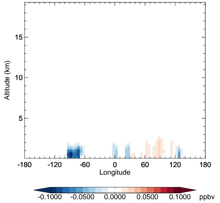
v11-02f-Run0 - v11-02e-Run1 HAC - Diff along 42N for Jul
