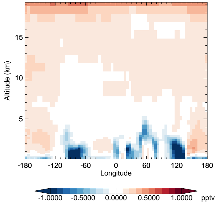
v11-02f-Run0 - v11-02e-Run1 HO2 - Diff along 42N for Jul
