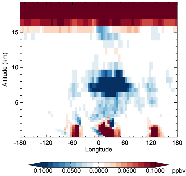
v11-02f-Run0 - v11-02e-Run1 HNO 3 - Diff along 15S for Jul
