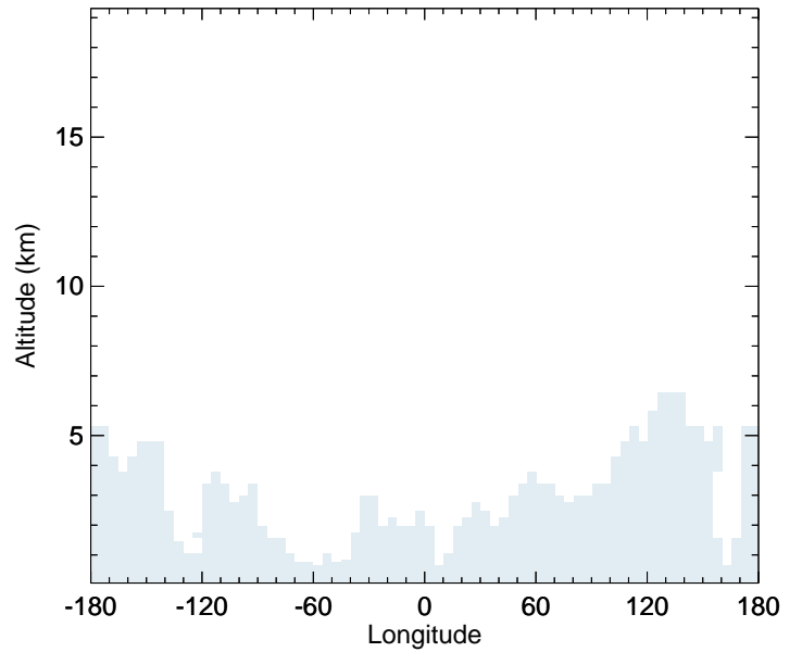
v11-02f-Run0 - v11-02e-Run0 HCFC22 - Diff along 42N for Jul
