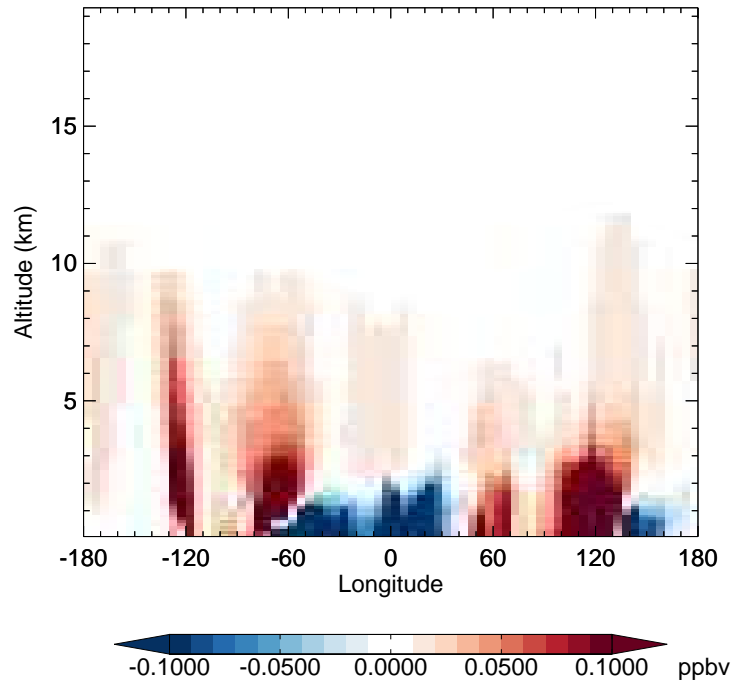
v11-02f-Run0 - v11-02e-Run0 BENZ - Diff along 42N for Jul
