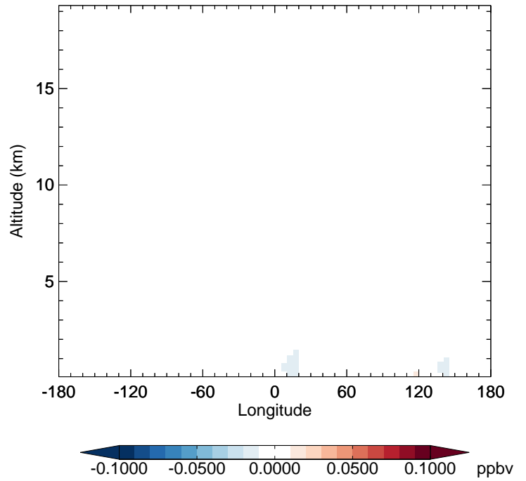
v11-02f-Run0 - v11-02e-Run0 ASOG3 - Diff along 42N for Jul
