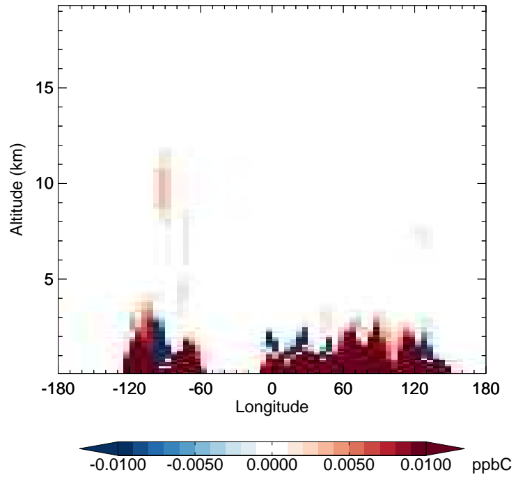
v11-02f-Run0 - v11-02e-Run0 PRPE - Diff along 42N for Jul
