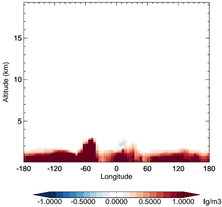
v11-02f-Run0 - v11-02e-Run0 NH3 - Diff along 15S for Jul
