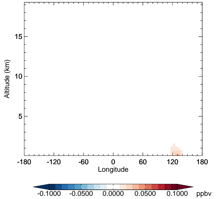
v11-02f-Run0 - v11-02e-Run1 TSOA2 - Diff along 42N for Jul
