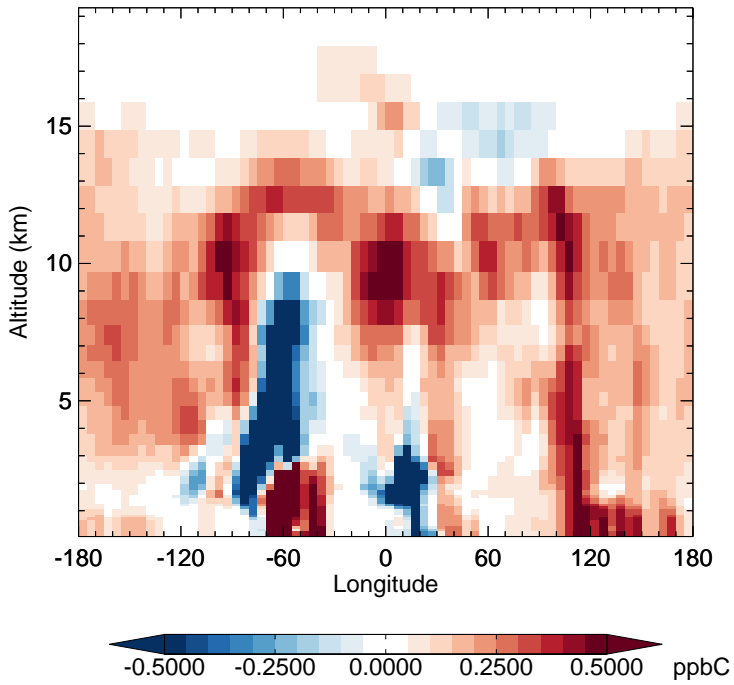
v11-02f-Run0 - v11-02e-Run0 ACET - Diff along 15S for Jul
