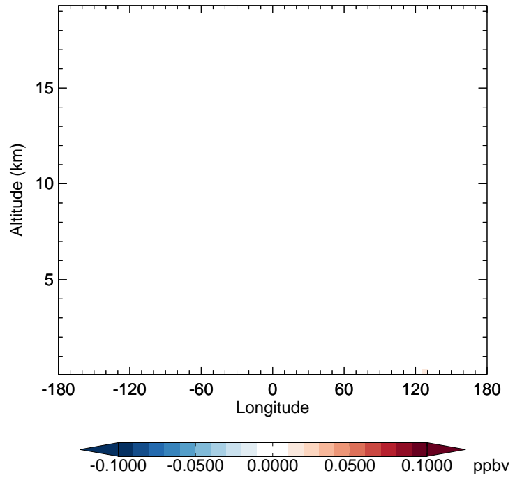
v11-02f-Run0 - v11-02e-Run1 TSOA3 - Diff along 42N for Jul
