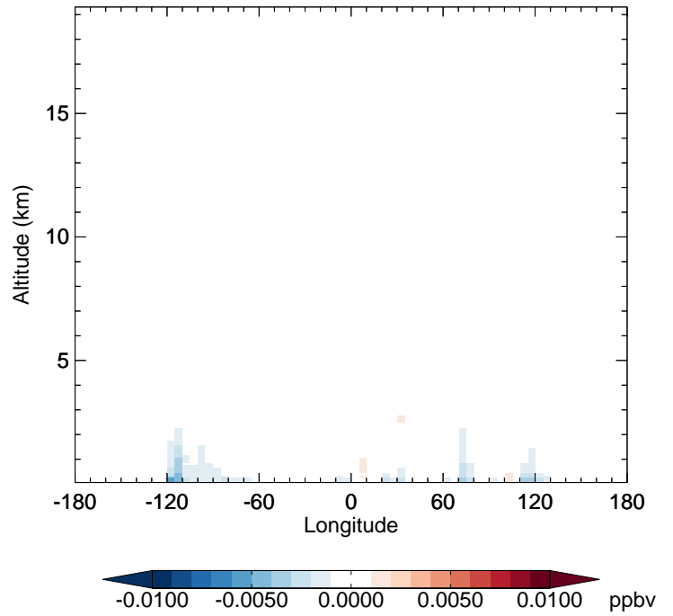
v11-02f-Run0 - v11-02e-Run0 NO3 - Diff along 42N for Jul
