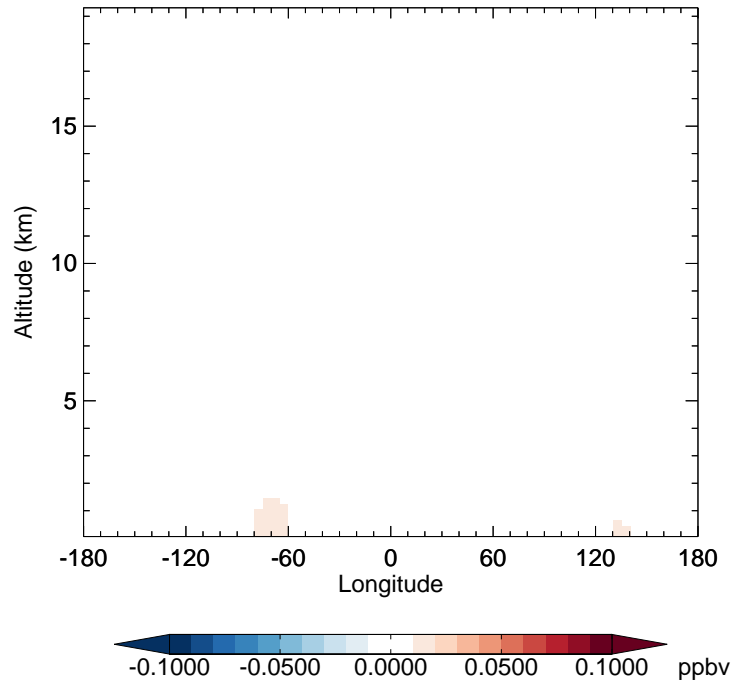
v11-02f-Run0 - v11-02e-Run0 TSOA0 - Diff along 42N for Jul
