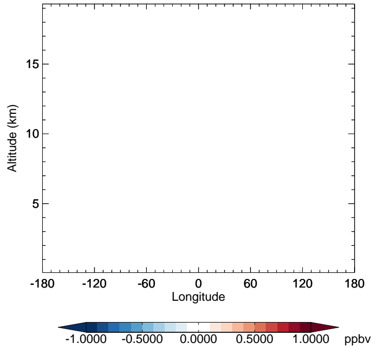
v11-02f-Run0 - v11-02e-Run0 HNO 2 - Diff along 42N for Jul
