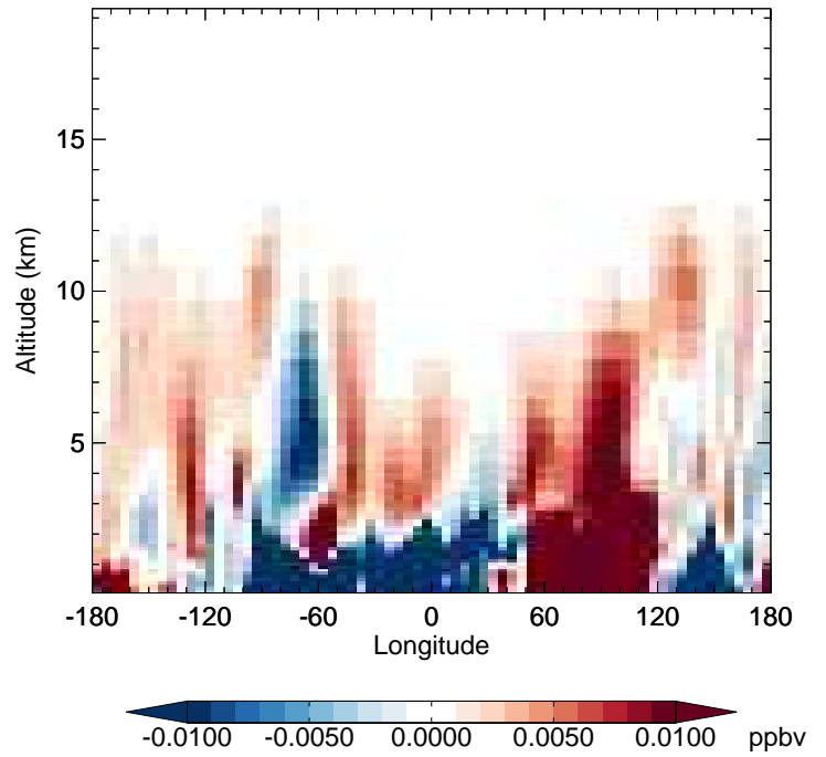
v11-02f-Run0 - v11-02e-Run0 MAP - Diff along 42N for Jul
