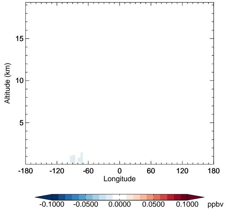
v11-02f-Run0 - v11-02e-Run1 IEPOXB - Diff along 42N for Jul
