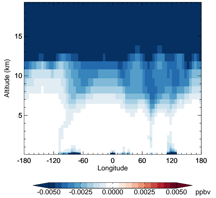
v11-02f-Run0 - v11-02e-Run1 N2O5 - Diff along 42N for Jul
