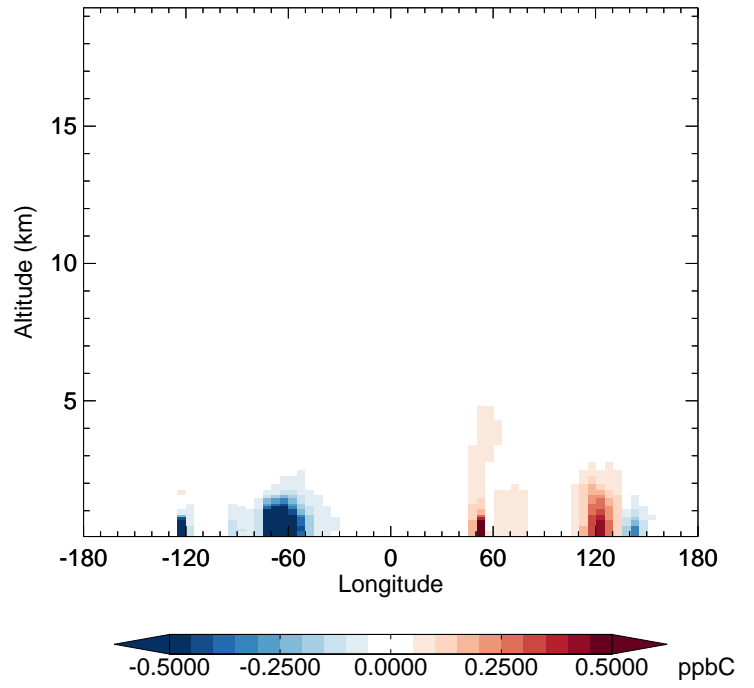
v11-02f-Run0 - v11-02e-Run1 ALK4 - Diff along 42N for Jul
