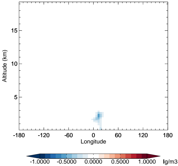
v11-02f-Run0 - v11-02e-Run0 BCPI - Diff along 15S for Jul
