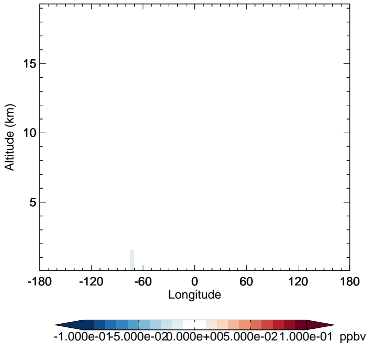
v11-02f-Run0 - v11-02e-Run1 SOAME - Diff along 15S for Jul
