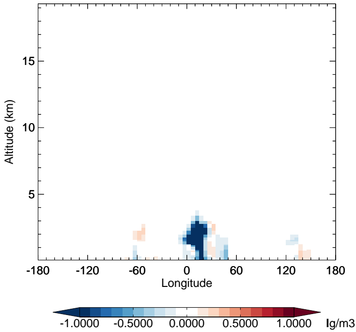
v11-02f-Run0 - v11-02e-Run0 OCPI - Diff along 15S for Jul
