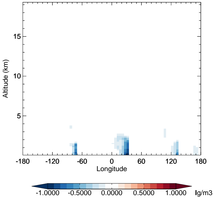
v11-02f-Run0 - v11-02e-Run0 SO 2 - Diff along 15S for Jul
