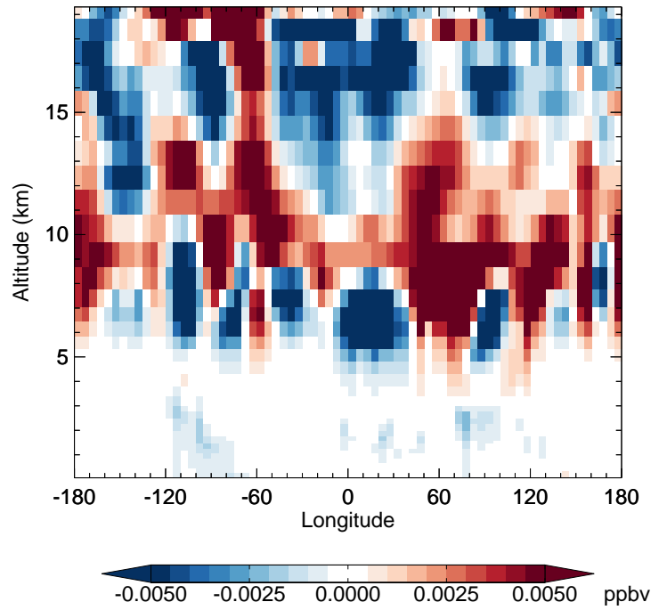
v11-02f-Run0 - v11-02e-Run0 HNO 4 - Diff along 42N for Jul
