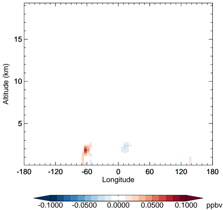
v11-02f-Run0 - v11-02e-Run0 ISOA1 - Diff along 15S for Jul
