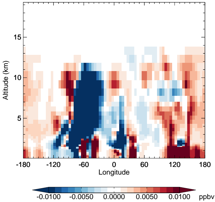
v11-02f-Run0 - v11-02e-Run0 MAP - Diff along 15S for Jul
