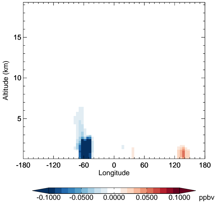
v11-02f-Run0 - v11-02e-Run1 GLYC - Diff along 15S for Jul
