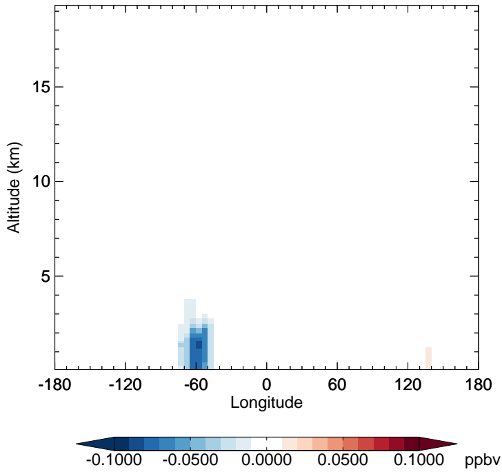
v11-02f-Run0 - v11-02e-Run1 IPMN - Diff along 15S for Jul
