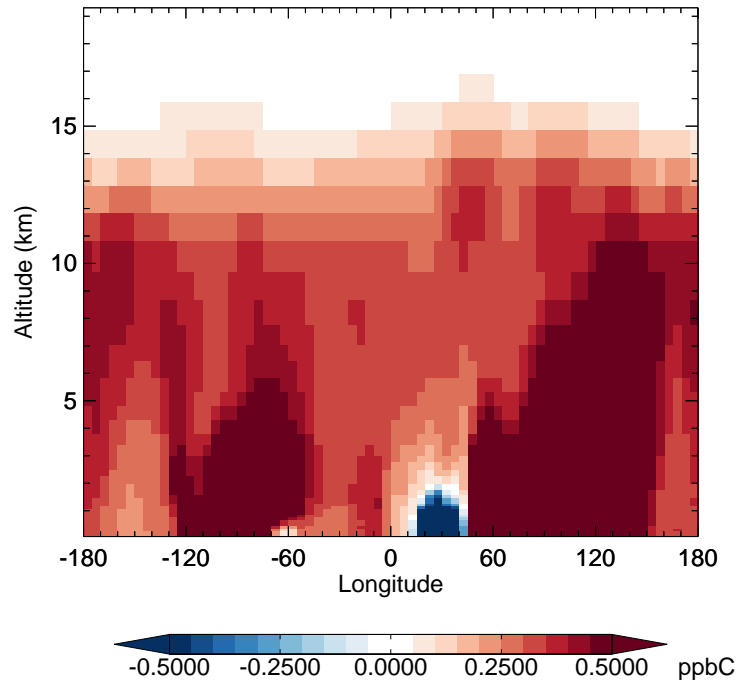
v11-02f-Run0 - v11-02e-Run1 C2H6 - Diff along 42N for Jul
