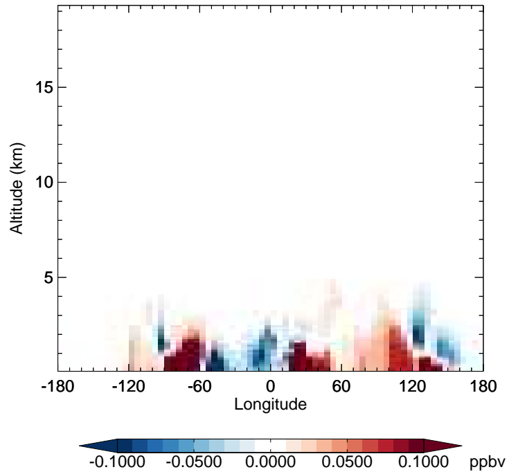
v11-02f-Run0 - v11-02e-Run0 INDIOL - Diff along 42N for Jul
