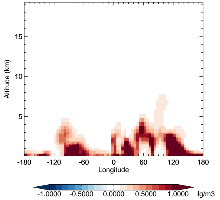
v11-02f-Run0 - v11-02e-Run1 NIT - Diff along 42N for Jul
