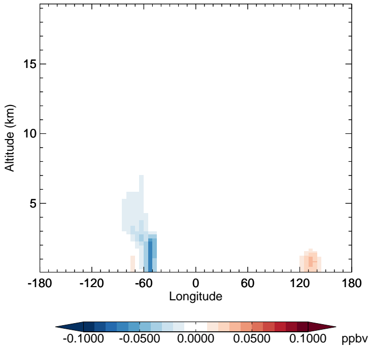
v11-02f-Run0 - v11-02e-Run1 IMAE - Diff along 15S for Jul
