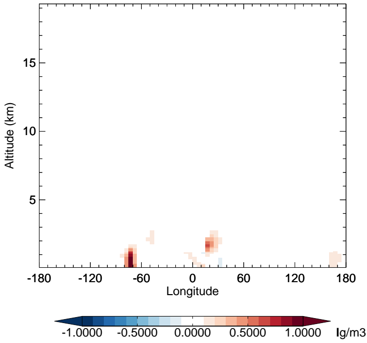
v11-02f-Run0 - v11-02e-Run1 NH4 - Diff along 15S for Jul
