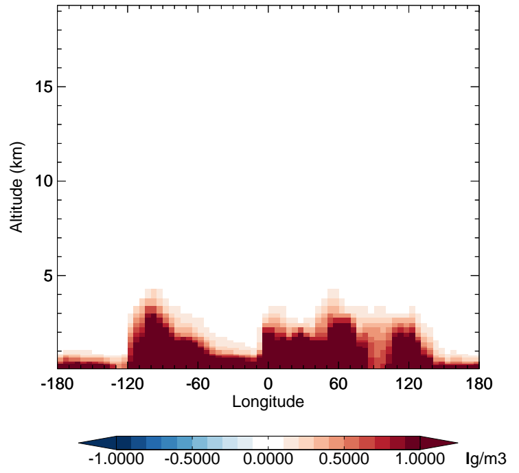
v11-02f-Run0 - v11-02e-Run1 NH3 - Diff along 42N for Jul
