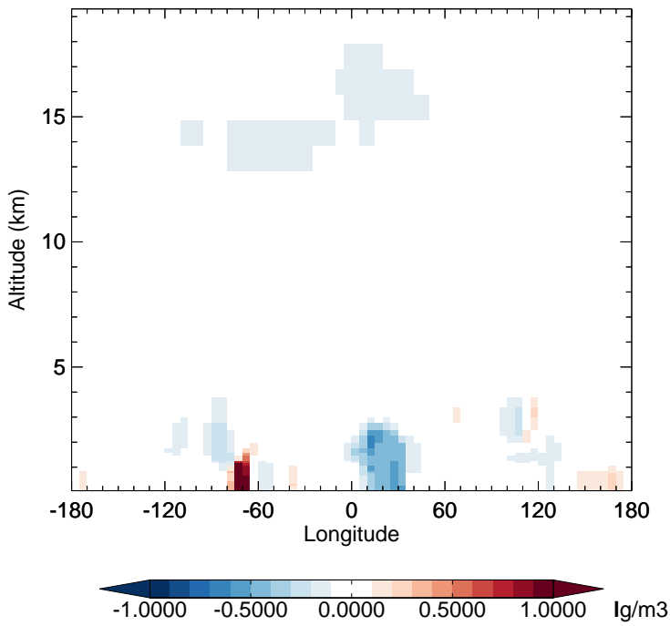
v11-02f-Run0 - v11-02e-Run0 SO4 - Diff along 15S for Jul
