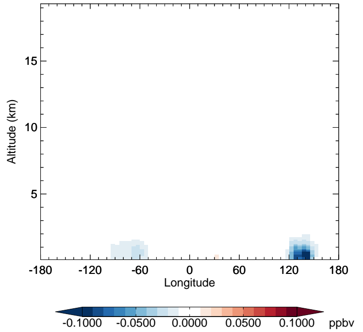
v11-02f-Run0 - v11-02e-Run1 SOAGX - Diff along 42N for Jul
