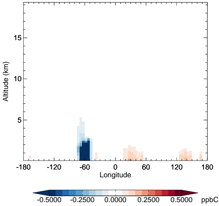
v11-02f-Run0 - v11-02e-Run1 ALD2 - Diff along 15S for Jul
