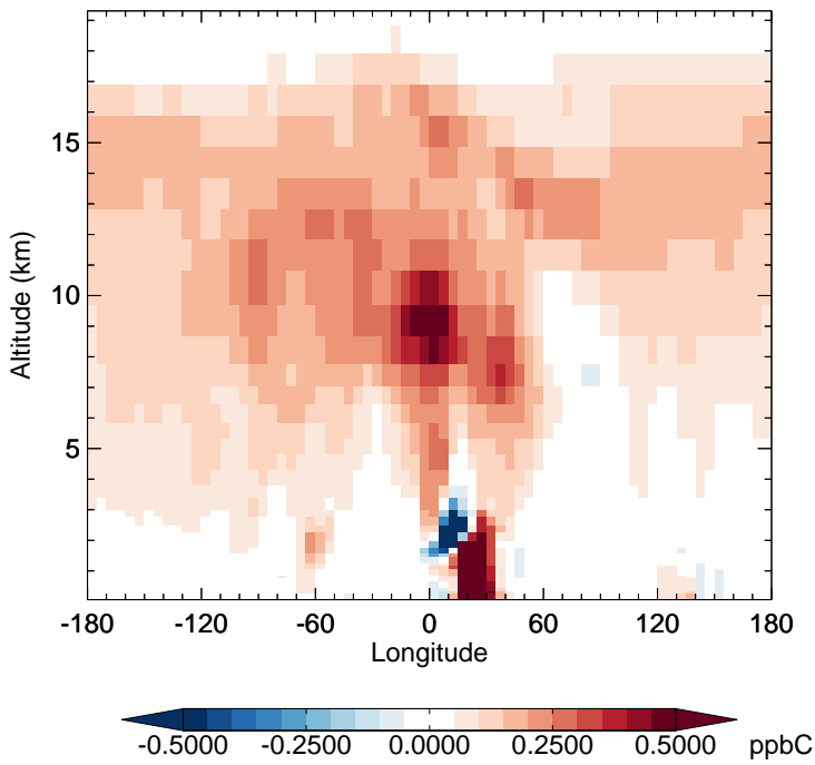
v11-02f-Run0 - v11-02e-Run0 C2H6 - Diff along 15S for Jul
