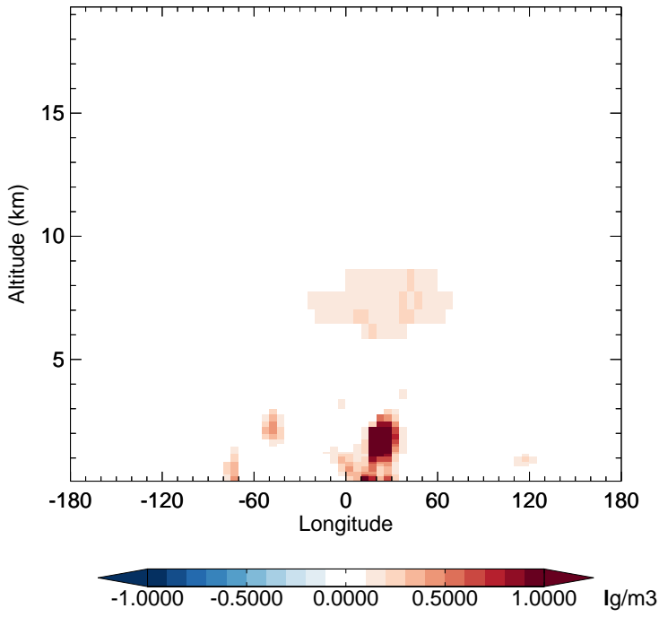
v11-02f-Run0 - v11-02e-Run1 NIT - Diff along 15S for Jul
