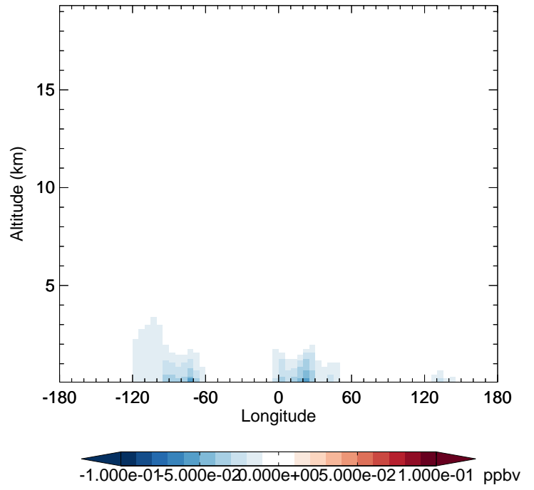
v11-02f-Run0 - v11-02e-Run1 MONITA - Diff along 42N for Jul
