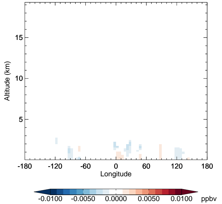
v11-02f-Run0 - v11-02e-Run0 MVKN - Diff along 42N for Jul
