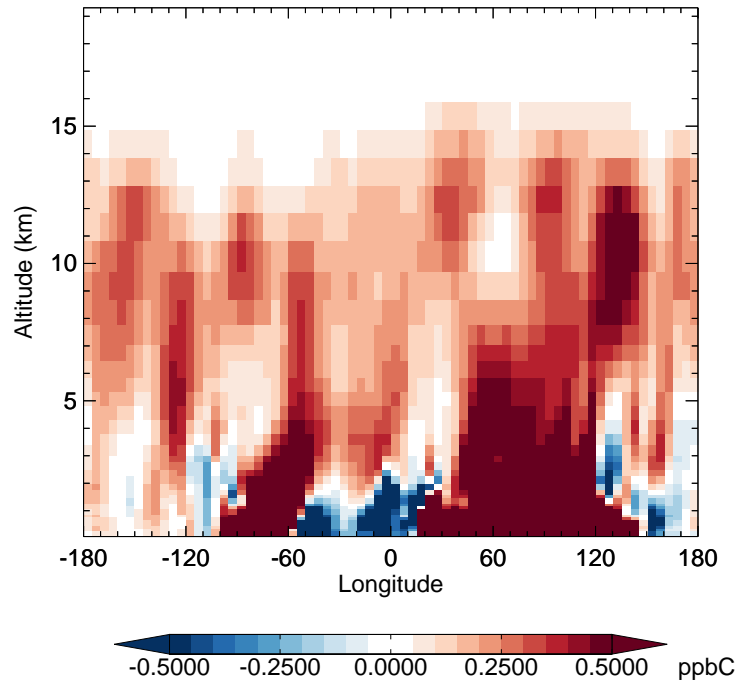
v11-02f-Run0 - v11-02e-Run0 ACET - Diff along 42N for Jul
