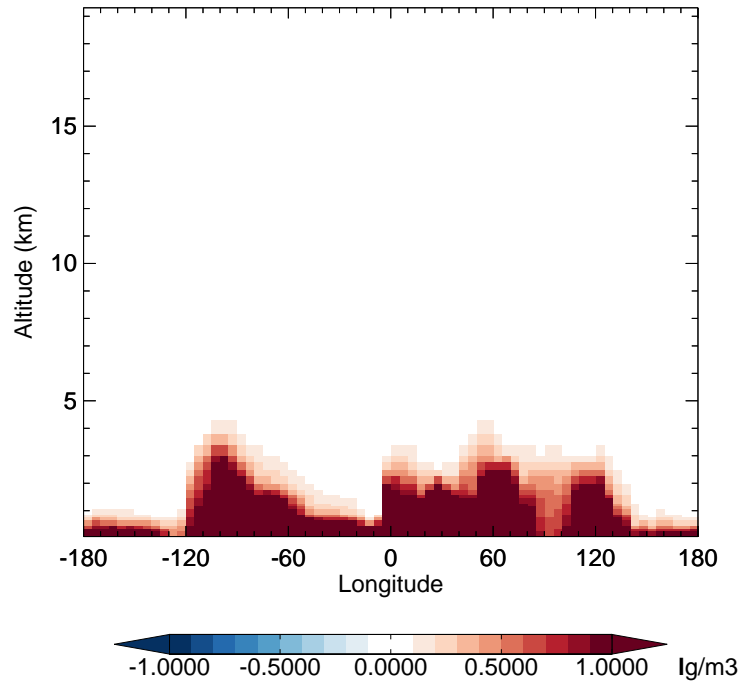
v11-02f-Run0 - v11-02e-Run0 NH3 - Diff along 42N for Jul
