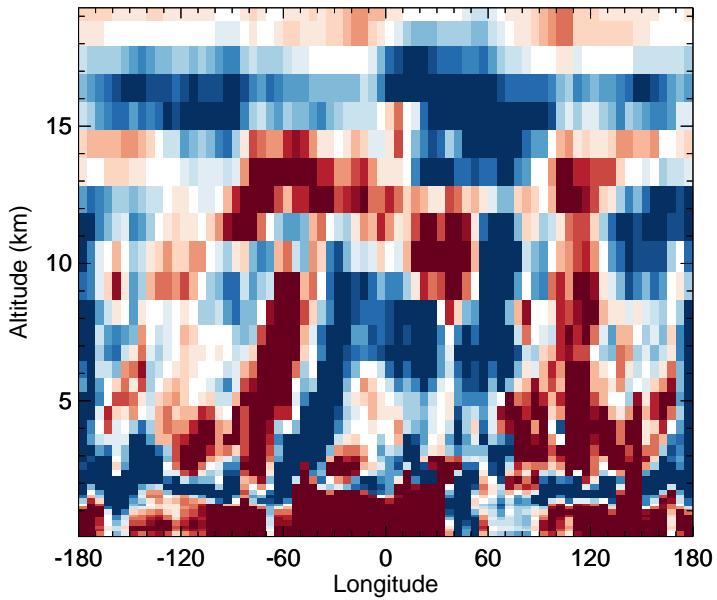
v11-02f-Run0 - v11-02e-Run0 OH - Diff along 15S for Jul
