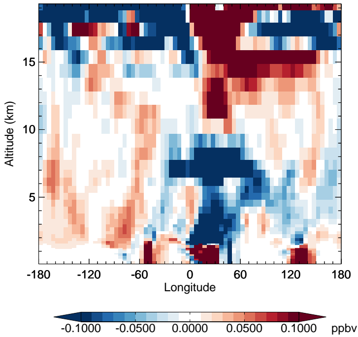
v11-02f-Run0 - v11-02e-Run0 HNO 3 - Diff along 15S for Jul
