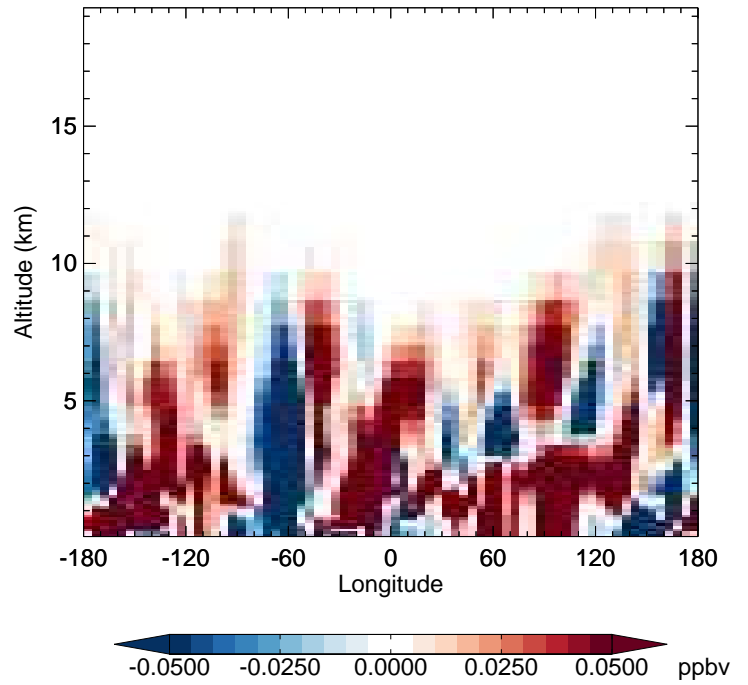
v11-02f-Run0 - v11-02e-Run0 MP - Diff along 42N for Jul
