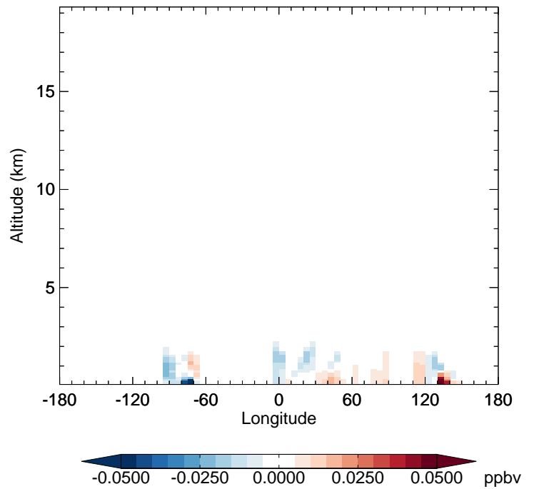
v11-02f-Run0 - v11-02e-Run0 MACR - Diff along 42N for Jul
