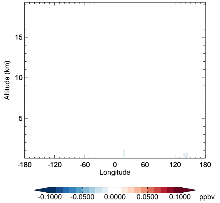
v11-02f-Run0 - v11-02e-Run1 ASOG3 - Diff along 42N for Jul
