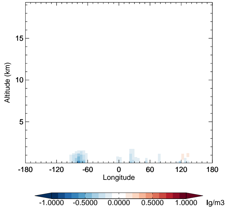
v11-02f-Run0 - v11-02e-Run1 SO 2 - Diff along 42N for Jul
