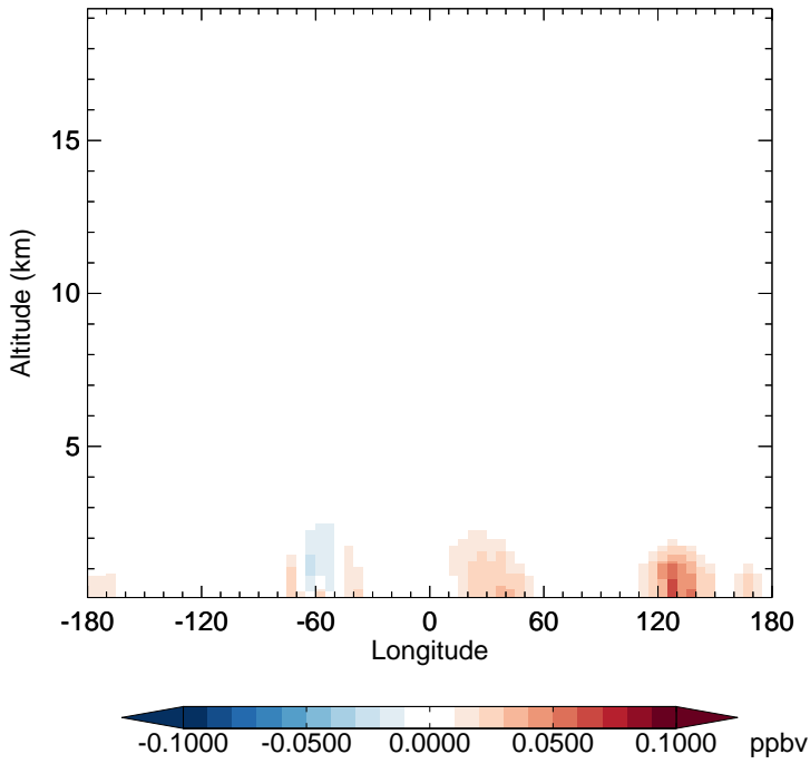
v11-02f-Run0 - v11-02e-Run1 TSOG3 - Diff along 15S for Jul
