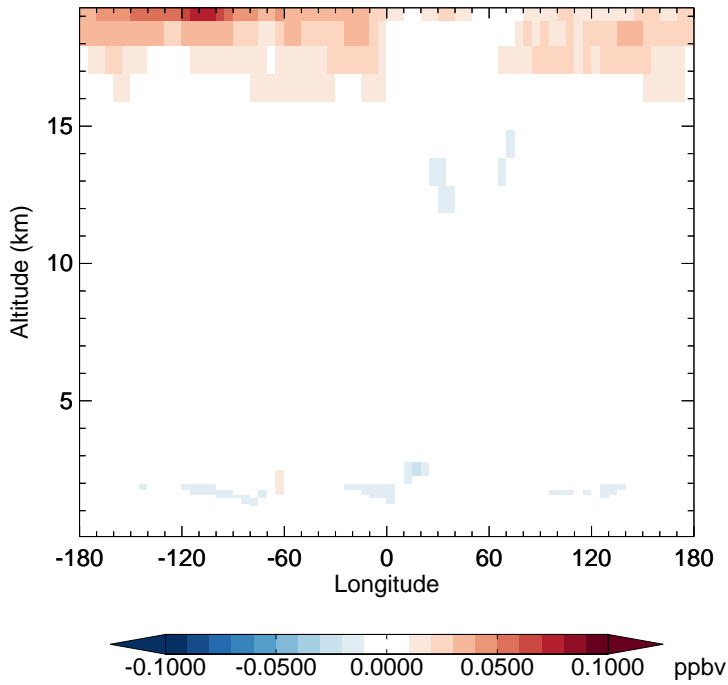
v11-02f-Run0 - v11-02e-Run0 CH3Cl - Diff along 15S for Jul
