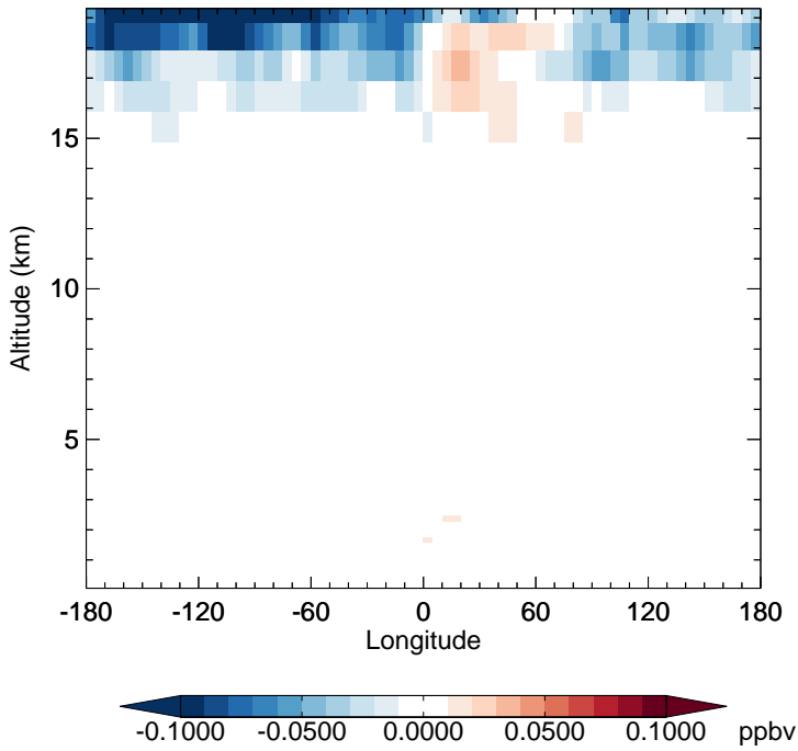
v11-02f-Run0 - v11-02e-Run0 HCl - Diff along 15S for Jul
