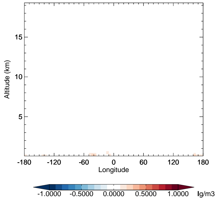
v11-02f-Run0 - v11-02e-Run0 DMS - Diff along 42N for Jul
