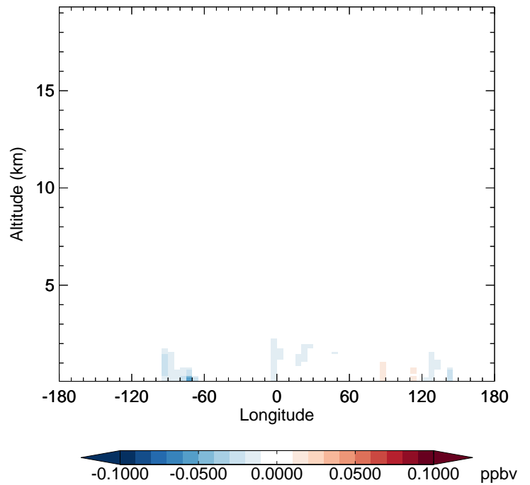
v11-02f-Run0 - v11-02e-Run0 MGLY - Diff along 42N for Jul
