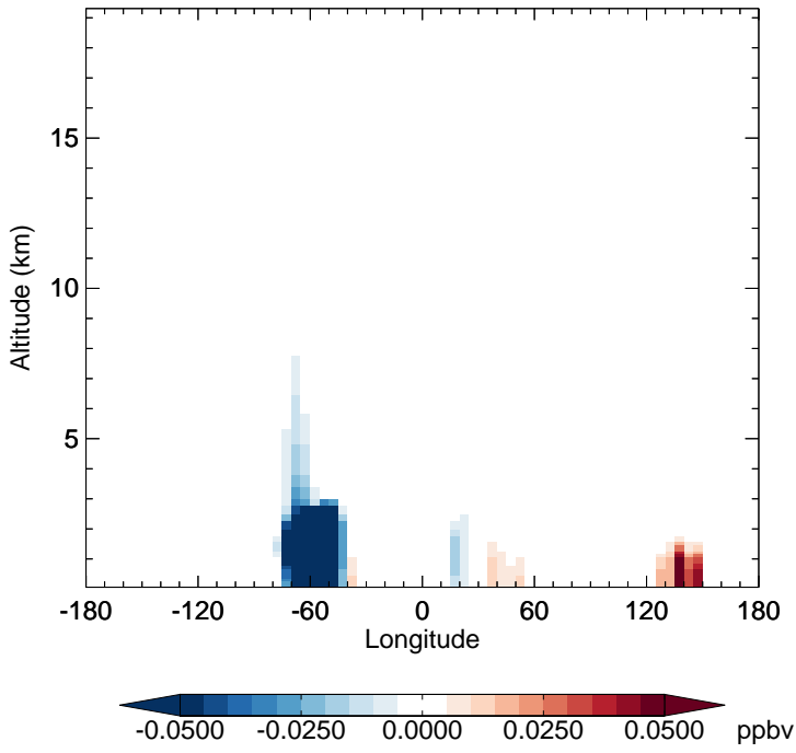
v11-02f-Run0 - v11-02e-Run1 MVK - Diff along 15S for Jul
