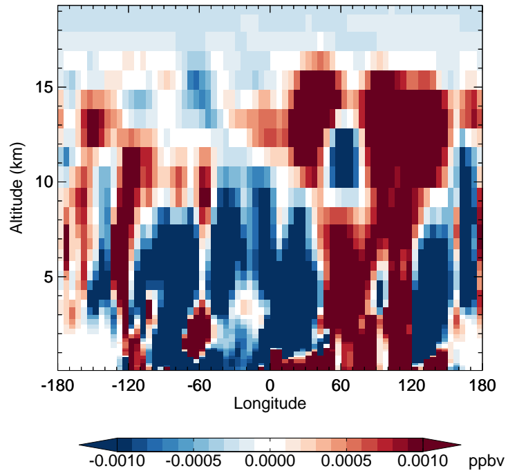
v11-02f-Run0 - v11-02e-Run0 PPN - Diff along 42N for Jul
