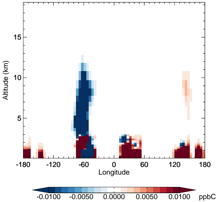
v11-02f-Run0 - v11-02e-Run0 PRPE - Diff along 15S for Jul
