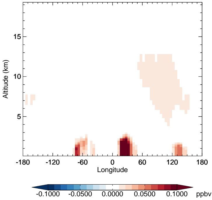
v11-02f-Run0 - v11-02e-Run1 PAN - Diff along 15S for Jul
