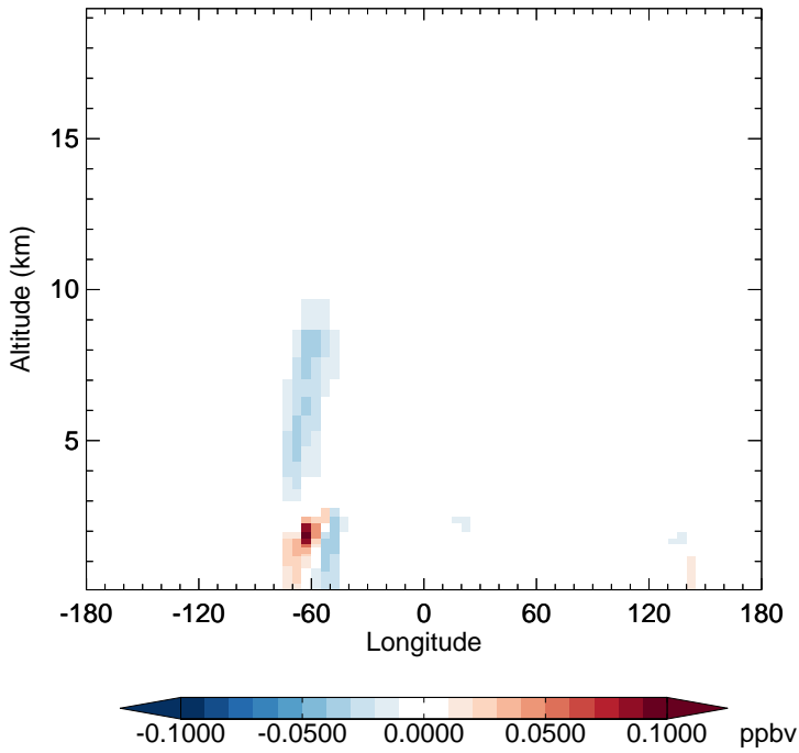
v11-02f-Run0 - v11-02e-Run0 IEPOXB - Diff along 15S for Jul
