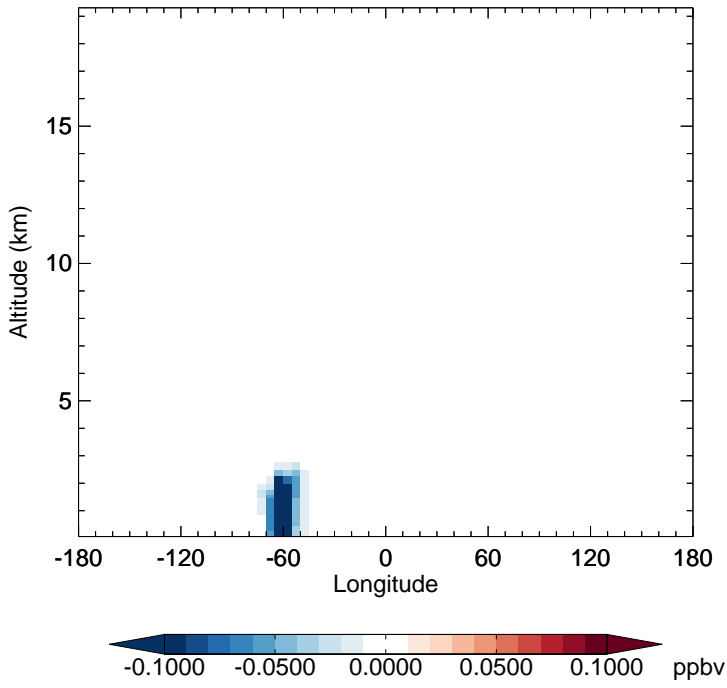
v11-02f-Run0 - v11-02e-Run1 RIPB - Diff along 15S for Jul
