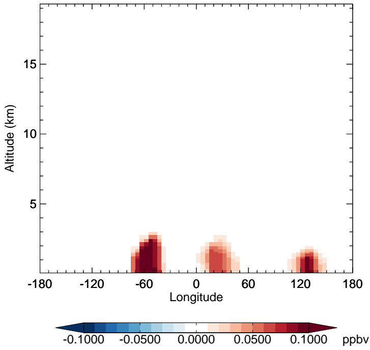
v11-02f-Run0 - v11-02e-Run1 INDIOL - Diff along 15S for Jul
