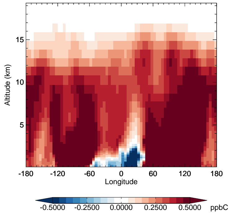
v11-02f-Run0 - v11-02e-Run0 C2H6 - Diff along 42N for Jul
