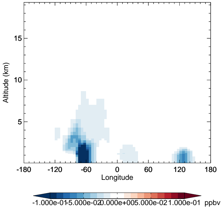
v11-02f-Run0 - v11-02e-Run1 SOAIE - Diff along 15S for Jul
