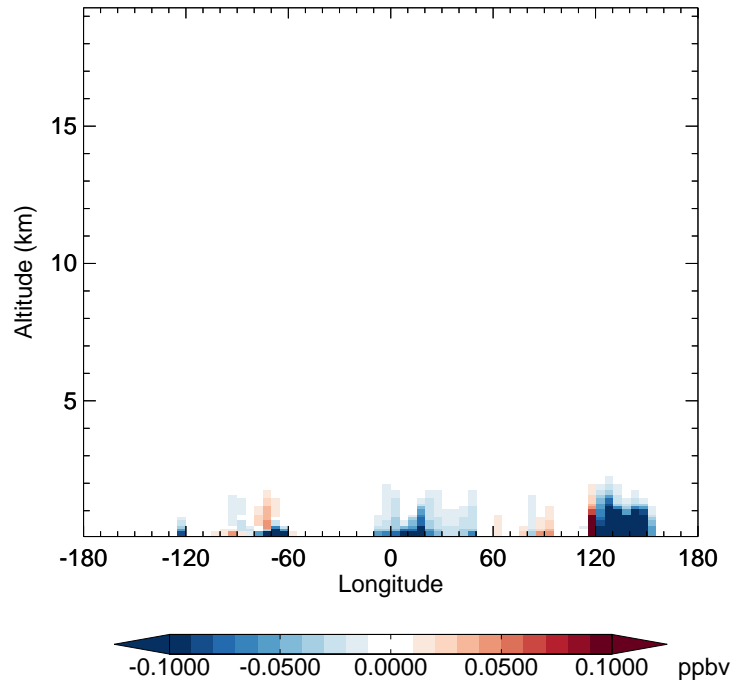
v11-02f-Run0 - v11-02e-Run0 XYLE - Diff along 42N for Jul
