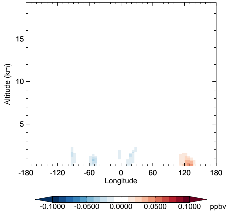
v11-02f-Run0 - v11-02e-Run0 TSOA2 - Diff along 42N for Jul
