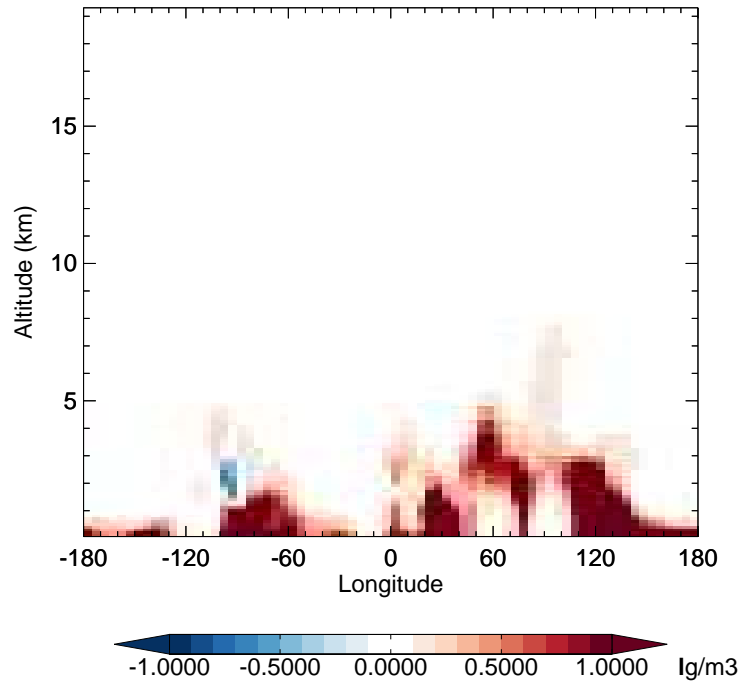
v11-02f-Run0 - v11-02e-Run0 NIT - Diff along 42N for Jul
