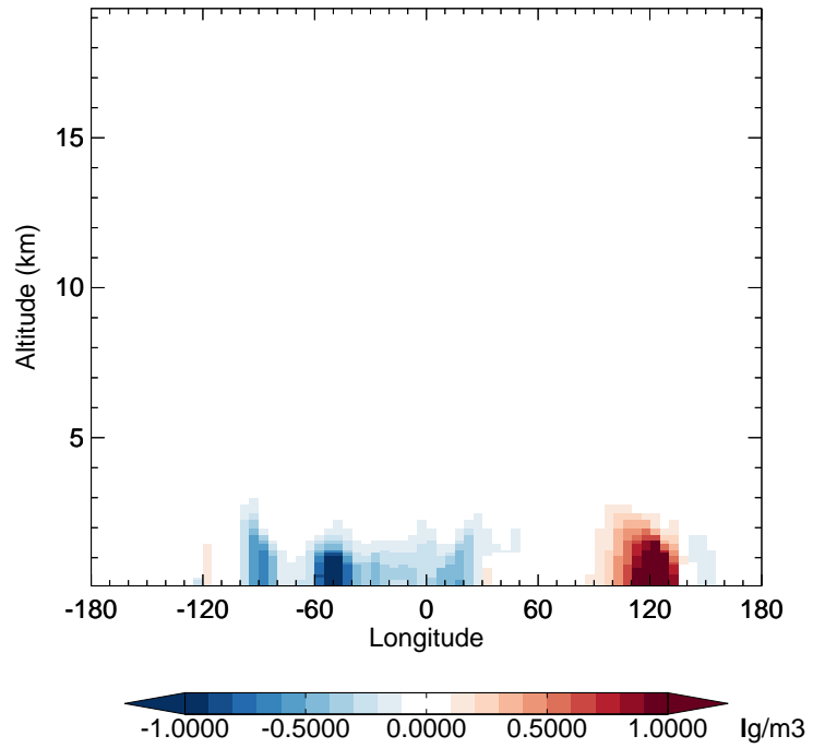
v11-02f-Run0 - v11-02e-Run0 OCPI - Diff along 42N for Jul
