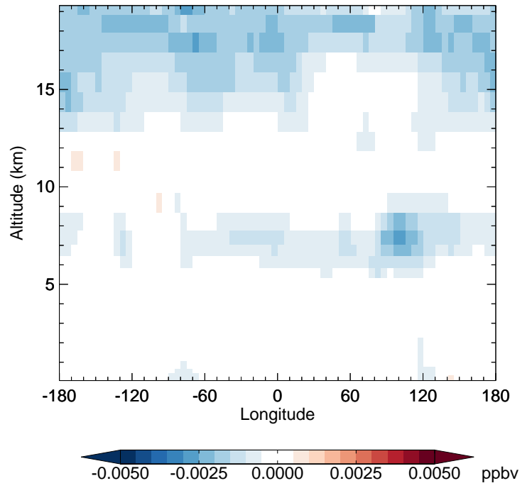
v11-02f-Run0 - v11-02e-Run1 HNO 4 - Diff along 42N for Jul
