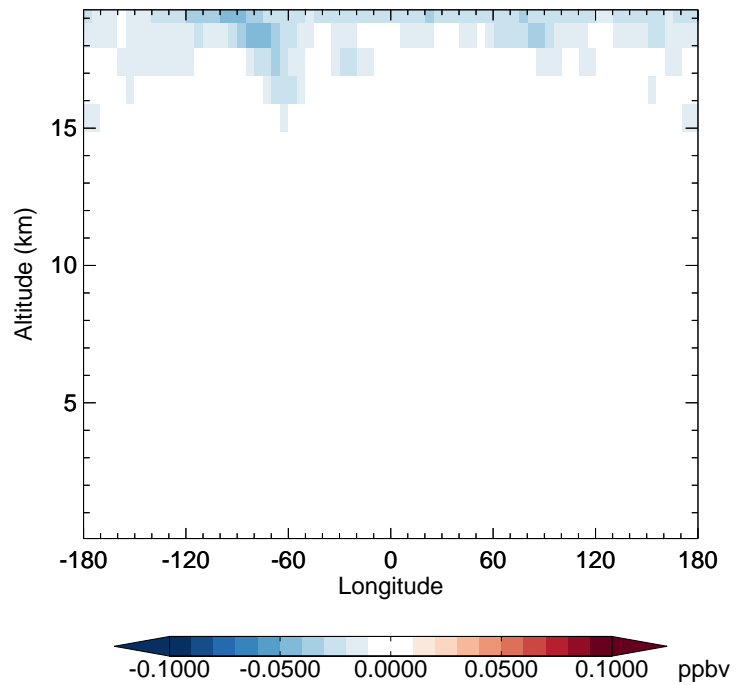
v11-02f-Run0 - v11-02e-Run0 OCS - Diff along 42N for Jul
