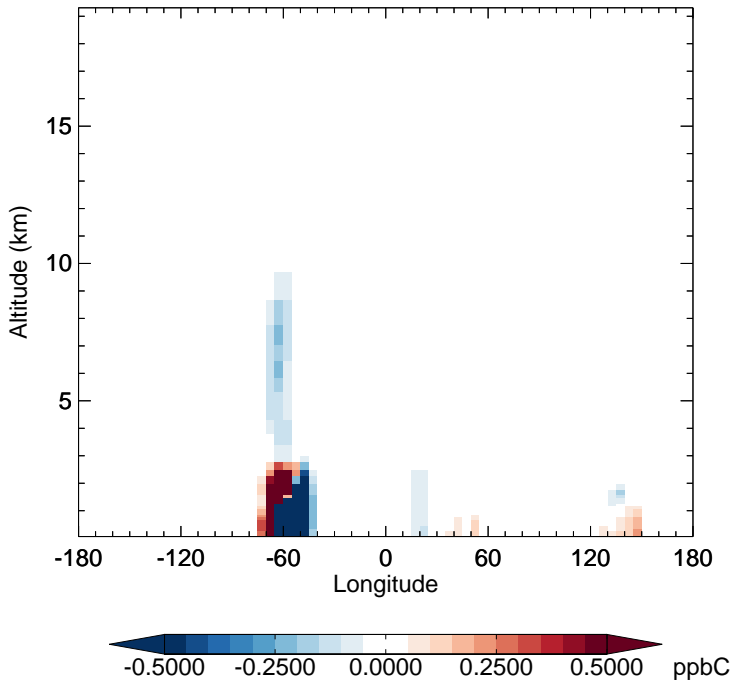
v11-02f-Run0 - v11-02e-Run0 ISOP - Diff along 15S for Jul
