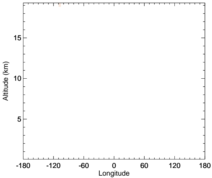
v11-02f-Run0 - v11-02e-Run0 CH3Br - Diff along 15S for Jul
