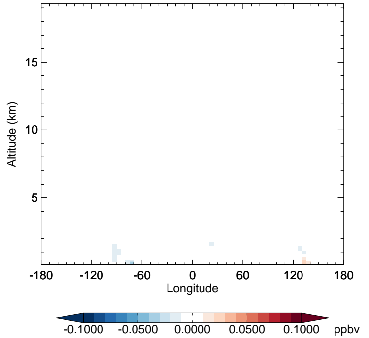
v11-02f-Run0 - v11-02e-Run0 IPMN - Diff along 42N for Jul
