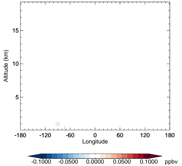
v11-02f-Run0 - v11-02e-Run0 IEPOXB - Diff along 42N for Jul
