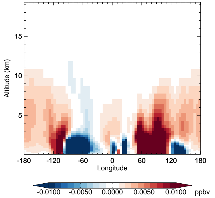
v11-02f-Run0 - v11-02e-Run1 MAP - Diff along 42N for Jul
