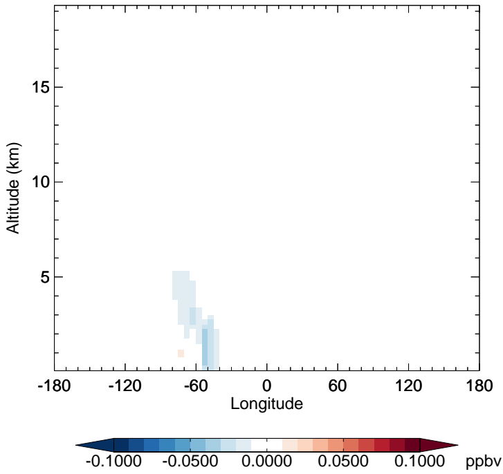
v11-02f-Run0 - v11-02e-Run1 HC187 - Diff along 15S for Jul
