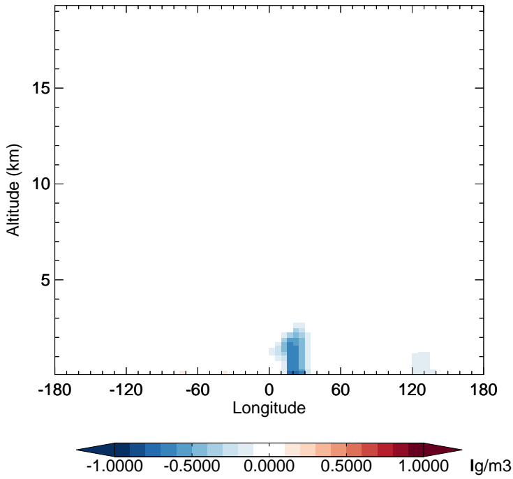
v11-02f-Run0 - v11-02e-Run1 OCPI - Diff along 15S for Jul
