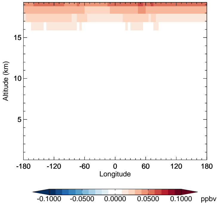
v11-02f-Run0 - v11-02e-Run1 N2O - Diff along 15S for Jul
