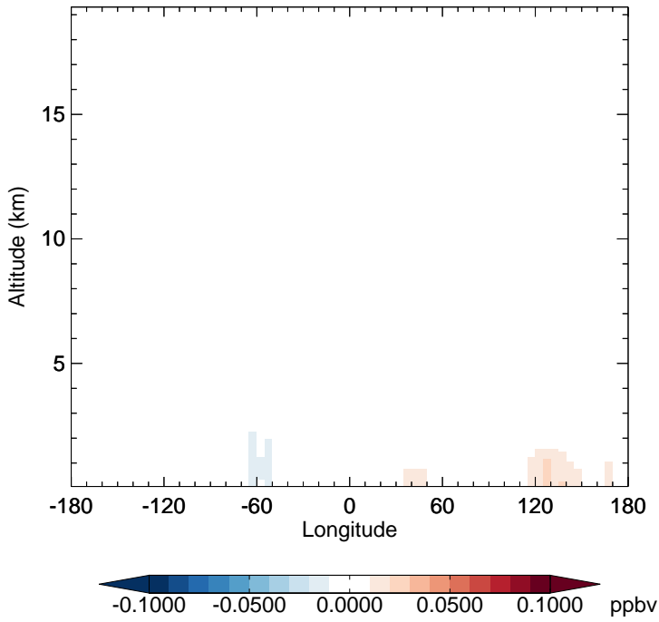
v11-02f-Run0 - v11-02e-Run1 TSOG2 - Diff along 15S for Jul
