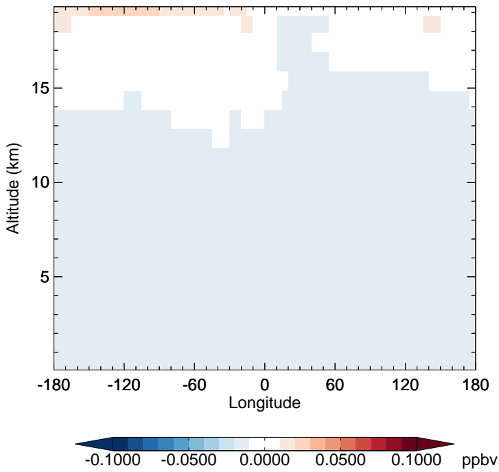
v11-02f-Run0 - v11-02e-Run0 CFC11 - Diff along 15S for Jul
