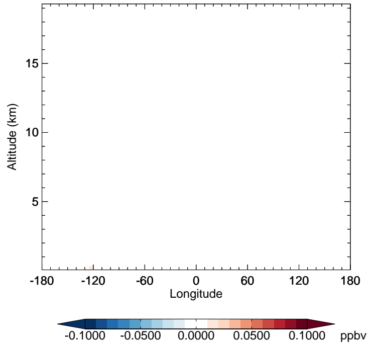
v11-02f-Run0 - v11-02e-Run1 MTPA - Diff along 42N for Jul
