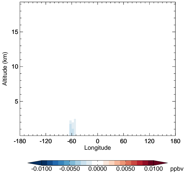
v11-02f-Run0 - v11-02e-Run1 MOBA - Diff along 15S for Jul
