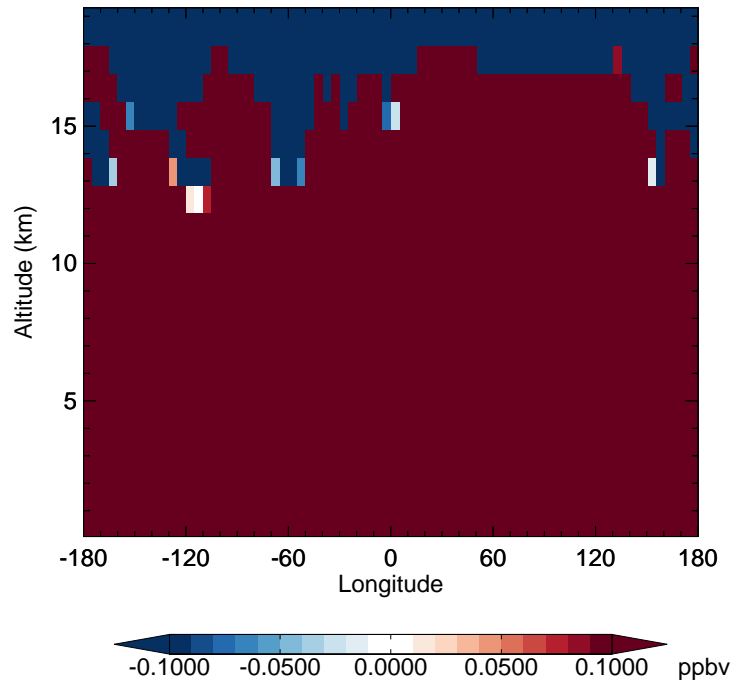
v11-02f-Run0 - v11-02e-Run0 N2O - Diff along 42N for Jul
