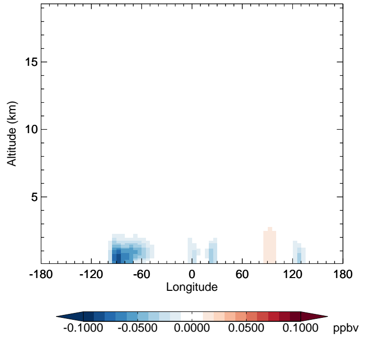
v11-02f-Run0 - v11-02e-Run1 ISO3 - Diff along 42N for Jul
