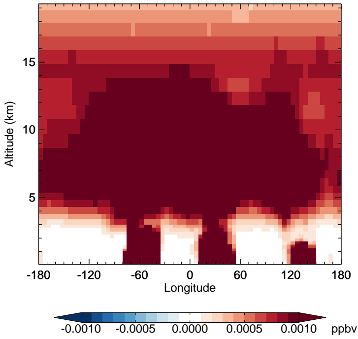
v11-02f-Run0 - v11-02e-Run1 PPN - Diff along 15S for Jul
