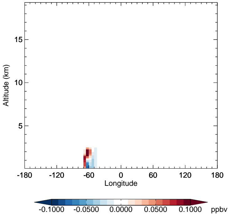
v11-02f-Run0 - v11-02e-Run0 HPALD - Diff along 15S for Jul
