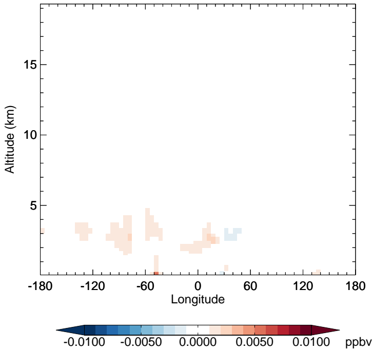
v11-02f-Run0 - v11-02e-Run0 NO3 - Diff along 15S for Jul
