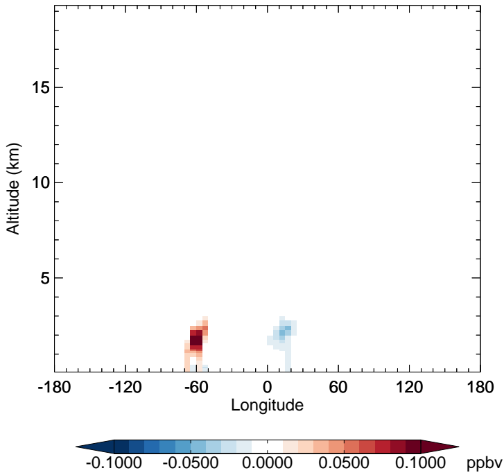
v11-02f-Run0 - v11-02e-Run0 TSOA2 - Diff along 15S for Jul
