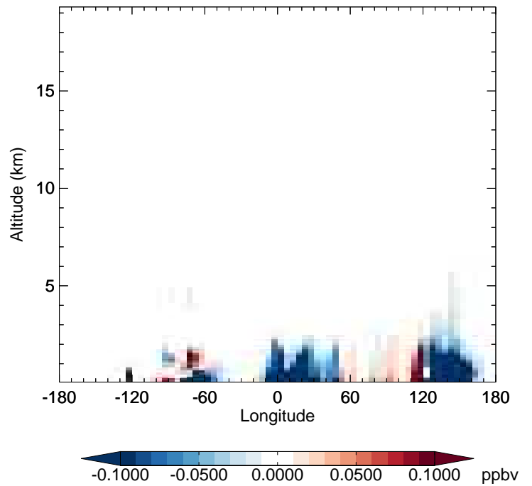
v11-02f-Run0 - v11-02e-Run0 TOLU - Diff along 42N for Jul
