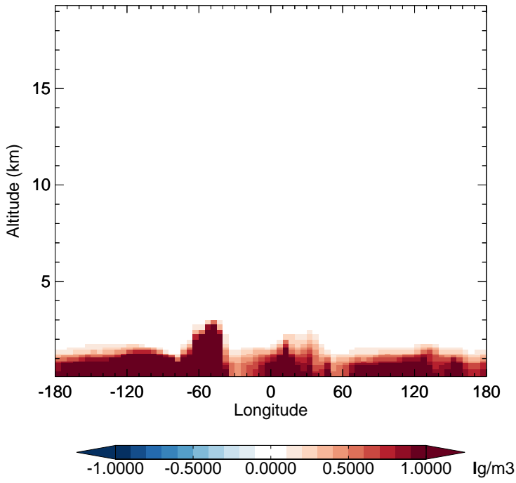
v11-02f-Run0 - v11-02e-Run1 NH3 - Diff along 15S for Jul
