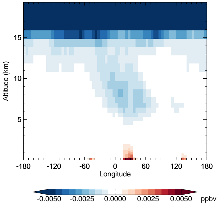
v11-02f-Run0 - v11-02e-Run1 N2O5 - Diff along 15S for Jul
