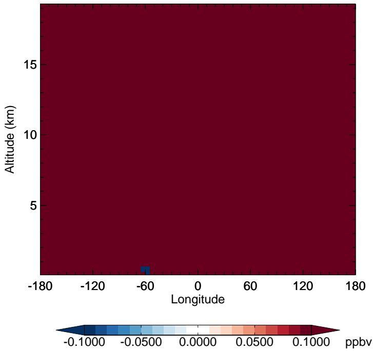
v11-02f-Run0 - v11-02e-Run0 CH4 - Diff along 15S for Jul
