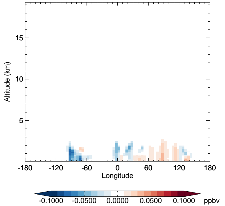
v11-02f-Run0 - v11-02e-Run0 HAC - Diff along 42N for Jul
