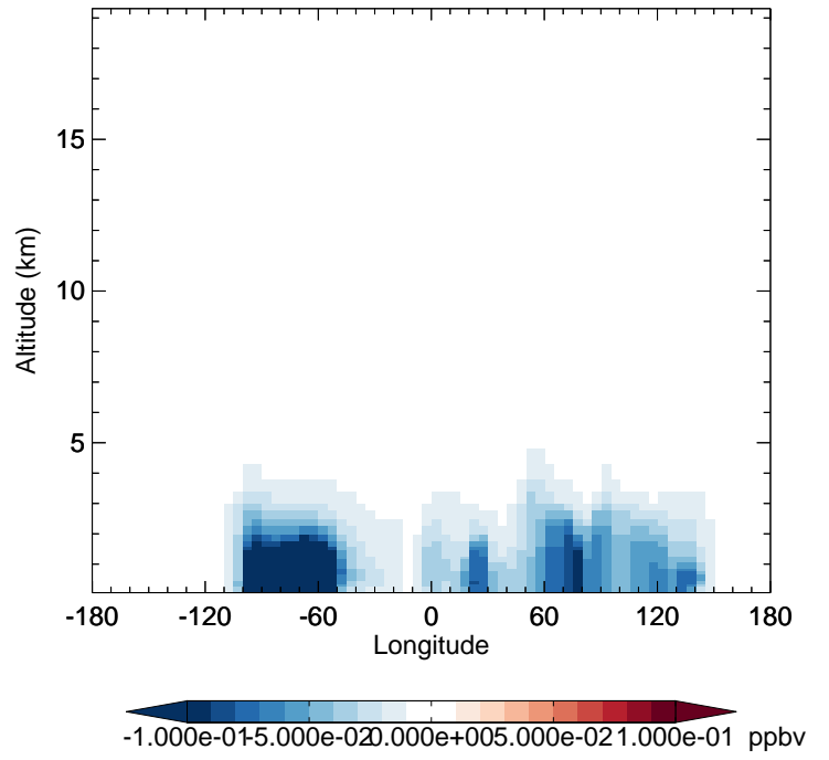
v11-02f-Run0 - v11-02e-Run1 SOAIE - Diff along 42N for Jul
