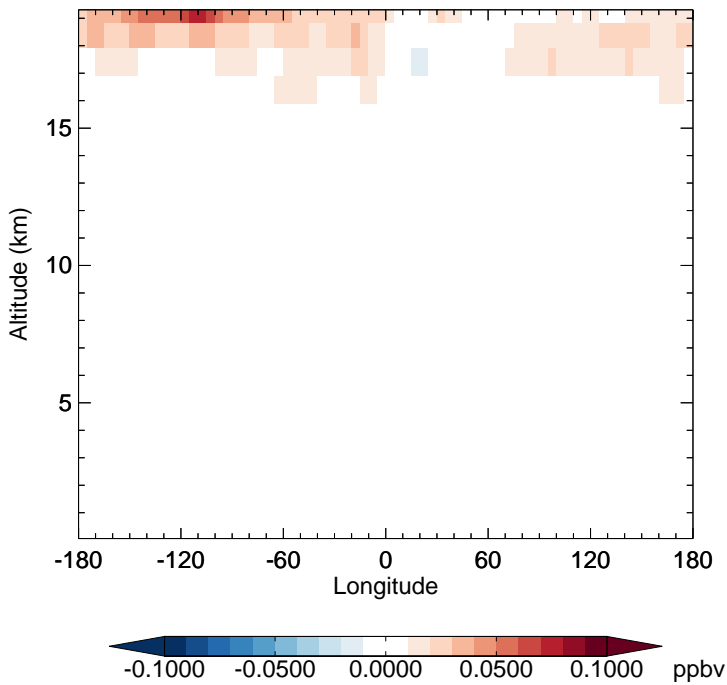
v11-02f-Run0 - v11-02e-Run0 OCS - Diff along 15S for Jul
