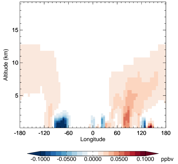
v11-02f-Run0 - v11-02e-Run1 PAN - Diff along 42N for Jul
