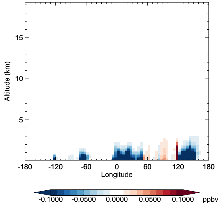
v11-02f-Run0 - v11-02e-Run1 TOLU - Diff along 42N for Jul
