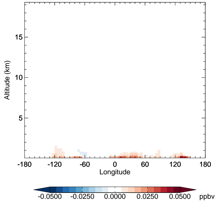
v11-02f-Run0 - v11-02e-Run1 RCHO - Diff along 42N for Jul
