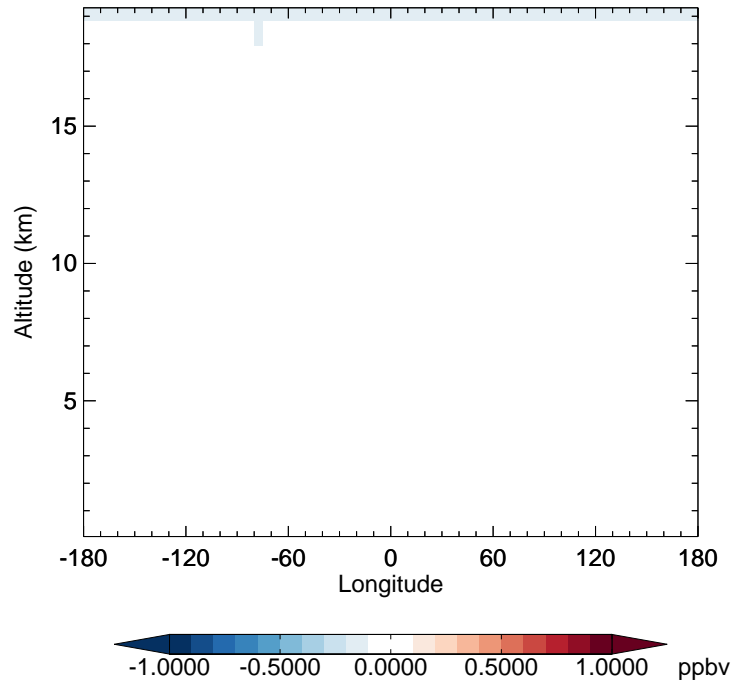
v11-02f-Run0 - v11-02e-Run1 NO - Diff along 42N for Jul
