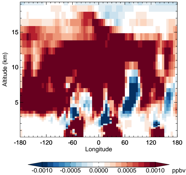
v11-02f-Run0 - v11-02e-Run0 PPN - Diff along 15S for Jul
