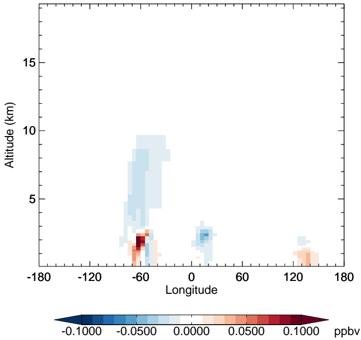
v11-02f-Run0 - v11-02e-Run0 ISO3 - Diff along 15S for Jul
