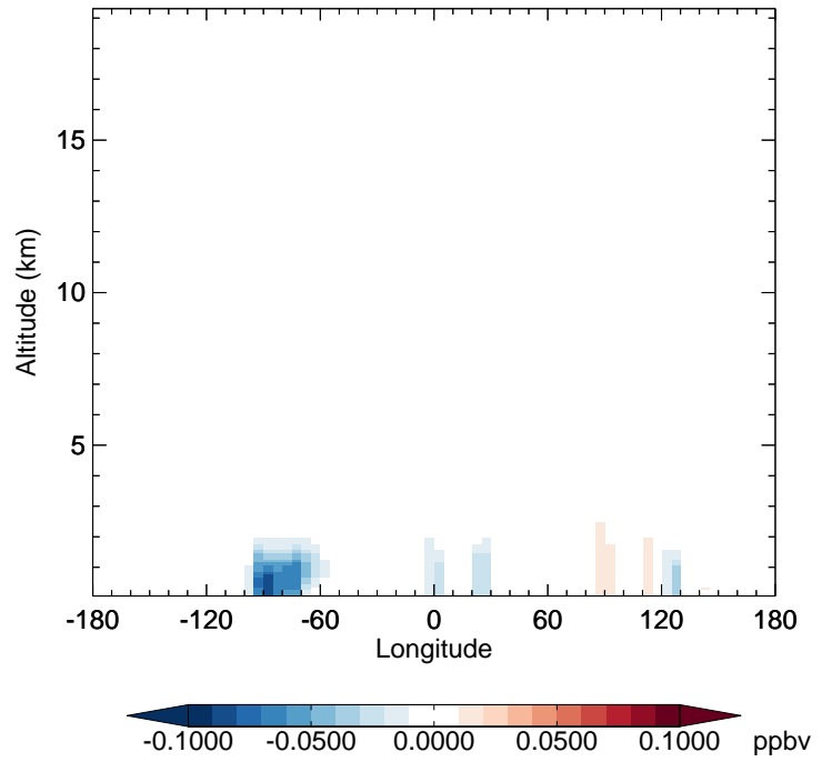
v11-02f-Run0 - v11-02e-Run1 IMAE - Diff along 42N for Jul
