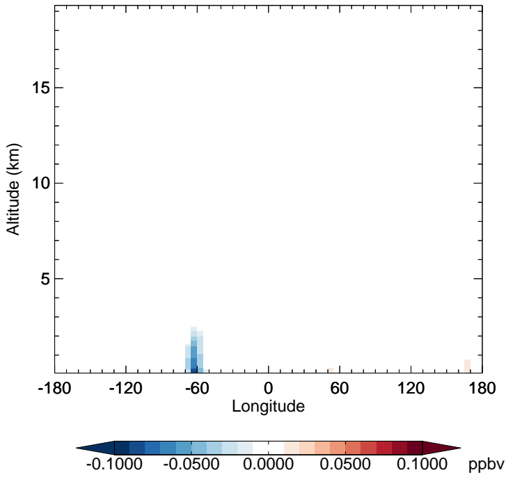
v11-02f-Run0 - v11-02e-Run1 MTPA - Diff along 15S for Jul
