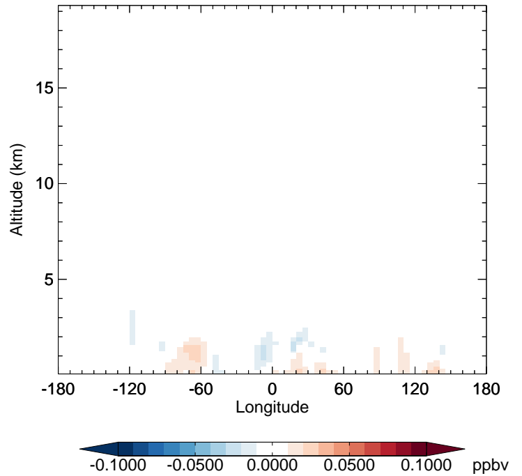
v11-02f-Run0 - v11-02e-Run0 TSOG2 - Diff along 42N for Jul
