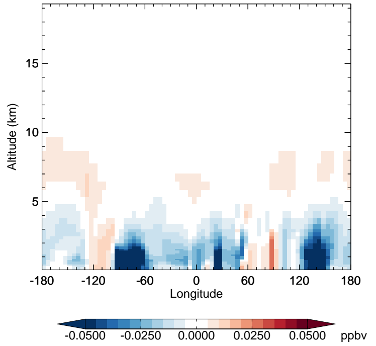
v11-02f-Run0 - v11-02e-Run1 MP - Diff along 42N for Jul
