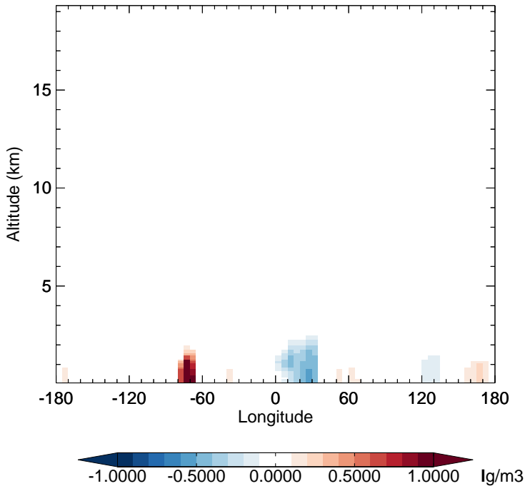
v11-02f-Run0 - v11-02e-Run1 SO4 - Diff along 15S for Jul
