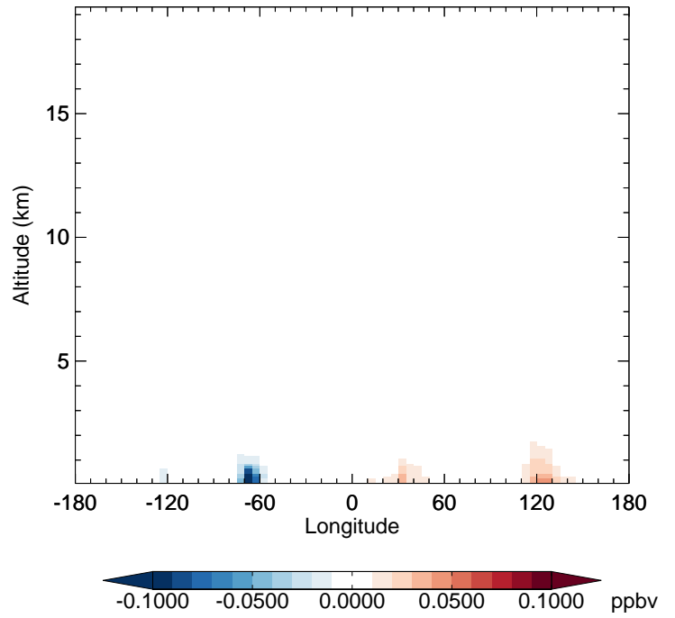
v11-02f-Run0 - v11-02e-Run1 SOAP - Diff along 42N for Jul
