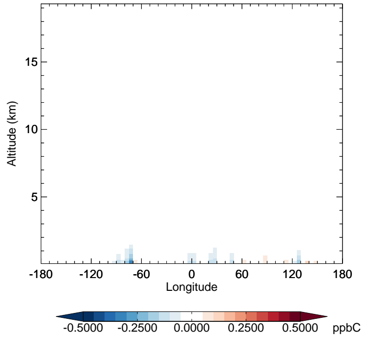
v11-02f-Run0 - v11-02e-Run1 ISOP - Diff along 42N for Jul
