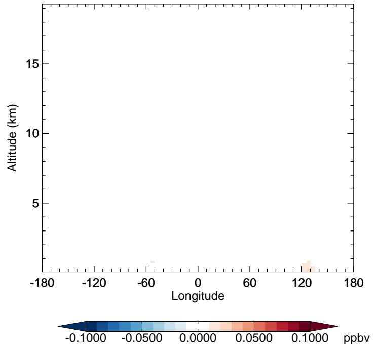
v11-02f-Run0 - v11-02e-Run0 TSOA3 - Diff along 42N for Jul
