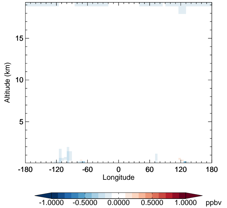
v11-02f-Run0 - v11-02e-Run0 NO2 - Diff along 42N for Jul
