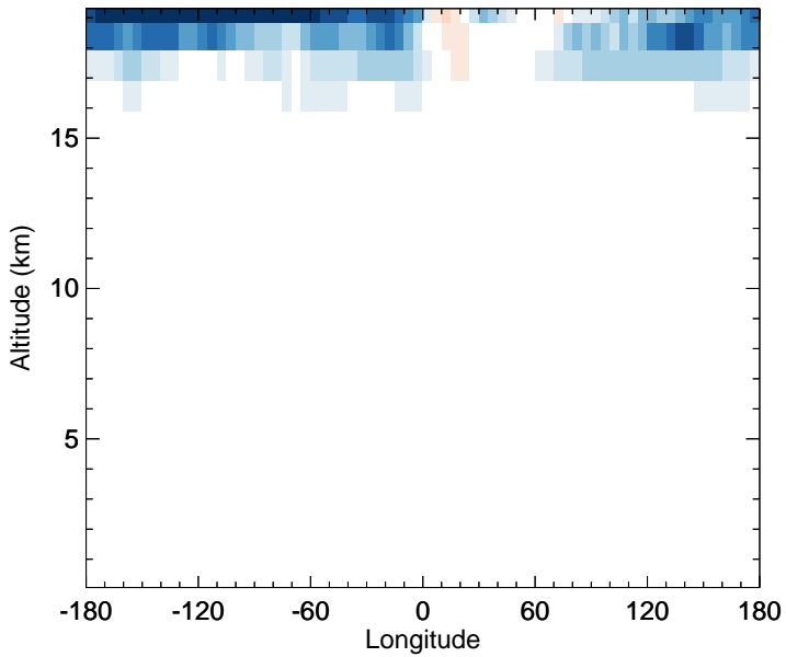
v11-02f-Run0 - v11-02e-Run0 ClNO 3 - Diff along 15S for Jul
