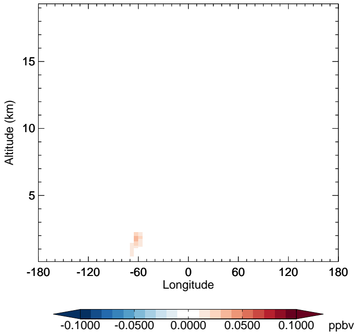
v11-02f-Run0 - v11-02e-Run0 TSOA1 - Diff along 15S for Jul
