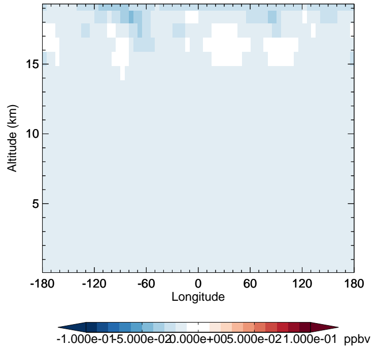
v11-02f-Run0 - v11-02e-Run0 CFC12 - Diff along 42N for Jul
