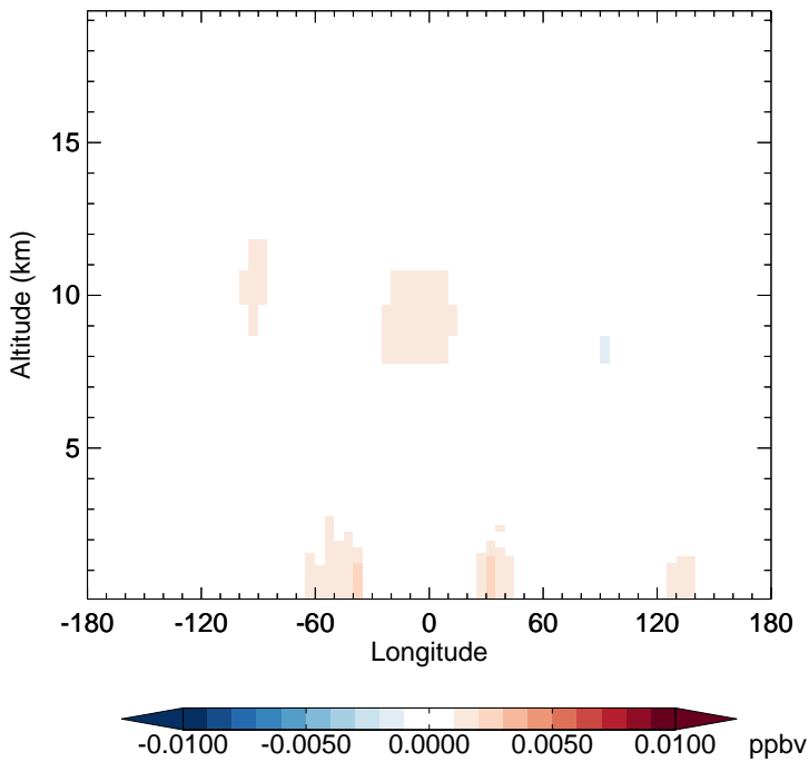
v11-02f-Run0 - v11-02e-Run0 R4N2 - Diff along 15S for Jul
