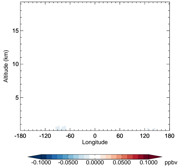
v11-02f-Run0 - v11-02e-Run1 GLYX - Diff along 42N for Jul
