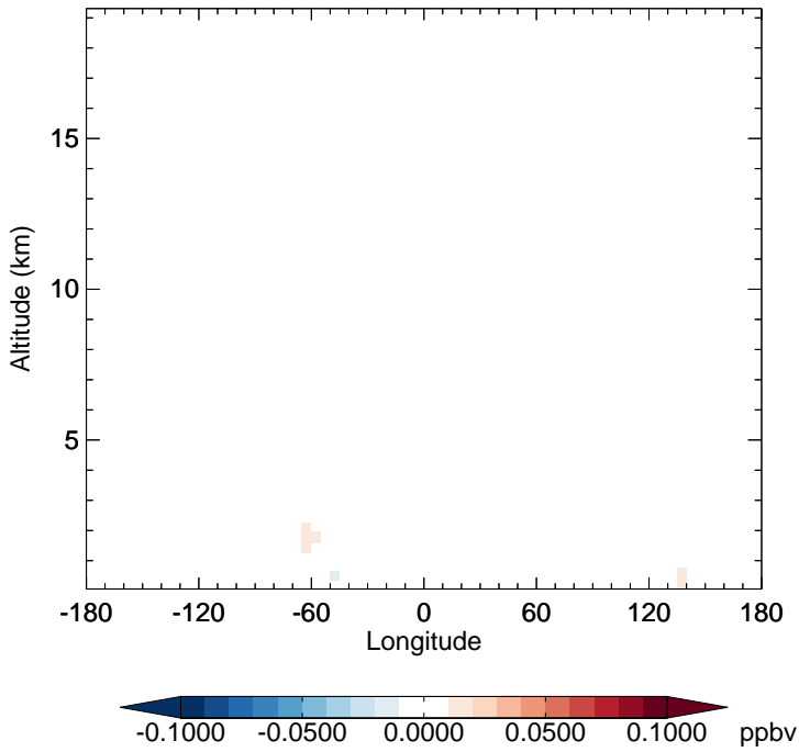
v11-02f-Run0 - v11-02e-Run0 GLYX - Diff along 15S for Jul
