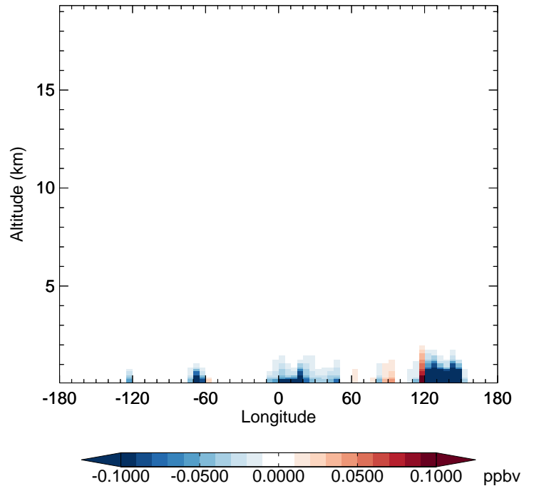
v11-02f-Run0 - v11-02e-Run1 XYLE - Diff along 42N for Jul
