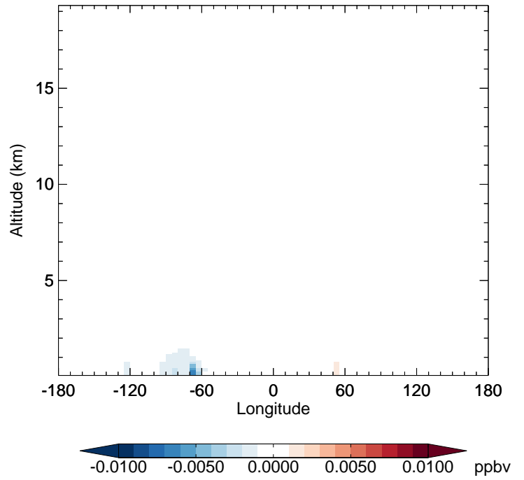
v11-02f-Run0 - v11-02e-Run1 R4N2 - Diff along 42N for Jul
