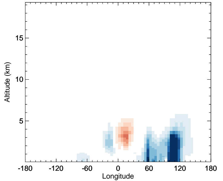
v11-02f-Run0 - v11-02e-Run0 DST1 - Diff along 42N for Jul
