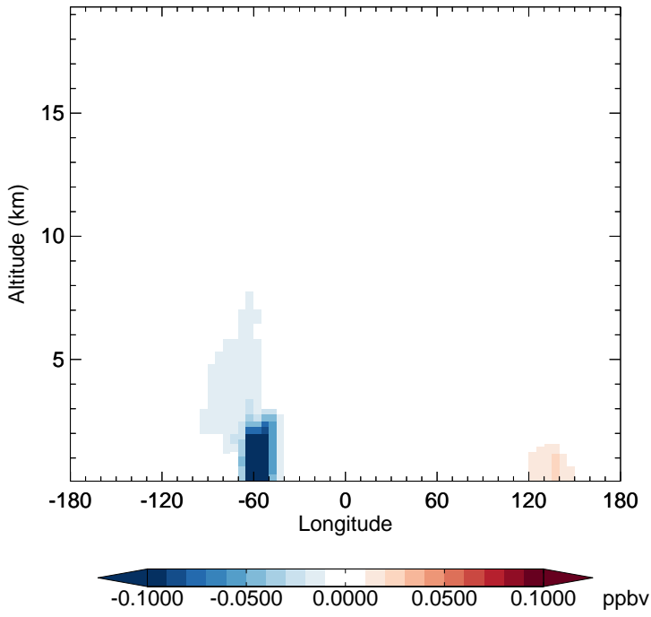
v11-02f-Run0 - v11-02e-Run1 ISO3 - Diff along 15S for Jul
