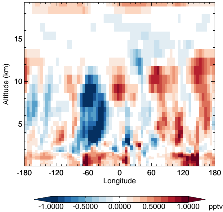
v11-02f-Run0 - v11-02e-Run0 HO2 - Diff along 15S for Jul
