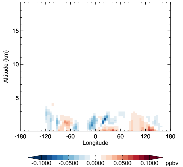
v11-02f-Run0 - v11-02e-Run0 TSOG3 - Diff along 42N for Jul
