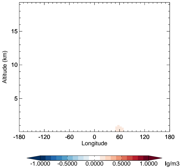
v11-02f-Run0 - v11-02e-Run0 DMS - Diff along 15S for Jul
