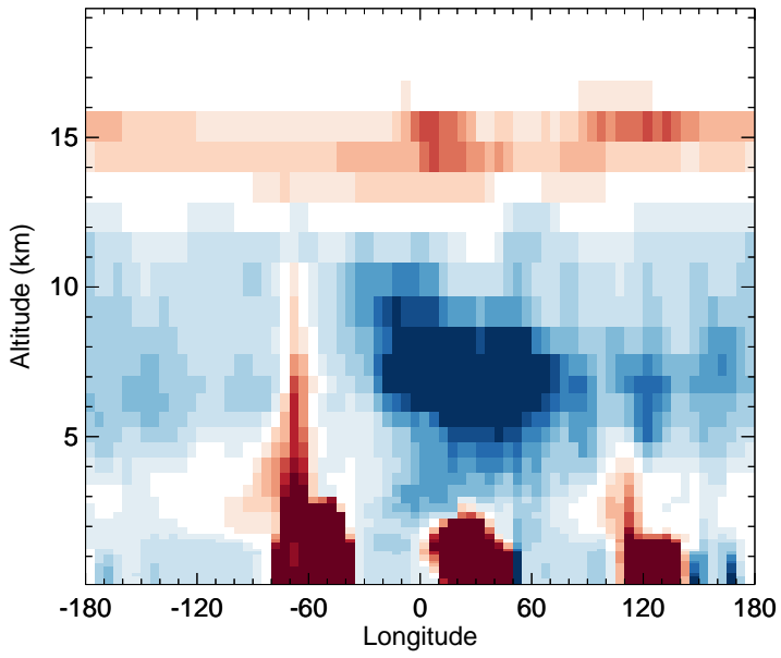
v11-02f-Run0 - v11-02e-Run1 OH - Diff along 15S for Jul
