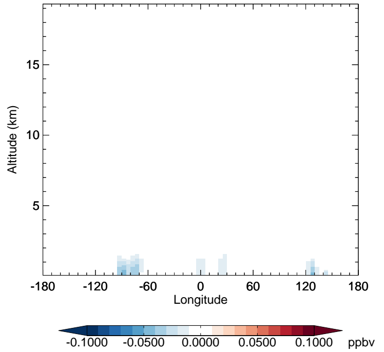
v11-02f-Run0 - v11-02e-Run1 MGLY - Diff along 42N for Jul
