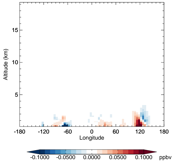
v11-02f-Run0 - v11-02e-Run0 SOAP - Diff along 42N for Jul
