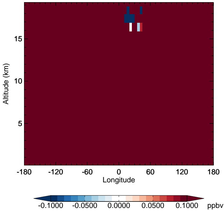
v11-02f-Run0 - v11-02e-Run0 N2O - Diff along 15S for Jul
