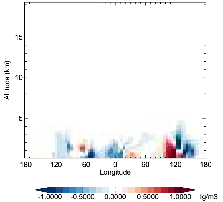
v11-02f-Run0 - v11-02e-Run0 SOAS - Diff along 42N for Jul
