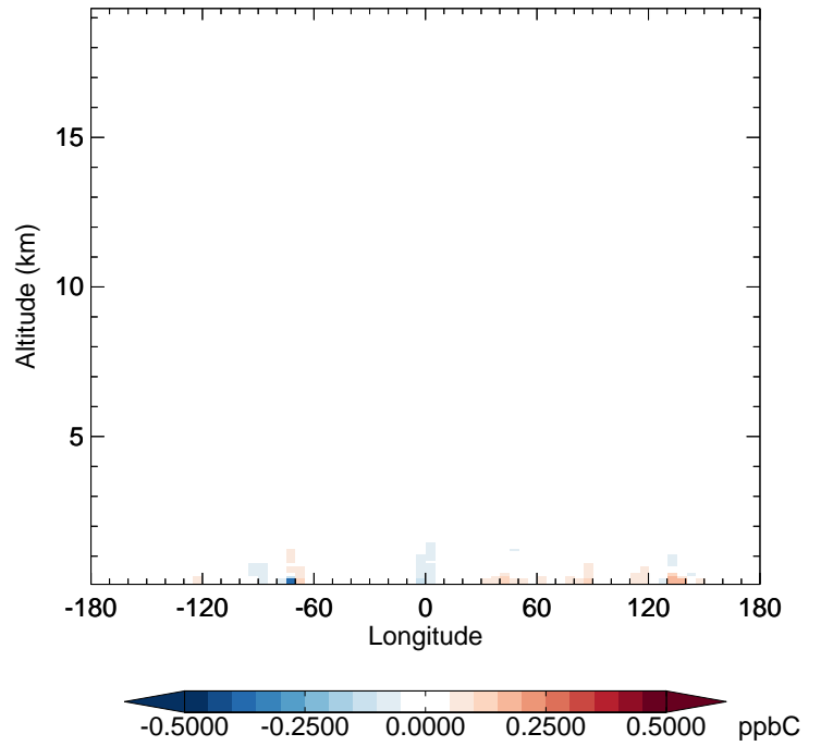
v11-02f-Run0 - v11-02e-Run0 ISOP - Diff along 42N for Jul
