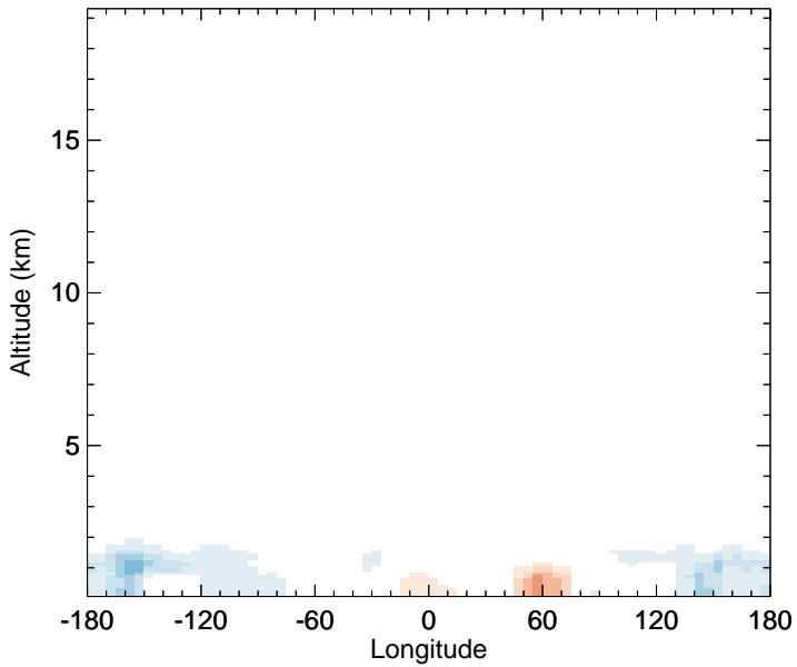
v11-02f-Run0 - v11-02e-Run0 SALA - Diff along 15S for Jul
