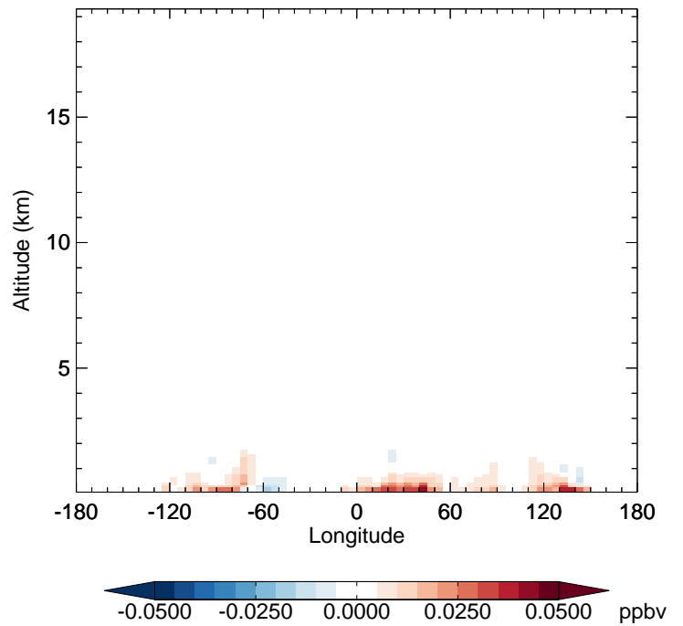
v11-02f-Run0 - v11-02e-Run0 RCHO - Diff along 42N for Jul
