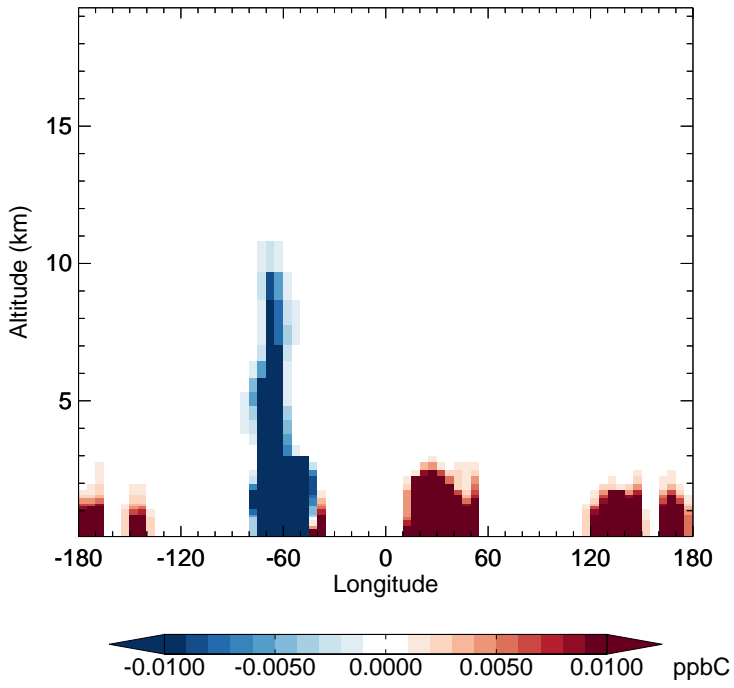
v11-02f-Run0 - v11-02e-Run1 PRPE - Diff along 15S for Jul
