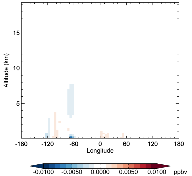
v11-02f-Run0 - v11-02e-Run0 R4N2 - Diff along 42N for Jul
