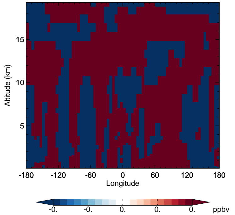
v11-02f-Run0 - v11-02e-Run0 H2O - Diff along 42N for Jul
