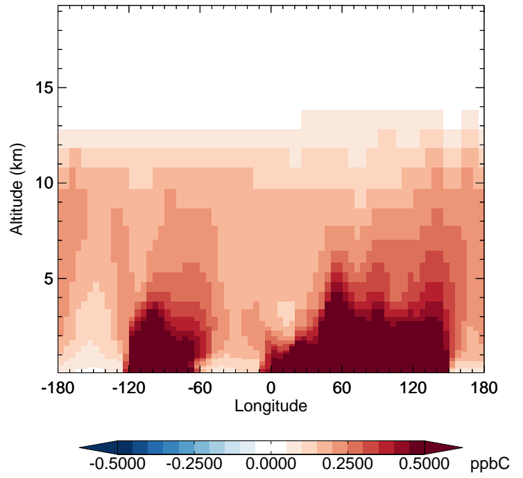
v11-02f-Run0 - v11-02e-Run1 ACET - Diff along 42N for Jul
