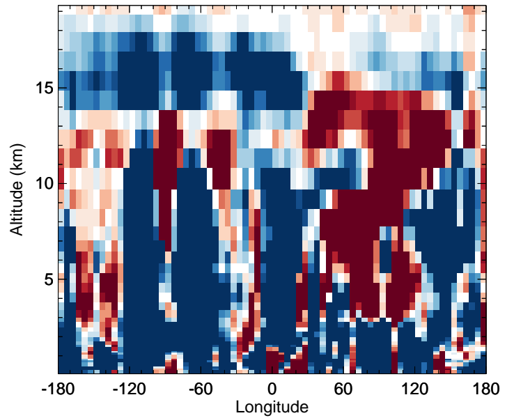
v11-02f-Run0 - v11-02e-Run0 OH - Diff along 42N for Jul
