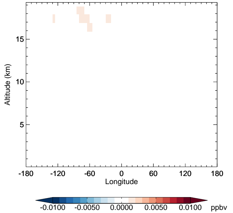
v11-02f-Run0 - v11-02e-Run0 BrNO 3 - Diff along 42N for Jul
