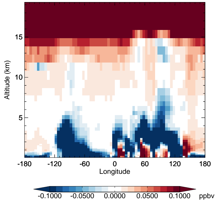
v11-02f-Run0 - v11-02e-Run1 HNO 3 - Diff along 42N for Jul
