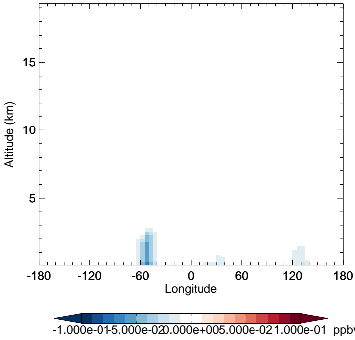
v11-02f-Run0 - v11-02e-Run1 MONITA - Diff along 15S for Jul
