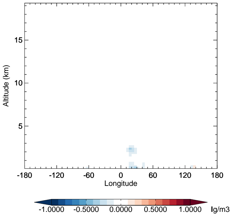
v11-02f-Run0 - v11-02e-Run0 OCPO - Diff along 15S for Jul
