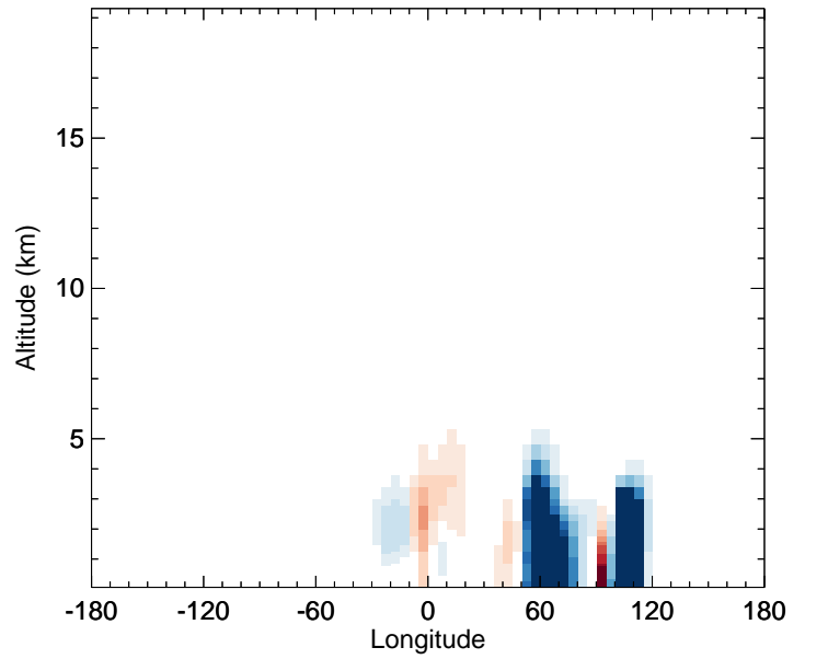
v11-02f-Run0 - v11-02e-Run0 DST3 - Diff along 42N for Jul
