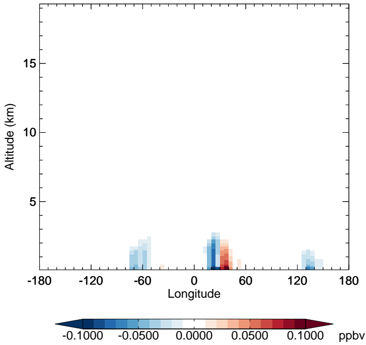
v11-02f-Run0 - v11-02e-Run1 TOLU - Diff along 15S for Jul
