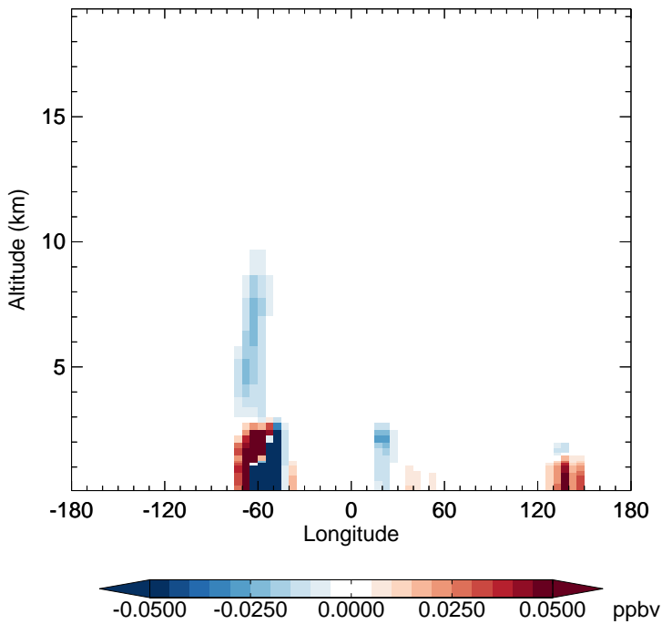
v11-02f-Run0 - v11-02e-Run0 MACR - Diff along 15S for Jul
