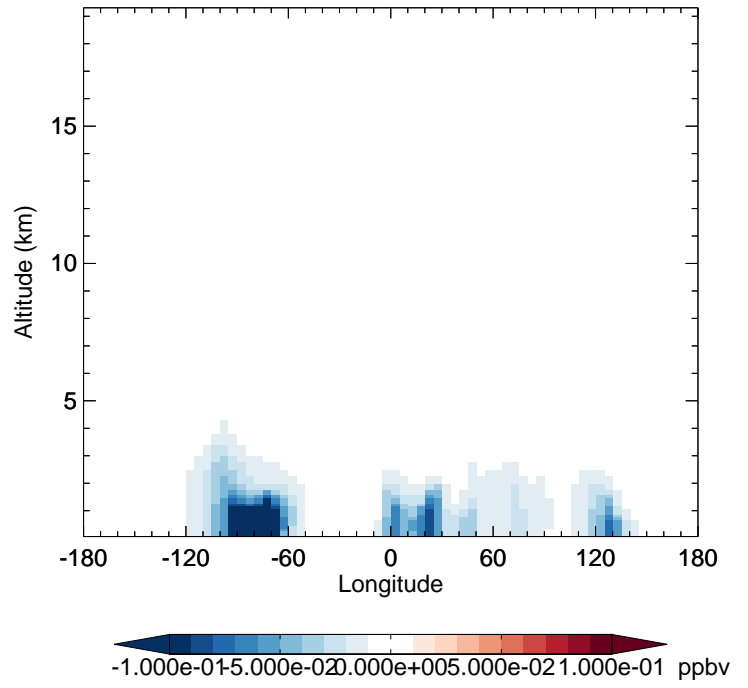
v11-02f-Run0 - v11-02e-Run1 IONITA - Diff along 42N for Jul
