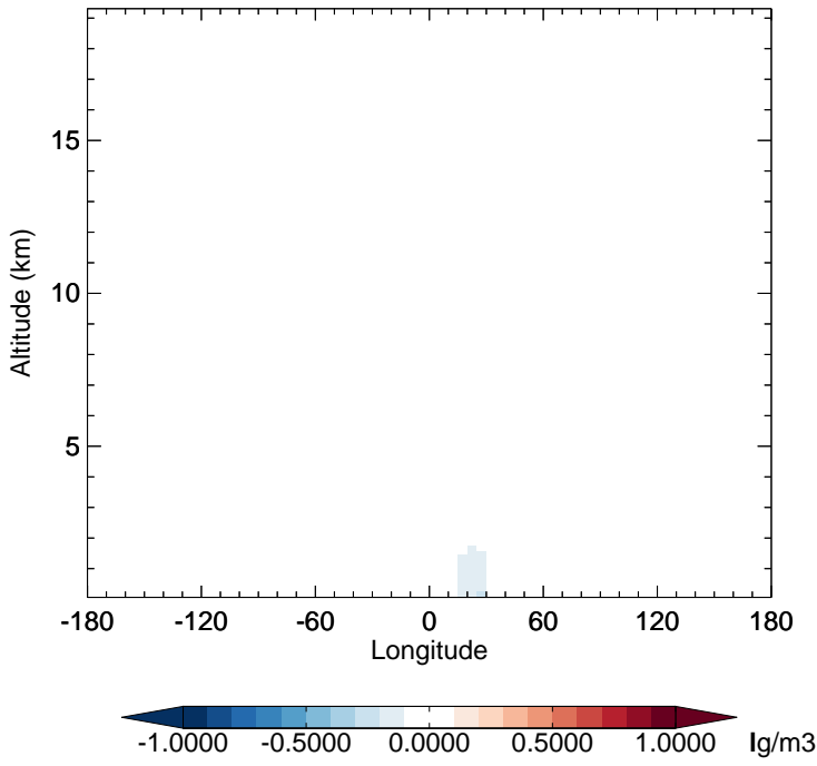
v11-02f-Run0 - v11-02e-Run1 OCPO - Diff along 15S for Jul
