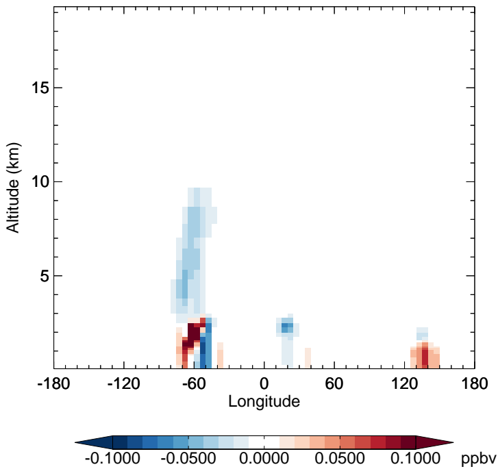
v11-02f-Run0 - v11-02e-Run0 GLYC - Diff along 15S for Jul
