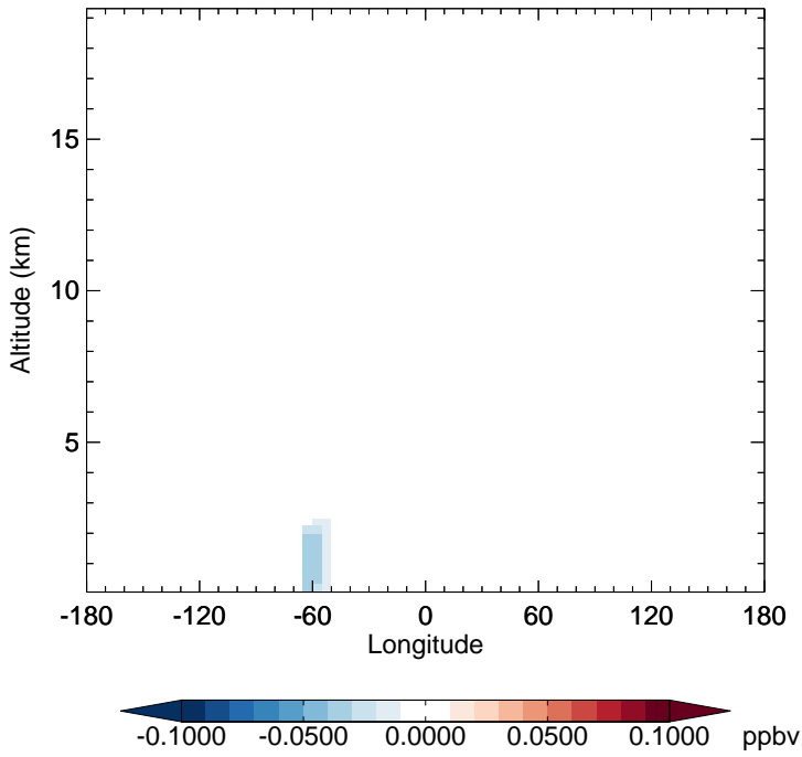
v11-02f-Run0 - v11-02e-Run1 TSOA2 - Diff along 15S for Jul
