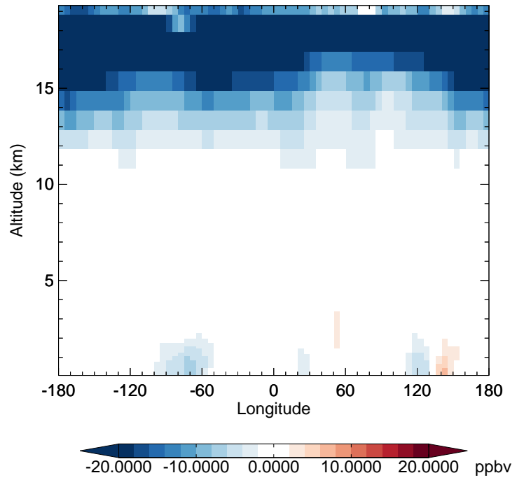
v11-02f-Run0 - v11-02e-Run1 O3 - Diff along 42N for Jul
