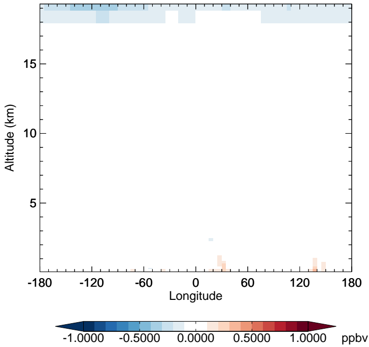
v11-02f-Run0 - v11-02e-Run0 NO2 - Diff along 15S for Jul
