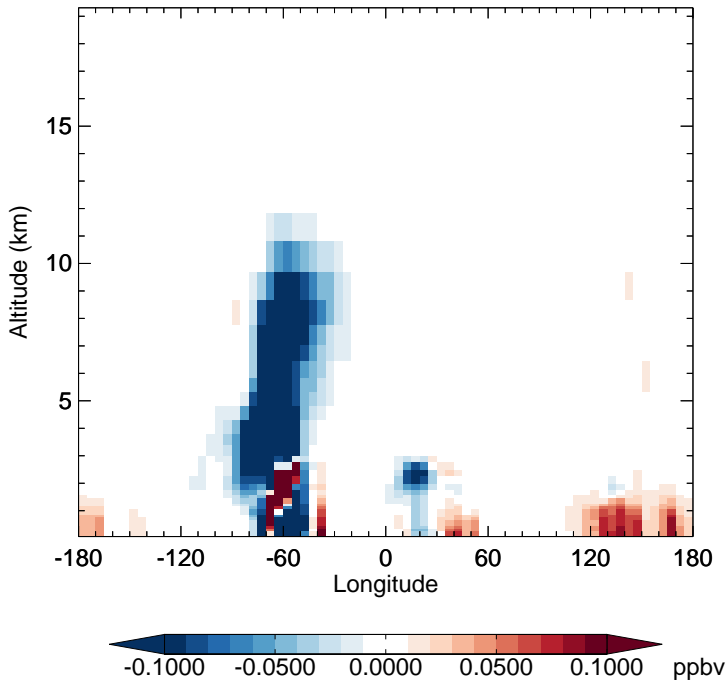
v11-02f-Run0 - v11-02e-Run0 EOH - Diff along 15S for Jul
