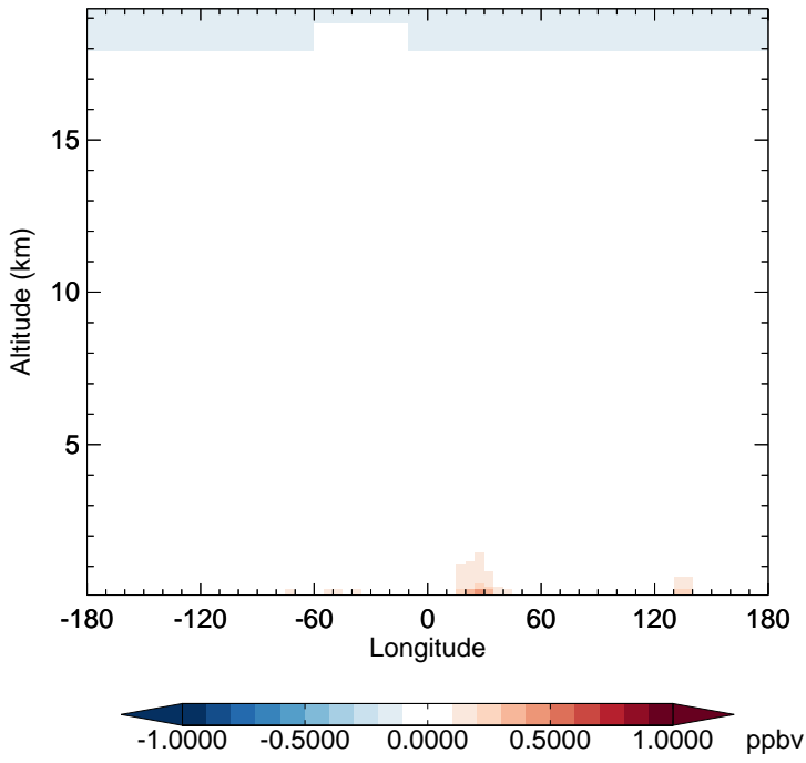
v11-02f-Run0 - v11-02e-Run1 NO2 - Diff along 15S for Jul
