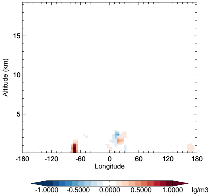
v11-02f-Run0 - v11-02e-Run0 NH4 - Diff along 15S for Jul
