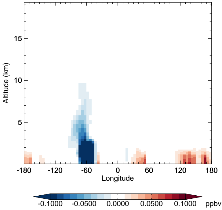
v11-02f-Run0 - v11-02e-Run1 EOH - Diff along 15S for Jul
