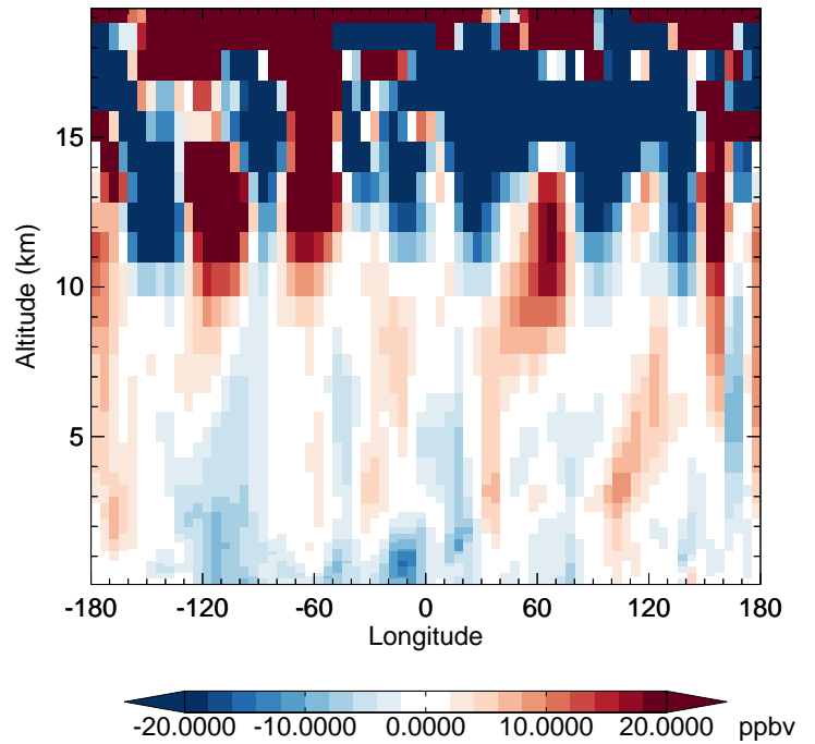
v11-02f-Run0 - v11-02e-Run0 O3 - Diff along 42N for Jul
