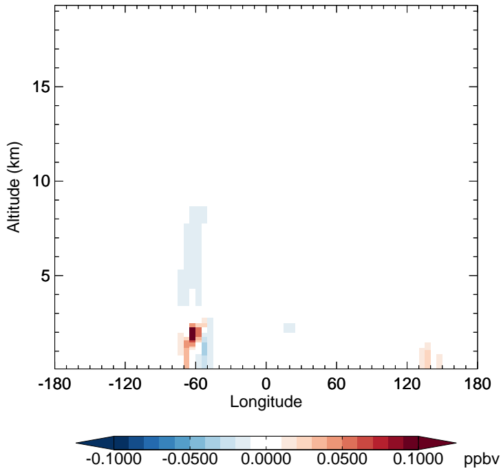
v11-02f-Run0 - v11-02e-Run0 IPMN - Diff along 15S for Jul
