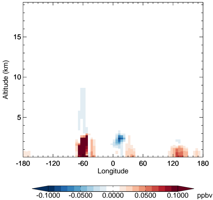
v11-02f-Run0 - v11-02e-Run0 TSOG3 - Diff along 15S for Jul
