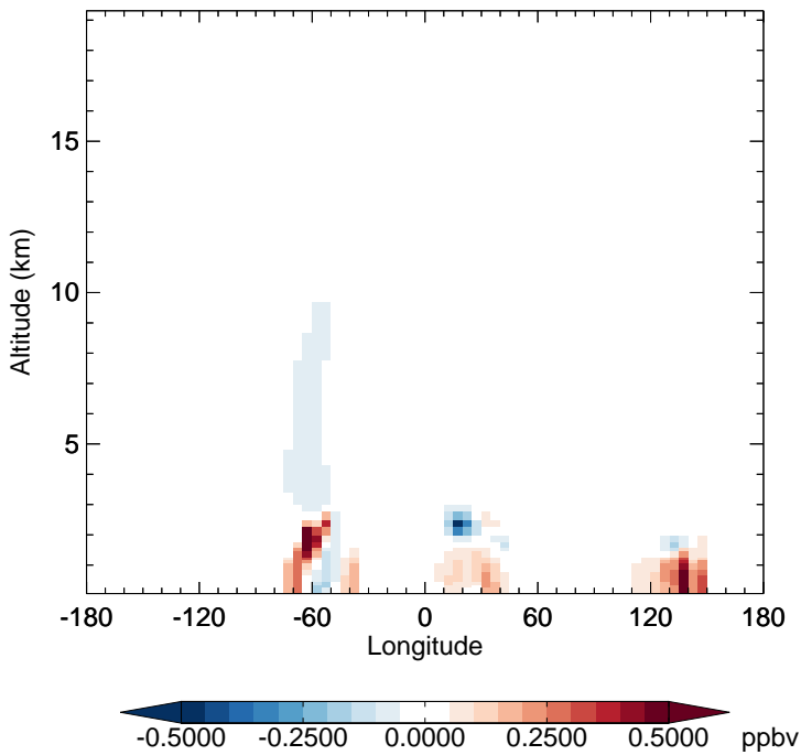
v11-02f-Run0 - v11-02e-Run0 CH 2 O - Diff along 15S for Jul
