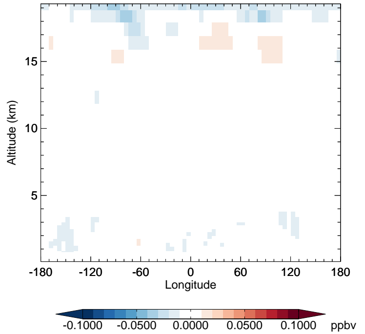
v11-02f-Run0 - v11-02e-Run0 CH3Cl - Diff along 42N for Jul
