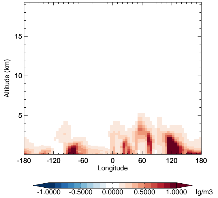
v11-02f-Run0 - v11-02e-Run1 NH4 - Diff along 42N for Jul
