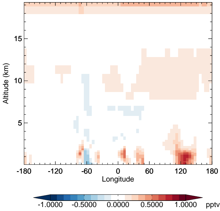
v11-02f-Run0 - v11-02e-Run1 HO2 - Diff along 15S for Jul
