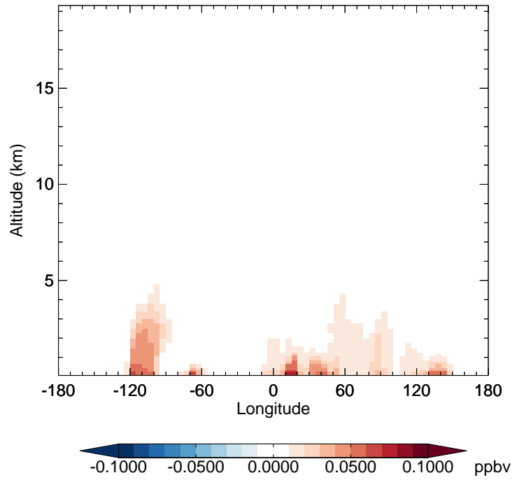
v11-02f-Run0 - v11-02e-Run1 TSOG3 - Diff along 42N for Jul
