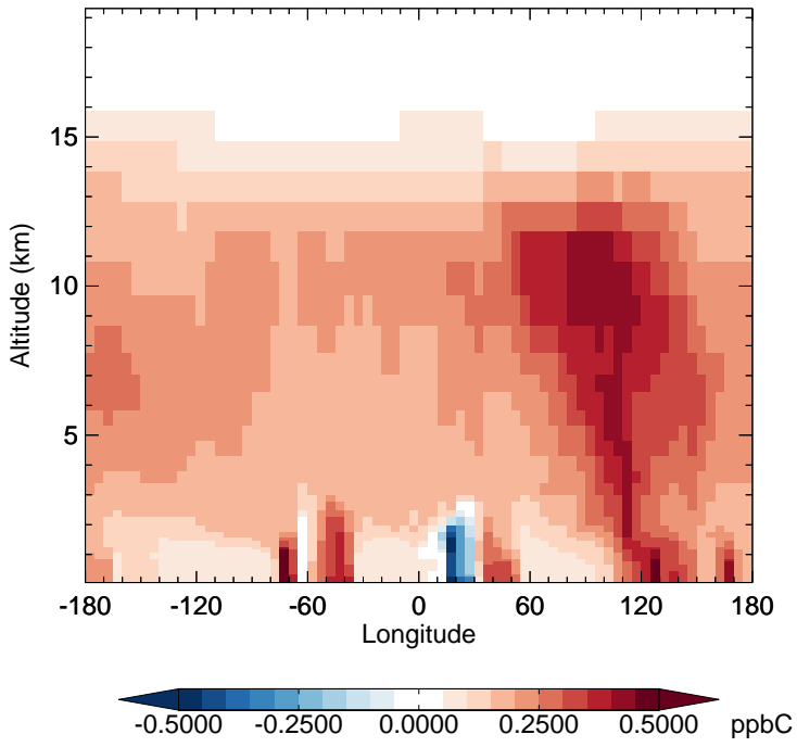
v11-02f-Run0 - v11-02e-Run1 ACET - Diff along 15S for Jul
