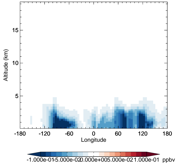
v11-02f-Run0 - v11-02e-Run0 SOAIE - Diff along 42N for Jul
