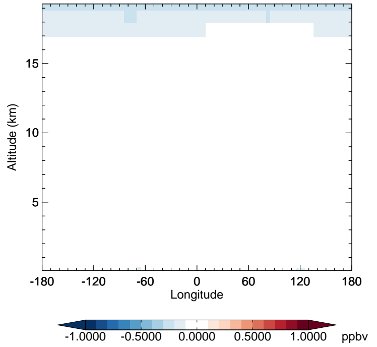
v11-02f-Run0 - v11-02e-Run1 NO2 - Diff along 42N for Jul
