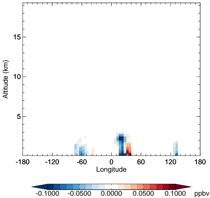
v11-02f-Run0 - v11-02e-Run0 TOLU - Diff along 15S for Jul
