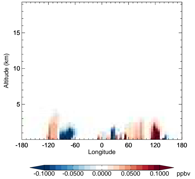
v11-02f-Run0 - v11-02e-Run1 EOH - Diff along 42N for Jul
