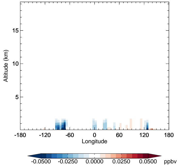
v11-02f-Run0 - v11-02e-Run1 MACR - Diff along 42N for Jul
