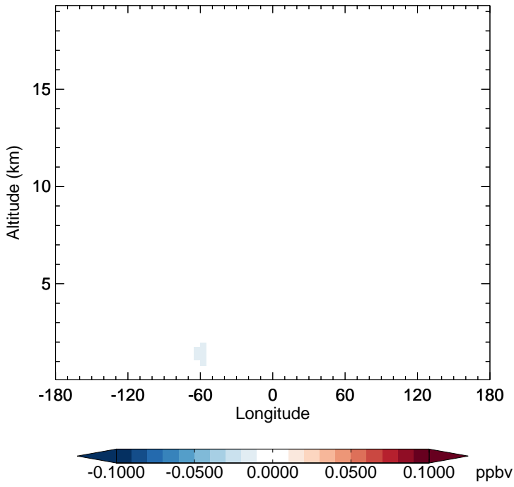
v11-02f-Run0 - v11-02e-Run1 ISOA3 - Diff along 15S for Jul
