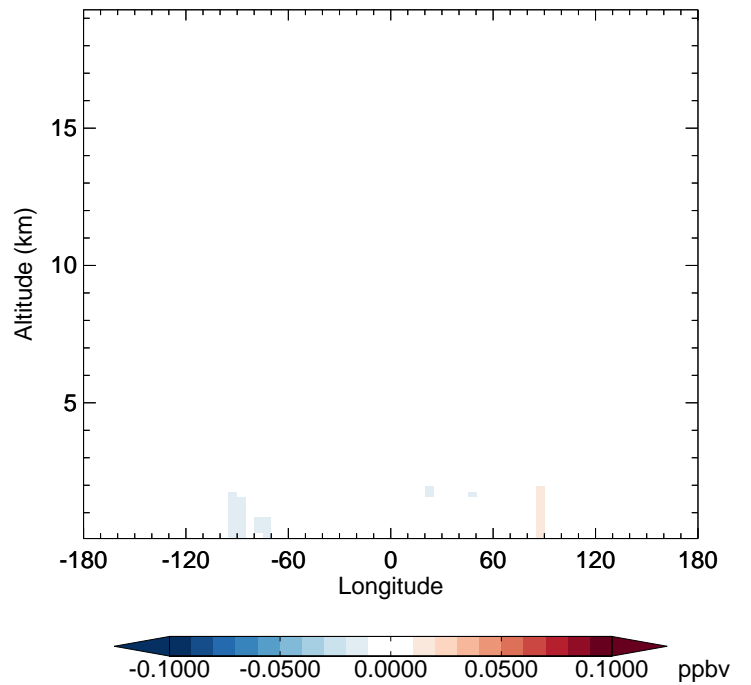
v11-02f-Run0 - v11-02e-Run0 HC187 - Diff along 42N for Jul
