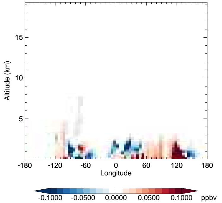
v11-02f-Run0 - v11-02e-Run0 EOH - Diff along 42N for Jul
