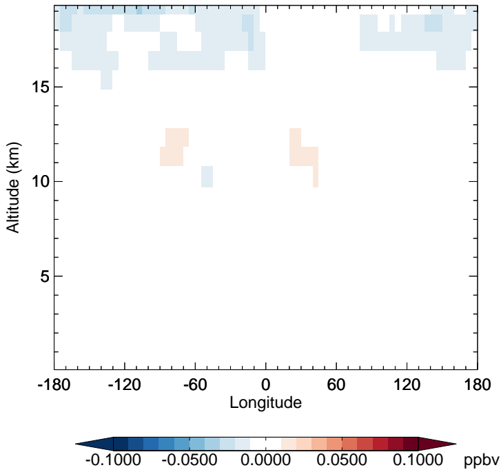
v11-02f-Run0 - v11-02e-Run0 MPN - Diff along 15S for Jul
