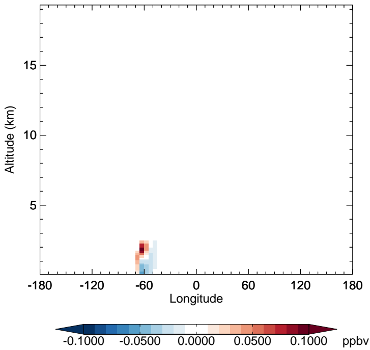
v11-02f-Run0 - v11-02e-Run0 RIPB - Diff along 15S for Jul
