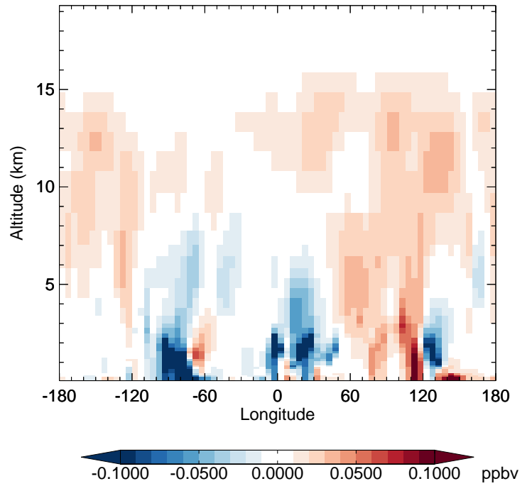
v11-02f-Run0 - v11-02e-Run0 PAN - Diff along 42N for Jul
