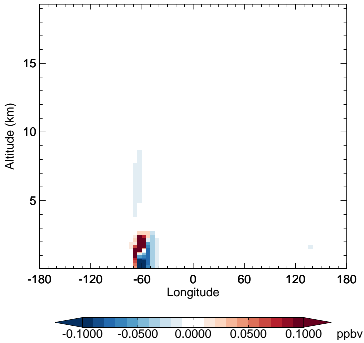
v11-02f-Run0 - v11-02e-Run0 RIPA - Diff along 15S for Jul
