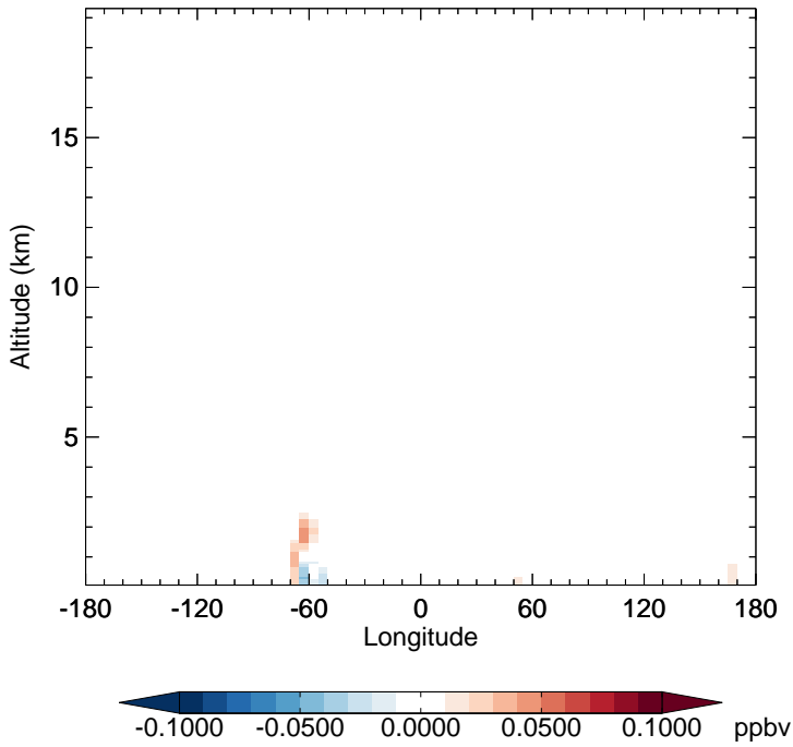
v11-02f-Run0 - v11-02e-Run0 MTPA - Diff along 15S for Jul
