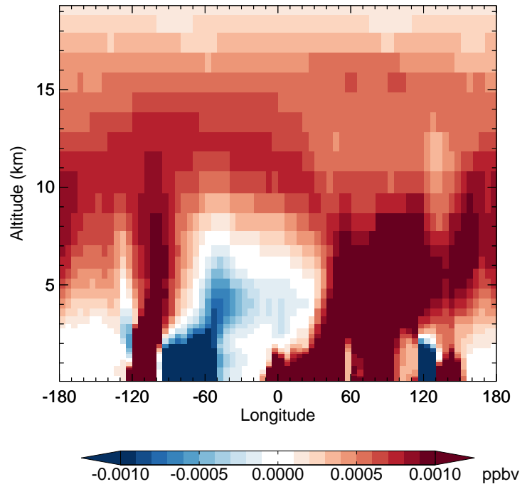
v11-02f-Run0 - v11-02e-Run1 PPN - Diff along 42N for Jul
