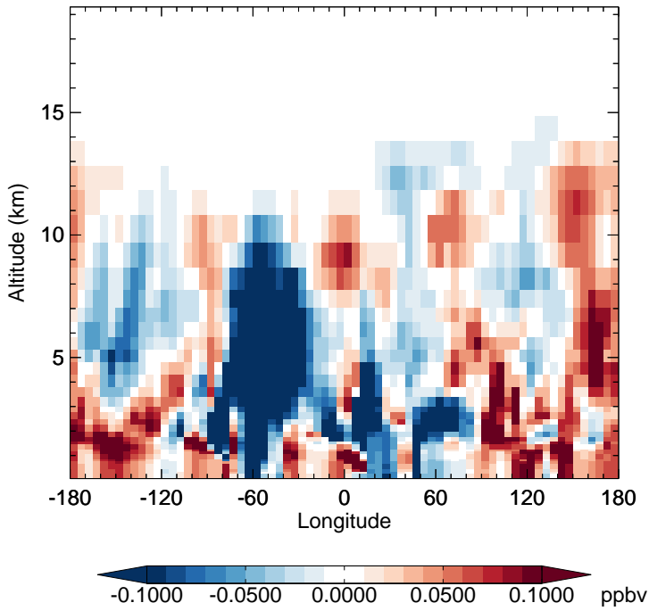
v11-02f-Run0 - v11-02e-Run0 H2O2 - Diff along 15S for Jul
