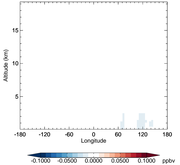
v11-02f-Run0 - v11-02e-Run0 SOAME - Diff along 42N for Jul
