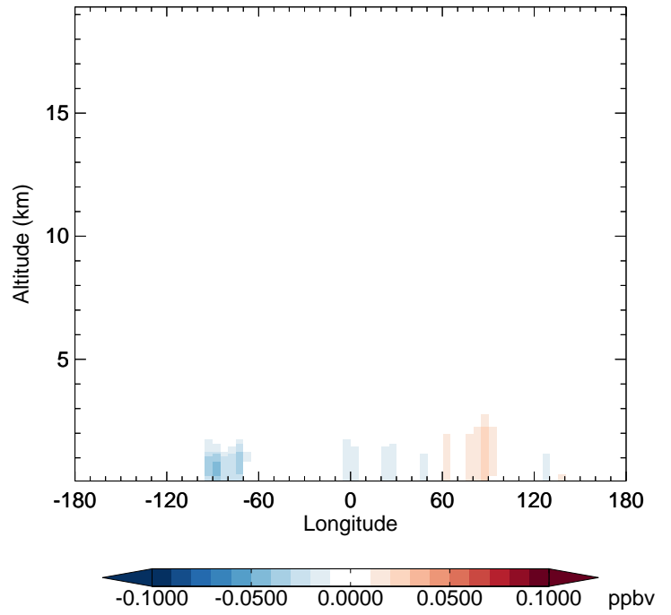
v11-02f-Run0 - v11-02e-Run1 IEPOXA - Diff along 42N for Jul
