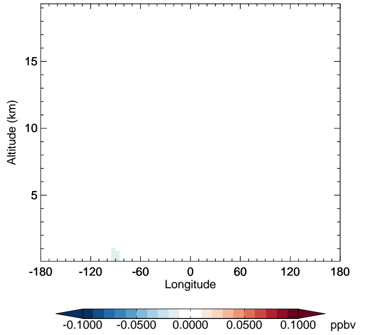
v11-02f-Run0 - v11-02e-Run1 ISO G 1 - Diff along 42N for Jul
