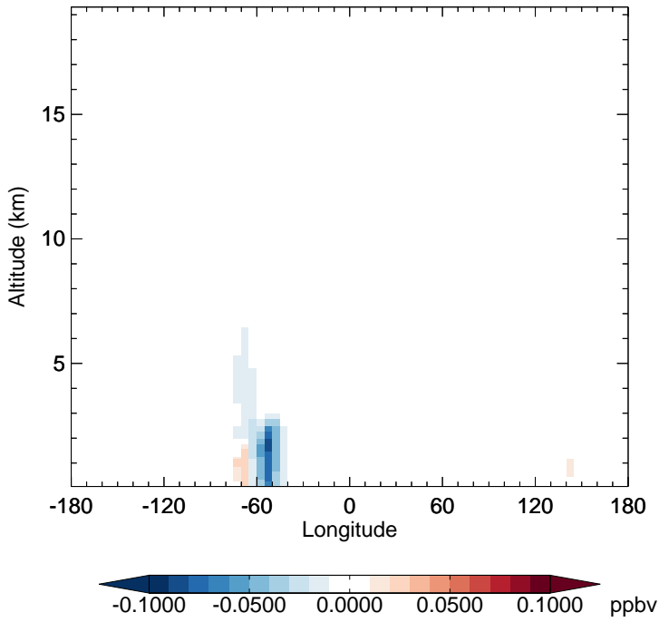
v11-02f-Run0 - v11-02e-Run1 IEPOXB - Diff along 15S for Jul
