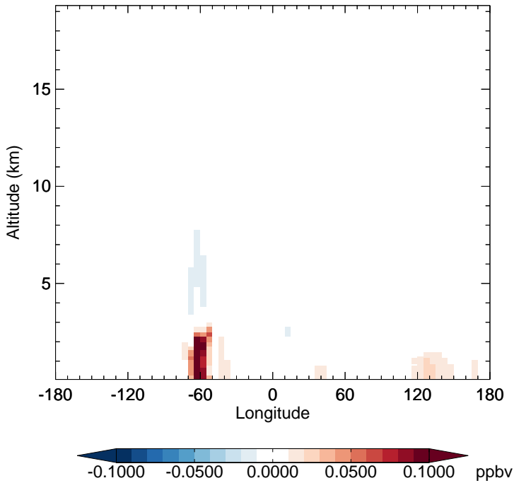
v11-02f-Run0 - v11-02e-Run0 TSOG2 - Diff along 15S for Jul
