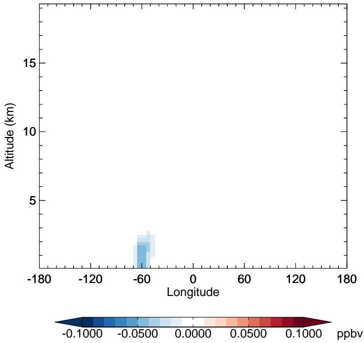
v11-02f-Run0 - v11-02e-Run1 ISOA1 - Diff along 15S for Jul
