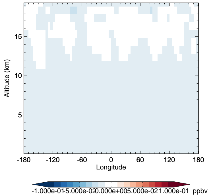
v11-02f-Run0 - v11-02e-Run0 CFC11 - Diff along 42N for Jul
