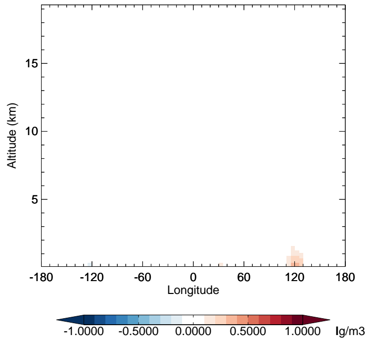
v11-02f-Run0 - v11-02e-Run0 OCPO - Diff along 42N for Jul
