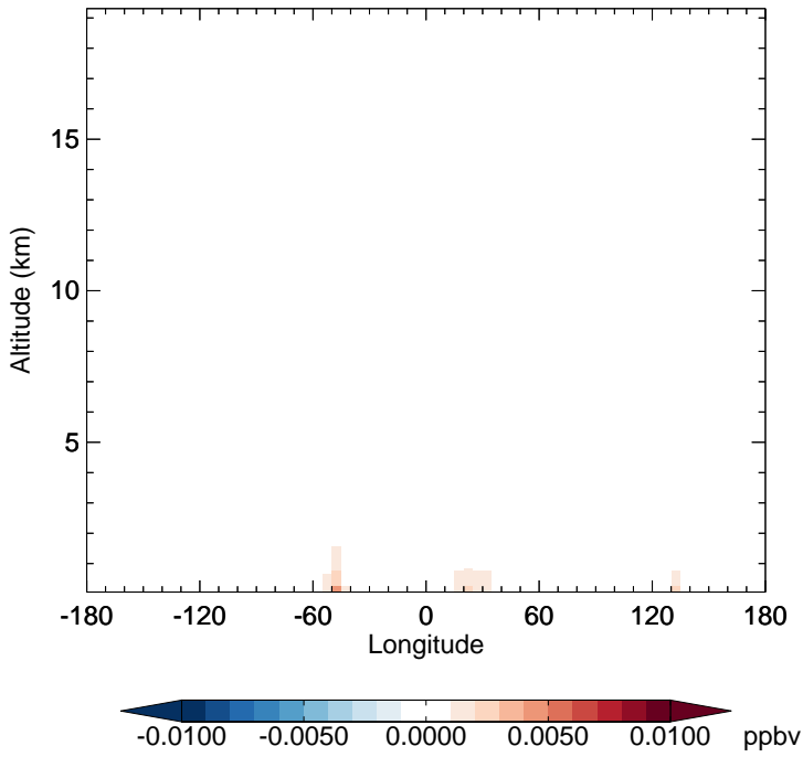
v11-02f-Run0 - v11-02e-Run1 NO3 - Diff along 15S for Jul
