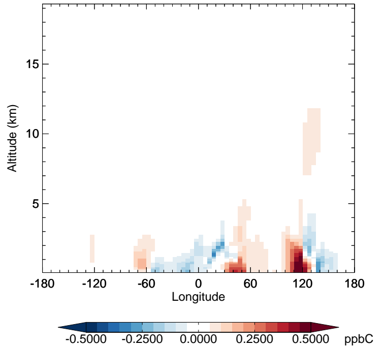
v11-02f-Run0 - v11-02e-Run0 C3H8 - Diff along 42N for Jul
