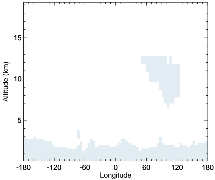
v11-02f-Run0 - v11-02e-Run0 HCFC22 - Diff along 15S for Jul
