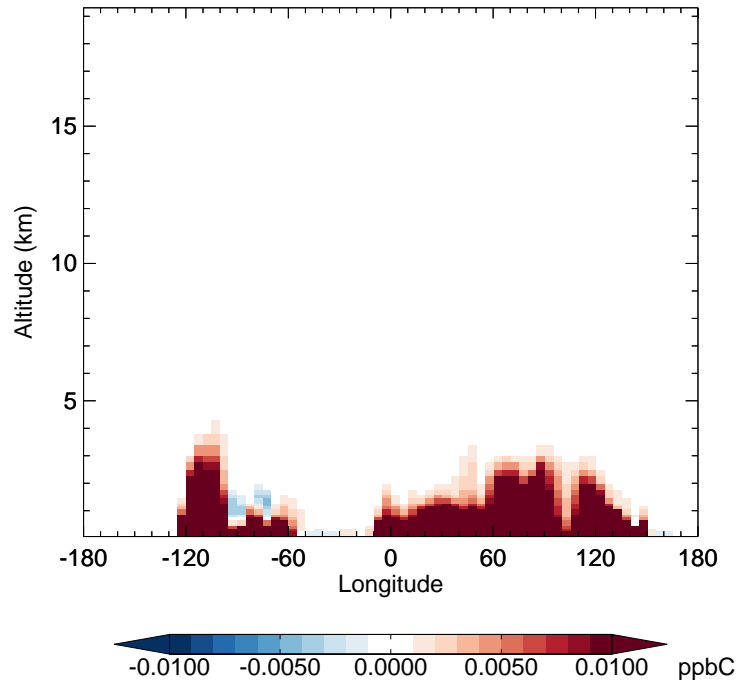
v11-02f-Run0 - v11-02e-Run1 PRPE - Diff along 42N for Jul
