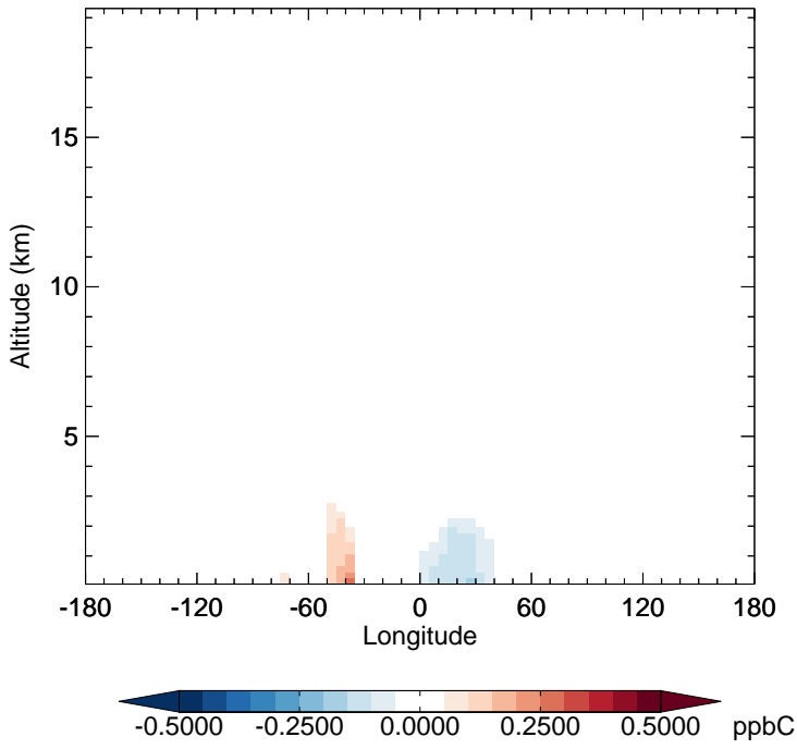
v11-02f-Run0 - v11-02e-Run1 C3H8 - Diff along 15S for Jul
