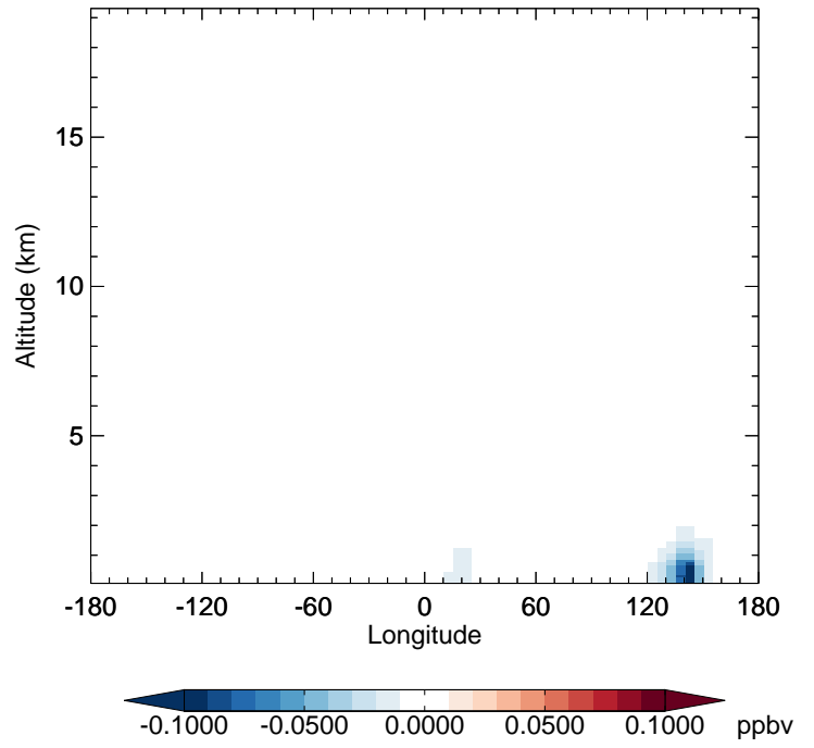
v11-02f-Run0 - v11-02e-Run1 ASOAN - Diff along 42N for Jul
