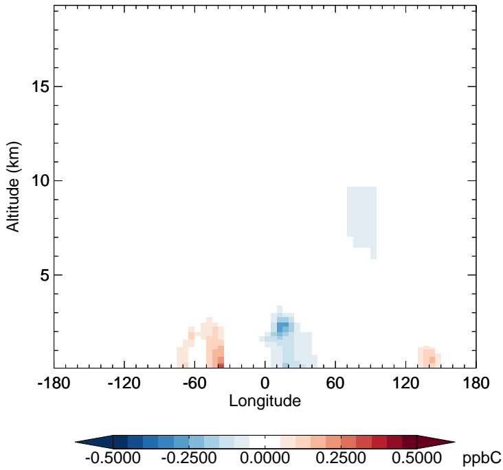
v11-02f-Run0 - v11-02e-Run0 C3H8 - Diff along 15S for Jul
