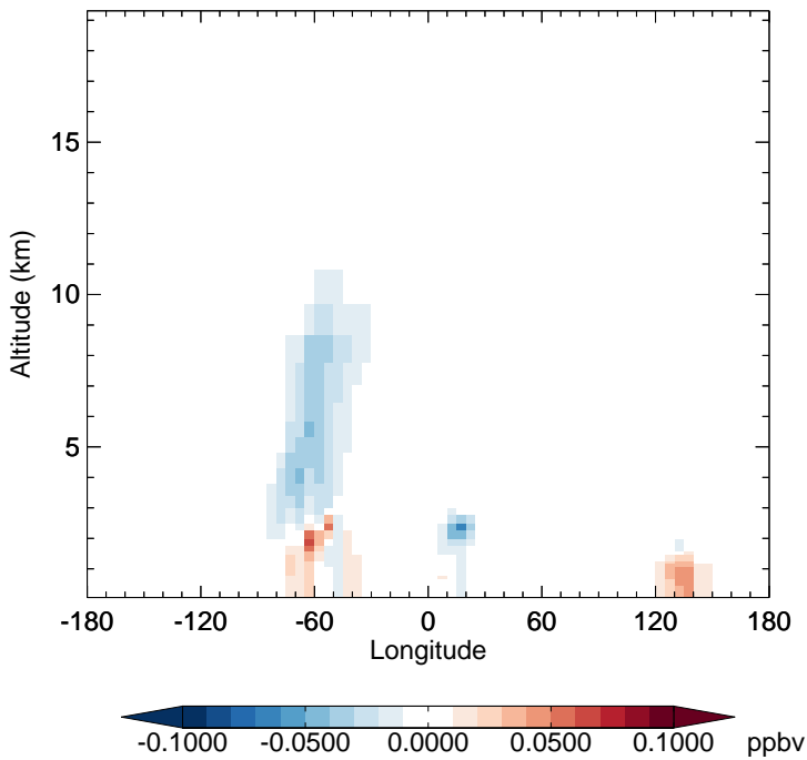
v11-02f-Run0 - v11-02e-Run0 IMAE - Diff along 15S for Jul
