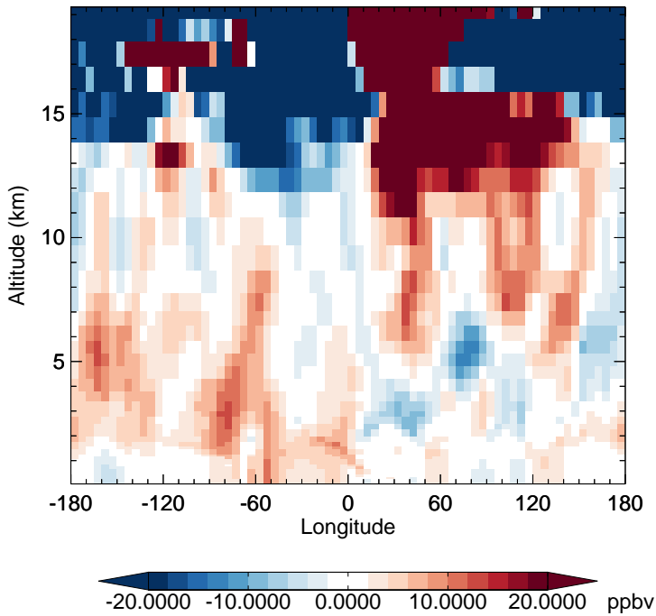
v11-02f-Run0 - v11-02e-Run0 O3 - Diff along 15S for Jul
