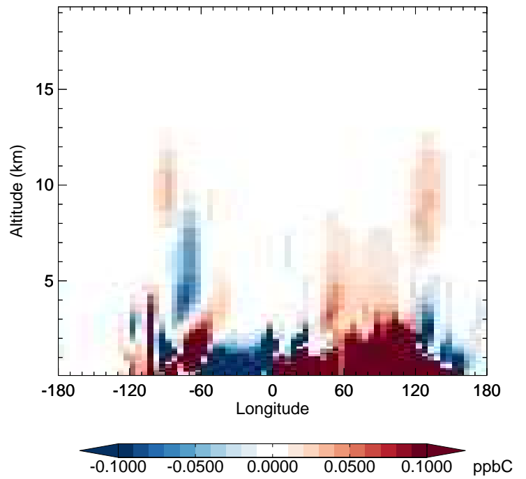
v11-02f-Run0 - v11-02e-Run0 MEK - Diff along 42N for Jul
