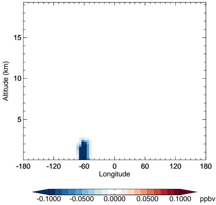
v11-02f-Run0 - v11-02e-Run1 HPALD - Diff along 15S for Jul
