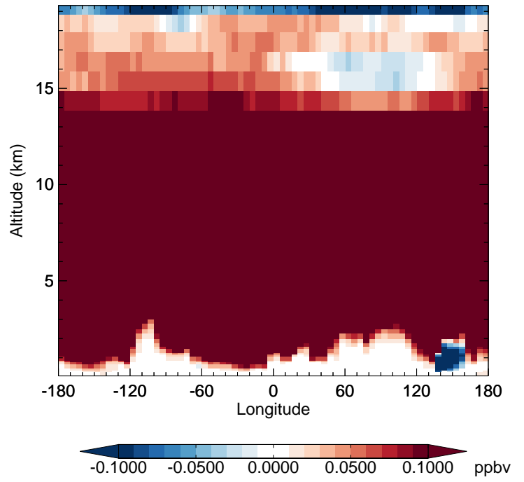
v11-02f-Run0 - v11-02e-Run1 CH4 - Diff along 42N for Jul
