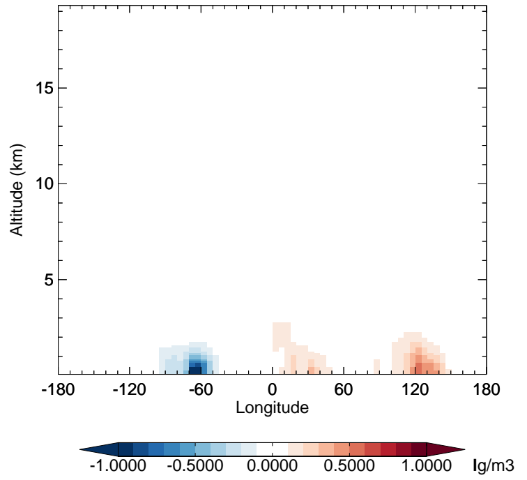
v11-02f-Run0 - v11-02e-Run1 SOAS - Diff along 42N for Jul
