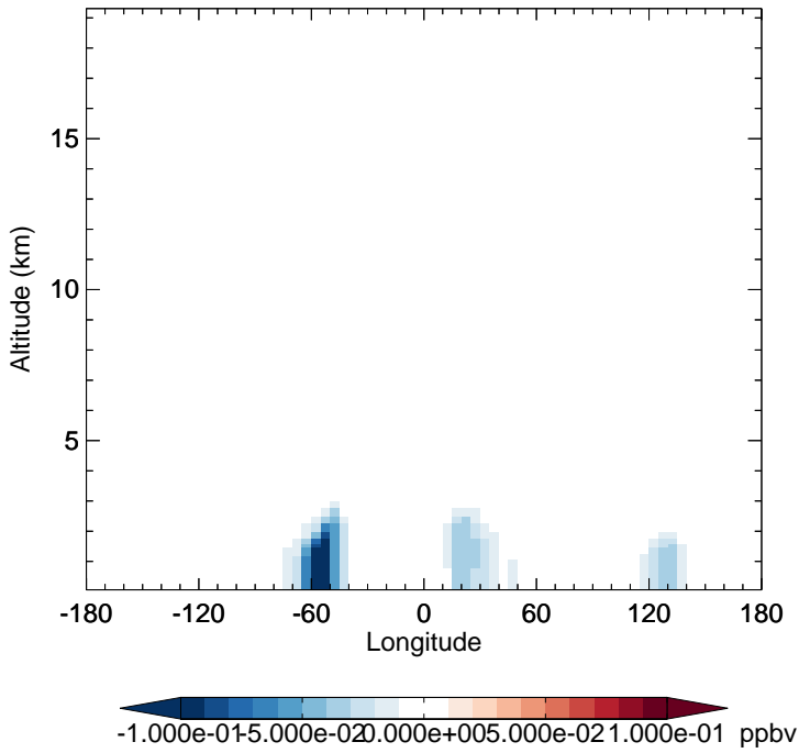
v11-02f-Run0 - v11-02e-Run0 IONITA - Diff along 15S for Jul
