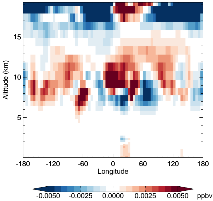
v11-02f-Run0 - v11-02e-Run0 HNO 4 - Diff along 15S for Jul
