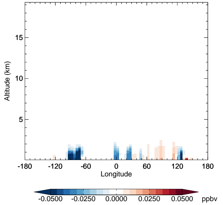
v11-02f-Run0 - v11-02e-Run1 MVK - Diff along 42N for Jul
