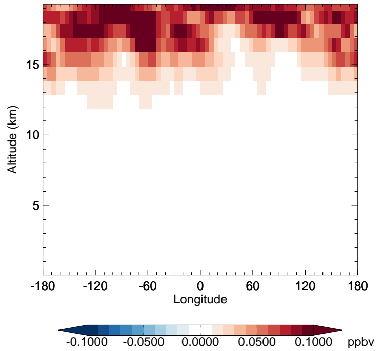
v11-02f-Run0 - v11-02e-Run0 HCl - Diff along 42N for Jul
