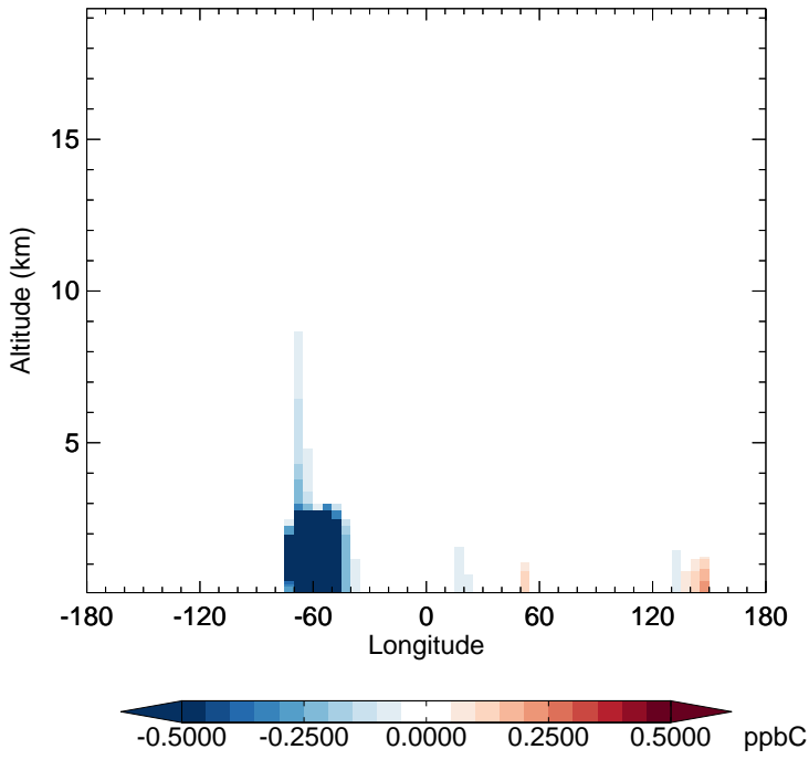
v11-02f-Run0 - v11-02e-Run1 ISOP - Diff along 15S for Jul
