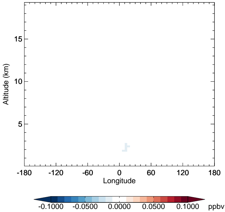
v11-02f-Run0 - v11-02e-Run0 ASOG3 - Diff along 15S for Jul
