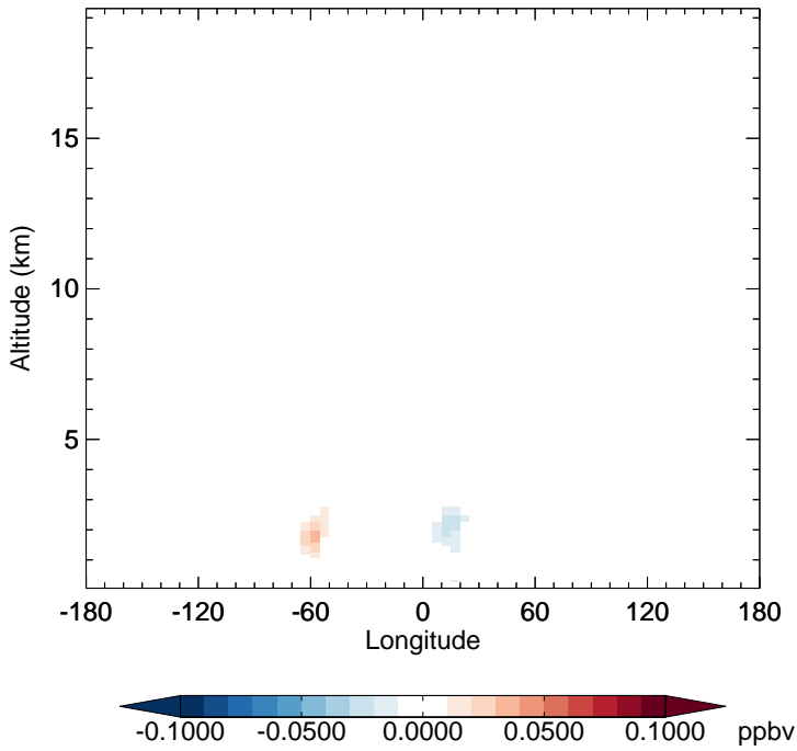
v11-02f-Run0 - v11-02e-Run0 TSOA3 - Diff along 15S for Jul
