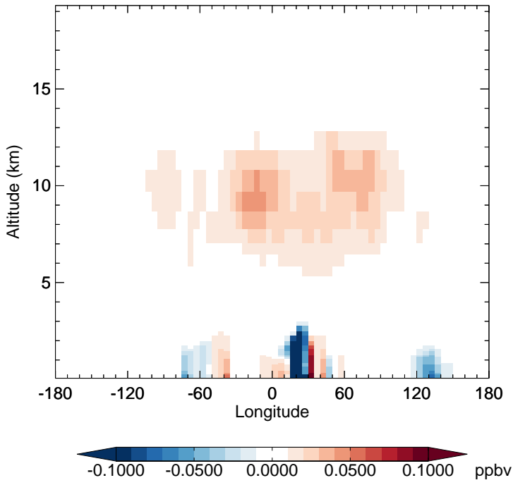
v11-02f-Run0 - v11-02e-Run1 BENZ - Diff along 15S for Jul
