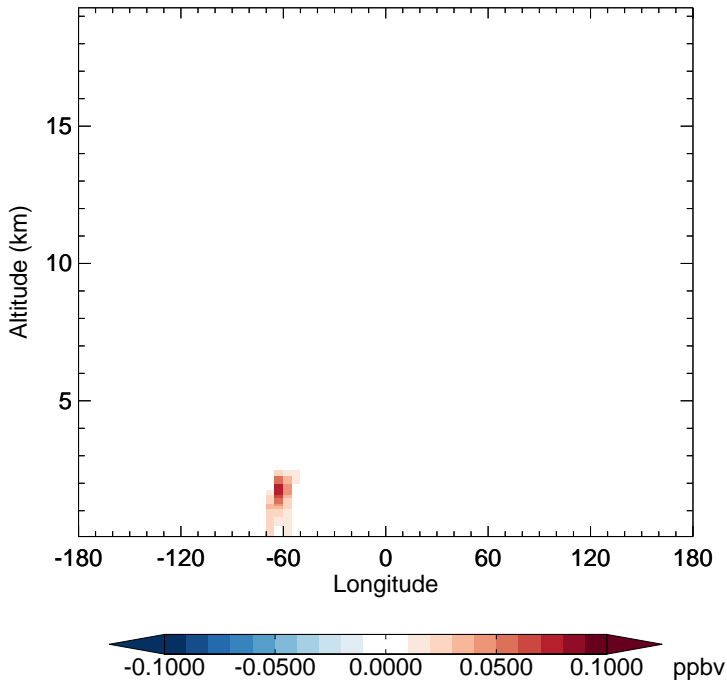
v11-02f-Run0 - v11-02e-Run0 TSOA0 - Diff along 15S for Jul
