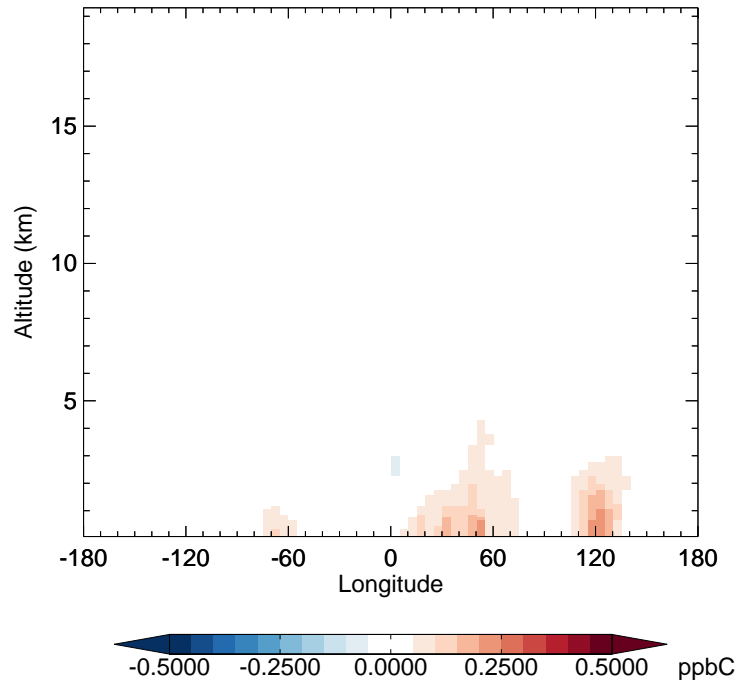
v11-02f-Run0 - v11-02e-Run1 C3H8 - Diff along 42N for Jul
