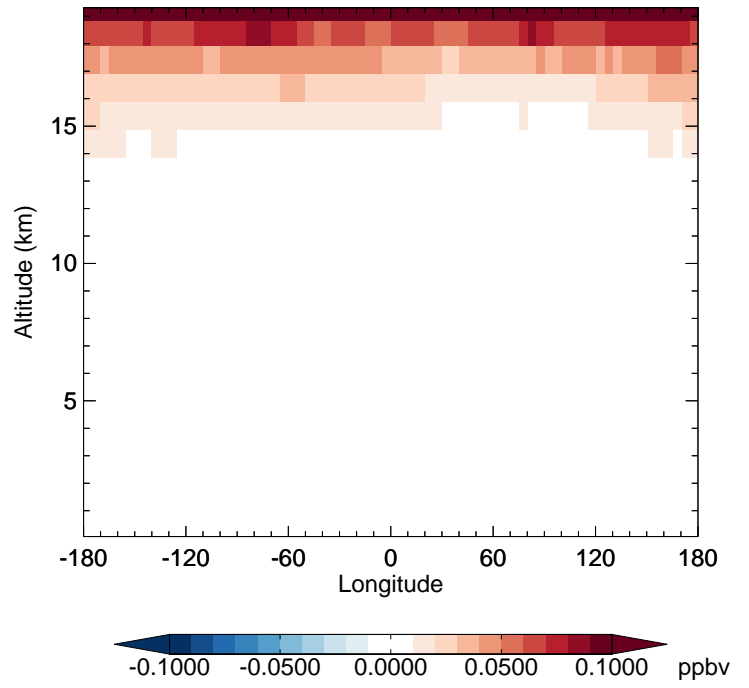
v11-02f-Run0 - v11-02e-Run1 N2O - Diff along 42N for Jul
