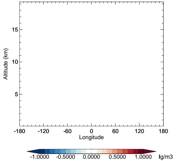
v11-02f-Run0 - v11-02e-Run0 BCPO - Diff along 42N for Jul
