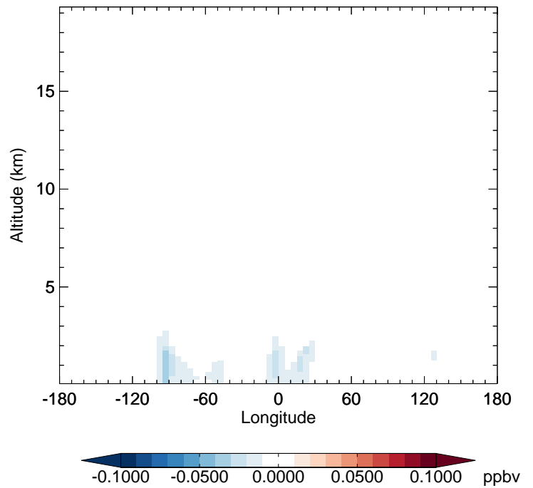
v11-02f-Run0 - v11-02e-Run0 ISOA1 - Diff along 42N for Jul
