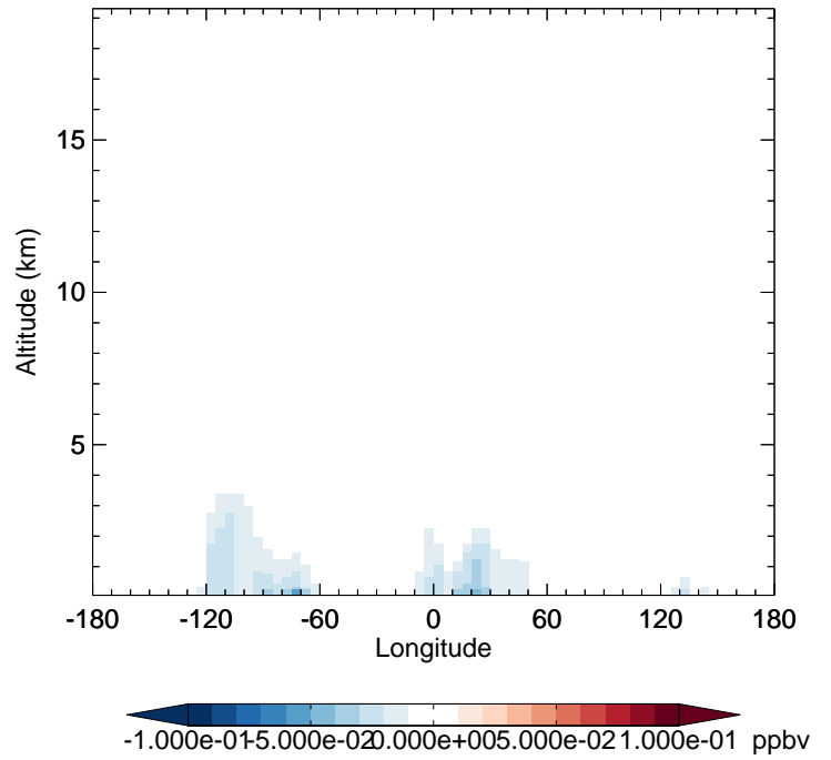
v11-02f-Run0 - v11-02e-Run0 MONITA - Diff along 42N for Jul
