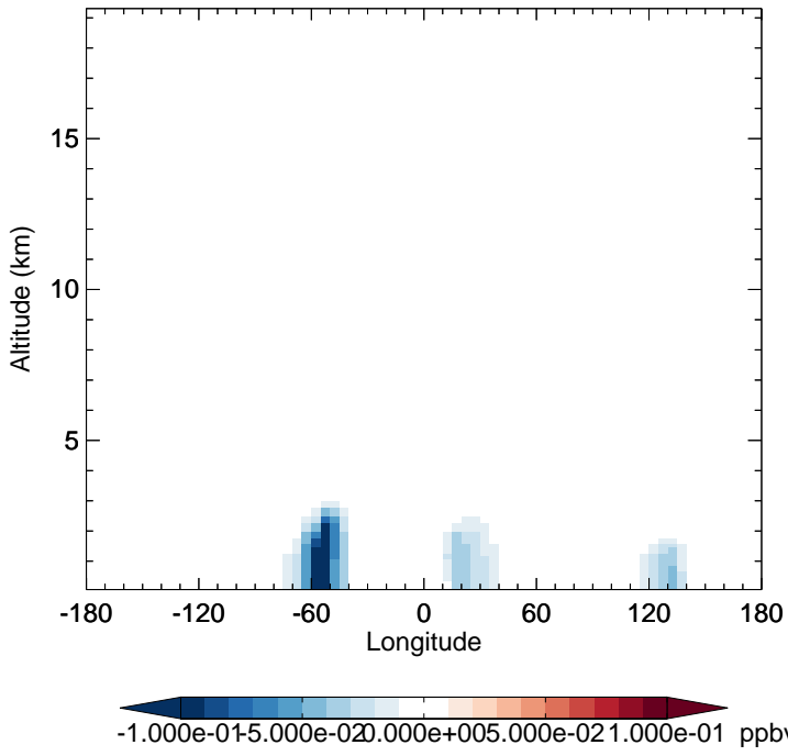
v11-02f-Run0 - v11-02e-Run1 IONITA - Diff along 15S for Jul
