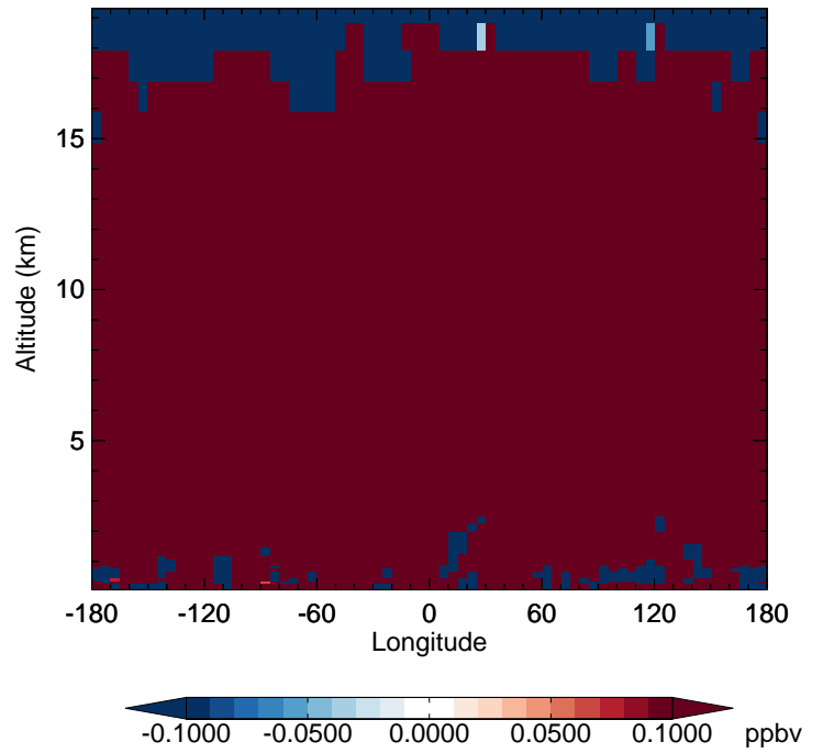
v11-02f-Run0 - v11-02e-Run0 CH4 - Diff along 42N for Jul
