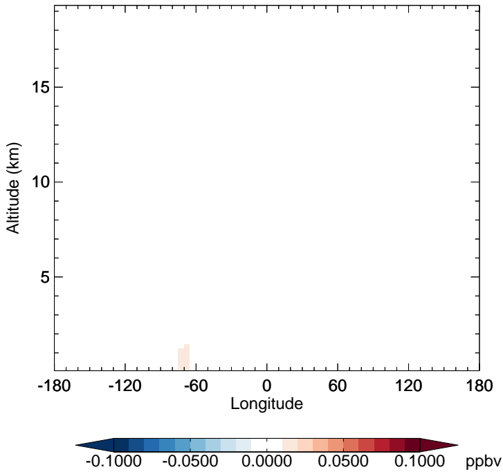
v11-02f-Run0 - v11-02e-Run1 SOAGX - Diff along 15S for Jul
