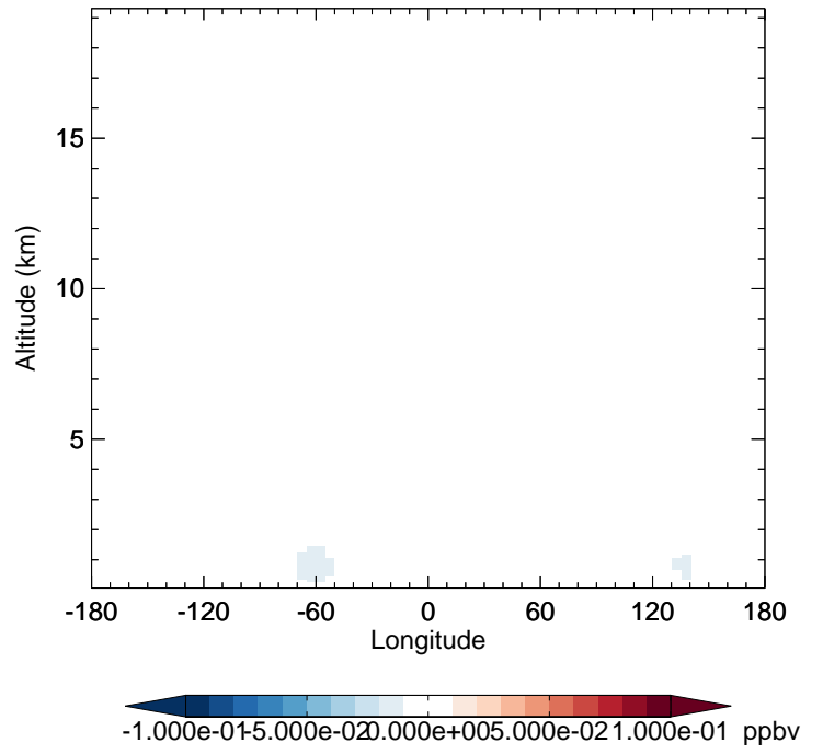
v11-02f-Run0 - v11-02e-Run1 SOAME - Diff along 42N for Jul
