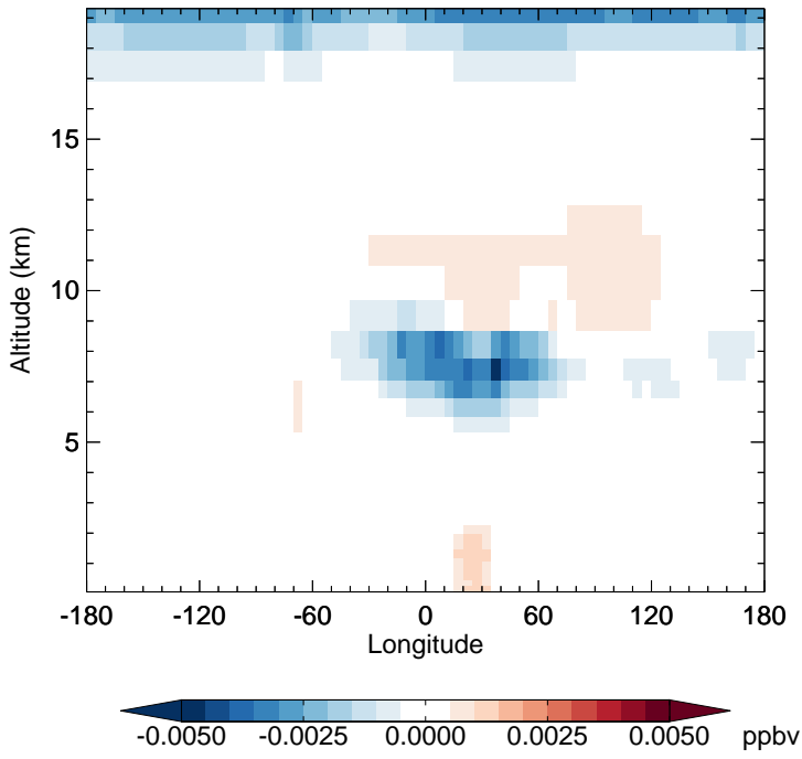
v11-02f-Run0 - v11-02e-Run1 HNO 4 - Diff along 15S for Jul
