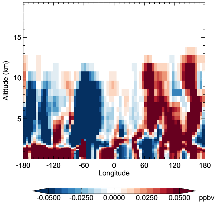
v11-02f-Run0 - v11-02e-Run0 MP - Diff along 15S for Jul
