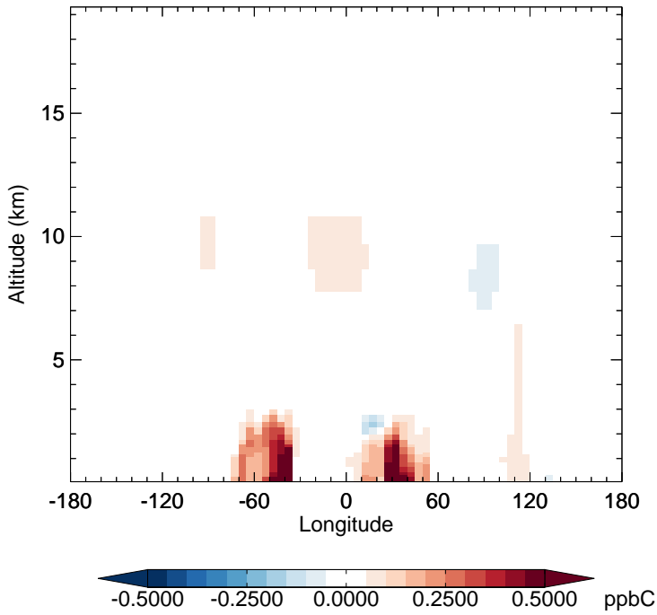
v11-02f-Run0 - v11-02e-Run0 ALK4 - Diff along 15S for Jul
