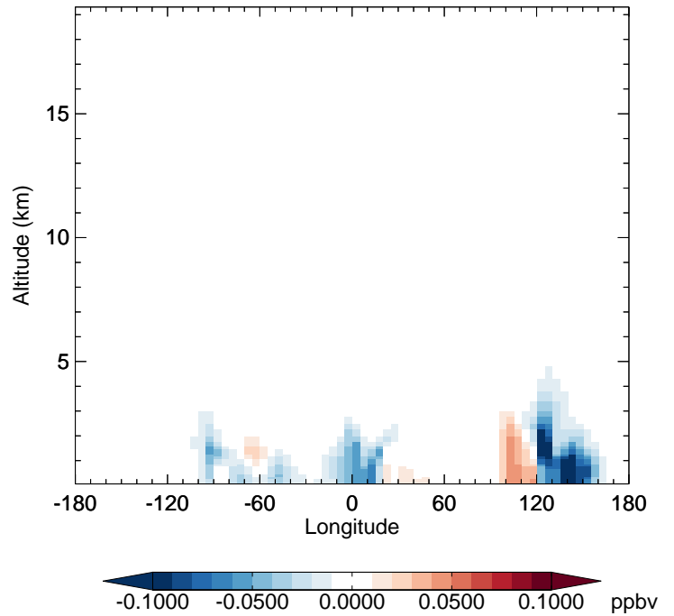
v11-02f-Run0 - v11-02e-Run0 SOAGX - Diff along 42N for Jul
