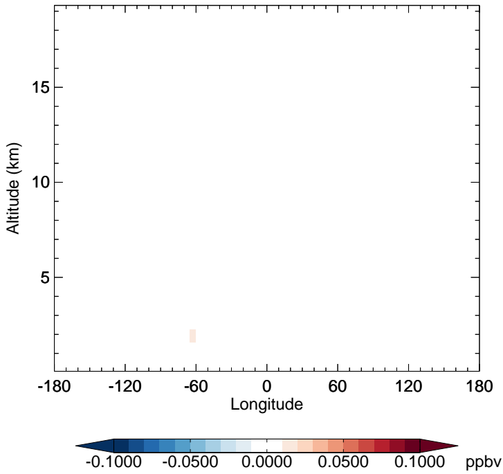
v11-02f-Run0 - v11-02e-Run0 RIPD - Diff along 15S for Jul
