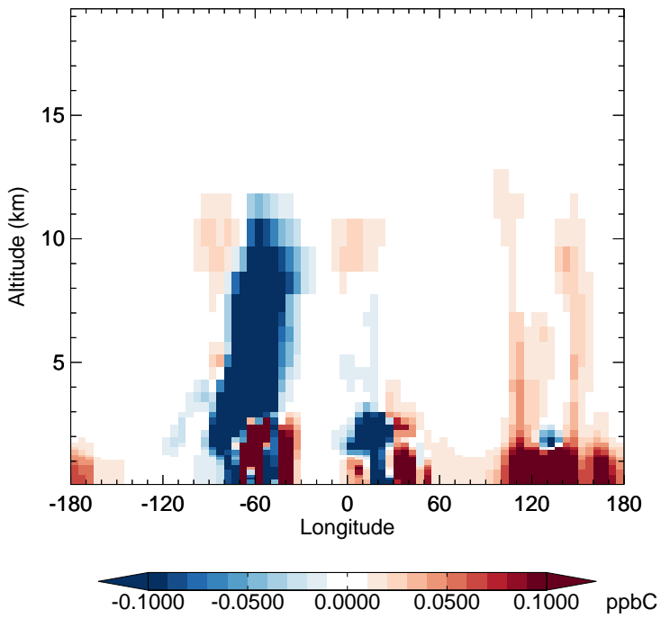
v11-02f-Run0 - v11-02e-Run0 MEK - Diff along 15S for Jul
