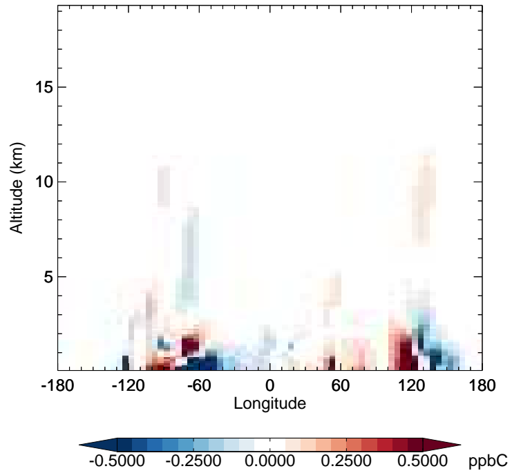
v11-02f-Run0 - v11-02e-Run0 ALK4 - Diff along 42N for Jul
