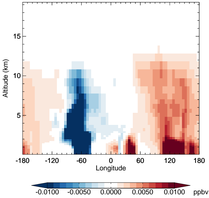
v11-02f-Run0 - v11-02e-Run1 MAP - Diff along 15S for Jul
