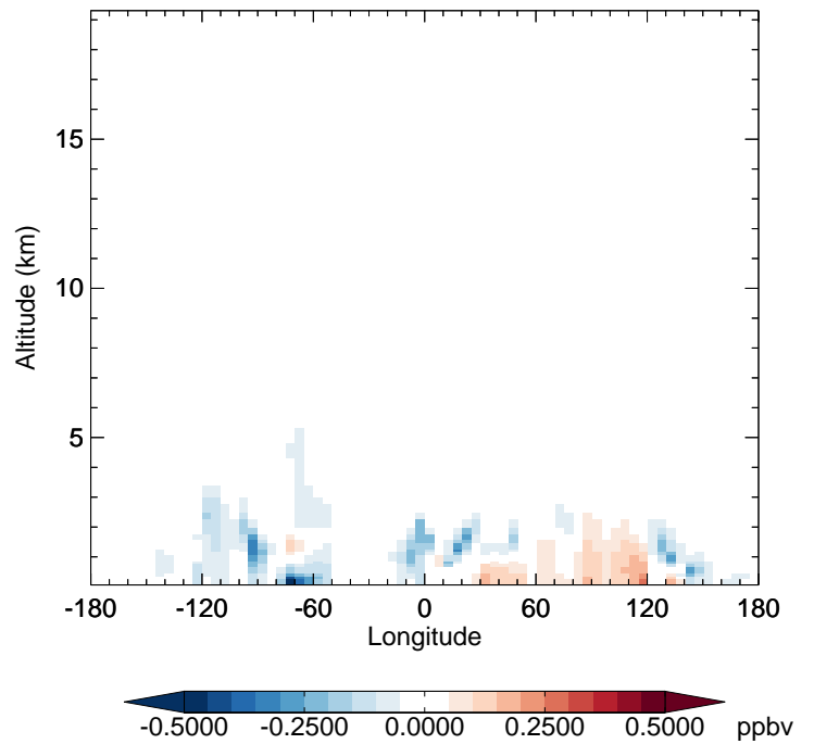
v11-02f-Run0 - v11-02e-Run0 CH 2 O - Diff along 42N for Jul
