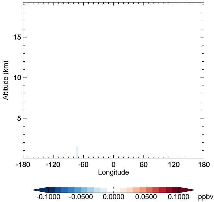
v11-02f-Run0 - v11-02e-Run0 SOAME - Diff along 15S for Jul
