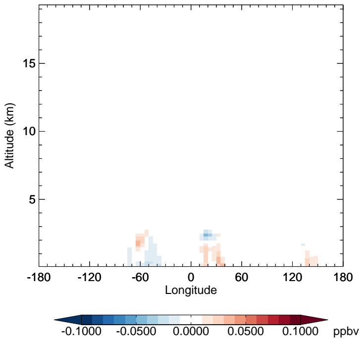
v11-02f-Run0 - v11-02e-Run0 SOAP - Diff along 15S for Jul
