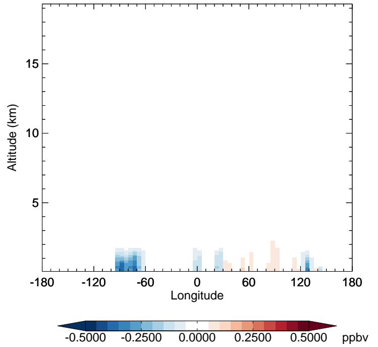
v11-02f-Run0 - v11-02e-Run1 CH 2 O - Diff along 42N for Jul
