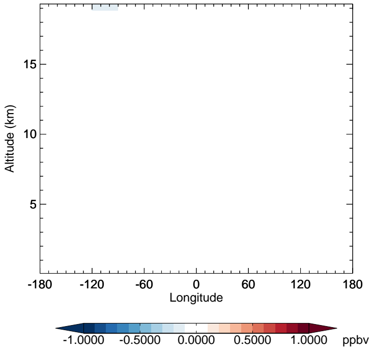
v11-02f-Run0 - v11-02e-Run0 NO - Diff along 15S for Jul
