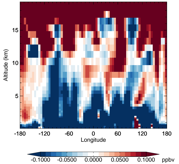
v11-02f-Run0 - v11-02e-Run0 HNO 3 - Diff along 42N for Jul
