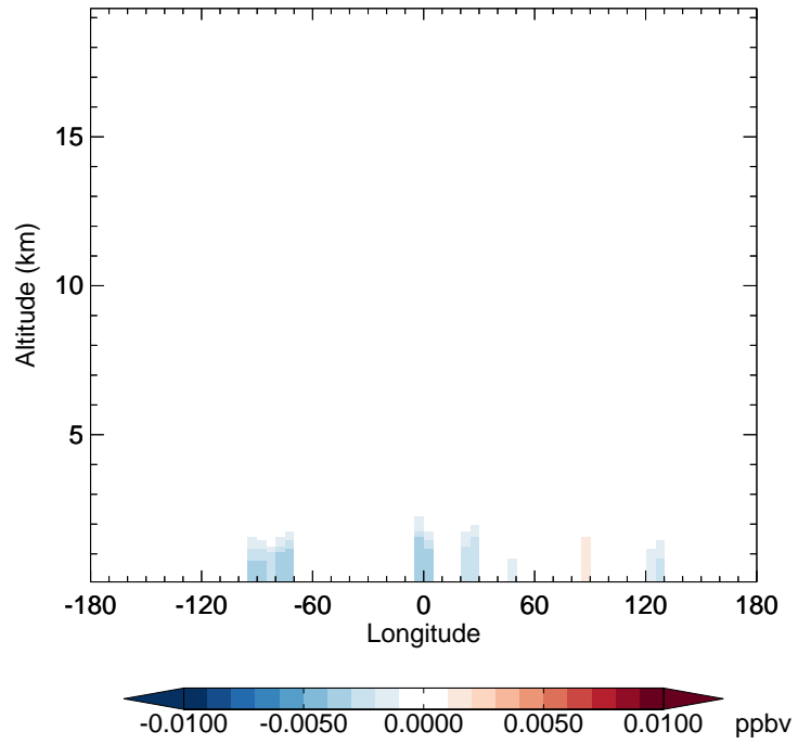
v11-02f-Run0 - v11-02e-Run1 MVKN - Diff along 42N for Jul
