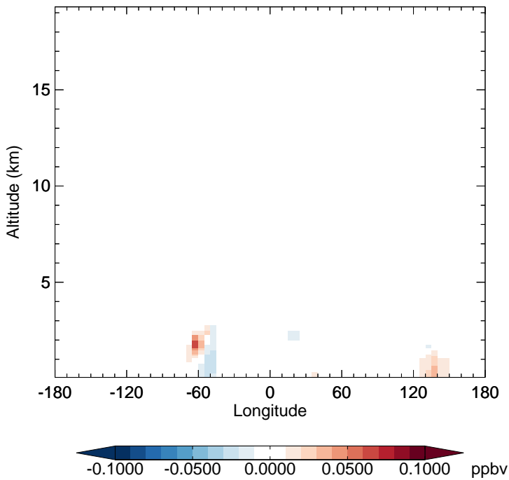
v11-02f-Run0 - v11-02e-Run0 MGLY - Diff along 15S for Jul
