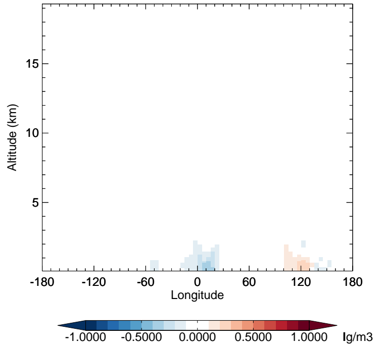
v11-02f-Run0 - v11-02e-Run0 BCPI - Diff along 42N for Jul
