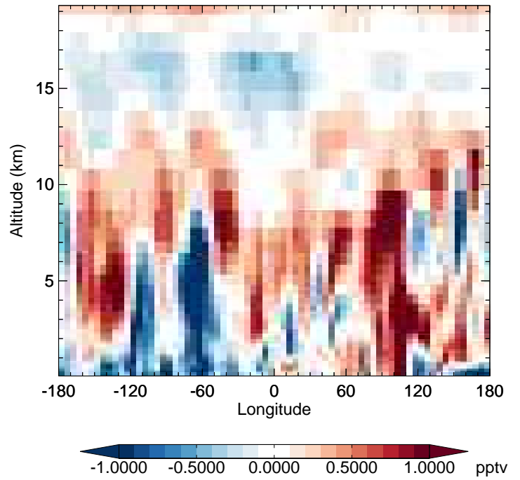
v11-02f-Run0 - v11-02e-Run0 HO2 - Diff along 42N for Jul
