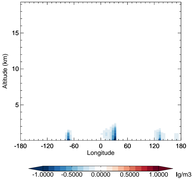
v11-02f-Run0 - v11-02e-Run1 SO 2 - Diff along 15S for Jul
