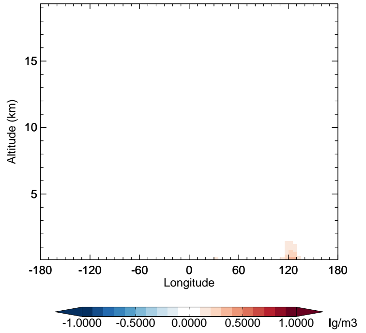
v11-02f-Run0 - v11-02e-Run1 OCPO - Diff along 42N for Jul
