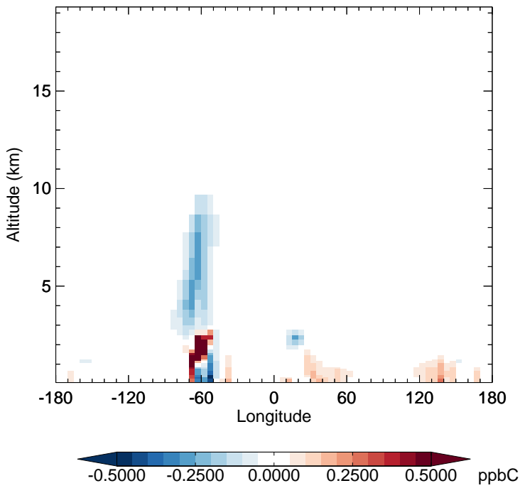
v11-02f-Run0 - v11-02e-Run0 ALD2 - Diff along 15S for Jul
