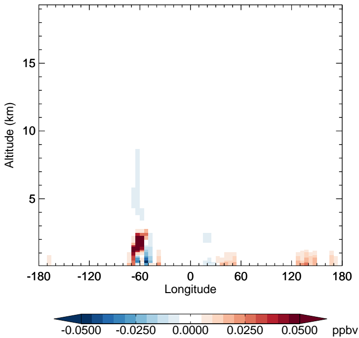
v11-02f-Run0 - v11-02e-Run0 RCHO - Diff along 15S for Jul
