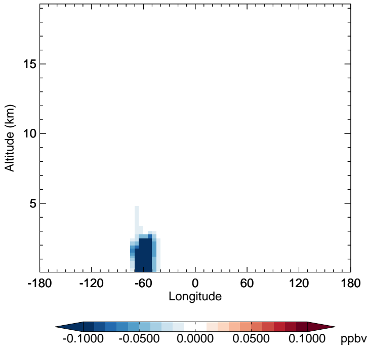
v11-02f-Run0 - v11-02e-Run1 RIPA - Diff along 15S for Jul
