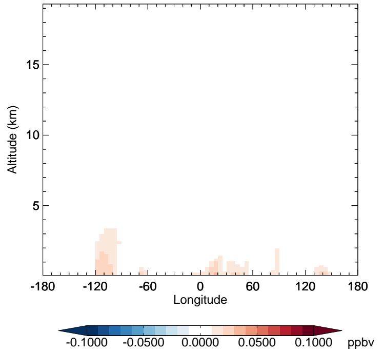
v11-02f-Run0 - v11-02e-Run1 TSOG2 - Diff along 42N for Jul
