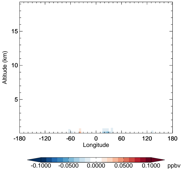
v11-02f-Run0 - v11-02e-Run0 XYLE - Diff along 15S for Jul
