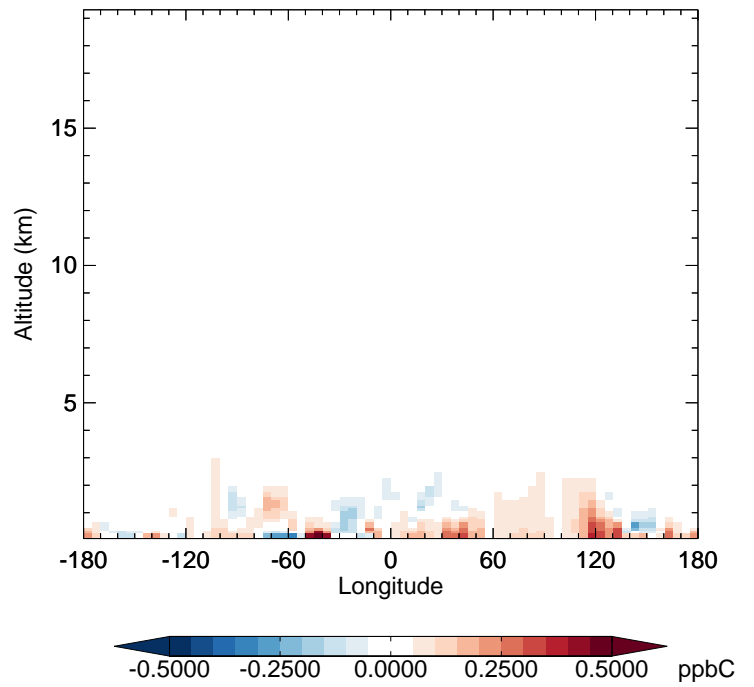
v11-02f-Run0 - v11-02e-Run0 ALD2 - Diff along 42N for Jul
