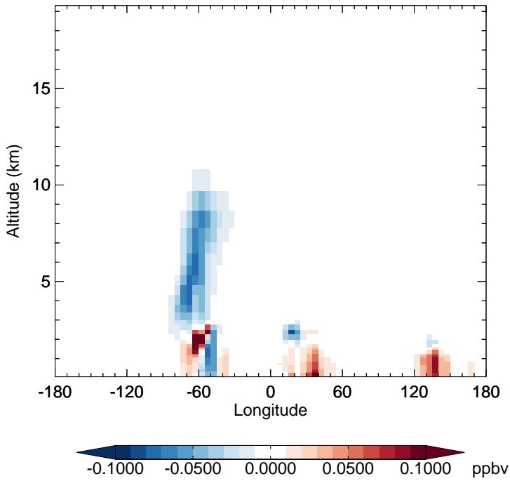
v11-02f-Run0 - v11-02e-Run0 HAC - Diff along 15S for Jul
