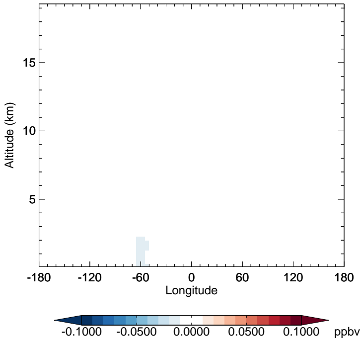
v11-02f-Run0 - v11-02e-Run1 TSOA0 - Diff along 15S for Jul
