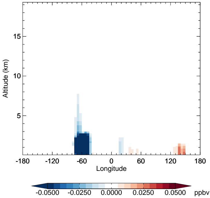
v11-02f-Run0 - v11-02e-Run1 MACR - Diff along 15S for Jul
