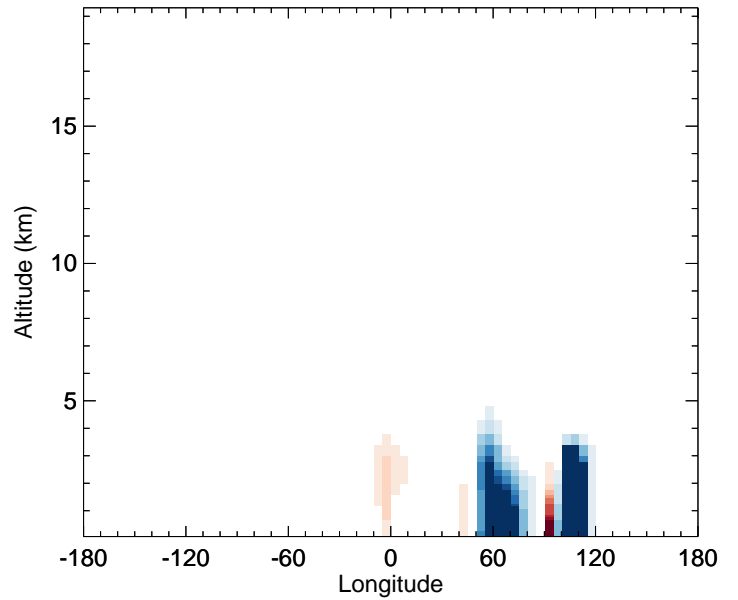
v11-02f-Run0 - v11-02e-Run0 DST4 - Diff along 42N for Jul
