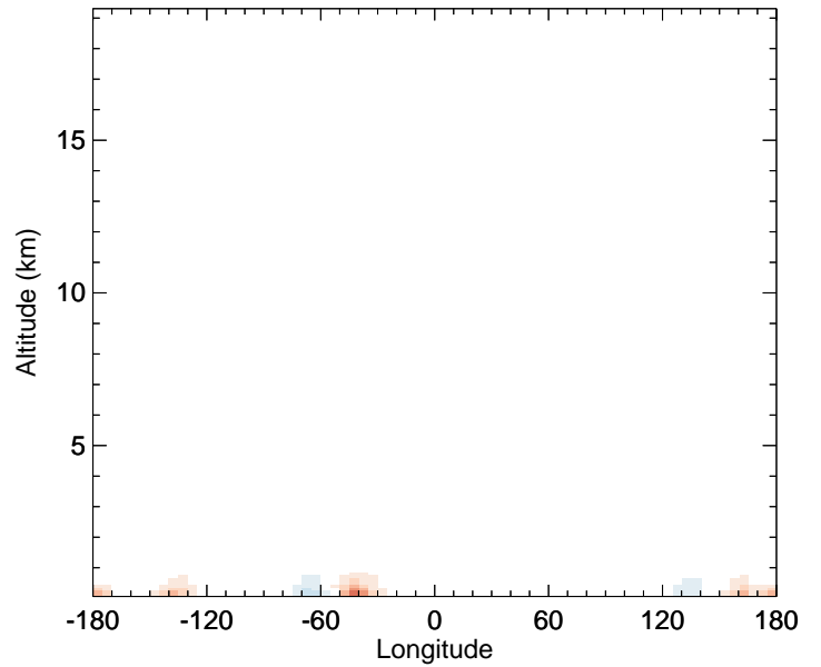
v11-02f-Run0 - v11-02e-Run0 SALA - Diff along 42N for Jul
