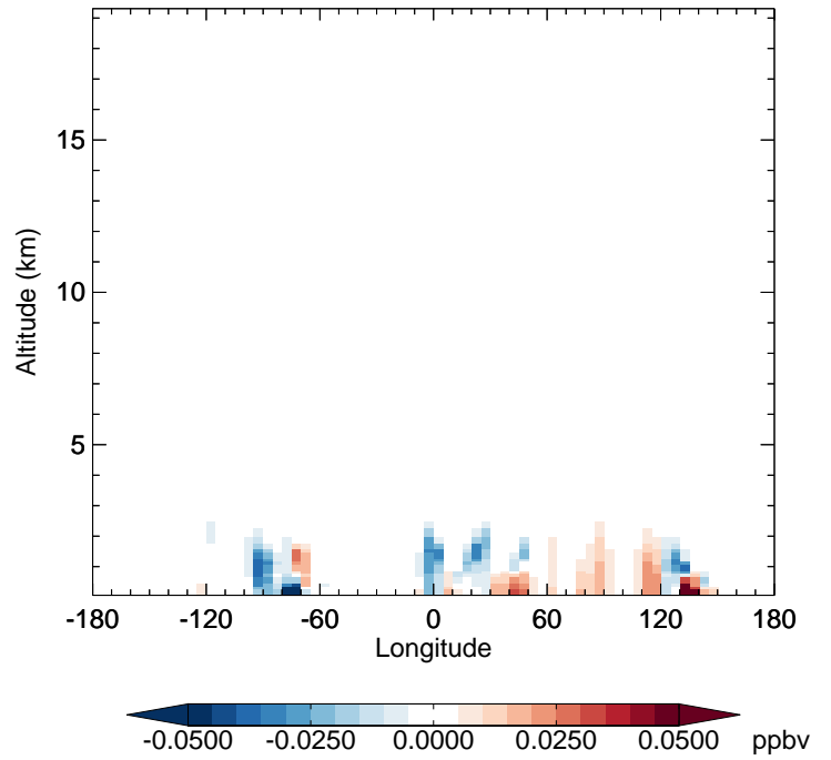
v11-02f-Run0 - v11-02e-Run0 MVK - Diff along 42N for Jul
