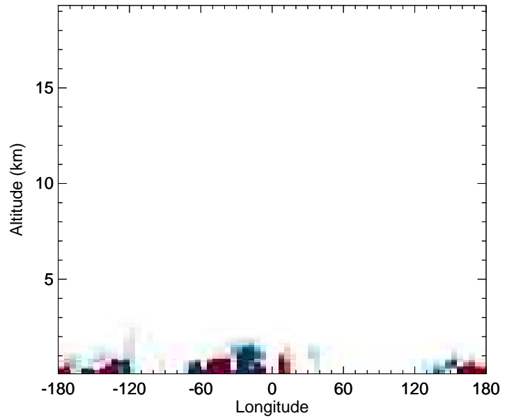
v11-02f-Run0 - v11-02e-Run0 SALC - Diff along 42N for Jul
