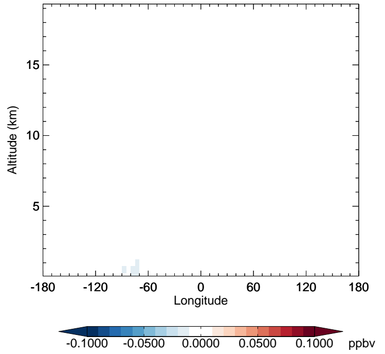
v11-02f-Run0 - v11-02e-Run1 RIPA - Diff along 42N for Jul
