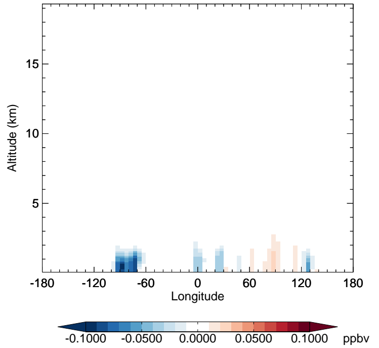
v11-02f-Run0 - v11-02e-Run1 GLYC - Diff along 42N for Jul
