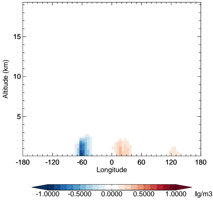
v11-02f-Run0 - v11-02e-Run1 SOAS - Diff along 15S for Jul
