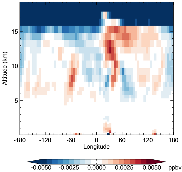
v11-02f-Run0 - v11-02e-Run0 N2O5 - Diff along 15S for Jul
