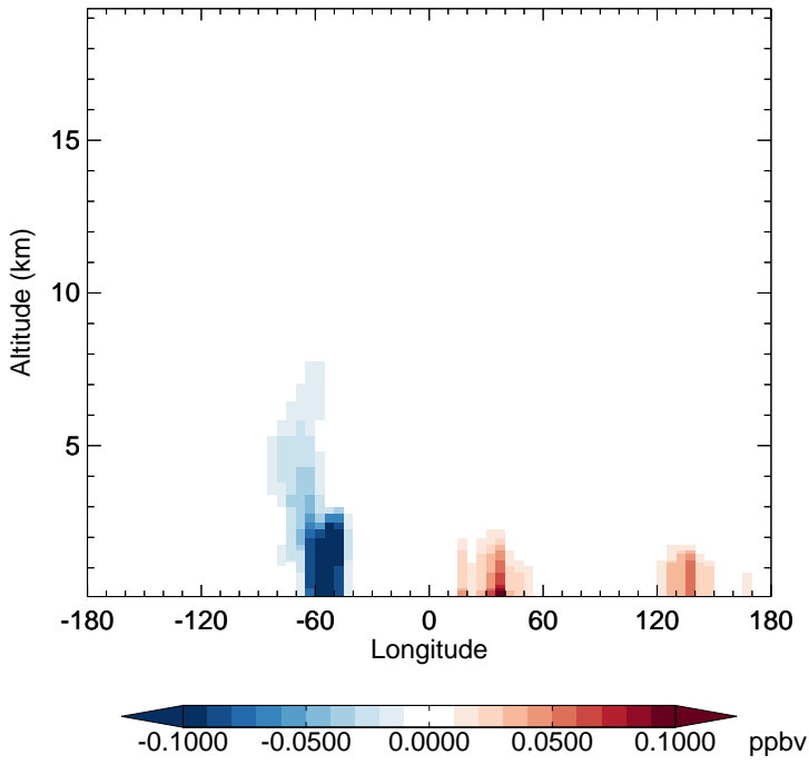
v11-02f-Run0 - v11-02e-Run1 HAC - Diff along 15S for Jul
