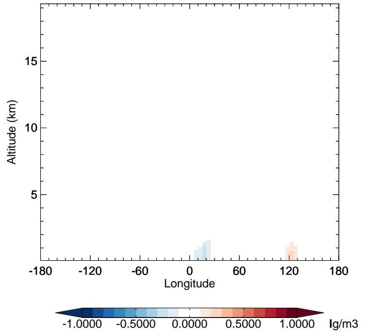
v11-02f-Run0 - v11-02e-Run1 BCPI - Diff along 42N for Jul
