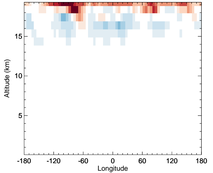
v11-02f-Run0 - v11-02e-Run0 ClNO 3 - Diff along 42N for Jul
