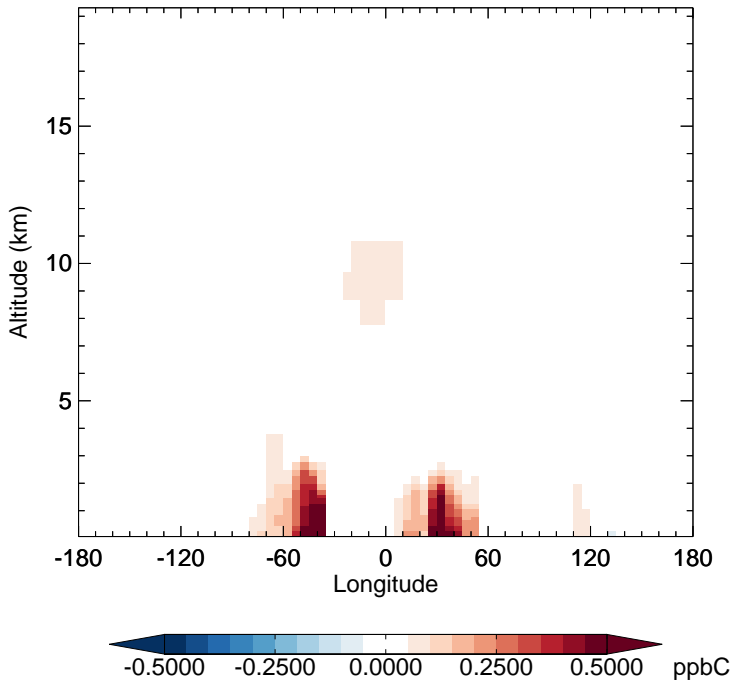
v11-02f-Run0 - v11-02e-Run1 ALK4 - Diff along 15S for Jul
