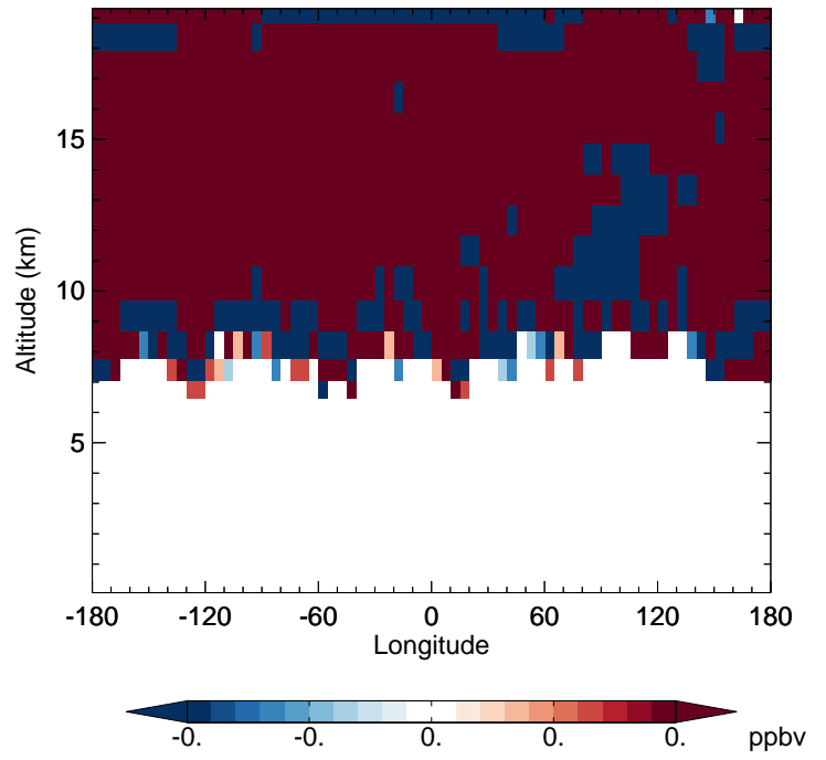
v11-02f-Run0 - v11-02e-Run1 H2O - Diff along 42N for Jul
