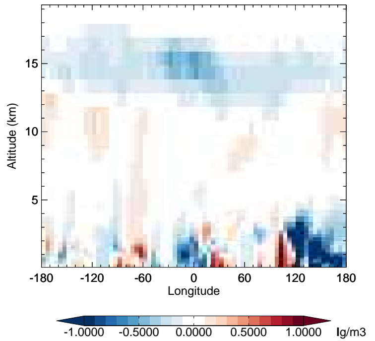
v11-02f-Run0 - v11-02e-Run0 SO4 - Diff along 42N for Jul
