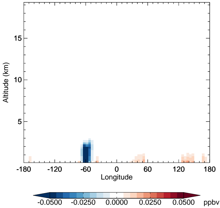
v11-02f-Run0 - v11-02e-Run1 RCHO - Diff along 15S for Jul
