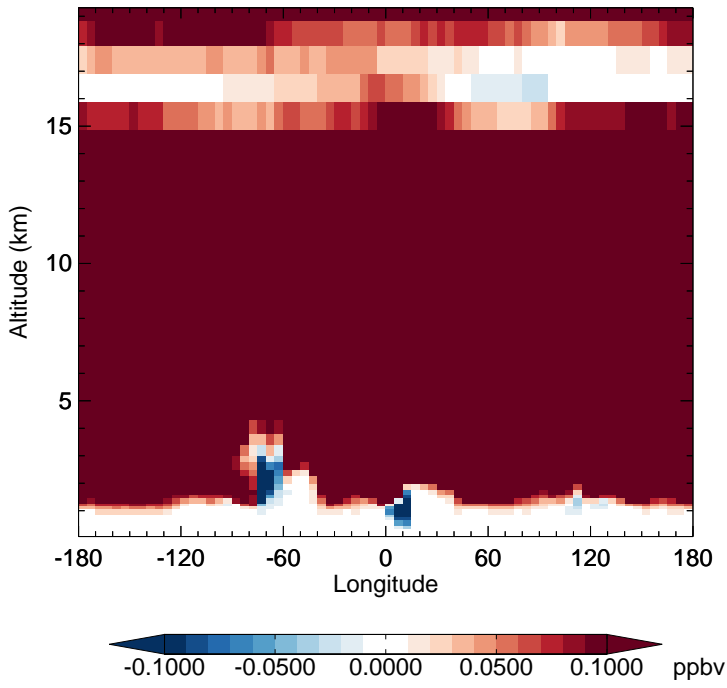
v11-02f-Run0 - v11-02e-Run1 CH4 - Diff along 15S for Jul
