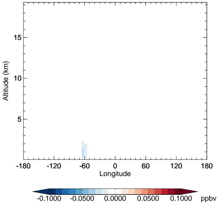
v11-02f-Run0 - v11-02e-Run1 RIPD - Diff along 15S for Jul
