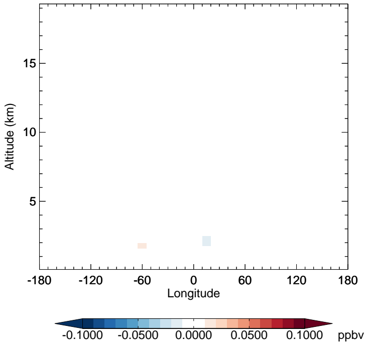
v11-02f-Run0 - v11-02e-Run0 ISOA3 - Diff along 15S for Jul
