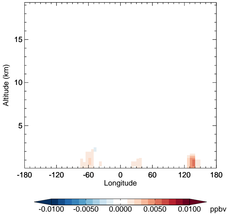
v11-02f-Run0 - v11-02e-Run1 MVKN - Diff along 15S for Jul
