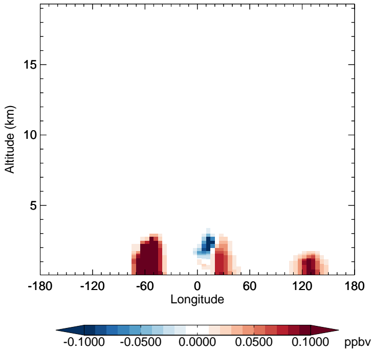
v11-02f-Run0 - v11-02e-Run0 INDIOL - Diff along 15S for Jul
