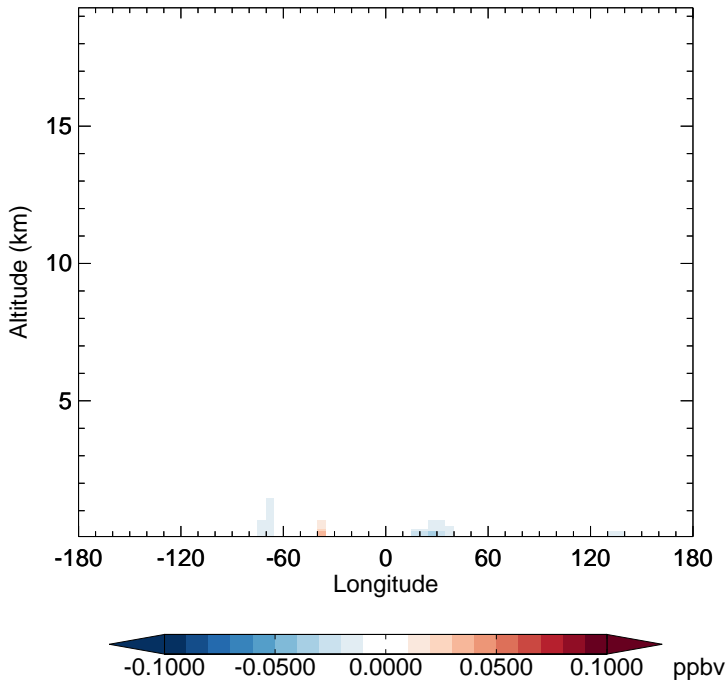
v11-02f-Run0 - v11-02e-Run1 XYLE - Diff along 15S for Jul
