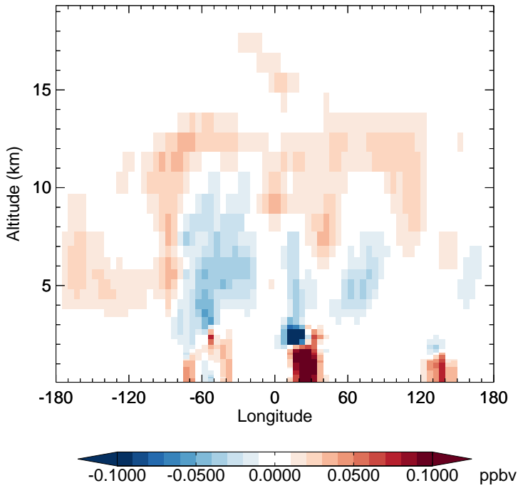
v11-02f-Run0 - v11-02e-Run0 PAN - Diff along 15S for Jul
