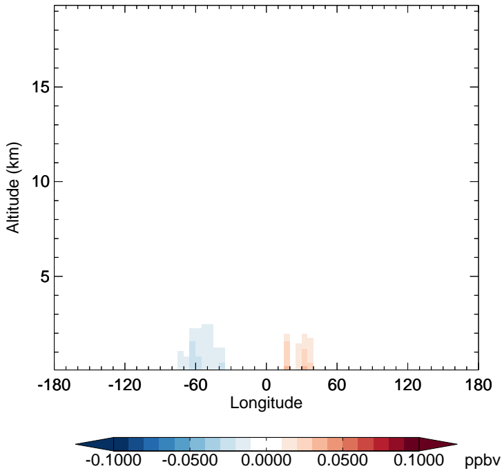
v11-02f-Run0 - v11-02e-Run1 SOAP - Diff along 15S for Jul
