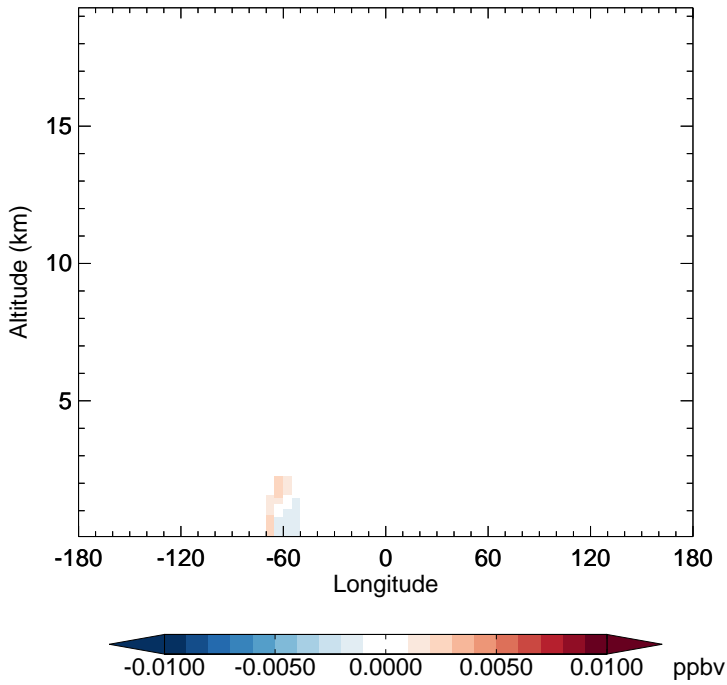
v11-02f-Run0 - v11-02e-Run0 MOBA - Diff along 15S for Jul
