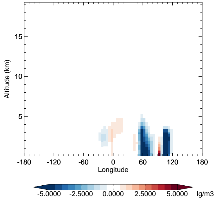
v11-02f-Run0 - v11-02e-Run0 DST2 - Diff along 42N for Jul
