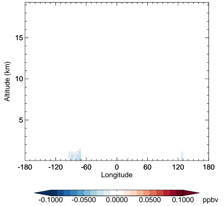
v11-02f-Run0 - v11-02e-Run1 IPMN - Diff along 42N for Jul
