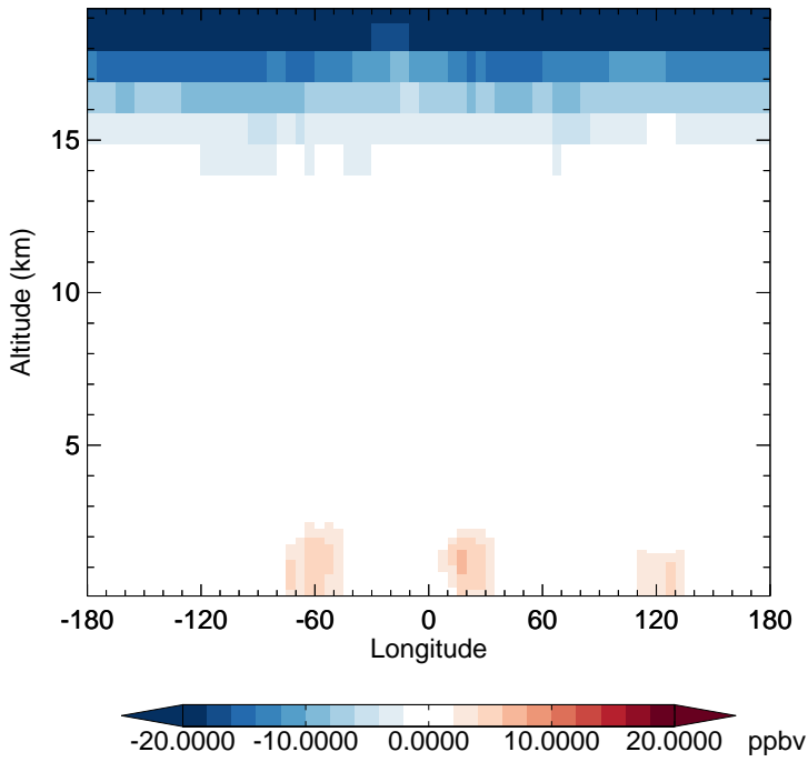
v11-02f-Run0 - v11-02e-Run1 O3 - Diff along 15S for Jul
