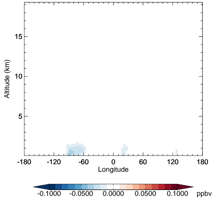
v11-02f-Run0 - v11-02e-Run1 ISOA1 - Diff along 42N for Jul
