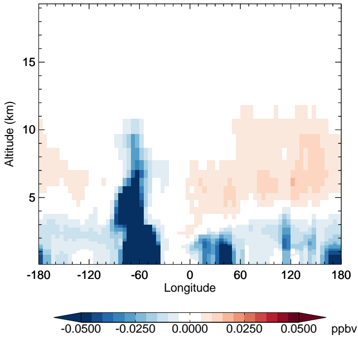
v11-02f-Run0 - v11-02e-Run1 MP - Diff along 15S for Jul
