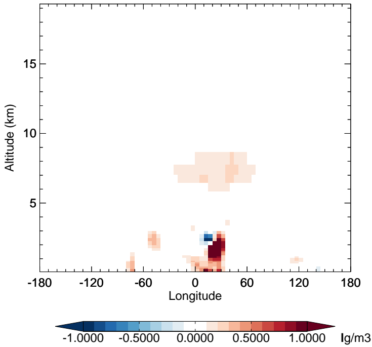
v11-02f-Run0 - v11-02e-Run0 NIT - Diff along 15S for Jul
