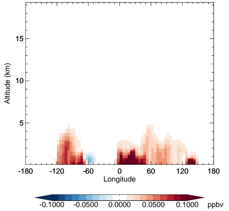
v11-02f-Run0 - v11-02e-Run1 INDIOL - Diff along 42N for Jul
