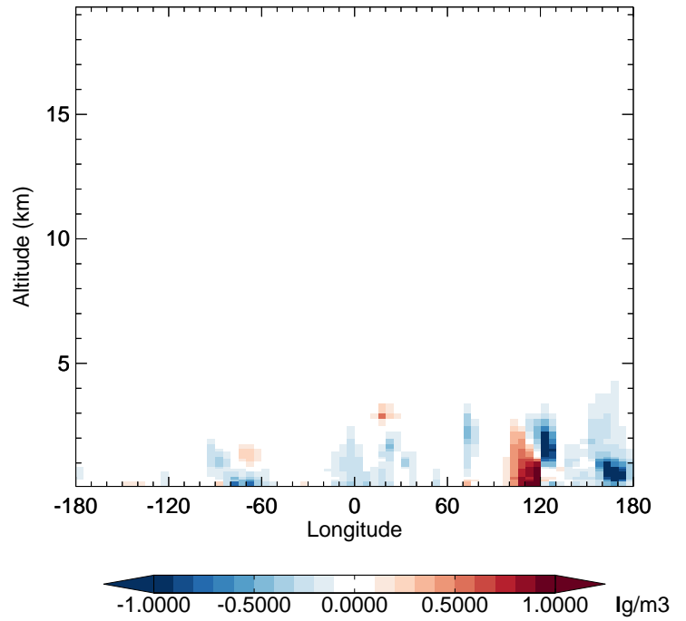
v11-02f-Run0 - v11-02e-Run0 SO 2 - Diff along 42N for Jul
