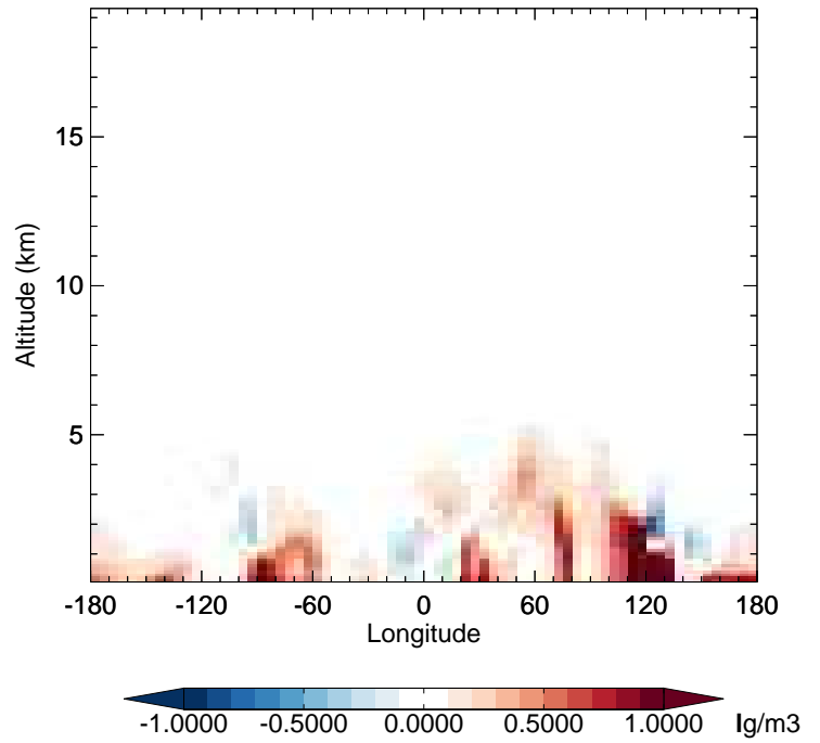
v11-02f-Run0 - v11-02e-Run0 NH4 - Diff along 42N for Jul
