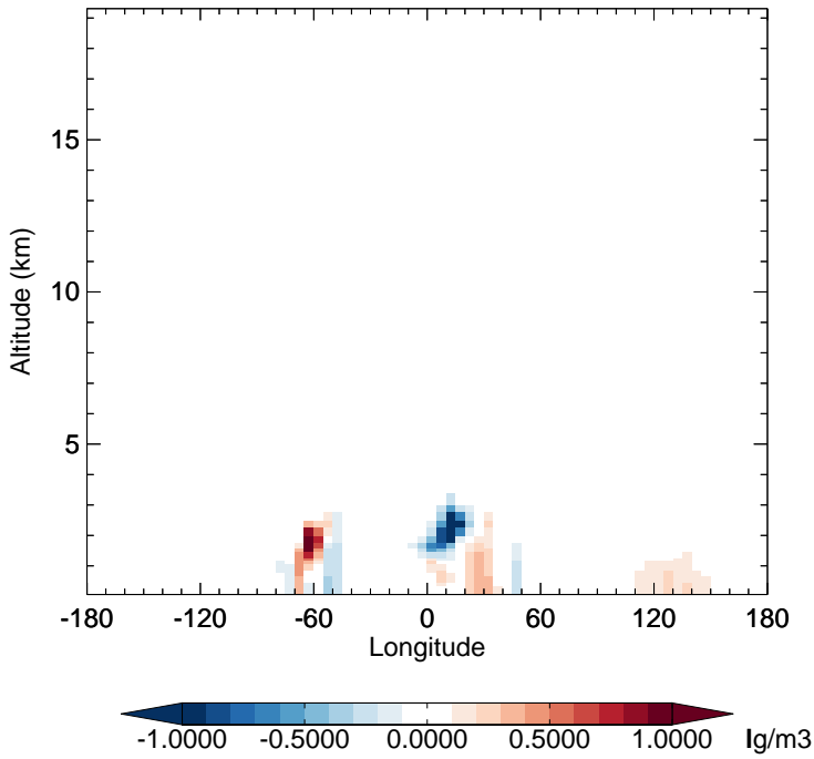
v11-02f-Run0 - v11-02e-Run0 SOAS - Diff along 15S for Jul
