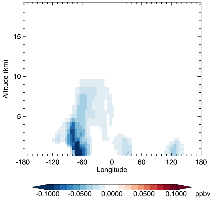
v11-02f-Run0 - v11-02e-Run0 SOAIE - Diff along 15S for Jul
