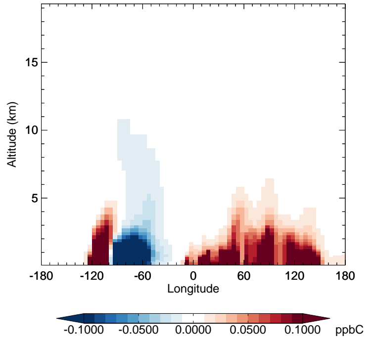
v11-02f-Run0 - v11-02e-Run1 MEK - Diff along 42N for Jul
