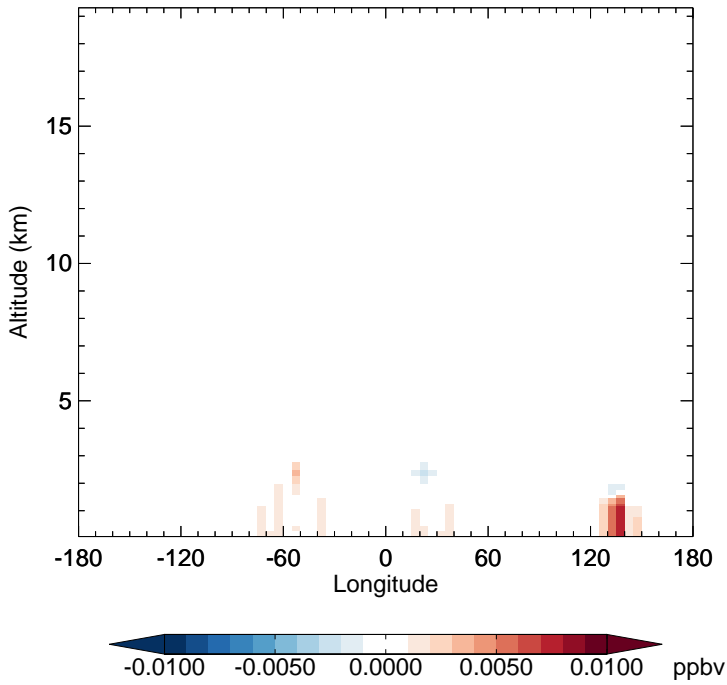
v11-02f-Run0 - v11-02e-Run0 MVKN - Diff along 15S for Jul
