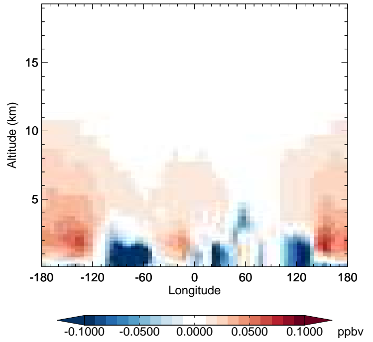
v11-02f-Run0 - v11-02e-Run1 H2O2 - Diff along 42N for Jul
