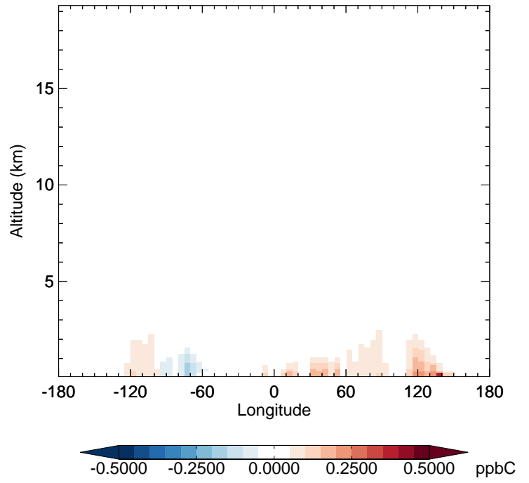
v11-02f-Run0 - v11-02e-Run1 ALD2 - Diff along 42N for Jul
