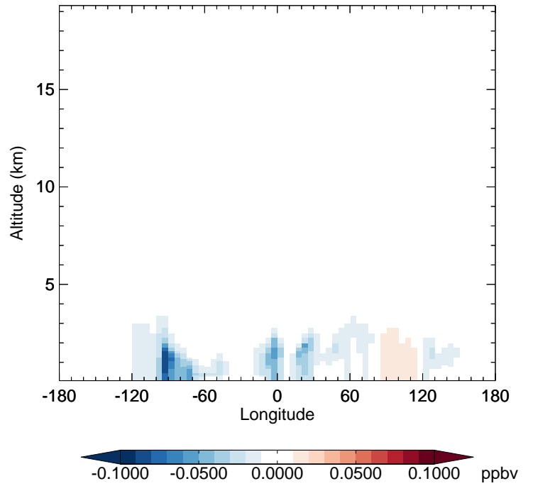
v11-02f-Run0 - v11-02e-Run0 ISO3 - Diff along 42N for Jul
