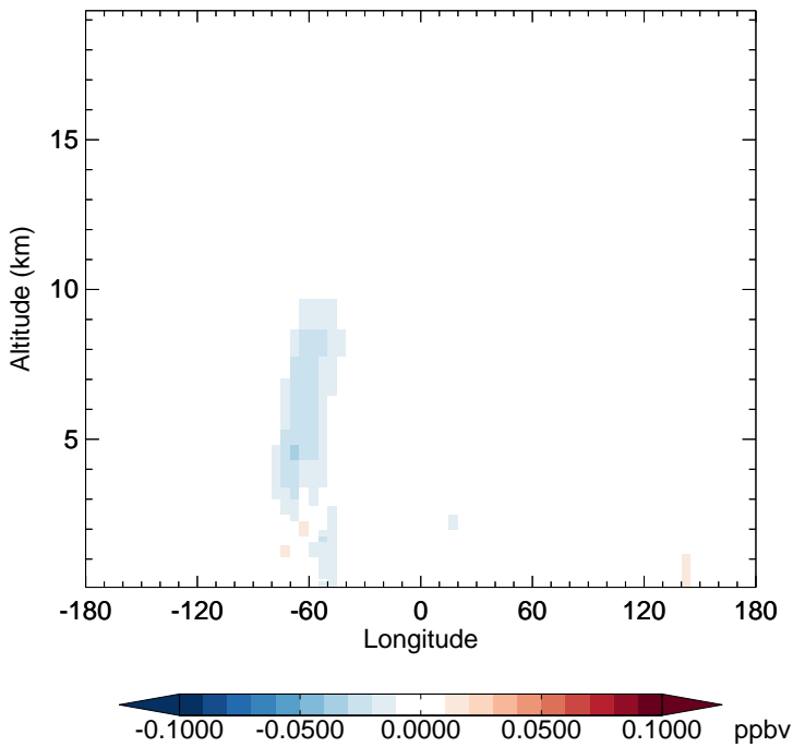
v11-02f-Run0 - v11-02e-Run0 HC187 - Diff along 15S for Jul
