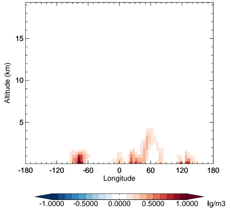
v11-02f-Run0 - v11-02e-Run1 SO4 - Diff along 42N for Jul
