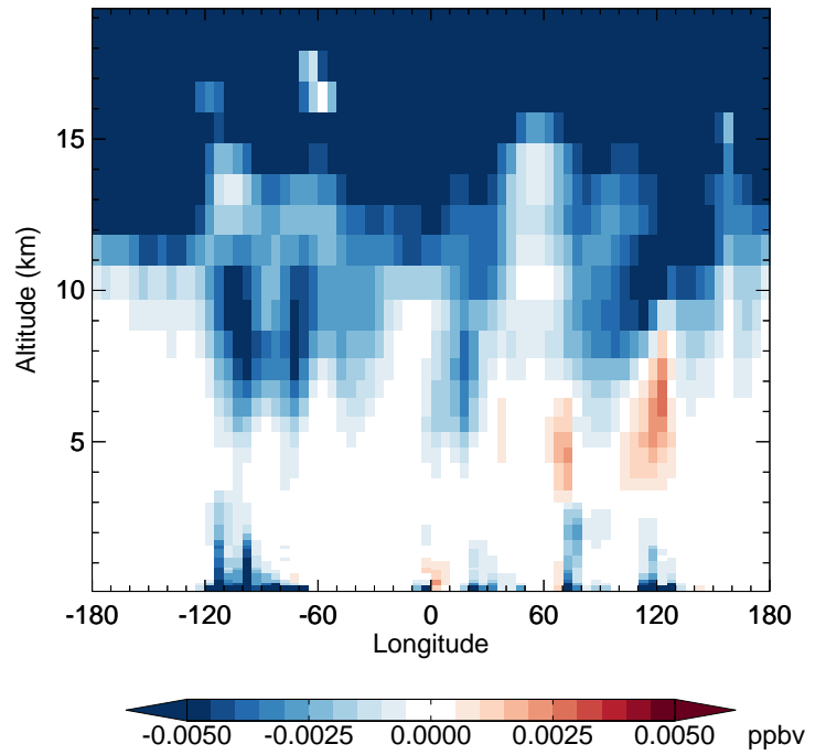
v11-02f-Run0 - v11-02e-Run0 N2O5 - Diff along 42N for Jul
