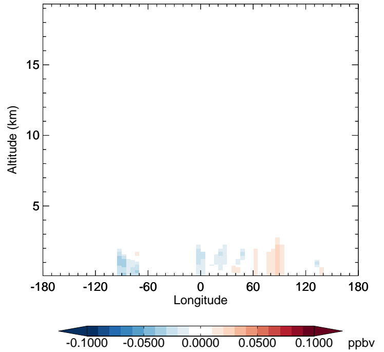
v11-02f-Run0 - v11-02e-Run0 IEPOXA - Diff along 42N for Jul
