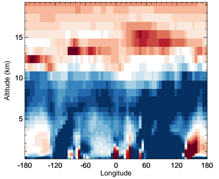
v11-02f-Run0 - v11-02e-Run1 OH - Diff along 42N for Jul
