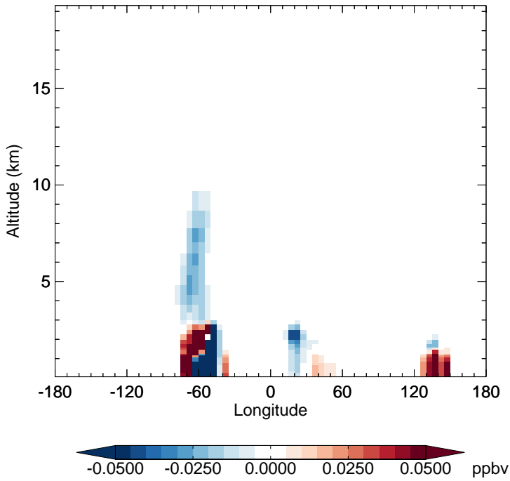
v11-02f-Run0 - v11-02e-Run0 MVK - Diff along 15S for Jul
