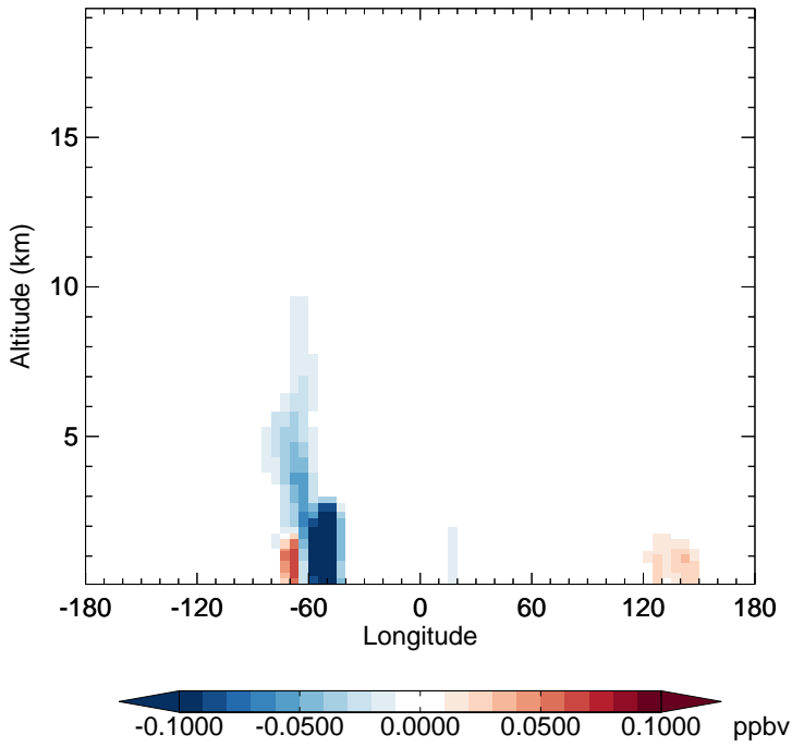
v11-02f-Run0 - v11-02e-Run1 IEPOXA - Diff along 15S for Jul
