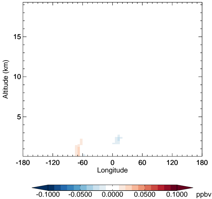
v11-02f-Run0 - v11-02e-Run0 SOAGX - Diff along 15S for Jul
