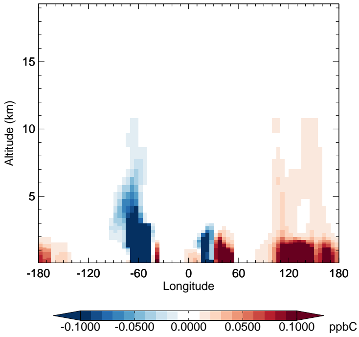
v11-02f-Run0 - v11-02e-Run1 MEK - Diff along 15S for Jul
