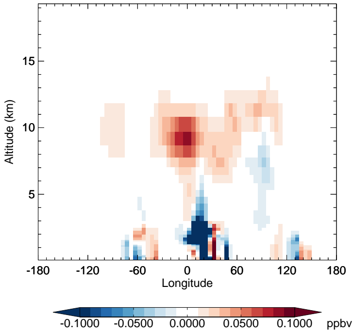
v11-02f-Run0 - v11-02e-Run0 BENZ - Diff along 15S for Jul
