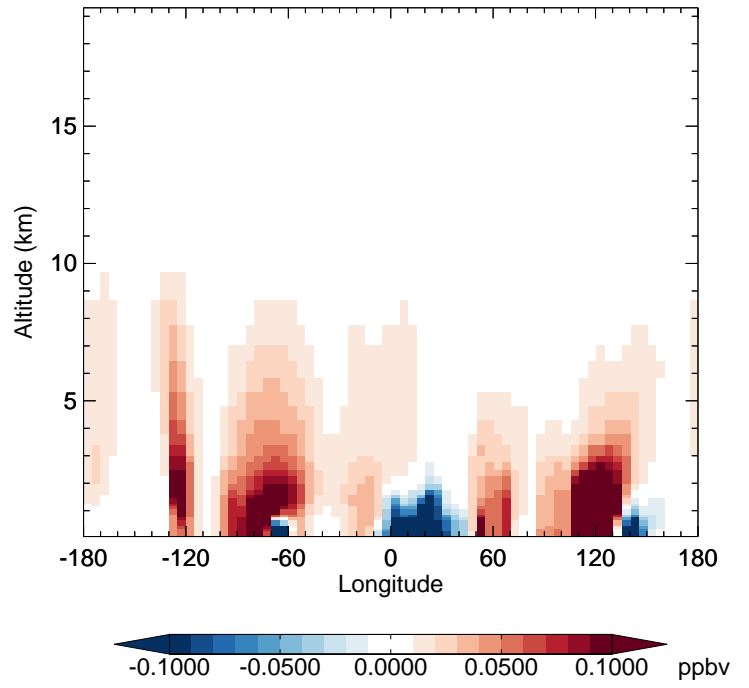
v11-02f-Run0 - v11-02e-Run1 BENZ - Diff along 42N for Jul
