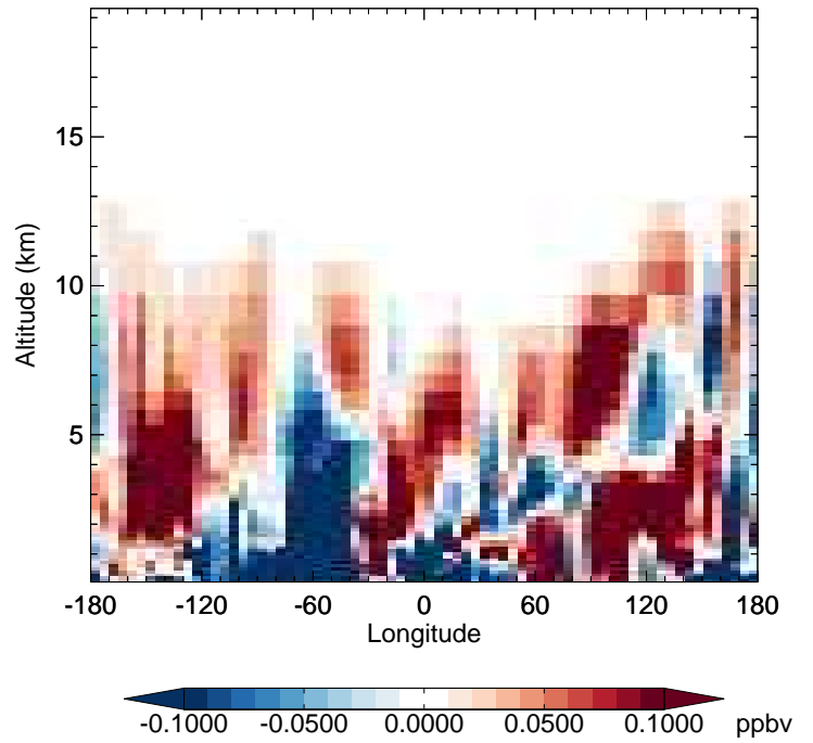
v11-02f-Run0 - v11-02e-Run0 H2O2 - Diff along 42N for Jul
