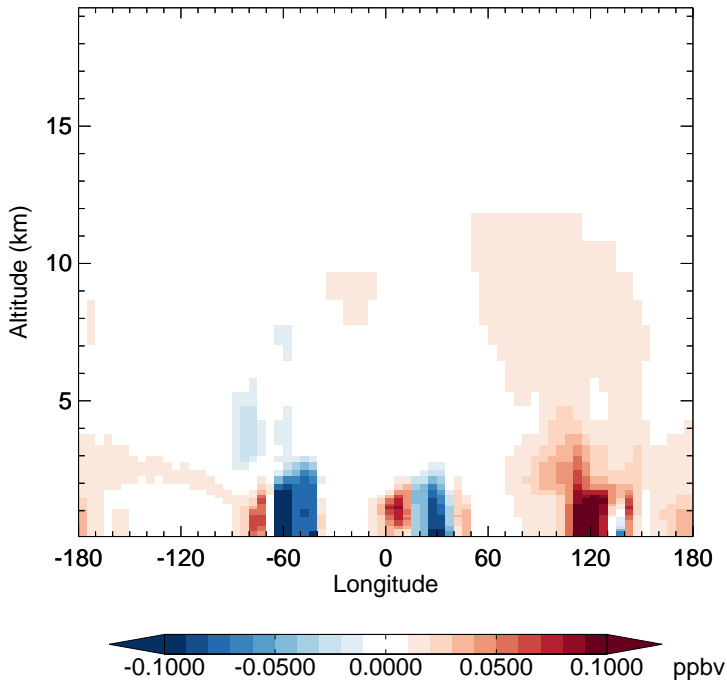
v11-02f-Run0 - v11-02e-Run1 H2O2 - Diff along 15S for Jul
