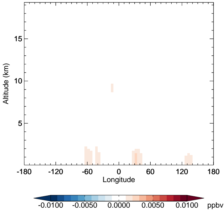
v11-02f-Run0 - v11-02e-Run1 R4N2 - Diff along 15S for Jul
