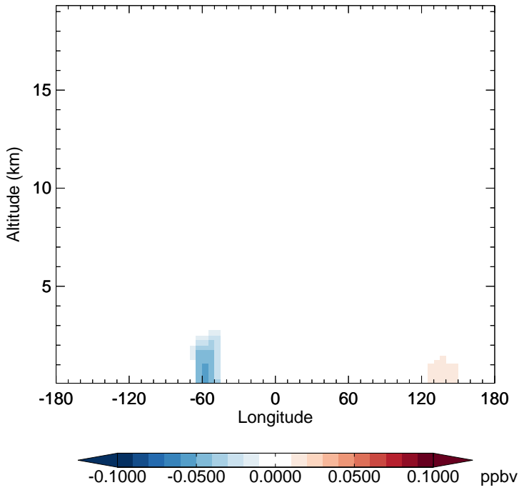
v11-02f-Run0 - v11-02e-Run1 MGLY - Diff along 15S for Jul
