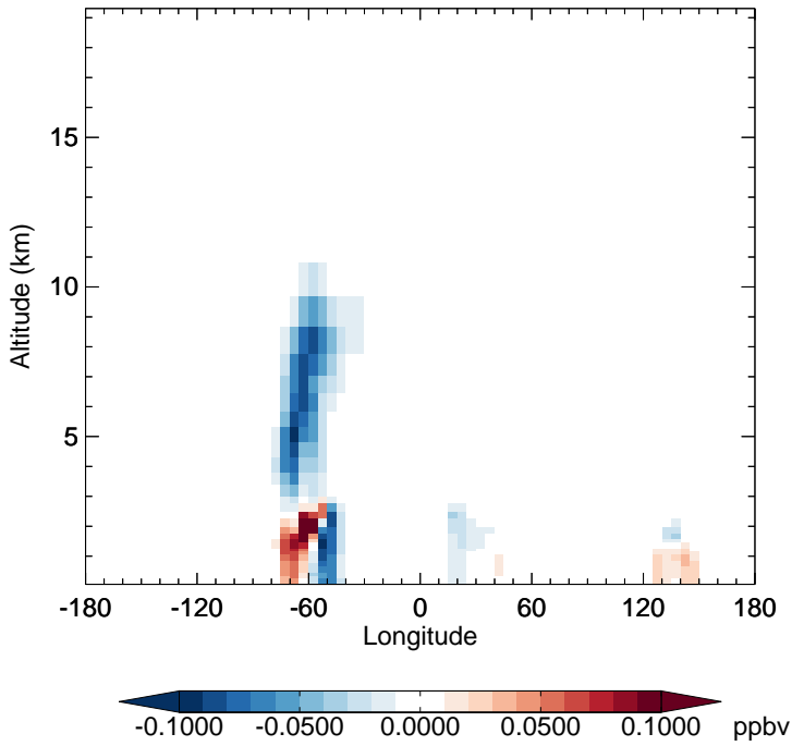
v11-02f-Run0 - v11-02e-Run0 IEPOXA - Diff along 15S for Jul
