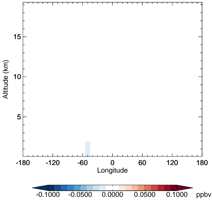
v11-02f-Run0 - v11-02e-Run1 GLYX - Diff along 15S for Jul
