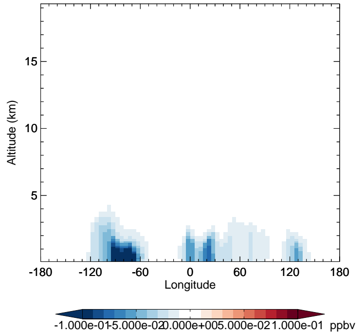
v11-02f-Run0 - v11-02e-Run0 IONITA - Diff along 42N for Jul
