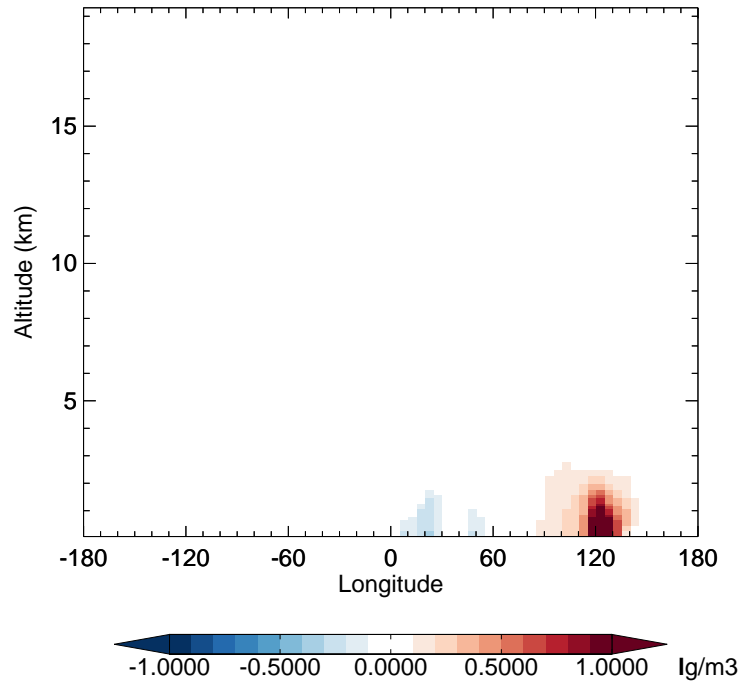
v11-02f-Run0 - v11-02e-Run1 OCPI - Diff along 42N for Jul
