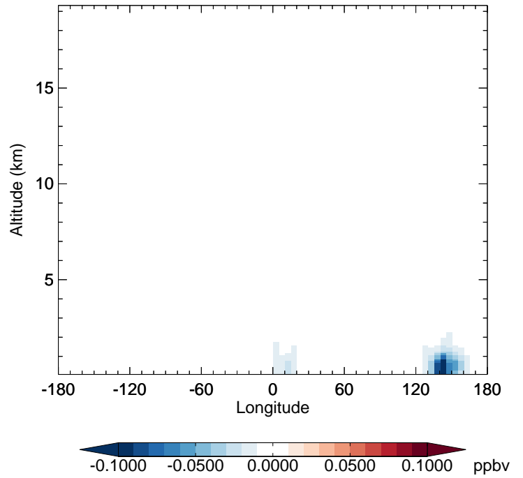
v11-02f-Run0 - v11-02e-Run0 ASOAN - Diff along 42N for Jul
