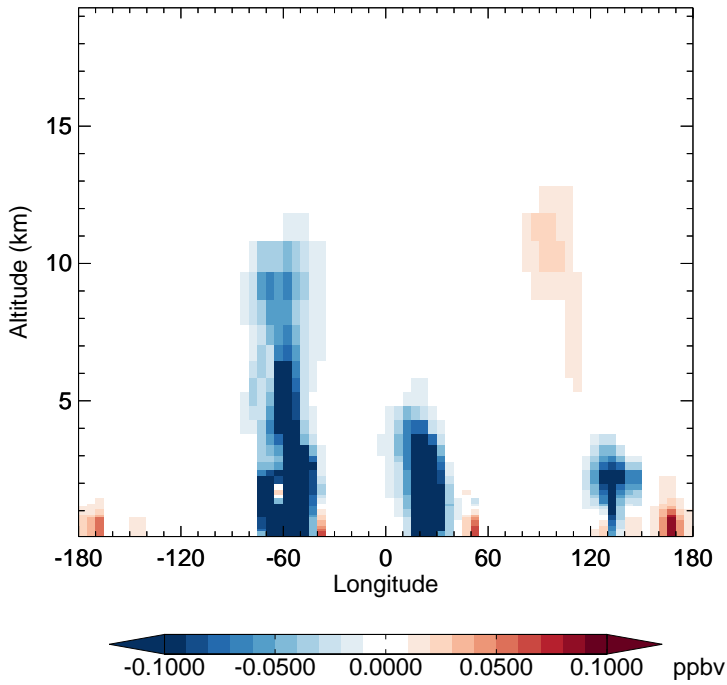
v11-02f-Run0 - v11-02e-Run0 EOH - Diff along 15S for Oct
