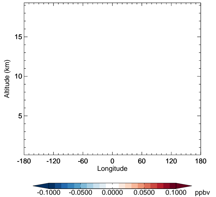
v11-02f-Run0 - v11-02e-Run0 TSOA3 - Diff along 42N for Oct
