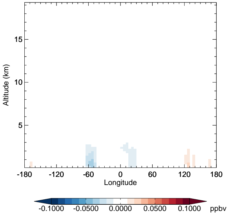
v11-02f-Run0 - v11-02e-Run1 TSOG2 - Diff along 15S for Oct
