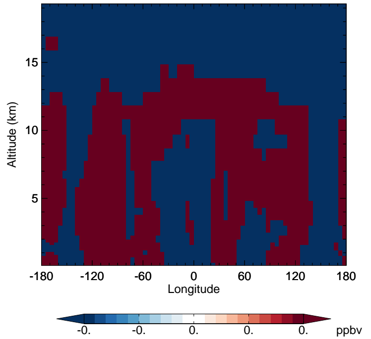
v11-02f-Run0 - v11-02e-Run0 H2O - Diff along 42N for Oct
