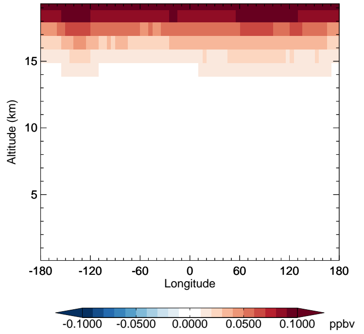
v11-02f-Run0 - v11-02e-Run1 N2O - Diff along 42N for Oct
