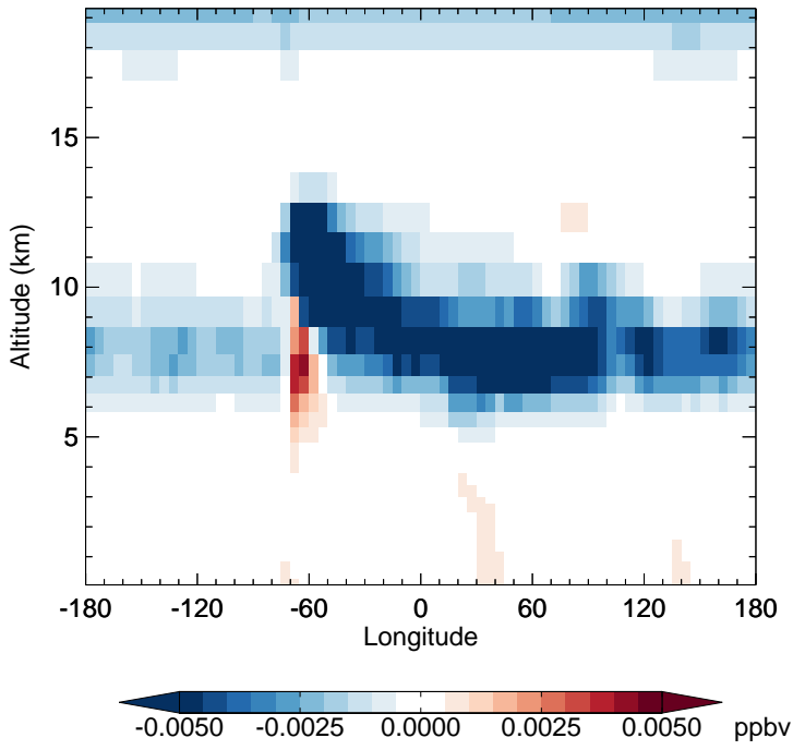
v11-02f-Run0 - v11-02e-Run1 HNO 4 - Diff along 15S for Oct
