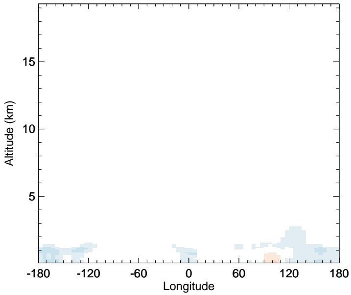
v11-02f-Run0 - v11-02e-Run0 SALA - Diff along 15S for Oct
