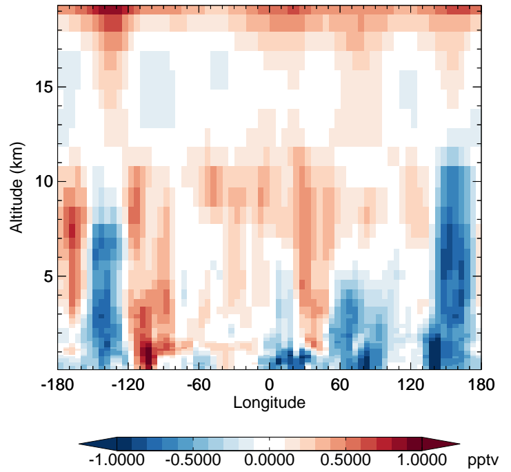
v11-02f-Run0 - v11-02e-Run0 HO2 - Diff along 42N for Oct
