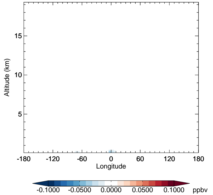
v11-02f-Run0 - v11-02e-Run0 CINO2 - Diff along 42N for Oct
