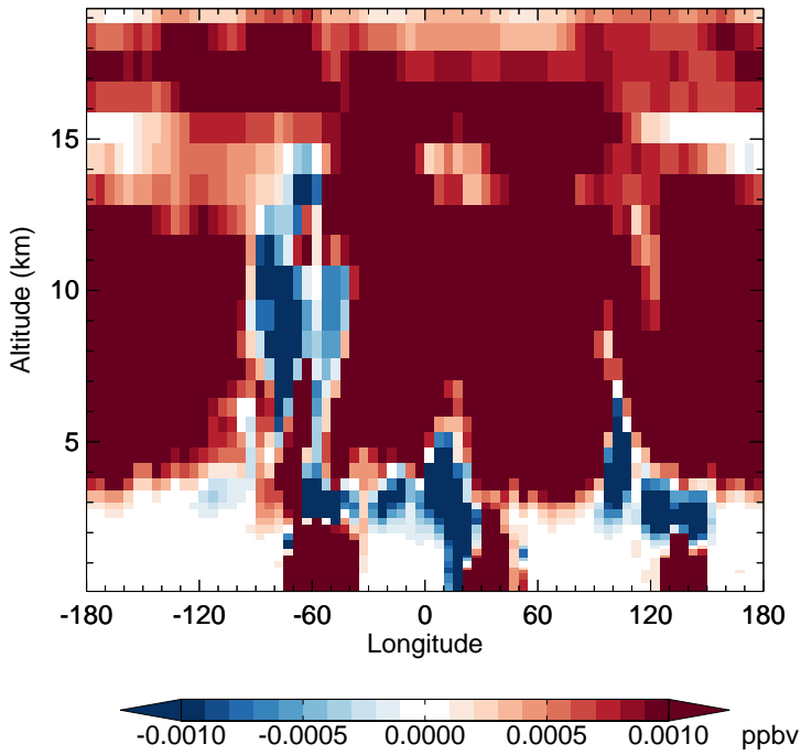
v11-02f-Run0 - v11-02e-Run0 PPN - Diff along 15S for Oct
