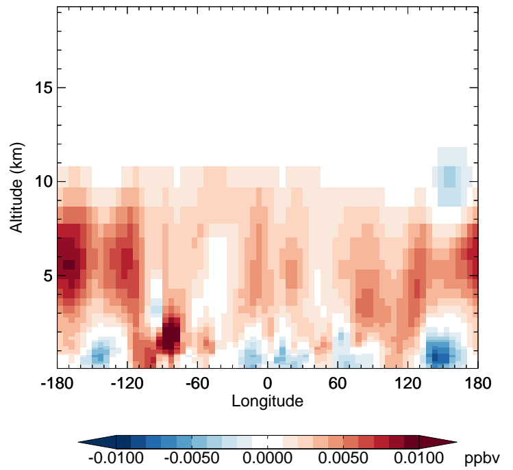
v11-02f-Run0 - v11-02e-Run0 MAP - Diff along 42N for Oct
