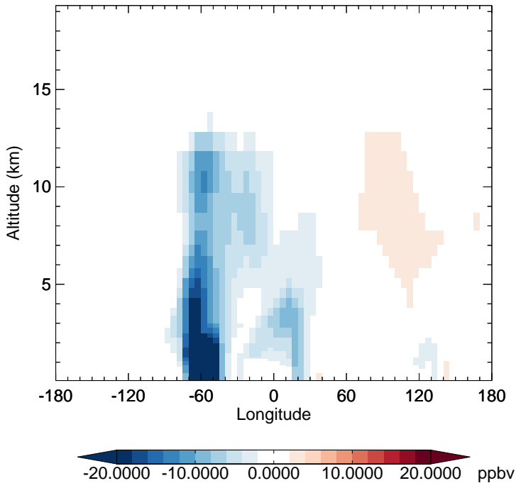
v11-02f-Run0 - v11-02e-Run1 CO - Diff along 15S for Oct
