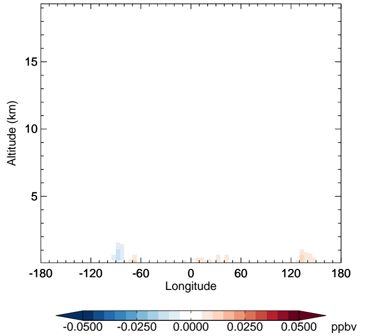
v11-02f-Run0 - v11-02e-Run1 MVK - Diff along 42N for Oct
