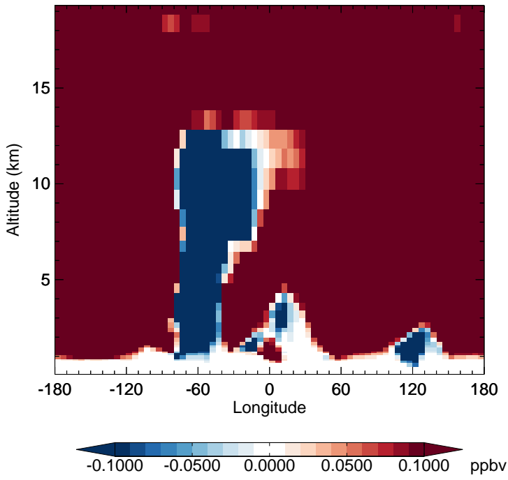
v11-02f-Run0 - v11-02e-Run1 CH4 - Diff along 15S for Oct
