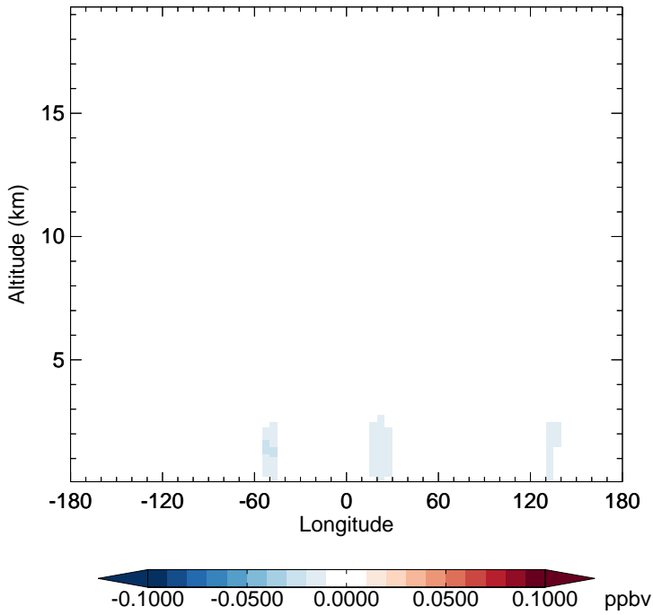
v11-02f-Run0 - v11-02e-Run0 GLYX - Diff along 15S for Oct
