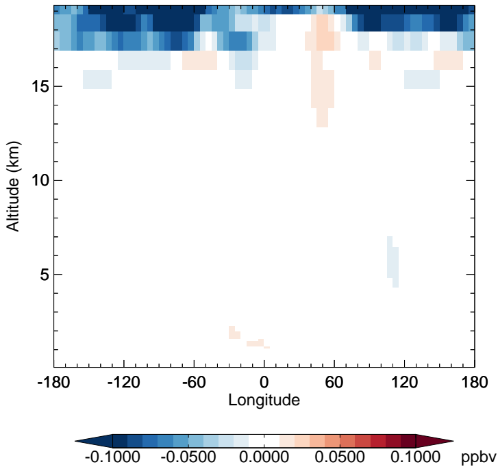
v11-02f-Run0 - v11-02e-Run0 HCl - Diff along 15S for Oct
