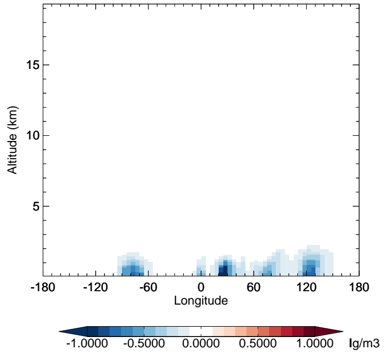
v11-02f-Run0 - v11-02e-Run1 SO 2 - Diff along 42N for Oct
