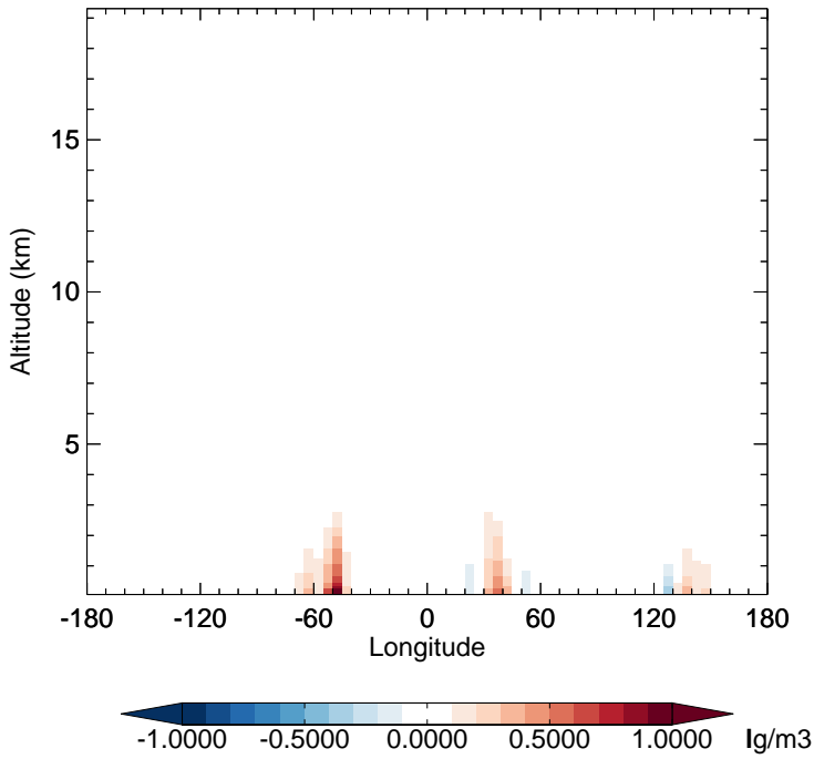
v11-02f-Run0 - v11-02e-Run0 OCPO - Diff along 15S for Oct
