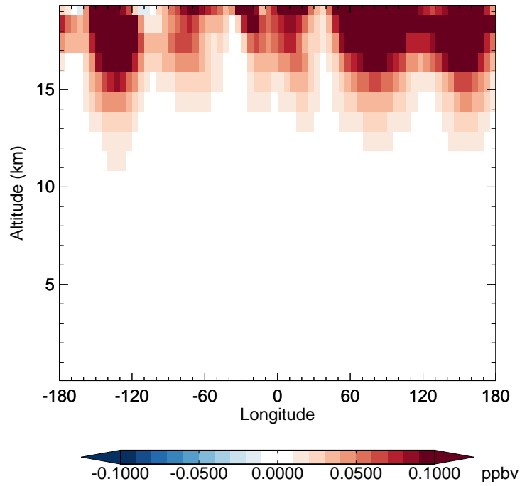
v11-02f-Run0 - v11-02e-Run0 HCl - Diff along 42N for Oct
