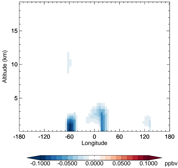
v11-02f-Run0 - v11-02e-Run1 ISOA1 - Diff along 15S for Oct
