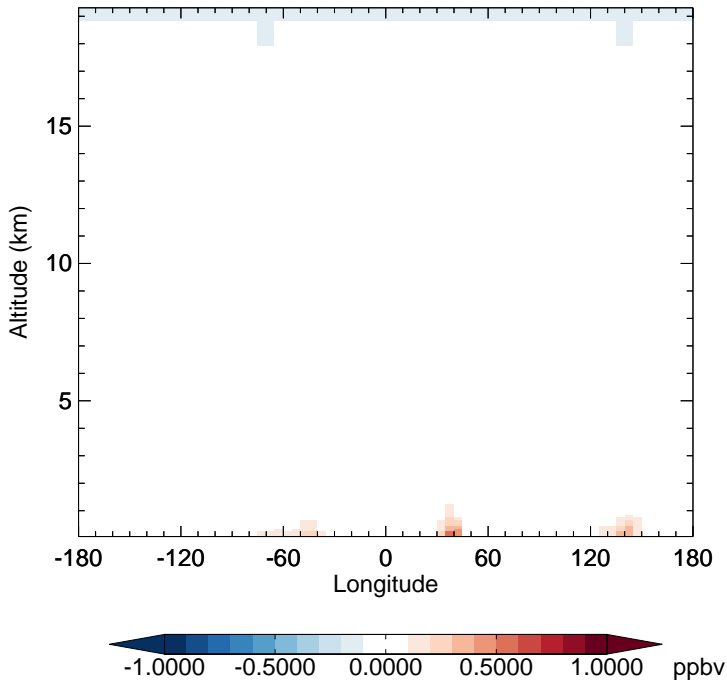
v11-02f-Run0 - v11-02e-Run1 NO 2 - Diff along 15S for Oct
