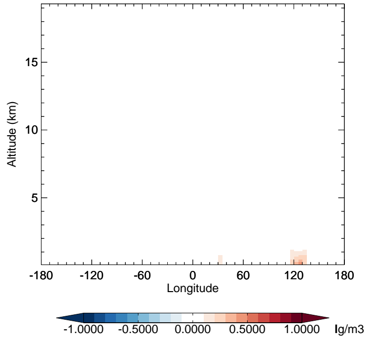
v11-02f-Run0 - v11-02e-Run0 OCPO - Diff along 42N for Oct
