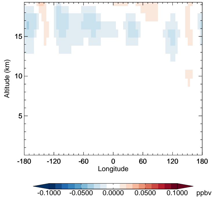
v11-02f-Run0 - v11-02e-Run0 MPN - Diff along 42N for Oct
