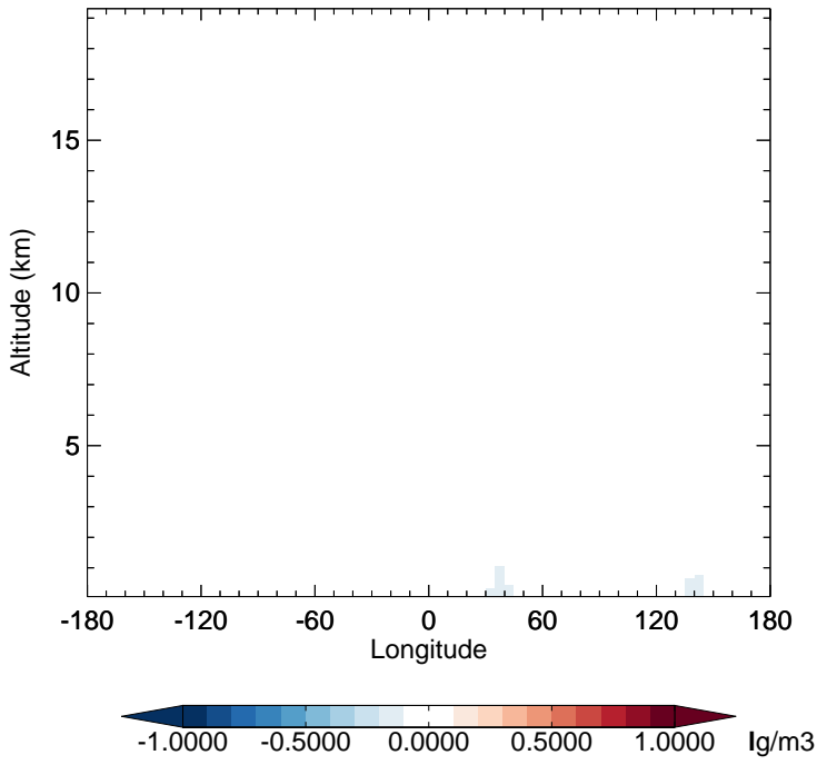
v11-02f-Run0 - v11-02e-Run1 OCPO - Diff along 15S for Oct
