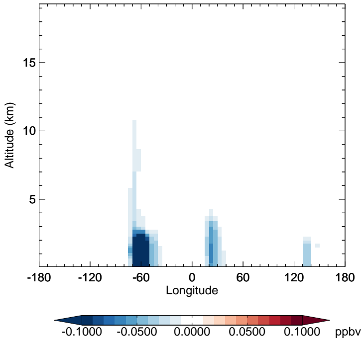
v11-02f-Run0 - v11-02e-Run1 RIPA - Diff along 15S for Oct
