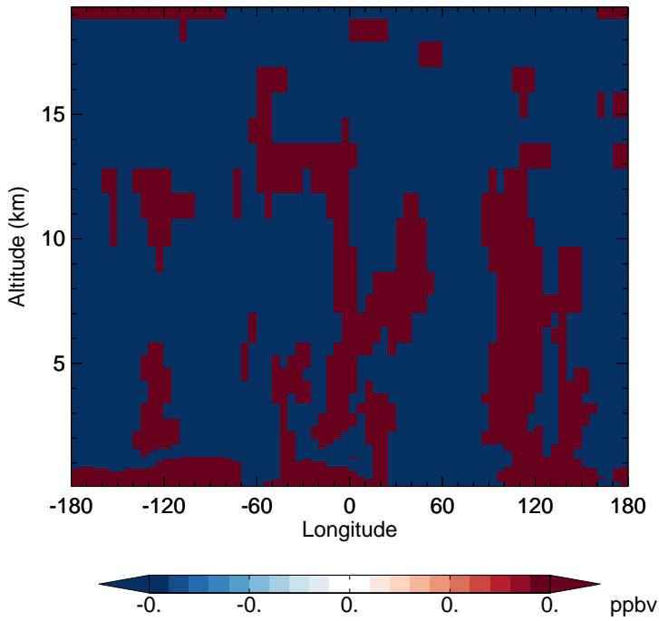
v11-02f-Run0 - v11-02e-Run0 H2O - Diff along 15S for Oct
