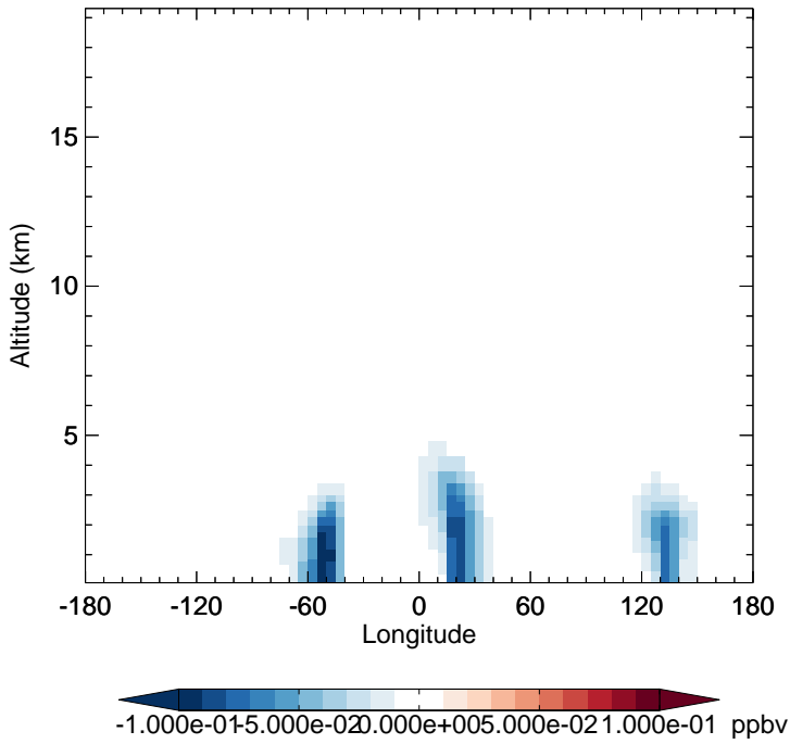
v11-02f-Run0 - v11-02e-Run0 IONITA - Diff along 15S for Oct
