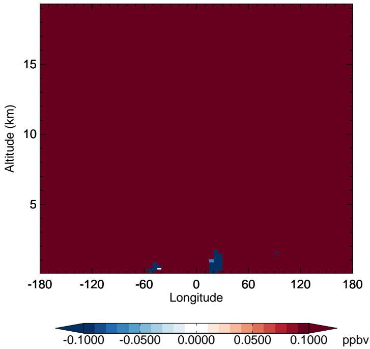
v11-02f-Run0 - v11-02e-Run0 CH4 - Diff along 15S for Oct
