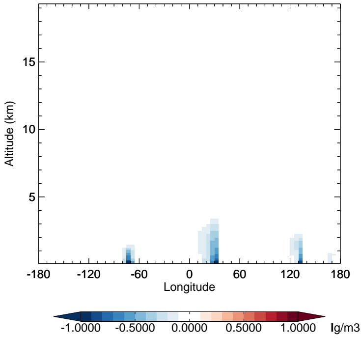
v11-02f-Run0 - v11-02e-Run1 SO 2 - Diff along 15S for Oct
