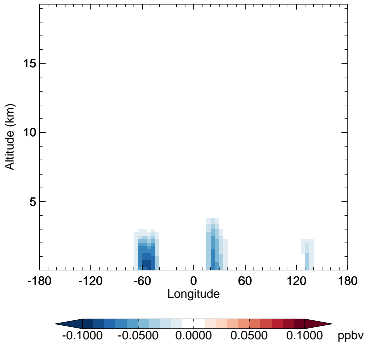
v11-02f-Run0 - v11-02e-Run1 MGLY - Diff along 15S for Oct
