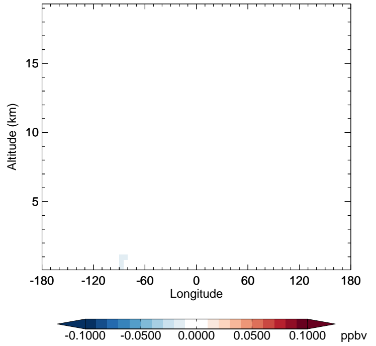
v11-02f-Run0 - v11-02e-Run1 IMAE - Diff along 42N for Oct
