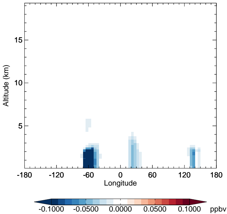
v11-02f-Run0 - v11-02e-Run0 RIPA - Diff along 15S for Oct
