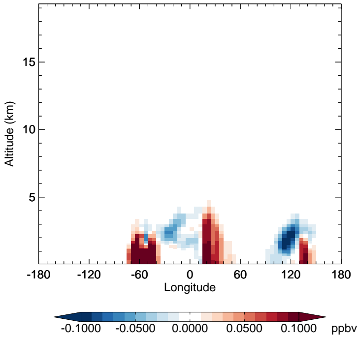
v11-02f-Run0 - v11-02e-Run0 INDIOL - Diff along 15S for Oct
