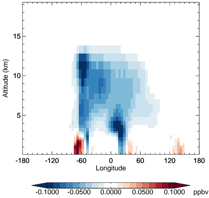
v11-02f-Run0 - v11-02e-Run1 PAN - Diff along 15S for Oct
