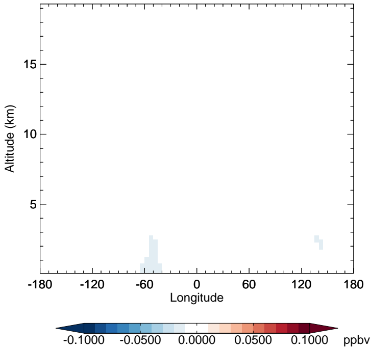
v11-02f-Run0 - v11-02e-Run0 ISOG1 - Diff along 15S for Oct
