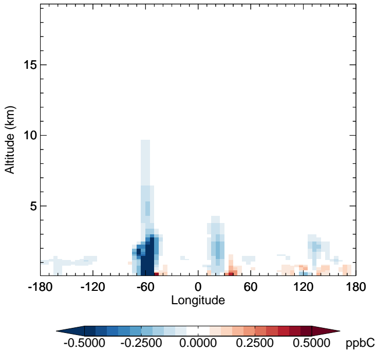
v11-02f-Run0 - v11-02e-Run0 ALD2 - Diff along 15S for Oct
