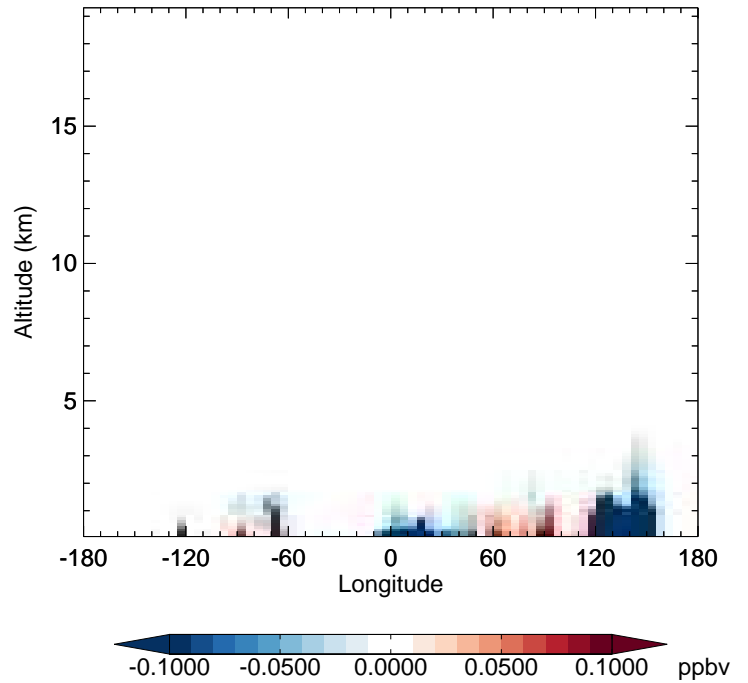
v11-02f-Run0 - v11-02e-Run0 XYLE - Diff along 42N for Oct
