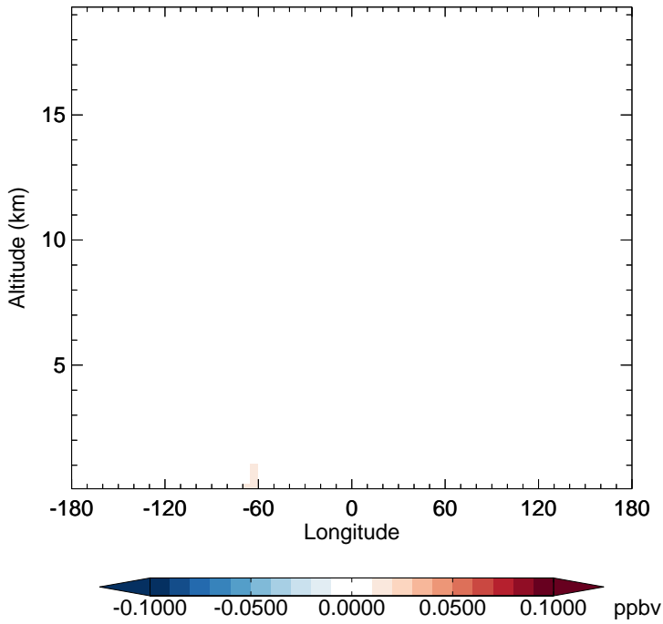
v11-02f-Run0 - v11-02e-Run0 ISOPNB - Diff along 15S for Oct
