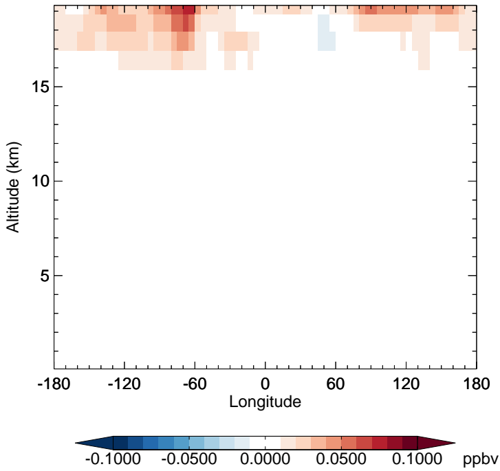
v11-02f-Run0 - v11-02e-Run0 OCS - Diff along 15S for Oct
