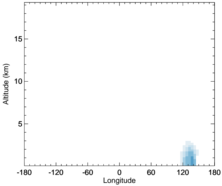
v11-02f-Run0 - v11-02e-Run0 DST4 - Diff along 15S for Oct
