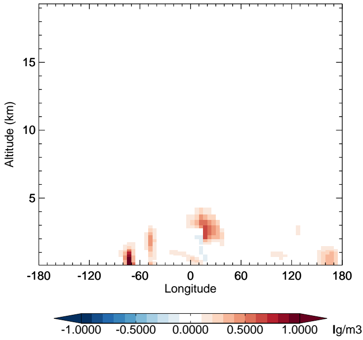
v11-02f-Run0 - v11-02e-Run1 NH4 - Diff along 15S for Oct
