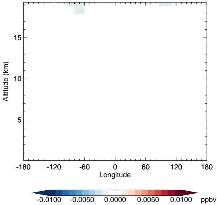
v11-02f-Run0 - v11-02e-Run0 BrNO3 - Diff along 15S for Oct
