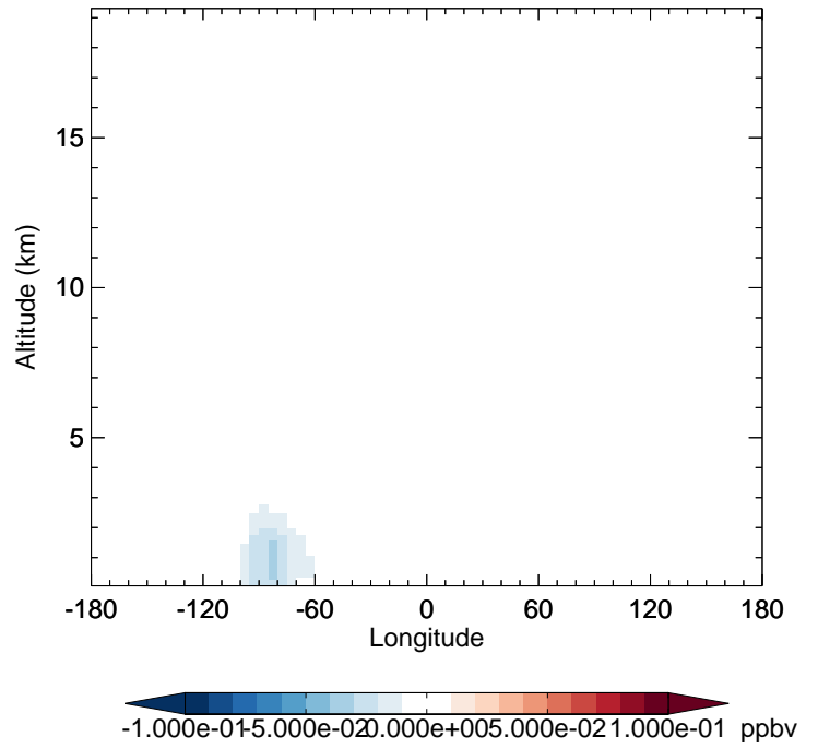
v11-02f-Run0 - v11-02e-Run1 SOAIE - Diff along 42N for Oct
