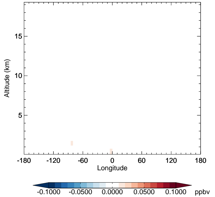
v11-02f-Run0 - v11-02e-Run0 IMAE - Diff along 42N for Oct
