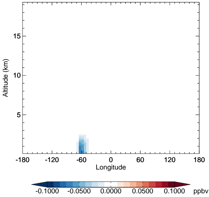
v11-02f-Run0 - v11-02e-Run1 TSOA0 - Diff along 15S for Oct
