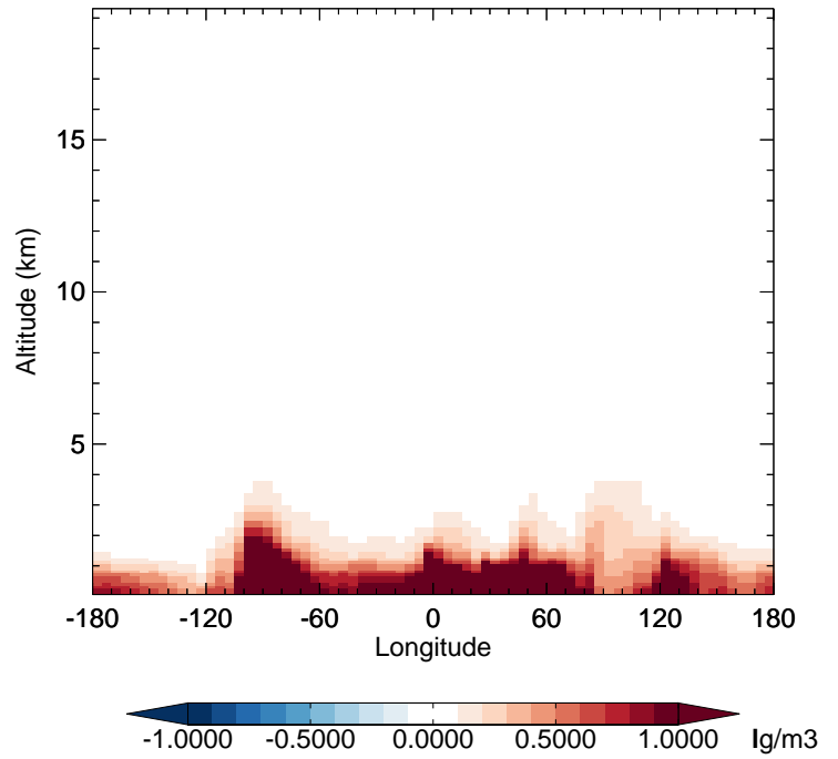
v11-02f-Run0 - v11-02e-Run0 NH3 - Diff along 42N for Oct
