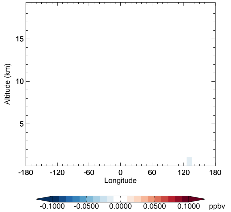
v11-02f-Run0 - v11-02e-Run1 ASOG3 - Diff along 42N for Oct
