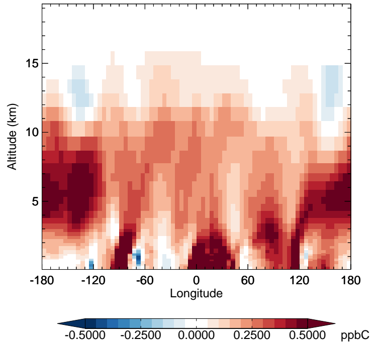
v11-02f-Run0 - v11-02e-Run0 ACET - Diff along 42N for Oct
