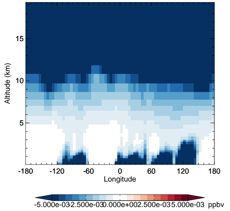
v11-02f-Run0 - v11-02e-Run1 N2O5 - Diff along 42N for Oct
