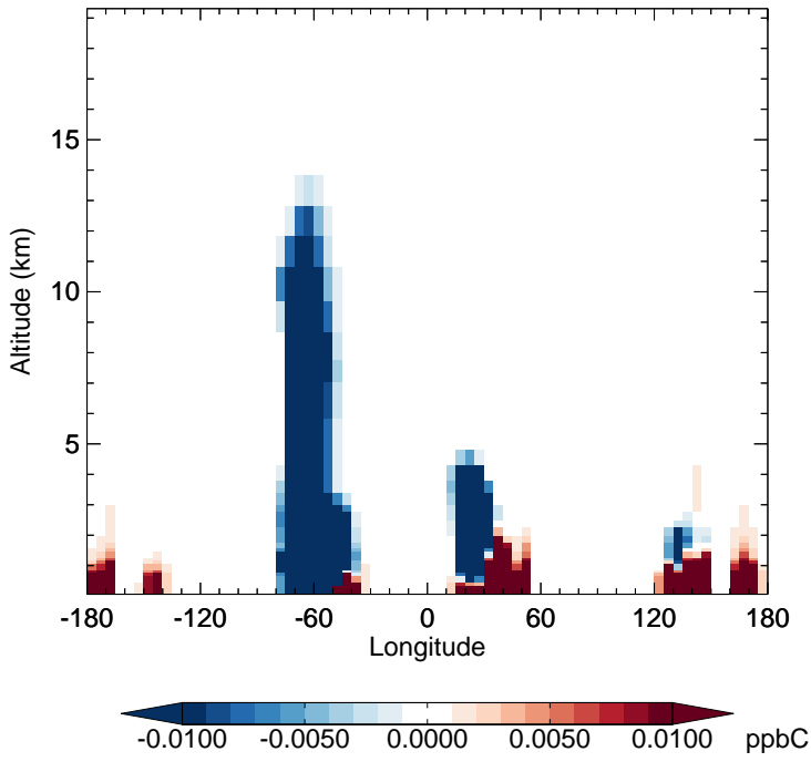
v11-02f-Run0 - v11-02e-Run1 PRPE - Diff along 15S for Oct
