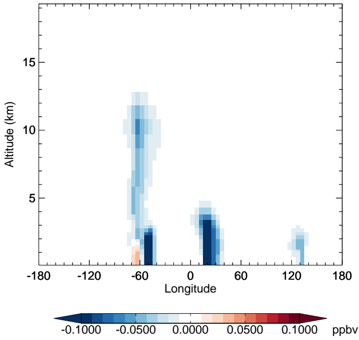
v11-02f-Run0 - v11-02e-Run1 IMAE - Diff along 15S for Oct
