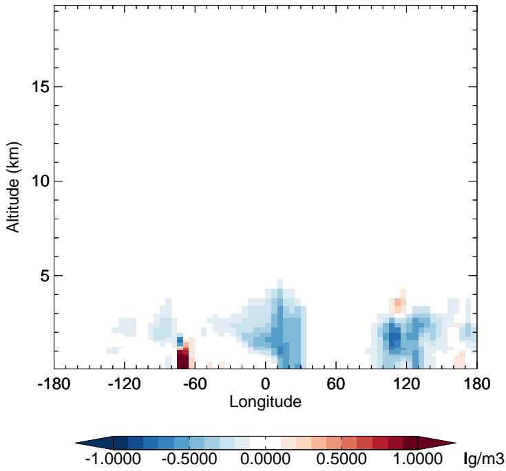
v11-02f-Run0 - v11-02e-Run0 SO4 - Diff along 15S for Oct
