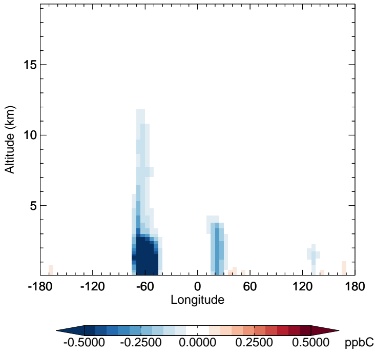
v11-02f-Run0 - v11-02e-Run1 ALD2 - Diff along 15S for Oct
