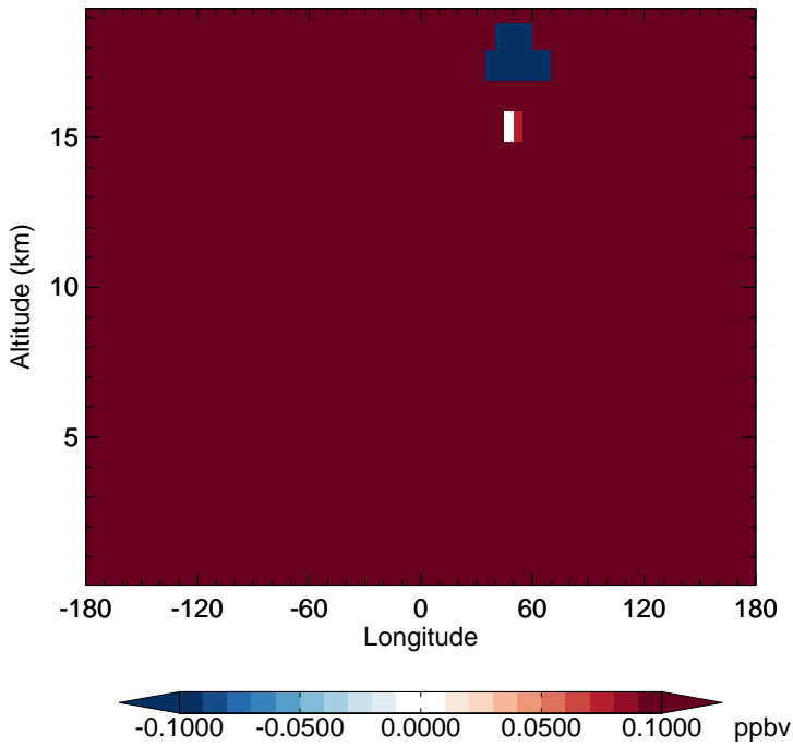
v11-02f-Run0 - v11-02e-Run0 N2O - Diff along 15S for Oct
