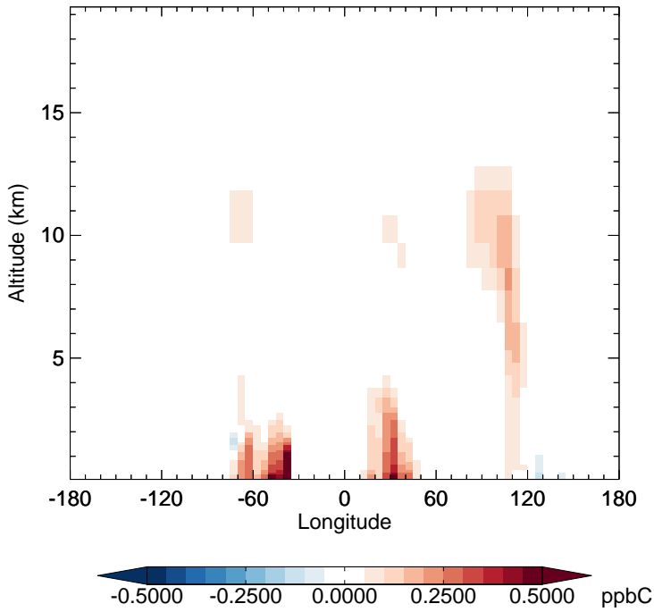
v11-02f-Run0 - v11-02e-Run0 ALK4 - Diff along 15S for Oct
