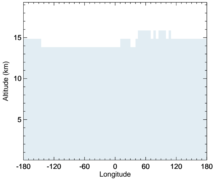
v11-02f-Run0 - v11-02e-Run0 HCFC22 - Diff along 15S for Oct
