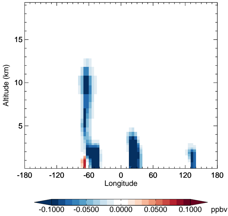
v11-02f-Run0 - v11-02e-Run1 IEPOXA - Diff along 15S for Oct
