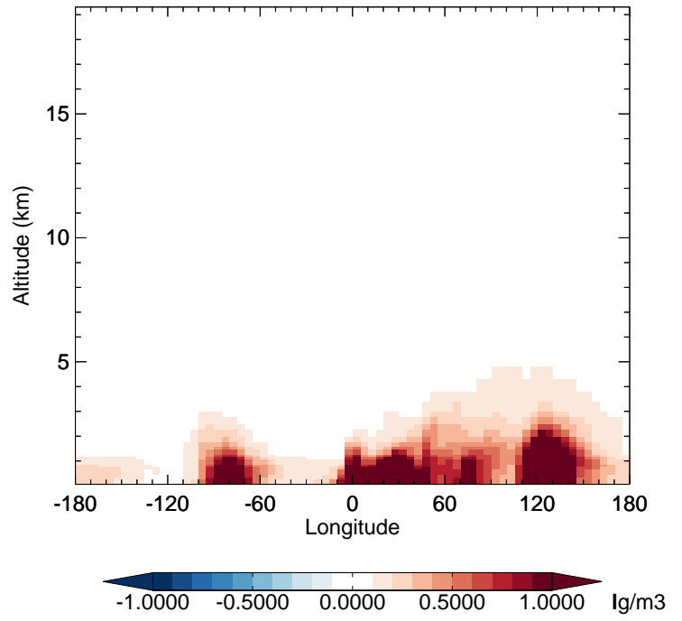
v11-02f-Run0 - v11-02e-Run1 NH4 - Diff along 42N for Oct
