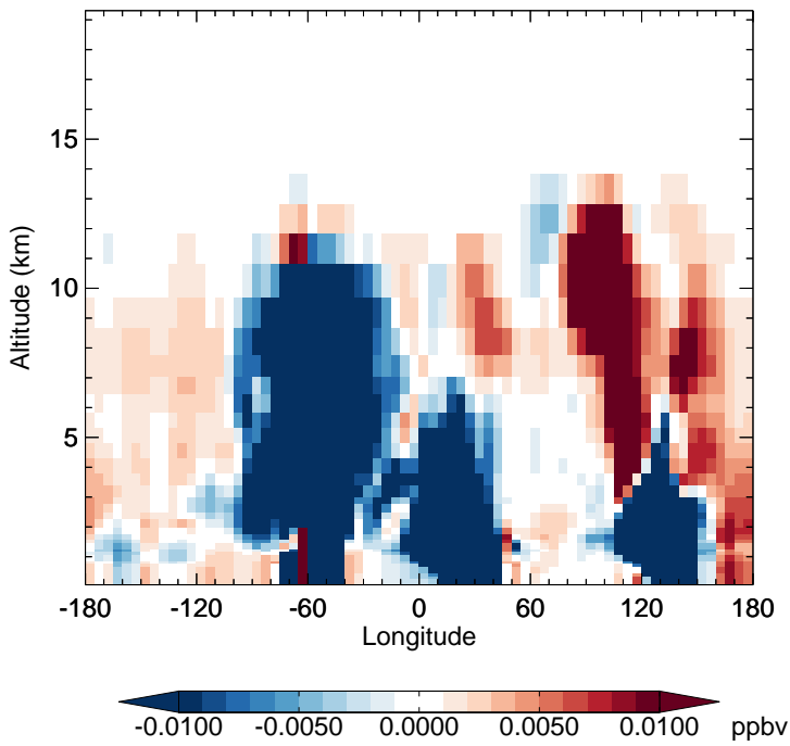
v11-02f-Run0 - v11-02e-Run0 MAP - Diff along 15S for Oct
