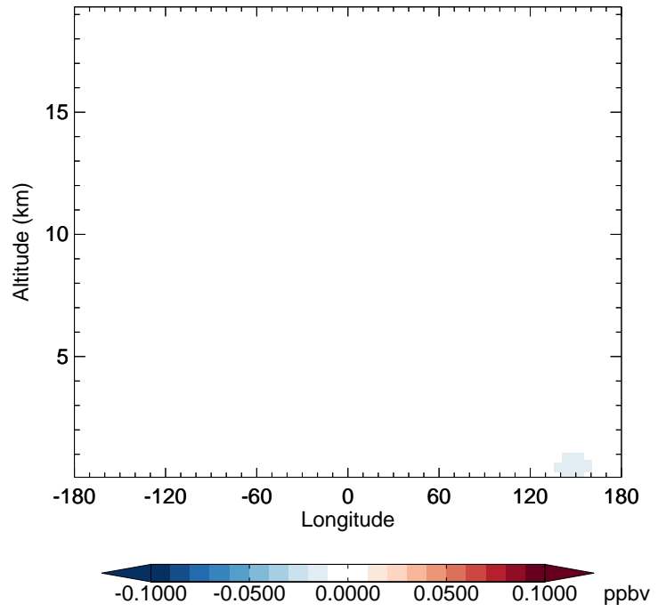
v11-02f-Run0 - v11-02e-Run1 ASOAN - Diff along 42N for Oct
