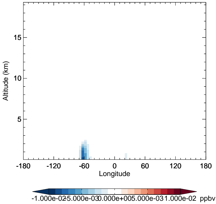
v11-02f-Run0 - v11-02e-Run1 MOBA - Diff along 15S for Oct
