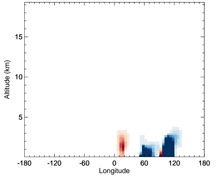
v11-02f-Run0 - v11-02e-Run0 DST4 - Diff along 42N for Oct
