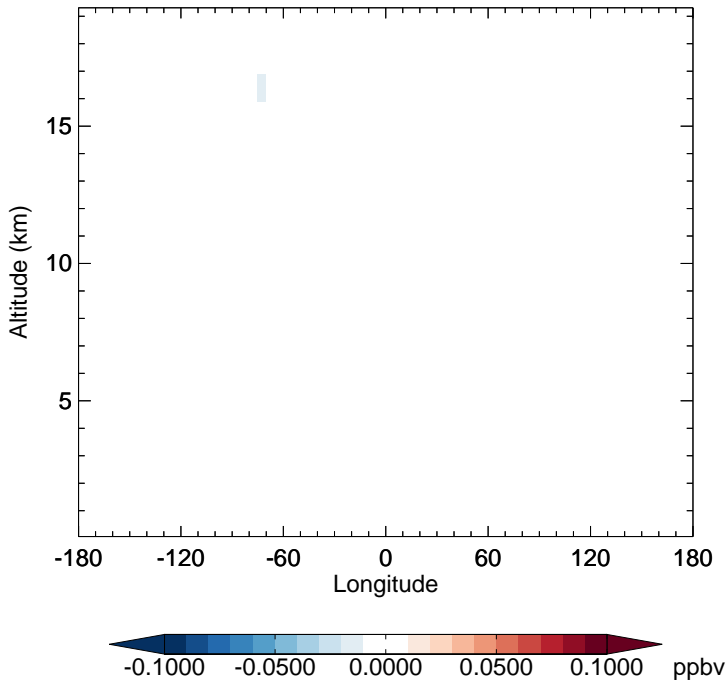
v11-02f-Run0 - v11-02e-Run0 HOCl - Diff along 15S for Oct
