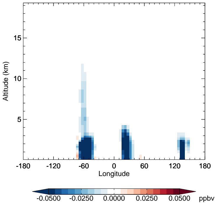
v11-02f-Run0 - v11-02e-Run0 MACR - Diff along 15S for Oct
