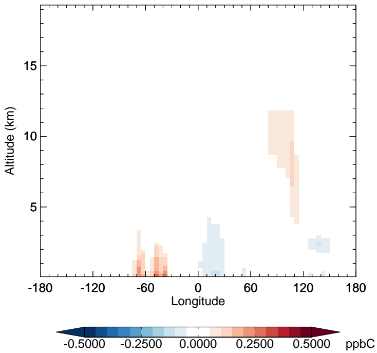
v11-02f-Run0 - v11-02e-Run0 C3H8 - Diff along 15S for Oct
