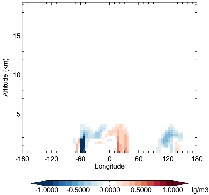
v11-02f-Run0 - v11-02e-Run0 SOAS - Diff along 15S for Oct
