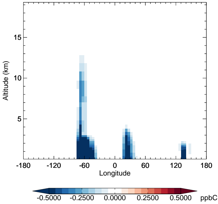
v11-02f-Run0 - v11-02e-Run1 ISOP - Diff along 15S for Oct
