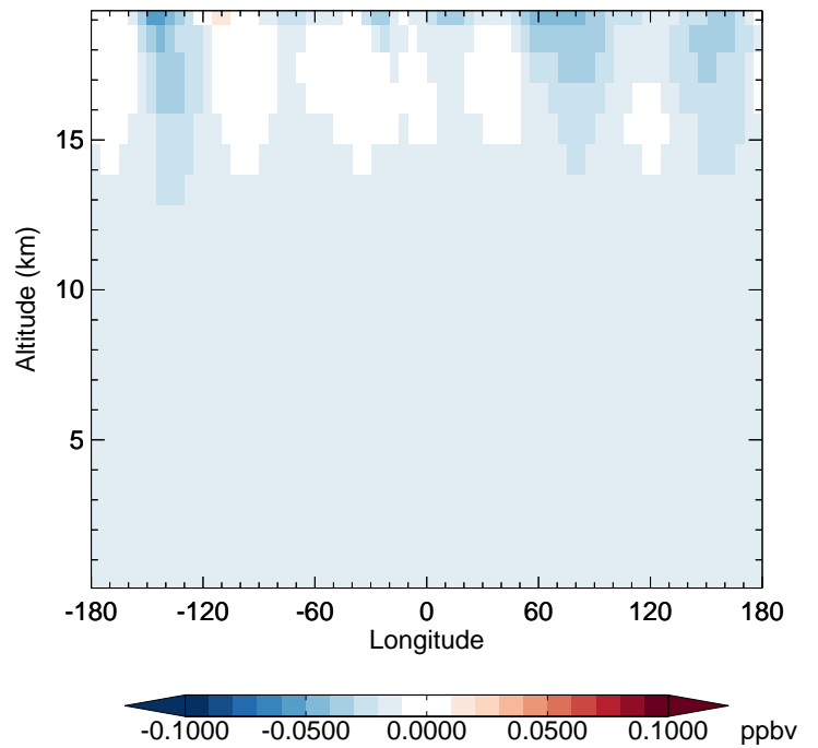
v11-02f-Run0 - v11-02e-Run0 CFC12 - Diff along 42N for Oct
