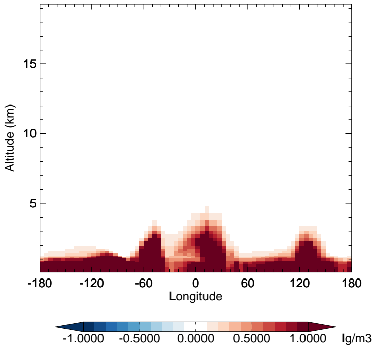
v11-02f-Run0 - v11-02e-Run1 NH3 - Diff along 15S for Oct
