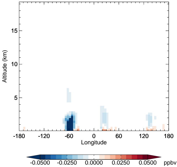
v11-02f-Run0 - v11-02e-Run0 RCHO - Diff along 15S for Oct
