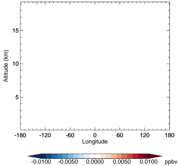
v11-02f-Run0 - v11-02e-Run0 BrO - Diff along 42N for Oct
