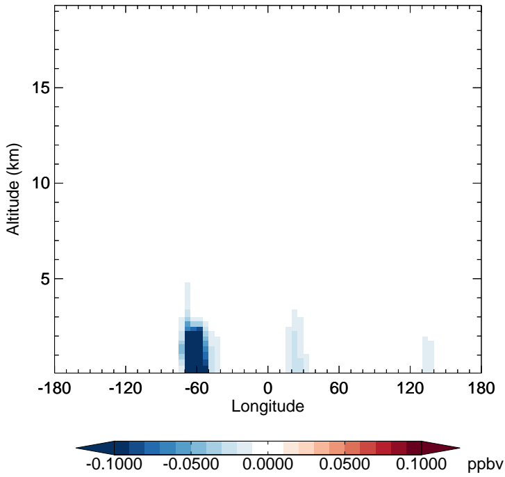
v11-02f-Run0 - v11-02e-Run1 HPALD - Diff along 15S for Oct
