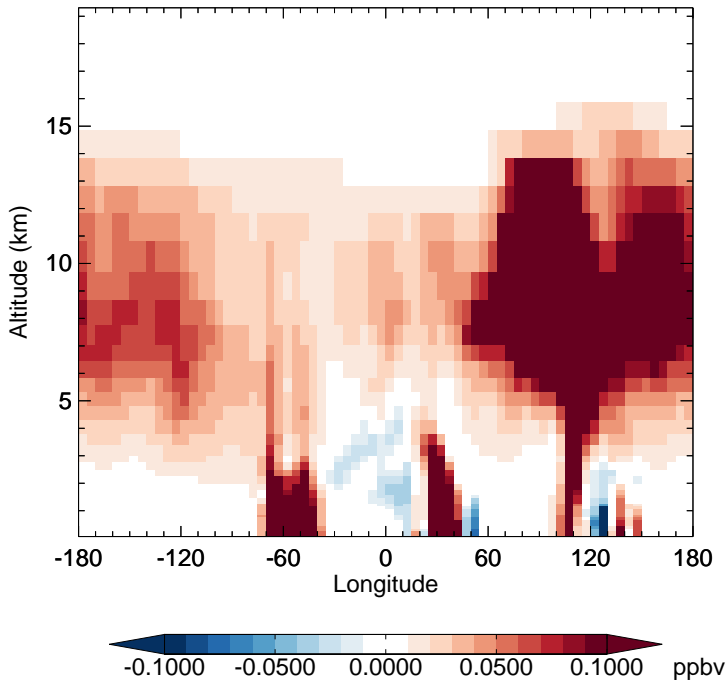
v11-02f-Run0 - v11-02e-Run0 BENZ - Diff along 15S for Oct
