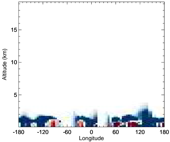
v11-02f-Run0 - v11-02e-Run0 SALC - Diff along 15S for Oct
