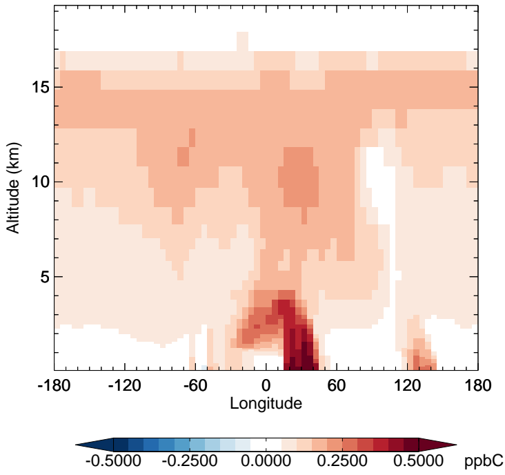
v11-02f-Run0 - v11-02e-Run1 C2H6 - Diff along 15S for Oct
