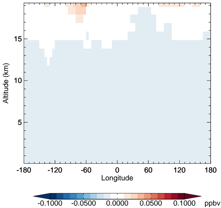
v11-02f-Run0 - v11-02e-Run0 CFC11 - Diff along 15S for Oct
