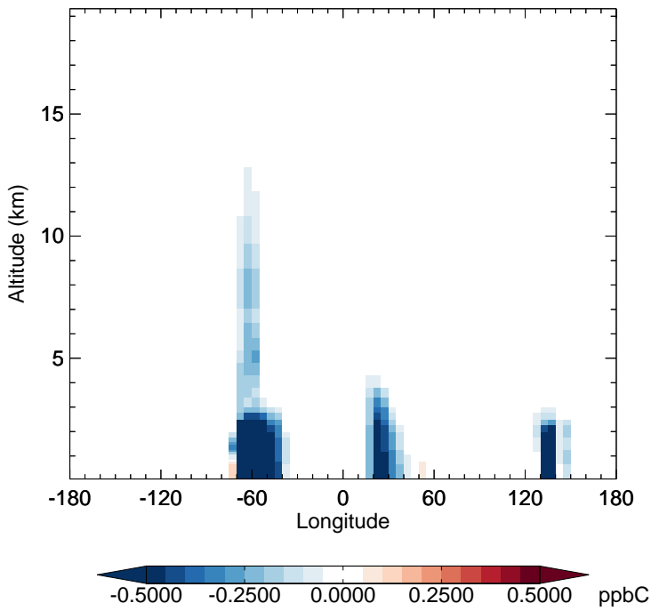
v11-02f-Run0 - v11-02e-Run0 ISOP - Diff along 15S for Oct
