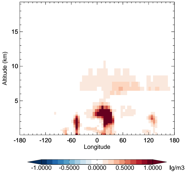
v11-02f-Run0 - v11-02e-Run1 NIT - Diff along 15S for Oct
