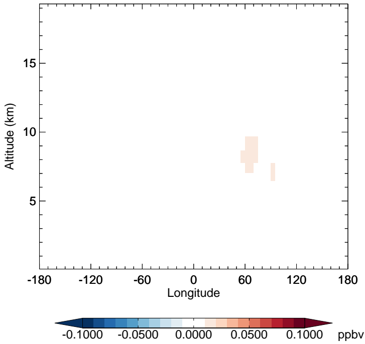
v11-02f-Run0 - v11-02e-Run1 ASOG3 - Diff along 15S for Oct
