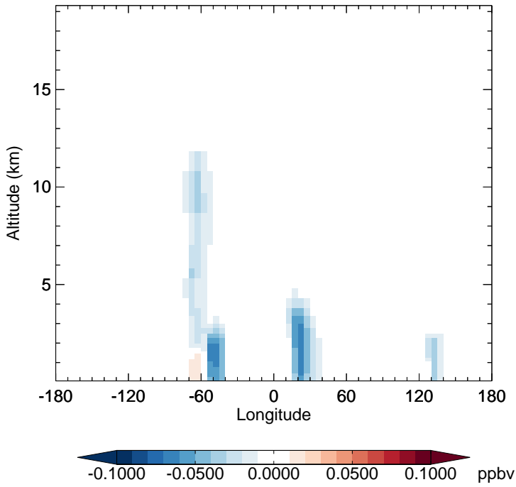
v11-02f-Run0 - v11-02e-Run1 HC187 - Diff along 15S for Oct
