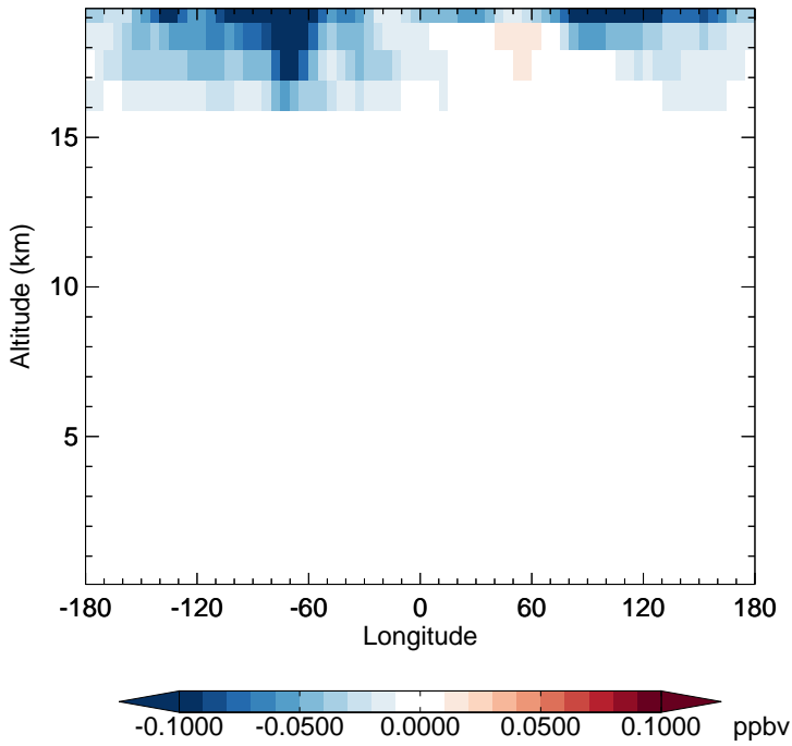
v11-02f-Run0 - v11-02e-Run0 CINO3 - Diff along 15S for Oct
