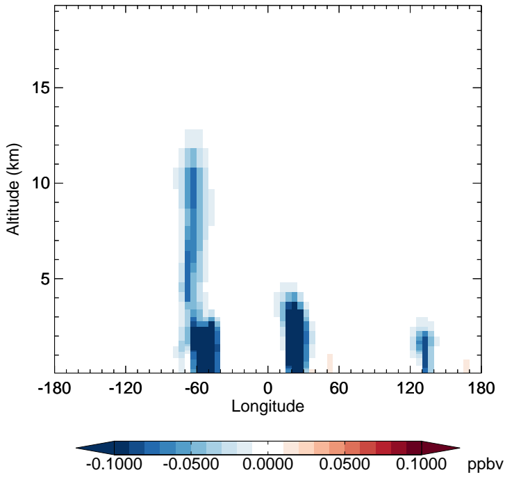
v11-02f-Run0 - v11-02e-Run1 HAC - Diff along 15S for Oct
