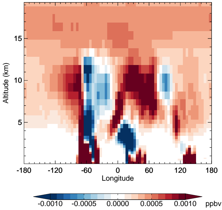
v11-02f-Run0 - v11-02e-Run1 PPN - Diff along 15S for Oct
