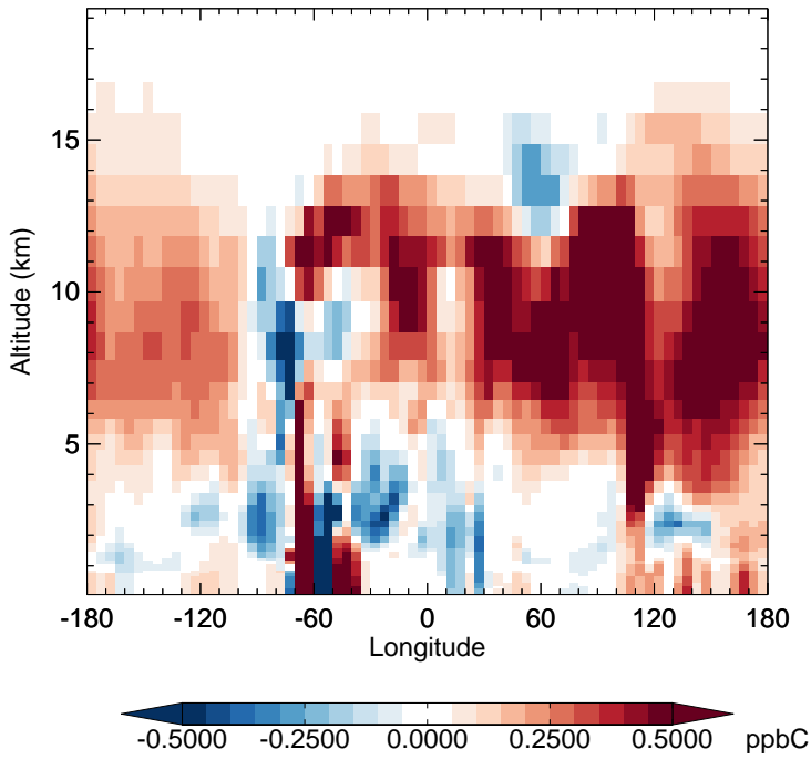
v11-02f-Run0 - v11-02e-Run0 ACET - Diff along 15S for Oct
