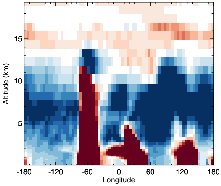
v11-02f-Run0 - v11-02e-Run1 OH - Diff along 15S for Oct
