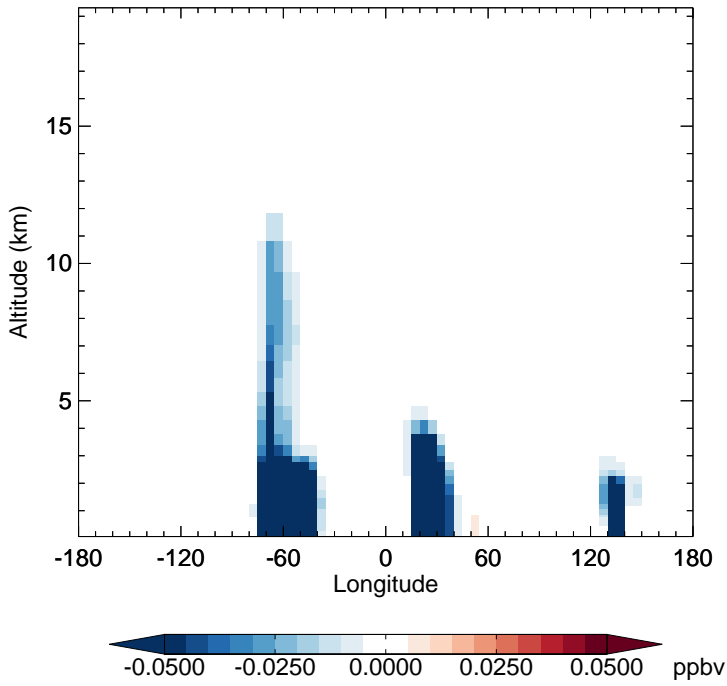
v11-02f-Run0 - v11-02e-Run1 MVK - Diff along 15S for Oct
