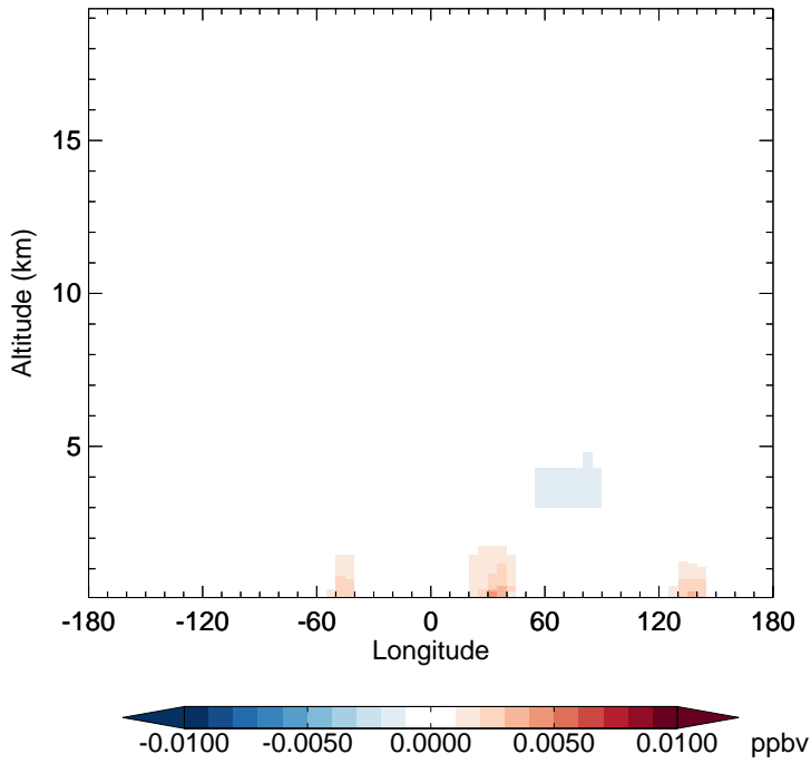
v11-02f-Run0 - v11-02e-Run1 NO3 - Diff along 15S for Oct
