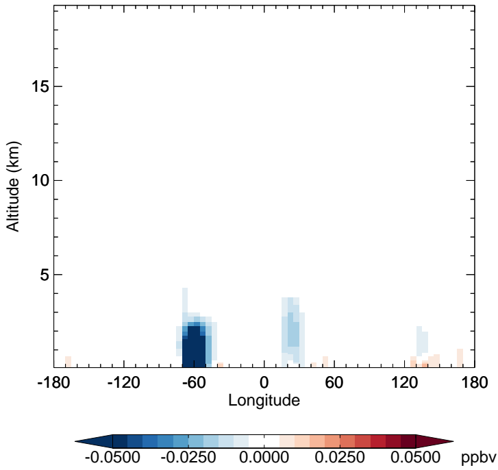
v11-02f-Run0 - v11-02e-Run1 RCHO - Diff along 15S for Oct
