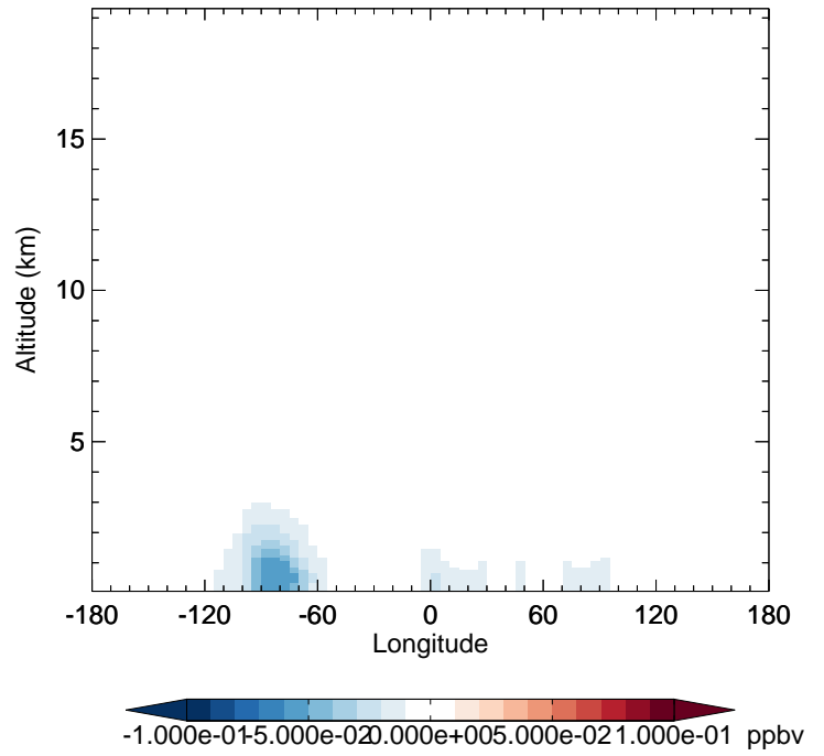
v11-02f-Run0 - v11-02e-Run1 IONITA - Diff along 42N for Oct
