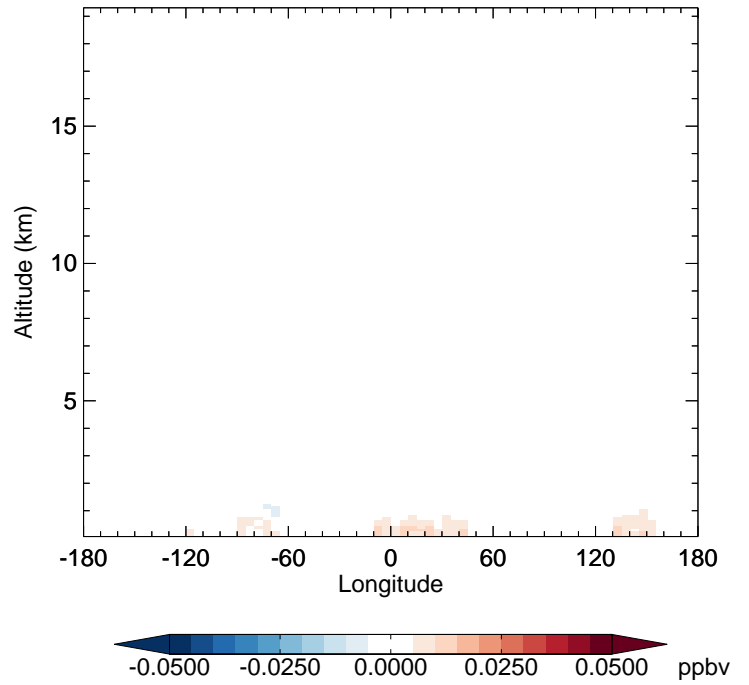
v11-02f-Run0 - v11-02e-Run0 RCHO - Diff along 42N for Oct
