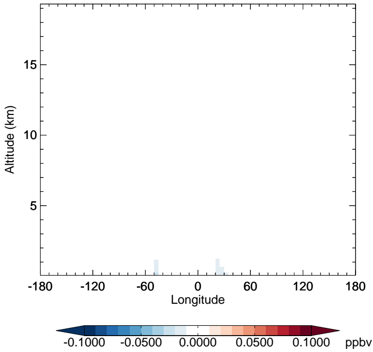
v11-02f-Run0 - v11-02e-Run1 ISN1 - Diff along 15S for Oct
