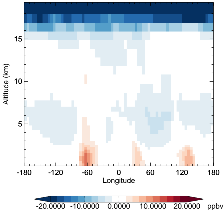
v11-02f-Run0 - v11-02e-Run1 O3 - Diff along 15S for Oct
