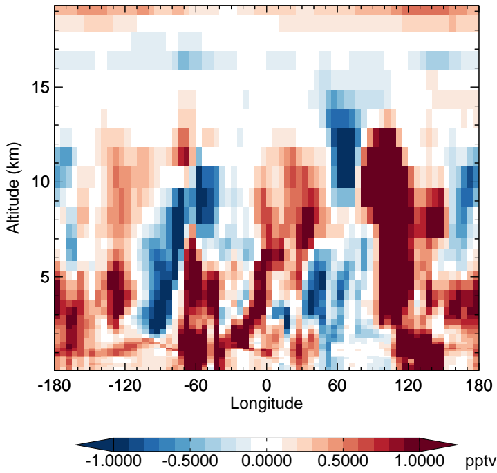
v11-02f-Run0 - v11-02e-Run0 HO2 - Diff along 15S for Oct
