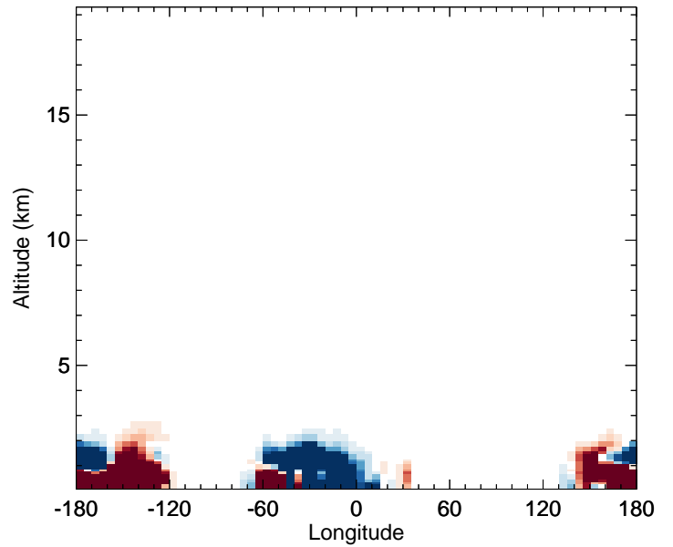
v11-02f-Run0 - v11-02e-Run0 SALC - Diff along 42N for Oct
