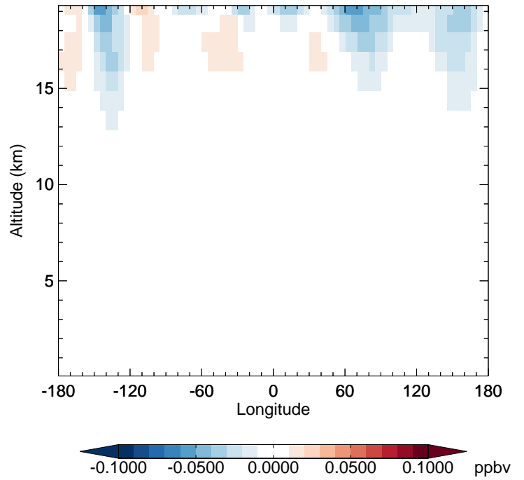
v11-02f-Run0 - v11-02e-Run0 OCS - Diff along 42N for Oct
