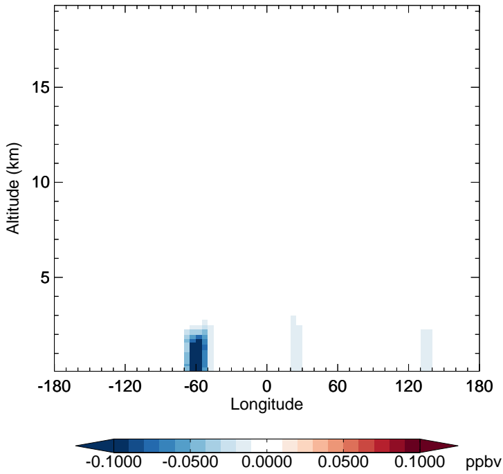
v11-02f-Run0 - v11-02e-Run0 RIPB - Diff along 15S for Oct
