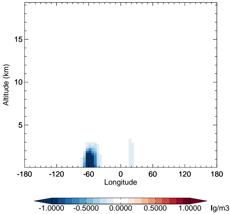
v11-02f-Run0 - v11-02e-Run1 SOAS - Diff along 15S for Oct
