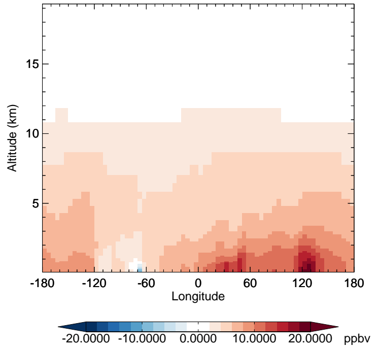
v11-02f-Run0 - v11-02e-Run1 CO - Diff along 42N for Oct
