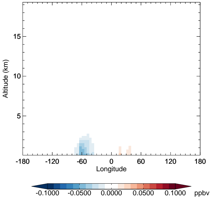
v11-02f-Run0 - v11-02e-Run1 SOAP - Diff along 15S for Oct
