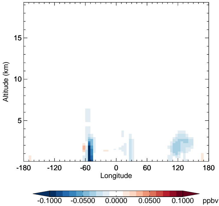
v11-02f-Run0 - v11-02e-Run0 TSOG2 - Diff along 15S for Oct
