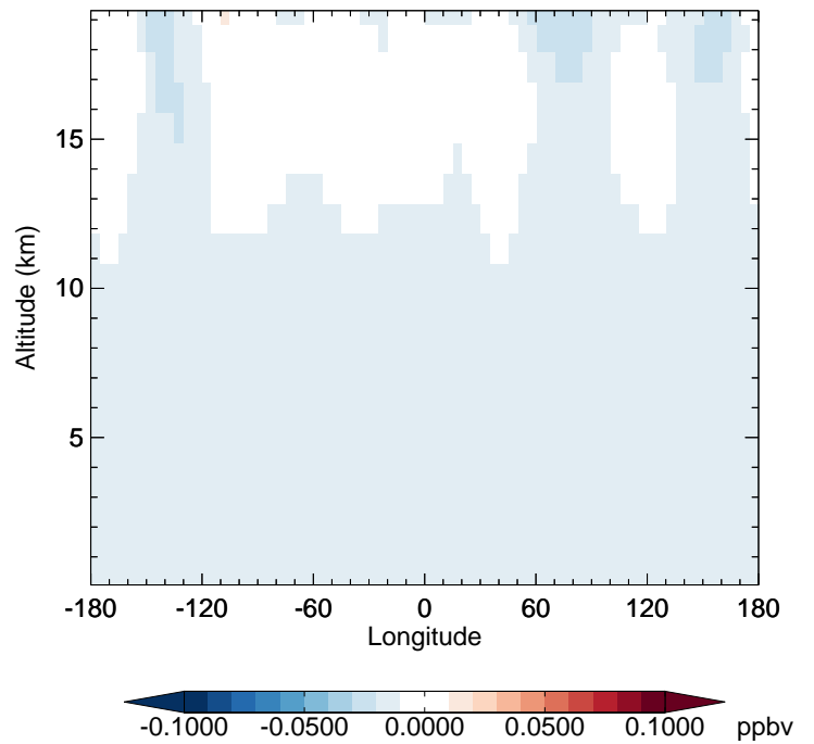
v11-02f-Run0 - v11-02e-Run0 CFC11 - Diff along 42N for Oct
