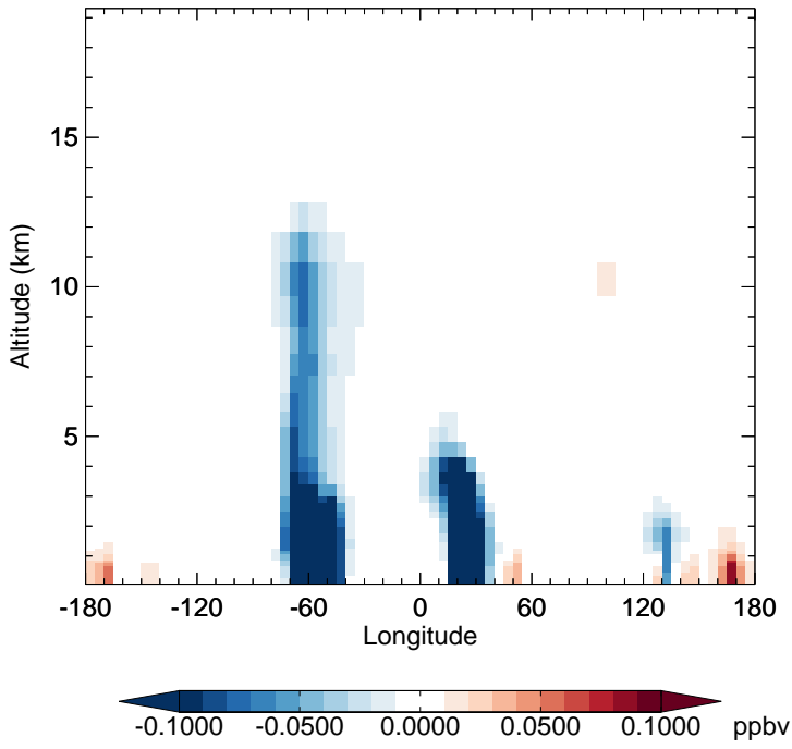
v11-02f-Run0 - v11-02e-Run1 EOH - Diff along 15S for Oct
