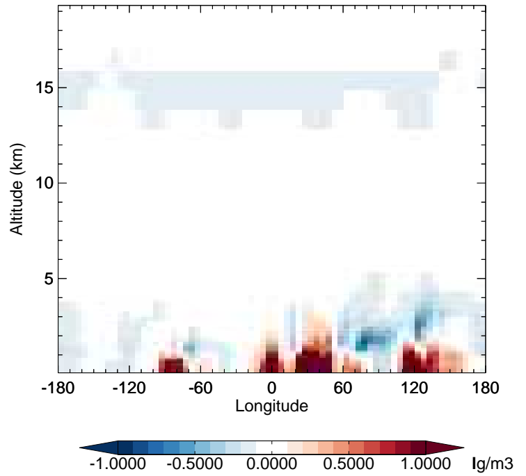
v11-02f-Run0 - v11-02e-Run0 SO4 - Diff along 42N for Oct
