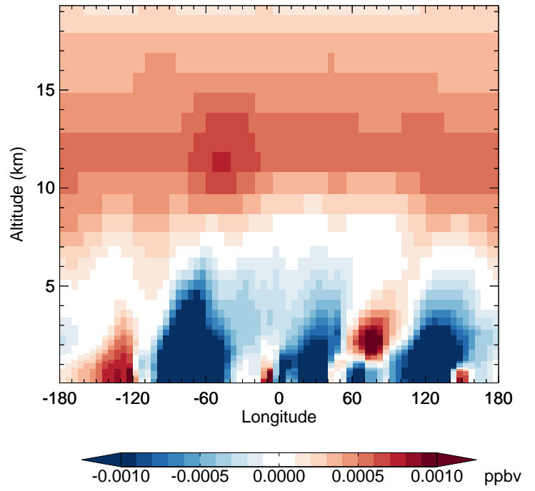
v11-02f-Run0 - v11-02e-Run1 PPN - Diff along 42N for Oct
