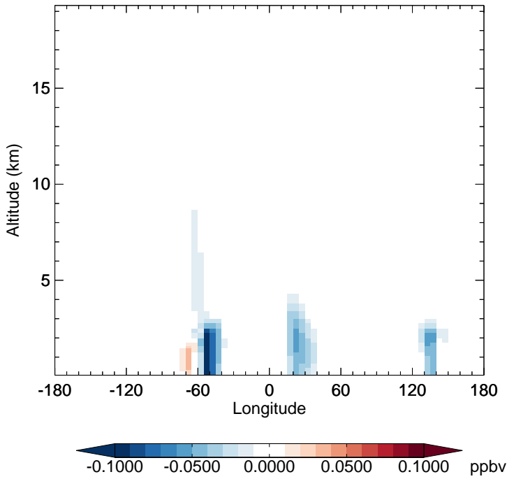
v11-02f-Run0 - v11-02e-Run0 IEPOXB - Diff along 15S for Oct
