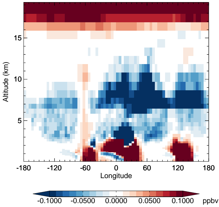
v11-02f-Run0 - v11-02e-Run1 HNO 3 - Diff along 15S for Oct
