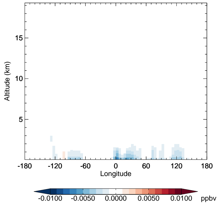
v11-02f-Run0 - v11-02e-Run0 NO3 - Diff along 42N for Oct
