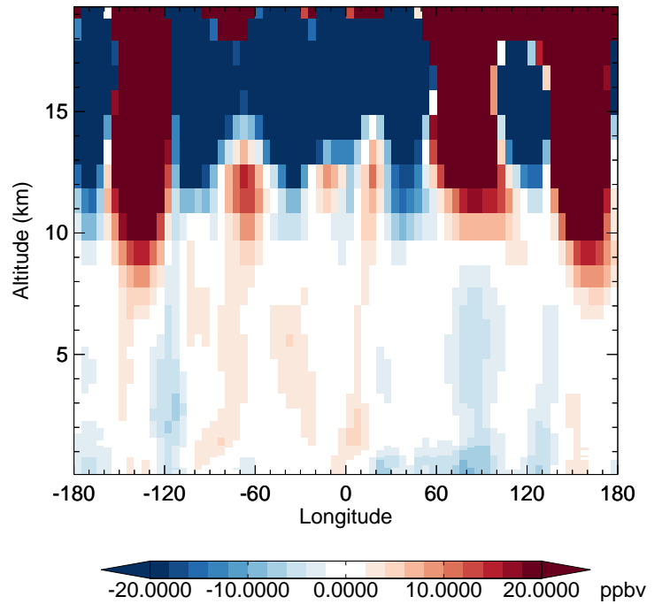
v11-02f-Run0 - v11-02e-Run0 O3 - Diff along 42N for Oct
