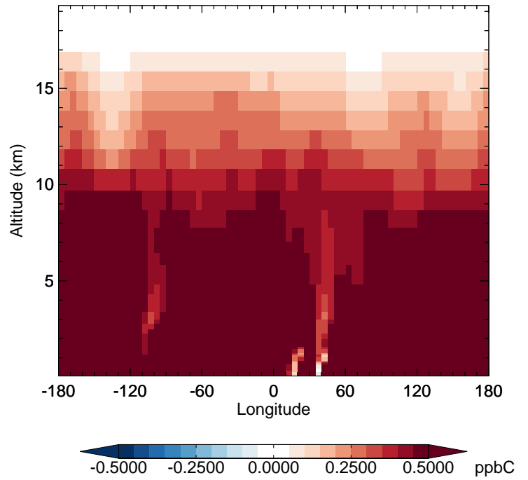
v11-02f-Run0 - v11-02e-Run0 C2H6 - Diff along 42N for Oct
