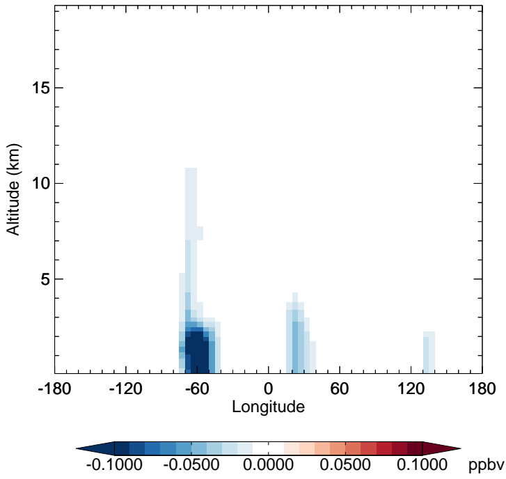
v11-02f-Run0 - v11-02e-Run1 IPMN - Diff along 15S for Oct
