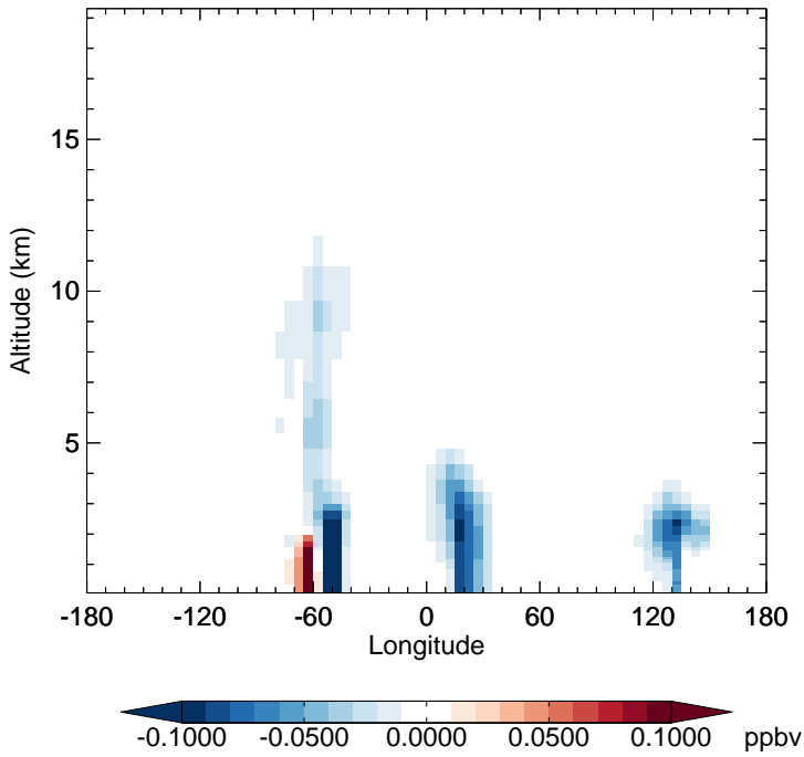
v11-02f-Run0 - v11-02e-Run0 IMAE - Diff along 15S for Oct
