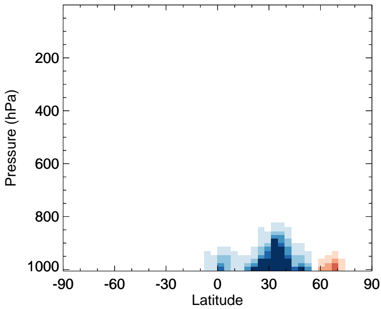
v11-02f-Run0 - v11-02e-Run1 XYLE - Zonal mean abs diff for Apr
