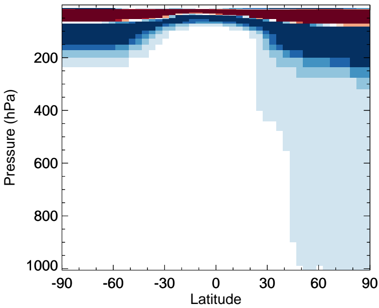
v11-02f-Run0 - v11-02e-Run1 O3 - Zonal mean abs diff for Apr
