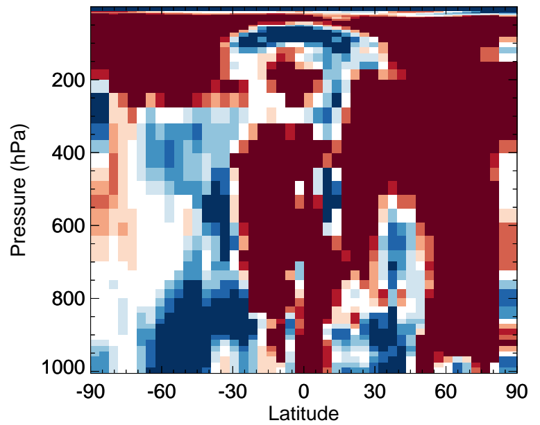
v11-02f-Run0 / v11-02e-Run0 OCIO - Zonal mean % diff for Apr
