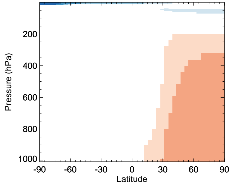
v11-02f-Run0 / v11-02e-Run1 CO - Zonal mean % diff for Apr
