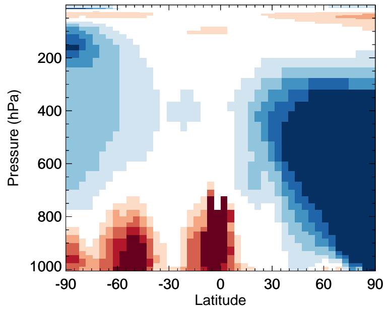
v11-02f-Run0 / v11-02e-Run1 MPN - Zonal mean % diff for Apr
