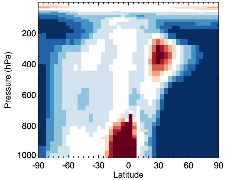
v11-02f-Run0 / v11-02e-Run1 CINO3 - Zonal mean % diff for Apr
