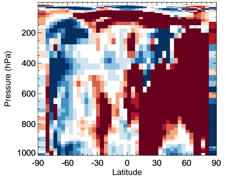
v11-02f-Run0 / v11-02e-Run0 HBr - Zonal mean % diff for Apr
