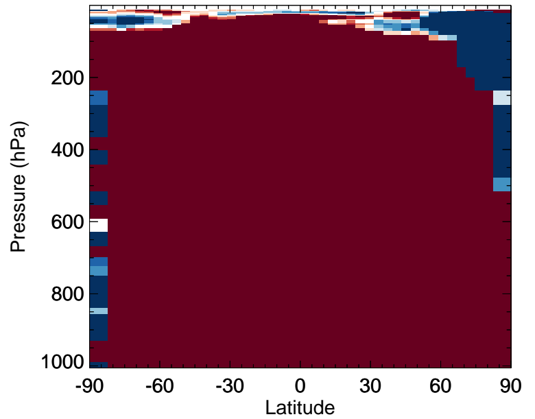
v11-02f-Run0 / v11-02e-Run0 MTPO - Zonal mean % diff for Apr
