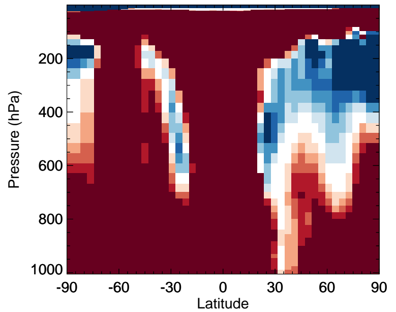
v11-02f-Run0 / v11-02e-Run0 TOLU - Zonal mean % diff for Apr
