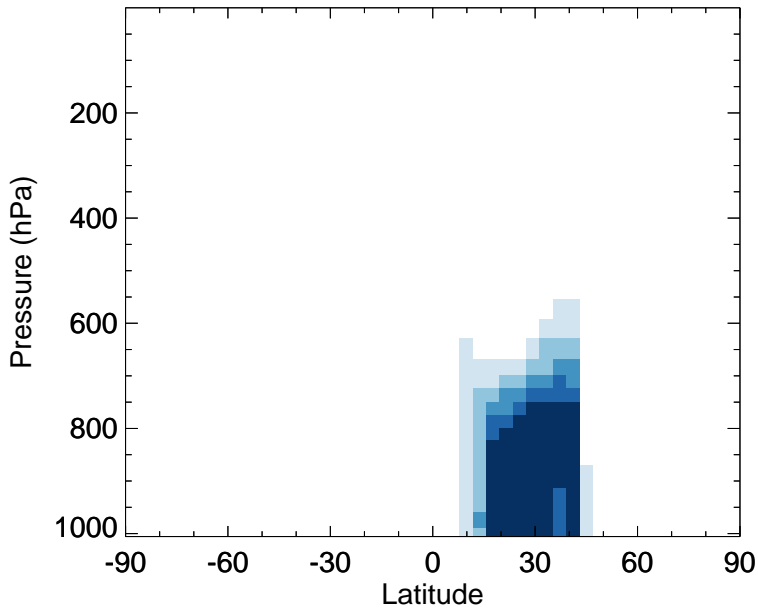
v11-02f-Run0 - v11-02e-Run0 DST4 - Zonal mean abs diff for Apr
