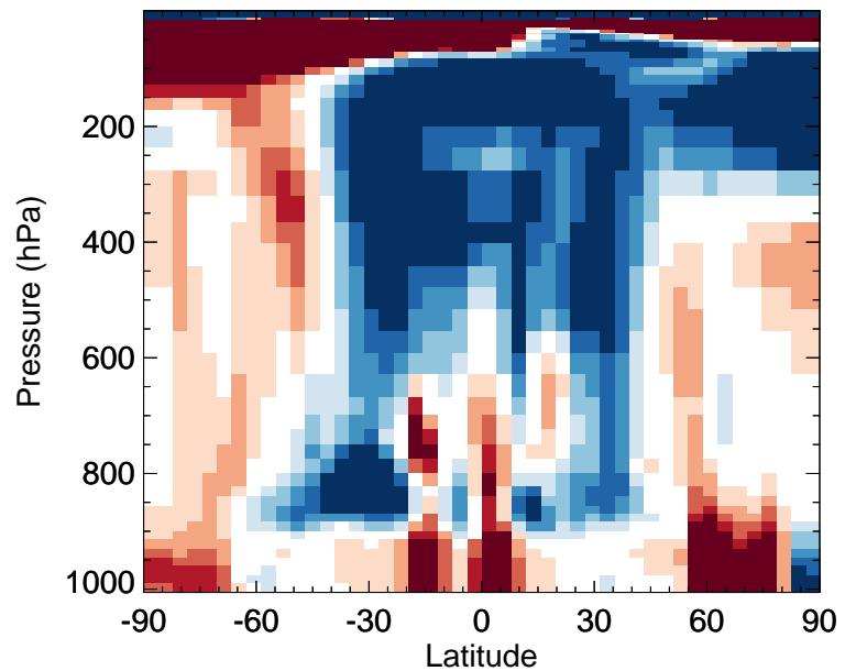
v11-02f-Run0 / v11-02e-Run0 SALA - Zonal mean % diff for Apr
