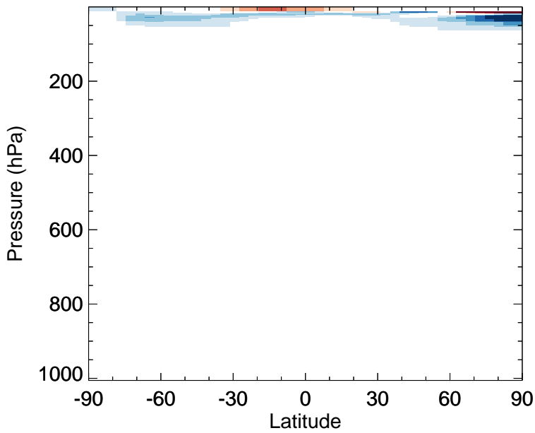
v11-02f-Run0 - v11-02e-Run0 NO - Zonal mean abs diff for Apr
