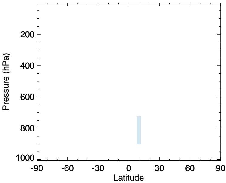
v11-02f-Run0 - v11-02e-Run1 CH 2 O - Zonal mean abs diff for Apr
