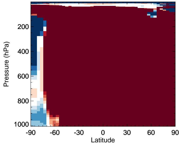
v11-02f-Run0 / v11-02e-Run0 HPALD - Zonal mean % diff for Apr
