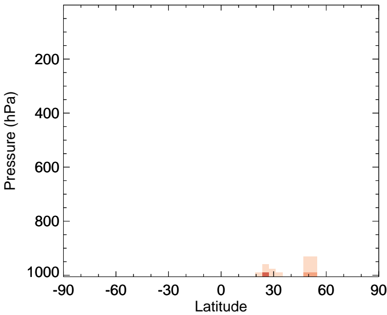
v11-02f-Run0 - v11-02e-Run0 OCPO - Zonal mean abs diff for Apr
