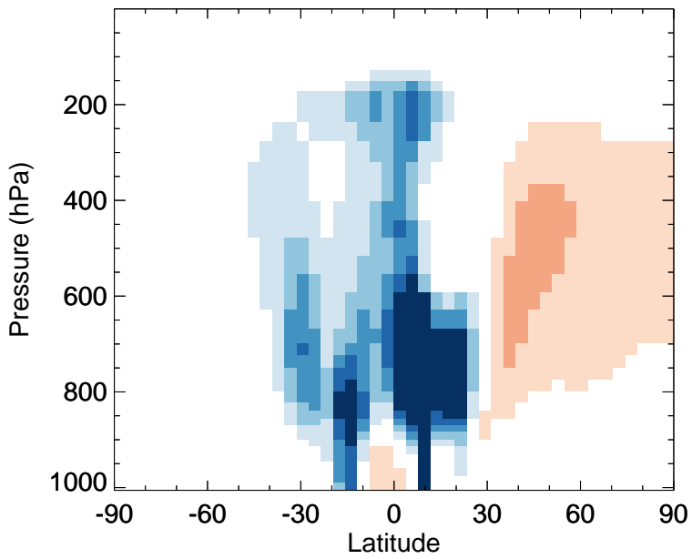
v11-02f-Run0 - v11-02e-Run1 MAP - Zonal mean abs diff for Apr
