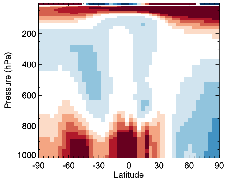
v11-02f-Run0 / v11-02e-Run1 PAN - Zonal mean % diff for Apr
