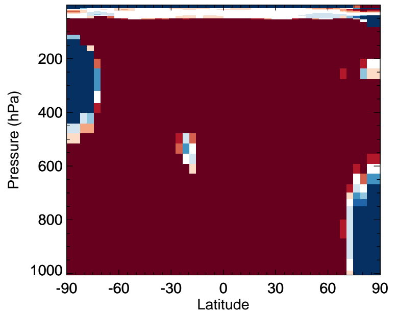
v11-02f-Run0 / v11-02e-Run0 NPMN - Zonal mean % diff for Apr
