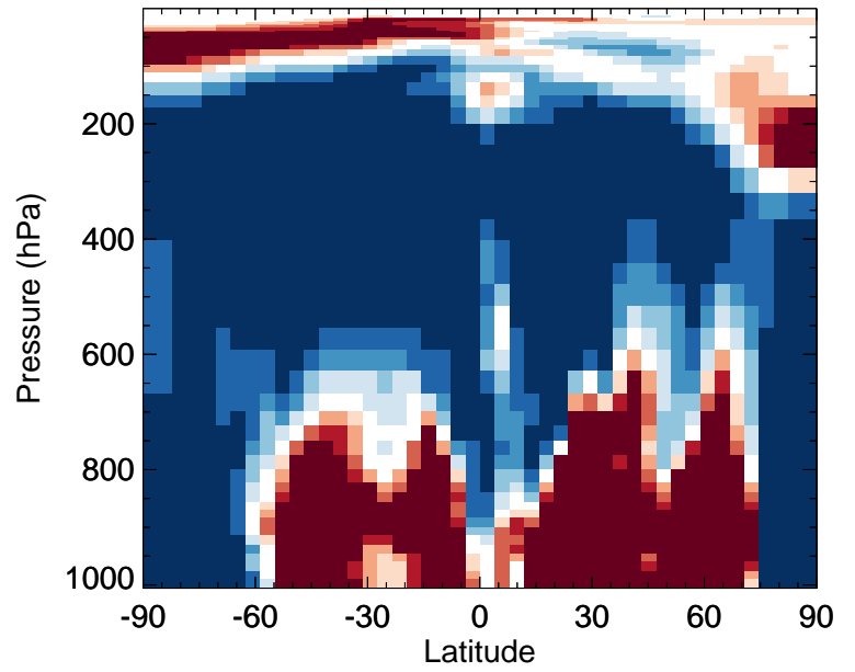
v11-02f-Run0 / v11-02e-Run0 DHDN - Zonal mean % diff for Apr
