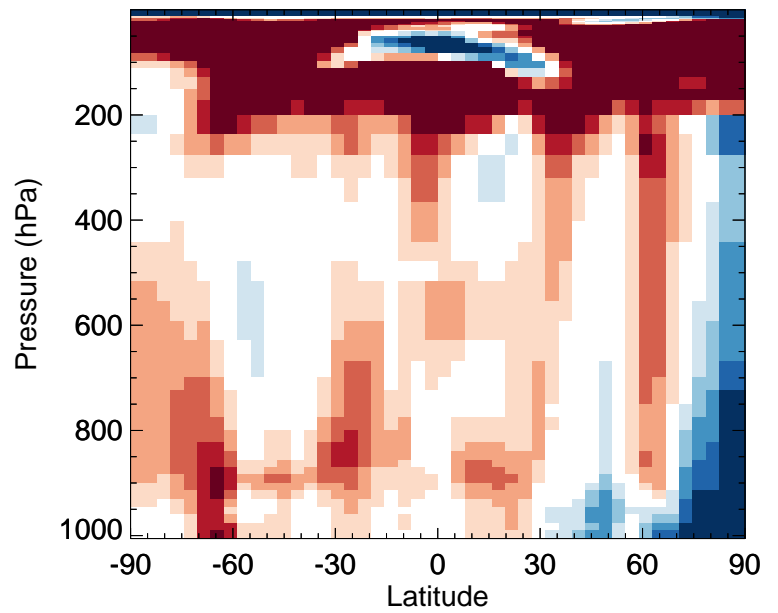
v11-02f-Run0 / v11-02e-Run0 H2O2 - Zonal mean % diff for Apr
