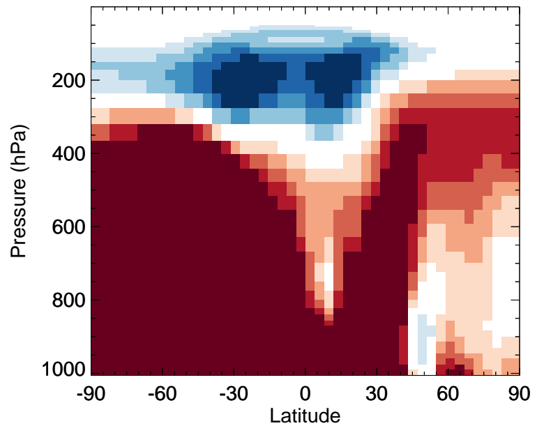
v11-02f-Run0 / v11-02e-Run1 TSOA3 - Zonal mean % diff for Apr
