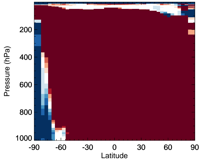
v11-02f-Run0 / v11-02e-Run0 RIPD - Zonal mean % diff for Apr
