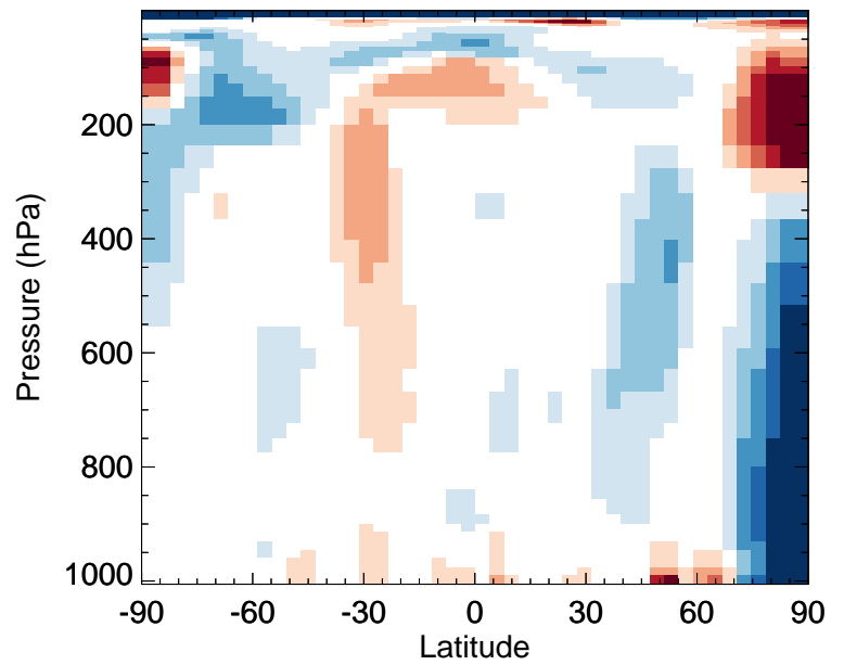
v11-02f-Run0 / v11-02e-Run0 CH 2 O - Zonal mean % diff for Apr
