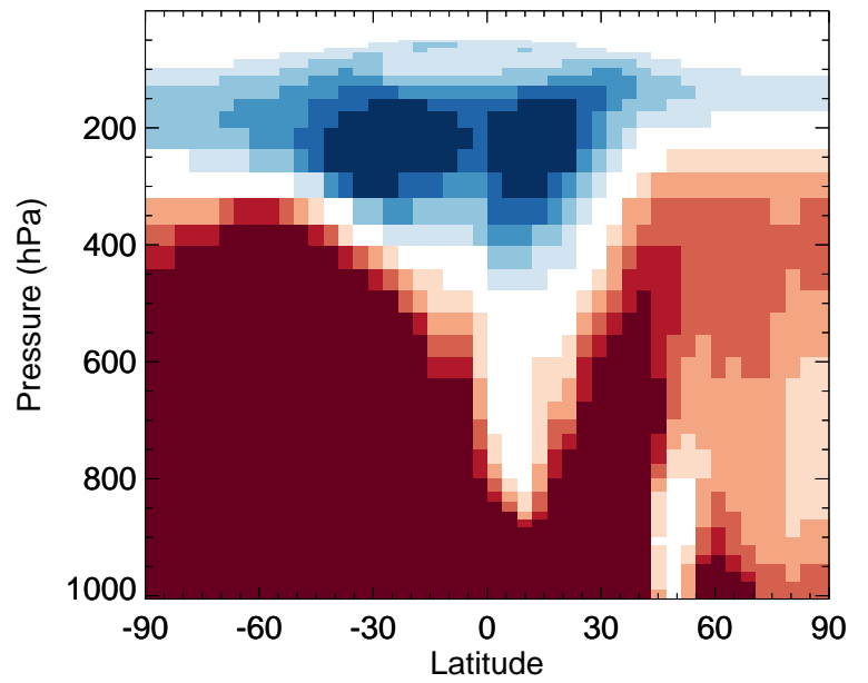
v11-02f-Run0 / v11-02e-Run1 TSOA2 - Zonal mean % diff for Apr
