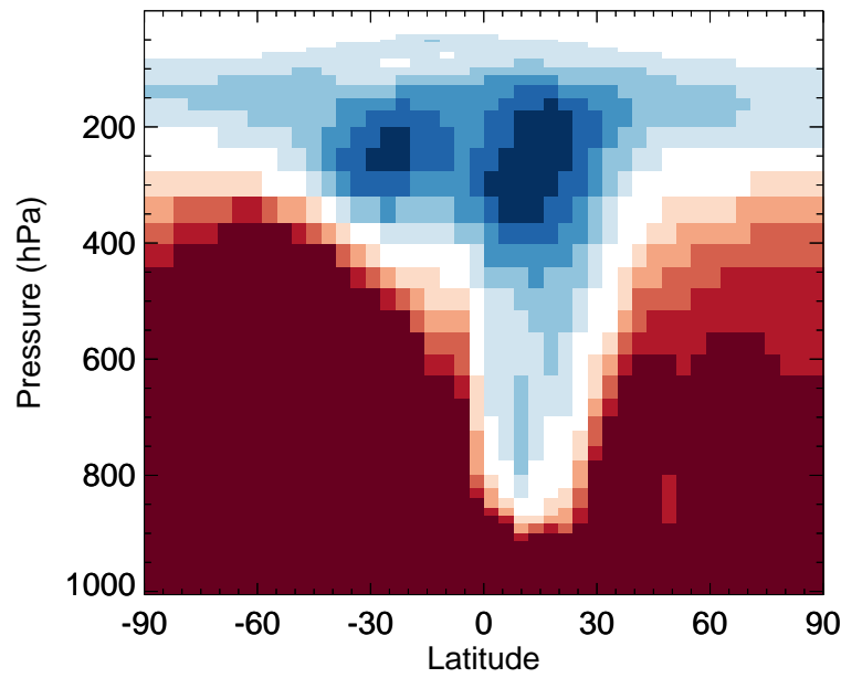
v11-02f-Run0 / v11-02e-Run1 TSOA1 - Zonal mean % diff for Apr
