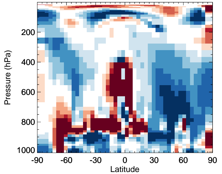
v11-02f-Run0 / v11-02e-Run0 HOBr - Zonal mean % diff for Apr
