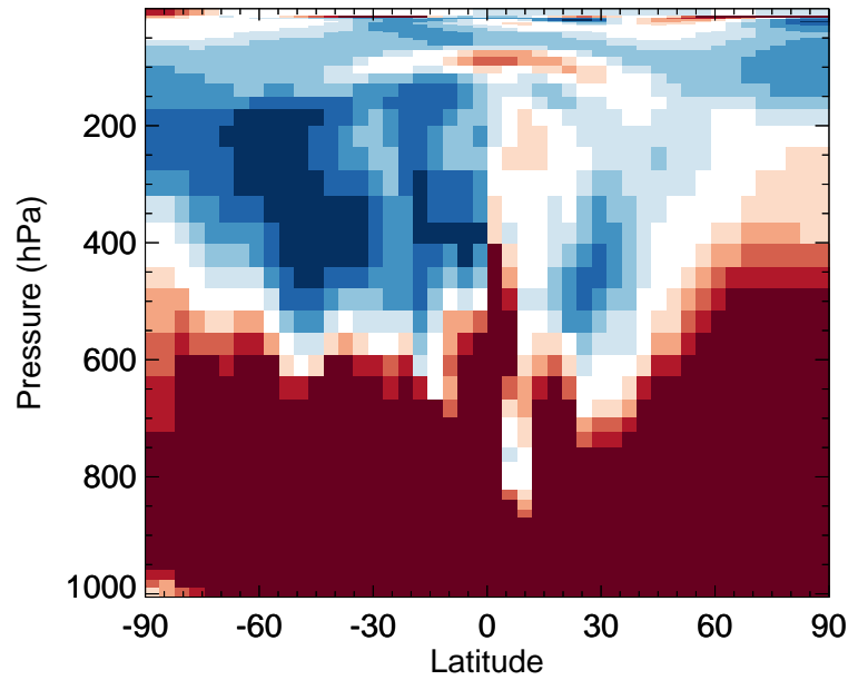
v11-02f-Run0 / v11-02e-Run0 TSOA0 - Zonal mean % diff for Apr
