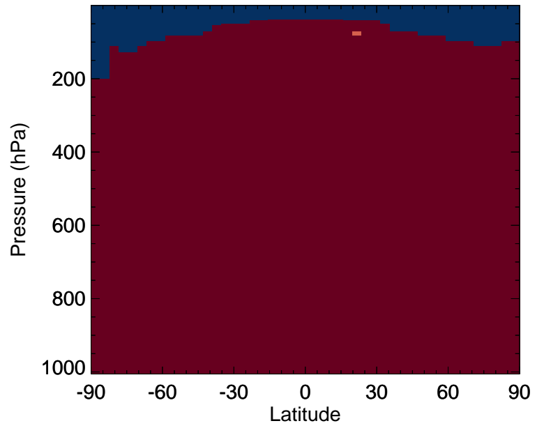
v11-02f-Run0 / v11-02e-Run1 NIT - Zonal mean % diff for Apr
