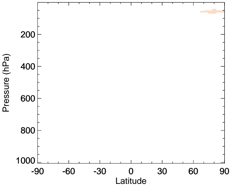
v11-02f-Run0 - v11-02e-Run0 BrO - Zonal mean abs diff for Apr
