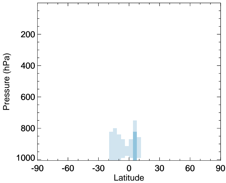
v11-02f-Run0 - v11-02e-Run1 RIPA - Zonal mean abs diff for Apr
