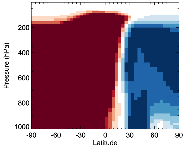
v11-02f-Run0 / v11-02e-Run1 ASOAN - Zonal mean % diff for Apr
