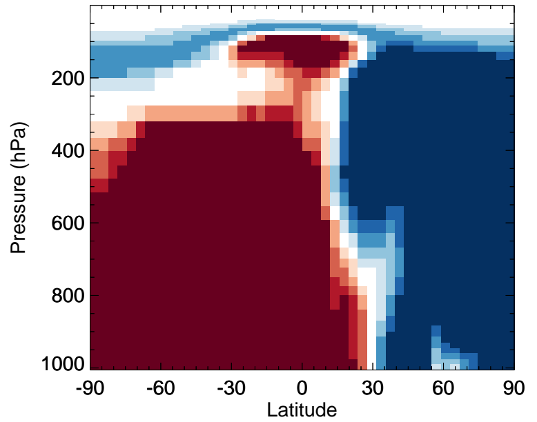
v11-02f-Run0 / v11-02e-Run1 ASOA2 - Zonal mean % diff for Apr
