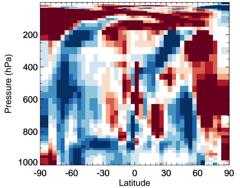
v11-02f-Run0 / v11-02e-Run0 Br2 - Zonal mean % diff for Apr
