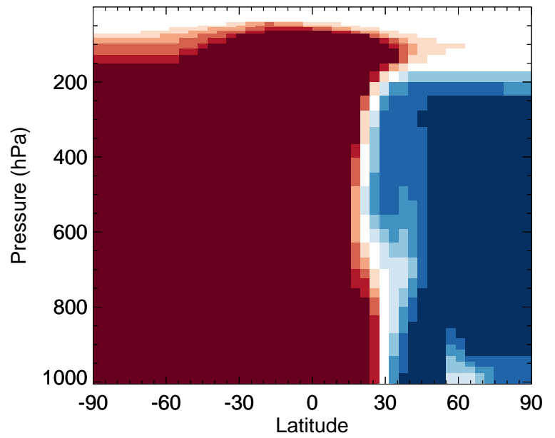
v11-02f-Run0 / v11-02e-Run1 ASOA1 - Zonal mean % diff for Apr
