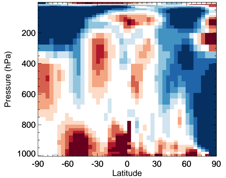
v11-02f-Run0 / v11-02e-Run0 NO 2 - Zonal mean % diff for Apr
