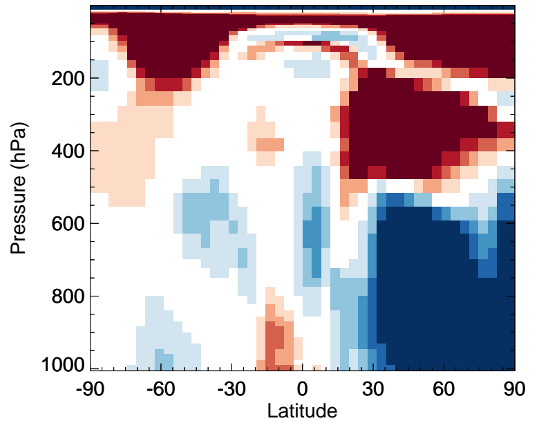
v11-02f-Run0 / v11-02e-Run1 HOCl - Zonal mean % diff for Apr
