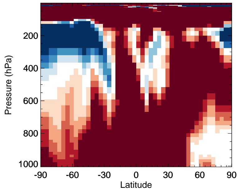
v11-02f-Run0 / v11-02e-Run0 EOH - Zonal mean % diff for Apr
