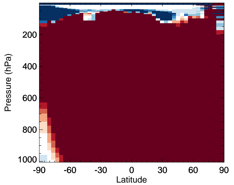
v11-02f-Run0 / v11-02e-Run1 ISOP - Zonal mean % diff for Apr
