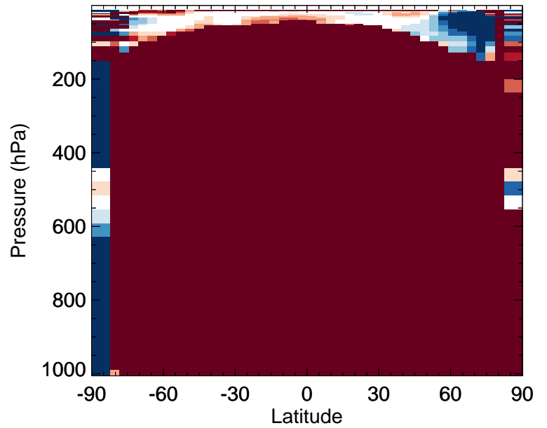
v11-02f-Run0 / v11-02e-Run0 LIMO - Zonal mean % diff for Apr
