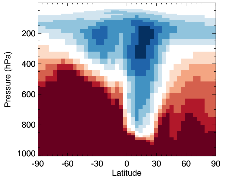
v11-02f-Run0 / v11-02e-Run1 TSOA0 - Zonal mean % diff for Apr
