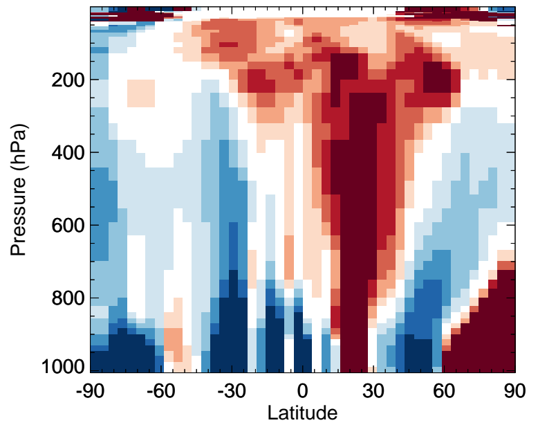
v11-02f-Run0 / v11-02e-Run1 BCPO - Zonal mean % diff for Apr
