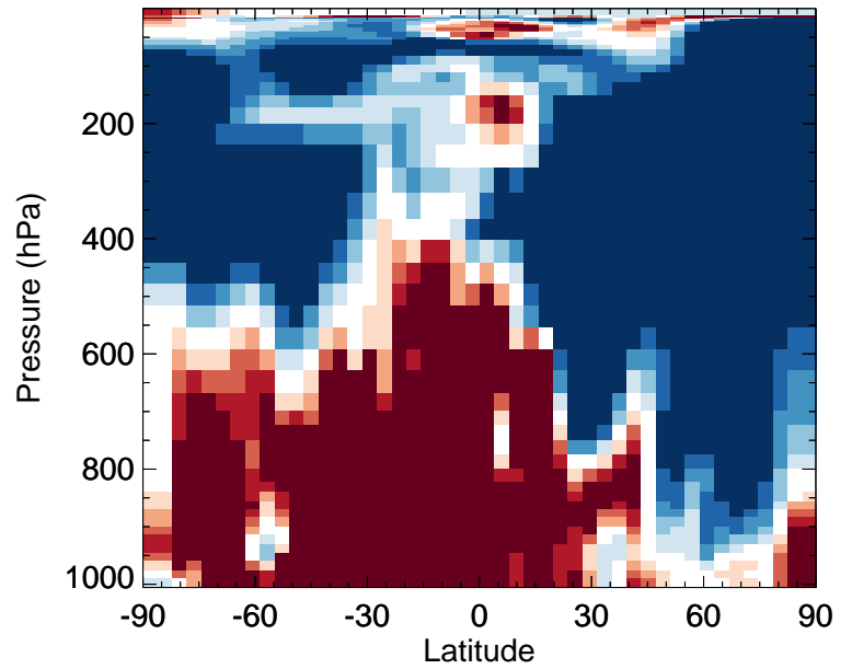
v11-02f-Run0 / v11-02e-Run0 ASOA2 - Zonal mean % diff for Apr
