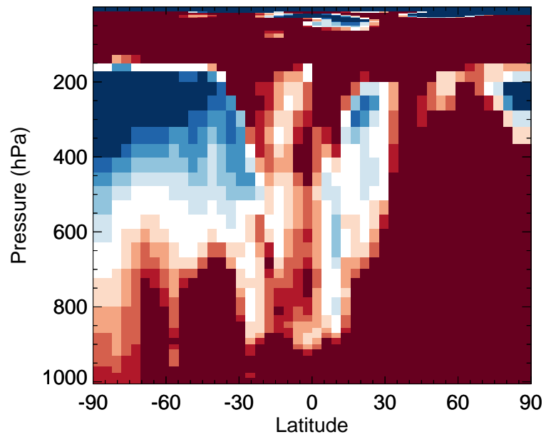
v11-02f-Run0 / v11-02e-Run0 HAC - Zonal mean % diff for Apr
