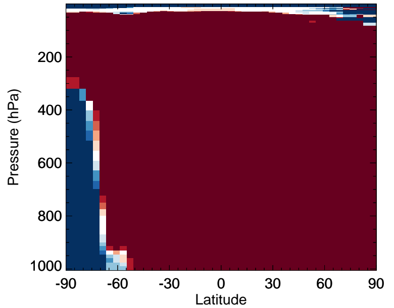
v11-02f-Run0 / v11-02e-Run0 LVOC - Zonal mean % diff for Apr
