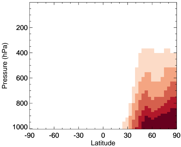
v11-02f-Run0 - v11-02e-Run0 C3H8 - Zonal mean abs diff for Apr
