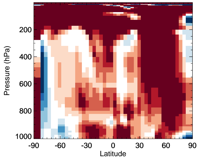
v11-02f-Run0 / v11-02e-Run0 ACTA - Zonal mean % diff for Apr
