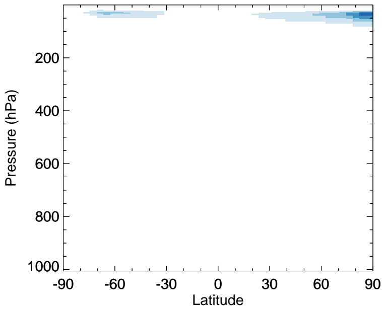
v11-02f-Run0 - v11-02e-Run1 NO - Zonal mean abs diff for Apr
