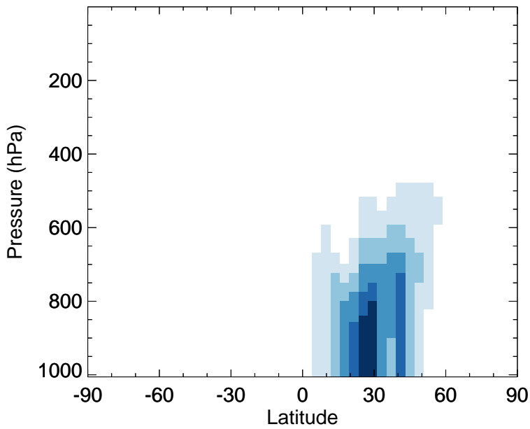
v11-02f-Run0 - v11-02e-Run0 DST1 - Zonal mean abs diff for Apr
