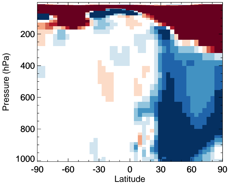
v11-02f-Run0 - v11-02e-Run0 HNO 3 - Zonal mean abs diff for Apr
