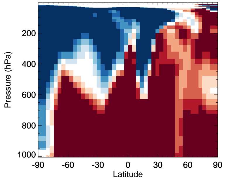
v11-02f-Run0 / v11-02e-Run1 MVKN - Zonal mean % diff for Apr
