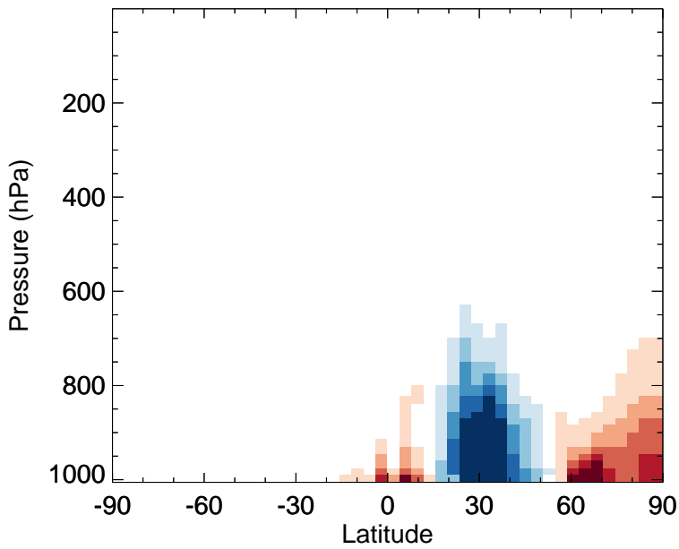
v11-02f-Run0 - v11-02e-Run0 TOLU - Zonal mean abs diff for Apr
