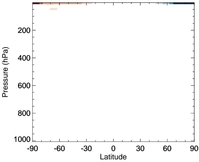
v11-02f-Run0 - v11-02e-Run1 ClO - Zonal mean abs diff for Apr
