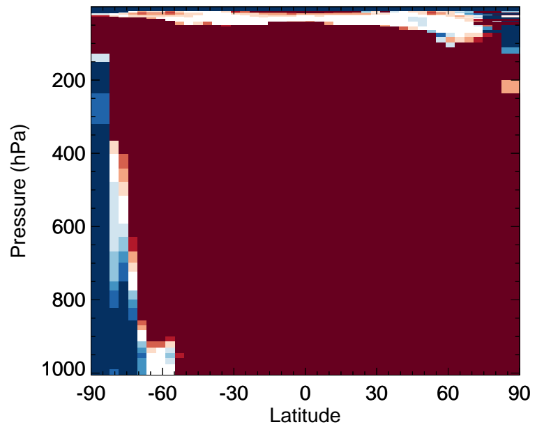
v11-02f-Run0 / v11-02e-Run0 RIPB - Zonal mean % diff for Apr
