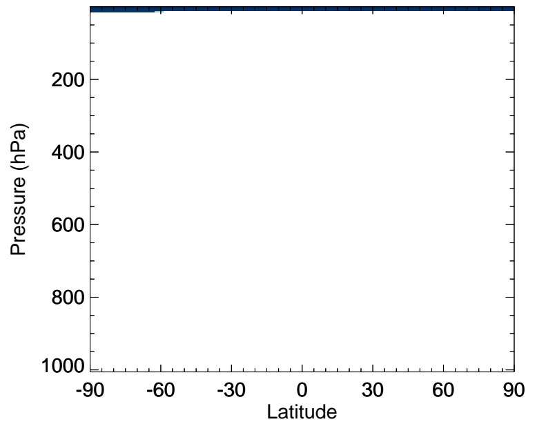
v11-02f-Run0 / v11-02e-Run1 CH3Cl - Zonal mean % diff for Apr
