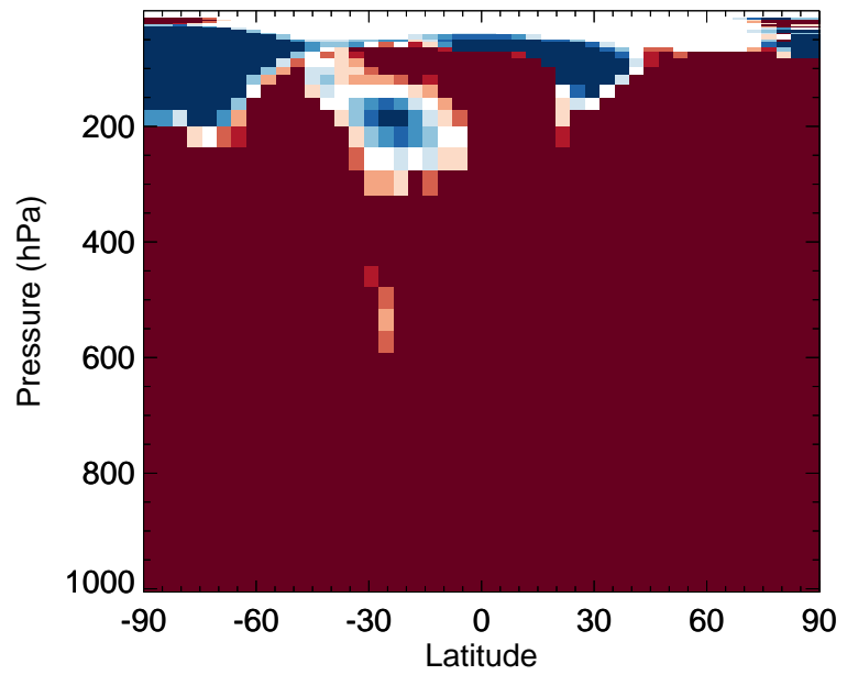
v11-02f-Run0 / v11-02e-Run1 ETHLN - Zonal mean % diff for Apr
