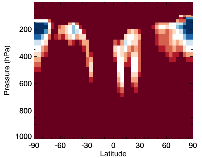
v11-02f-Run0 / v11-02e-Run0 MEK - Zonal mean % diff for Apr
