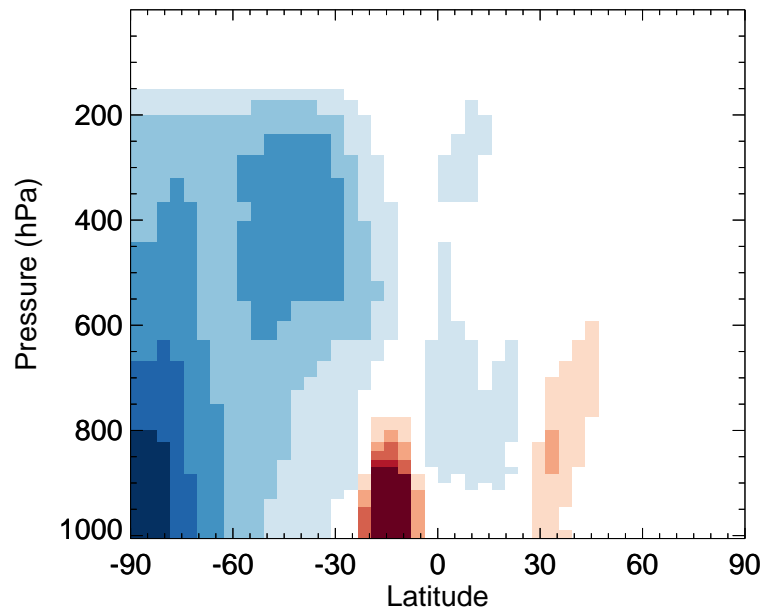
v11-02f-Run0 / v11-02e-Run1 SOAS - Zonal mean % diff for Apr
