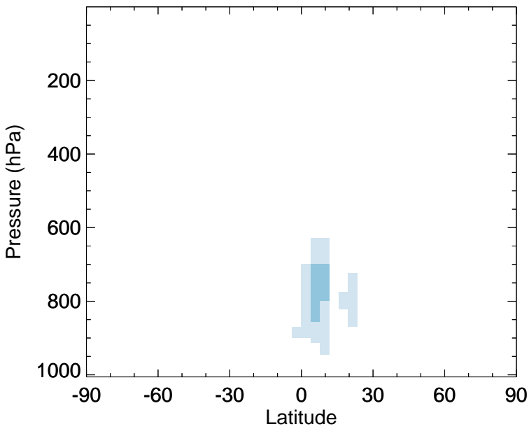
v11-02f-Run0 - v11-02e-Run0 HAC - Zonal mean abs diff for Apr
