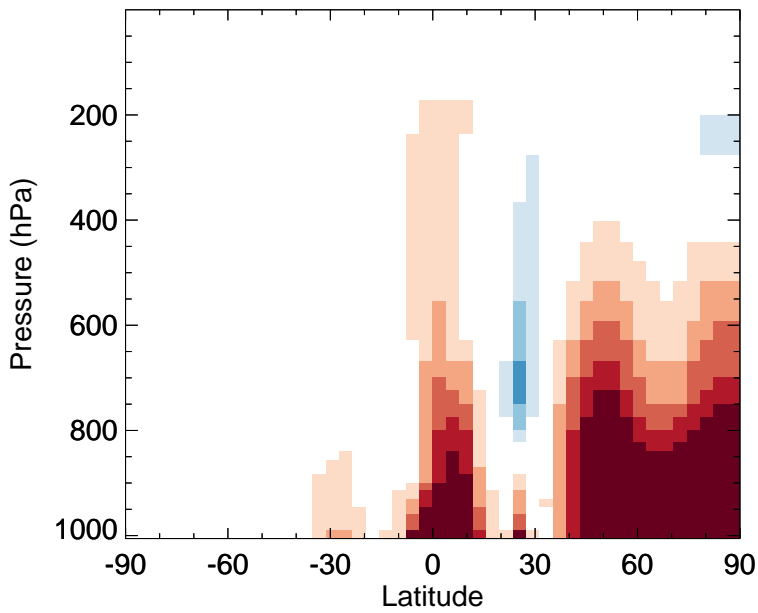
v11-02f-Run0 - v11-02e-Run0 BENZ - Zonal mean abs diff for Apr
