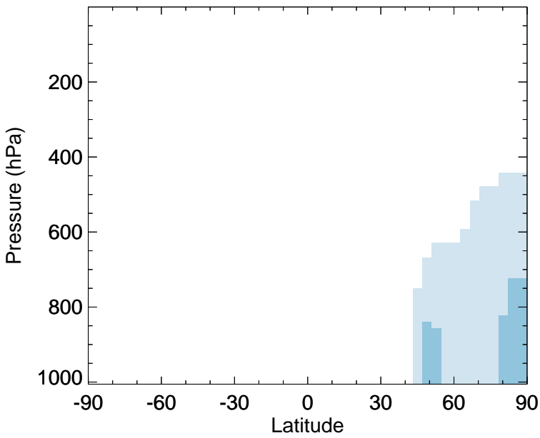
v11-02f-Run0 - v11-02e-Run1 PAN - Zonal mean abs diff for Apr
