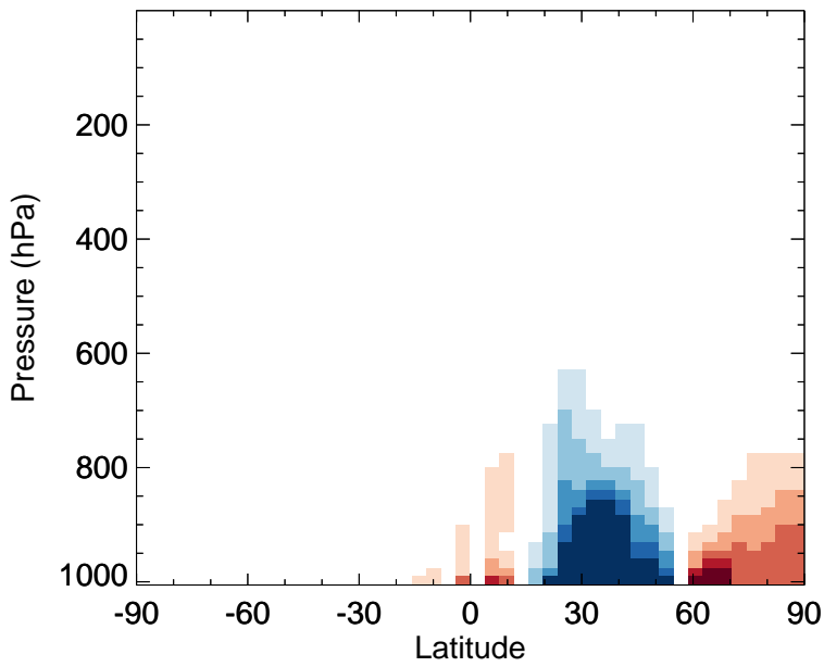
v11-02f-Run0 - v11-02e-Run1 TOLU - Zonal mean abs diff for Apr
