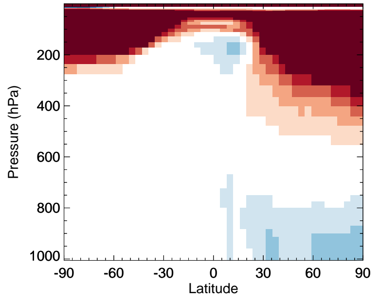
v11-02f-Run0 / v11-02e-Run1 MP - Zonal mean % diff for Apr
