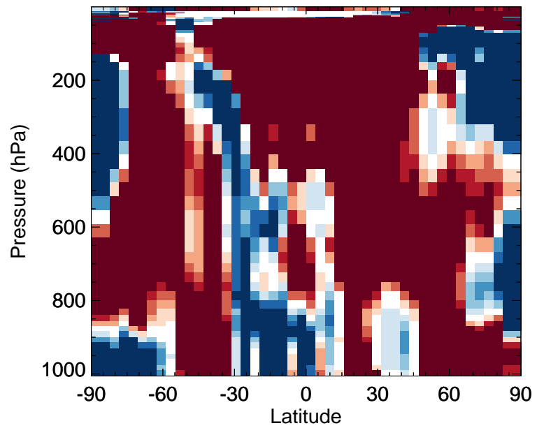
v11-02f-Run0 / v11-02e-Run0 BCPO - Zonal mean % diff for Apr
