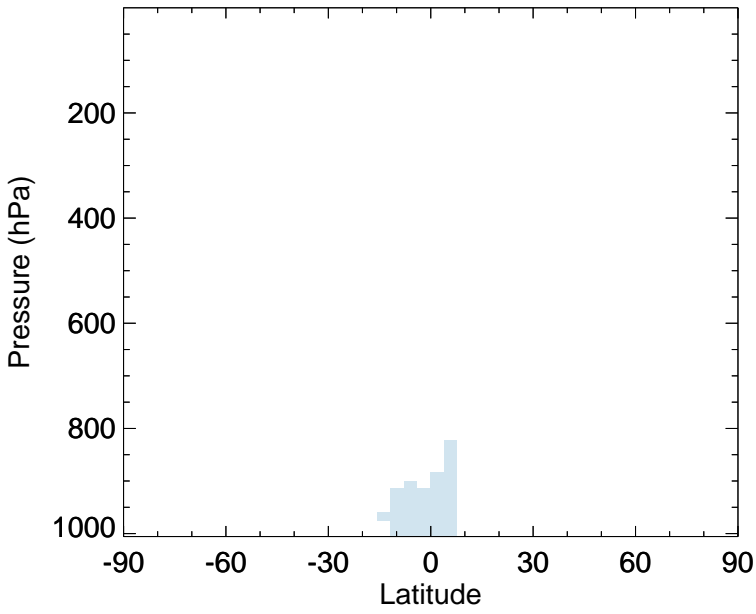
v11-02f-Run0 - v11-02e-Run1 HPALD - Zonal mean abs diff for Apr
