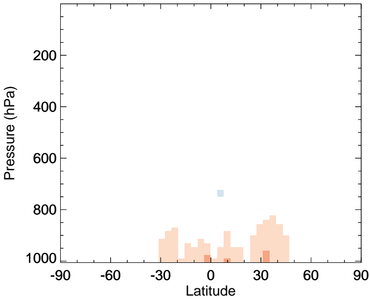
v11-02f-Run0 - v11-02e-Run0 INDIOL - Zonal mean abs diff for Apr
