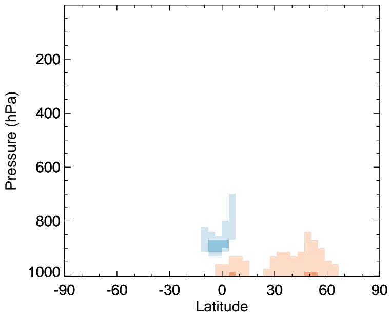
v11-02f-Run0 - v11-02e-Run0 ALD2 - Zonal mean abs diff for Apr
