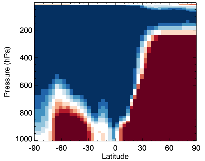
v11-02f-Run0 / v11-02e-Run1 IMAE - Zonal mean % diff for Apr
