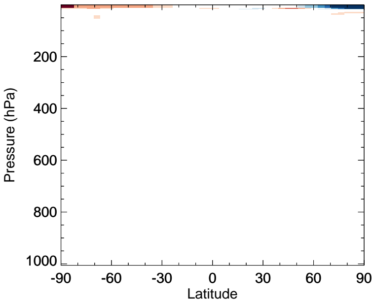
v11-02f-Run0 - v11-02e-Run0 ClO - Zonal mean abs diff for Apr
