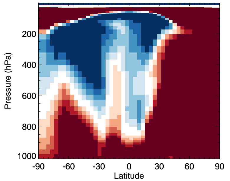
v11-02f-Run0 / v11-02e-Run1 HAC - Zonal mean % diff for Apr
