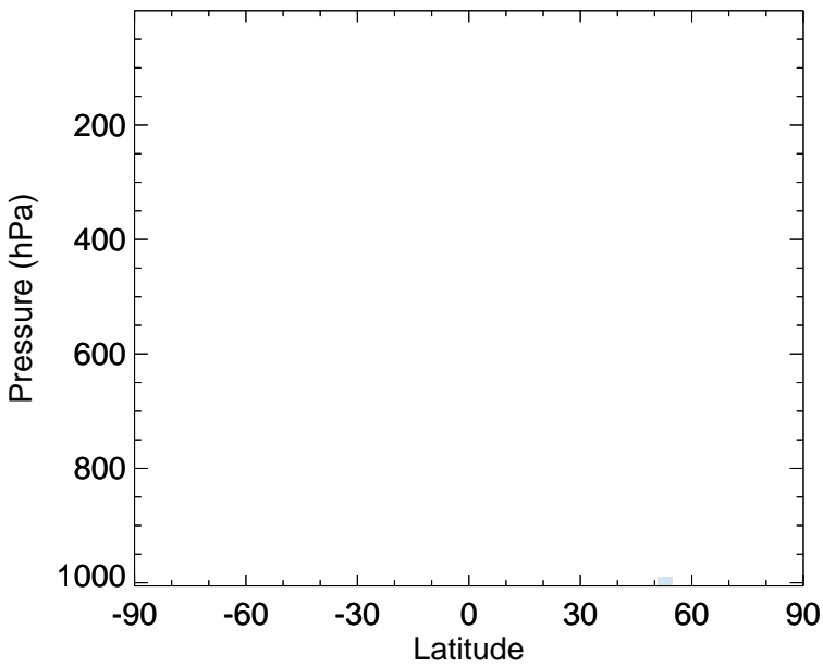
v11-02f-Run0 - v11-02e-Run0 SO2 - Zonal mean abs diff for Apr
