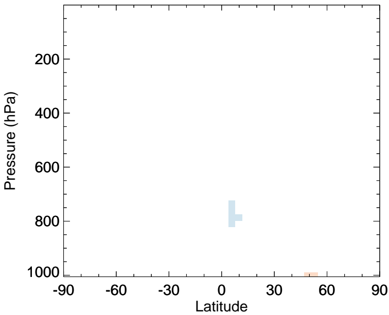
v11-02f-Run0 - v11-02e-Run0 CH 2 O - Zonal mean abs diff for Apr
