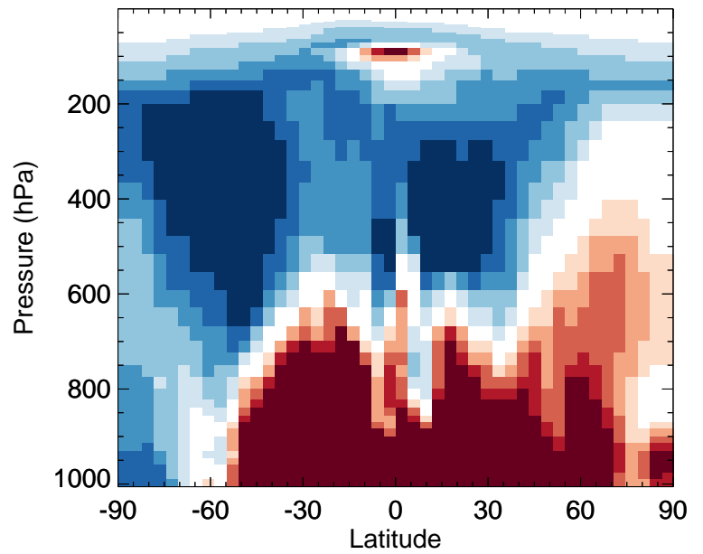
v11-02f-Run0 / v11-02e-Run0 TSOG3 - Zonal mean % diff for Apr
