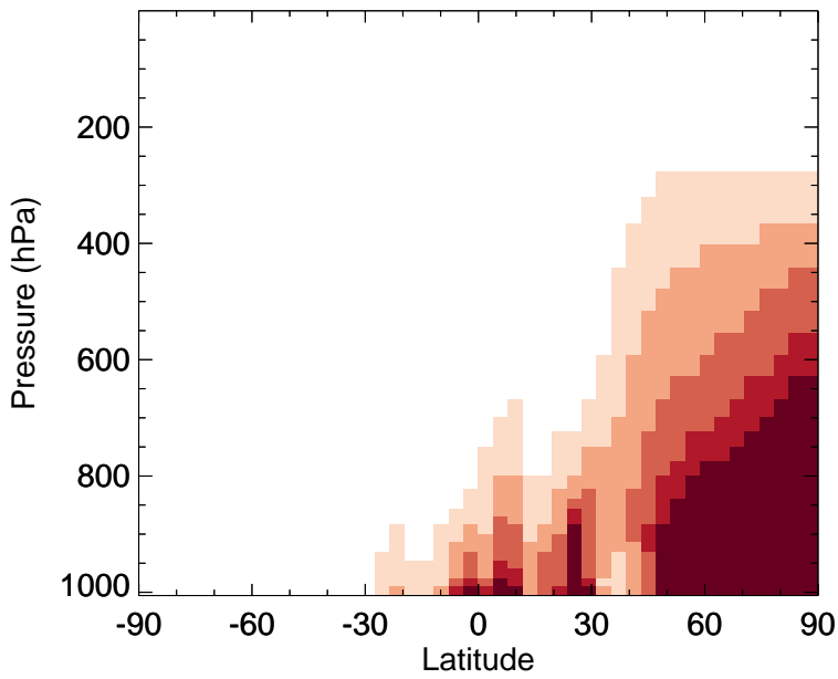
v11-02f-Run0 - v11-02e-Run1 ALK4 - Zonal mean abs diff for Apr
