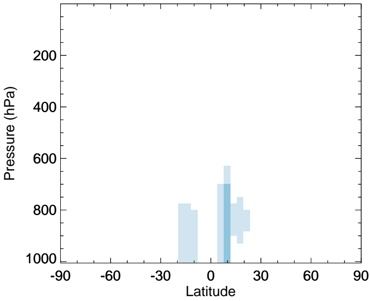
v11-02f-Run0 - v11-02e-Run1 GLYC - Zonal mean abs diff for Apr
