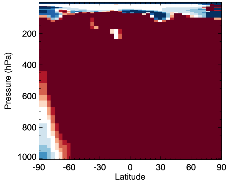
v11-02f-Run0 / v11-02e-Run1 RIPD - Zonal mean % diff for Apr
