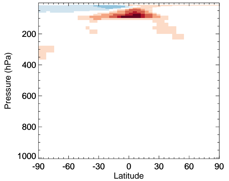
v11-02f-Run0 / v11-02e-Run1 SALC - Zonal mean % diff for Apr
