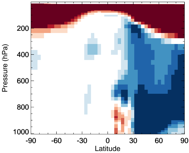
v11-02f-Run0 - v11-02e-Run1 HNO 3 - Zonal mean abs diff for Apr
