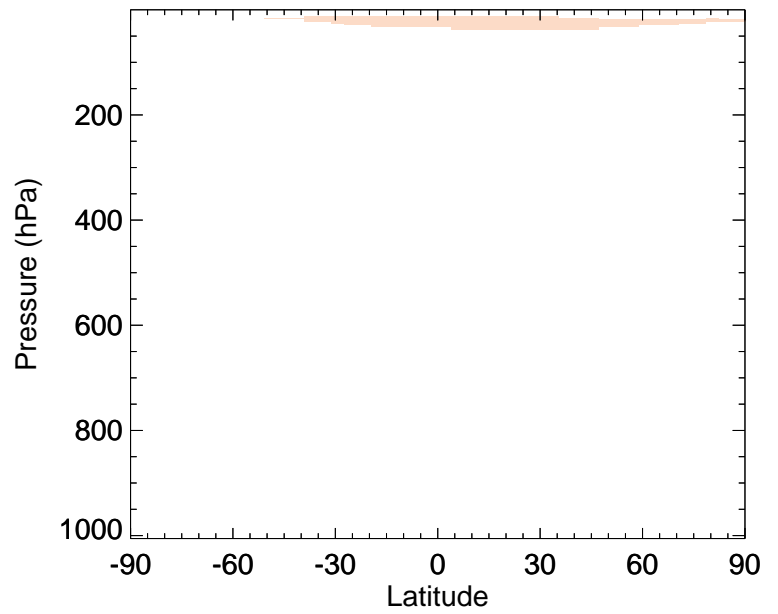
v11-02f-Run0 / v11-02e-Run1 CH 2 Br 2 - Zonal mean % diff for Apr
