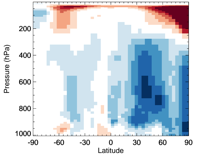
v11-02f-Run0 / v11-02e-Run1 HOBr - Zonal mean % diff for Apr
