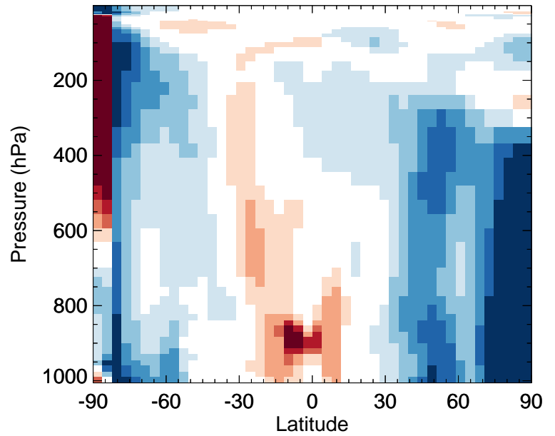
v11-02f-Run0 / v11-02e-Run0 OH - Zonal mean % diff for Apr
