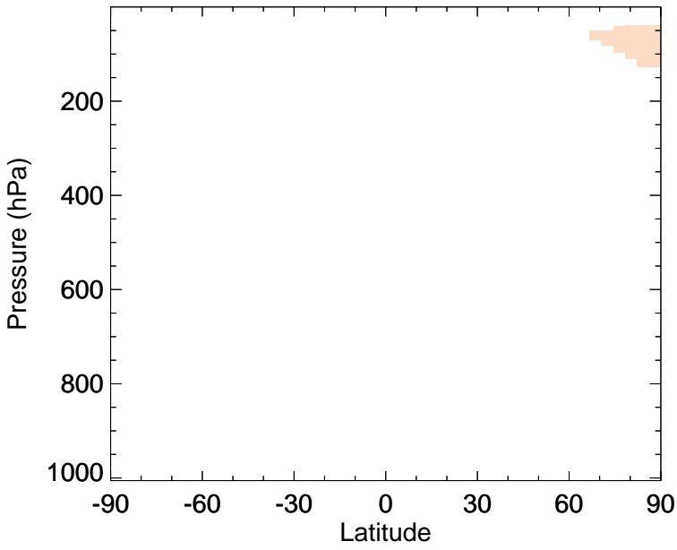
v11-02f-Run0 - v11-02e-Run1 BrO - Zonal mean abs diff for Apr
