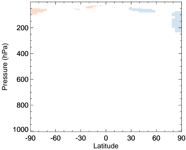
v11-02f-Run0 - v11-02e-Run0 CFC11 - Zonal mean abs diff for Apr
