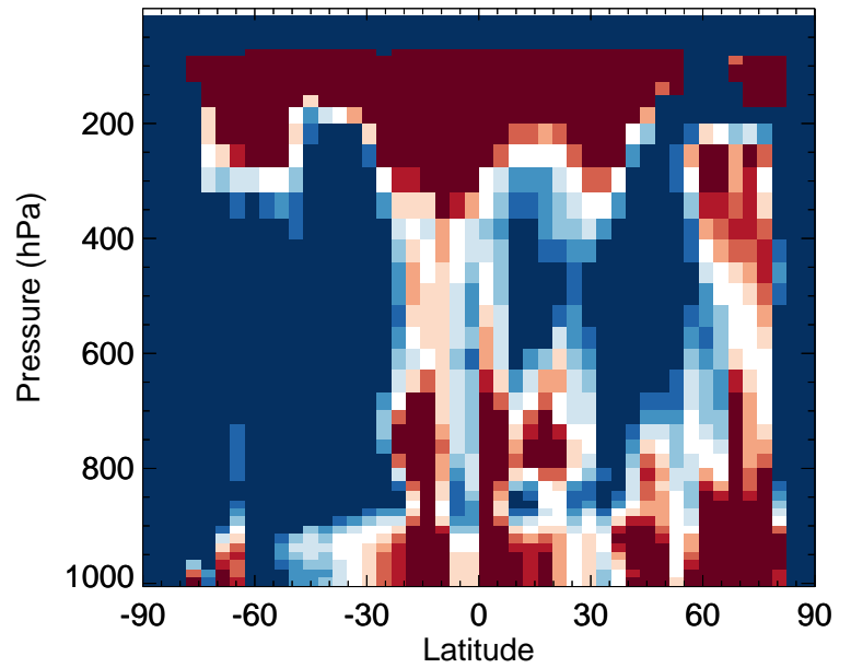
v11-02f-Run0 / v11-02e-Run0 SO4s - Zonal mean % diff for Apr
