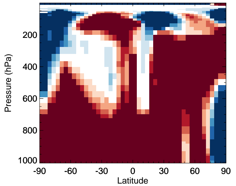
v11-02f-Run0 / v11-02e-Run1 NPMN - Zonal mean % diff for Apr
