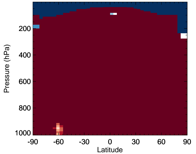
v11-02f-Run0 / v11-02e-Run0 NIT - Zonal mean % diff for Apr
