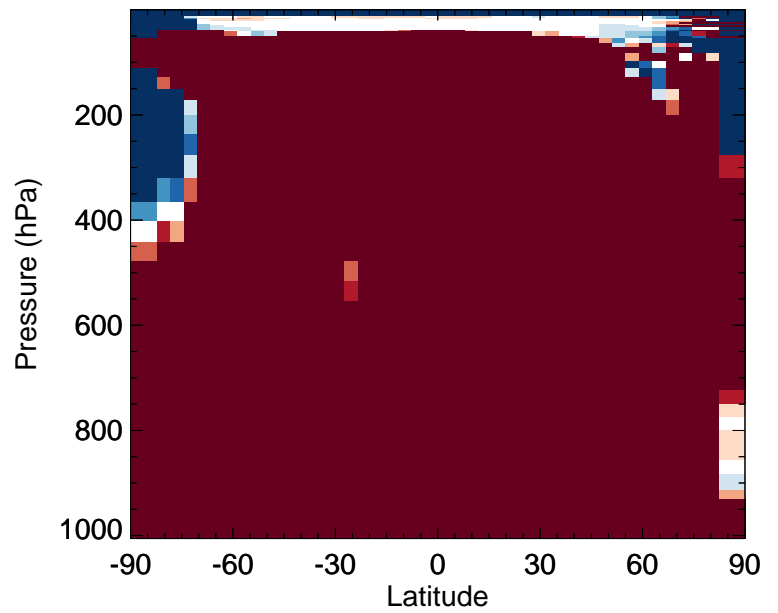
v11-02f-Run0 / v11-02e-Run0 ISN1 - Zonal mean % diff for Apr
