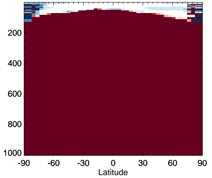
v11-02f-Run0 / v11-02e-Run1 MTPA - Zonal mean % diff for Apr
