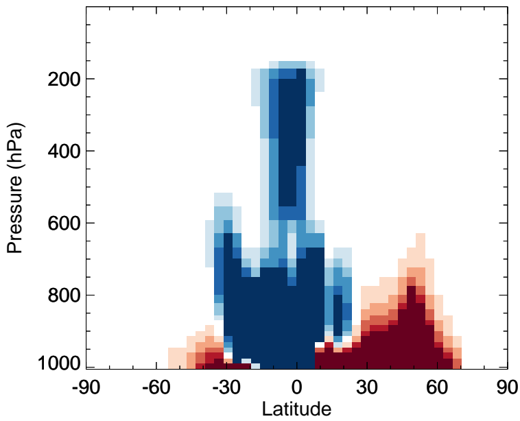
v11-02f-Run0 - v11-02e-Run1 PRPE - Zonal mean abs diff for Apr
