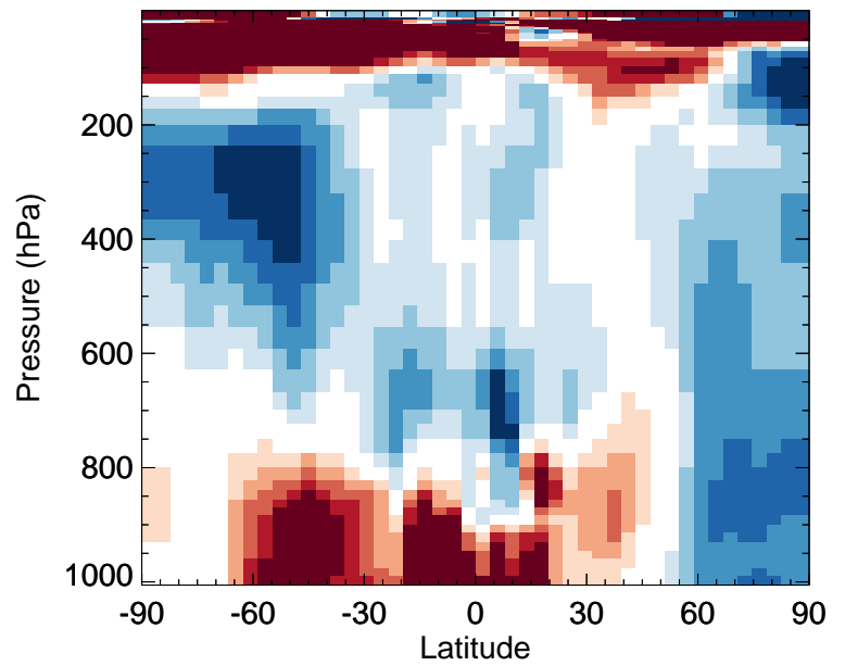
v11-02f-Run0 / v11-02e-Run0 PAN - Zonal mean % diff for Apr
