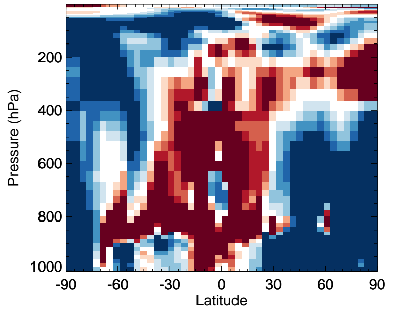
v11-02f-Run0 / v11-02e-Run0 CINO3 - Zonal mean % diff for Apr
