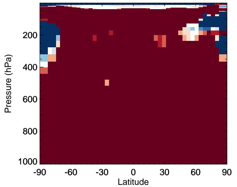
v11-02f-Run0 / v11-02e-Run0 MACR - Zonal mean % diff for Apr
