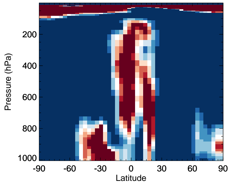
v11-02f-Run0 / v11-02e-Run0 DST1 - Zonal mean % diff for Apr
