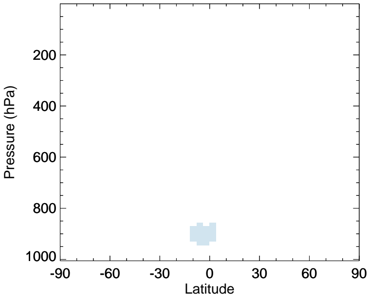
v11-02f-Run0 - v11-02e-Run0 HPALD - Zonal mean abs diff for Apr
