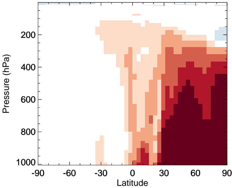
v11-02f-Run0 - v11-02e-Run0 CO - Zonal mean abs diff for Apr
