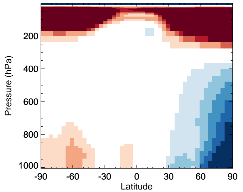
v11-02f-Run0 / v11-02e-Run1 H2O2 - Zonal mean % diff for Apr
