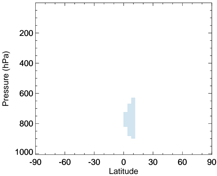
v11-02f-Run0 - v11-02e-Run0 IMAE - Zonal mean abs diff for Apr
