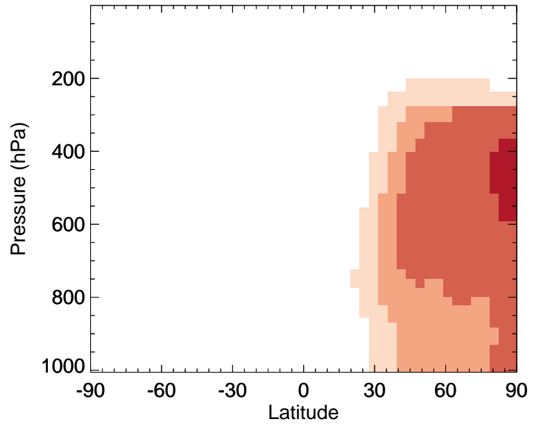
v11-02f-Run0 / v11-02e-Run1 MSA - Zonal mean % diff for Apr
