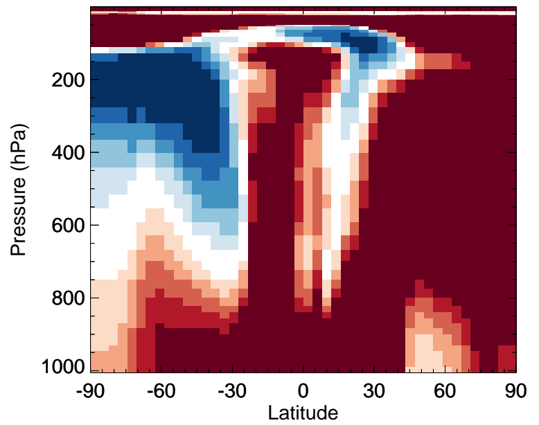
v11-02f-Run0 / v11-02e-Run1 EOH - Zonal mean % diff for Apr
