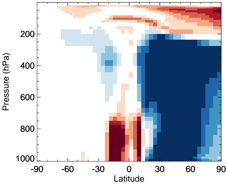
v11-02f-Run0 - v11-02e-Run1 OH - Zonal mean abs diff for Apr
