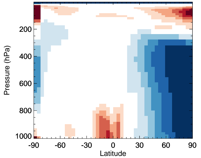
v11-02f-Run0 / v11-02e-Run1 OH - Zonal mean % diff for Apr
