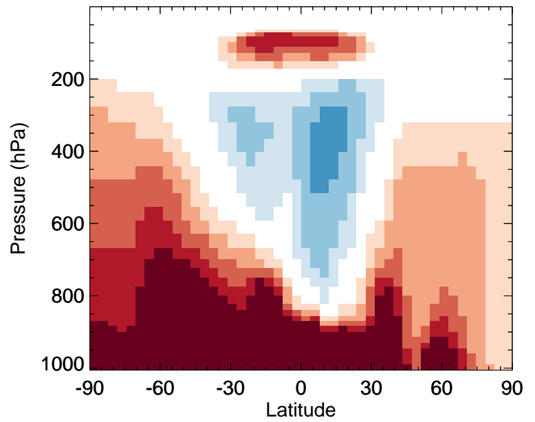
v11-02f-Run0 / v11-02e-Run1 TSOG2 - Zonal mean % diff for Apr
