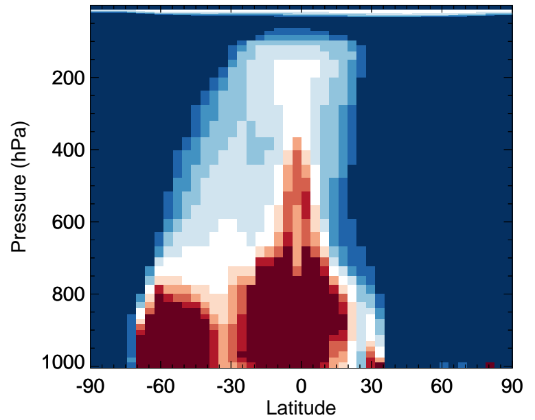
v11-02f-Run0 / v11-02e-Run1 N2O5 - Zonal mean % diff for Apr
