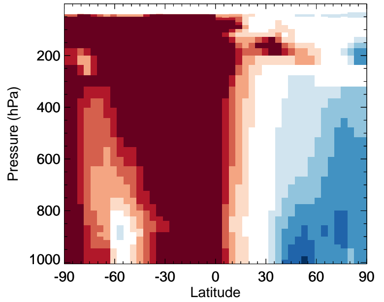
v11-02f-Run0 / v11-02e-Run1 NITs - Zonal mean % diff for Apr
