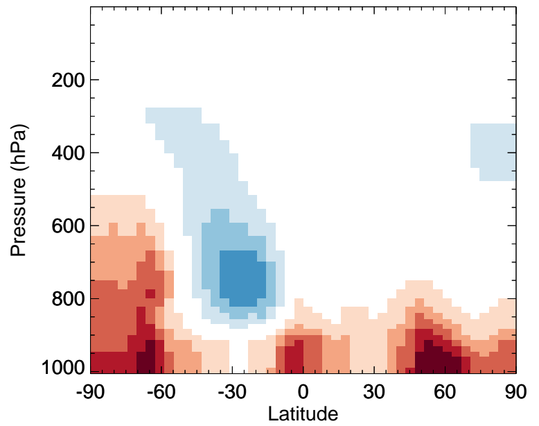
v11-02f-Run0 / v11-02e-Run1 SO4 - Zonal mean % diff for Apr
