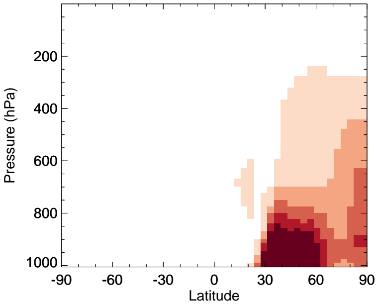
v11-02f-Run0 - v11-02e-Run0 NH4 - Zonal mean abs diff for Apr
