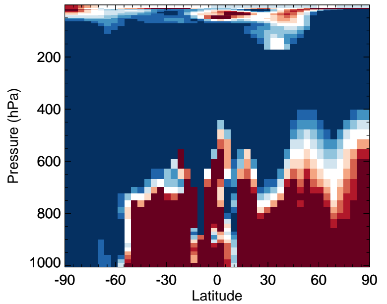
v11-02f-Run0 / v11-02e-Run0 ISOA3 - Zonal mean % diff for Apr
