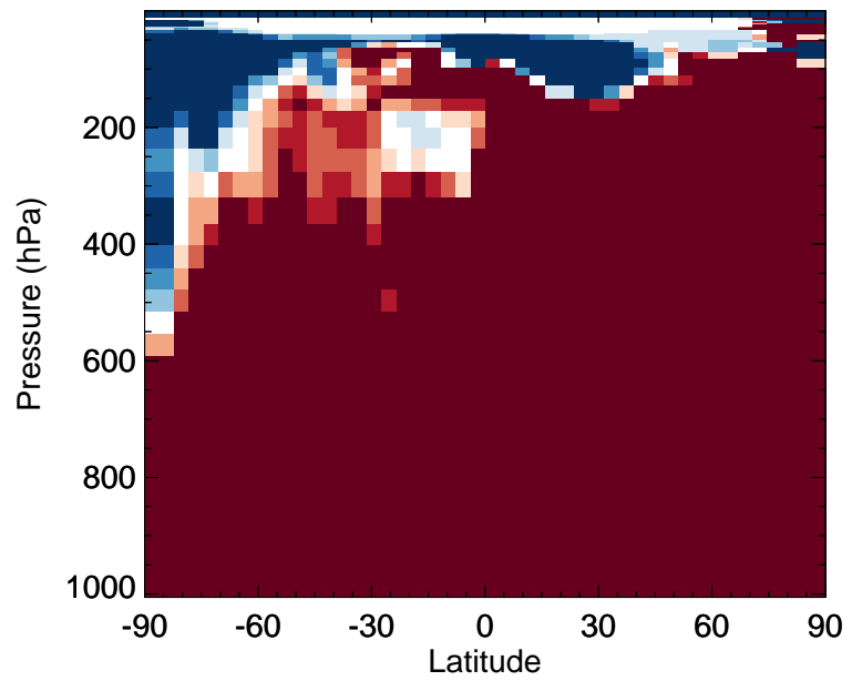
v11-02f-Run0 / v11-02e-Run1 ISN1 - Zonal mean % diff for Apr
