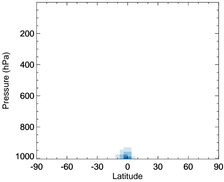
v11-02f-Run0 - v11-02e-Run1 MTPA - Zonal mean abs diff for Apr
