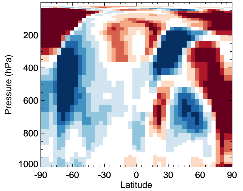
v11-02f-Run0 / v11-02e-Run1 Br2 - Zonal mean % diff for Apr
