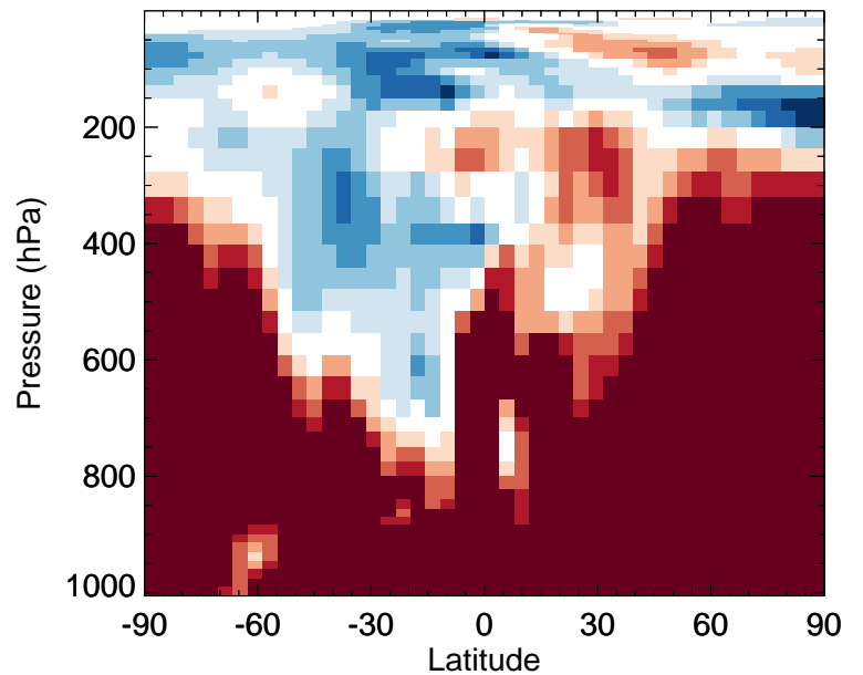
v11-02f-Run0 / v11-02e-Run0 OCPI - Zonal mean % diff for Apr
