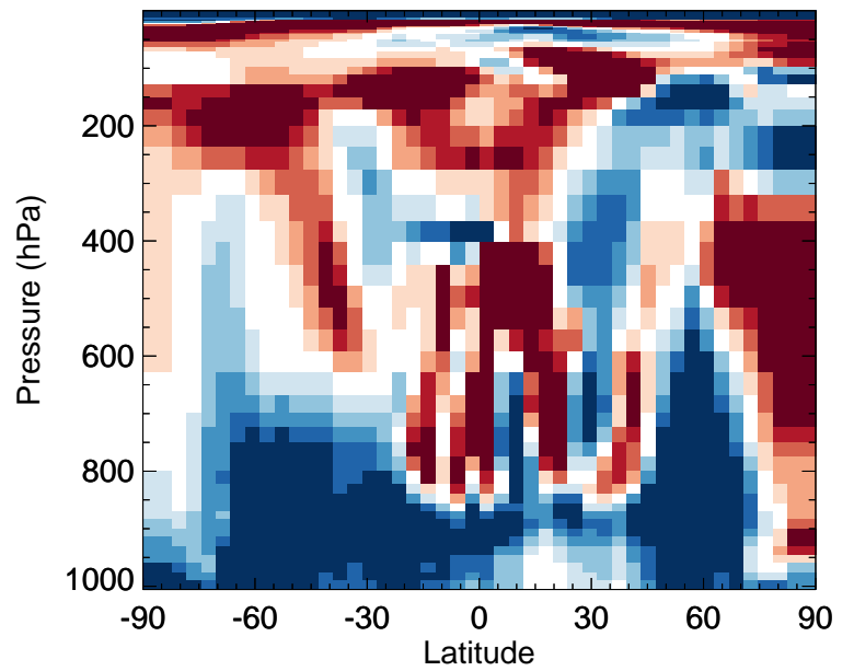
v11-02f-Run0 / v11-02e-Run0 SO2 - Zonal mean % diff for Apr
