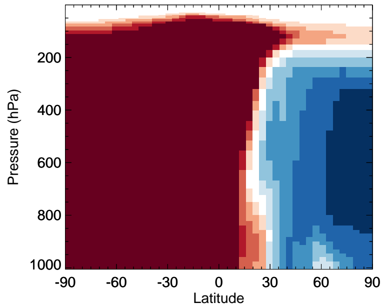
v11-02f-Run0 / v11-02e-Run1 ASOG3 - Zonal mean % diff for Apr
