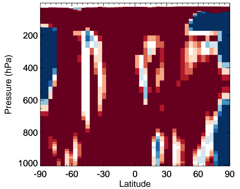
v11-02f-Run0 / v11-02e-Run0 SOAP - Zonal mean % diff for Apr
