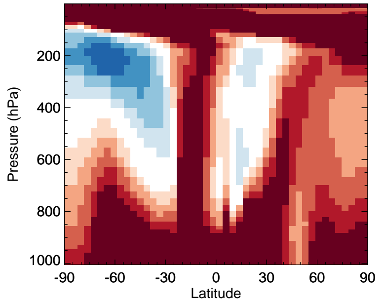
v11-02f-Run0 / v11-02e-Run1 MEK - Zonal mean % diff for Apr
