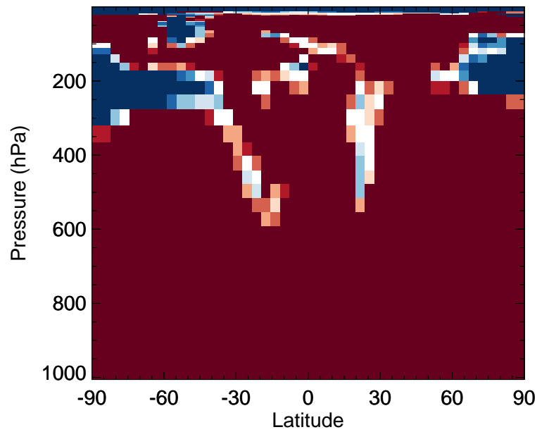
v11-02f-Run0 / v11-02e-Run0 IEPOXB - Zonal mean % diff for Apr
