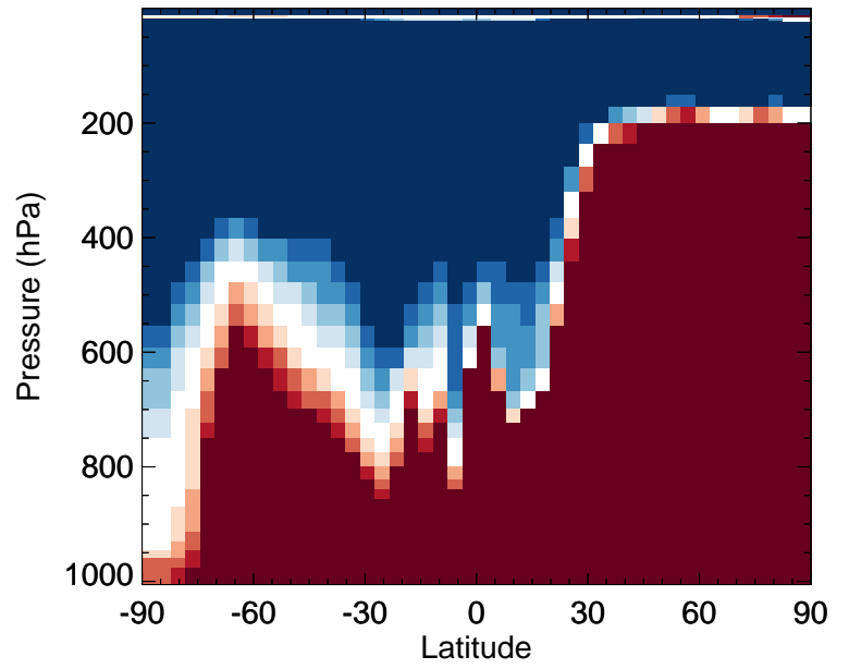
v11-02f-Run0 / v11-02e-Run1 GLYC - Zonal mean % diff for Apr
