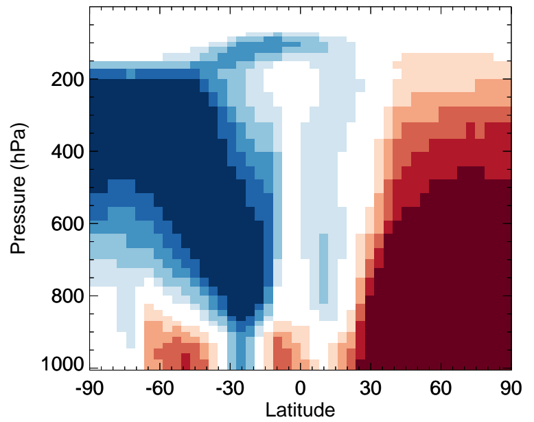
v11-02f-Run0 / v11-02e-Run1 SOAMG - Zonal mean % diff for Apr
