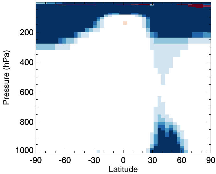
v11-02f-Run0 - v11-02e-Run0 N2O5 - Zonal mean abs diff for Apr
