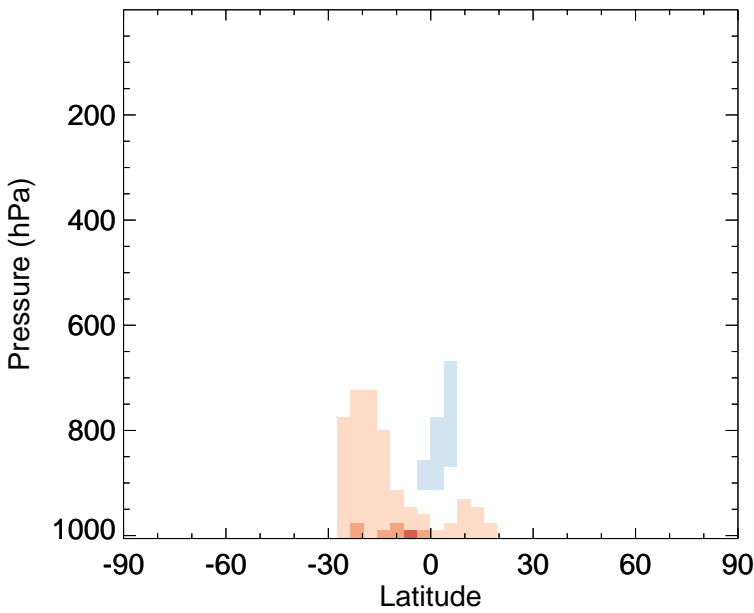
v11-02f-Run0 - v11-02e-Run0 TSOG3 - Zonal mean abs diff for Apr
