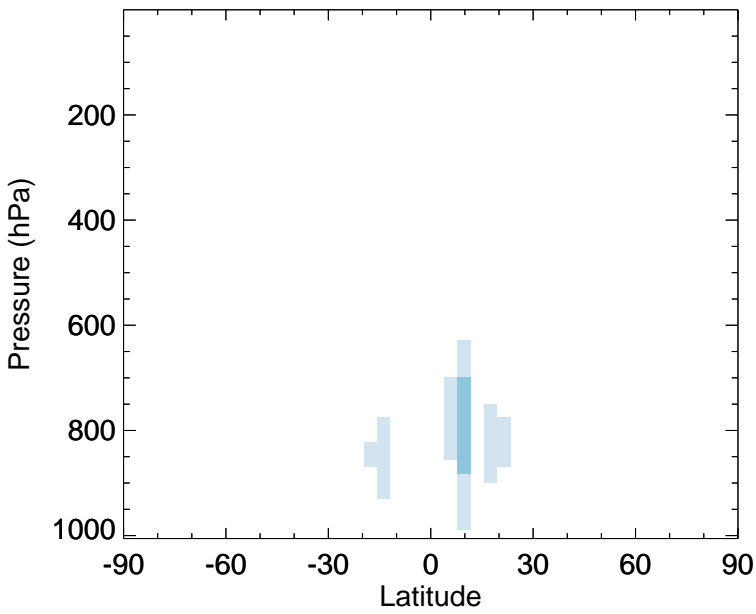
v11-02f-Run0 - v11-02e-Run1 HAC - Zonal mean abs diff for Apr
