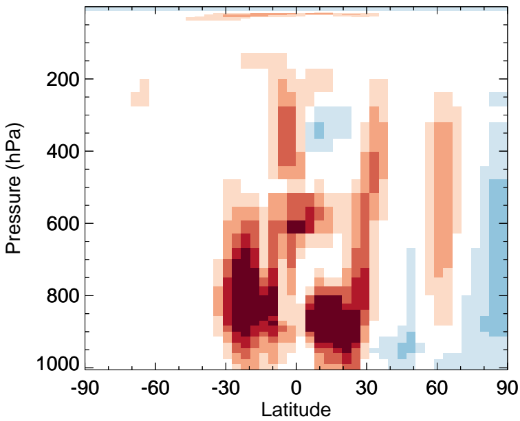
v11-02f-Run0 - v11-02e-Run0 H2O2 - Zonal mean abs diff for Apr
