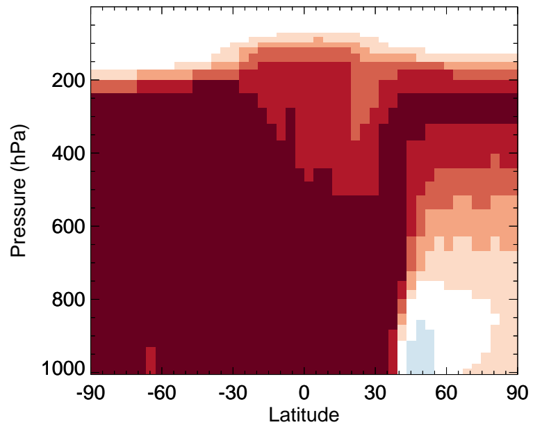
v11-02f-Run0 / v11-02e-Run1 OCPI - Zonal mean % diff for Apr
