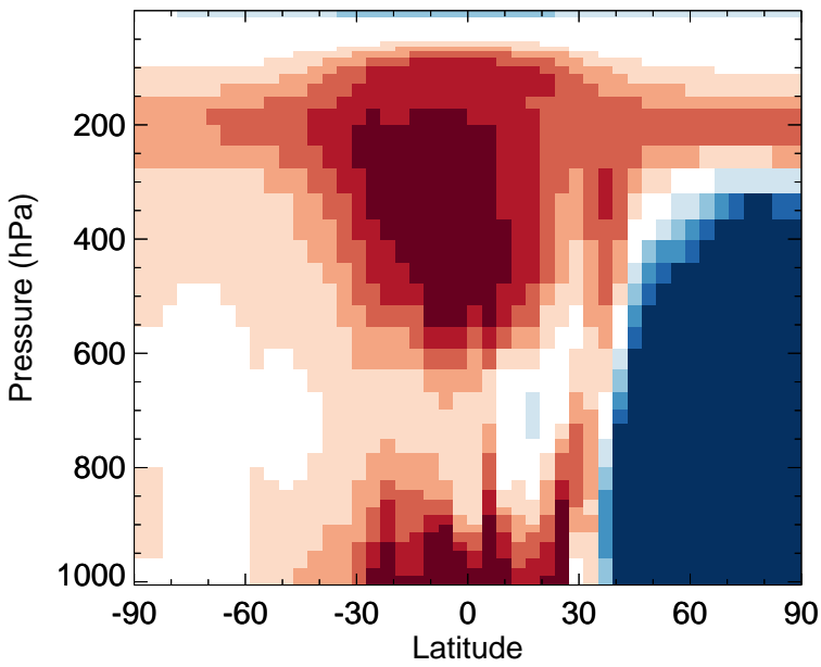
v11-02f-Run0 - v11-02e-Run1 PPN - Zonal mean abs diff for Apr
