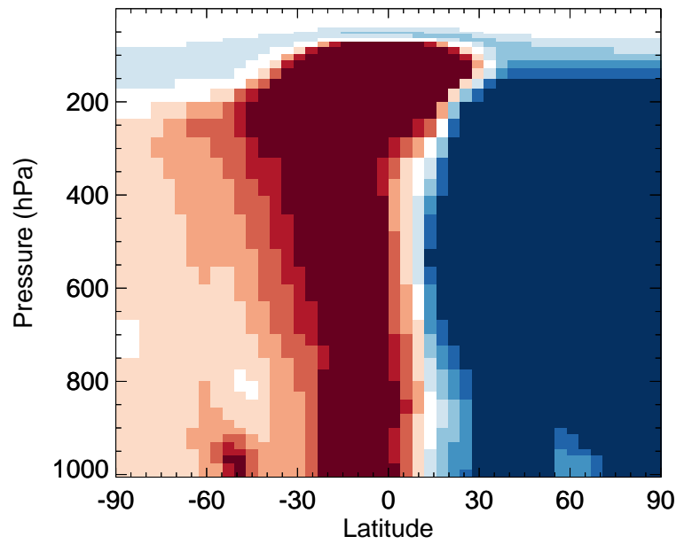
v11-02f-Run0 / v11-02e-Run1 ASOG2 - Zonal mean % diff for Apr
