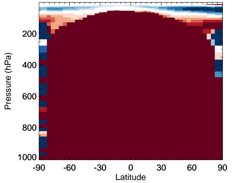
v11-02f-Run0 / v11-02e-Run1 MTPO - Zonal mean % diff for Apr
