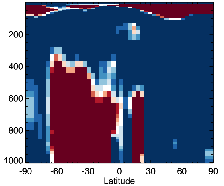
v11-02f-Run0 / v11-02e-Run0 DST2 - Zonal mean % diff for Apr
