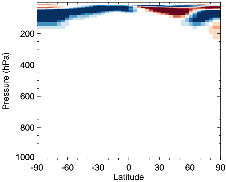
v11-02f-Run0 - v11-02e-Run0 CINO3 - Zonal mean abs diff for Apr
