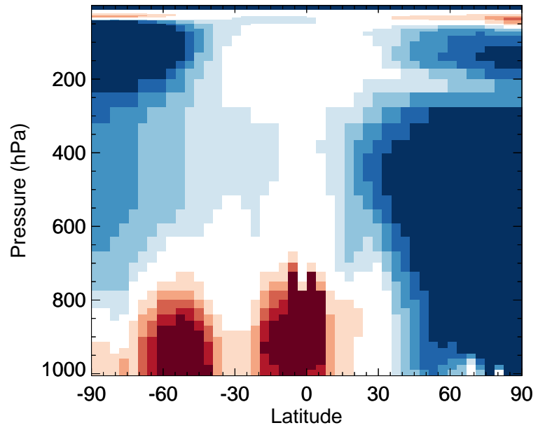
v11-02f-Run0 / v11-02e-Run1 HNO 4 - Zonal mean % diff for Apr
