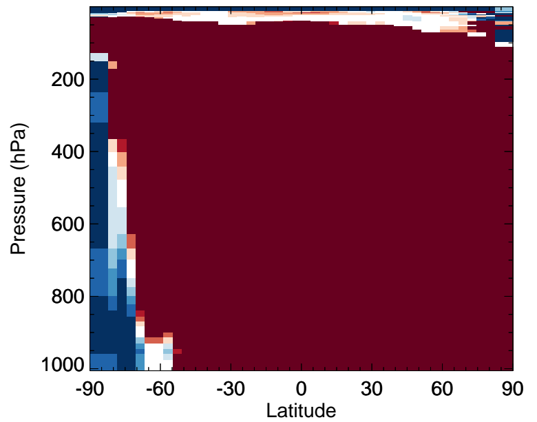
v11-02f-Run0 / v11-02e-Run0 RIPA - Zonal mean % diff for Apr
