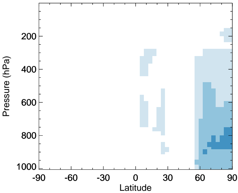
v11-02f-Run0 - v11-02e-Run0 PAN - Zonal mean abs diff for Apr
