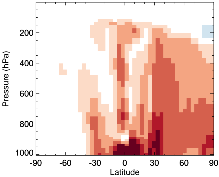
v11-02f-Run0 - v11-02e-Run0 ACET - Zonal mean abs diff for Apr
