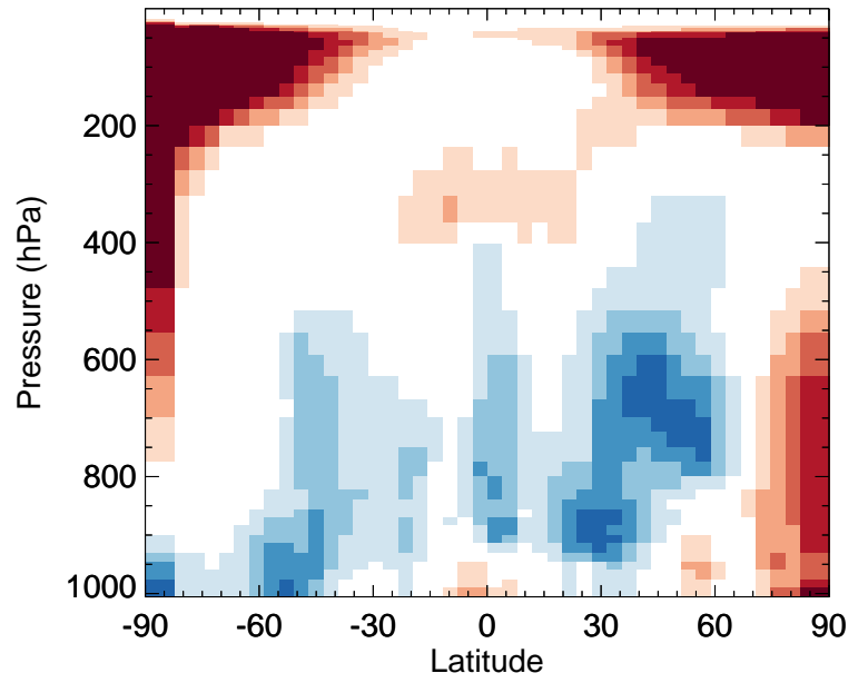
v11-02f-Run0 / v11-02e-Run1 BrO - Zonal mean % diff for Apr
