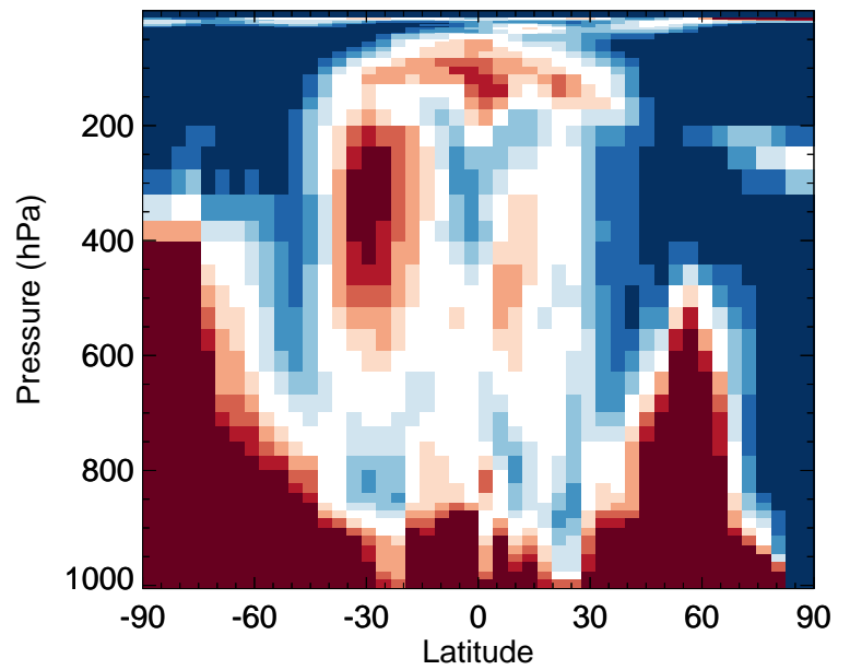
v11-02f-Run0 / v11-02e-Run0 HNO 2 - Zonal mean % diff for Apr
