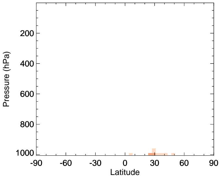
v11-02f-Run0 - v11-02e-Run0 SOAP - Zonal mean abs diff for Apr
