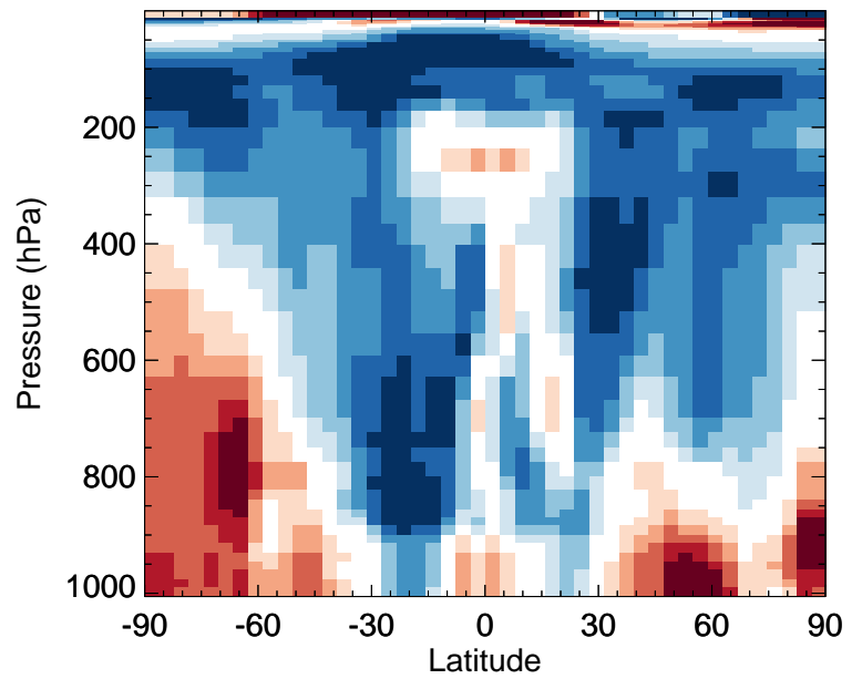
v11-02f-Run0 / v11-02e-Run0 SO4 - Zonal mean % diff for Apr
