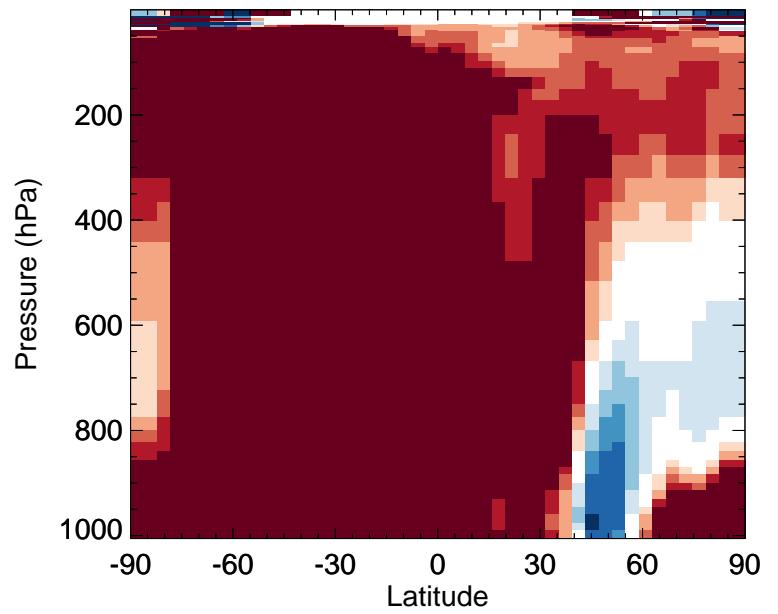
v11-02f-Run0 / v11-02e-Run1 OCPO - Zonal mean % diff for Apr
