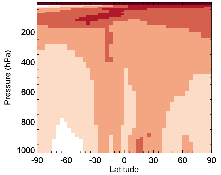
v11-02f-Run0 / v11-02e-Run1 ACET - Zonal mean % diff for Apr
