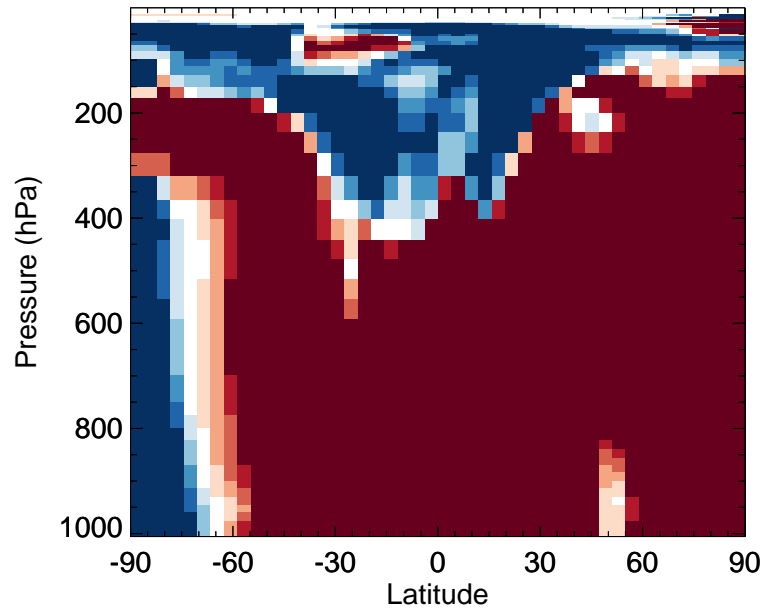
v11-02f-Run0 / v11-02e-Run1 LVOC - Zonal mean % diff for Apr
