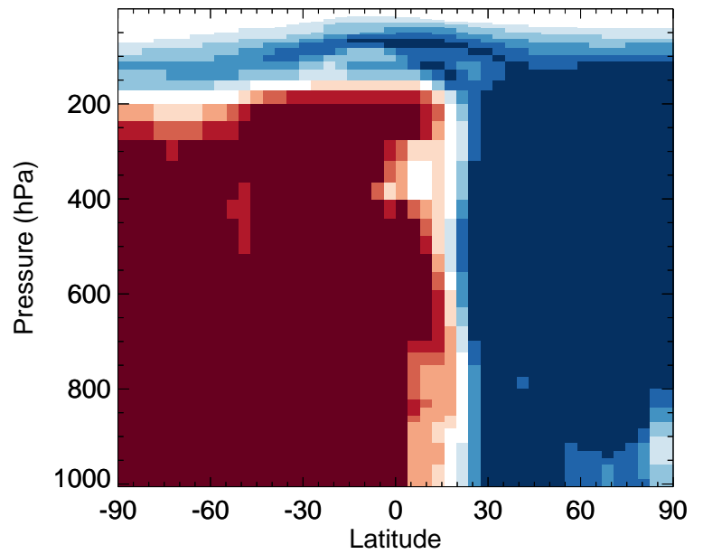
v11-02f-Run0 / v11-02e-Run0 ASOAN - Zonal mean % diff for Apr
