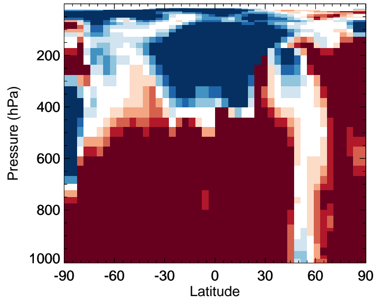
v11-02f-Run0 / v11-02e-Run1 ISN1OG - Zonal mean % diff for Apr
