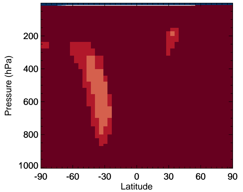
v11-02f-Run0 / v11-02e-Run1 ALK4 - Zonal mean % diff for Apr
