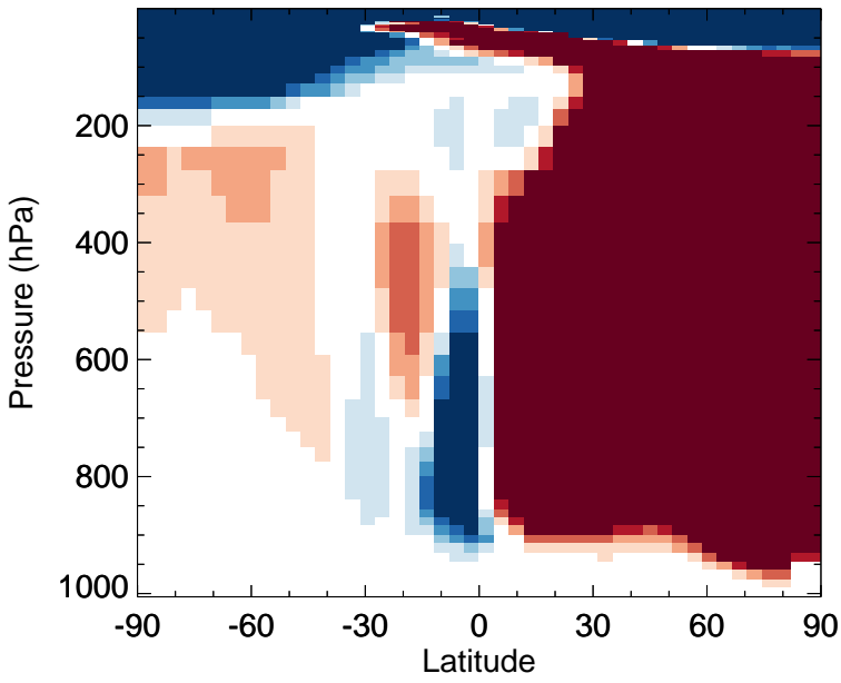
v11-02f-Run0 - v11-02e-Run1 CH4 - Zonal mean abs diff for Apr
