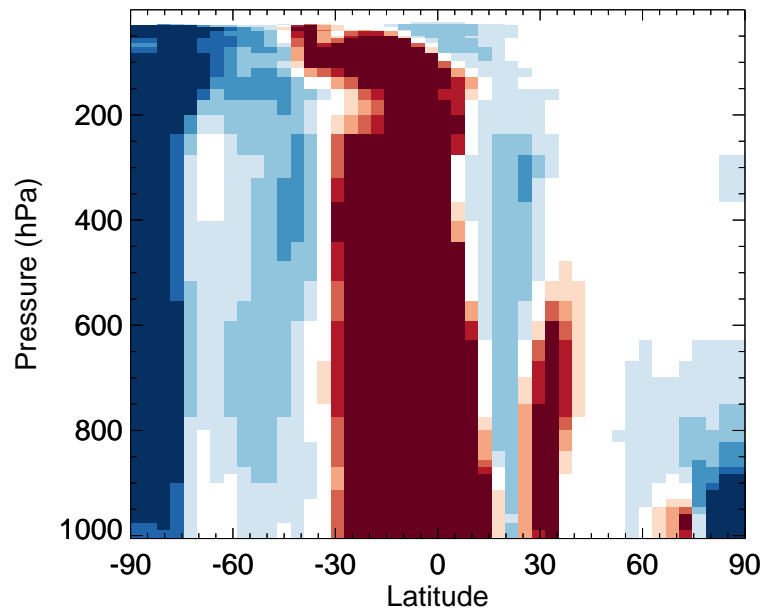
v11-02f-Run0 / v11-02e-Run1 SOAP - Zonal mean % diff for Apr
