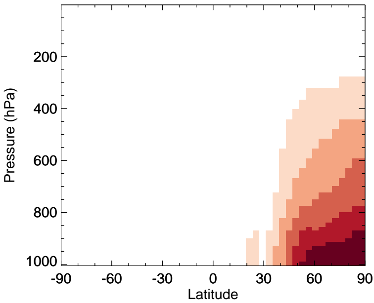
v11-02f-Run0 - v11-02e-Run1 C3H8 - Zonal mean abs diff for Apr
