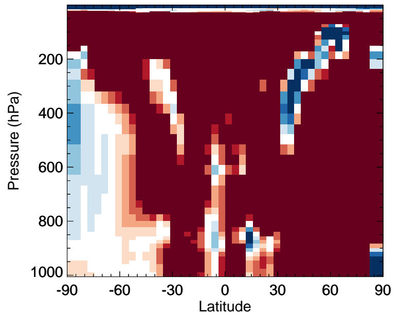
v11-02f-Run0 / v11-02e-Run0 DMS - Zonal mean % diff for Apr
