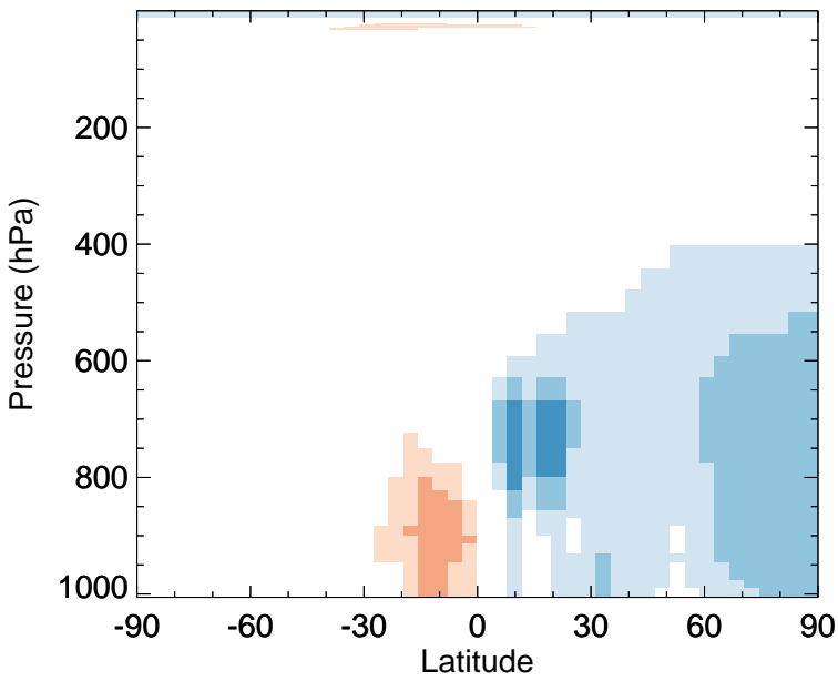
v11-02f-Run0 - v11-02e-Run1 H2O2 - Zonal mean abs diff for Apr
