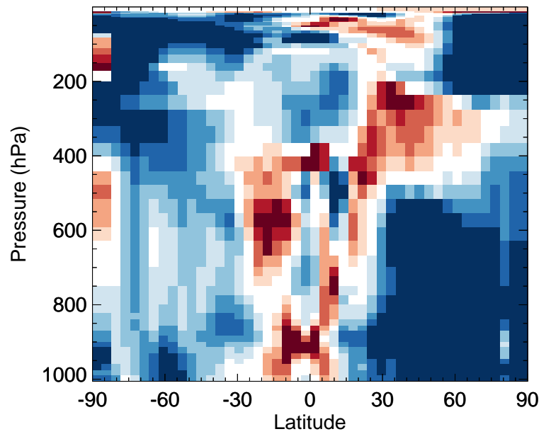
v11-02f-Run0 / v11-02e-Run0 ClOO - Zonal mean % diff for Apr
