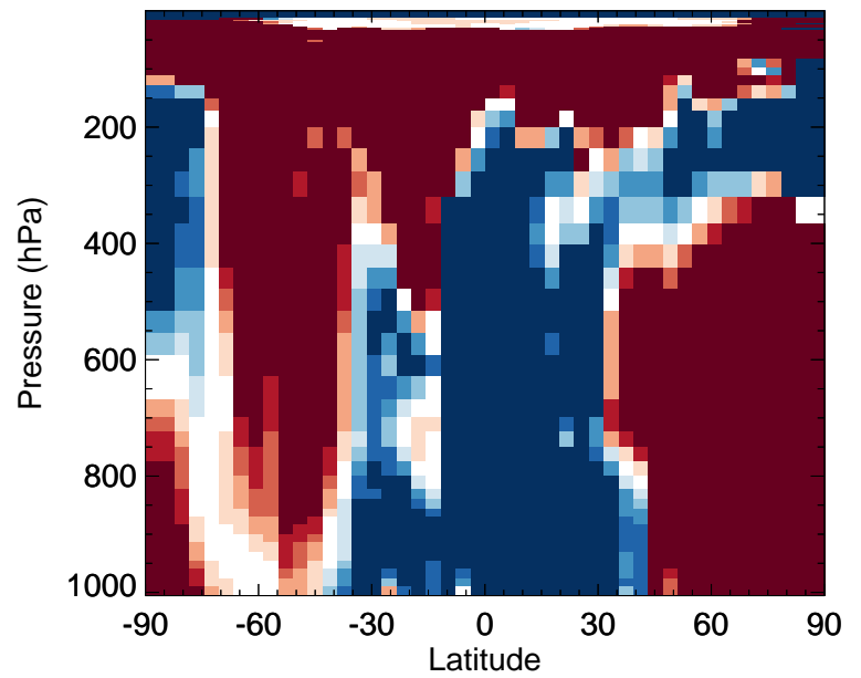
v11-02f-Run0 / v11-02e-Run0 XYLE - Zonal mean % diff for Apr
