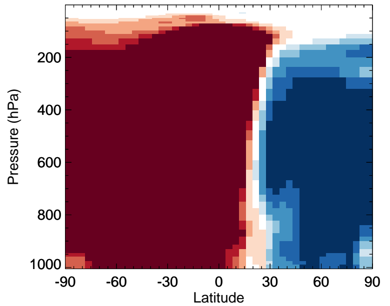
v11-02f-Run0 / v11-02e-Run0 ASOG3 - Zonal mean % diff for Apr
