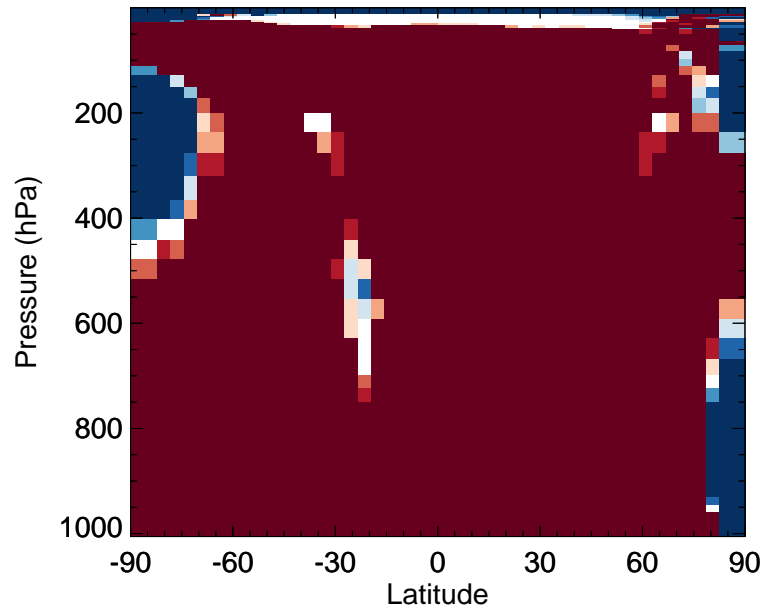
v11-02f-Run0 / v11-02e-Run0 MVKN - Zonal mean % diff for Apr
