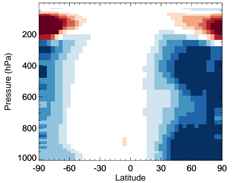
v11-02f-Run0 / v11-02e-Run1 HCl - Zonal mean % diff for Apr
