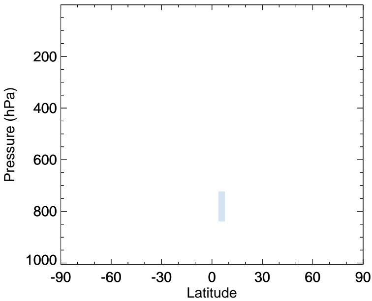
v11-02f-Run0 - v11-02e-Run0 IEPOXB - Zonal mean abs diff for Apr
