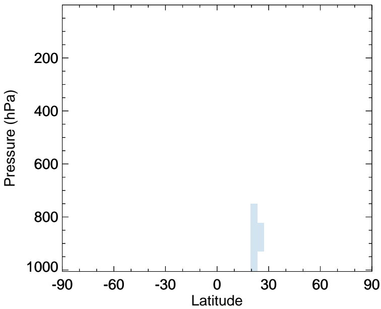
v11-02f-Run0 - v11-02e-Run0 SOAGX - Zonal mean abs diff for Apr
