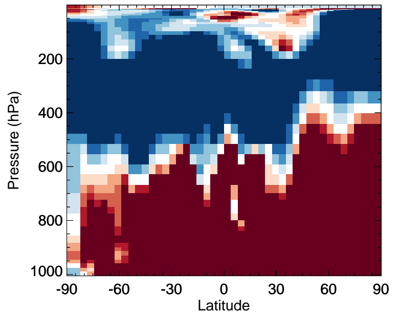
v11-02f-Run0 / v11-02e-Run0 TSOA3 - Zonal mean % diff for Apr
