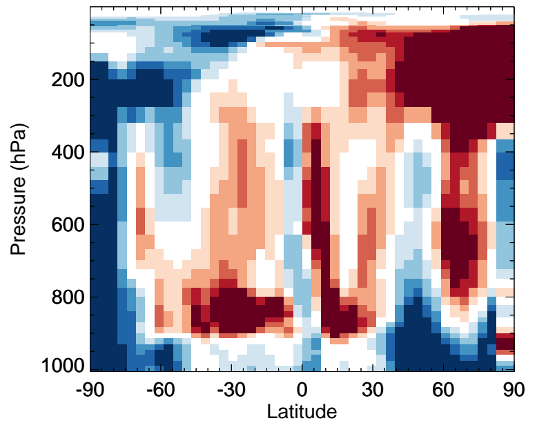
v11-02f-Run0 / v11-02e-Run0 HCl - Zonal mean % diff for Apr
