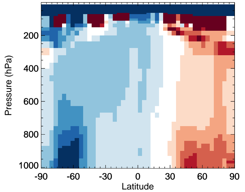
v11-02f-Run0 / v11-02e-Run1 SO4s - Zonal mean % diff for Apr
