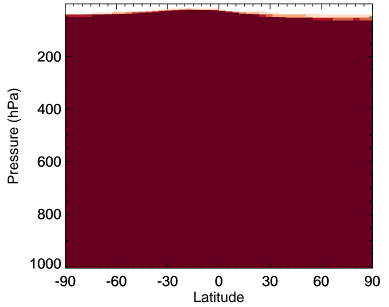
v11-02f-Run0 / v11-02e-Run1 NH3 - Zonal mean % diff for Apr
