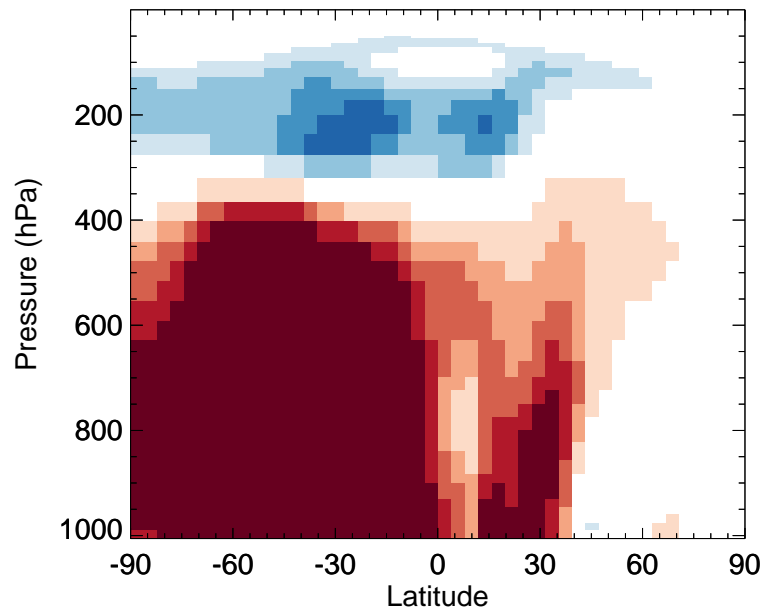
v11-02f-Run0 / v11-02e-Run1 ISOA2 - Zonal mean % diff for Apr
