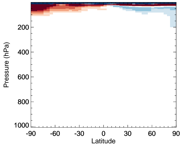
v11-02f-Run0 / v11-02e-Run0 CH3Cl - Zonal mean % diff for Apr
