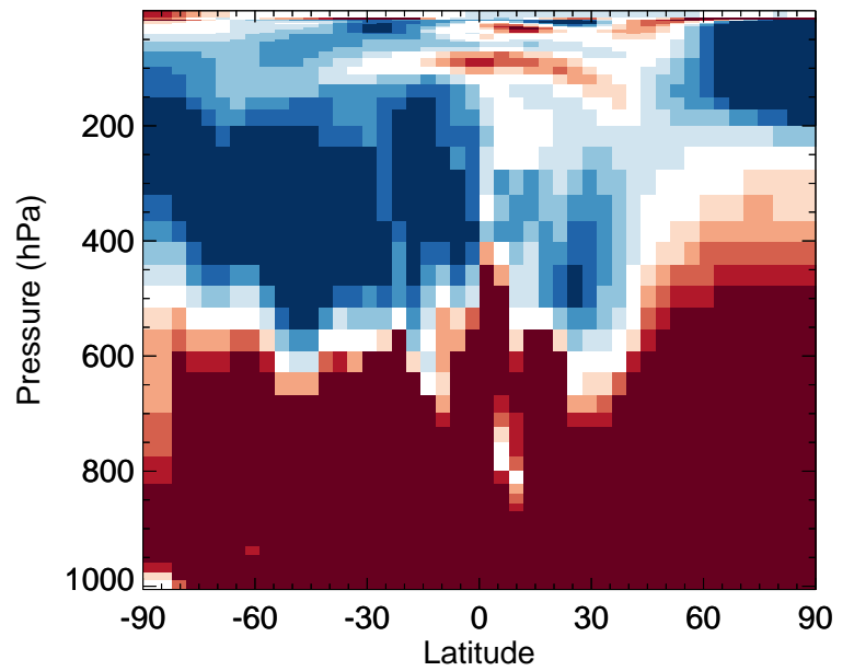
v11-02f-Run0 / v11-02e-Run0 TSOA1 - Zonal mean % diff for Apr
