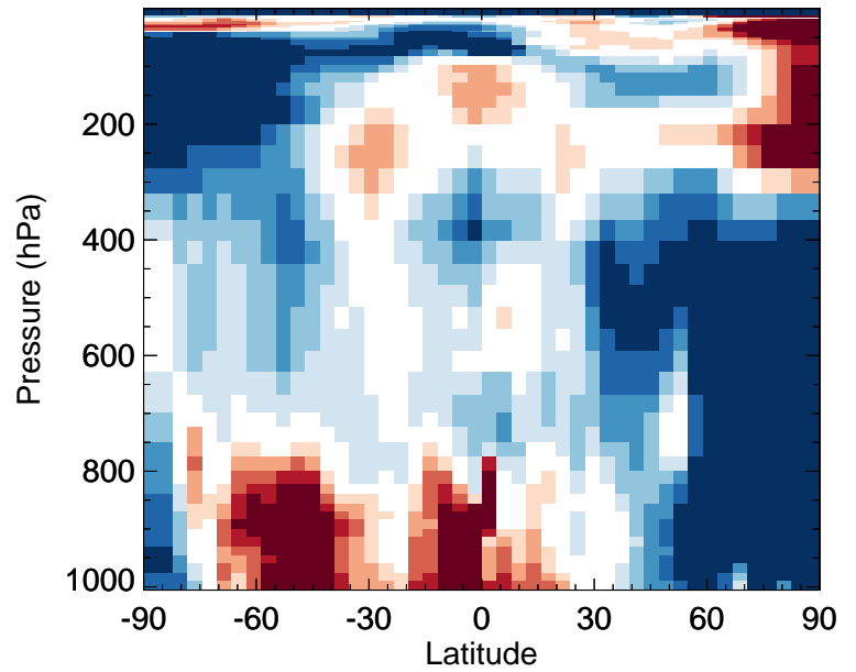
v11-02f-Run0 / v11-02e-Run0 HNO 4 - Zonal mean % diff for Apr
