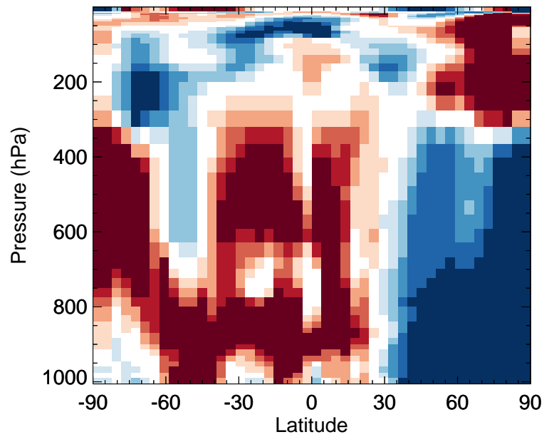
v11-02f-Run0 / v11-02e-Run0 NO 3 - Zonal mean % diff for Apr
