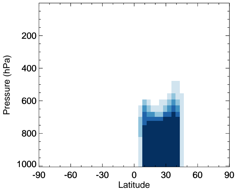
v11-02f-Run0 - v11-02e-Run0 DST3 - Zonal mean abs diff for Apr
