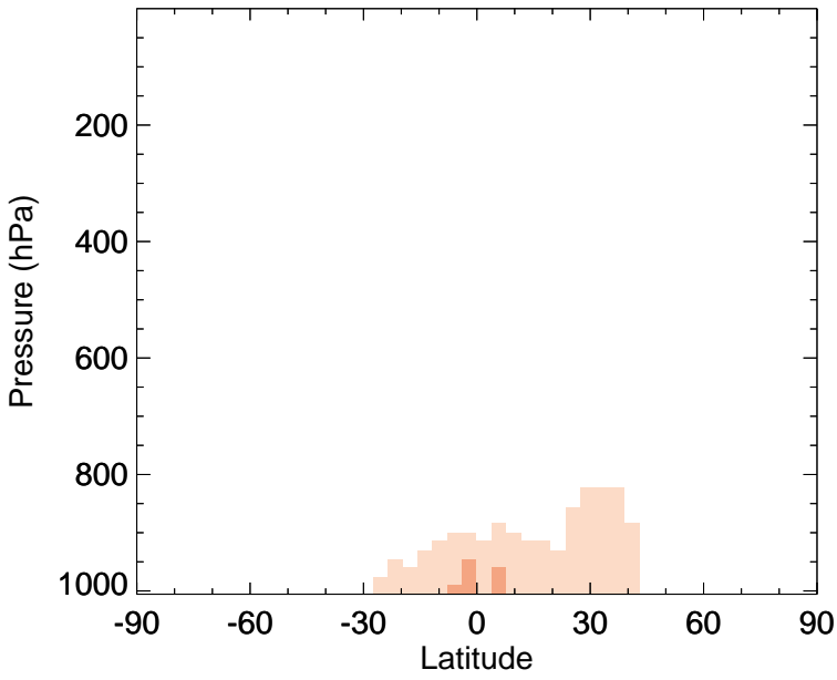
v11-02f-Run0 - v11-02e-Run1 INDIOL - Zonal mean abs diff for Apr
