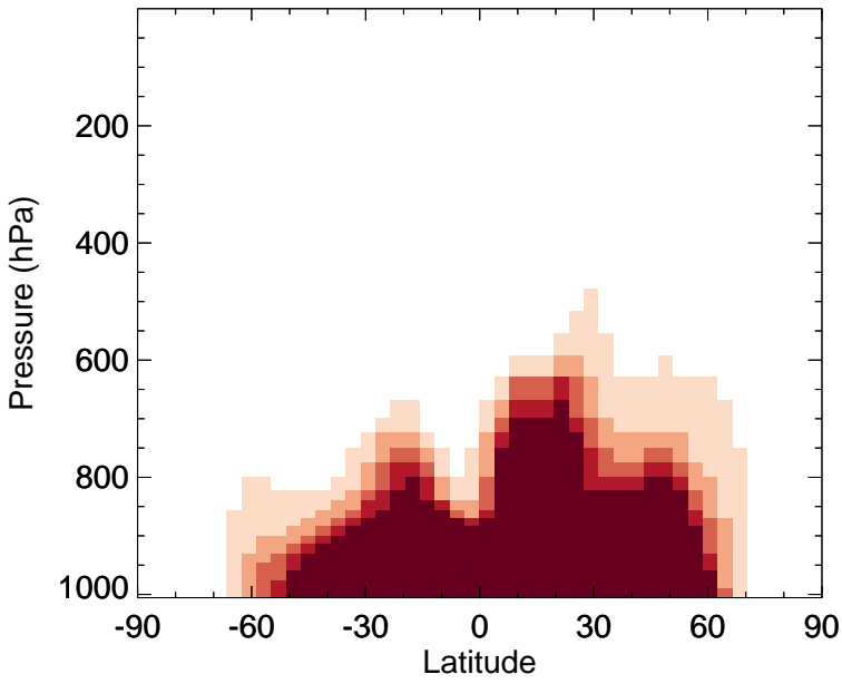
v11-02f-Run0 - v11-02e-Run1 NH3 - Zonal mean abs diff for Apr
