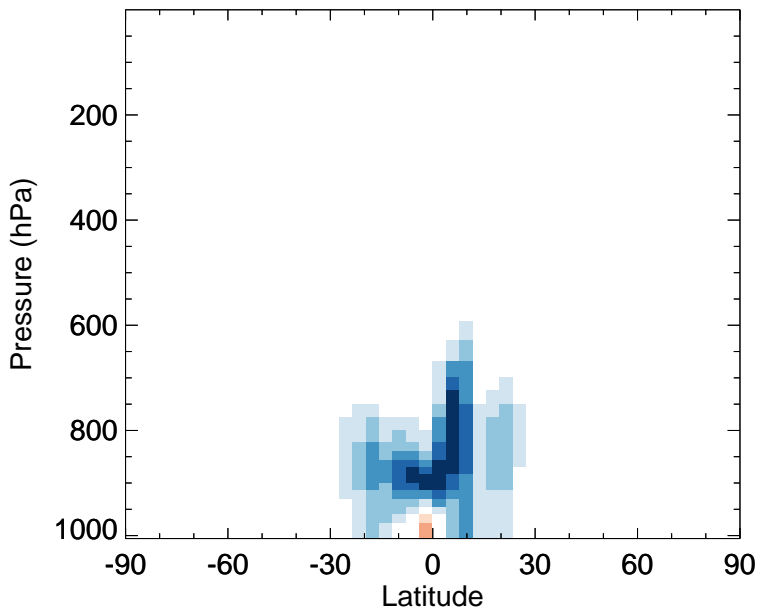
v11-02f-Run0 - v11-02e-Run0 MVK - Zonal mean abs diff for Apr
