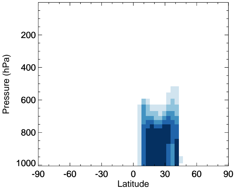
v11-02f-Run0 - v11-02e-Run0 DST2 - Zonal mean abs diff for Apr
