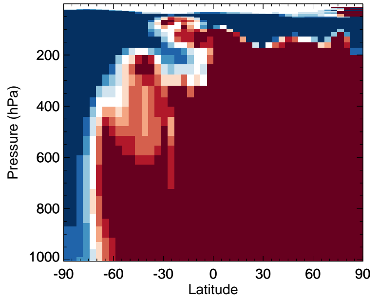
v11-02f-Run0 / v11-02e-Run1 HPALD - Zonal mean % diff for Apr
