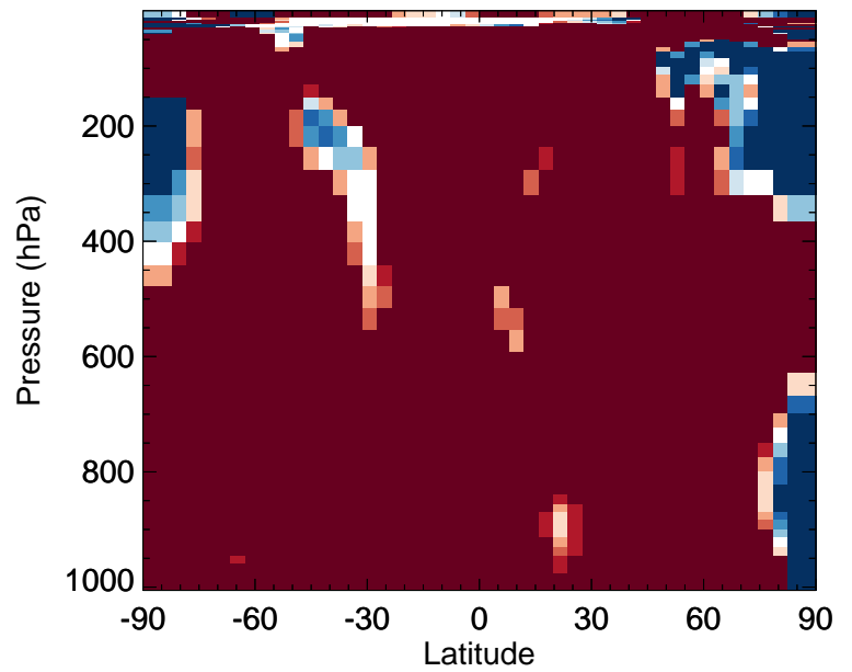
v11-02f-Run0 / v11-02e-Run0 OCPO - Zonal mean % diff for Apr
