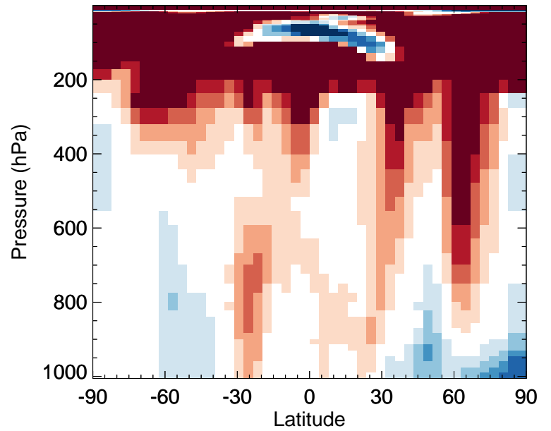
v11-02f-Run0 / v11-02e-Run0 MP - Zonal mean % diff for Apr
