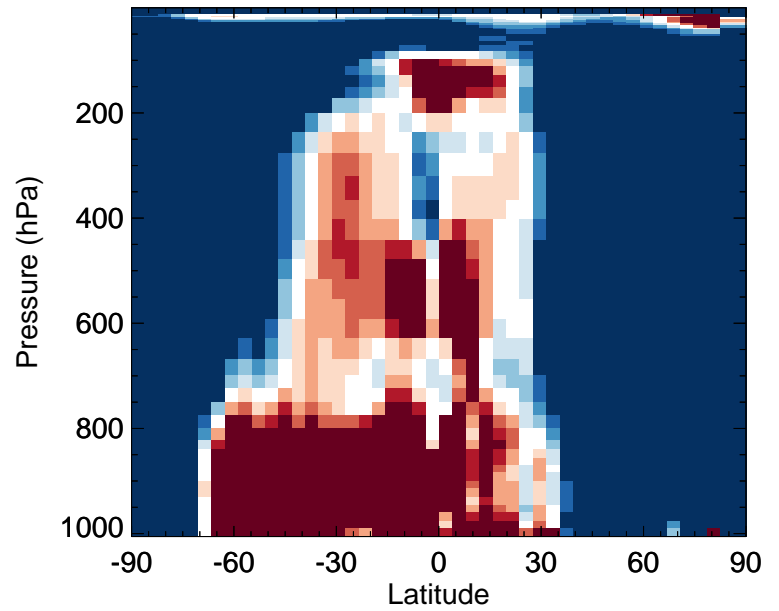
v11-02f-Run0 / v11-02e-Run0 N2O5 - Zonal mean % diff for Apr
