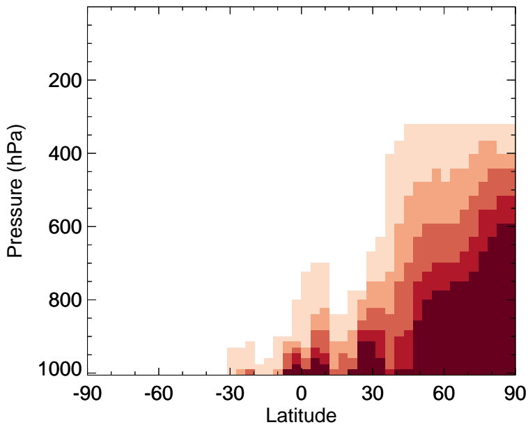
v11-02f-Run0 - v11-02e-Run0 ALK4 - Zonal mean abs diff for Apr
