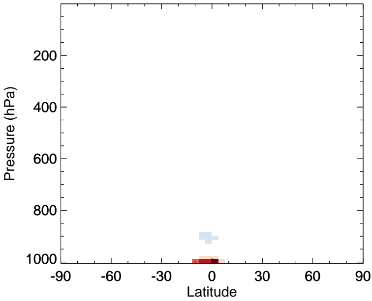
v11-02f-Run0 - v11-02e-Run0 MTPA - Zonal mean abs diff for Apr
