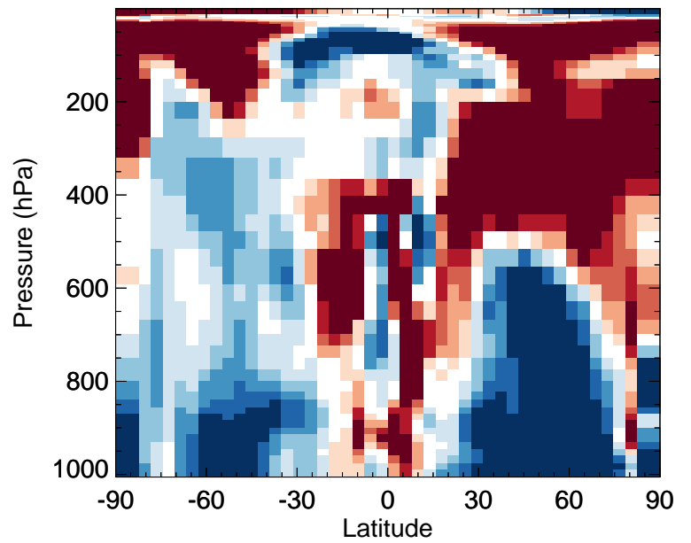
v11-02f-Run0 / v11-02e-Run0 ClO - Zonal mean % diff for Apr
