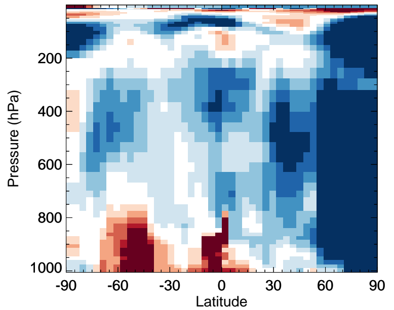
v11-02f-Run0 / v11-02e-Run0 MPN - Zonal mean % diff for Apr
