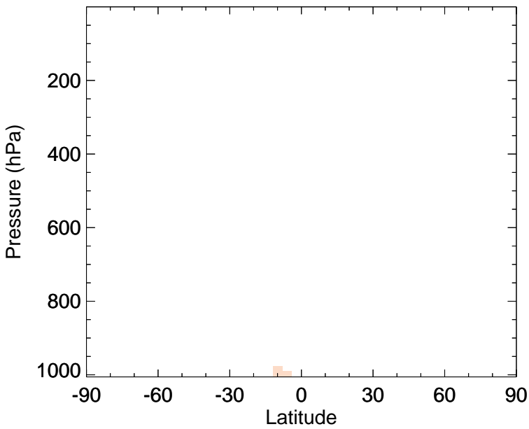
v11-02f-Run0 - v11-02e-Run0 TSOG2 - Zonal mean abs diff for Apr
