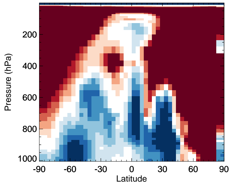
v11-02f-Run0 / v11-02e-Run1 OCIO - Zonal mean % diff for Apr
