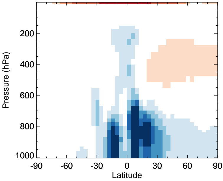
v11-02f-Run0 - v11-02e-Run1 MP - Zonal mean abs diff for Apr
