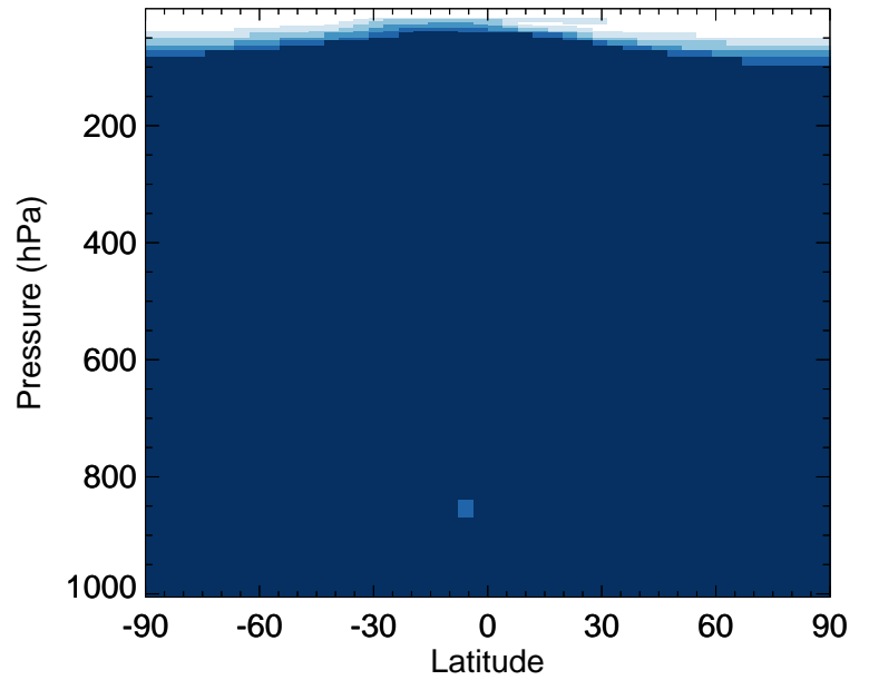
v11-02f-Run0 / v11-02e-Run0 SOAME - Zonal mean % diff for Apr
