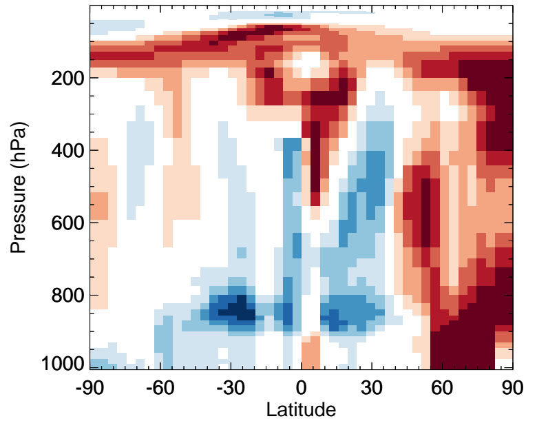
v11-02f-Run0 / v11-02e-Run0 MSA - Zonal mean % diff for Apr
