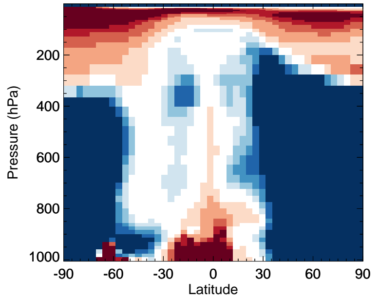
v11-02f-Run0 / v11-02e-Run1 HNO 3 - Zonal mean % diff for Apr
