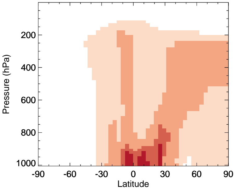
v11-02f-Run0 - v11-02e-Run1 ACET - Zonal mean abs diff for Apr
