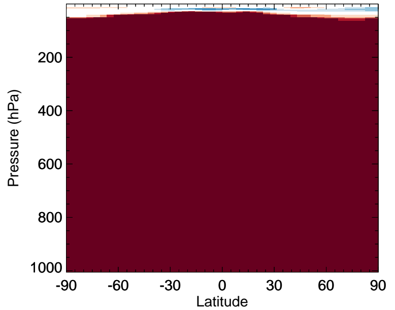
v11-02f-Run0 / v11-02e-Run0 NH3 - Zonal mean % diff for Apr
