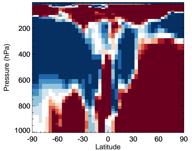
v11-02f-Run0 / v11-02e-Run0 IMAE - Zonal mean % diff for Apr
