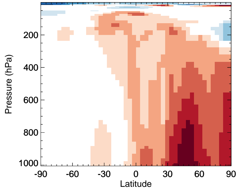
v11-02f-Run0 / v11-02e-Run0 CO - Zonal mean % diff for Apr
