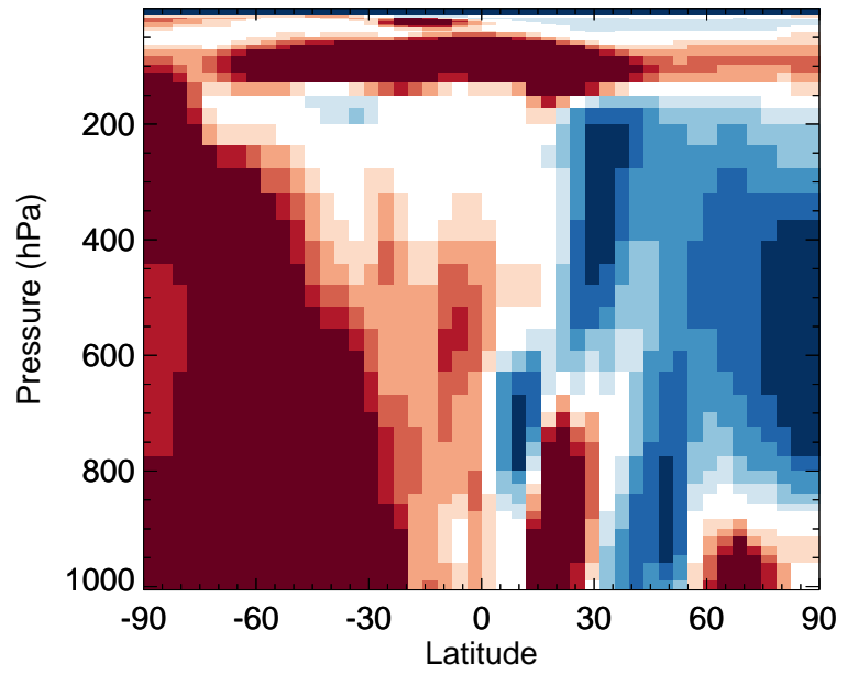
v11-02f-Run0 / v11-02e-Run1 GLYX - Zonal mean % diff for Apr
