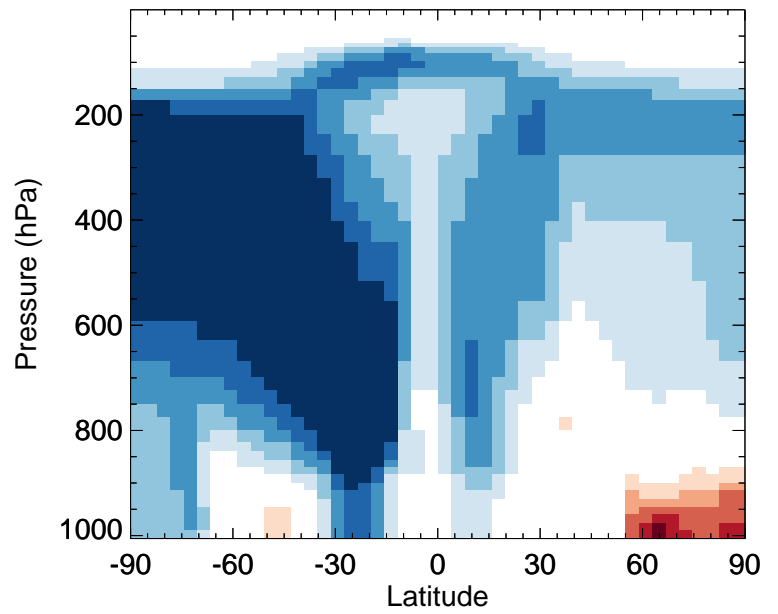
v11-02f-Run0 / v11-02e-Run1 SOAGX - Zonal mean % diff for Apr
