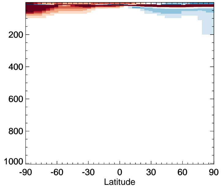
v11-02f-Run0 / v11-02e-Run0 CFC12 - Zonal mean % diff for Apr
