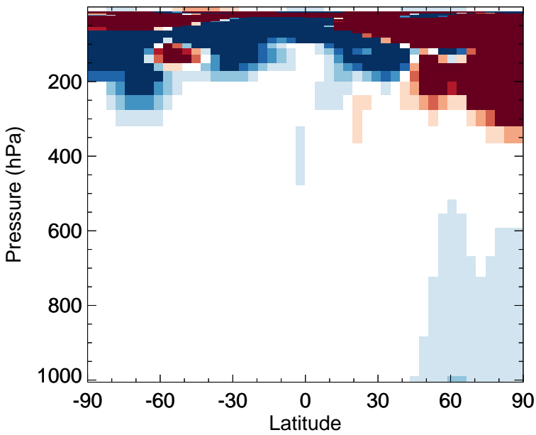
v11-02f-Run0 - v11-02e-Run0 O3 - Zonal mean abs diff for Apr
