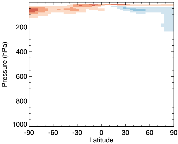
v11-02f-Run0 - v11-02e-Run0 CH3Cl - Zonal mean abs diff for Apr
