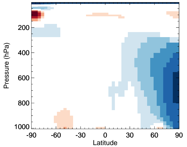
v11-02f-Run0 / v11-02e-Run1 CH 2 O - Zonal mean % diff for Apr
