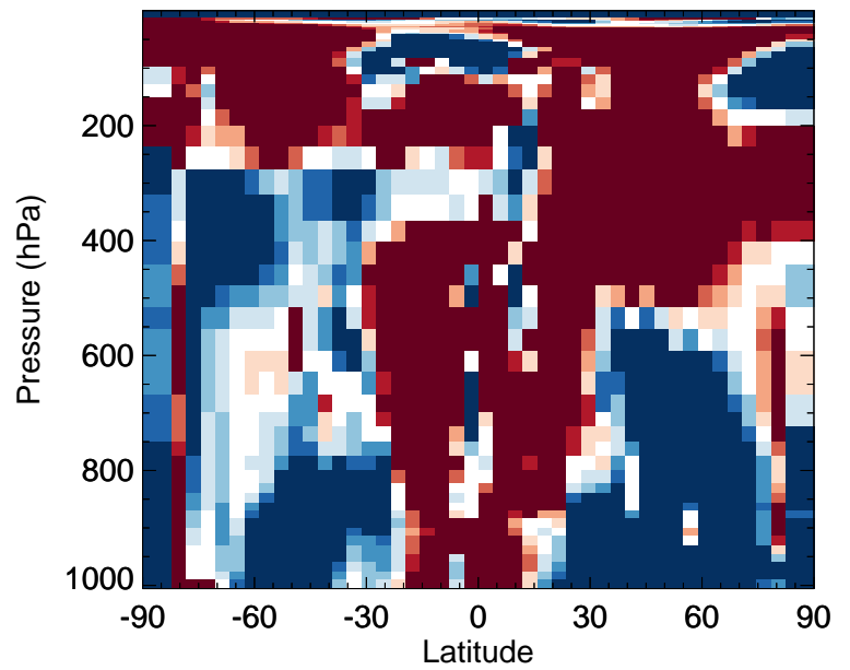
v11-02f-Run0 / v11-02e-Run0 Cl2O2 - Zonal mean % diff for Apr
