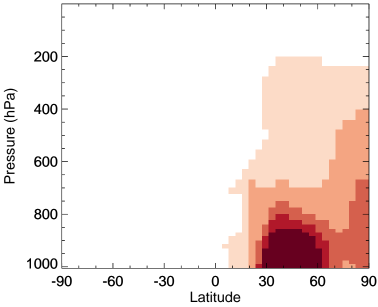
v11-02f-Run0 - v11-02e-Run1 NH4 - Zonal mean abs diff for Apr
