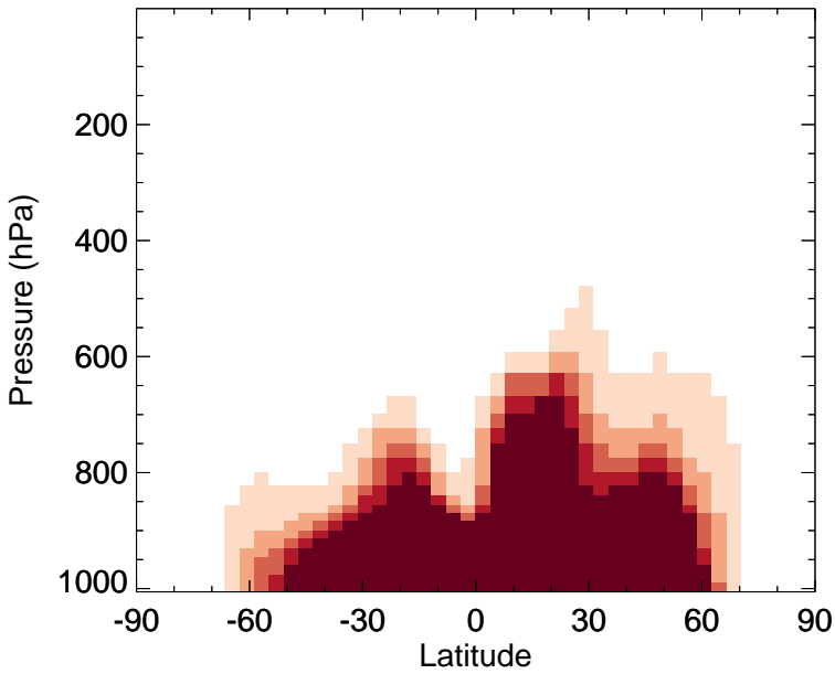
v11-02f-Run0 - v11-02e-Run0 NH3 - Zonal mean abs diff for Apr
