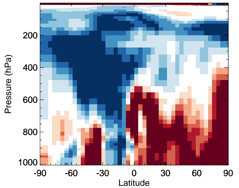
v11-02f-Run0 / v11-02e-Run0 BCPI - Zonal mean % diff for Apr
