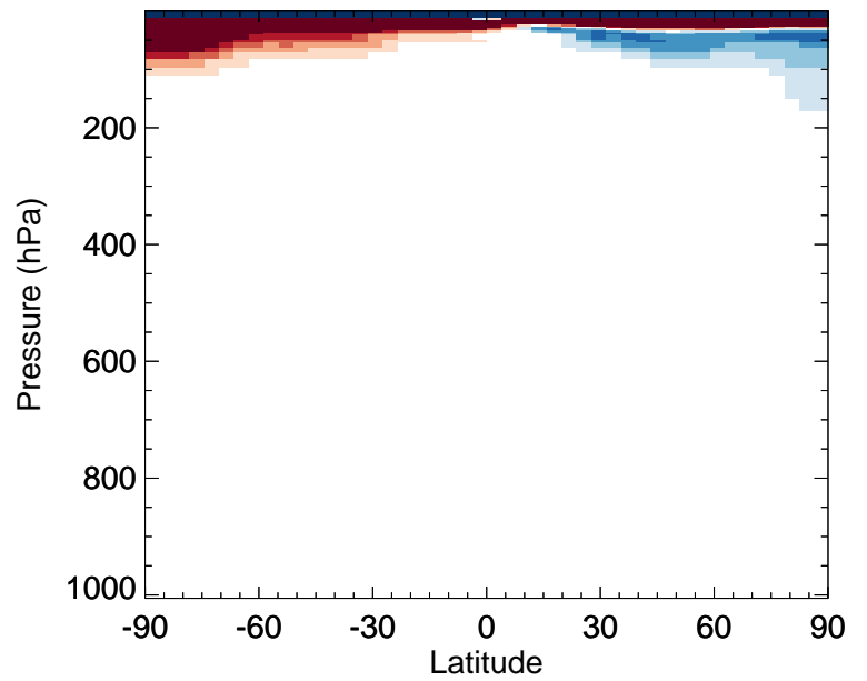
v11-02f-Run0 / v11-02e-Run0 OCS - Zonal mean % diff for Apr
