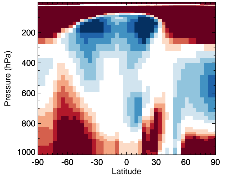
v11-02f-Run0 / v11-02e-Run1 MGLY - Zonal mean % diff for Apr
