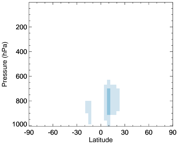
v11-02f-Run0 - v11-02e-Run1 ISO3 - Zonal mean abs diff for Apr
