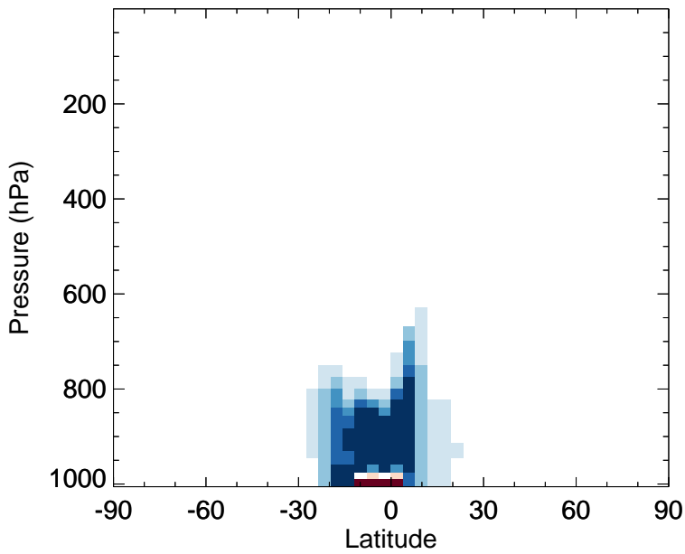
v11-02f-Run0 - v11-02e-Run0 ISOP - Zonal mean abs diff for Apr
