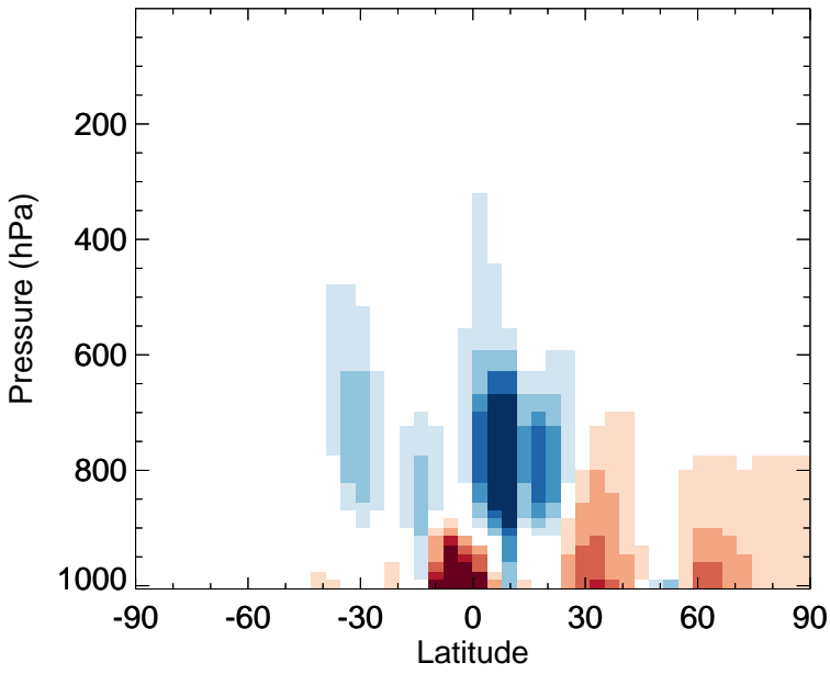
v11-02f-Run0 - v11-02e-Run1 MEK - Zonal mean abs diff for Apr
