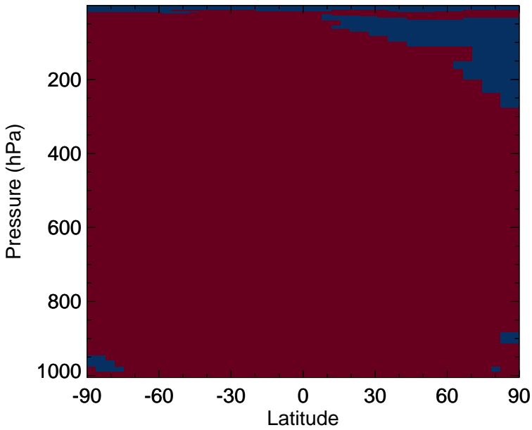
v11-02f-Run0 - v11-02e-Run0 CH4 - Zonal mean abs diff for Apr
