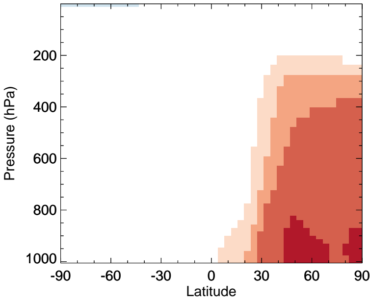
v11-02f-Run0 - v11-02e-Run1 CO - Zonal mean abs diff for Apr
