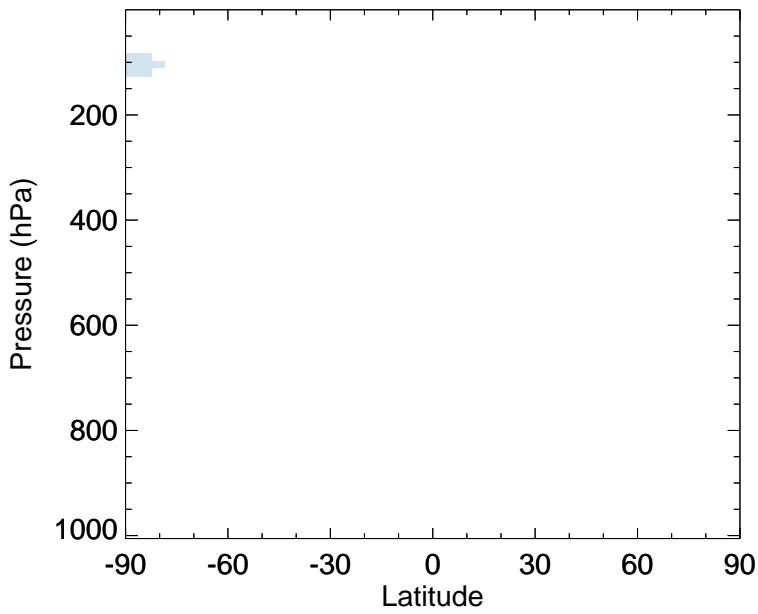
v11-02f-Run0 - v11-02e-Run1 MPN - Zonal mean abs diff for Apr
