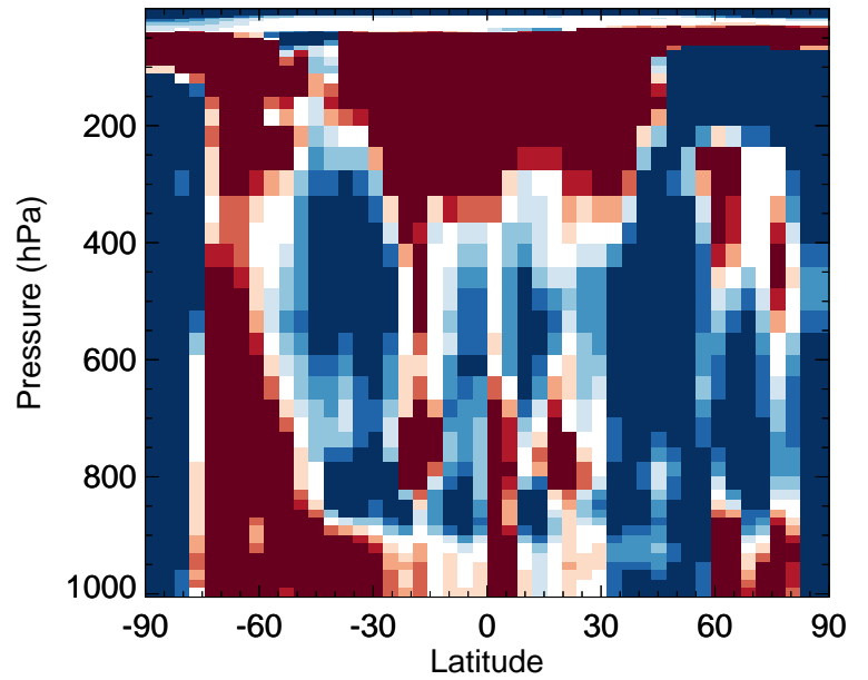
v11-02f-Run0 / v11-02e-Run0 NITs - Zonal mean % diff for Apr
