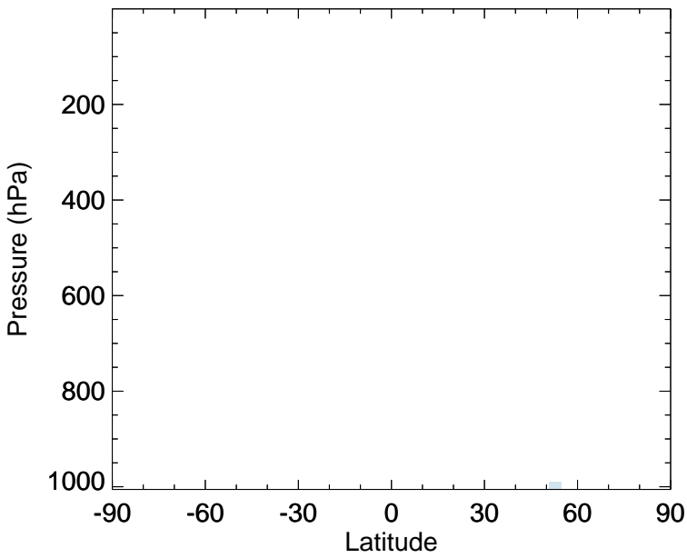
v11-02f-Run0 - v11-02e-Run1 SO2 - Zonal mean abs diff for Apr
