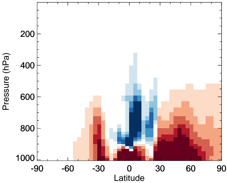
v11-02f-Run0 - v11-02e-Run0 MEK - Zonal mean abs diff for Apr
