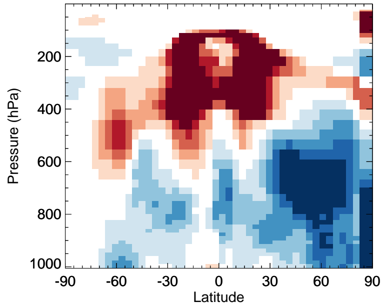
v11-02f-Run0 / v11-02e-Run1 BrCl - Zonal mean % diff for Apr
