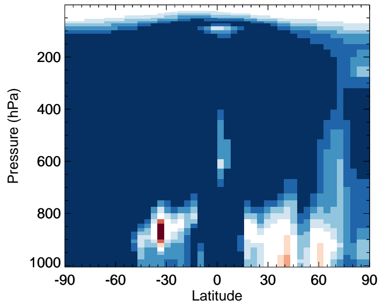
v11-02f-Run0 / v11-02e-Run0 ISO3 - Zonal mean % diff for Apr
