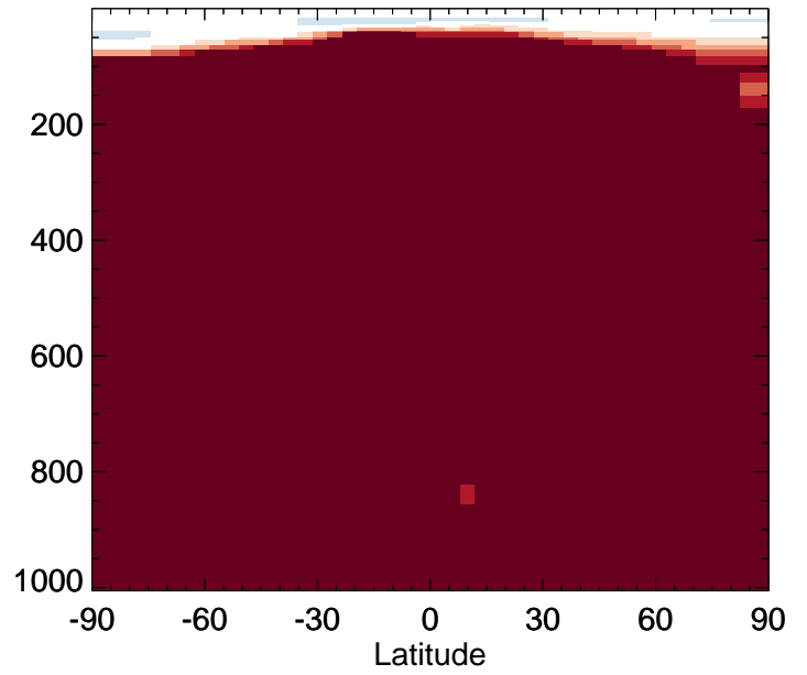
v11-02f-Run0 / v11-02e-Run0 NH4 - Zonal mean % diff for Apr
