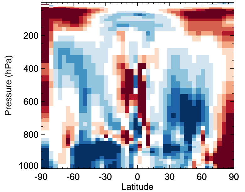
v11-02f-Run0 / v11-02e-Run0 BrO - Zonal mean % diff for Apr
