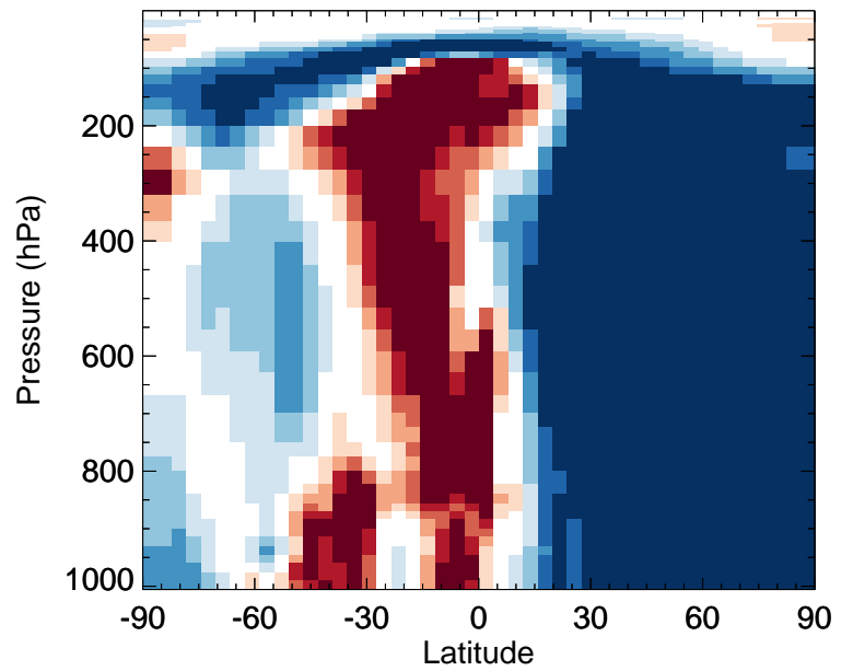
v11-02f-Run0 / v11-02e-Run0 ASOG2 - Zonal mean % diff for Apr
