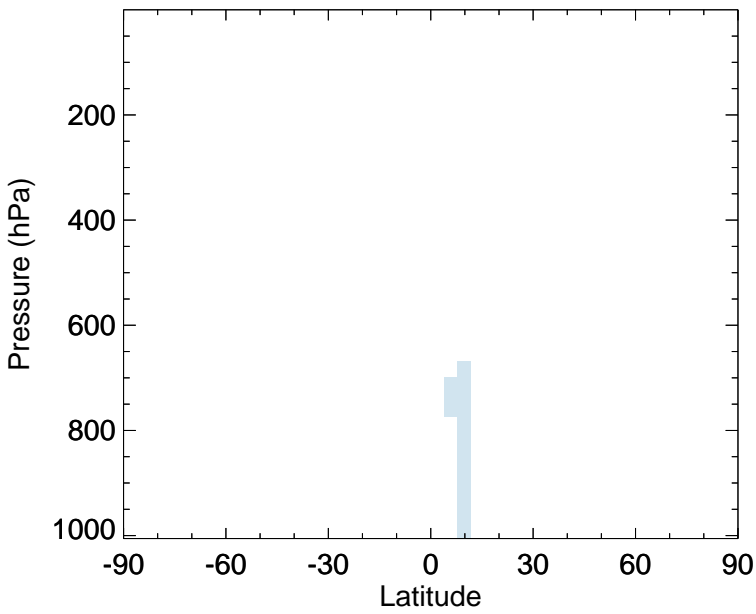
v11-02f-Run0 - v11-02e-Run1 IMAE - Zonal mean abs diff for Apr
