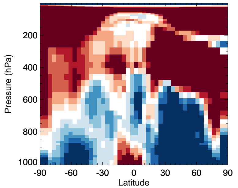
v11-02f-Run0 / v11-02e-Run1 Cl2O2 - Zonal mean % diff for Apr
