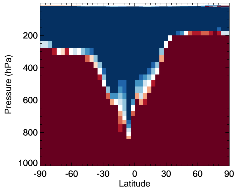
v11-02f-Run0 / v11-02e-Run1 IEPOXB - Zonal mean % diff for Apr
