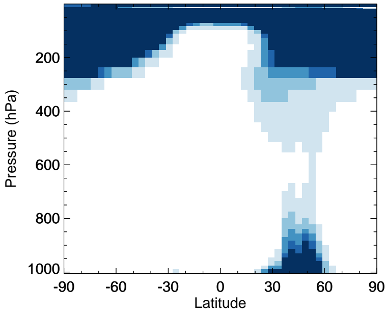
v11-02f-Run0 - v11-02e-Run1 N2O5 - Zonal mean abs diff for Apr
