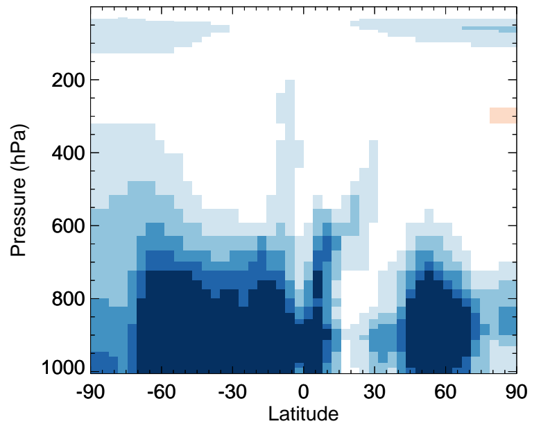
v11-02f-Run0 / v11-02e-Run1 SO2 - Zonal mean % diff for Apr
