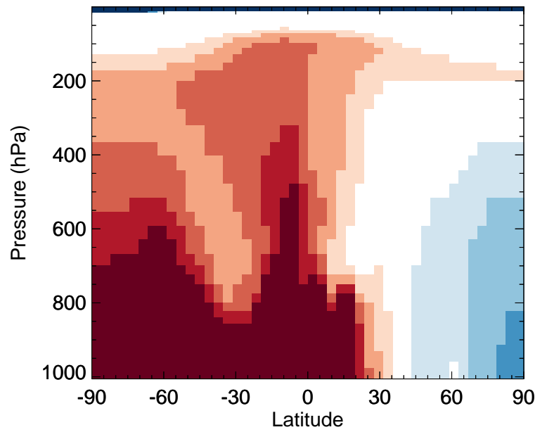
v11-02f-Run0 / v11-02e-Run1 PPN - Zonal mean % diff for Apr
