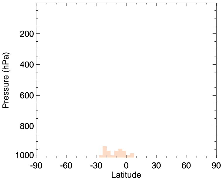
v11-02f-Run0 - v11-02e-Run1 TSOG3 - Zonal mean abs diff for Apr
