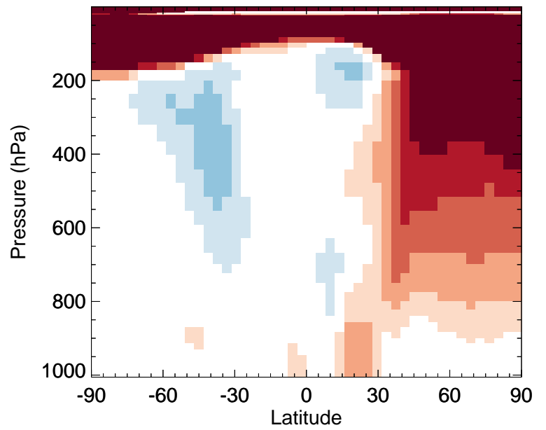
v11-02f-Run0 / v11-02e-Run1 MAP - Zonal mean % diff for Apr
