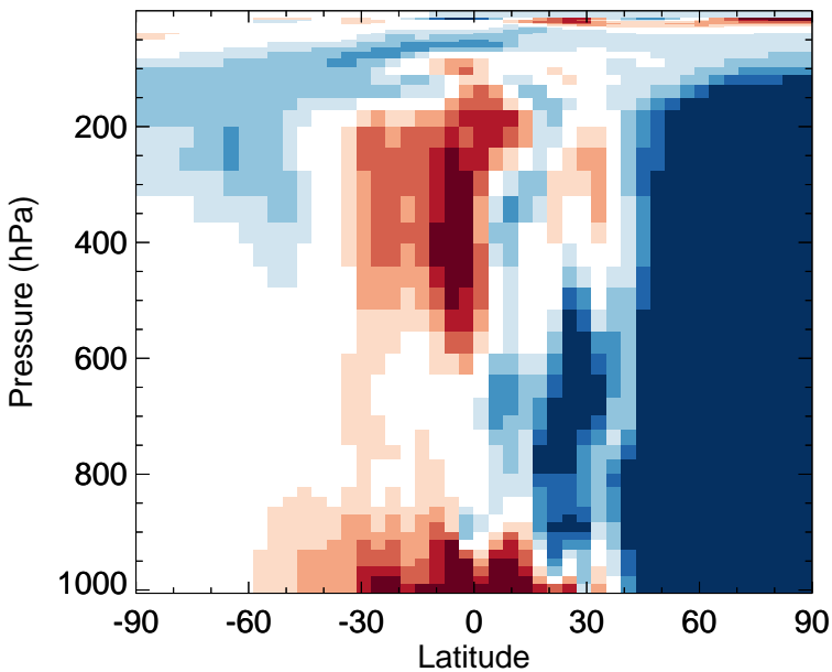
v11-02f-Run0 - v11-02e-Run0 PPN - Zonal mean abs diff for Apr
