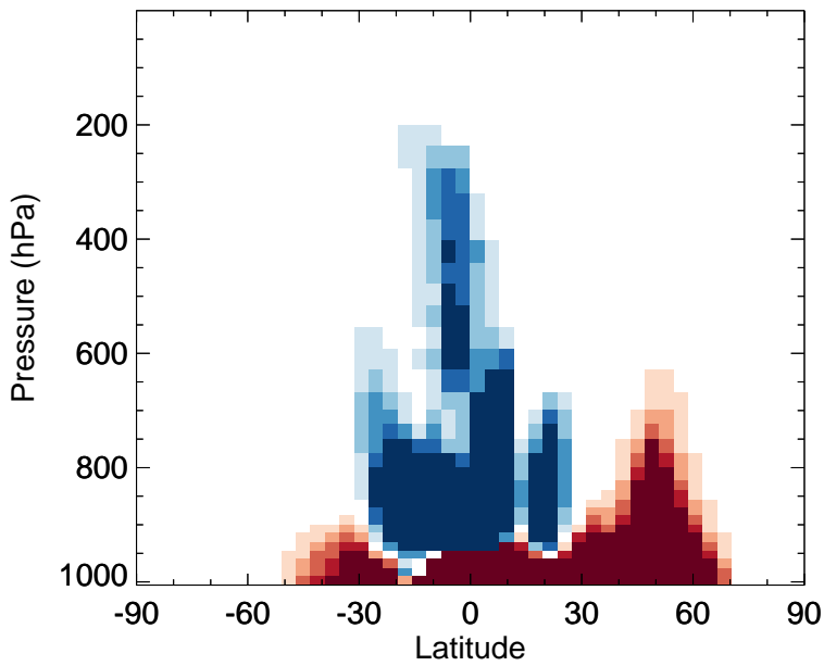
v11-02f-Run0 - v11-02e-Run0 PRPE - Zonal mean abs diff for Apr
