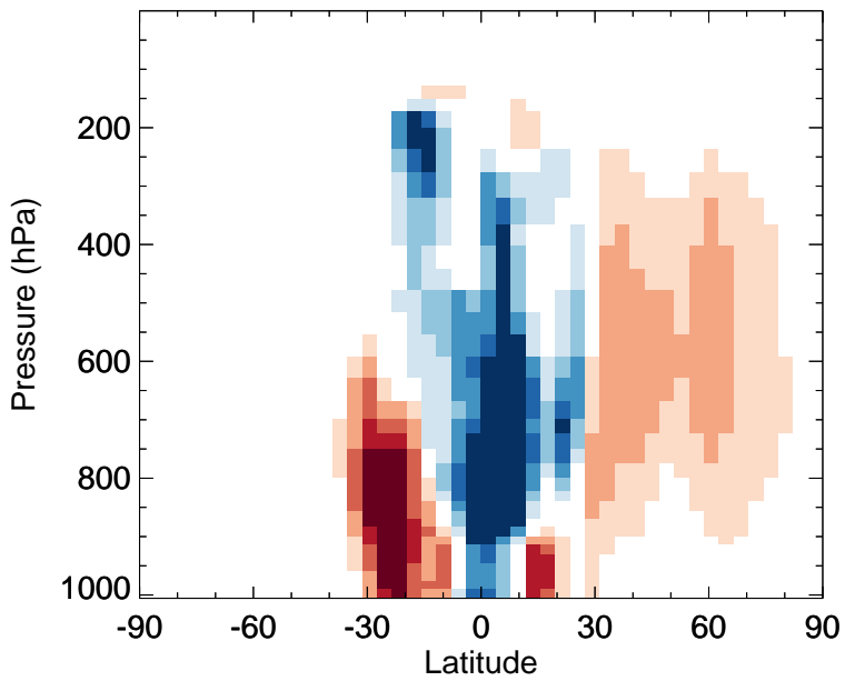
v11-02f-Run0 - v11-02e-Run0 MAP - Zonal mean abs diff for Apr
