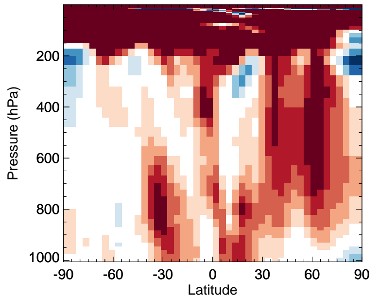
v11-02f-Run0 / v11-02e-Run0 MAP - Zonal mean % diff for Apr
