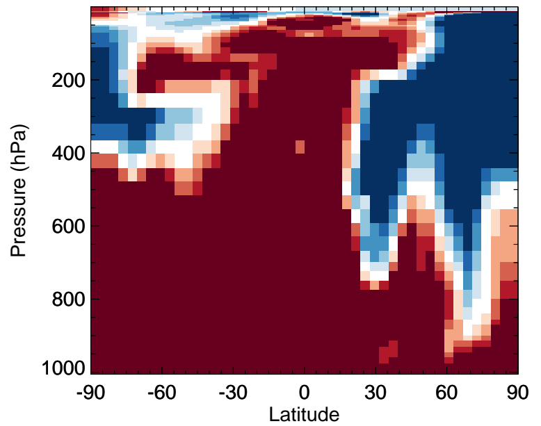
v11-02f-Run0 / v11-02e-Run0 ASOA3 - Zonal mean % diff for Apr
