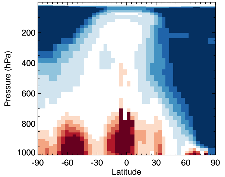
v11-02f-Run0 / v11-02e-Run1 NO 2 - Zonal mean % diff for Apr
