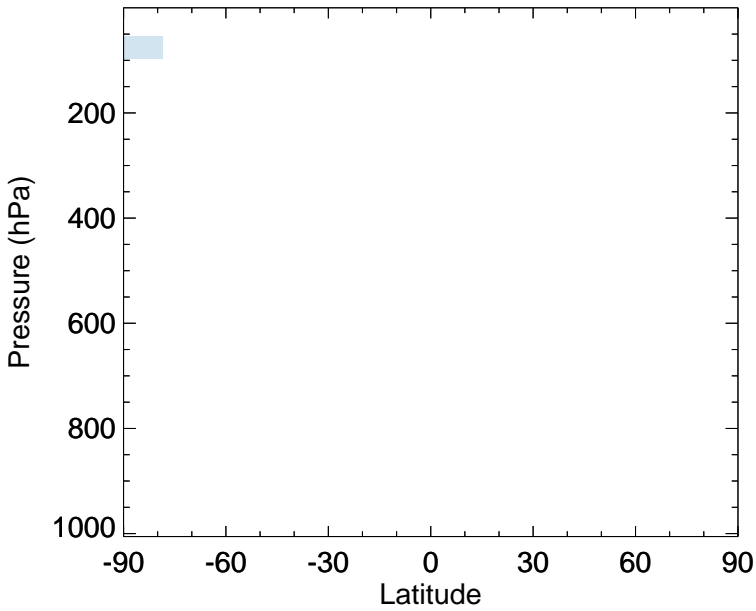
v11-02f-Run0 - v11-02e-Run0 HOBr - Zonal mean abs diff for Apr
