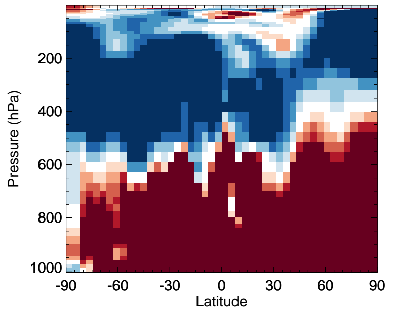
v11-02f-Run0 / v11-02e-Run0 TSOA2 - Zonal mean % diff for Apr
