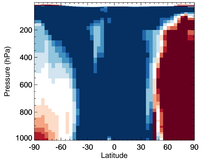
v11-02f-Run0 / v11-02e-Run1 XYLE - Zonal mean % diff for Apr
