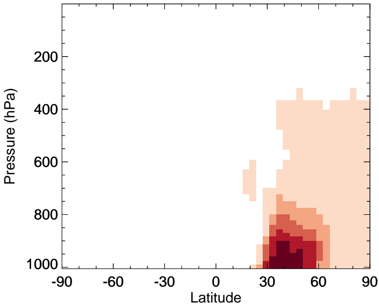
v11-02f-Run0 - v11-02e-Run0 NIT - Zonal mean abs diff for Apr
