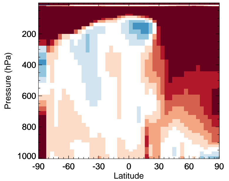
v11-02f-Run0 / v11-02e-Run1 ACTA - Zonal mean % diff for Apr
