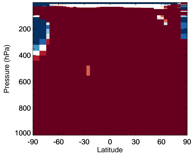
v11-02f-Run0 / v11-02e-Run0 MVK - Zonal mean % diff for Apr
