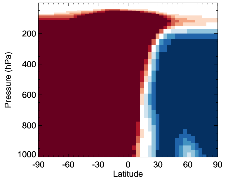
v11-02f-Run0 / v11-02e-Run1 ASOG1 - Zonal mean % diff for Apr
