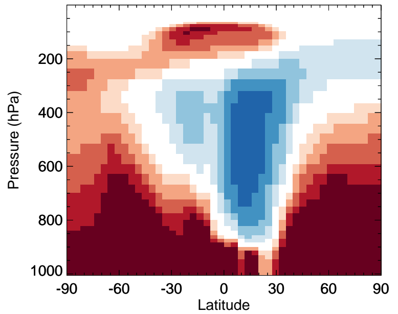
v11-02f-Run0 / v11-02e-Run1 TSOG1 - Zonal mean % diff for Apr
