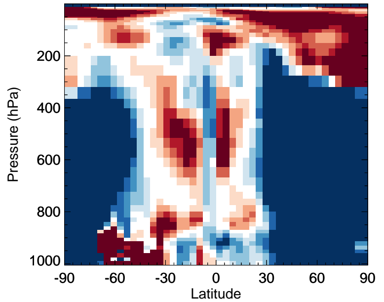
v11-02f-Run0 / v11-02e-Run0 HNO 3 - Zonal mean % diff for Apr
