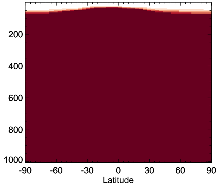
v11-02f-Run0 / v11-02e-Run1 NH4 - Zonal mean % diff for Apr
