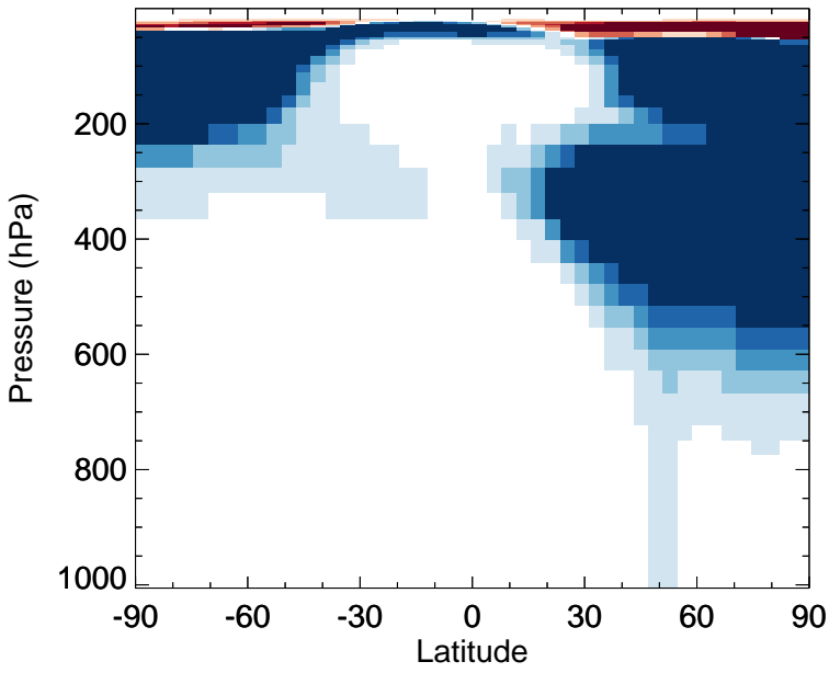
v11-02f-Run0 - v11-02e-Run1 HNO 4 - Zonal mean abs diff for Apr
