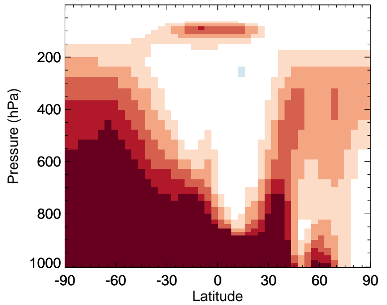
v11-02f-Run0 / v11-02e-Run1 TSOG3 - Zonal mean % diff for Apr
