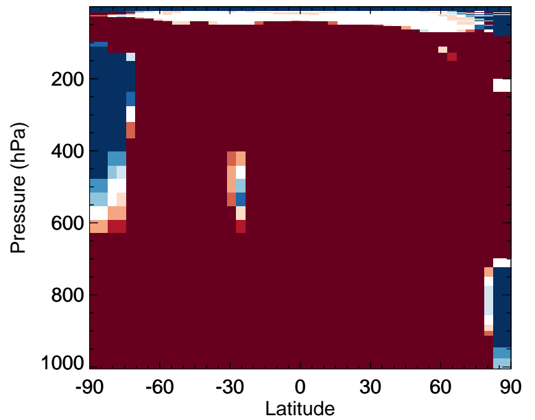
v11-02f-Run0 / v11-02e-Run0 ETHLN - Zonal mean % diff for Apr
