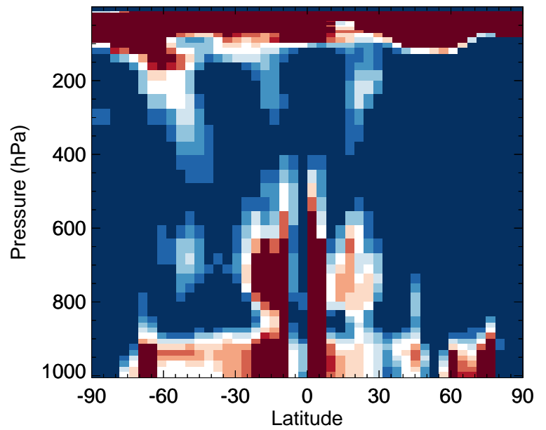
v11-02f-Run0 / v11-02e-Run0 SALC - Zonal mean % diff for Apr
