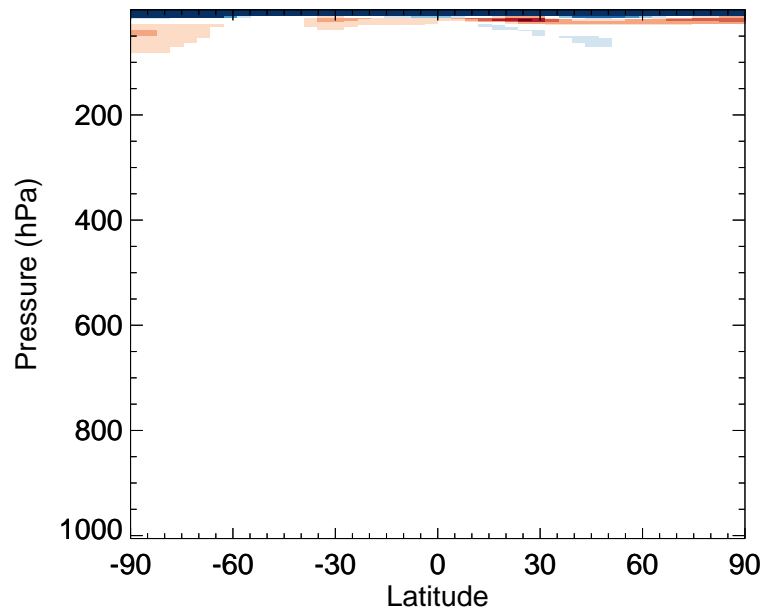
v11-02f-Run0 / v11-02e-Run0 CFC114 - Zonal mean % diff for Apr
