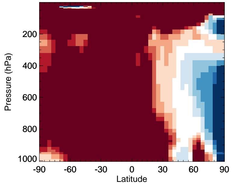
v11-02f-Run0 / v11-02e-Run0 R4N2 - Zonal mean % diff for Apr
