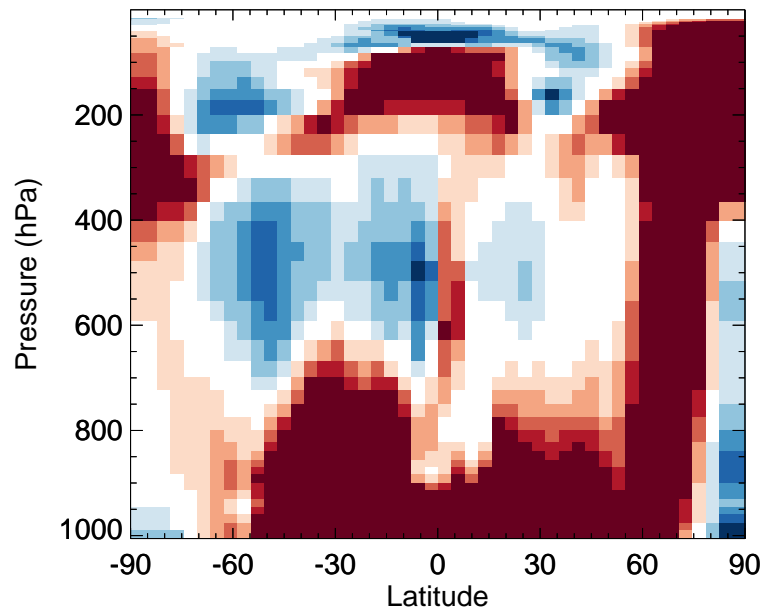
v11-02f-Run0 / v11-02e-Run0 TSOG1 - Zonal mean % diff for Apr
