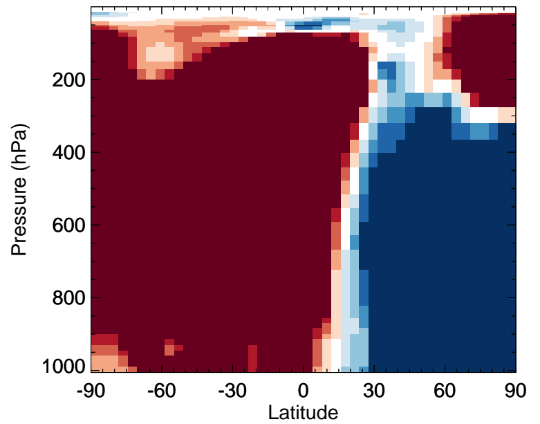
v11-02f-Run0 / v11-02e-Run0 ASOG1 - Zonal mean % diff for Apr
