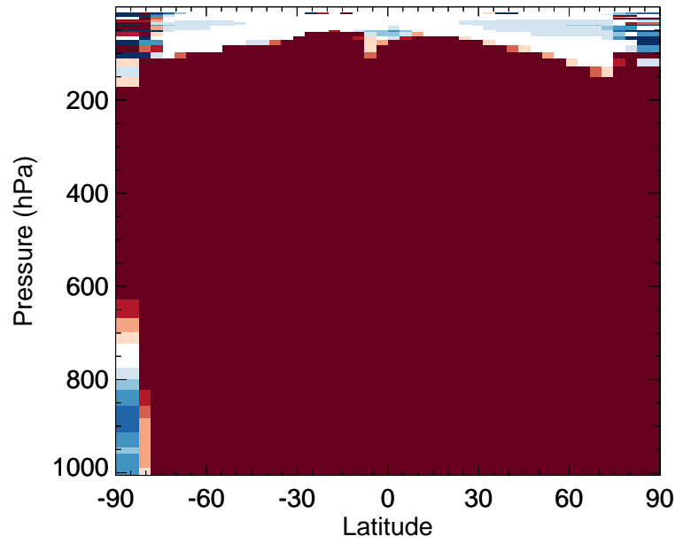
v11-02f-Run0 / v11-02e-Run1 LIMO - Zonal mean % diff for Apr
