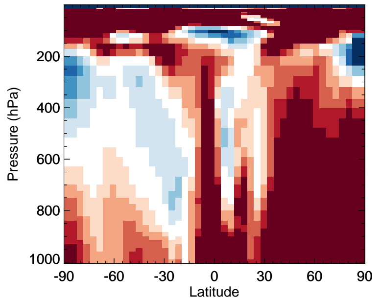
v11-02f-Run0 / v11-02e-Run0 C3H8 - Zonal mean % diff for Apr
