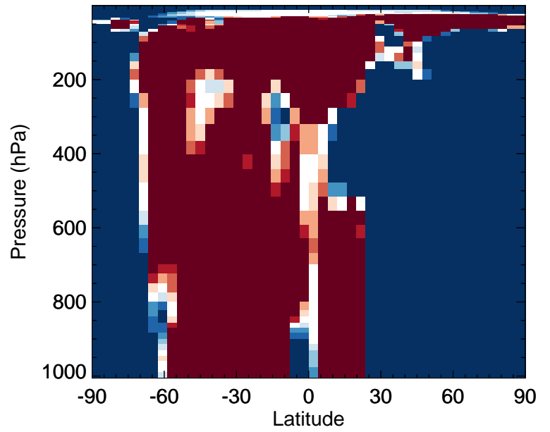
v11-02f-Run0 / v11-02e-Run0 DST4 - Zonal mean % diff for Apr
