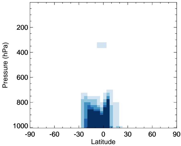
v11-02f-Run0 - v11-02e-Run1 ISOP - Zonal mean abs diff for Apr
