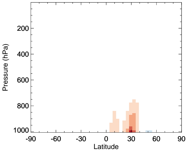
v11-02f-Run0 - v11-02e-Run1 OCPI - Zonal mean abs diff for Apr
