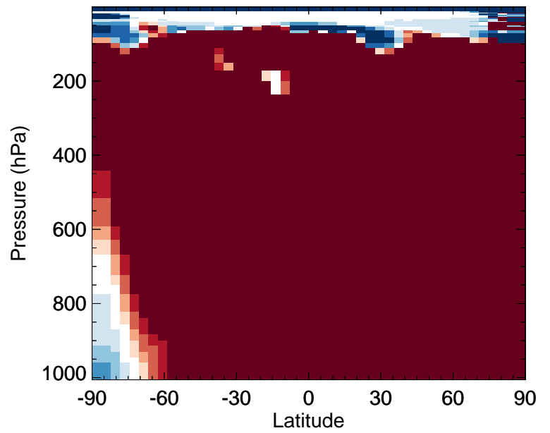
v11-02f-Run0 / v11-02e-Run1 RIPB - Zonal mean % diff for Apr
