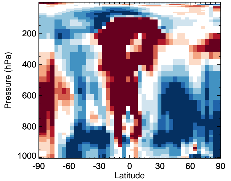
v11-02f-Run0 / v11-02e-Run0 BrCl - Zonal mean % diff for Apr
