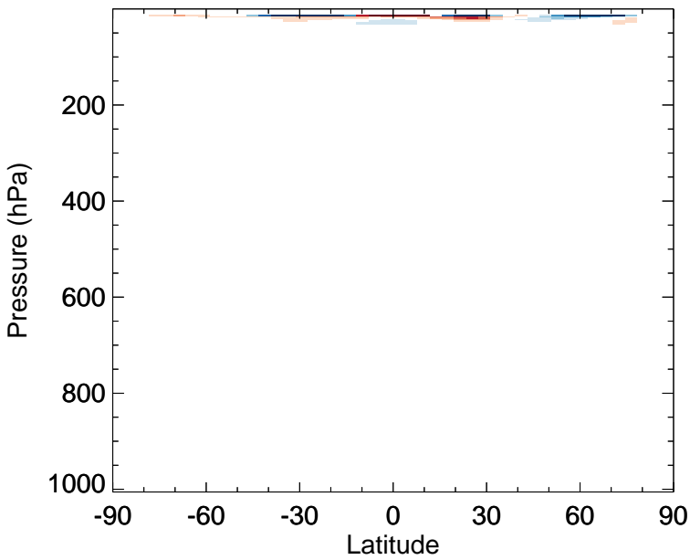
v11-02f-Run0 - v11-02e-Run0 NO 3 - Zonal mean abs diff for Apr
