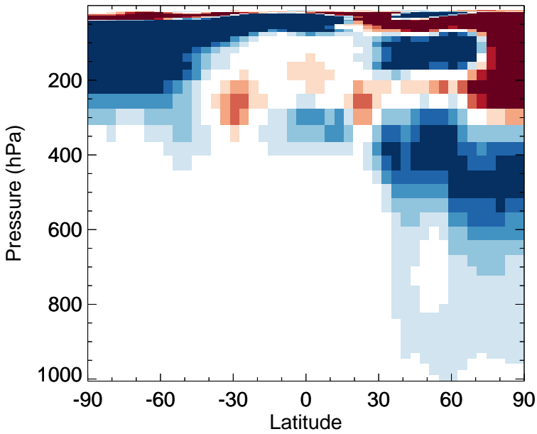
v11-02f-Run0 - v11-02e-Run0 HNO 4 - Zonal mean abs diff for Apr
