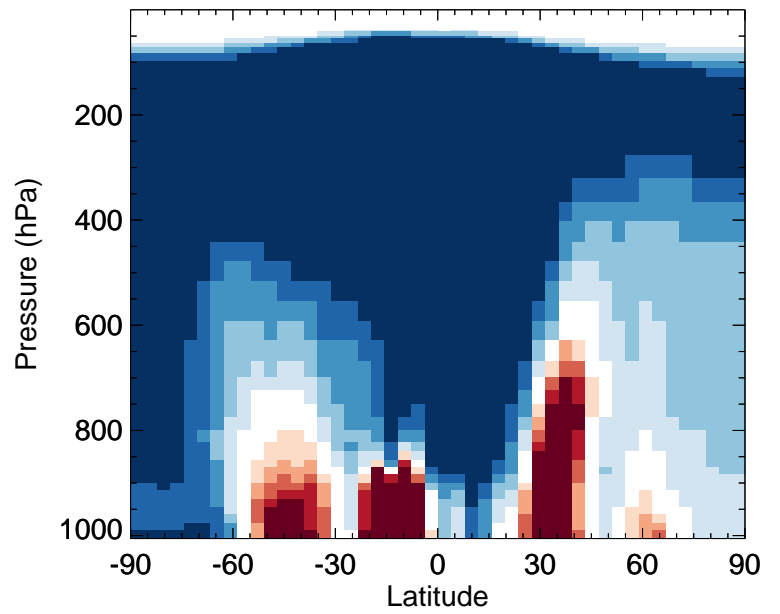
v11-02f-Run0 / v11-02e-Run1 ISOA3 - Zonal mean % diff for Apr
