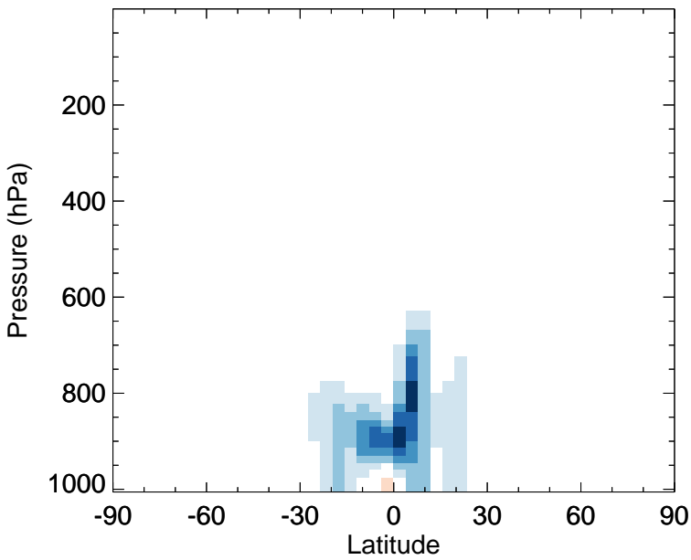
v11-02f-Run0 - v11-02e-Run0 MACR - Zonal mean abs diff for Apr
