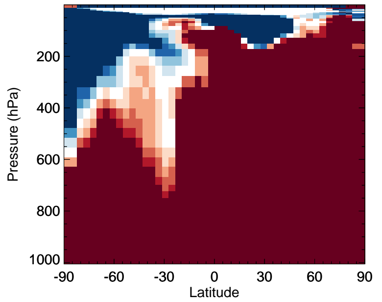
v11-02f-Run0 / v11-02e-Run1 MVK - Zonal mean % diff for Apr
