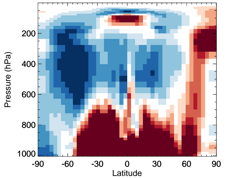
v11-02f-Run0 / v11-02e-Run0 TSOG2 - Zonal mean % diff for Apr
