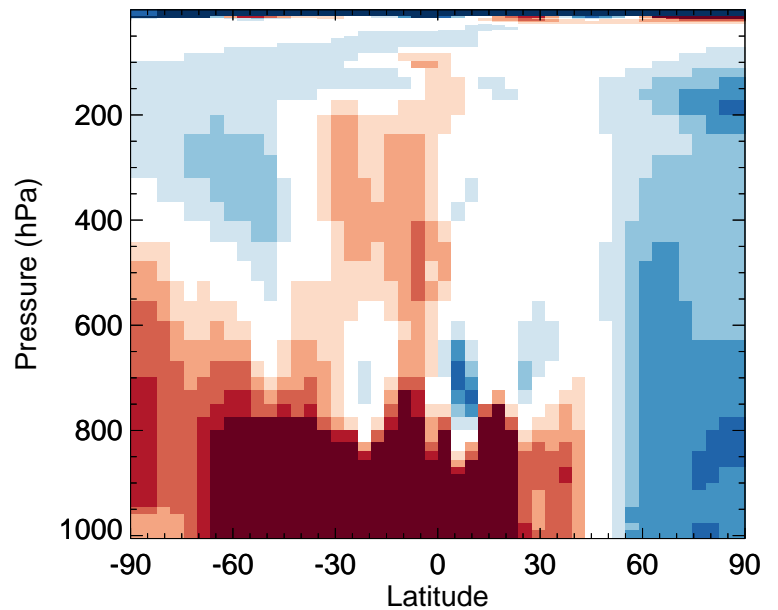
v11-02f-Run0 / v11-02e-Run0 PPN - Zonal mean % diff for Apr
