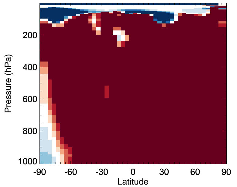
v11-02f-Run0 / v11-02e-Run1 RIPA - Zonal mean % diff for Apr
