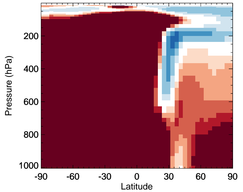
v11-02f-Run0 / v11-02e-Run1 BENZ - Zonal mean % diff for Apr
