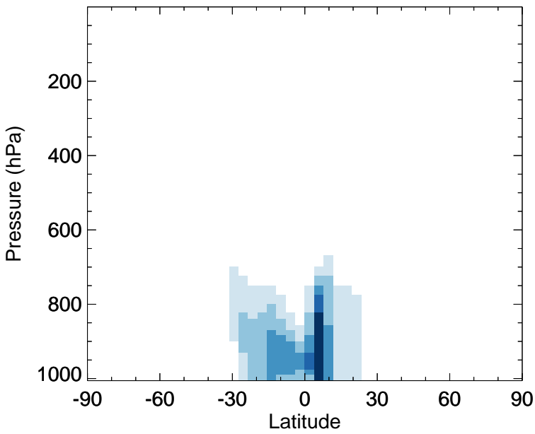
v11-02f-Run0 - v11-02e-Run1 MACR - Zonal mean abs diff for Apr
