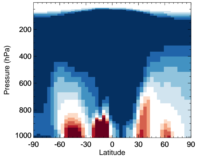
v11-02f-Run0 / v11-02e-Run1 ISOA1 - Zonal mean % diff for Apr
