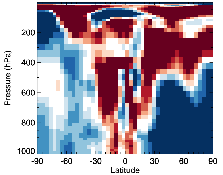
v11-02f-Run0 / v11-02e-Run0 HOCl - Zonal mean % diff for Apr
