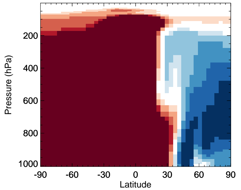
v11-02f-Run0 / v11-02e-Run1 ASOA3 - Zonal mean % diff for Apr
