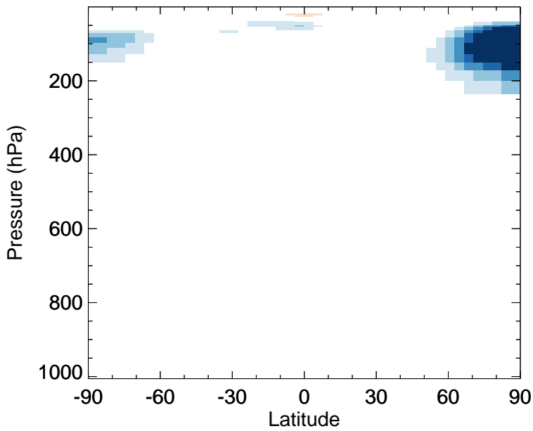
v11-02f-Run0 - v11-02e-Run0 MPN - Zonal mean abs diff for Apr
