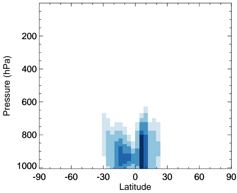
v11-02f-Run0 - v11-02e-Run1 MVK - Zonal mean abs diff for Apr
