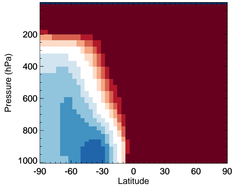
v11-02f-Run0 / v11-02e-Run1 C2H6 - Zonal mean % diff for Apr
