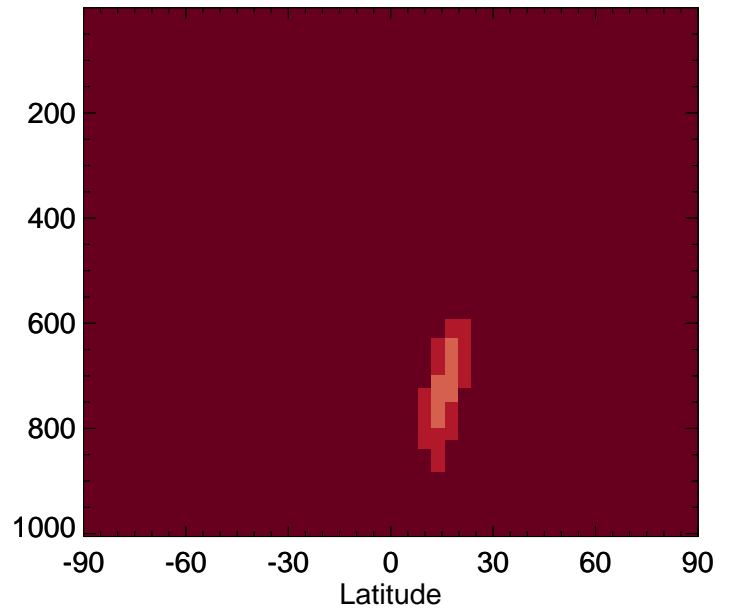
v11-02f-Run0 / v11-02e-Run1 INDIOL - Zonal mean % diff for Apr
