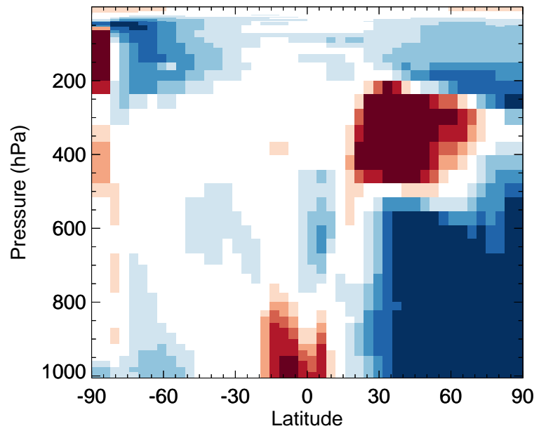
v11-02f-Run0 / v11-02e-Run1 ClOO - Zonal mean % diff for Apr
