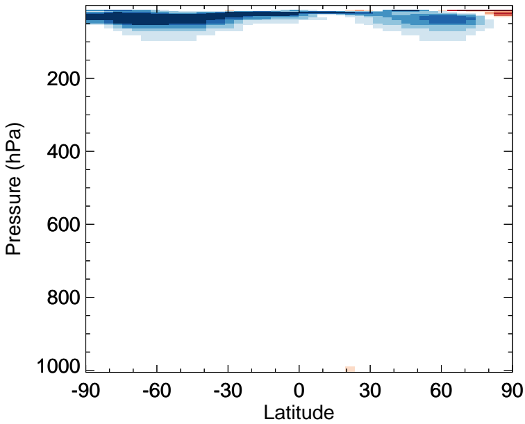
v11-02f-Run0 - v11-02e-Run0 NO 2 - Zonal mean abs diff for Apr
