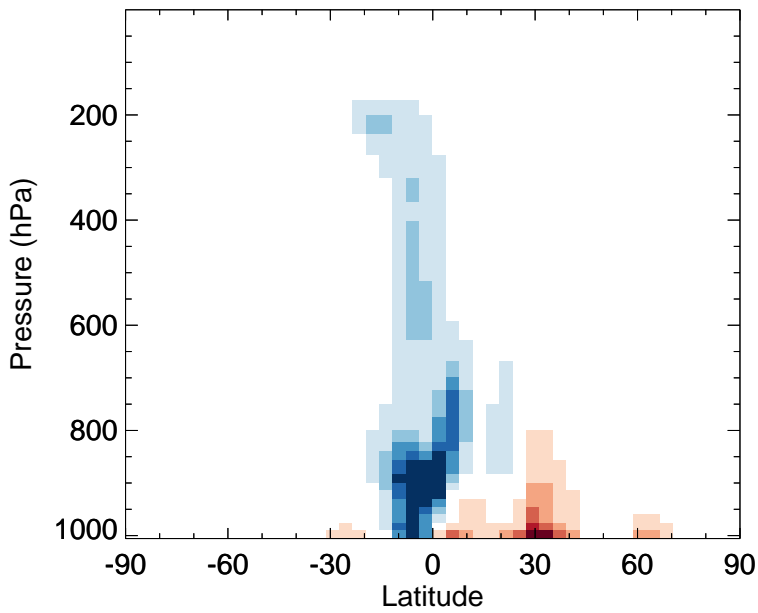
v11-02f-Run0 - v11-02e-Run0 EOH - Zonal mean abs diff for Apr
