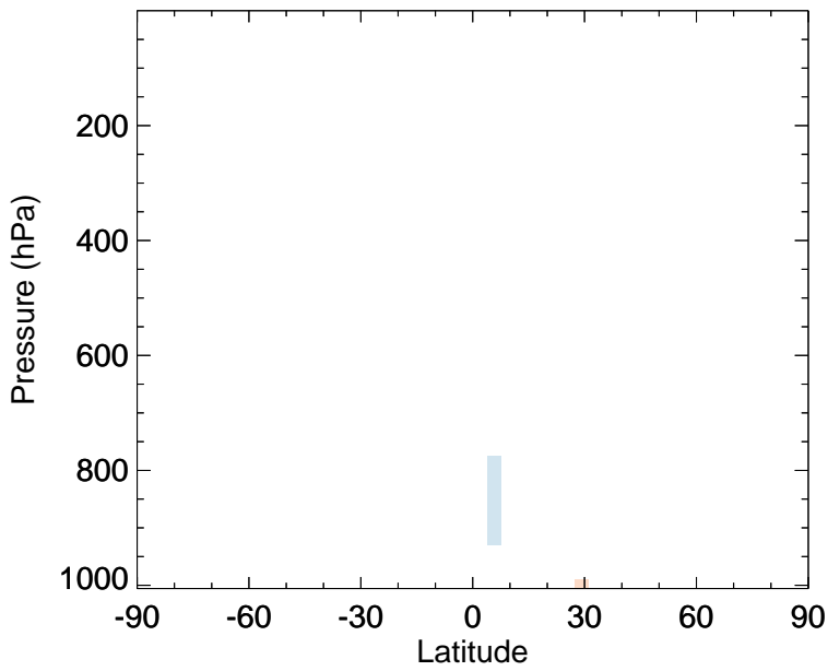
v11-02f-Run0 - v11-02e-Run1 ALD2 - Zonal mean abs diff for Apr
