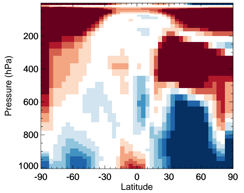
v11-02f-Run0 / v11-02e-Run1 ClO - Zonal mean % diff for Apr
