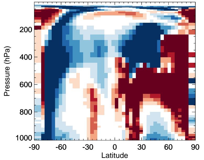
v11-02f-Run0 / v11-02e-Run1 HBr - Zonal mean % diff for Apr
