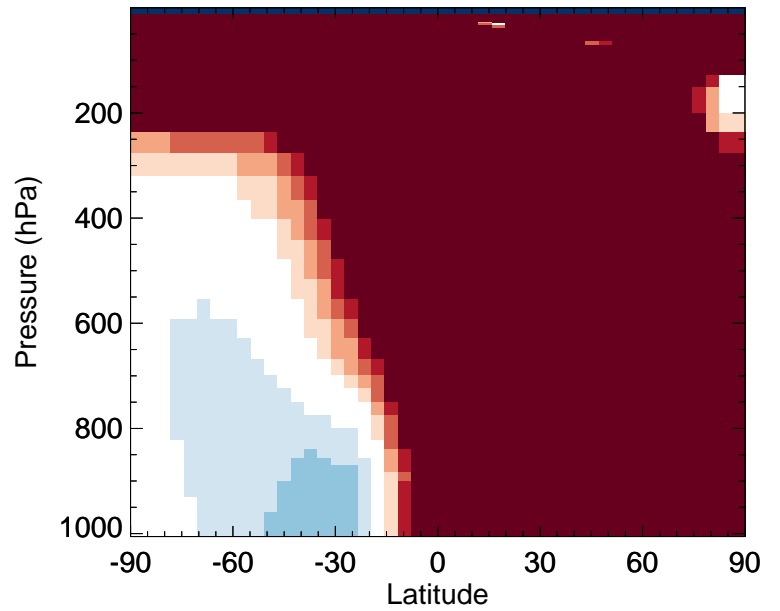
v11-02f-Run0 / v11-02e-Run0 C2H6 - Zonal mean % diff for Apr
