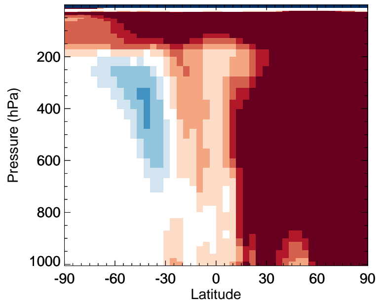
v11-02f-Run0 / v11-02e-Run1 ALD2 - Zonal mean % diff for Apr
