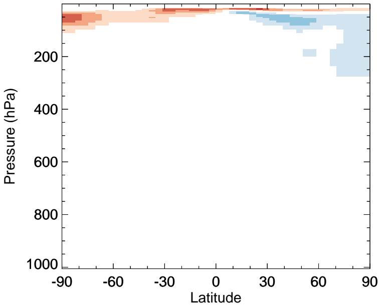
v11-02f-Run0 - v11-02e-Run0 CFC12 - Zonal mean abs diff for Apr
