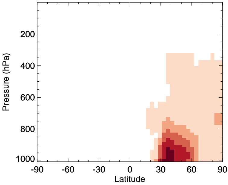
v11-02f-Run0 - v11-02e-Run1 NIT - Zonal mean abs diff for Apr
