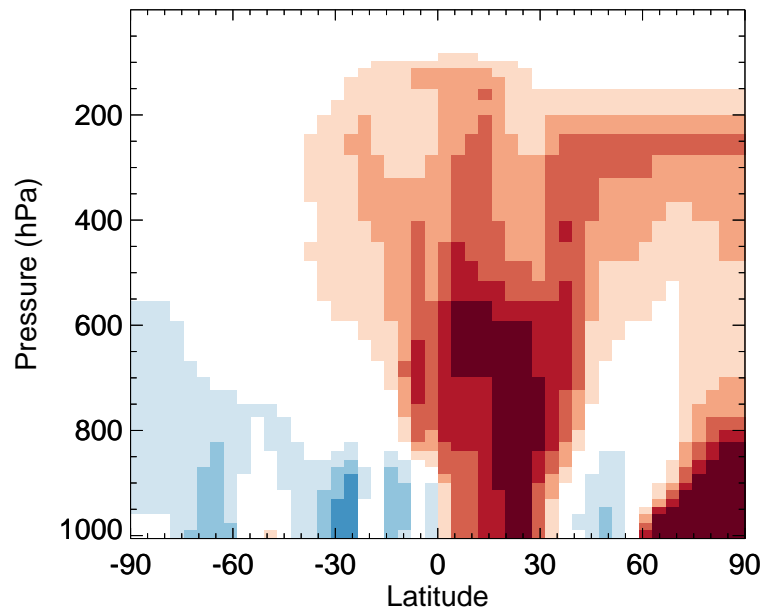
v11-02f-Run0 / v11-02e-Run1 BCPI - Zonal mean % diff for Apr
