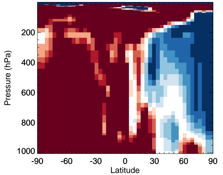
v11-02f-Run0 / v11-02e-Run0 GLYX - Zonal mean % diff for Apr
