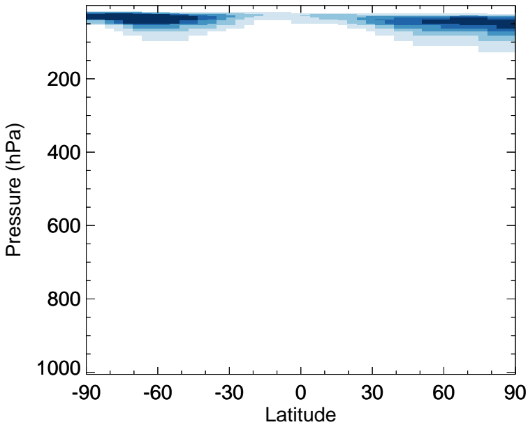
v11-02f-Run0 - v11-02e-Run1 NO 2 - Zonal mean abs diff for Apr
