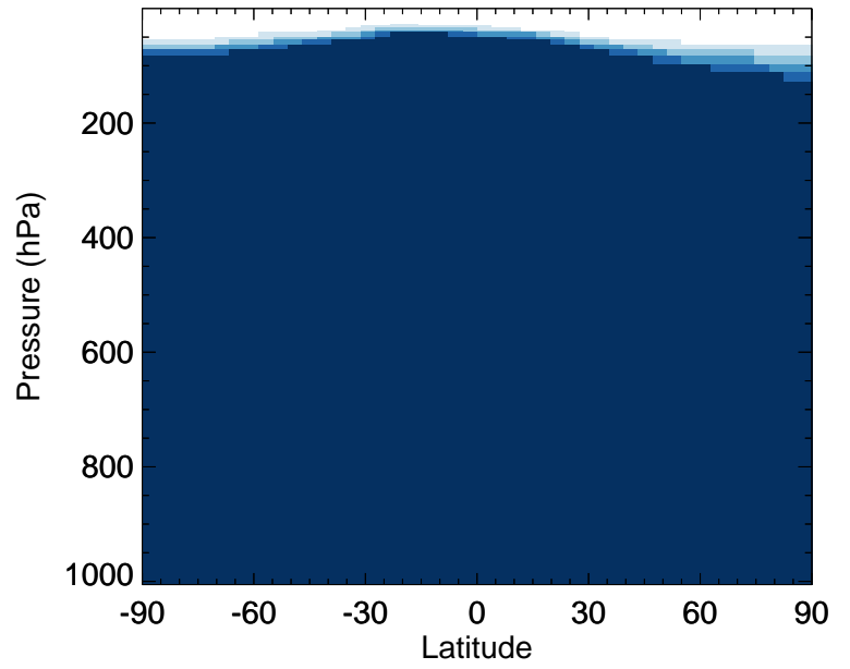
v11-02f-Run0 / v11-02e-Run1 SOAME - Zonal mean % diff for Apr
