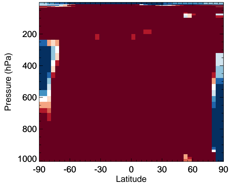
v11-02f-Run0 / v11-02e-Run0 ISN1OG - Zonal mean % diff for Apr
