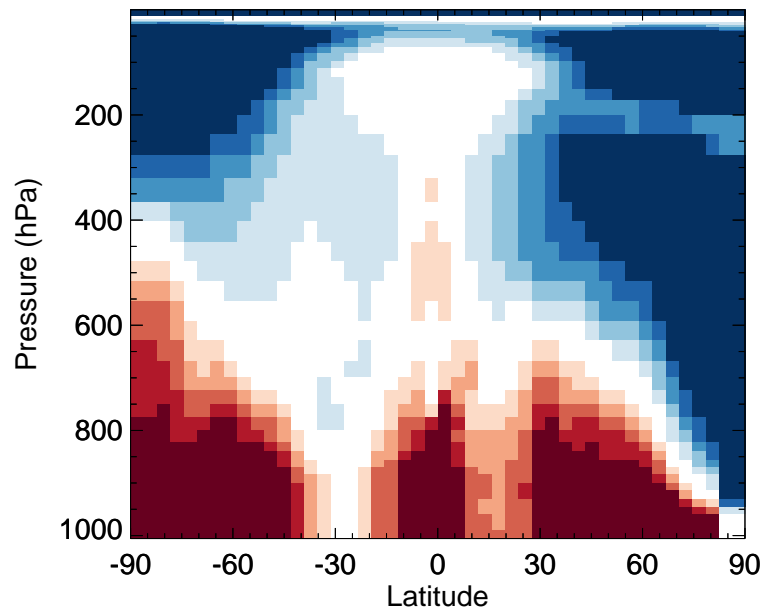
v11-02f-Run0 / v11-02e-Run1 HNO 2 - Zonal mean % diff for Apr
