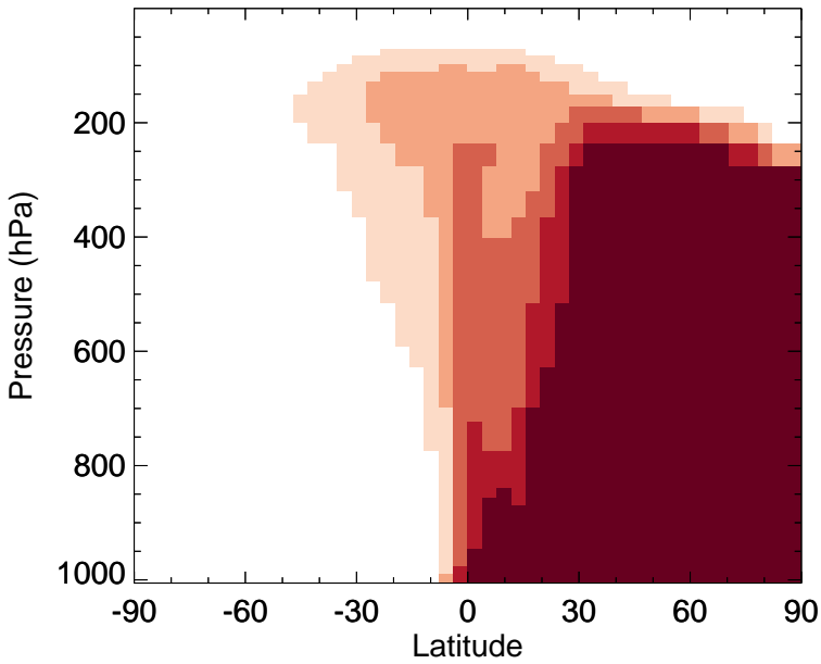
v11-02f-Run0 - v11-02e-Run0 C2H6 - Zonal mean abs diff for Apr
