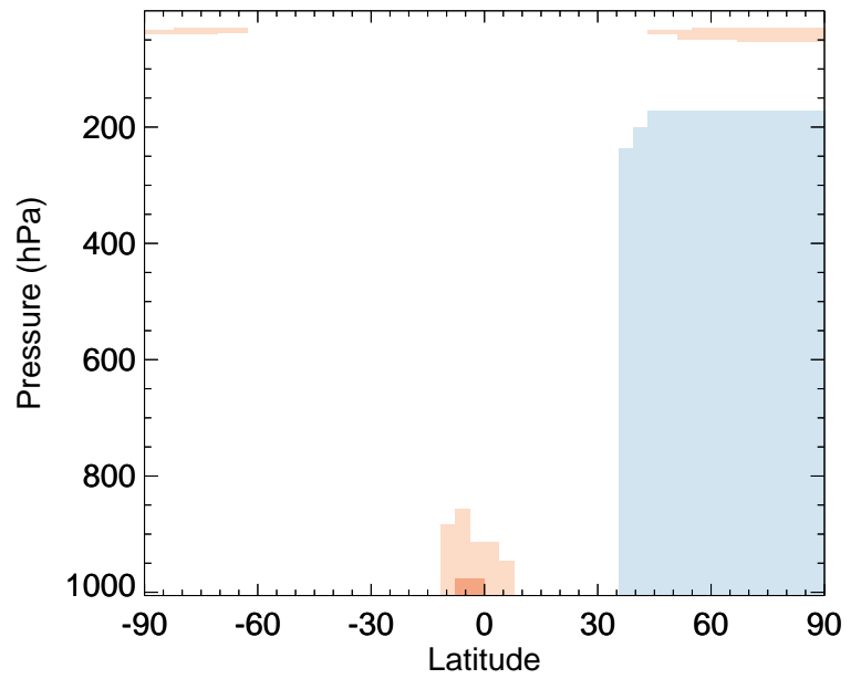
v11-02f-Run0 / v11-02e-Run1 O3 - Zonal mean % diff for Apr
