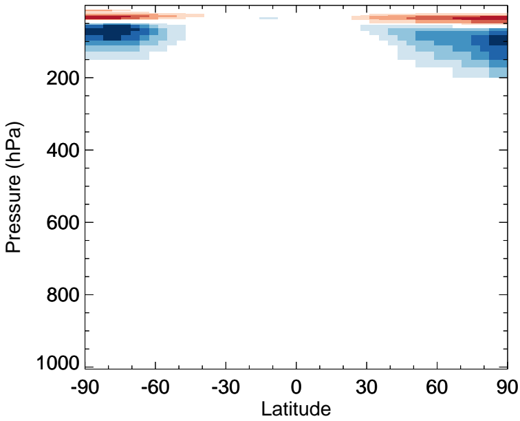
v11-02f-Run0 - v11-02e-Run1 CINO3 - Zonal mean abs diff for Apr
