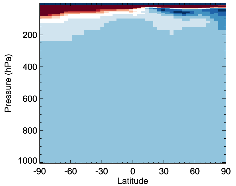
v11-02f-Run0 / v11-02e-Run0 CCI4 - Zonal mean % diff for Apr
