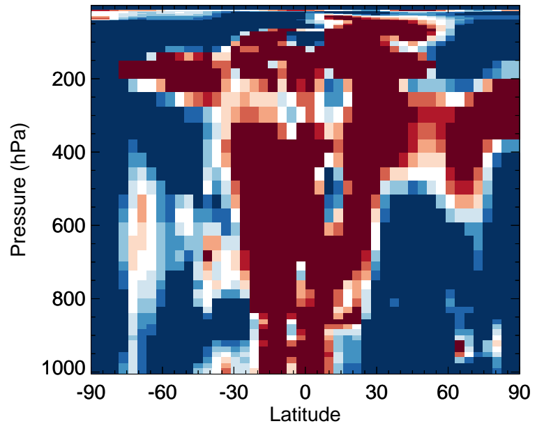
v11-02f-Run0 / v11-02e-Run0 Cl2 - Zonal mean % diff for Apr
