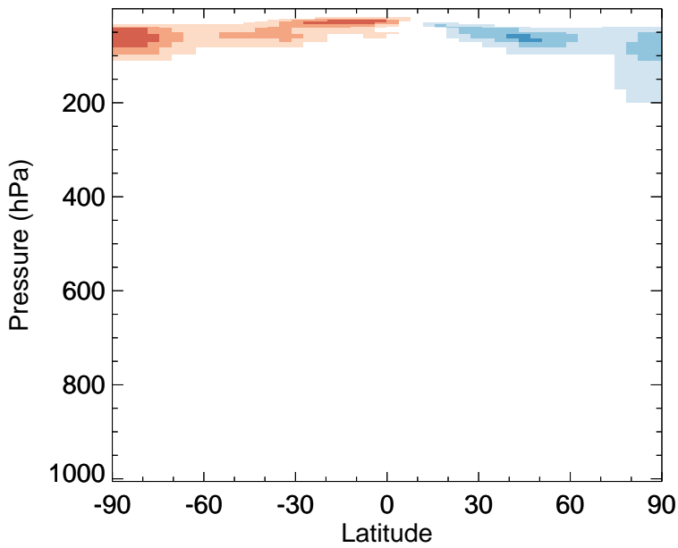
v11-02f-Run0 - v11-02e-Run0 OCS - Zonal mean abs diff for Apr
