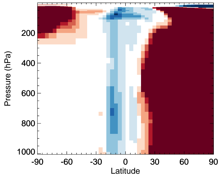
v11-02f-Run0 / v11-02e-Run1 DMS - Zonal mean % diff for Apr
