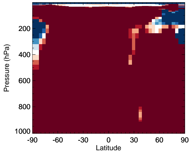
v11-02f-Run0 / v11-02e-Run0 PRPE - Zonal mean % diff for Apr
