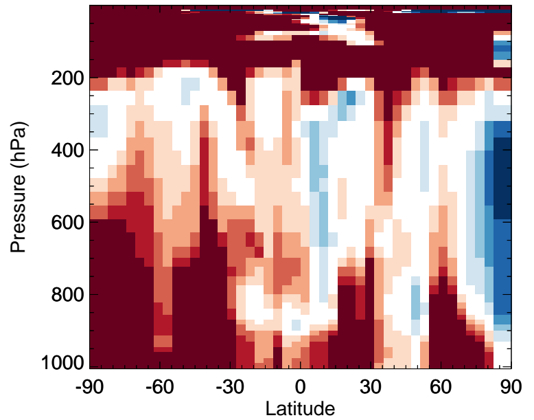
v11-02f-Run0 / v11-02e-Run0 MGLY - Zonal mean % diff for Apr
