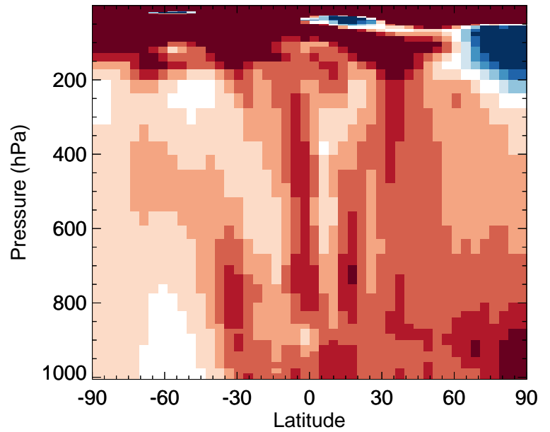
v11-02f-Run0 / v11-02e-Run0 ACET - Zonal mean % diff for Apr
