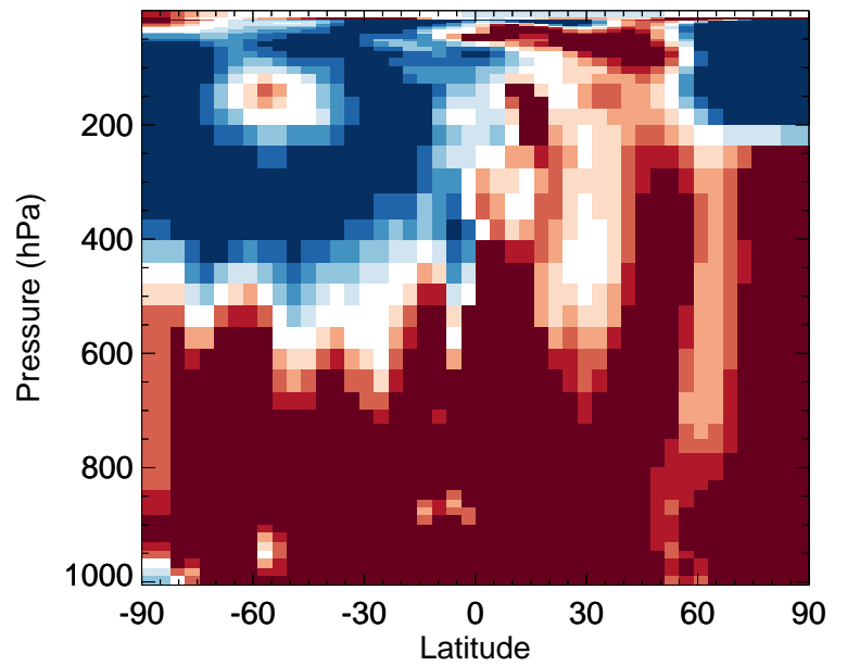
v11-02f-Run0 / v11-02e-Run0 ISOA2 - Zonal mean % diff for Apr
