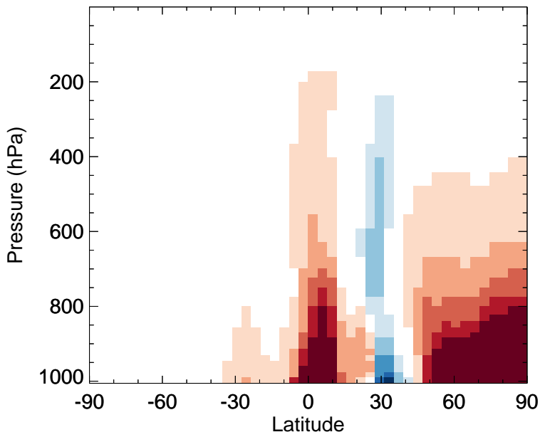
v11-02f-Run0 - v11-02e-Run1 BENZ - Zonal mean abs diff for Apr
