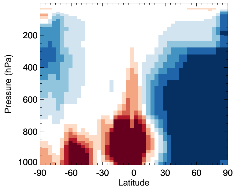
v11-02f-Run0 / v11-02e-Run1 NO 3 - Zonal mean % diff for Apr
