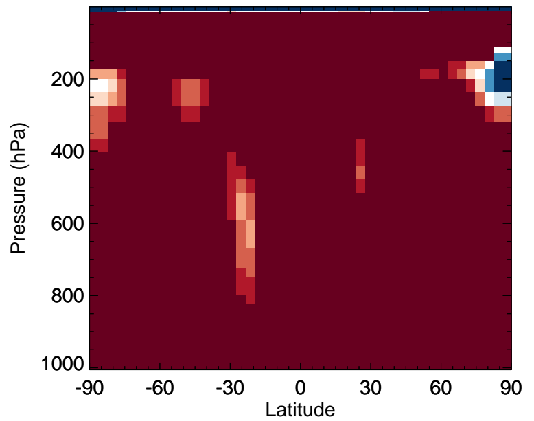
v11-02f-Run0 / v11-02e-Run0 ALK4 - Zonal mean % diff for Apr
