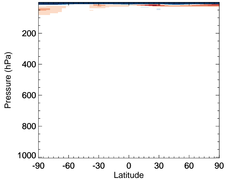
v11-02f-Run0 / v11-02e-Run0 CH4 - Zonal mean % diff for Apr
