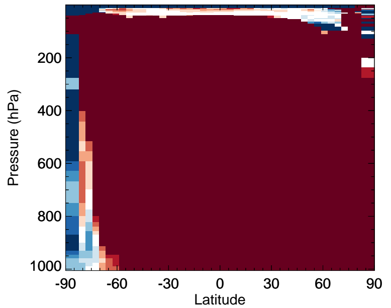
v11-02f-Run0 / v11-02e-Run0 ISOP - Zonal mean % diff for Apr
