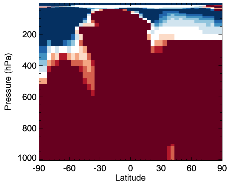
v11-02f-Run0 / v11-02e-Run1 PRPE - Zonal mean % diff for Apr
