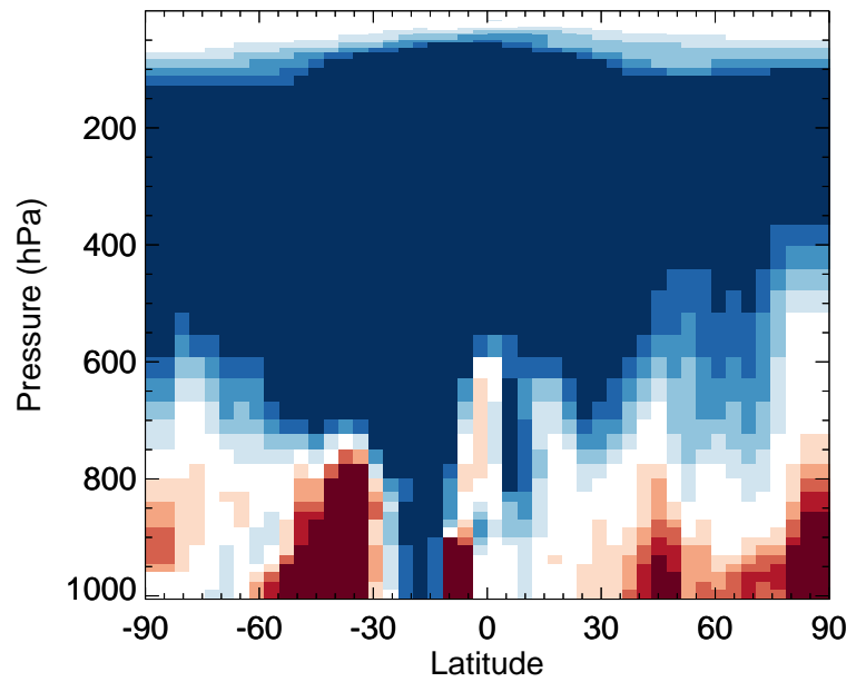
v11-02f-Run0 / v11-02e-Run0 SOAGX - Zonal mean % diff for Apr
