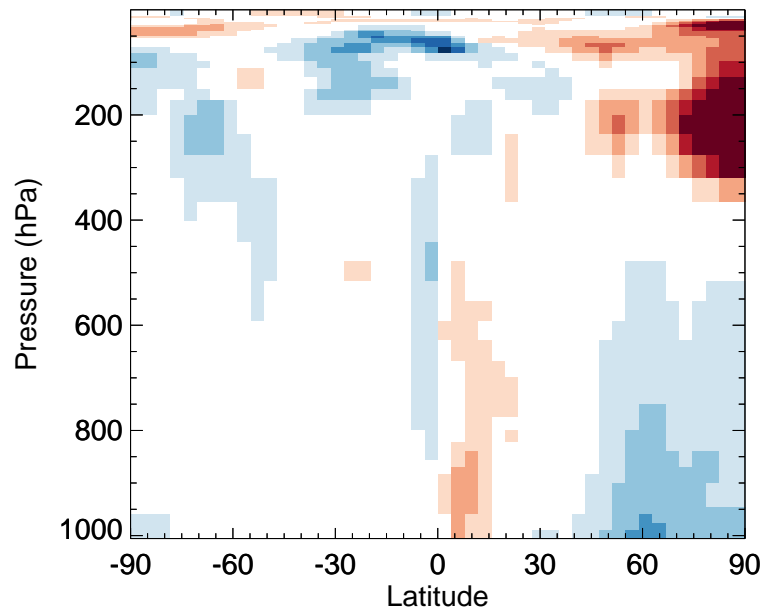
v11-02f-Run0 / v11-02e-Run0 O3 - Zonal mean % diff for Apr
