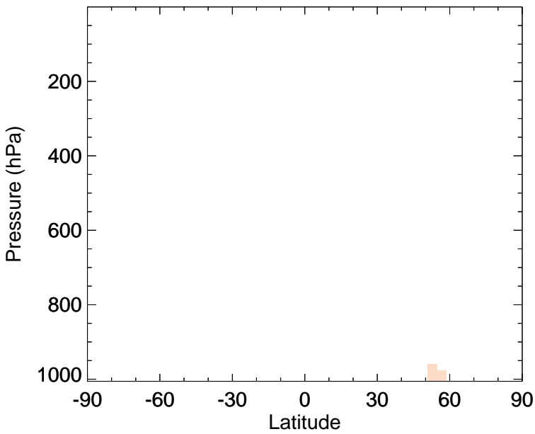
v11-02f-Run0 - v11-02e-Run0 SO4 - Zonal mean abs diff for Apr
