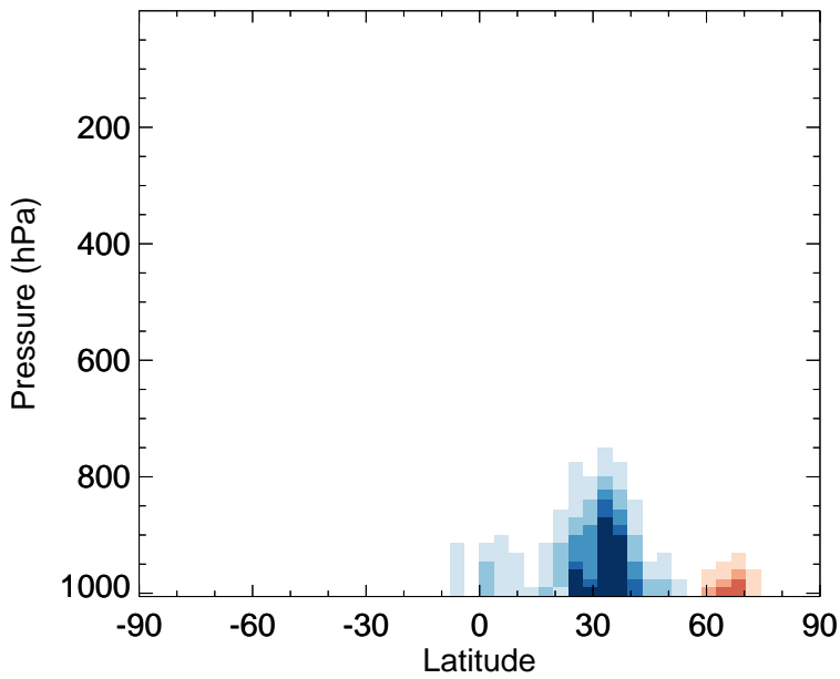
v11-02f-Run0 - v11-02e-Run0 XYLE - Zonal mean abs diff for Apr
