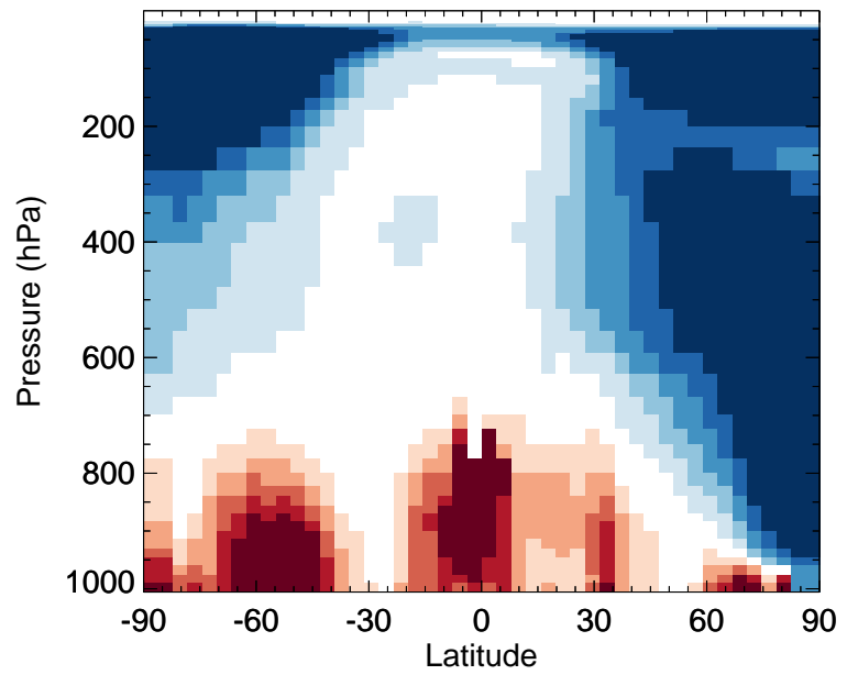
v11-02f-Run0 / v11-02e-Run1 NO - Zonal mean % diff for Apr
