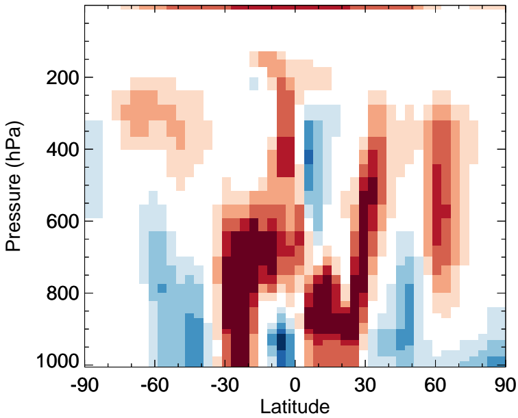
v11-02f-Run0 - v11-02e-Run0 MP - Zonal mean abs diff for Apr
