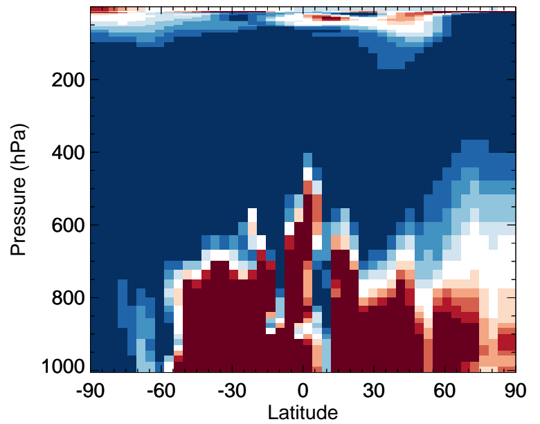
v11-02f-Run0 / v11-02e-Run0 ISOA1 - Zonal mean % diff for Apr
