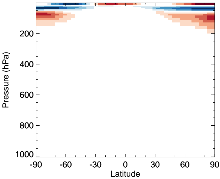
v11-02f-Run0 - v11-02e-Run1 HCl - Zonal mean abs diff for Apr
