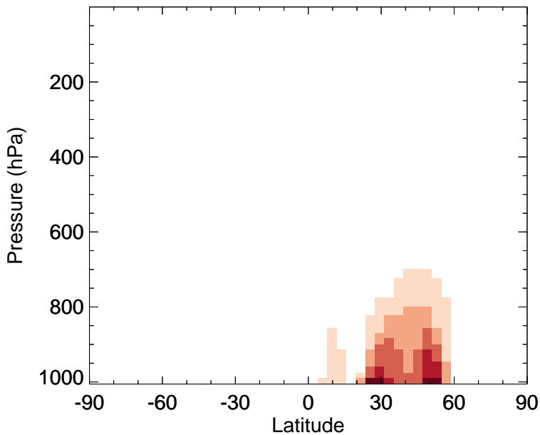
v11-02f-Run0 - v11-02e-Run0 OCPI - Zonal mean abs diff for Apr
