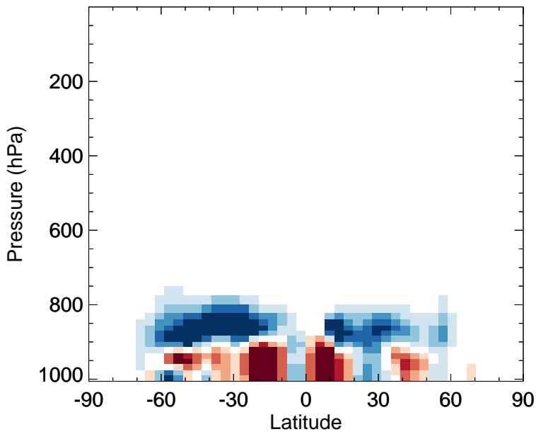
v11-02f-Run0 - v11-02e-Run0 SALC - Zonal mean abs diff for Apr
