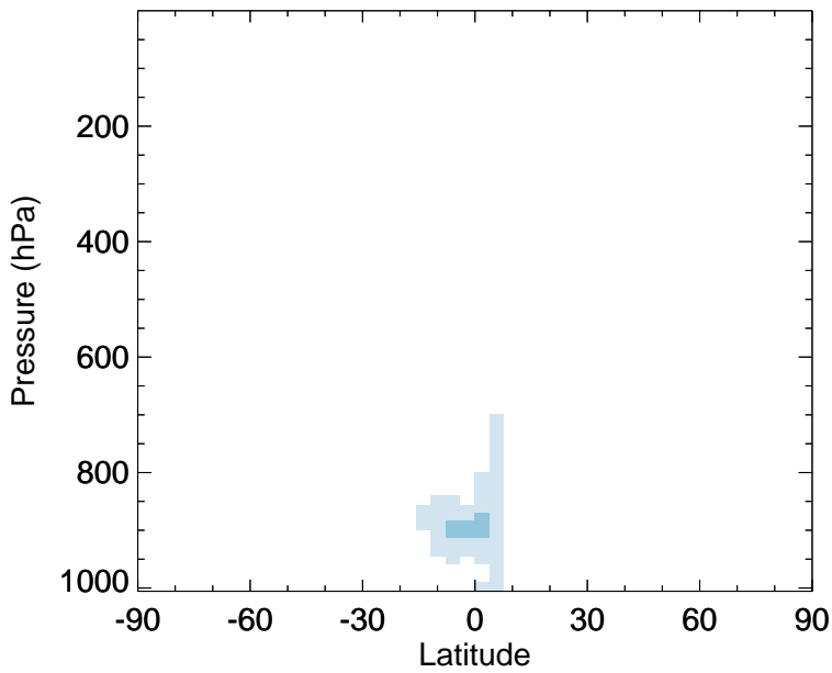
v11-02f-Run0 - v11-02e-Run0 RIPA - Zonal mean abs diff for Apr
