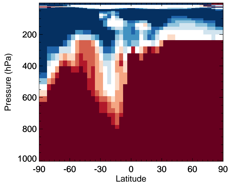
v11-02f-Run0 / v11-02e-Run1 MACR - Zonal mean % diff for Apr
