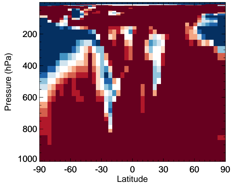
v11-02f-Run0 / v11-02e-Run0 GLYC - Zonal mean % diff for Apr
