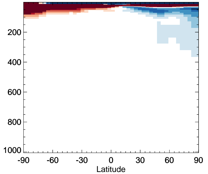
v11-02f-Run0 / v11-02e-Run0 CFC11 - Zonal mean % diff for Apr
