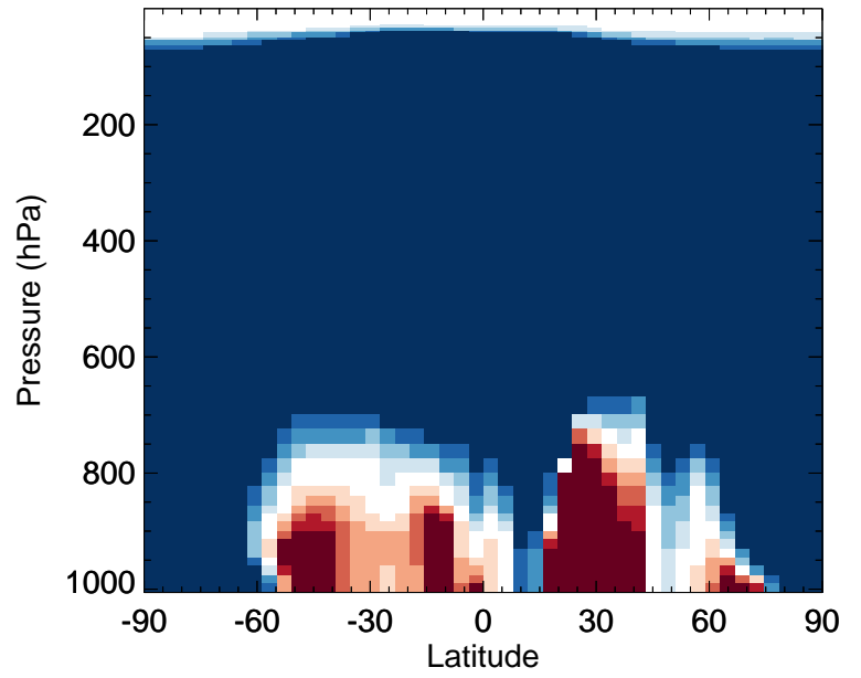
v11-02f-Run0 / v11-02e-Run1 DHDN - Zonal mean % diff for Apr
