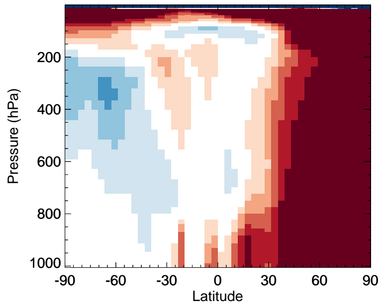
v11-02f-Run0 / v11-02e-Run1 C3H8 - Zonal mean % diff for Apr
