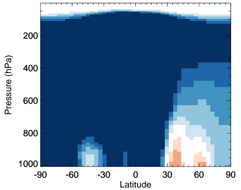
v11-02f-Run0 / v11-02e-Run1 ISO3 - Zonal mean % diff for Apr
