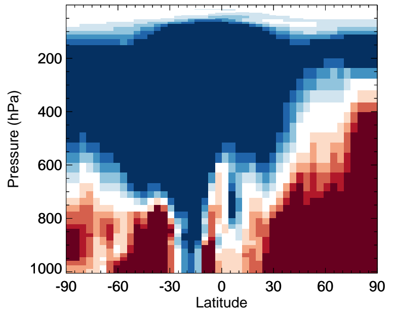
v11-02f-Run0 / v11-02e-Run0 SOAMG - Zonal mean % diff for Apr
