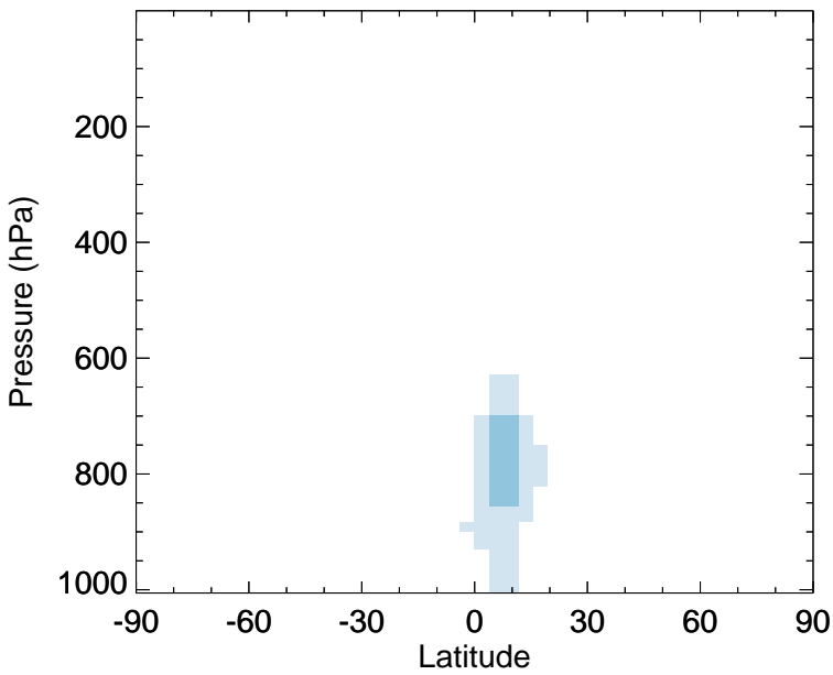
v11-02f-Run0 - v11-02e-Run0 ISO3 - Zonal mean abs diff for Apr
