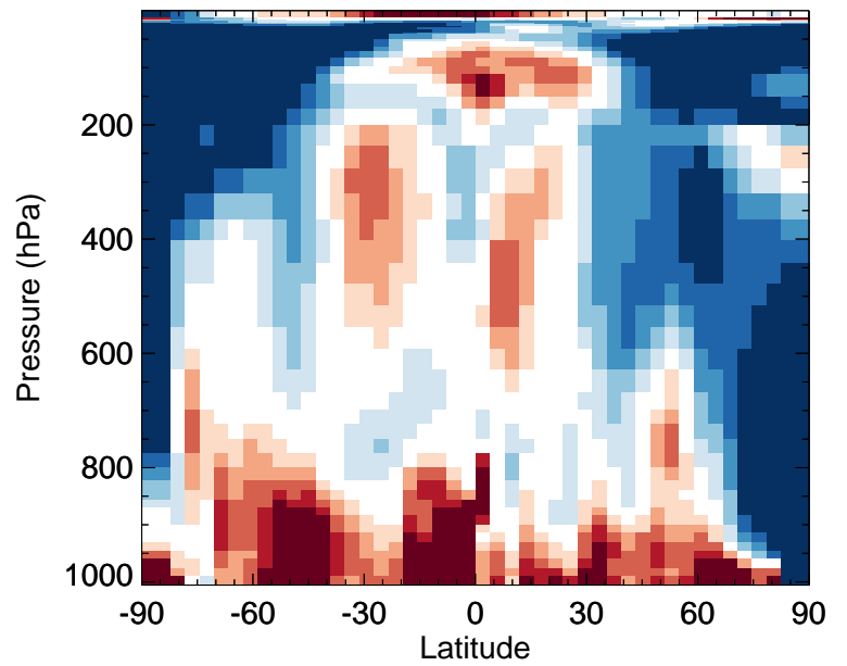
v11-02f-Run0 / v11-02e-Run0 NO - Zonal mean % diff for Apr
