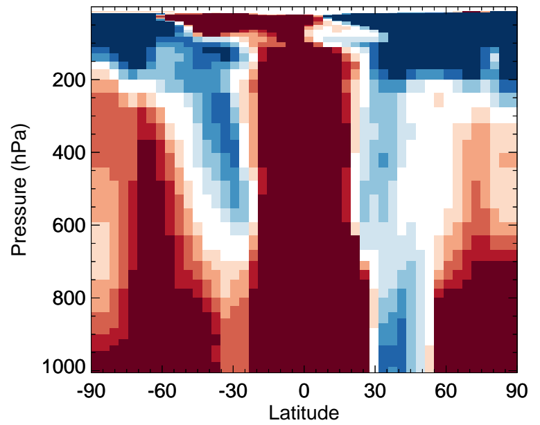
v11-02f-Run0 / v11-02e-Run1 TOLU - Zonal mean % diff for Apr
