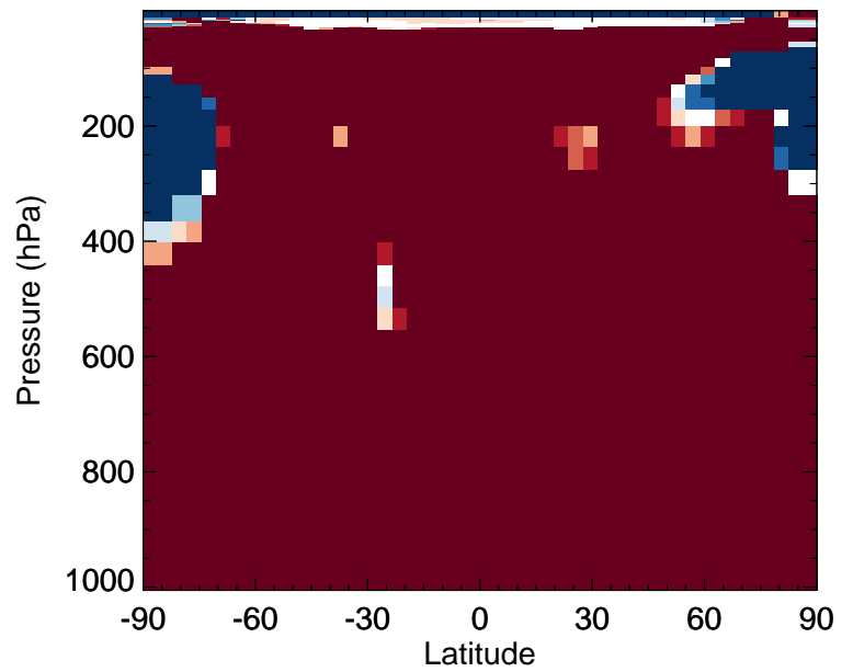
v11-02f-Run0 / v11-02e-Run0 IPMN - Zonal mean % diff for Apr
