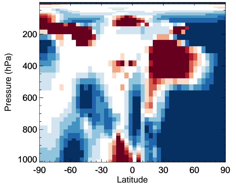
v11-02f-Run0 / v11-02e-Run1 Cl2 - Zonal mean % diff for Apr
