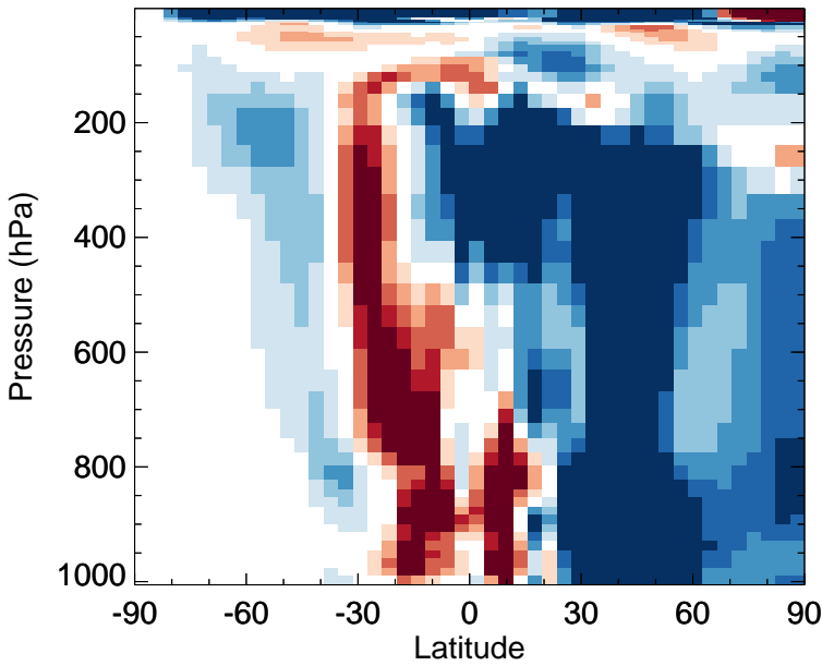
v11-02f-Run0 - v11-02e-Run0 OH - Zonal mean abs diff for Apr
