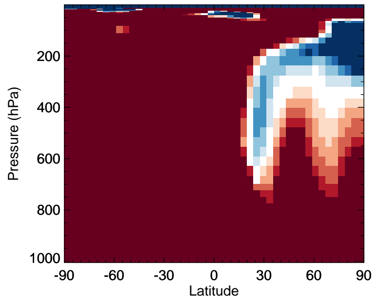
v11-02f-Run0 / v11-02e-Run0 BENZ - Zonal mean % diff for Apr
