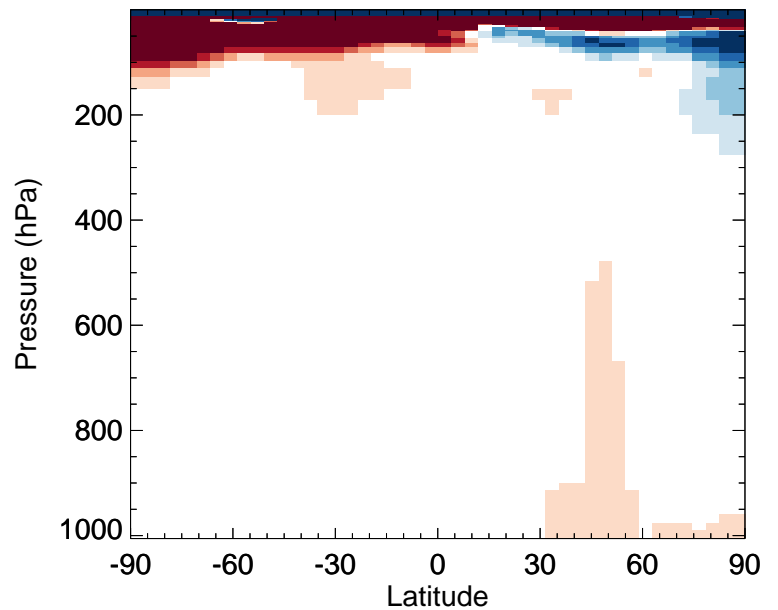
v11-02f-Run0 / v11-02e-Run0 CH 2 Br 2 - Zonal mean % diff for Apr
