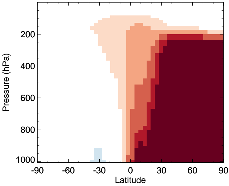
v11-02f-Run0 - v11-02e-Run1 C2H6 - Zonal mean abs diff for Apr
