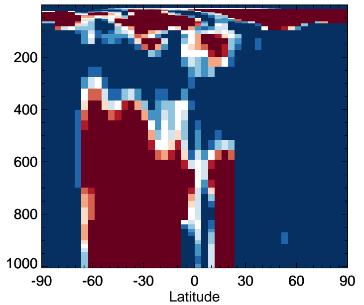
v11-02f-Run0 / v11-02e-Run0 DST3 - Zonal mean % diff for Apr
