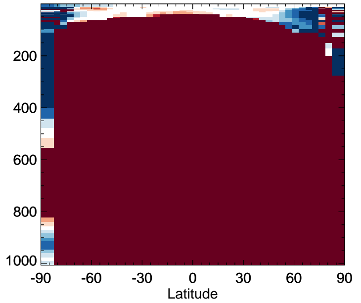
v11-02f-Run0 / v11-02e-Run0 MTPA - Zonal mean % diff for Apr
