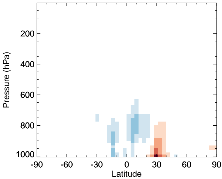
v11-02f-Run0 - v11-02e-Run1 EOH - Zonal mean abs diff for Apr
