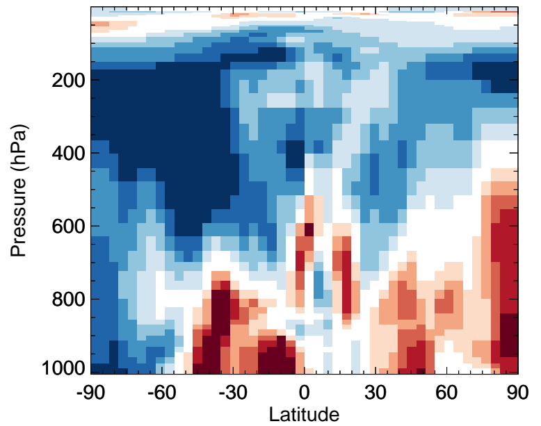
v11-02f-Run0 / v11-02e-Run0 SOAS - Zonal mean % diff for Apr
