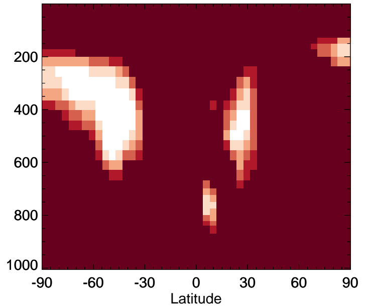
v11-02f-Run0 / v11-02e-Run0 INDIOL - Zonal mean % diff for Apr
