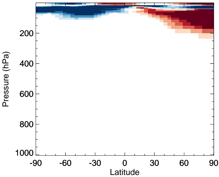
v11-02f-Run0 - v11-02e-Run0 HCl - Zonal mean abs diff for Apr
