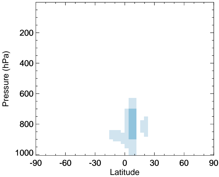
v11-02f-Run0 - v11-02e-Run0 GLYC - Zonal mean abs diff for Apr
