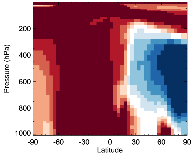
v11-02f-Run0 / v11-02e-Run1 R4N2 - Zonal mean % diff for Apr
