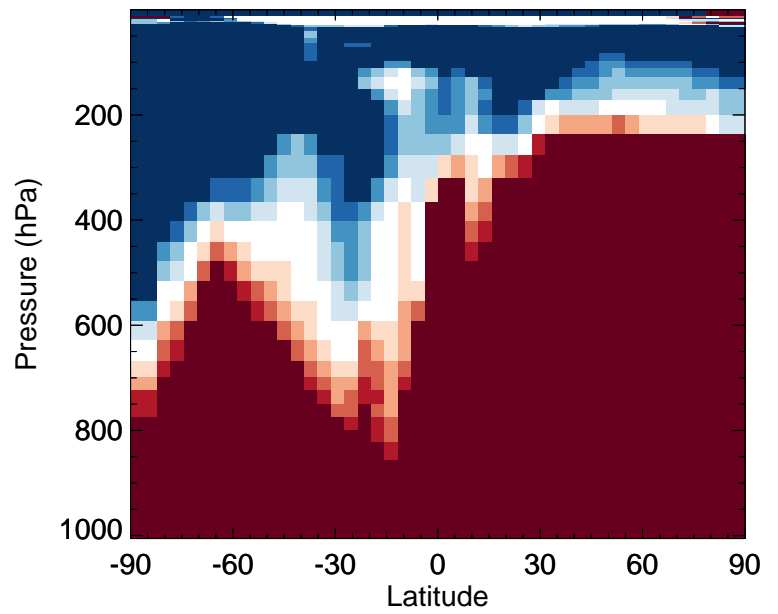
v11-02f-Run0 / v11-02e-Run1 IPMN - Zonal mean % diff for Apr
