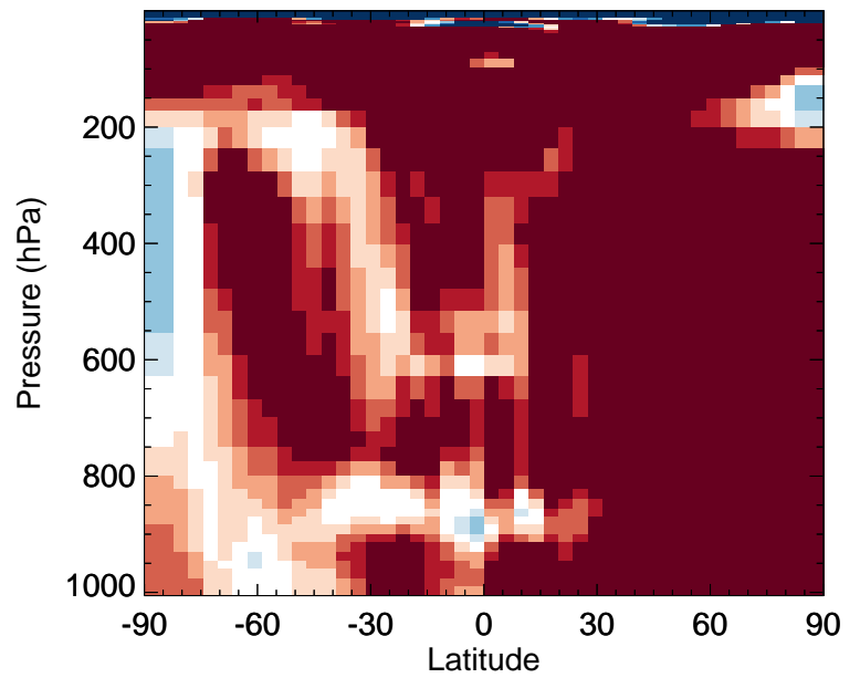
v11-02f-Run0 / v11-02e-Run0 ALD2 - Zonal mean % diff for Apr
