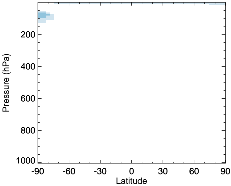
v11-02f-Run0 - v11-02e-Run0 HOCl - Zonal mean abs diff for Apr
