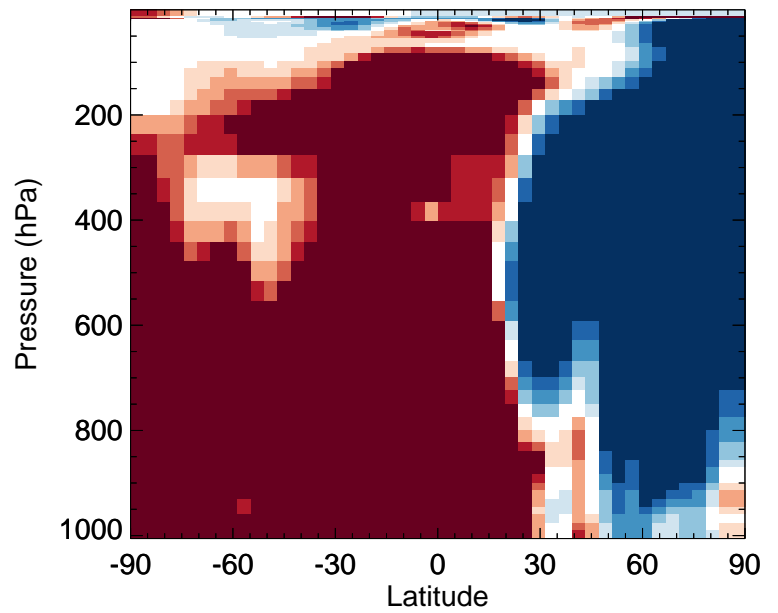
v11-02f-Run0 / v11-02e-Run0 ASOA1 - Zonal mean % diff for Apr
