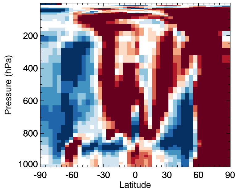
v11-02f-Run0 / v11-02e-Run0 Br2 - Zonal mean % diff for Jan
