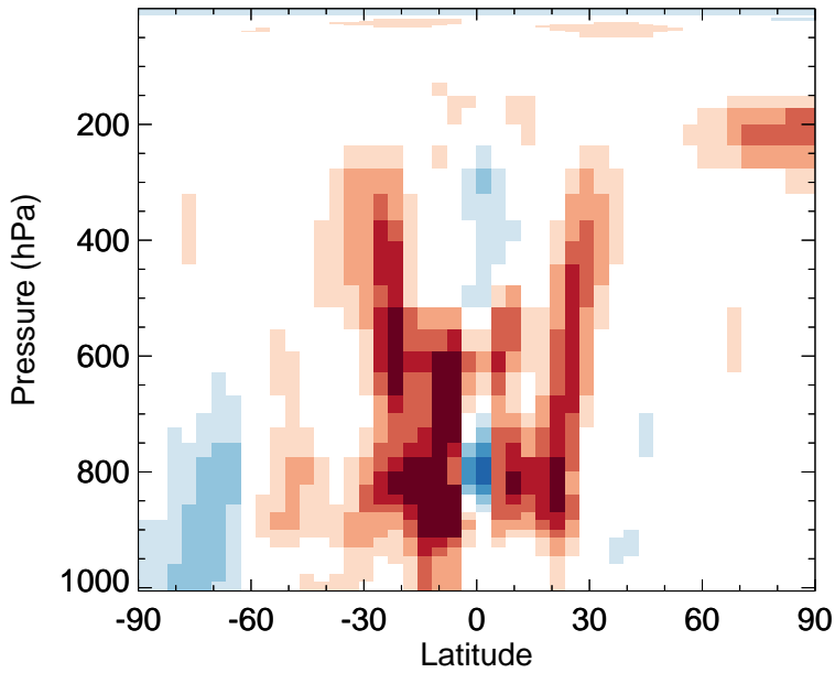
v11-02f-Run0 - v11-02e-Run0 H2O2 - Zonal mean abs diff for Jan
