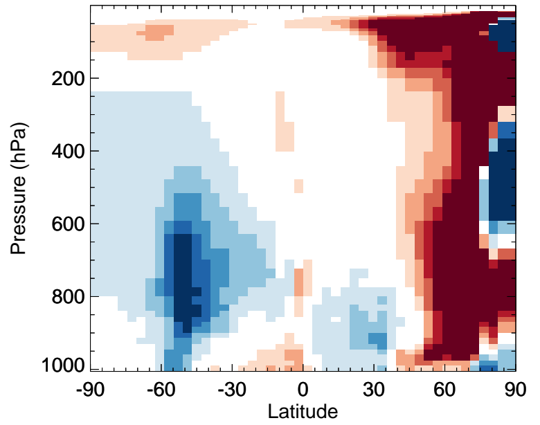
v11-02f-Run0 / v11-02e-Run1 BrO - Zonal mean % diff for Jan
