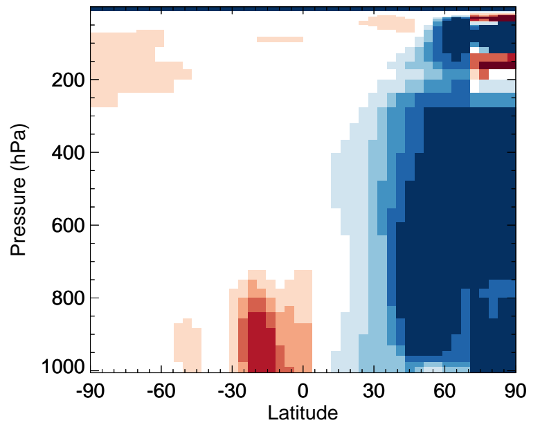
v11-02f-Run0 / v11-02e-Run1 OH - Zonal mean % diff for Jan
