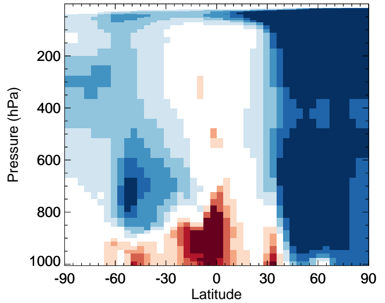
v11-02f-Run0 / v11-02e-Run1 BrNO2 - Zonal mean % diff for Jan
