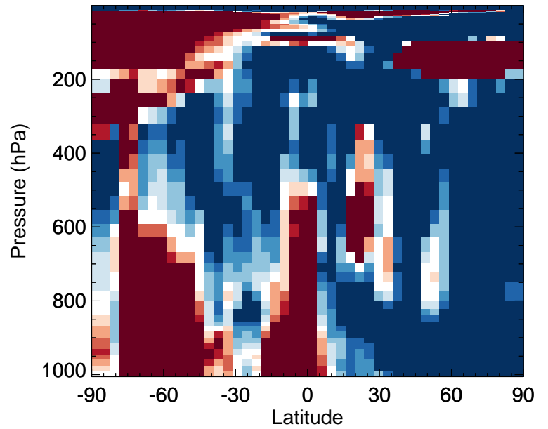
v11-02f-Run0 / v11-02e-Run0 CINO2 - Zonal mean % diff for Jan
