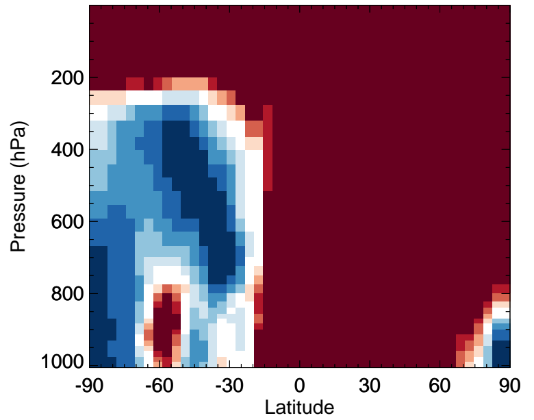
v11-02f-Run0 / v11-02e-Run0 INDIOL - Zonal mean % diff for Jan
