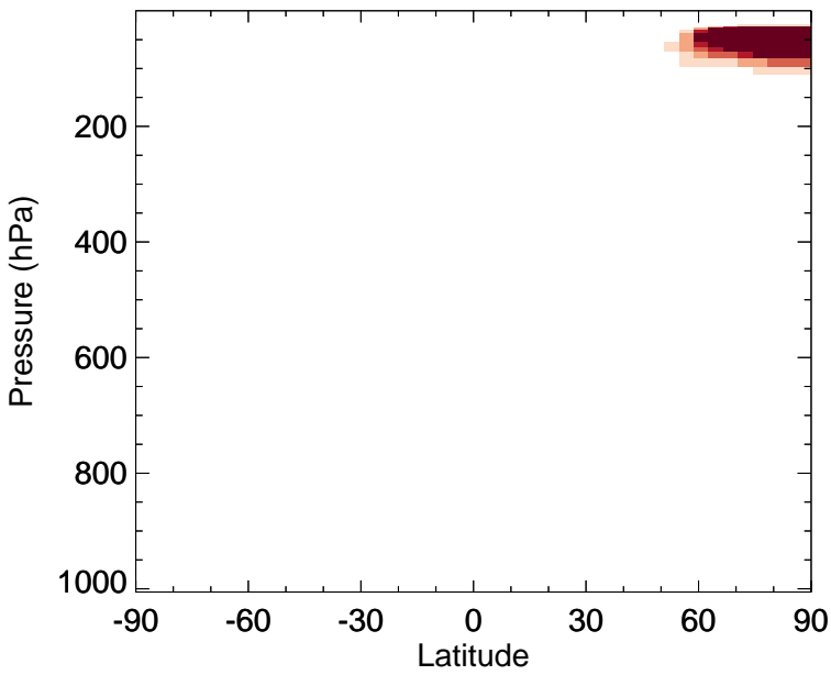
v11-02f-Run0 - v11-02e-Run1 Cl2O2 - Zonal mean abs diff for Jan
