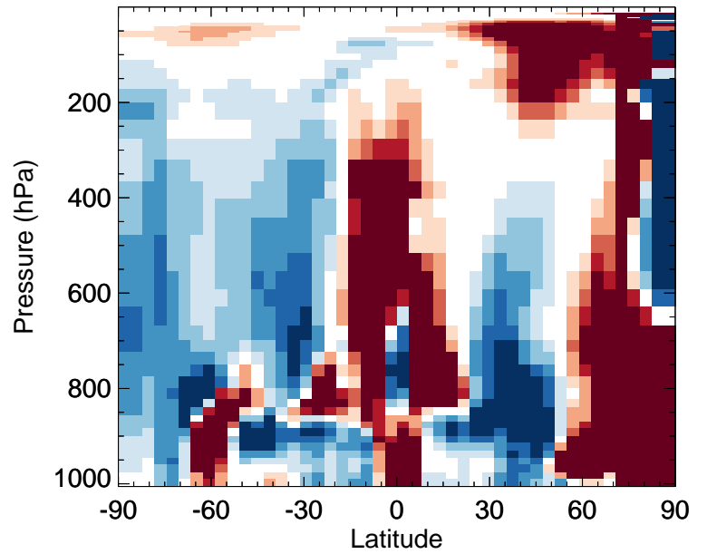
v11-02f-Run0 / v11-02e-Run0 BrO - Zonal mean % diff for Jan
