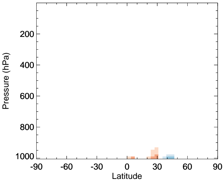
v11-02f-Run0 - v11-02e-Run0 SOAP - Zonal mean abs diff for Jan
