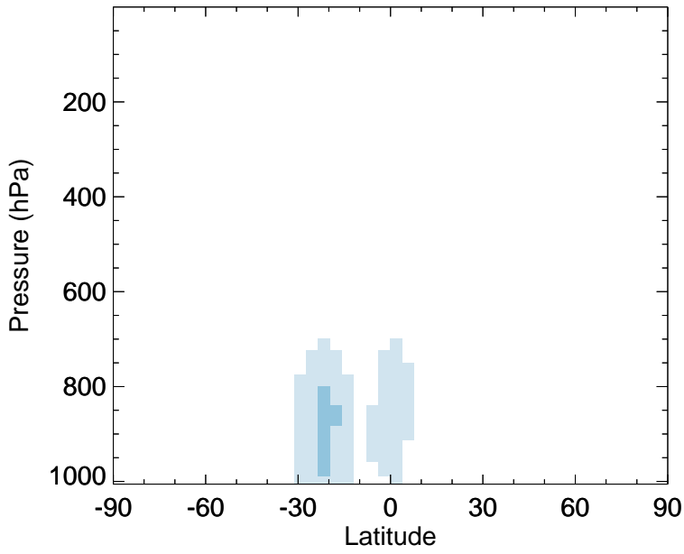
v11-02f-Run0 - v11-02e-Run1 GLYC - Zonal mean abs diff for Jan
