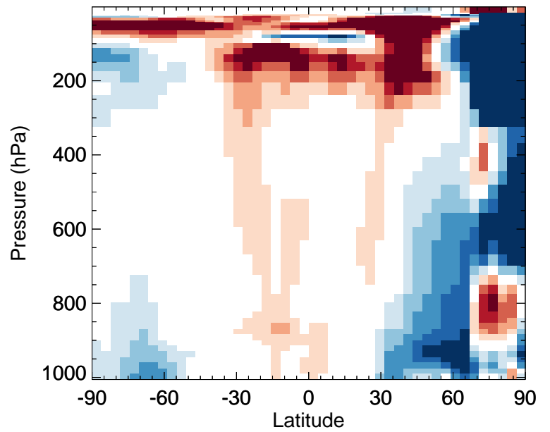
v11-02f-Run0 / v11-02e-Run0 HO2 - Zonal mean % diff for Jan
