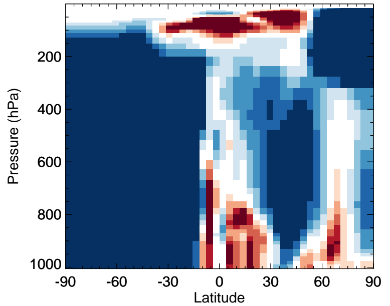
v11-02f-Run0 / v11-02e-Run0 ISO G 1 - Zonal mean % diff for Jan
