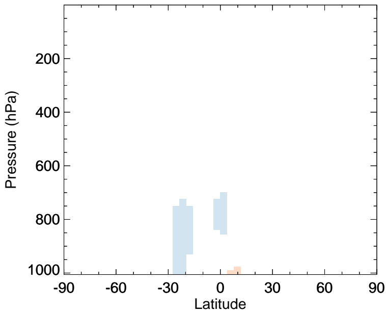
v11-02f-Run0 - v11-02e-Run1 HAC - Zonal mean abs diff for Jan
