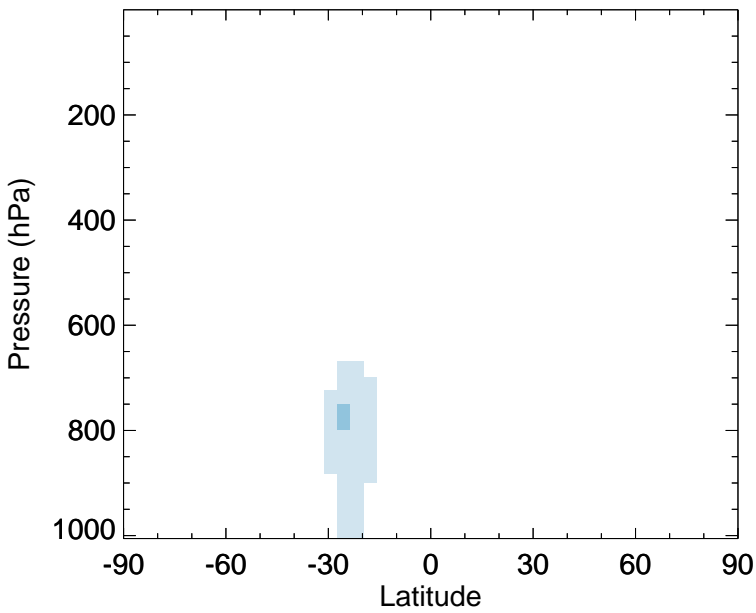
v11-02f-Run0 - v11-02e-Run0 IEPOXA - Zonal mean abs diff for Jan
