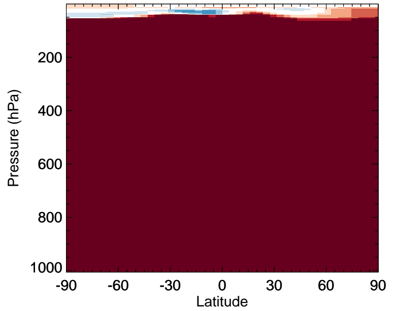
v11-02f-Run0 / v11-02e-Run0 NH3 - Zonal mean % diff for Jan
