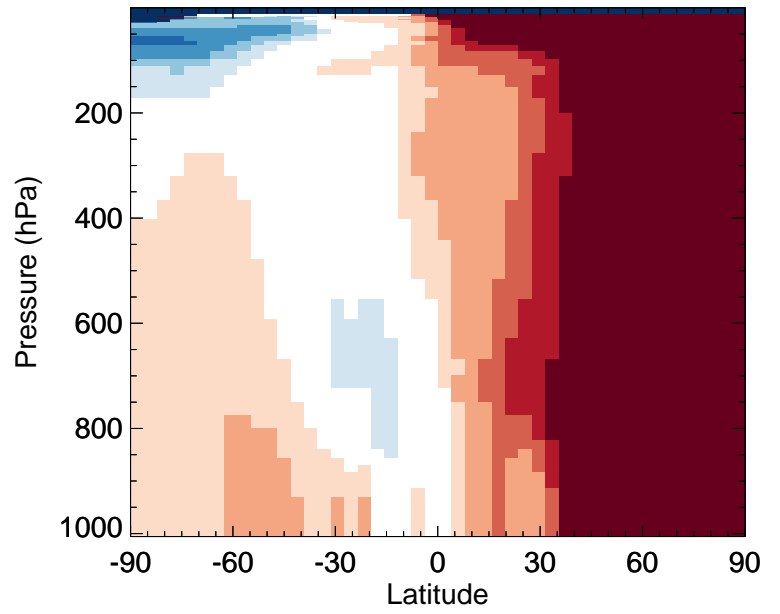
v11-02f-Run0 / v11-02e-Run1 C3H8 - Zonal mean % diff for Jan
