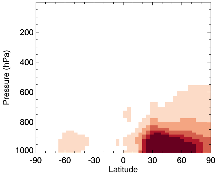
v11-02f-Run0 - v11-02e-Run1 NH4 - Zonal mean abs diff for Jan
