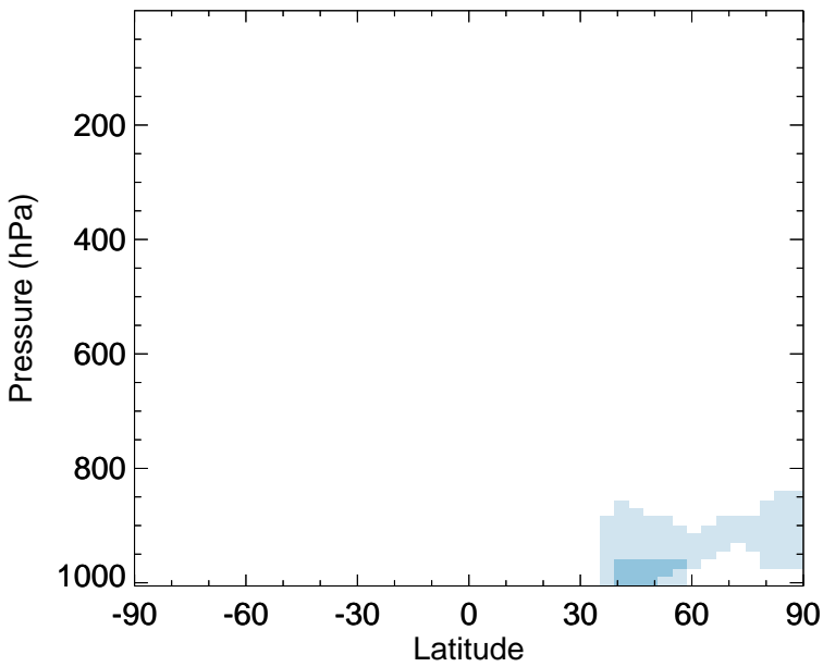
v11-02f-Run0 - v11-02e-Run0 SO 2 - Zonal mean abs diff for Jan
