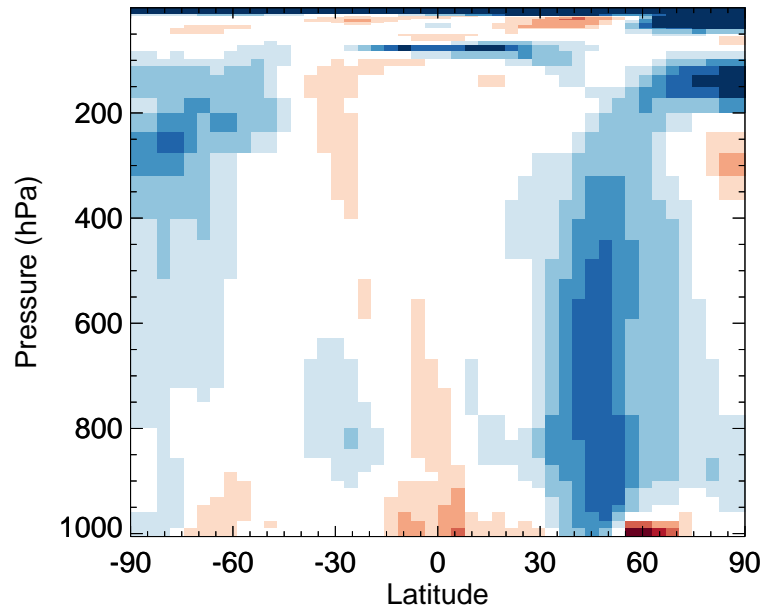
v11-02f-Run0 / v11-02e-Run0 CH 2 O - Zonal mean % diff for Jan
