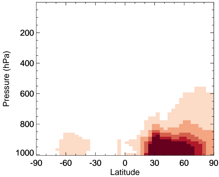
v11-02f-Run0 - v11-02e-Run0 NH4 - Zonal mean abs diff for Jan
