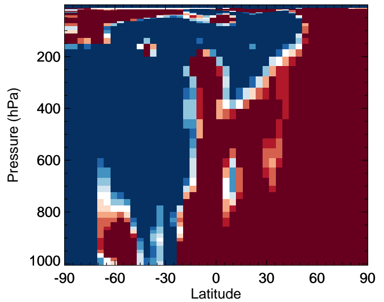
v11-02f-Run0 / v11-02e-Run0 IMAE - Zonal mean % diff for Jan
