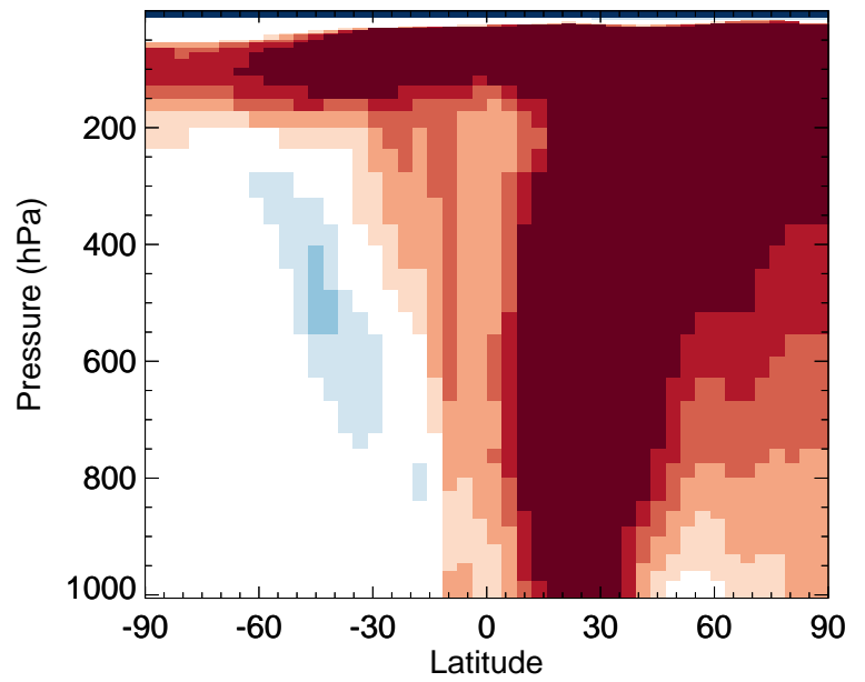
v11-02f-Run0 / v11-02e-Run1 ALD2 - Zonal mean % diff for Jan
