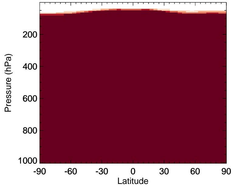
v11-02f-Run0 / v11-02e-Run1 NH4 - Zonal mean % diff for Jan
