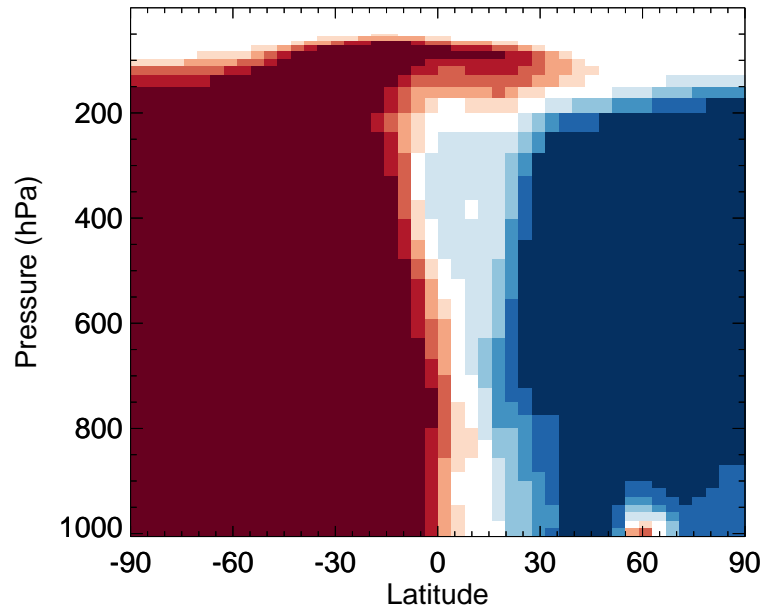
v11-02f-Run0 / v11-02e-Run1 ASOA1 - Zonal mean % diff for Jan
