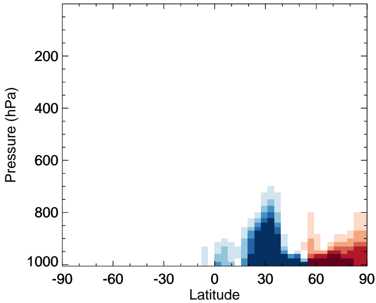
v11-02f-Run0 - v11-02e-Run0 XYLE - Zonal mean abs diff for Jan
