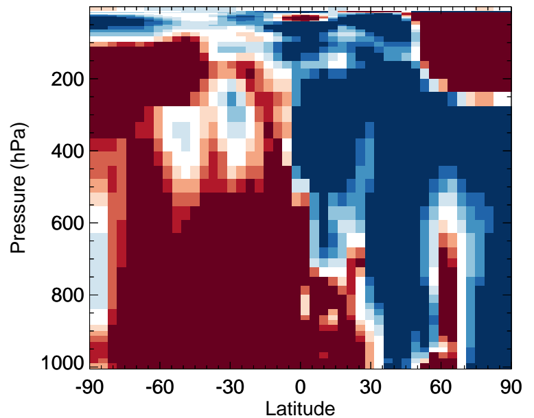
v11-02f-Run0 / v11-02e-Run0 ASOA3 - Zonal mean % diff for Jan
