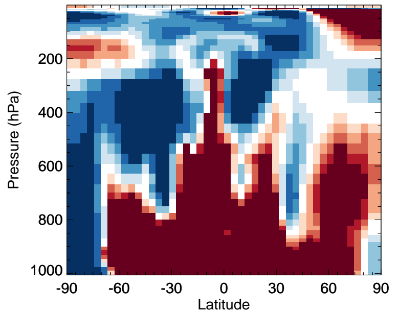
v11-02f-Run0 / v11-02e-Run0 TSOA1 - Zonal mean % diff for Jan
