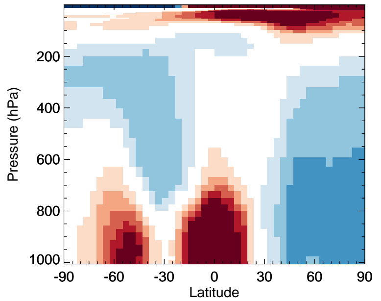
v11-02f-Run0 / v11-02e-Run1 PAN - Zonal mean % diff for Jan
