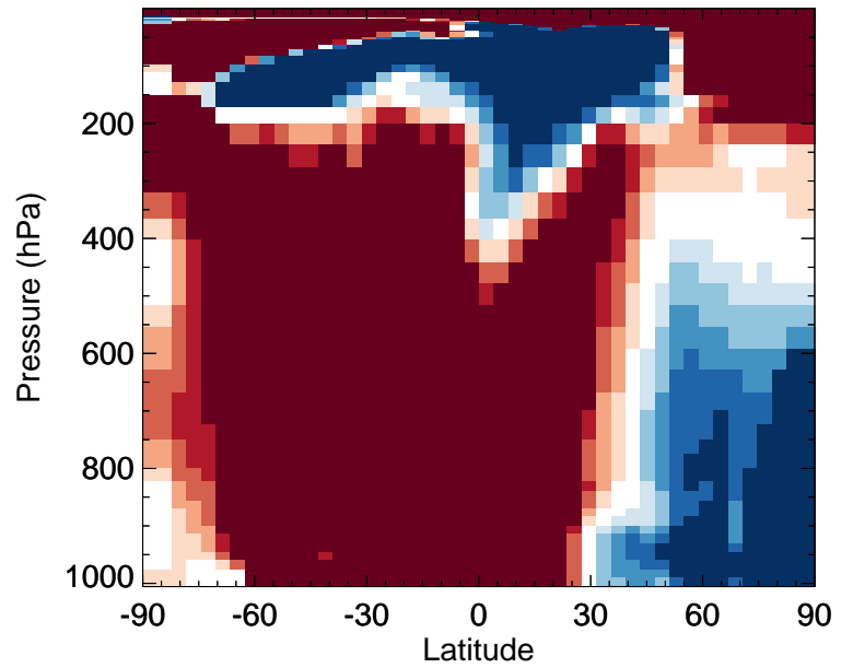
v11-02f-Run0 / v11-02e-Run0 R4N2 - Zonal mean % diff for Jan
