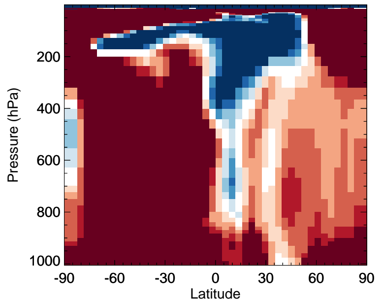
v11-02f-Run0 / v11-02e-Run0 BENZ - Zonal mean % diff for Jan
