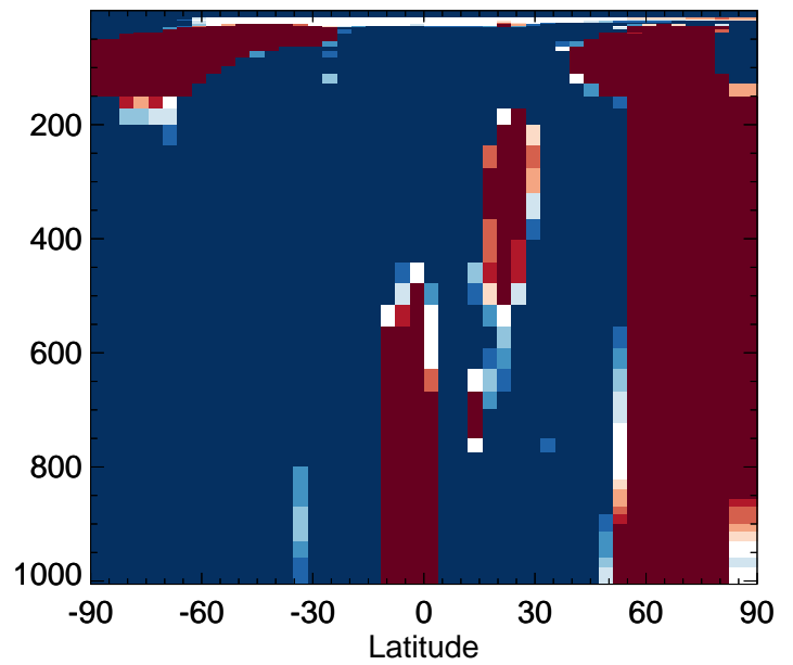
v11-02f-Run0 / v11-02e-Run0 DST4 - Zonal mean % diff for Jan
