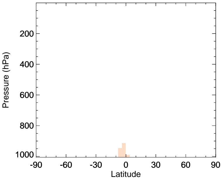
v11-02f-Run0 - v11-02e-Run0 TSOA2 - Zonal mean abs diff for Jan
