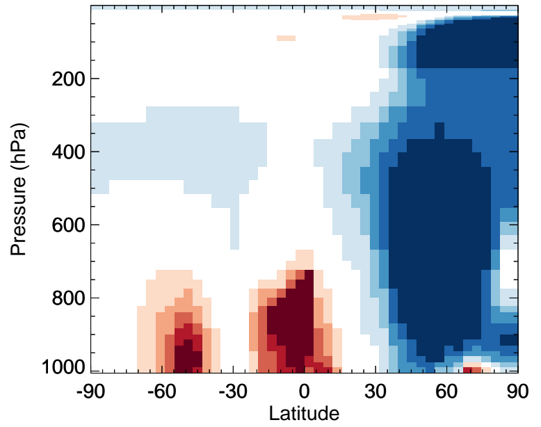
v11-02f-Run0 / v11-02e-Run1 MPN - Zonal mean % diff for Jan
