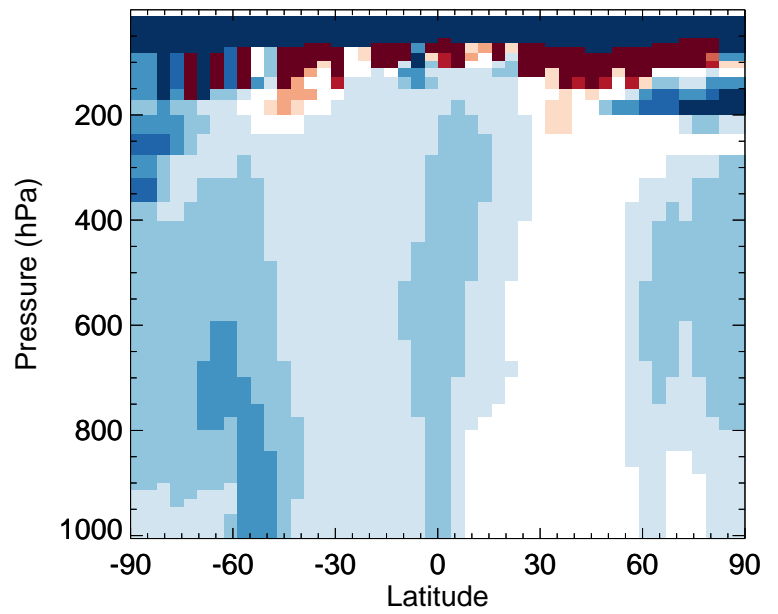
v11-02f-Run0 / v11-02e-Run1 SO 4 s - Zonal mean % diff for Jan
