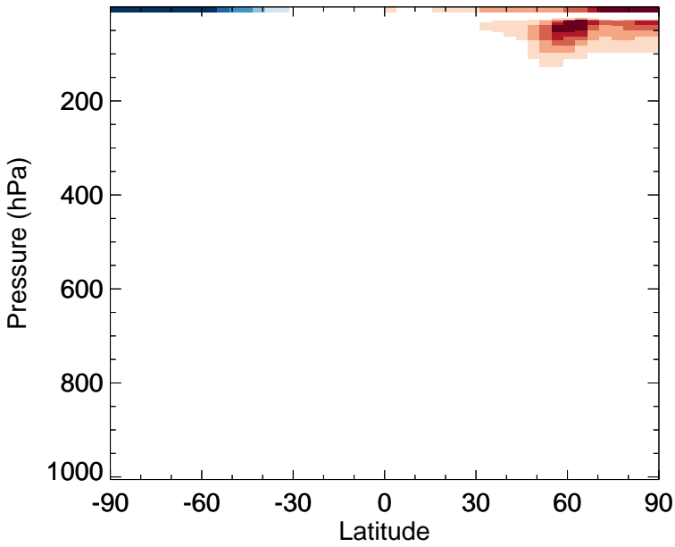
v11-02f-Run0 - v11-02e-Run1 ClO - Zonal mean abs diff for Jan
