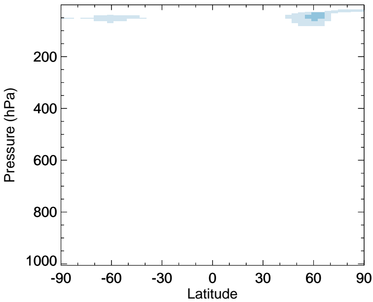
v11-02f-Run0 - v11-02e-Run0 BrNO3 - Zonal mean abs diff for Jan
