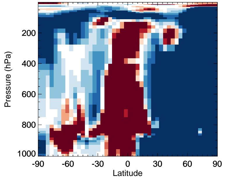
v11-02f-Run0 / v11-02e-Run0 ClNO 3 - Zonal mean % diff for Jan
