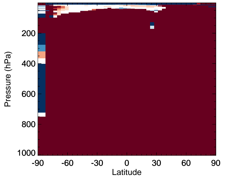
v11-02f-Run0 / v11-02e-Run0 ISOP - Zonal mean % diff for Jan
