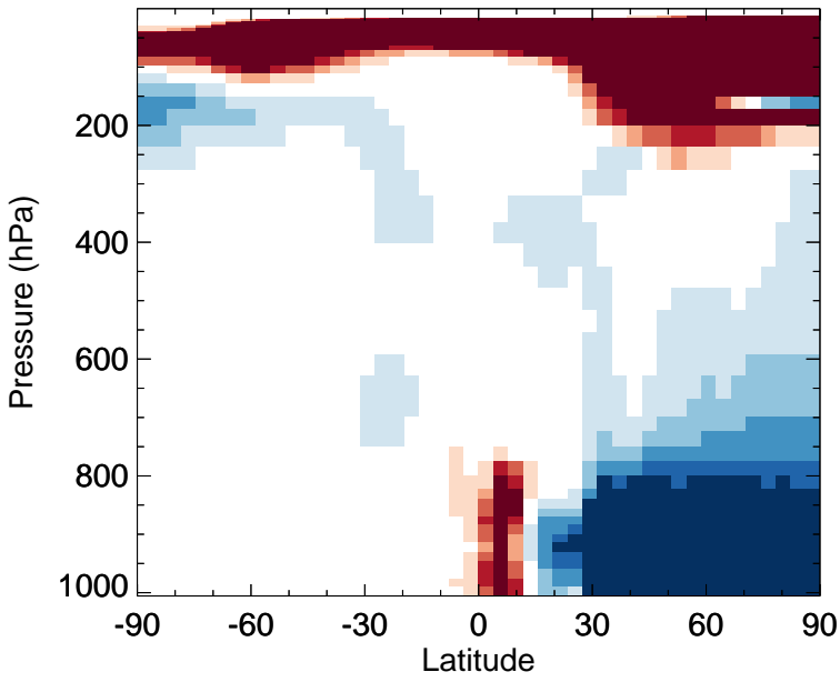
v11-02f-Run0 - v11-02e-Run1 HNO 3 - Zonal mean abs diff for Jan
