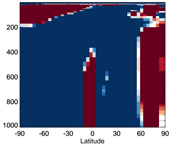
v11-02f-Run0 / v11-02e-Run0 DST3 - Zonal mean % diff for Jan
