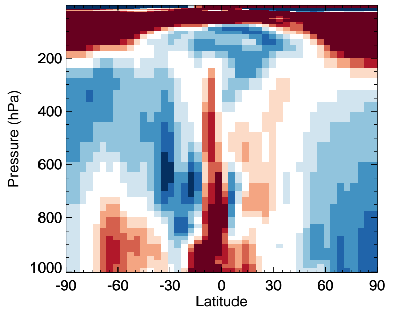
v11-02f-Run0 / v11-02e-Run0 PAN - Zonal mean % diff for Jan
