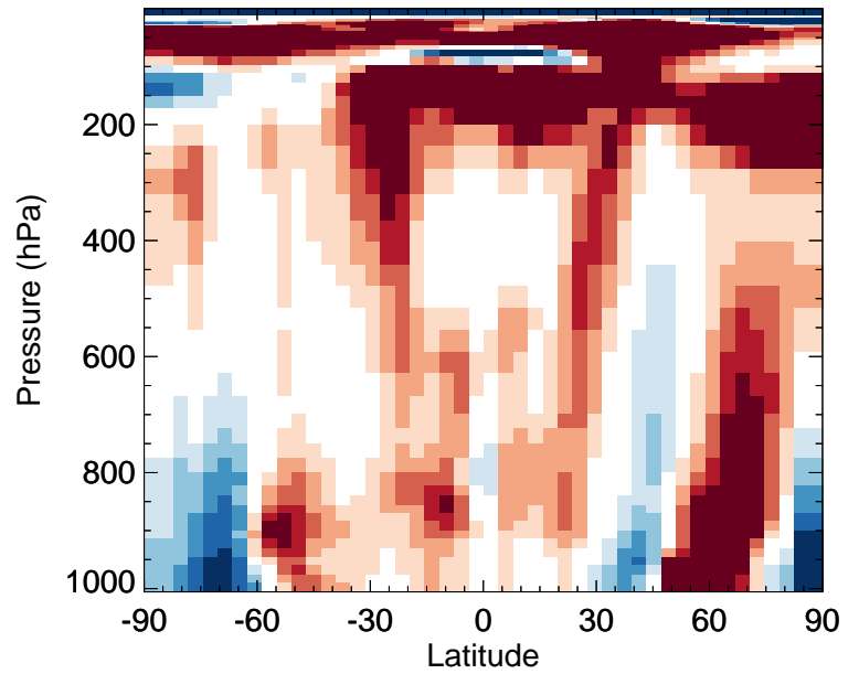
v11-02f-Run0 / v11-02e-Run0 H2O2 - Zonal mean % diff for Jan
