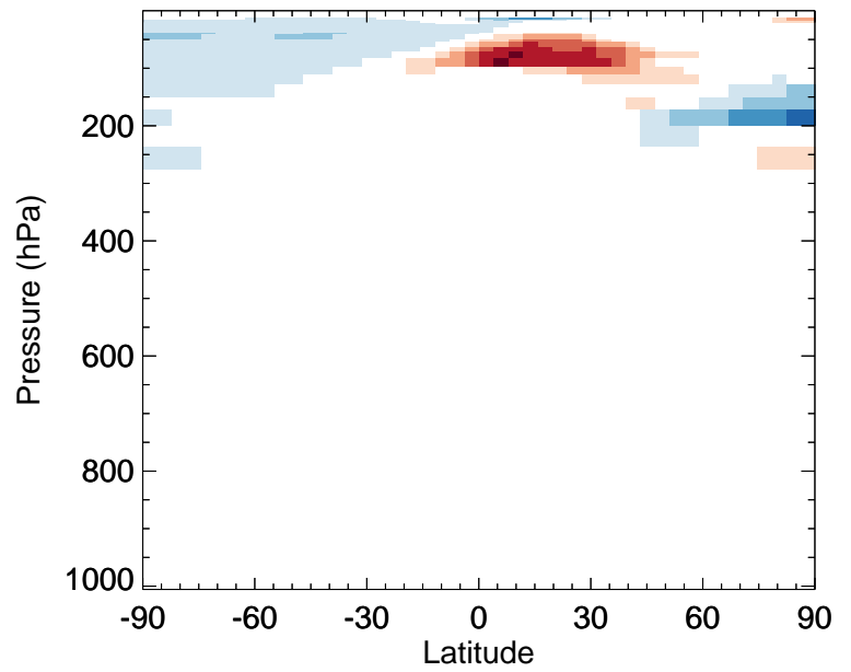
v11-02f-Run0 / v11-02e-Run1 SALC - Zonal mean % diff for Jan
