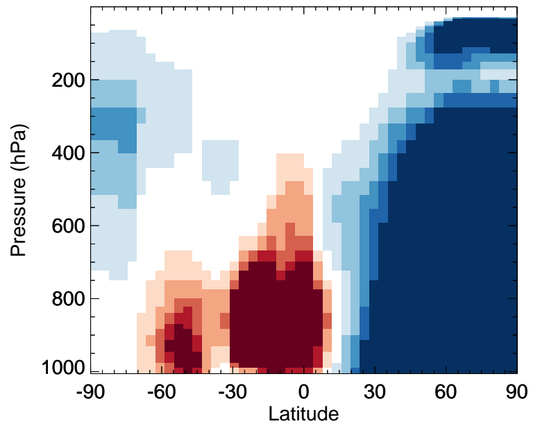
v11-02f-Run0 / v11-02e-Run1 NO3 - Zonal mean % diff for Jan
