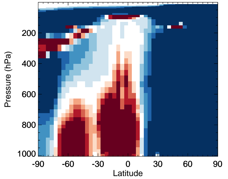
v11-02f-Run0 / v11-02e-Run1 CINO2 - Zonal mean % diff for Jan
