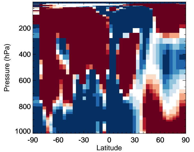
v11-02f-Run0 / v11-02e-Run0 XYLE - Zonal mean % diff for Jan
