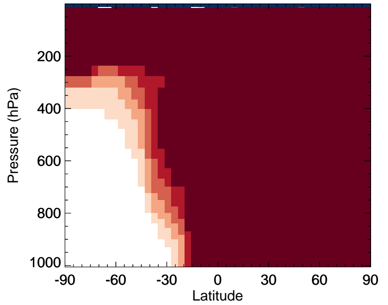
v11-02f-Run0 / v11-02e-Run0 C2H6 - Zonal mean % diff for Jan
