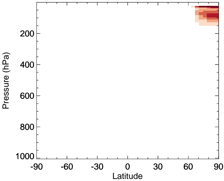
v11-02f-Run0 - v11-02e-Run0 Cl2 - Zonal mean abs diff for Jan
