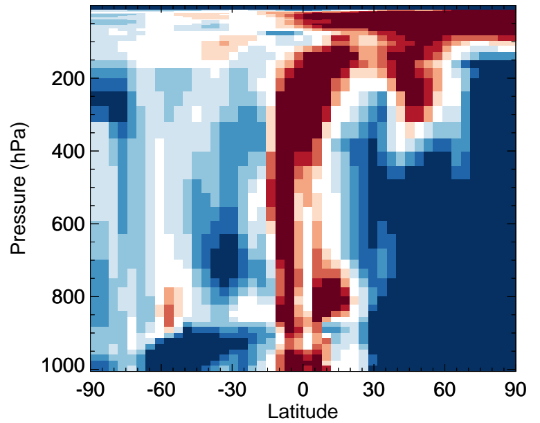
v11-02f-Run0 / v11-02e-Run0 HNO 3 - Zonal mean % diff for Jan
