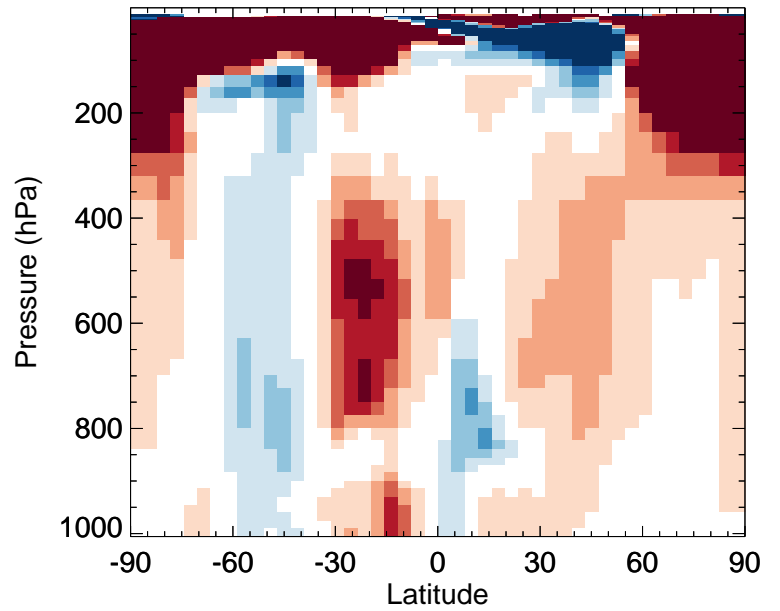
v11-02f-Run0 / v11-02e-Run0 CHBr3 - Zonal mean % diff for Jan
