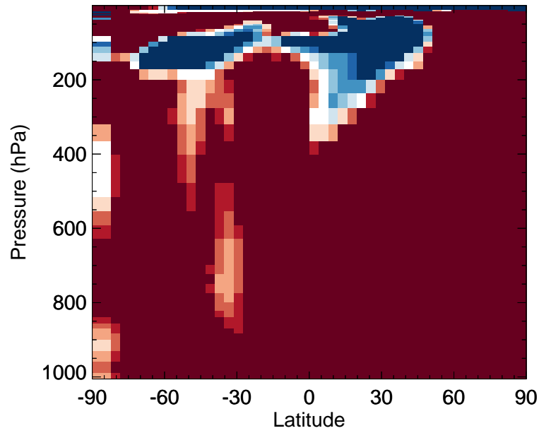
v11-02f-Run0 / v11-02e-Run0 ALK4 - Zonal mean % diff for Jan
