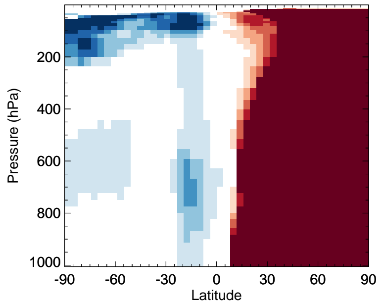
v11-02f-Run0 / v11-02e-Run1 DMS - Zonal mean % diff for Jan
