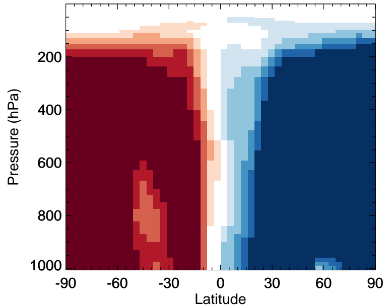
v11-02f-Run0 / v11-02e-Run1 ASOAN - Zonal mean % diff for Jan
