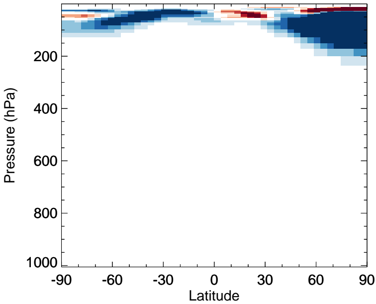
v11-02f-Run0 - v11-02e-Run0 ClNO 3 - Zonal mean abs diff for Jan
