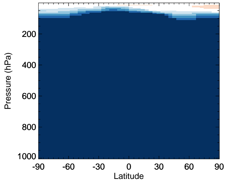
v11-02f-Run0 / v11-02e-Run0 SOAIE - Zonal mean % diff for Jan
