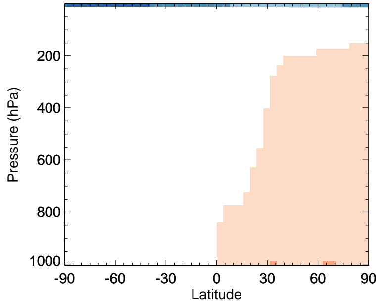
v11-02f-Run0 / v11-02e-Run1 CO - Zonal mean % diff for Jan
