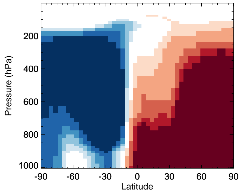
v11-02f-Run0 / v11-02e-Run1 SOAMG - Zonal mean % diff for Jan
