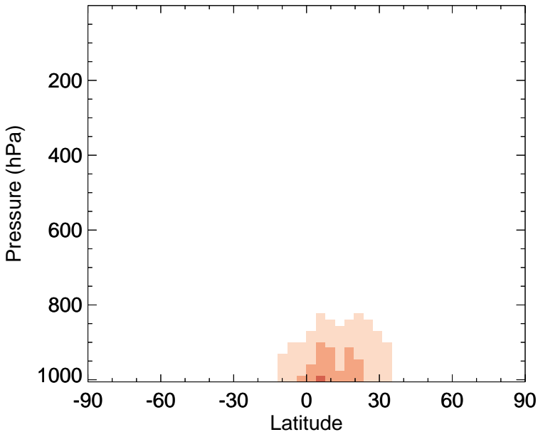
v11-02f-Run0 - v11-02e-Run1 INDIOL - Zonal mean abs diff for Jan
