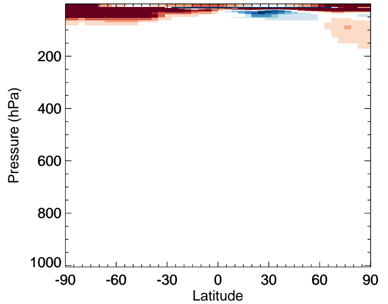
v11-02f-Run0 / v11-02e-Run0 OCS - Zonal mean % diff for Jan
