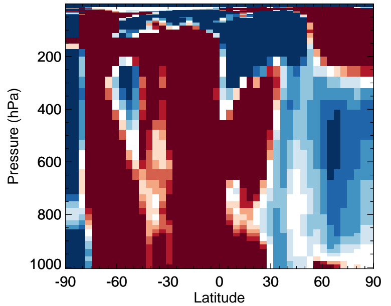
v11-02f-Run0 / v11-02e-Run0 TOLU - Zonal mean % diff for Jan
