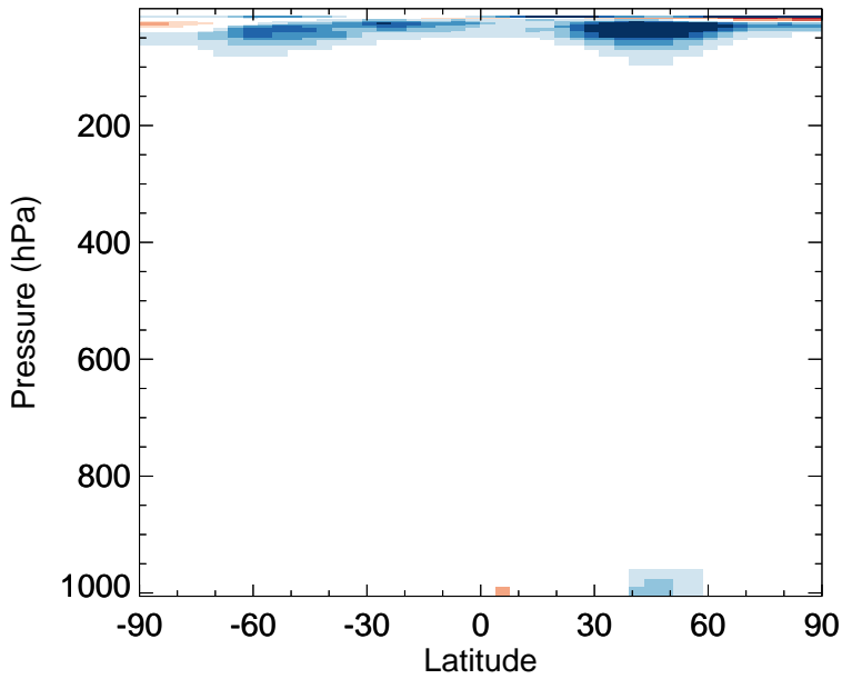
v11-02f-Run0 - v11-02e-Run0 NO 2 - Zonal mean abs diff for Jan
