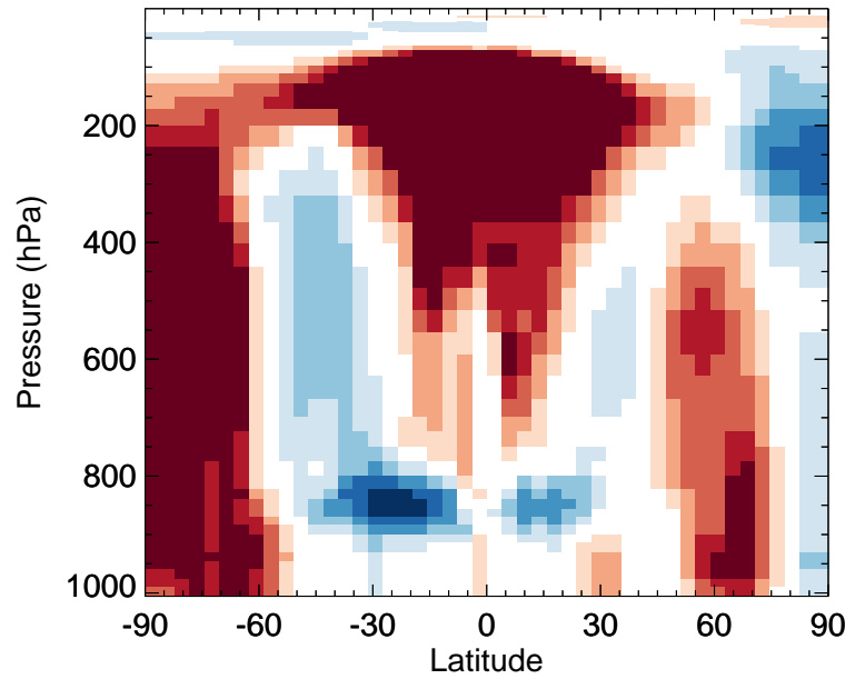
v11-02f-Run0 / v11-02e-Run0 MSA - Zonal mean % diff for Jan
