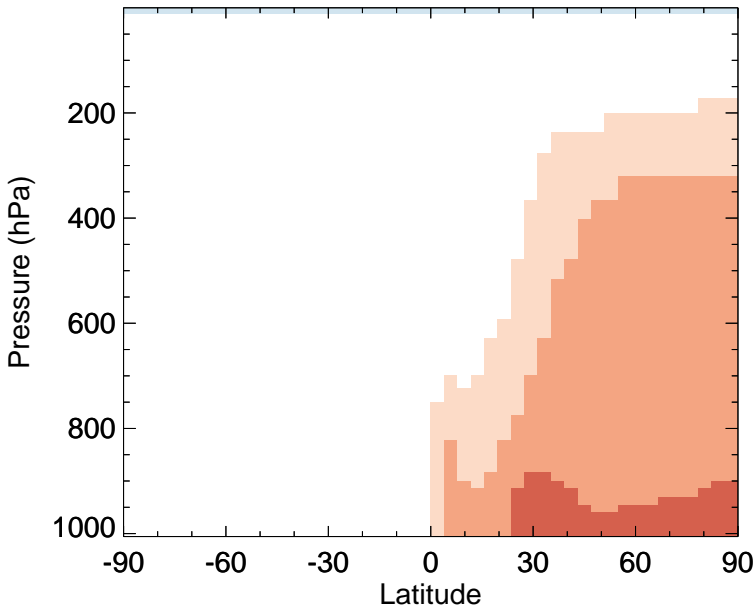
v11-02f-Run0 - v11-02e-Run1 CO - Zonal mean abs diff for Jan
