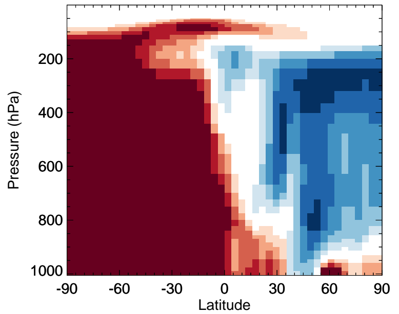
v11-02f-Run0 / v11-02e-Run1 ASOA3 - Zonal mean % diff for Jan
