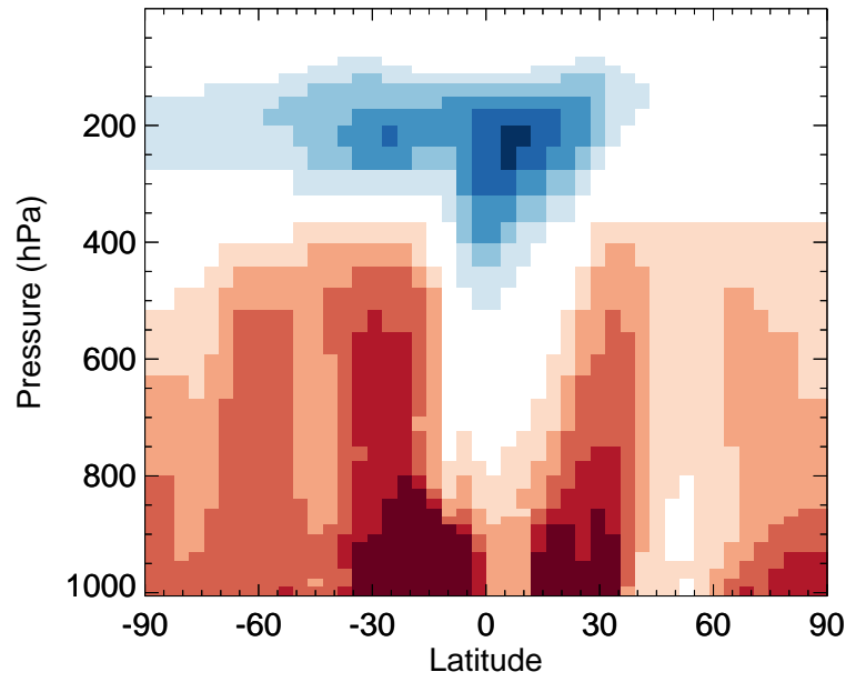
v11-02f-Run0 / v11-02e-Run1 ISOA2 - Zonal mean % diff for Jan
