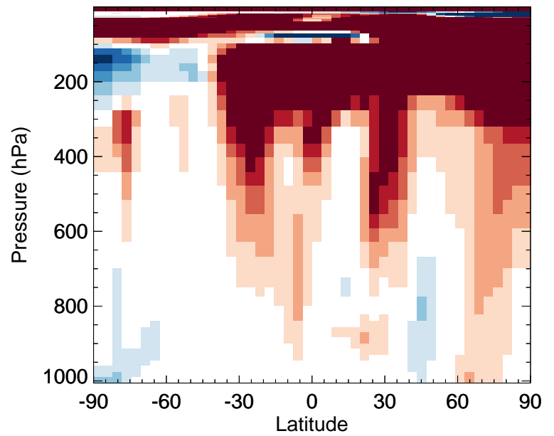
v11-02f-Run0 / v11-02e-Run0 MP - Zonal mean % diff for Jan
