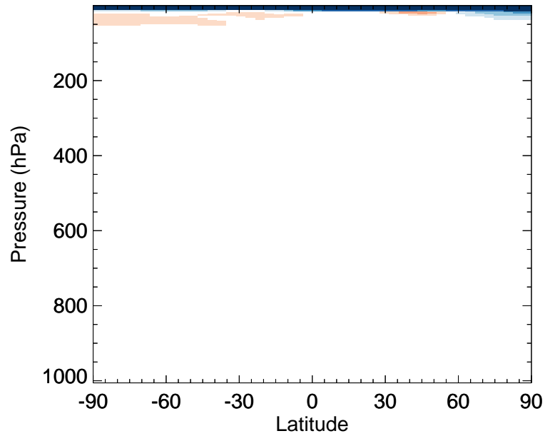
v11-02f-Run0 / v11-02e-Run0 CH4 - Zonal mean % diff for Jan
