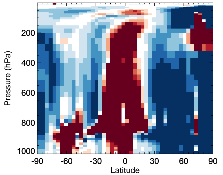
v11-02f-Run0 / v11-02e-Run0 BrNO3 - Zonal mean % diff for Jan
