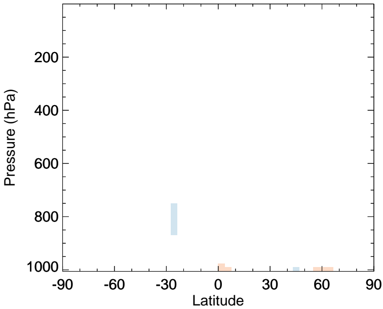
v11-02f-Run0 - v11-02e-Run0 CH 2 O - Zonal mean abs diff for Jan
