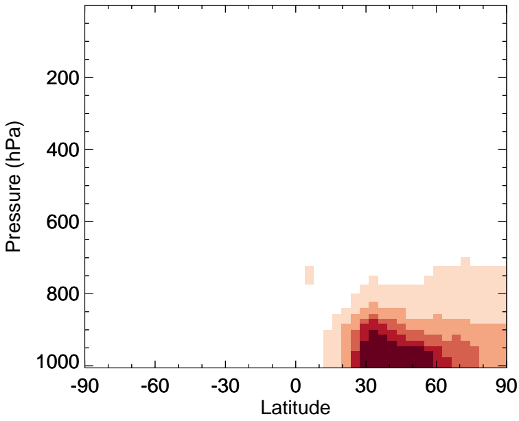
v11-02f-Run0 - v11-02e-Run1 NIT - Zonal mean abs diff for Jan
