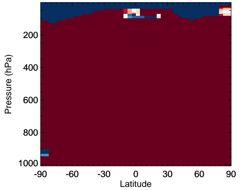
v11-02f-Run0 / v11-02e-Run1 NIT - Zonal mean % diff for Jan
