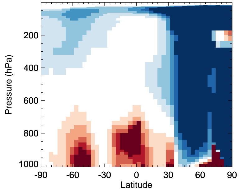
v11-02f-Run0 / v11-02e-Run1 NO - Zonal mean % diff for Jan
