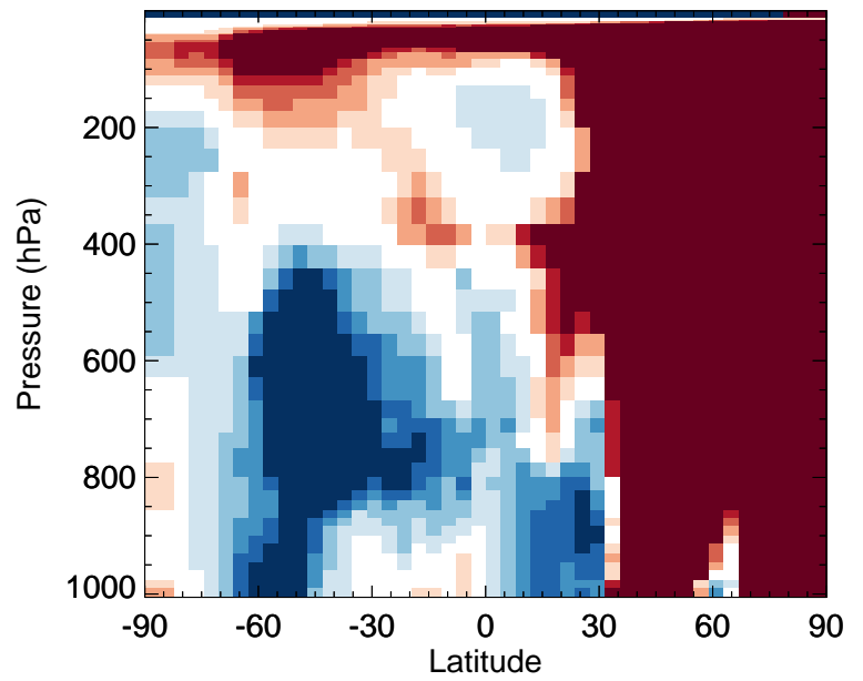
v11-02f-Run0 / v11-02e-Run1 OCIO - Zonal mean % diff for Jan
