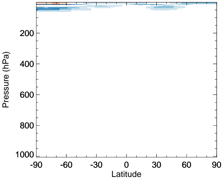
v11-02f-Run0 - v11-02e-Run0 NO - Zonal mean abs diff for Jan
