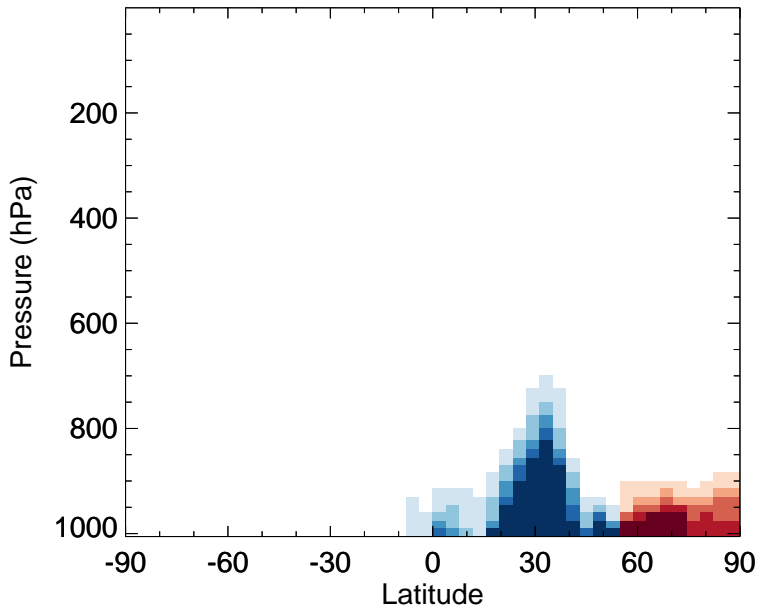
v11-02f-Run0 - v11-02e-Run1 XYLE - Zonal mean abs diff for Jan
