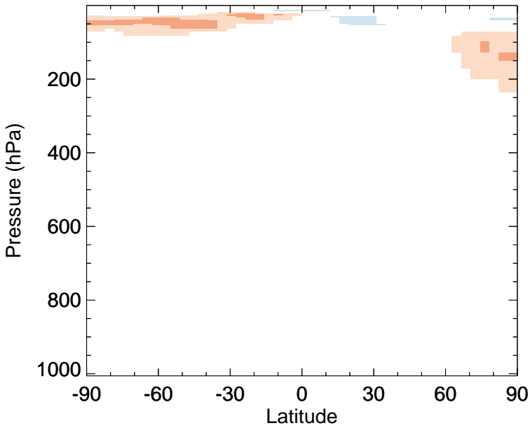
v11-02f-Run0 - v11-02e-Run0 CH3Cl - Zonal mean abs diff for Jan
