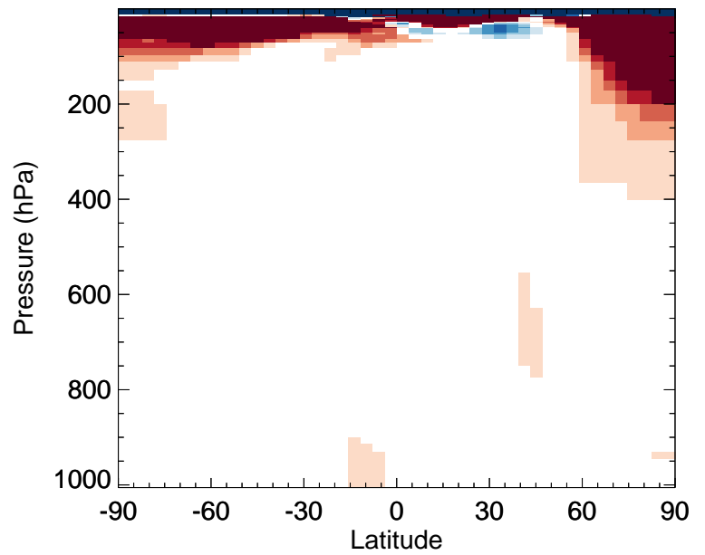
v11-02f-Run0 / v11-02e-Run0 CH 2 Br 2 - Zonal mean % diff for Jan
