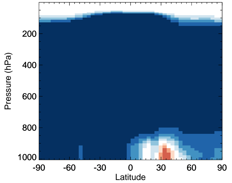
v11-02f-Run0 / v11-02e-Run1 ISO3 - Zonal mean % diff for Jan
