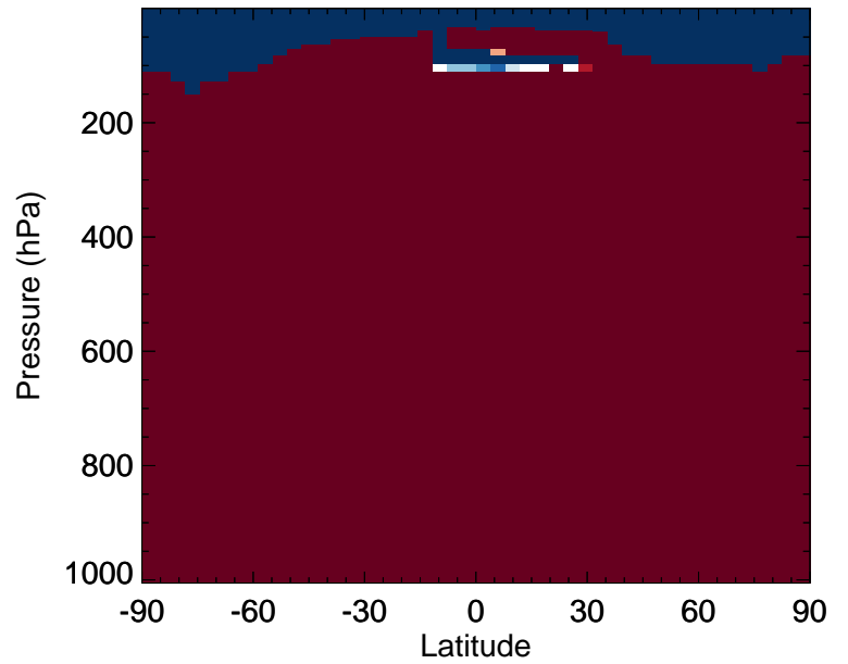
v11-02f-Run0 / v11-02e-Run0 NIT - Zonal mean % diff for Jan
