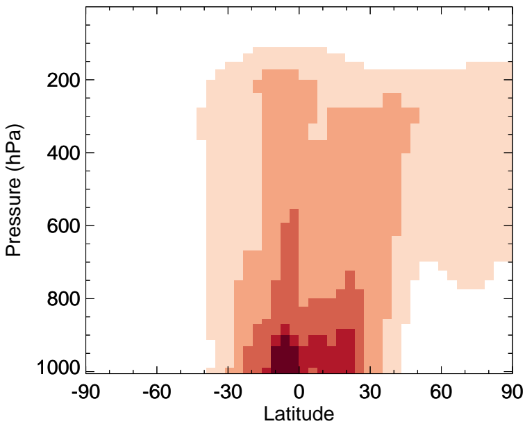
v11-02f-Run0 - v11-02e-Run1 ACET - Zonal mean abs diff for Jan
