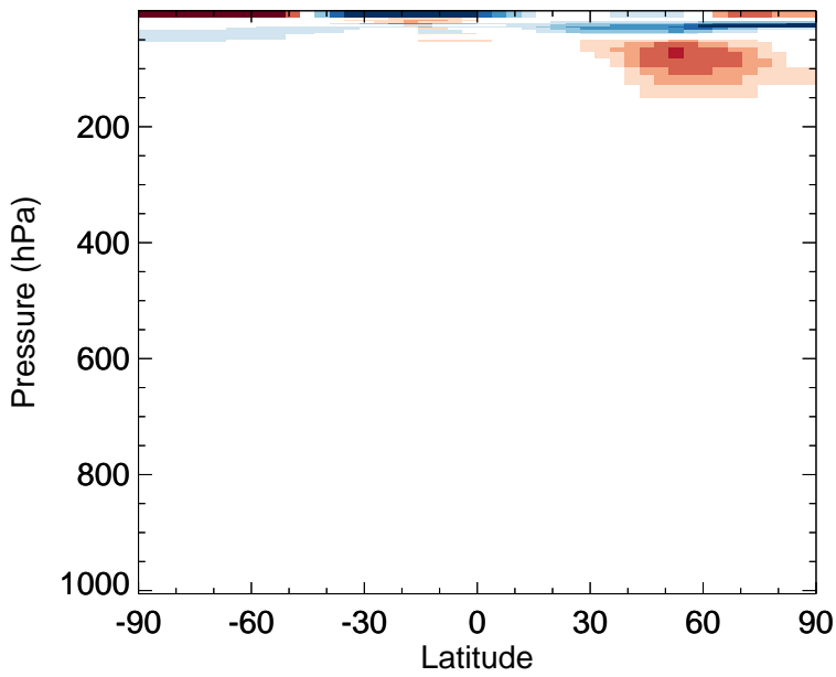
v11-02f-Run0 - v11-02e-Run1 HCl - Zonal mean abs diff for Jan
