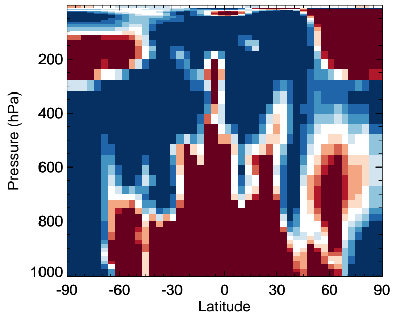
v11-02f-Run0 / v11-02e-Run0 TSOA3 - Zonal mean % diff for Jan
