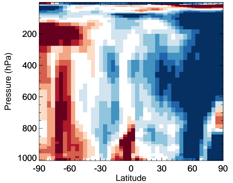
v11-02f-Run0 / v11-02e-Run0 MPN - Zonal mean % diff for Jan
