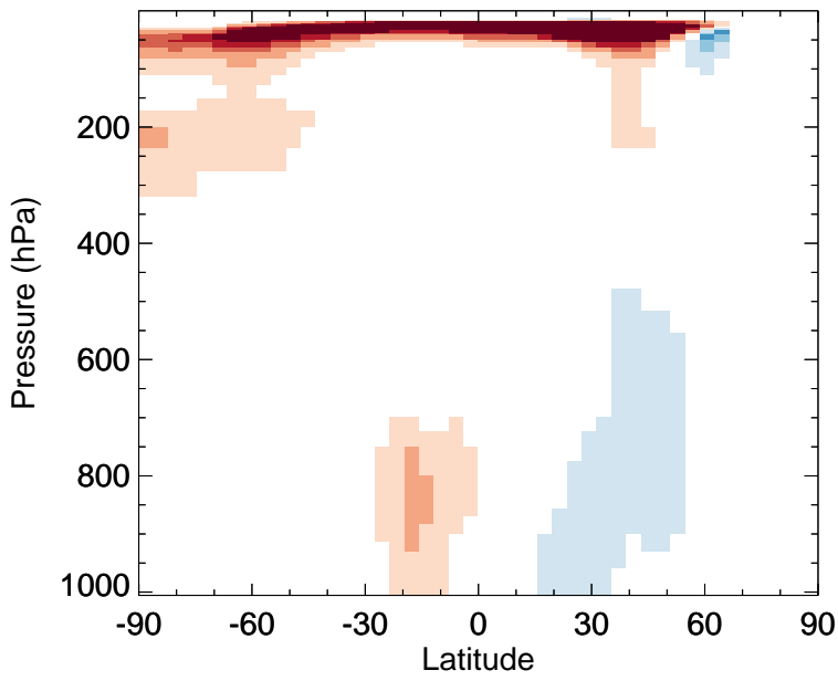
v11-02f-Run0 - v11-02e-Run1 HO2 - Zonal mean abs diff for Jan
