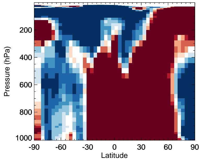
v11-02f-Run0 / v11-02e-Run1 ISN1OG - Zonal mean % diff for Jan
