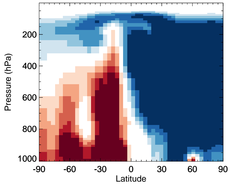
v11-02f-Run0 / v11-02e-Run1 ASOA2 - Zonal mean % diff for Jan
