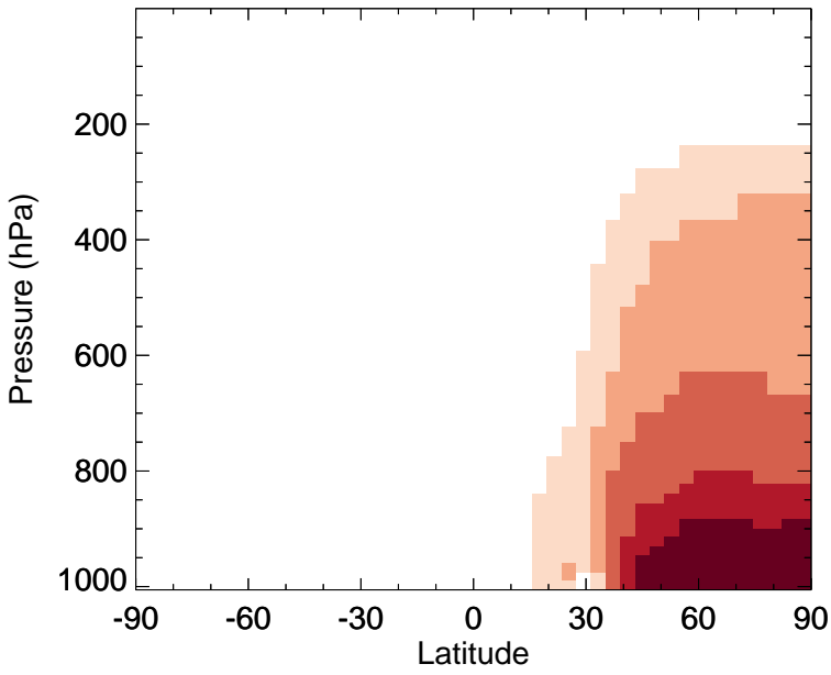
v11-02f-Run0 - v11-02e-Run1 C3H8 - Zonal mean abs diff for Jan
