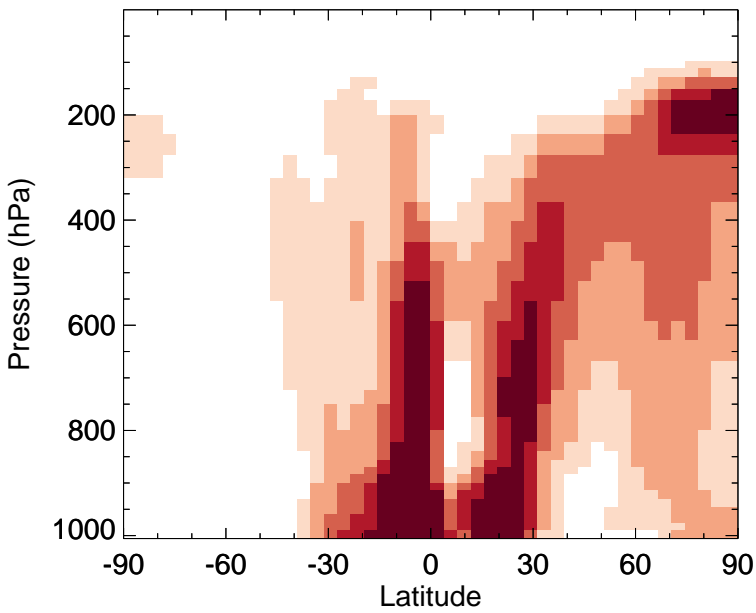
v11-02f-Run0 - v11-02e-Run0 ACET - Zonal mean abs diff for Jan
