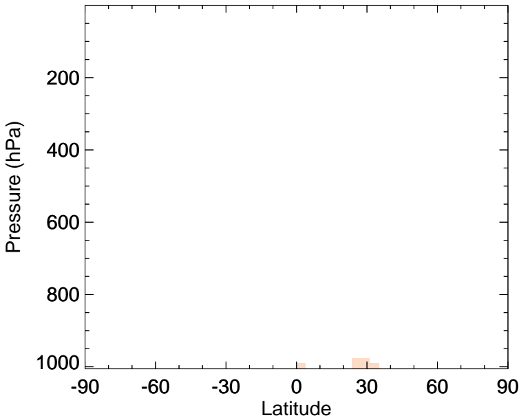
v11-02f-Run0 - v11-02e-Run0 OCPO - Zonal mean abs diff for Jan
