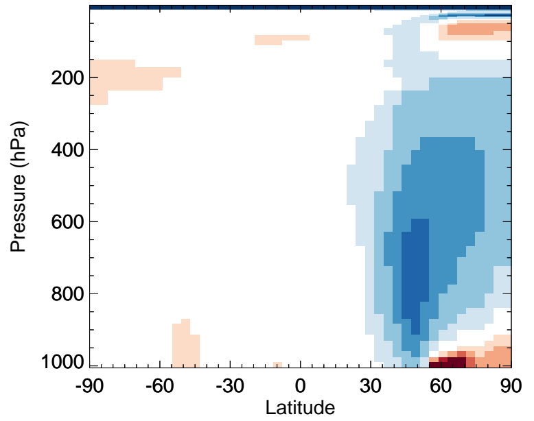
v11-02f-Run0 / v11-02e-Run1 CH 2 O - Zonal mean % diff for Jan
