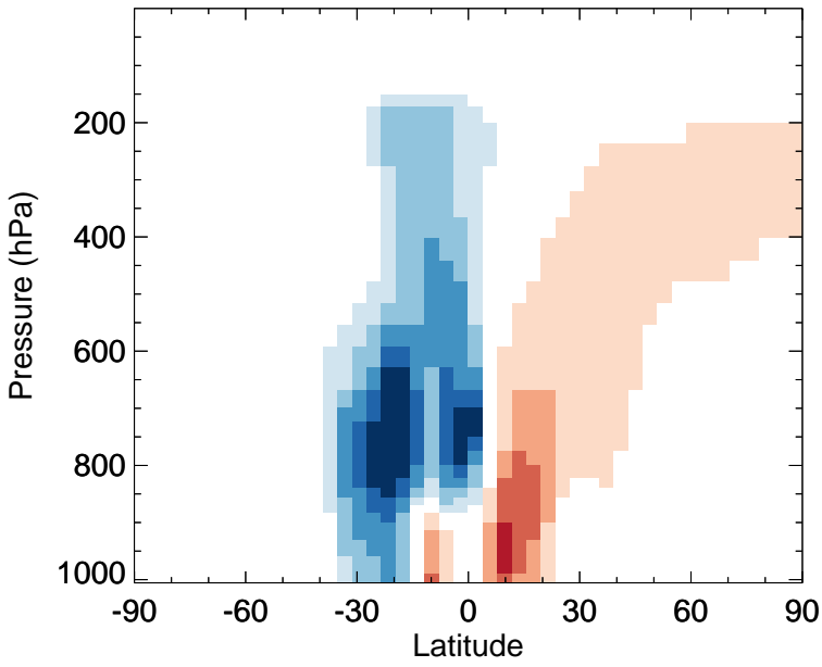
v11-02f-Run0 - v11-02e-Run1 MAP - Zonal mean abs diff for Jan
