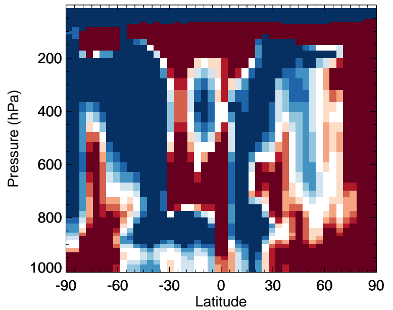
v11-02f-Run0 / v11-02e-Run0 SO 4 s - Zonal mean % diff for Jan
