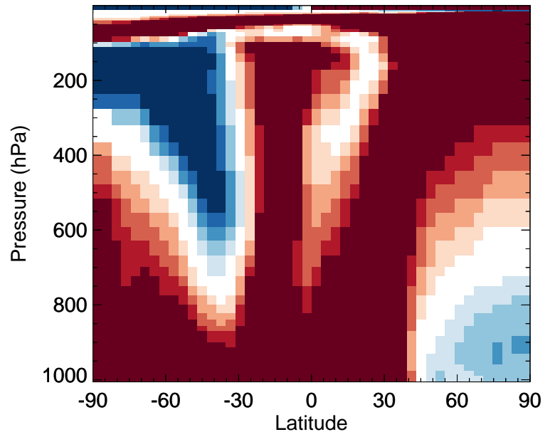
v11-02f-Run0 / v11-02e-Run1 EOH - Zonal mean % diff for Jan
