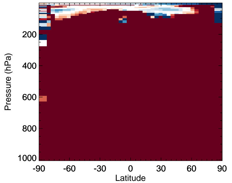
v11-02f-Run0 / v11-02e-Run0 LIMO - Zonal mean % diff for Jan
