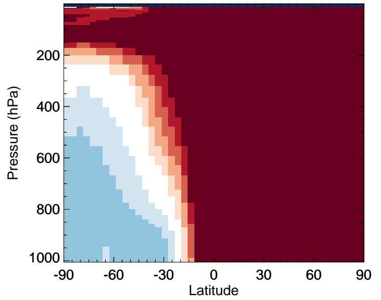
v11-02f-Run0 / v11-02e-Run1 C2H6 - Zonal mean % diff for Jan
