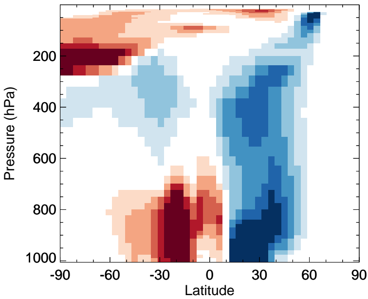
v11-02f-Run0 - v11-02e-Run1 OH - Zonal mean abs diff for Jan
