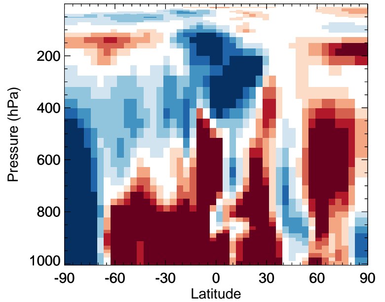
v11-02f-Run0 / v11-02e-Run0 OCPI - Zonal mean % diff for Jan
