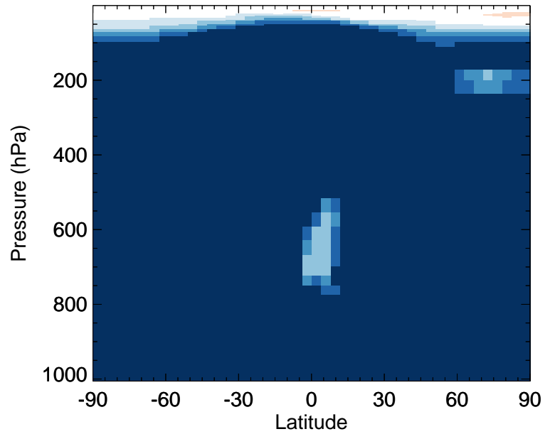
v11-02f-Run0 / v11-02e-Run0 SOAME - Zonal mean % diff for Jan
