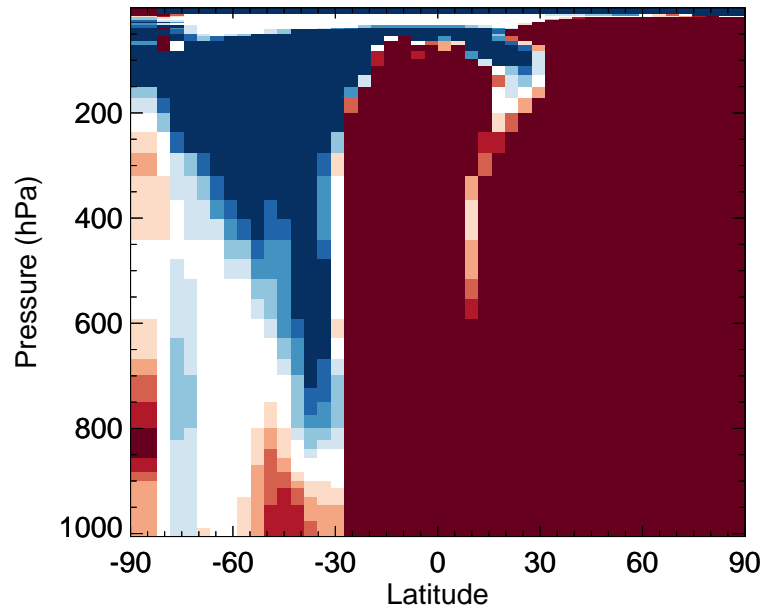
v11-02f-Run0 / v11-02e-Run1 MVK - Zonal mean % diff for Jan
