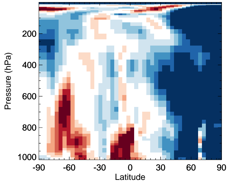
v11-02f-Run0 / v11-02e-Run0 HNO 4 - Zonal mean % diff for Jan
