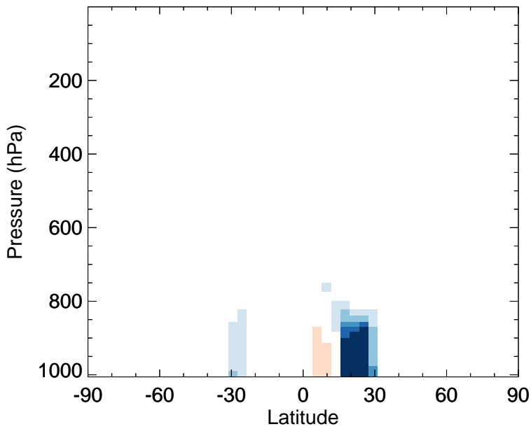
v11-02f-Run0 - v11-02e-Run0 DST4 - Zonal mean abs diff for Jan
