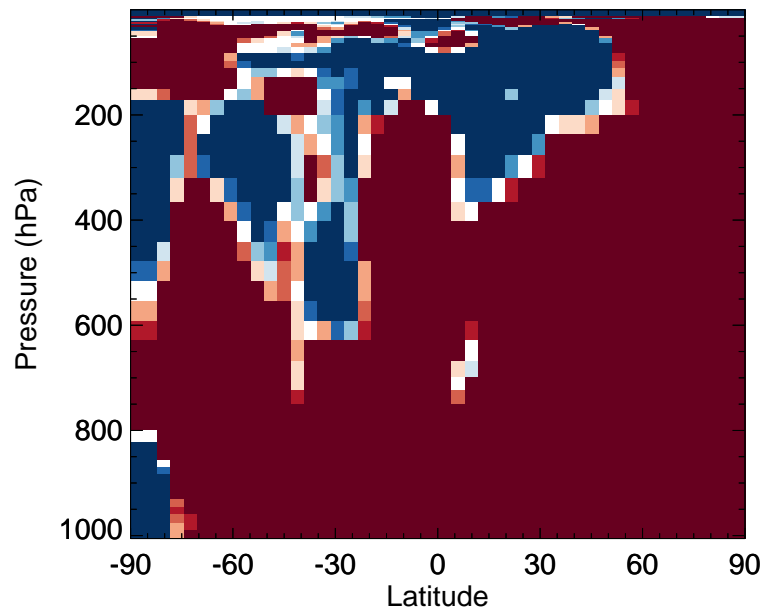
v11-02f-Run0 / v11-02e-Run0 IEPOXA - Zonal mean % diff for Jan
