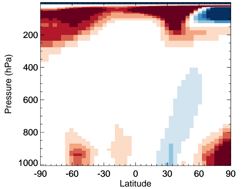
v11-02f-Run0 / v11-02e-Run1 H2O2 - Zonal mean % diff for Jan
