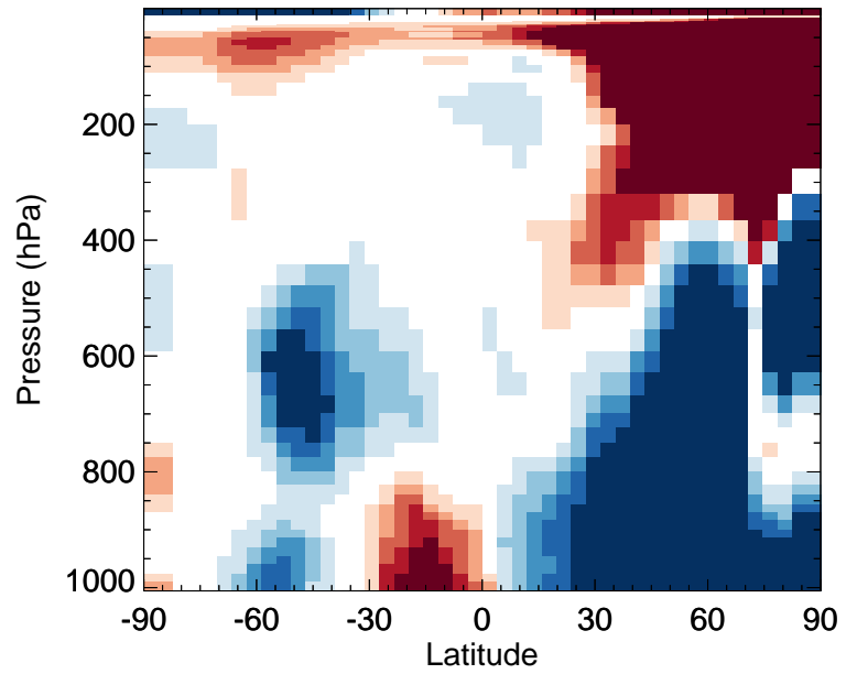
v11-02f-Run0 / v11-02e-Run1 ClO - Zonal mean % diff for Jan
