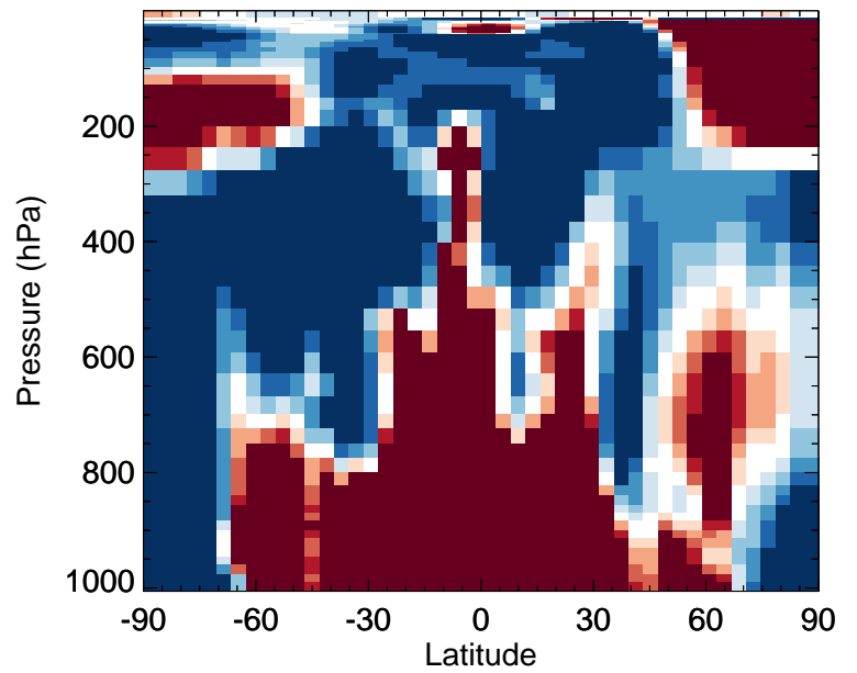
v11-02f-Run0 / v11-02e-Run0 TSOA2 - Zonal mean % diff for Jan
