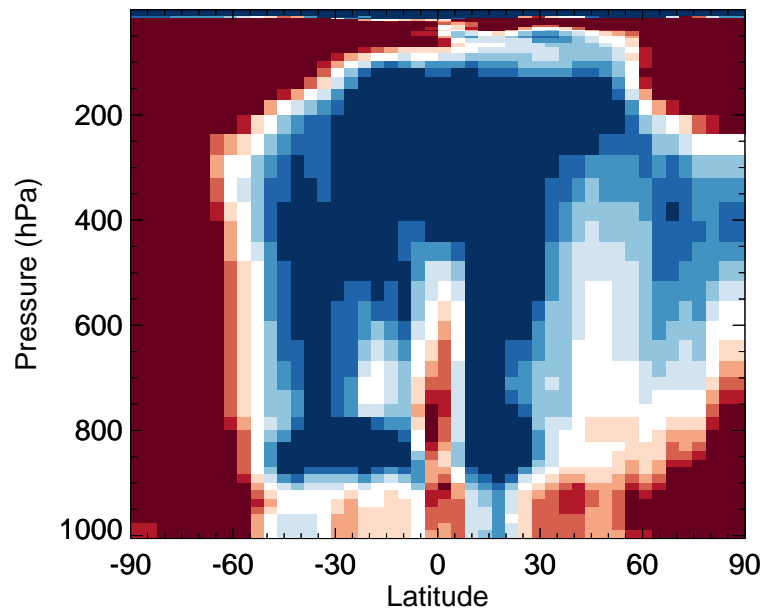
v11-02f-Run0 / v11-02e-Run0 SALA - Zonal mean % diff for Jan
