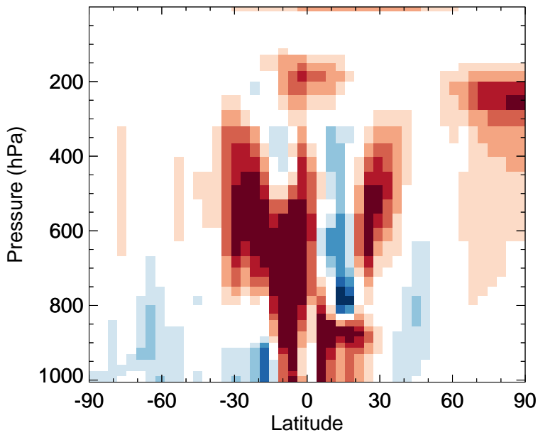
v11-02f-Run0 - v11-02e-Run0 MP - Zonal mean abs diff for Jan
