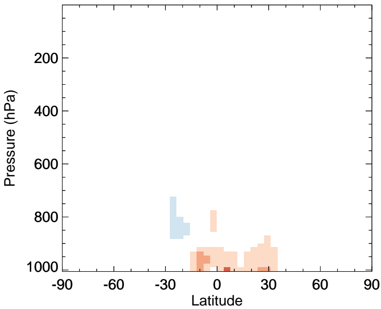
v11-02f-Run0 - v11-02e-Run0 ALD2 - Zonal mean abs diff for Jan
