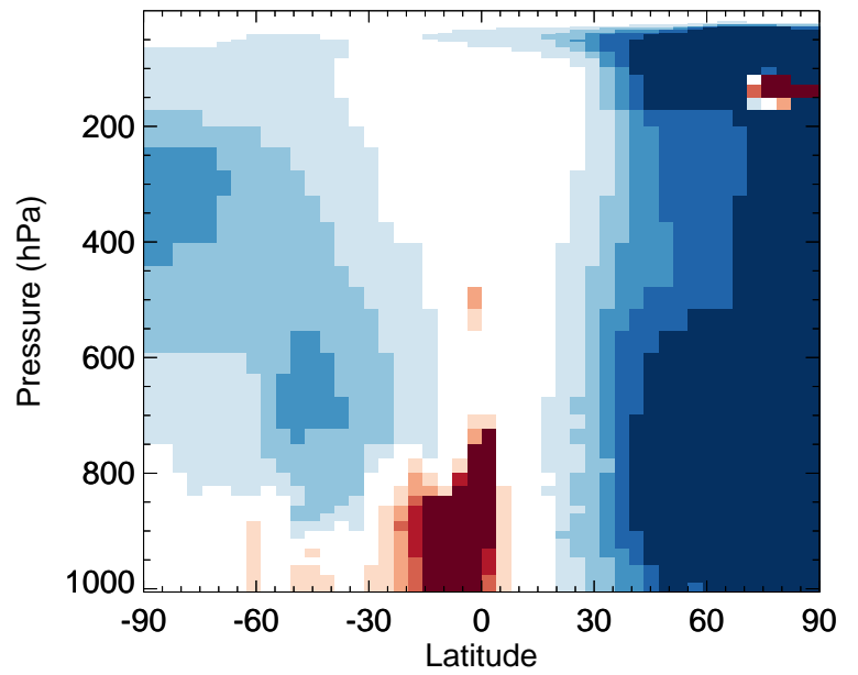
v11-02f-Run0 / v11-02e-Run1 BrNO3 - Zonal mean % diff for Jan
