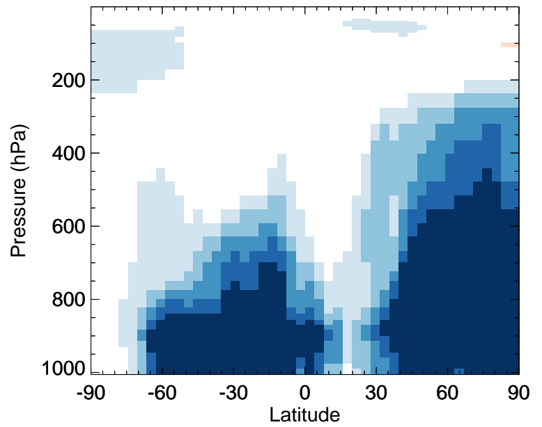
v11-02f-Run0 / v11-02e-Run1 SO 2 - Zonal mean % diff for Jan
