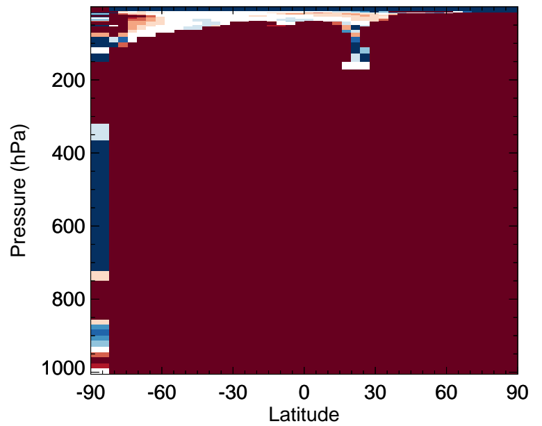
v11-02f-Run0 / v11-02e-Run0 RIPA - Zonal mean % diff for Jan
