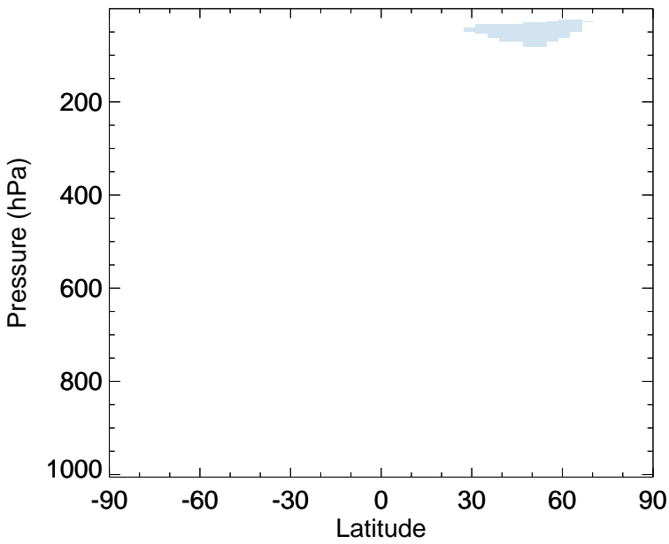
v11-02f-Run0 - v11-02e-Run1 BrNO3 - Zonal mean abs diff for Jan
