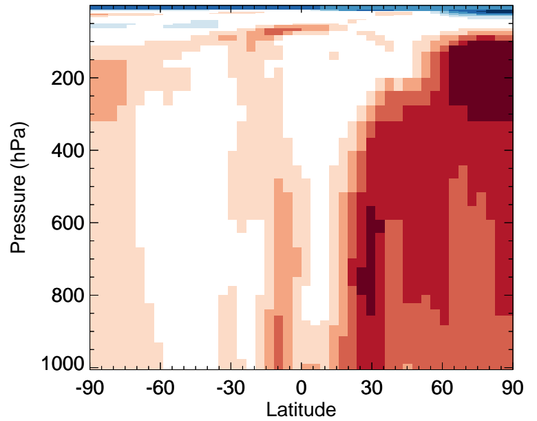
v11-02f-Run0 / v11-02e-Run0 CO - Zonal mean % diff for Jan
