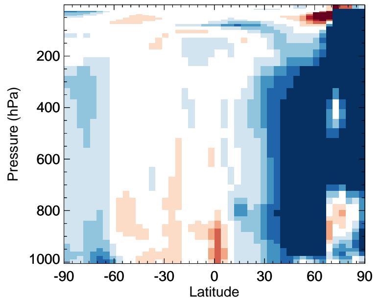
v11-02f-Run0 / v11-02e-Run0 OH - Zonal mean % diff for Jan
