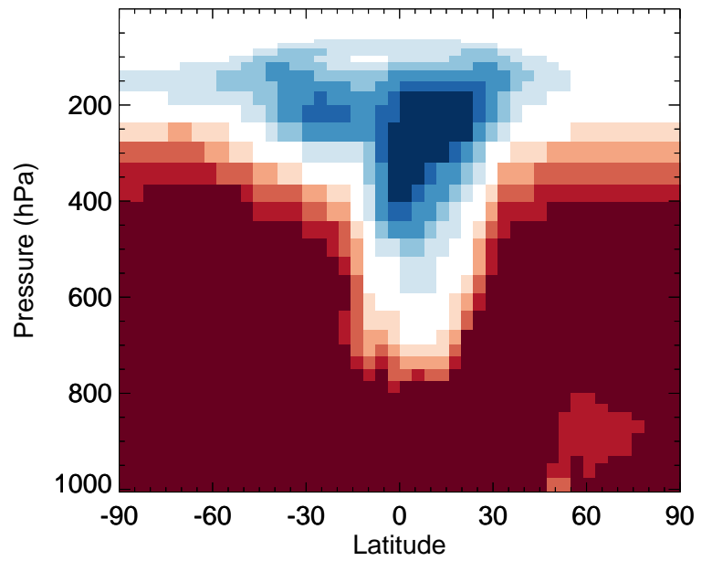
v11-02f-Run0 / v11-02e-Run1 TSOA2 - Zonal mean % diff for Jan
