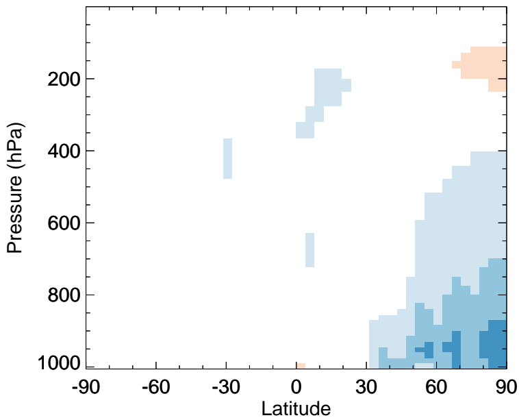
v11-02f-Run0 - v11-02e-Run0 PAN - Zonal mean abs diff for Jan
