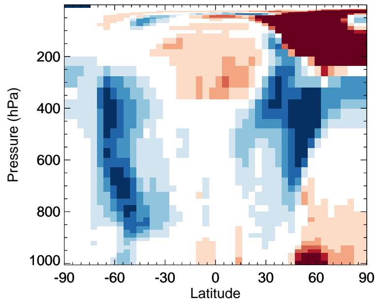
v11-02f-Run0 / v11-02e-Run1 Br2 - Zonal mean % diff for Jan
