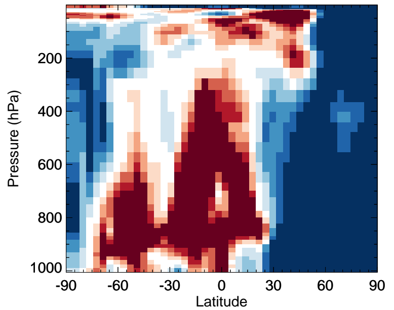
v11-02f-Run0 / v11-02e-Run0 NO3 - Zonal mean % diff for Jan
