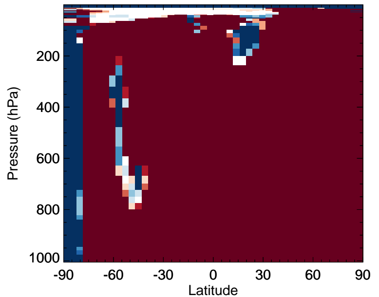
v11-02f-Run0 / v11-02e-Run0 ISN1 - Zonal mean % diff for Jan
