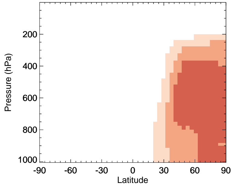
v11-02f-Run0 / v11-02e-Run1 MSA - Zonal mean % diff for Jan
