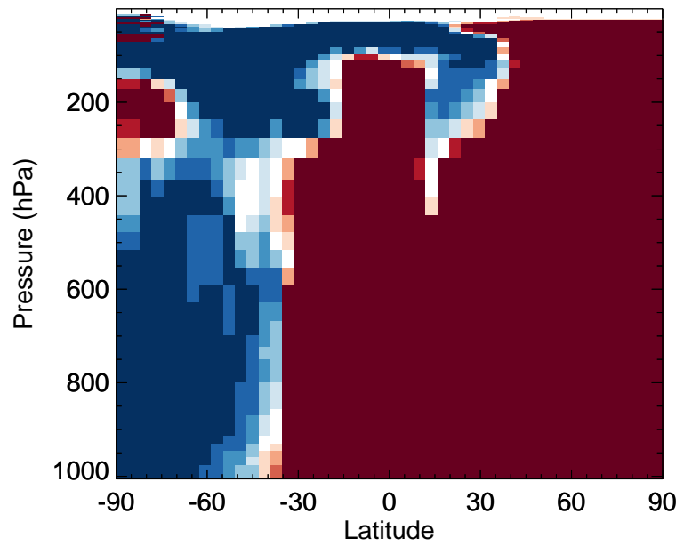
v11-02f-Run0 / v11-02e-Run1 LVOC - Zonal mean % diff for Jan
