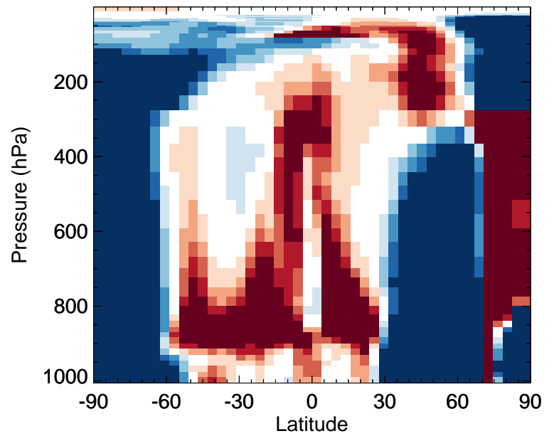
v11-02f-Run0 / v11-02e-Run0 HCl - Zonal mean % diff for Jan
