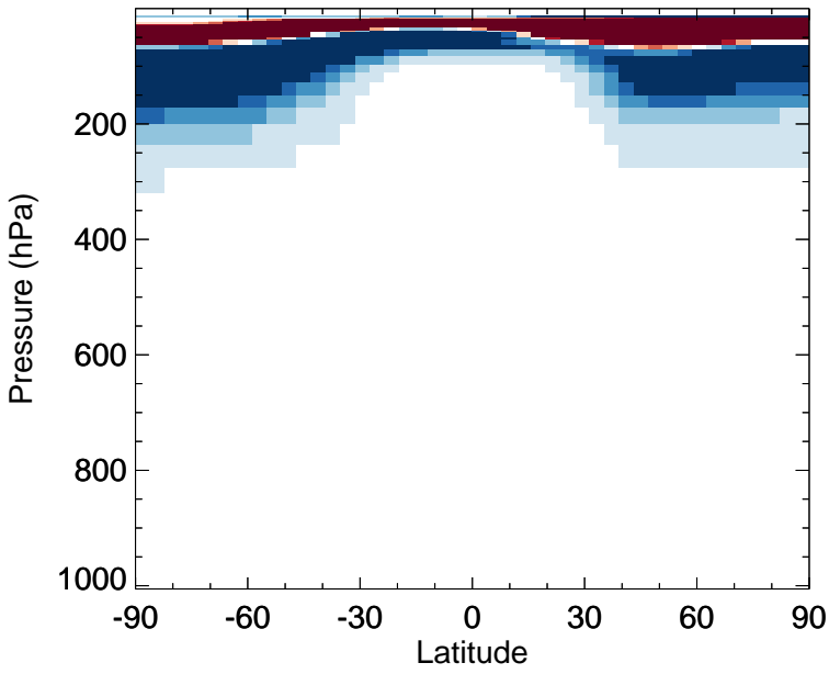
v11-02f-Run0 - v11-02e-Run1 O3 - Zonal mean abs diff for Jan
