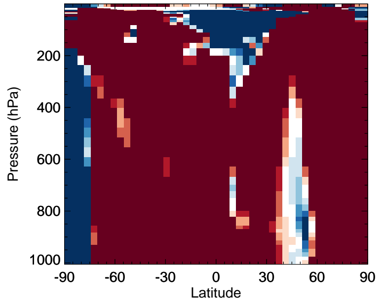
v11-02f-Run0 / v11-02e-Run0 OCPO - Zonal mean % diff for Jan
