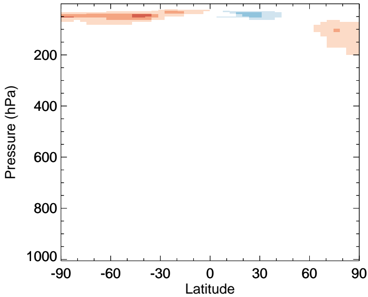
v11-02f-Run0 - v11-02e-Run0 OCS - Zonal mean abs diff for Jan
