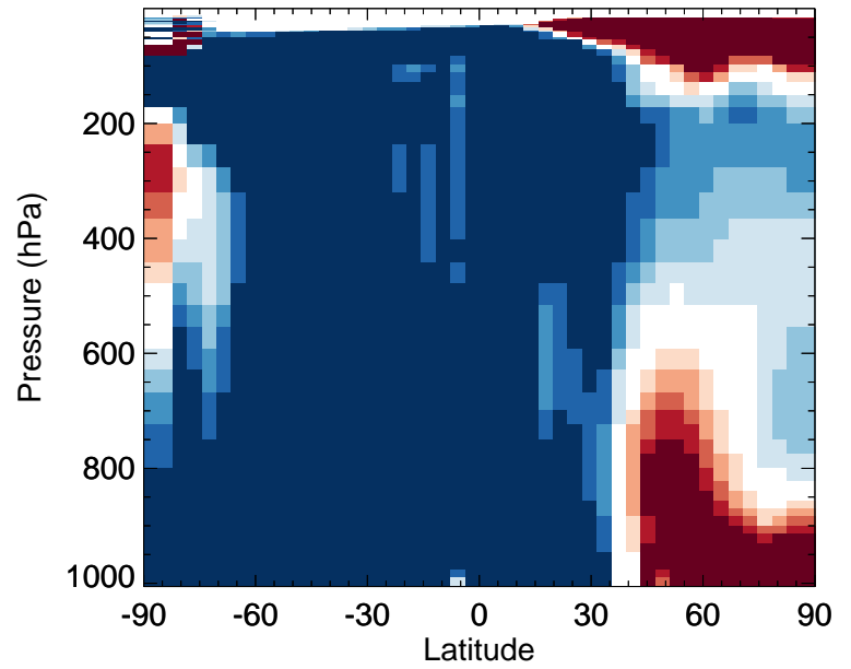
v11-02f-Run0 / v11-02e-Run1 XYLE - Zonal mean % diff for Jan
