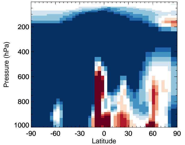
v11-02f-Run0 / v11-02e-Run0 SOAGX - Zonal mean % diff for Jan
