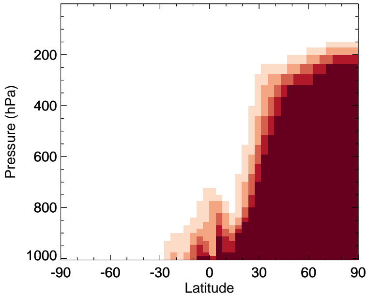
v11-02f-Run0 - v11-02e-Run0 ALK4 - Zonal mean abs diff for Jan
