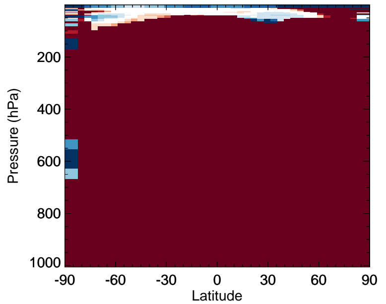
v11-02f-Run0 / v11-02e-Run0 MTPA - Zonal mean % diff for Jan
