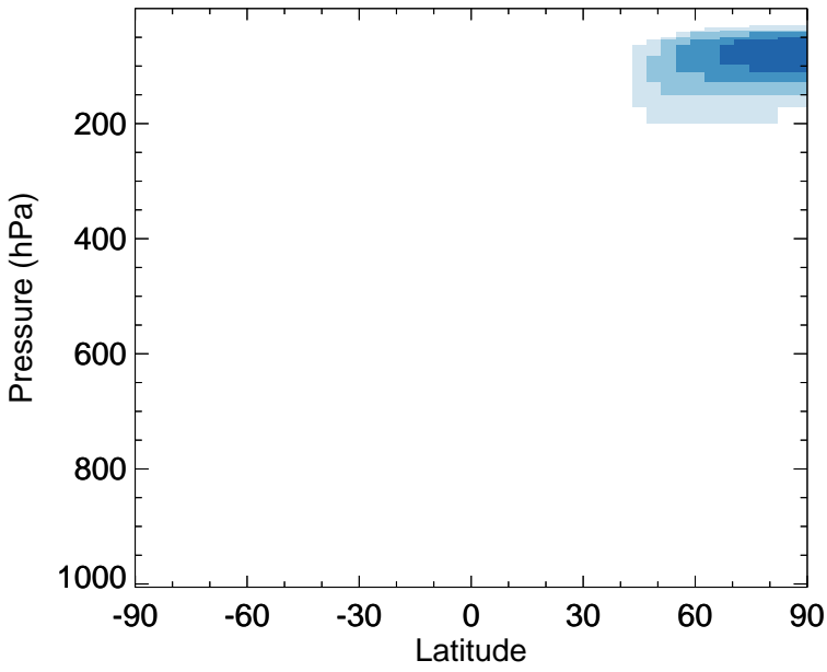
v11-02f-Run0 - v11-02e-Run1 MPN - Zonal mean abs diff for Jan
