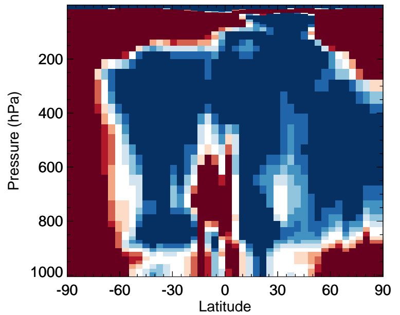
v11-02f-Run0 / v11-02e-Run0 SALC - Zonal mean % diff for Jan
