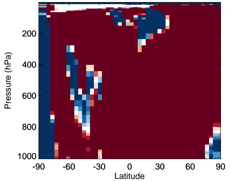
v11-02f-Run0 / v11-02e-Run0 MVKN - Zonal mean % diff for Jan
