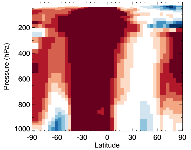
v11-02f-Run0 / v11-02e-Run1 NITs - Zonal mean % diff for Jan
