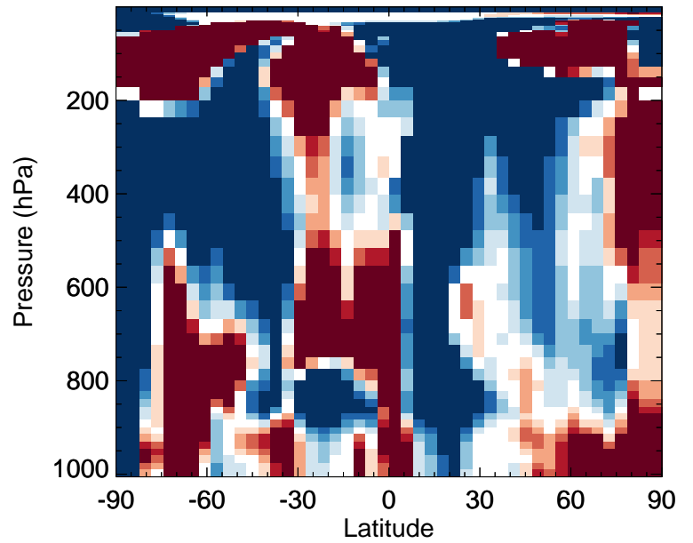
v11-02f-Run0 / v11-02e-Run0 NITs - Zonal mean % diff for Jan
