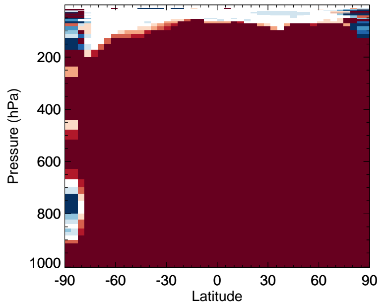
v11-02f-Run0 / v11-02e-Run1 LIMO - Zonal mean % diff for Jan
