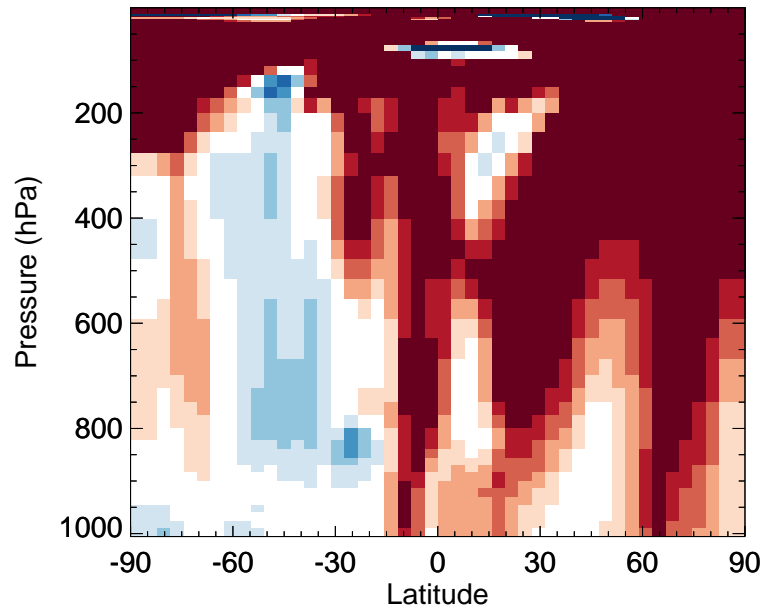
v11-02f-Run0 / v11-02e-Run0 MAP - Zonal mean % diff for Jan
