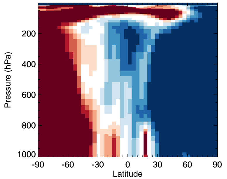
v11-02f-Run0 / v11-02e-Run1 GLYX - Zonal mean % diff for Jan
