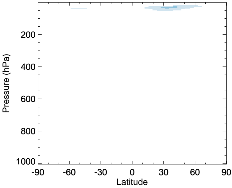
v11-02f-Run0 - v11-02e-Run1 NO - Zonal mean abs diff for Jan
