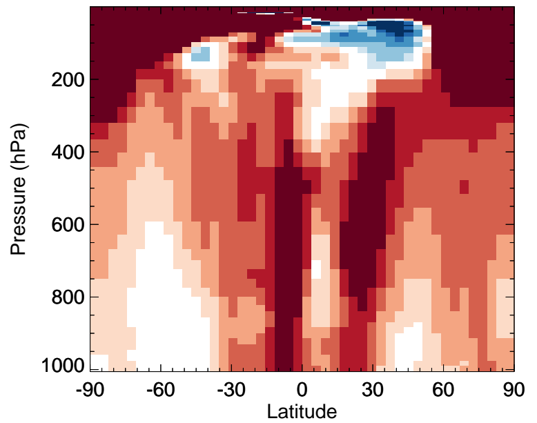
v11-02f-Run0 / v11-02e-Run0 ACET - Zonal mean % diff for Jan
