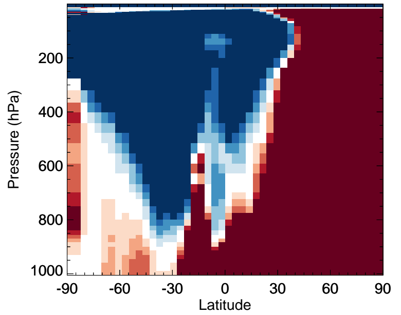
v11-02f-Run0 / v11-02e-Run1 GLYC - Zonal mean % diff for Jan
