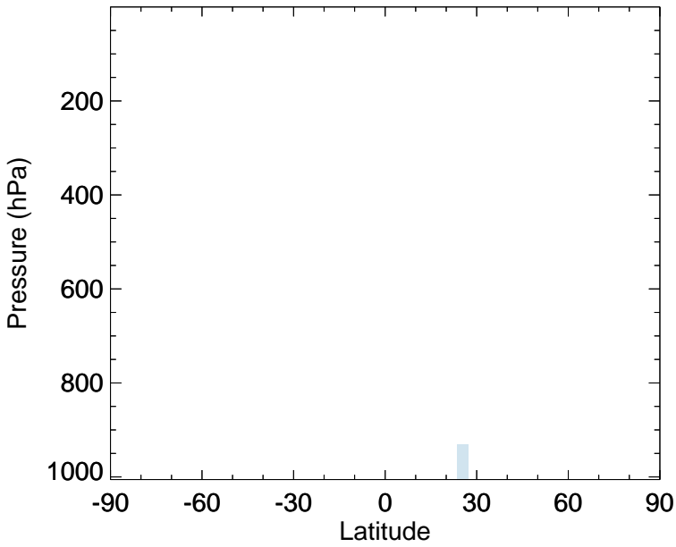
v11-02f-Run0 - v11-02e-Run1 SOAGX - Zonal mean abs diff for Jan
