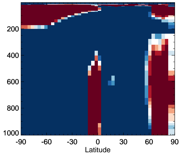
v11-02f-Run0 / v11-02e-Run0 DST2 - Zonal mean % diff for Jan
