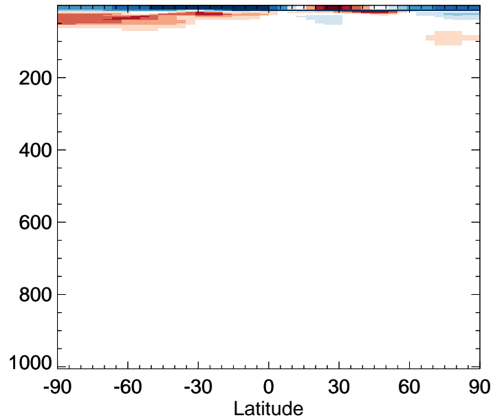
v11-02f-Run0 / v11-02e-Run0 N2O - Zonal mean % diff for Jan
