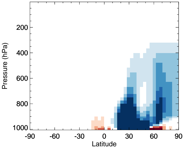
v11-02f-Run0 - v11-02e-Run0 TOLU - Zonal mean abs diff for Jan
