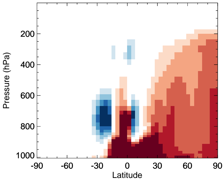
v11-02f-Run0 - v11-02e-Run0 MEK - Zonal mean abs diff for Jan
