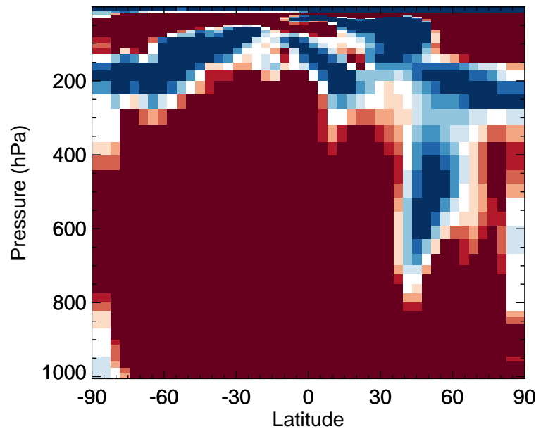
v11-02f-Run0 / v11-02e-Run0 HONIT - Zonal mean % diff for Jan
