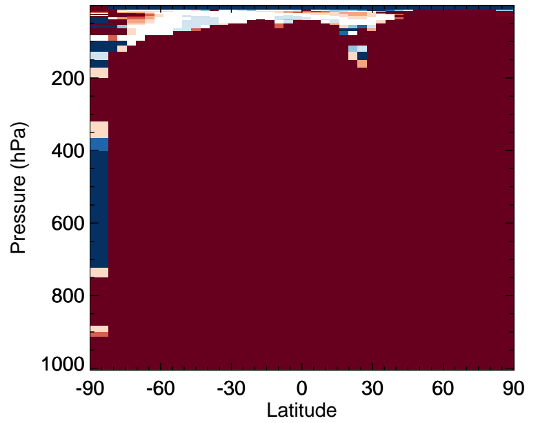
v11-02f-Run0 / v11-02e-Run0 RIPD - Zonal mean % diff for Jan
