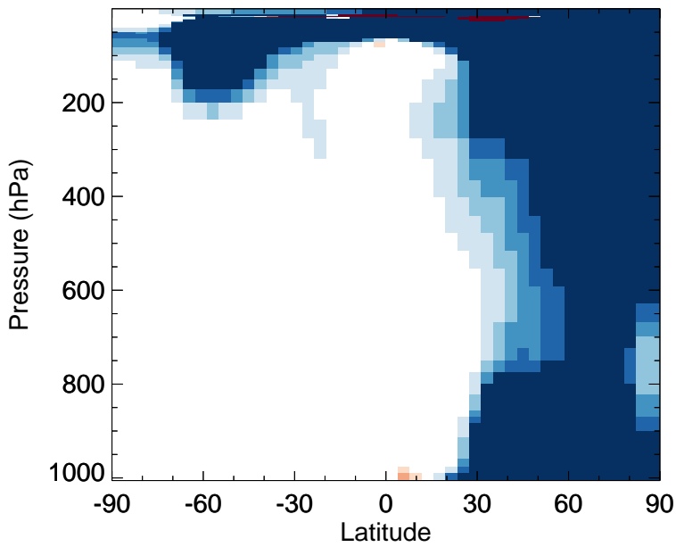
v11-02f-Run0 - v11-02e-Run0 N2O5 - Zonal mean abs diff for Jan
