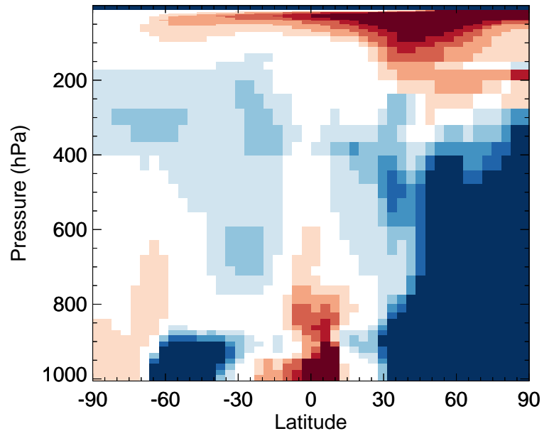
v11-02f-Run0 / v11-02e-Run1 HNO 3 - Zonal mean % diff for Jan
