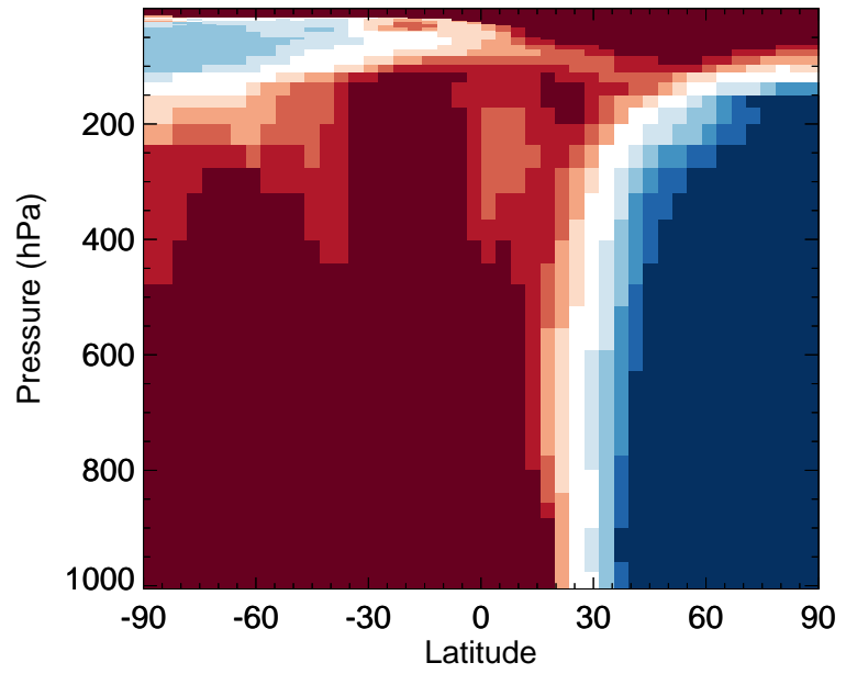
v11-02f-Run0 / v11-02e-Run1 R4N2 - Zonal mean % diff for Jan
