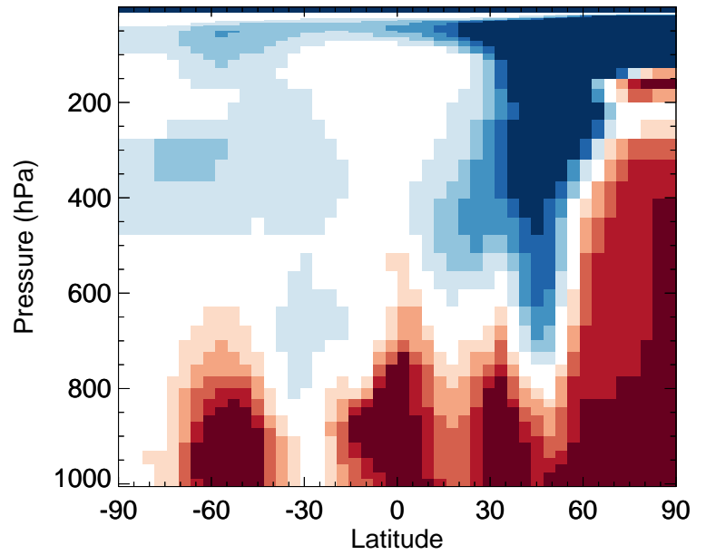
v11-02f-Run0 / v11-02e-Run1 HNO 2 - Zonal mean % diff for Jan
