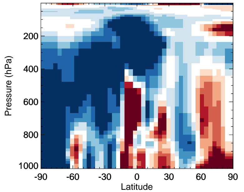
v11-02f-Run0 / v11-02e-Run0 BCPI - Zonal mean % diff for Jan
