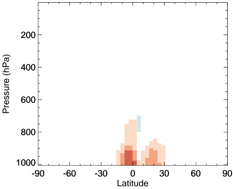
v11-02f-Run0 - v11-02e-Run0 INDIOL - Zonal mean abs diff for Jan
