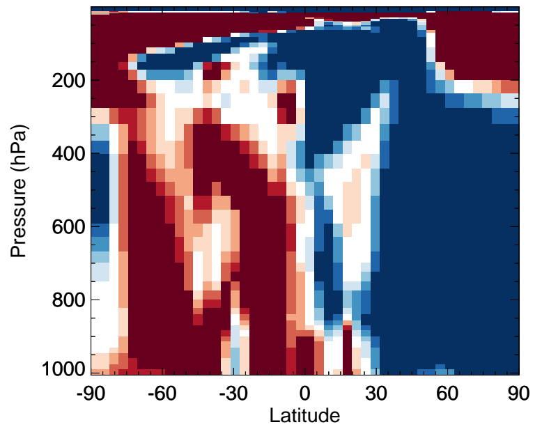
v11-02f-Run0 / v11-02e-Run0 GLYX - Zonal mean % diff for Jan
