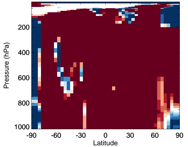
v11-02f-Run0 / v11-02e-Run0 NPMN - Zonal mean % diff for Jan
