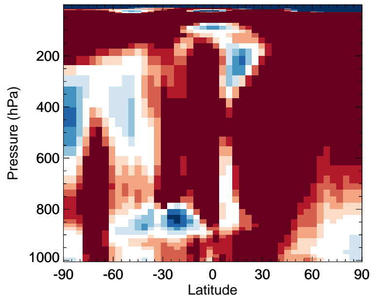
v11-02f-Run0 / v11-02e-Run0 ALD2 - Zonal mean % diff for Jan
