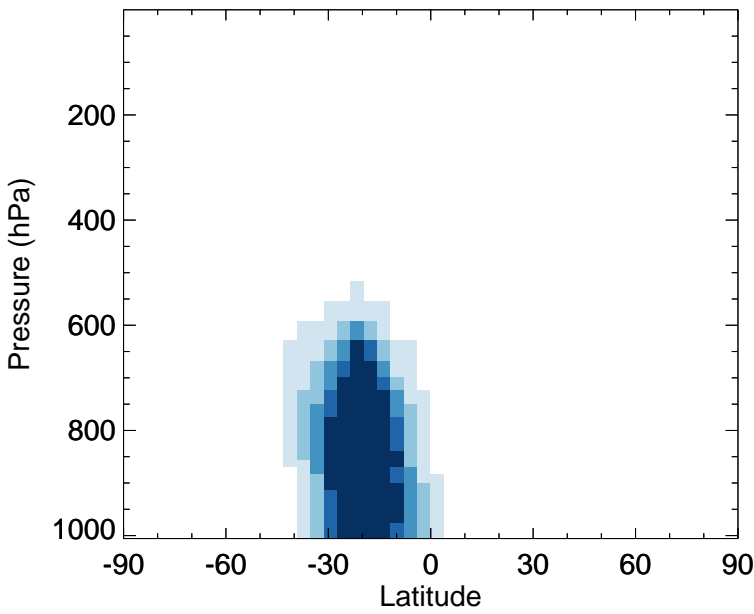
v11-02f-Run0 - v11-02e-Run1 SOAIE - Zonal mean abs diff for Jan
