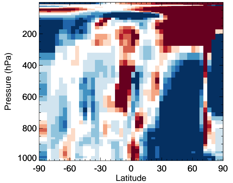
v11-02f-Run0 / v11-02e-Run0 ClO - Zonal mean % diff for Jan
