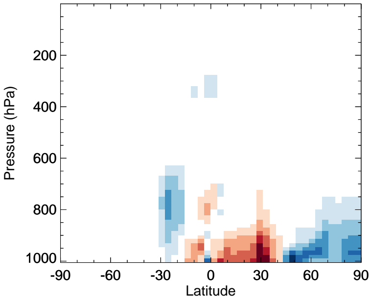
v11-02f-Run0 - v11-02e-Run0 EOH - Zonal mean abs diff for Jan
