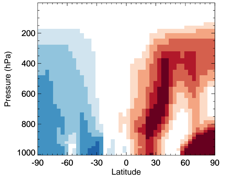
v11-02f-Run0 / v11-02e-Run1 BCPI - Zonal mean % diff for Jan
