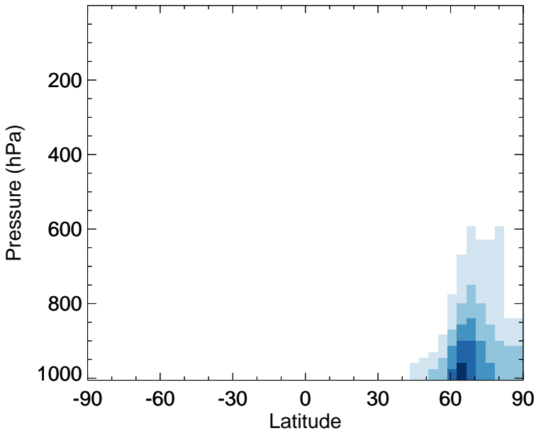
v11-02f-Run0 - v11-02e-Run0 CINO2 - Zonal mean abs diff for Jan
