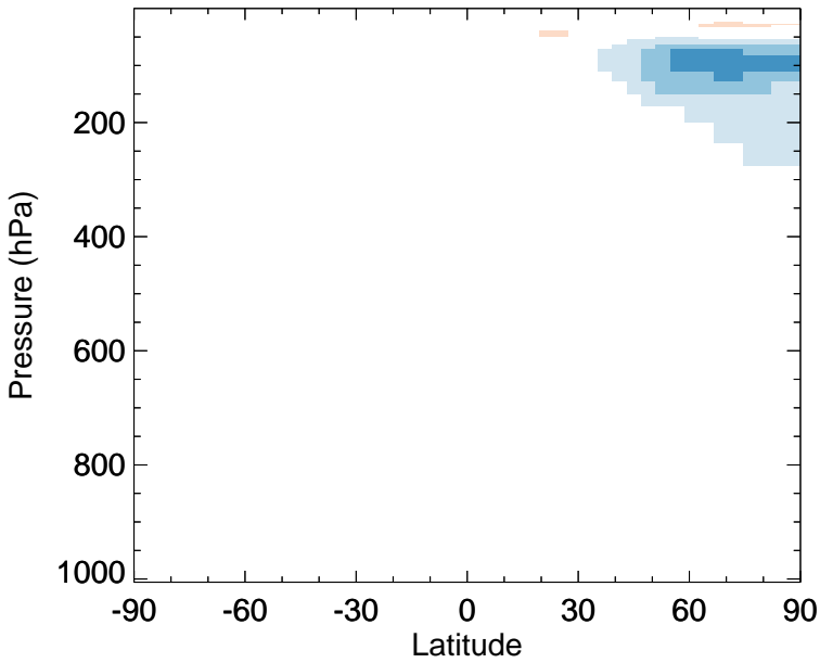
v11-02f-Run0 - v11-02e-Run0 MPN - Zonal mean abs diff for Jan
