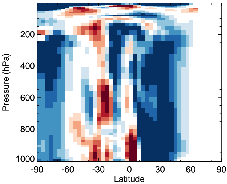
v11-02f-Run0 - v11-02e-Run0 OH - Zonal mean abs diff for Jan
