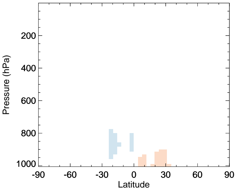
v11-02f-Run0 - v11-02e-Run1 ALD2 - Zonal mean abs diff for Jan
