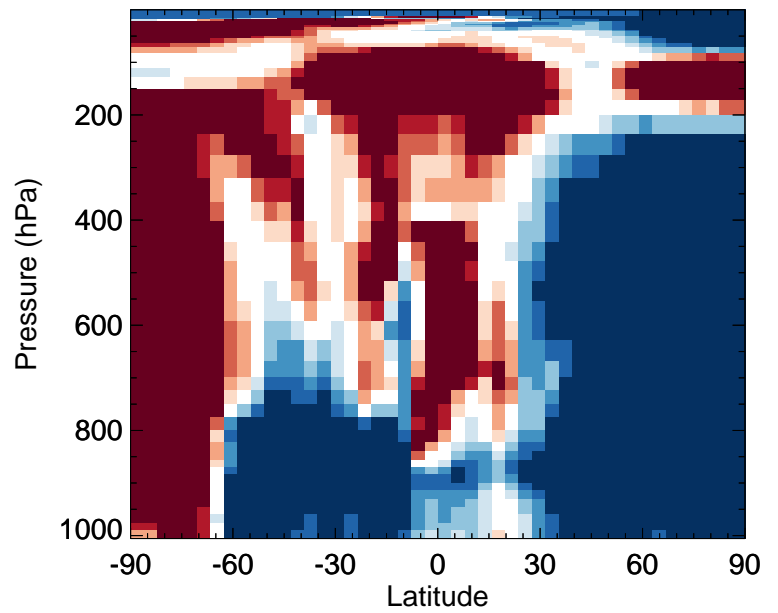
v11-02f-Run0 / v11-02e-Run0 SO 2 - Zonal mean % diff for Jan
