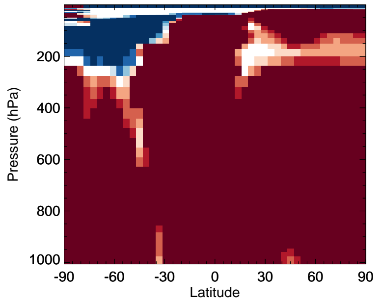
v11-02f-Run0 / v11-02e-Run1 PRPE - Zonal mean % diff for Jan
