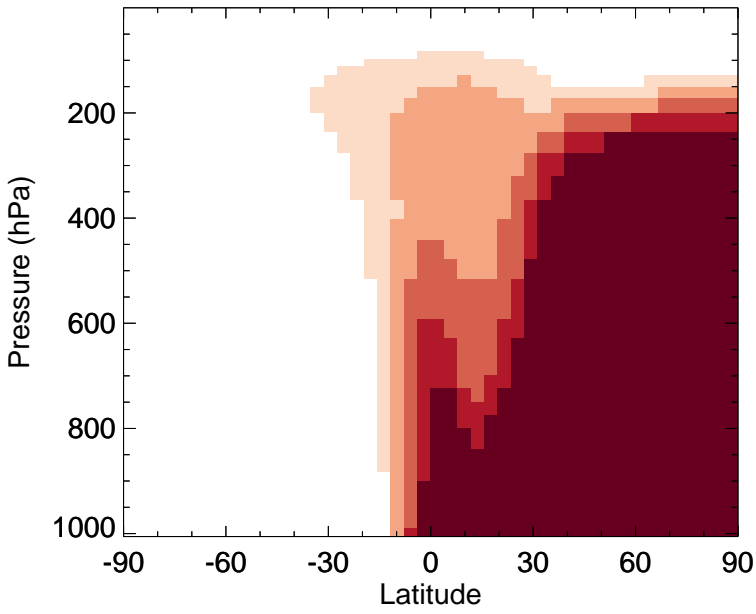
v11-02f-Run0 - v11-02e-Run1 C2H6 - Zonal mean abs diff for Jan
