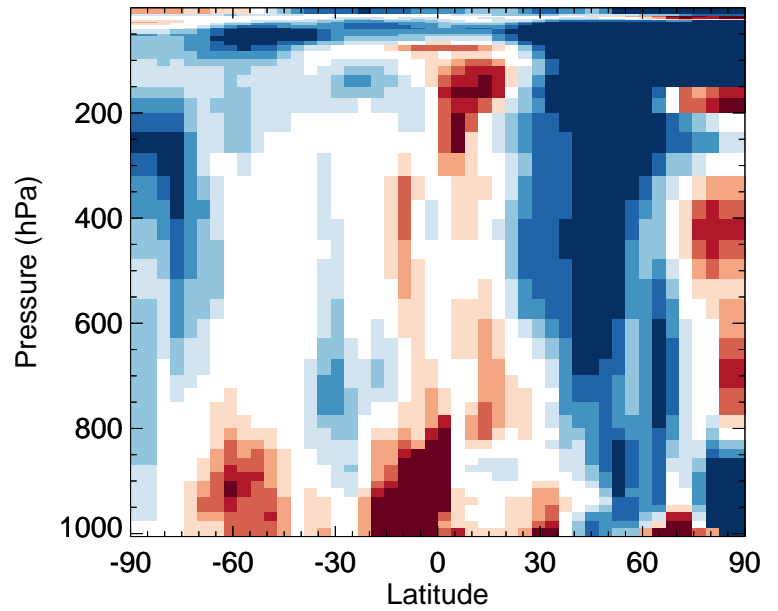
v11-02f-Run0 / v11-02e-Run0 NO 2 - Zonal mean % diff for Jan
