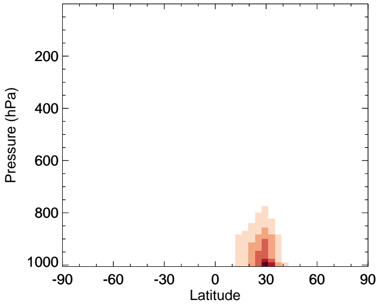
v11-02f-Run0 - v11-02e-Run1 OCPI - Zonal mean abs diff for Jan
