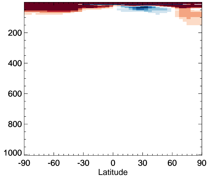
v11-02f-Run0 / v11-02e-Run0 CFC11 - Zonal mean % diff for Jan
