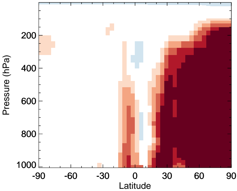
v11-02f-Run0 - v11-02e-Run0 CO - Zonal mean abs diff for Jan
