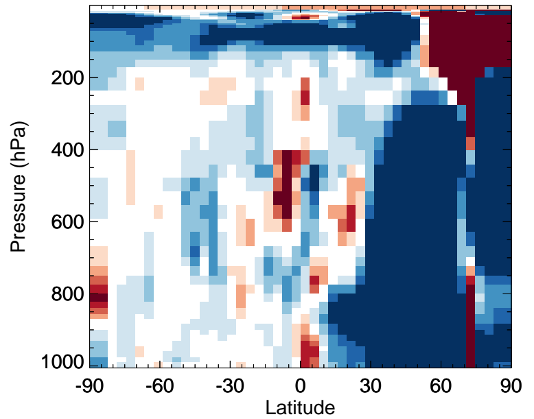
v11-02f-Run0 / v11-02e-Run0 C100 - Zonal mean % diff for Jan
