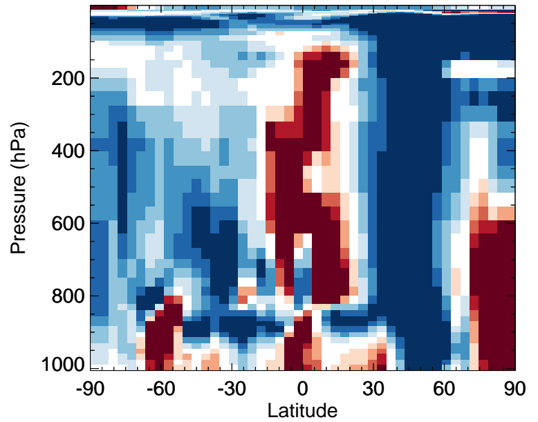
v11-02f-Run0 / v11-02e-Run0 BrNO2 - Zonal mean % diff for Jan
