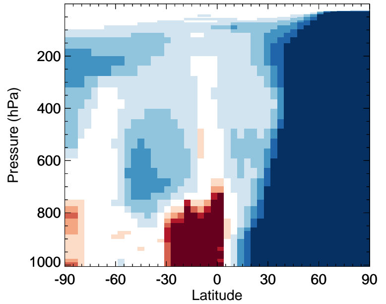
v11-02f-Run0 / v11-02e-Run1 ClNO 3 - Zonal mean % diff for Jan
