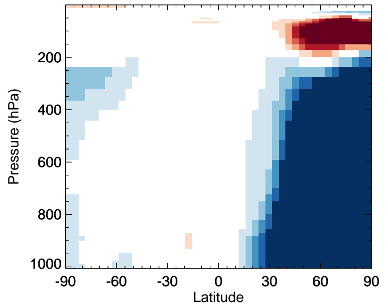
v11-02f-Run0 / v11-02e-Run1 HCl - Zonal mean % diff for Jan
