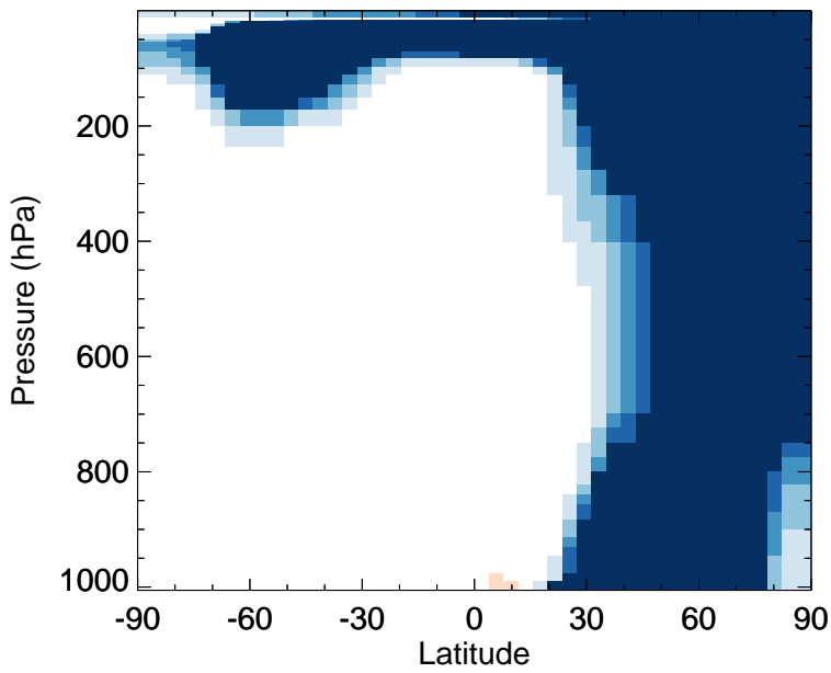
v11-02f-Run0 - v11-02e-Run1 N2O5 - Zonal mean abs diff for Jan
