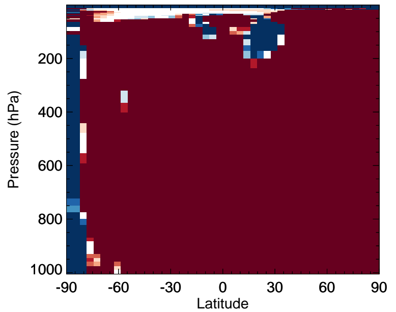
v11-02f-Run0 / v11-02e-Run0 HPALD - Zonal mean % diff for Jan
