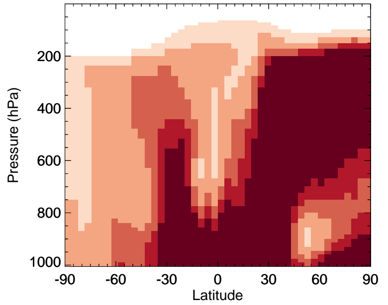
v11-02f-Run0 / v11-02e-Run1 OCPI - Zonal mean % diff for Jan
