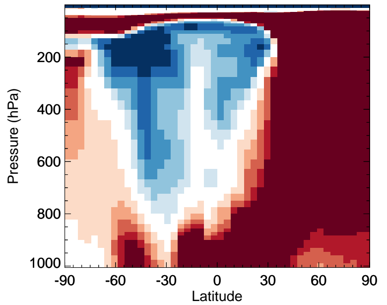
v11-02f-Run0 / v11-02e-Run1 HAC - Zonal mean % diff for Jan
