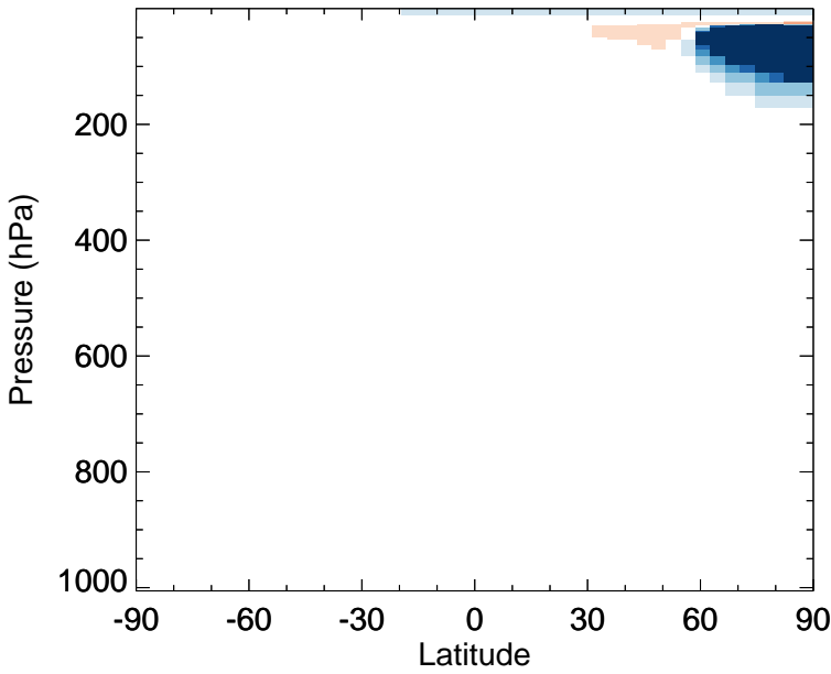
v11-02f-Run0 - v11-02e-Run1 HOCl - Zonal mean abs diff for Jan
