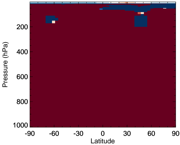
v11-02f-Run0 - v11-02e-Run0 N2O - Zonal mean abs diff for Jan
