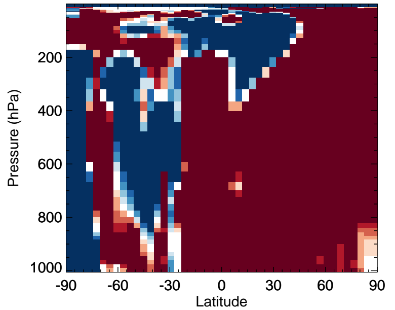
v11-02f-Run0 / v11-02e-Run0 GLYC - Zonal mean % diff for Jan
