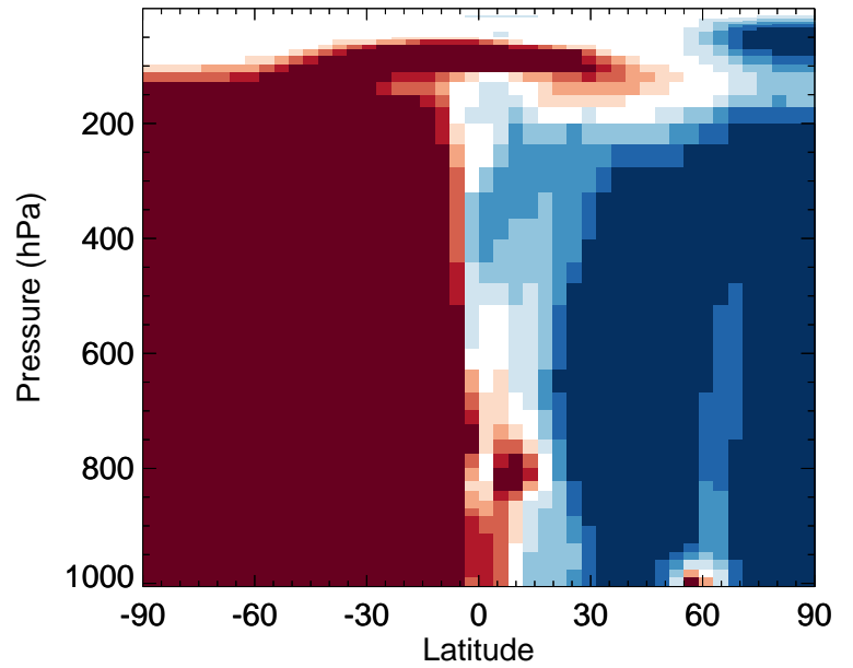
v11-02f-Run0 / v11-02e-Run0 ASOG3 - Zonal mean % diff for Jan
