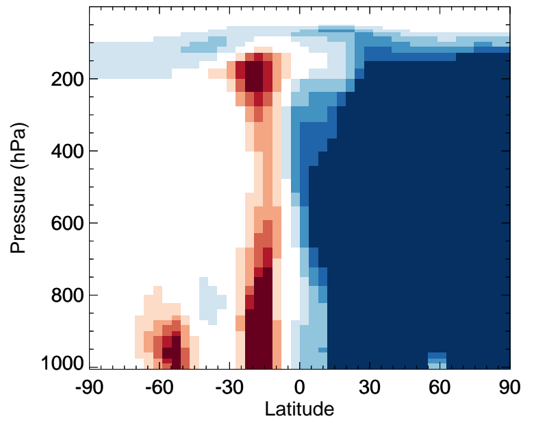
v11-02f-Run0 / v11-02e-Run1 ASOG2 - Zonal mean % diff for Jan
