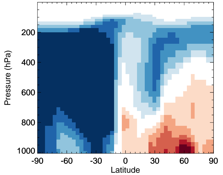
v11-02f-Run0 / v11-02e-Run1 SOAGX - Zonal mean % diff for Jan
