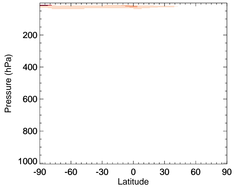
v11-02f-Run0 / v11-02e-Run1 CH 2 Br 2 - Zonal mean % diff for Jan
