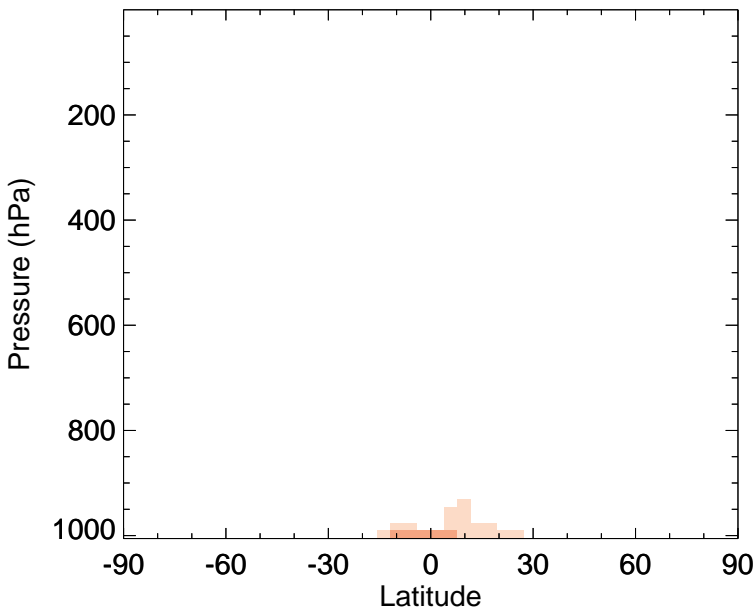
v11-02f-Run0 - v11-02e-Run1 RCHO - Zonal mean abs diff for Jan
