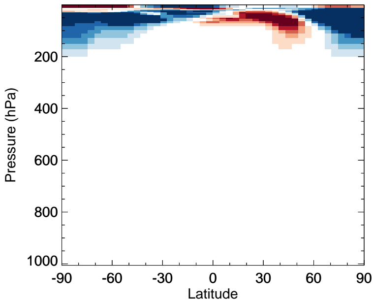
v11-02f-Run0 - v11-02e-Run0 HCl - Zonal mean abs diff for Jan
