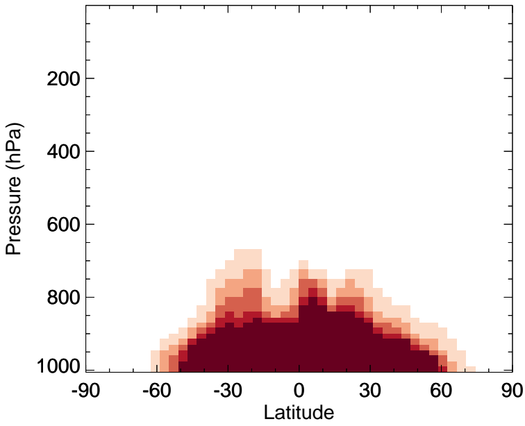
v11-02f-Run0 - v11-02e-Run1 NH3 - Zonal mean abs diff for Jan
