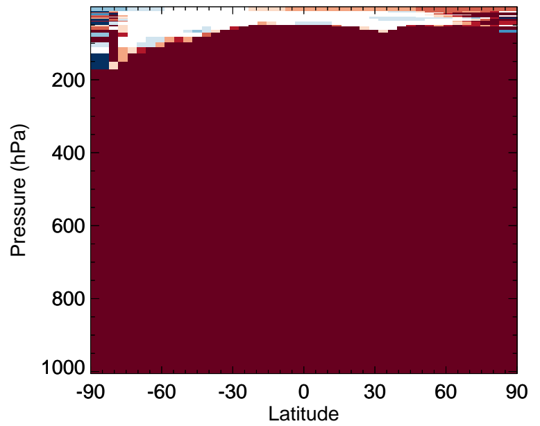
v11-02f-Run0 / v11-02e-Run1 MTPA - Zonal mean % diff for Jan
