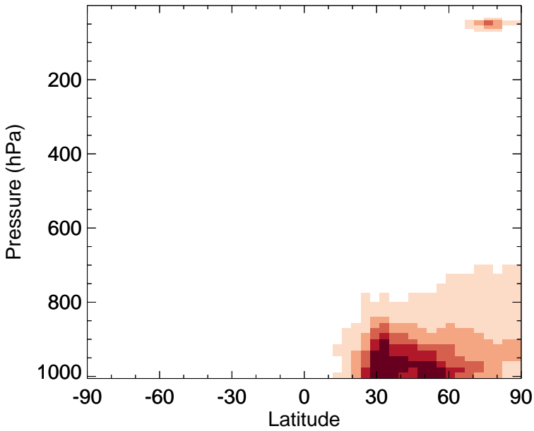
v11-02f-Run0 - v11-02e-Run0 NIT - Zonal mean abs diff for Jan
