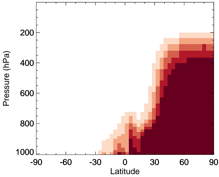
v11-02f-Run0 - v11-02e-Run1 ALK4 - Zonal mean abs diff for Jan
