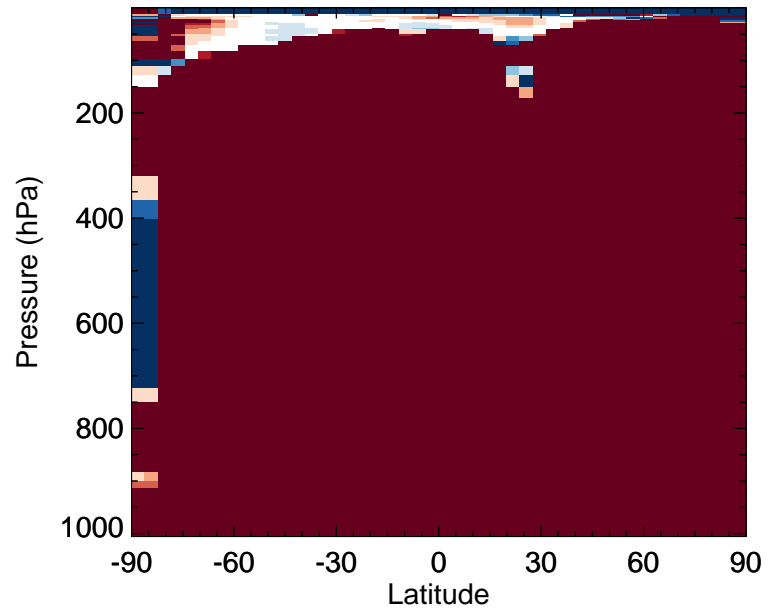
v11-02f-Run0 / v11-02e-Run0 RIPB - Zonal mean % diff for Jan
