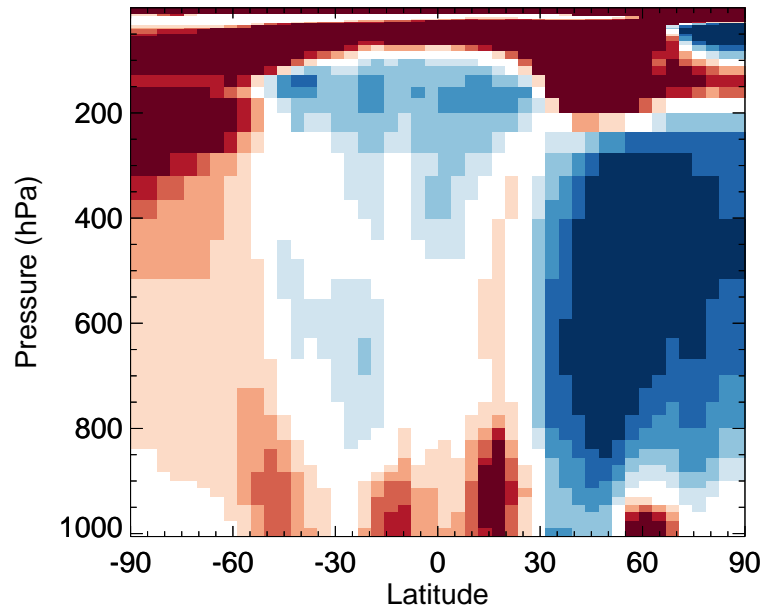
v11-02f-Run0 / v11-02e-Run1 MGLY - Zonal mean % diff for Jan
