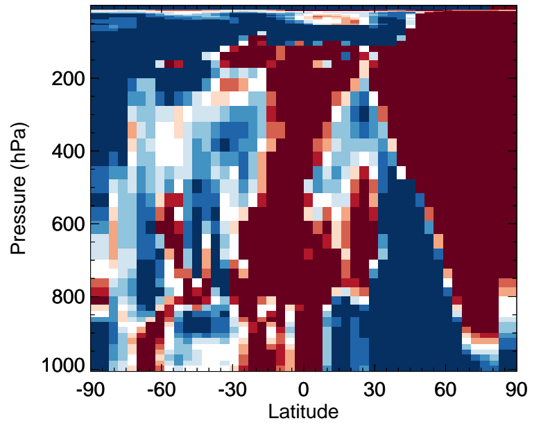
v11-02f-Run0 / v11-02e-Run0 Cl2 - Zonal mean % diff for Jan
