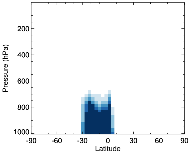
v11-02f-Run0 - v11-02e-Run1 ISOP - Zonal mean abs diff for Jan
