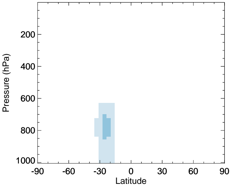
v11-02f-Run0 - v11-02e-Run0 ISO3 - Zonal mean abs diff for Jan
