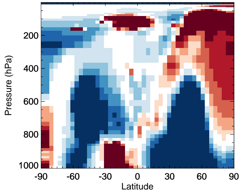
v11-02f-Run0 / v11-02e-Run1 Cl2 - Zonal mean % diff for Jan
