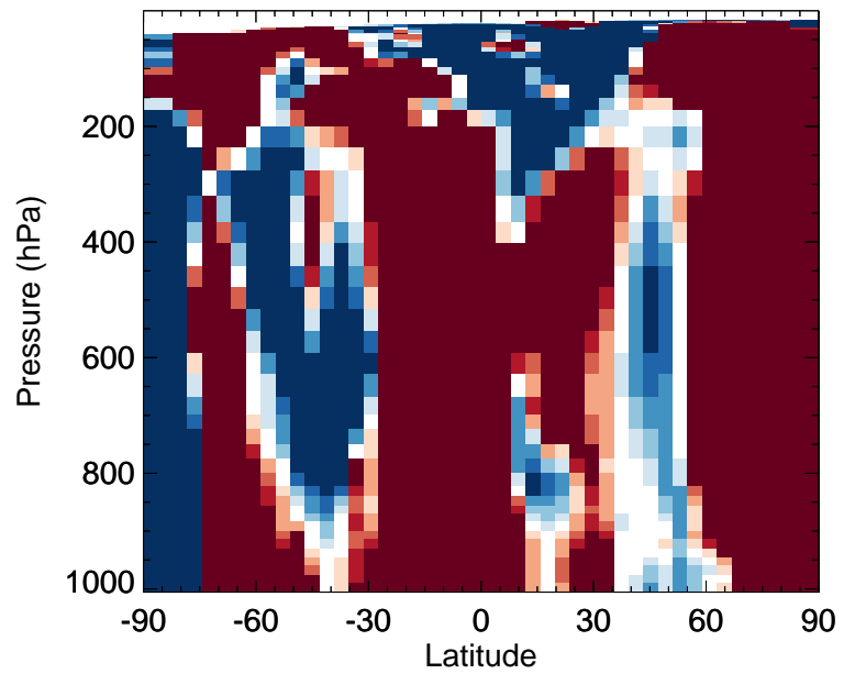
v11-02f-Run0 / v11-02e-Run0 SOAP - Zonal mean % diff for Jan
