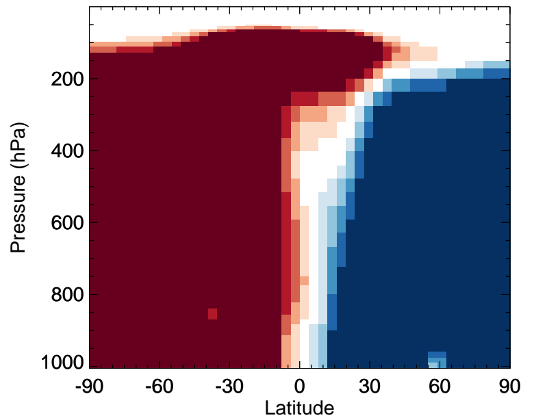
v11-02f-Run0 / v11-02e-Run1 ASOG1 - Zonal mean % diff for Jan
