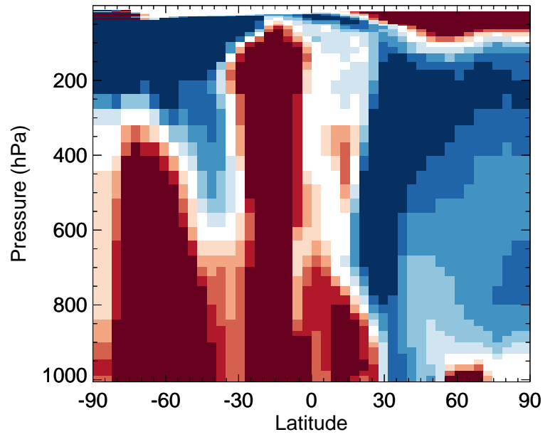
v11-02f-Run0 / v11-02e-Run1 TOLU - Zonal mean % diff for Jan
