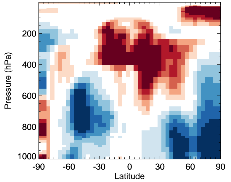
v11-02f-Run0 / v11-02e-Run1 BrCl - Zonal mean % diff for Jan
