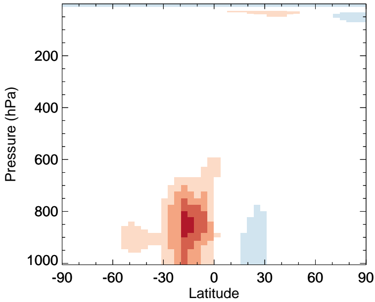
v11-02f-Run0 - v11-02e-Run1 H2O2 - Zonal mean abs diff for Jan
