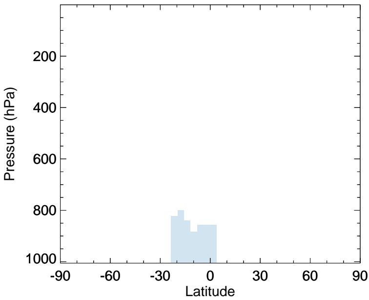
v11-02f-Run0 - v11-02e-Run1 HPALD - Zonal mean abs diff for Jan
