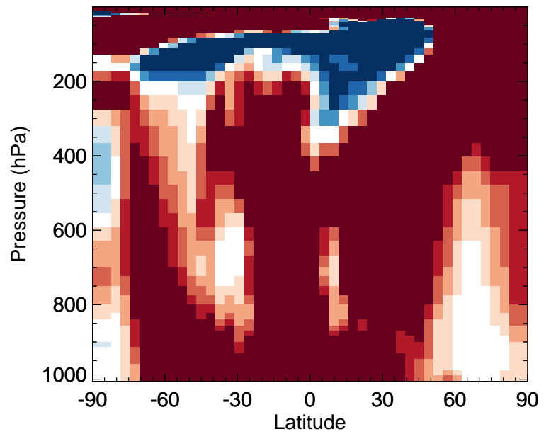
v11-02f-Run0 / v11-02e-Run0 RCHO - Zonal mean % diff for Jan
