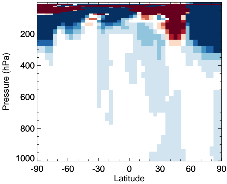
v11-02f-Run0 - v11-02e-Run0 O3 - Zonal mean abs diff for Jan
