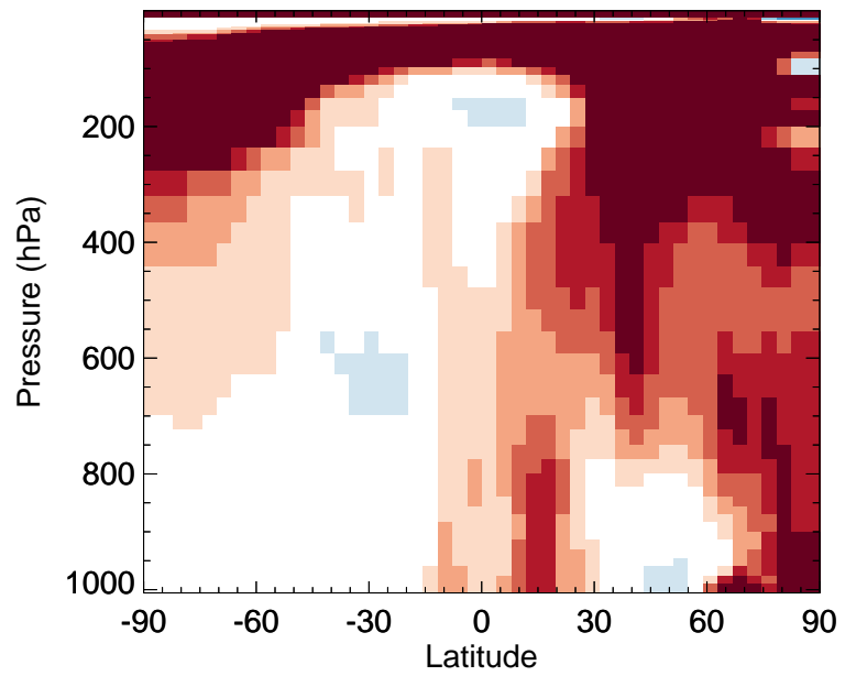
v11-02f-Run0 / v11-02e-Run1 ACTA - Zonal mean % diff for Jan
