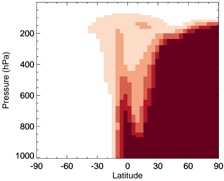
v11-02f-Run0 - v11-02e-Run0 C2H6 - Zonal mean abs diff for Jan
