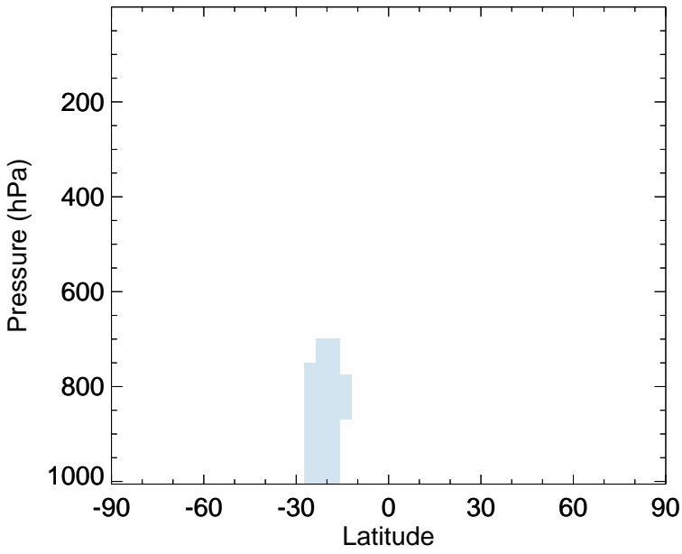
v11-02f-Run0 - v11-02e-Run1 ISO3 - Zonal mean abs diff for Jan
