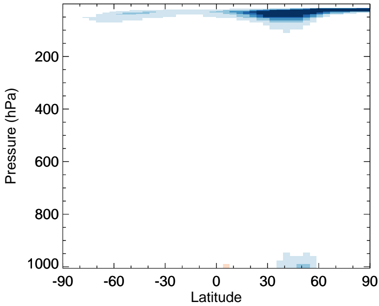
v11-02f-Run0 - v11-02e-Run1 NO 2 - Zonal mean abs diff for Jan
