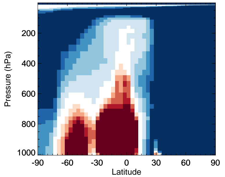
v11-02f-Run0 / v11-02e-Run1 N2O5 - Zonal mean % diff for Jan
