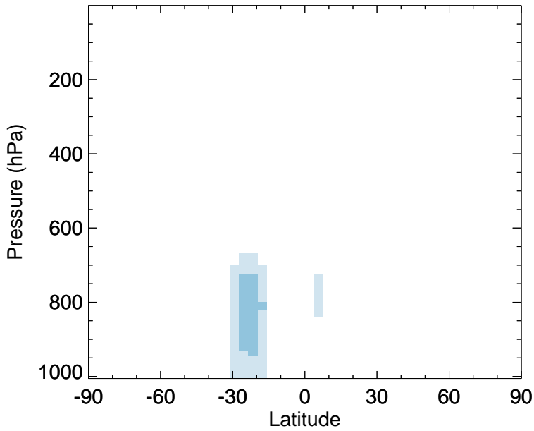
v11-02f-Run0 - v11-02e-Run0 GLYC - Zonal mean abs diff for Jan
