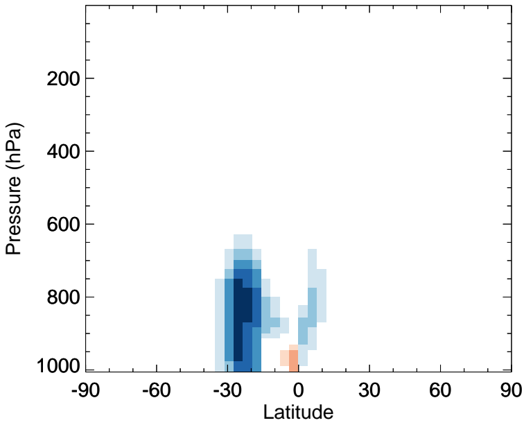
v11-02f-Run0 - v11-02e-Run0 MVK - Zonal mean abs diff for Jan
