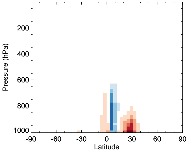
v11-02f-Run0 - v11-02e-Run0 OCPI - Zonal mean abs diff for Jan
