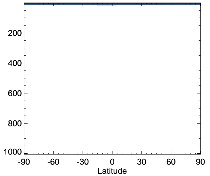
v11-02f-Run0 / v11-02e-Run1 CCI4 - Zonal mean % diff for Jan
