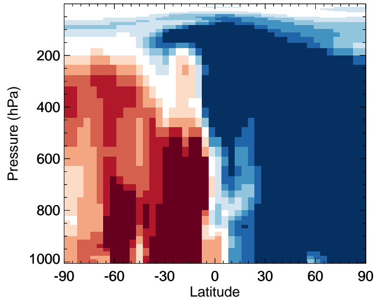
v11-02f-Run0 / v11-02e-Run0 ASOAN - Zonal mean % diff for Jan
