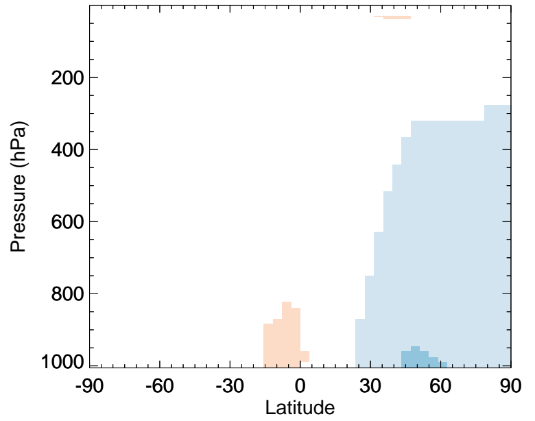
v11-02f-Run0 / v11-02e-Run1 O3 - Zonal mean % diff for Jan
