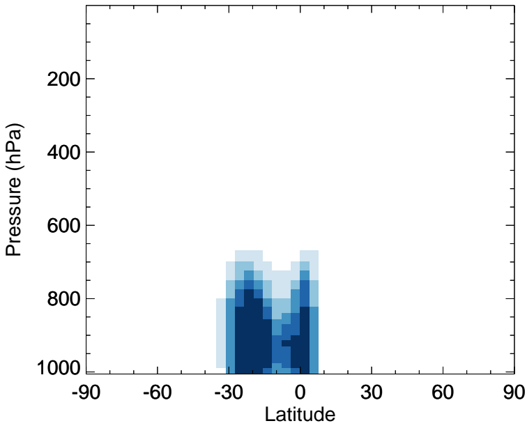
v11-02f-Run0 - v11-02e-Run1 MVK - Zonal mean abs diff for Jan
