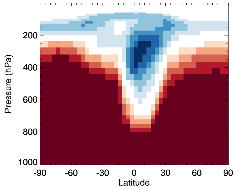
v11-02f-Run0 / v11-02e-Run1 TSOA1 - Zonal mean % diff for Jan
