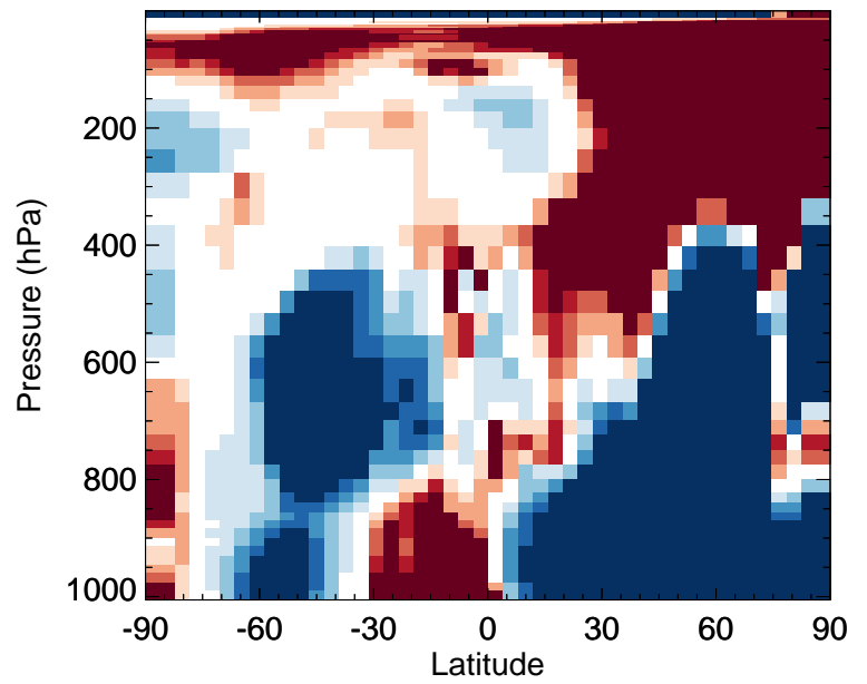
v11-02f-Run0 / v11-02e-Run1 Cl2O2 - Zonal mean % diff for Jan
