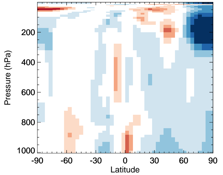
v11-02f-Run0 / v11-02e-Run0 O3 - Zonal mean % diff for Jan
