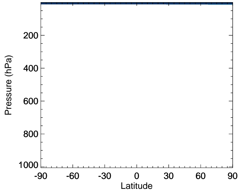
v11-02f-Run0 / v11-02e-Run1 CH4 - Zonal mean % diff for Jan
