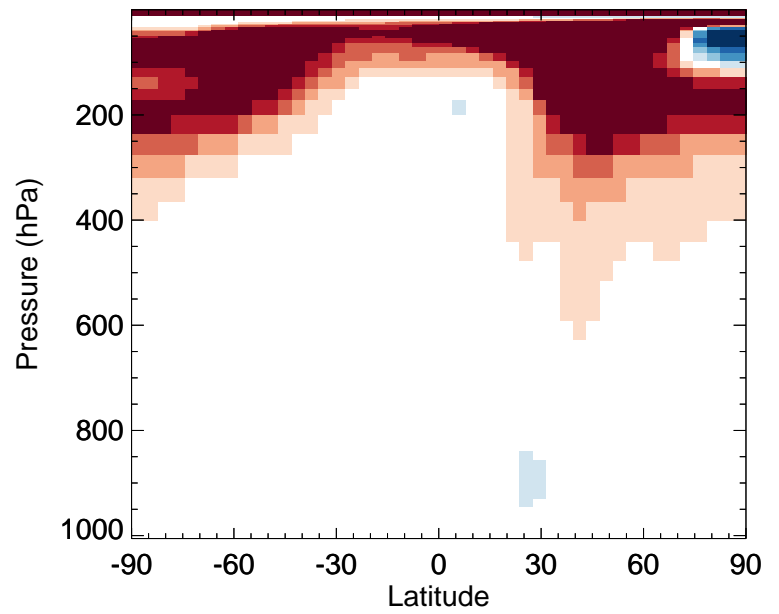
v11-02f-Run0 / v11-02e-Run1 MP - Zonal mean % diff for Jan
