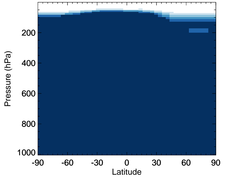
v11-02f-Run0 / v11-02e-Run1 SOAME - Zonal mean % diff for Jan
