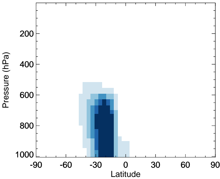
v11-02f-Run0 - v11-02e-Run0 SOAIE - Zonal mean abs diff for Jan
