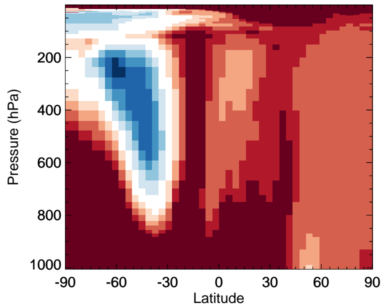
v11-02f-Run0 / v11-02e-Run1 MEK - Zonal mean % diff for Jan
