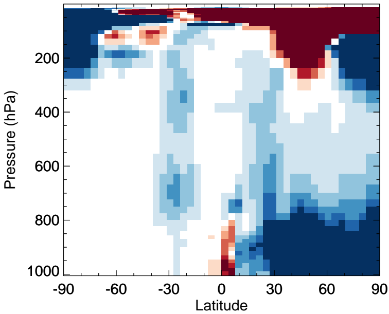
v11-02f-Run0 - v11-02e-Run0 HNO 3 - Zonal mean abs diff for Jan
