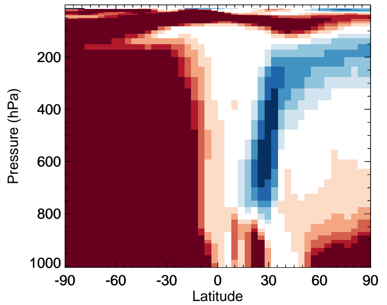
v11-02f-Run0 / v11-02e-Run1 BENZ - Zonal mean % diff for Jan
