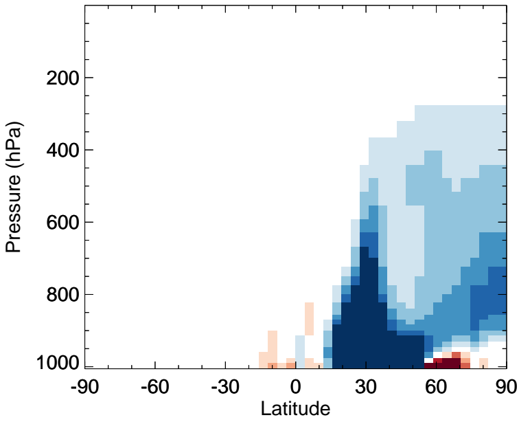
v11-02f-Run0 - v11-02e-Run1 TOLU - Zonal mean abs diff for Jan
