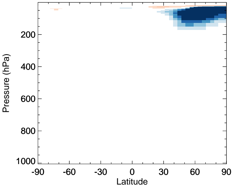
v11-02f-Run0 - v11-02e-Run1 ClNO 3 - Zonal mean abs diff for Jan
