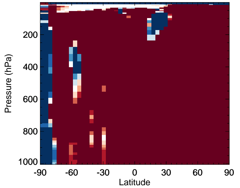
v11-02f-Run0 / v11-02e-Run0 MVK - Zonal mean % diff for Jan
