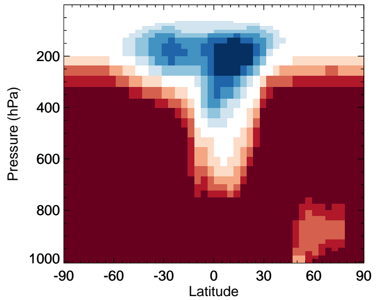
v11-02f-Run0 / v11-02e-Run1 TSOA3 - Zonal mean % diff for Jan
