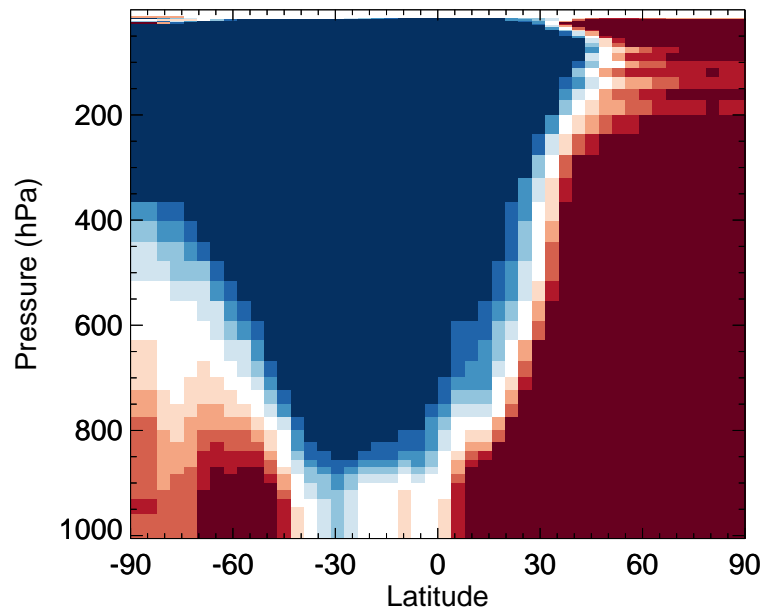
v11-02f-Run0 / v11-02e-Run1 IMAE - Zonal mean % diff for Jan
