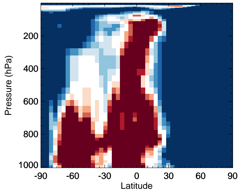
v11-02f-Run0 / v11-02e-Run0 N2O5 - Zonal mean % diff for Jan
