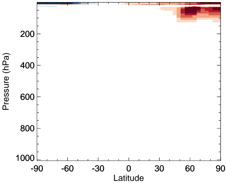
v11-02f-Run0 - v11-02e-Run0 ClO - Zonal mean abs diff for Jan
