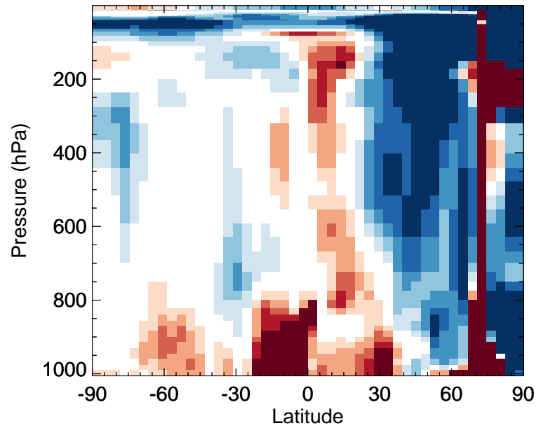
v11-02f-Run0 / v11-02e-Run0 NO - Zonal mean % diff for Jan
