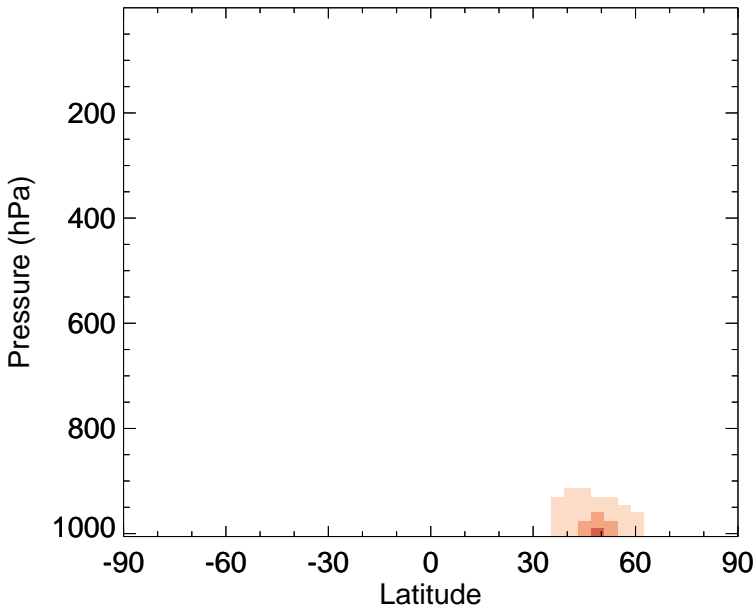
v11-02f-Run0 - v11-02e-Run1 SO4 - Zonal mean abs diff for Jan
