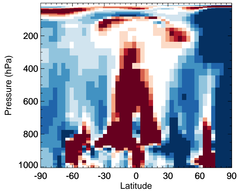
v11-02f-Run0 / v11-02e-Run0 HOBr - Zonal mean % diff for Jan
