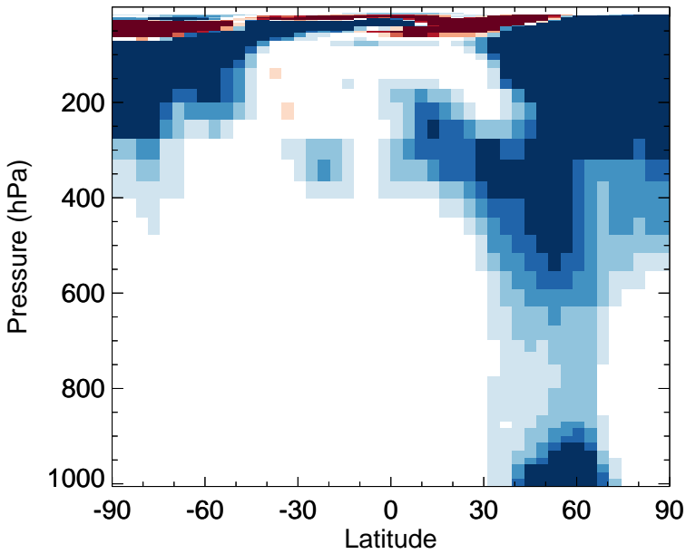
v11-02f-Run0 - v11-02e-Run0 HNO 4 - Zonal mean abs diff for Jan
