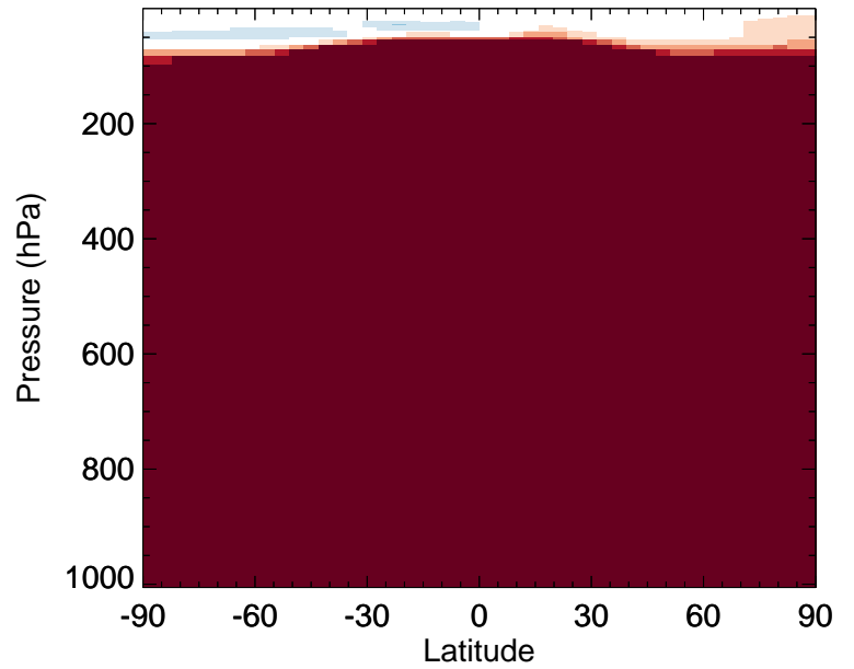
v11-02f-Run0 / v11-02e-Run0 NH4 - Zonal mean % diff for Jan
