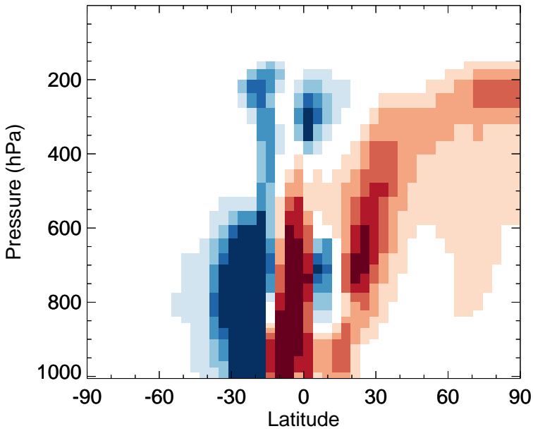
v11-02f-Run0 - v11-02e-Run0 MAP - Zonal mean abs diff for Jan
