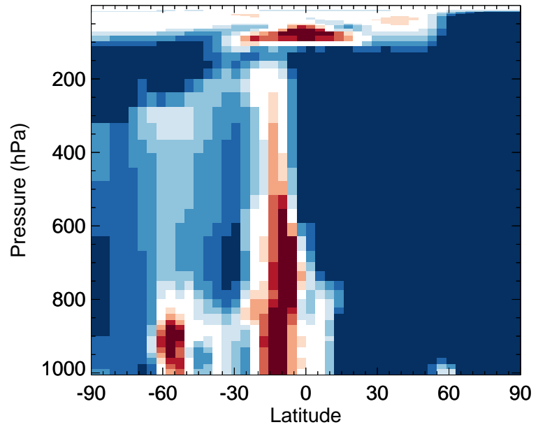
v11-02f-Run0 / v11-02e-Run0 ASOG2 - Zonal mean % diff for Jan
