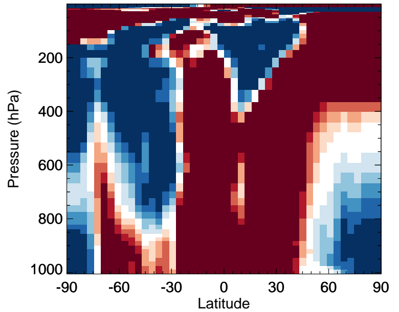
v11-02f-Run0 / v11-02e-Run0 EOH - Zonal mean % diff for Jan
