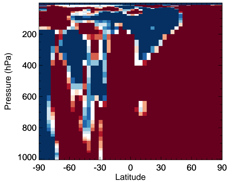
v11-02f-Run0 / v11-02e-Run0 HC187 - Zonal mean % diff for Jan
