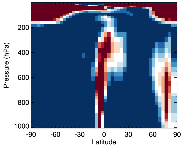
v11-02f-Run0 / v11-02e-Run0 DST1 - Zonal mean % diff for Jan
