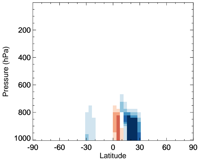
v11-02f-Run0 - v11-02e-Run0 DST3 - Zonal mean abs diff for Jan
