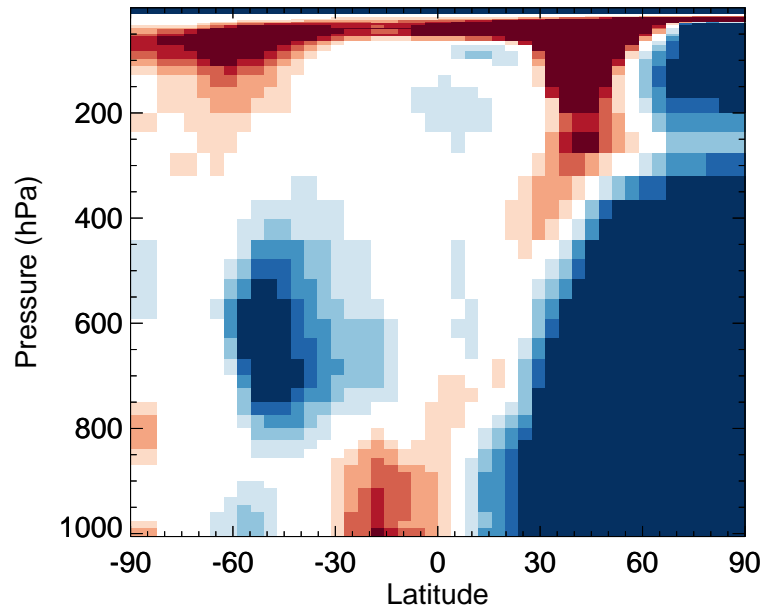
v11-02f-Run0 / v11-02e-Run1 HOCl - Zonal mean % diff for Jan
