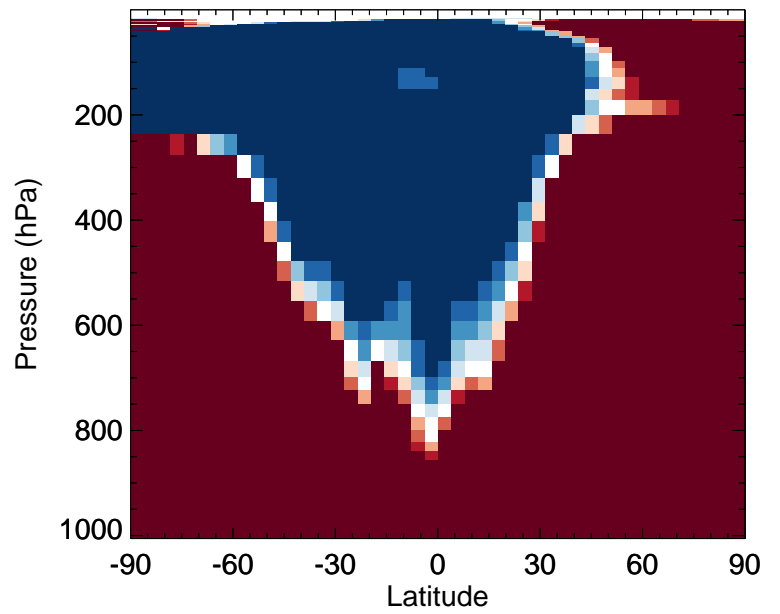
v11-02f-Run0 / v11-02e-Run1 IEPOXA - Zonal mean % diff for Jan
