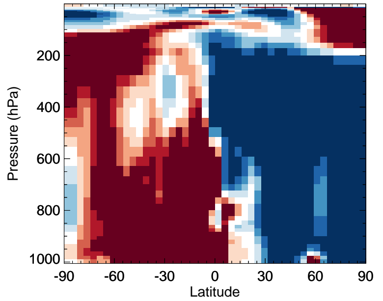
v11-02f-Run0 / v11-02e-Run0 ASOA1 - Zonal mean % diff for Jan
