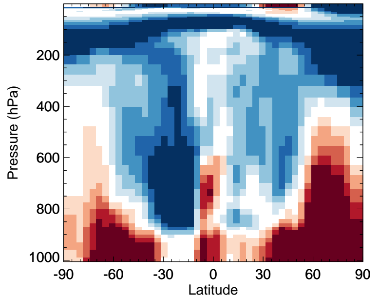
v11-02f-Run0 / v11-02e-Run0 SO4 - Zonal mean % diff for Jan
