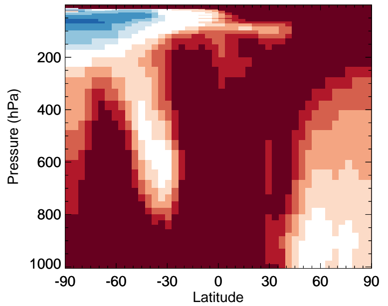
v11-02f-Run0 / v11-02e-Run1 RCHO - Zonal mean % diff for Jan
