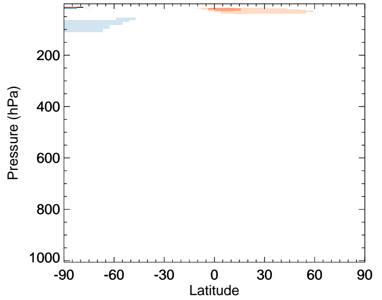
v11-02f-Run0 / v11-02e-Run1 CHBr3 - Zonal mean % diff for Jan
