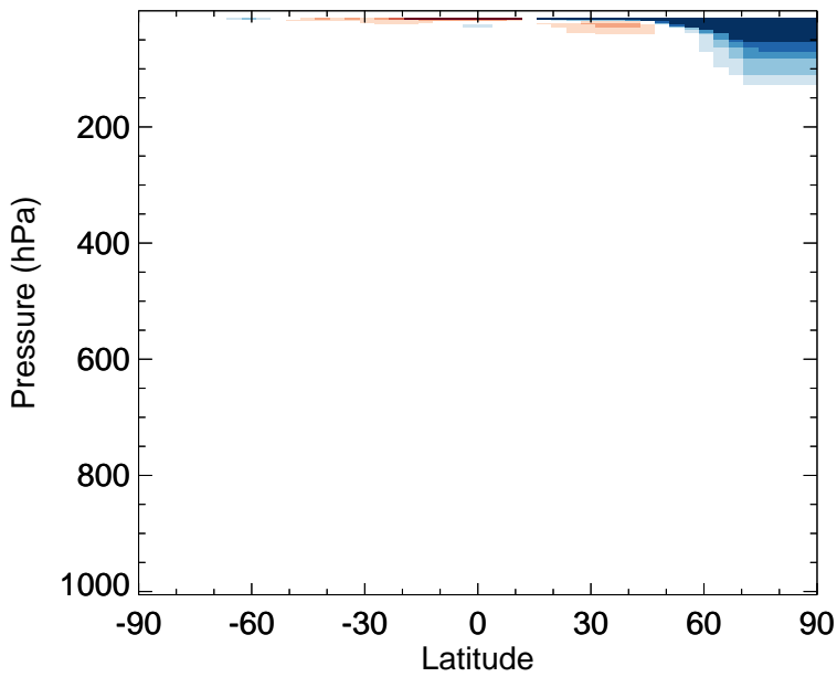
v11-02f-Run0 - v11-02e-Run0 NO3 - Zonal mean abs diff for Jan
