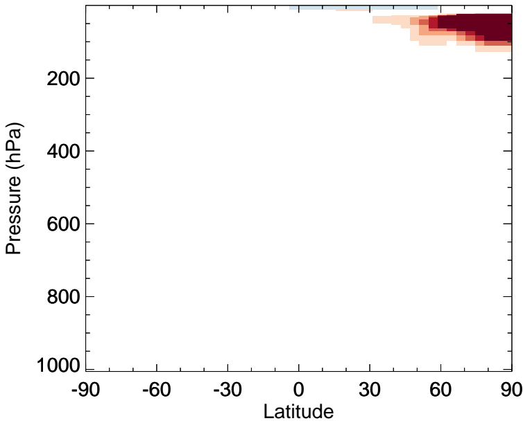
v11-02f-Run0 - v11-02e-Run0 HOCl - Zonal mean abs diff for Jan
