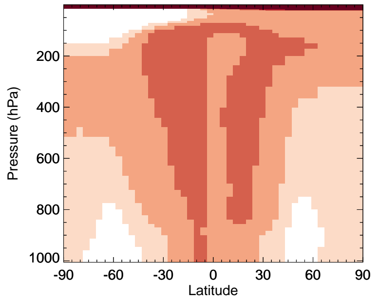
v11-02f-Run0 / v11-02e-Run1 ACET - Zonal mean % diff for Jan
