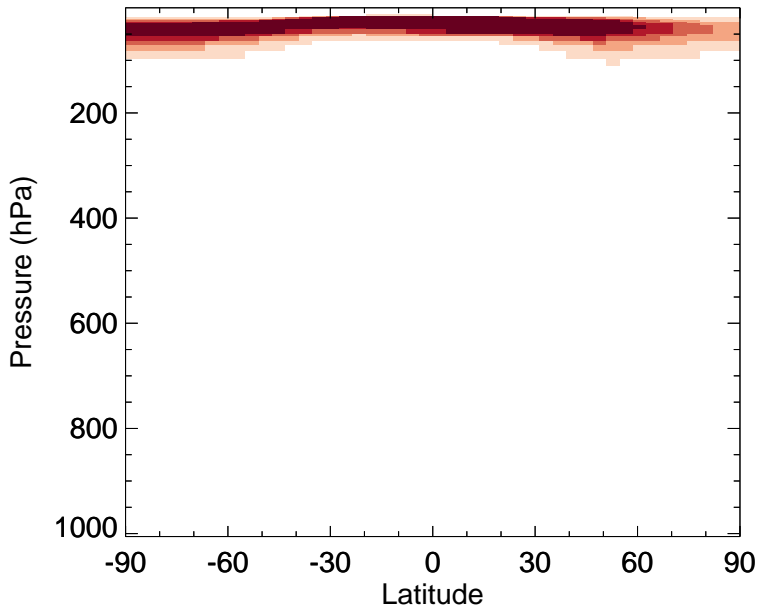
v11-02f-Run0 - v11-02e-Run1 N2O - Zonal mean abs diff for Jan
