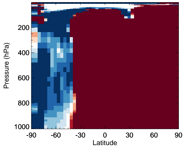
v11-02f-Run0 / v11-02e-Run1 ISOP - Zonal mean % diff for Jan
