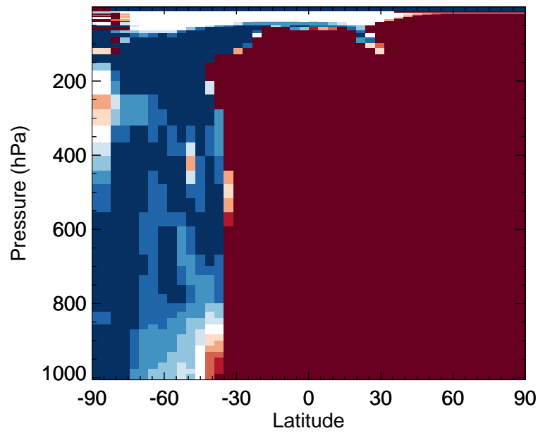
v11-02f-Run0 / v11-02e-Run1 RIPA - Zonal mean % diff for Jan
