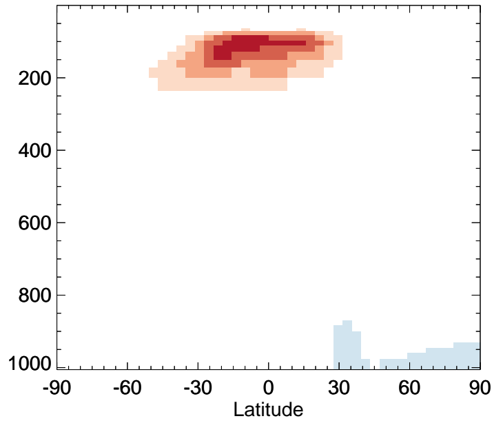
v11-02f-Run0 / v11-02e-Run1 ISO2 - Zonal mean % diff for Jan
