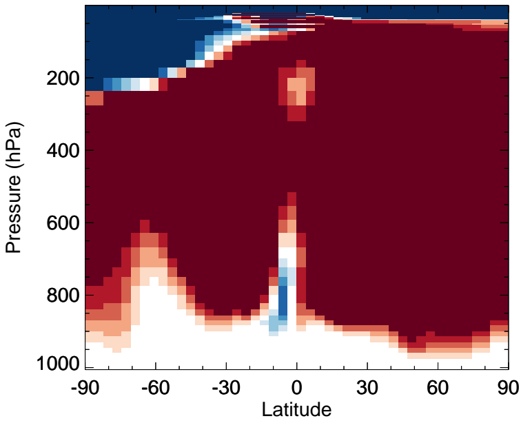
v11-02f-Run0 - v11-02e-Run1 CH4 - Zonal mean abs diff for Jan
