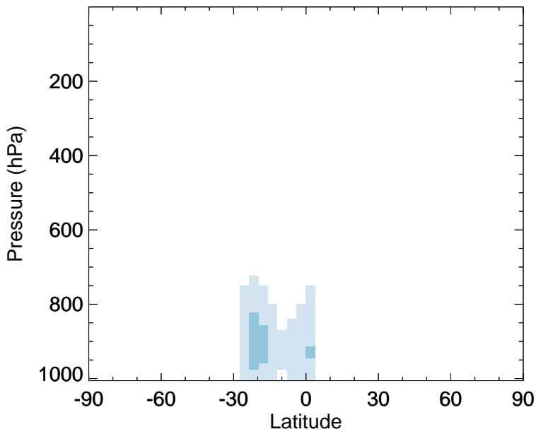
v11-02f-Run0 - v11-02e-Run1 RIPA - Zonal mean abs diff for Jan
