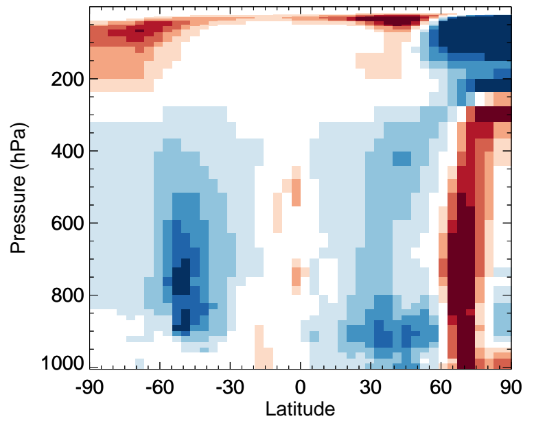
v11-02f-Run0 / v11-02e-Run1 HOBr - Zonal mean % diff for Jan
