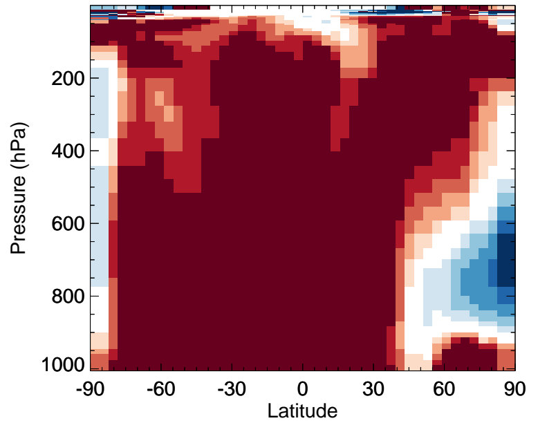
v11-02f-Run0 / v11-02e-Run1 OCPO - Zonal mean % diff for Jan
