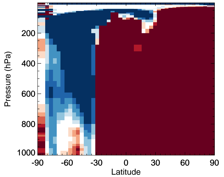
v11-02f-Run0 / v11-02e-Run1 ISN1 - Zonal mean % diff for Jan
