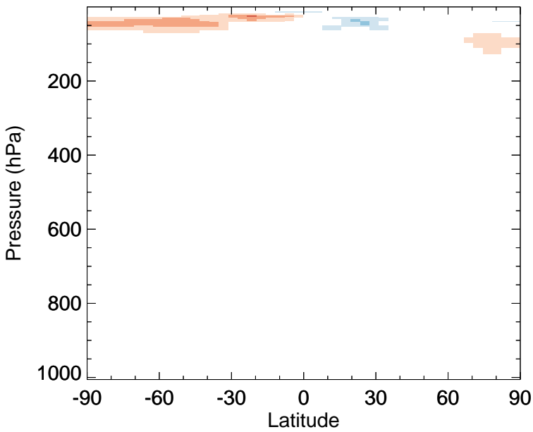
v11-02f-Run0 - v11-02e-Run0 CFC12 - Zonal mean abs diff for Jan
