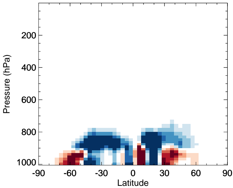
v11-02f-Run0 - v11-02e-Run0 SALC - Zonal mean abs diff for Jan
