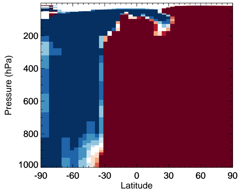
v11-02f-Run0 / v11-02e-Run1 HPALD - Zonal mean % diff for Jan
