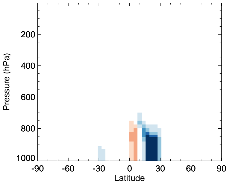
v11-02f-Run0 - v11-02e-Run0 DST2 - Zonal mean abs diff for Jan
