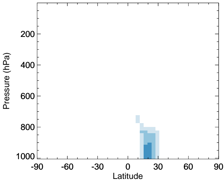
v11-02f-Run0 - v11-02e-Run0 DST1 - Zonal mean abs diff for Jan
