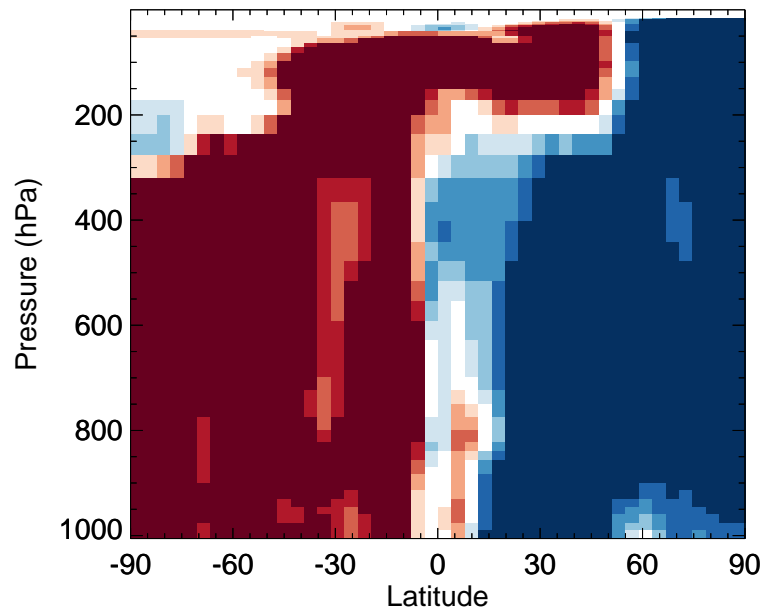
v11-02f-Run0 / v11-02e-Run0 ASOG1 - Zonal mean % diff for Jan
