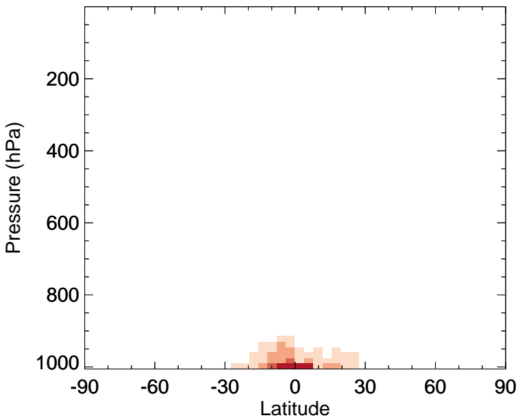
v11-02f-Run0 - v11-02e-Run0 RCHO - Zonal mean abs diff for Jan
