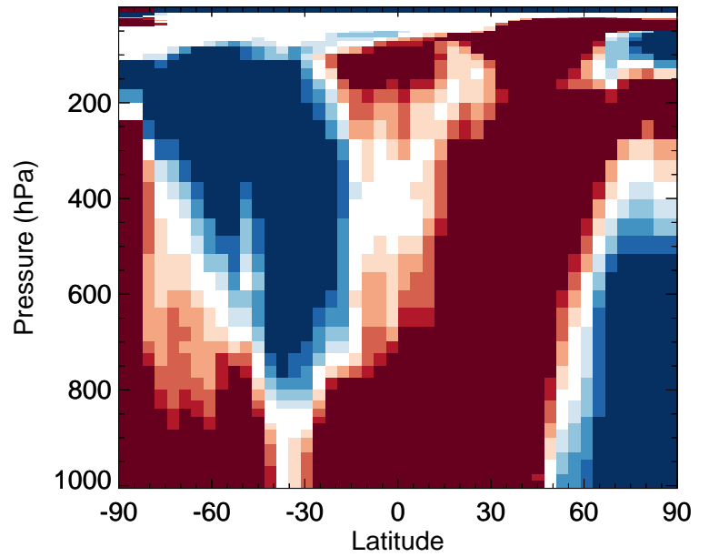
v11-02f-Run0 / v11-02e-Run1 NPMN - Zonal mean % diff for Jan
