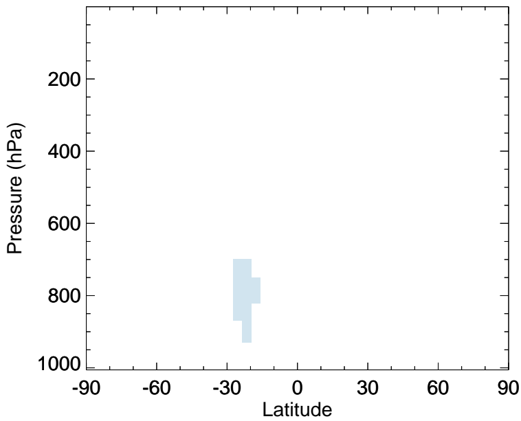
v11-02f-Run0 - v11-02e-Run0 IMAE - Zonal mean abs diff for Jan
