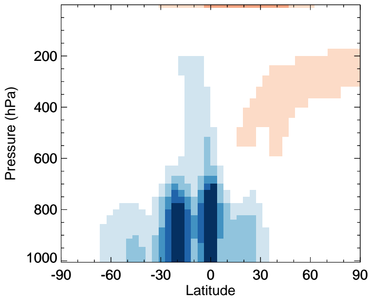
v11-02f-Run0 - v11-02e-Run1 MP - Zonal mean abs diff for Jan
