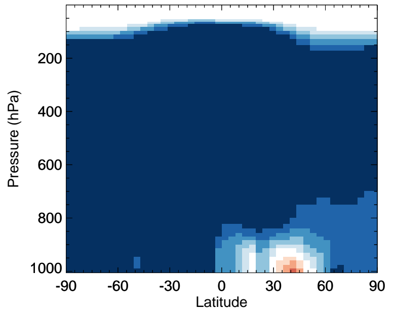
v11-02f-Run0 / v11-02e-Run1 ISO G 1 - Zonal mean % diff for Jan
