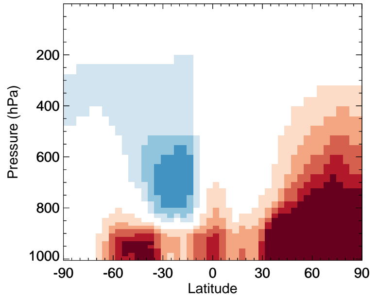
v11-02f-Run0 / v11-02e-Run1 SO4 - Zonal mean % diff for Jan
