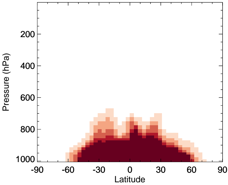
v11-02f-Run0 - v11-02e-Run0 NH3 - Zonal mean abs diff for Jan
