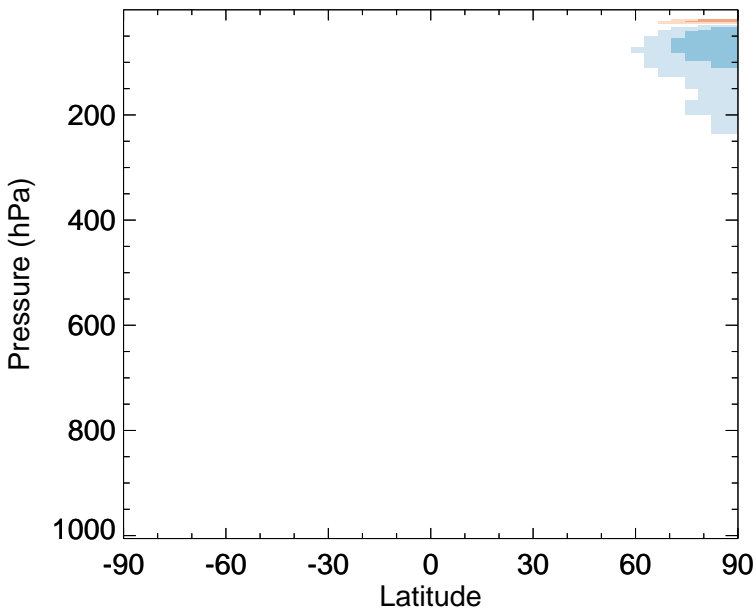
v11-02f-Run0 - v11-02e-Run0 HOBr - Zonal mean abs diff for Jan
