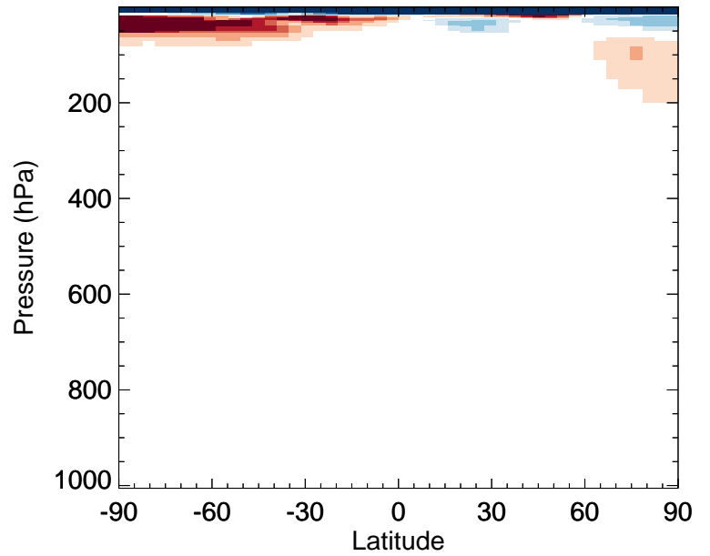
v11-02f-Run0 / v11-02e-Run0 CH3Cl - Zonal mean % diff for Jan
