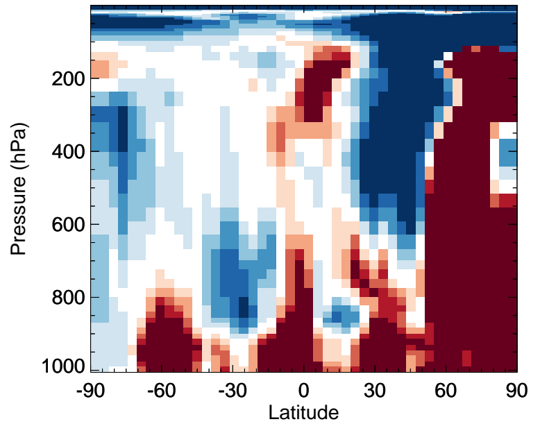
v11-02f-Run0 / v11-02e-Run0 HNO 2 - Zonal mean % diff for Jan
