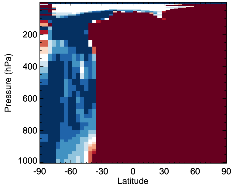
v11-02f-Run0 / v11-02e-Run1 RIPD - Zonal mean % diff for Jan
