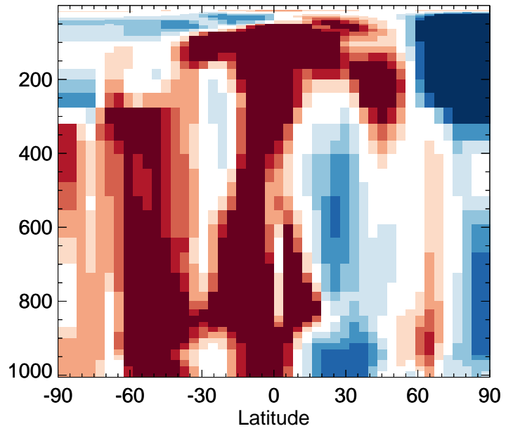
v11-02f-Run0 / v11-02e-Run0 ISO2 - Zonal mean % diff for Jan
