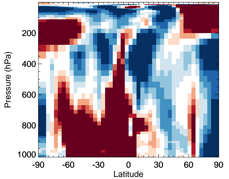
v11-02f-Run0 / v11-02e-Run0 ISOA2 - Zonal mean % diff for Jan
