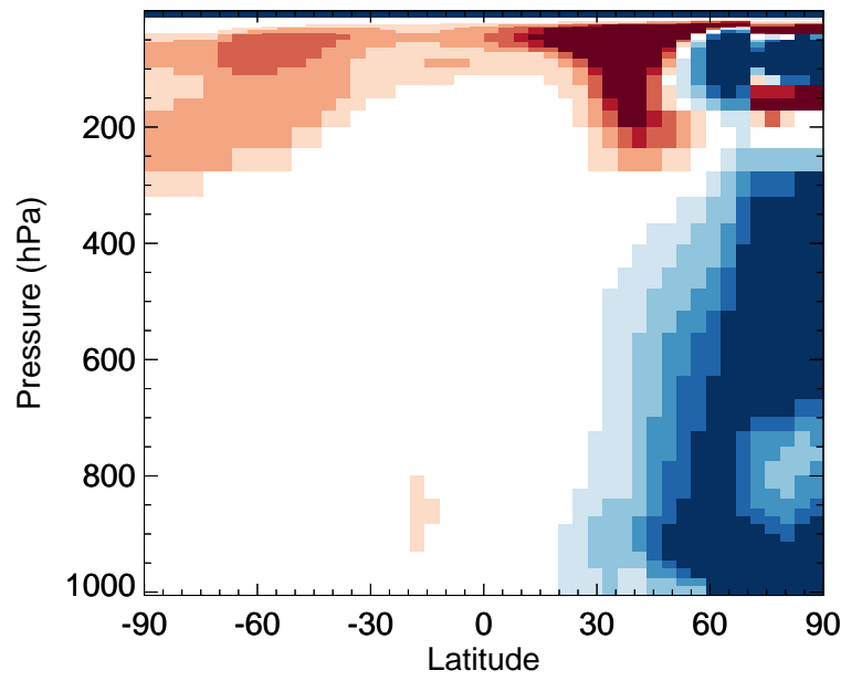
v11-02f-Run0 / v11-02e-Run1 HO2 - Zonal mean % diff for Jan
