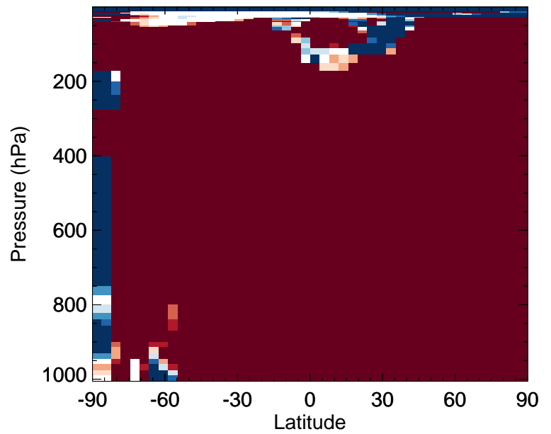
v11-02f-Run0 / v11-02e-Run0 LVOC - Zonal mean % diff for Jan
