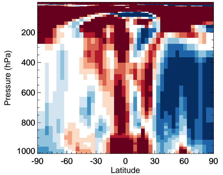
v11-02f-Run0 / v11-02e-Run0 MGLY - Zonal mean % diff for Jan
