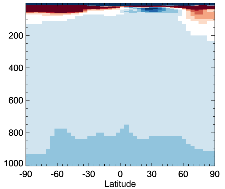
v11-02f-Run0 / v11-02e-Run0 CCI4 - Zonal mean % diff for Jan
