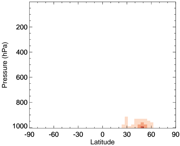
v11-02f-Run0 - v11-02e-Run0 SO4 - Zonal mean abs diff for Jan
