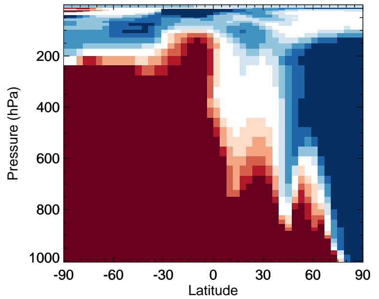
v11-02f-Run0 / v11-02e-Run1 HONIT - Zonal mean % diff for Jan
