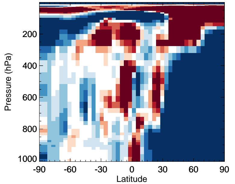
v11-02f-Run0 / v11-02e-Run0 HOCl - Zonal mean % diff for Jan
