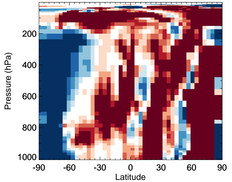
v11-02f-Run0 / v11-02e-Run0 HBr - Zonal mean % diff for Jan
