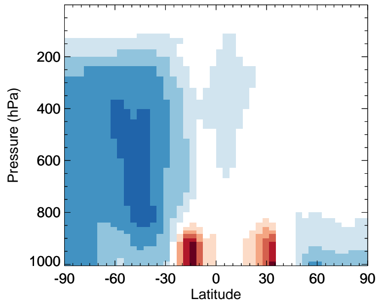
v11-02f-Run0 / v11-02e-Run1 SOAS - Zonal mean % diff for Jan
