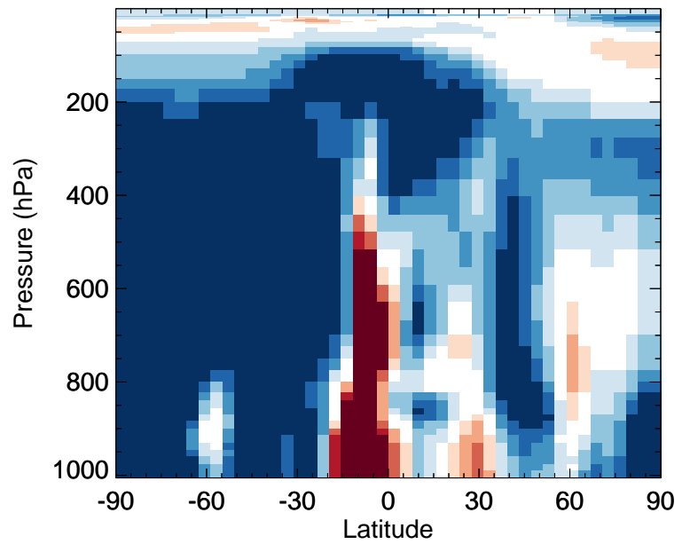
v11-02f-Run0 / v11-02e-Run0 SOAS - Zonal mean % diff for Jan
