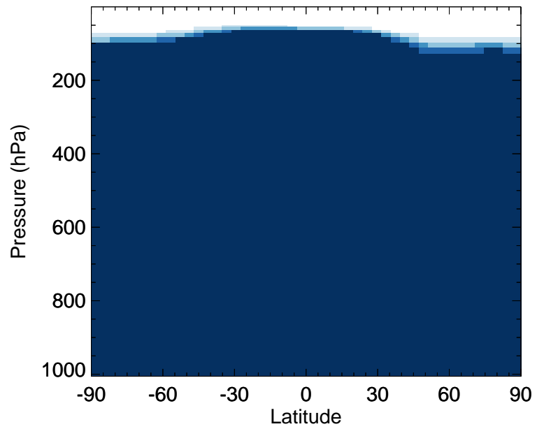
v11-02f-Run0 / v11-02e-Run1 SOAIE - Zonal mean % diff for Jan
