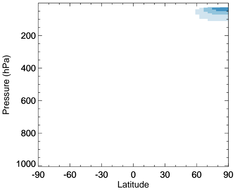
v11-02f-Run0 - v11-02e-Run1 HOBr - Zonal mean abs diff for Jan
