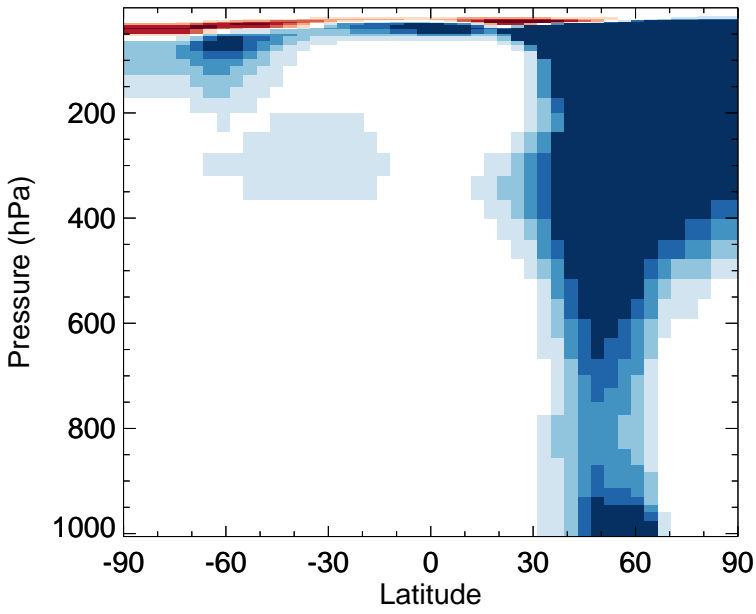
v11-02f-Run0 - v11-02e-Run1 HNO 4 - Zonal mean abs diff for Jan
