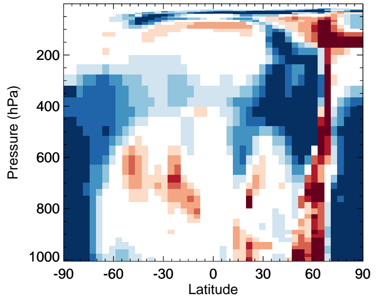
v11-02f-Run0 / v11-02e-Run1 HBr - Zonal mean % diff for Jan
