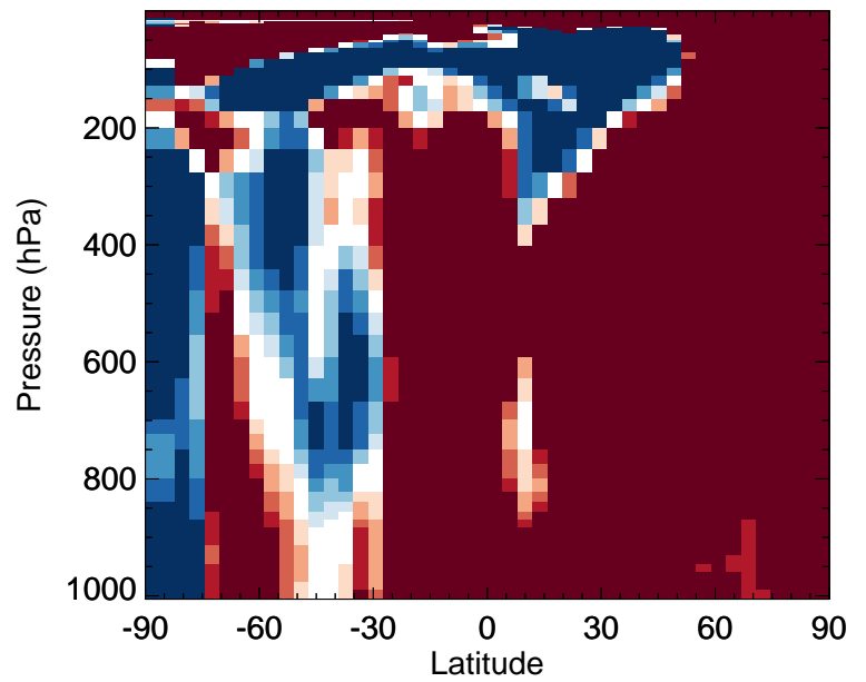
v11-02f-Run0 / v11-02e-Run0 MEK - Zonal mean % diff for Jan
