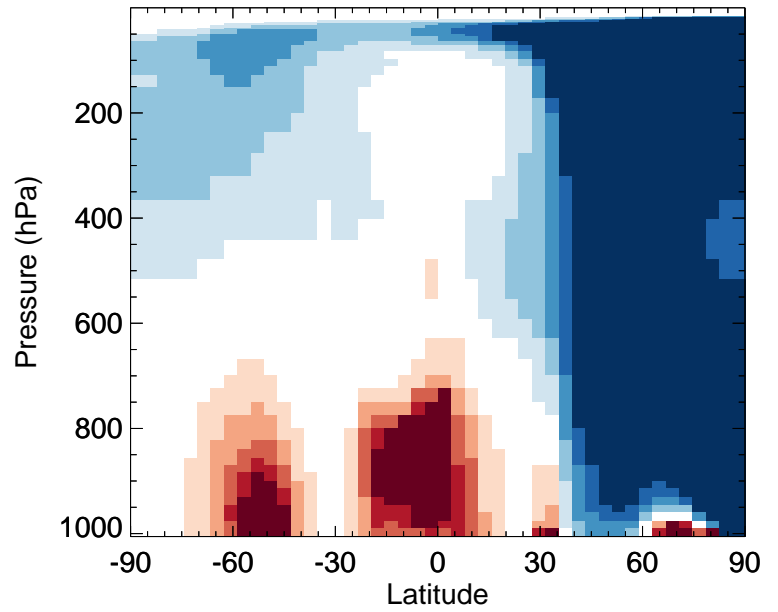
v11-02f-Run0 / v11-02e-Run1 NO 2 - Zonal mean % diff for Jan
