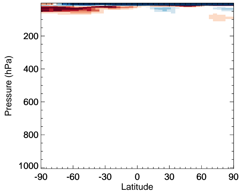
v11-02f-Run0 / v11-02e-Run0 CFC12 - Zonal mean % diff for Jan
