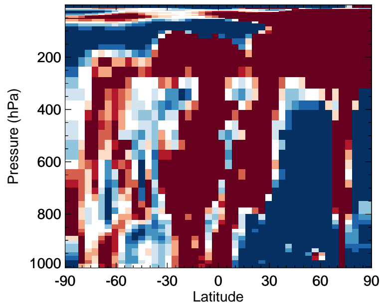
v11-02f-Run0 / v11-02e-Run0 Cl2O2 - Zonal mean % diff for Jan
