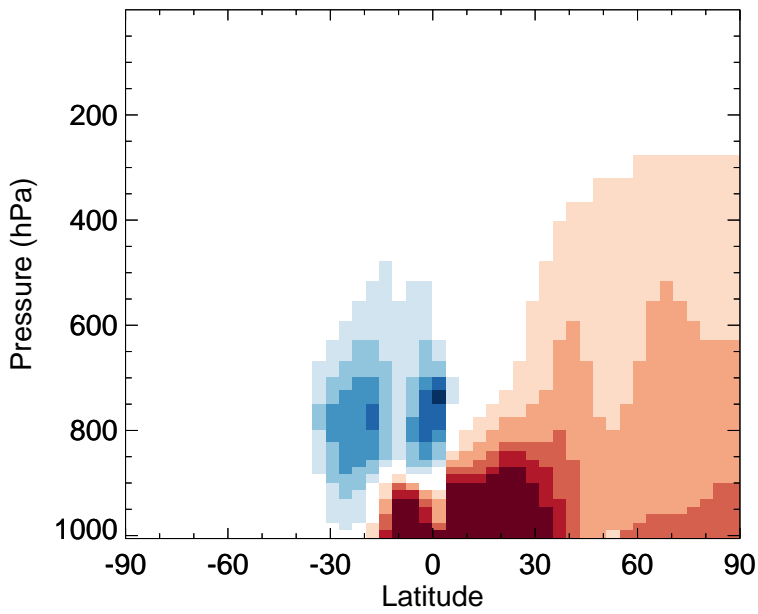
v11-02f-Run0 - v11-02e-Run1 MEK - Zonal mean abs diff for Jan
