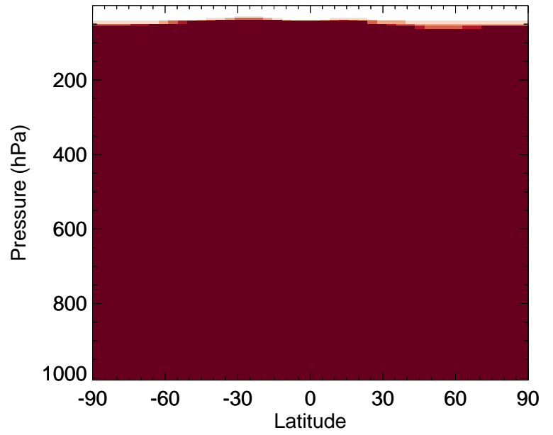
v11-02f-Run0 / v11-02e-Run1 NH3 - Zonal mean % diff for Jan
