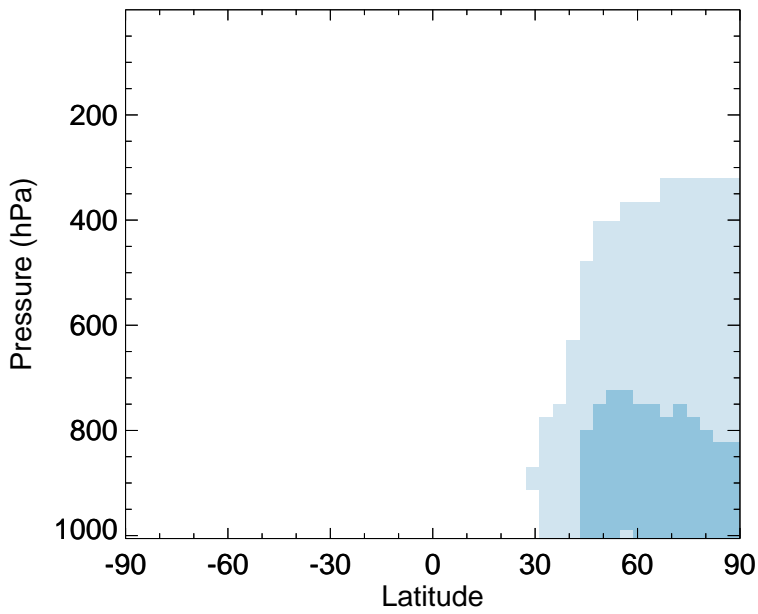
v11-02f-Run0 - v11-02e-Run1 PAN - Zonal mean abs diff for Jan
