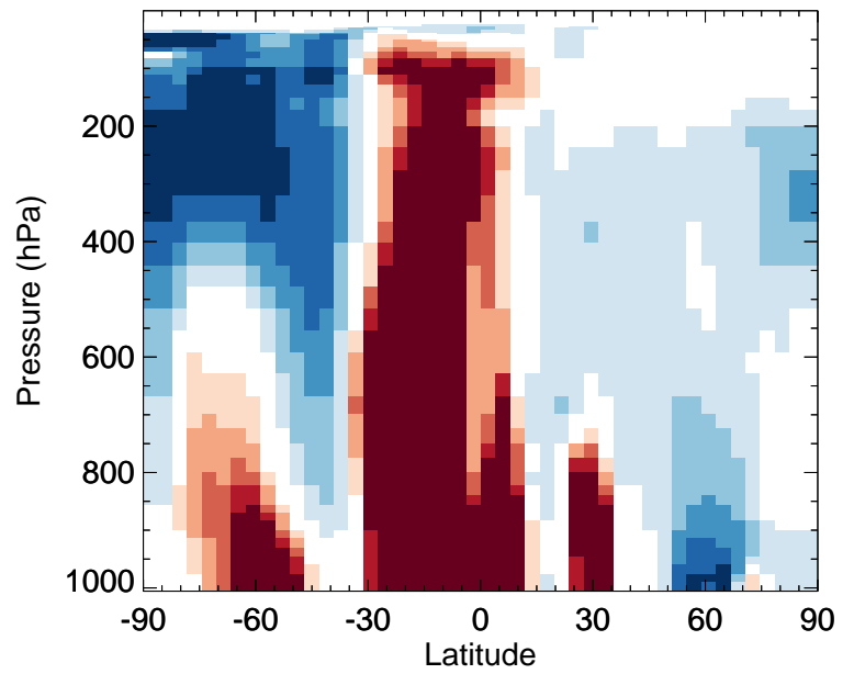
v11-02f-Run0 / v11-02e-Run1 SOAP - Zonal mean % diff for Jan
