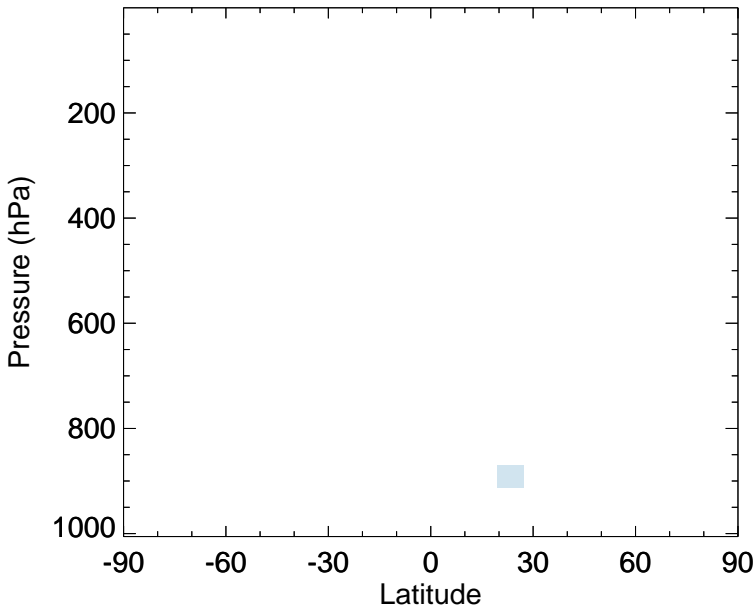
v11-02f-Run0 - v11-02e-Run0 SOAGX - Zonal mean abs diff for Jan
