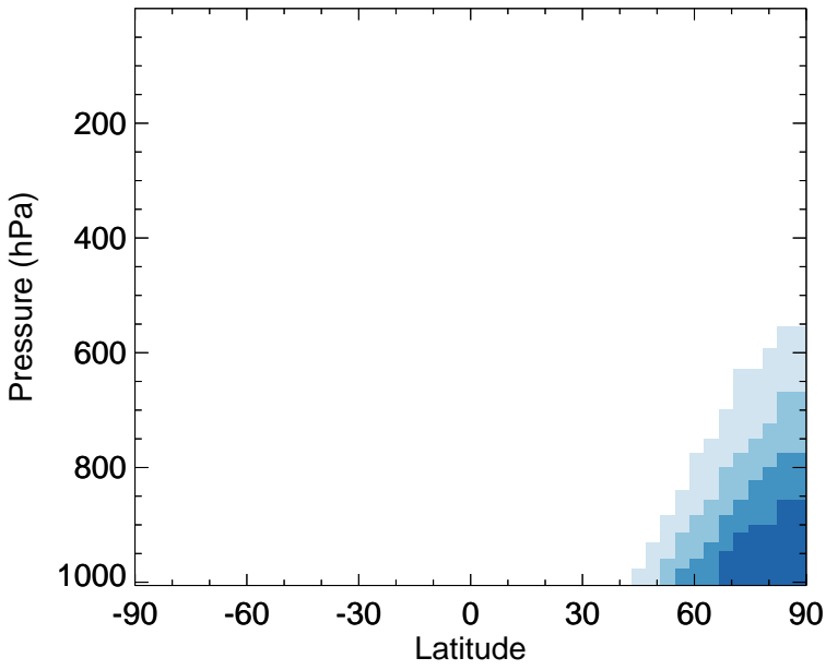
v11-02f-Run0 - v11-02e-Run1 CINO2 - Zonal mean abs diff for Jan
