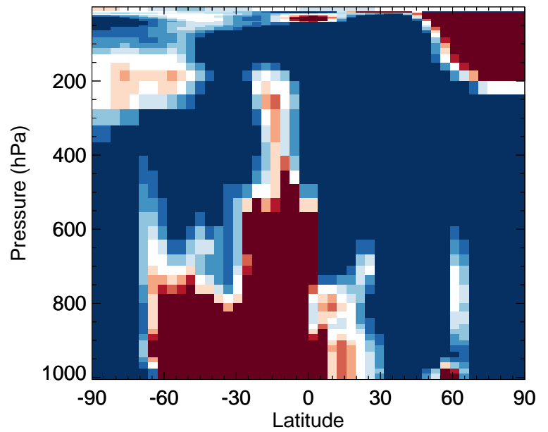
v11-02f-Run0 / v11-02e-Run0 ASOA2 - Zonal mean % diff for Jan
