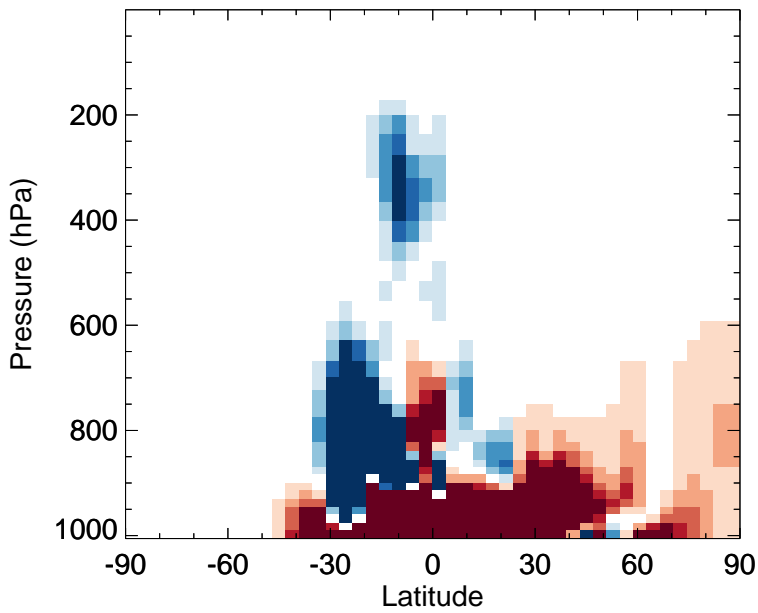
v11-02f-Run0 - v11-02e-Run0 PRPE - Zonal mean abs diff for Jan
