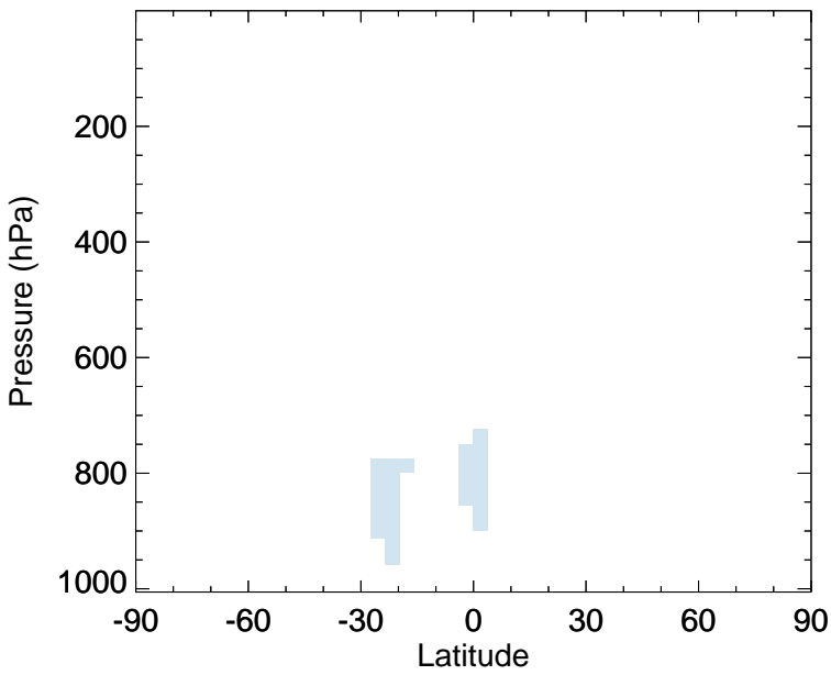
v11-02f-Run0 - v11-02e-Run1 IEPOXA - Zonal mean abs diff for Jan
