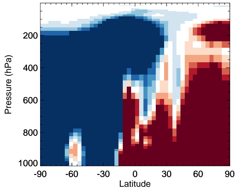
v11-02f-Run0 / v11-02e-Run0 SOAMG - Zonal mean % diff for Jan
