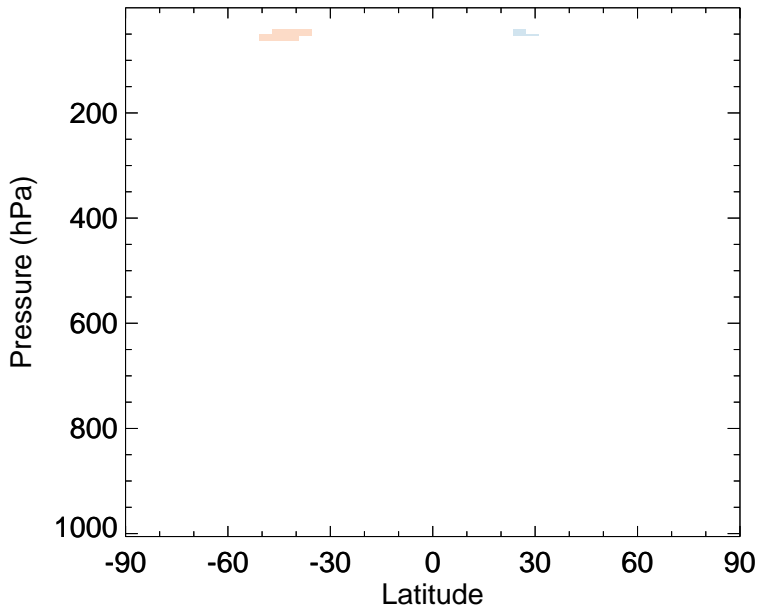
v11-02f-Run0 - v11-02e-Run0 CFC11 - Zonal mean abs diff for Jan
