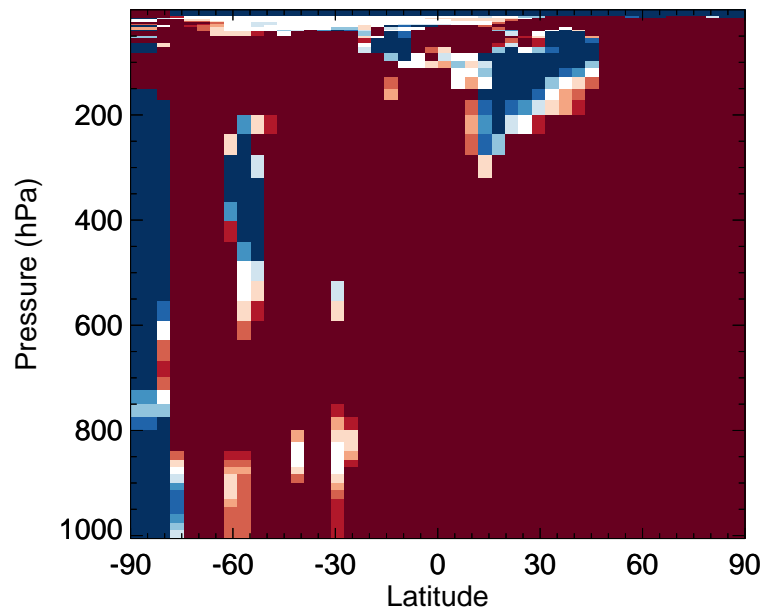
v11-02f-Run0 / v11-02e-Run0 IPMN - Zonal mean % diff for Jan
