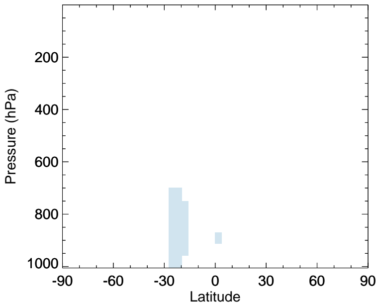
v11-02f-Run0 - v11-02e-Run0 RIPA - Zonal mean abs diff for Jan
