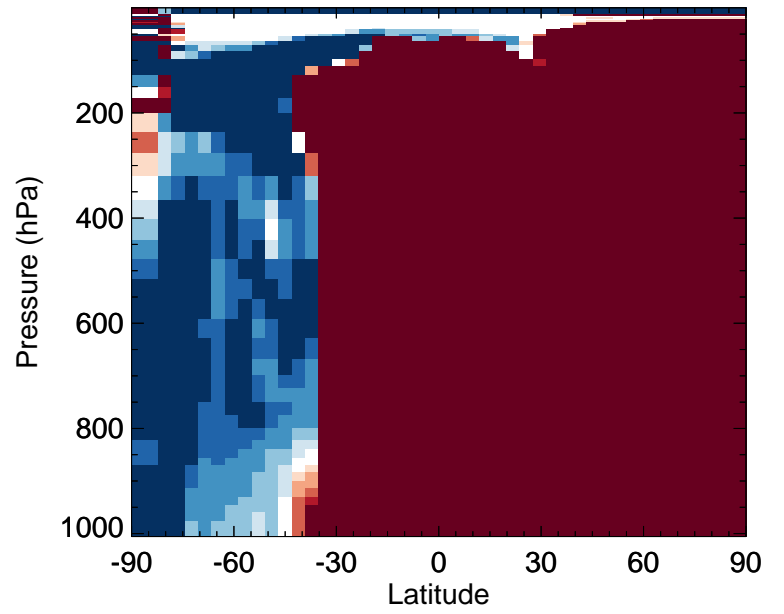
v11-02f-Run0 / v11-02e-Run1 RIPB - Zonal mean % diff for Jan
