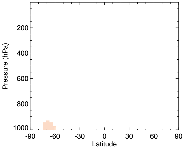
v11-02f-Run0 - v11-02e-Run0 DMS - Zonal mean abs diff for Jan
