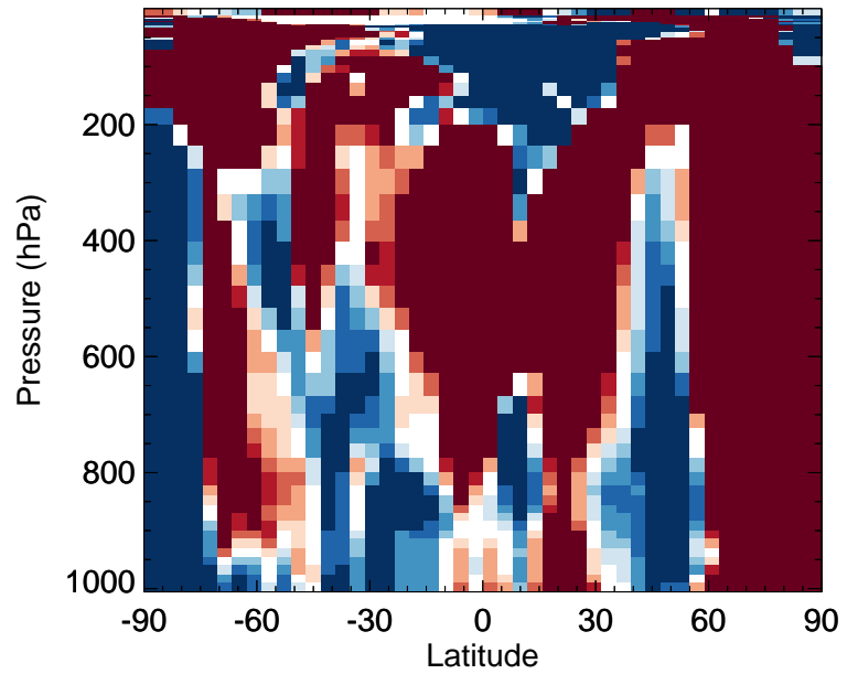
v11-02f-Run0 / v11-02e-Run0 BCPO - Zonal mean % diff for Jan
