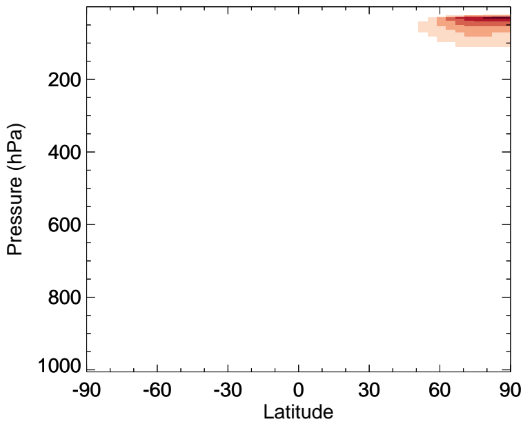
v11-02f-Run0 - v11-02e-Run1 OCIO - Zonal mean abs diff for Jan
