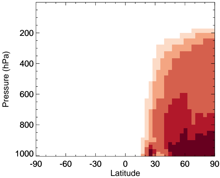
v11-02f-Run0 - v11-02e-Run0 C3H8 - Zonal mean abs diff for Jan
