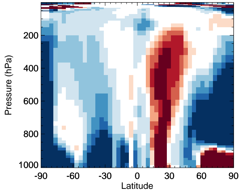
v11-02f-Run0 / v11-02e-Run1 BCPO - Zonal mean % diff for Jan
