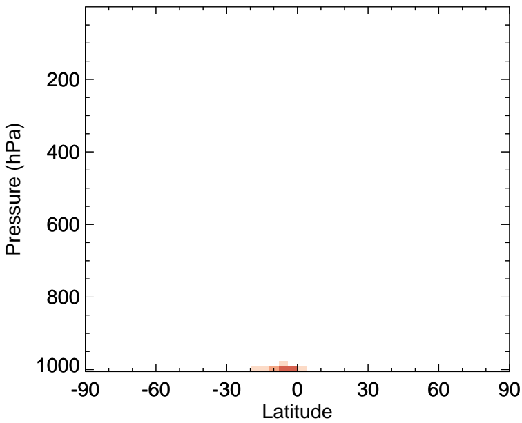
v11-02f-Run0 - v11-02e-Run0 MTPA - Zonal mean abs diff for Jan
