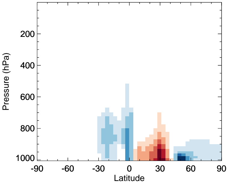
v11-02f-Run0 - v11-02e-Run1 EOH - Zonal mean abs diff for Jan
