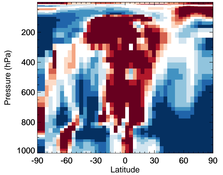
v11-02f-Run0 / v11-02e-Run0 BrCl - Zonal mean % diff for Jan
