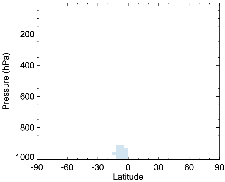
v11-02f-Run0 - v11-02e-Run1 MTPA - Zonal mean abs diff for Jan
