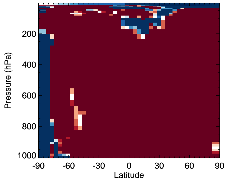
v11-02f-Run0 / v11-02e-Run0 ISN1OG - Zonal mean % diff for Jan
