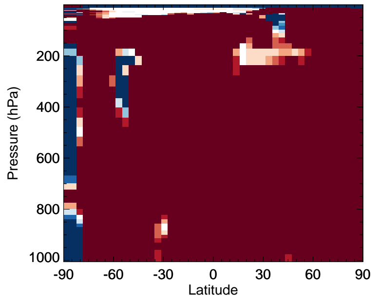
v11-02f-Run0 / v11-02e-Run0 PRPE - Zonal mean % diff for Jan
