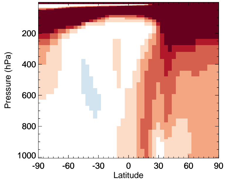
v11-02f-Run0 / v11-02e-Run1 MAP - Zonal mean % diff for Jan
