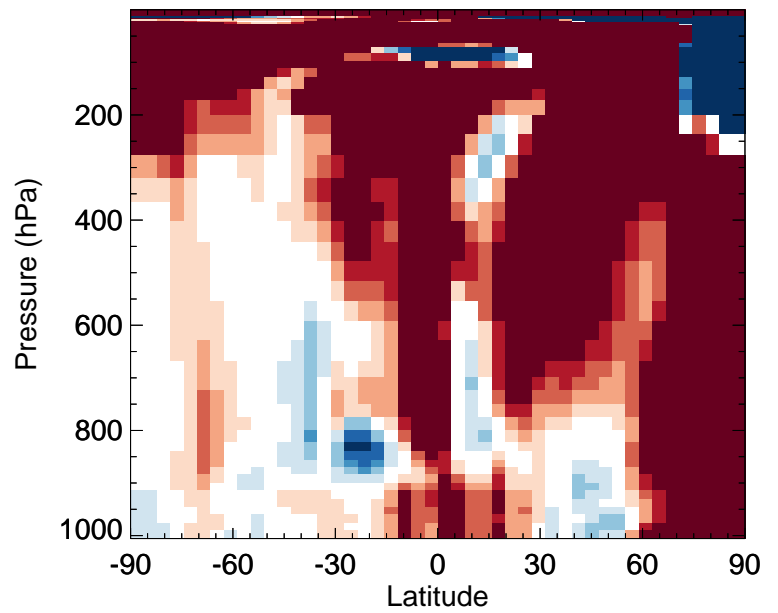
v11-02f-Run0 / v11-02e-Run0 ACTA - Zonal mean % diff for Jan
