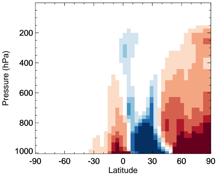
v11-02f-Run0 - v11-02e-Run0 BENZ - Zonal mean abs diff for Jan
