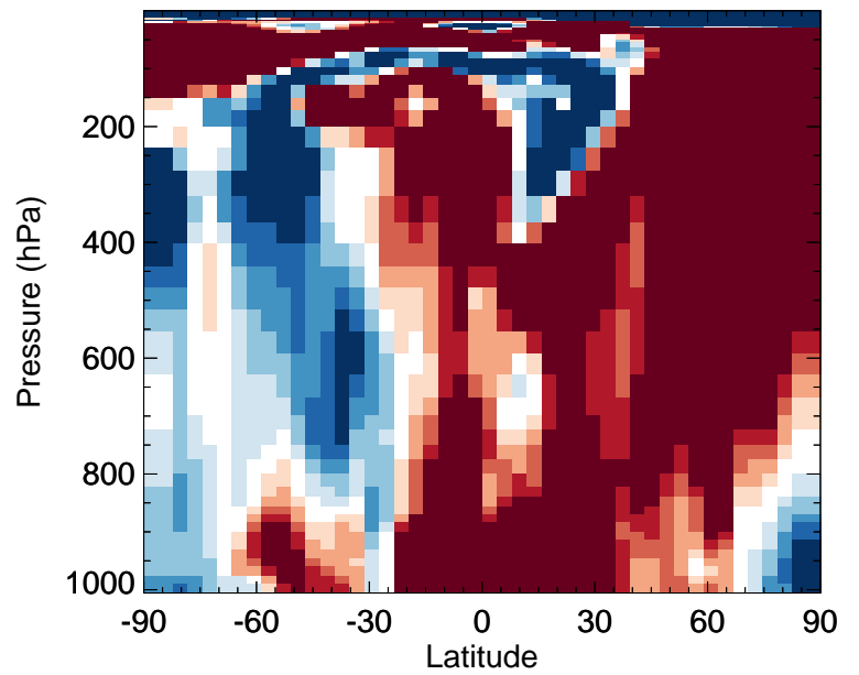
v11-02f-Run0 / v11-02e-Run0 HAC - Zonal mean % diff for Jan
