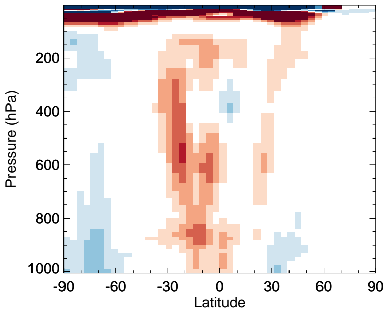
v11-02f-Run0 - v11-02e-Run0 HO2 - Zonal mean abs diff for Jan
