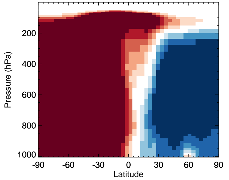
v11-02f-Run0 / v11-02e-Run1 ASOG3 - Zonal mean % diff for Jan
