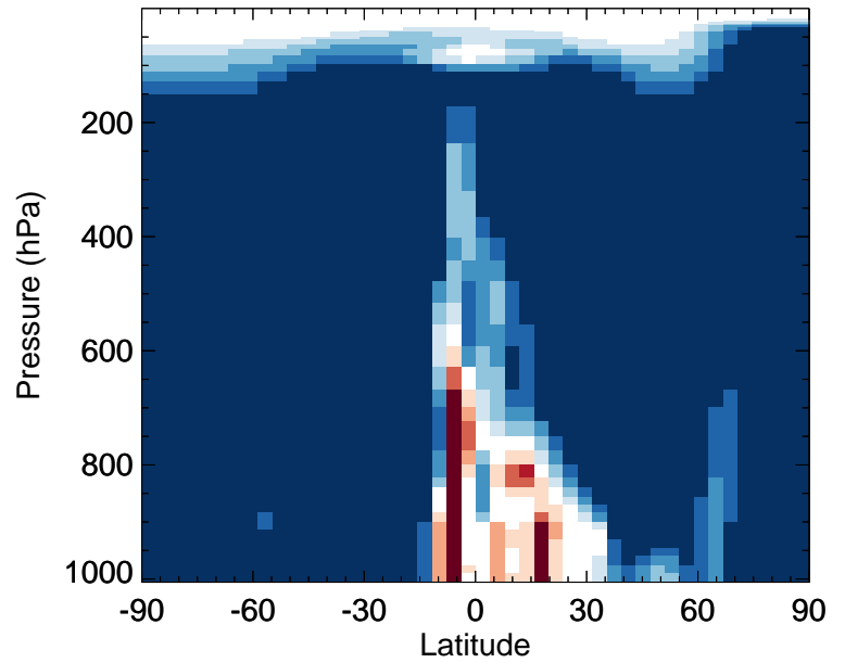
v11-02f-Run0 / v11-02e-Run0 ISO3 - Zonal mean % diff for Jan
