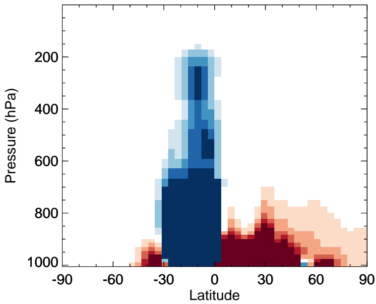
v11-02f-Run0 - v11-02e-Run1 PRPE - Zonal mean abs diff for Jan
