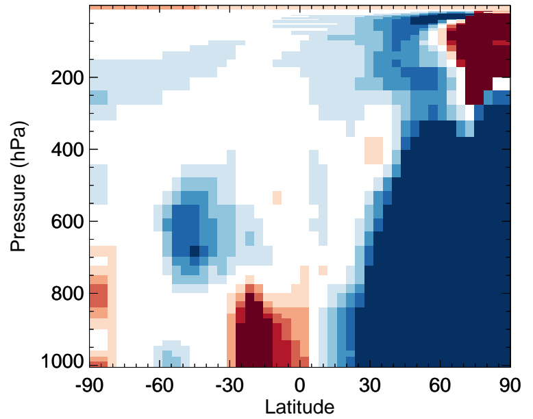
v11-02f-Run0 / v11-02e-Run1 C100 - Zonal mean % diff for Jan
