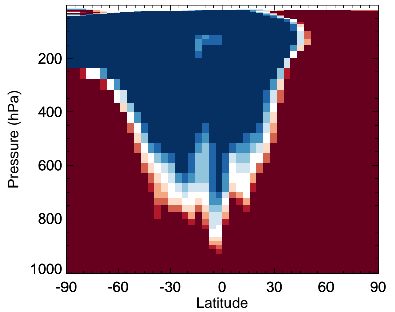
v11-02f-Run0 / v11-02e-Run1 HC187 - Zonal mean % diff for Jan
