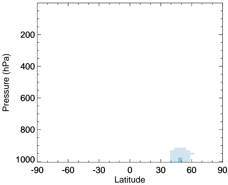
v11-02f-Run0 - v11-02e-Run1 SO 2 - Zonal mean abs diff for Jan
