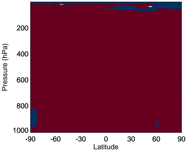
v11-02f-Run0 - v11-02e-Run0 CH4 - Zonal mean abs diff for Jan
