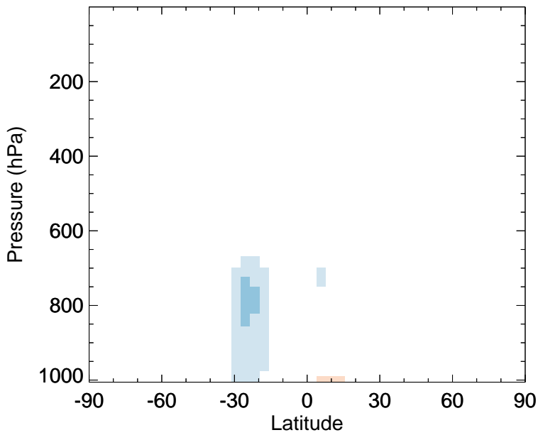
v11-02f-Run0 - v11-02e-Run0 HAC - Zonal mean abs diff for Jan
