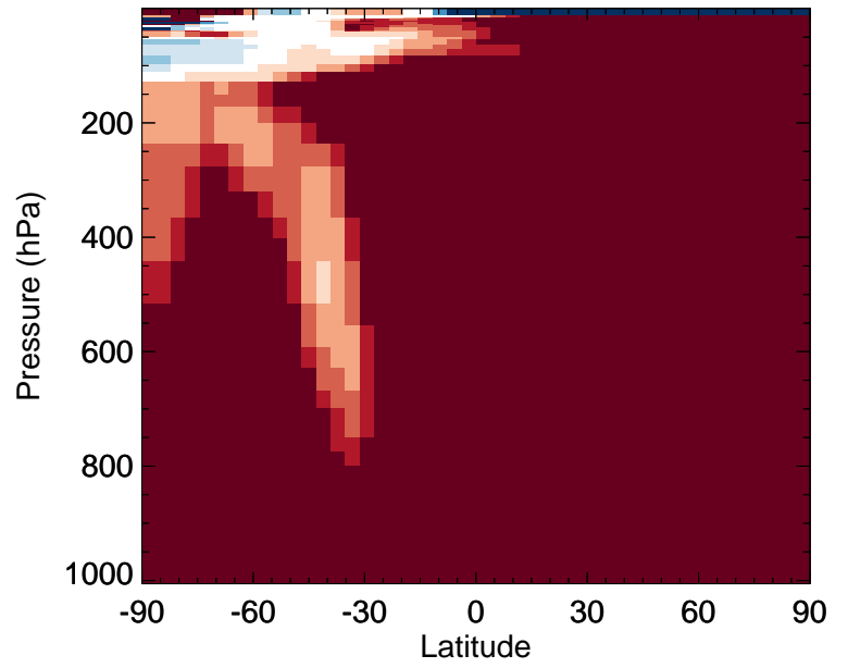
v11-02f-Run0 / v11-02e-Run1 ALK4 - Zonal mean % diff for Jan
