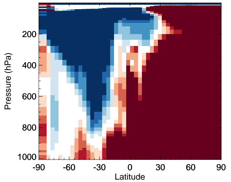
v11-02f-Run0 / v11-02e-Run1 IPMN - Zonal mean % diff for Jan
