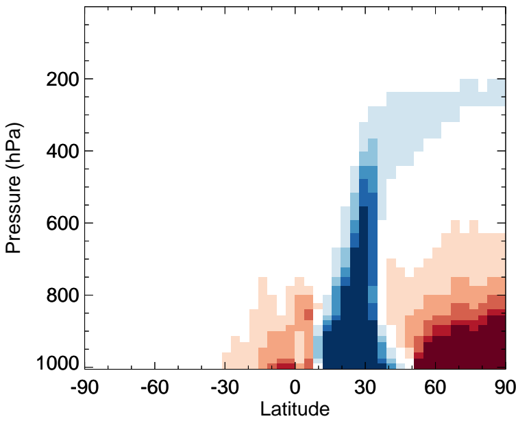
v11-02f-Run0 - v11-02e-Run1 BENZ - Zonal mean abs diff for Jan
