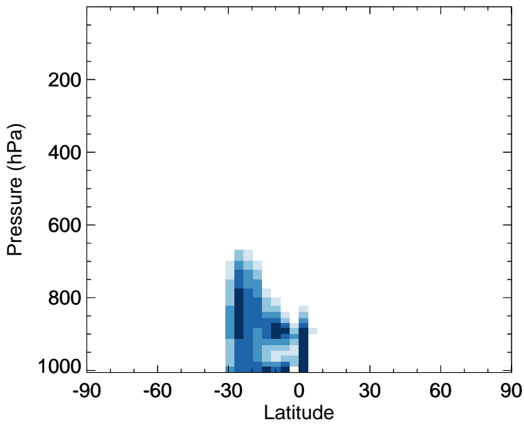
v11-02f-Run0 - v11-02e-Run0 ISOP - Zonal mean abs diff for Jan
