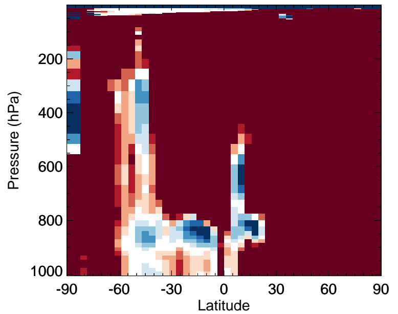
v11-02f-Run0 / v11-02e-Run0 DMS - Zonal mean % diff for Jan
