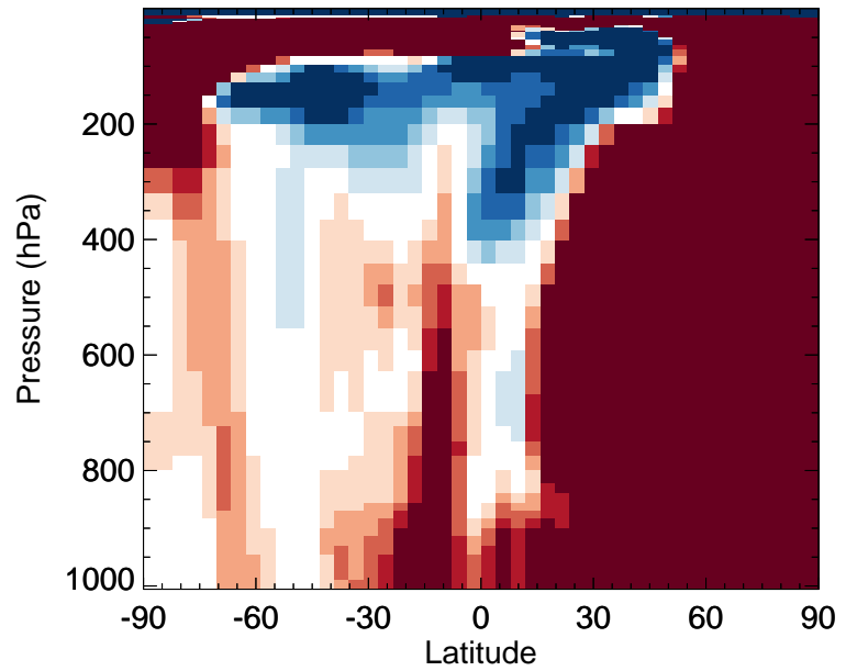
v11-02f-Run0 / v11-02e-Run0 C3H8 - Zonal mean % diff for Jan
