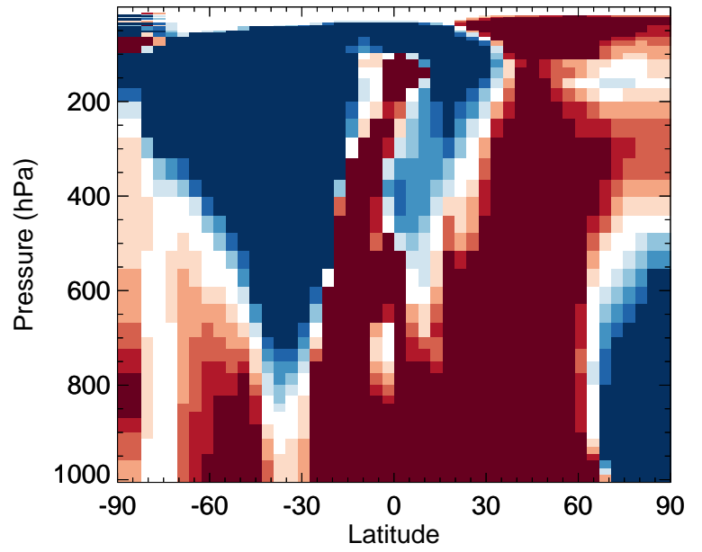
v11-02f-Run0 / v11-02e-Run1 MVKN - Zonal mean % diff for Jan
