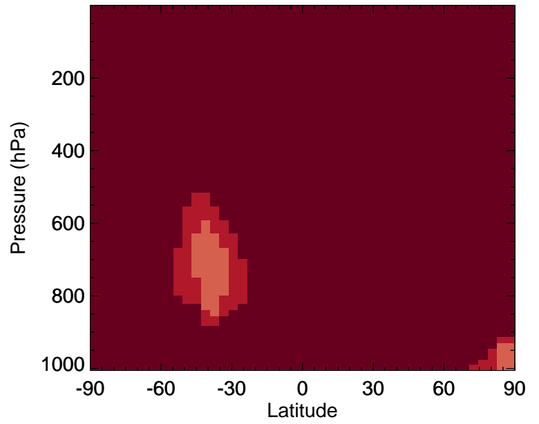
v11-02f-Run0 / v11-02e-Run1 INDIOL - Zonal mean % diff for Jan
