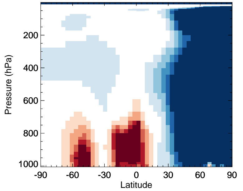
v11-02f-Run0 / v11-02e-Run1 HNO 4 - Zonal mean % diff for Jan
