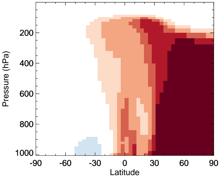
v11-02f-Run0 - v11-02e-Run1 C2H6 - Zonal mean abs diff for Jul
