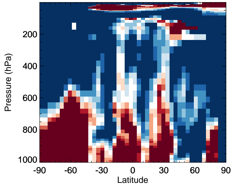
v11-02f-Run0 / v11-02e-Run0 CINO2 - Zonal mean % diff for Jul
