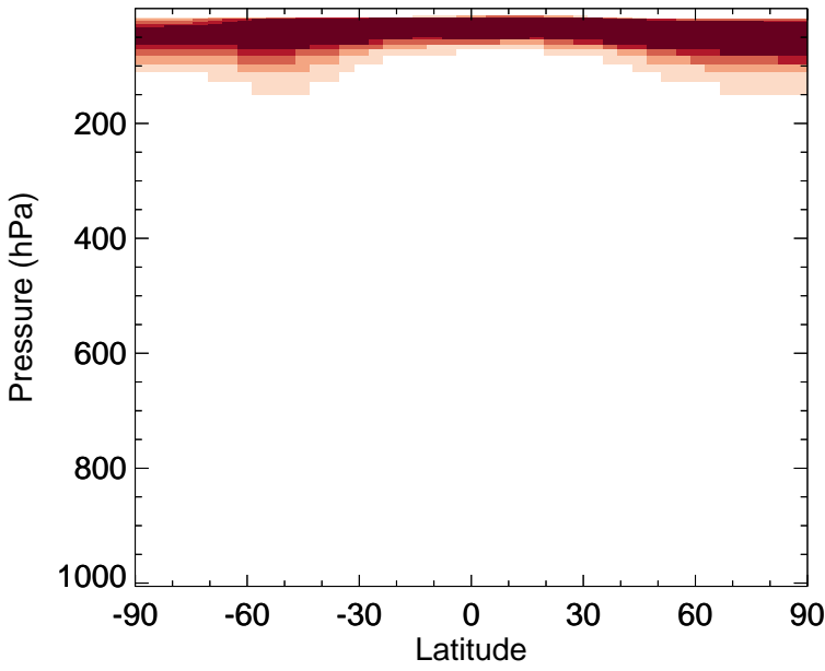
v11-02f-Run0 - v11-02e-Run1 N2O - Zonal mean abs diff for Jul
