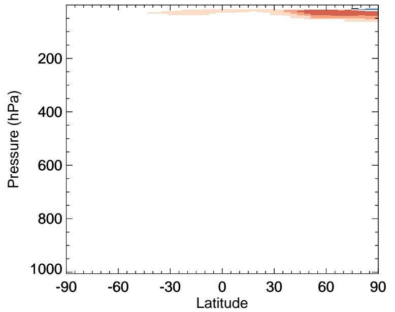
v11-02f-Run0 / v11-02e-Run1 CHBr3 - Zonal mean % diff for Jul
