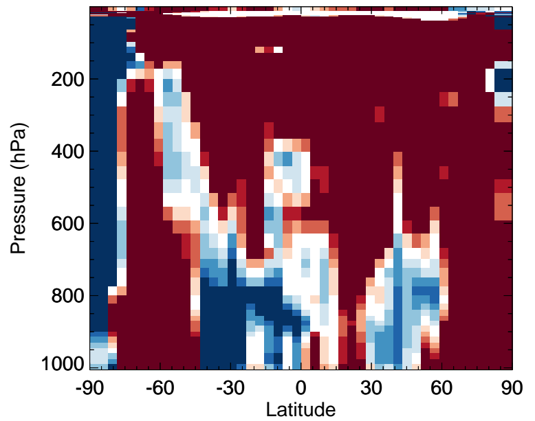
v11-02f-Run0 / v11-02e-Run0 BCPO - Zonal mean % diff for Jul
