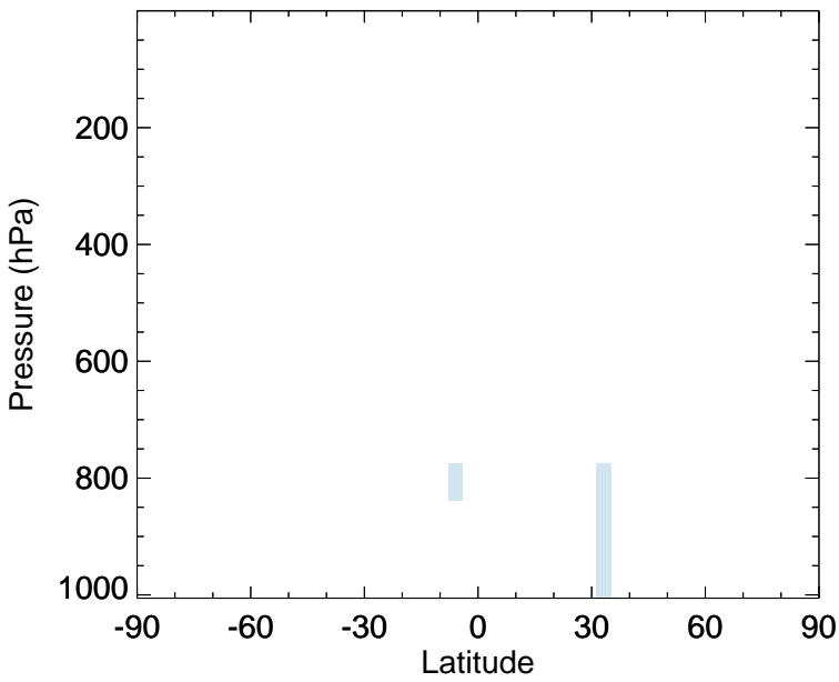
v11-02f-Run0 - v11-02e-Run1 IEPOXA - Zonal mean abs diff for Jul
