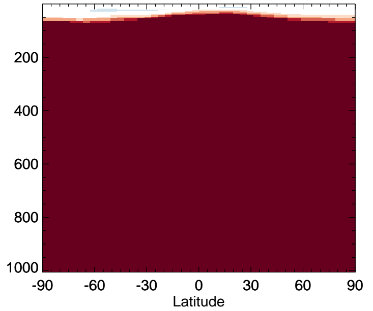
v11-02f-Run0 / v11-02e-Run0 NH4 - Zonal mean % diff for Jul
