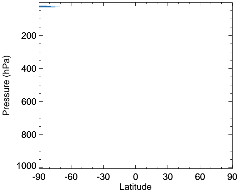
v11-02f-Run0 - v11-02e-Run0 CINO2 - Zonal mean abs diff for Jul
