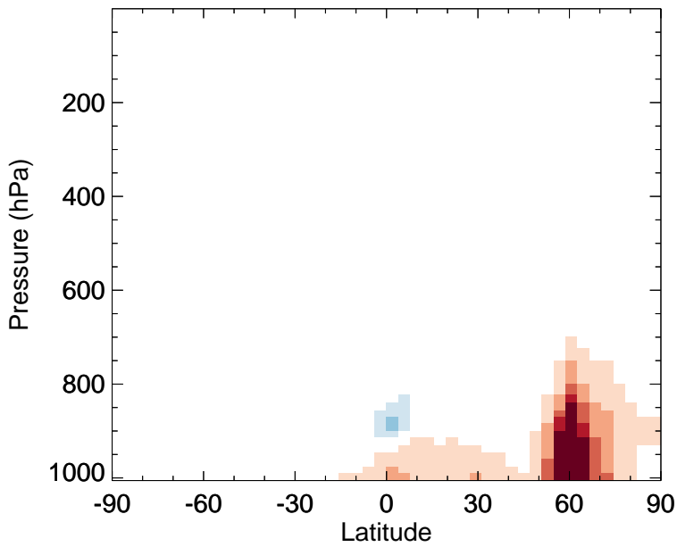
v11-02f-Run0 - v11-02e-Run0 ALD2 - Zonal mean abs diff for Jul
