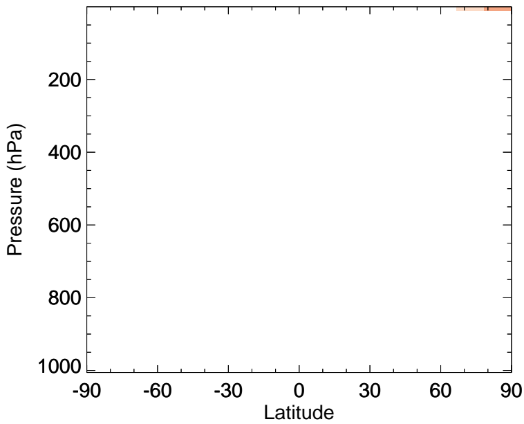
v11-02f-Run0 - v11-02e-Run0 ACTA - Zonal mean abs diff for Jul
