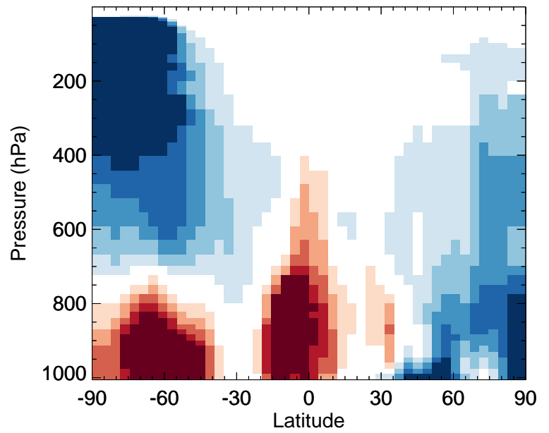
v11-02f-Run0 / v11-02e-Run1 NO 3 - Zonal mean % diff for Jul
