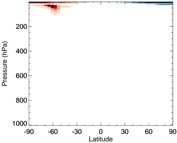
v11-02f-Run0 - v11-02e-Run0 ClO - Zonal mean abs diff for Jul
