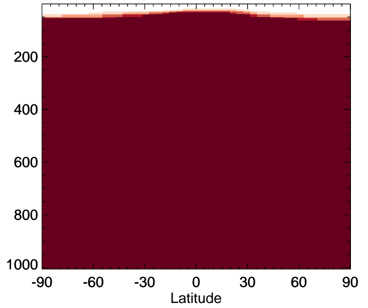
v11-02f-Run0 / v11-02e-Run1 NH4 - Zonal mean % diff for Jul
