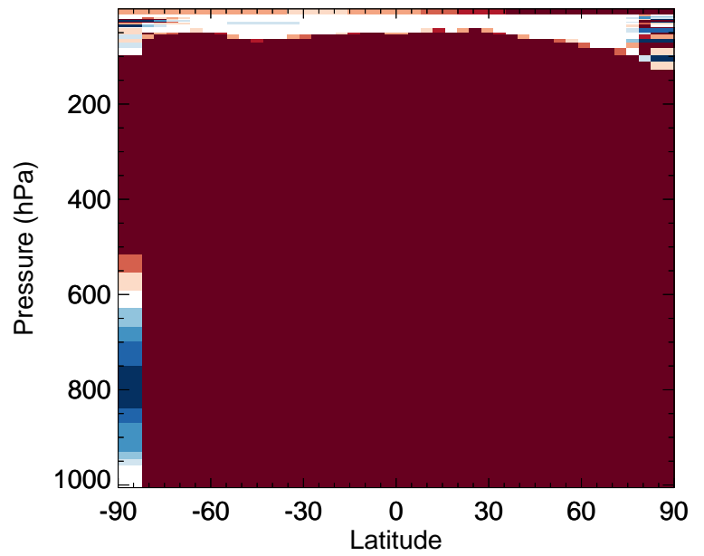
v11-02f-Run0 / v11-02e-Run1 MTPA - Zonal mean % diff for Jul
