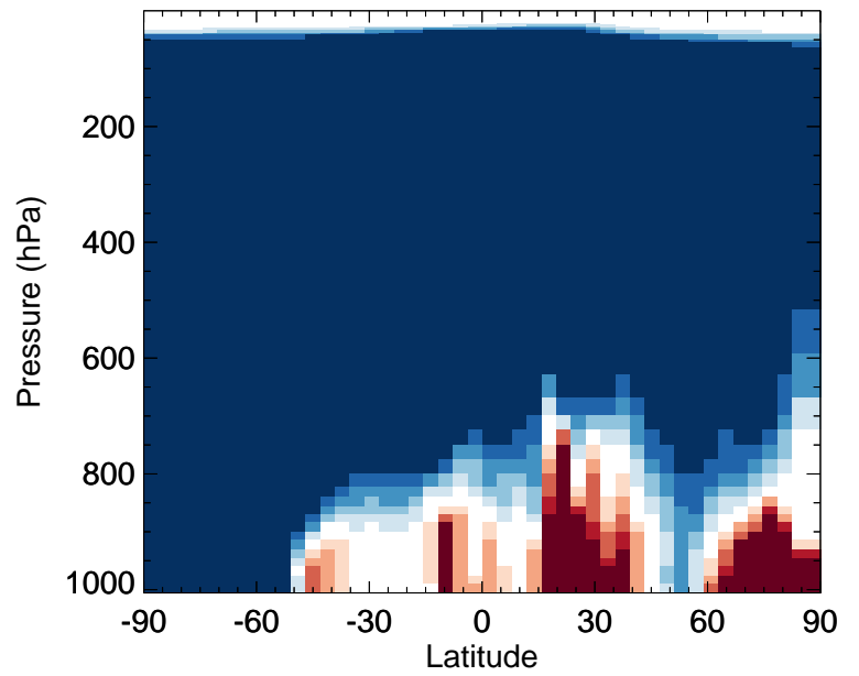
v11-02f-Run0 / v11-02e-Run1 DHDN - Zonal mean % diff for Jul
