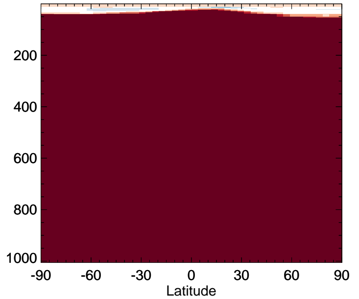
v11-02f-Run0 / v11-02e-Run0 NH3 - Zonal mean % diff for Jul
