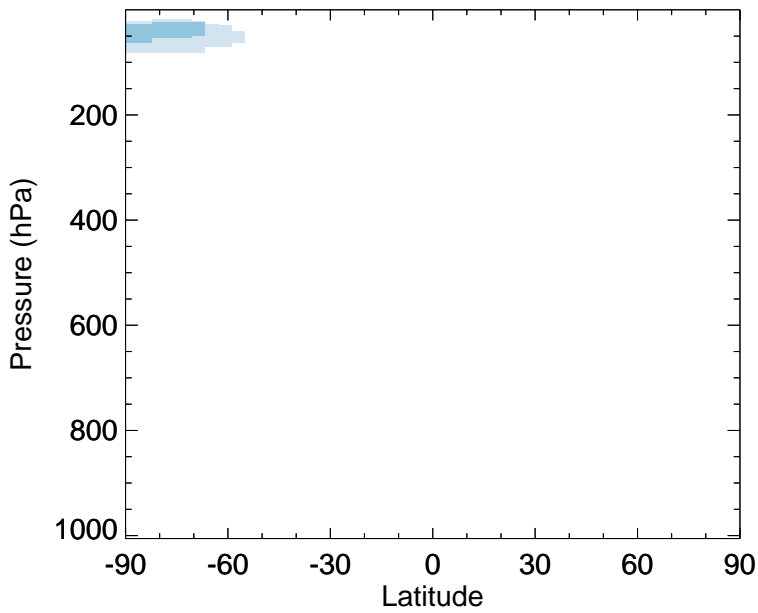
v11-02f-Run0 - v11-02e-Run0 HOBr - Zonal mean abs diff for Jul
