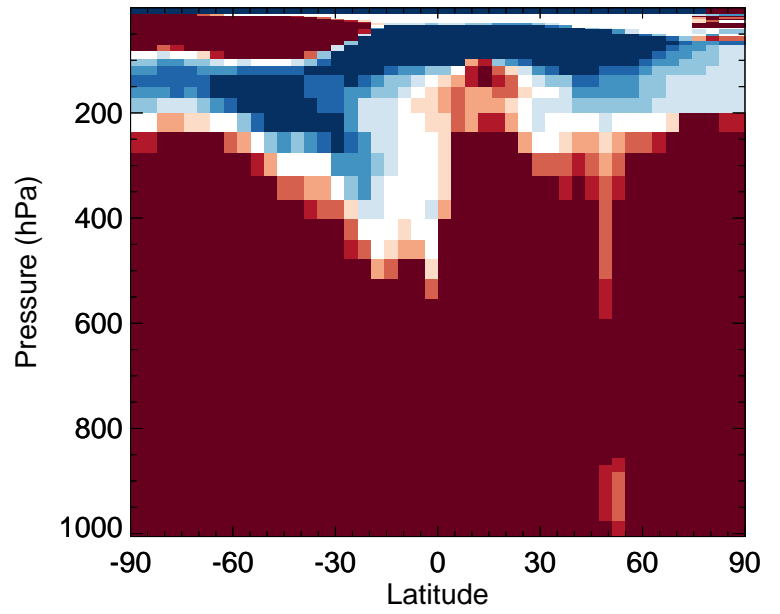
v11-02f-Run0 / v11-02e-Run1 IPMN - Zonal mean % diff for Jul
