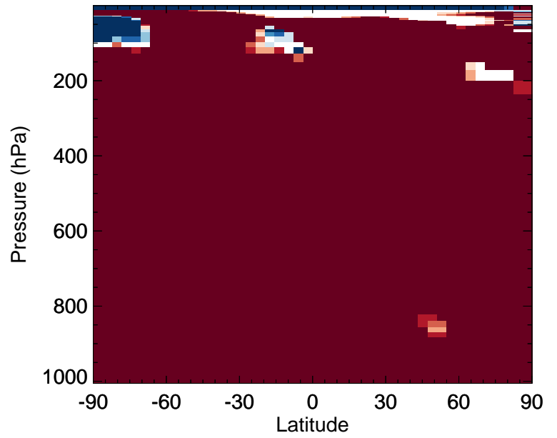
v11-02f-Run0 / v11-02e-Run0 IPMN - Zonal mean % diff for Jul
