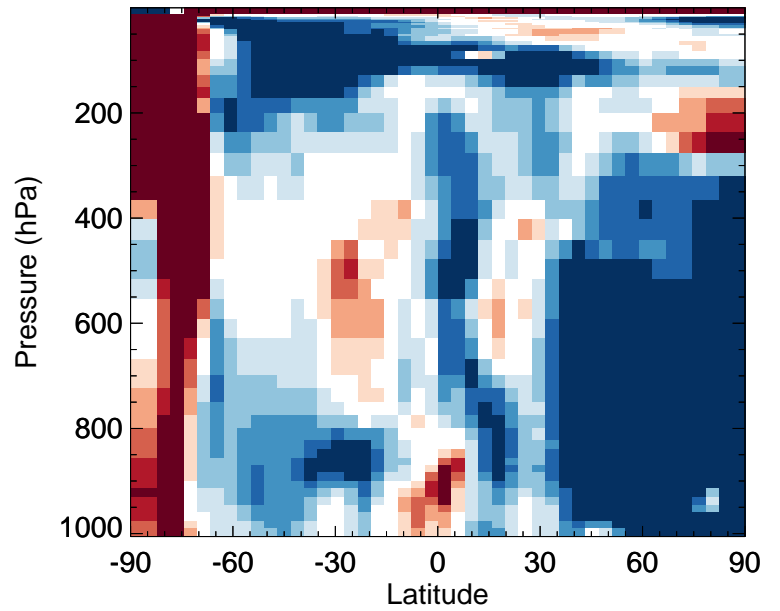
v11-02f-Run0 / v11-02e-Run0 Cl - Zonal mean % diff for Jul
