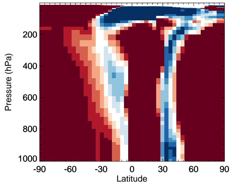
v11-02f-Run0 / v11-02e-Run1 TOLU - Zonal mean % diff for Jul
