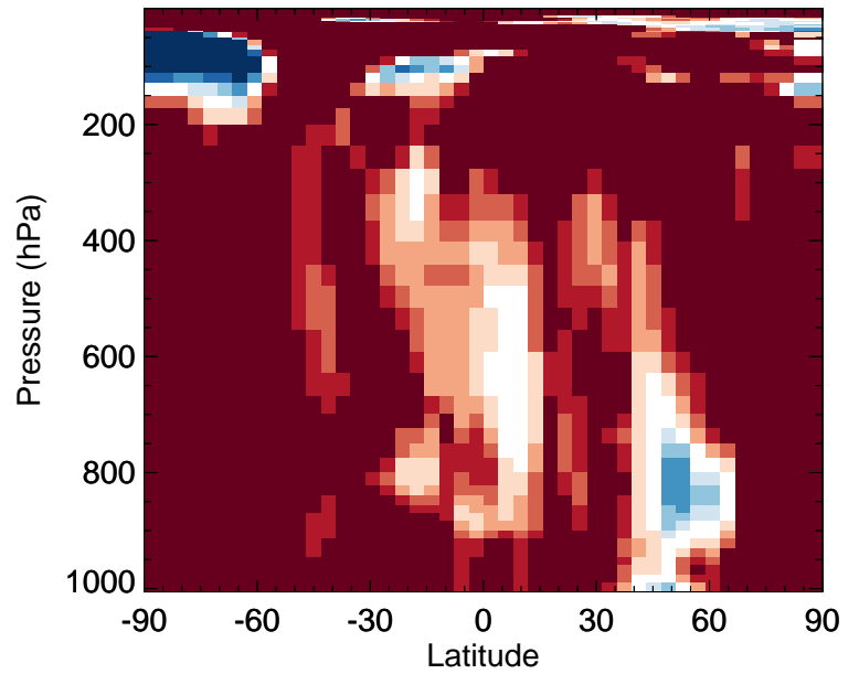
v11-02f-Run0 / v11-02e-Run0 MGLY - Zonal mean % diff for Jul
