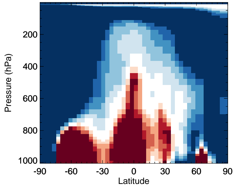
v11-02f-Run0 / v11-02e-Run1 N2O5 - Zonal mean % diff for Jul
