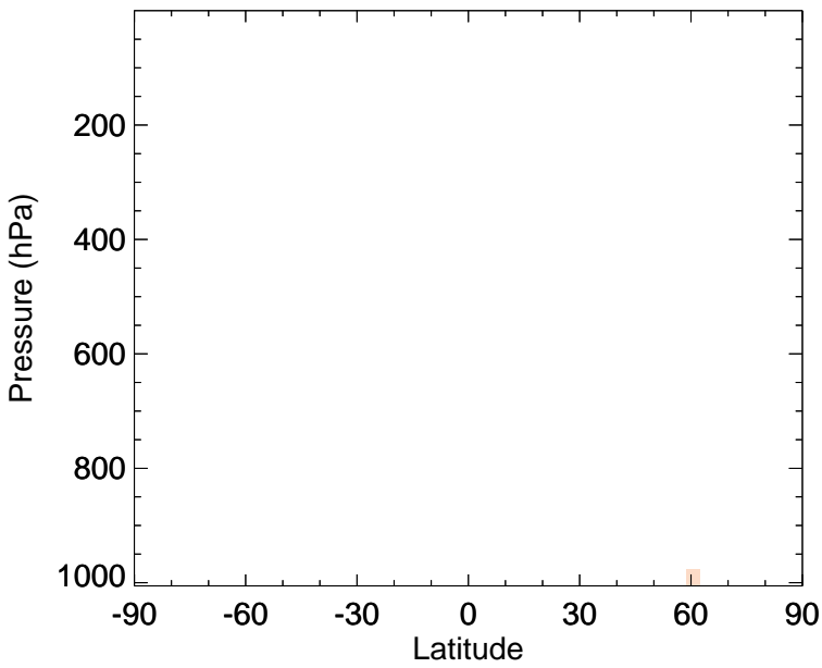
v11-02f-Run0 - v11-02e-Run1 SOAP - Zonal mean abs diff for Jul
