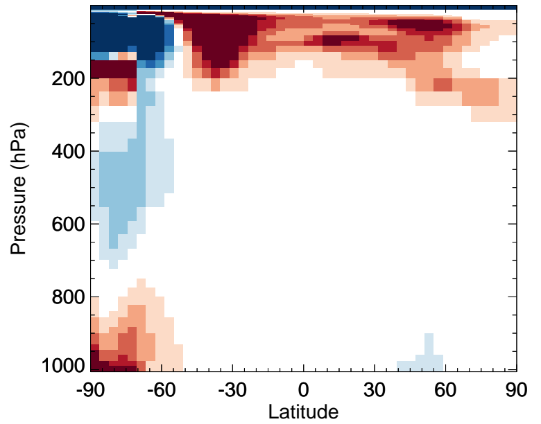
v11-02f-Run0 / v11-02e-Run1 HO2 - Zonal mean % diff for Jul
