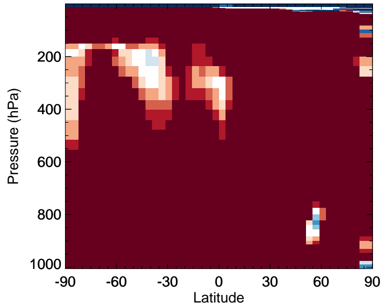
v11-02f-Run0 / v11-02e-Run0 HONIT - Zonal mean % diff for Jul
