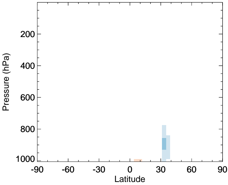
v11-02f-Run0 - v11-02e-Run1 HAC - Zonal mean abs diff for Jul
