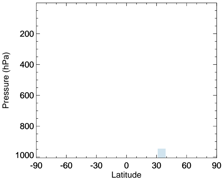
v11-02f-Run0 - v11-02e-Run1 SOAGX - Zonal mean abs diff for Jul
