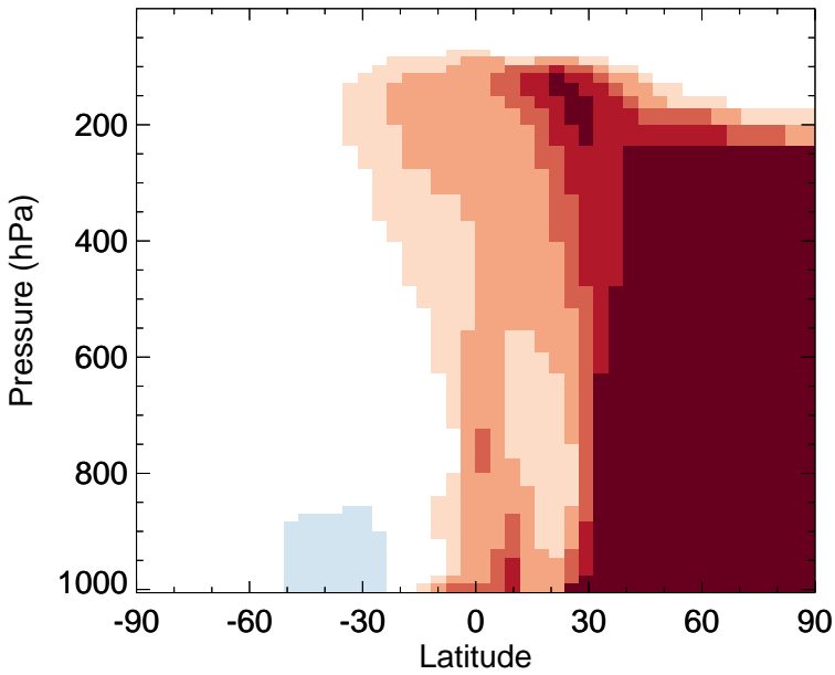
v11-02f-Run0 - v11-02e-Run0 C2H6 - Zonal mean abs diff for Jul
