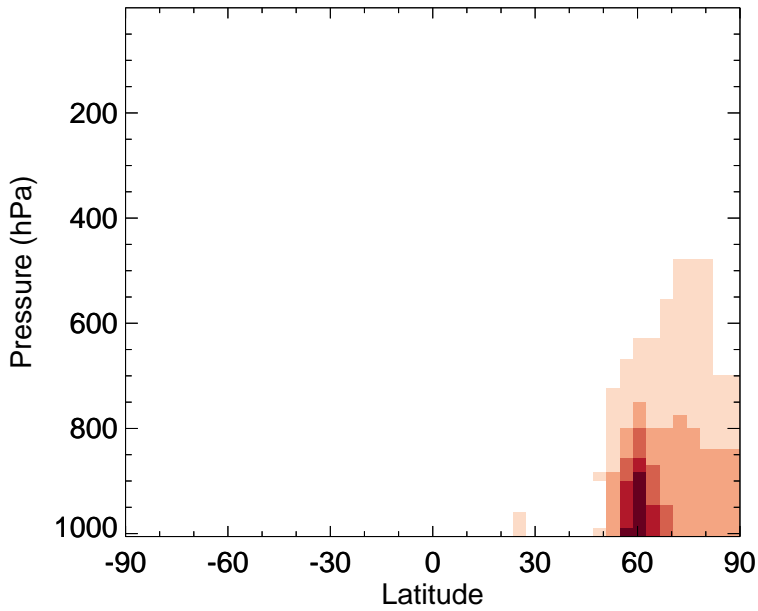
v11-02f-Run0 - v11-02e-Run0 C3H8 - Zonal mean abs diff for Jul
