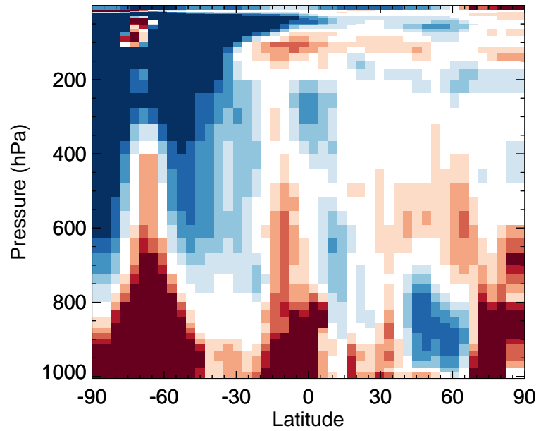
v11-02f-Run0 / v11-02e-Run0 NO 2 - Zonal mean % diff for Jul
