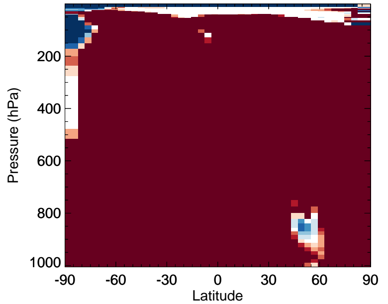
v11-02f-Run0 / v11-02e-Run0 ISN1 - Zonal mean % diff for Jul
