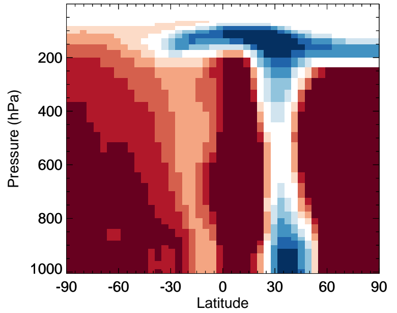
v11-02f-Run0 / v11-02e-Run1 ASOAN - Zonal mean % diff for Jul
