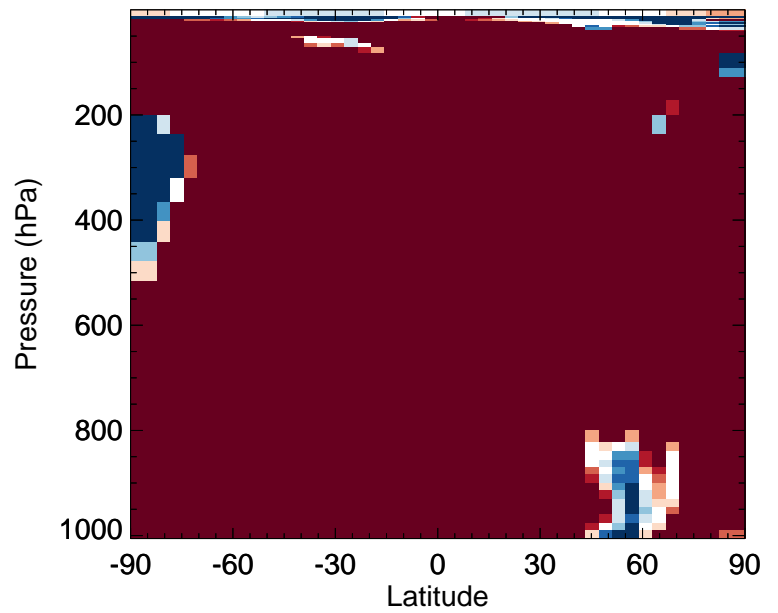
v11-02f-Run0 / v11-02e-Run0 ISN1OG - Zonal mean % diff for Jul
