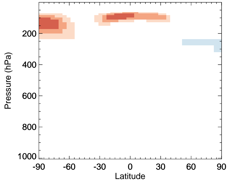
v11-02f-Run0 / v11-02e-Run1 ISOG2 - Zonal mean % diff for Jul
