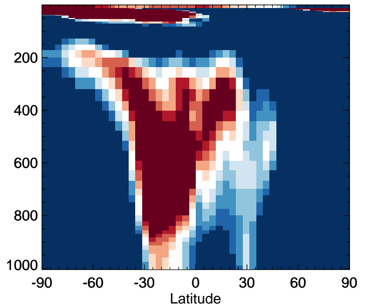
v11-02f-Run0 / v11-02e-Run0 DST1 - Zonal mean % diff for Jul
