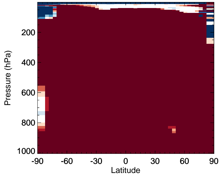
v11-02f-Run0 / v11-02e-Run0 ISOP - Zonal mean % diff for Jul
