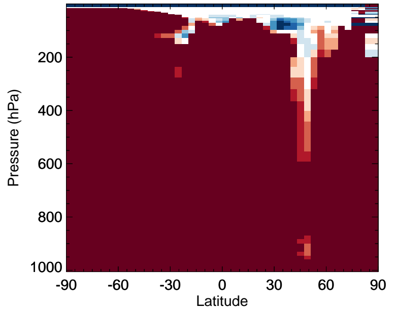
v11-02f-Run0 / v11-02e-Run1 RIPA - Zonal mean % diff for Jul
