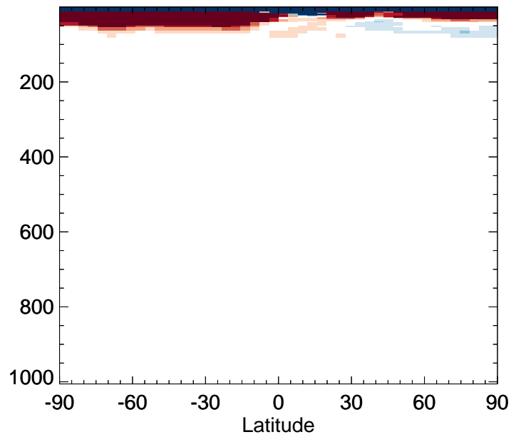
v11-02f-Run0 / v11-02e-Run0 CH3Br - Zonal mean % diff for Jul
