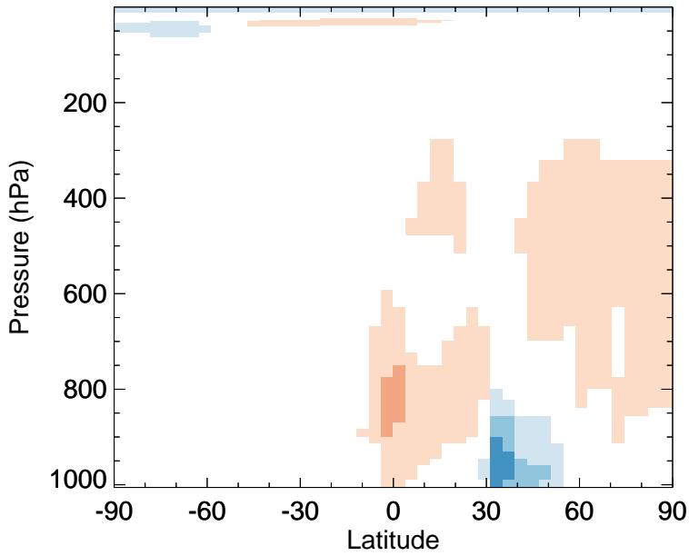
v11-02f-Run0 - v11-02e-Run1 H2O2 - Zonal mean abs diff for Jul
