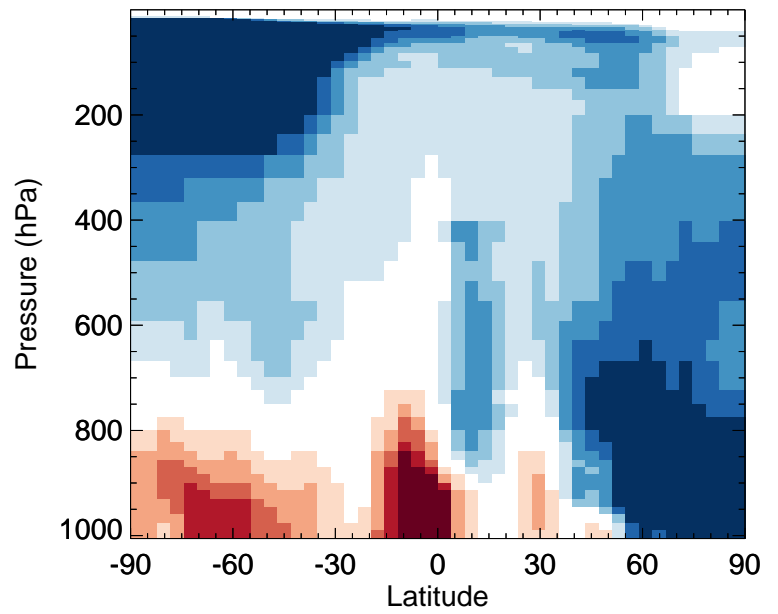
v11-02f-Run0 / v11-02e-Run1 BrNO 2 - Zonal mean % diff for Jul
