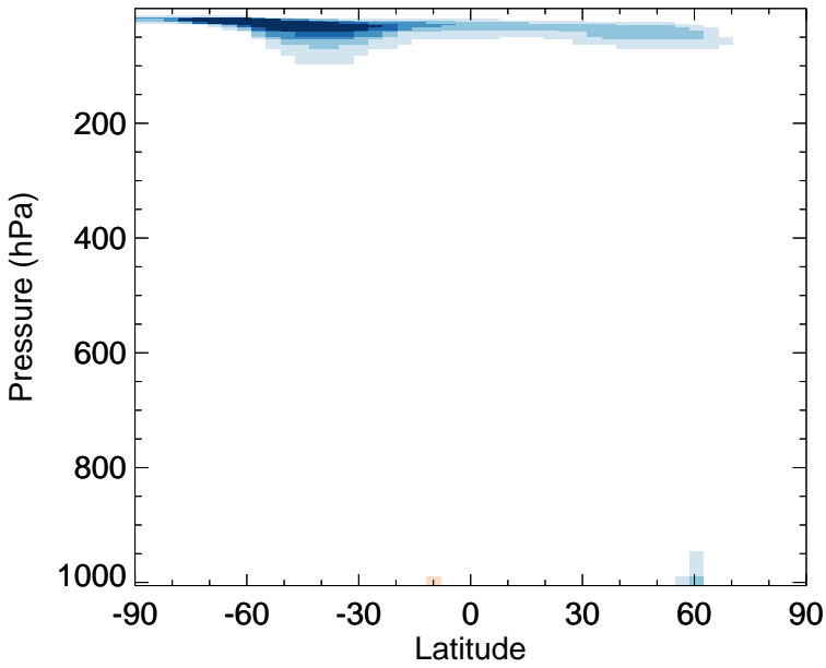
v11-02f-Run0 - v11-02e-Run1 NO 2 - Zonal mean abs diff for Jul
