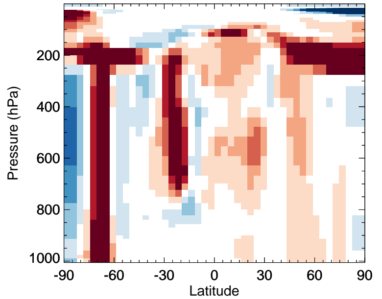
v11-02f-Run0 / v11-02e-Run0 H2O - Zonal mean % diff for Jul
