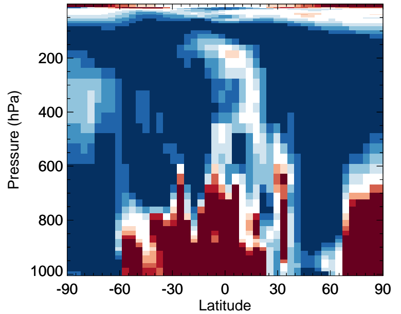
v11-02f-Run0 / v11-02e-Run0 ISOA1 - Zonal mean % diff for Jul
