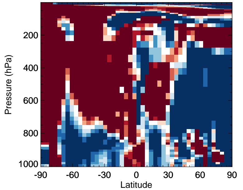
v11-02f-Run0 / v11-02e-Run0 Cl2O2 - Zonal mean % diff for Jul
