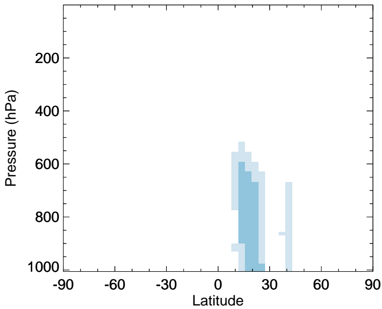
v11-02f-Run0 - v11-02e-Run0 DST1 - Zonal mean abs diff for Jul
