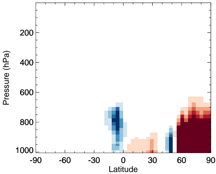
v11-02f-Run0 - v11-02e-Run0 OCPI - Zonal mean abs diff for Jul
