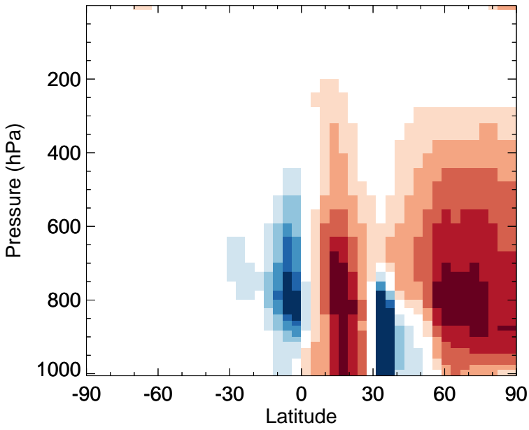
v11-02f-Run0 - v11-02e-Run1 MAP - Zonal mean abs diff for Jul
