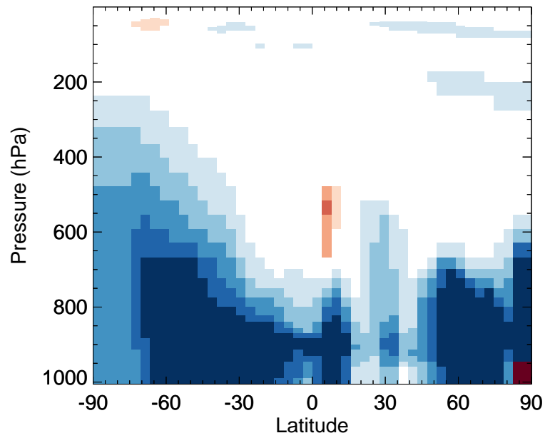
v11-02f-Run0 / v11-02e-Run1 SO 2 - Zonal mean % diff for Jul
