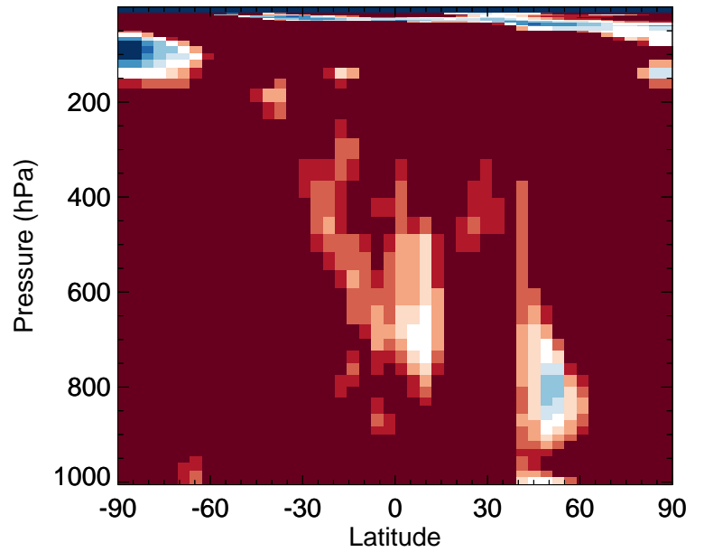
v11-02f-Run0 / v11-02e-Run0 HAC - Zonal mean % diff for Jul
