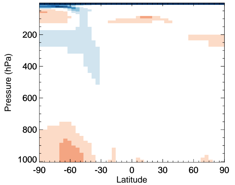
v11-02f-Run0 / v11-02e-Run1 CH 2 O - Zonal mean % diff for Jul
