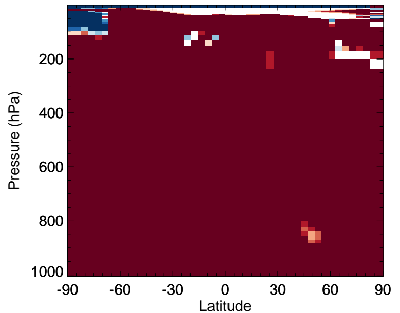
v11-02f-Run0 / v11-02e-Run0 MACR - Zonal mean % diff for Jul
