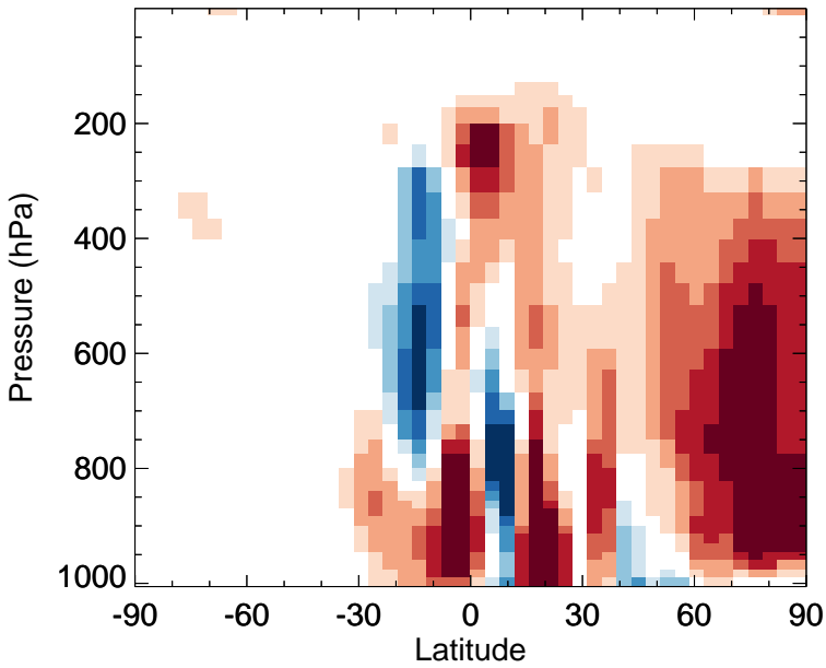
v11-02f-Run0 - v11-02e-Run0 MAP - Zonal mean abs diff for Jul
