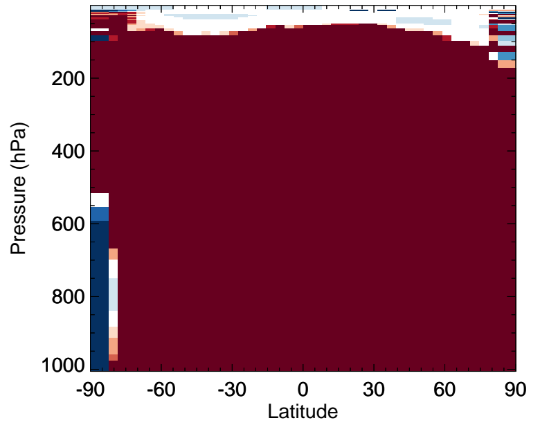
v11-02f-Run0 / v11-02e-Run1 LIMO - Zonal mean % diff for Jul
