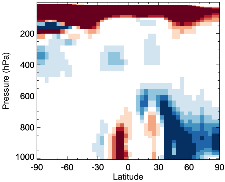
v11-02f-Run0 - v11-02e-Run1 HNO 3 - Zonal mean abs diff for Jul
