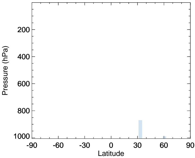
v11-02f-Run0 - v11-02e-Run1 CH 2 O - Zonal mean abs diff for Jul
