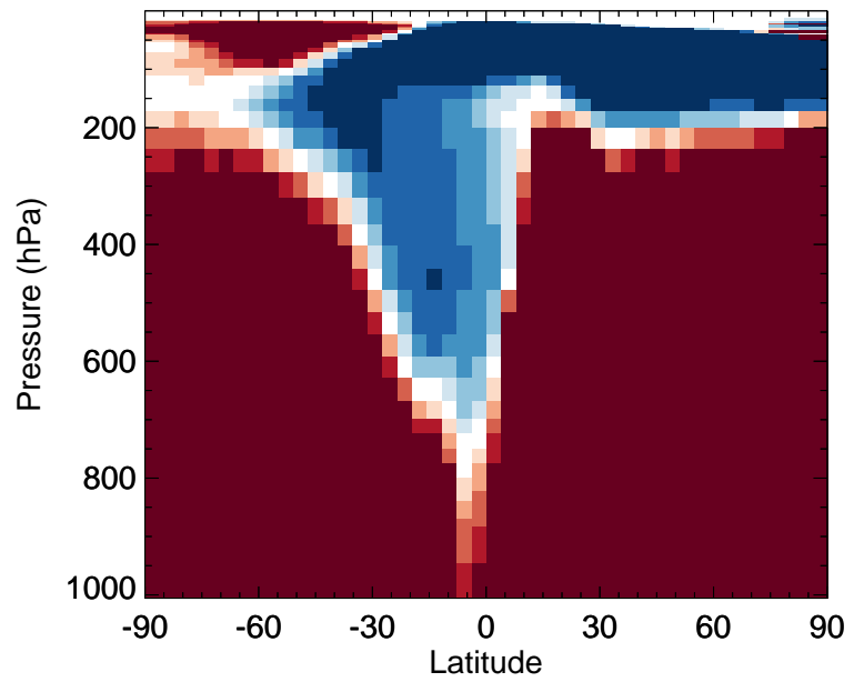
v11-02f-Run0 / v11-02e-Run1 HC187 - Zonal mean % diff for Jul
