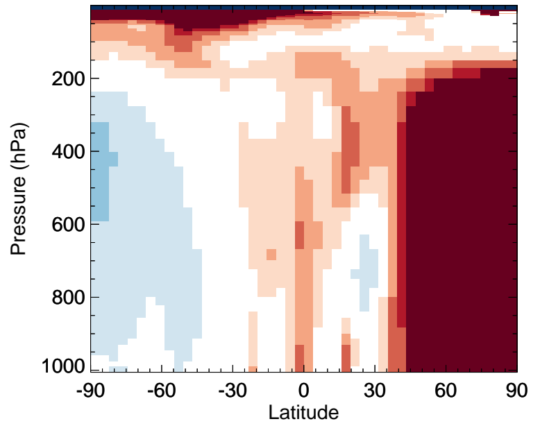
v11-02f-Run0 / v11-02e-Run1 C3H8 - Zonal mean % diff for Jul
