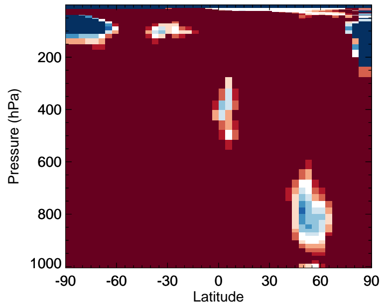
v11-02f-Run0 / v11-02e-Run0 GLYC - Zonal mean % diff for Jul
