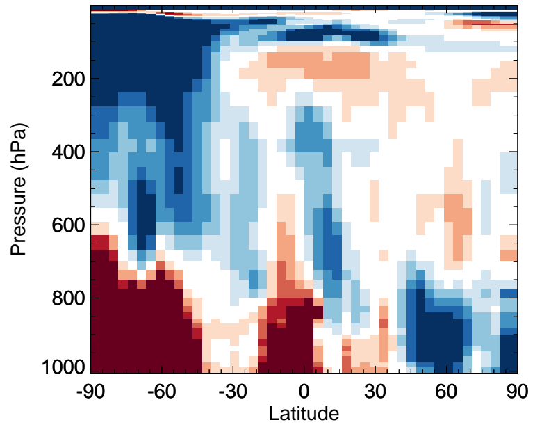
v11-02f-Run0 / v11-02e-Run0 HNO 4 - Zonal mean % diff for Jul
