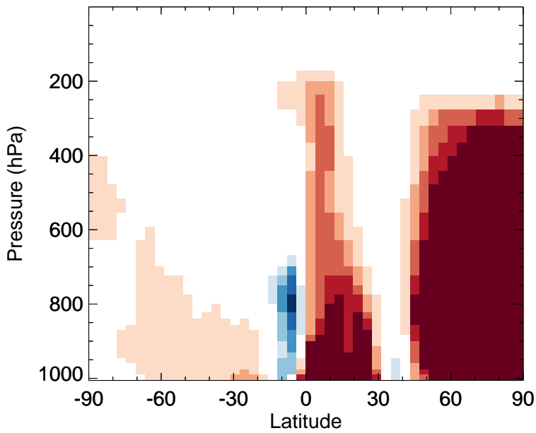
v11-02f-Run0 - v11-02e-Run0 BENZ - Zonal mean abs diff for Jul
