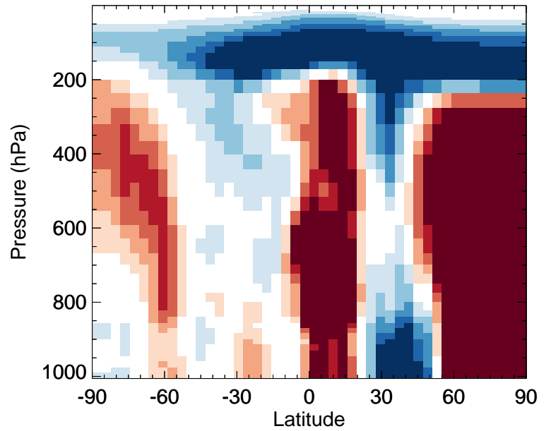
v11-02f-Run0 / v11-02e-Run0 ASOAN - Zonal mean % diff for Jul
