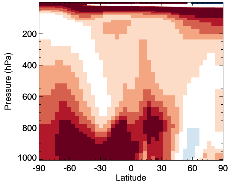
v11-02f-Run0 / v11-02e-Run1 PAN - Zonal mean % diff for Jul
