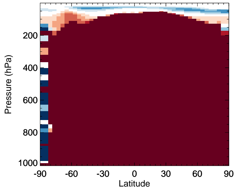
v11-02f-Run0 / v11-02e-Run1 MTPO - Zonal mean % diff for Jul
