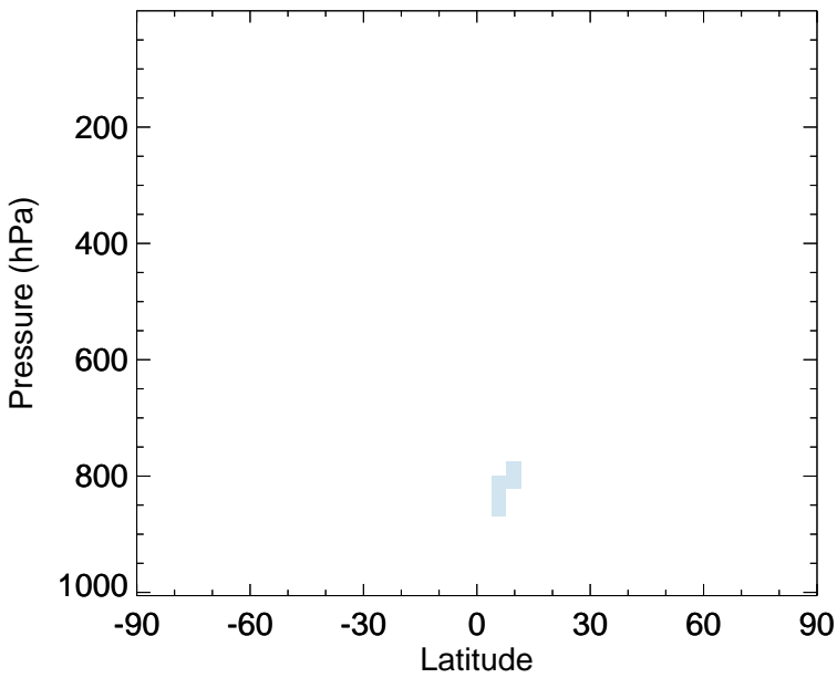
v11-02f-Run0 - v11-02e-Run0 IEPOXA - Zonal mean abs diff for Jul
