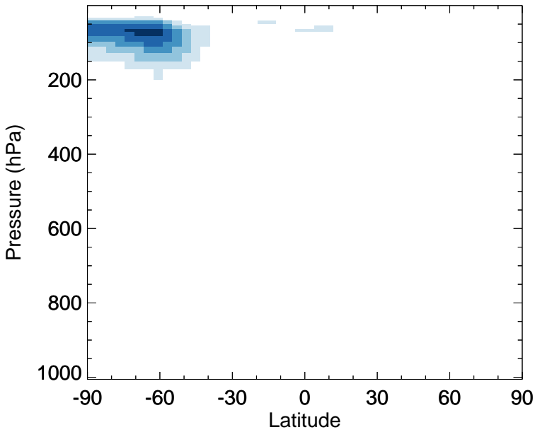
v11-02f-Run0 - v11-02e-Run0 MPN - Zonal mean abs diff for Jul
