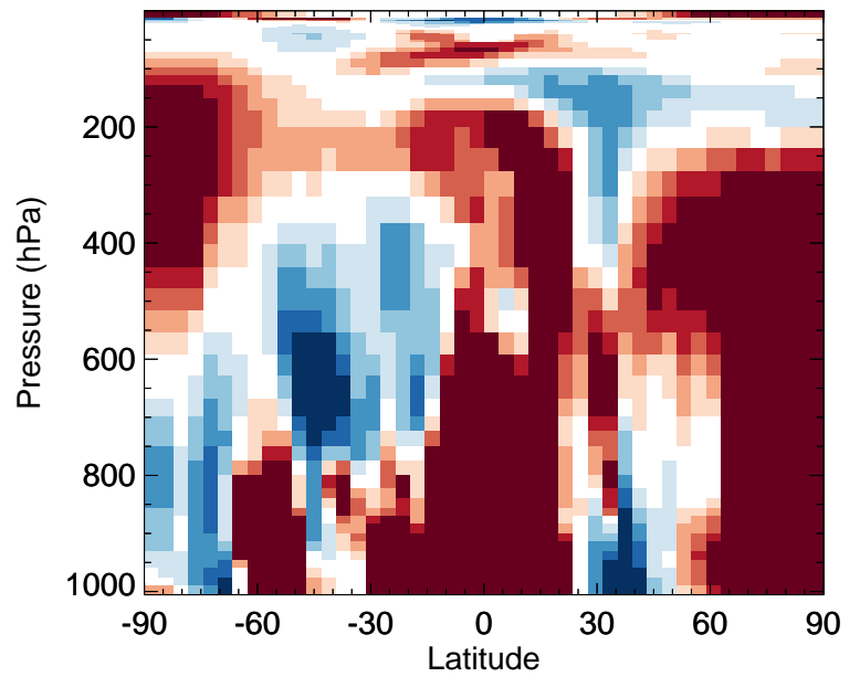
v11-02f-Run0 / v11-02e-Run0 ASOA1 - Zonal mean % diff for Jul
