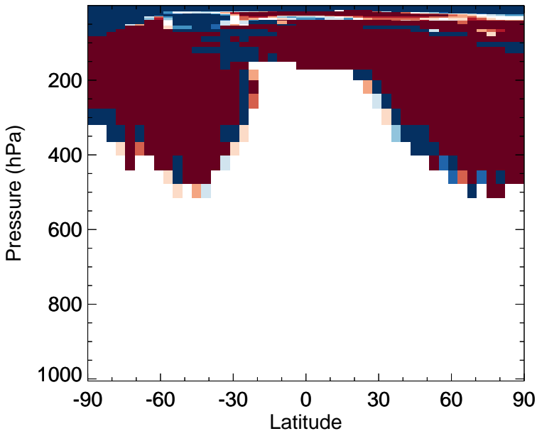
v11-02f-Run0 - v11-02e-Run1 H2O - Zonal mean abs diff for Jul
