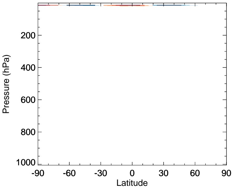
v11-02f-Run0 - v11-02e-Run0 NO 3 - Zonal mean abs diff for Jul
