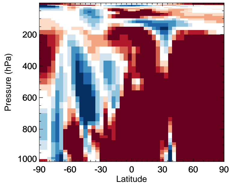
v11-02f-Run0 / v11-02e-Run0 ASOA3 - Zonal mean % diff for Jul
