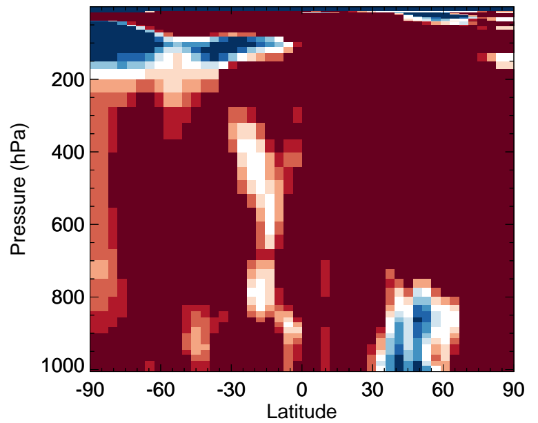
v11-02f-Run0 / v11-02e-Run0 GLYX - Zonal mean % diff for Jul
