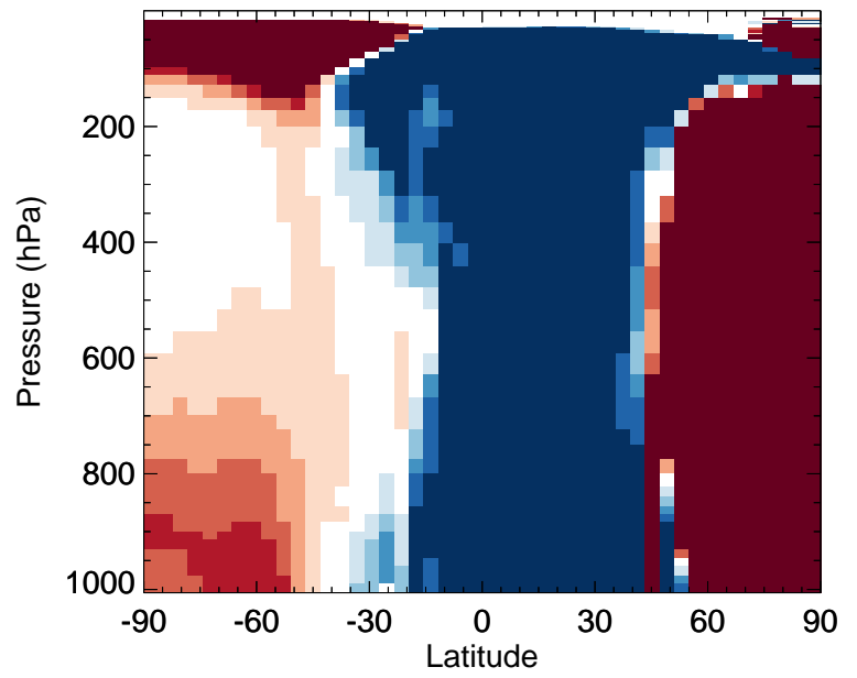
v11-02f-Run0 / v11-02e-Run1 XYLE - Zonal mean % diff for Jul
