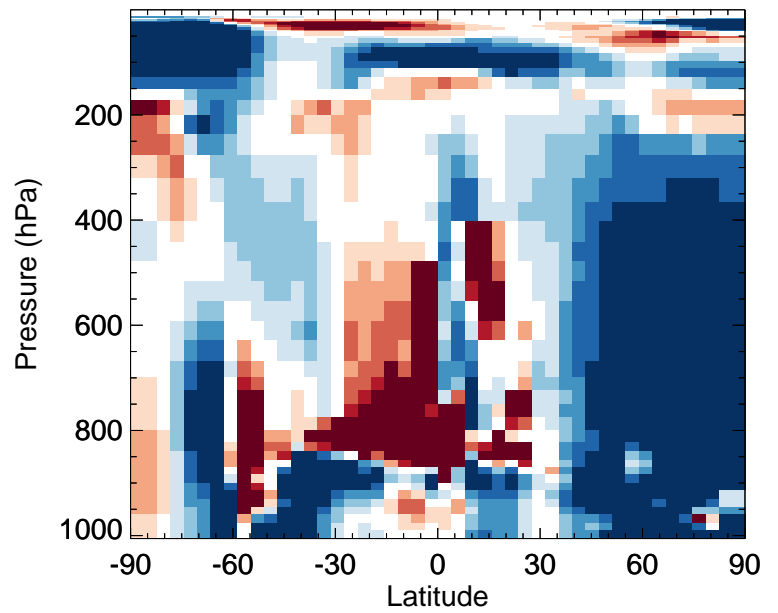
v11-02f-Run0 / v11-02e-Run0 HOBr - Zonal mean % diff for Jul
