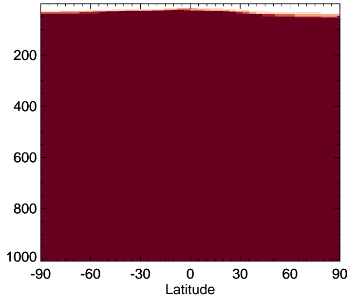
v11-02f-Run0 / v11-02e-Run1 NH3 - Zonal mean % diff for Jul
