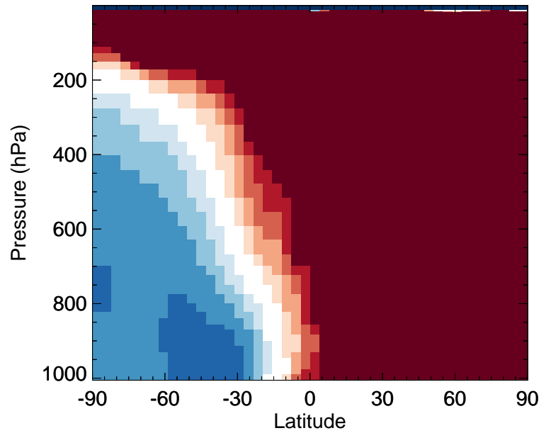
v11-02f-Run0 / v11-02e-Run0 C2H6 - Zonal mean % diff for Jul
