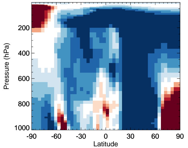
v11-02f-Run0 / v11-02e-Run0 ASOG2 - Zonal mean % diff for Jul
