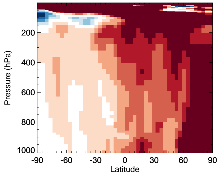
v11-02f-Run0 / v11-02e-Run0 ACET - Zonal mean % diff for Jul
