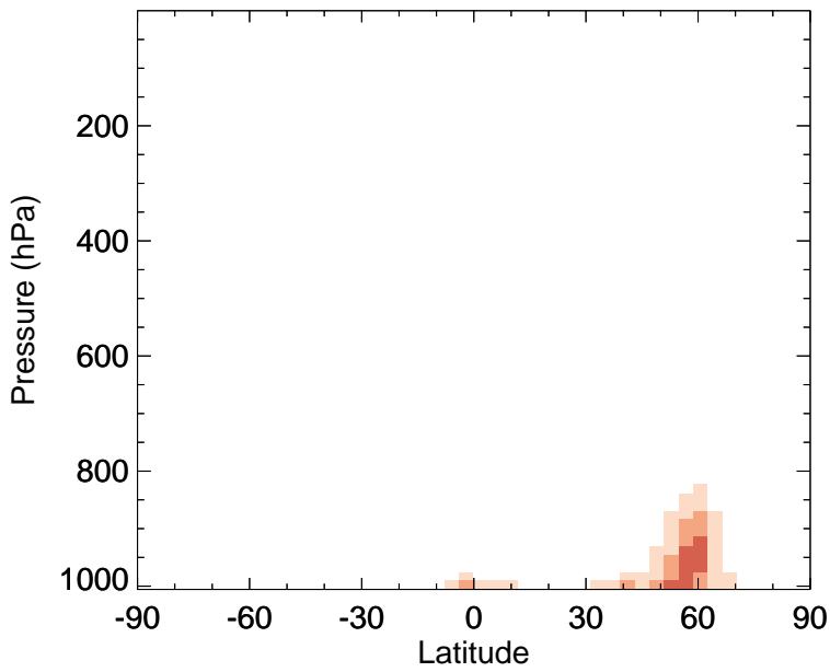
v11-02f-Run0 - v11-02e-Run1 RCHO - Zonal mean abs diff for Jul
