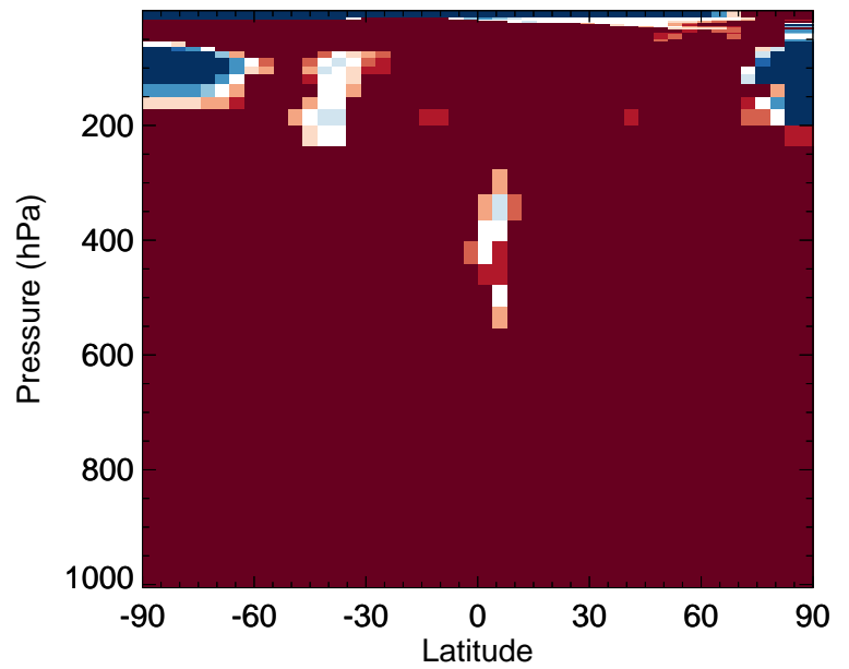
v11-02f-Run0 / v11-02e-Run0 IEPOXA - Zonal mean % diff for Jul
