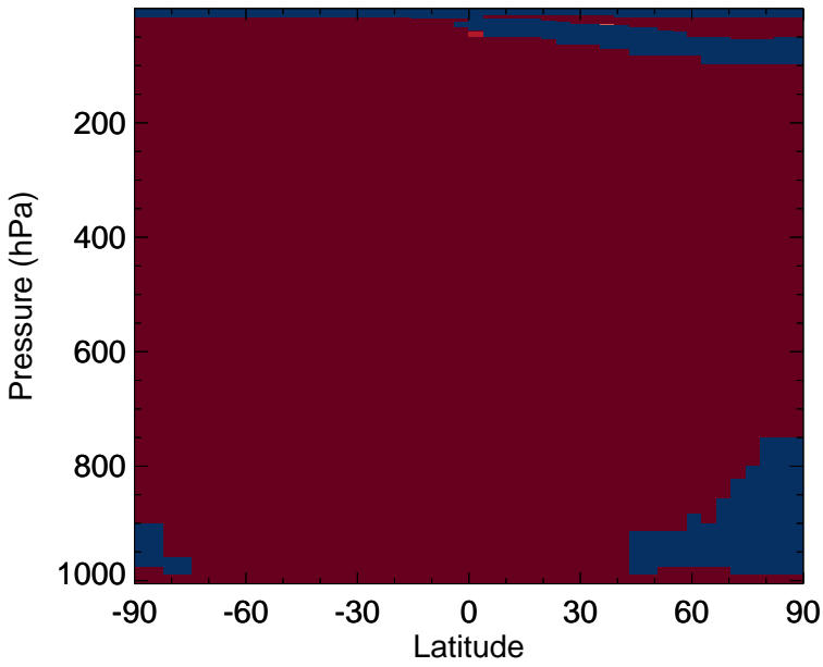
v11-02f-Run0 - v11-02e-Run0 CH4 - Zonal mean abs diff for Jul
