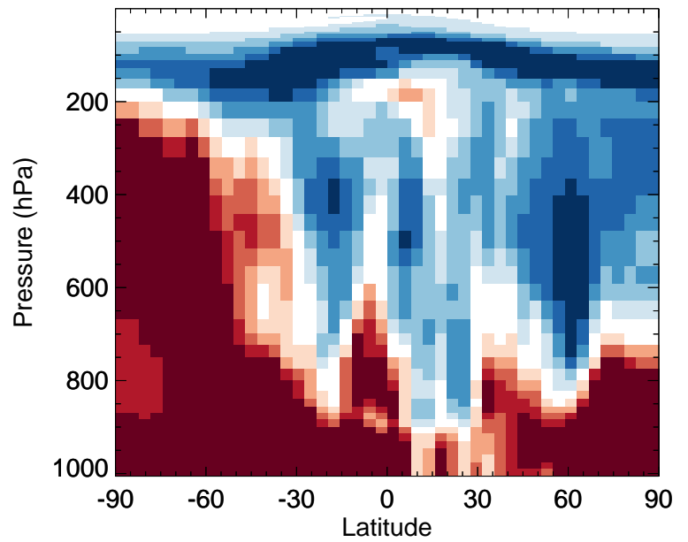
v11-02f-Run0 / v11-02e-Run0 SOAMG - Zonal mean % diff for Jul
