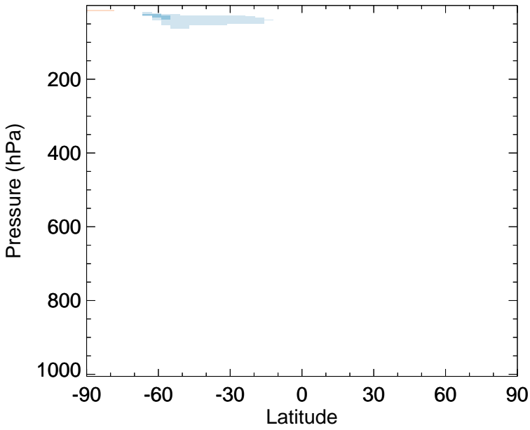
v11-02f-Run0 - v11-02e-Run0 BrNO3 - Zonal mean abs diff for Jul
