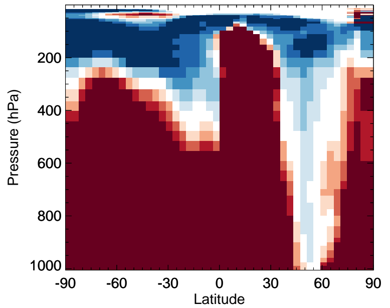
v11-02f-Run0 / v11-02e-Run1 MVKN - Zonal mean % diff for Jul
