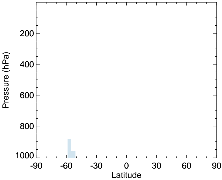
v11-02f-Run0 - v11-02e-Run0 SALA - Zonal mean abs diff for Jul
