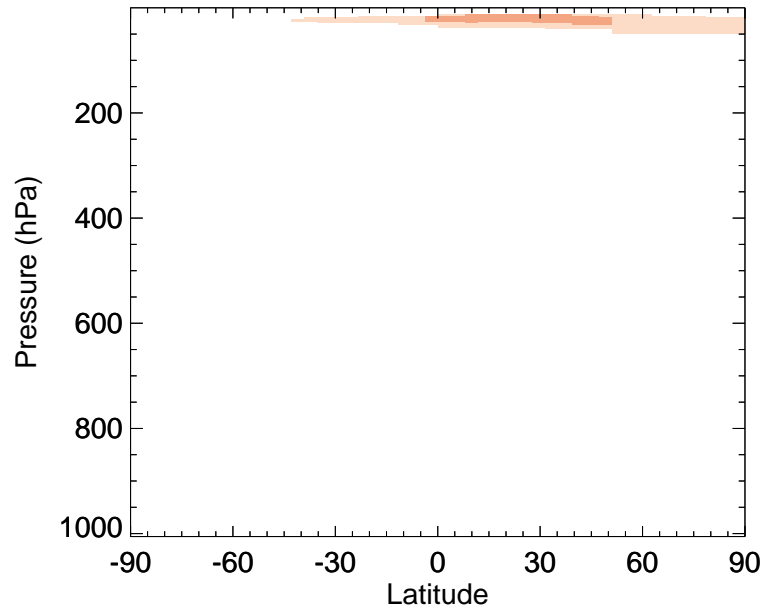
v11-02f-Run0 / v11-02e-Run1 H1211 - Zonal mean % diff for Jul
