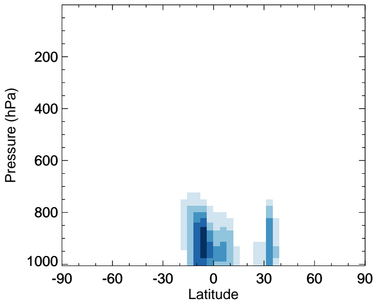
v11-02f-Run0 - v11-02e-Run1 MACR - Zonal mean abs diff for Jul
