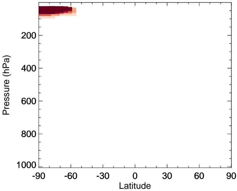
v11-02f-Run0 - v11-02e-Run0 Cl2O2 - Zonal mean abs diff for Jul
