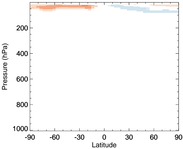
v11-02f-Run0 - v11-02e-Run0 CFC12 - Zonal mean abs diff for Jul
