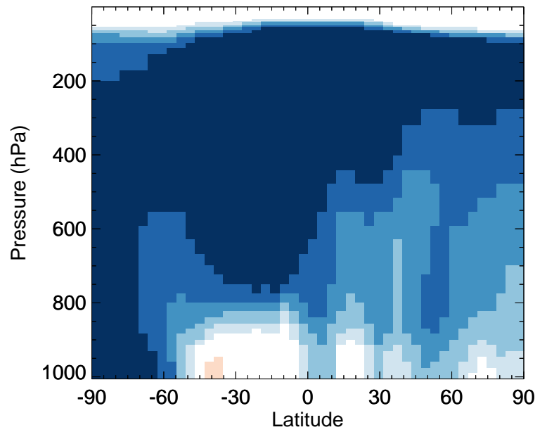
v11-02f-Run0 / v11-02e-Run1 ISOG1 - Zonal mean % diff for Jul
