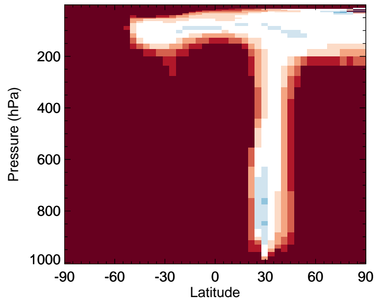
v11-02f-Run0 / v11-02e-Run1 RCHO - Zonal mean % diff for Jul
