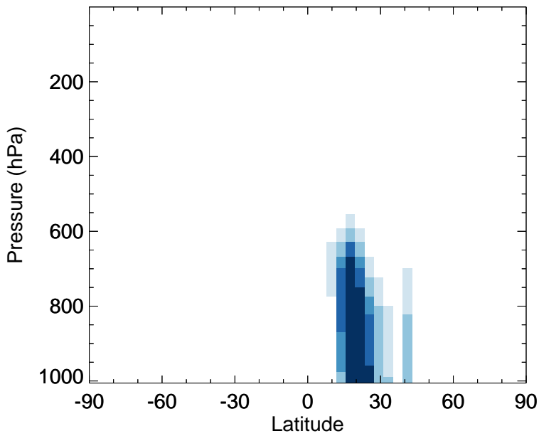
v11-02f-Run0 - v11-02e-Run0 DST4 - Zonal mean abs diff for Jul
