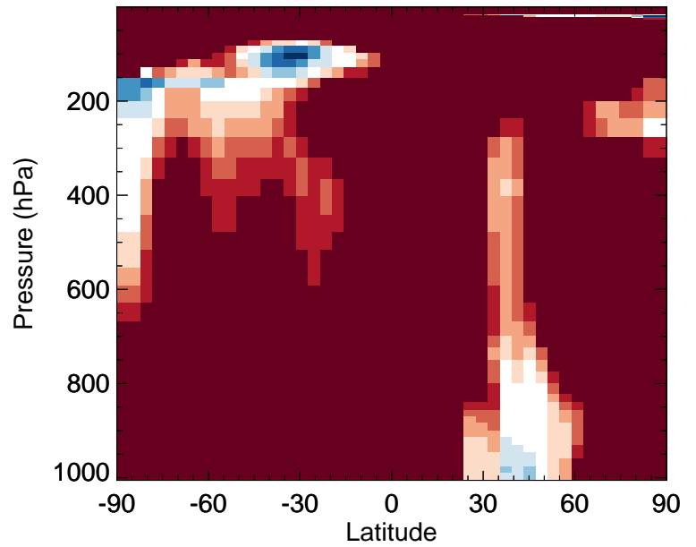
v11-02f-Run0 / v11-02e-Run0 R4N2 - Zonal mean % diff for Jul
