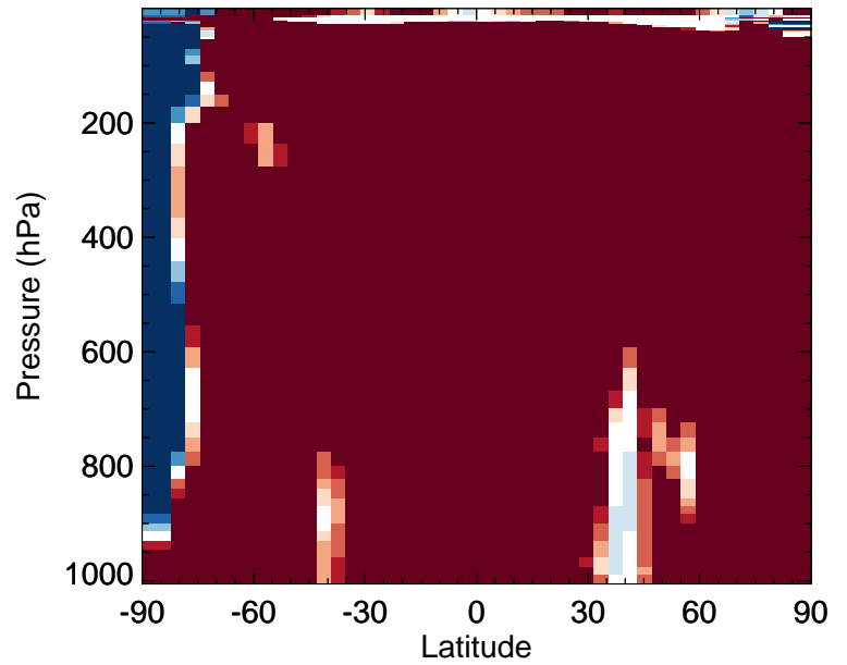
v11-02f-Run0 / v11-02e-Run0 OCPO - Zonal mean % diff for Jul
