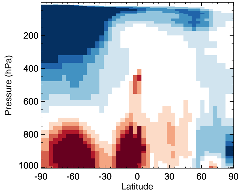
v11-02f-Run0 / v11-02e-Run1 NO 2 - Zonal mean % diff for Jul
