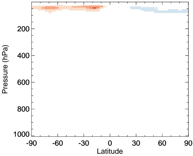
v11-02f-Run0 - v11-02e-Run0 OCS - Zonal mean abs diff for Jul
