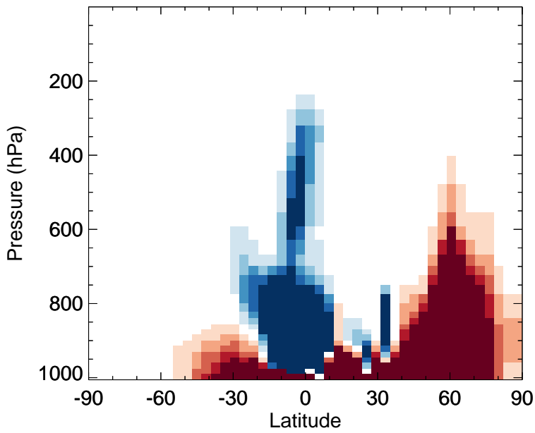
v11-02f-Run0 - v11-02e-Run1 PRPE - Zonal mean abs diff for Jul
