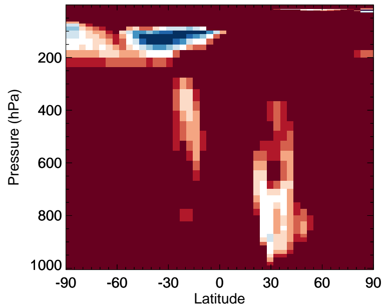
v11-02f-Run0 / v11-02e-Run0 RCHO - Zonal mean % diff for Jul
