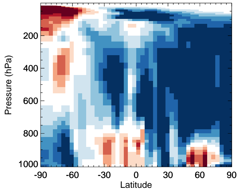
v11-02f-Run0 / v11-02e-Run0 ISOG1 - Zonal mean % diff for Jul
