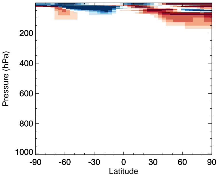
v11-02f-Run0 - v11-02e-Run0 HCl - Zonal mean abs diff for Jul
