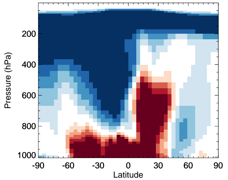
v11-02f-Run0 / v11-02e-Run1 ISOA3 - Zonal mean % diff for Jul
