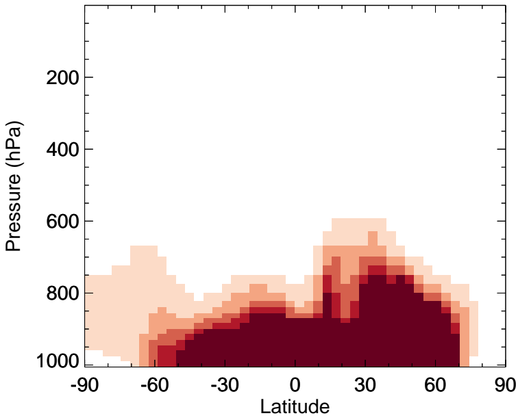
v11-02f-Run0 - v11-02e-Run1 NH3 - Zonal mean abs diff for Jul
