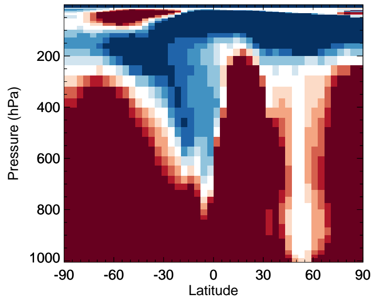
v11-02f-Run0 / v11-02e-Run1 GLYC - Zonal mean % diff for Jul
