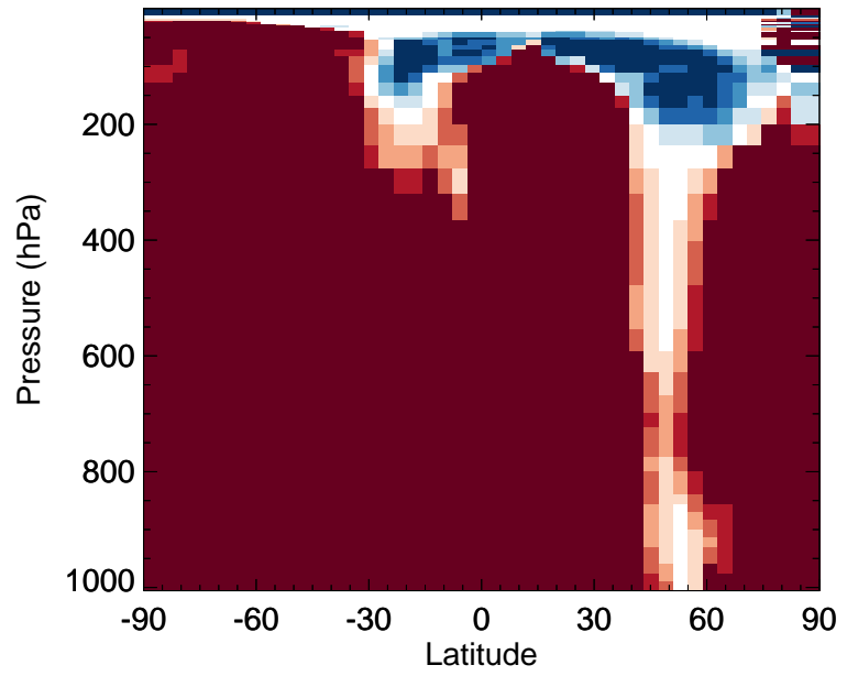
v11-02f-Run0 / v11-02e-Run1 ISN1 - Zonal mean % diff for Jul
