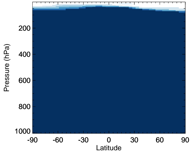
v11-02f-Run0 / v11-02e-Run0 SOAIE - Zonal mean % diff for Jul
