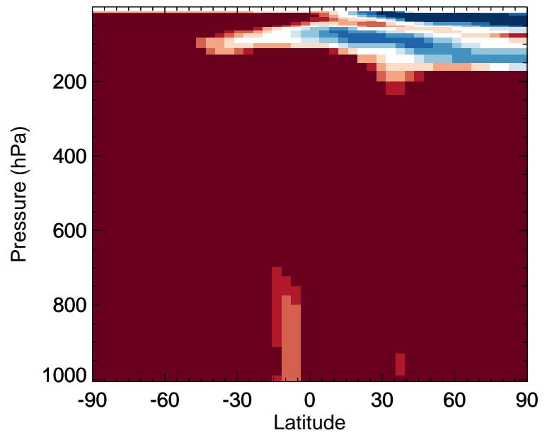
v11-02f-Run0 / v11-02e-Run1 BENZ - Zonal mean % diff for Jul
