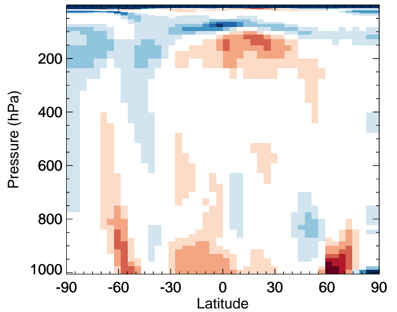
v11-02f-Run0 / v11-02e-Run0 CH 2 O - Zonal mean % diff for Jul
