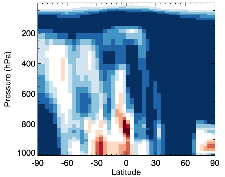
v11-02f-Run0 / v11-02e-Run0 ISN1OA - Zonal mean % diff for Jul
