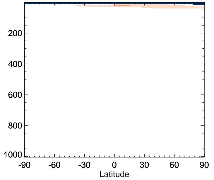
v11-02f-Run0 / v11-02e-Run1 H2402 - Zonal mean % diff for Jul
