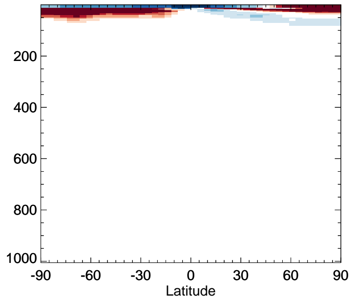
v11-02f-Run0 / v11-02e-Run0 CFC12 - Zonal mean % diff for Jul
