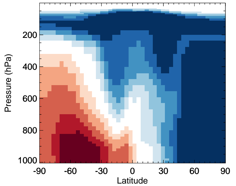
v11-02f-Run0 / v11-02e-Run1 ISN1OA - Zonal mean % diff for Jul
