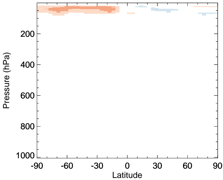
v11-02f-Run0 - v11-02e-Run0 CH3Cl - Zonal mean abs diff for Jul
