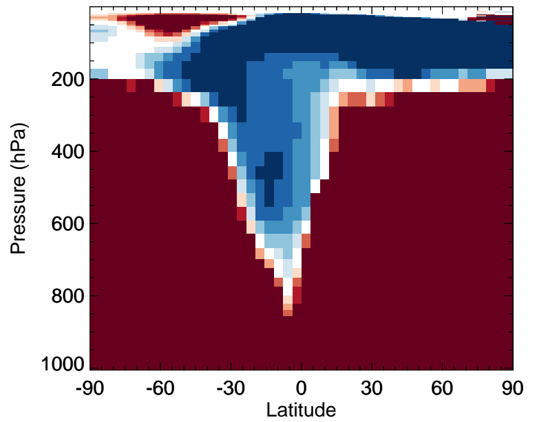
v11-02f-Run0 / v11-02e-Run1 IEPOXD - Zonal mean % diff for Jul
