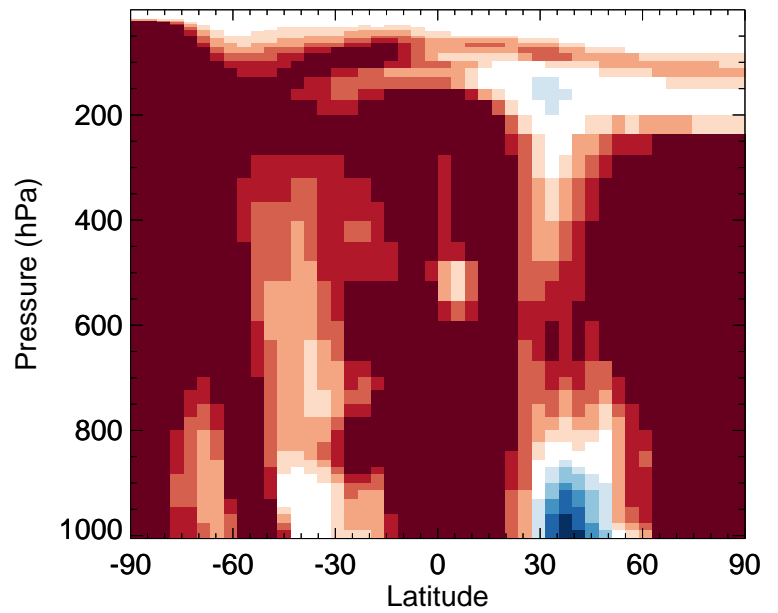
v11-02f-Run0 / v11-02e-Run0 ASOG3 - Zonal mean % diff for Jul
