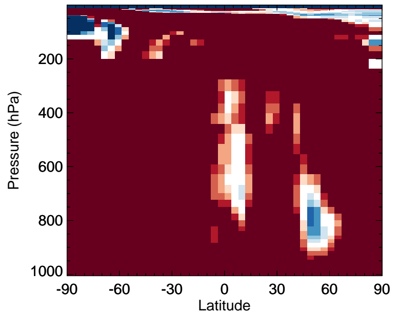
v11-02f-Run0 / v11-02e-Run0 HCOOH - Zonal mean % diff for Jul
