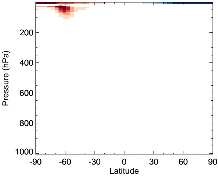
v11-02f-Run0 - v11-02e-Run1 ClO - Zonal mean abs diff for Jul
