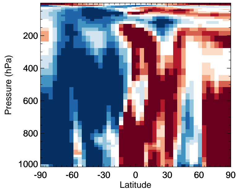
v11-02f-Run0 / v11-02e-Run0 ISOA2 - Zonal mean % diff for Jul
