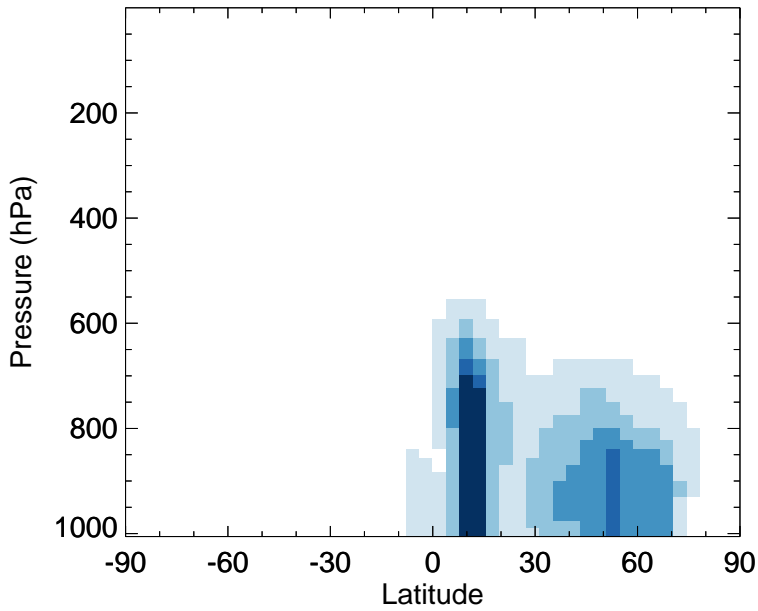
v11-02f-Run0 - v11-02e-Run0 SOAIE - Zonal mean abs diff for Jul
