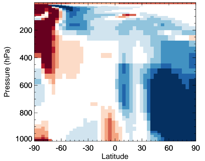
v11-02f-Run0 / v11-02e-Run1 CIOO - Zonal mean % diff for Jul
