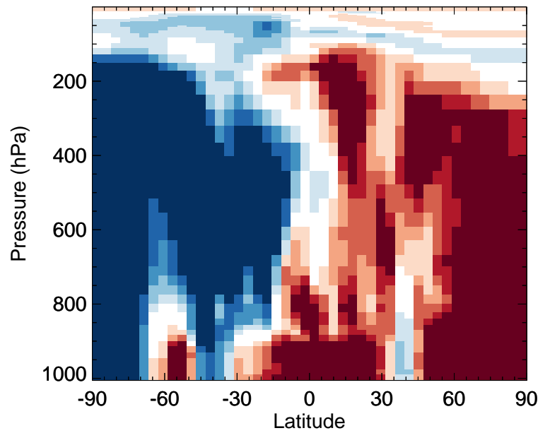
v11-02f-Run0 / v11-02e-Run0 OCPI - Zonal mean % diff for Jul
