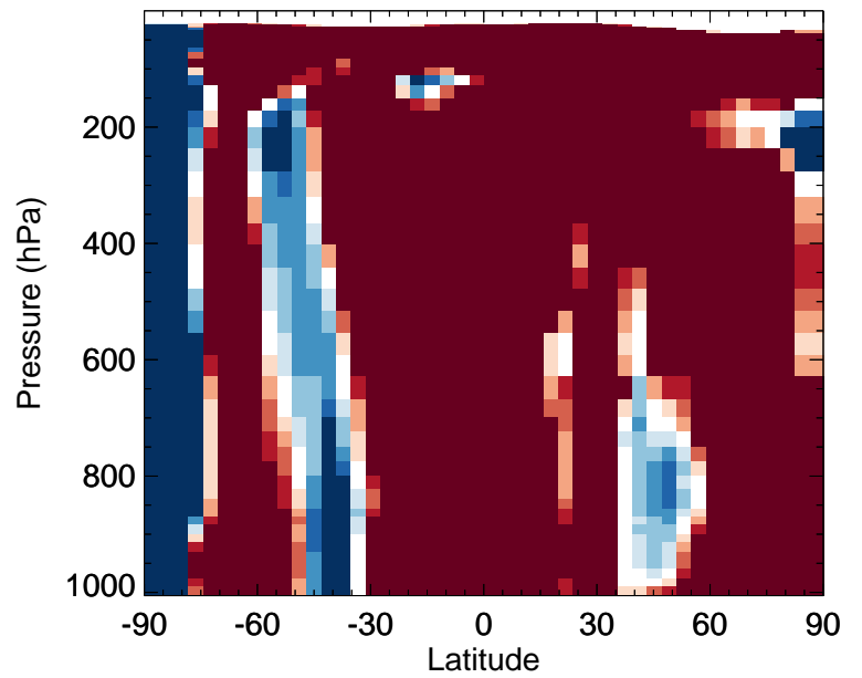
v11-02f-Run0 / v11-02e-Run0 SOAP - Zonal mean % diff for Jul
