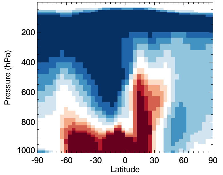
v11-02f-Run0 / v11-02e-Run1 ISOA1 - Zonal mean % diff for Jul
