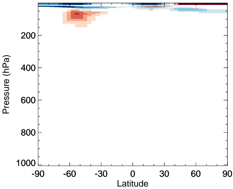
v11-02f-Run0 - v11-02e-Run1 HCl - Zonal mean abs diff for Jul
