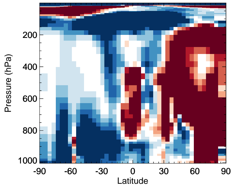
v11-02f-Run0 / v11-02e-Run0 SO 2 - Zonal mean % diff for Jul
