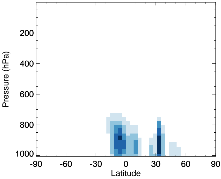
v11-02f-Run0 - v11-02e-Run1 MVK - Zonal mean abs diff for Jul
