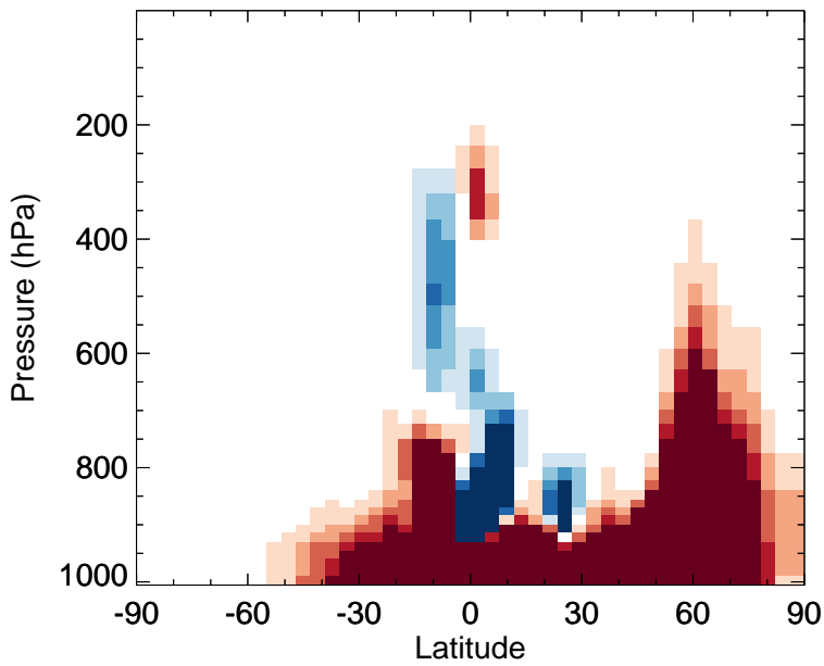
v11-02f-Run0 - v11-02e-Run0 PRPE - Zonal mean abs diff for Jul
