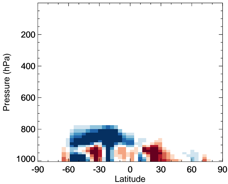
v11-02f-Run0 - v11-02e-Run0 SALC - Zonal mean abs diff for Jul
