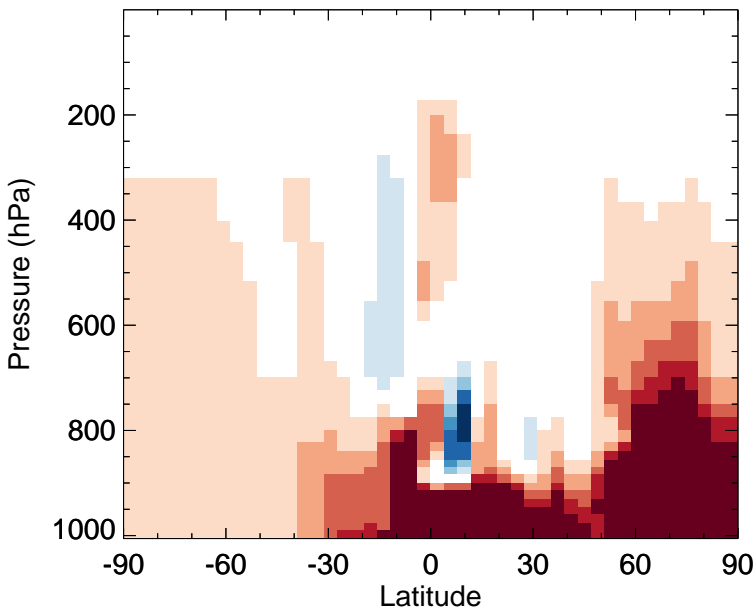
v11-02f-Run0 - v11-02e-Run0 MEK - Zonal mean abs diff for Jul
