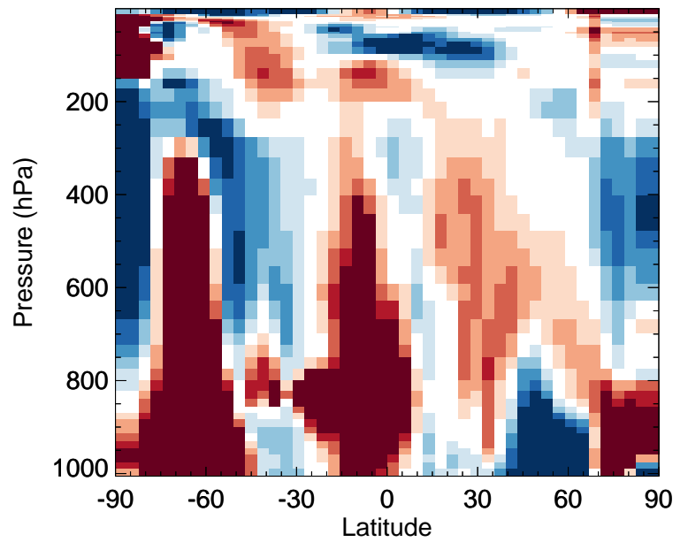
v11-02f-Run0 / v11-02e-Run0 NO 3 - Zonal mean % diff for Jul
