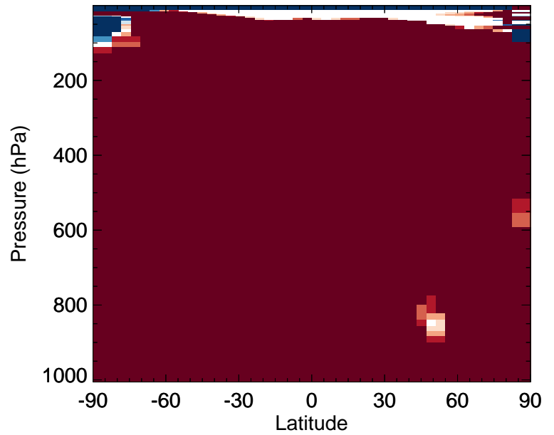
v11-02f-Run0 / v11-02e-Run0 MVK - Zonal mean % diff for Jul
