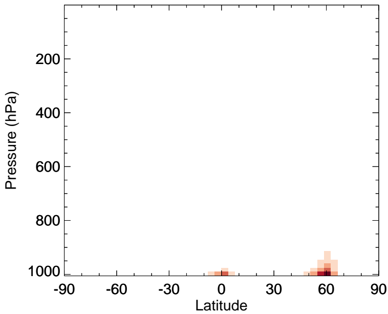
v11-02f-Run0 - v11-02e-Run0 MTPA - Zonal mean abs diff for Jul
