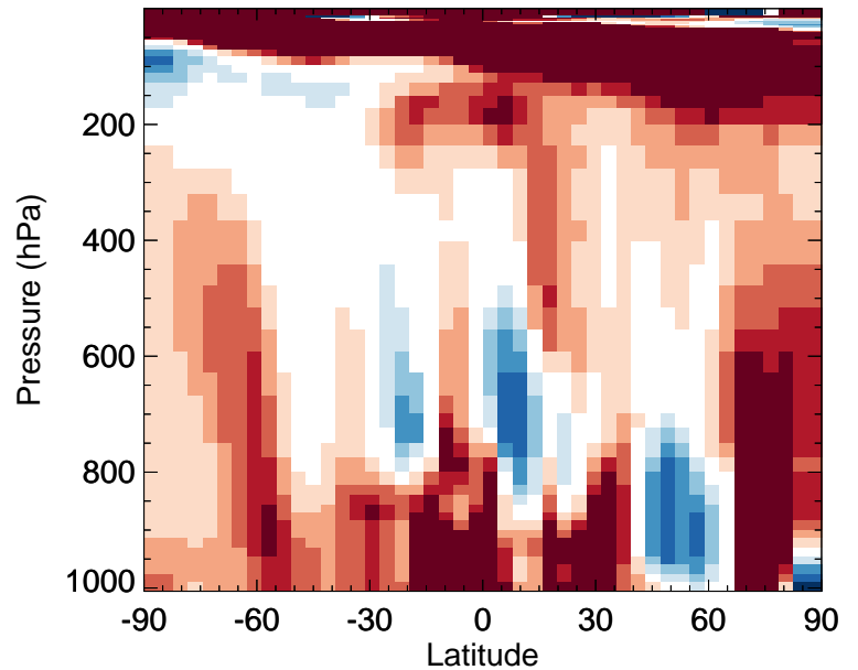
v11-02f-Run0 / v11-02e-Run0 PAN - Zonal mean % diff for Jul
