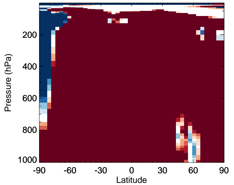
v11-02f-Run0 / v11-02e-Run0 NPMN - Zonal mean % diff for Jul
