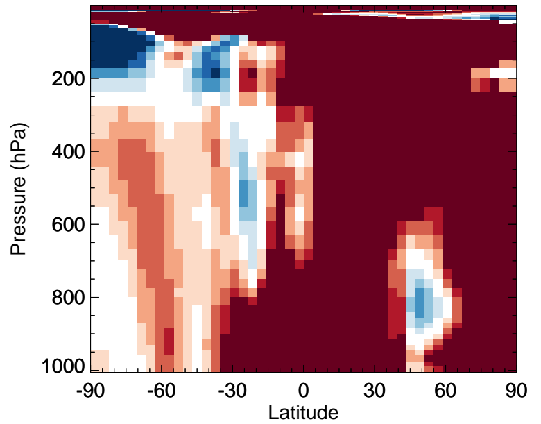
v11-02f-Run0 / v11-02e-Run0 EOH - Zonal mean % diff for Jul
