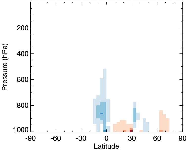
v11-02f-Run0 - v11-02e-Run1 EOH - Zonal mean abs diff for Jul
