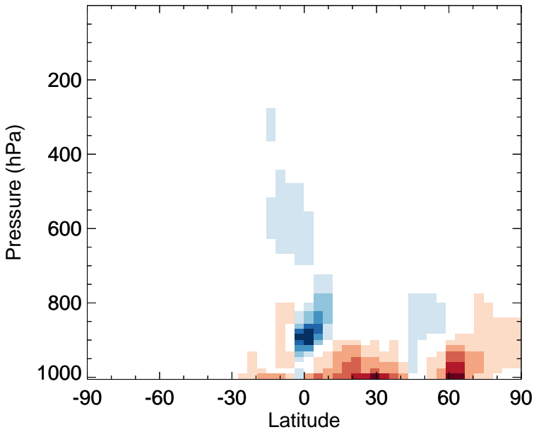
v11-02f-Run0 - v11-02e-Run0 EOH - Zonal mean abs diff for Jul
