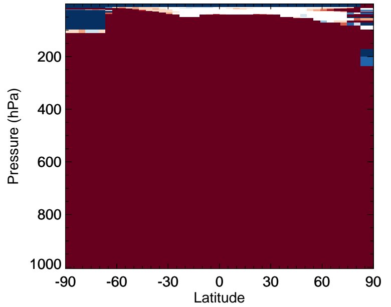
v11-02f-Run0 / v11-02e-Run0 RIPA - Zonal mean % diff for Jul
