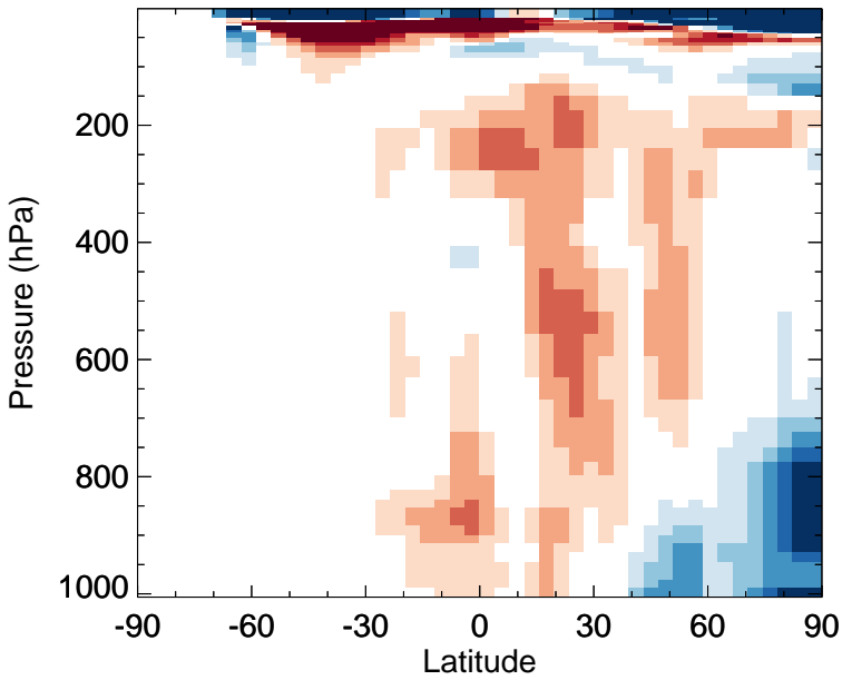
v11-02f-Run0 - v11-02e-Run0 HO2 - Zonal mean abs diff for Jul
