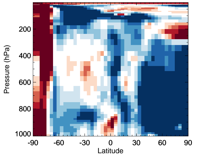
v11-02f-Run0 / v11-02e-Run0 CIOO - Zonal mean % diff for Jul
