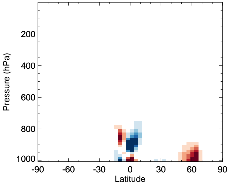
v11-02f-Run0 - v11-02e-Run0 ISOP - Zonal mean abs diff for Jul
