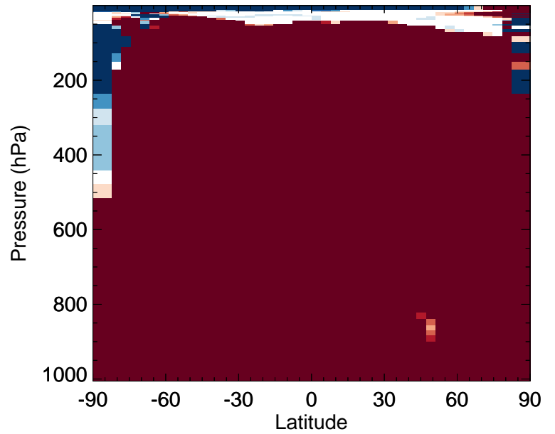
v11-02f-Run0 / v11-02e-Run0 MOBA - Zonal mean % diff for Jul
