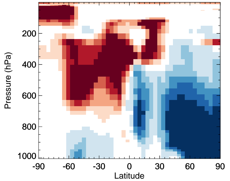
v11-02f-Run0 / v11-02e-Run1 BrCl - Zonal mean % diff for Jul
