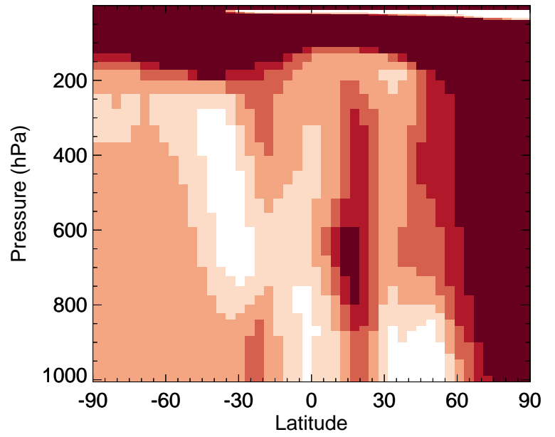
v11-02f-Run0 / v11-02e-Run1 MAP - Zonal mean % diff for Jul
