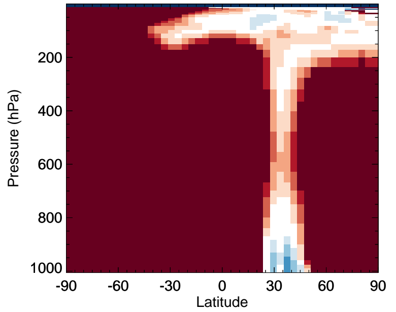
v11-02f-Run0 / v11-02e-Run1 ALK4 - Zonal mean % diff for Jul
