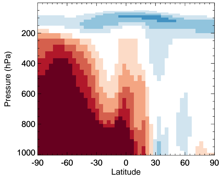
v11-02f-Run0 / v11-02e-Run1 SOAGX - Zonal mean % diff for Jul
