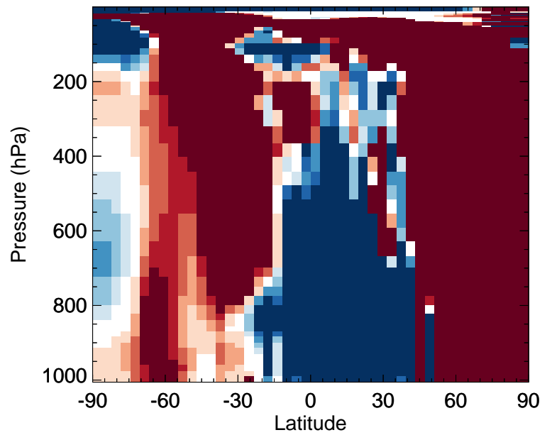
v11-02f-Run0 / v11-02e-Run0 XYLE - Zonal mean % diff for Jul
