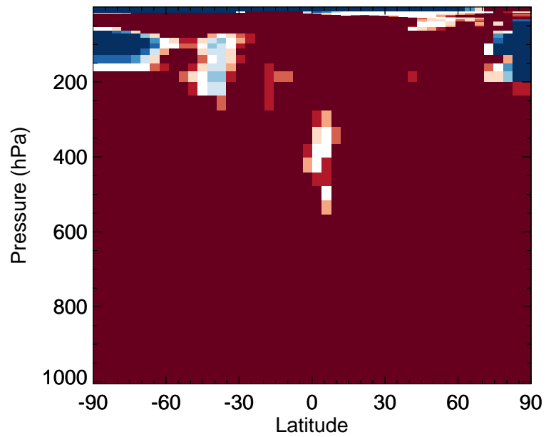
v11-02f-Run0 / v11-02e-Run0 IEPOXD - Zonal mean % diff for Jul
