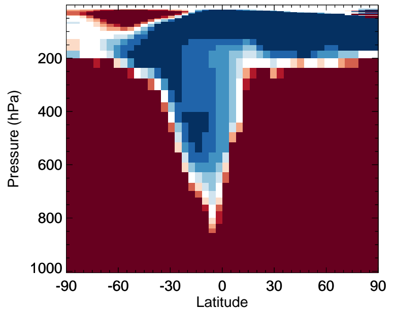
v11-02f-Run0 / v11-02e-Run1 IEPOXA - Zonal mean % diff for Jul
