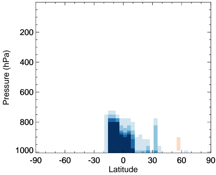
v11-02f-Run0 - v11-02e-Run1 ISOP - Zonal mean abs diff for Jul
