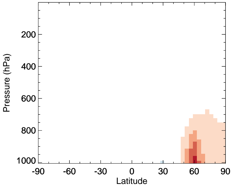
v11-02f-Run0 - v11-02e-Run1 C3H8 - Zonal mean abs diff for Jul
