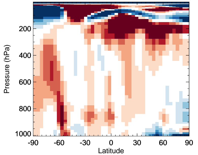
v11-02f-Run0 / v11-02e-Run0 H2O2 - Zonal mean % diff for Jul
