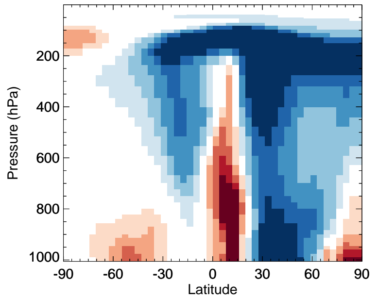
v11-02f-Run0 / v11-02e-Run1 ASOG2 - Zonal mean % diff for Jul
