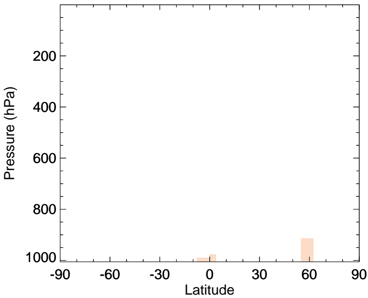
v11-02f-Run0 - v11-02e-Run0 TSOA2 - Zonal mean abs diff for Jul
