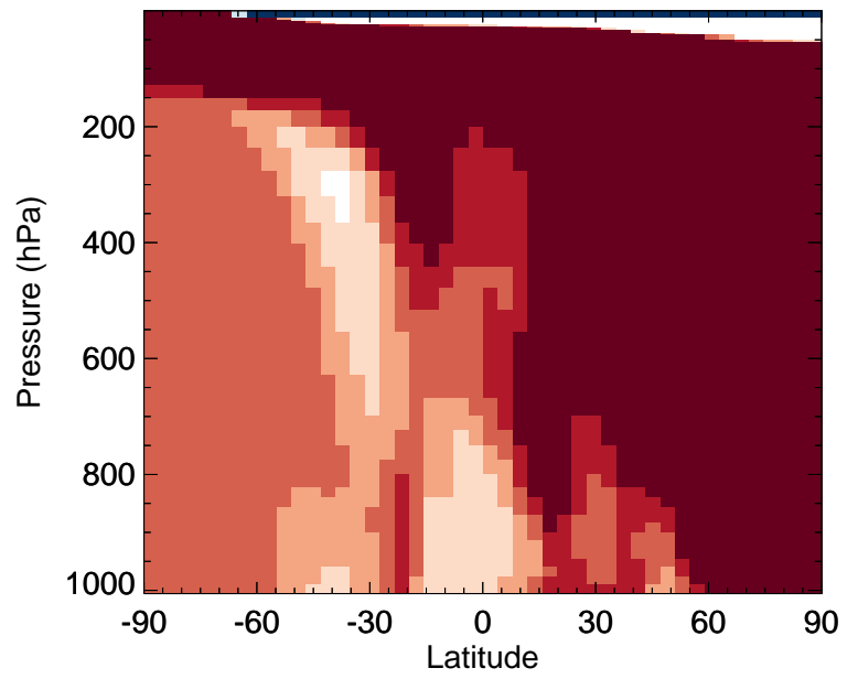
v11-02f-Run0 / v11-02e-Run1 ALD2 - Zonal mean % diff for Jul
