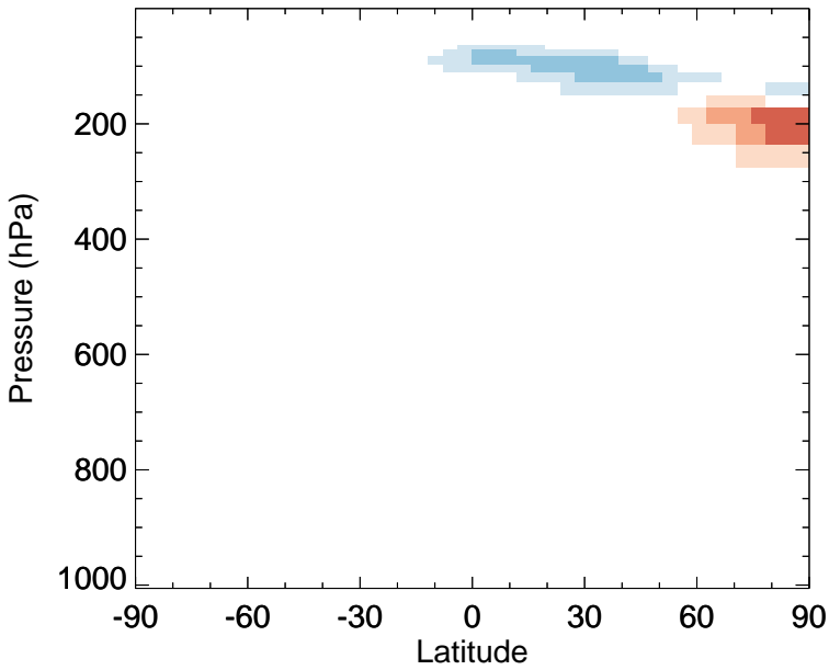
v11-02f-Run0 - v11-02e-Run0 SO4 - Zonal mean abs diff for Jul
