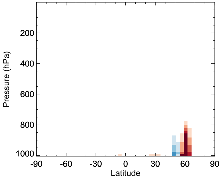
v11-02f-Run0 - v11-02e-Run0 OCPO - Zonal mean abs diff for Jul
