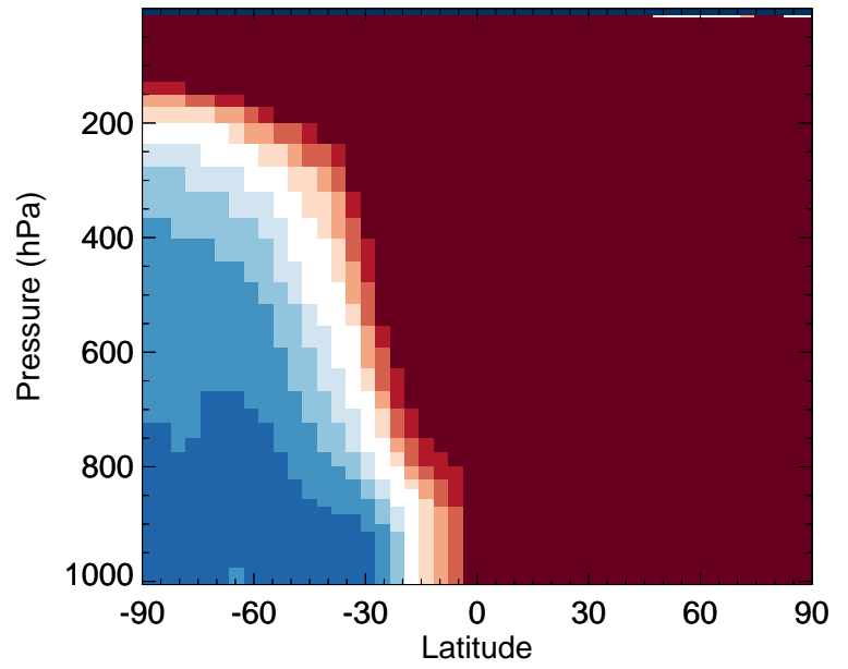
v11-02f-Run0 / v11-02e-Run1 C2H6 - Zonal mean % diff for Jul
