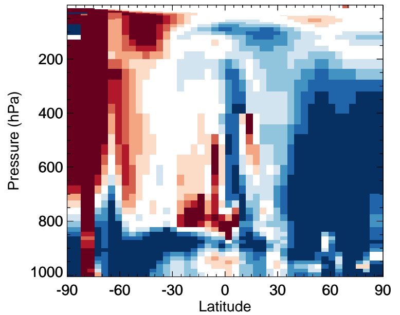
v11-02f-Run0 / v11-02e-Run0 BrO - Zonal mean % diff for Jul
