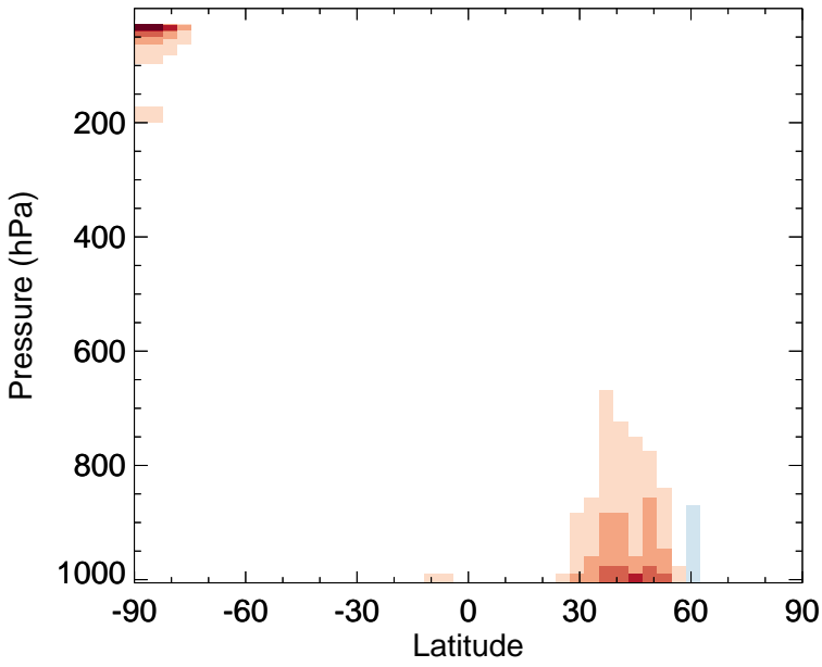
v11-02f-Run0 - v11-02e-Run1 NIT - Zonal mean abs diff for Jul
