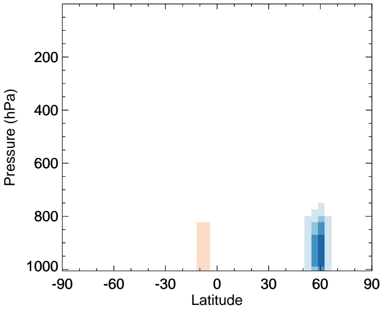
v11-02f-Run0 - v11-02e-Run1 PAN - Zonal mean abs diff for Jul
