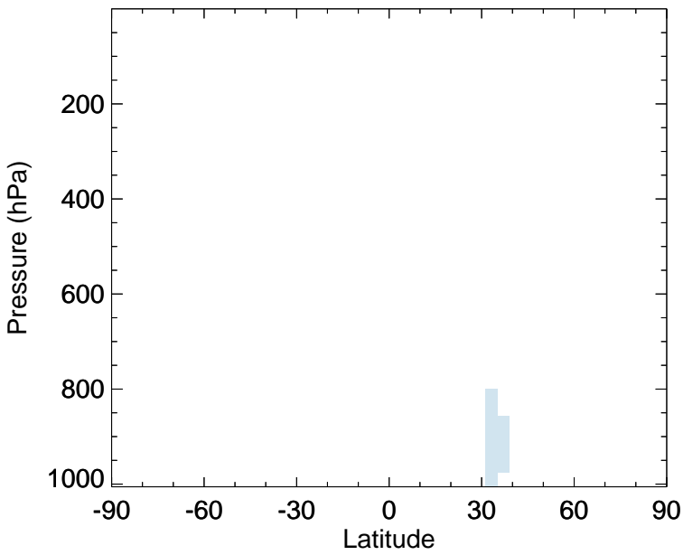
v11-02f-Run0 - v11-02e-Run1 ISOG3 - Zonal mean abs diff for Jul
