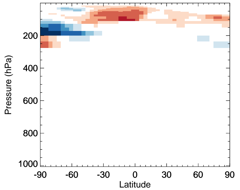
v11-02f-Run0 / v11-02e-Run1 SALC - Zonal mean % diff for Jul
