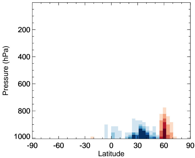
v11-02f-Run0 - v11-02e-Run0 XYLE - Zonal mean abs diff for Jul
