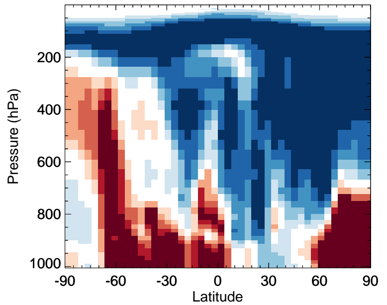
v11-02f-Run0 / v11-02e-Run0 SOAGX - Zonal mean % diff for Jul
