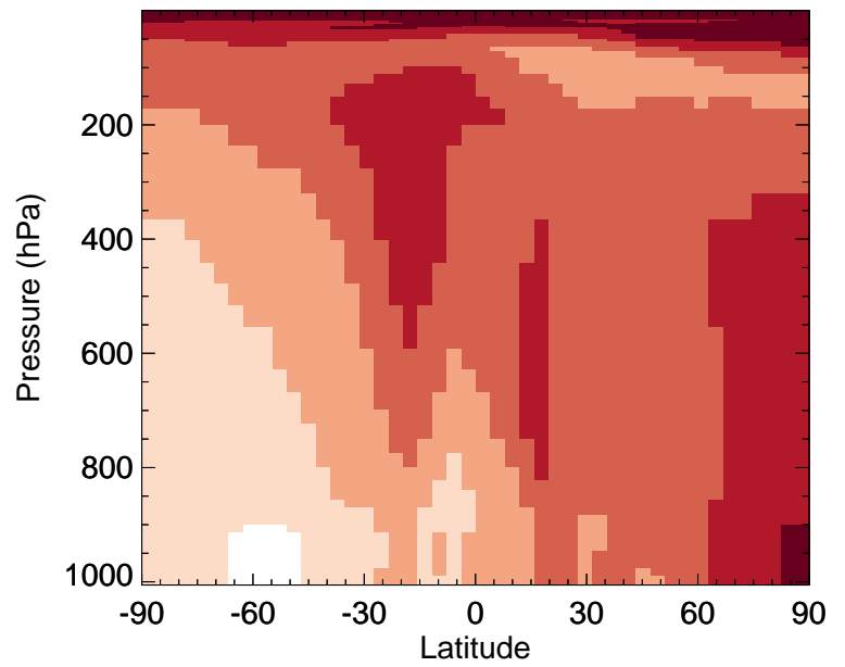
v11-02f-Run0 / v11-02e-Run1 ACET - Zonal mean % diff for Jul
