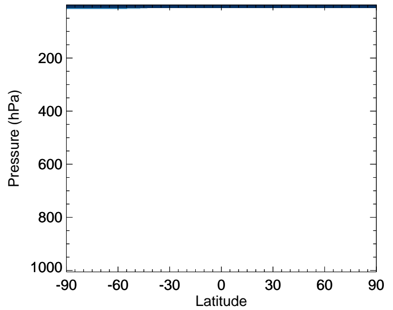
v11-02f-Run0 / v11-02e-Run1 CH3Cl - Zonal mean % diff for Jul
