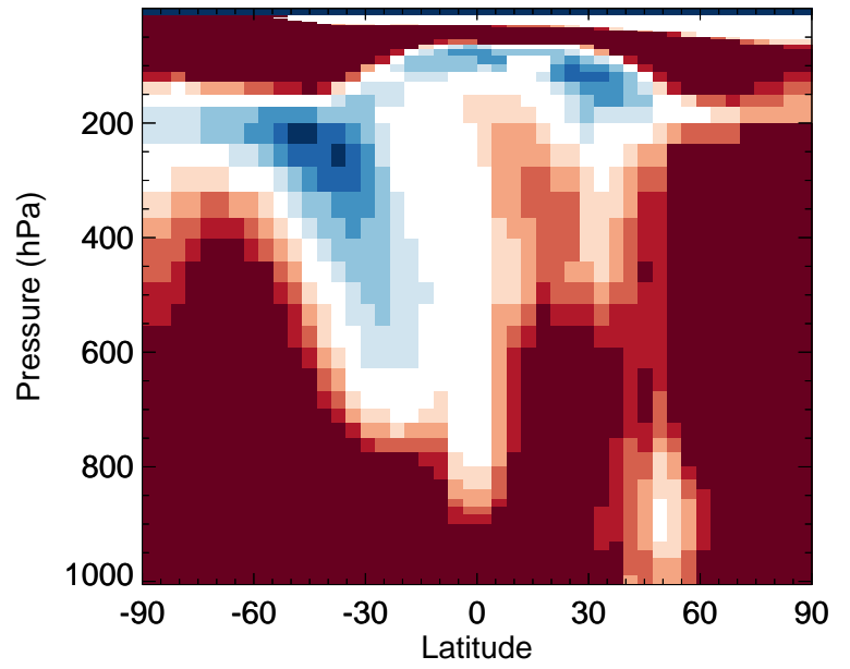
v11-02f-Run0 / v11-02e-Run1 HAC - Zonal mean % diff for Jul
