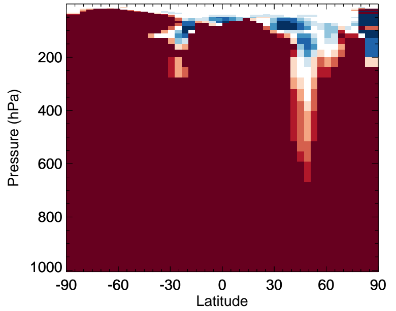
v11-02f-Run0 / v11-02e-Run1 MOBA - Zonal mean % diff for Jul
