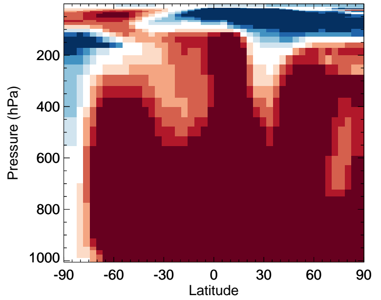
v11-02f-Run0 / v11-02e-Run1 HONIT - Zonal mean % diff for Jul
