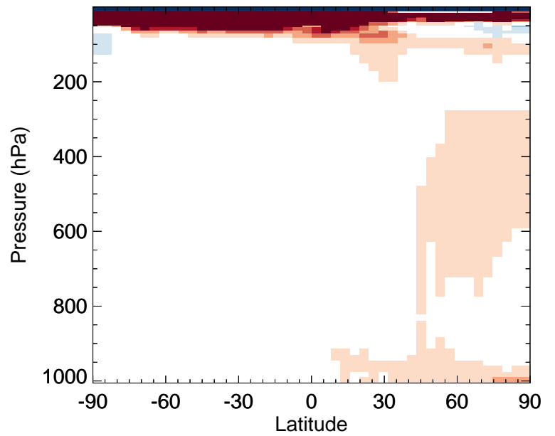
v11-02f-Run0 / v11-02e-Run0 CH2Br2 - Zonal mean % diff for Jul
