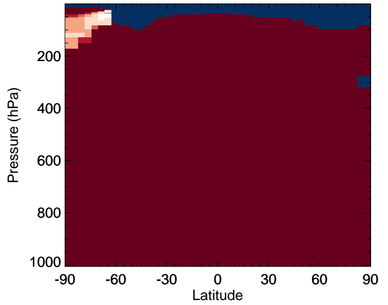
v11-02f-Run0 / v11-02e-Run1 NIT - Zonal mean % diff for Jul
