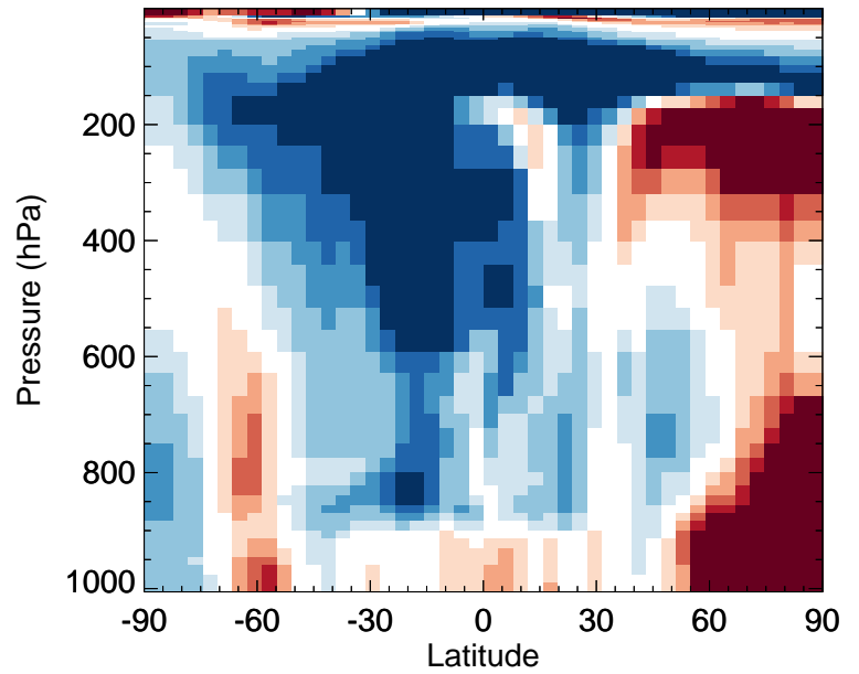
v11-02f-Run0 / v11-02e-Run0 SO4 - Zonal mean % diff for Jul
