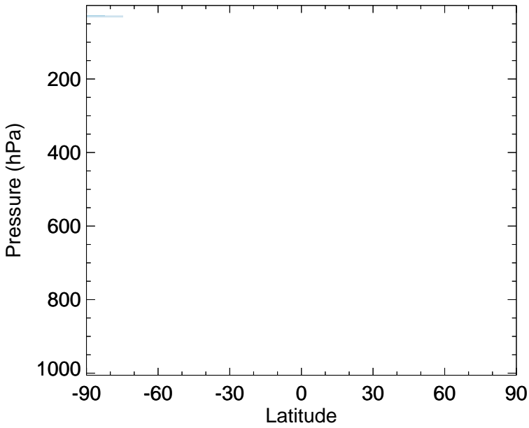
v11-02f-Run0 - v11-02e-Run1 CINO2 - Zonal mean abs diff for Jul
