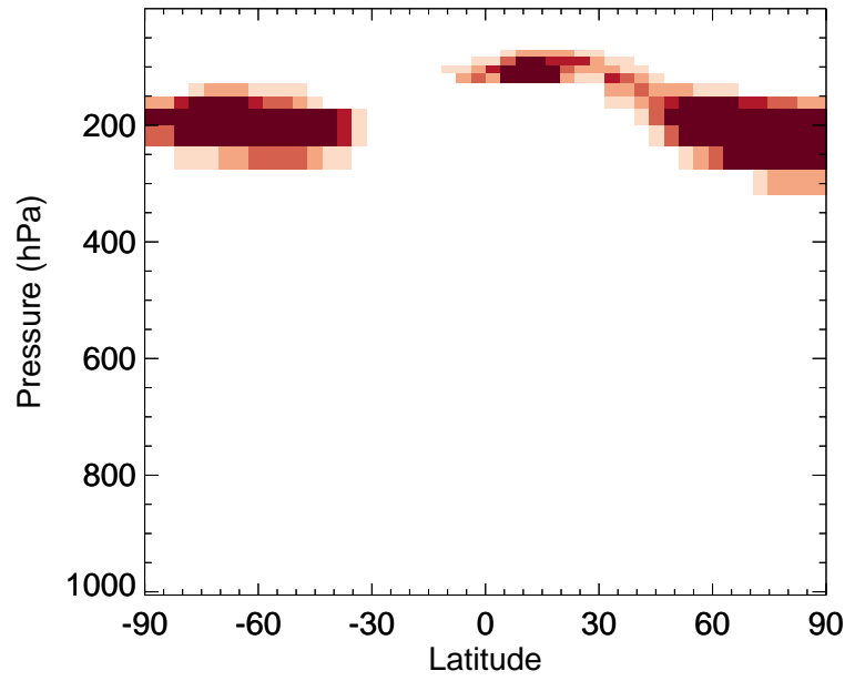
v11-02f-Run0 / v11-02e-Run1 H2O - Zonal mean % diff for Jul
