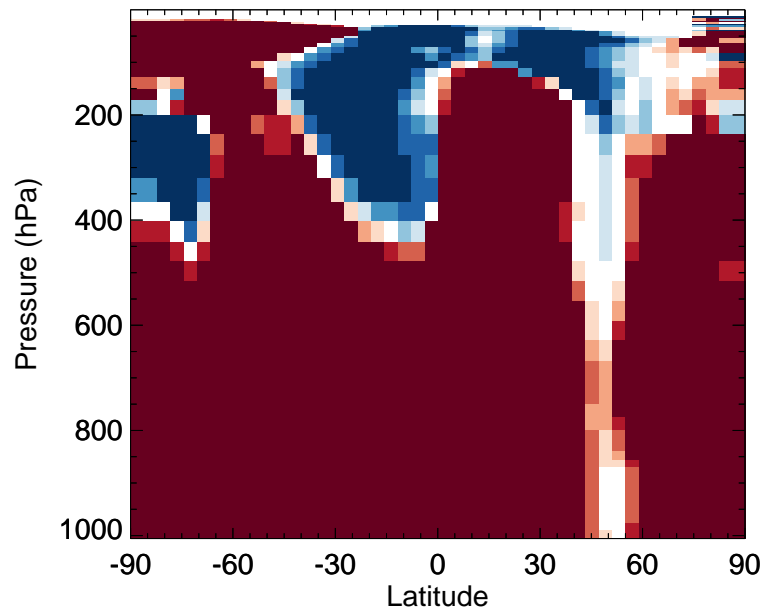
v11-02f-Run0 / v11-02e-Run1 LVOC - Zonal mean % diff for Jul
