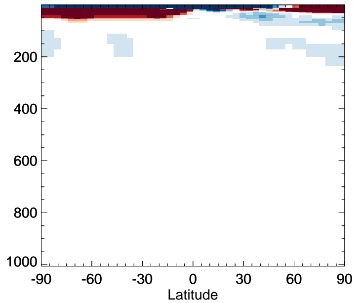
v11-02f-Run0 / v11-02e-Run0 CFC11 - Zonal mean % diff for Jul
