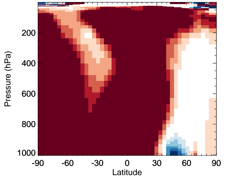
v11-02f-Run0 / v11-02e-Run1 OCPO - Zonal mean % diff for Jul
