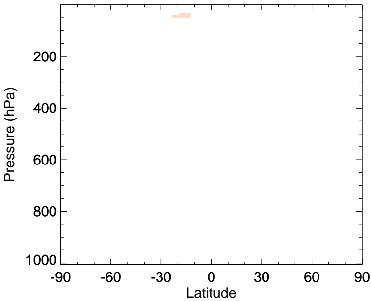
v11-02f-Run0 - v11-02e-Run0 CFC11 - Zonal mean abs diff for Jul
