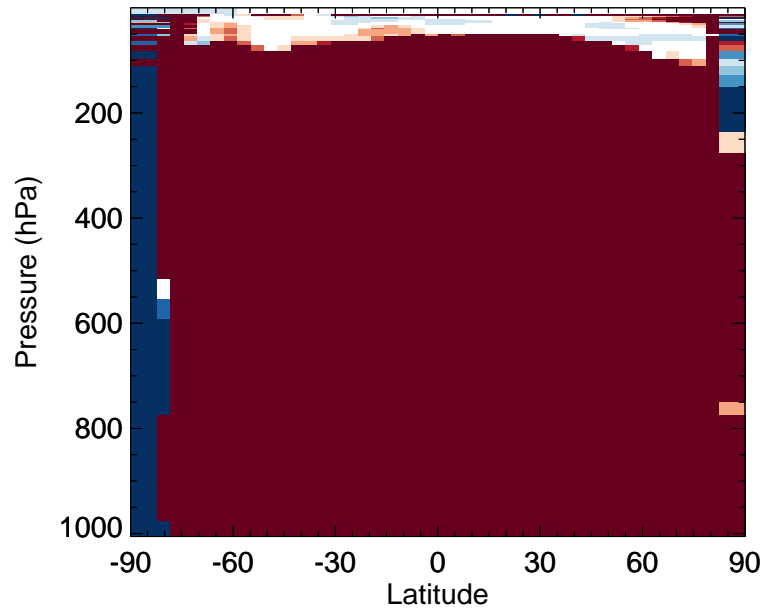
v11-02f-Run0 / v11-02e-Run0 LIMO - Zonal mean % diff for Jul
