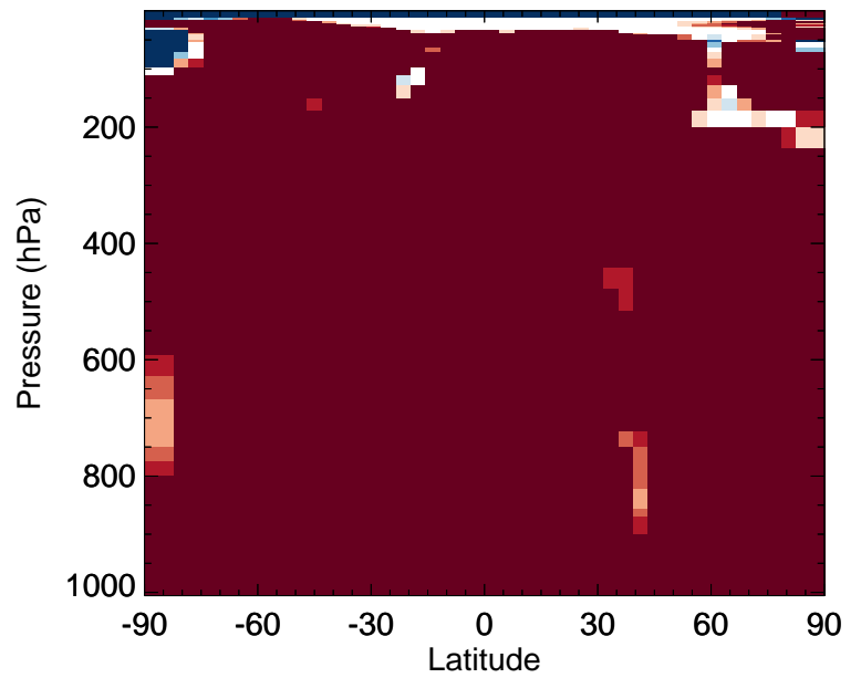
v11-02f-Run0 / v11-02e-Run0 PRPE - Zonal mean % diff for Jul
