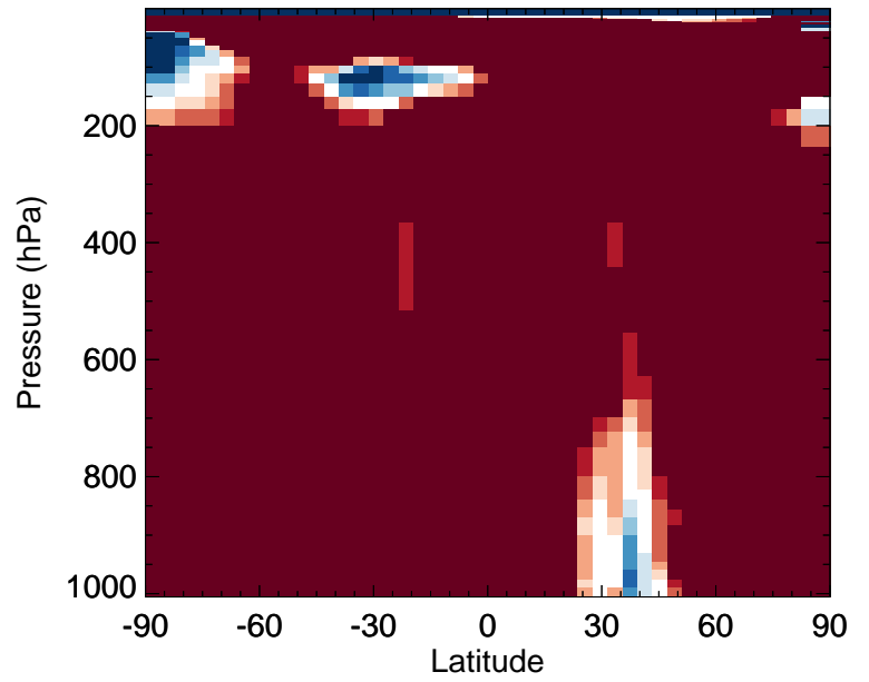
v11-02f-Run0 / v11-02e-Run0 ALK4 - Zonal mean % diff for Jul
