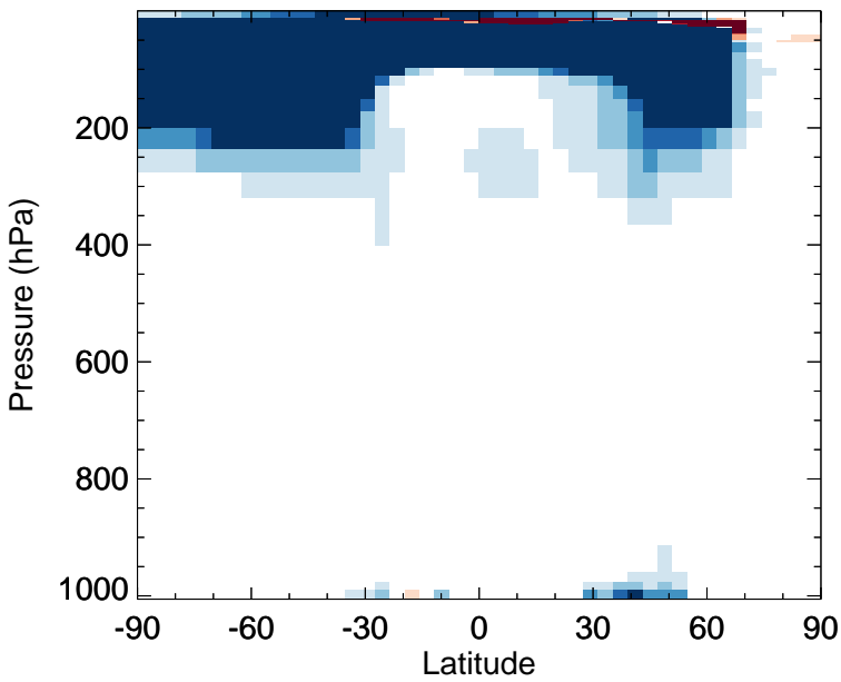
v11-02f-Run0 - v11-02e-Run0 N2O5 - Zonal mean abs diff for Jul
