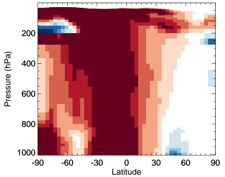
v11-02f-Run0 / v11-02e-Run1 NITs - Zonal mean % diff for Jul
