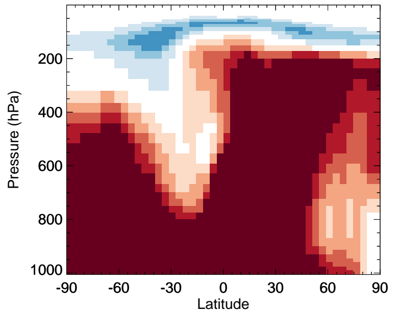
v11-02f-Run0 / v11-02e-Run1 TSOA2 - Zonal mean % diff for Jul
