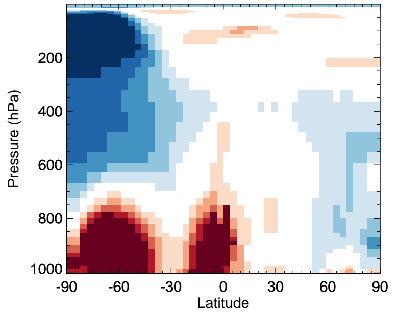
v11-02f-Run0 / v11-02e-Run1 MPN - Zonal mean % diff for Jul
