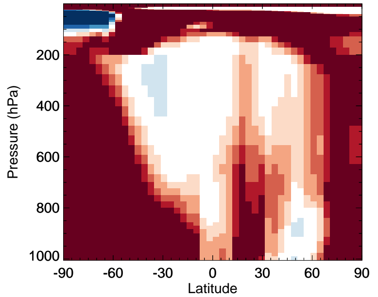
v11-02f-Run0 / v11-02e-Run1 MGLY - Zonal mean % diff for Jul
