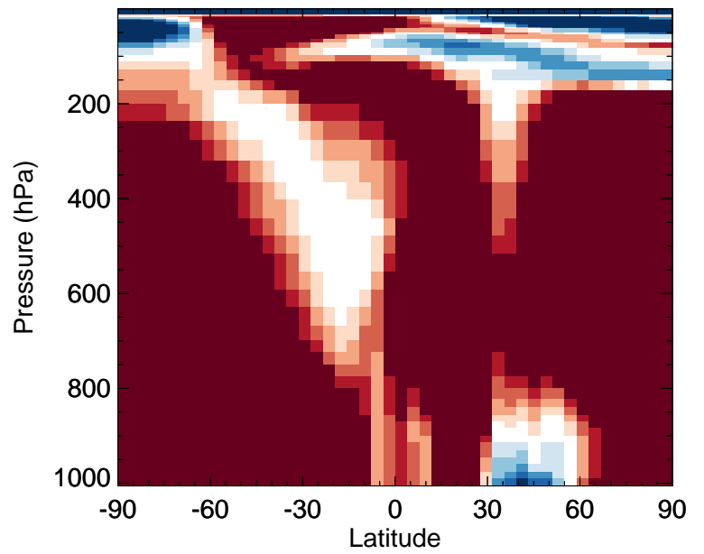
v11-02f-Run0 / v11-02e-Run1 GLYX - Zonal mean % diff for Jul
