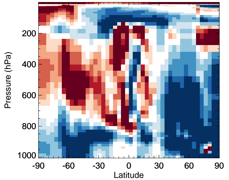
v11-02f-Run0 / v11-02e-Run0 BrCl - Zonal mean % diff for Jul
