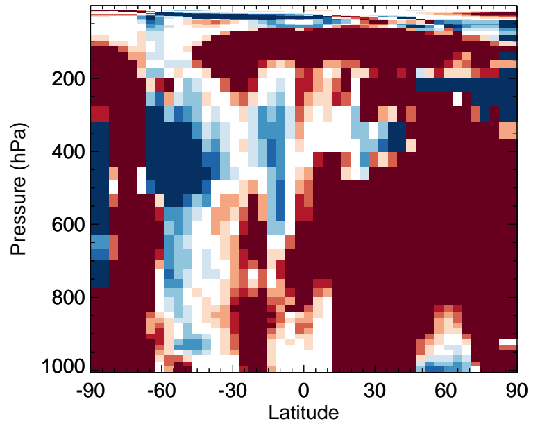
v11-02f-Run0 / v11-02e-Run0 HBr - Zonal mean % diff for Jul
