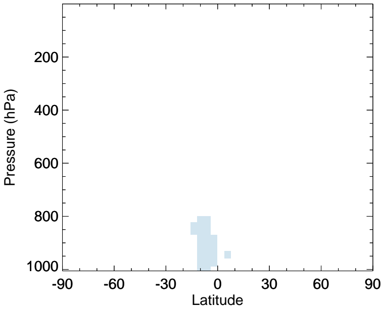
v11-02f-Run0 - v11-02e-Run1 RIPA - Zonal mean abs diff for Jul
