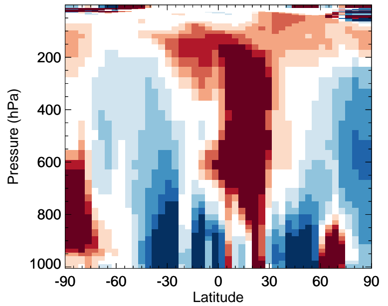
v11-02f-Run0 / v11-02e-Run1 BCPO - Zonal mean % diff for Jul
