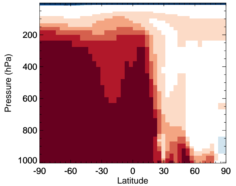
v11-02f-Run0 / v11-02e-Run1 PPN - Zonal mean % diff for Jul
