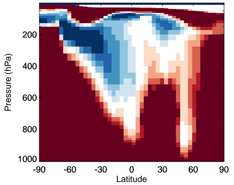
v11-02f-Run0 / v11-02e-Run1 HCOOH - Zonal mean % diff for Jul
