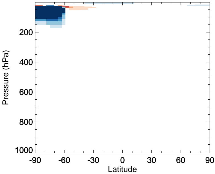
v11-02f-Run0 - v11-02e-Run0 HOCl - Zonal mean abs diff for Jul
