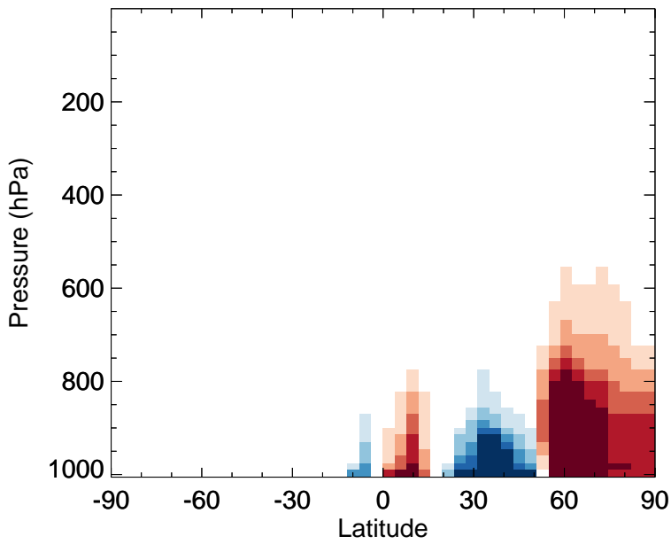
v11-02f-Run0 - v11-02e-Run1 TOLU - Zonal mean abs diff for Jul
