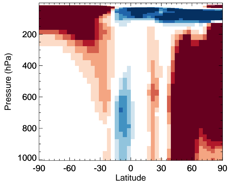
v11-02f-Run0 / v11-02e-Run1 DMS - Zonal mean % diff for Jul
