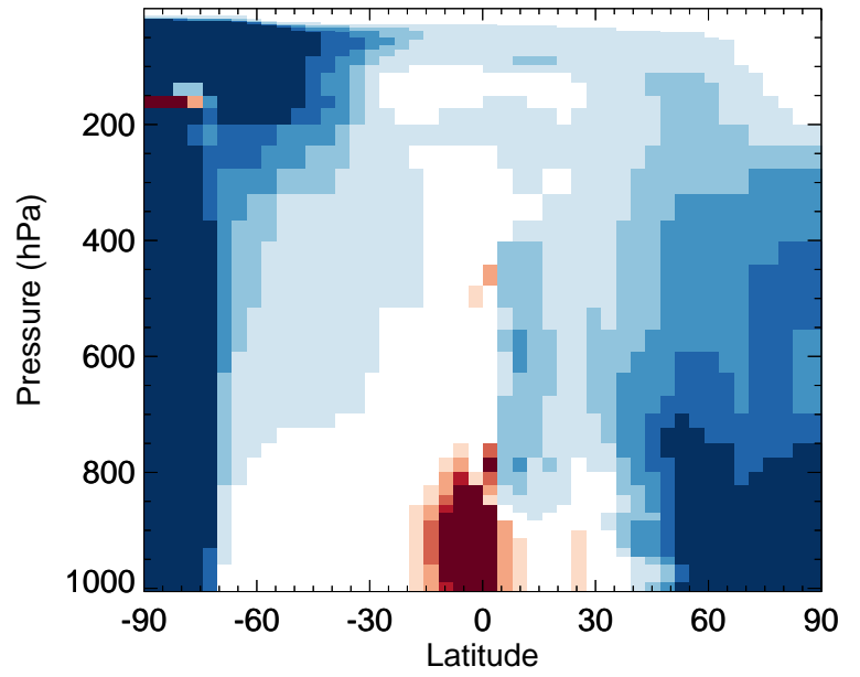
v11-02f-Run0 / v11-02e-Run1 BrNO3 - Zonal mean % diff for Jul
