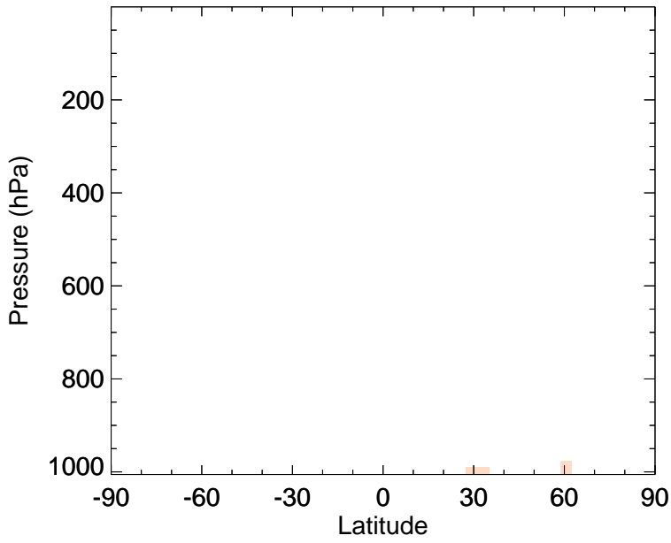
v11-02f-Run0 - v11-02e-Run1 OCPO - Zonal mean abs diff for Jul
