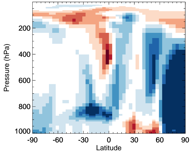
v11-02f-Run0 / v11-02e-Run0 MSA - Zonal mean % diff for Jul
