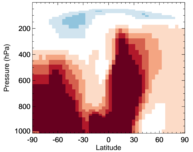
v11-02f-Run0 / v11-02e-Run1 ISOA2 - Zonal mean % diff for Jul
