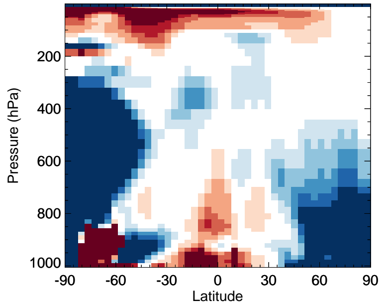
v11-02f-Run0 / v11-02e-Run1 HNO 3 - Zonal mean % diff for Jul
