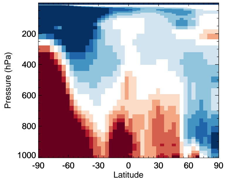
v11-02f-Run0 / v11-02e-Run1 HNO 2 - Zonal mean % diff for Jul
