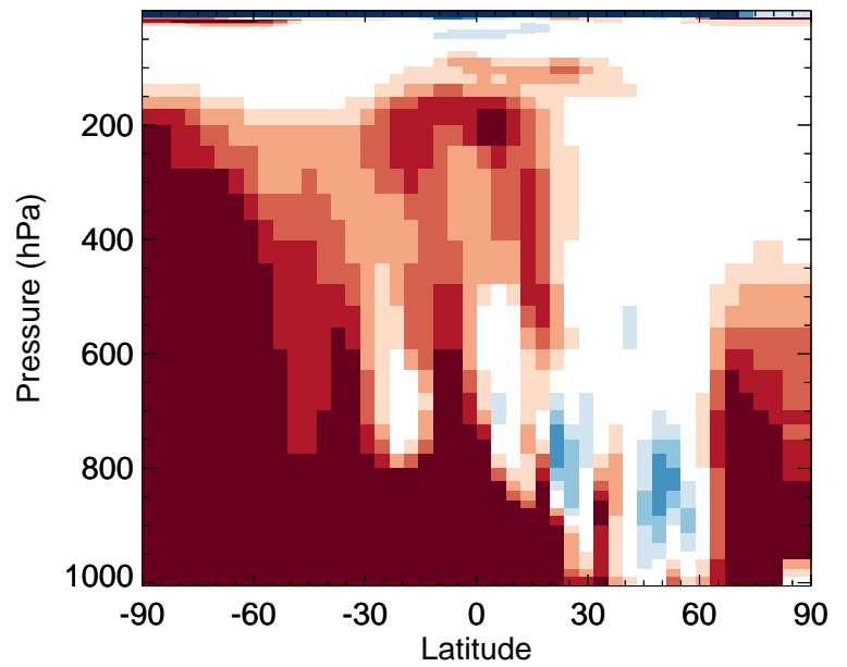
v11-02f-Run0 / v11-02e-Run0 PPN - Zonal mean % diff for Jul
