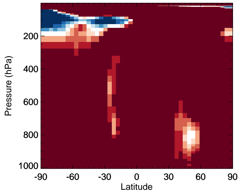
v11-02f-Run0 / v11-02e-Run0 MEK - Zonal mean % diff for Jul
