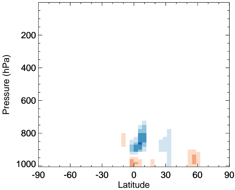
v11-02f-Run0 - v11-02e-Run0 MVK - Zonal mean abs diff for Jul
