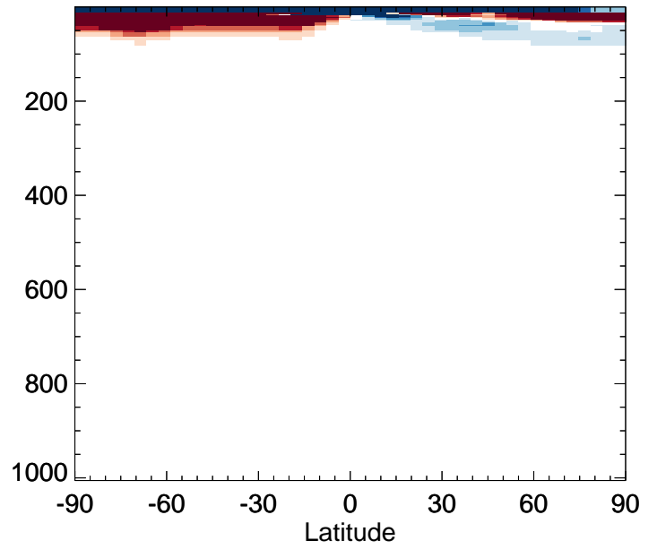
v11-02f-Run0 / v11-02e-Run0 OCS - Zonal mean % diff for Jul
