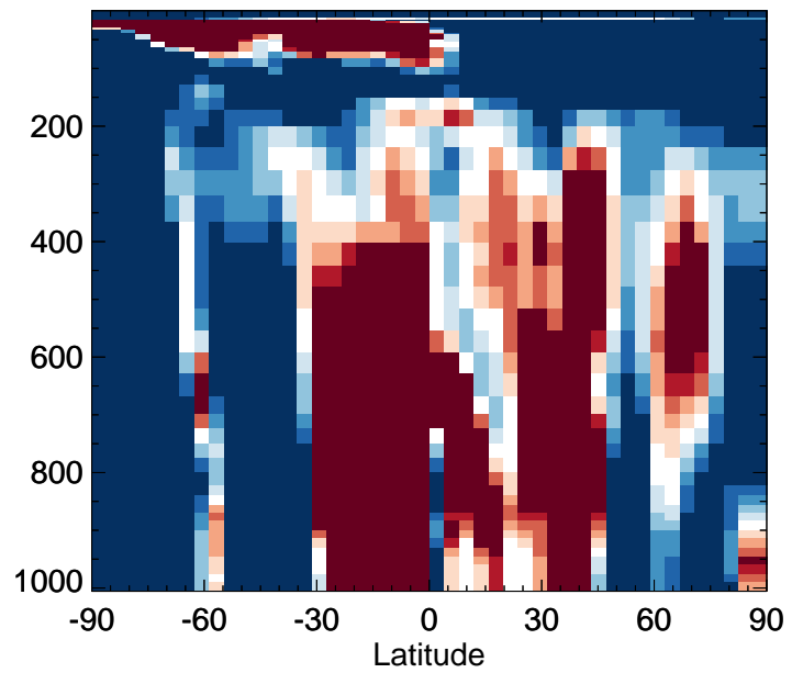
v11-02f-Run0 / v11-02e-Run0 DST2 - Zonal mean % diff for Jul
