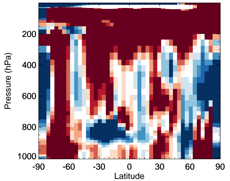
v11-02f-Run0 / v11-02e-Run0 NITs - Zonal mean % diff for Jul
