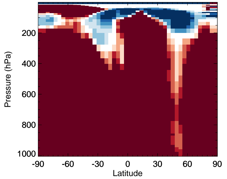
v11-02f-Run0 / v11-02e-Run1 MVK - Zonal mean % diff for Jul
