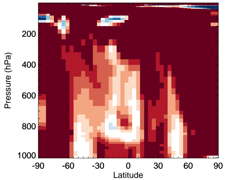
v11-02f-Run0 / v11-02e-Run0 ACTA - Zonal mean % diff for Jul
