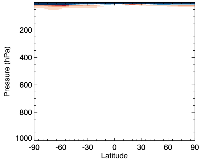
v11-02f-Run0 / v11-02e-Run0 CFC114 - Zonal mean % diff for Jul
