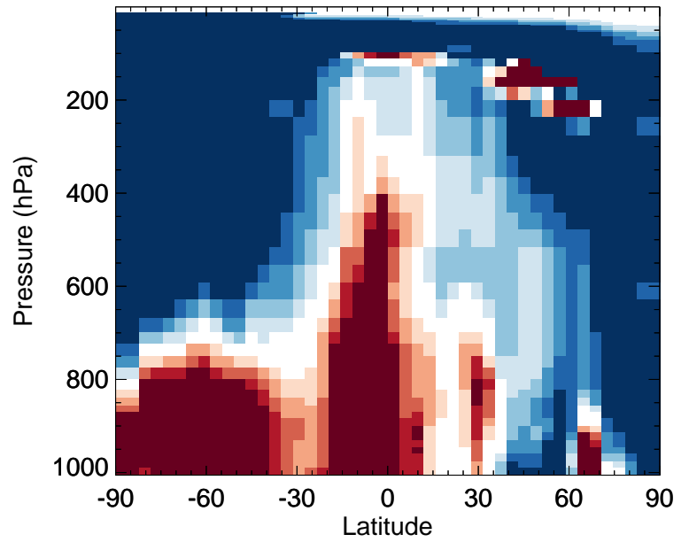
v11-02f-Run0 / v11-02e-Run1 CINO2 - Zonal mean % diff for Jul
