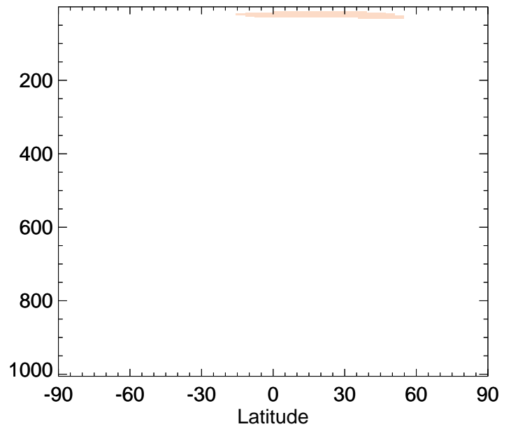
v11-02f-Run0 / v11-02e-Run1 CH3Br - Zonal mean % diff for Jul
