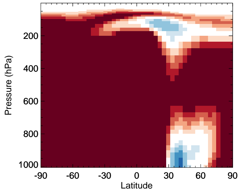
v11-02f-Run0 / v11-02e-Run1 ASOA1 - Zonal mean % diff for Jul
