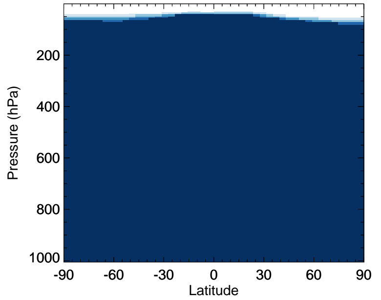
v11-02f-Run0 / v11-02e-Run1 SOAIE - Zonal mean % diff for Jul
