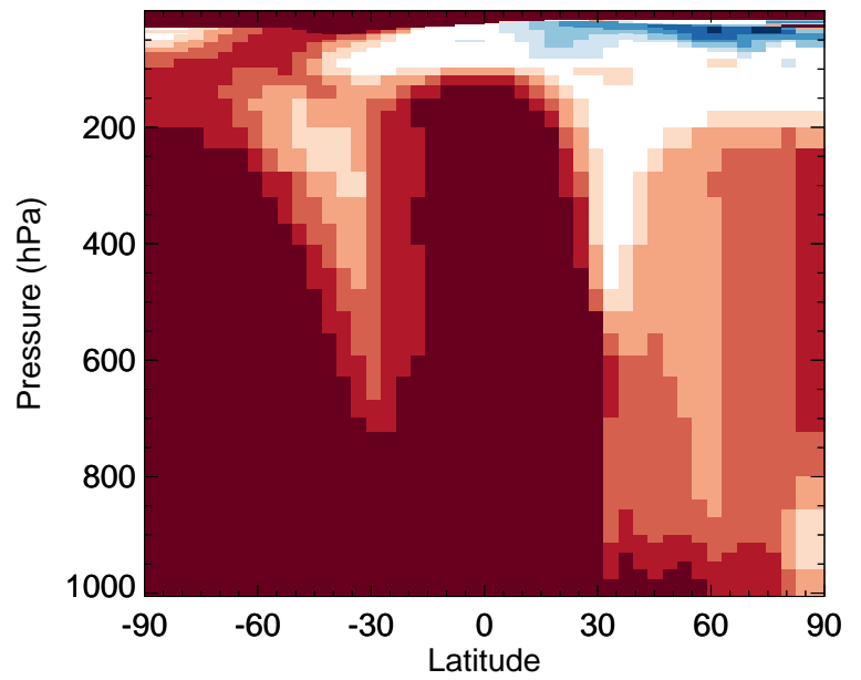
v11-02f-Run0 / v11-02e-Run1 MEK - Zonal mean % diff for Jul
