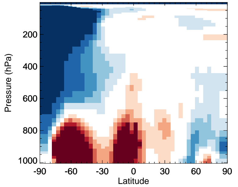
v11-02f-Run0 / v11-02e-Run1 HNO 4 - Zonal mean % diff for Jul
