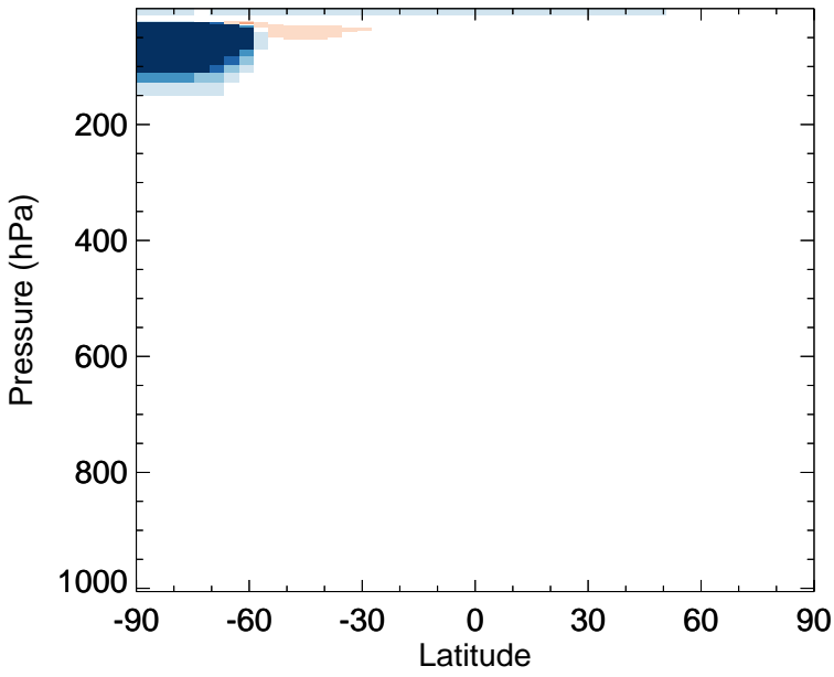
v11-02f-Run0 - v11-02e-Run1 HOCl - Zonal mean abs diff for Jul
