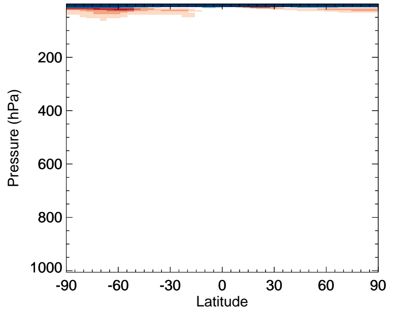
v11-02f-Run0 / v11-02e-Run0 CH4 - Zonal mean % diff for Jul
