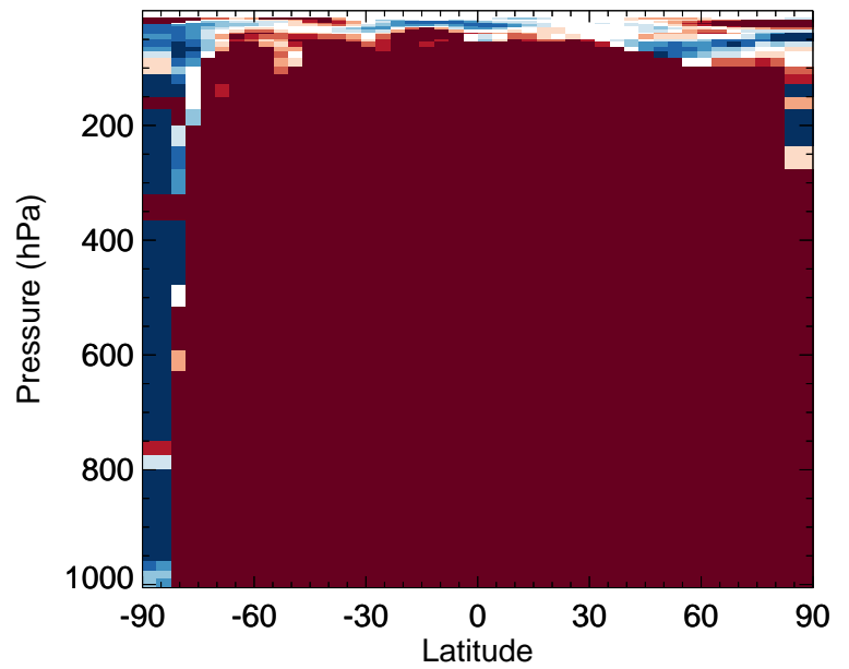
v11-02f-Run0 / v11-02e-Run0 MTPO - Zonal mean % diff for Jul
