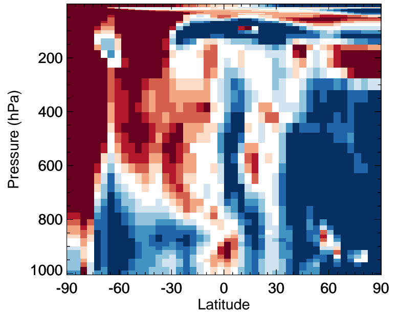
v11-02f-Run0 / v11-02e-Run0 ClO - Zonal mean % diff for Jul
