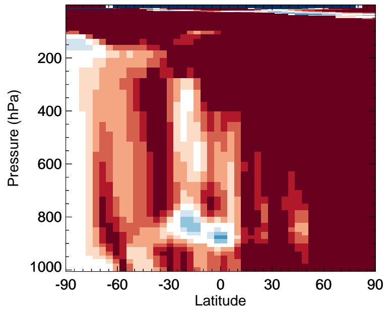
v11-02f-Run0 / v11-02e-Run0 ALD2 - Zonal mean % diff for Jul
