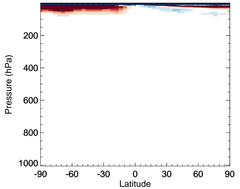
v11-02f-Run0 / v11-02e-Run0 CH3Cl - Zonal mean % diff for Jul
