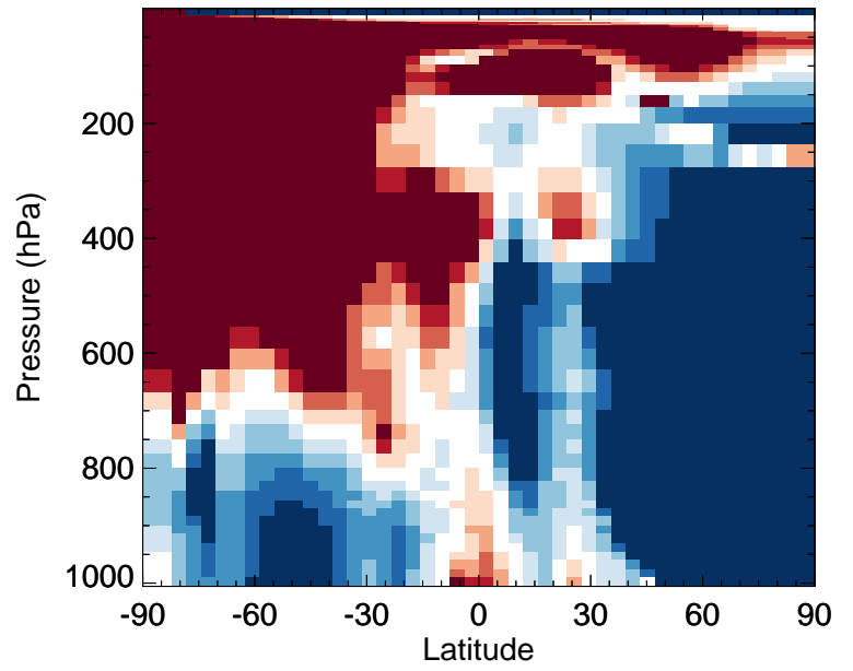
v11-02f-Run0 / v11-02e-Run1 Cl2O2 - Zonal mean % diff for Jul
