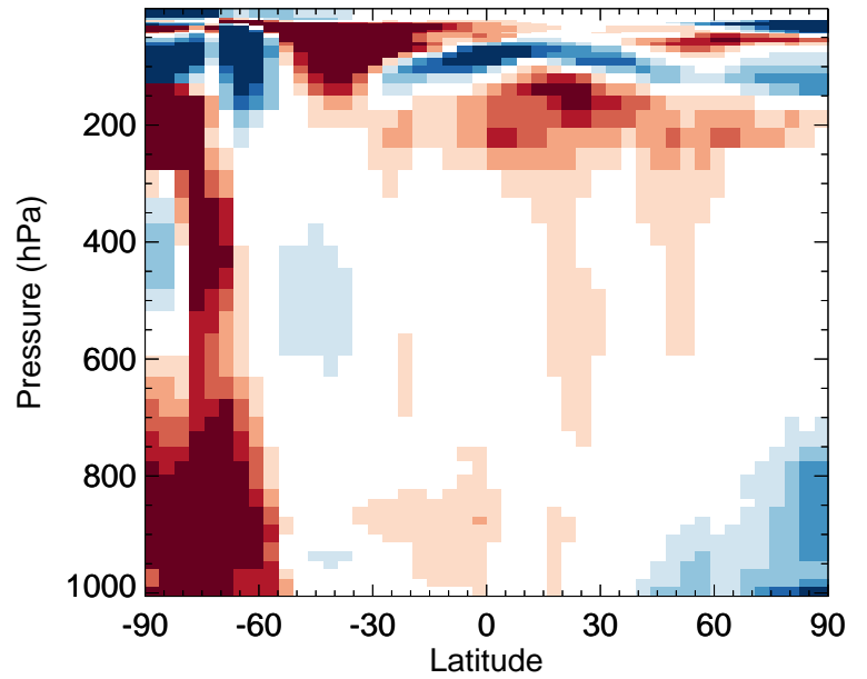
v11-02f-Run0 / v11-02e-Run0 HO2 - Zonal mean % diff for Jul
