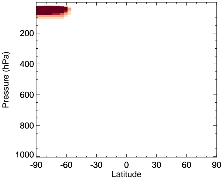
v11-02f-Run0 - v11-02e-Run1 Cl2O2 - Zonal mean abs diff for Jul
