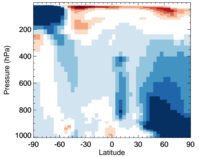
v11-02f-Run0 / v11-02e-Run1 HOBr - Zonal mean % diff for Jul
