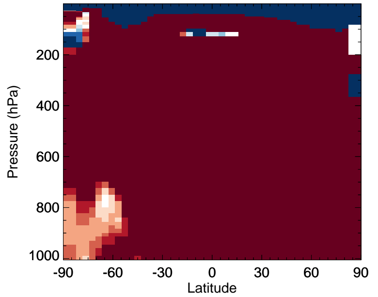
v11-02f-Run0 / v11-02e-Run0 NIT - Zonal mean % diff for Jul
