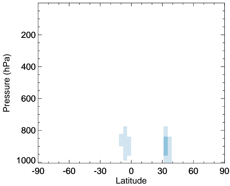
v11-02f-Run0 - v11-02e-Run1 GLYC - Zonal mean abs diff for Jul
