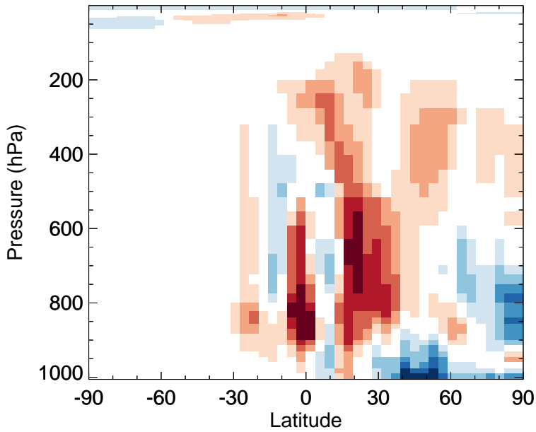
v11-02f-Run0 - v11-02e-Run0 H2O2 - Zonal mean abs diff for Jul
