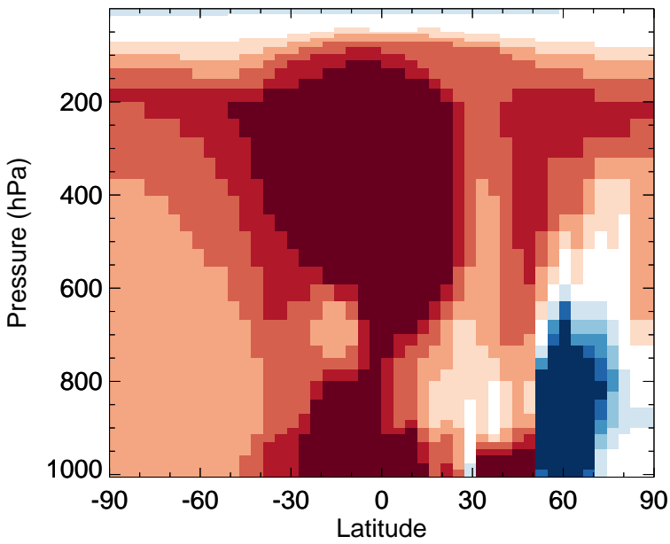
v11-02f-Run0 - v11-02e-Run1 PPN - Zonal mean abs diff for Jul
