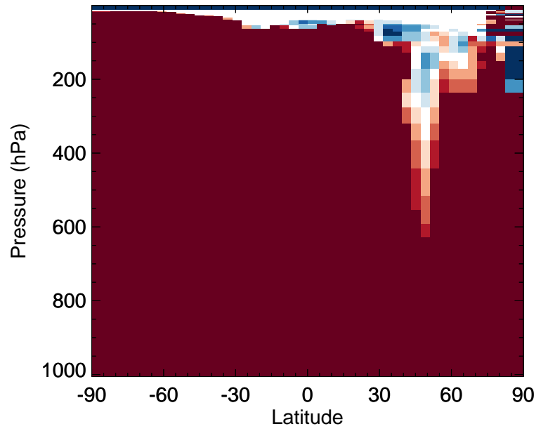
v11-02f-Run0 / v11-02e-Run1 ISOP - Zonal mean % diff for Jul
