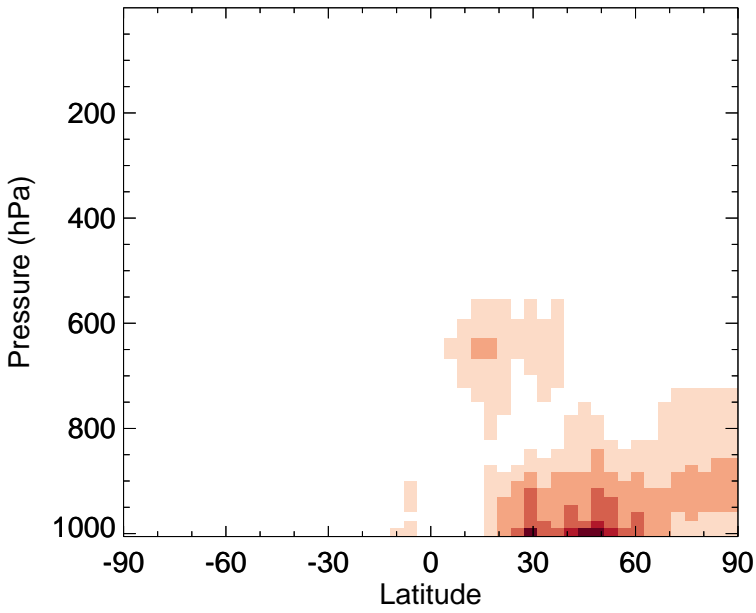
v11-02f-Run0 - v11-02e-Run0 NH4 - Zonal mean abs diff for Jul
