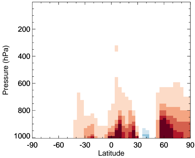
v11-02f-Run0 - v11-02e-Run0 ALK4 - Zonal mean abs diff for Jul
