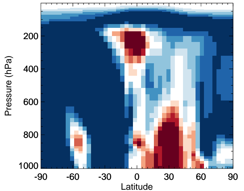
v11-02f-Run0 / v11-02e-Run0 ISN1OA - Zonal mean % diff for Oct
