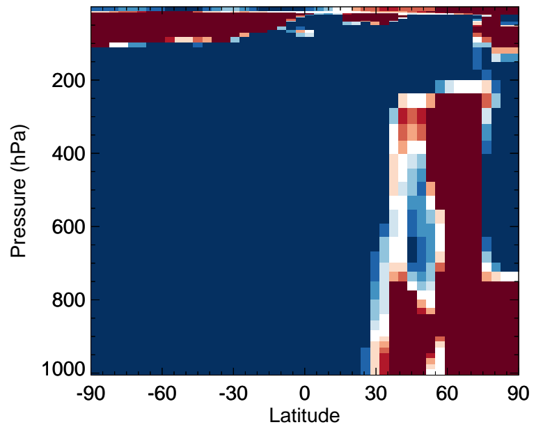
v11-02f-Run0 / v11-02e-Run0 DST3 - Zonal mean % diff for Oct
