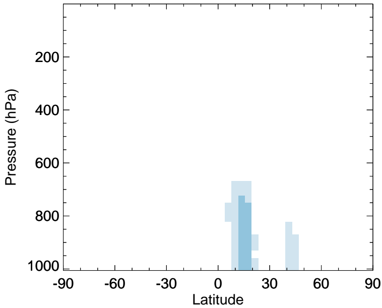
v11-02f-Run0 - v11-02e-Run0 DST1 - Zonal mean abs diff for Oct
