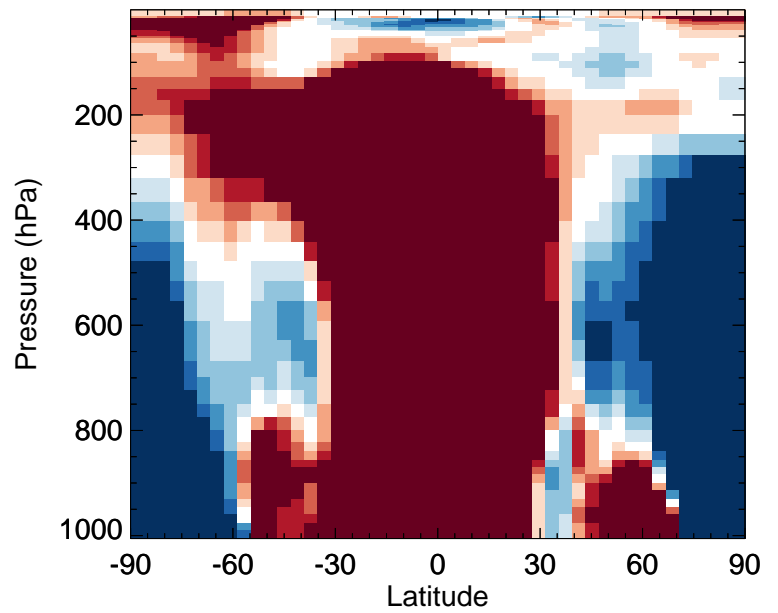
v11-02f-Run0 / v11-02e-Run0 ASOA1 - Zonal mean % diff for Oct
