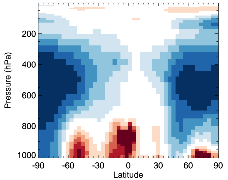
v11-02f-Run0 / v11-02e-Run1 MPN - Zonal mean % diff for Oct
