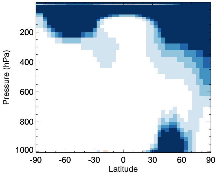
v11-02f-Run0 - v11-02e-Run1 N2O5 - Zonal mean abs diff for Oct
