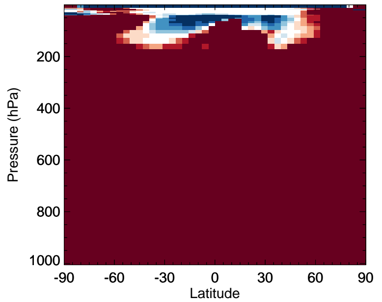
v11-02f-Run0 / v11-02e-Run1 MVK - Zonal mean % diff for Oct
