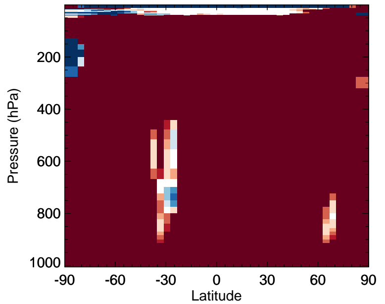
v11-02f-Run0 / v11-02e-Run0 MVK - Zonal mean % diff for Oct
