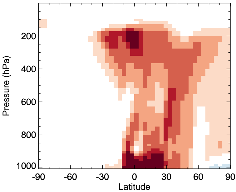
v11-02f-Run0 - v11-02e-Run0 ACET - Zonal mean abs diff for Oct
