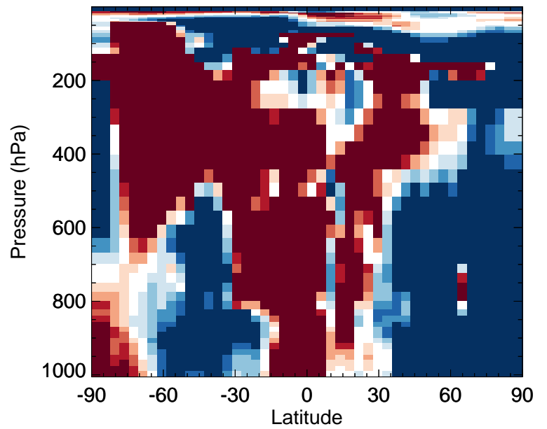
v11-02f-Run0 / v11-02e-Run0 Cl2 - Zonal mean % diff for Oct
