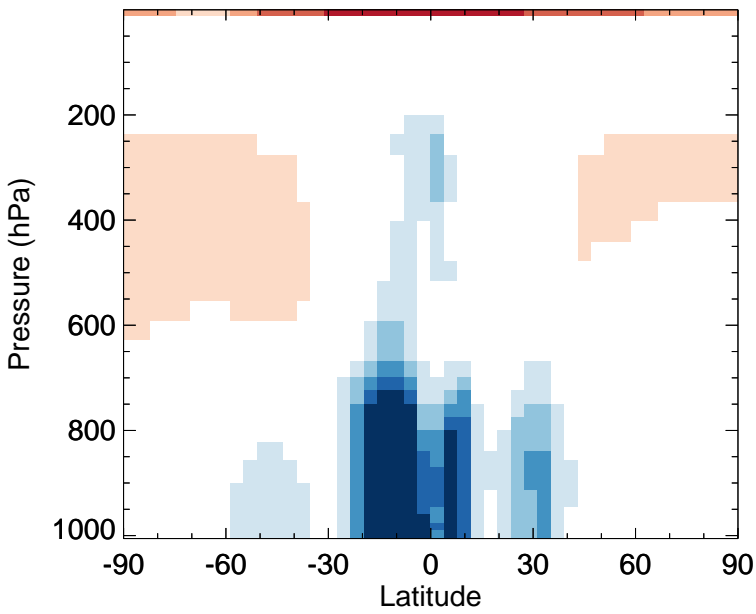
v11-02f-Run0 - v11-02e-Run1 MP - Zonal mean abs diff for Oct
