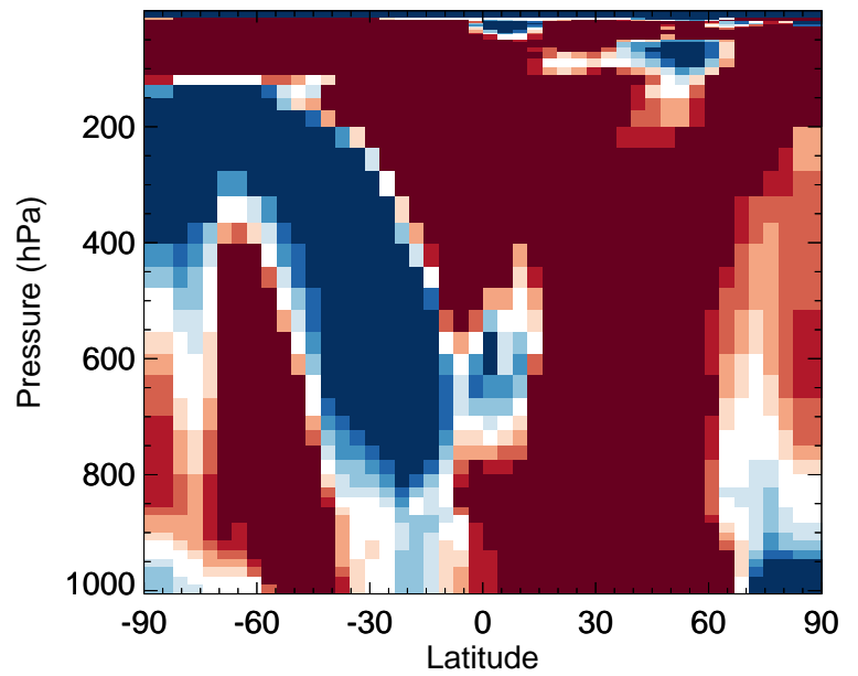
v11-02f-Run0 / v11-02e-Run0 IMAE - Zonal mean % diff for Oct
