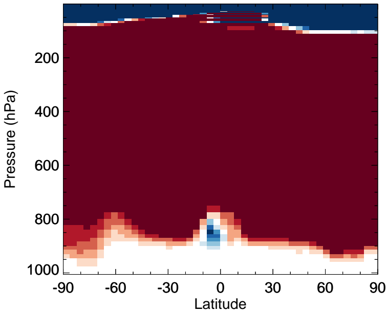
v11-02f-Run0 - v11-02e-Run1 CH4 - Zonal mean abs diff for Oct
