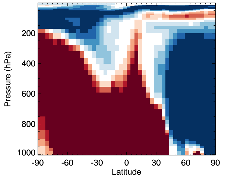
v11-02f-Run0 / v11-02e-Run1 HONIT - Zonal mean % diff for Oct
