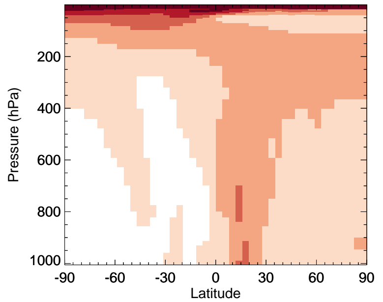
v11-02f-Run0 / v11-02e-Run1 ACET - Zonal mean % diff for Oct
