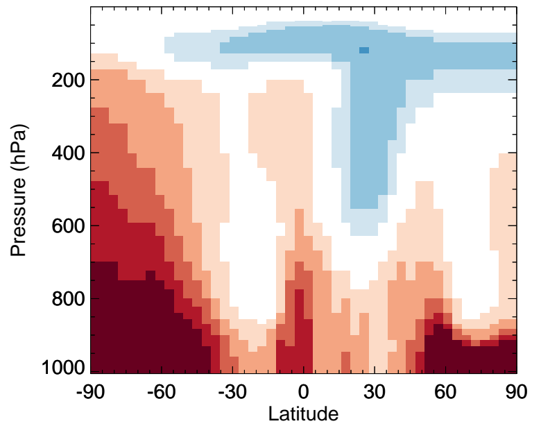
v11-02f-Run0 / v11-02e-Run1 SOAGX - Zonal mean % diff for Oct
