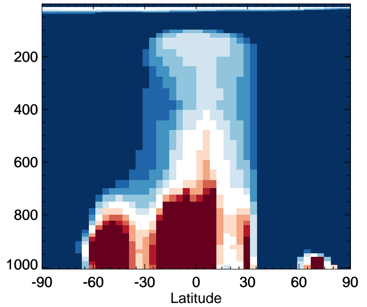
v11-02f-Run0 / v11-02e-Run1 N2O5 - Zonal mean % diff for Oct
