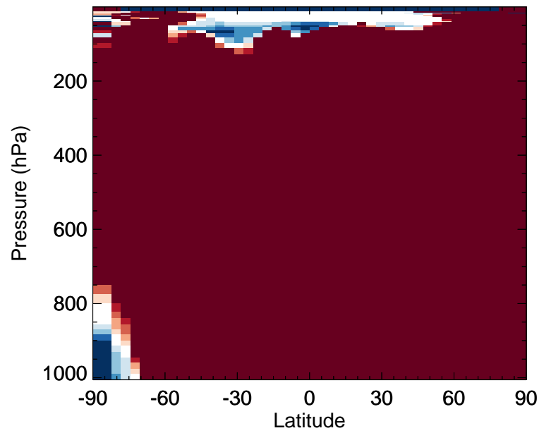
v11-02f-Run0 / v11-02e-Run1 ISOP - Zonal mean % diff for Oct
