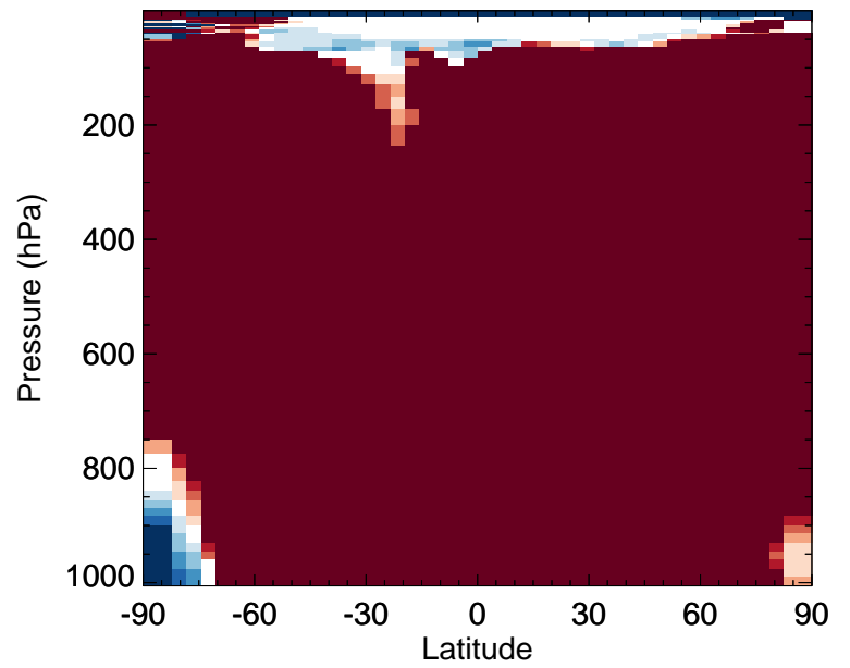
v11-02f-Run0 / v11-02e-Run1 RIPD - Zonal mean % diff for Oct
