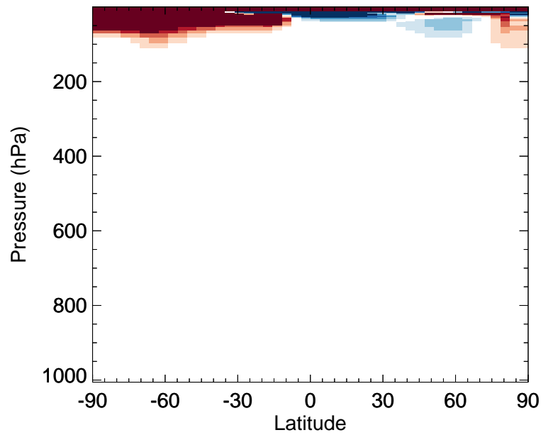
v11-02f-Run0 / v11-02e-Run0 OCS - Zonal mean % diff for Oct
