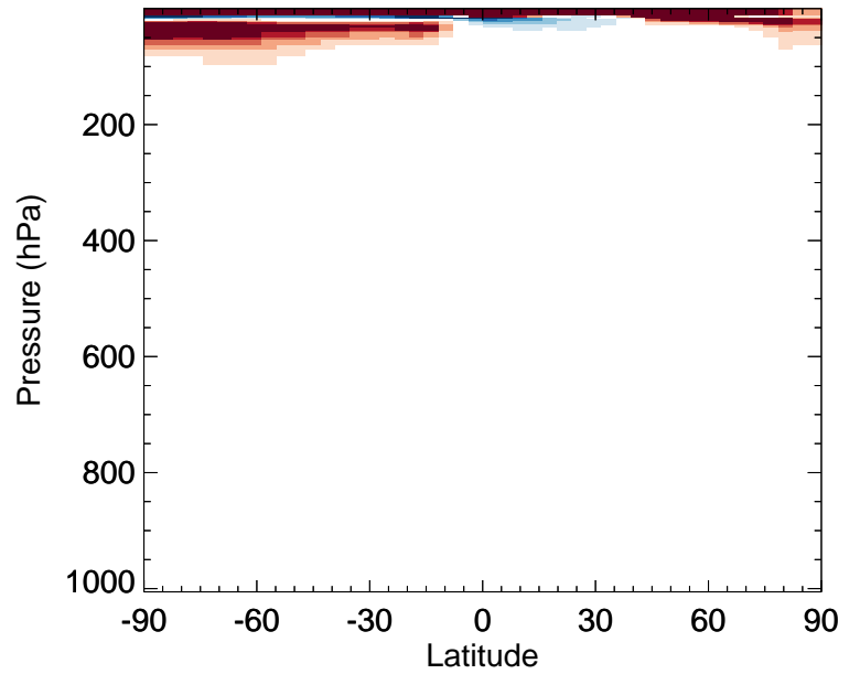
v11-02f-Run0 / v11-02e-Run0 N2O - Zonal mean % diff for Oct
