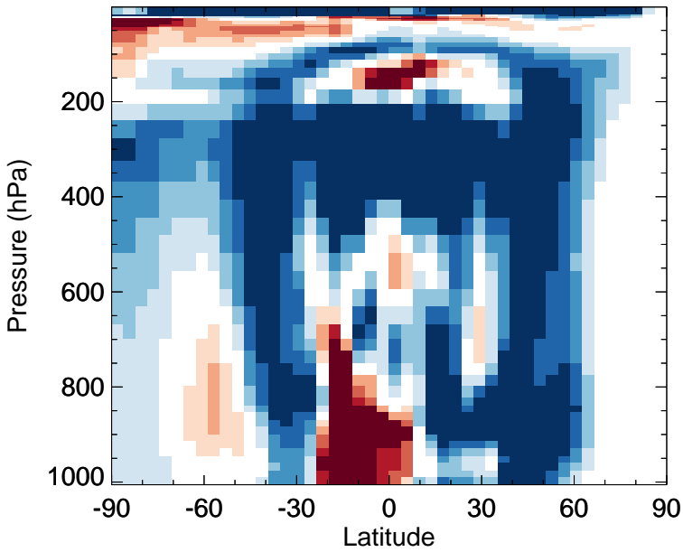
v11-02f-Run0 - v11-02e-Run0 OH - Zonal mean abs diff for Oct
