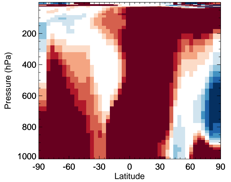
v11-02f-Run0 / v11-02e-Run1 OCPO - Zonal mean % diff for Oct
