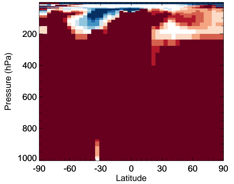
v11-02f-Run0 / v11-02e-Run1 PRPE - Zonal mean % diff for Oct
