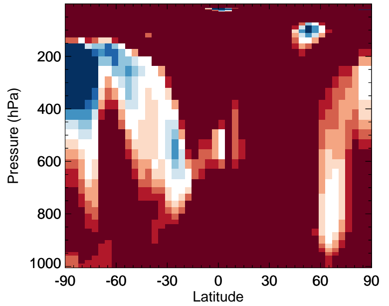
v11-02f-Run0 / v11-02e-Run0 MEK - Zonal mean % diff for Oct
