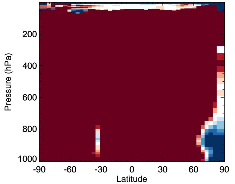
v11-02f-Run0 / v11-02e-Run0 RIPA - Zonal mean % diff for Oct
