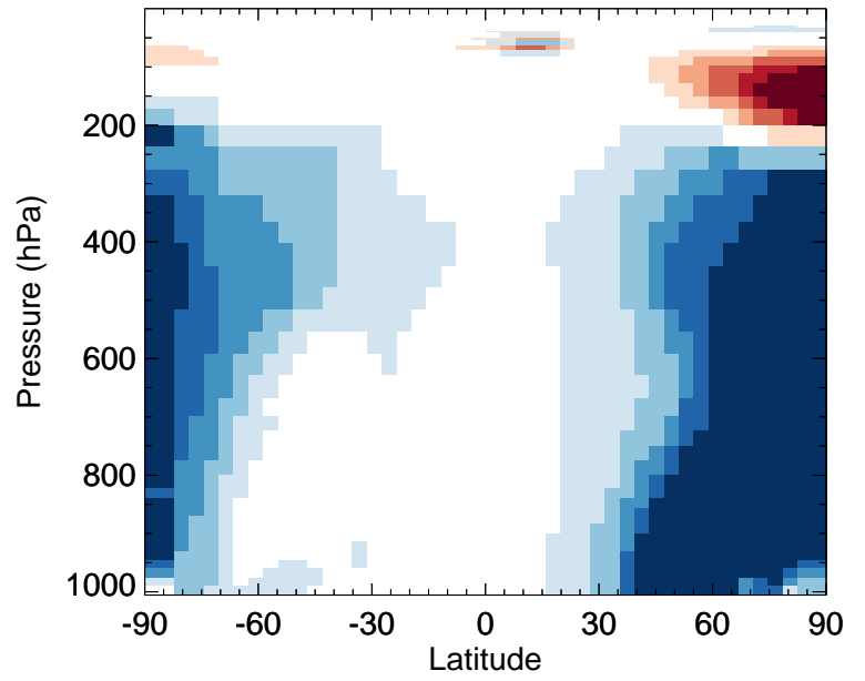
v11-02f-Run0 / v11-02e-Run1 HCl - Zonal mean % diff for Oct
