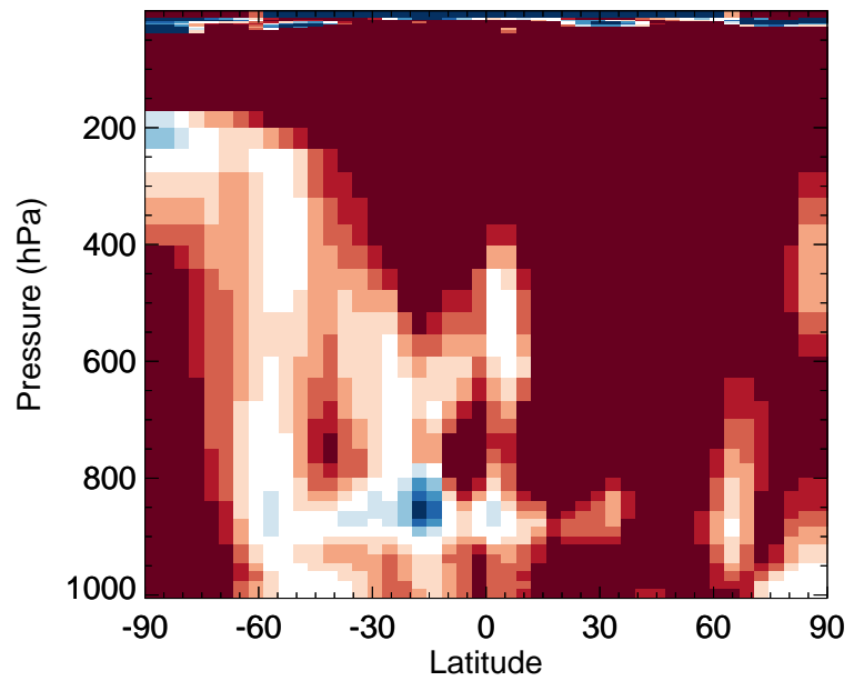
v11-02f-Run0 / v11-02e-Run0 ALD2 - Zonal mean % diff for Oct
