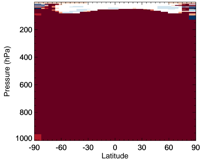
v11-02f-Run0 / v11-02e-Run1 MTPA - Zonal mean % diff for Oct
