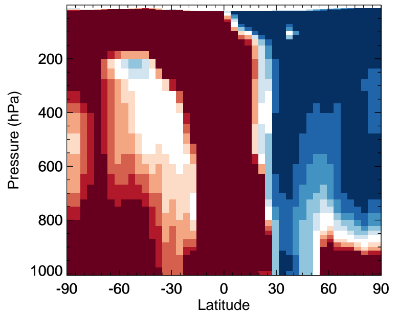
v11-02f-Run0 / v11-02e-Run1 TOLU - Zonal mean % diff for Oct
