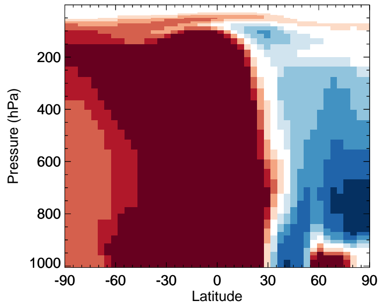
v11-02f-Run0 / v11-02e-Run1 ASOA1 - Zonal mean % diff for Oct
