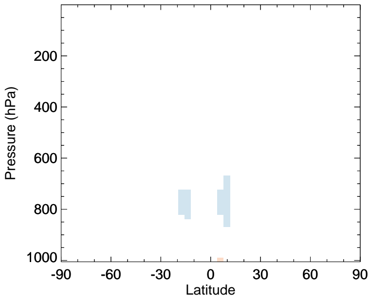
v11-02f-Run0 - v11-02e-Run0 HAC - Zonal mean abs diff for Oct
