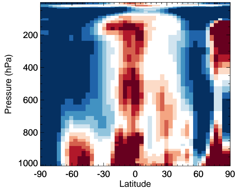
v11-02f-Run0 / v11-02e-Run0 NO 2 - Zonal mean % diff for Oct
