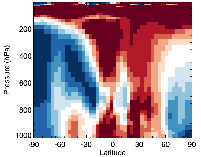
v11-02f-Run0 / v11-02e-Run0 PAN - Zonal mean % diff for Oct
