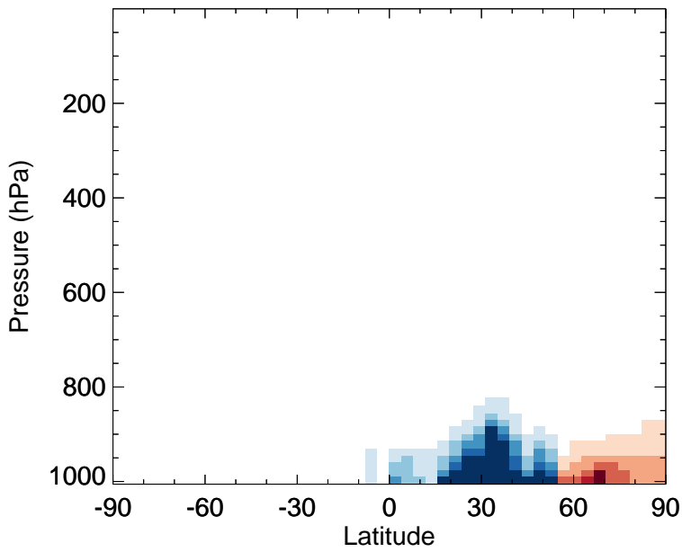
v11-02f-Run0 - v11-02e-Run1 XYLE - Zonal mean abs diff for Oct
