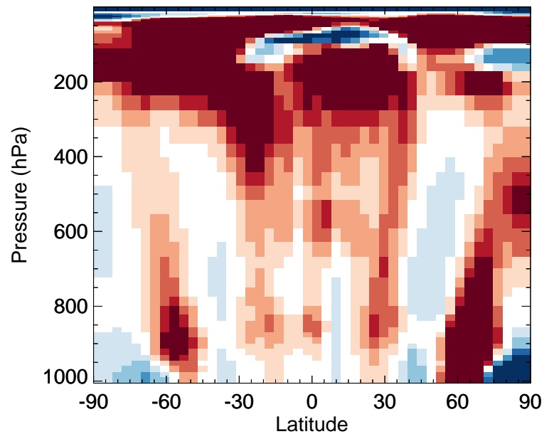
v11-02f-Run0 / v11-02e-Run0 H2O2 - Zonal mean % diff for Oct
