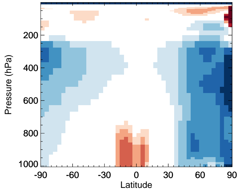
v11-02f-Run0 / v11-02e-Run1 OH - Zonal mean % diff for Oct
