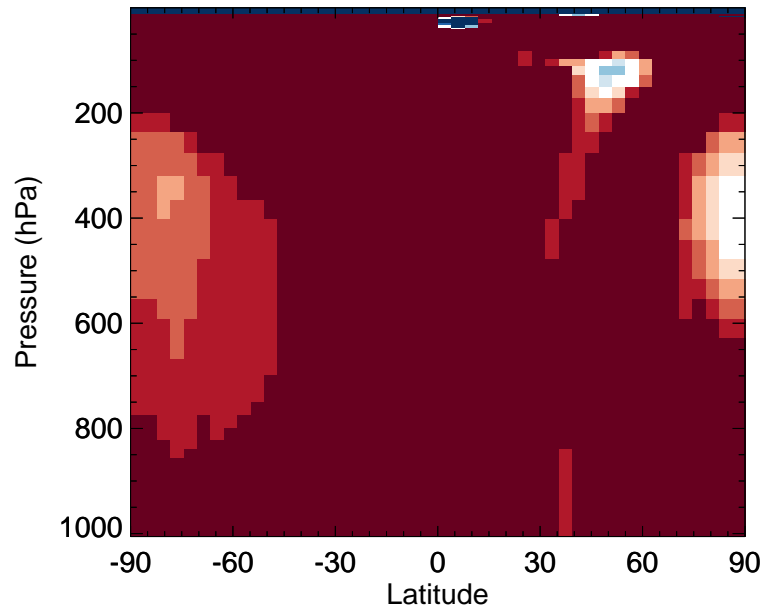
v11-02f-Run0 / v11-02e-Run0 BENZ - Zonal mean % diff for Oct
