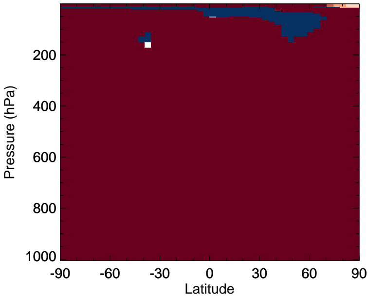
v11-02f-Run0 - v11-02e-Run0 N2O - Zonal mean abs diff for Oct
