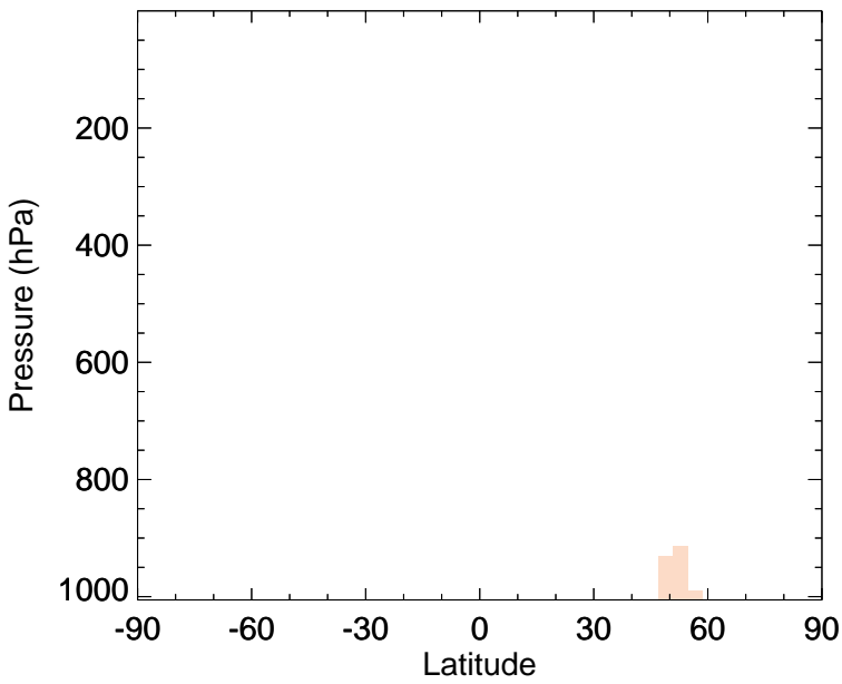
v11-02f-Run0 - v11-02e-Run1 SO4 - Zonal mean abs diff for Oct
