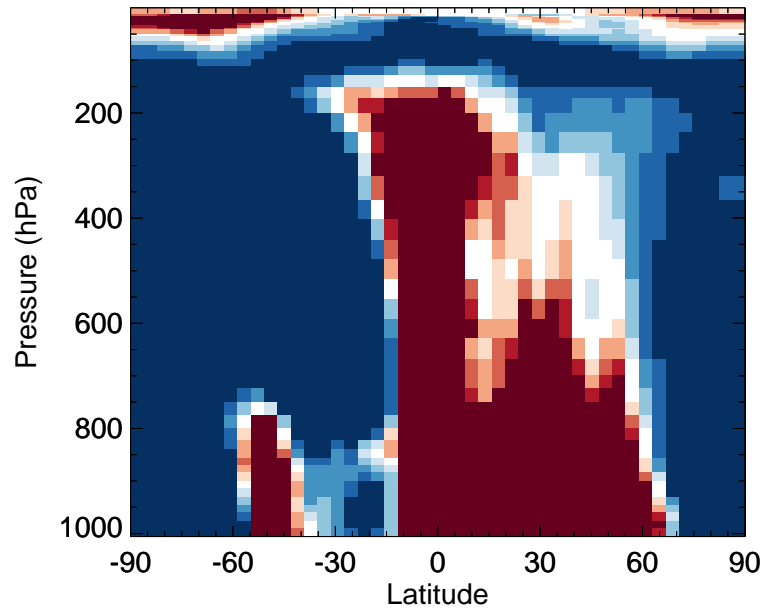
v11-02f-Run0 / v11-02e-Run0 ISOA1 - Zonal mean % diff for Oct
