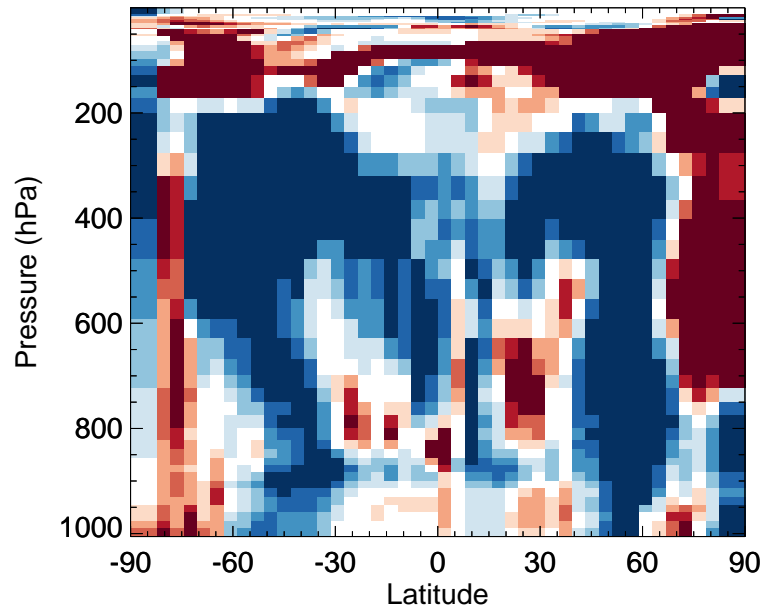
v11-02f-Run0 / v11-02e-Run0 Br2 - Zonal mean % diff for Oct
