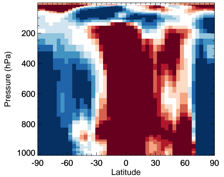
v11-02f-Run0 / v11-02e-Run0 ISOA2 - Zonal mean % diff for Oct
