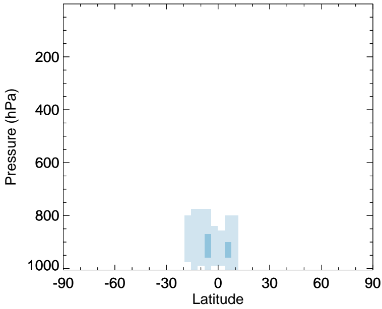
v11-02f-Run0 - v11-02e-Run1 RIPA - Zonal mean abs diff for Oct
