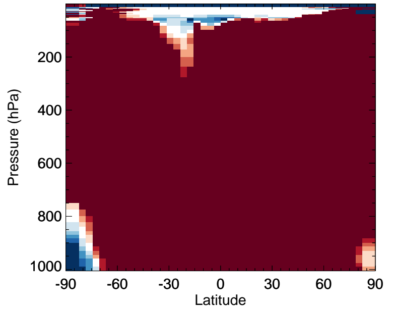
v11-02f-Run0 / v11-02e-Run1 RIPA - Zonal mean % diff for Oct
