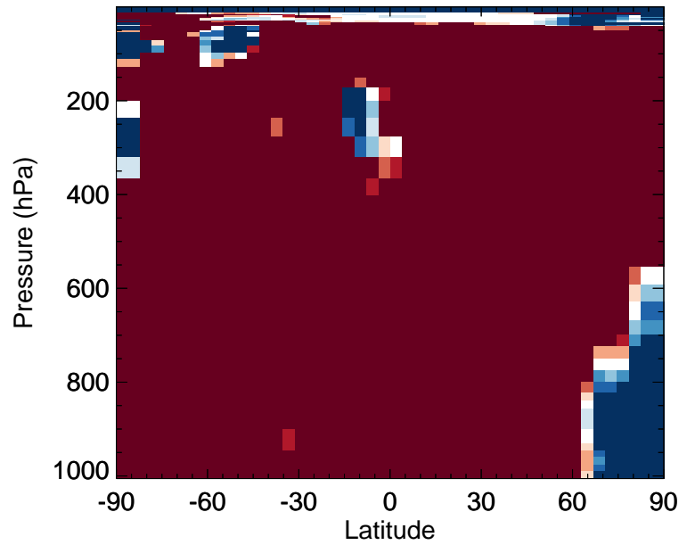
v11-02f-Run0 / v11-02e-Run0 LVOC - Zonal mean % diff for Oct
