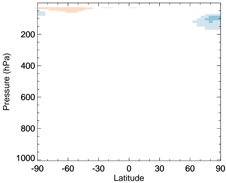
v11-02f-Run0 - v11-02e-Run0 MPN - Zonal mean abs diff for Oct
