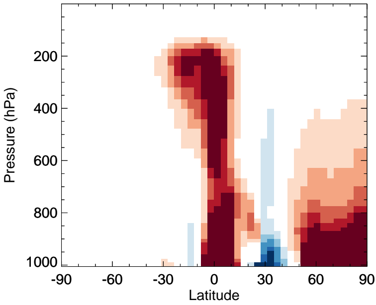
v11-02f-Run0 - v11-02e-Run1 BENZ - Zonal mean abs diff for Oct
