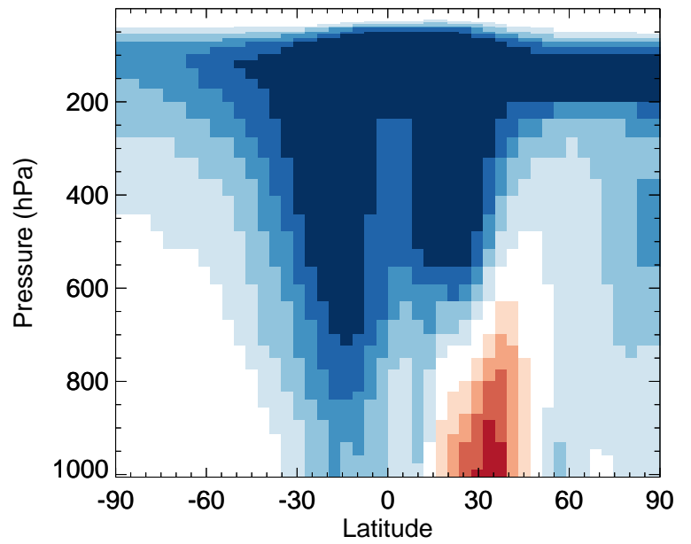
v11-02f-Run0 / v11-02e-Run1 ISN1OA - Zonal mean % diff for Oct
