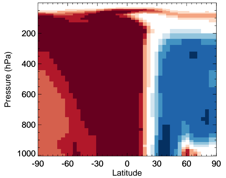
v11-02f-Run0 / v11-02e-Run1 ASOG1 - Zonal mean % diff for Oct
