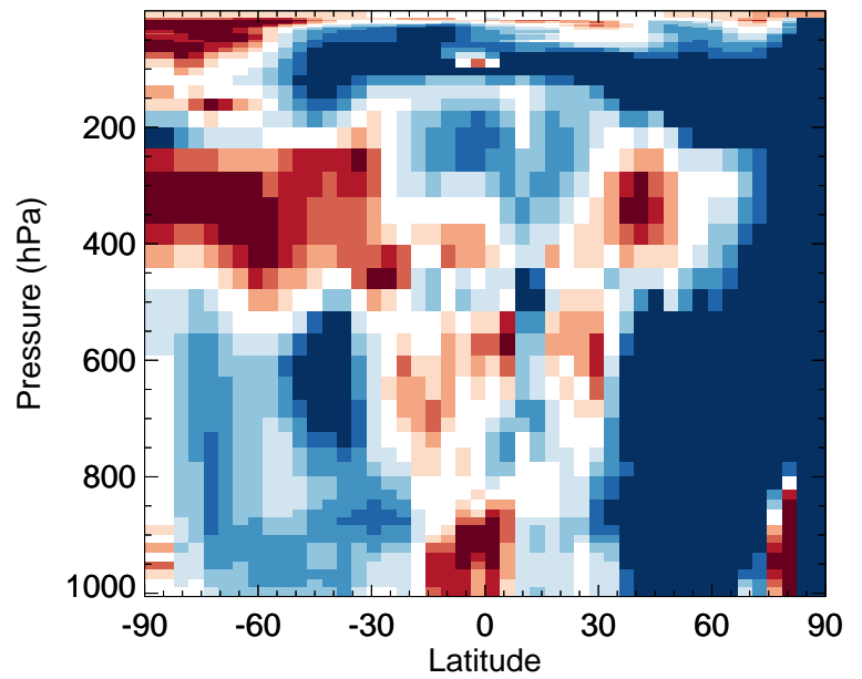
v11-02f-Run0 / v11-02e-Run0 ClOO - Zonal mean % diff for Oct
