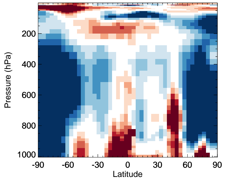
v11-02f-Run0 / v11-02e-Run0 MPN - Zonal mean % diff for Oct
