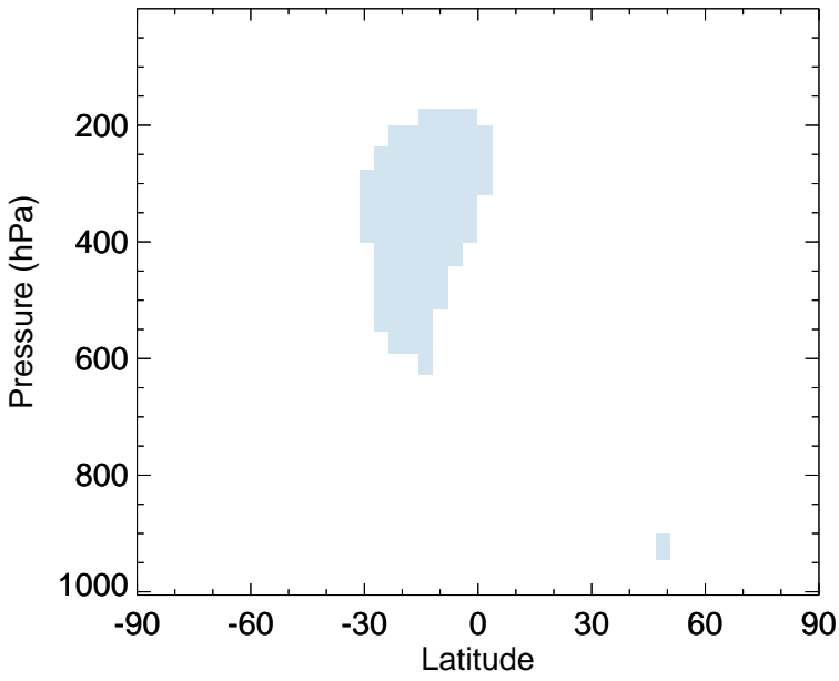
v11-02f-Run0 - v11-02e-Run1 PAN - Zonal mean abs diff for Oct
