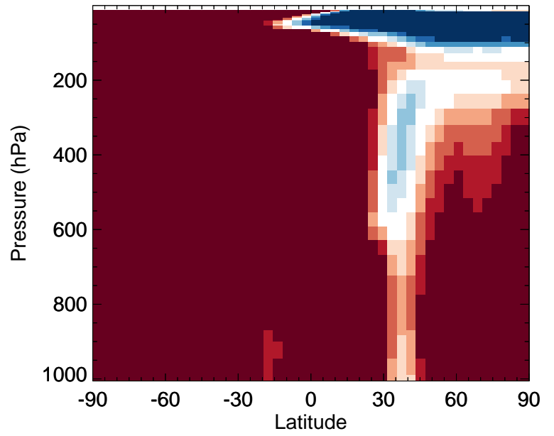
v11-02f-Run0 / v11-02e-Run1 BENZ - Zonal mean % diff for Oct
