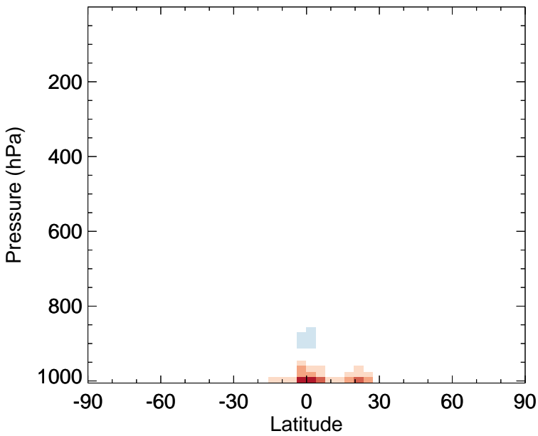
v11-02f-Run0 - v11-02e-Run0 RCHO - Zonal mean abs diff for Oct
