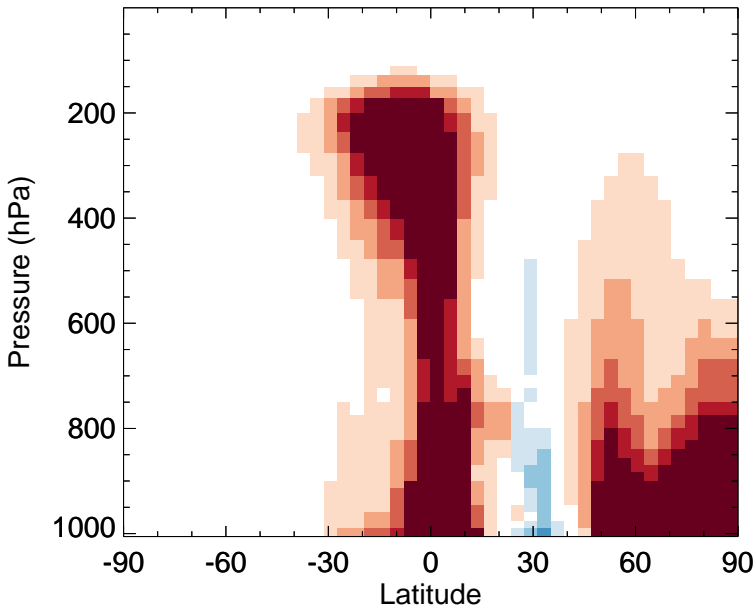
v11-02f-Run0 - v11-02e-Run0 BENZ - Zonal mean abs diff for Oct
