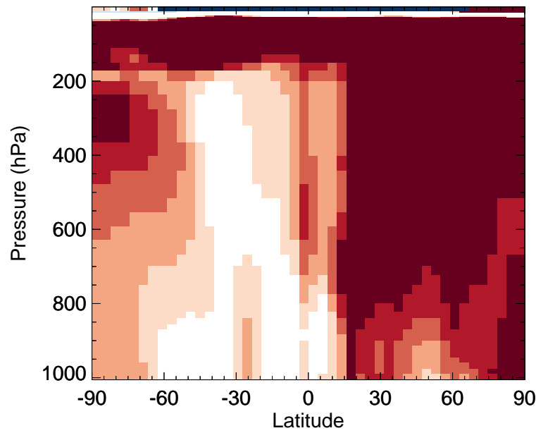
v11-02f-Run0 / v11-02e-Run1 ALD2 - Zonal mean % diff for Oct
