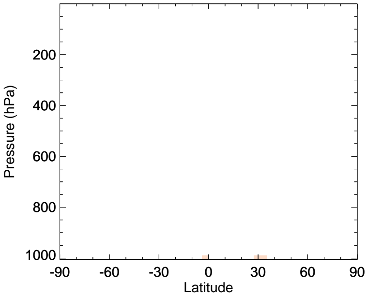
v11-02f-Run0 - v11-02e-Run1 OCPO - Zonal mean abs diff for Oct
