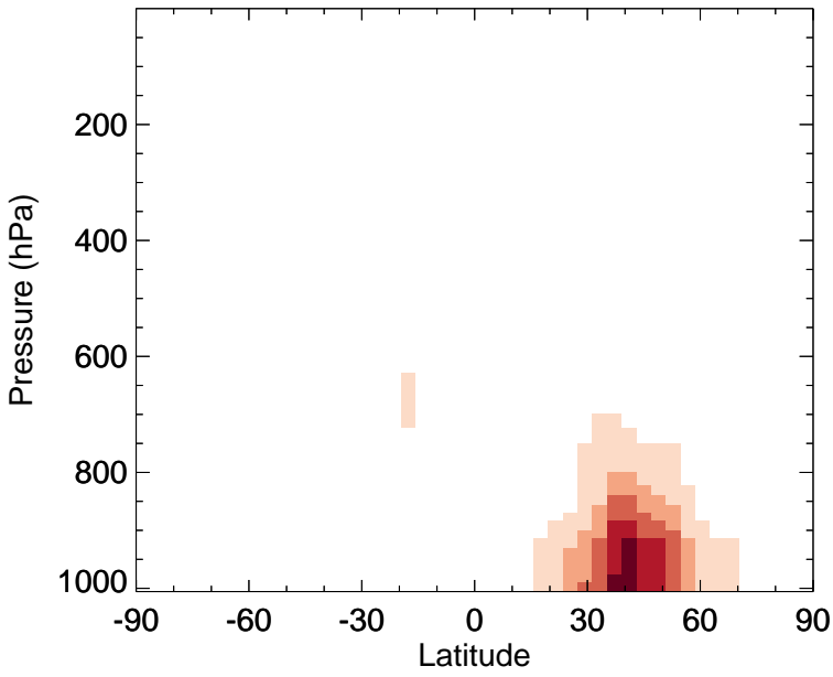
v11-02f-Run0 - v11-02e-Run1 NIT - Zonal mean abs diff for Oct
