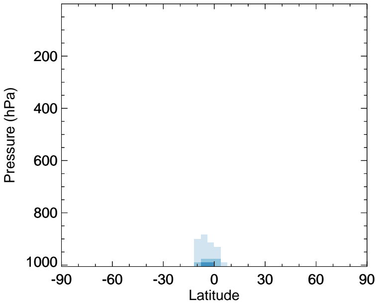
v11-02f-Run0 - v11-02e-Run1 MTPA - Zonal mean abs diff for Oct
