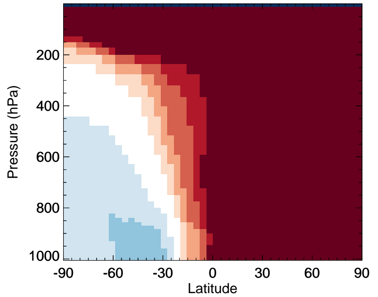
v11-02f-Run0 / v11-02e-Run1 C2H6 - Zonal mean % diff for Oct
