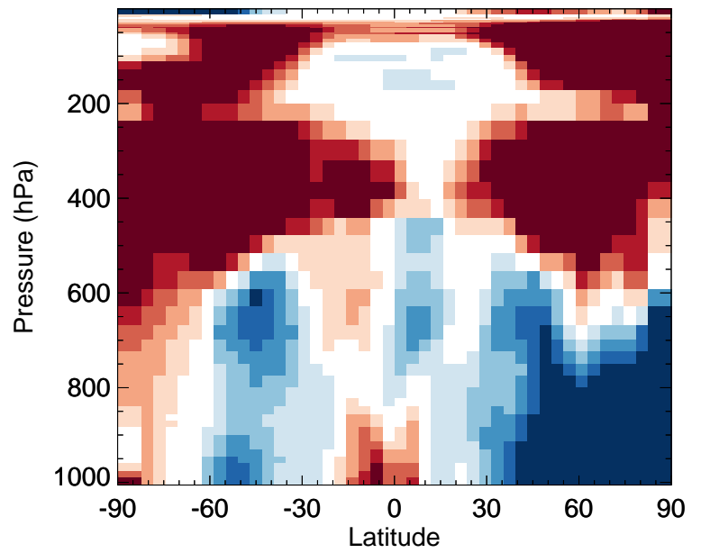
v11-02f-Run0 / v11-02e-Run1 ClO - Zonal mean % diff for Oct
