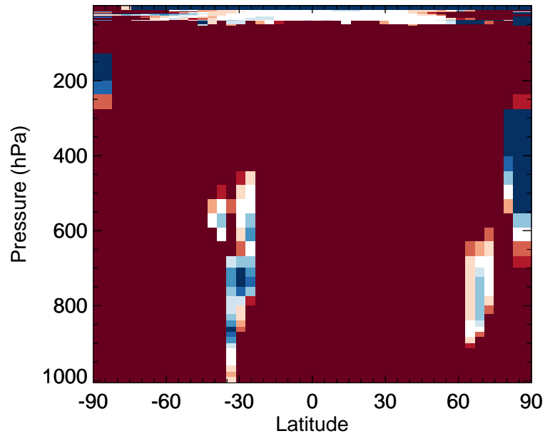
v11-02f-Run0 / v11-02e-Run0 ISN1 - Zonal mean % diff for Oct
