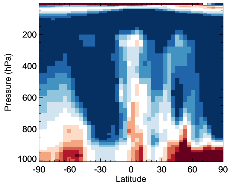
v11-02f-Run0 / v11-02e-Run0 SO4 - Zonal mean % diff for Oct
