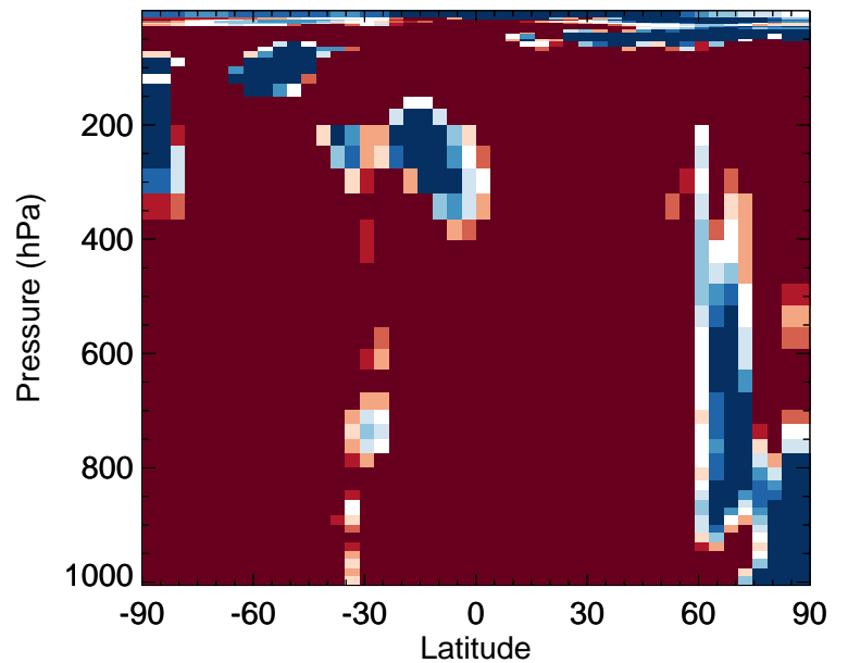
v11-02f-Run0 / v11-02e-Run0 ISN1OG - Zonal mean % diff for Oct
