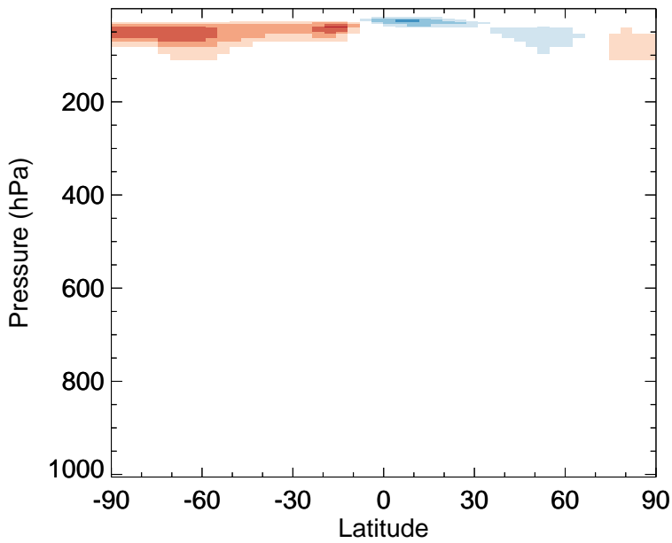
v11-02f-Run0 - v11-02e-Run0 OCS - Zonal mean abs diff for Oct
