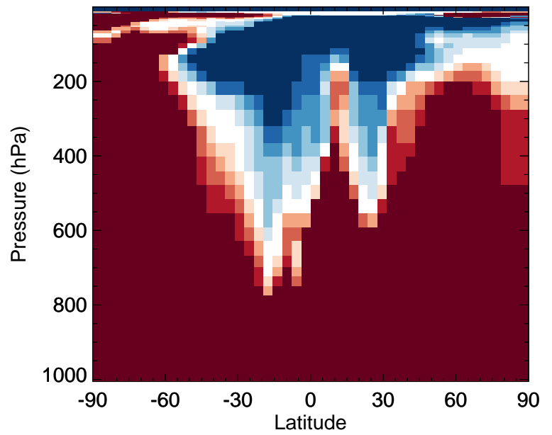
v11-02f-Run0 / v11-02e-Run1 GLYC - Zonal mean % diff for Oct
