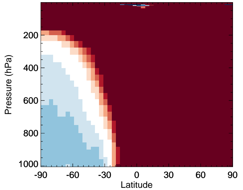
v11-02f-Run0 / v11-02e-Run0 C2H6 - Zonal mean % diff for Oct
