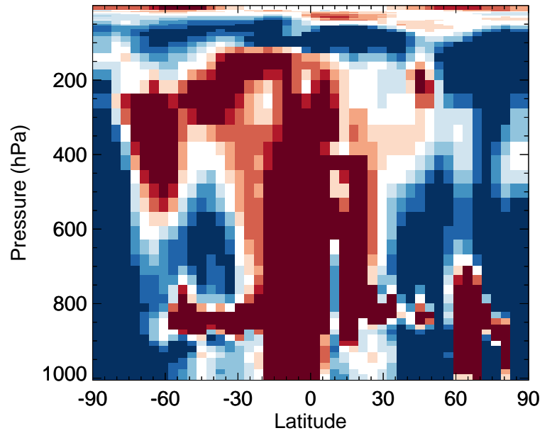
v11-02f-Run0 / v11-02e-Run0 CINO3 - Zonal mean % diff for Oct
