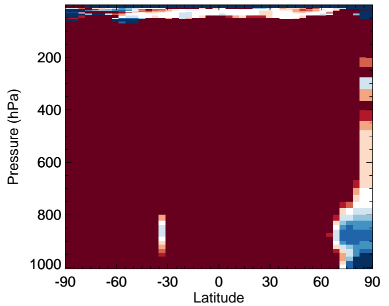
v11-02f-Run0 / v11-02e-Run0 RIPB - Zonal mean % diff for Oct
