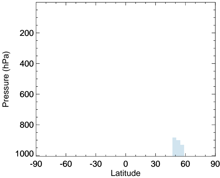
v11-02f-Run0 - v11-02e-Run0 SO 2 - Zonal mean abs diff for Oct
