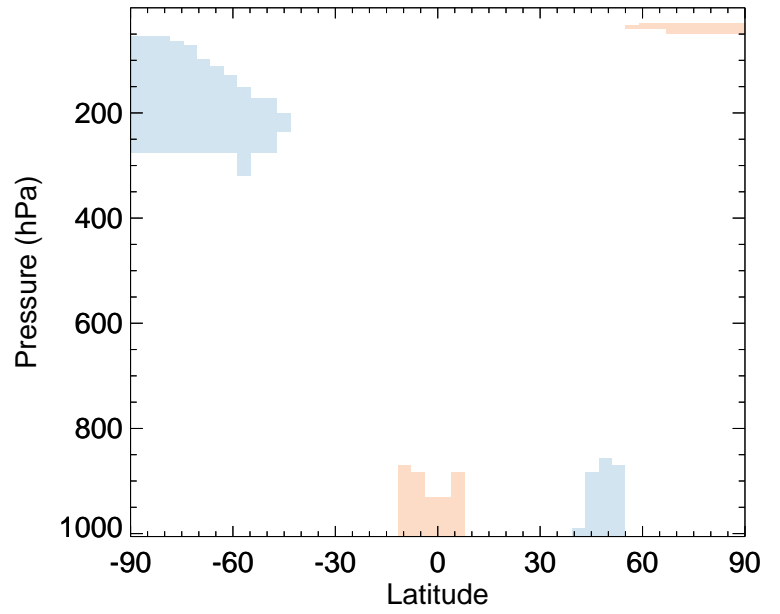
v11-02f-Run0 / v11-02e-Run1 O3 - Zonal mean % diff for Oct
