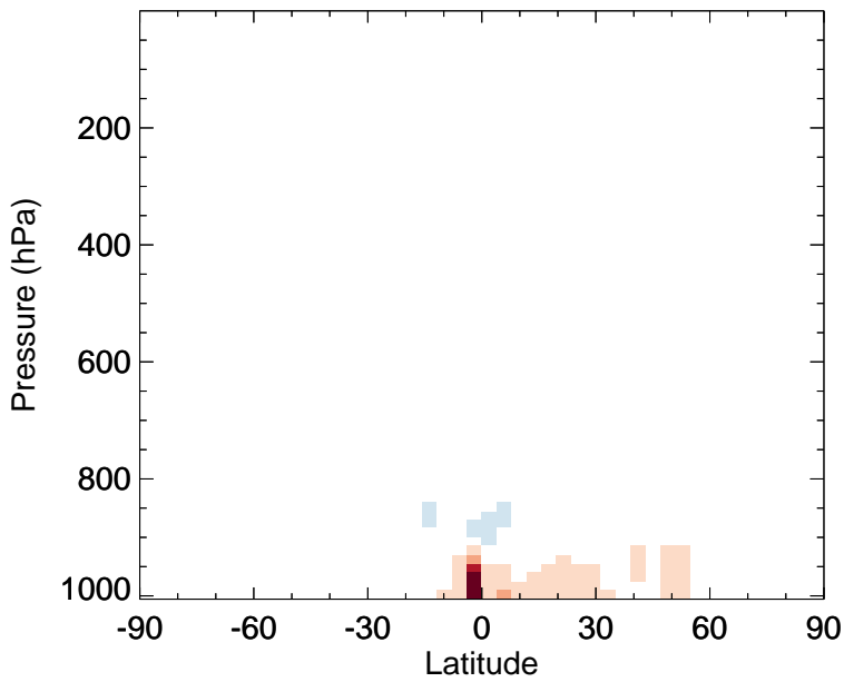
v11-02f-Run0 - v11-02e-Run0 ALD2 - Zonal mean abs diff for Oct
