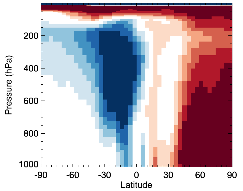
v11-02f-Run0 / v11-02e-Run1 C3H8 - Zonal mean % diff for Oct
