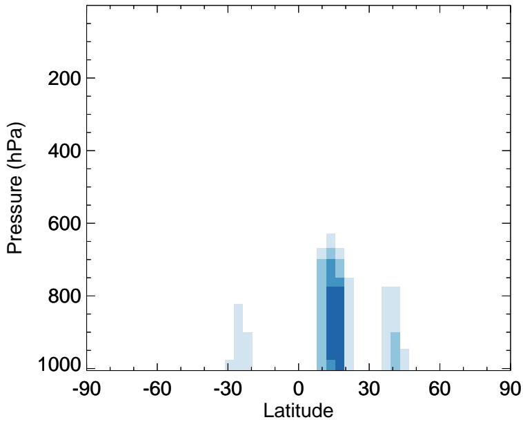
v11-02f-Run0 - v11-02e-Run0 DST2 - Zonal mean abs diff for Oct
