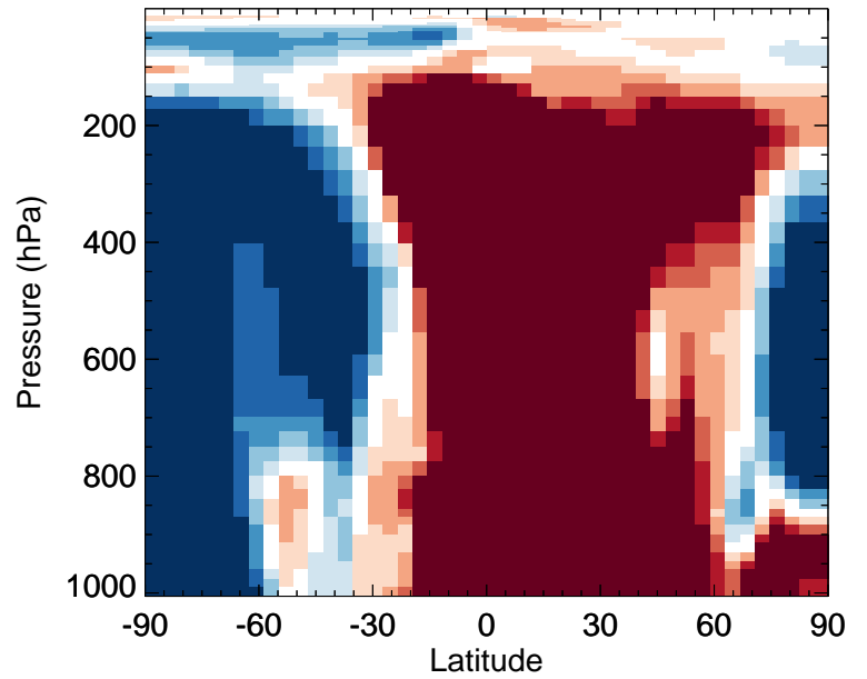
v11-02f-Run0 / v11-02e-Run0 OCPI - Zonal mean % diff for Oct
