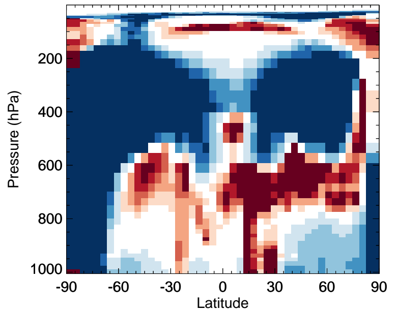
v11-02f-Run0 / v11-02e-Run1 HBr - Zonal mean % diff for Oct
