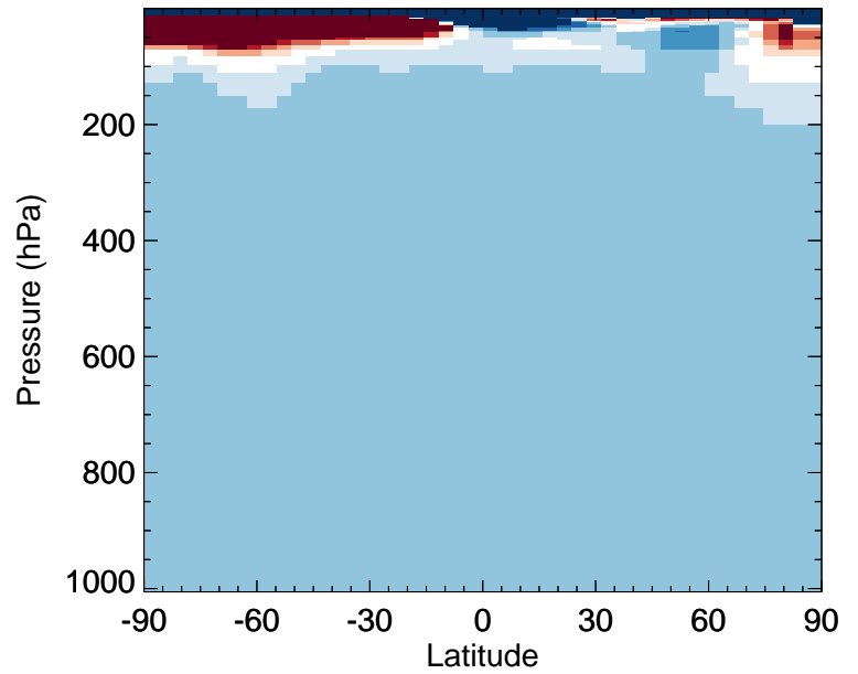
v11-02f-Run0 / v11-02e-Run0 CCI4 - Zonal mean % diff for Oct
