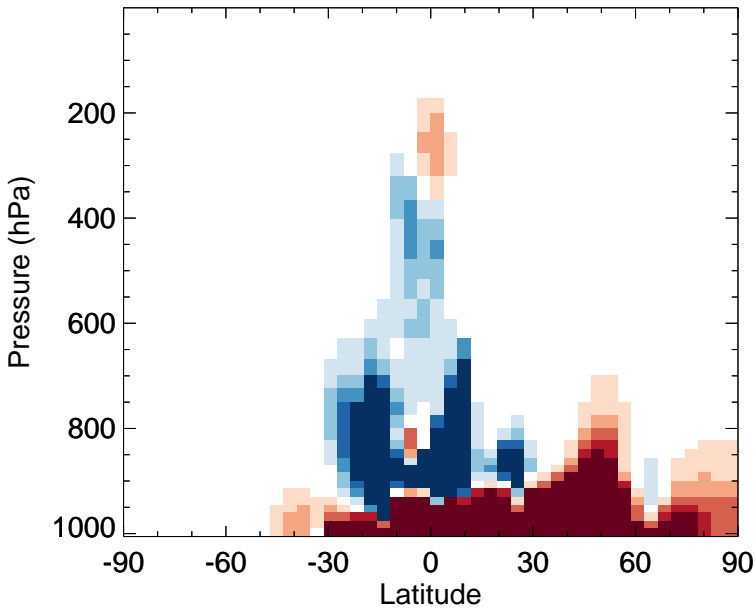
v11-02f-Run0 - v11-02e-Run0 PRPE - Zonal mean abs diff for Oct
