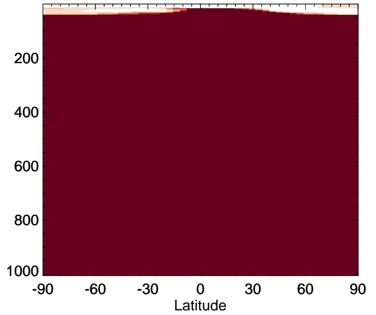
v11-02f-Run0 / v11-02e-Run0 NH3 - Zonal mean % diff for Oct
