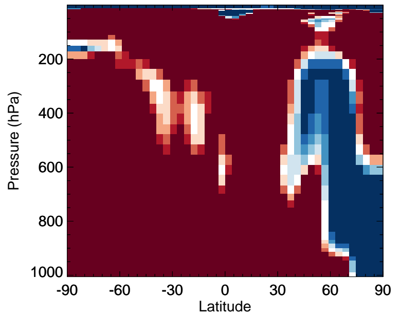
v11-02f-Run0 / v11-02e-Run0 HONIT - Zonal mean % diff for Oct
