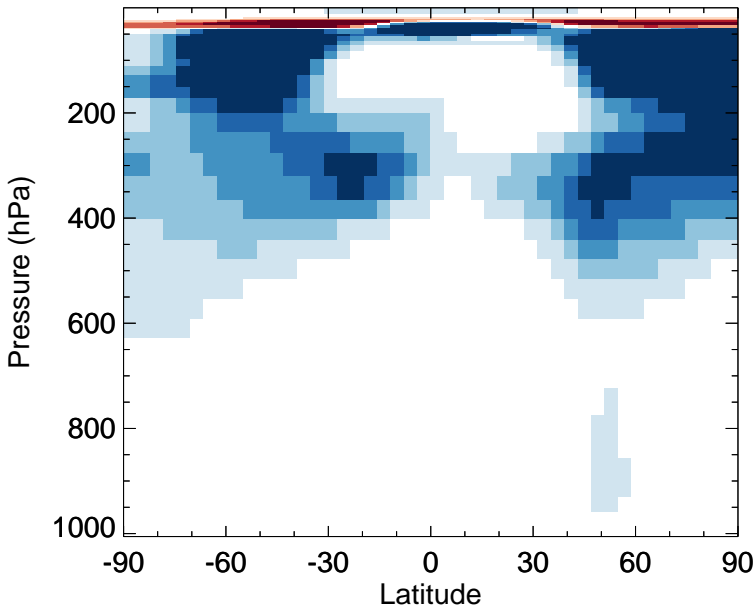
v11-02f-Run0 - v11-02e-Run1 HNO 4 - Zonal mean abs diff for Oct
