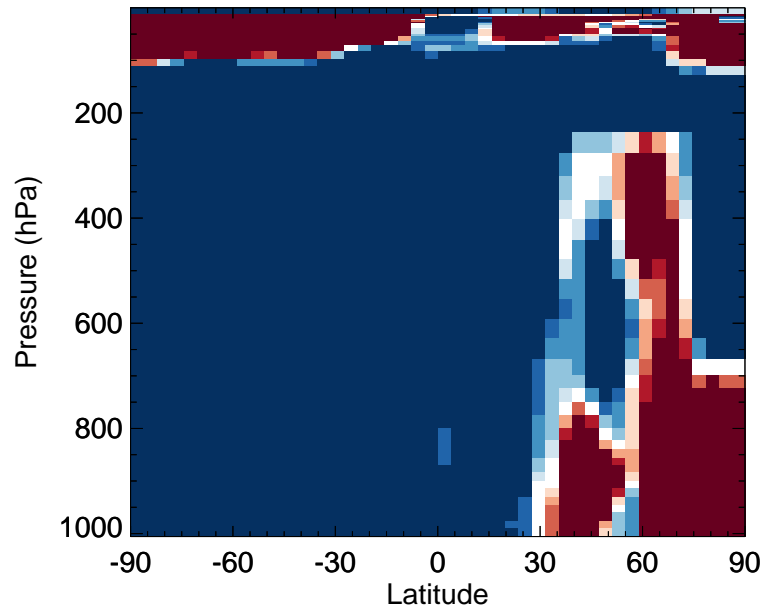
v11-02f-Run0 / v11-02e-Run0 DST2 - Zonal mean % diff for Oct
