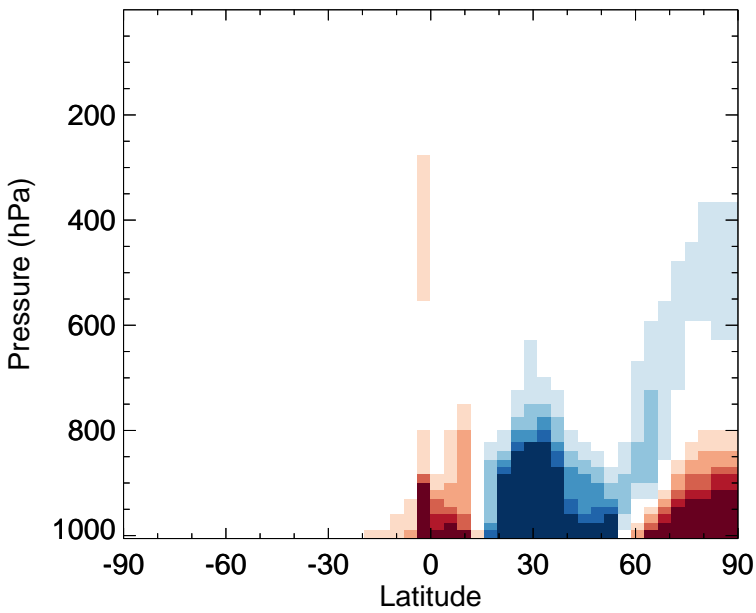
v11-02f-Run0 - v11-02e-Run0 TOLU - Zonal mean abs diff for Oct
