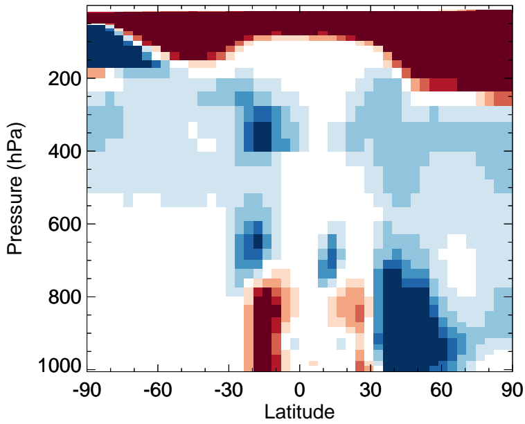
v11-02f-Run0 - v11-02e-Run1 HNO 3 - Zonal mean abs diff for Oct
