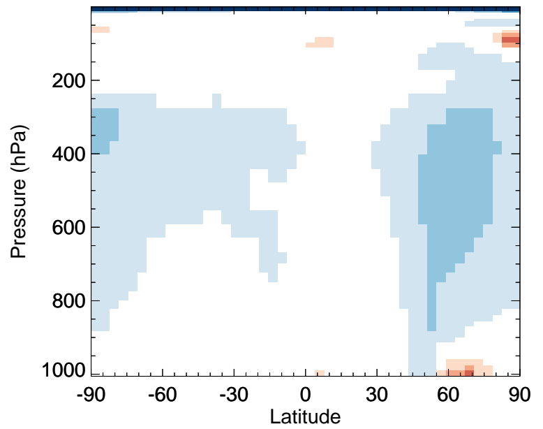
v11-02f-Run0 / v11-02e-Run1 CH 2 O - Zonal mean % diff for Oct
