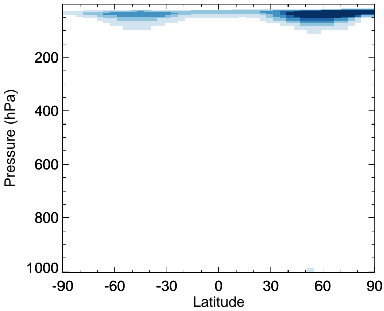
v11-02f-Run0 - v11-02e-Run1 NO 2 - Zonal mean abs diff for Oct
