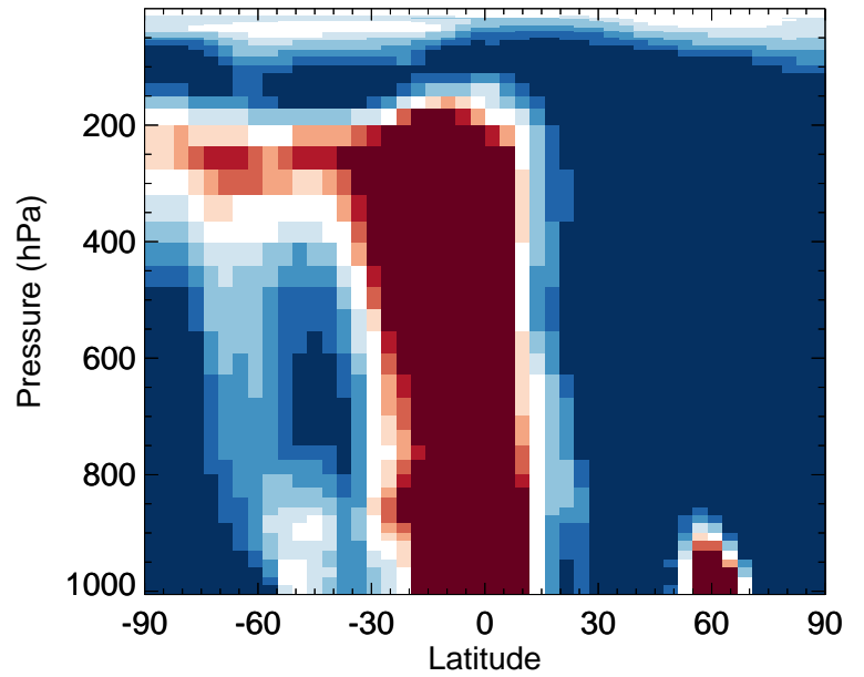
v11-02f-Run0 / v11-02e-Run0 ASOG2 - Zonal mean % diff for Oct
