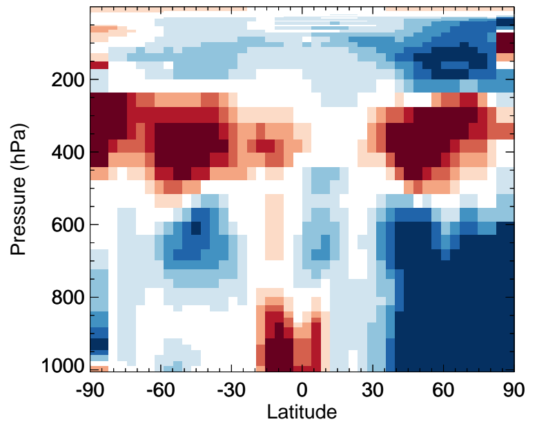
v11-02f-Run0 / v11-02e-Run1 ClOO - Zonal mean % diff for Oct
