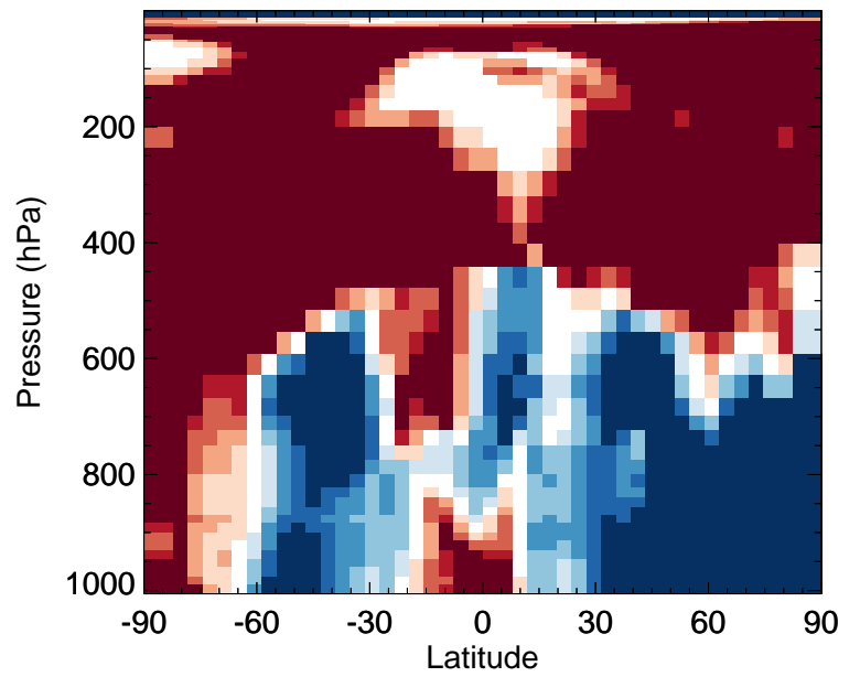
v11-02f-Run0 / v11-02e-Run1 Cl2O2 - Zonal mean % diff for Oct
