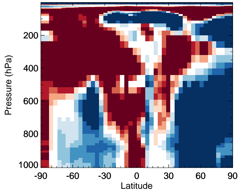
v11-02f-Run0 / v11-02e-Run0 HOCl - Zonal mean % diff for Oct
