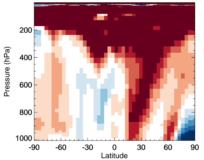
v11-02f-Run0 / v11-02e-Run0 MAP - Zonal mean % diff for Oct
