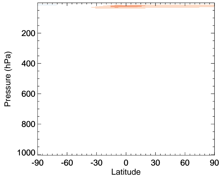
v11-02f-Run0 / v11-02e-Run1 CH 2 Br 2 - Zonal mean % diff for Oct
