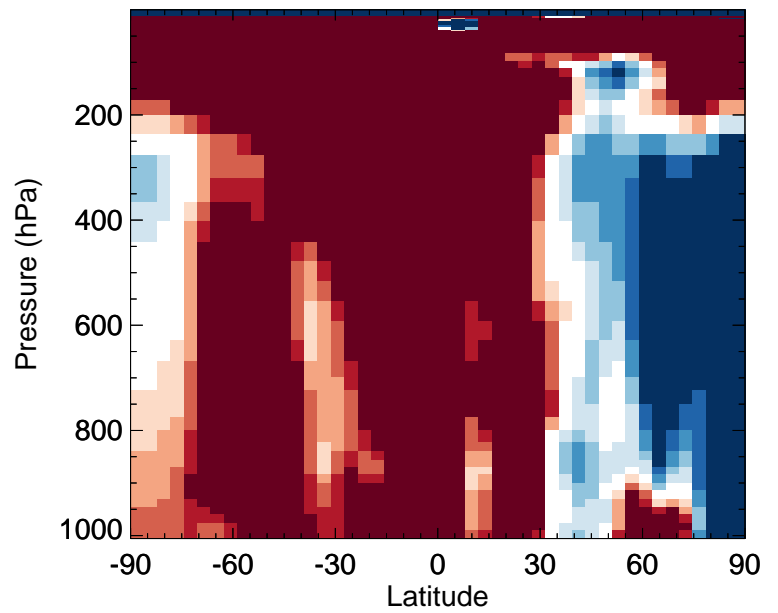
v11-02f-Run0 / v11-02e-Run0 GLYX - Zonal mean % diff for Oct
