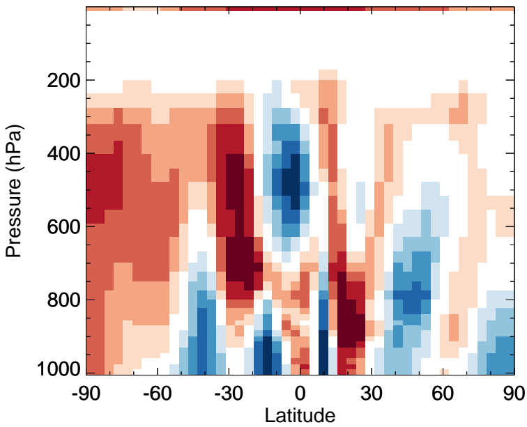
v11-02f-Run0 - v11-02e-Run0 MP - Zonal mean abs diff for Oct
