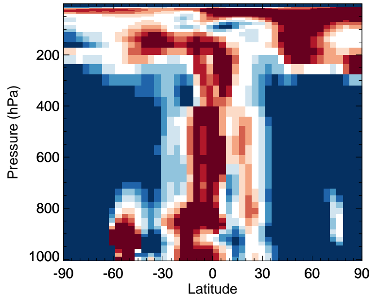
v11-02f-Run0 / v11-02e-Run0 HNO 3 - Zonal mean % diff for Oct
