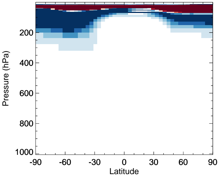
v11-02f-Run0 - v11-02e-Run1 O3 - Zonal mean abs diff for Oct
