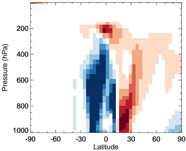
v11-02f-Run0 - v11-02e-Run0 MAP - Zonal mean abs diff for Oct
