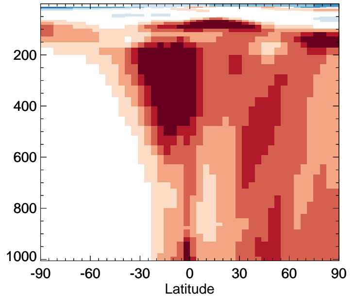
v11-02f-Run0 / v11-02e-Run0 CO - Zonal mean % diff for Oct
