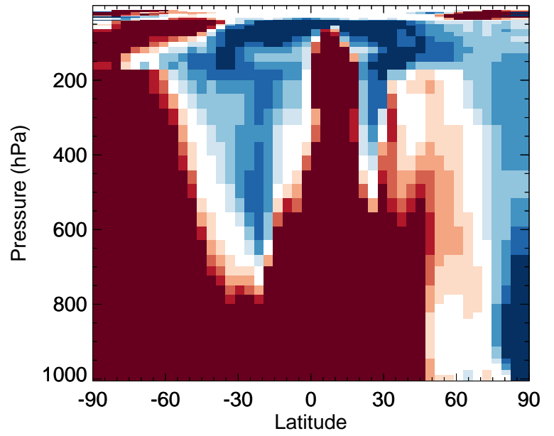
v11-02f-Run0 / v11-02e-Run1 MVKN - Zonal mean % diff for Oct
