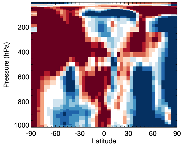
v11-02f-Run0 / v11-02e-Run0 ClO - Zonal mean % diff for Oct
