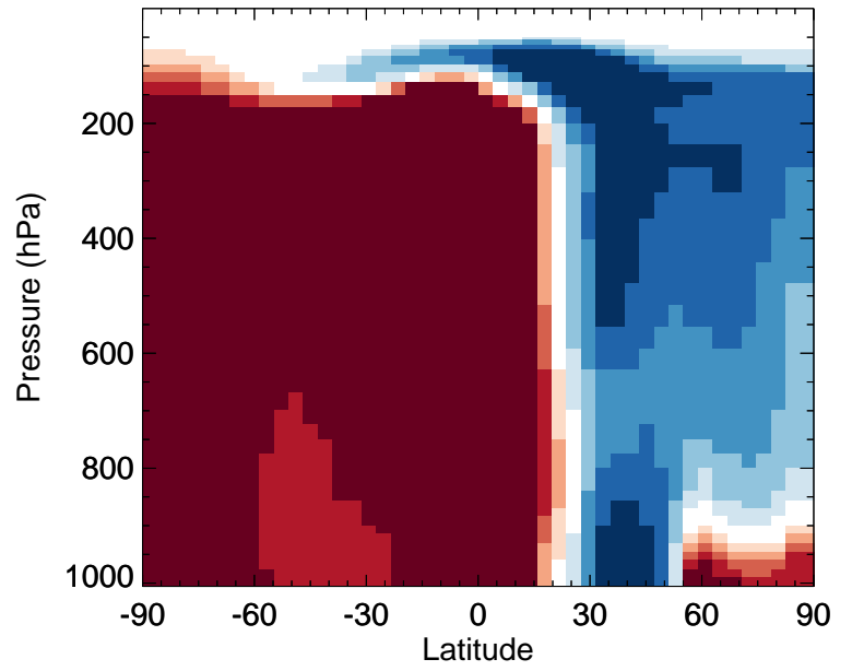
v11-02f-Run0 / v11-02e-Run1 ASOAN - Zonal mean % diff for Oct
