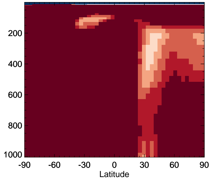
v11-02f-Run0 / v11-02e-Run1 ALK4 - Zonal mean % diff for Oct
