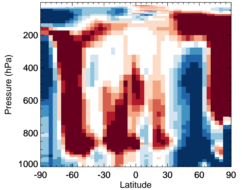
v11-02f-Run0 / v11-02e-Run0 HCl - Zonal mean % diff for Oct
