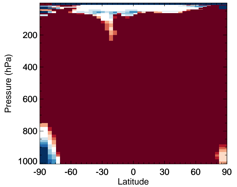
v11-02f-Run0 / v11-02e-Run1 RIPB - Zonal mean % diff for Oct
