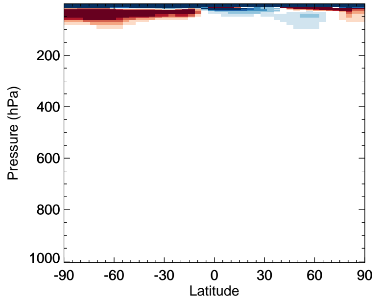
v11-02f-Run0 / v11-02e-Run0 CFC113 - Zonal mean % diff for Oct
