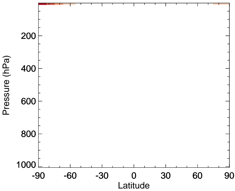
v11-02f-Run0 - v11-02e-Run1 ACTA - Zonal mean abs diff for Oct
