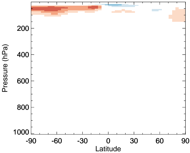
v11-02f-Run0 - v11-02e-Run0 CH3Cl - Zonal mean abs diff for Oct
