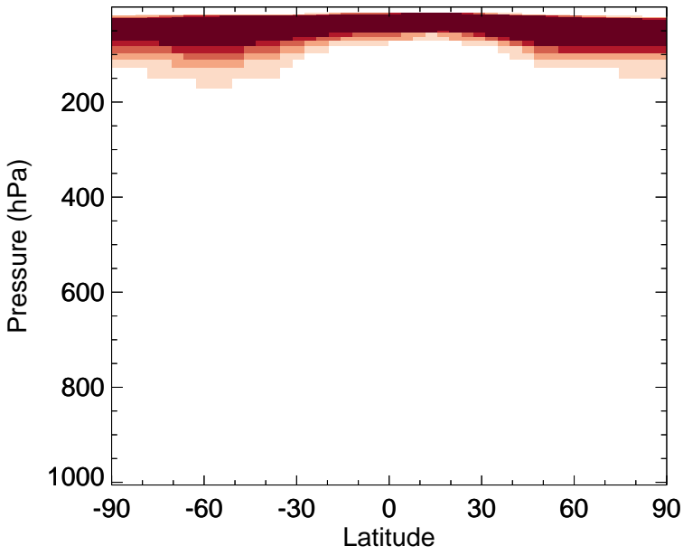
v11-02f-Run0 - v11-02e-Run1 N2O - Zonal mean abs diff for Oct
