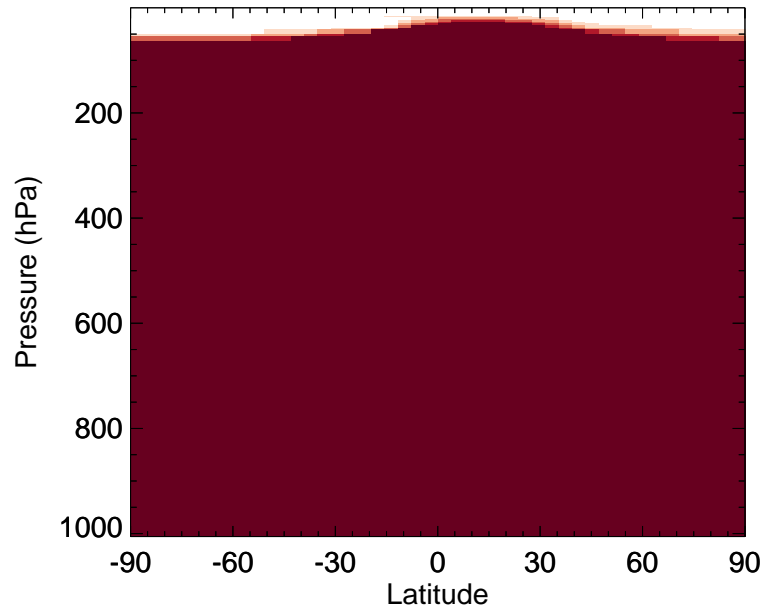
v11-02f-Run0 / v11-02e-Run0 NH4 - Zonal mean % diff for Oct
