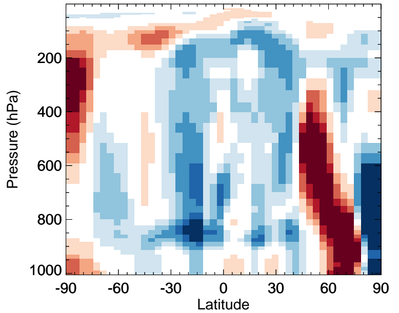
v11-02f-Run0 / v11-02e-Run0 MSA - Zonal mean % diff for Oct
