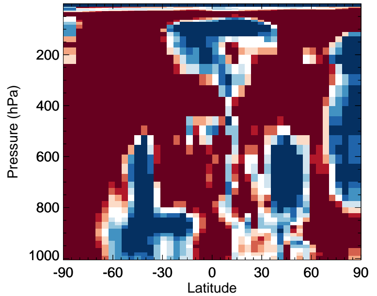
v11-02f-Run0 / v11-02e-Run0 OCIO - Zonal mean % diff for Oct
