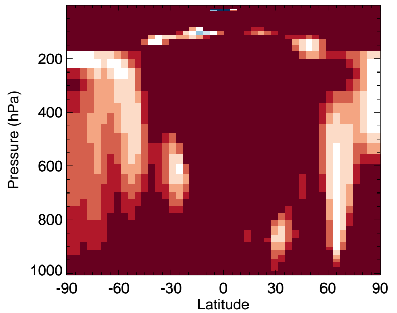
v11-02f-Run0 / v11-02e-Run0 RCHO - Zonal mean % diff for Oct
