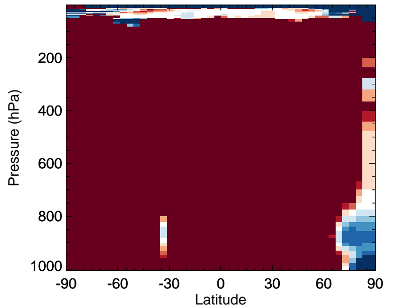
v11-02f-Run0 / v11-02e-Run0 RIPD - Zonal mean % diff for Oct
