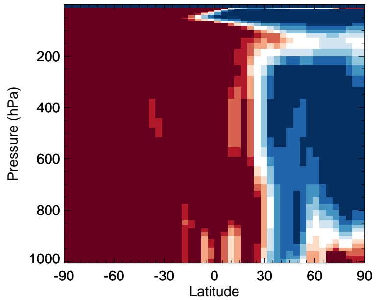
v11-02f-Run0 / v11-02e-Run1 GLYX - Zonal mean % diff for Oct
