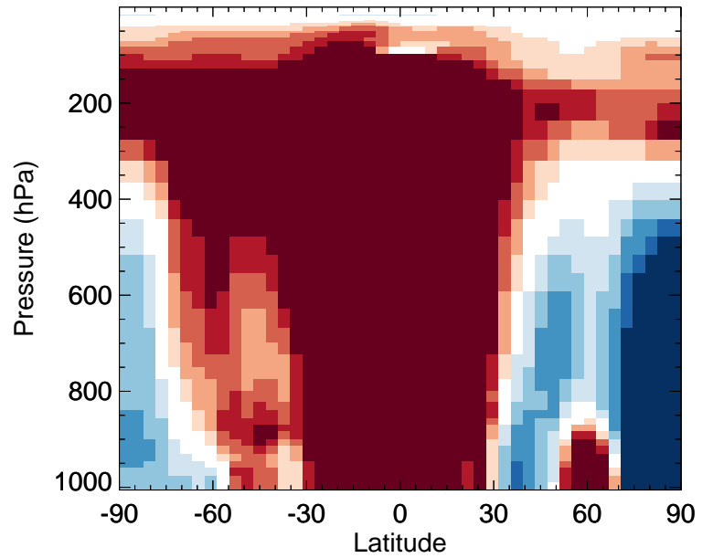
v11-02f-Run0 / v11-02e-Run0 ASOG3 - Zonal mean % diff for Oct
