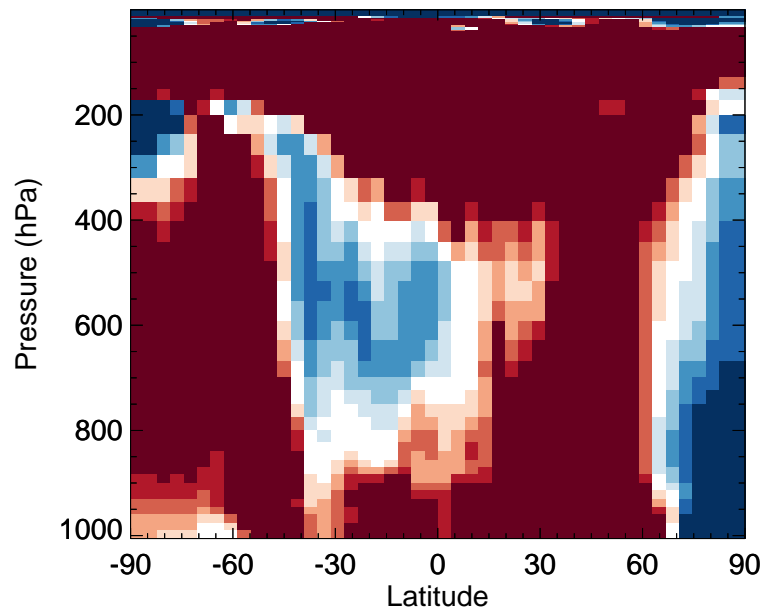
v11-02f-Run0 / v11-02e-Run0 HAC - Zonal mean % diff for Oct
