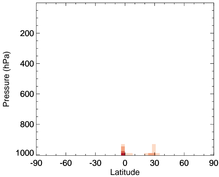
v11-02f-Run0 - v11-02e-Run0 SOAP - Zonal mean abs diff for Oct
