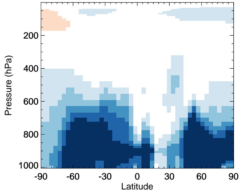
v11-02f-Run0 / v11-02e-Run1 SO 2 - Zonal mean % diff for Oct
