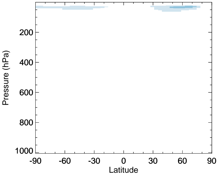
v11-02f-Run0 - v11-02e-Run1 NO - Zonal mean abs diff for Oct
