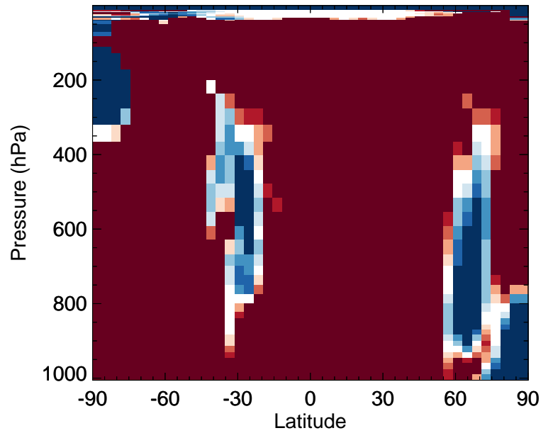
v11-02f-Run0 / v11-02e-Run0 MVKN - Zonal mean % diff for Oct
