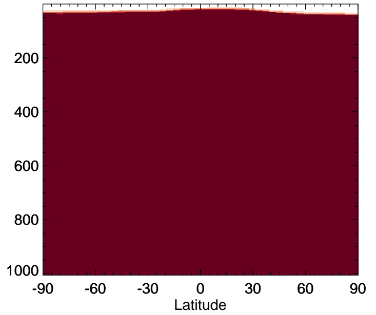
v11-02f-Run0 / v11-02e-Run1 NH3 - Zonal mean % diff for Oct
