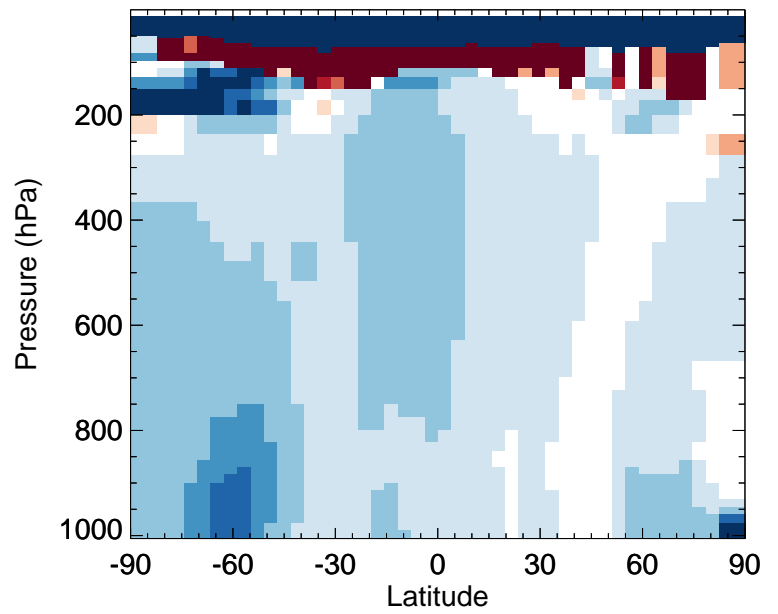
v11-02f-Run0 / v11-02e-Run1 SO4s - Zonal mean % diff for Oct
