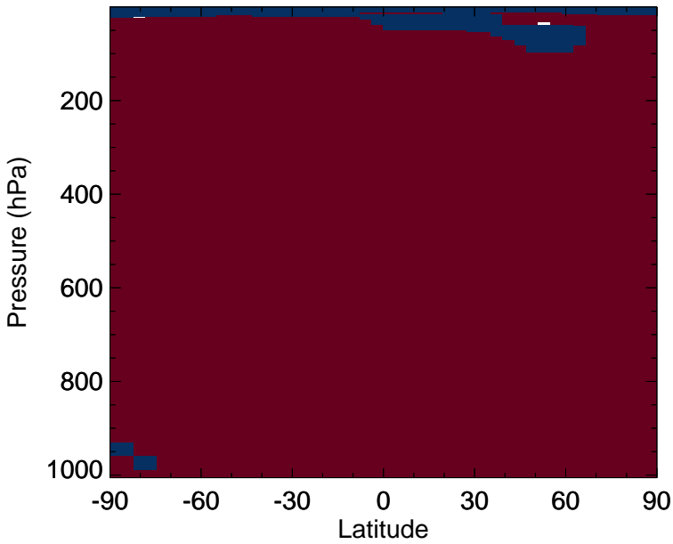
v11-02f-Run0 - v11-02e-Run0 CH4 - Zonal mean abs diff for Oct
