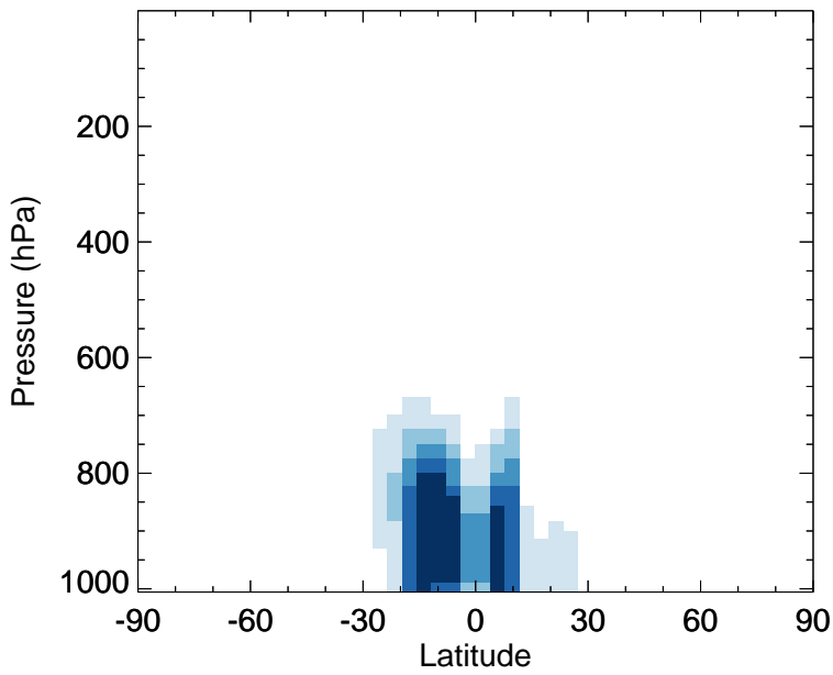
v11-02f-Run0 - v11-02e-Run1 MVK - Zonal mean abs diff for Oct
