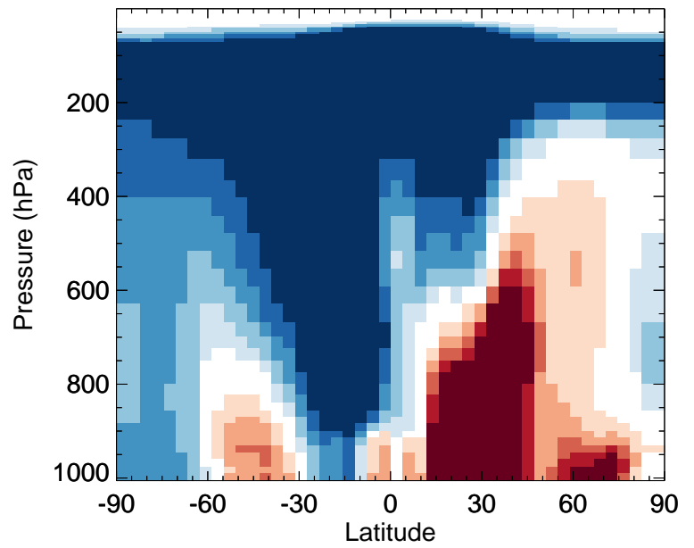
v11-02f-Run0 / v11-02e-Run1 ISOA3 - Zonal mean % diff for Oct
