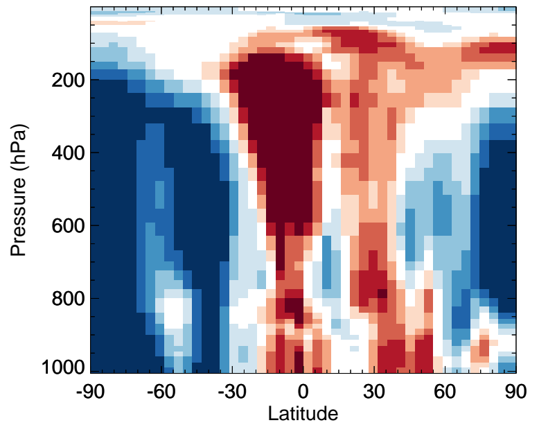
v11-02f-Run0 / v11-02e-Run0 SOAS - Zonal mean % diff for Oct
