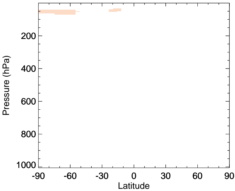
v11-02f-Run0 - v11-02e-Run0 CFC11 - Zonal mean abs diff for Oct
