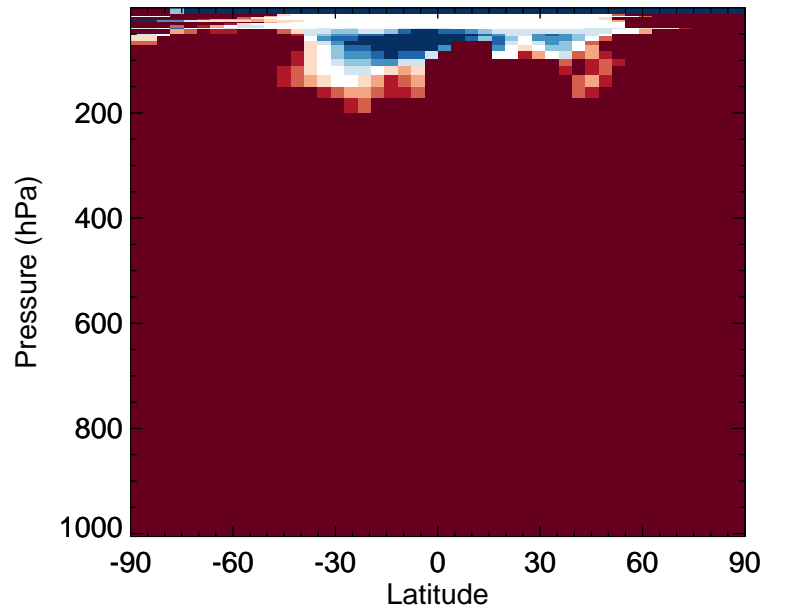
v11-02f-Run0 / v11-02e-Run1 ISN1 - Zonal mean % diff for Oct
