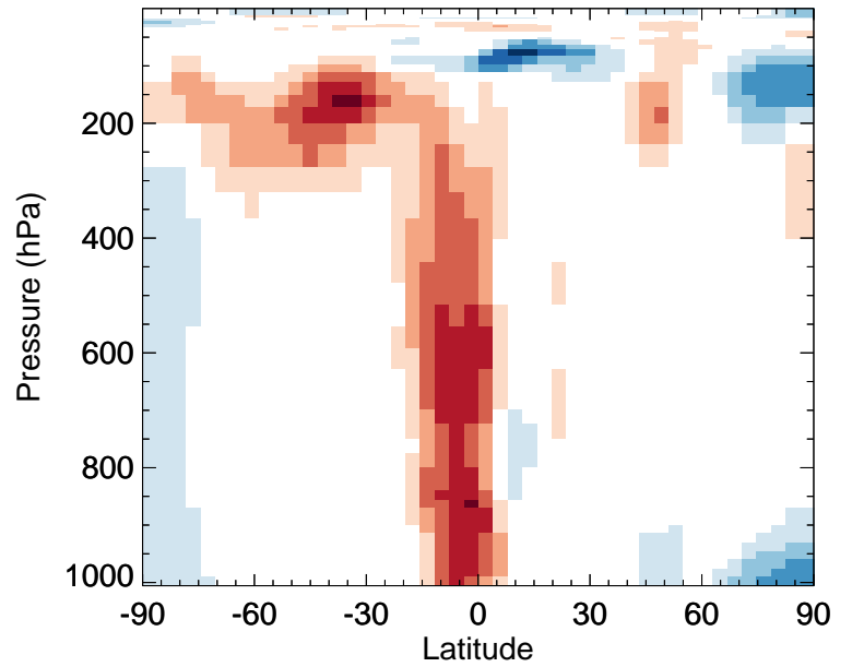
v11-02f-Run0 / v11-02e-Run0 O3 - Zonal mean % diff for Oct
