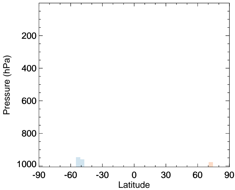
v11-02f-Run0 - v11-02e-Run0 SALA - Zonal mean abs diff for Oct
