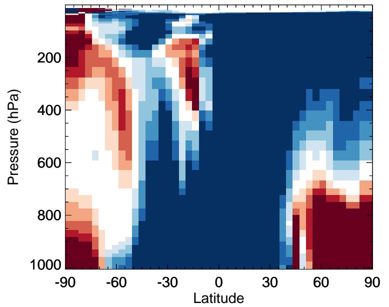
v11-02f-Run0 / v11-02e-Run1 XYLE - Zonal mean % diff for Oct
