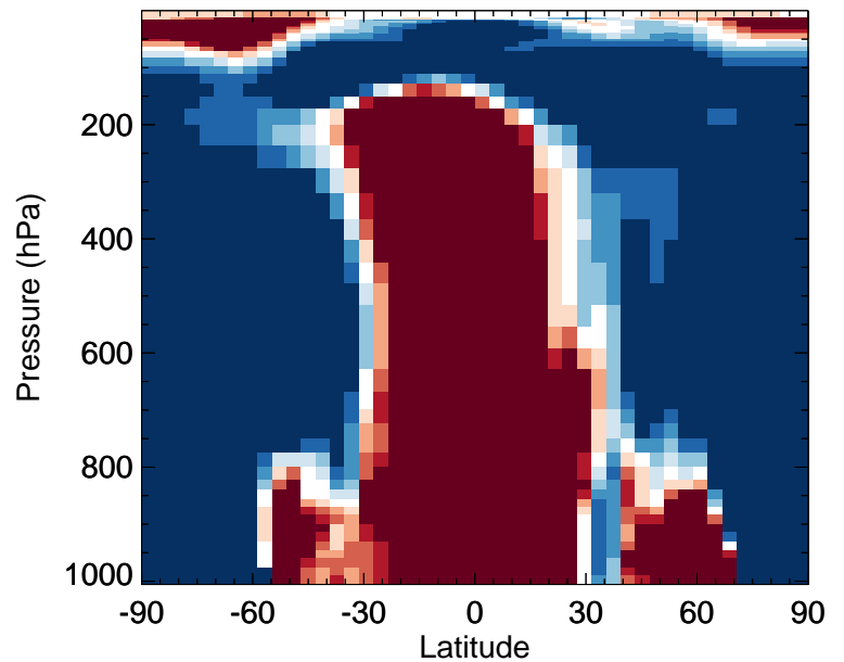
v11-02f-Run0 / v11-02e-Run0 ASOA2 - Zonal mean % diff for Oct
