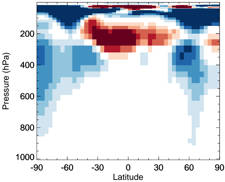
v11-02f-Run0 - v11-02e-Run0 HNO 4 - Zonal mean abs diff for Oct
