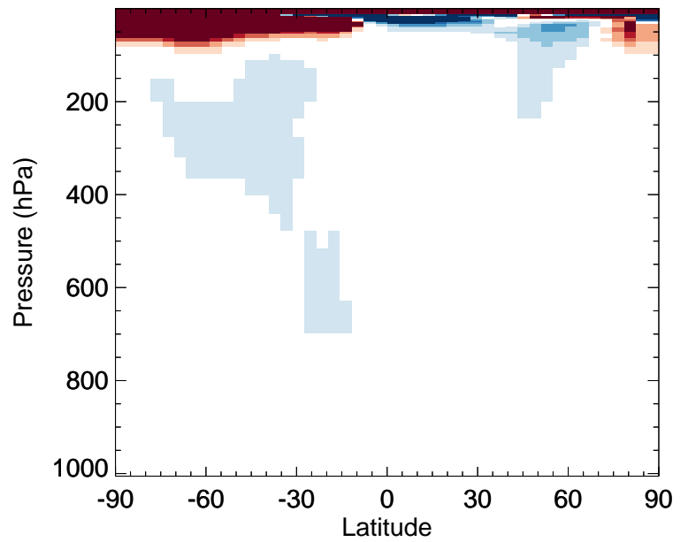
v11-02f-Run0 / v11-02e-Run0 CFC11 - Zonal mean % diff for Oct
