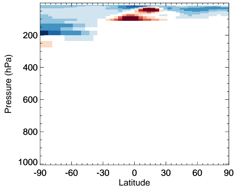
v11-02f-Run0 / v11-02e-Run1 SALC - Zonal mean % diff for Oct
