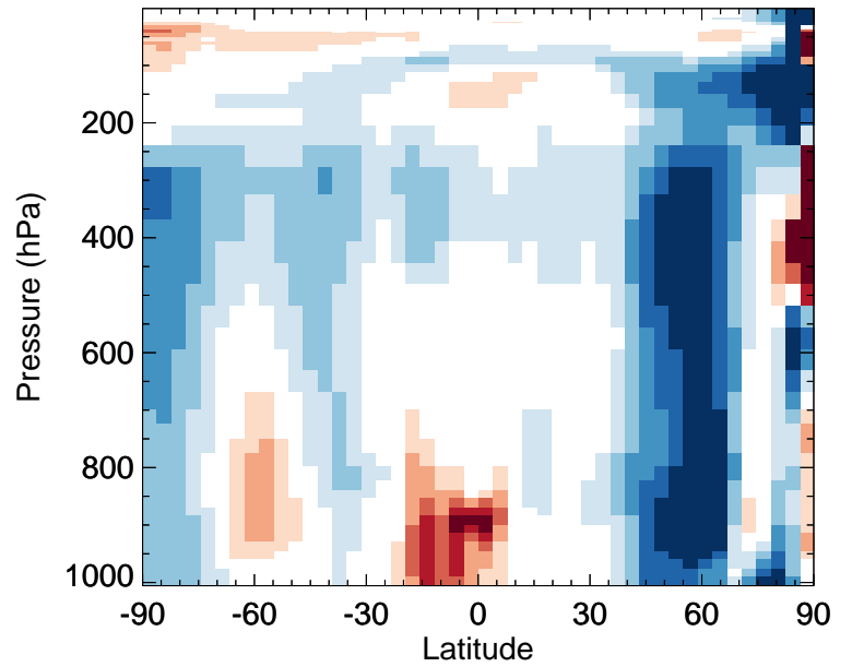
v11-02f-Run0 / v11-02e-Run0 OH - Zonal mean % diff for Oct
