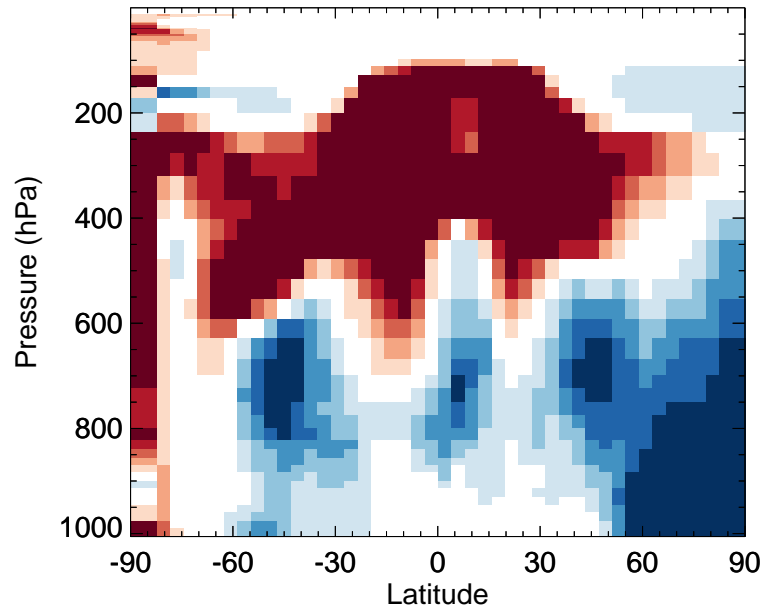
v11-02f-Run0 / v11-02e-Run1 BrCl - Zonal mean % diff for Oct
