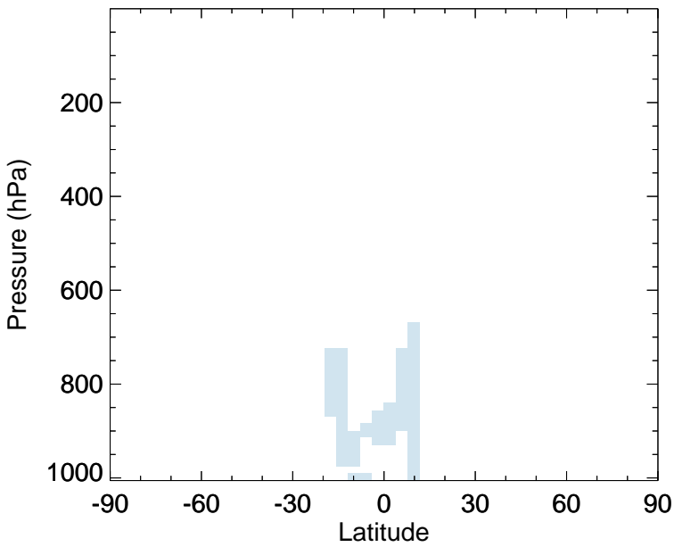
v11-02f-Run0 - v11-02e-Run0 GLYC - Zonal mean abs diff for Oct
