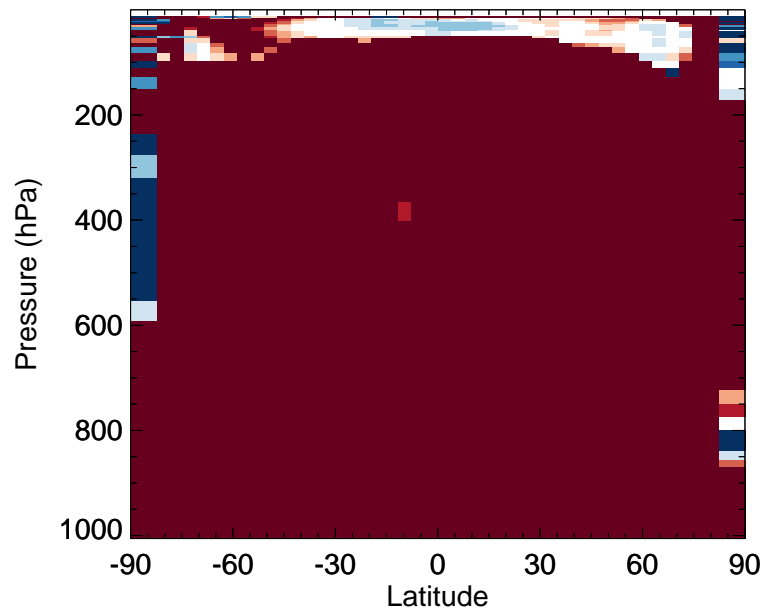
v11-02f-Run0 / v11-02e-Run0 LIMO - Zonal mean % diff for Oct
