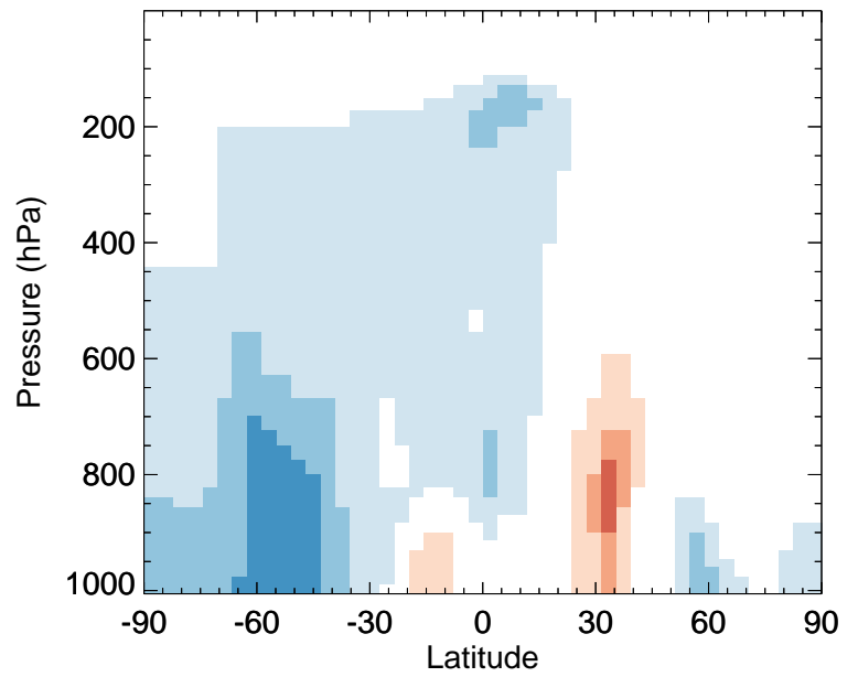
v11-02f-Run0 / v11-02e-Run1 SOAS - Zonal mean % diff for Oct
