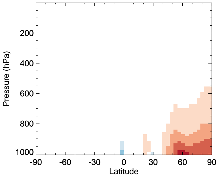
v11-02f-Run0 - v11-02e-Run1 C3H8 - Zonal mean abs diff for Oct
