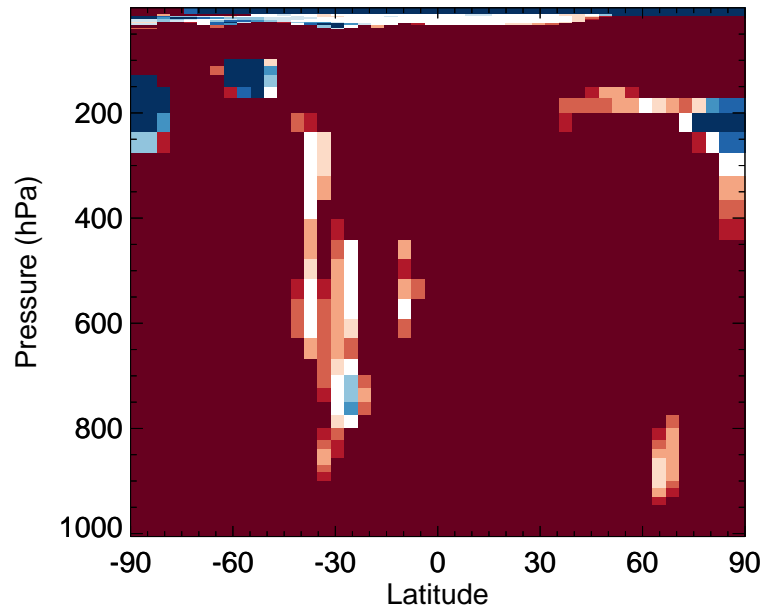
v11-02f-Run0 / v11-02e-Run0 IPMN - Zonal mean % diff for Oct
