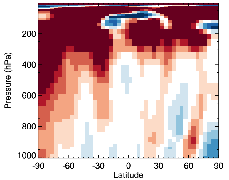
v11-02f-Run0 / v11-02e-Run0 MP - Zonal mean % diff for Oct
