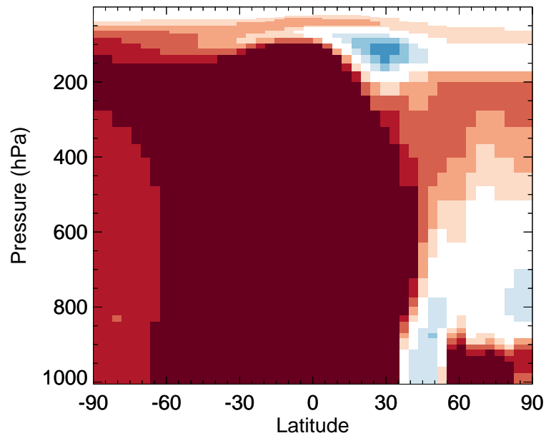
v11-02f-Run0 / v11-02e-Run1 ASOA3 - Zonal mean % diff for Oct
