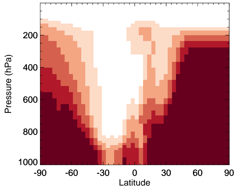
v11-02f-Run0 / v11-02e-Run1 SOAMG - Zonal mean % diff for Oct
