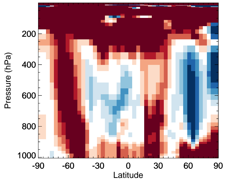
v11-02f-Run0 / v11-02e-Run0 MGLY - Zonal mean % diff for Oct
