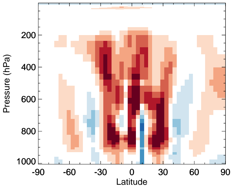
v11-02f-Run0 - v11-02e-Run0 H2O2 - Zonal mean abs diff for Oct
