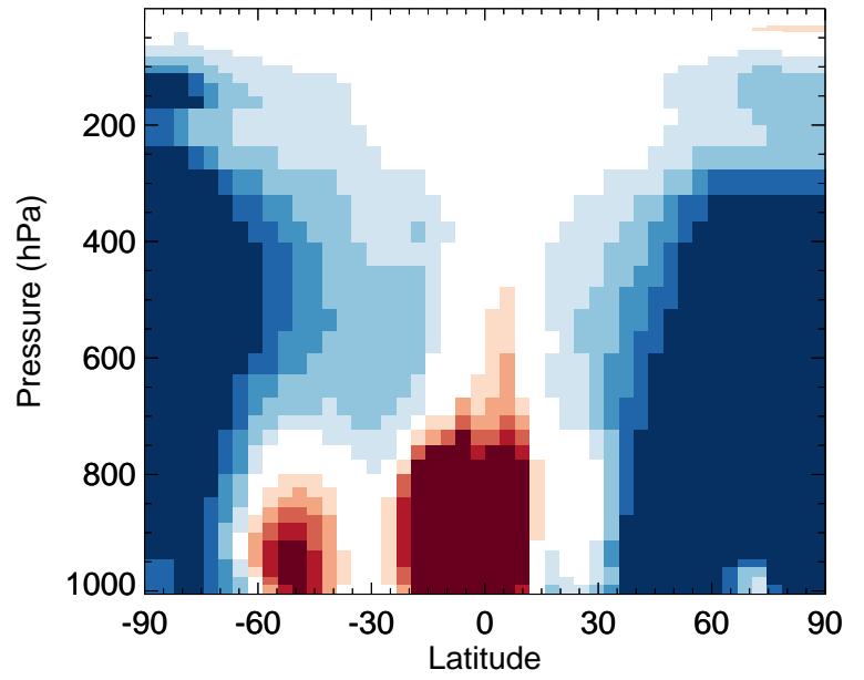
v11-02f-Run0 / v11-02e-Run1 NO3 - Zonal mean % diff for Oct
