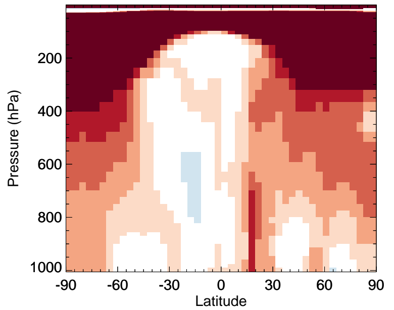
v11-02f-Run0 / v11-02e-Run1 ACTA - Zonal mean % diff for Oct
