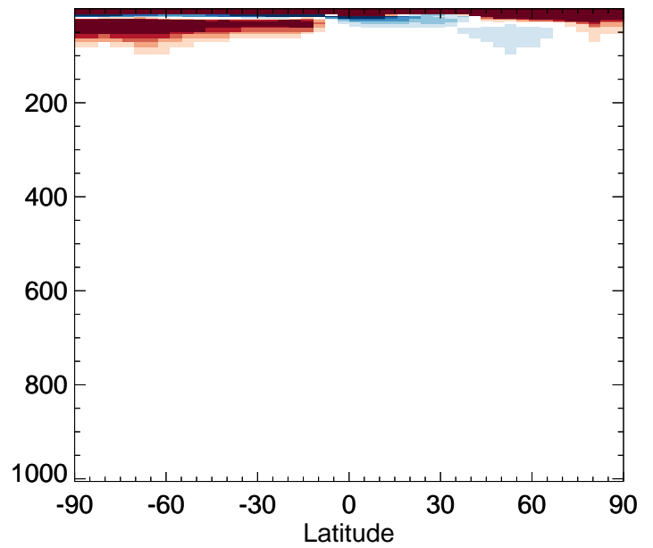
v11-02f-Run0 / v11-02e-Run0 CFC12 - Zonal mean % diff for Oct
