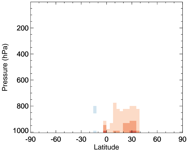
v11-02f-Run0 - v11-02e-Run1 OCPI - Zonal mean abs diff for Oct
