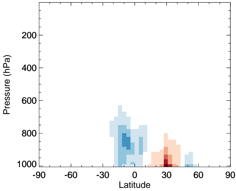
v11-02f-Run0 - v11-02e-Run1 EOH - Zonal mean abs diff for Oct
