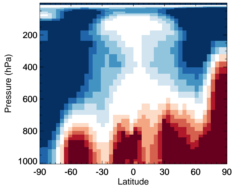
v11-02f-Run0 / v11-02e-Run1 HNO 2 - Zonal mean % diff for Oct
