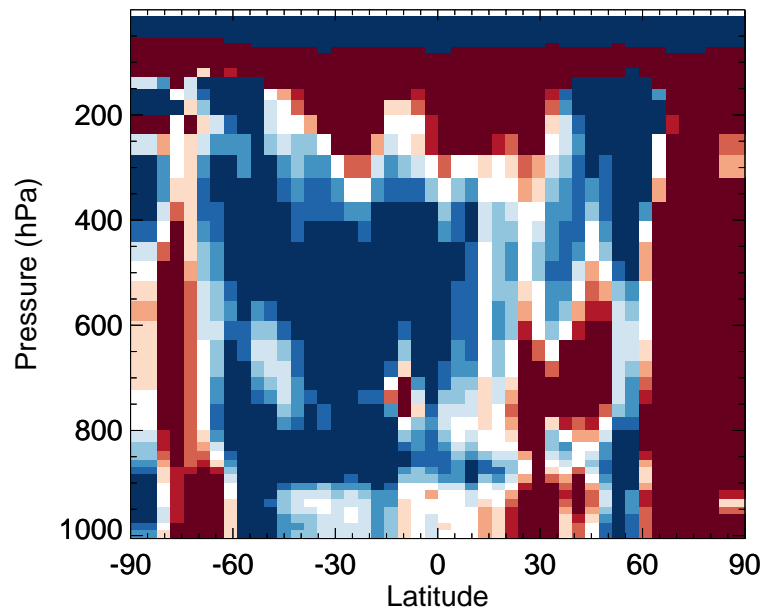
v11-02f-Run0 / v11-02e-Run0 SO4s - Zonal mean % diff for Oct
