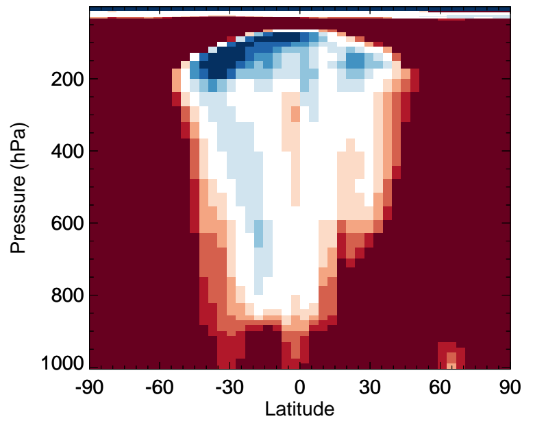
v11-02f-Run0 / v11-02e-Run1 HAC - Zonal mean % diff for Oct
