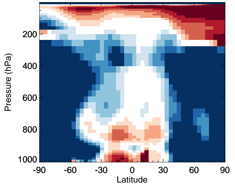
v11-02f-Run0 / v11-02e-Run1 HNO 3 - Zonal mean % diff for Oct
