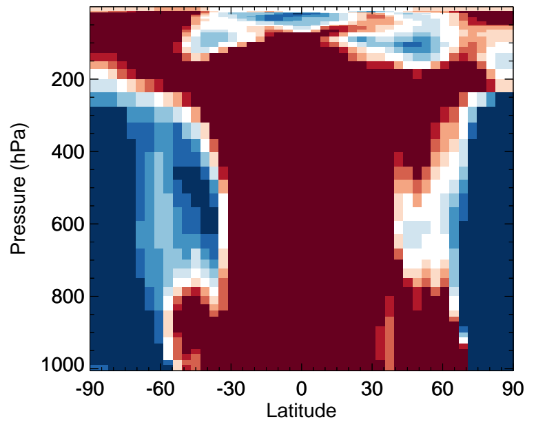
v11-02f-Run0 / v11-02e-Run0 ASOA3 - Zonal mean % diff for Oct
