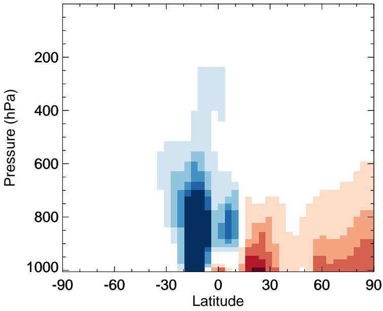
v11-02f-Run0 - v11-02e-Run1 MEK - Zonal mean abs diff for Oct
