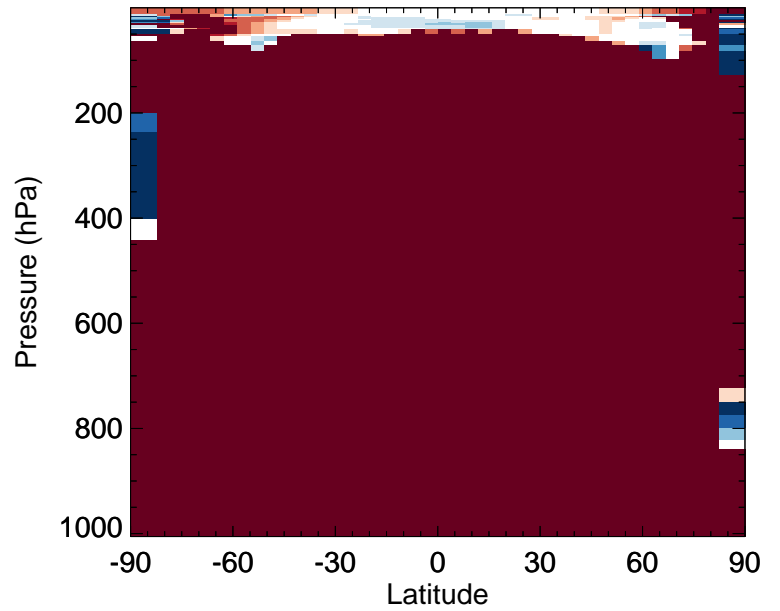
v11-02f-Run0 / v11-02e-Run0 MTPA - Zonal mean % diff for Oct
