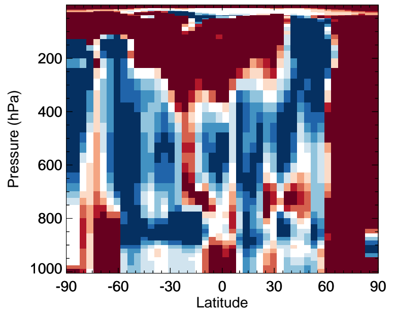
v11-02f-Run0 / v11-02e-Run0 NITs - Zonal mean % diff for Oct
