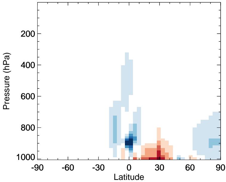
v11-02f-Run0 - v11-02e-Run0 EOH - Zonal mean abs diff for Oct
