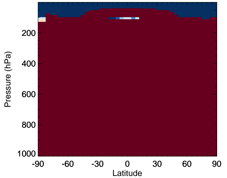
v11-02f-Run0 / v11-02e-Run0 NIT - Zonal mean % diff for Oct
