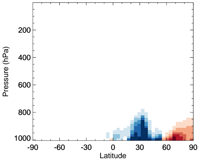
v11-02f-Run0 - v11-02e-Run0 XYLE - Zonal mean abs diff for Oct
