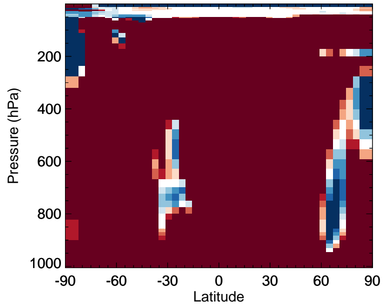
v11-02f-Run0 / v11-02e-Run0 NPMN - Zonal mean % diff for Oct
