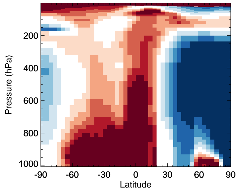
v11-02f-Run0 / v11-02e-Run1 R4N2 - Zonal mean % diff for Oct
