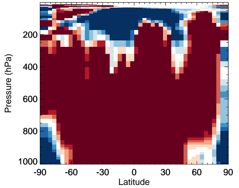
v11-02f-Run0 / v11-02e-Run1 LVOC - Zonal mean % diff for Oct
