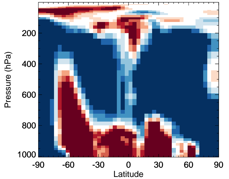
v11-02f-Run0 / v11-02e-Run0 DHDN - Zonal mean % diff for Oct
