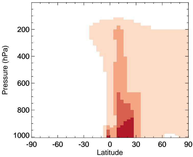
v11-02f-Run0 - v11-02e-Run1 ACET - Zonal mean abs diff for Oct
