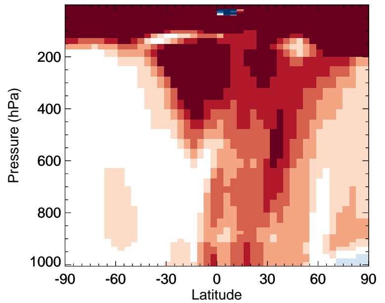
v11-02f-Run0 / v11-02e-Run0 ACET - Zonal mean % diff for Oct
