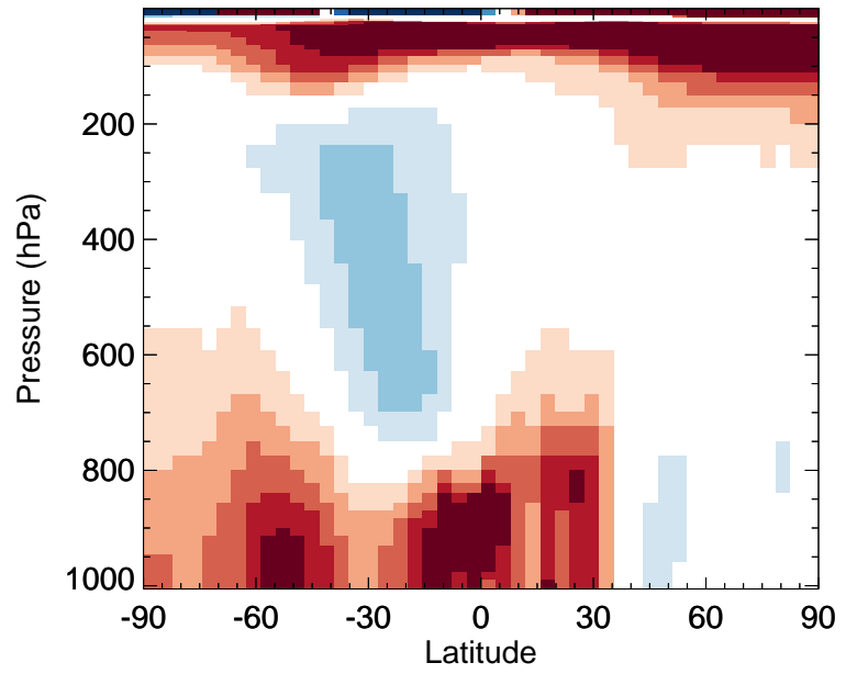
v11-02f-Run0 / v11-02e-Run1 PAN - Zonal mean % diff for Oct
