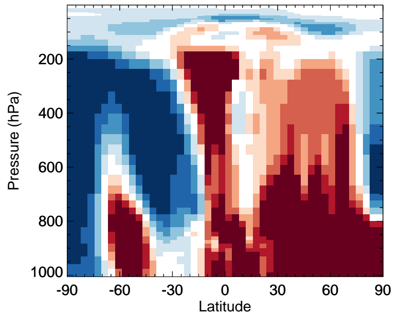
v11-02f-Run0 / v11-02e-Run0 SOAMG - Zonal mean % diff for Oct
