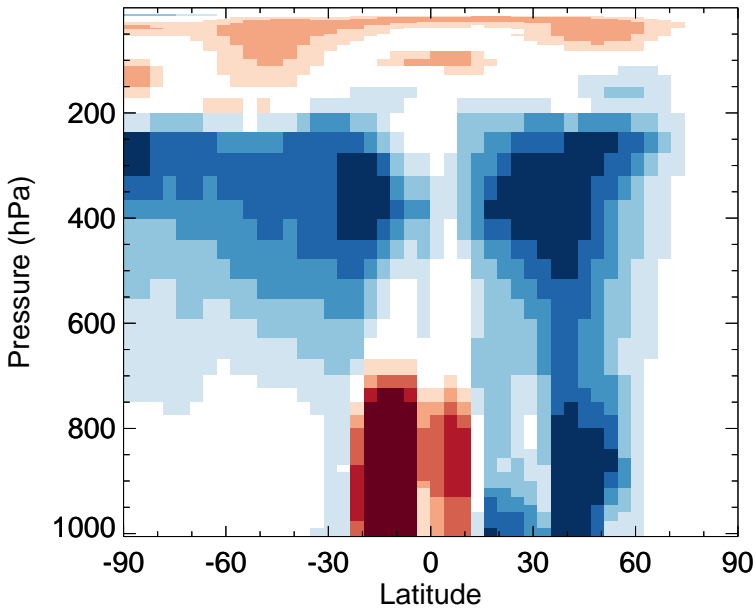
v11-02f-Run0 - v11-02e-Run1 OH - Zonal mean abs diff for Oct
