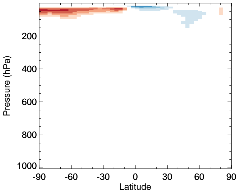
v11-02f-Run0 - v11-02e-Run0 CFC12 - Zonal mean abs diff for Oct
