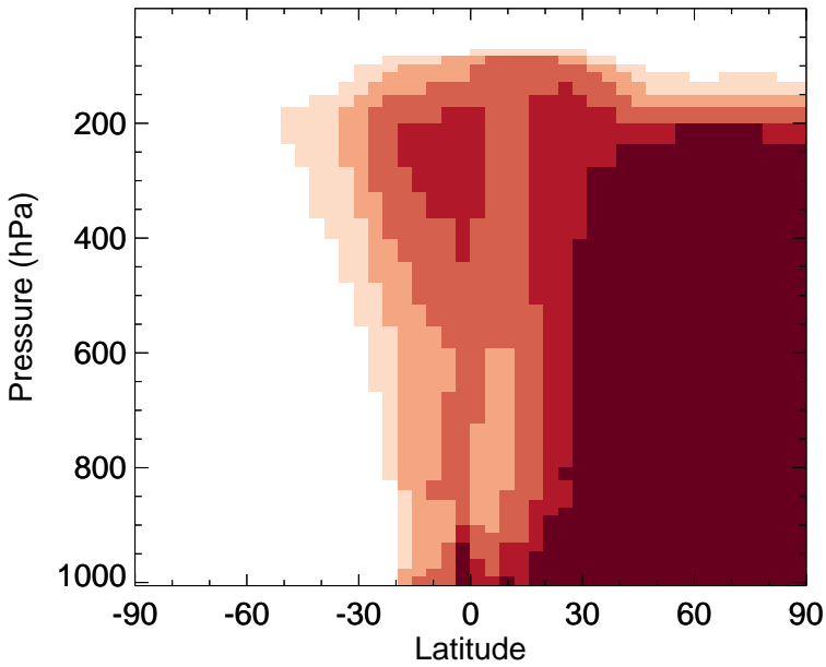
v11-02f-Run0 - v11-02e-Run0 C2H6 - Zonal mean abs diff for Oct
