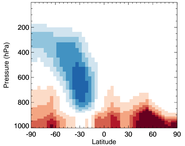
v11-02f-Run0 / v11-02e-Run1 SO4 - Zonal mean % diff for Oct
