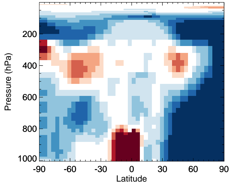
v11-02f-Run0 / v11-02e-Run1 CINO3 - Zonal mean % diff for Oct
