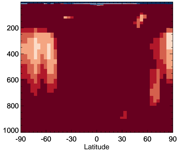
v11-02f-Run0 / v11-02e-Run0 ALK4 - Zonal mean % diff for Oct
