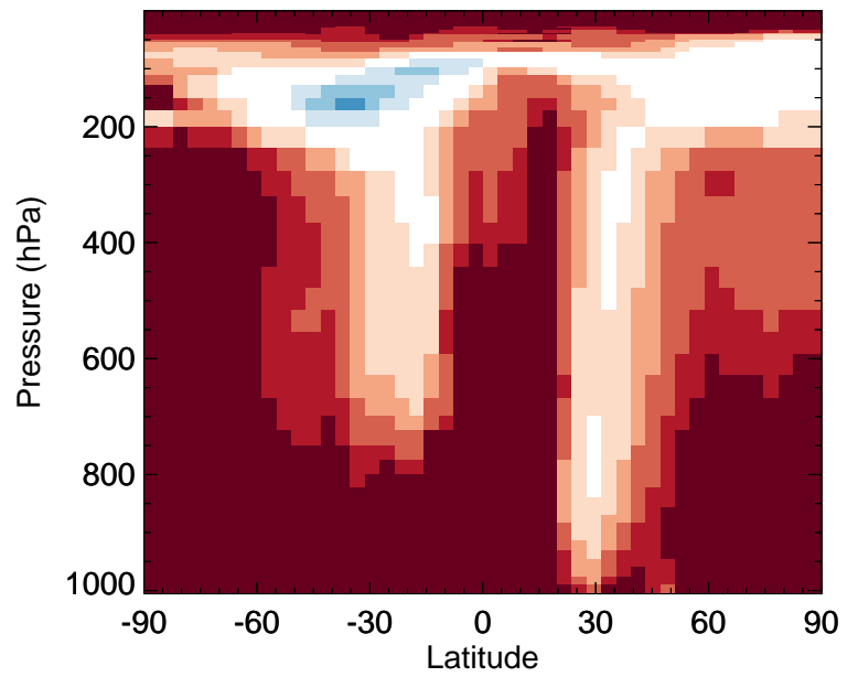
v11-02f-Run0 / v11-02e-Run1 RCHO - Zonal mean % diff for Oct
