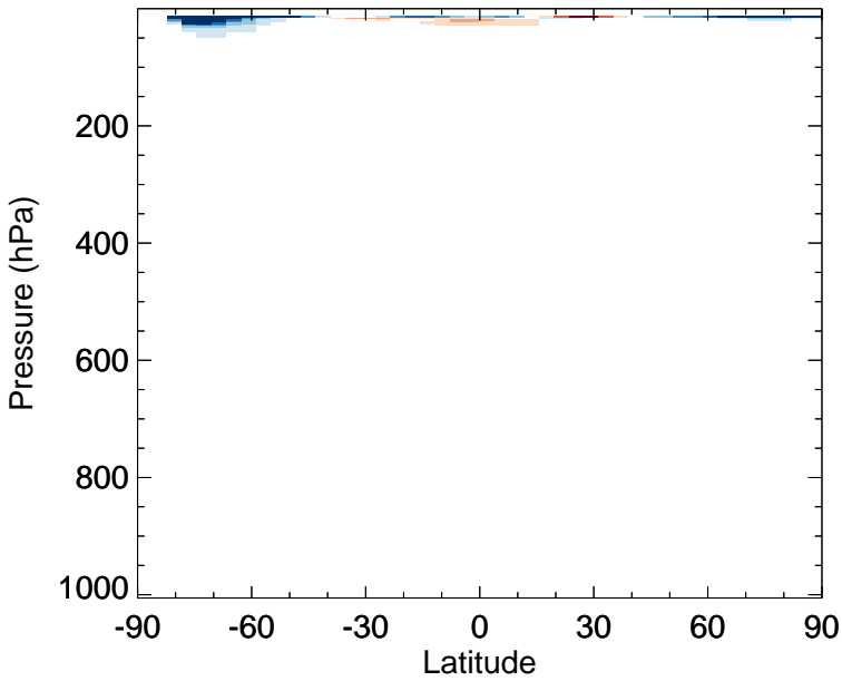
v11-02f-Run0 - v11-02e-Run0 NO3 - Zonal mean abs diff for Oct
