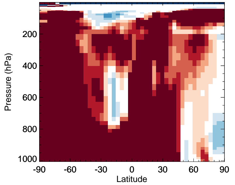
v11-02f-Run0 / v11-02e-Run1 NPMN - Zonal mean % diff for Oct
