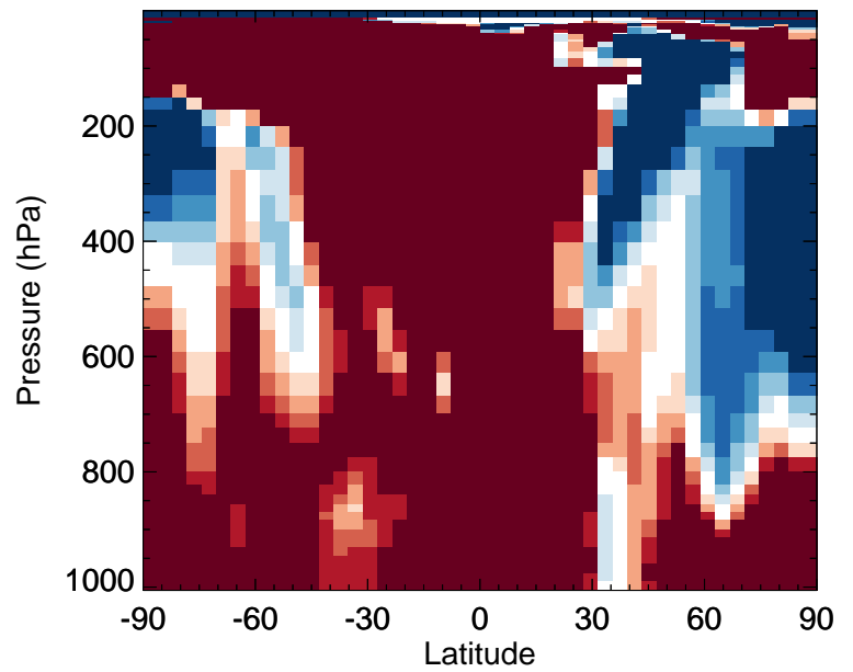
v11-02f-Run0 / v11-02e-Run0 TOLU - Zonal mean % diff for Oct
