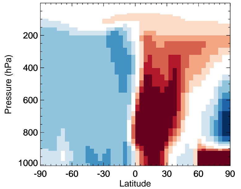
v11-02f-Run0 / v11-02e-Run1 BCPI - Zonal mean % diff for Oct
