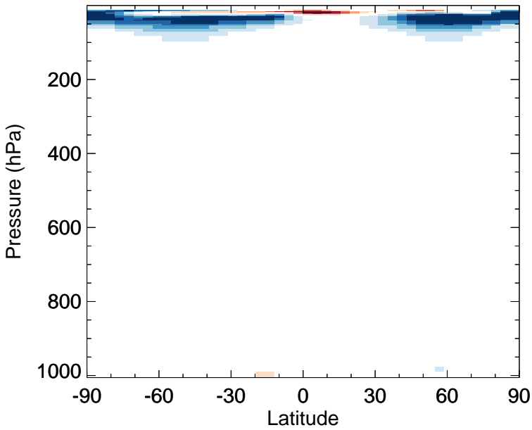
v11-02f-Run0 - v11-02e-Run0 NO 2 - Zonal mean abs diff for Oct
