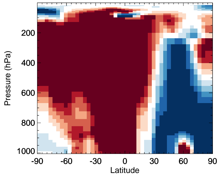
v11-02f-Run0 / v11-02e-Run0 ASOG1 - Zonal mean % diff for Oct
