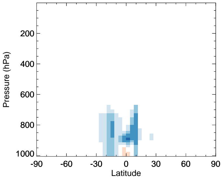
v11-02f-Run0 - v11-02e-Run0 MVK - Zonal mean abs diff for Oct
