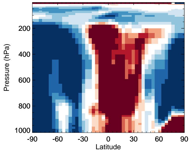
v11-02f-Run0 / v11-02e-Run0 BCPI - Zonal mean % diff for Oct
