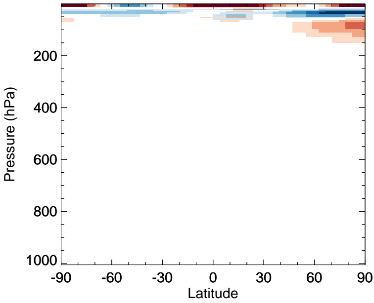
v11-02f-Run0 - v11-02e-Run1 HCl - Zonal mean abs diff for Oct
