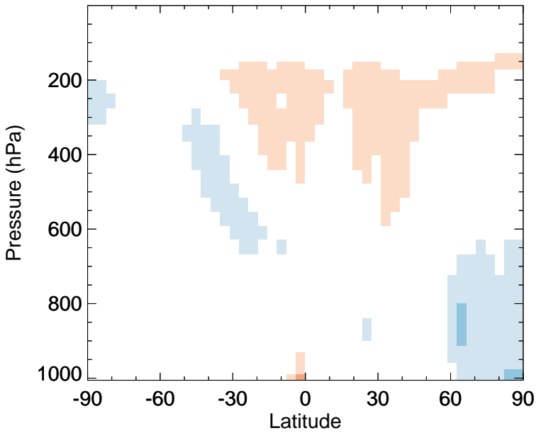
v11-02f-Run0 - v11-02e-Run0 PAN - Zonal mean abs diff for Oct
