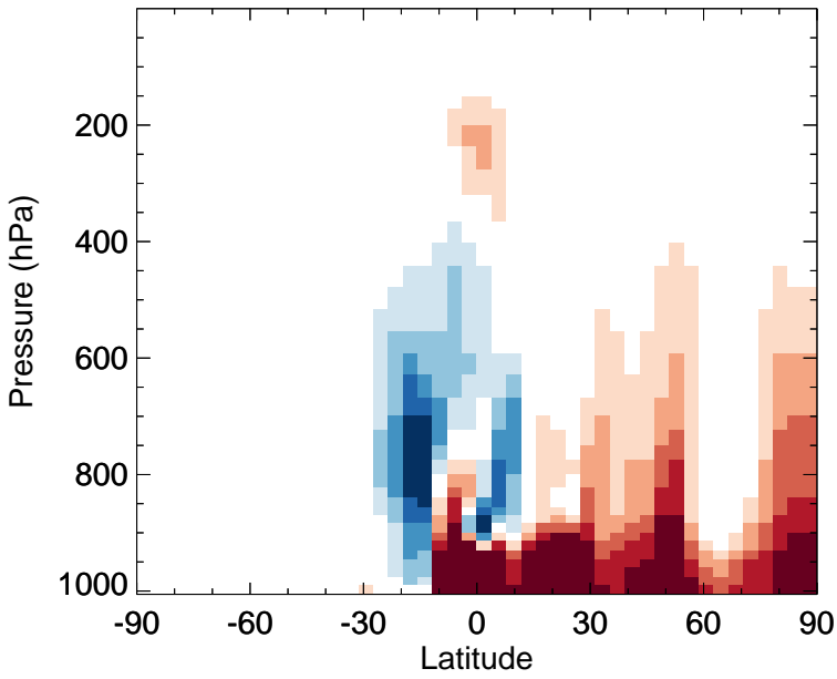
v11-02f-Run0 - v11-02e-Run0 MEK - Zonal mean abs diff for Oct
