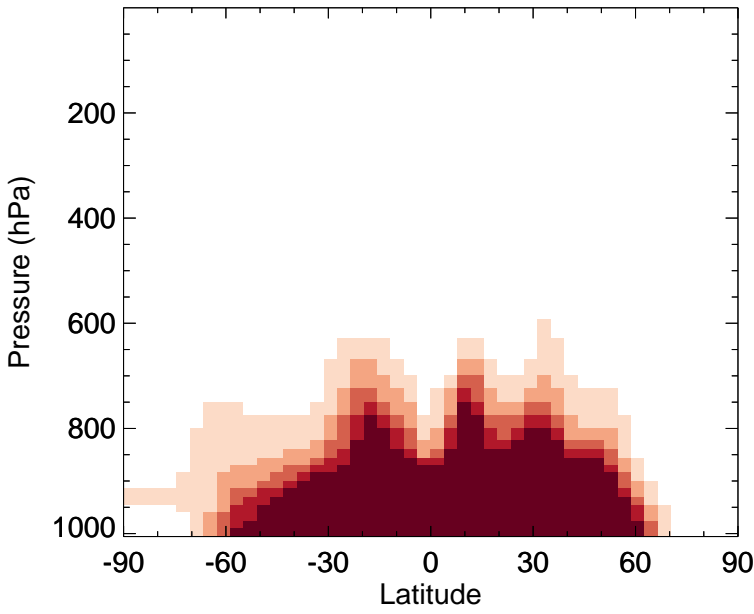
v11-02f-Run0 - v11-02e-Run1 NH3 - Zonal mean abs diff for Oct
