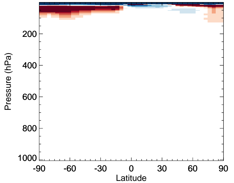
v11-02f-Run0 / v11-02e-Run0 CH3Cl - Zonal mean % diff for Oct
