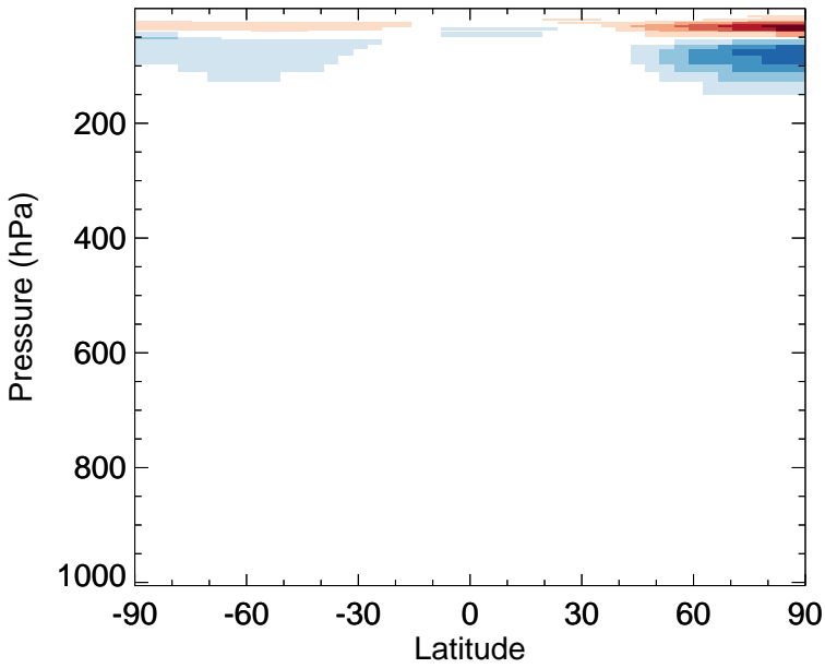
v11-02f-Run0 - v11-02e-Run1 CINO3 - Zonal mean abs diff for Oct
