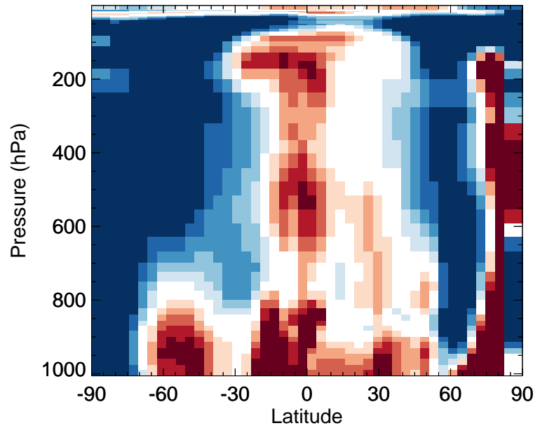
v11-02f-Run0 / v11-02e-Run0 NO - Zonal mean % diff for Oct
