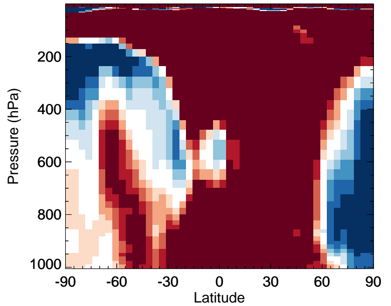
v11-02f-Run0 / v11-02e-Run0 EOH - Zonal mean % diff for Oct
