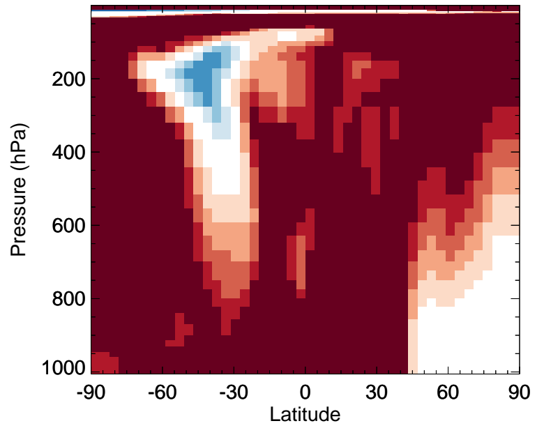
v11-02f-Run0 / v11-02e-Run1 EOH - Zonal mean % diff for Oct
