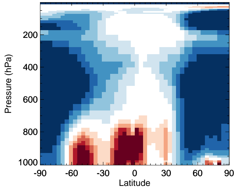
v11-02f-Run0 / v11-02e-Run1 HNO 4 - Zonal mean % diff for Oct
