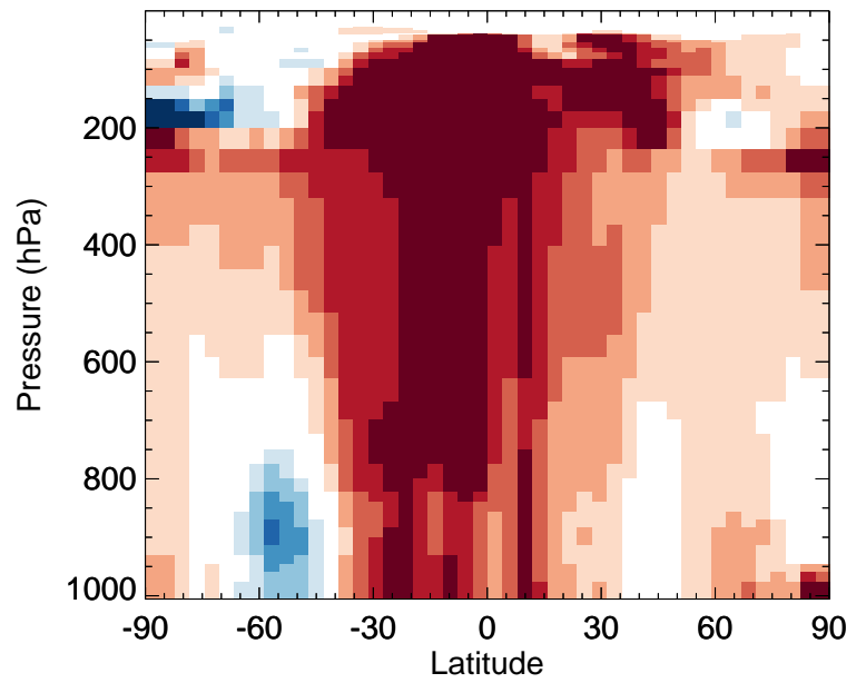
v11-02f-Run0 / v11-02e-Run1 NITs - Zonal mean % diff for Oct
