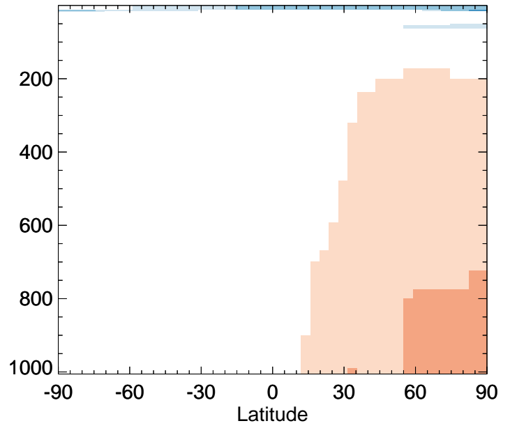
v11-02f-Run0 / v11-02e-Run1 CO - Zonal mean % diff for Oct
