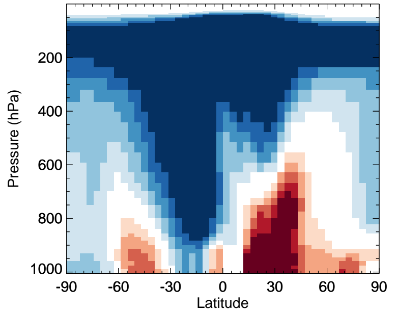
v11-02f-Run0 / v11-02e-Run1 ISOA1 - Zonal mean % diff for Oct
