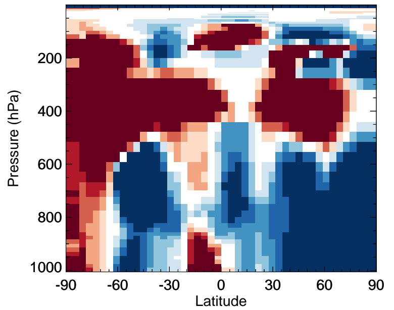
v11-02f-Run0 / v11-02e-Run1 Cl2 - Zonal mean % diff for Oct
