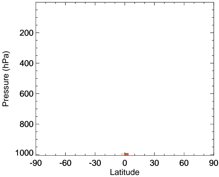
v11-02f-Run0 - v11-02e-Run0 MTPA - Zonal mean abs diff for Oct
