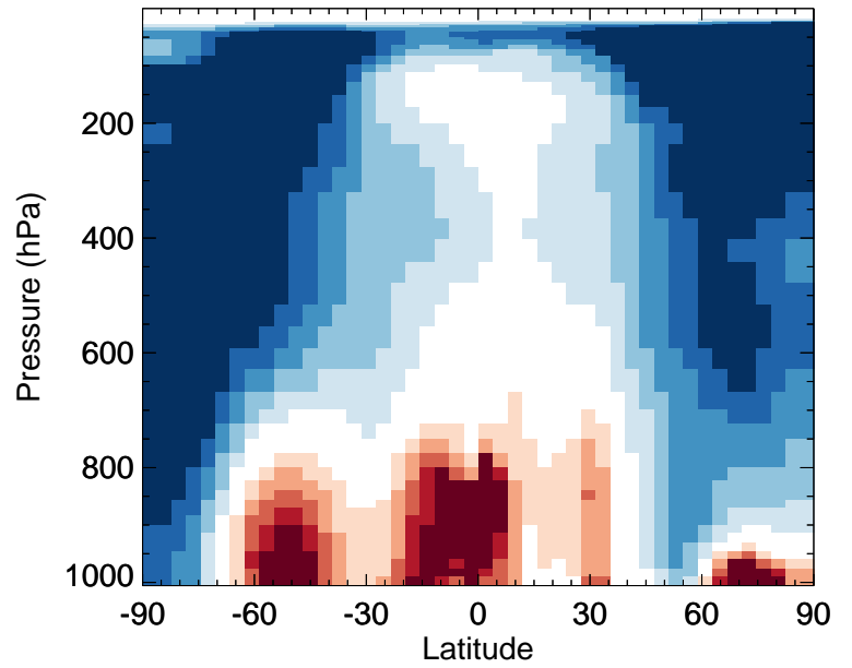
v11-02f-Run0 / v11-02e-Run1 NO 2 - Zonal mean % diff for Oct
