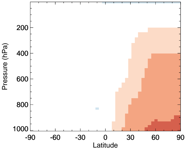
v11-02f-Run0 - v11-02e-Run1 CO - Zonal mean abs diff for Oct
