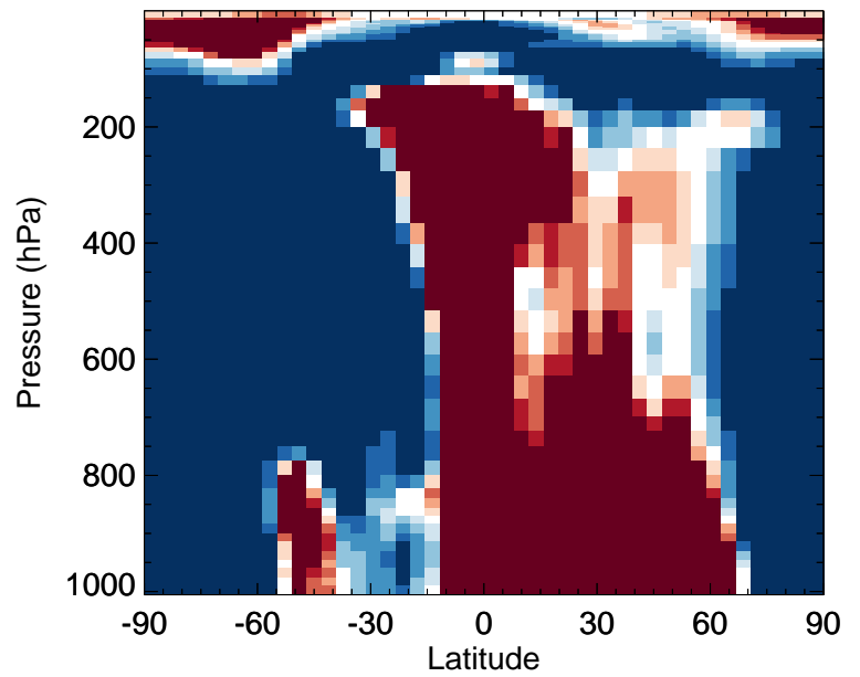
v11-02f-Run0 / v11-02e-Run0 ISOA3 - Zonal mean % diff for Oct
