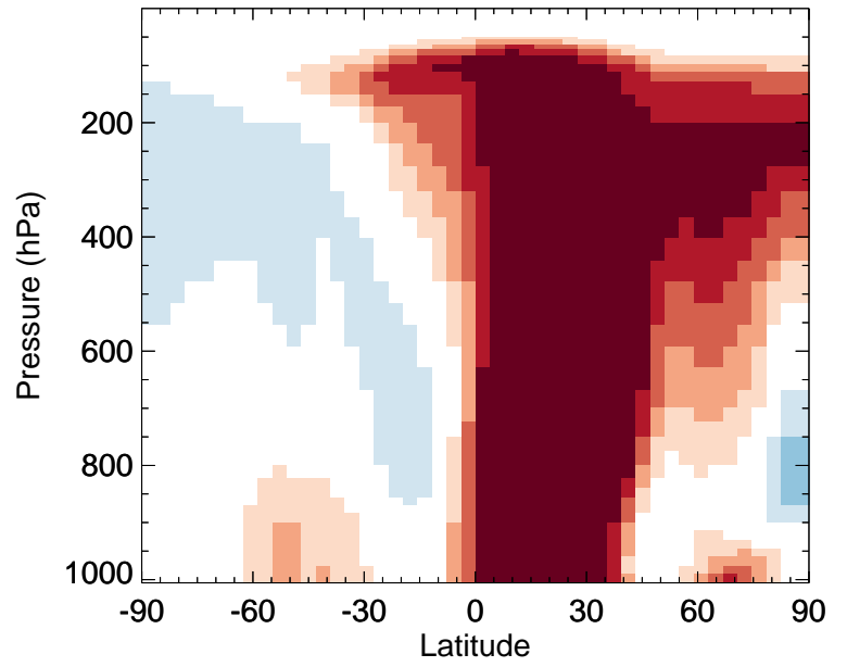
v11-02f-Run0 / v11-02e-Run1 OCPI - Zonal mean % diff for Oct
