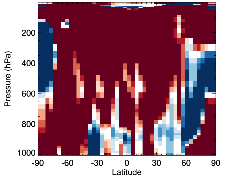
v11-02f-Run0 / v11-02e-Run0 BCPO - Zonal mean % diff for Oct
