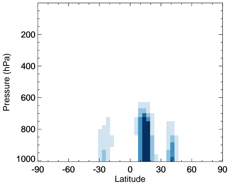
v11-02f-Run0 - v11-02e-Run0 DST3 - Zonal mean abs diff for Oct
