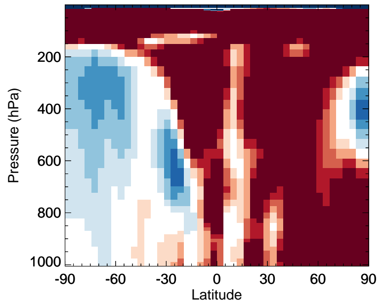
v11-02f-Run0 / v11-02e-Run0 C3H8 - Zonal mean % diff for Oct
