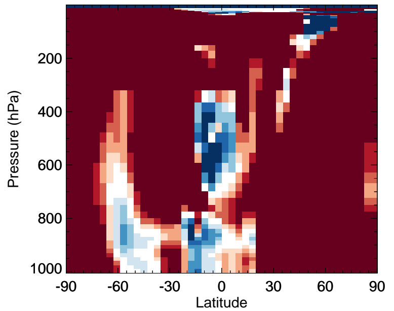
v11-02f-Run0 / v11-02e-Run0 DMS - Zonal mean % diff for Oct
