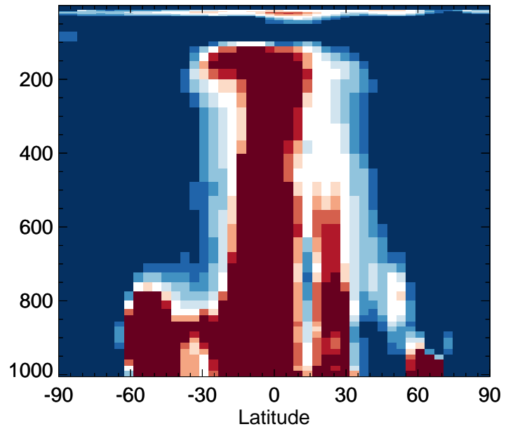
v11-02f-Run0 / v11-02e-Run0 N2O5 - Zonal mean % diff for Oct
