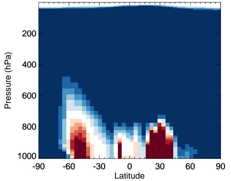
v11-02f-Run0 / v11-02e-Run1 DHDN - Zonal mean % diff for Oct
