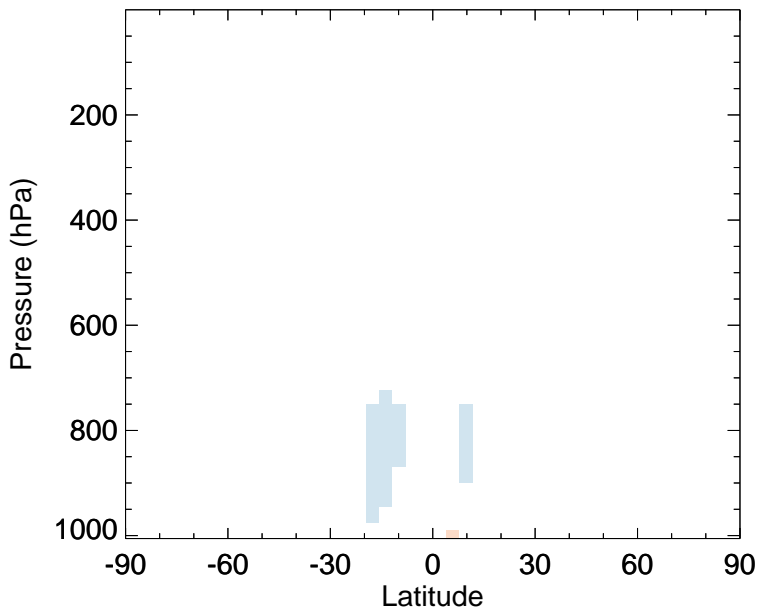
v11-02f-Run0 - v11-02e-Run1 HAC - Zonal mean abs diff for Oct
