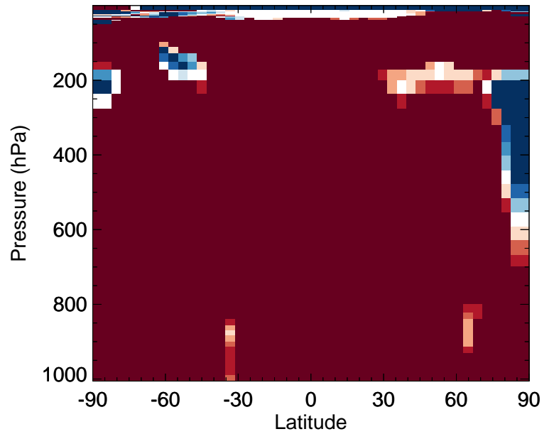
v11-02f-Run0 / v11-02e-Run0 PRPE - Zonal mean % diff for Oct
