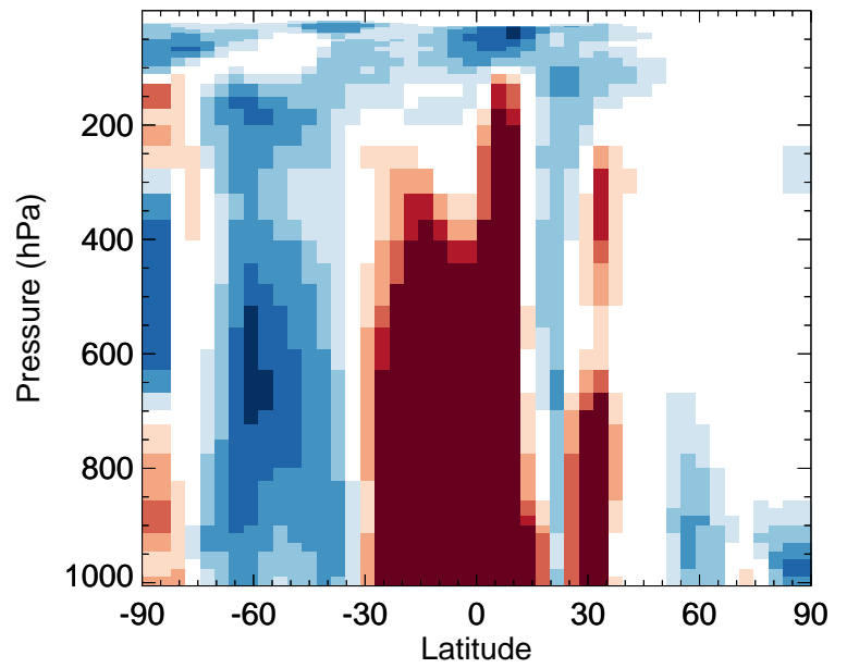
v11-02f-Run0 / v11-02e-Run1 SOAP - Zonal mean % diff for Oct
