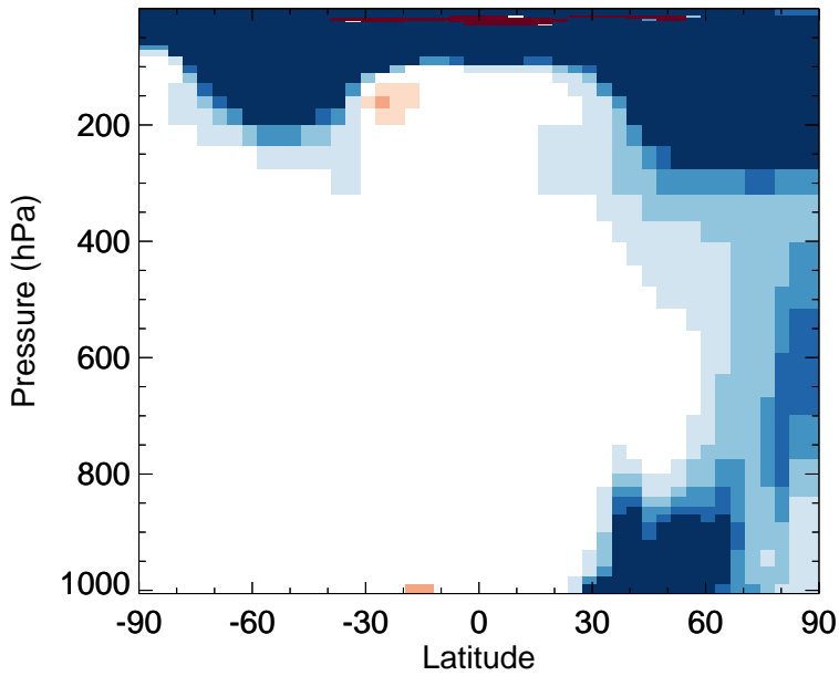
v11-02f-Run0 - v11-02e-Run0 N2O5 - Zonal mean abs diff for Oct
