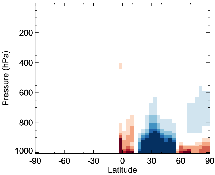
v11-02f-Run0 - v11-02e-Run1 TOLU - Zonal mean abs diff for Oct
