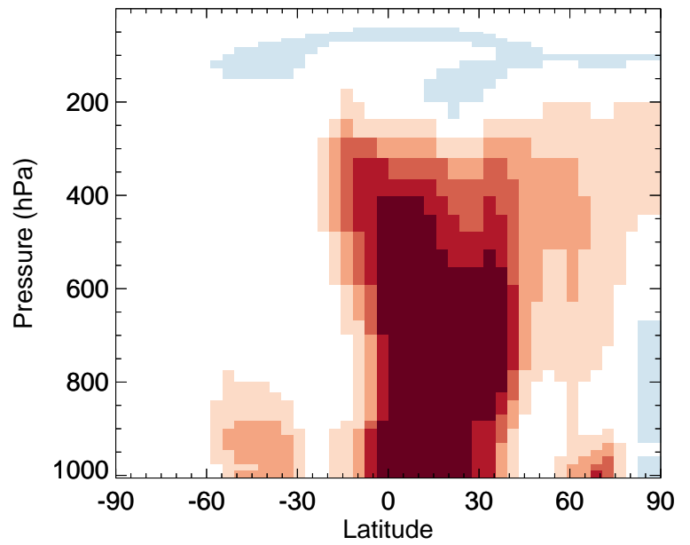
v11-02f-Run0 / v11-02e-Run1 ISOA2 - Zonal mean % diff for Oct
