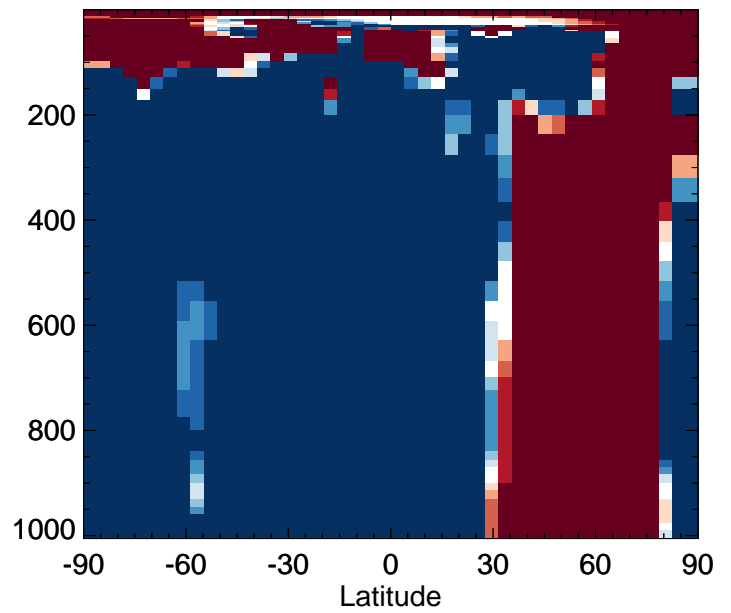
v11-02f-Run0 / v11-02e-Run0 DST4 - Zonal mean % diff for Oct
