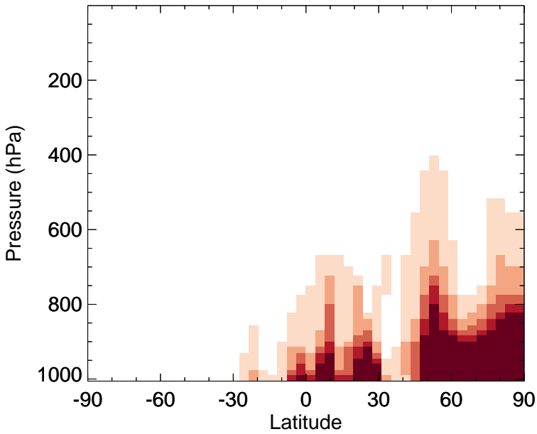
v11-02f-Run0 - v11-02e-Run0 ALK4 - Zonal mean abs diff for Oct
