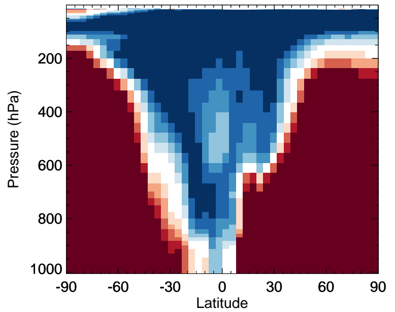
v11-02f-Run0 / v11-02e-Run1 IMAE - Zonal mean % diff for Oct
