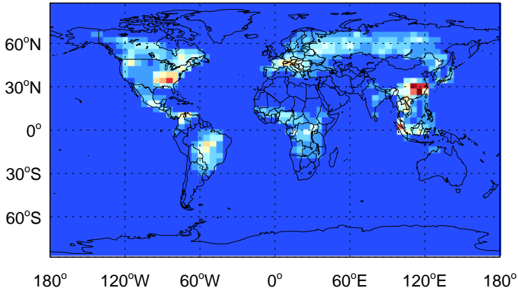
MONITA - Species map @ surface for Jul
