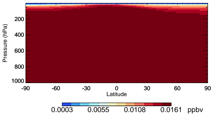
v11-02f-Run0 CFC114 - Species Zonal Mean for Apr
