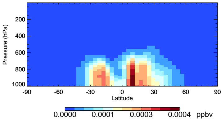
v11-02f-Run0 ISN10A - Species Zonal Mean for Apr
