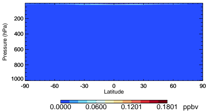
v11-02f-Run0 NO3 - Species Zonal Mean for Apr
