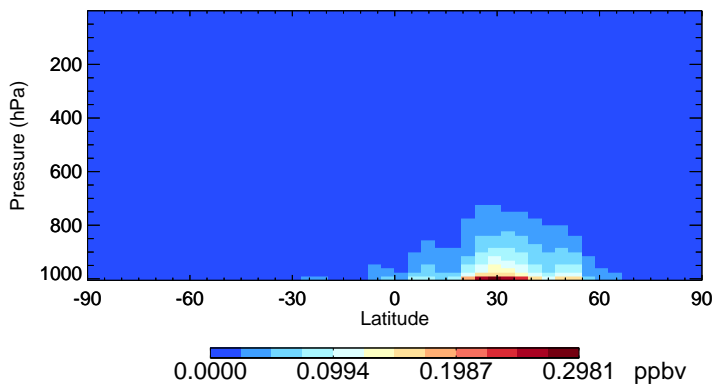
v11-02f-Run0 BCPO - Species Zonal Mean for Apr
