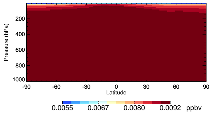
v11-02f-Run0 CFC115 - Species Curtain @ -180.000 for Apr
