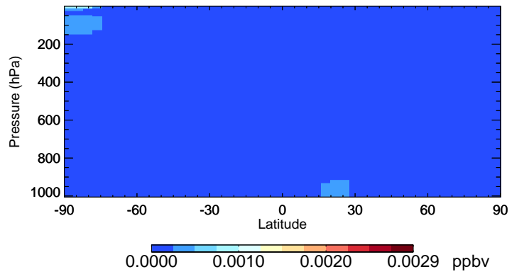
v11-02f-Run0 Br2 - Species Curtain @ -180.000 for Apr
