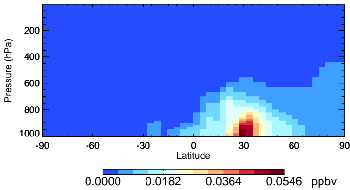
v11-02f-Run0 SOAGX - Species Zonal Mean for Apr
