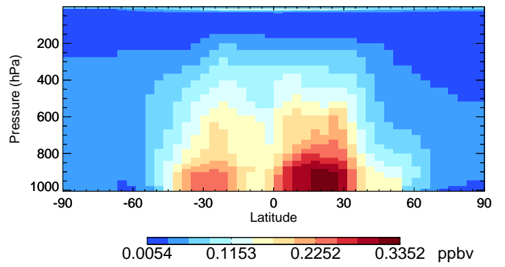
v11-02e-Run1 CH2O - Species Curtain @ -180.000 for Apr
