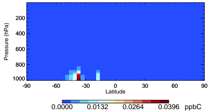
v11-02f-Run0 ISOP - Species Curtain @ -180.000 for Apr
