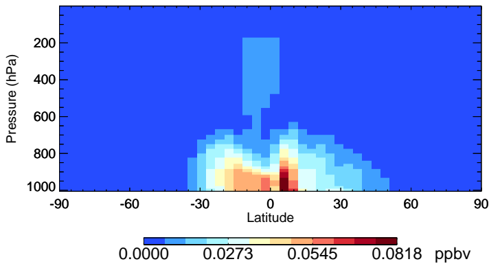
v11-02f-Run0 HAC - Species Zonal Mean for Apr
