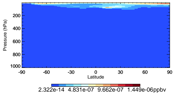
v11-02f-Run0 CIOO - Species Curtain @ -180.000 for Apr
