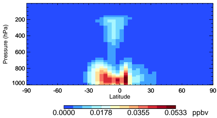
v11-02f-Run0 IEPOXA - Species Zonal Mean for Apr
