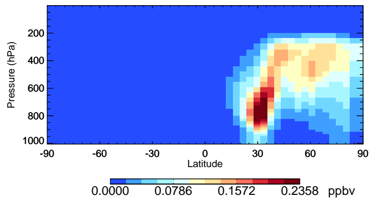
v11-02f-Run0 DST2 - Species Curtain @ -180.000 for Apr
