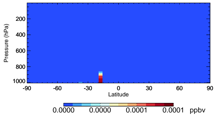
v11-02e-Run1 LIMO - Species Curtain @ -180.000 for Apr
