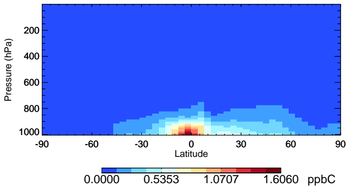
v11-02f-Run0 ALD2 - Species Zonal Mean for Apr
