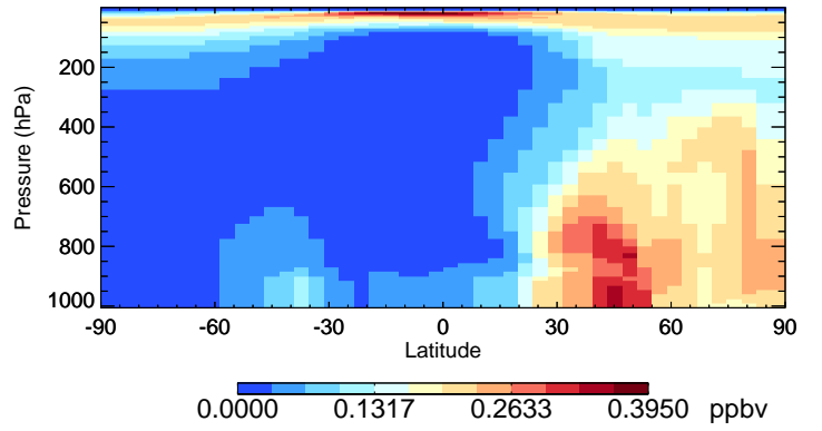
v11-02e-Run1 SO4 - Species Curtain @ -180.000 for Apr
