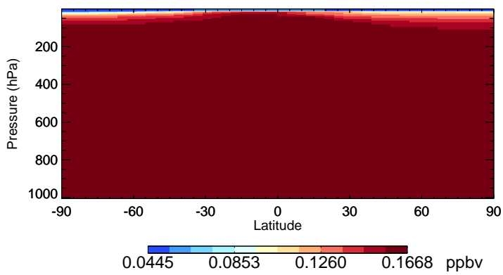
v11-02f-Run0 HCFC22 - Species Zonal Mean for Apr
