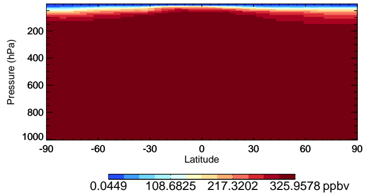
v11-02e-Run0 N2O - Species Curtain @ -180.000 for Apr
