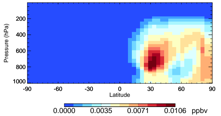
v11-02f-Run0 SOAGX - Species Curtain @ -180.000 for Apr
