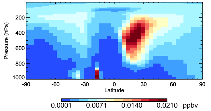
v11-02e-Run0 TSOG3 - Species Curtain @ -180.000 for Apr
