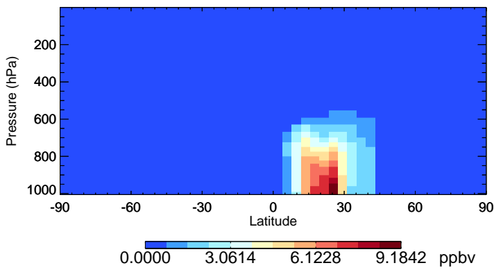
v11-02f-Run0 DST2 - Species Zonal Mean for Apr
