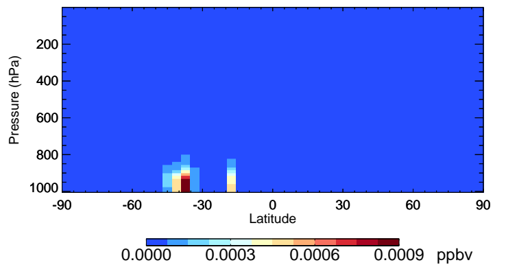
v11-02f-Run0 MONITS - Species Curtain @ -180.000 for Apr
