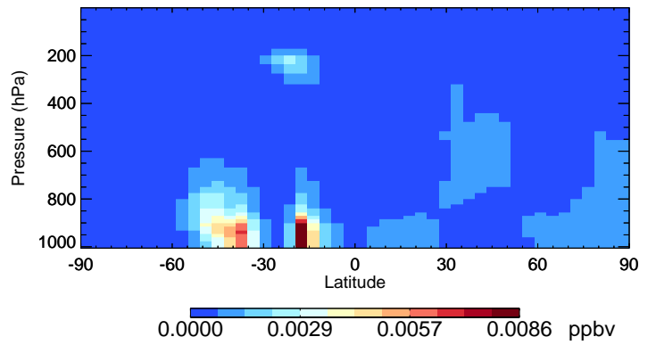
v11-02f-Run0 HAC - Species Curtain @ -180.000 for Apr
