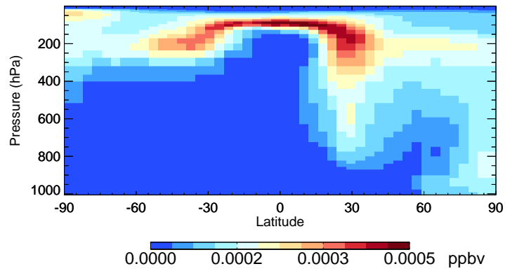
v11-02f-Run0 TSOA1 - Species Curtain @ -180.000 for Apr
