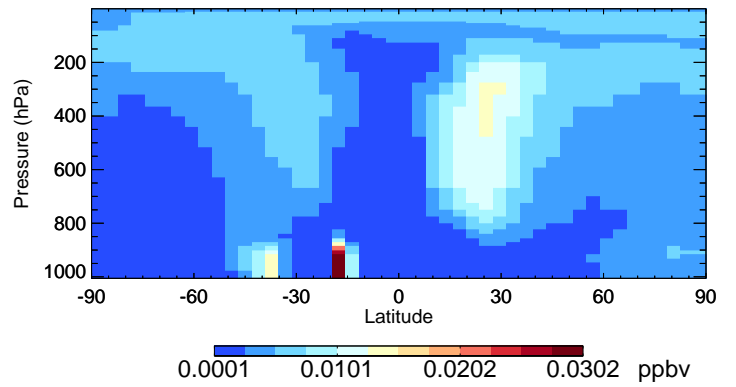
v11-02f-Run0 TSOG3 - Species Curtain @ -180.000 for Apr
