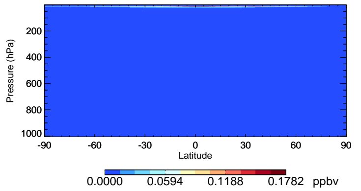
v11-02e-Run1 NO3 - Species Curtain @ -180.000 for Apr
