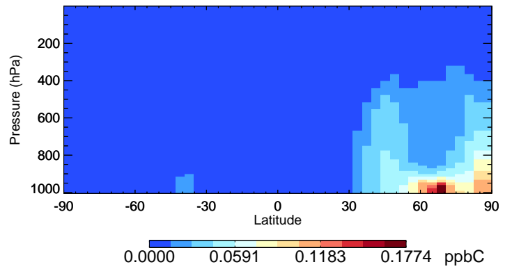
v11-02f-Run0 TOLU - Species Curtain @ -180.000 for Apr
