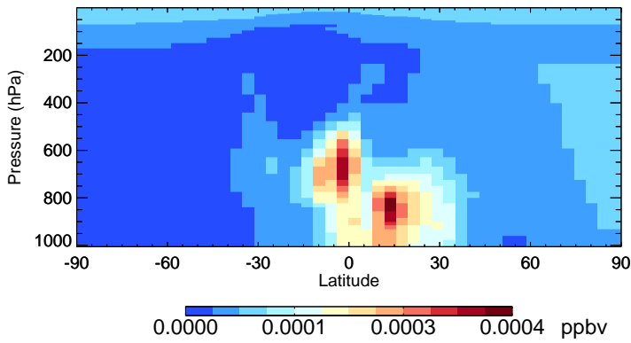
v11-02f-Run0 SOAME - Species Zonal Mean for Apr
