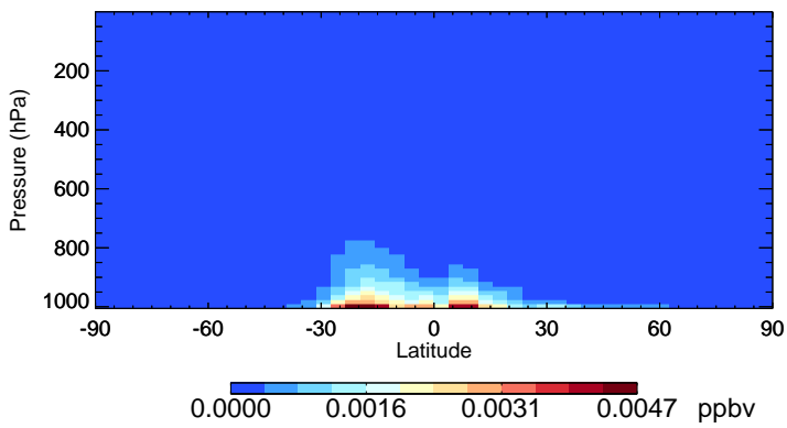
v11-02f-Run0 MONITS - Species Zonal Mean for Apr
