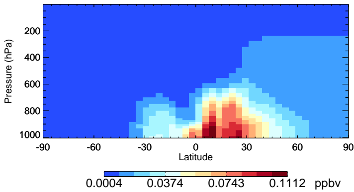
v11-02f-Run0 INDIOL - Species Zonal Mean for Apr
