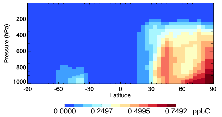
v11-02e-Run1 ALK4 - Species Curtain @ -180.000 for Apr
