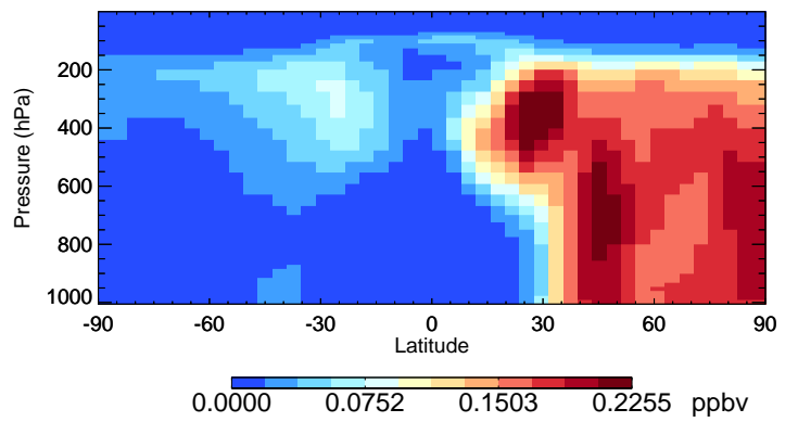
v11-02f-Run0 PAN - Species Curtain @ -180.000 for Apr
