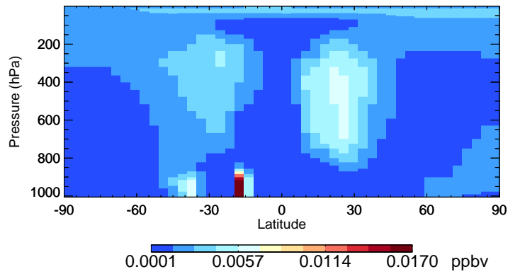
v11-02f-Run0 TSOG2 - Species Curtain @ -180.000 for Apr
