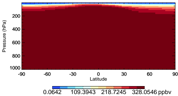
v11-02f-Run0 N2O - Species Zonal Mean for Apr
