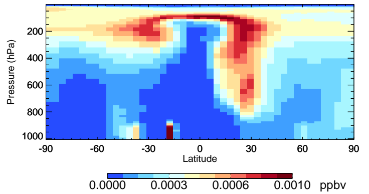
v11-02f-Run0 TSOA0 - Species Curtain @ -180.000 for Apr
