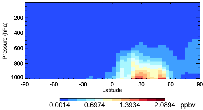
v11-02f-Run0 OCPI - Species Zonal Mean for Apr
