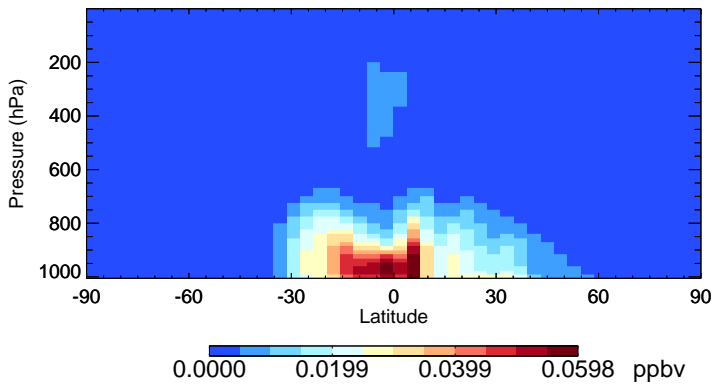
v11-02f-Run0 GLYC - Species Zonal Mean for Apr
