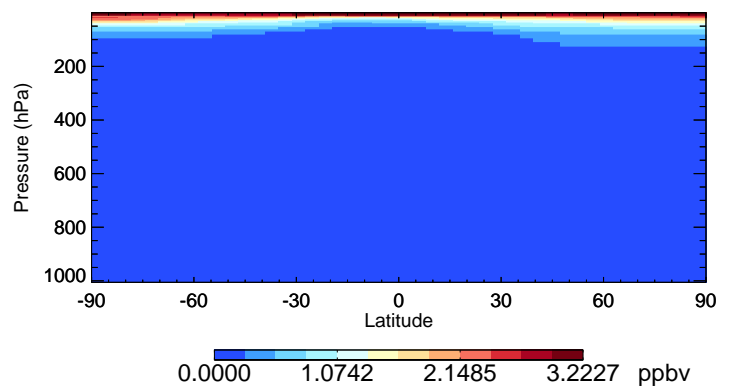
v11-02f-Run0 HCl - Species Curtain @ -180.000 for Apr
