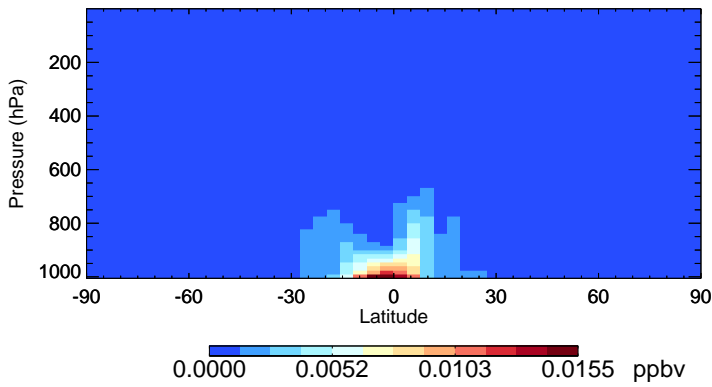
v11-02f-Run0 TSOA1 - Species Zonal Mean for Apr
