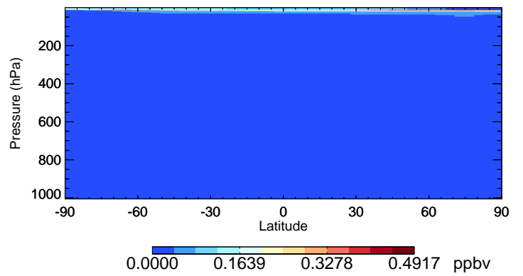
v11-02f-Run0 ClO - Species Curtain @ -180.000 for Apr
