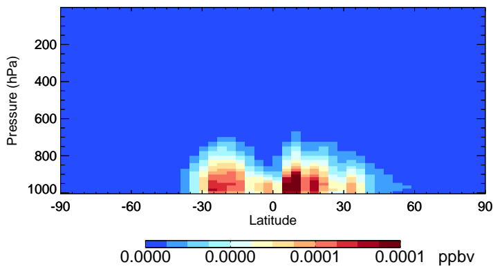
v11-02f-Run0 ETHLN - Species Zonal Mean for Apr
