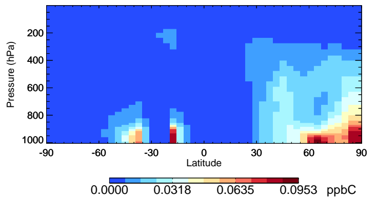
v11-02f-Run0 EOH - Species Curtain @ -180.000 for Apr
