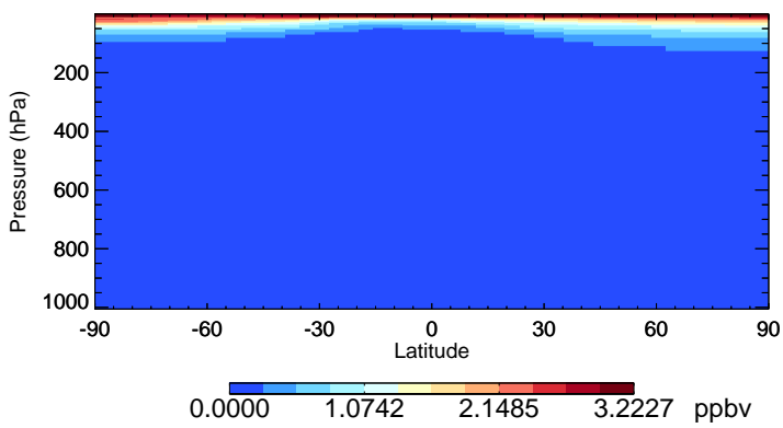
v11-02f-Run0 HCl - Species Zonal Mean for Apr
