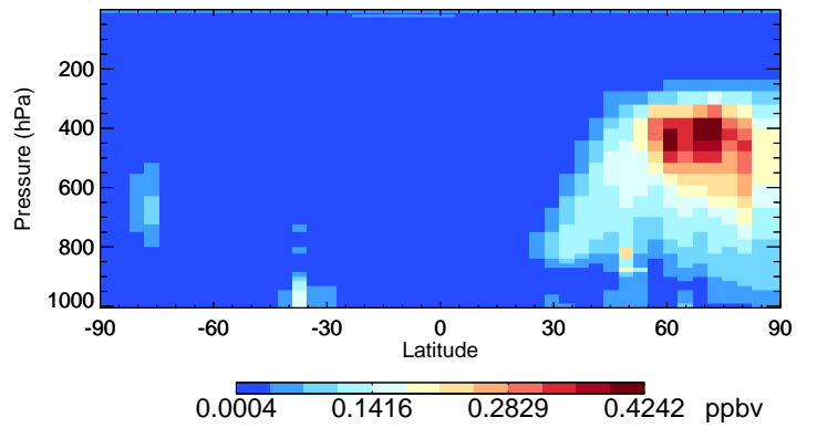
v11-02f-Run0 SO2 - Species Curtain @ -180.000 for Apr
