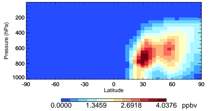
v11-02e-Run0 DST1 - Species Curtain @ -180.000 for Apr
