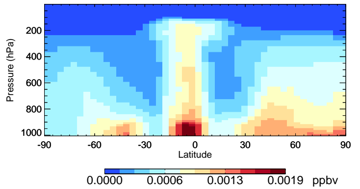
v11-02f-Run0 CHBr3 - Species Curtain @ -180.000 for Apr
