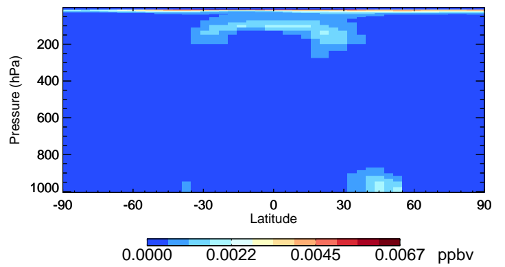
v11-02f-Run0 HNO 2 - Species Curtain @ -180.000 for Apr
