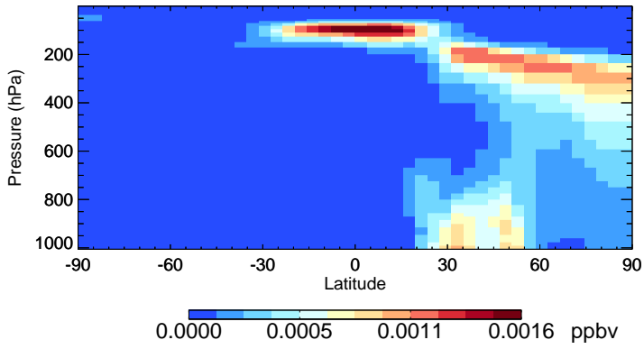
v11-02e-Run1 ASOA3 - Species Zonal Mean for Apr
