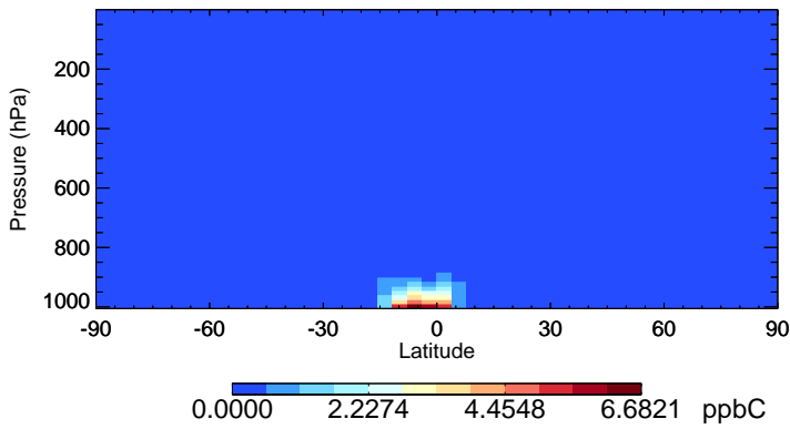
v11-02f-Run0 ISOP - Species Zonal Mean for Apr
