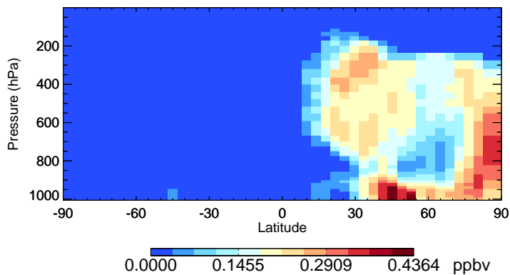
v11-02f-Run0 NIT - Species Curtain @ -180.000 for Apr
