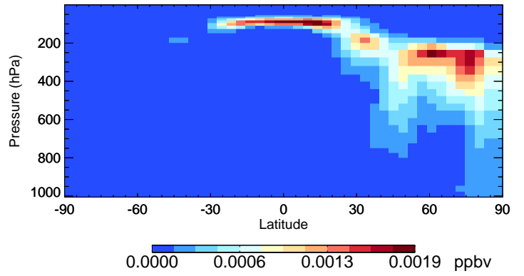
v11-02e-Run1 ASOA3 - Species Curtain @ -180.000 for Apr
