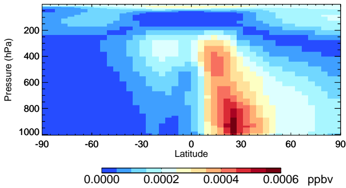
v11-02f-Run0 ASOG1 - Species Zonal Mean for Apr
