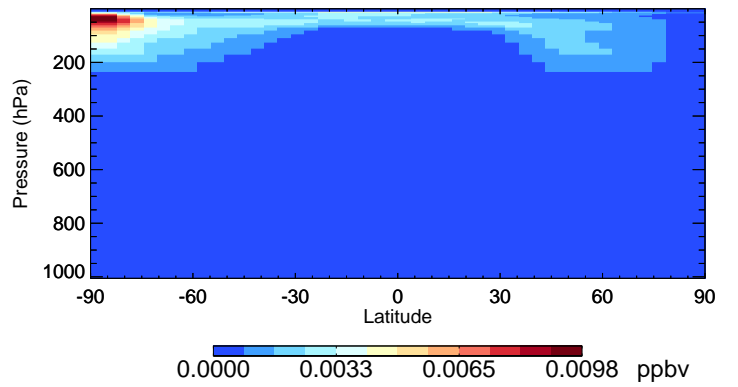
v11-02f-Run0 HOBr - Species Curtain @ -180.000 for Apr
