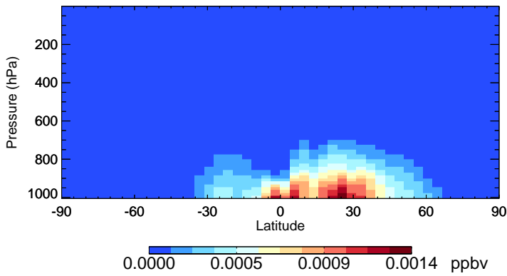
v11-02f-Run0 IONITA - Species Zonal Mean for Apr
