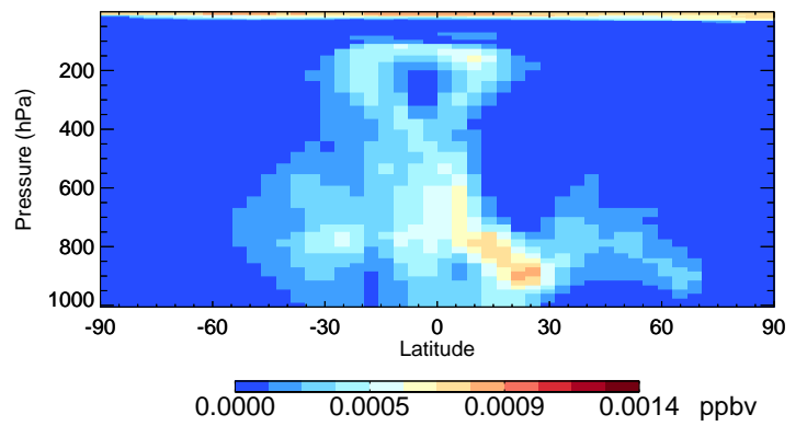
v11-02f-Run0 HBr - Species Curtain @ -180.000 for Apr
