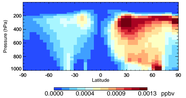
v11-02f-Run0 R4N2 - Species Curtain @ -180.000 for Apr
