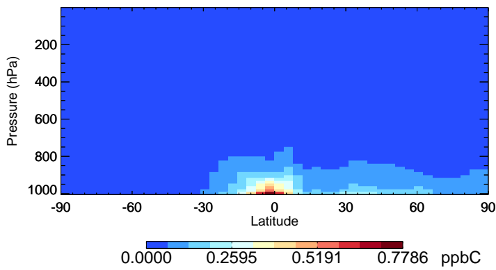
v11-02f-Run0 EOH - Species Zonal Mean for Apr
