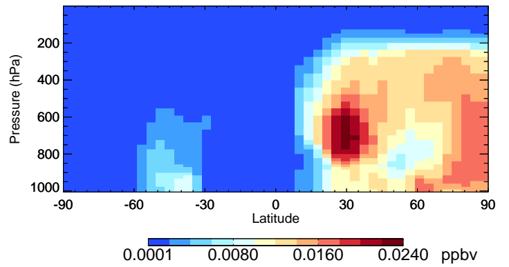
v11-02f-Run0 INDIOL - Species Curtain @ -180.000 for Apr
