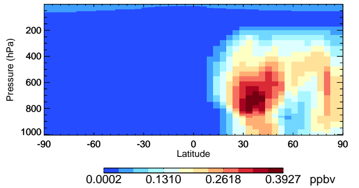
v11-02f-Run0 OCPI - Species Curtain @ -180.000 for Apr
