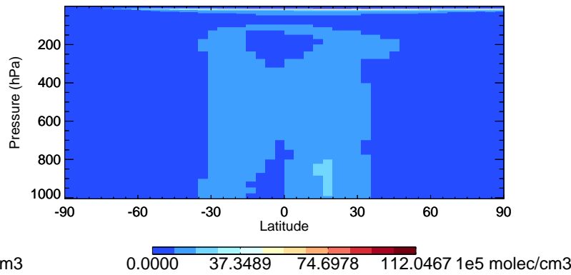
v11-02f-Run0 OH - Species Curtain @ -180.000 for Apr
