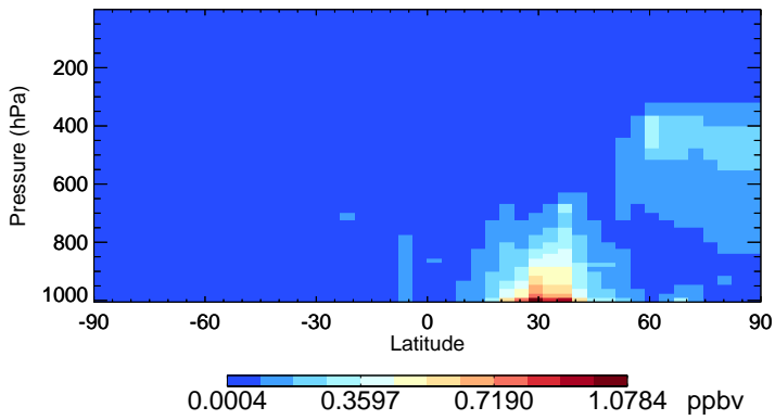
v11-02f-Run0 SO2 - Species Zonal Mean for Apr
