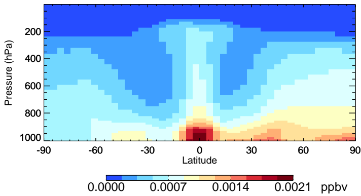
v11-02f-Run0 CHBr3 - Species Zonal Mean for Apr
