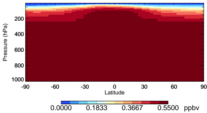
v11-02f-Run0 CH3Cl - Species Zonal Mean for Apr
