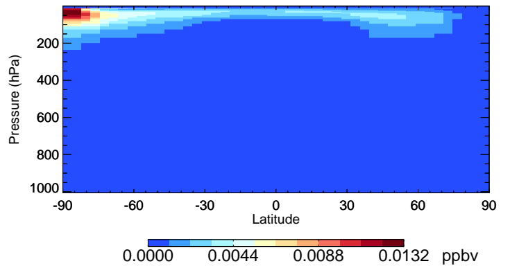
v11-02f-Run0 BrCl - Species Curtain @ -180.000 for Apr
