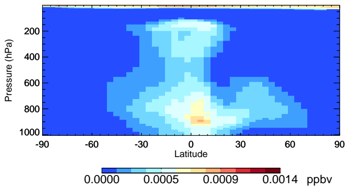
v11-02f-Run0 HBr - Species Zonal Mean for Apr
