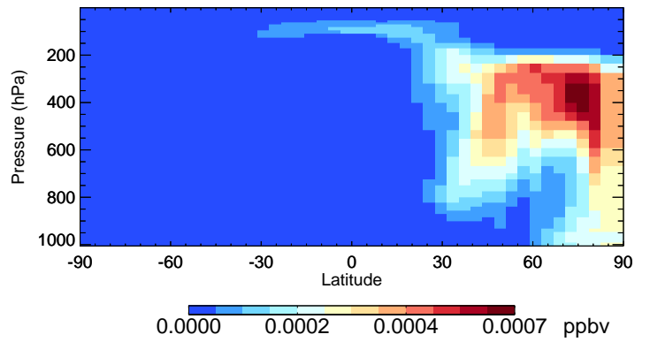
v11-02f-Run0 ASOA2 - Species Curtain @ -180.000 for Apr
