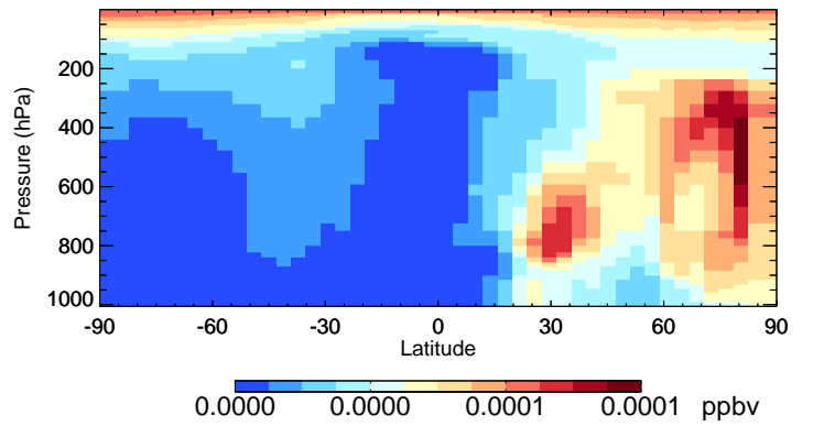
v11-02f-Run0 SOAME - Species Curtain @ -180.000 for Apr
