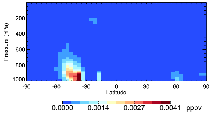
v11-02f-Run0 GLYC - Species Curtain @ -180.000 for Apr
