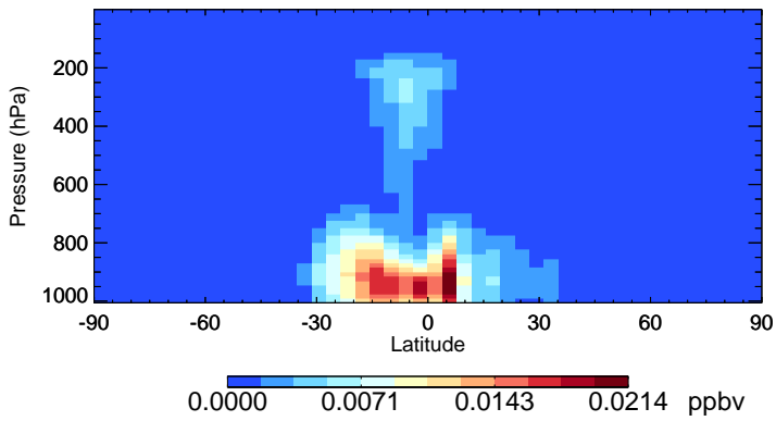
v11-02f-Run0 IEPOXB - Species Zonal Mean for Apr
