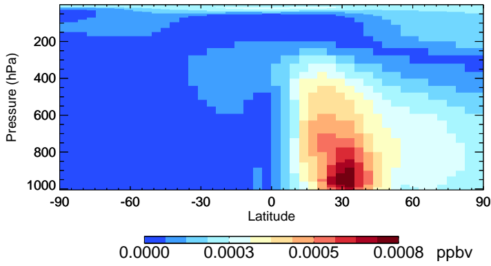
v11-02e-Run1 ASOG1 - Species Zonal Mean for Apr
