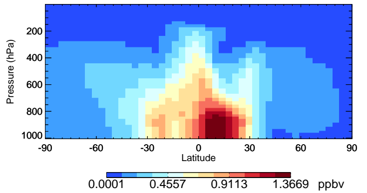
v11-02f-Run0 MP - Species Curtain @ -180.000 for Apr
