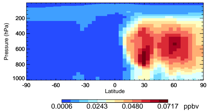
v11-02e-Run0 SOAS - Species Curtain @ -180.000 for Apr
