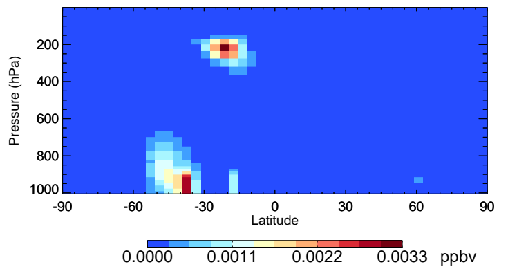
v11-02f-Run0 IEPOXA - Species Curtain @ -180.000 for Apr
