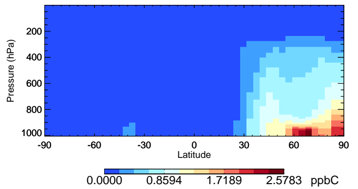
v11-02f-Run0 ALK4 - Species Curtain @ -180.000 for Apr
