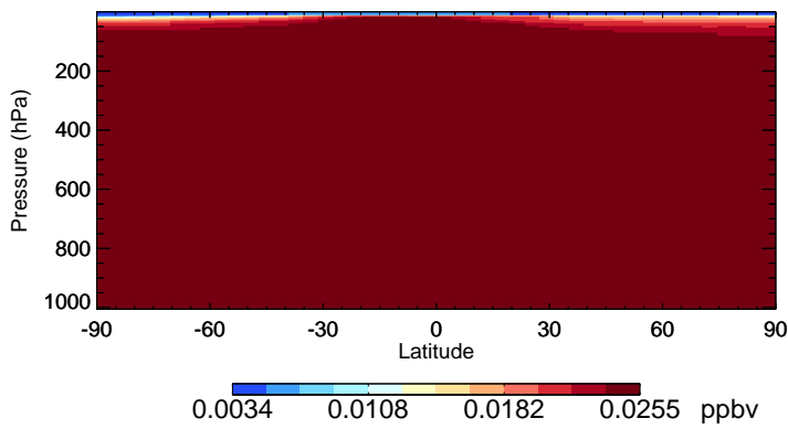
v11-02f-Run0 HCFC142b - Species Zonal Mean for Apr
