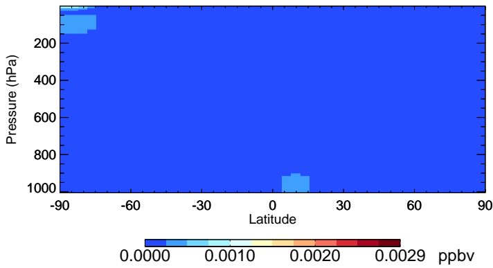
v11-02f-Run0 Br2 - Species Zonal Mean for Apr
