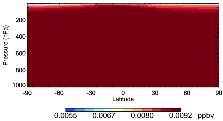
v11-02f-Run0 CFC115 - Species Zonal Mean for Apr
