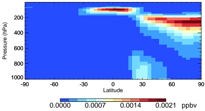
v11-02e-Run0 ASOA3 - Species Zonal Mean for Apr
