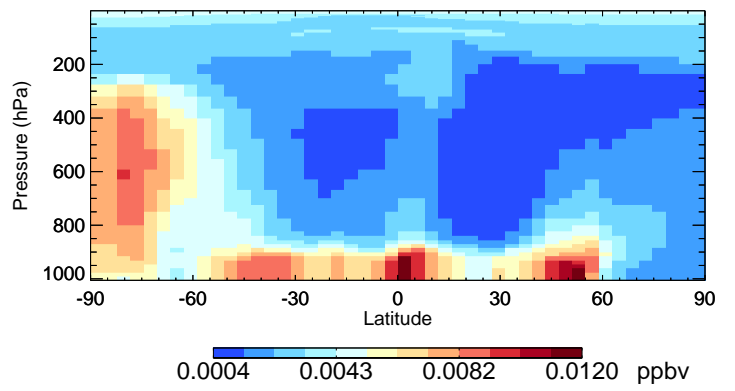
v11-02f-Run0 MSA - Species Curtain @ -180.000 for Apr
