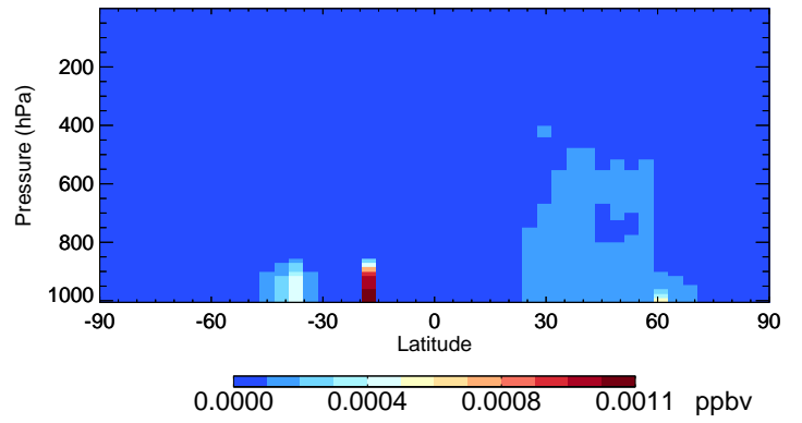
v11-02e-Run0 GLYX - Species Curtain @ -180.000 for Apr
