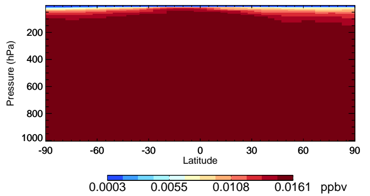
v11-02f-Run0 CFC114 - Species Curtain @ -180.000 for Apr
