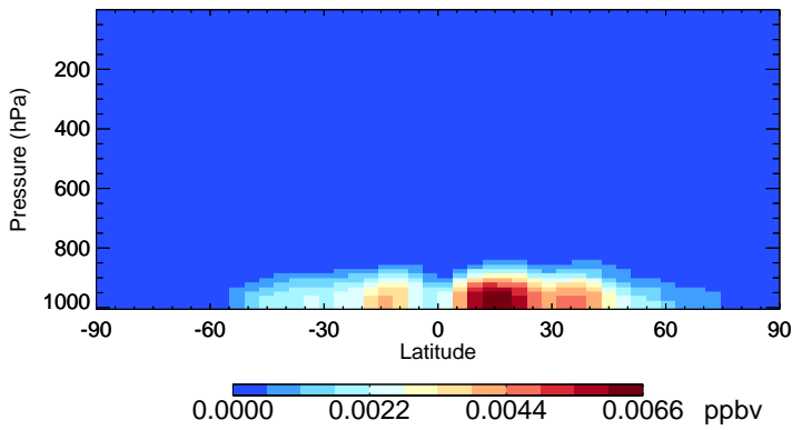
v11-02f-Run0 NITs - Species Zonal Mean for Apr
