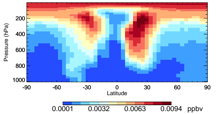
v11-02f-Run0 ISOG3 - Species Curtain @ -180.000 for Apr
