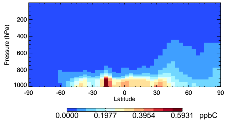
v11-02f-Run0 ALD2 - Species Curtain @ -180.000 for Apr
