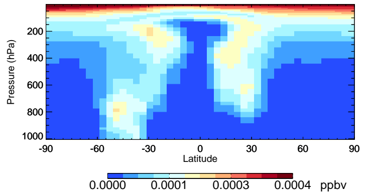
v11-02f-Run0 LVOCOA - Species Curtain @ -180.000 for Apr
