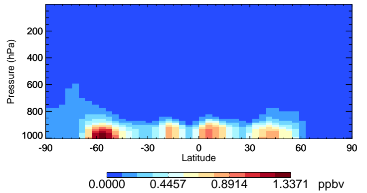
v11-02f-Run0 SALA - Species Curtain @ -180.000 for Apr
