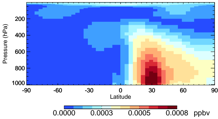
v11-02e-Run0 ASOG1 - Species Zonal Mean for Apr
