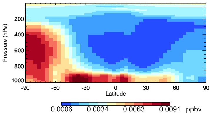
v11-02f-Run0 MSA - Species Zonal Mean for Apr
