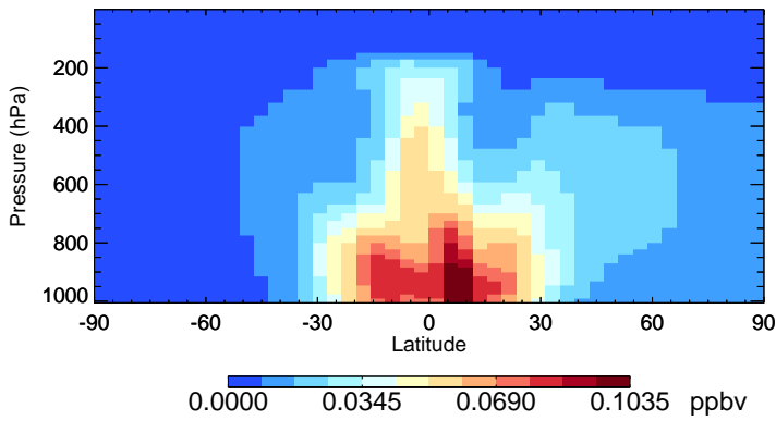
v11-02f-Run0 MAP - Species Zonal Mean for Apr
