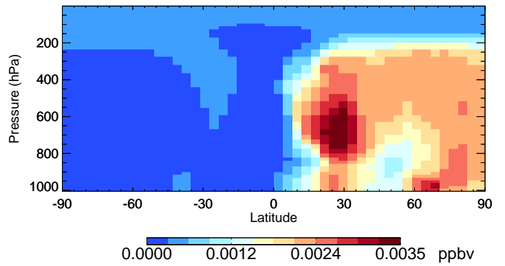
v11-02f-Run0 ASOAN - Species Curtain @ -180.000 for Apr
