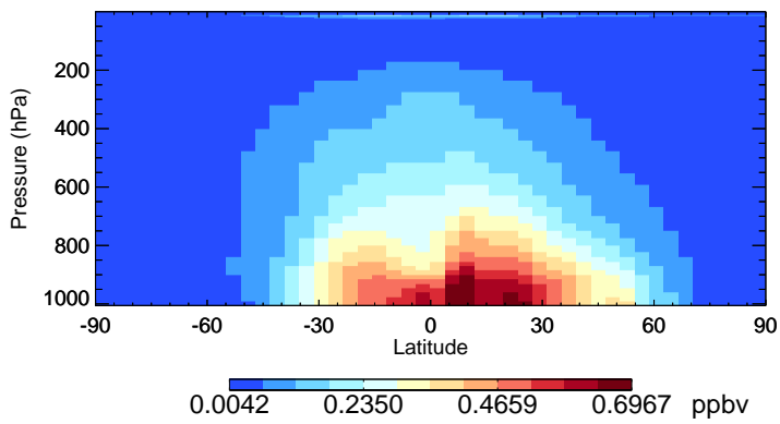
v11-02f-Run0 CH2O - Species Zonal Mean for Apr
