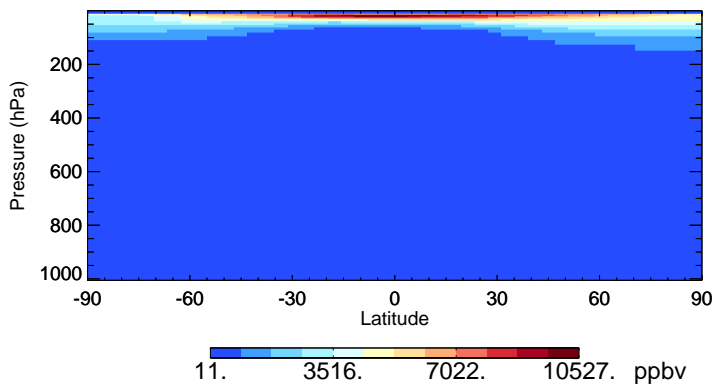
v11-02f-Run0 O3 - Species Zonal Mean for Apr
