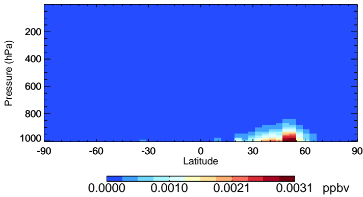
v11-02f-Run0 CINO2 - Species Zonal Mean for Apr
