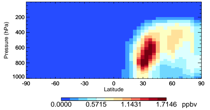
v11-02e-Run1 DST1 - Species Curtain @ -180.000 for Apr
