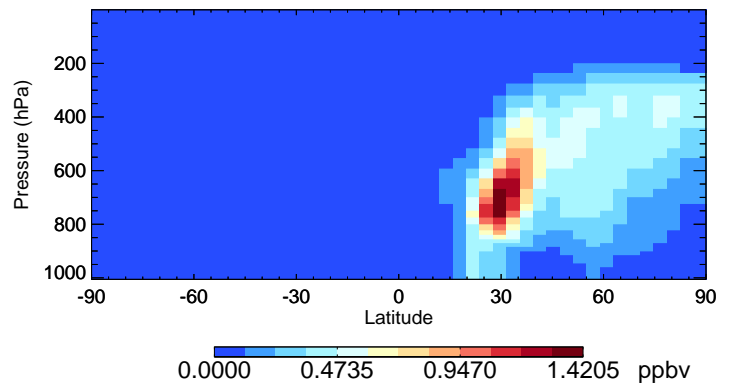
v11-02e-Run0 DST2 - Species Curtain @ -180.000 for Apr
