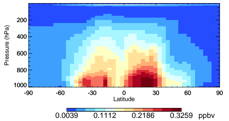
v11-02f-Run0 CH2O - Species Curtain @ -180.000 for Apr
