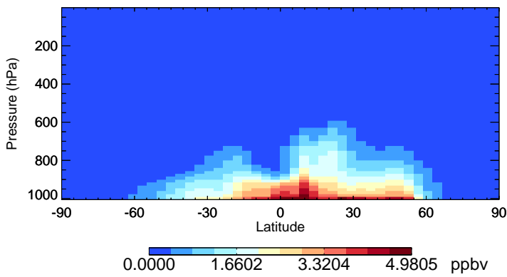
v11-02f-Run0 NH3 - Species Zonal Mean for Apr
