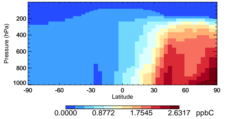
v11-02e-Run1 C2H6 - Species Curtain @ -180.000 for Apr
