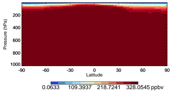
v11-02f-Run0 N2O - Species Curtain @ -180.000 for Apr
