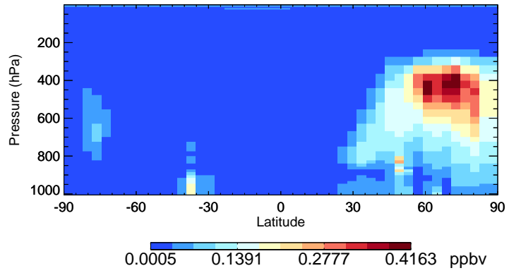
v11-02e-Run1 SO2 - Species Curtain @ -180.000 for Apr
