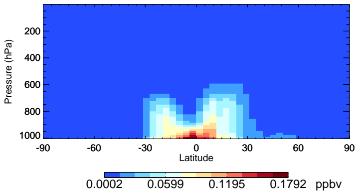
v11-02f-Run0 TSOG3 - Species Zonal Mean for Apr
