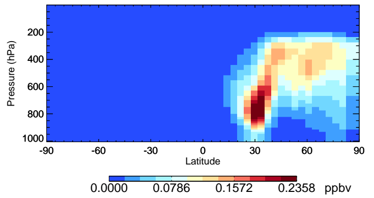
v11-02e-Run1 DST2 - Species Curtain @ -180.000 for Apr
