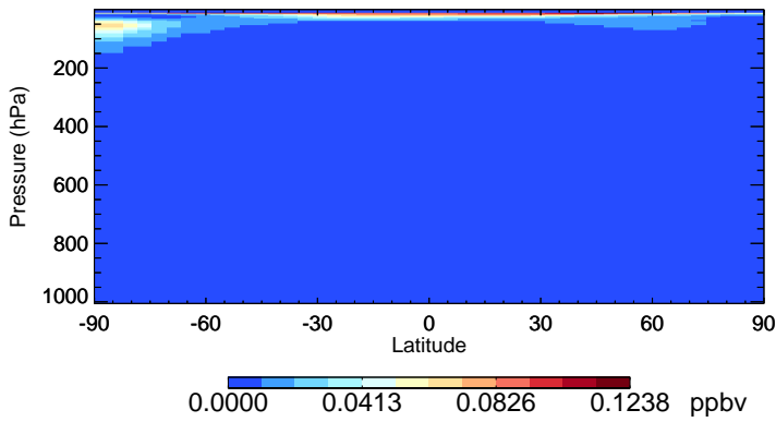
v11-02f-Run0 HOCl - Species Zonal Mean for Apr
