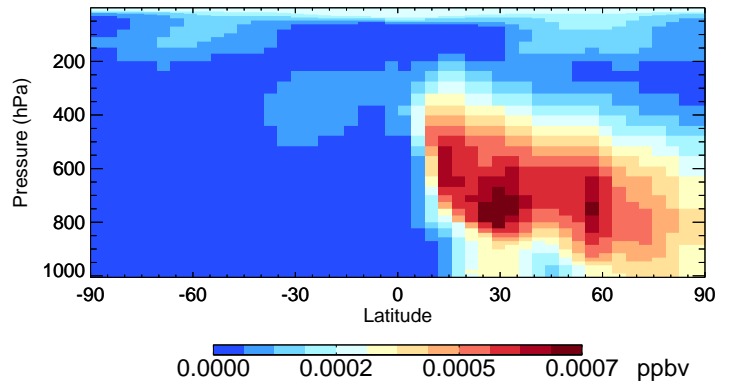
v11-02e-Run0 ASOG1 - Species Curtain @ -180.000 for Apr
