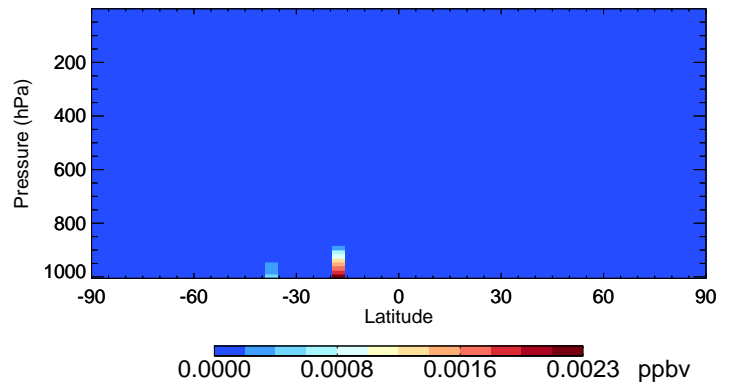
v11-02f-Run0 MTPO - Species Curtain @ -180.000 for Apr
