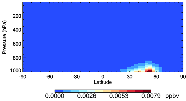
v11-02e-Run0 CINO2 - Species Zonal Mean for Apr
