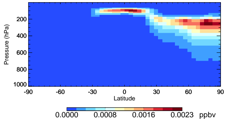
v11-02e-Run0 ASOA3 - Species Curtain @ -180.000 for Apr
