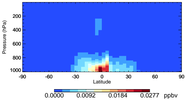
v11-02f-Run0 IPMN - Species Zonal Mean for Apr
