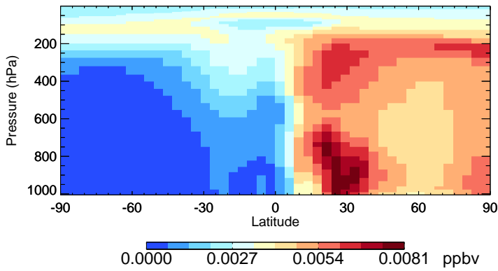
v11-02f-Run0 ASOG3 - Species Zonal Mean for Apr
