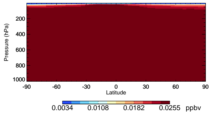
v11-02f-Run0 HCFC142b - Species Curtain @ -180.000 for Apr
