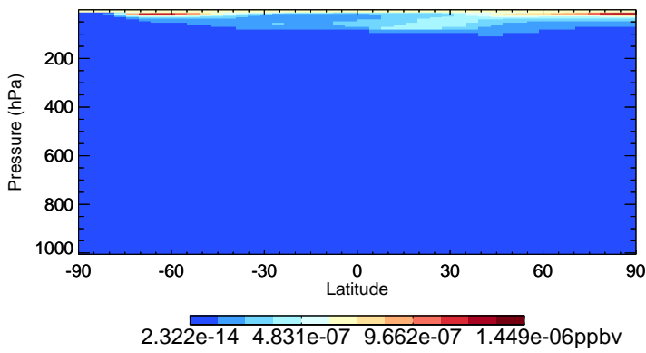
v11-02f-Run0 CIOO - Species Zonal Mean for Apr
