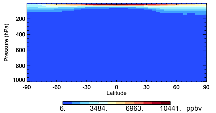
v11-02f-Run0 O3 - Species Curtain @ -180.000 for Apr
