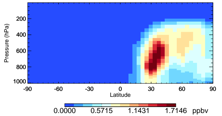
v11-02f-Run0 DST1 - Species Curtain @ -180.000 for Apr
