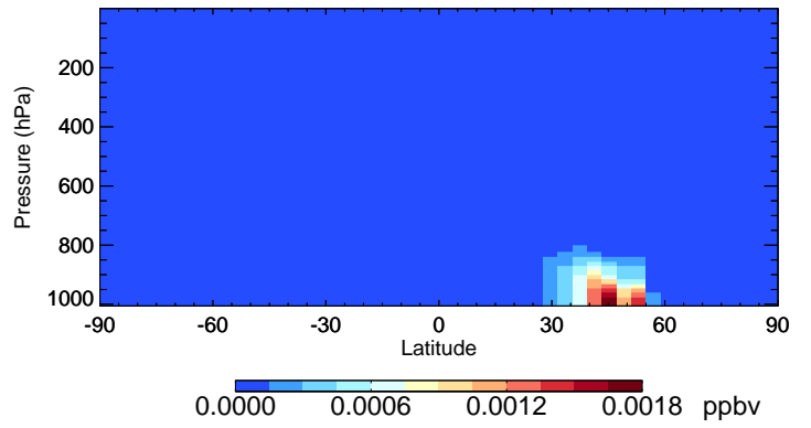
v11-02e-Run0 CINO2 - Species Curtain @ -180.000 for Apr
