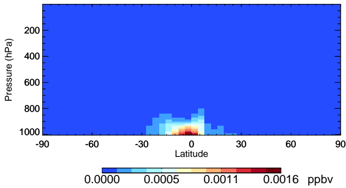
v11-02f-Run0 MOBA - Species Zonal Mean for Apr
