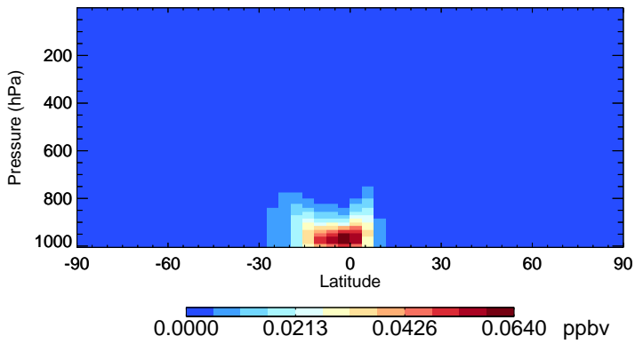
v11-02f-Run0 RIPA - Species Zonal Mean for Apr
