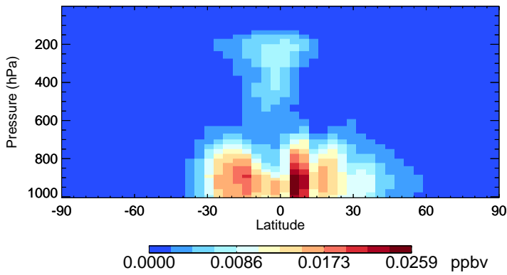
v11-02f-Run0 IMAE - Species Zonal Mean for Apr
