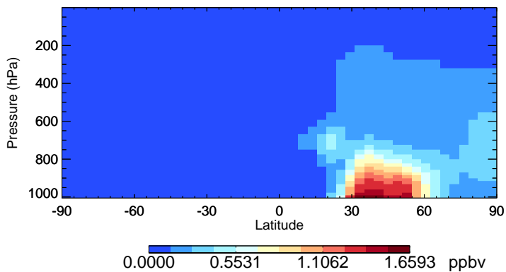
v11-02f-Run0 NIT - Species Zonal Mean for Apr
