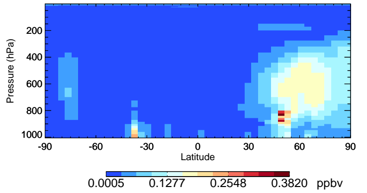
v11-02e-Run0 SO2 - Species Curtain @ -180.000 for Apr
