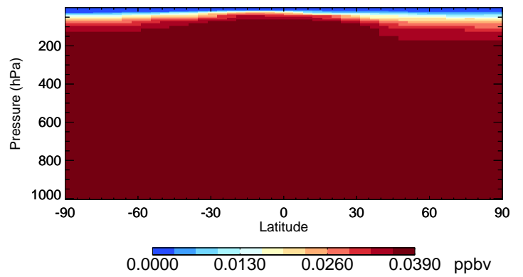
v11-02f-Run0 HCFC141b - Species Curtain @ -180.000 for Apr
