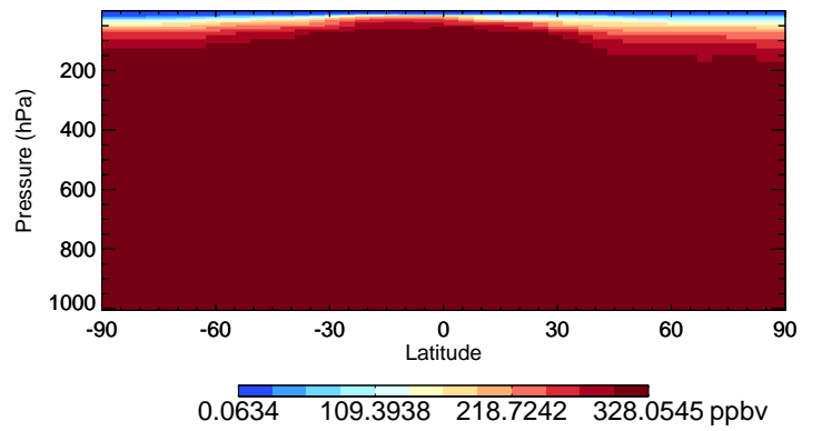
v11-02e-Run1 N2O - Species Curtain @ -180.000 for Apr
