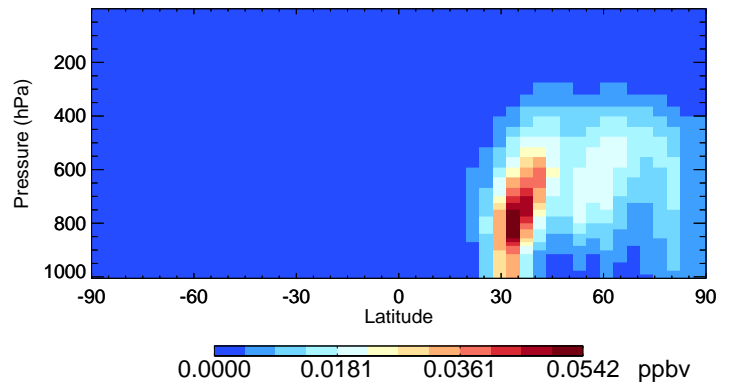
v11-02f-Run0 DST4 - Species Curtain @ -180.000 for Apr
