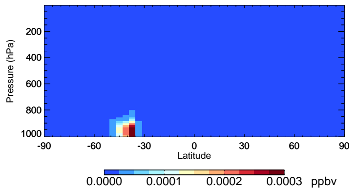
v11-02f-Run0 ISN1 - Species Curtain @ -180.000 for Apr
