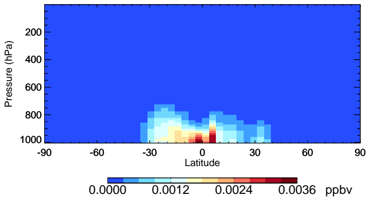
v11-02f-Run0 ISOPNB - Species Zonal Mean for Apr
