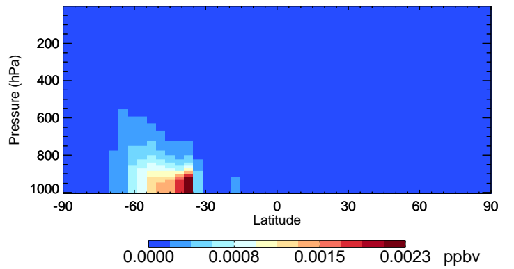
v11-02f-Run0 IPMN - Species Curtain @ -180.000 for Apr
