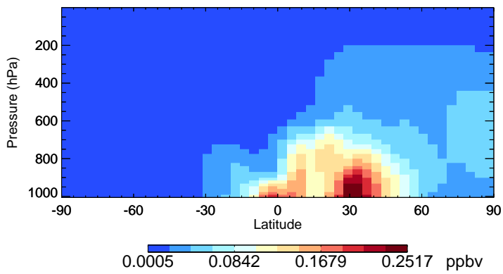
v11-02f-Run0 SOAS - Species Zonal Mean for Apr
