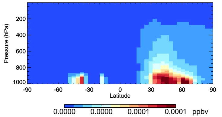
v11-02f-Run0 IONITA - Species Curtain @ -180.000 for Apr
