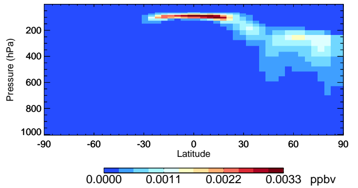
v11-02f-Run0 ASOA3 - Species Curtain @ -180.000 for Apr
