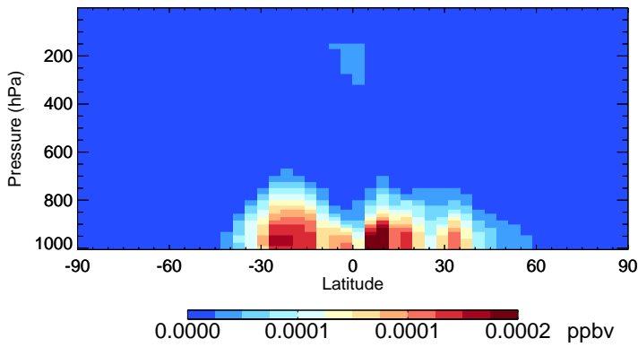
v11-02f-Run0 MACRN - Species Zonal Mean for Apr
