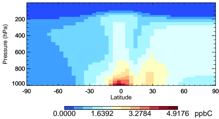
v11-02f-Run0 ACET - Species Zonal Mean for Apr
