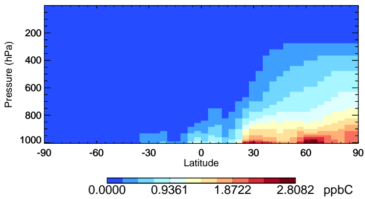
v11-02f-Run0 ALK4 - Species Zonal Mean for Apr
