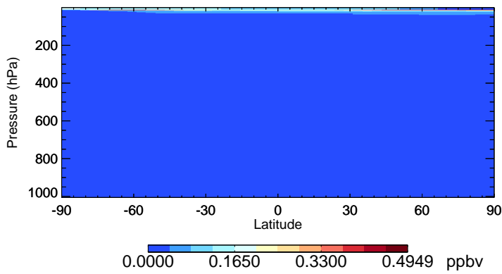
v11-02f-Run0 ClO - Species Zonal Mean for Apr
