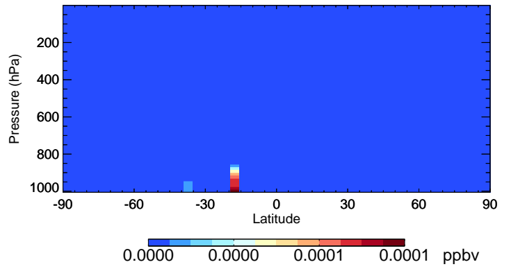
v11-02e-Run0 LIMO - Species Curtain @ -180.000 for Apr
