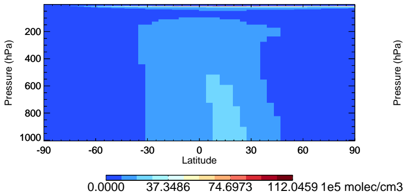
v11-02f-Run0 OH - Species Zonal Mean for Apr
