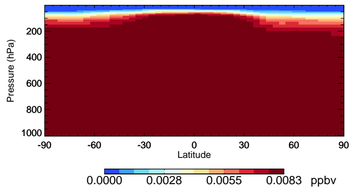
v11-02f-Run0 CH3CCI3 - Species Curtain @ -180.000 for Apr
