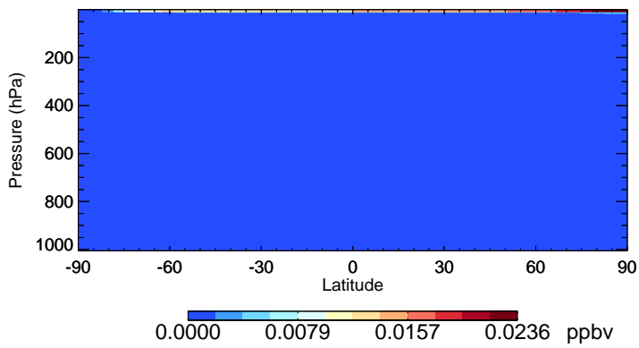
v11-02f-Run0 Br - Species Zonal Mean for Apr
