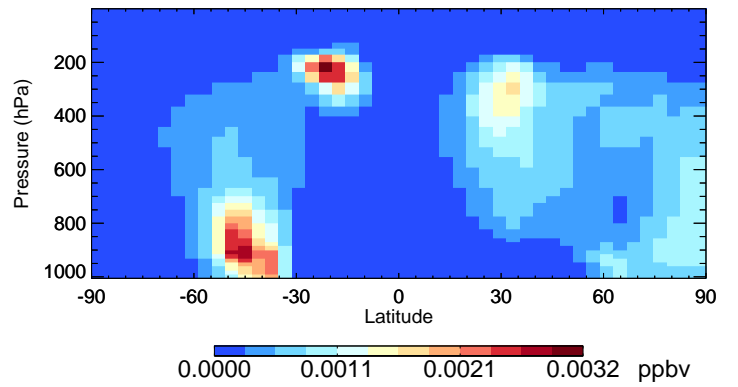
v11-02f-Run0 IMAE - Species Curtain @ -180.000 for Apr
