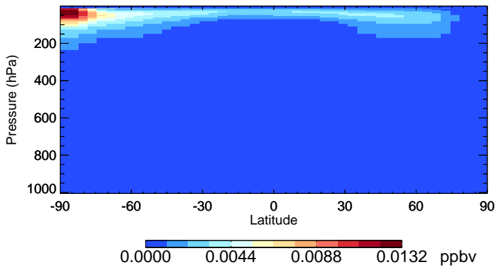
v11-02f-Run0 BrCl - Species Zonal Mean for Apr
