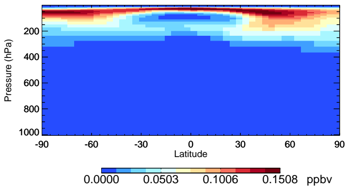
v11-02f-Run0 MPN - Species Zonal Mean for Apr
