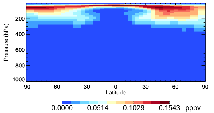
v11-02f-Run0 MPN - Species Curtain @ -180.000 for Apr
