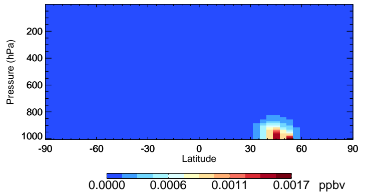
v11-02f-Run0 CINO2 - Species Curtain @ -180.000 for Apr
