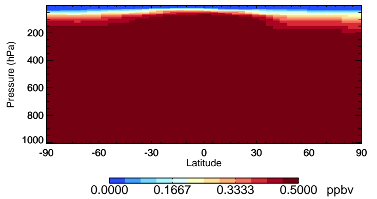
v11-02f-Run0 OCS - Species Curtain @ -180.000 for Apr
