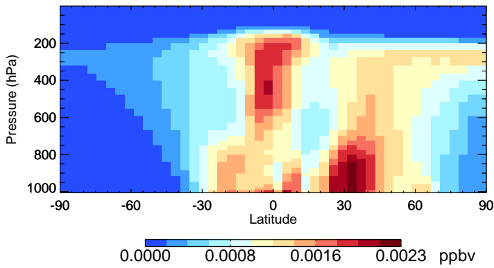
v11-02f-Run0 R4N2 - Species Zonal Mean for Apr
