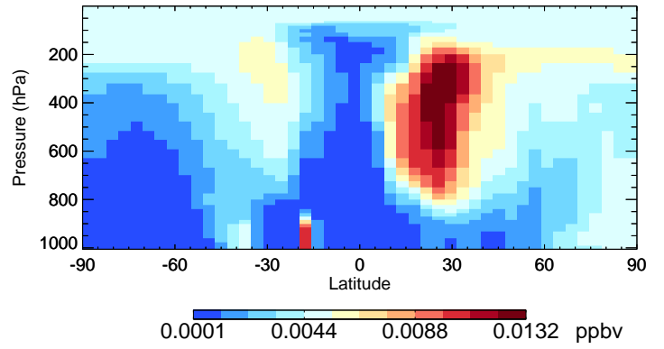
v11-02e-Run1 TSOG3 - Species Curtain @ -180.000 for Apr
