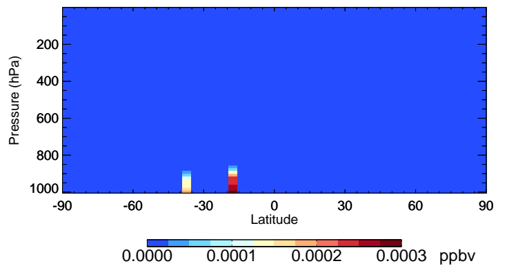
v11-02f-Run0 LIMO - Species Curtain @ -180.000 for Apr
