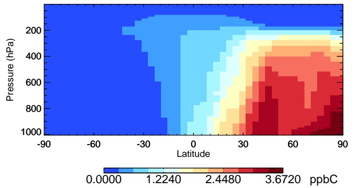
v11-02f-Run0 C2H6 - Species Curtain @ -180.000 for Apr
