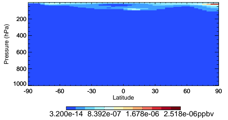
v11-02e-Run0 CIOO - Species Curtain @ -180.000 for Apr
