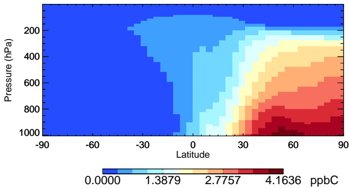
v11-02f-Run0 C2H6 - Species Zonal Mean for Apr
