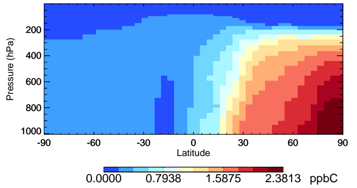
v11-02e-Run0 C2H6 - Species Curtain @ -180.000 for Apr
