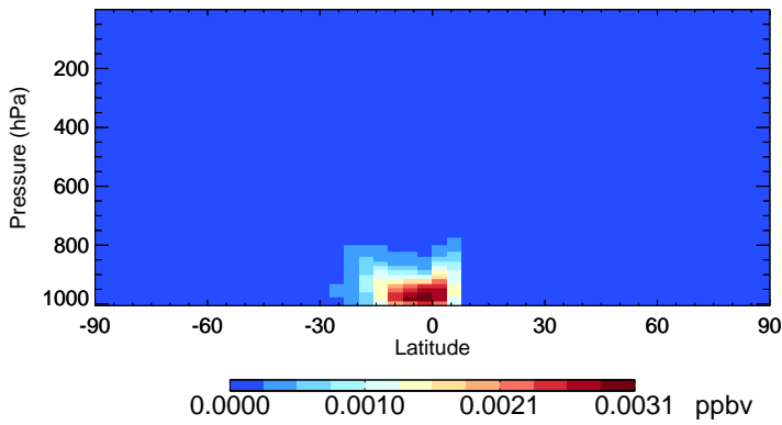
v11-02f-Run0 RIPD - Species Zonal Mean for Apr
