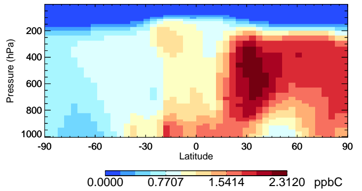
v11-02f-Run0 ACET - Species Curtain @ -180.000 for Apr
