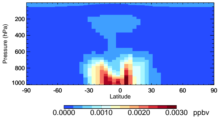
v11-02f-Run0 LVOCOA - Species Zonal Mean for Apr
