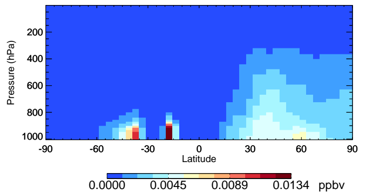
v11-02f-Run0 RCHO - Species Curtain @ -180.000 for Apr
