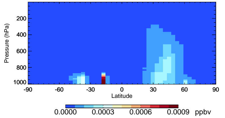
v11-02e-Run1 GLYX - Species Curtain @ -180.000 for Apr
