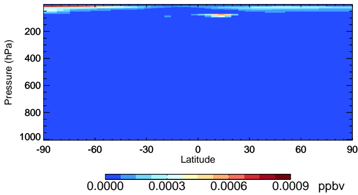
v11-02f-Run0 Cl2 - Species Zonal Mean for Apr
