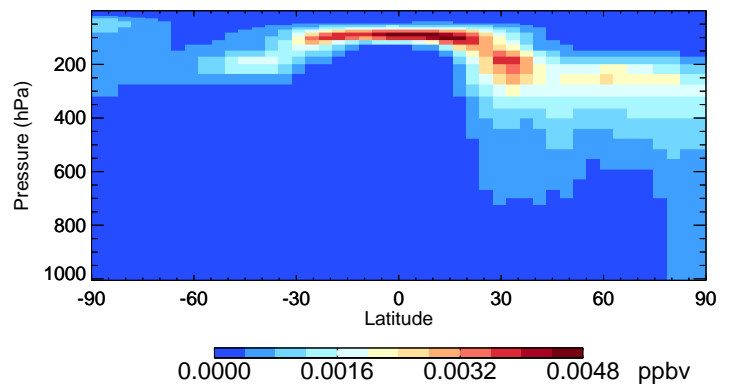
v11-02f-Run0 TSOA2 - Species Curtain @ -180.000 for Apr
