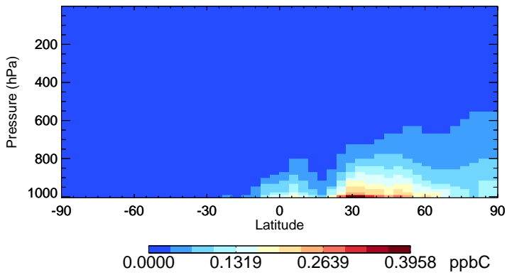
v11-02f-Run0 TOLU - Species Zonal Mean for Apr
