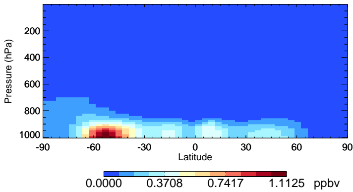
v11-02f-Run0 SALA - Species Zonal Mean for Apr
