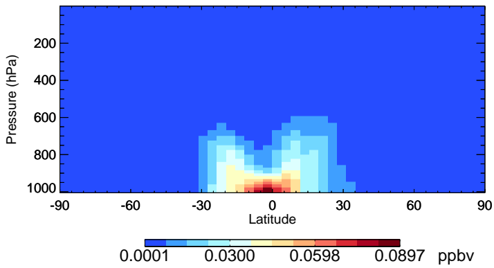
v11-02f-Run0 TSOG2 - Species Zonal Mean for Apr
