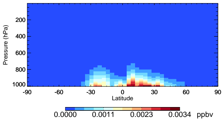
v11-02f-Run0 ISN1 - Species Zonal Mean for Apr
