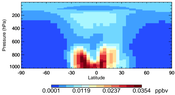
v11-02f-Run0 ISOG3 - Species Zonal Mean for Apr
