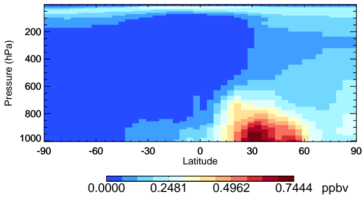
v11-02f-Run0 SO4 - Species Zonal Mean for Apr
