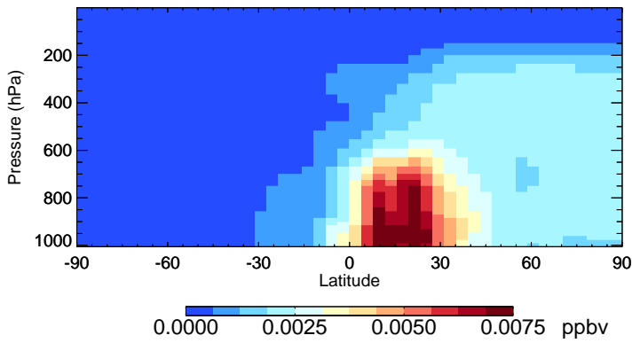
v11-02f-Run0 ASOAN - Species Zonal Mean for Apr
