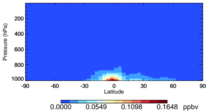
v11-02f-Run0 RCHO - Species Zonal Mean for Apr
