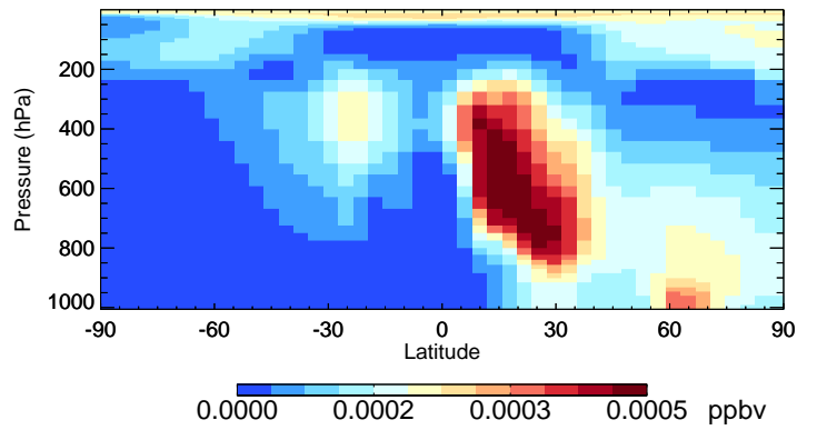
v11-02f-Run0 ASOG1 - Species Curtain @ -180.000 for Apr
