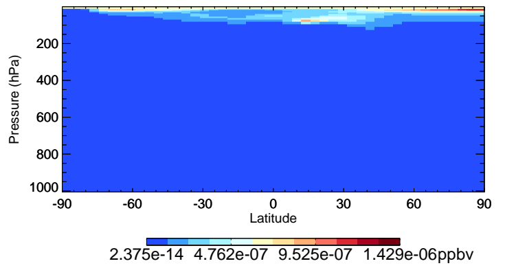
v11-02e-Run1 CIOO - Species Curtain @ -180.000 for Apr
