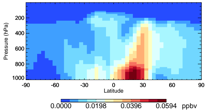
v11-02f-Run0 MAP - Species Curtain @ -180.000 for Apr
