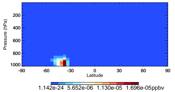
v11-02f-Run0 ETHLN - Species Curtain @ -180.000 for Apr
