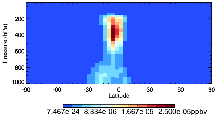
v11-02f-Run0 LVOC - Species Zonal Mean for Apr
