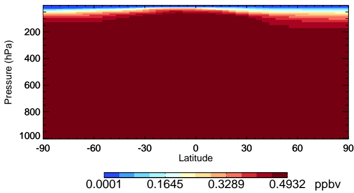
v11-02f-Run0 CFC12 - Species Zonal Mean for Apr
