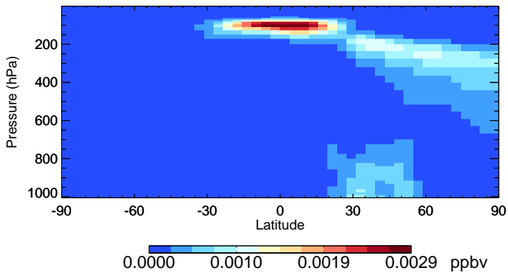
v11-02f-Run0 ASOA3 - Species Zonal Mean for Apr
