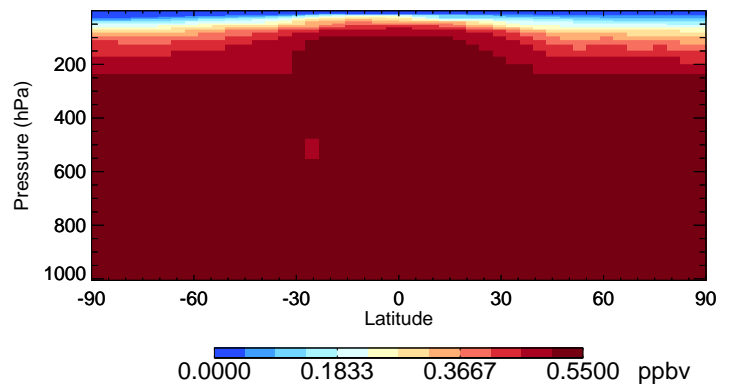
v11-02f-Run0 CH3Cl - Species Curtain @ -180.000 for Apr
