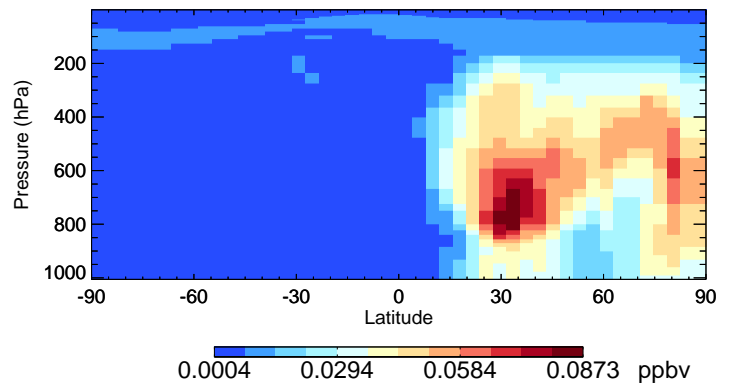
v11-02e-Run1 SOAS - Species Curtain @ -180.000 for Apr
