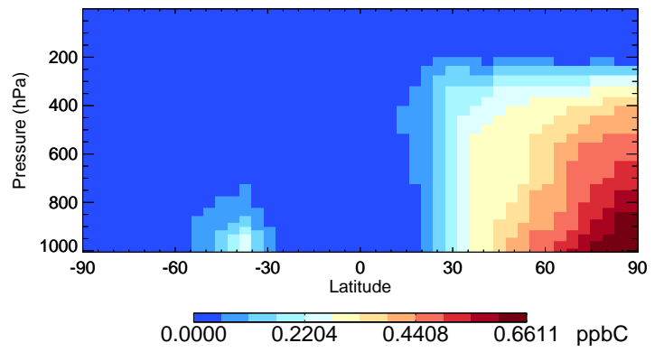
v11-02e-Run0 ALK4 - Species Curtain @ -180.000 for Apr
