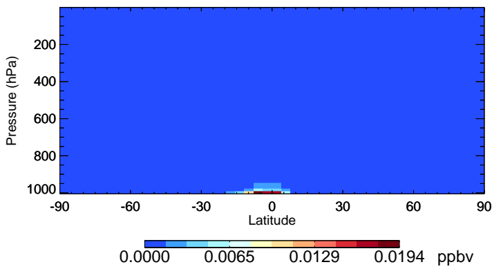
v11-02f-Run0 LIMO - Species Zonal Mean for Apr
