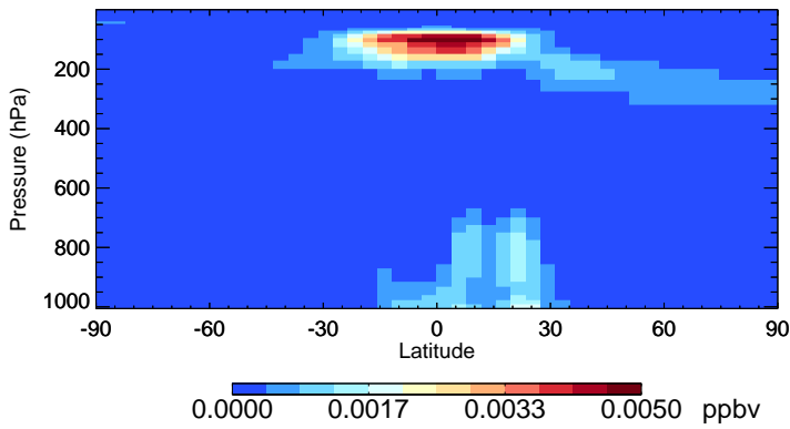
v11-02f-Run0 ISOA3 - Species Zonal Mean for Apr
