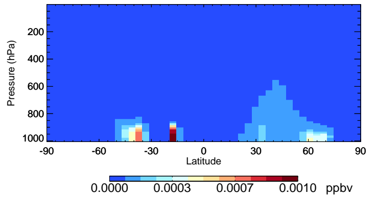
v11-02f-Run0 GLYX - Species Curtain @ -180.000 for Apr
