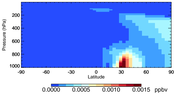
v11-02f-Run0 ASOA2 - Species Zonal Mean for Apr
