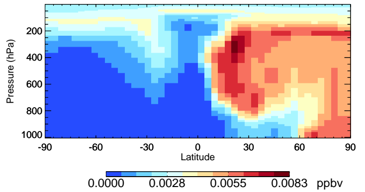
v11-02f-Run0 ASOG3 - Species Curtain @ -180.000 for Apr
