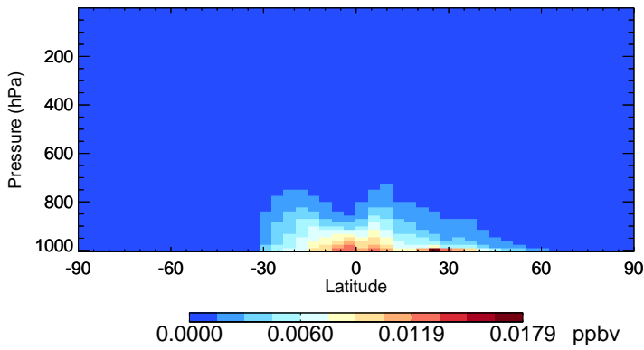
v11-02f-Run0 GLYX - Species Zonal Mean for Apr
