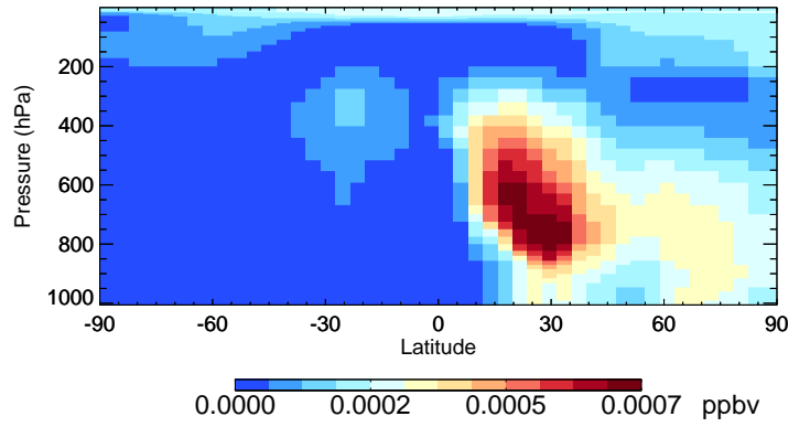
v11-02e-Run1 ASOG1 - Species Curtain @ -180.000 for Apr
