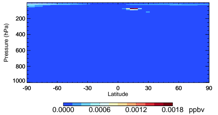
v11-02f-Run0 Cl2 - Species Curtain @ -180.000 for Apr
