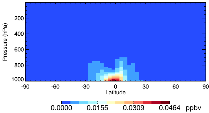
v11-02f-Run0 TSOA0 - Species Zonal Mean for Apr
