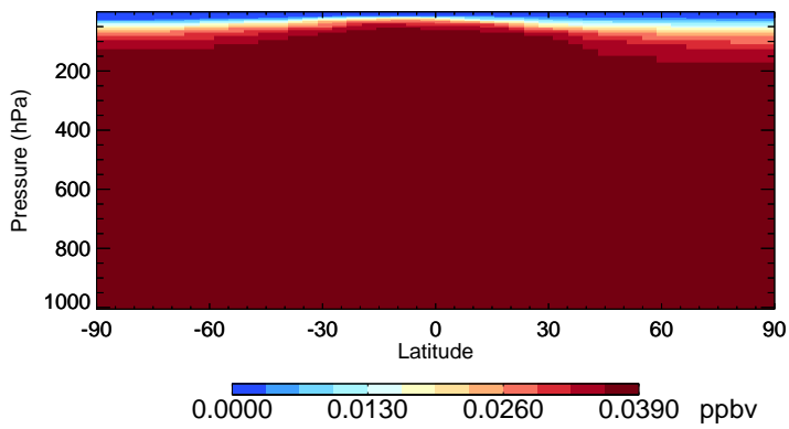
v11-02f-Run0 HCFC141b - Species Zonal Mean for Apr
