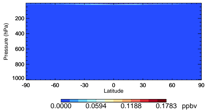
v11-02f-Run0 NO3 - Species Curtain @ -180.000 for Apr
