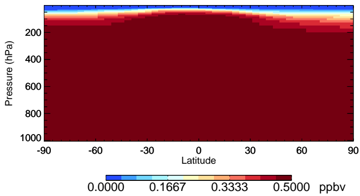
v11-02f-Run0 OCS - Species Zonal Mean for Apr
