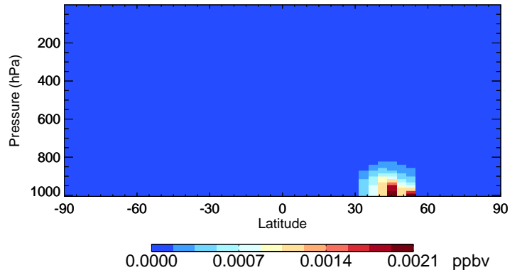
v11-02e-Run1 CINO2 - Species Curtain @ -180.000 for Apr
