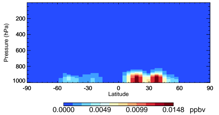
v11-02f-Run0 NITs - Species Curtain @ -180.000 for Apr
