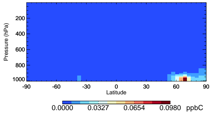
v11-02f-Run0 XYLE - Species Curtain @ -180.000 for Apr
