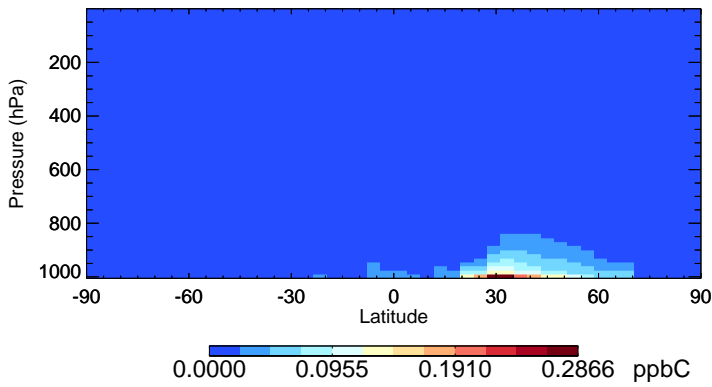
v11-02f-Run0 XYLE - Species Zonal Mean for Apr
