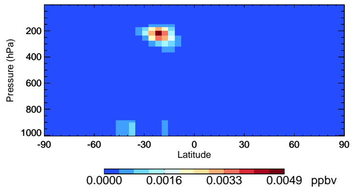
v11-02e-Run1 IEPOXA - Species Curtain @ -180.000 for Apr
