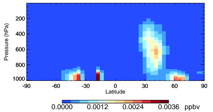
v11-02f-Run0 BCPO - Species Curtain @ -180.000 for Apr
