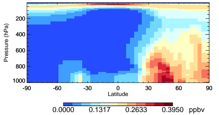
v11-02f-Run0 SO4 - Species Curtain @ -180.000 for Apr
