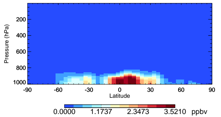
v11-02f-Run0 NH3 - Species Curtain @ -180.000 for Apr
