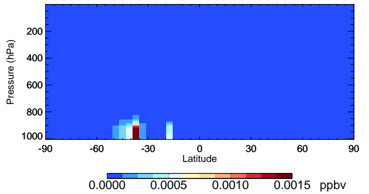
v11-02f-Run0 RIPA - Species Curtain @ -180.000 for Apr
