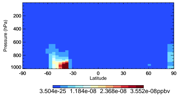
v11-02f-Run0 NPMN - Species Curtain @ -180.000 for Apr
