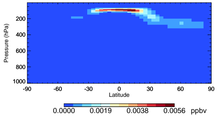
v11-02f-Run0 ISOA3 - Species Curtain @ -180.000 for Apr
