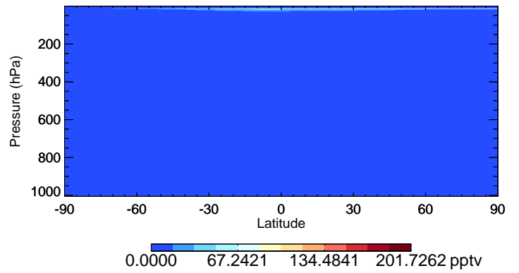
v11-02f-Run0 HO2 - Species Curtain @ -180.000 for Apr
