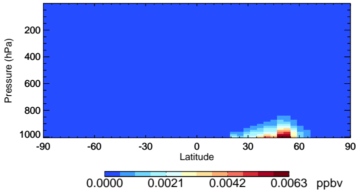
v11-02e-Run1 CINO2 - Species Zonal Mean for Apr
