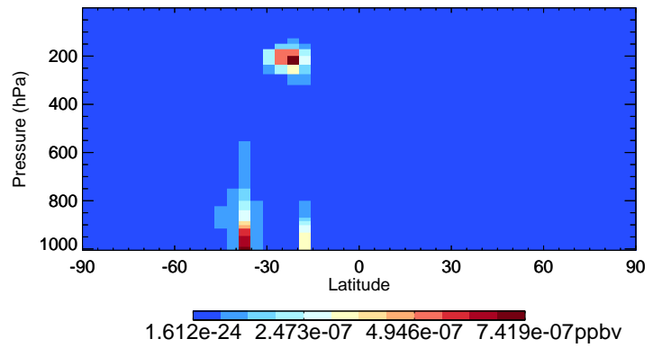
v11-02f-Run0 LVOC - Species Curtain @ -180.000 for Apr
