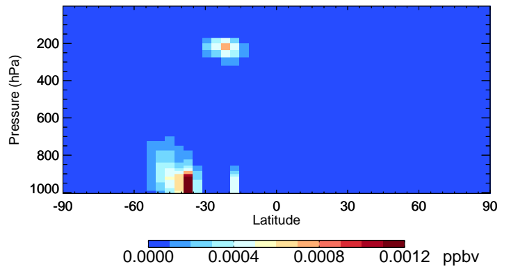
v11-02f-Run0 IEPOXB - Species Curtain @ -180.000 for Apr
