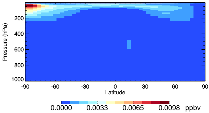
v11-02f-Run0 HOBr - Species Zonal Mean for Apr
