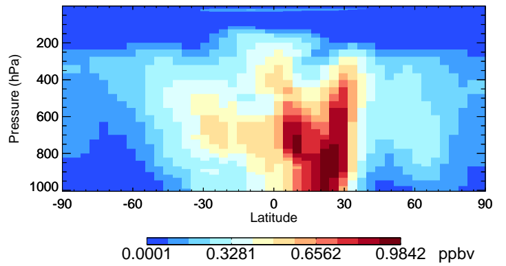
v11-02f-Run0 H2O2 - Species Curtain @ -180.000 for Apr
