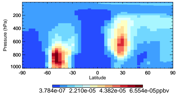
v11-02f-Run0 ISN10A - Species Curtain @ -180.000 for Apr
