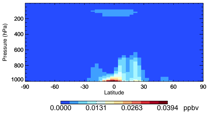
v11-02f-Run0 TSOA2 - Species Zonal Mean for Apr
