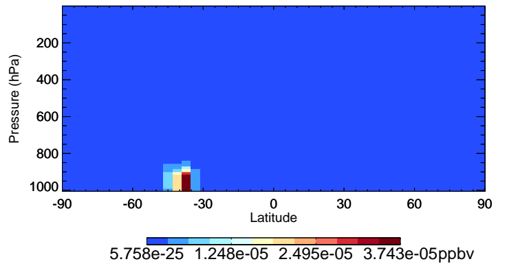
v11-02f-Run0 MACRN - Species Curtain @ -180.000 for Apr
