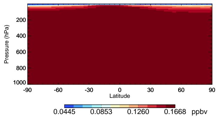
v11-02f-Run0 HCFC22 - Species Curtain @ -180.000 for Apr
