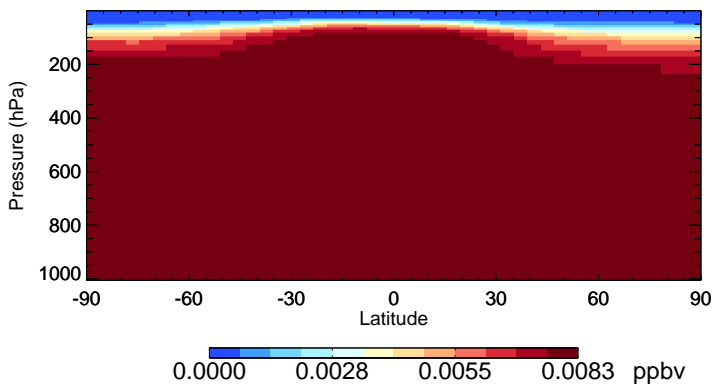
v11-02f-Run0 CH3CCI3 - Species Zonal Mean for Apr
