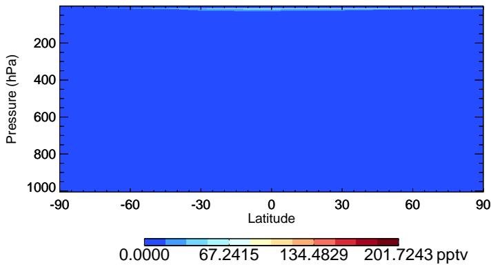
v11-02f-Run0 HO2 - Species Zonal Mean for Apr
