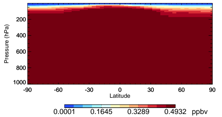
v11-02f-Run0 CFC12 - Species Curtain @ -180.000 for Apr
