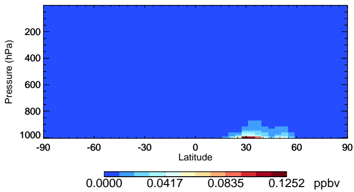
v11-02f-Run0 HNO 2 - Species Zonal Mean for Apr
