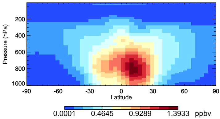
v11-02f-Run0 H2O2 - Species Zonal Mean for Apr
