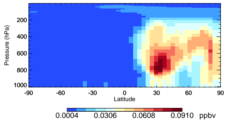
v11-02f-Run0 SOAS - Species Curtain @ -180.000 for Apr
