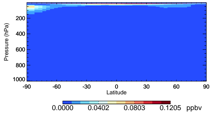
v11-02f-Run0 HOCl - Species Curtain @ -180.000 for Apr
