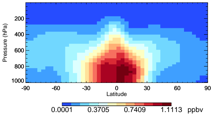
v11-02f-Run0 MP - Species Zonal Mean for Apr
