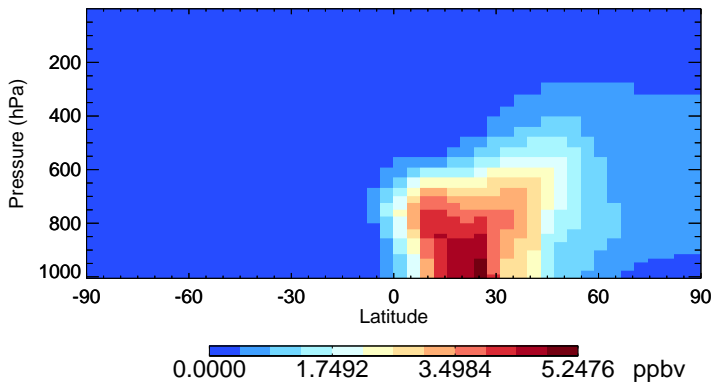
v11-02f-Run0 DST1 - Species Zonal Mean for Apr
