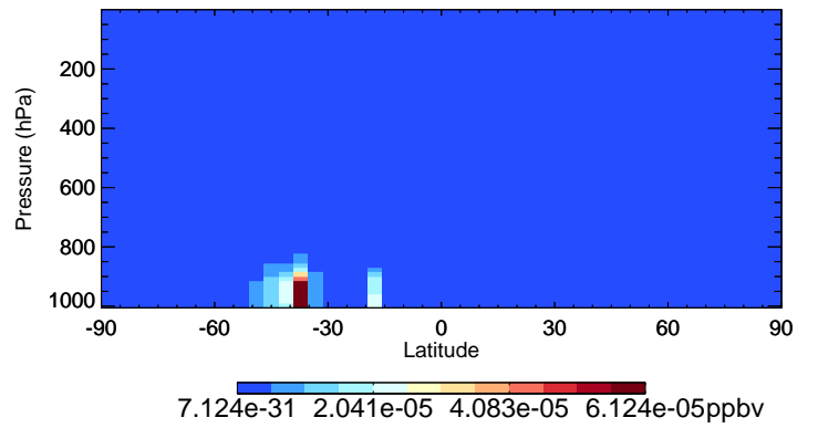
v11-02f-Run0 RIPD - Species Curtain @ -180.000 for Apr
