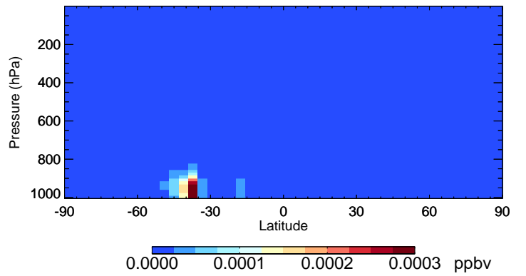
v11-02f-Run0 ISOPNB - Species Curtain @ -180.000 for Apr
