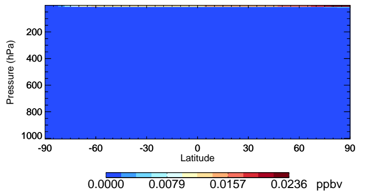
v11-02f-Run0 Br - Species Curtain @ -180.000 for Apr
