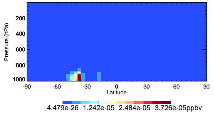
v11-02f-Run0 MOBA - Species Curtain @ -180.000 for Apr
