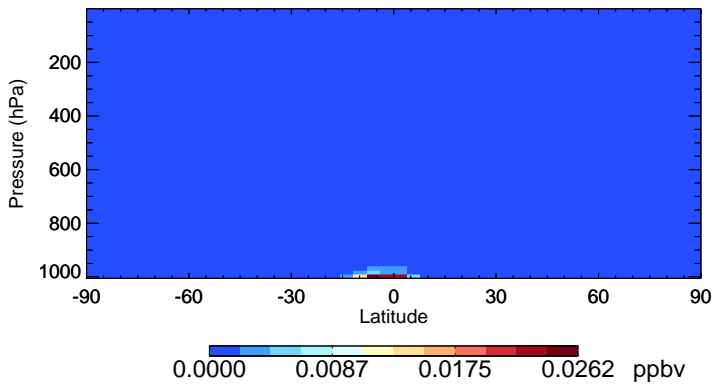
v11-02f-Run0 MTPO - Species Zonal Mean for Apr
