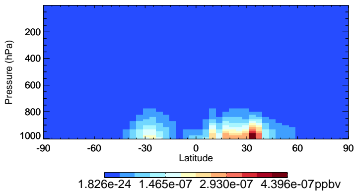
v11-02f-Run0 NPMN - Species Zonal Mean for Apr
