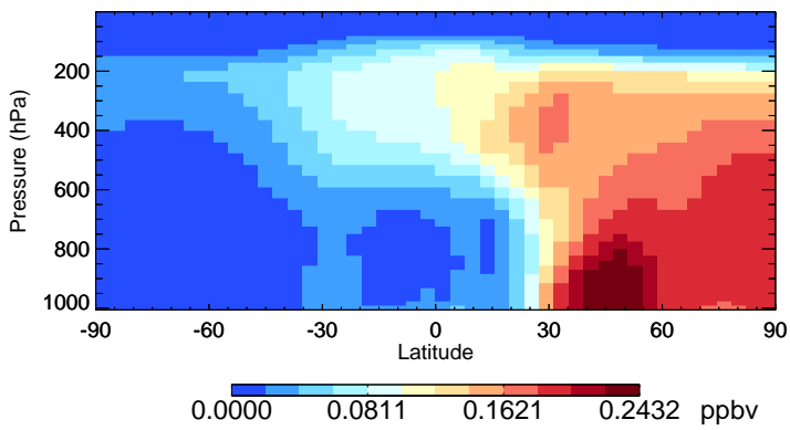
v11-02f-Run0 PAN - Species Zonal Mean for Apr
