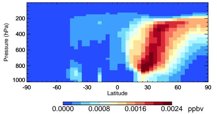
v11-02f-Run0 R4N2 - Species Curtain @ -180.000 for Jan
