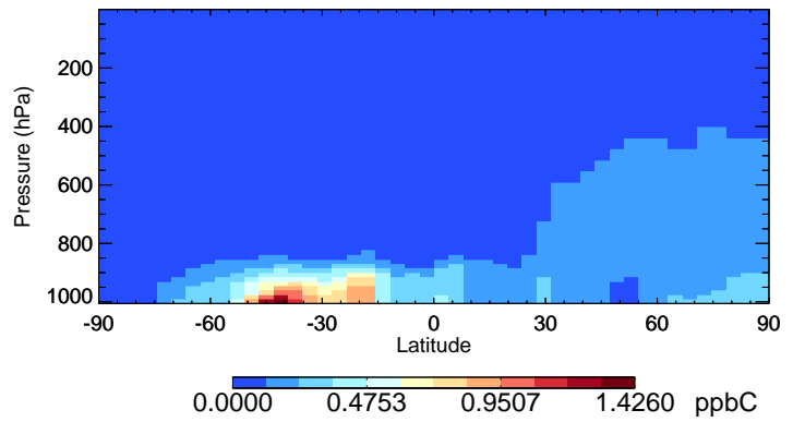
v11-02f-Run0 ALD2 - Species Curtain @ -180.000 for Jan
