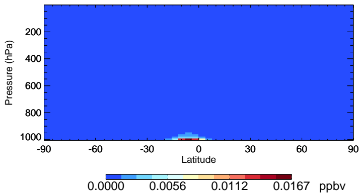
v11-02e-Run0 MTPO - Species Zonal Mean for Jan
