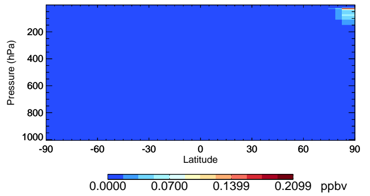
v11-02e-Run1 Cl2 - Species Curtain @ -180.000 for Jan
