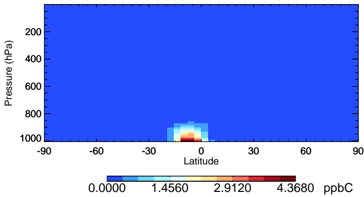
v11-02f-Run0 ISOP - Species Zonal Mean for Jan
