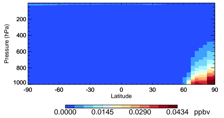
v11-02e-Run0 HNO2 - Species Curtain @ -180.000 for Jan
