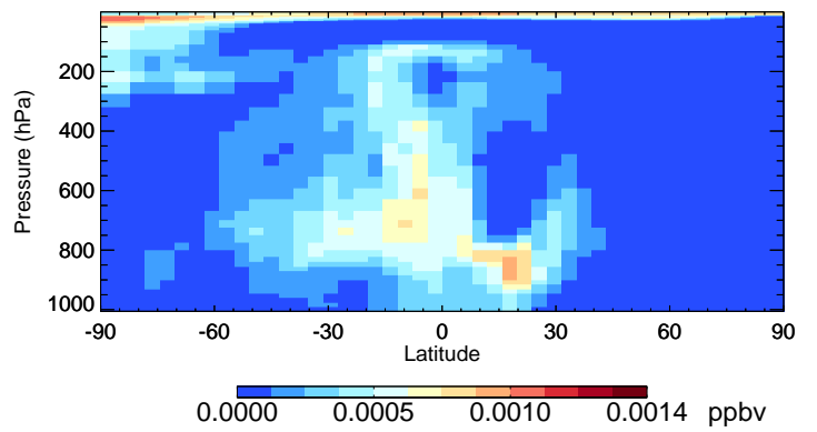
v11-02f-Run0 HBr - Species Curtain @ -180.000 for Jan
