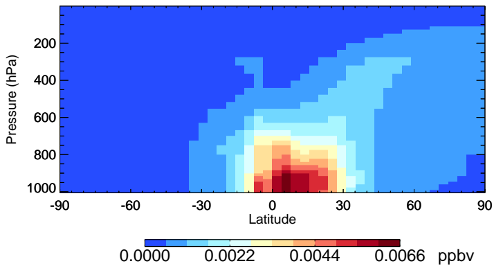
v11-02f-Run0 ASOAN - Species Zonal Mean for Jan
