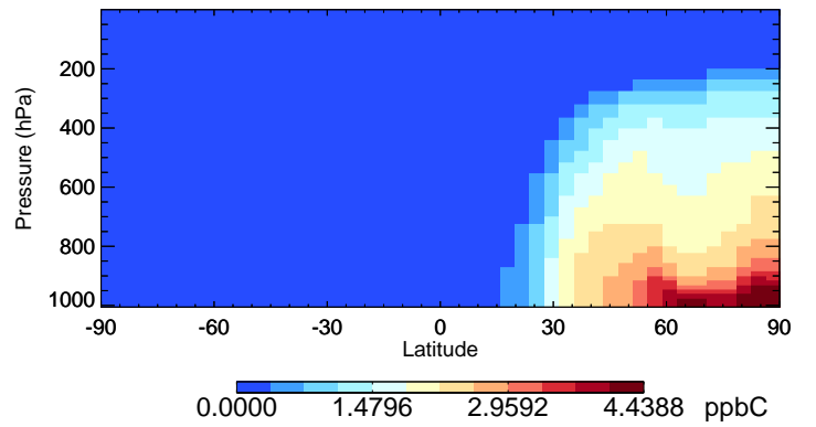
v11-02f-Run0 ALK4 - Species Curtain @ -180.000 for Jan
