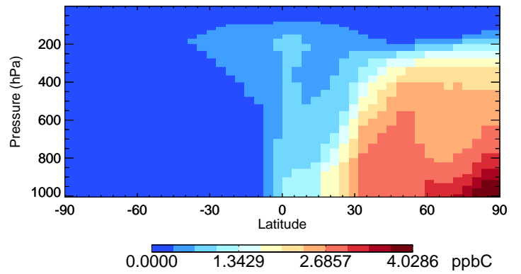
v11-02f-Run0 C2H6 - Species Curtain @ -180.000 for Jan
