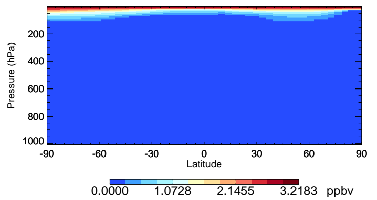
v11-02f-Run0 HCl - Species Curtain @ -180.000 for Jan
