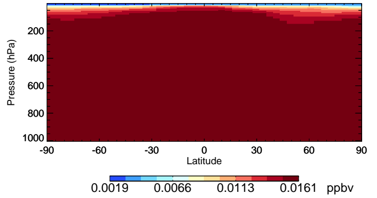
v11-02e-Run1 CFC114 - Species Curtain @ -180.000 for Jan
