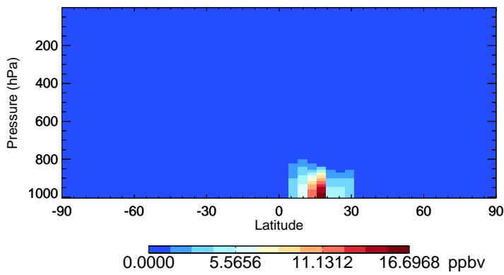
v11-02f-Run0 DST4 - Species Zonal Mean for Jan
