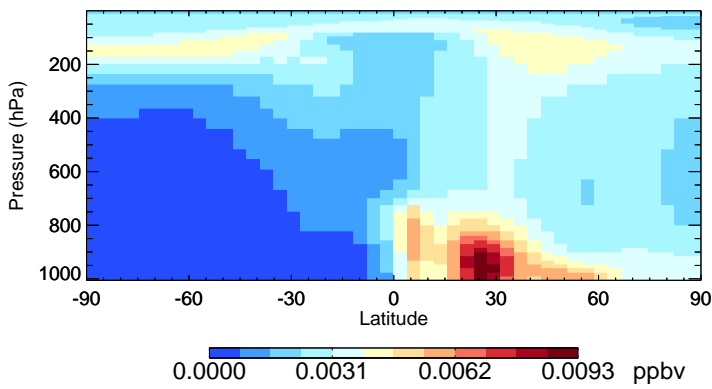
v11-02f-Run0 ASOG3 - Species Zonal Mean for Jan
