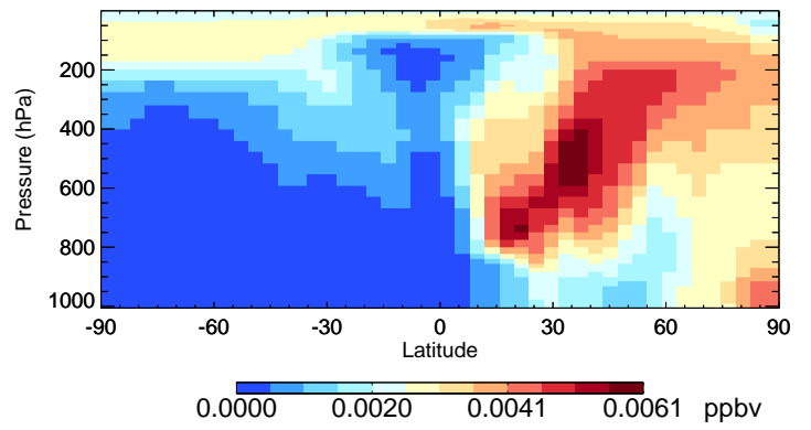
v11-02e-Run1 ASOG3 - Species Curtain @ -180.000 for Jan
