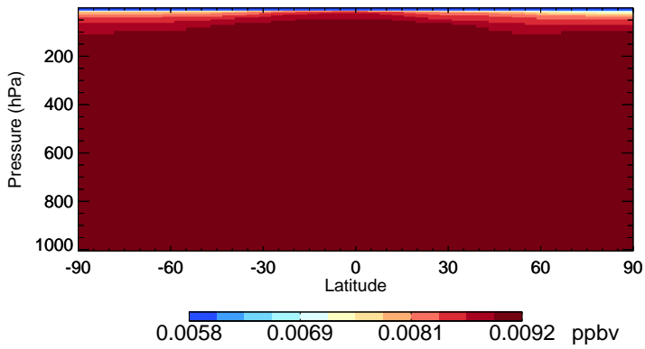
v11-02f-Run0 CFC115 - Species Zonal Mean for Jan
