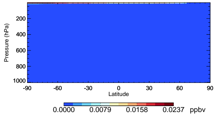
v11-02f-Run0 Br - Species Curtain @ -180.000 for Jan
