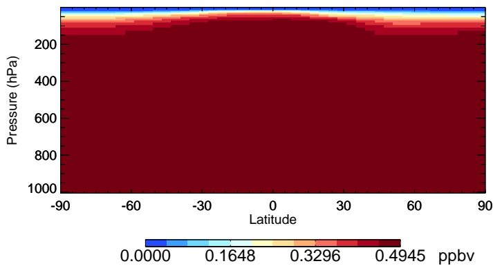
v11-02f-Run0 CFC12 - Species Zonal Mean for Jan
