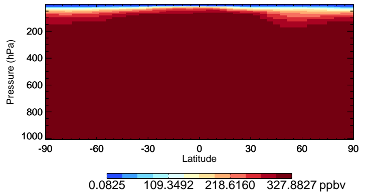
v11-02f-Run0 N2O - Species Curtain @ -180.000 for Jan
