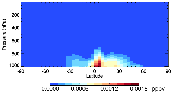
v11-02f-Run0 IONITA - Species Zonal Mean for Jan
