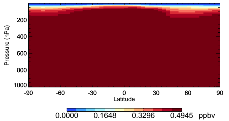
v11-02f-Run0 CFC12 - Species Curtain @ -180.000 for Jan
