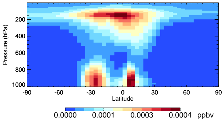
DHDN - Species Zonal Mean for Jan
