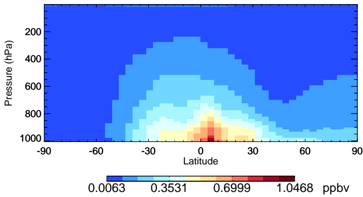
v11-02f-Run0 CH2O - Species Zonal Mean for Jan
