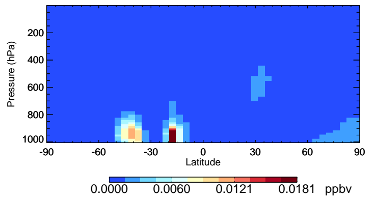
v11-02f-Run0 HAC - Species Curtain @ -180.000 for Jan
