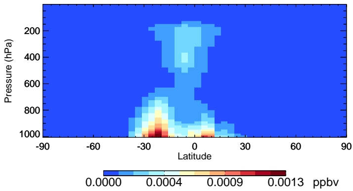
v11-02f-Run0 HONIT - Species Zonal Mean for Jan
