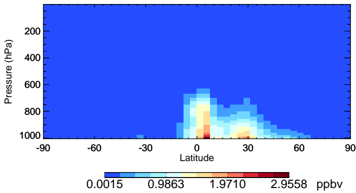
v11-02f-Run0 OCPI - Species Zonal Mean for Jan
