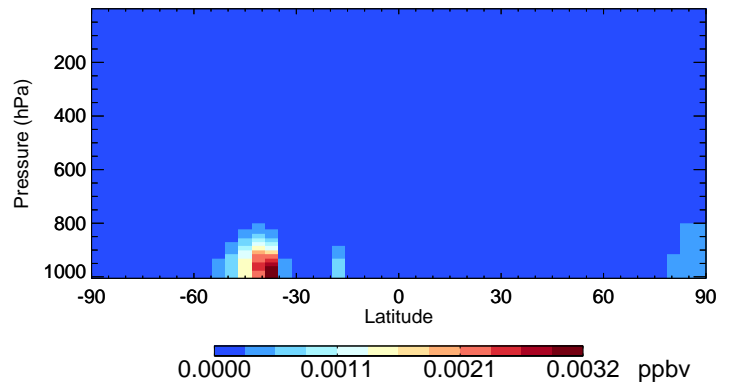
v11-02f-Run0 IPMN - Species Curtain @ -180.000 for Jan
