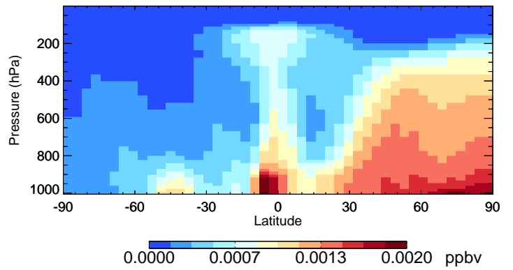
v11-02f-Run0 CHBr3 - Species Curtain @ -180.000 for Jan
