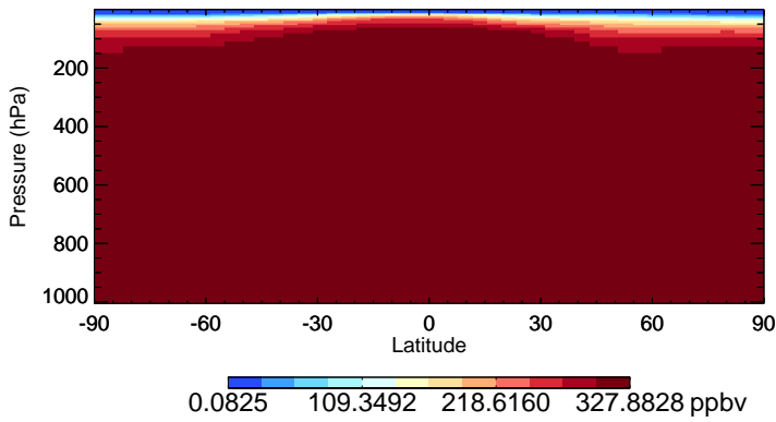
v11-02f-Run0 N2O - Species Zonal Mean for Jan
