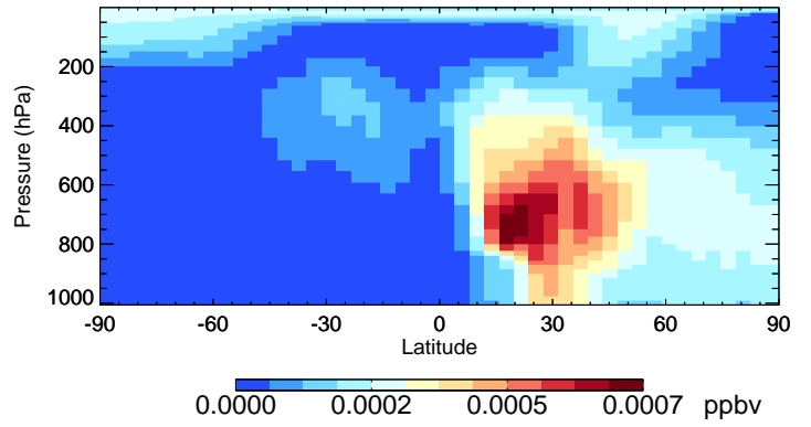
v11-02e-Run1 ASOG1 - Species Curtain @ -180.000 for Jan
