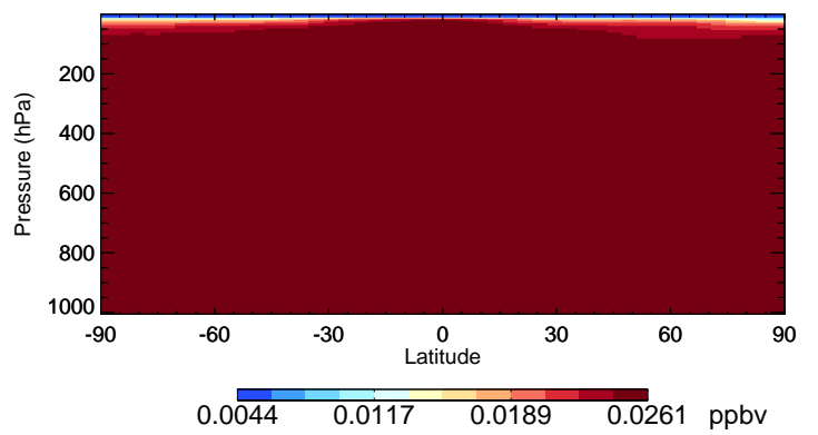
v11-02f-Run0 HCFC142b - Species Curtain @ -180.000 for Jan
