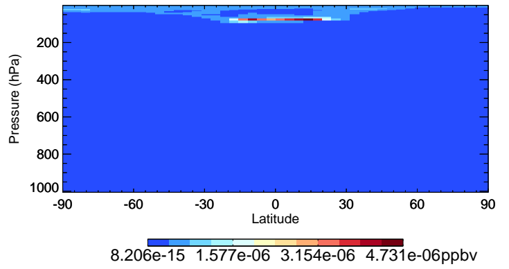
v11-02e-Run0 CIOO - Species Curtain @ -180.000 for Jan
