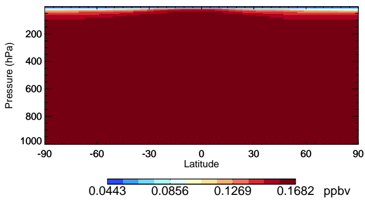
v11-02f-Run0 HCFC22 - Species Zonal Mean for Jan
