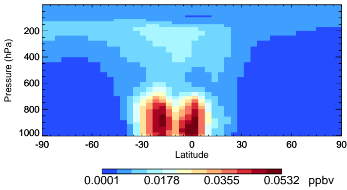
v11-02e-Run1 ISOG3 - Species Zonal Mean for Jan
