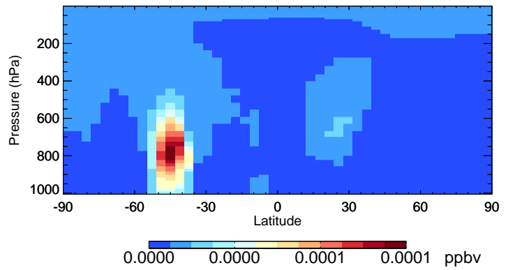
v11-02f-Run0 ISN1OA - Species Curtain @ -180.000 for Jan
