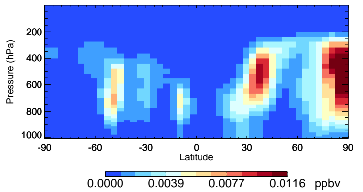
v11-02f-Run0 DST2 - Species Curtain @ -180.000 for Jan
