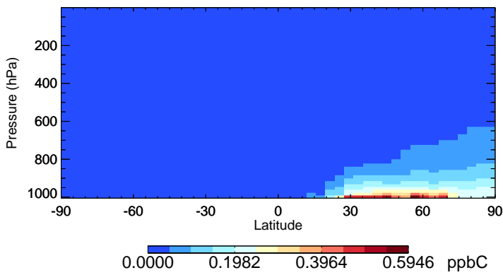
v11-02f-Run0 XYLE - Species Zonal Mean for Jan
