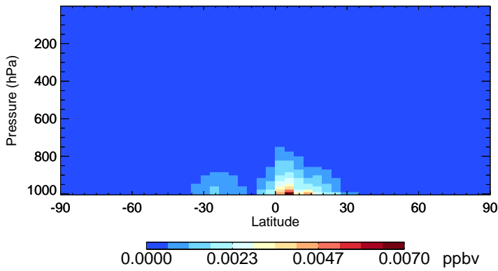
v11-02f-Run0 ISN1 - Species Zonal Mean for Jan
