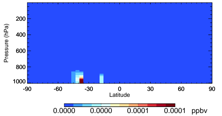
v11-02f-Run0 RIPD - Species Curtain @ -180.000 for Jan
