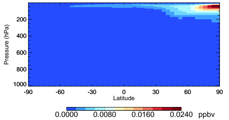
v11-02f-Run0 BrCl - Species Curtain @ -180.000 for Jan
