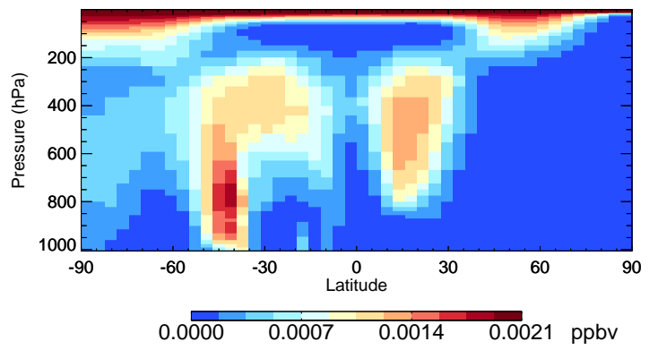
v11-02f-Run0 ISOG1 - Species Curtain @ -180.000 for Jan
