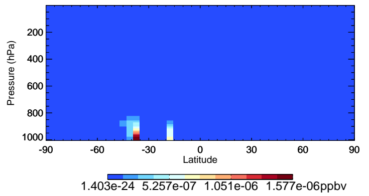
v11-02f-Run0 LVOC - Species Curtain @ -180.000 for Jan
