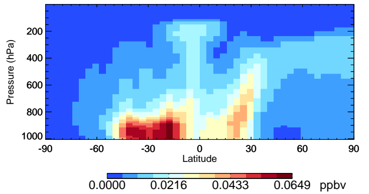
v11-02f-Run0 MAP - Species Curtain @ -180.000 for Jan
