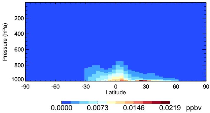
v11-02f-Run0 GLYX - Species Zonal Mean for Jan
