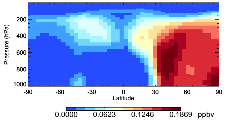
v11-02f-Run0 PAN - Species Curtain @ -180.000 for Jan
