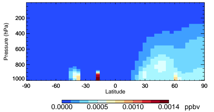
v11-02f-Run0 GLYX - Species Curtain @ -180.000 for Jan
