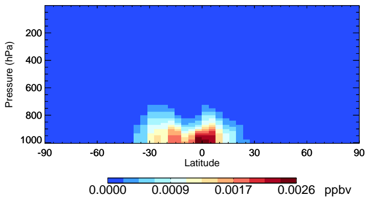
v11-02f-Run0 ISOPNB - Species Zonal Mean for Jan
