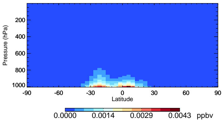
v11-02f-Run0 MONITS - Species Zonal Mean for Jan
