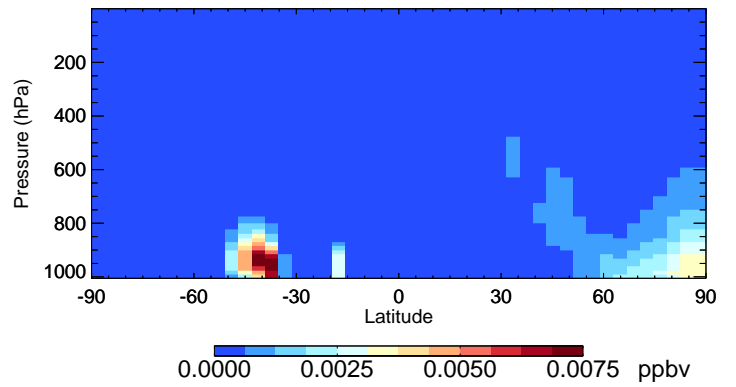
v11-02f-Run0 GLYC - Species Curtain @ -180.000 for Jan
