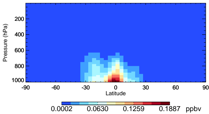
v11-02f-Run0 TSOG3 - Species Zonal Mean for Jan
