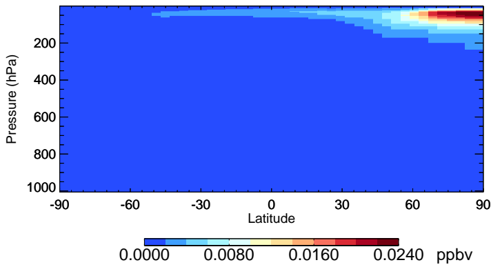
v11-02f-Run0 BrCl - Species Zonal Mean for Jan
