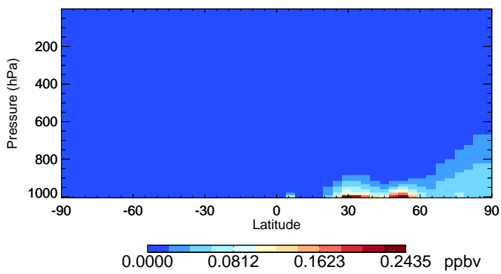
v11-02f-Run0 HNO2 - Species Zonal Mean for Jan
