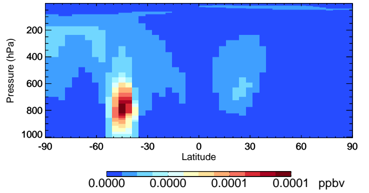
v11-02e-Run1 ISN1OA - Species Curtain @ -180.000 for Jan
