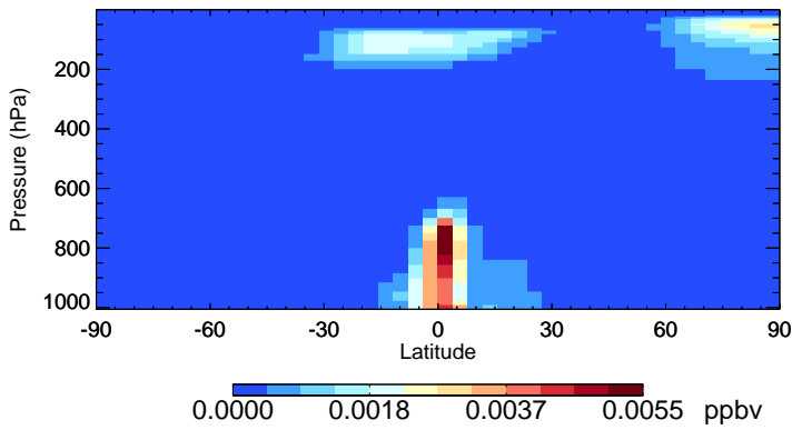
v11-02f-Run0 ISOA3 - Species Zonal Mean for Jan
