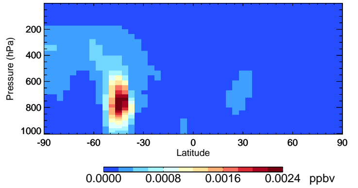
v11-02e-Run1 SOAME - Species Curtain @ -180.000 for Jan
