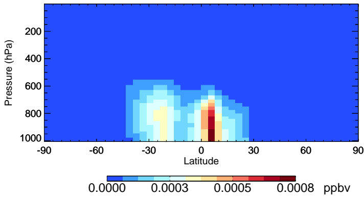
v11-02e-Run0 ISN1OA - Species Zonal Mean for Jan
