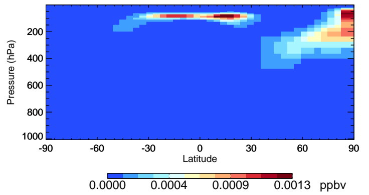
v11-02e-Run1 ASOA3 - Species Curtain @ -180.000 for Jan
