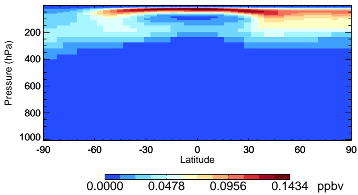
v11-02f-Run0 MPN - Species Zonal Mean for Jan
