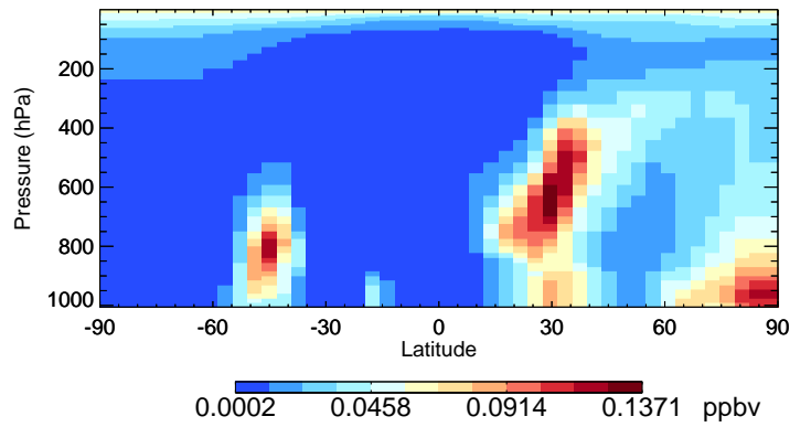
v11-02f-Run0 OCPI - Species Curtain @ -180.000 for Jan
