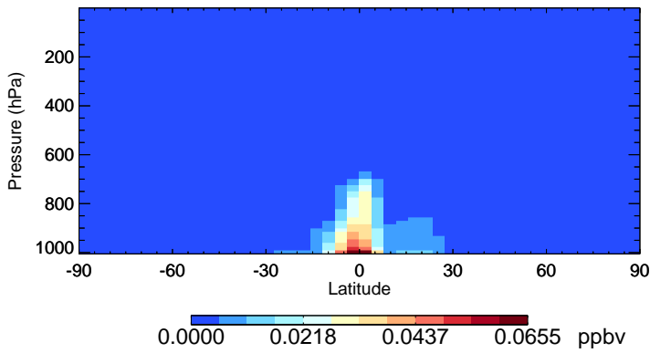
v11-02f-Run0 TSOA2 - Species Zonal Mean for Jan
