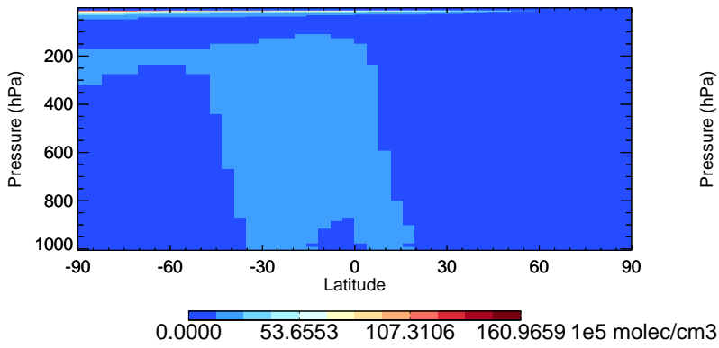
v11-02f-Run0 OH - Species Zonal Mean for Jan
