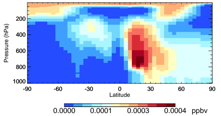
v11-02f-Run0 ASOG1 - Species Curtain @ -180.000 for Jan
