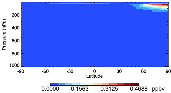
v11-02f-Run0 HOCl - Species Zonal Mean for Jan
