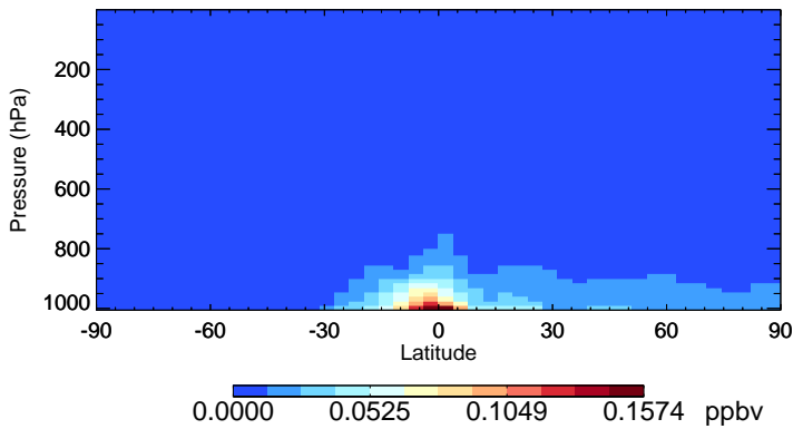
v11-02f-Run0 RCHO - Species Zonal Mean for Jan
