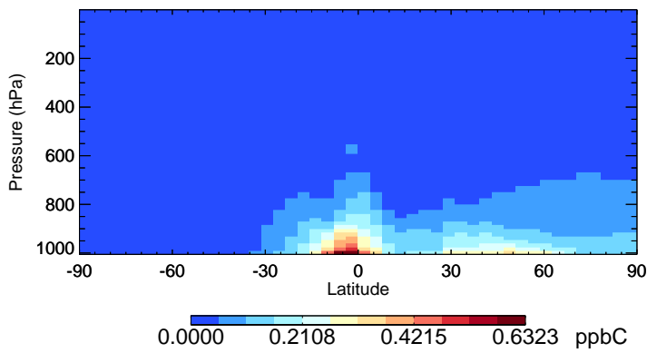
v11-02f-Run0 EOH - Species Zonal Mean for Jan
