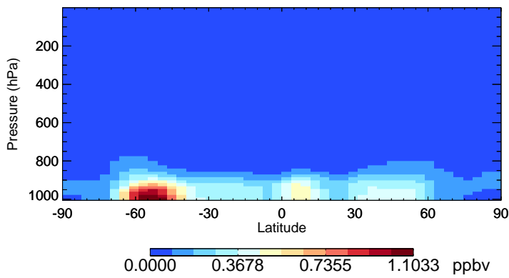
v11-02f-Run0 SALA - Species Zonal Mean for Jan
