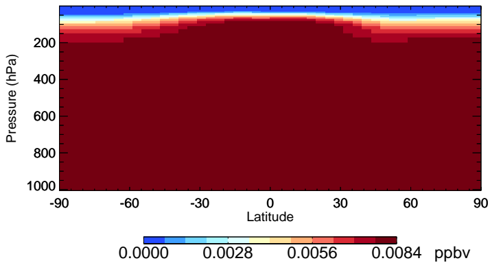
v11-02f-Run0 CH3CCI3 - Species Zonal Mean for Jan
