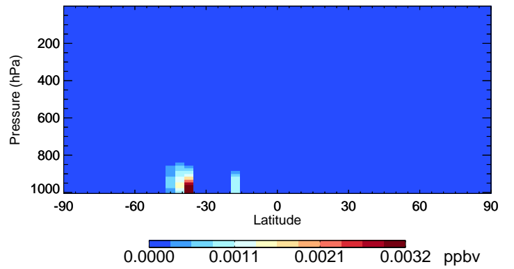
v11-02f-Run0 RIPA - Species Curtain @ -180.000 for Jan
