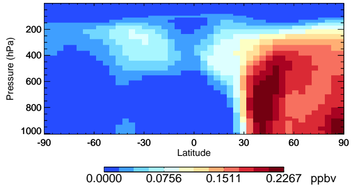
v11-02e-Run1 PAN - Species Curtain @ -180.000 for Jan
