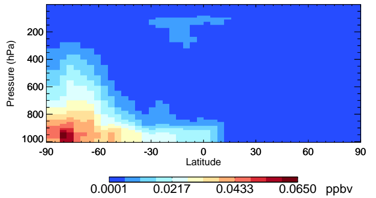
v11-02f-Run0 MSA - Species Curtain @ -180.000 for Jan
