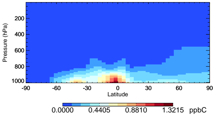
v11-02e-Run0 ALD2 - Species Zonal Mean for Jan
