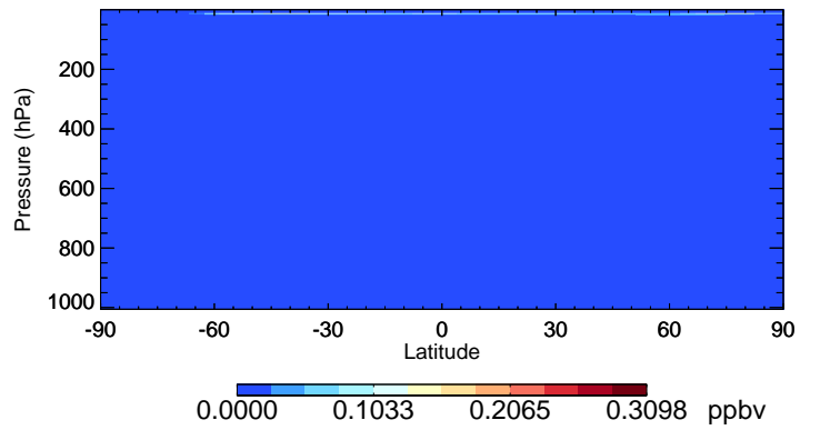
v11-02f-Run0 NO3 - Species Curtain @ -180.000 for Jan
