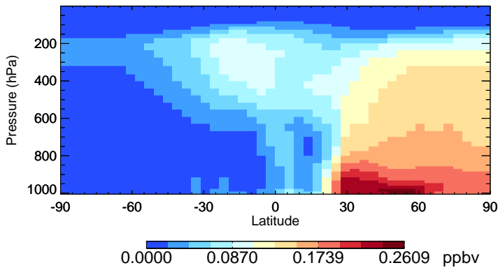
v11-02f-Run0 PAN - Species Zonal Mean for Jan
