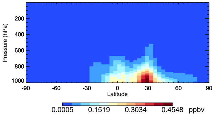
v11-02f-Run0 SOAS - Species Zonal Mean for Jan
