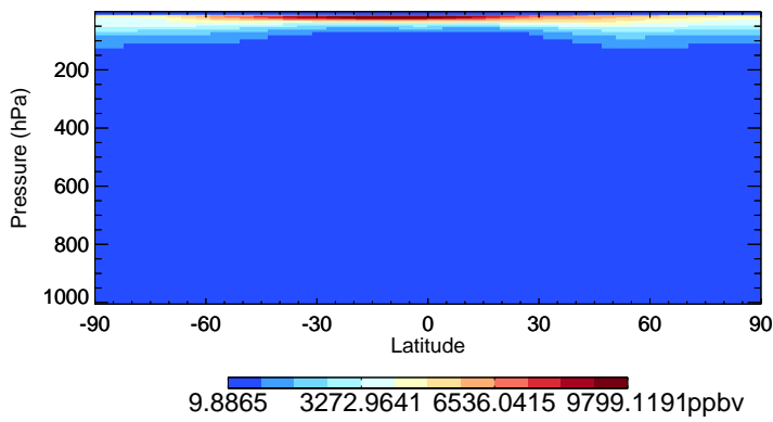
v11-02f-Run0 O3 - Species Zonal Mean for Jan
