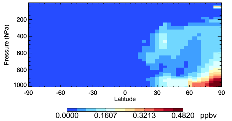
v11-02f-Run0 NIT - Species Curtain @ -180.000 for Jan
