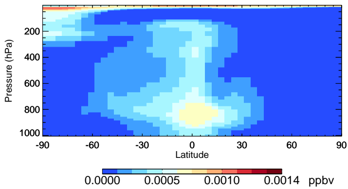
v11-02f-Run0 HBr - Species Zonal Mean for Jan
