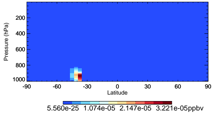
v11-02e-Run1 MACRN - Species Curtain @ -180.000 for Jan
