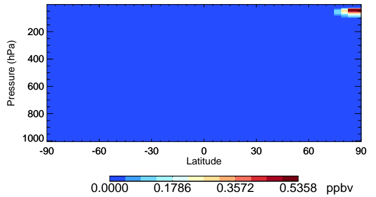
v11-02f-Run0 Cl2O2 - Species Curtain @ -180.000 for Jan
