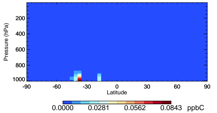
v11-02f-Run0 ISOP - Species Curtain @ -180.000 for Jan
