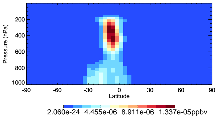
v11-02f-Run0 LVOC - Species Zonal Mean for Jan
