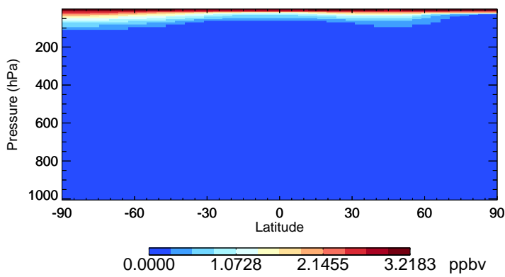
v11-02f-Run0 HCl - Species Zonal Mean for Jan
