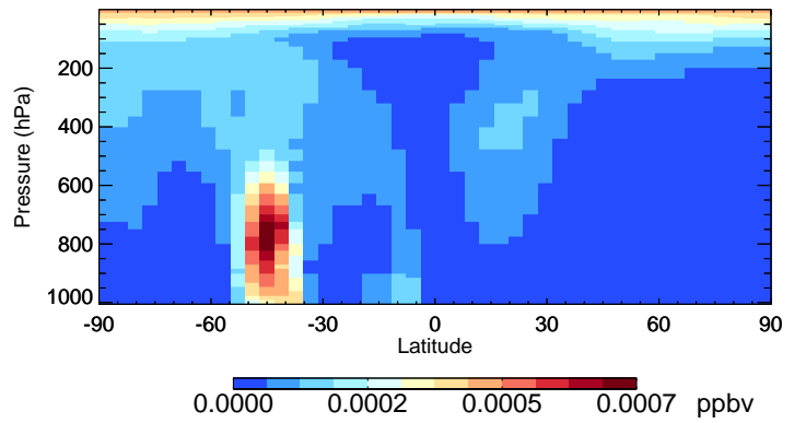
v11-02f-Run0 LVOCOA - Species Curtain @ -180.000 for Jan
