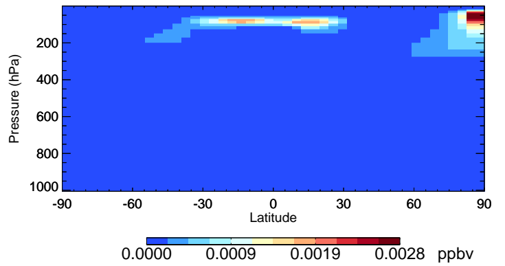
v11-02f-Run0 ISOA3 - Species Curtain @ -180.000 for Jan
