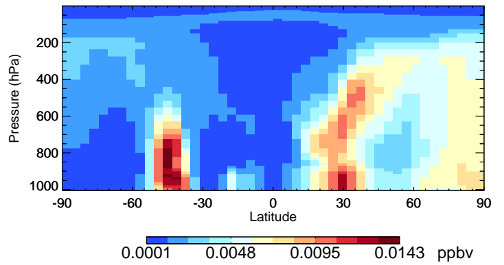
v11-02f-Run0 INDIOL - Species Curtain @ -180.000 for Jan
