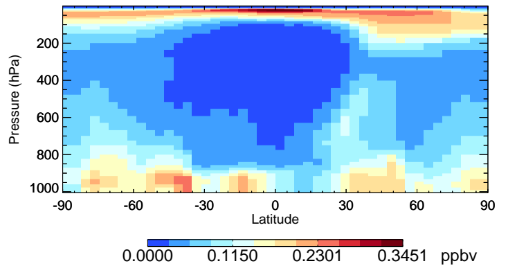
v11-02f-Run0 SO4 - Species Curtain @ -180.000 for Jan
