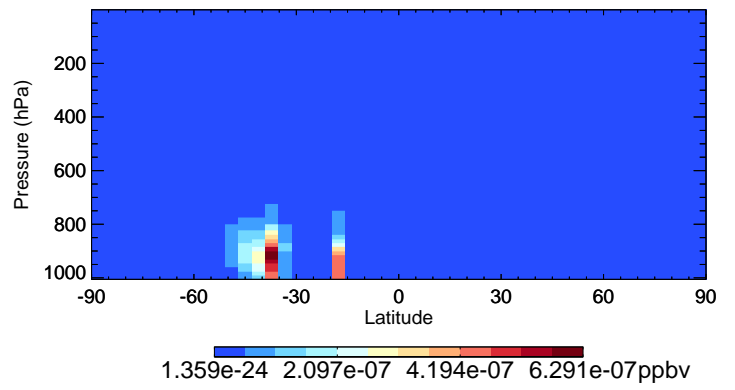
v11-02e-Run0 LVOC - Species Curtain @ -180.000 for Jan
