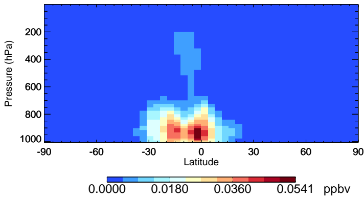
v11-02f-Run0 IEPOXA - Species Zonal Mean for Jan
