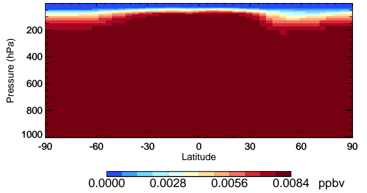
v11-02e-Run1 CH3CCI3 - Species Curtain @ -180.000 for Jan
