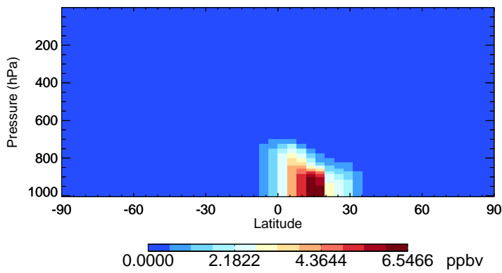
v11-02f-Run0 DST1 - Species Zonal Mean for Jan
