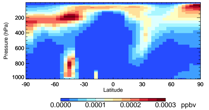
v11-02f-Run0 TSOA1 - Species Curtain @ -180.000 for Jan
