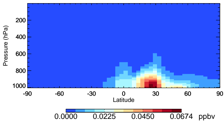
v11-02f-Run0 SOAGX - Species Zonal Mean for Jan
