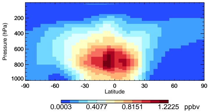
v11-02f-Run0 H2O2 - Species Zonal Mean for Jan
