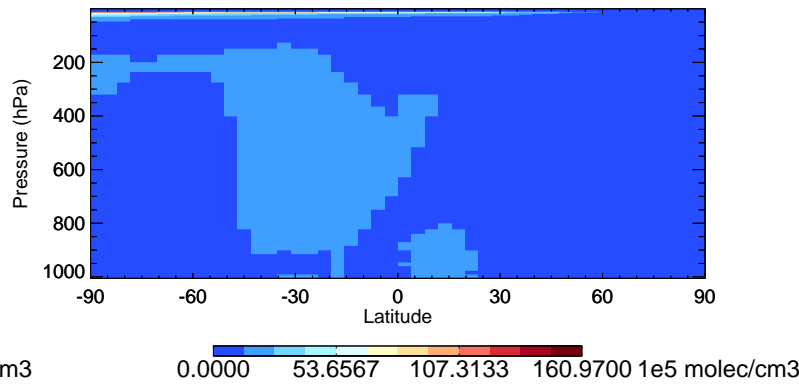
v11-02f-Run0 OH - Species Curtain @ -180.000 for Jan
