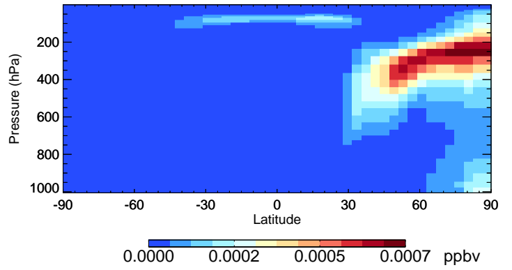
v11-02e-Run1 ASOA2 - Species Curtain @ -180.000 for Jan
