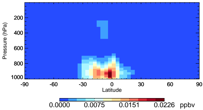
v11-02f-Run0 IEPOXB - Species Zonal Mean for Jan
