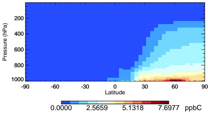
v11-02f-Run0 ALK4 - Species Zonal Mean for Jan
