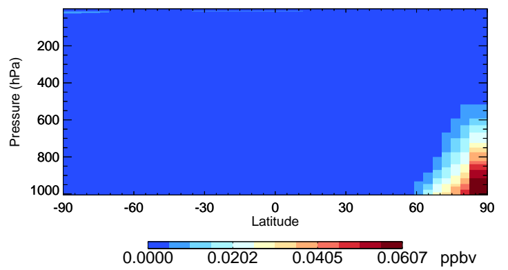
v11-02f-Run0 HNO2 - Species Curtain @ -180.000 for Jan
