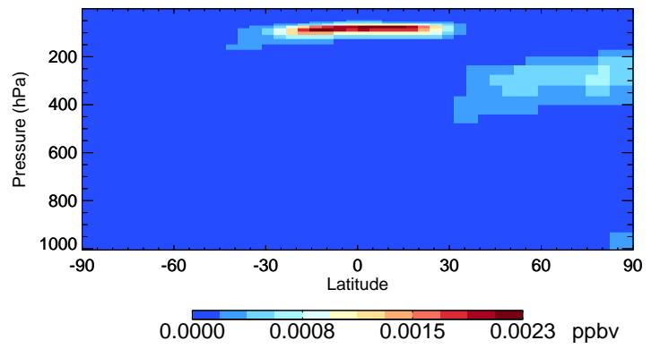
v11-02e-Run0 ASOA3 - Species Curtain @ -180.000 for Jan
