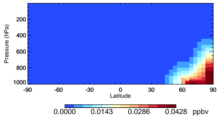
v11-02f-Run0 ClNO 2 - Species Curtain @ -180.000 for Jan
