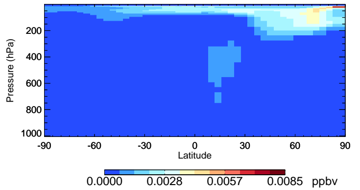
v11-02f-Run0 HOBr - Species Curtain @ -180.000 for Jan
