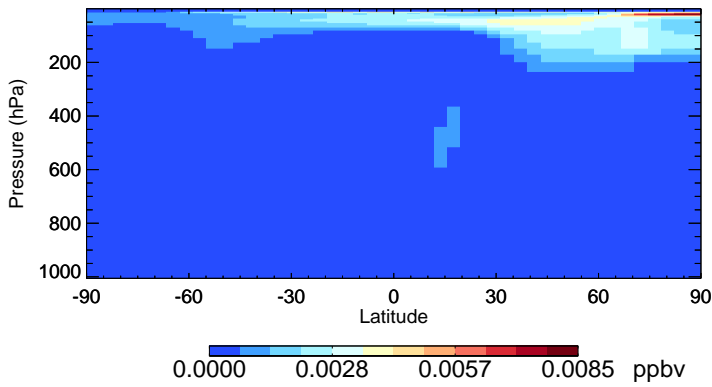
v11-02f-Run0 HOBr - Species Zonal Mean for Jan
