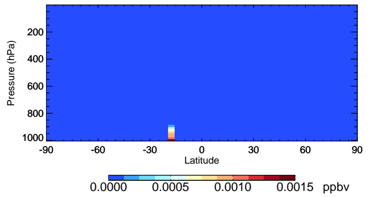
v11-02e-Run0 MTPO - Species Curtain @ -180.000 for Jan
