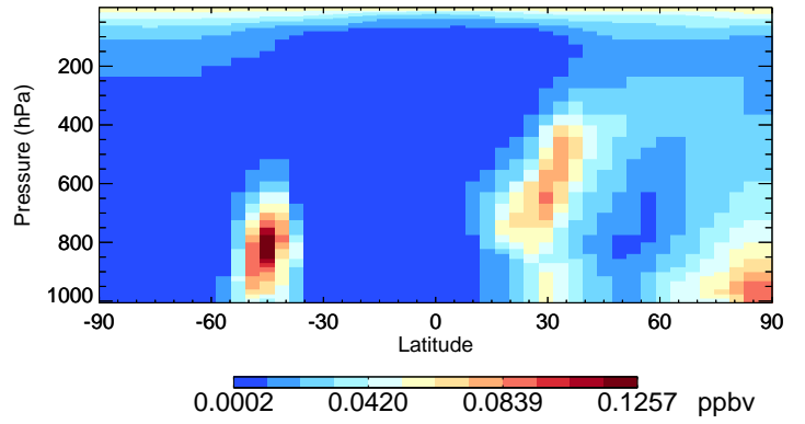
v11-02e-Run1 OCPI - Species Curtain @ -180.000 for Jan
