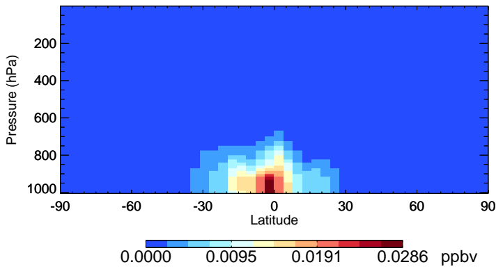
v11-02f-Run0 IPMN - Species Zonal Mean for Jan
