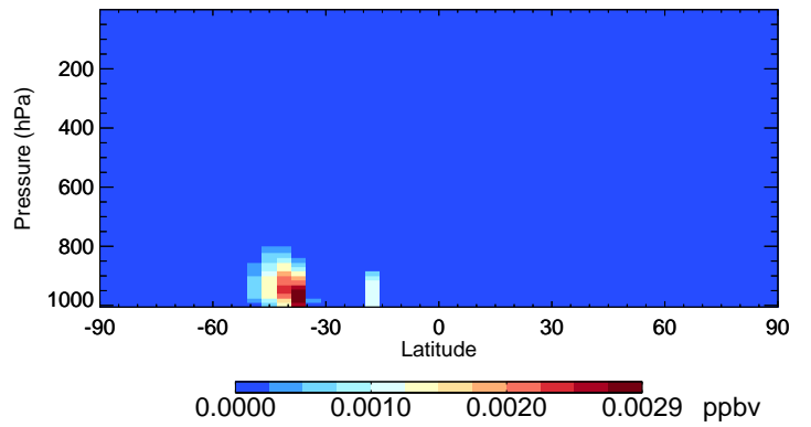
v11-02f-Run0 IEPOXB - Species Curtain @ -180.000 for Jan
