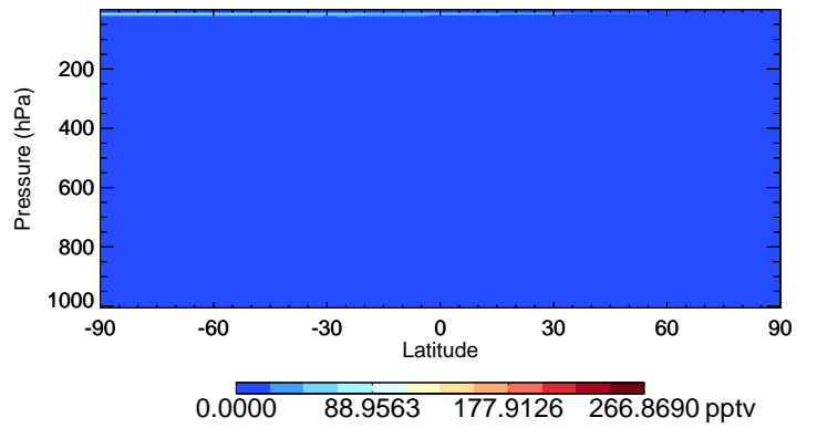
v11-02f-Run0 HO2 - Species Curtain @ -180.000 for Jan
