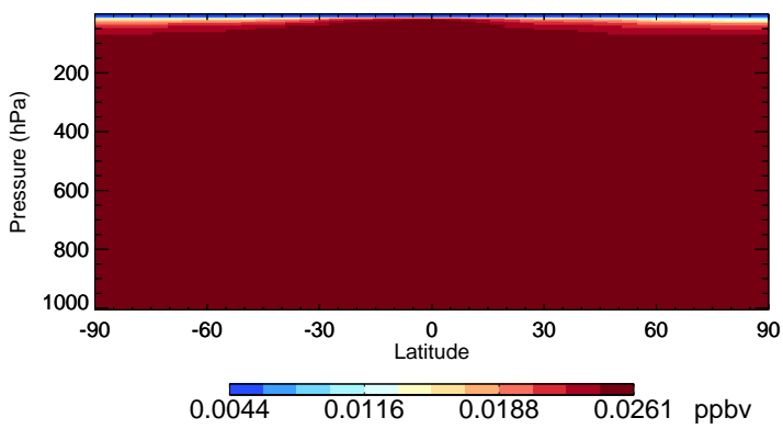
v11-02f-Run0 HCFC142b - Species Zonal Mean for Jan
