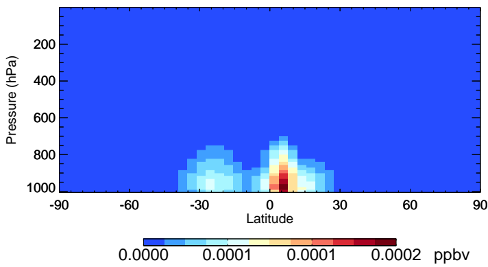
v11-02f-Run0 ETHLN - Species Zonal Mean for Jan
