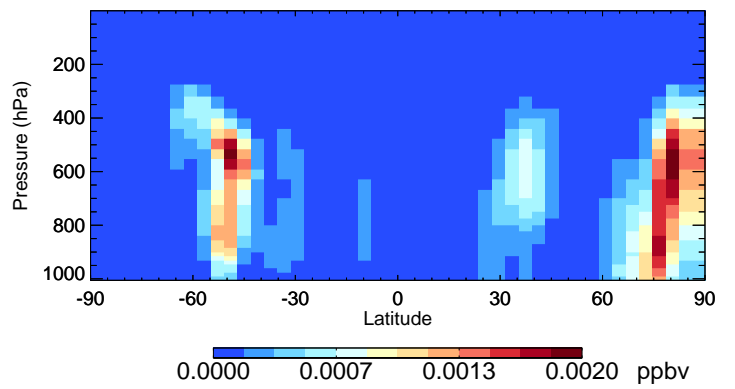
v11-02f-Run0 DST4 - Species Curtain @ -180.000 for Jan
