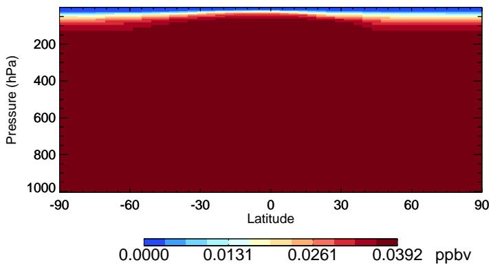
v11-02f-Run0 HCFC141b - Species Zonal Mean for Jan
