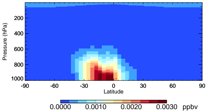
v11-02f-Run0 LVOCOA - Species Zonal Mean for Jan
