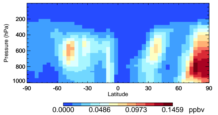
v11-02f-Run0 DST1 - Species Curtain @ -180.000 for Jan
