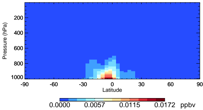
v11-02f-Run0 TSOA1 - Species Zonal Mean for Jan
