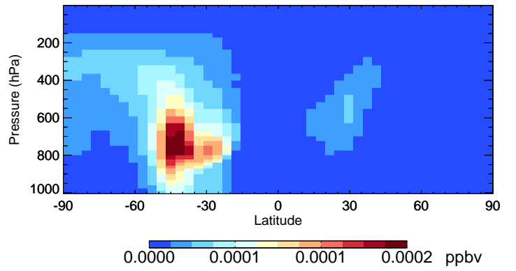
v11-02e-Run0 ISN1OA - Species Curtain @ -180.000 for Jan
