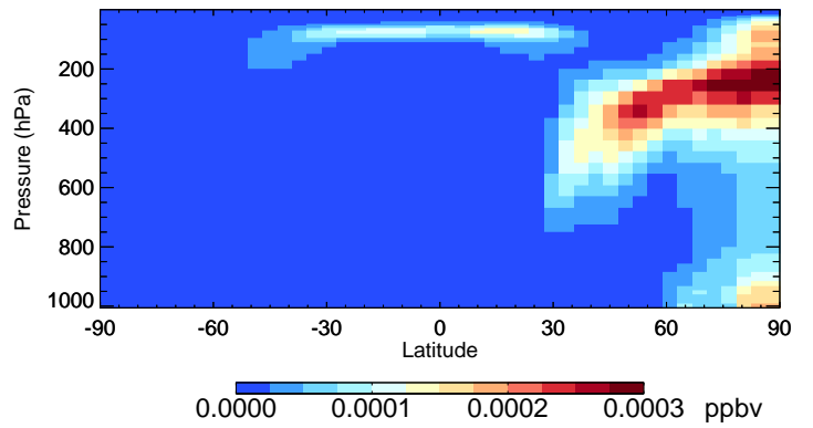
v11-02f-Run0 ASOA2 - Species Curtain @ -180.000 for Jan
