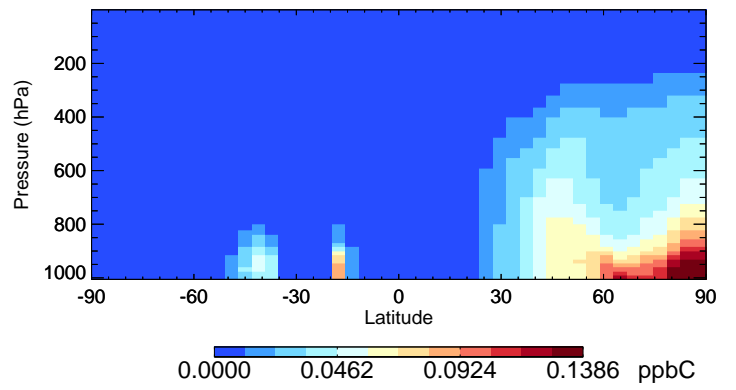
v11-02e-Run1 EOH - Species Curtain @ -180.000 for Jan
