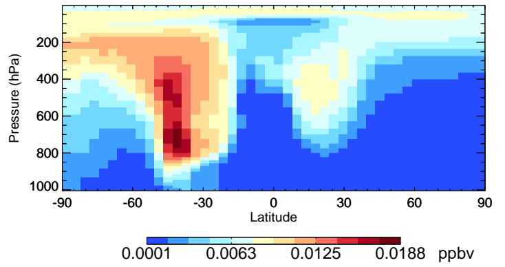
v11-02e-Run0 ISOG3 - Species Curtain @ -180.000 for Jan
