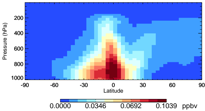
v11-02f-Run0 MAP - Species Zonal Mean for Jan
