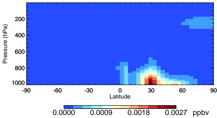
v11-02f-Run0 ASOA2 - Species Zonal Mean for Jan
