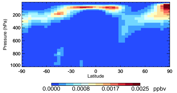
v11-02f-Run0 TSOA2 - Species Curtain @ -180.000 for Jan
