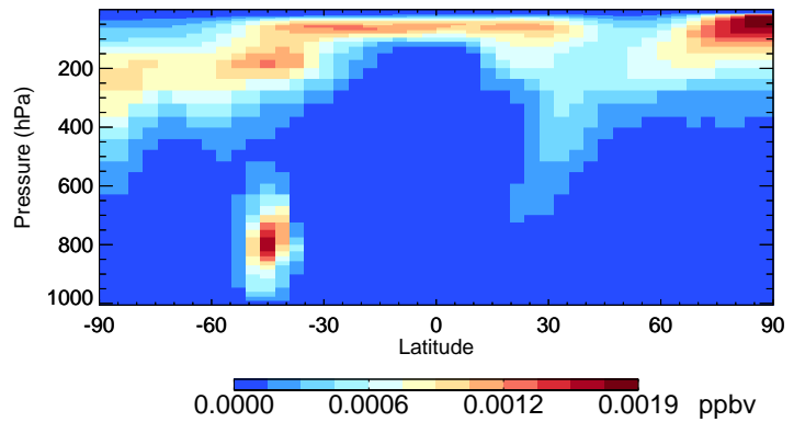
ISOA1 - Species Curtain @ -180.000 for Jan
