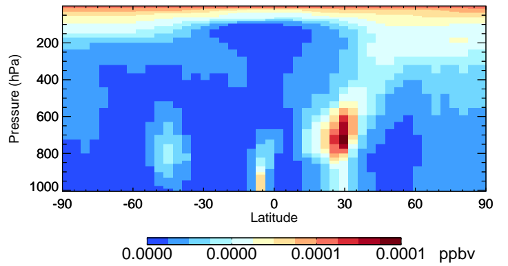
v11-02f-Run0 SOAME - Species Curtain @ -180.000 for Jan
