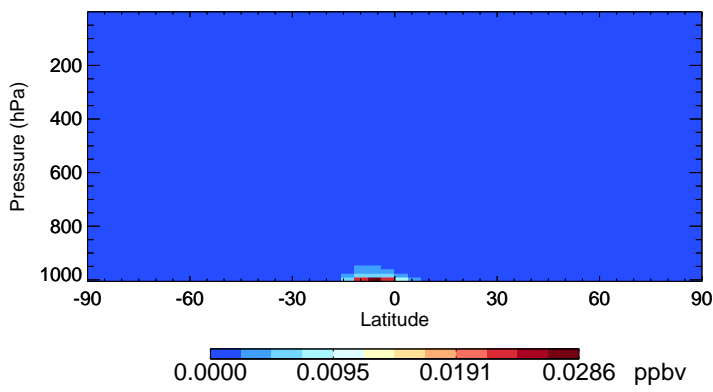
v11-02e-Run1 MTPO - Species Zonal Mean for Jan
