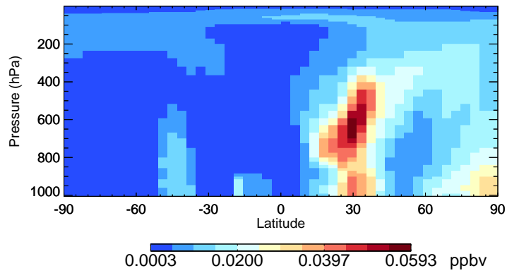
v11-02f-Run0 SOAS - Species Curtain @ -180.000 for Jan
