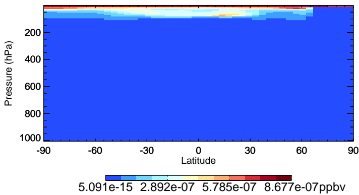
v11-02f-Run0 CIOO - Species Zonal Mean for Jan
