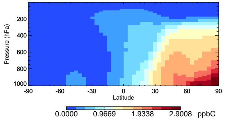
v11-02e-Run0 C2H6 - Species Curtain @ -180.000 for Jan
