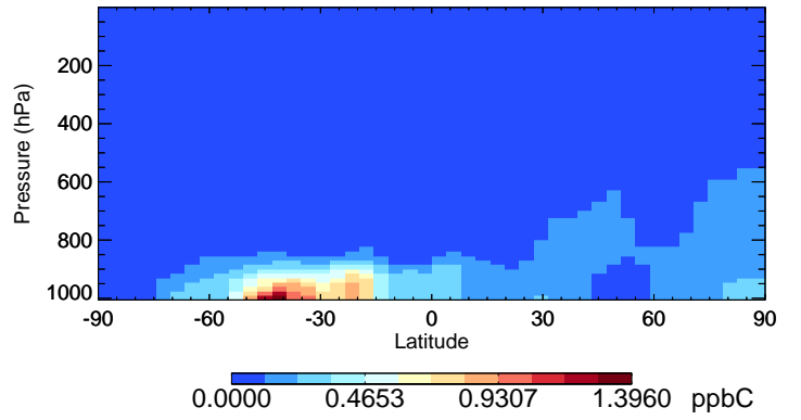
v11-02e-Run1 ALD2 - Species Curtain @ -180.000 for Jan
