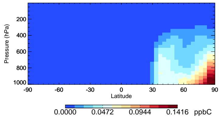
v11-02e-Run1 XYLE - Species Curtain @ -180.000 for Jan
