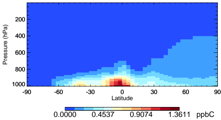
v11-02f-Run0 ALD2 - Species Zonal Mean for Jan
