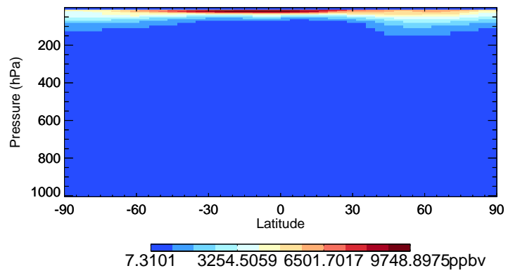
v11-02f-Run0 O3 - Species Curtain @ -180.000 for Jan
