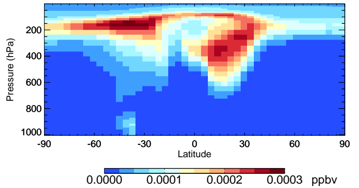
DHDN - Species Curtain @ -180.000 for Jan
