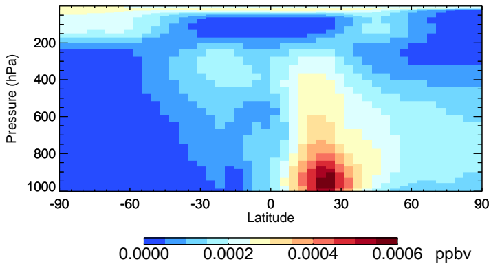
v11-02f-Run0 ASOG1 - Species Zonal Mean for Jan
