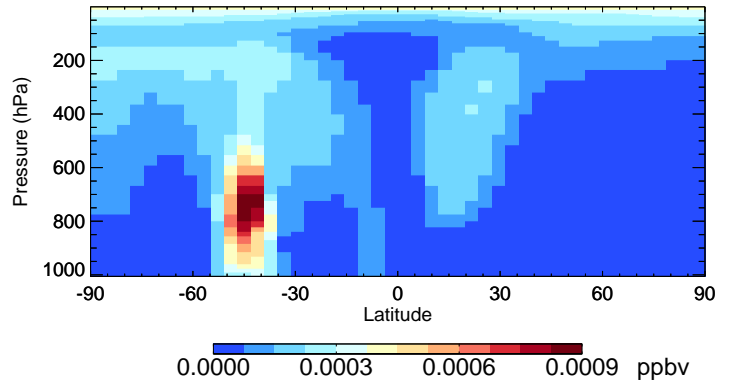
v11-02e-Run1 LVOCOA - Species Curtain @ -180.000 for Jan
