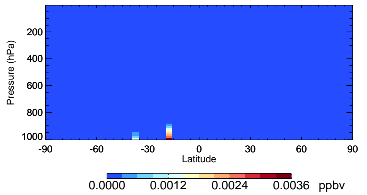
v11-02f-Run0 MTPO - Species Curtain @ -180.000 for Jan
