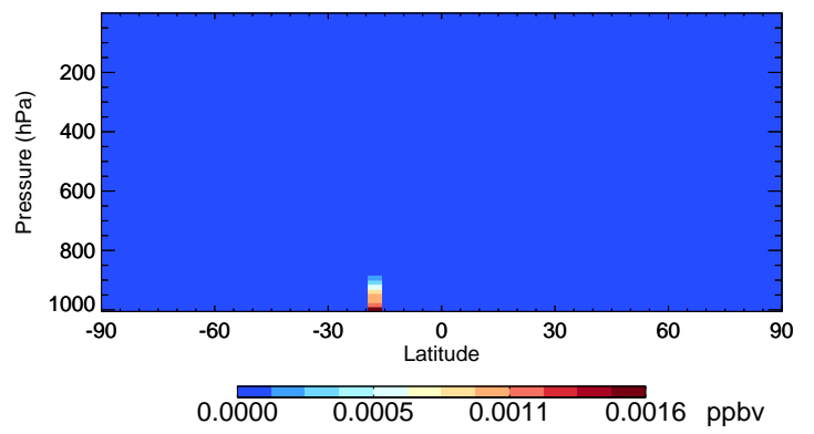
v11-02e-Run1 MTPO - Species Curtain @ -180.000 for Jan
