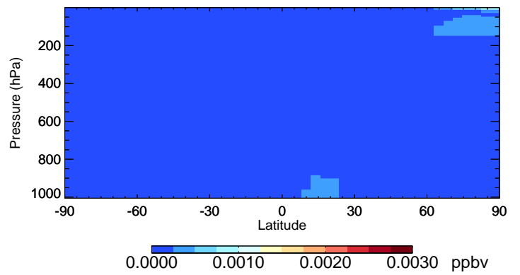
v11-02f-Run0 Br2 - Species Curtain @ -180.000 for Jan
