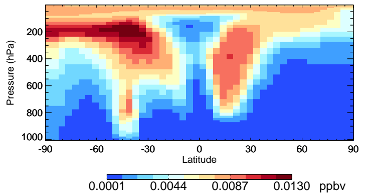
v11-02e-Run1 ISOG3 - Species Curtain @ -180.000 for Jan
