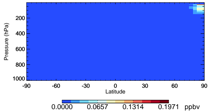
v11-02f-Run0 Cl2 - Species Curtain @ -180.000 for Jan
