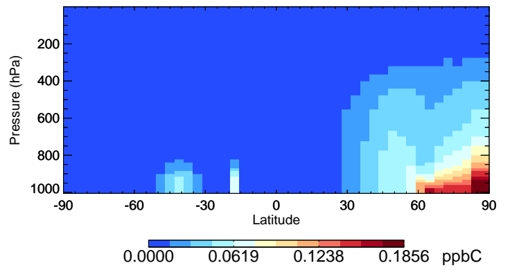
v11-02e-Run0 EOH - Species Curtain @ -180.000 for Jan
