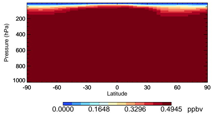
v11-02e-Run1 CFC12 - Species Curtain @ -180.000 for Jan
