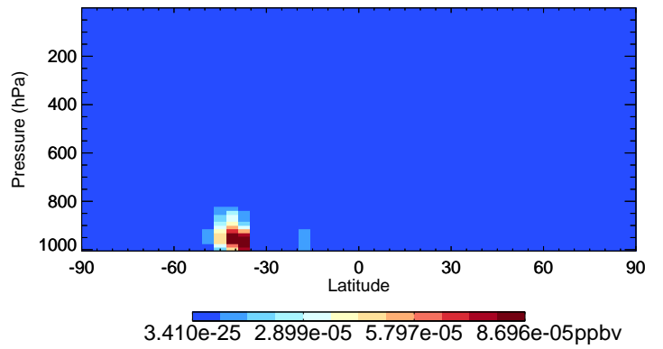
v11-02f-Run0 ISN1 - Species Curtain @ -180.000 for Jan
