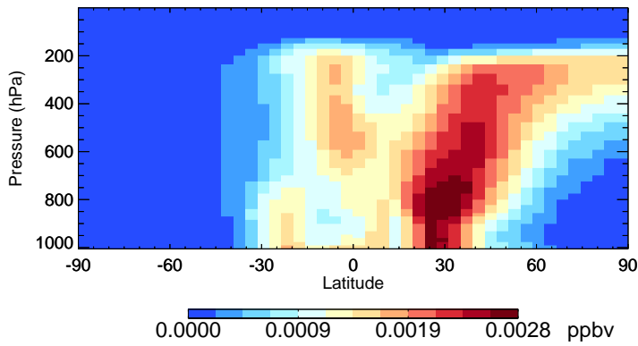
v11-02f-Run0 R4N2 - Species Zonal Mean for Jan
