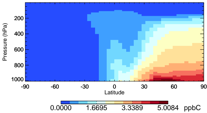
v11-02f-Run0 C2H6 - Species Zonal Mean for Jan
