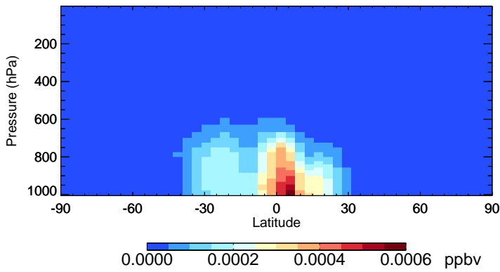
v11-02f-Run0 ISN1OA - Species Zonal Mean for Jan
