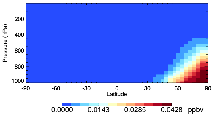
v11-02f-Run0 ClNO 2 - Species Zonal Mean for Jan
