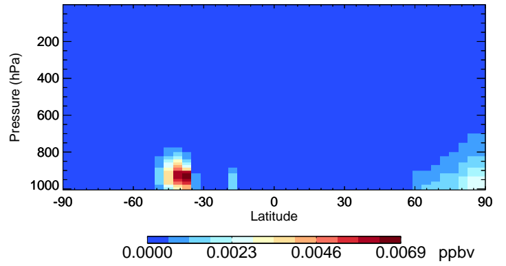
v11-02e-Run1 GLYC - Species Curtain @ -180.000 for Jan
