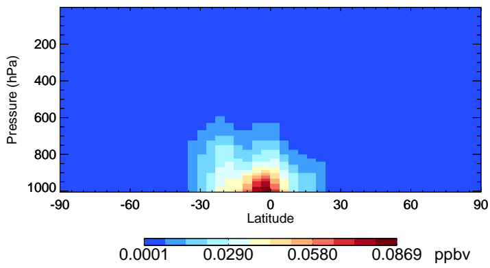
v11-02f-Run0 TSOG2 - Species Zonal Mean for Jan
