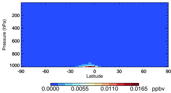
v11-02f-Run0 LIMO - Species Zonal Mean for Jan
