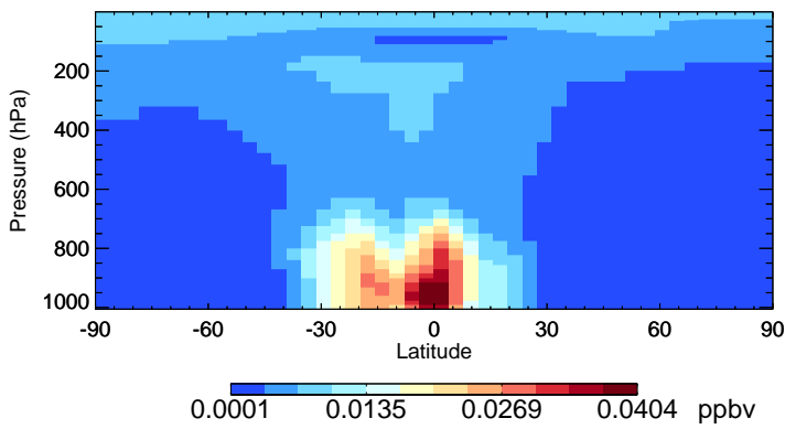
v11-02f-Run0 ISOG3 - Species Zonal Mean for Jan
