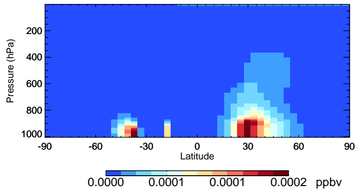
v11-02f-Run0 IONITA - Species Curtain @ -180.000 for Jan
