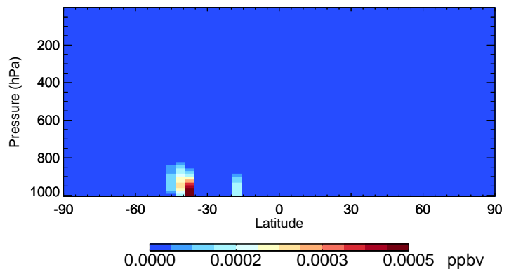
v11-02f-Run0 ISOPNB - Species Curtain @ -180.000 for Jan
