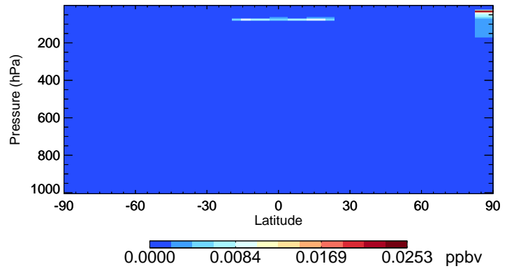
v11-02e-Run0 Cl2 - Species Curtain @ -180.000 for Jan
