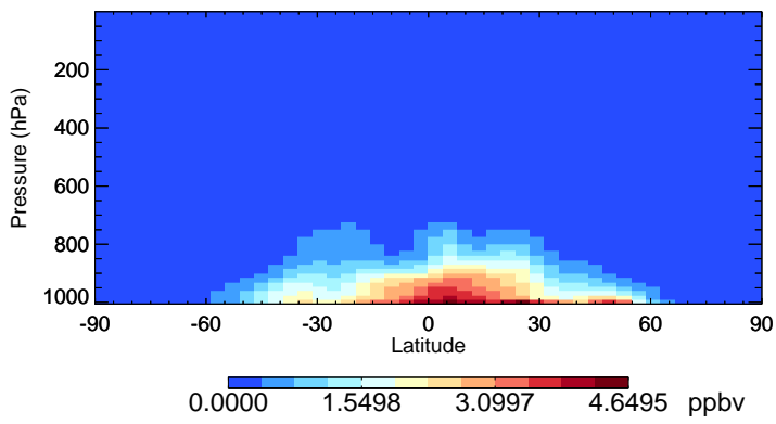
v11-02f-Run0 NH3 - Species Zonal Mean for Jan
