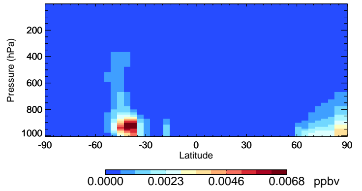
v11-02e-Run0 GLYC - Species Curtain @ -180.000 for Jan
