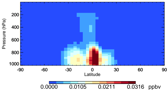
v11-02f-Run0 IMAE - Species Zonal Mean for Jan
