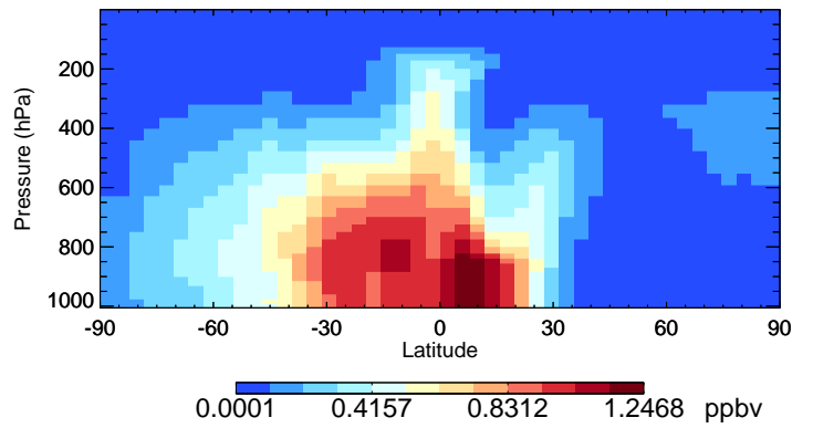
v11-02f-Run0 MP - Species Curtain @ -180.000 for Jan
