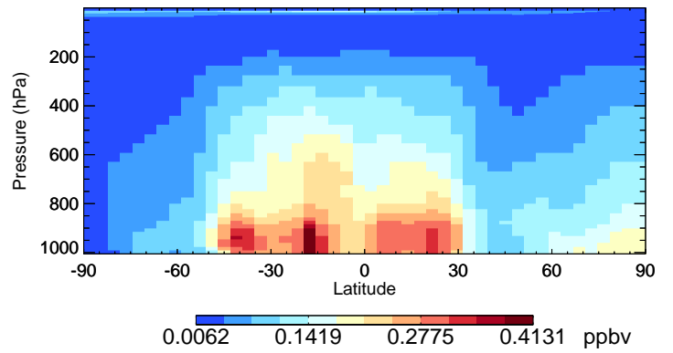
v11-02f-Run0 CH2O - Species Curtain @ -180.000 for Jan
