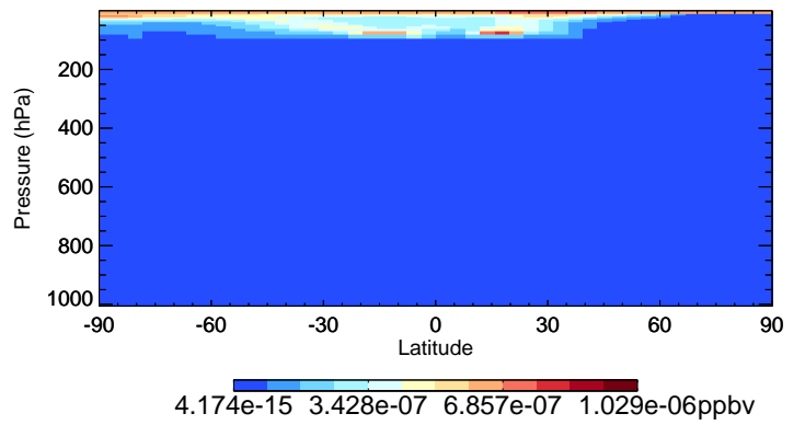
v11-02e-Run1 CIOO - Species Curtain @ -180.000 for Jan
