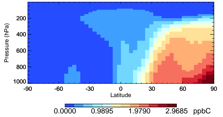
v11-02e-Run1 C2H6 - Species Curtain @ -180.000 for Jan
