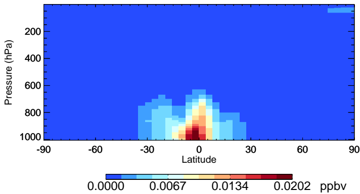
ISOA1 - Species Zonal Mean for Jan
