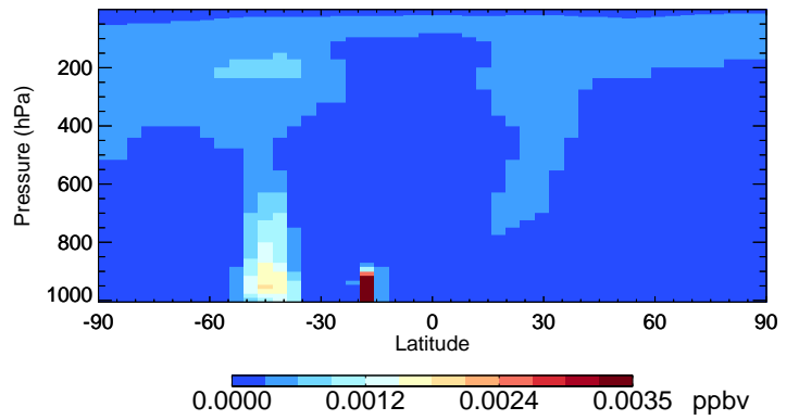
v11-02f-Run0 TSOA0 - Species Curtain @ -180.000 for Jan
