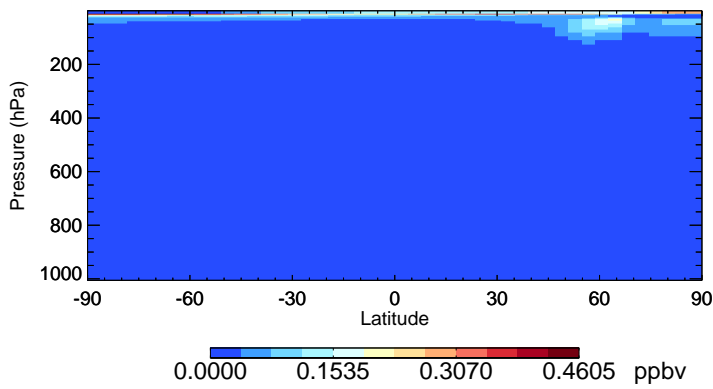
v11-02f-Run0 CIO - Species Zonal Mean for Jan
