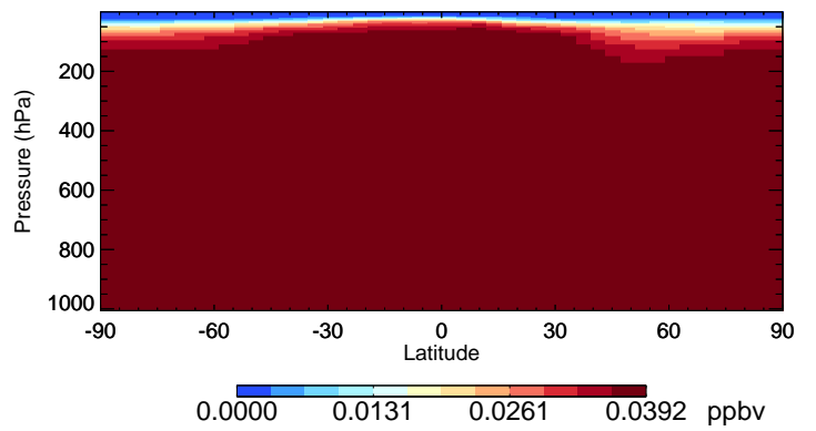
v11-02f-Run0 HCFC141b - Species Curtain @ -180.000 for Jan
