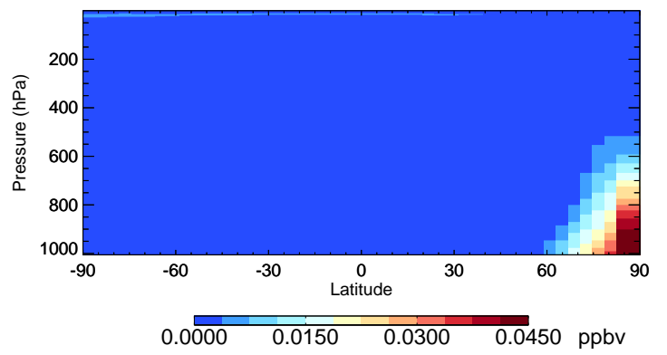
v11-02e-Run1 HNO2 - Species Curtain @ -180.000 for Jan
