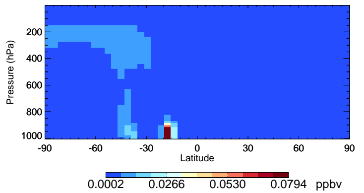
v11-02f-Run0 TSOG3 - Species Curtain @ -180.000 for Jan
