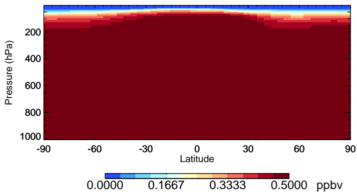
v11-02f-Run0 OCS - Species Zonal Mean for Jan
