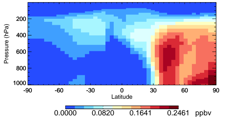
v11-02e-Run0 PAN - Species Curtain @ -180.000 for Jan
