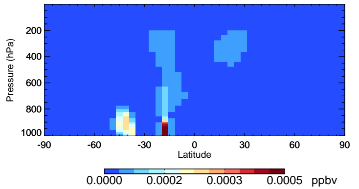
v11-02f-Run0 HONIT - Species Curtain @ -180.000 for Jan
