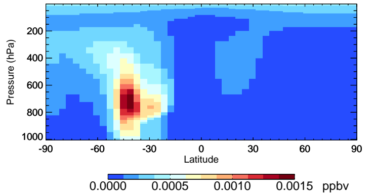
v11-02e-Run0 LVOCOA - Species Curtain @ -180.000 for Jan
