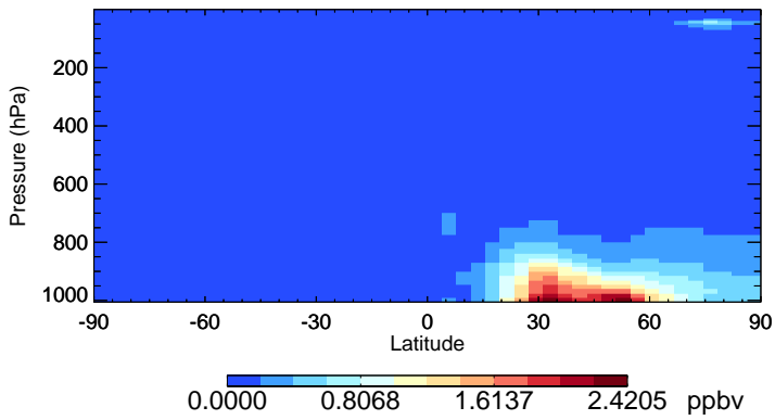
v11-02f-Run0 NIT - Species Zonal Mean for Jan
