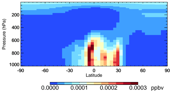
v11-02f-Run0 SOAME - Species Zonal Mean for Jan
