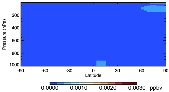
v11-02f-Run0 Br2 - Species Zonal Mean for Jan
