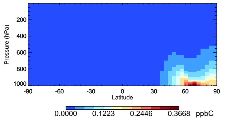
v11-02f-Run0 XYLE - Species Curtain @ -180.000 for Jan
