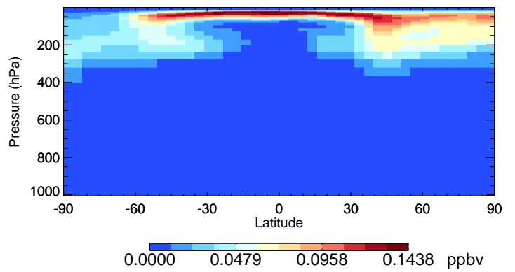
v11-02f-Run0 MPN - Species Curtain @ -180.000 for Jan
