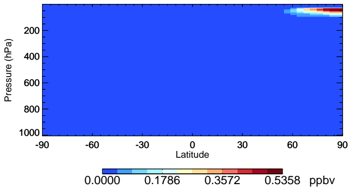
v11-02f-Run0 Cl2O2 - Species Zonal Mean for Jan
