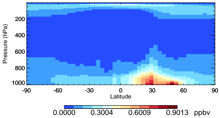
v11-02f-Run0 SO4 - Species Zonal Mean for Jan
