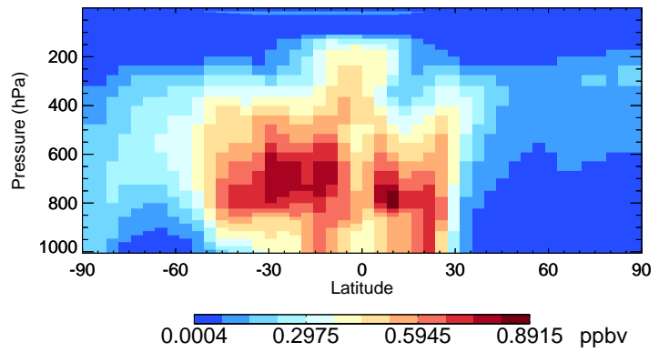
v11-02f-Run0 H2O2 - Species Curtain @ -180.000 for Jan
