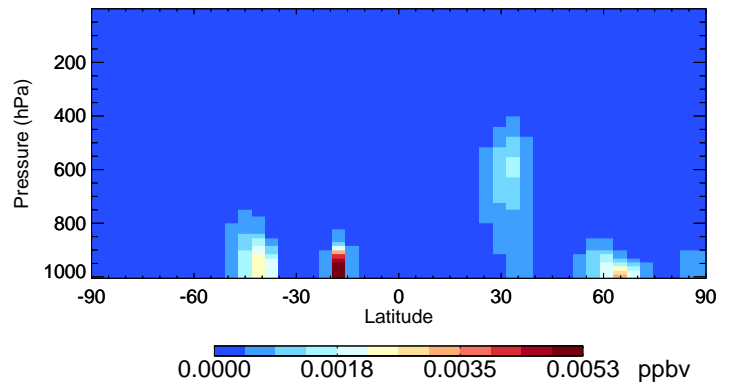
v11-02f-Run0 BCPO - Species Curtain @ -180.000 for Jan
