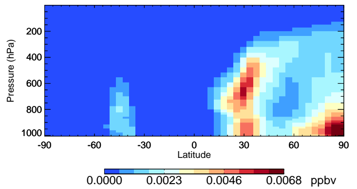
v11-02f-Run0 SOAGX - Species Curtain @ -180.000 for Jan
