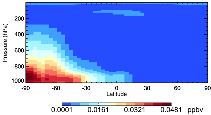
v11-02f-Run0 MSA - Species Zonal Mean for Jan
