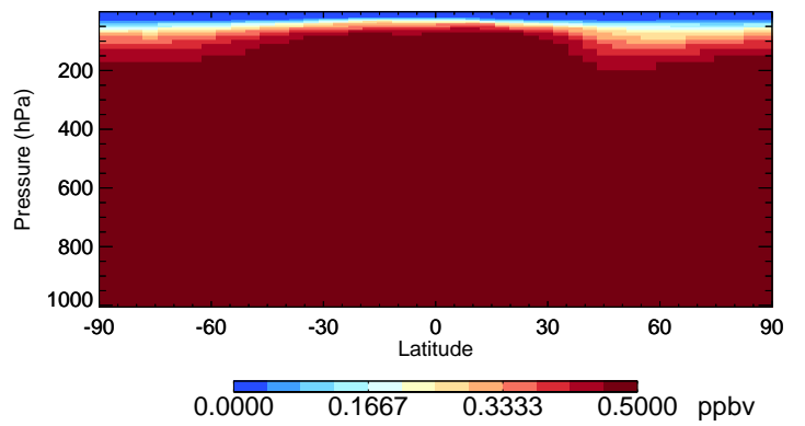
v11-02f-Run0 OCS - Species Curtain @ -180.000 for Jan
