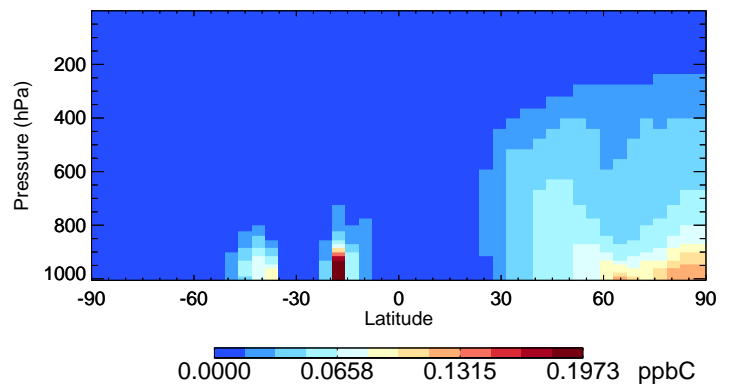
v11-02f-Run0 EOH - Species Curtain @ -180.000 for Jan
