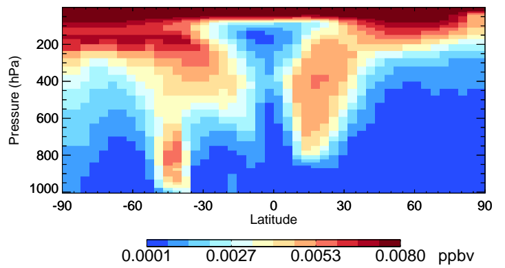
v11-02f-Run0 ISOG3 - Species Curtain @ -180.000 for Jan
