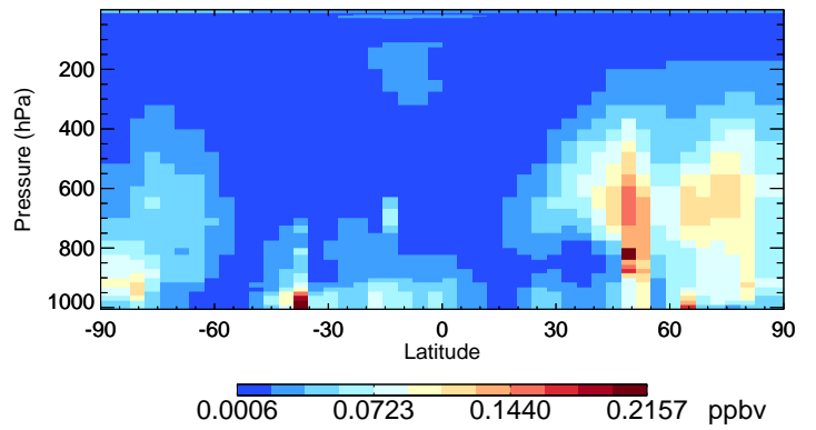
v11-02f-Run0 SO2 - Species Curtain @ -180.000 for Jan
