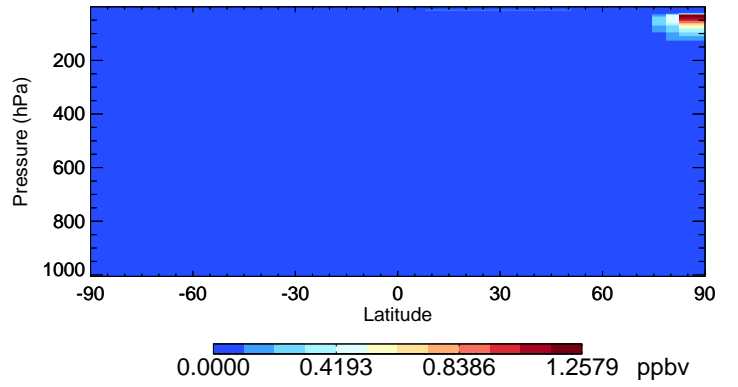
v11-02e-Run1 HOCl - Species Curtain @ -180.000 for Jan
