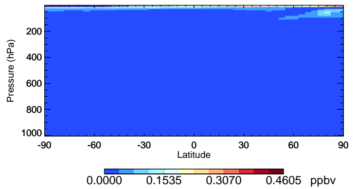
v11-02f-Run0 CIO - Species Curtain @ -180.000 for Jan
