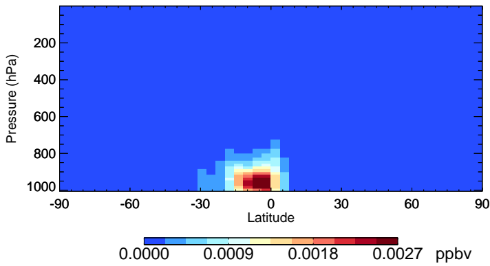
v11-02f-Run0 RIPD - Species Zonal Mean for Jan
