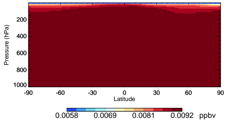
v11-02f-Run0 CFC115 - Species Curtain @ -180.000 for Jan
