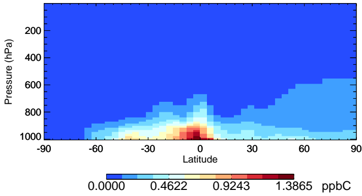
v11-02e-Run1 ALD2 - Species Zonal Mean for Jan
