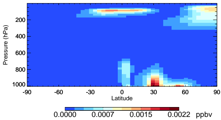
v11-02f-Run0 ASOA3 - Species Zonal Mean for Jan
