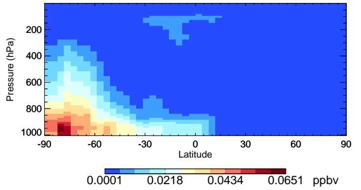
v11-02e-Run1 MSA - Species Curtain @ -180.000 for Jan
