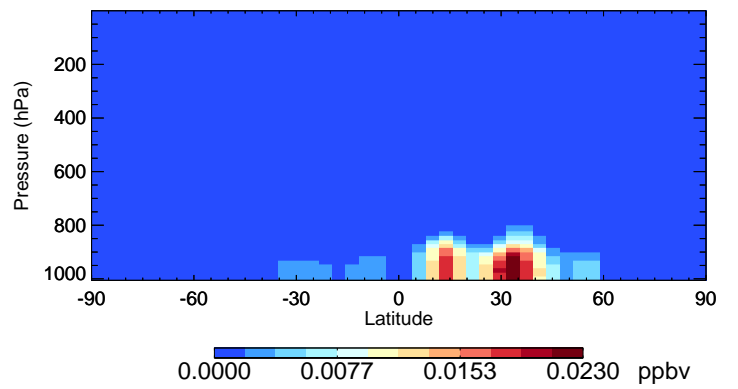
v11-02f-Run0 NITs - Species Curtain @ -180.000 for Jan
