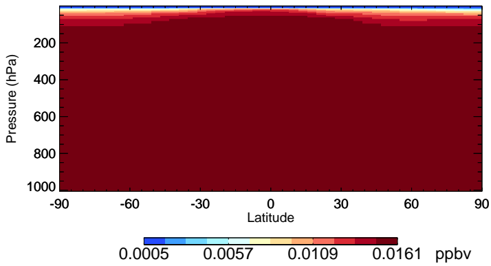
v11-02f-Run0 CFC114 - Species Zonal Mean for Jan
