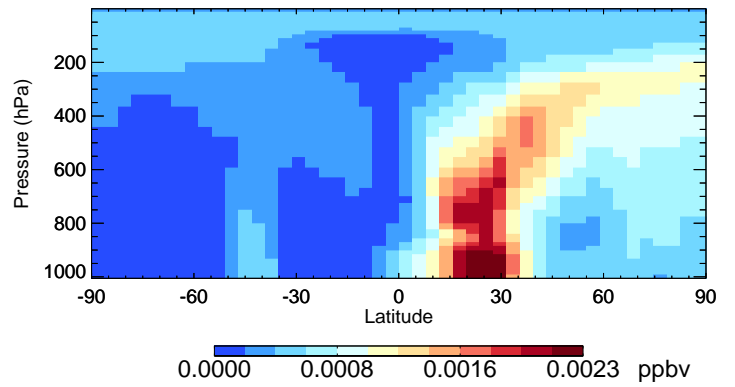
v11-02f-Run0 ASOAN - Species Curtain @ -180.000 for Jan
