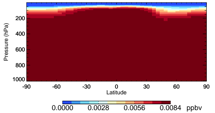
v11-02f-Run0 CH3CCI3 - Species Curtain @ -180.000 for Jan
