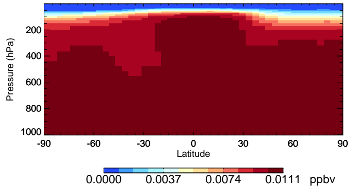
v11-02e-Run0 CH3CCI3 - Species Curtain @ -180.000 for Jan
