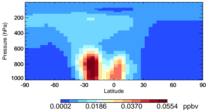
v11-02e-Run0 ISOG3 - Species Zonal Mean for Jan
