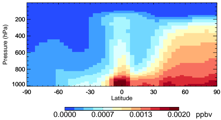
v11-02f-Run0 CHBr3 - Species Zonal Mean for Jan
