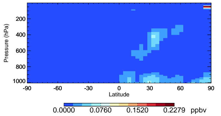
v11-02e-Run1 NIT - Species Curtain @ -180.000 for Jan
