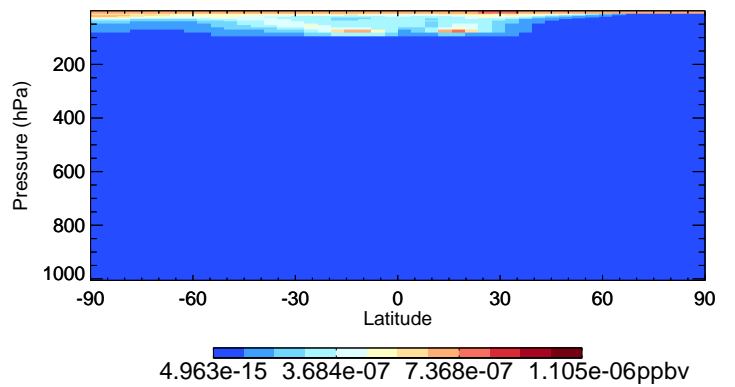
v11-02f-Run0 CIOO - Species Curtain @ -180.000 for Jan
