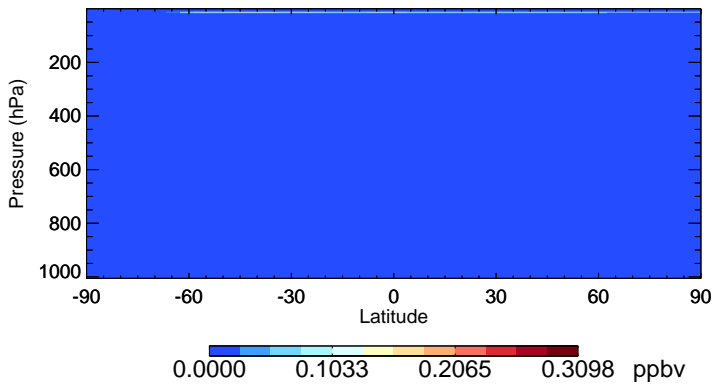
v11-02f-Run0 NO3 - Species Zonal Mean for Jan
