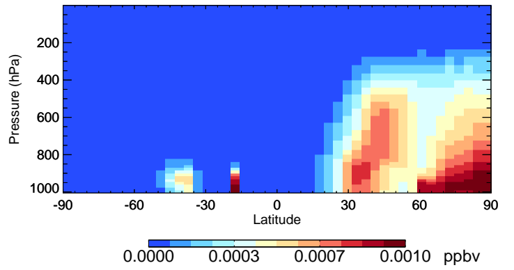
v11-02e-Run0 GLYX - Species Curtain @ -180.000 for Jan
