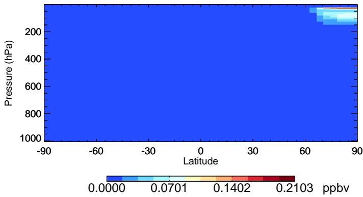
v11-02f-Run0 Cl2 - Species Zonal Mean for Jan
