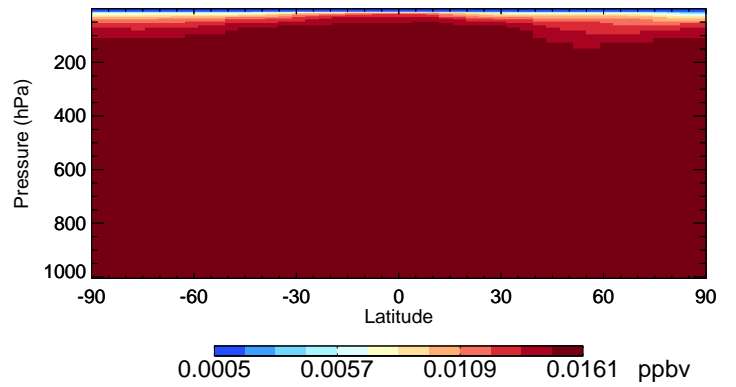
v11-02f-Run0 CFC114 - Species Curtain @ -180.000 for Jan
