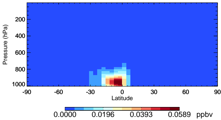
v11-02f-Run0 RIPA - Species Zonal Mean for Jan
