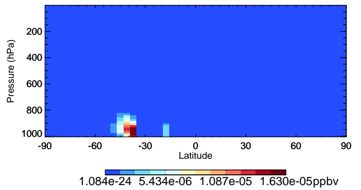
v11-02f-Run0 ETHLN - Species Curtain @ -180.000 for Jan
