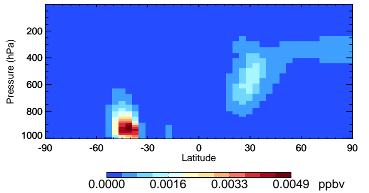
v11-02f-Run0 IMAE - Species Curtain @ -180.000 for Jan
