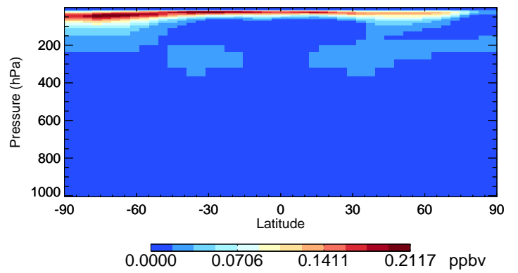
v11-02f-Run0 HNO4 - Species Curtain @ -180.000 for Jan
