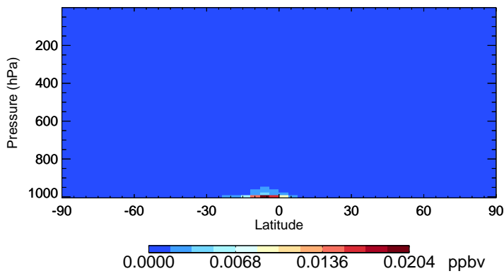
v11-02f-Run0 MTPO - Species Zonal Mean for Jan
