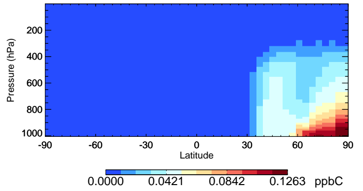
v11-02e-Run0 XYLE - Species Curtain @ -180.000 for Jan
