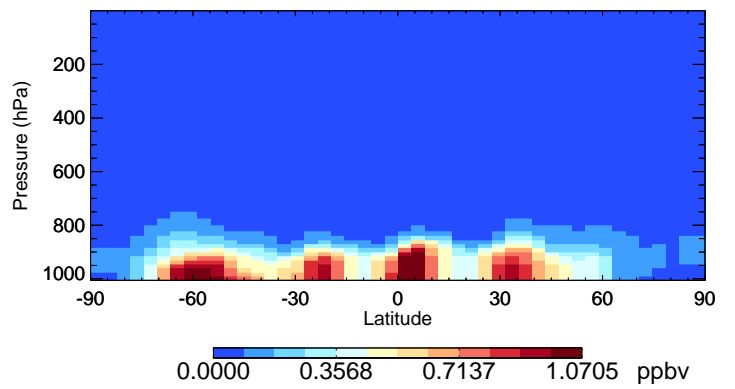
v11-02f-Run0 SALA - Species Curtain @ -180.000 for Jan
