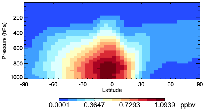
v11-02f-Run0 MP - Species Zonal Mean for Jan
