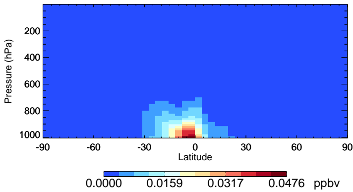
v11-02f-Run0 TSOA0 - Species Zonal Mean for Jan
