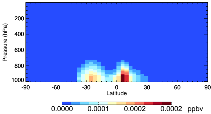
v11-02f-Run0 MACRN - Species Zonal Mean for Jan
