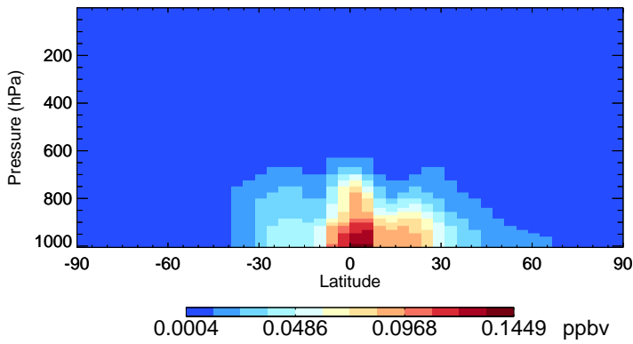
v11-02f-Run0 INDIOL - Species Zonal Mean for Jan
