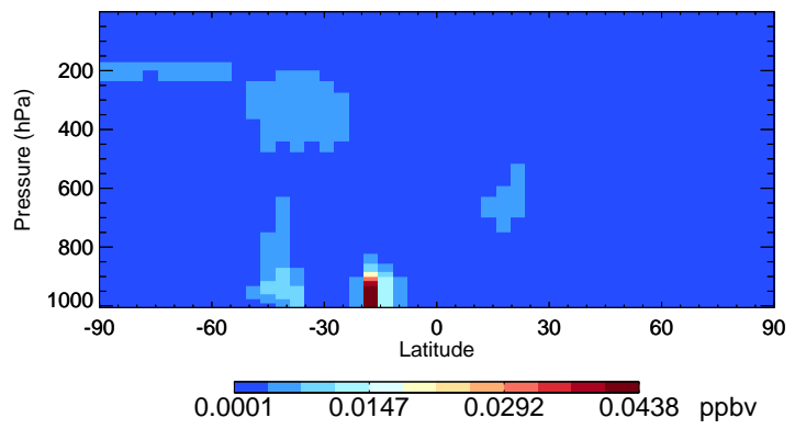
v11-02f-Run0 TSOG2 - Species Curtain @ -180.000 for Jan
