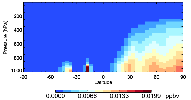
v11-02f-Run0 RCHO - Species Curtain @ -180.000 for Jan
