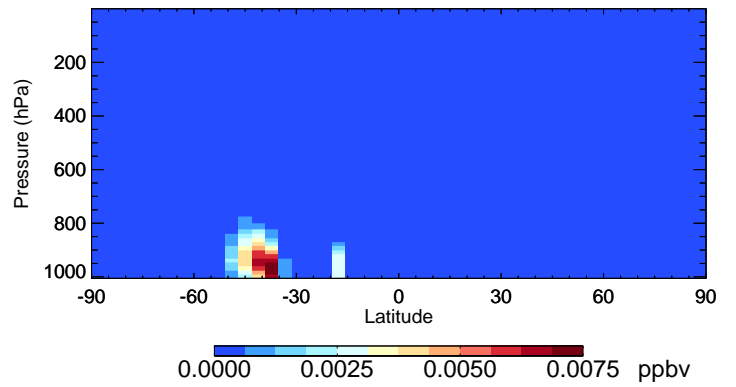
v11-02f-Run0 IEPOXA - Species Curtain @ -180.000 for Jan
