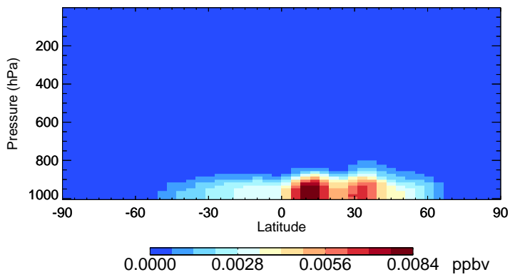
v11-02f-Run0 NITs - Species Zonal Mean for Jan
