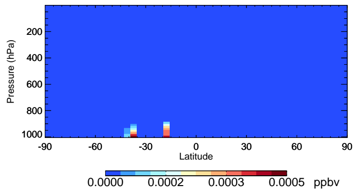
v11-02f-Run0 LIMO - Species Curtain @ -180.000 for Jan
