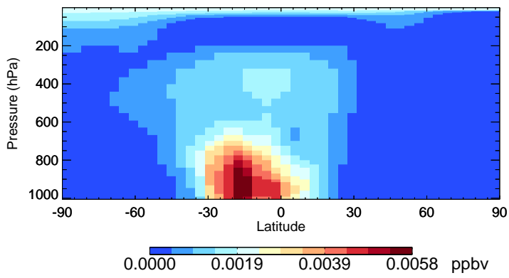
v11-02f-Run0 ISOG1 - Species Zonal Mean for Jan
