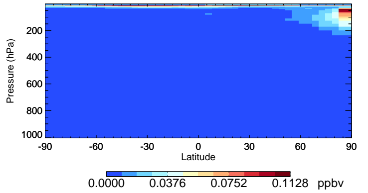
v11-02e-Run0 HOCl - Species Curtain @ -180.000 for Jan
