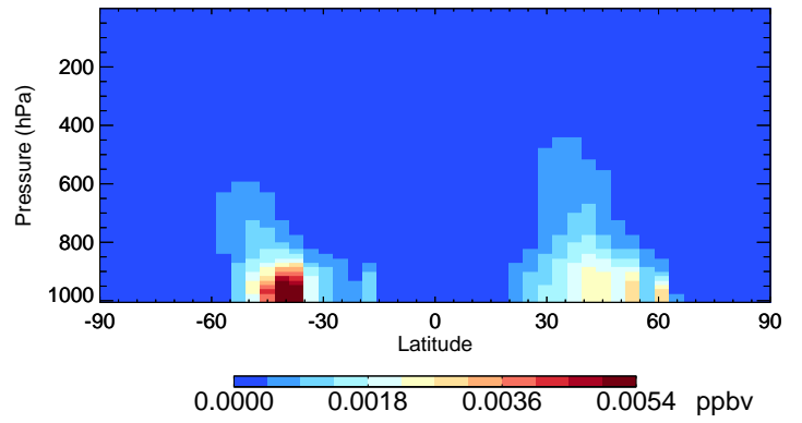
v11-02e-Run0 BCPO - Species Curtain @ -180.000 for Jan
