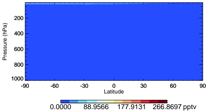
v11-02f-Run0 HO2 - Species Zonal Mean for Jan
