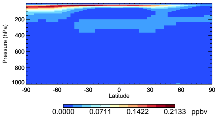
v11-02f-Run0 HNO4 - Species Zonal Mean for Jan
