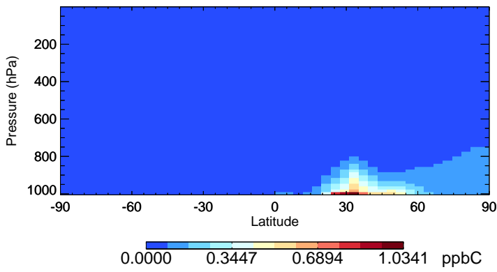
v11-02e-Run1 XYLE - Species Zonal Mean for Jan
