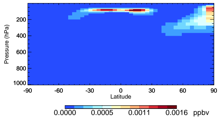
v11-02f-Run0 ASOA3 - Species Curtain @ -180.000 for Jan
