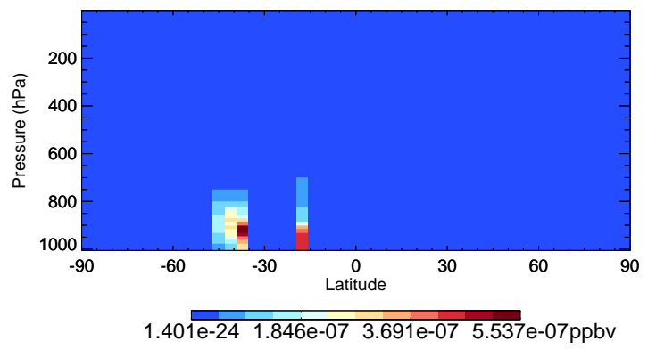
v11-02e-Run1 LVOC - Species Curtain @ -180.000 for Jan
