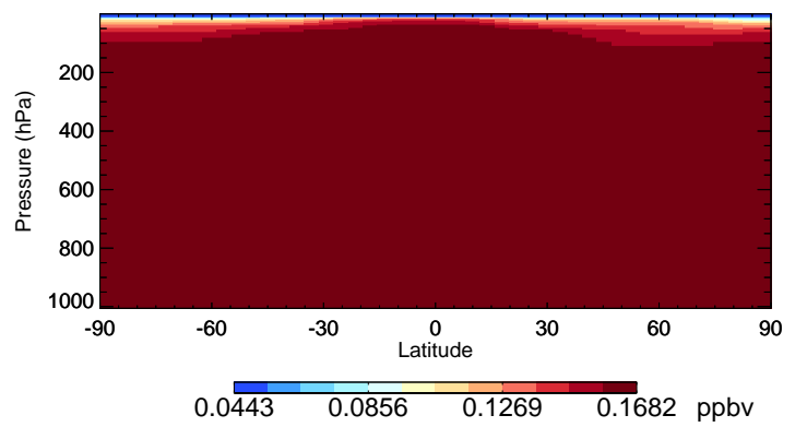
v11-02f-Run0 HCFC22 - Species Curtain @ -180.000 for Jan
