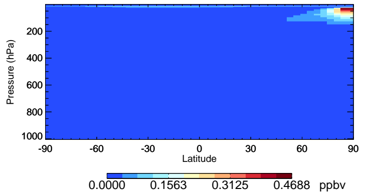
v11-02f-Run0 HOCl - Species Curtain @ -180.000 for Jan
