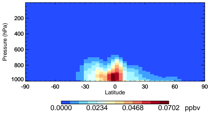
v11-02f-Run0 GLYC - Species Zonal Mean for Jan
