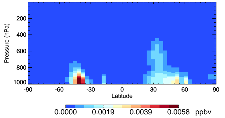
v11-02e-Run1 BCPO - Species Curtain @ -180.000 for Jan
