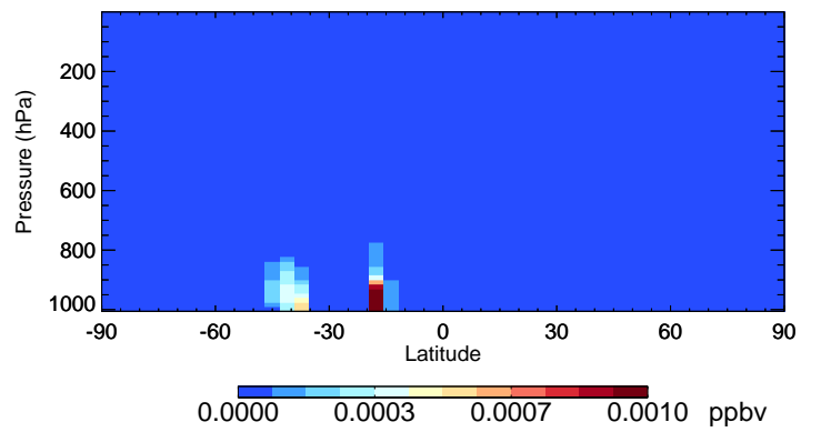
v11-02f-Run0 MONITS - Species Curtain @ -180.000 for Jan
