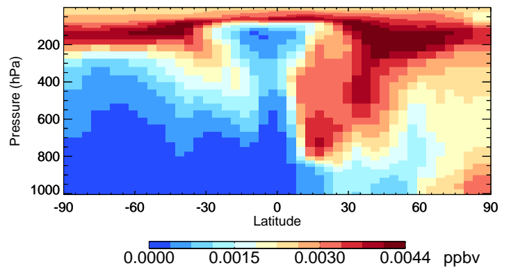
v11-02f-Run0 ASOG3 - Species Curtain @ -180.000 for Jan
