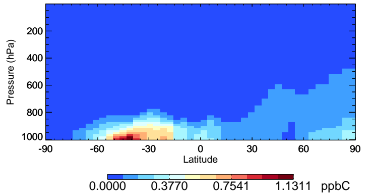
v11-02e-Run0 ALD2 - Species Curtain @ -180.000 for Jan
