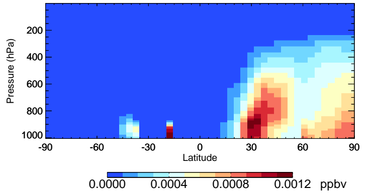
v11-02e-Run1 GLYX - Species Curtain @ -180.000 for Jan
