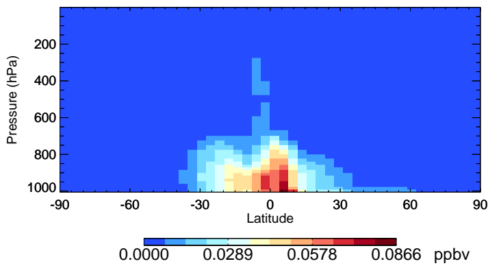
v11-02f-Run0 HAC - Species Zonal Mean for Jan
