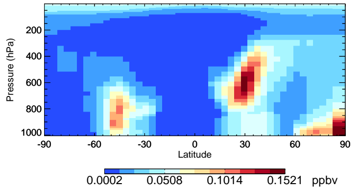
v11-02e-Run0 OCPI - Species Curtain @ -180.000 for Jan
