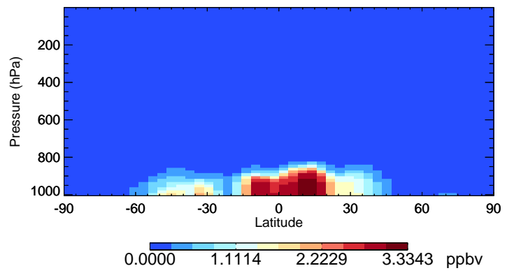
v11-02f-Run0 NH3 - Species Curtain @ -180.000 for Jan
