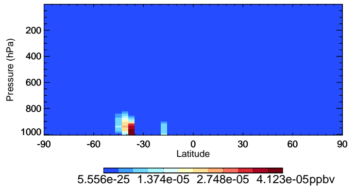
v11-02f-Run0 MACRN - Species Curtain @ -180.000 for Jan
