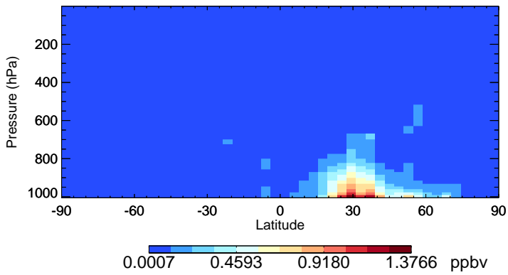
v11-02f-Run0 SO2 - Species Zonal Mean for Jan
