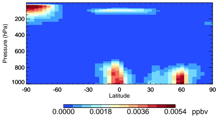
v11-02f-Run0 ISOA3 - Species Zonal Mean for Jul
