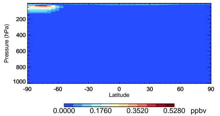
v11-02f-Run0 HOCl - Species Curtain @ -180.000 for Jul
