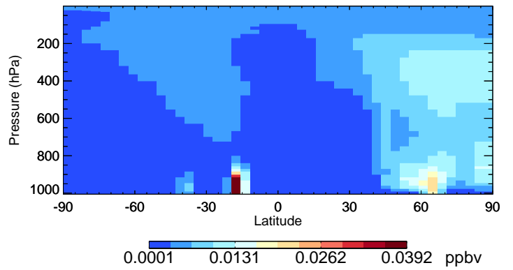
v11-02f-Run0 TSOG3 - Species Curtain @ -180.000 for Jul
