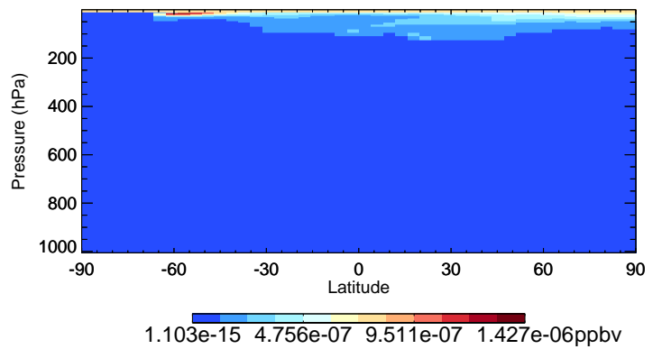
v11-02f-Run0 CIOO - Species Curtain @ -180.000 for Jul
