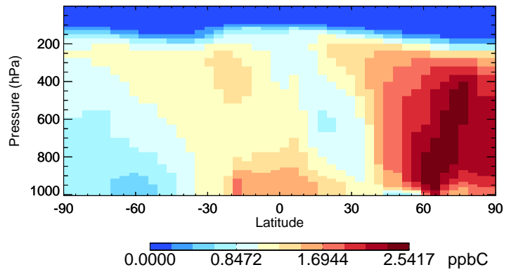
v11-02f-Run0 ACET - Species Curtain @ -180.000 for Jul
