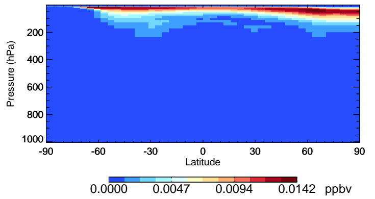
v11-02e-Run0 BrNO3 - Species Curtain @ -180.000 for Jul
