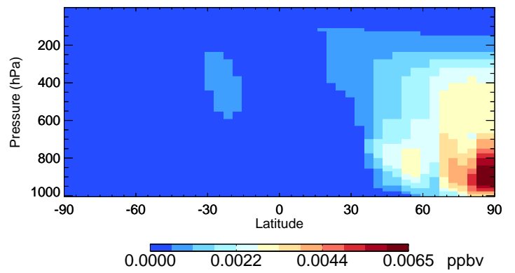
v11-02f-Run0 ASOAN - Species Curtain @ -180.000 for Jul
