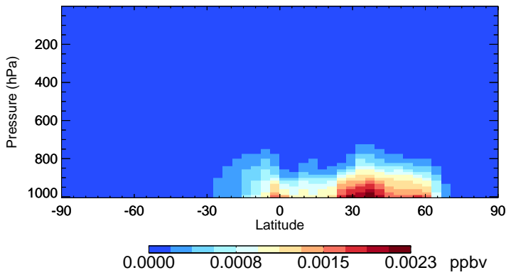
v11-02f-Run0 IONITA - Species Zonal Mean for Jul
