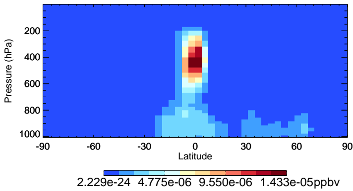
v11-02f-Run0 LVOC - Species Zonal Mean for Jul
