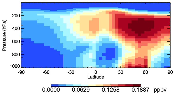
v11-02f-Run0 PAN - Species Zonal Mean for Jul
