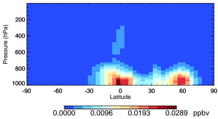
v11-02f-Run0 IPMN - Species Zonal Mean for Jul
