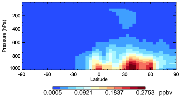
v11-02f-Run0 SOAS - Species Zonal Mean for Jul
