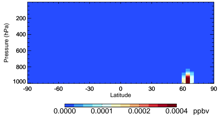
v11-02e-Run1 MOBA - Species Curtain @ -180.000 for Jul
