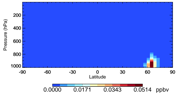
v11-02f-Run0 MACR - Species Curtain @ -180.000 for Jul
