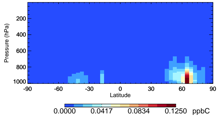
v11-02e-Run0 EOH - Species Curtain @ -180.000 for Jul
