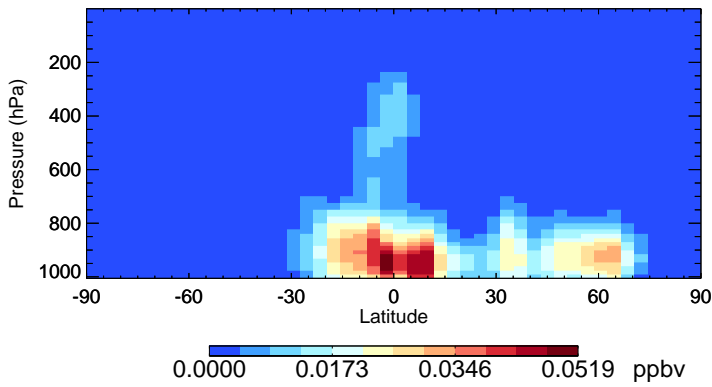
v11-02f-Run0 IEPOXA - Species Zonal Mean for Jul
