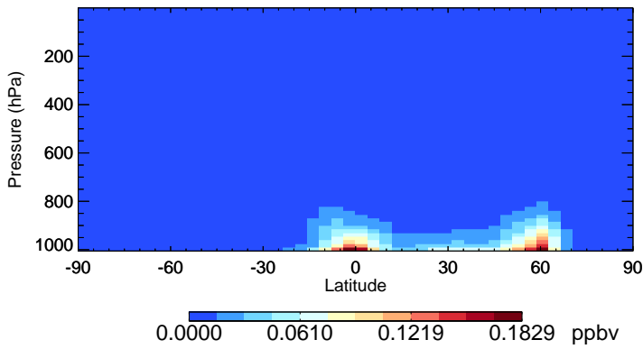
v11-02f-Run0 RCHO - Species Zonal Mean for Jul
