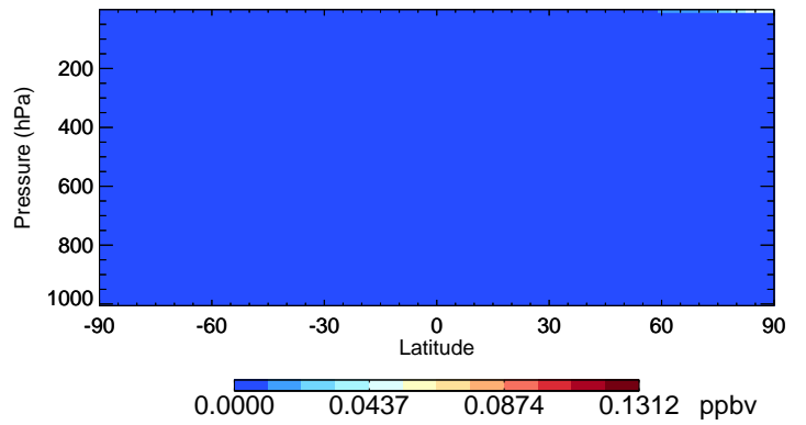
v11-02f-Run0 ACTA - Species Curtain @ -180.000 for Jul
