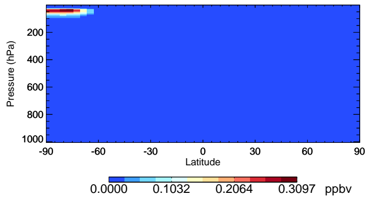
v11-02e-Run1 Cl2O2 - Species Curtain @ -180.000 for Jul
