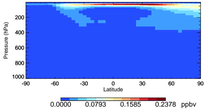
v11-02e-Run0 HNO4 - Species Curtain @ -180.000 for Jul
