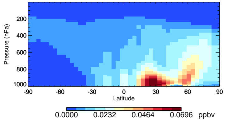
v11-02e-Run1 MAP - Species Curtain @ -180.000 for Jul
