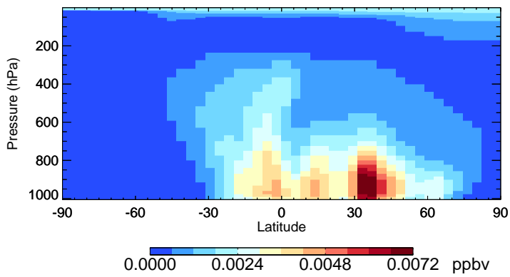
v11-02f-Run0 ISOG1 - Species Zonal Mean for Jul
