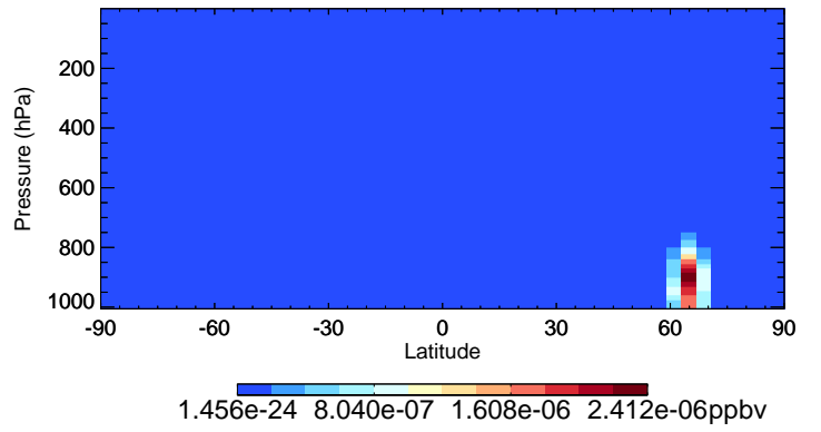
v11-02e-Run0 LVOC - Species Curtain @ -180.000 for Jul
