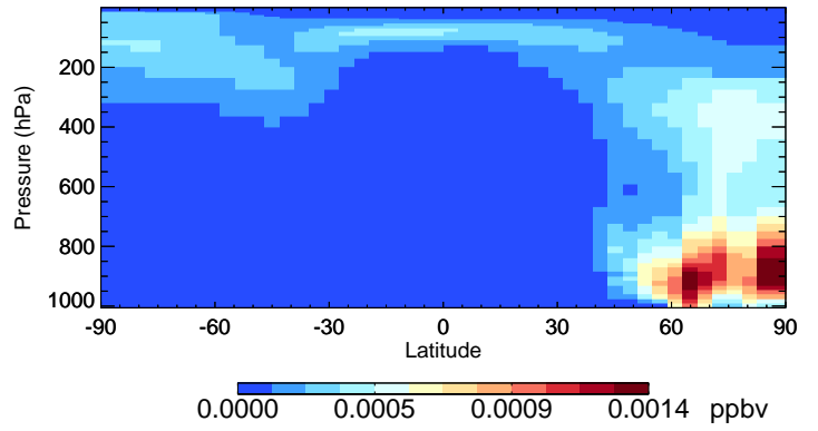
v11-02e-Run1 TSOA1 - Species Curtain @ -180.000 for Jul
