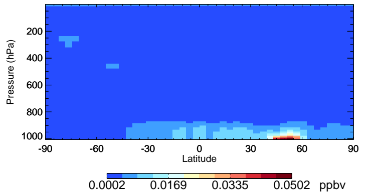
v11-02f-Run0 MSA - Species Curtain @ -180.000 for Jul
