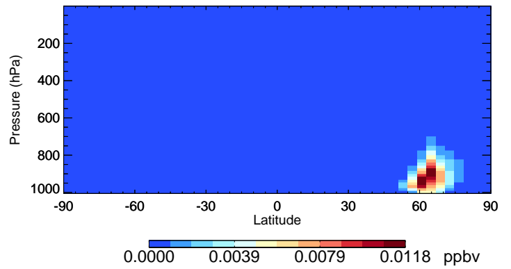
v11-02f-Run0 IEPOXB - Species Curtain @ -180.000 for Jul
