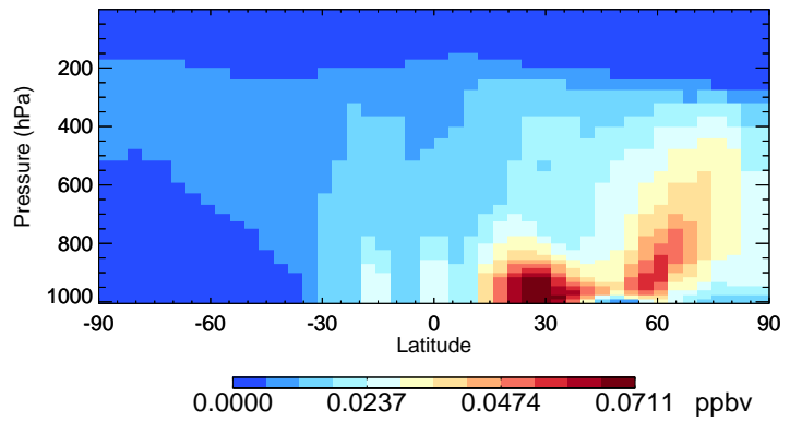
v11-02f-Run0 MAP - Species Curtain @ -180.000 for Jul
