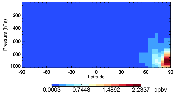
v11-02f-Run0 OCPI - Species Curtain @ -180.000 for Jul
