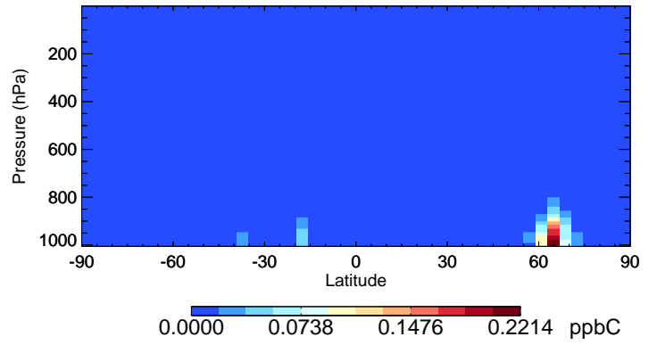
v11-02e-Run1 PRPE - Species Curtain @ -180.000 for Jul
