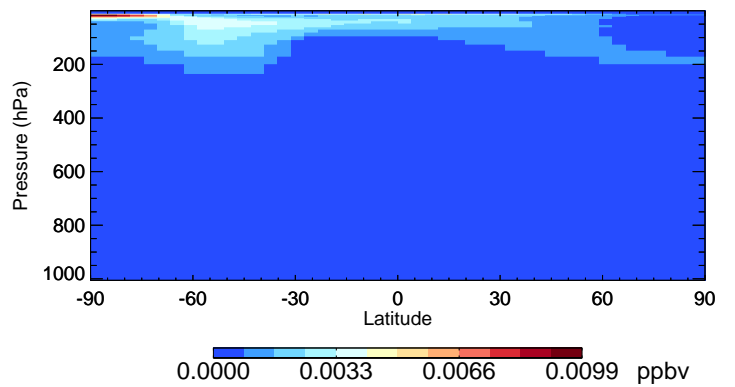
v11-02f-Run0 HOBr - Species Curtain @ -180.000 for Jul
