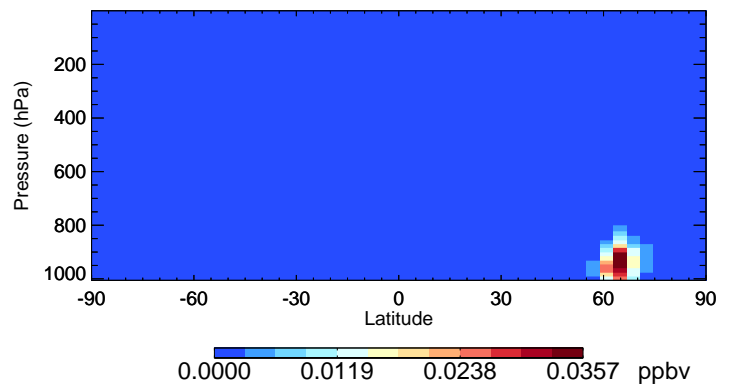
v11-02f-Run0 RIPA - Species Curtain @ -180.000 for Jul
