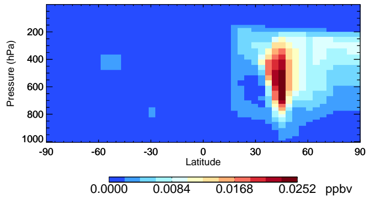
v11-02f-Run0 DST2 - Species Curtain @ -180.000 for Jul
