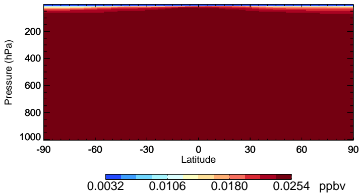
v11-02f-Run0 HCFC142b - Species Zonal Mean for Jul
