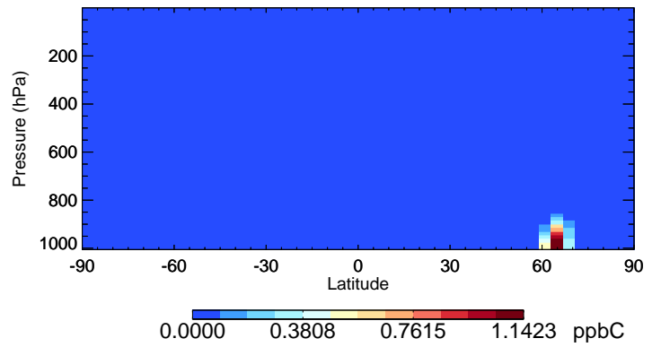
v11-02f-Run0 ISOP - Species Curtain @ -180.000 for Jul
