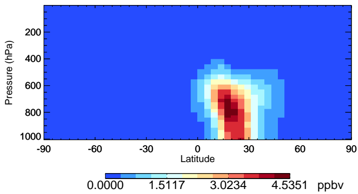
v11-02f-Run0 DST1 - Species Zonal Mean for Jul
