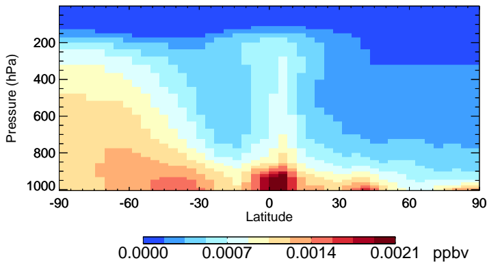
v11-02f-Run0 CHBr3 - Species Zonal Mean for Jul
