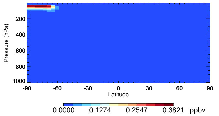
v11-02e-Run0 Cl2O2 - Species Curtain @ -180.000 for Jul
