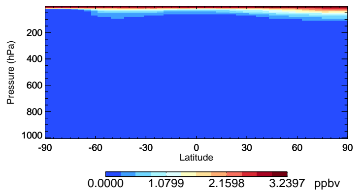
v11-02f-Run0 HCl - Species Curtain @ -180.000 for Jul
