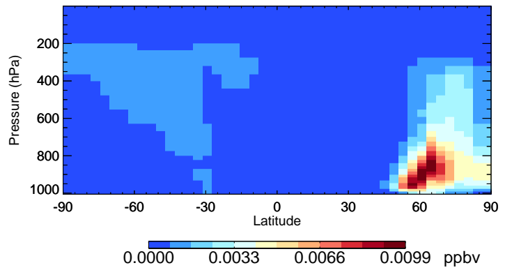
v11-02f-Run0 IMAE - Species Curtain @ -180.000 for Jul
