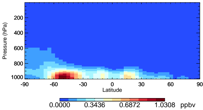
v11-02f-Run0 SALA - Species Zonal Mean for Jul
