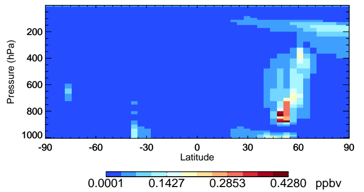
v11-02f-Run0 SO2 - Species Curtain @ -180.000 for Jul
