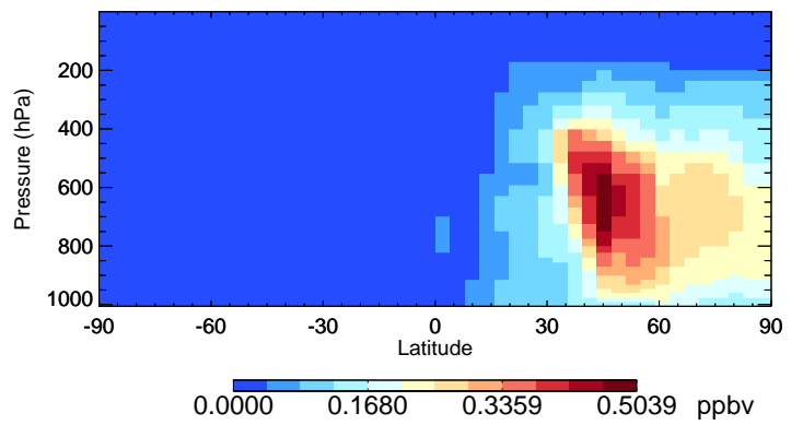
v11-02f-Run0 DST1 - Species Curtain @ -180.000 for Jul
