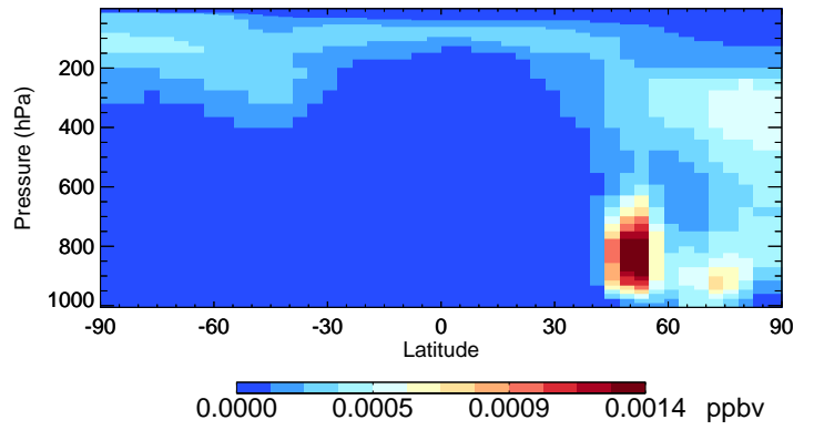
v11-02e-Run0 TSOA1 - Species Curtain @ -180.000 for Jul
