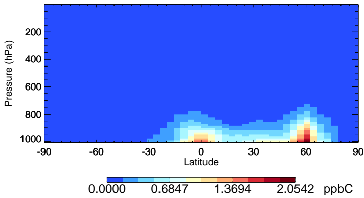
v11-02f-Run0 ALD2 - Species Zonal Mean for Jul
