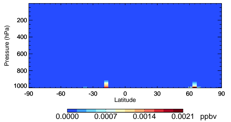
v11-02f-Run0 MTPO - Species Curtain @ -180.000 for Jul
