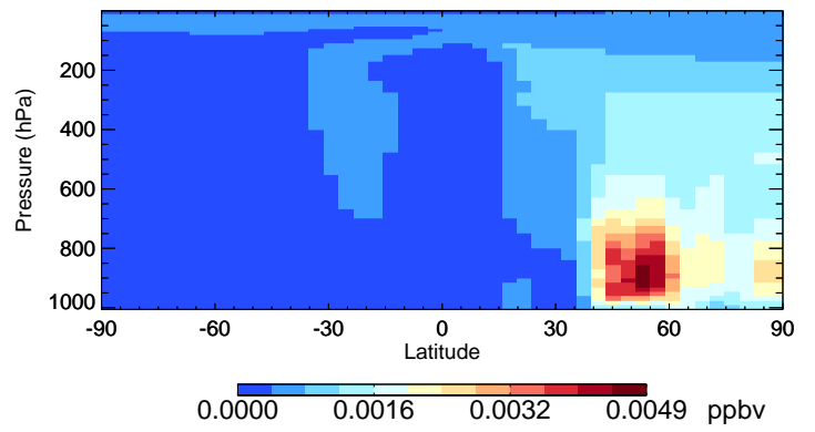
v11-02e-Run1 ASOAN - Species Curtain @ -180.000 for Jul
