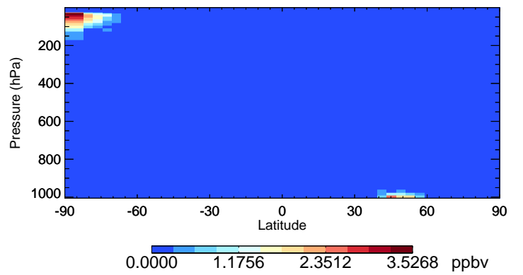
v11-02f-Run0 NIT - Species Curtain @ -180.000 for Jul
