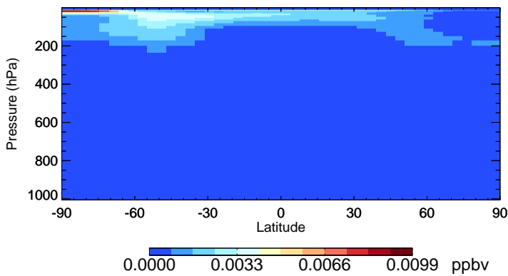
v11-02f-Run0 HOBr - Species Zonal Mean for Jul
