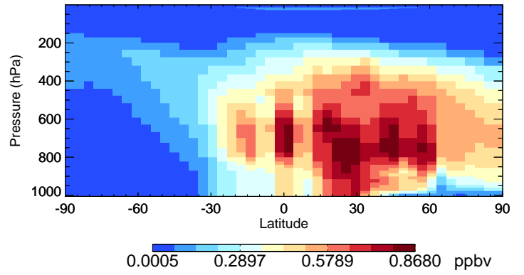
v11-02e-Run1 H2O2 - Species Curtain @ -180.000 for Jul
