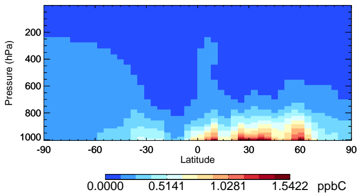
v11-02f-Run0 ALK4 - Species Zonal Mean for Jul
