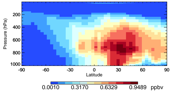
v11-02e-Run0 H2O2 - Species Curtain @ -180.000 for Jul
