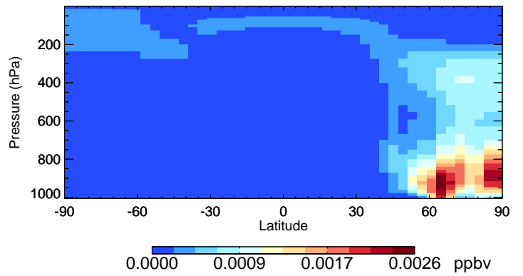
v11-02f-Run0 TSOA1 - Species Curtain @ -180.000 for Jul
