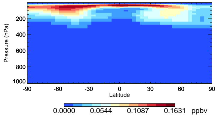
v11-02f-Run0 MPN - Species Curtain @ -180.000 for Jul
