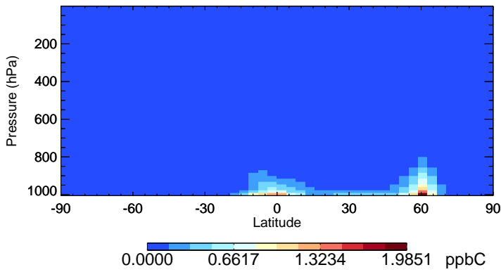
v11-02f-Run0 PRPE - Species Zonal Mean for Jul
