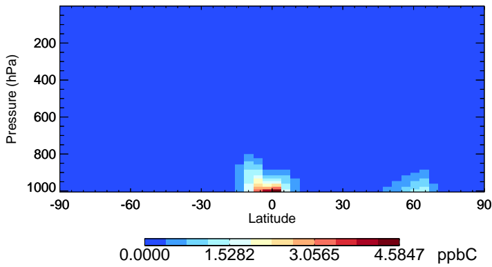
v11-02f-Run0 ISOP - Species Zonal Mean for Jul
