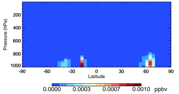
v11-02e-Run0 GLYX - Species Curtain @ -180.000 for Jul
