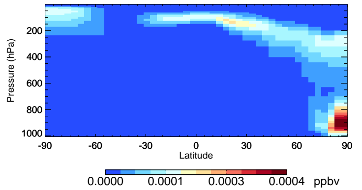
v11-02f-Run0 ASOA2 - Species Curtain @ -180.000 for Jul
