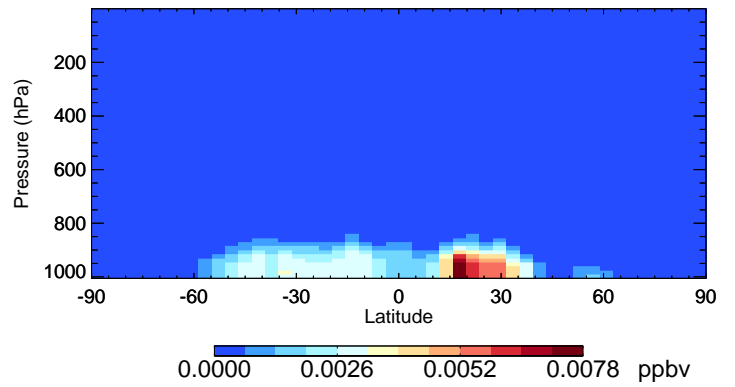
v11-02f-Run0 NITs - Species Curtain @ -180.000 for Jul
