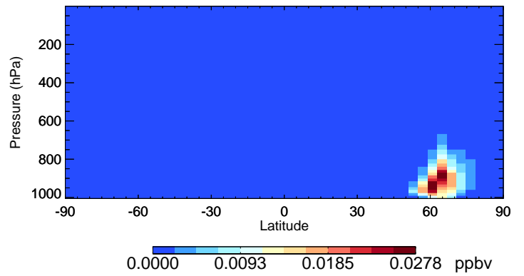
v11-02f-Run0 IEPOXA - Species Curtain @ -180.000 for Jul
