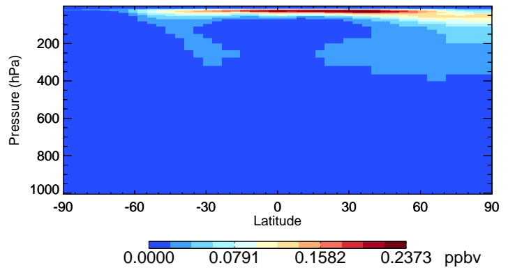
v11-02f-Run0 HNO4 - Species Curtain @ -180.000 for Jul
