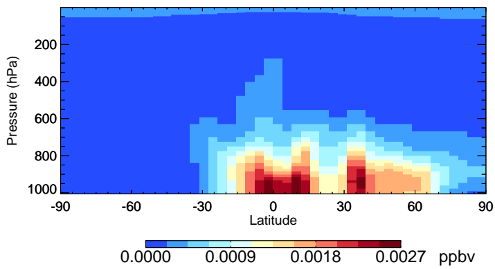
v11-02f-Run0 LVOCOA - Species Zonal Mean for Jul
