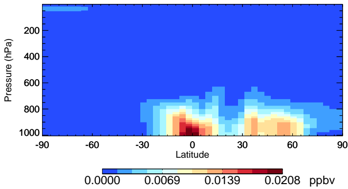
v11-02f-Run0 ISOA1 - Species Zonal Mean for Jul
