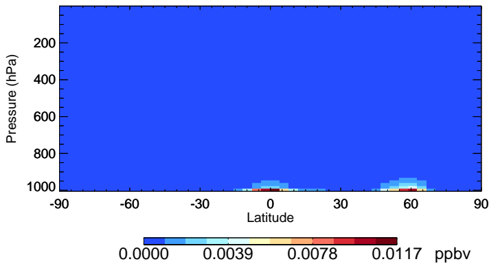
v11-02f-Run0 LIMO - Species Zonal Mean for Jul
