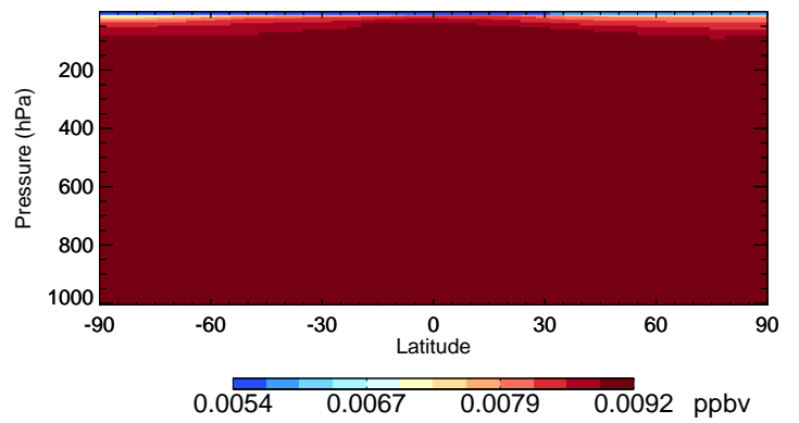
v11-02f-Run0 CFC115 - Species Curtain @ -180.000 for Jul
