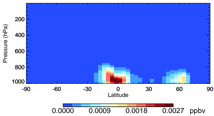
v11-02f-Run0 RIPD - Species Zonal Mean for Jul
