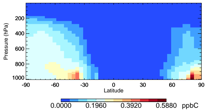
v11-02f-Run0 ALK4 - Species Curtain @ -180.000 for Jul
