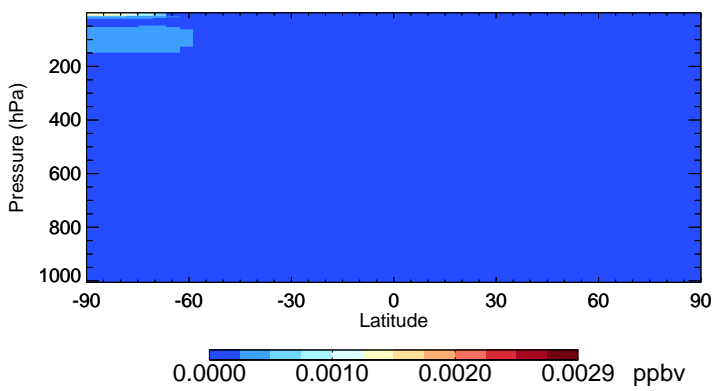
v11-02f-Run0 Br2 - Species Zonal Mean for Jul
