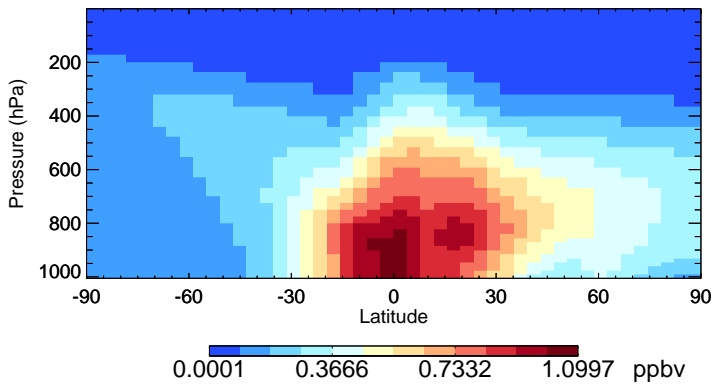
v11-02f-Run0 MP - Species Zonal Mean for Jul
