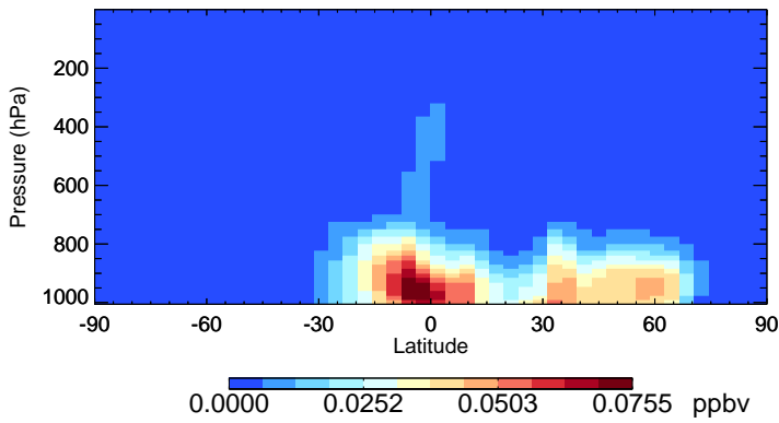
v11-02f-Run0 GLYC - Species Zonal Mean for Jul
