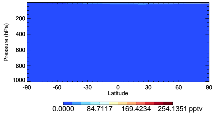
v11-02f-Run0 HO2 - Species Curtain @ -180.000 for Jul
