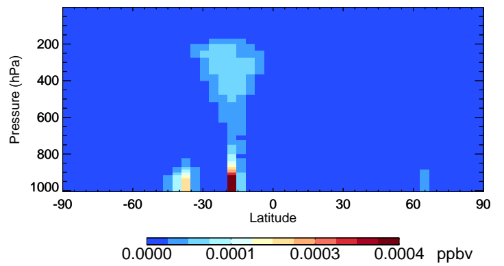
v11-02f-Run0 HONIT - Species Curtain @ -180.000 for Jul
