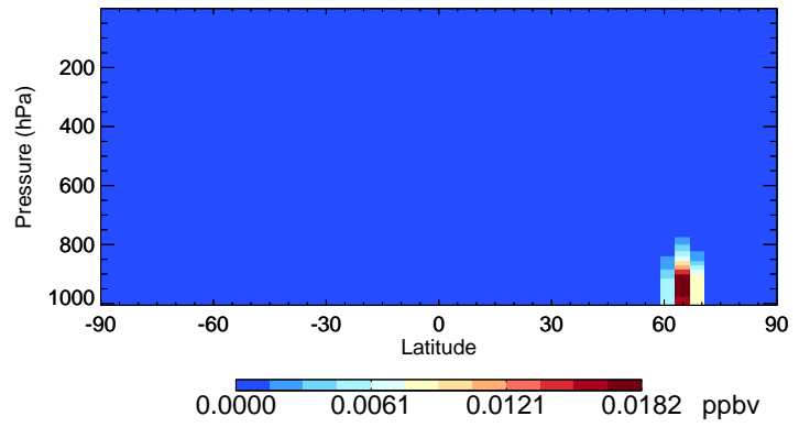
v11-02e-Run0 MACR - Species Curtain @ -180.000 for Jul
