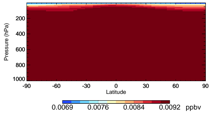
v11-02e-Run1 CFC115 - Species Curtain @ -180.000 for Jul
