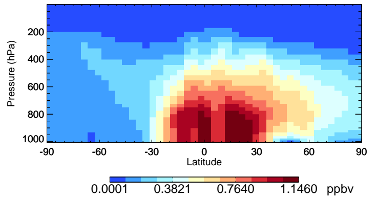
v11-02f-Run0 MP - Species Curtain @ -180.000 for Jul
