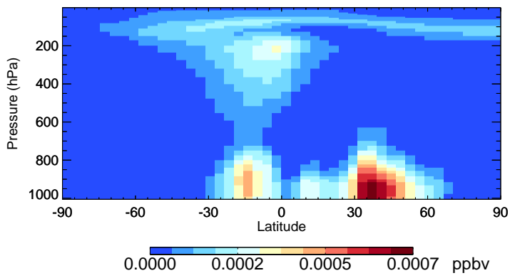
v11-02f-Run0 DHDN - Species Zonal Mean for Jul
