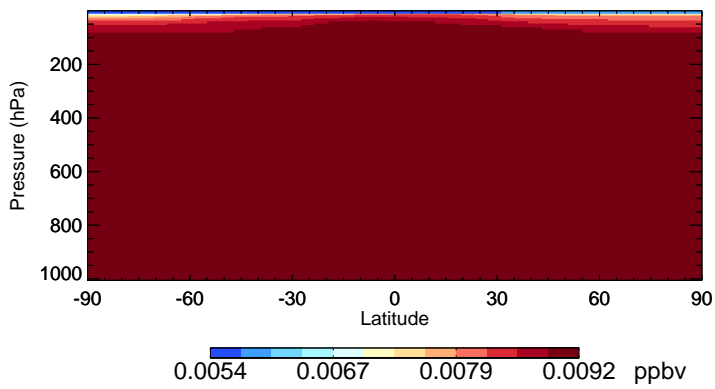
v11-02f-Run0 CFC115 - Species Zonal Mean for Jul
