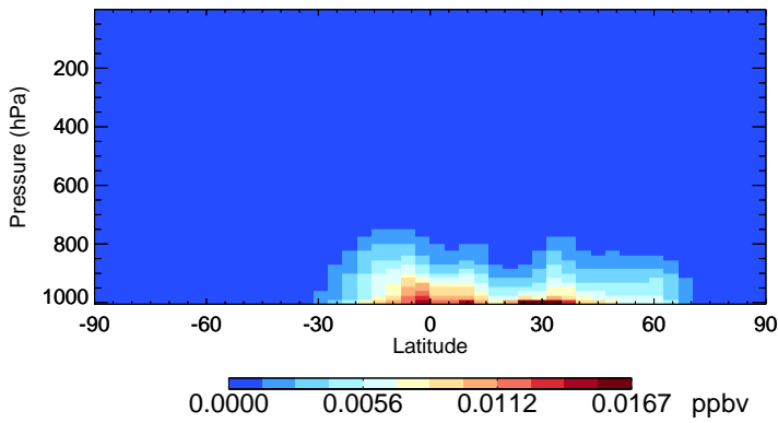
v11-02f-Run0 GLYX - Species Zonal Mean for Jul
