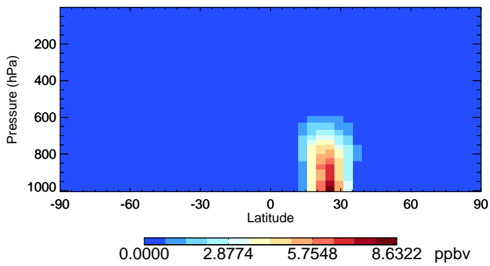
v11-02f-Run0 DST4 - Species Zonal Mean for Jul
