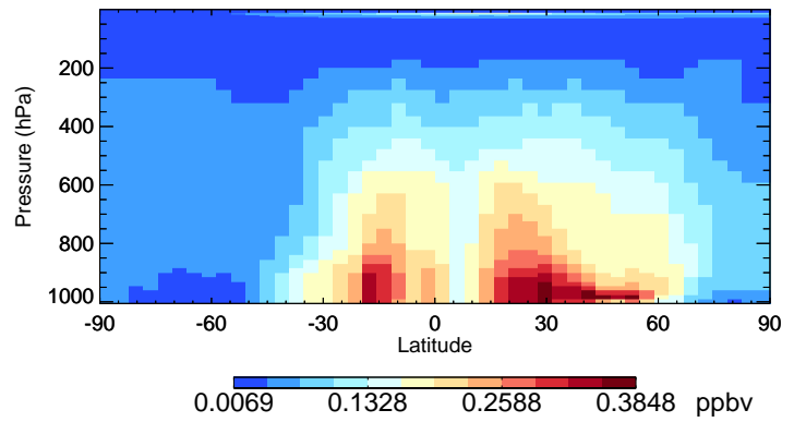
v11-02f-Run0 CH2O - Species Curtain @ -180.000 for Jul
