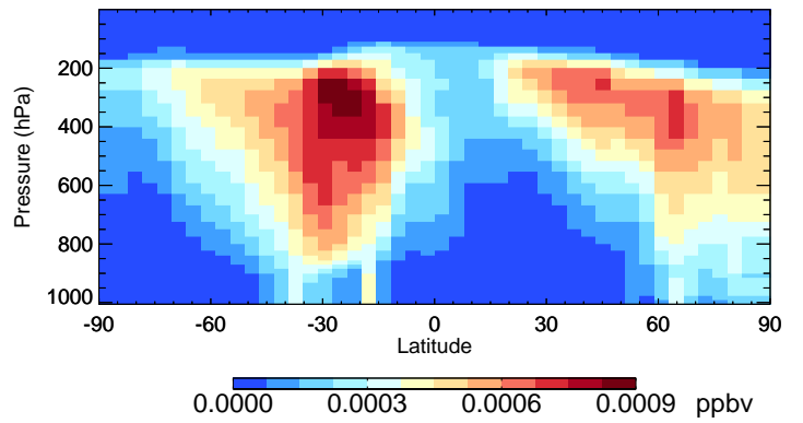
v11-02f-Run0 R4N2 - Species Curtain @ -180.000 for Jul
