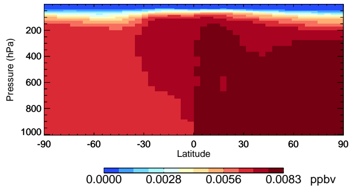
v11-02f-Run0 CH3Br - Species Curtain @ -180.000 for Jul
