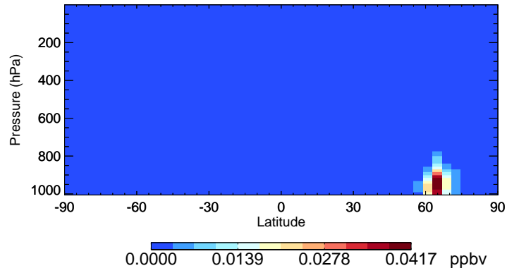
v11-02e-Run1 MACR - Species Curtain @ -180.000 for Jul
