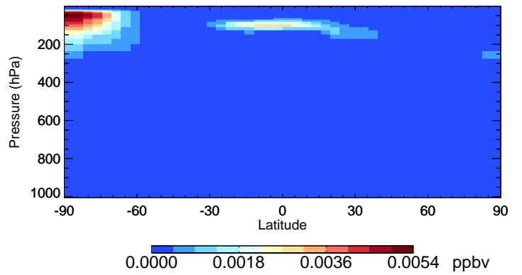
v11-02f-Run0 ISOA3 - Species Curtain @ -180.000 for Jul
