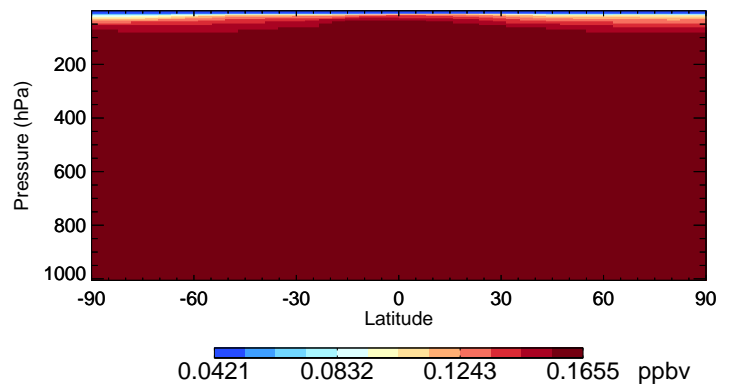
v11-02f-Run0 HCFC22 - Species Curtain @ -180.000 for Jul
