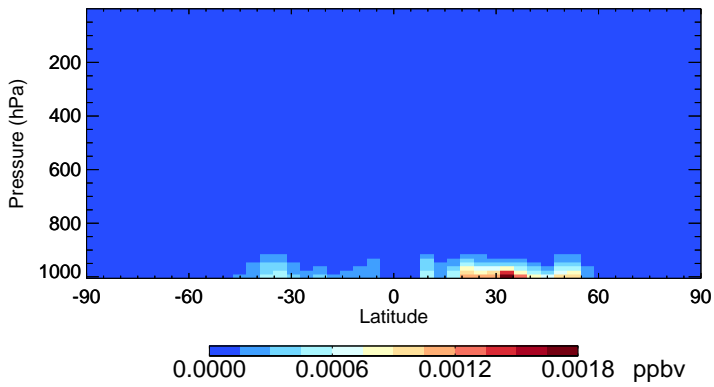
v11-02f-Run0 ClNO 2 - Species Zonal Mean for Jul
