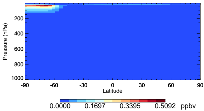
v11-02f-Run0 HOCl - Species Zonal Mean for Jul
