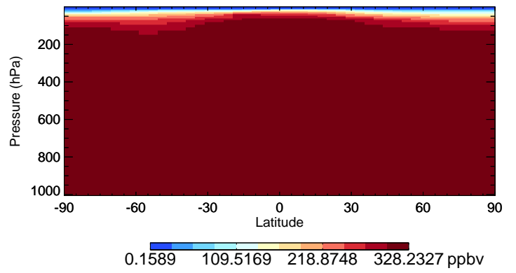
v11-02e-Run1 N2O - Species Curtain @ -180.000 for Jul
