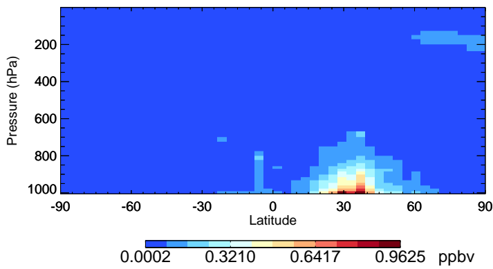
v11-02f-Run0 SO2 - Species Zonal Mean for Jul
