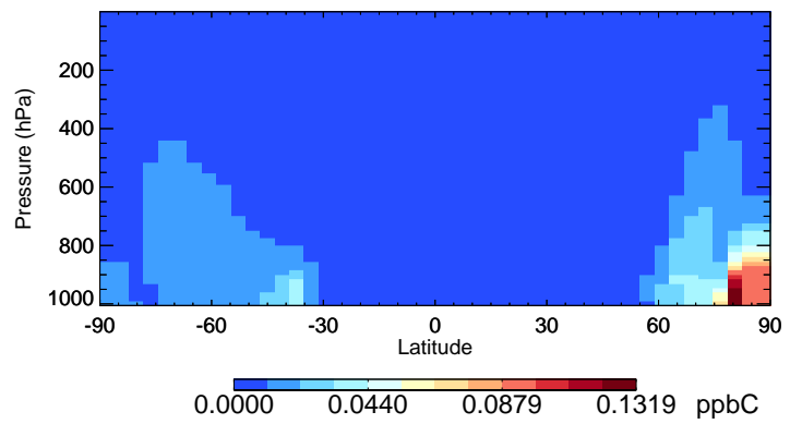
v11-02f-Run0 TOLU - Species Curtain @ -180.000 for Jul
