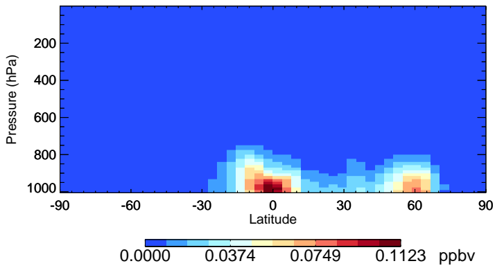
v11-02f-Run0 MACR - Species Zonal Mean for Jul
