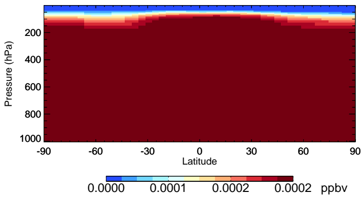
v11-02f-Run0 H2402 - Species Zonal Mean for Jul
