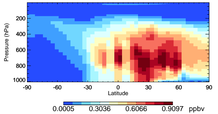
v11-02f-Run0 H2O2 - Species Curtain @ -180.000 for Jul
