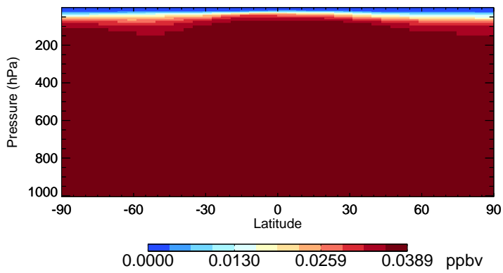
v11-02f-Run0 HCFC141b - Species Zonal Mean for Jul
