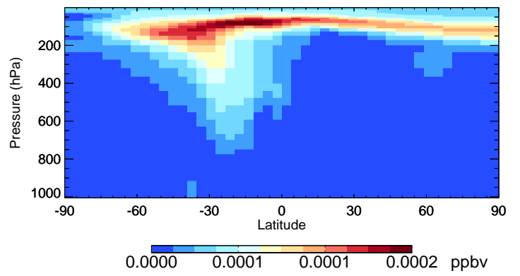
v11-02f-Run0 DHDN - Species Curtain @ -180.000 for Jul
