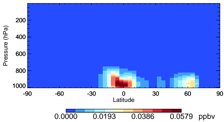
v11-02f-Run0 RIPA - Species Zonal Mean for Jul
