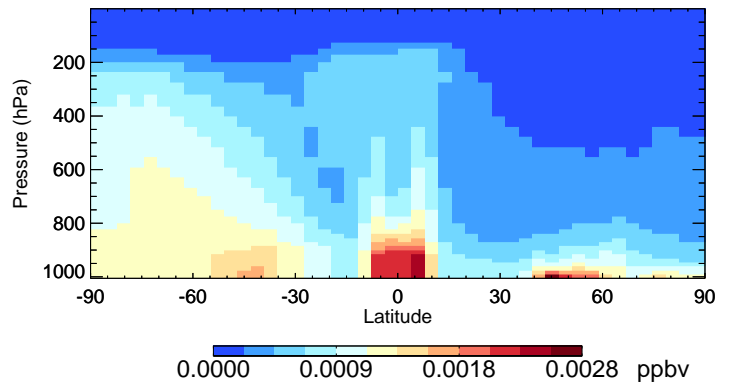
v11-02f-Run0 CHBr3 - Species Curtain @ -180.000 for Jul
