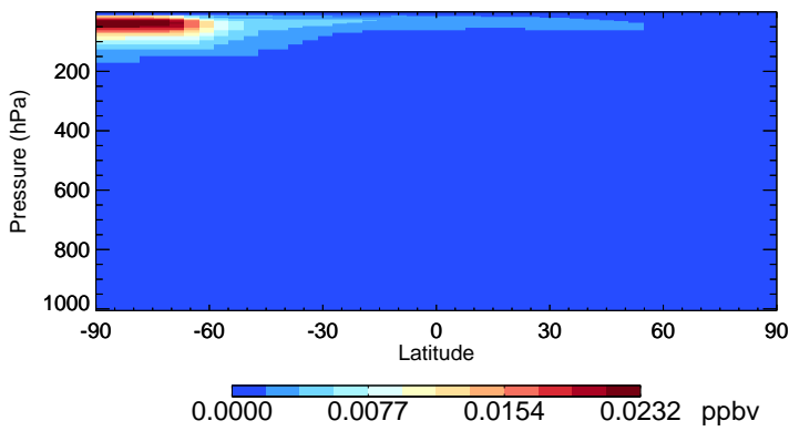
v11-02f-Run0 BrCl - Species Zonal Mean for Jul
