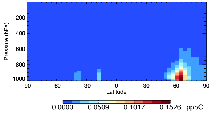
v11-02e-Run1 EOH - Species Curtain @ -180.000 for Jul
