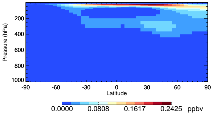
v11-02f-Run0 HNO4 - Species Zonal Mean for Jul
