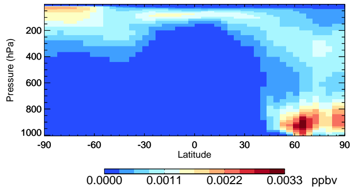
v11-02f-Run0 ISOA1 - Species Curtain @ -180.000 for Jul
