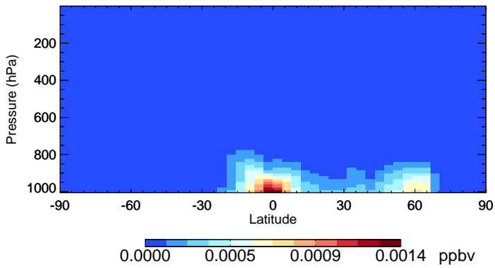
v11-02f-Run0 MOBA - Species Zonal Mean for Jul
