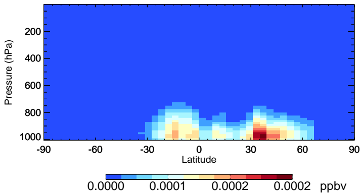
v11-02f-Run0 ETHLN - Species Zonal Mean for Jul
