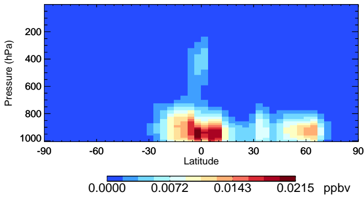
v11-02f-Run0 IEPOXB - Species Zonal Mean for Jul
