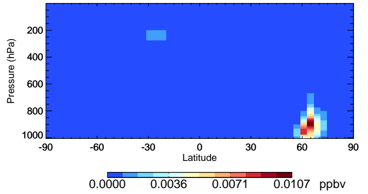
v11-02e-Run1 IEPOXA - Species Curtain @ -180.000 for Jul
