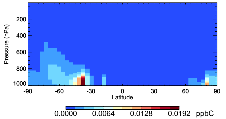
v11-02f-Run0 XYLE - Species Curtain @ -180.000 for Jul
