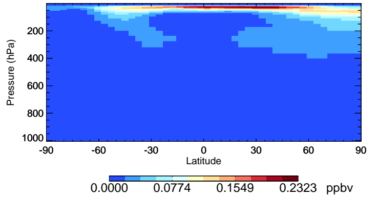
v11-02e-Run1 HNO4 - Species Curtain @ -180.000 for Jul
