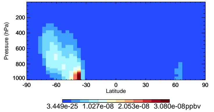
v11-02e-Run1 NPMN - Species Curtain @ -180.000 for Jul
