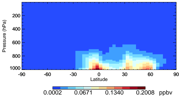
v11-02f-Run0 TSOG3 - Species Zonal Mean for Jul
