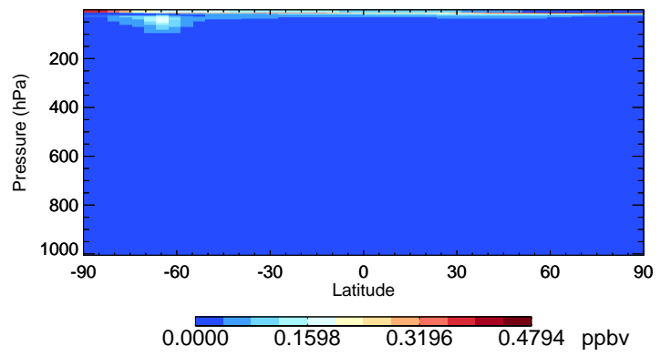
v11-02f-Run0 CIO - Species Curtain @ -180.000 for Jul
