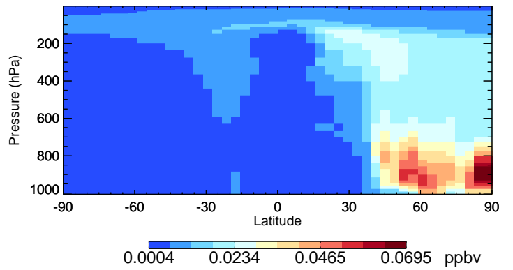
v11-02f-Run0 SOAS - Species Curtain @ -180.000 for Jul
