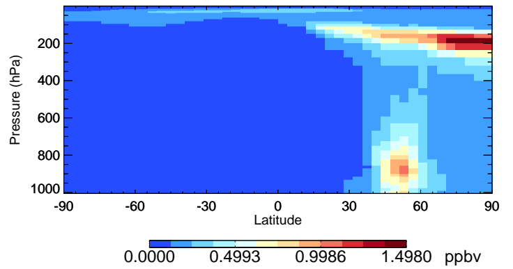
v11-02f-Run0 SO4 - Species Curtain @ -180.000 for Jul
