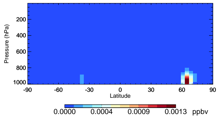
v11-02f-Run0 ISOPNB - Species Curtain @ -180.000 for Jul
