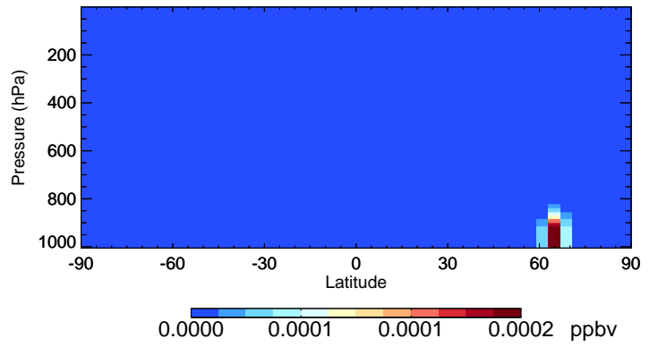
v11-02e-Run0 MOBA - Species Curtain @ -180.000 for Jul
