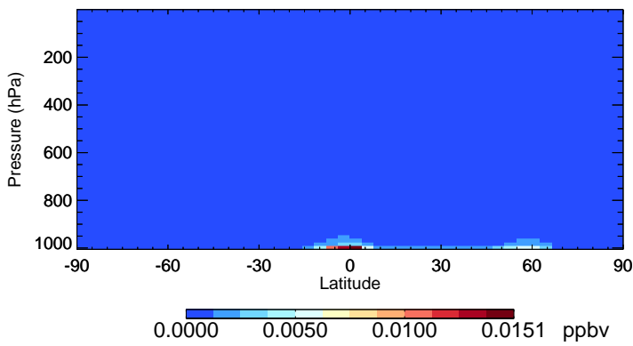
v11-02f-Run0 MTPO - Species Zonal Mean for Jul
