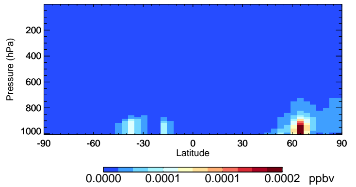
v11-02f-Run0 IONITA - Species Curtain @ -180.000 for Jul
