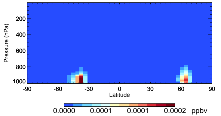
v11-02f-Run0 ISN1 - Species Curtain @ -180.000 for Jul
