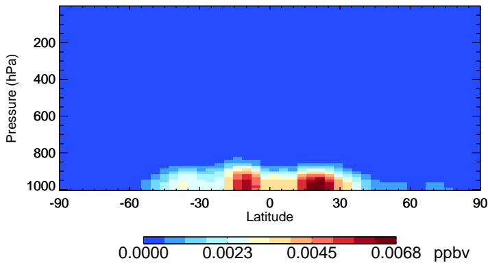
v11-02f-Run0 NITs - Species Zonal Mean for Jul
