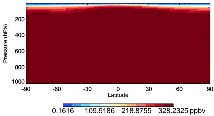
v11-02f-Run0 N2O - Species Zonal Mean for Jul
