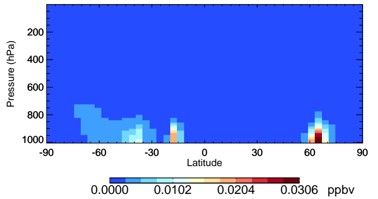
v11-02f-Run0 RCHO - Species Curtain @ -180.000 for Jul
