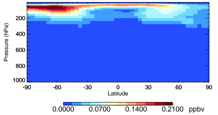
v11-02e-Run0 MPN - Species Curtain @ -180.000 for Jul
