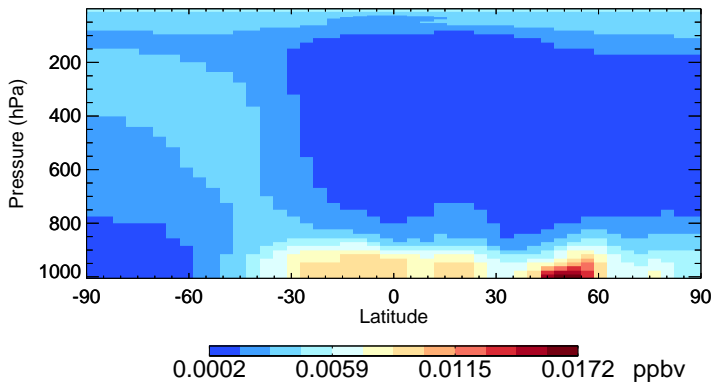
v11-02f-Run0 MSA - Species Zonal Mean for Jul
