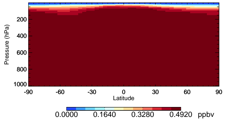
v11-02f-Run0 CFC12 - Species Curtain @ -180.000 for Jul
