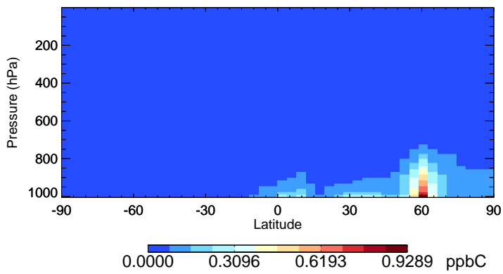
v11-02f-Run0 TOLU - Species Zonal Mean for Jul
