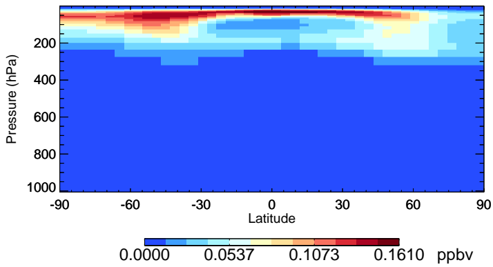
v11-02f-Run0 MPN - Species Zonal Mean for Jul
