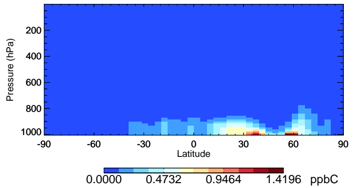
v11-02f-Run0 ALD2 - Species Curtain @ -180.000 for Jul
