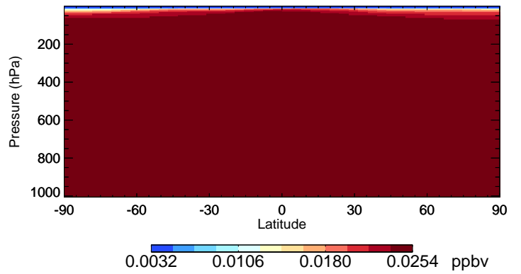
v11-02f-Run0 HCFC142b - Species Curtain @ -180.000 for Jul
