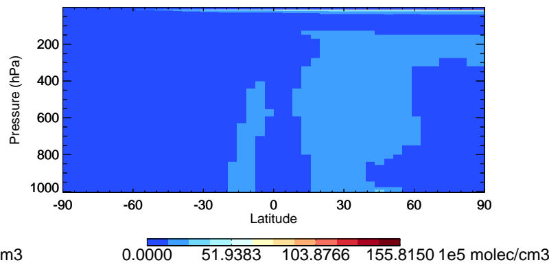
v11-02f-Run0 OH - Species Curtain @ -180.000 for Jul
