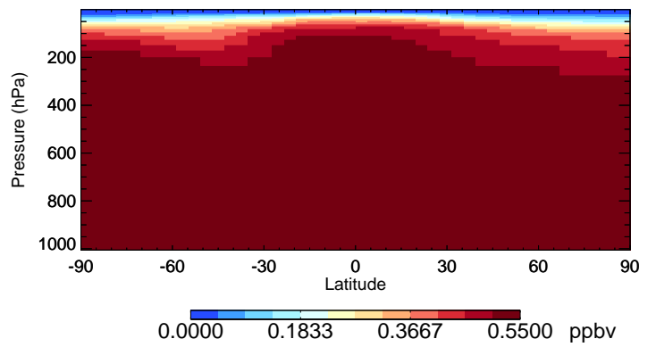
v11-02f-Run0 CH3Cl - Species Curtain @ -180.000 for Jul
