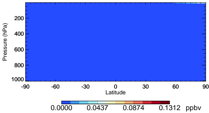
v11-02f-Run0 ACTA - Species Zonal Mean for Jul
