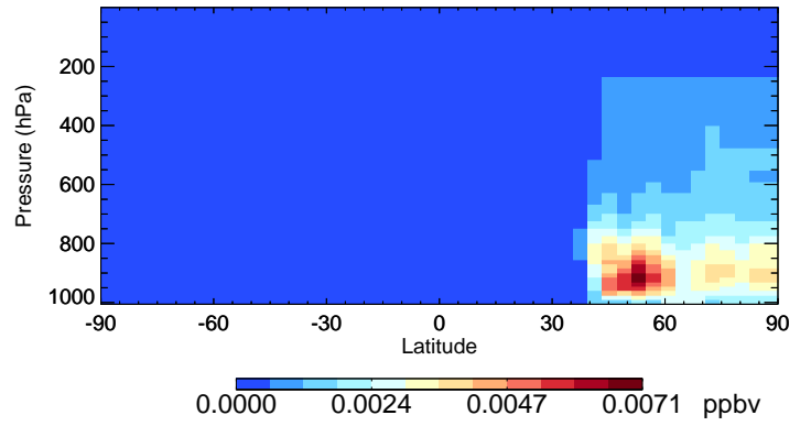
v11-02e-Run1 SOAME - Species Curtain @ -180.000 for Jul
