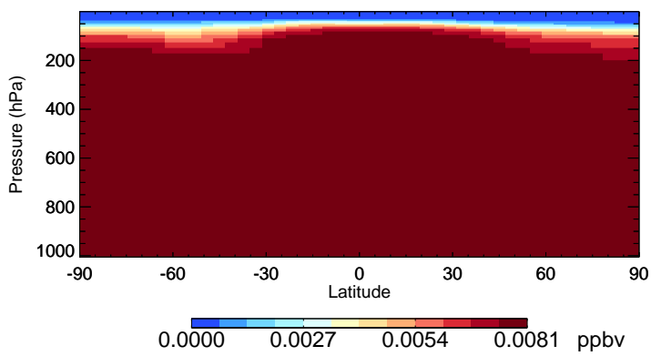
v11-02f-Run0 CH3CCI3 - Species Zonal Mean for Jul
