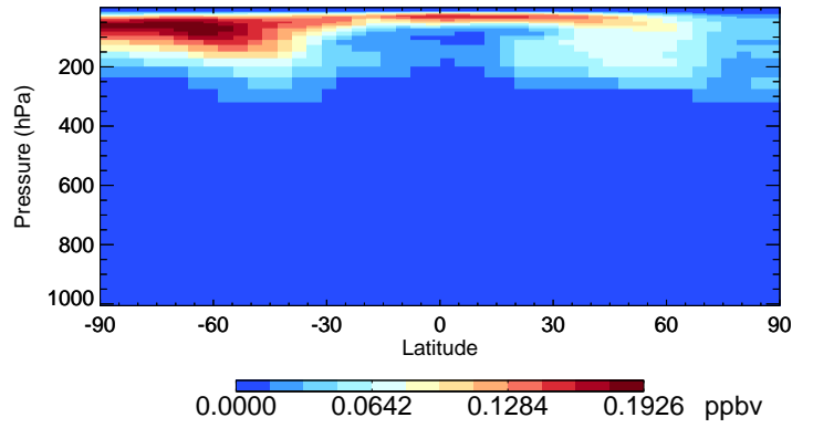
v11-02e-Run1 MPN - Species Curtain @ -180.000 for Jul
