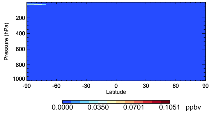
v11-02e-Run0 ClNO 2 - Species Curtain @ -180.000 for Jul
