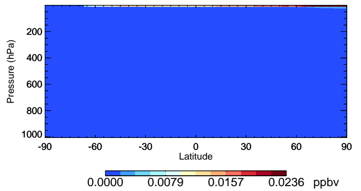
v11-02f-Run0 Br - Species Curtain @ -180.000 for Jul
