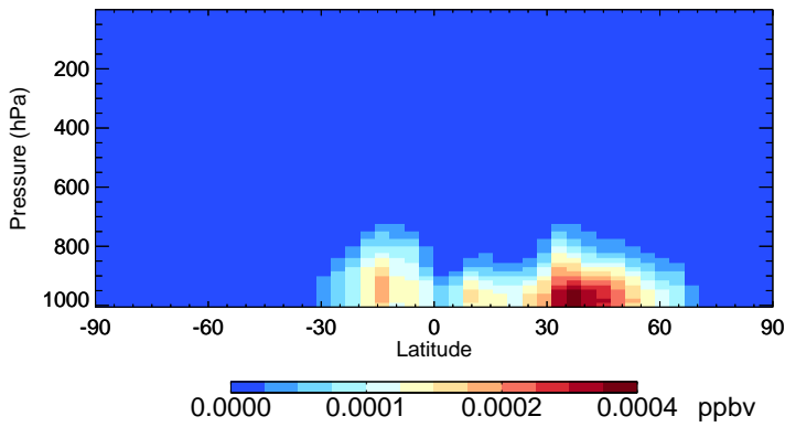
v11-02f-Run0 MACRN - Species Zonal Mean for Jul
