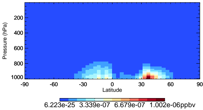
v11-02f-Run0 NPMN - Species Zonal Mean for Jul
