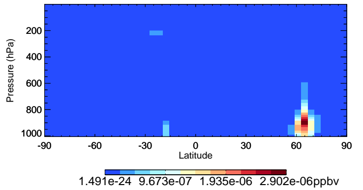
v11-02f-Run0 LVOC - Species Curtain @ -180.000 for Jul
