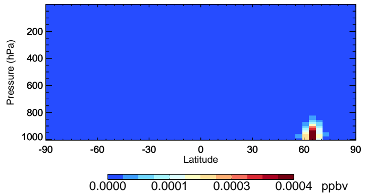
v11-02f-Run0 MOBA - Species Curtain @ -180.000 for Jul
