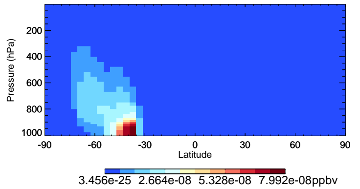
v11-02f-Run0 NPMN - Species Curtain @ -180.000 for Jul
