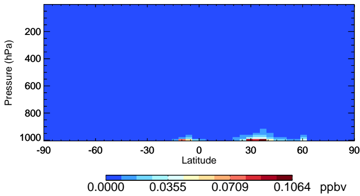
v11-02f-Run0 HNO 2 - Species Zonal Mean for Jul
