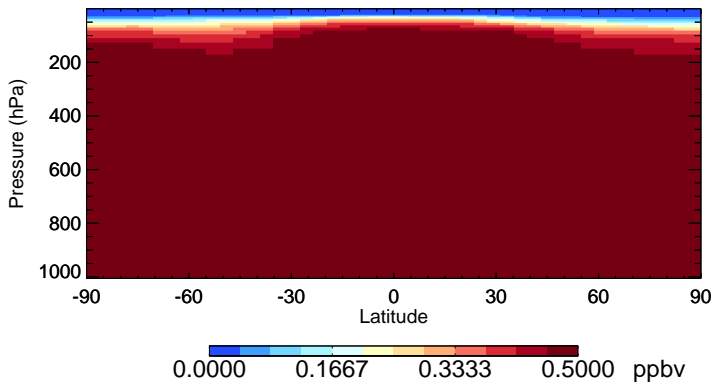
v11-02f-Run0 OCS - Species Zonal Mean for Jul
