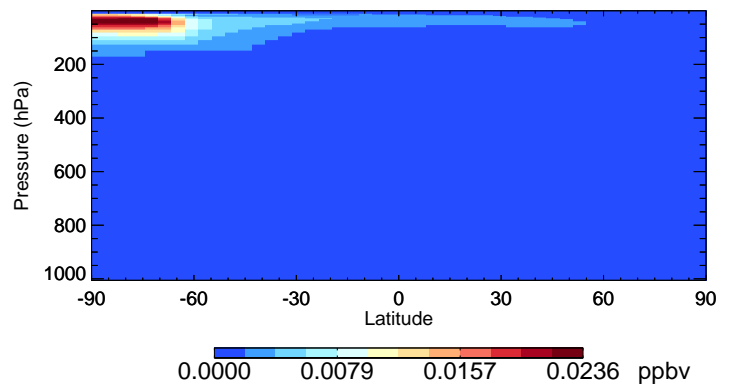
v11-02f-Run0 BrCl - Species Curtain @ -180.000 for Jul
