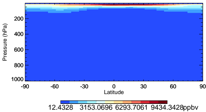
v11-02f-Run0 O3 - Species Zonal Mean for Jul
