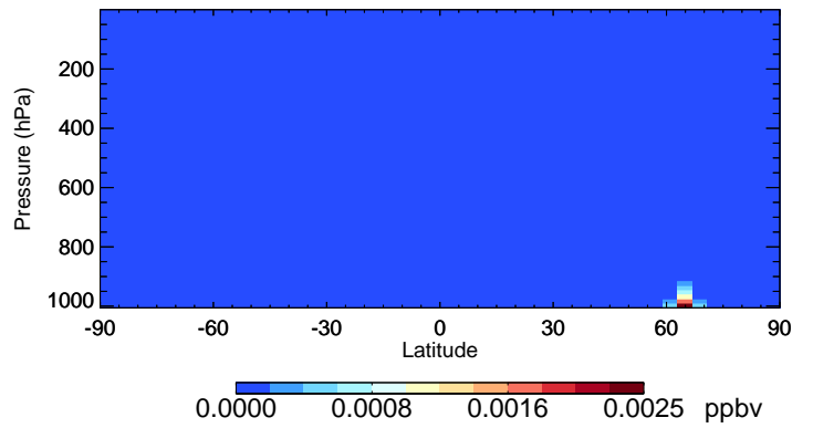
v11-02f-Run0 LIMO - Species Curtain @ -180.000 for Jul
