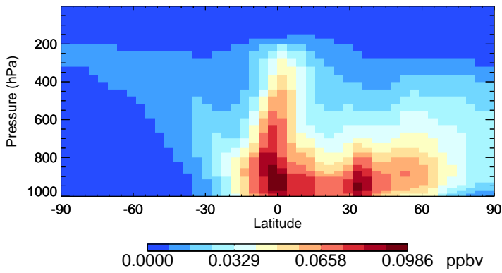
v11-02f-Run0 MAP - Species Zonal Mean for Jul
