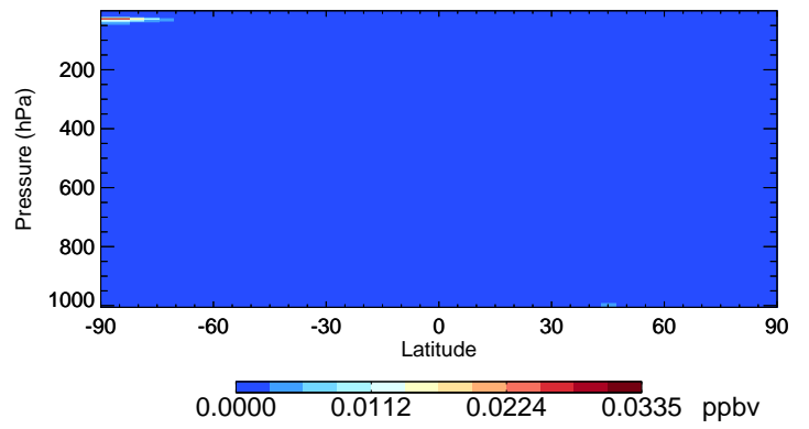
v11-02e-Run1 ClNO 2 - Species Curtain @ -180.000 for Jul
