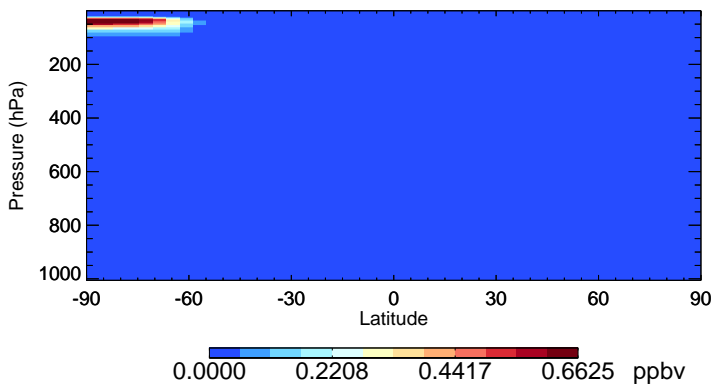
v11-02f-Run0 Cl2O2 - Species Zonal Mean for Jul
