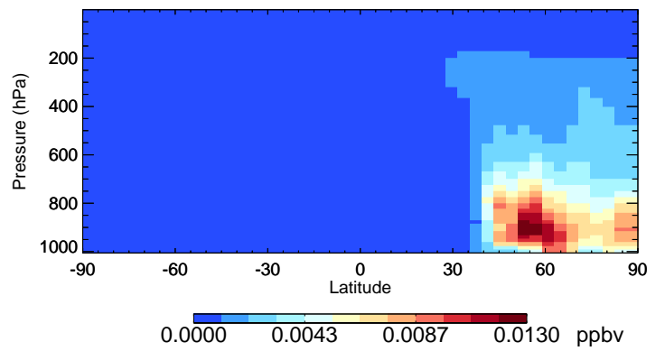
v11-02f-Run0 SOAGX - Species Curtain @ -180.000 for Jul
