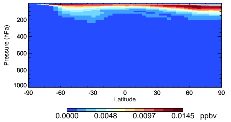
v11-02e-Run1 BrNO3 - Species Curtain @ -180.000 for Jul
