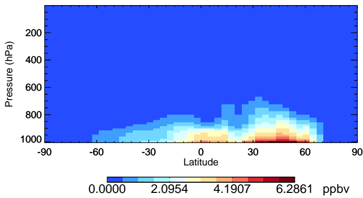
v11-02f-Run0 NH3 - Species Zonal Mean for Jul
