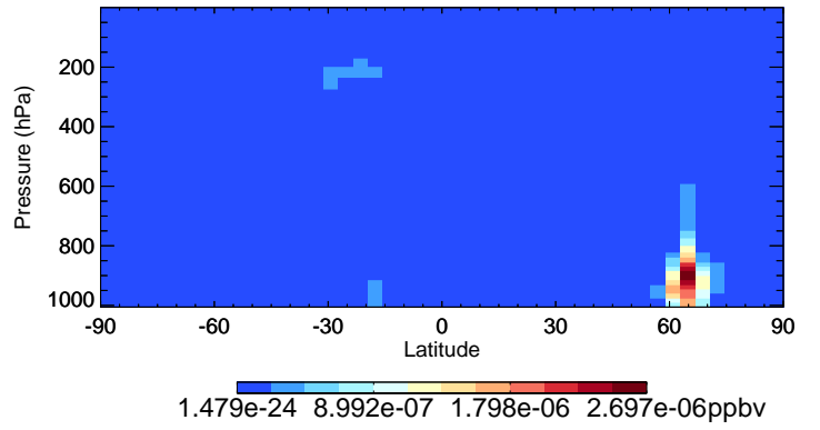
v11-02e-Run1 LVOC - Species Curtain @ -180.000 for Jul
