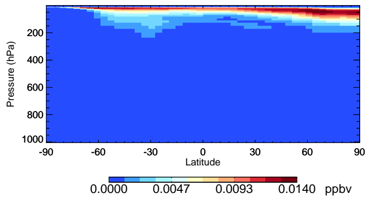
v11-02f-Run0 BrNO3 - Species Curtain @ -180.000 for Jul
