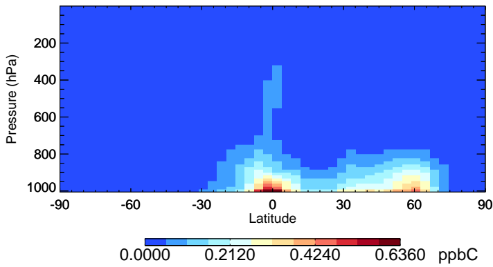
v11-02f-Run0 EOH - Species Zonal Mean for Jul
