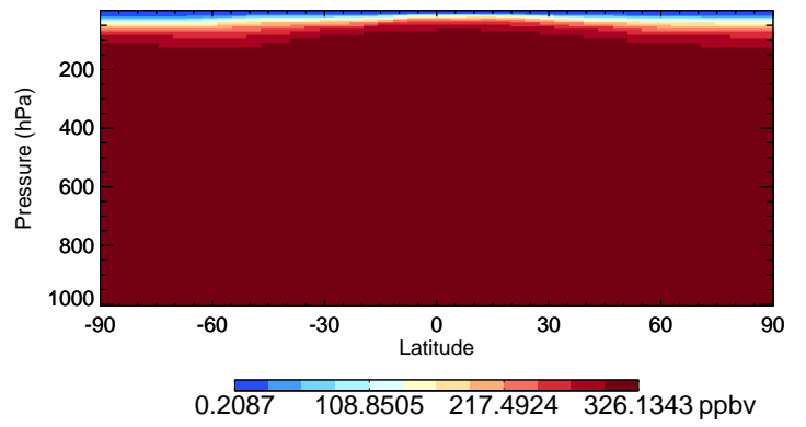
v11-02e-Run0 N2O - Species Curtain @ -180.000 for Jul
