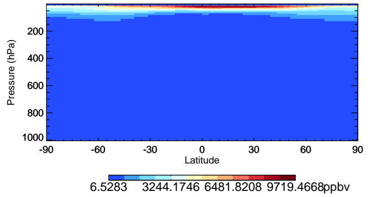
v11-02e-Run0 O3 - Species Curtain @ -180.000 for Jul
