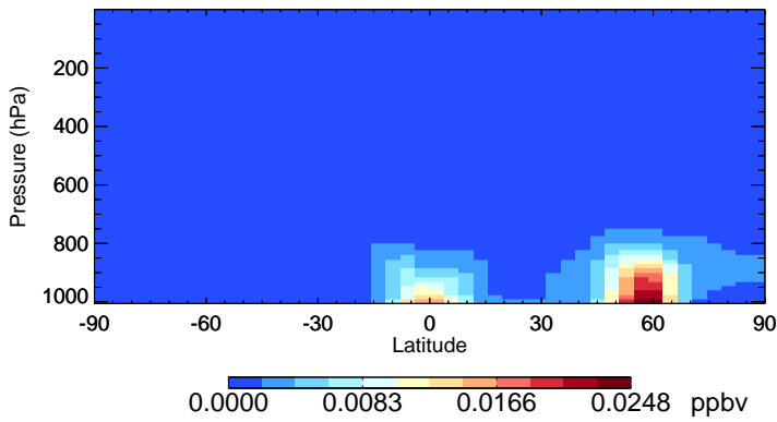
v11-02f-Run0 TSOA1 - Species Zonal Mean for Jul
