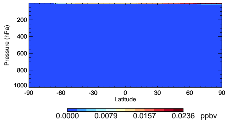
v11-02e-Run0 Br - Species Curtain @ -180.000 for Jul
