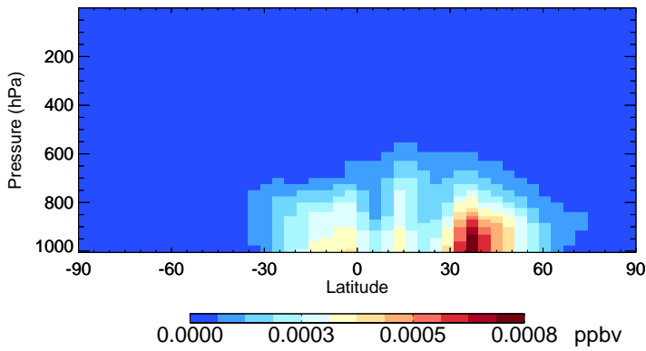
v11-02f-Run0 ISN10A - Species Zonal Mean for Jul
