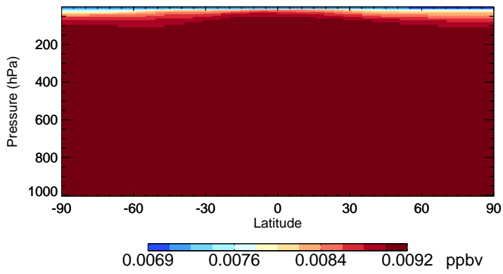
v11-02e-Run1 CFC115 - Species Zonal Mean for Jul
