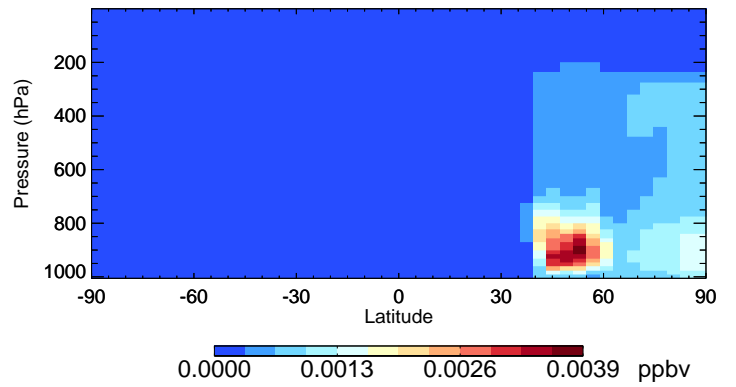
v11-02f-Run0 SOAME - Species Curtain @ -180.000 for Jul
