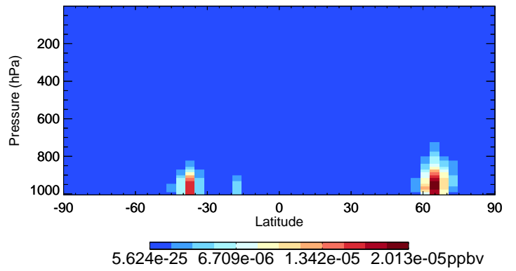
v11-02f-Run0 MACRN - Species Curtain @ -180.000 for Jul
