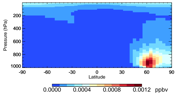
v11-02f-Run0 LVOCOA - Species Curtain @ -180.000 for Jul
