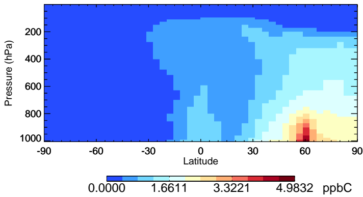
v11-02f-Run0 C2H6 - Species Zonal Mean for Jul
