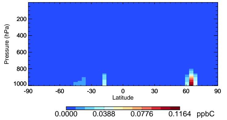
v11-02e-Run0 PRPE - Species Curtain @ -180.000 for Jul
