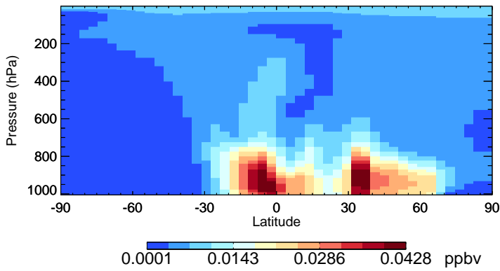
v11-02f-Run0 ISO3 - Species Zonal Mean for Jul
