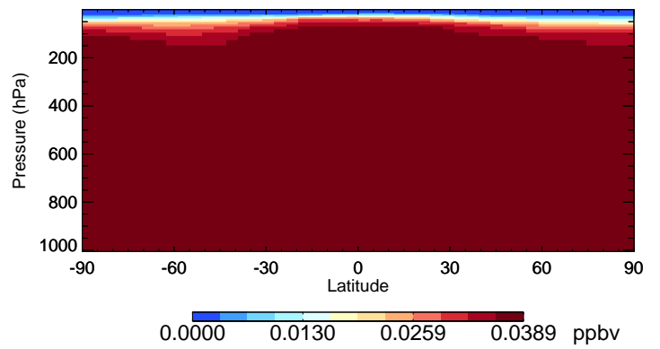
v11-02f-Run0 HCFC141b - Species Curtain @ -180.000 for Jul
