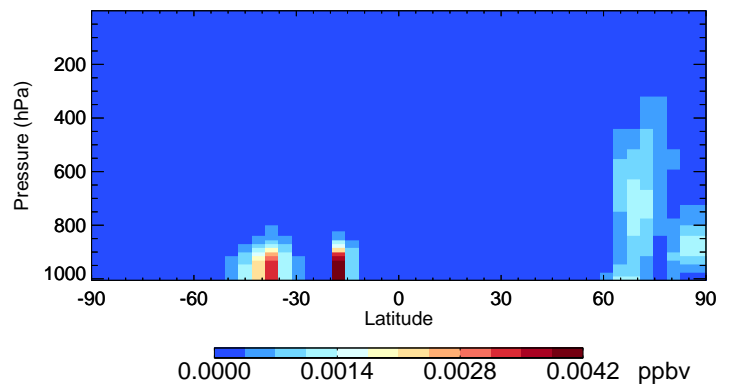
v11-02f-Run0 BCPO - Species Curtain @ -180.000 for Jul
