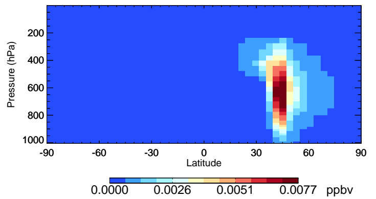
v11-02f-Run0 DST4 - Species Curtain @ -180.000 for Jul
