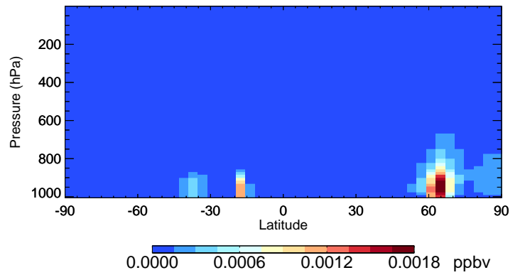
v11-02f-Run0 GLYX - Species Curtain @ -180.000 for Jul
