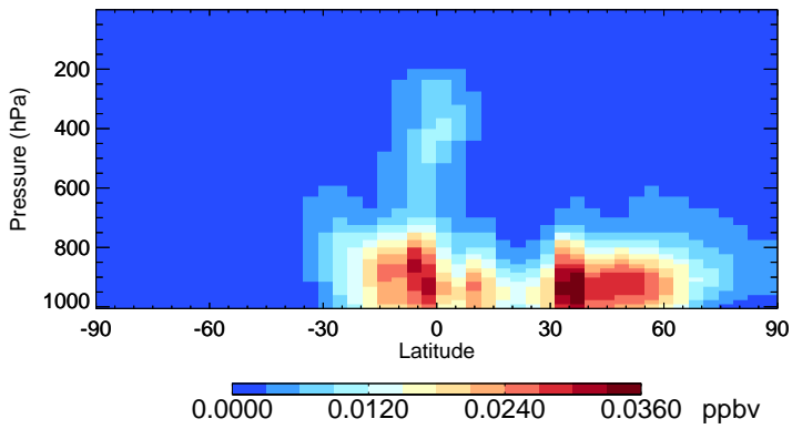
v11-02f-Run0 IMAE - Species Zonal Mean for Jul
