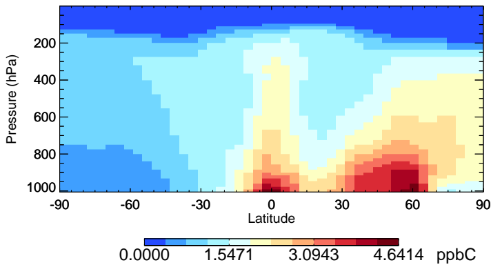
v11-02f-Run0 ACET - Species Zonal Mean for Jul
