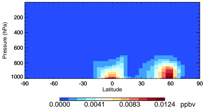
v11-02e-Run0 TSOA1 - Species Zonal Mean for Jul
