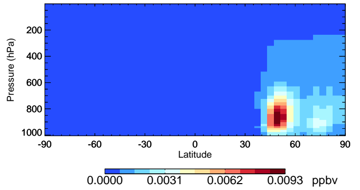
v11-02e-Run0 SOAME - Species Curtain @ -180.000 for Jul
