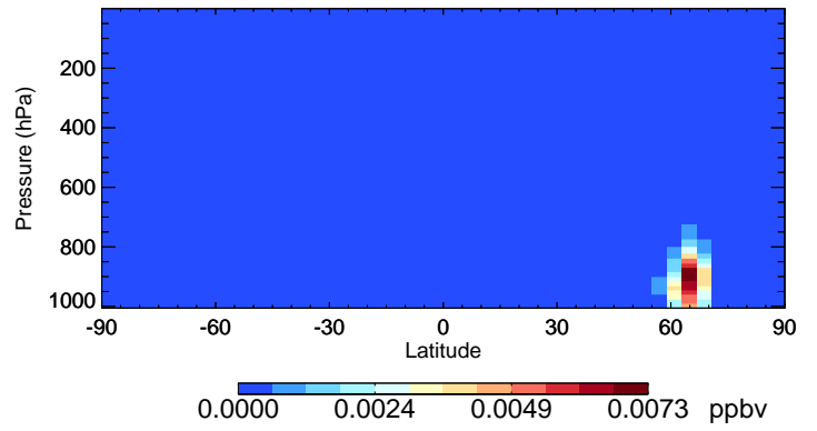
v11-02e-Run0 IEPOXA - Species Curtain @ -180.000 for Jul
