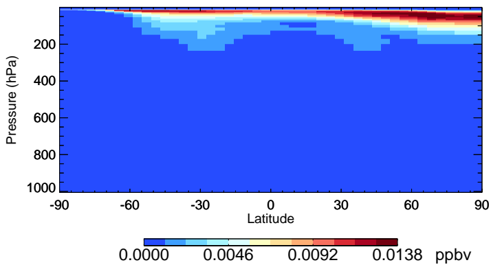
v11-02f-Run0 BrNO3 - Species Zonal Mean for Jul
