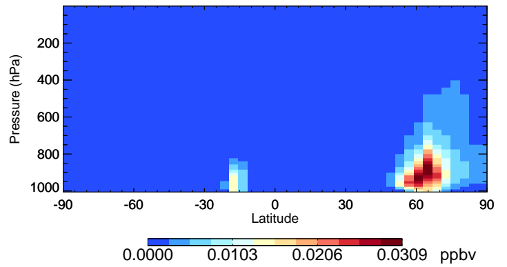
v11-02f-Run0 HAC - Species Curtain @ -180.000 for Jul
