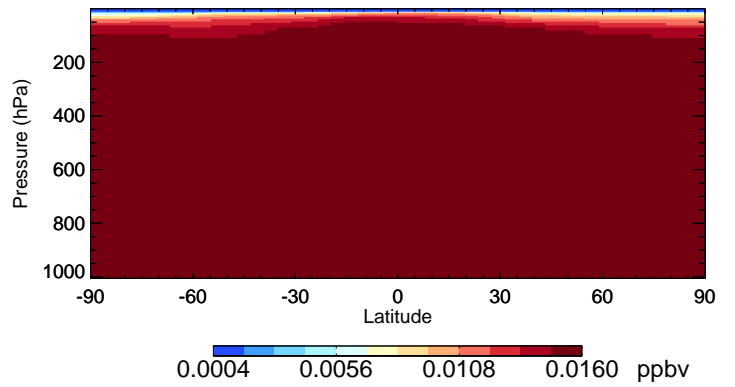
v11-02f-Run0 CFC114 - Species Curtain @ -180.000 for Jul
