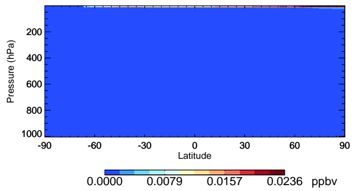
v11-02e-Run1 Br - Species Curtain @ -180.000 for Jul
