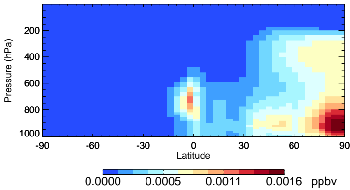
v11-02f-Run0 SOAME - Species Zonal Mean for Jul
