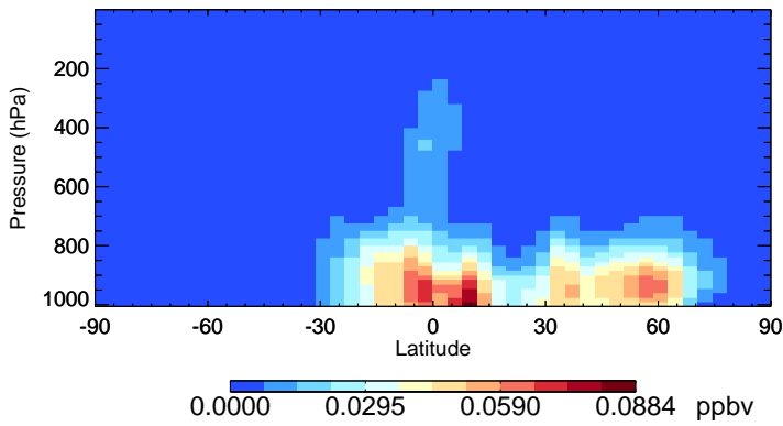
v11-02f-Run0 HAC - Species Zonal Mean for Jul
