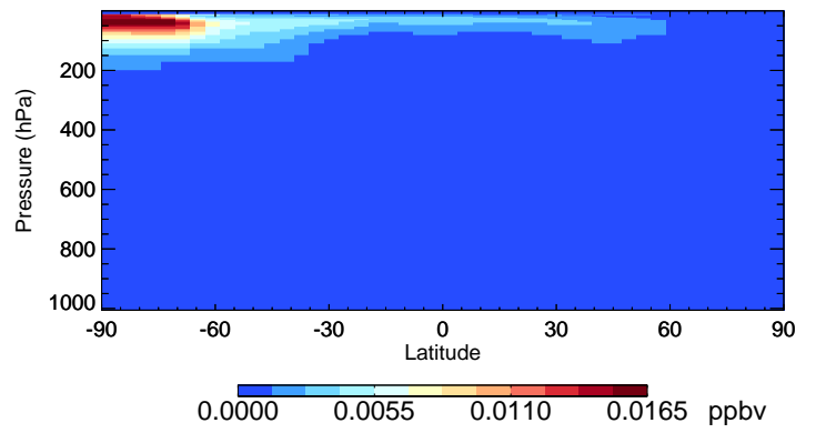
v11-02e-Run1 BrCl - Species Curtain @ -180.000 for Jul
