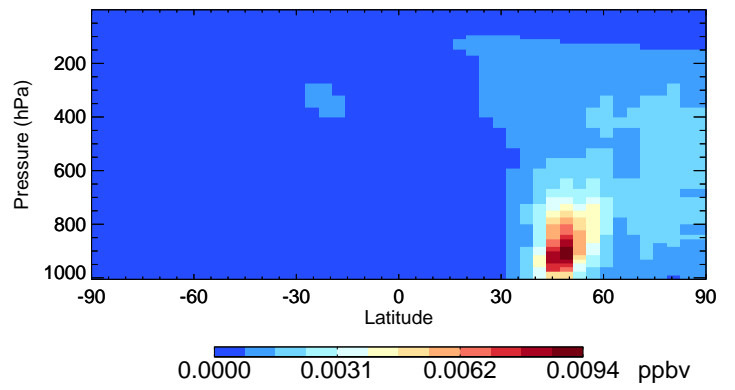
v11-02e-Run0 ASOAN - Species Curtain @ -180.000 for Jul
