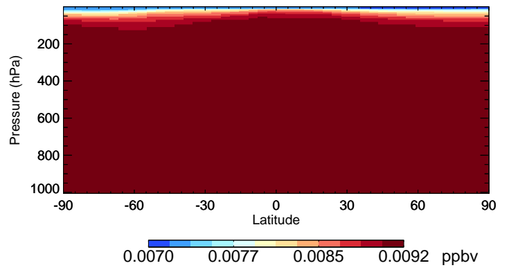
v11-02e-Run0 CFC115 - Species Curtain @ -180.000 for Jul
