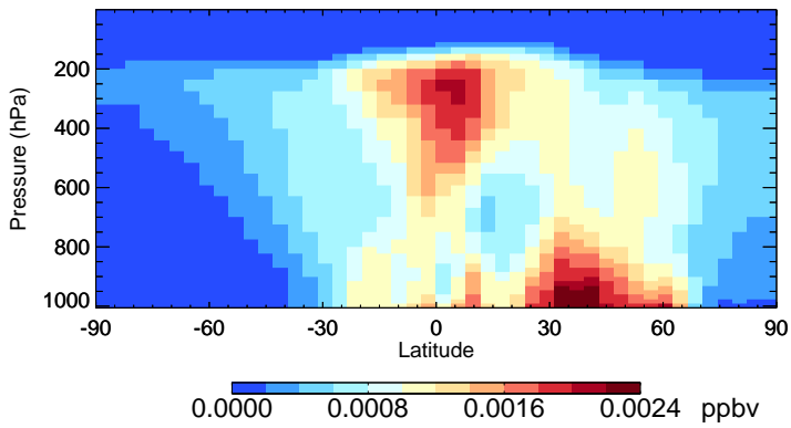
v11-02f-Run0 R4N2 - Species Zonal Mean for Jul
