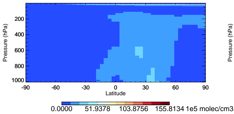
v11-02f-Run0 OH - Species Zonal Mean for Jul
