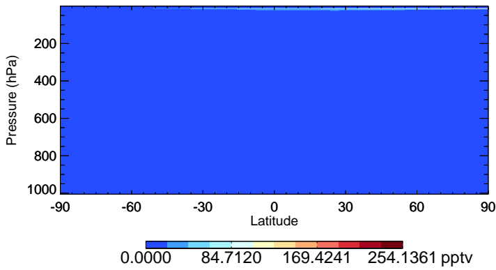
v11-02f-Run0 HO2 - Species Zonal Mean for Jul
