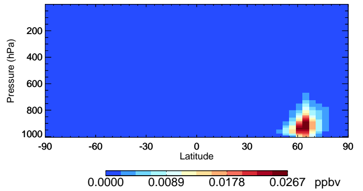
v11-02f-Run0 GLYC - Species Curtain @ -180.000 for Jul
