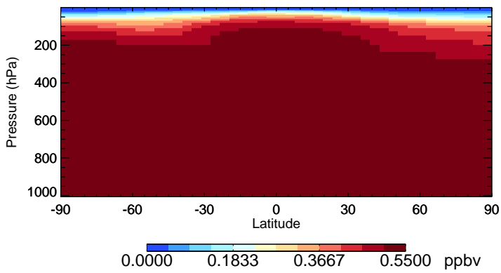
v11-02f-Run0 CH3Cl - Species Zonal Mean for Jul
