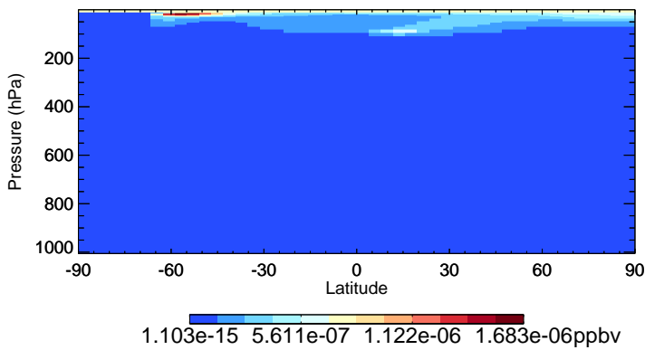
v11-02f-Run0 CIOO - Species Zonal Mean for Jul
