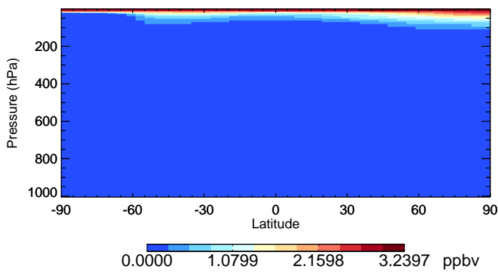
v11-02f-Run0 HCl - Species Zonal Mean for Jul
