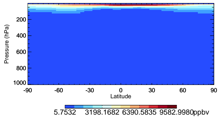
v11-02f-Run0 O3 - Species Curtain @ -180.000 for Jul
