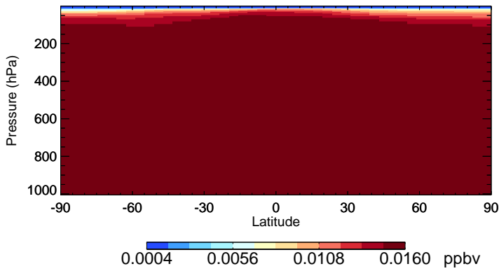
v11-02f-Run0 CFC114 - Species Zonal Mean for Jul
