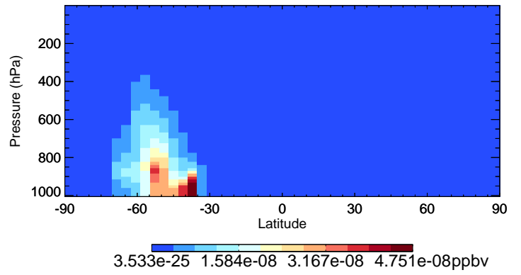
v11-02e-Run0 NPMN - Species Curtain @ -180.000 for Jul
