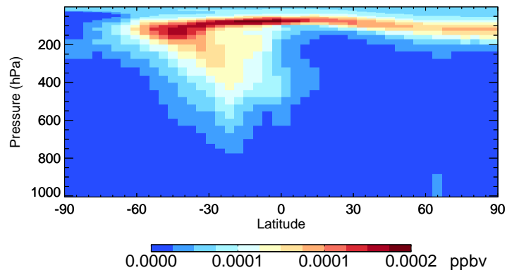
v11-02e-Run0 DHDN - Species Curtain @ -180.000 for Jul
