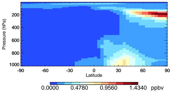
v11-02f-Run0 SO4 - Species Zonal Mean for Jul
