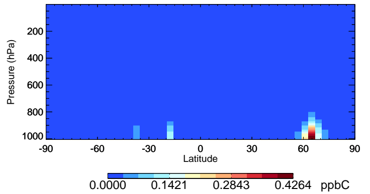
v11-02f-Run0 PRPE - Species Curtain @ -180.000 for Jul
