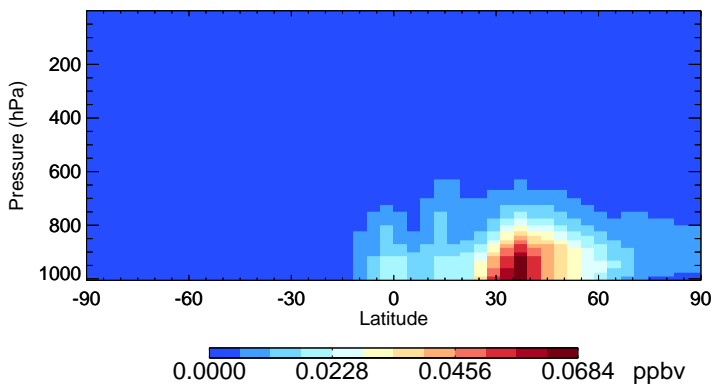
v11-02f-Run0 SOAGX - Species Zonal Mean for Jul
