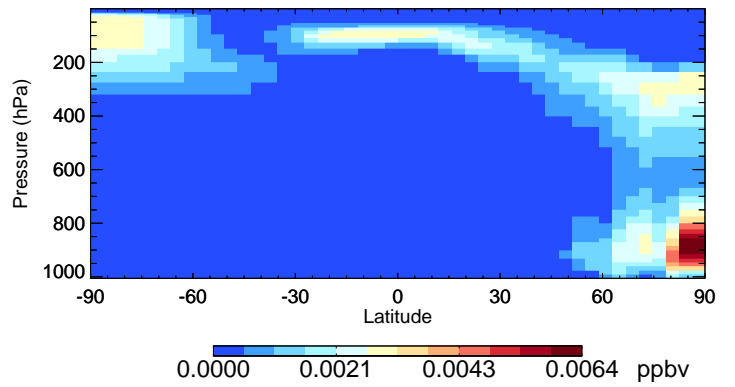
v11-02f-Run0 TSOA2 - Species Curtain @ -180.000 for Jul
