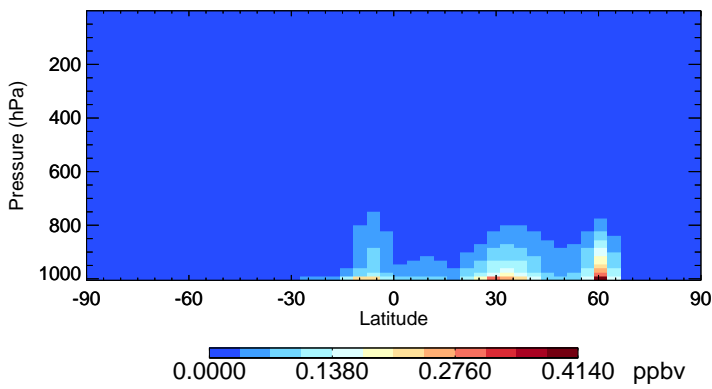
v11-02f-Run0 BCPO - Species Zonal Mean for Jul
