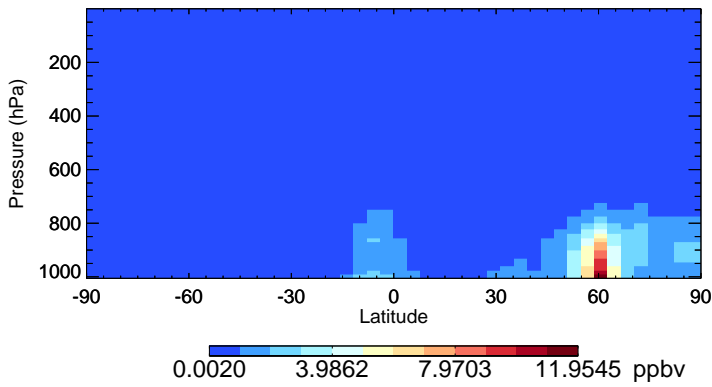
v11-02f-Run0 OCPI - Species Zonal Mean for Jul
