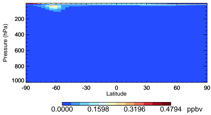
v11-02f-Run0 CIO - Species Zonal Mean for Jul
