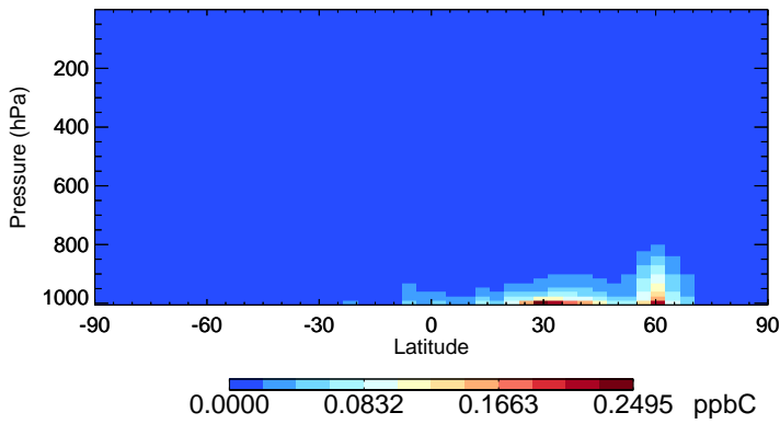
v11-02f-Run0 XYLE - Species Zonal Mean for Jul
