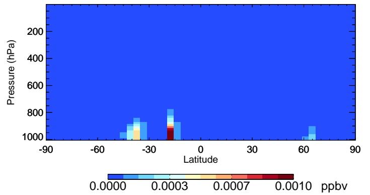
v11-02f-Run0 MONITS - Species Curtain @ -180.000 for Jul
