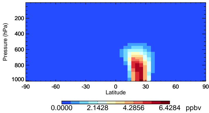
v11-02f-Run0 DST2 - Species Zonal Mean for Jul
