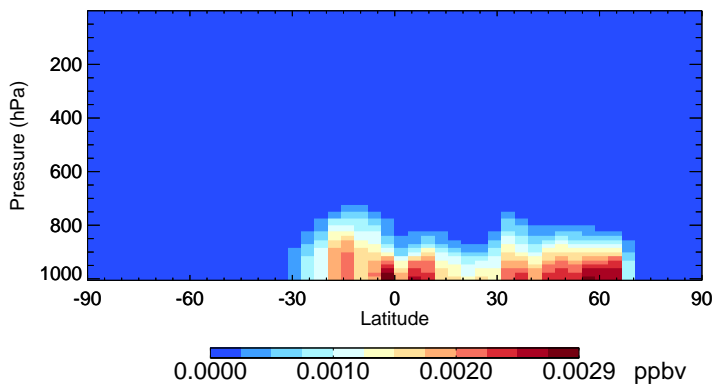
v11-02f-Run0 ISOPNB - Species Zonal Mean for Jul
