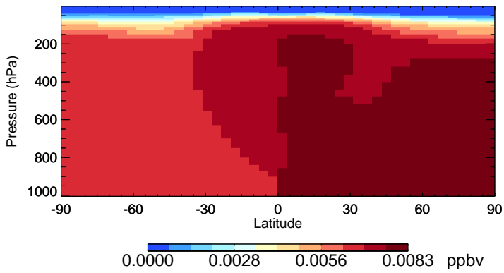
v11-02f-Run0 CH3Br - Species Zonal Mean for Jul
