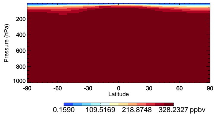
v11-02f-Run0 N2O - Species Curtain @ -180.000 for Jul
