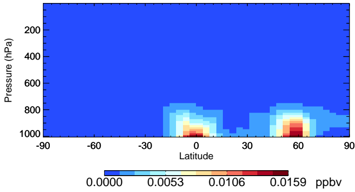
v11-02e-Run1 TSOA1 - Species Zonal Mean for Jul
