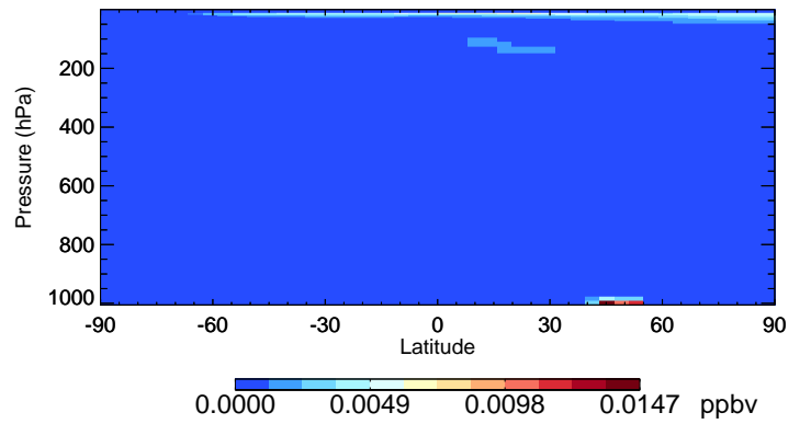
v11-02f-Run0 HNO 2 - Species Curtain @ -180.000 for Jul
