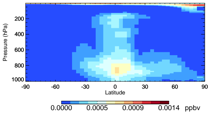
v11-02f-Run0 HBr - Species Zonal Mean for Jul
