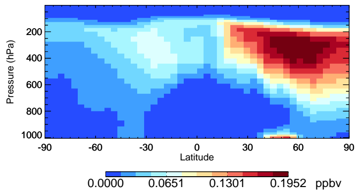
v11-02f-Run0 PAN - Species Curtain @ -180.000 for Jul
