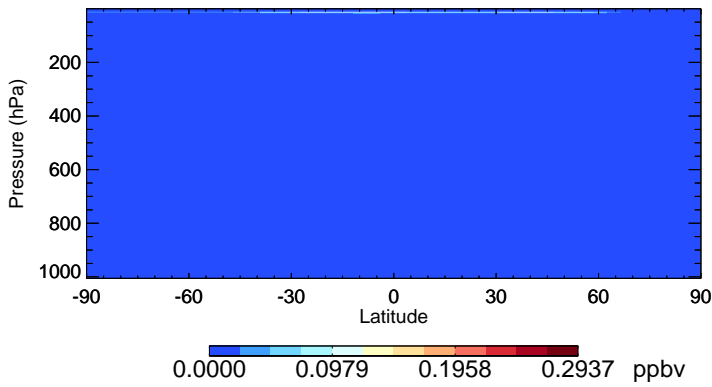
v11-02f-Run0 NO3 - Species Zonal Mean for Jul
