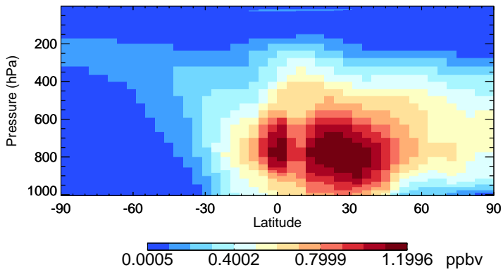
v11-02f-Run0 H2O2 - Species Zonal Mean for Jul
