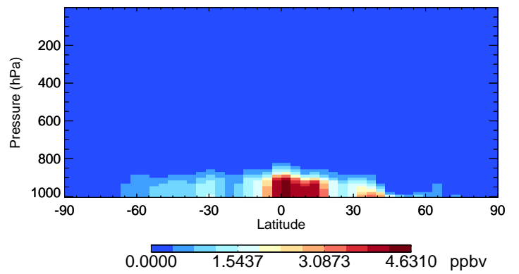
v11-02f-Run0 NH3 - Species Curtain @ -180.000 for Jul
