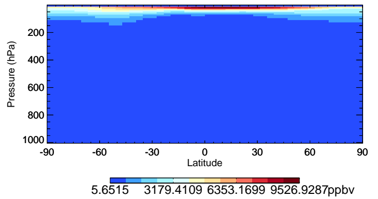
v11-02e-Run1 O3 - Species Curtain @ -180.000 for Jul
