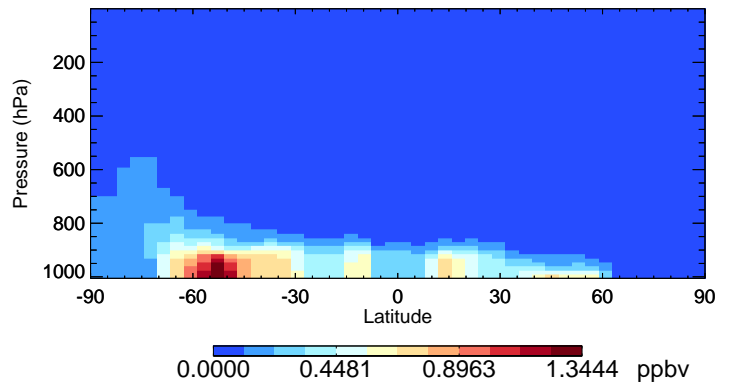
v11-02f-Run0 SALA - Species Curtain @ -180.000 for Jul
