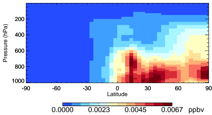
v11-02f-Run0 ASOAN - Species Zonal Mean for Jul
