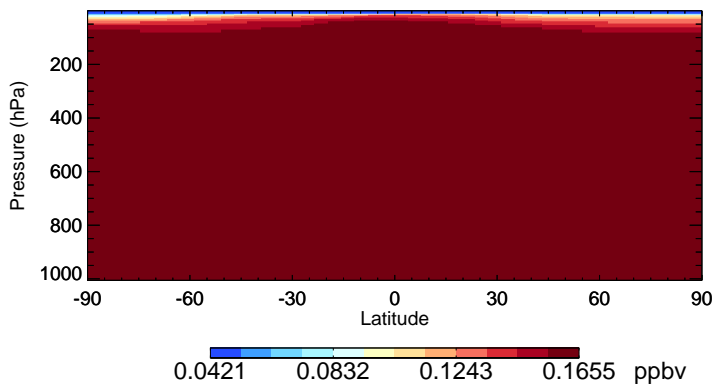
v11-02f-Run0 HCFC22 - Species Zonal Mean for Jul
