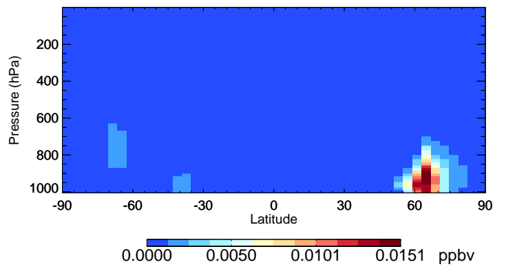
v11-02f-Run0 IPMN - Species Curtain @ -180.000 for Jul
