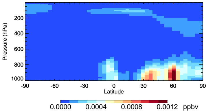
v11-02f-Run0 ASOA2 - Species Zonal Mean for Jul
