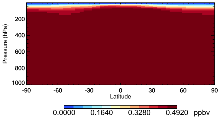
v11-02f-Run0 CFC12 - Species Zonal Mean for Jul
