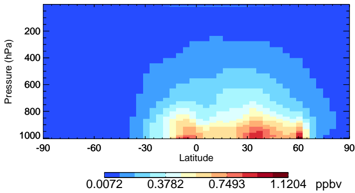
v11-02f-Run0 CH2O - Species Zonal Mean for Jul
