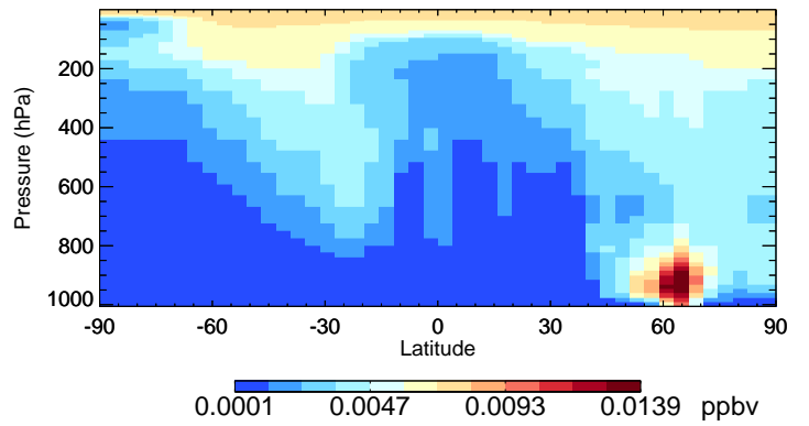
v11-02f-Run0 ISO3 - Species Curtain @ -180.000 for Jul
