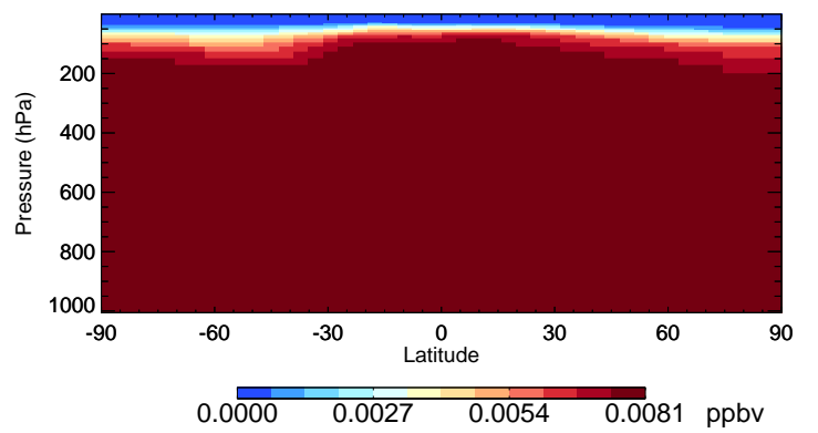
v11-02f-Run0 CH3CCI3 - Species Curtain @ -180.000 for Jul
