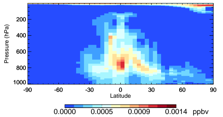
v11-02f-Run0 HBr - Species Curtain @ -180.000 for Jul
