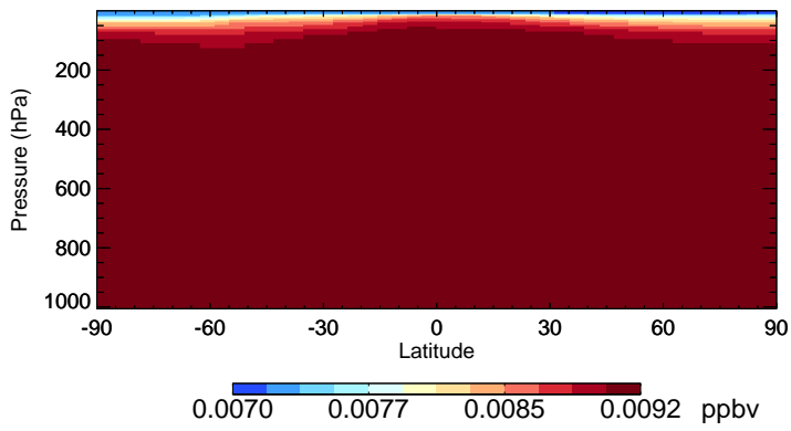
v11-02e-Run0 CFC115 - Species Zonal Mean for Jul
