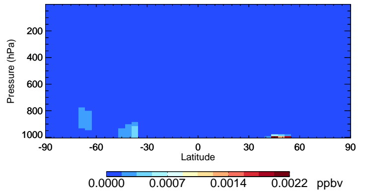
v11-02f-Run0 ClNO 2 - Species Curtain @ -180.000 for Jul
