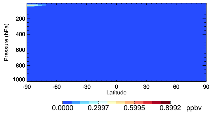
v11-02f-Run0 Cl2 - Species Curtain @ -180.000 for Jul
