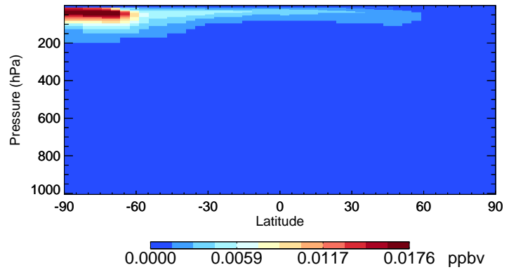
v11-02e-Run0 BrCl - Species Curtain @ -180.000 for Jul
