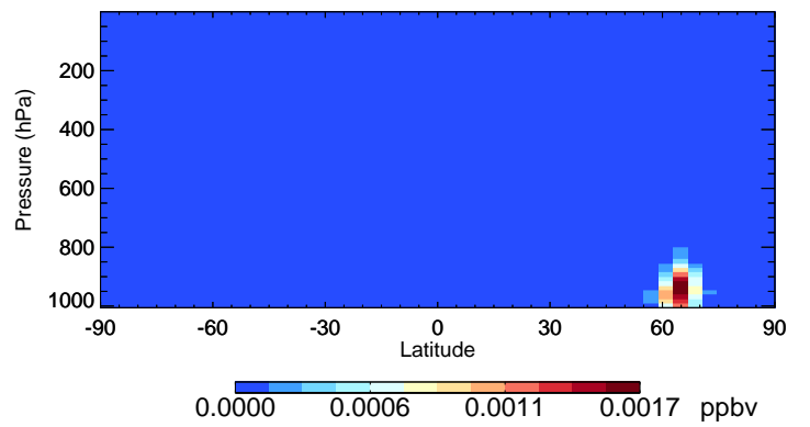
v11-02f-Run0 RIPD - Species Curtain @ -180.000 for Jul
