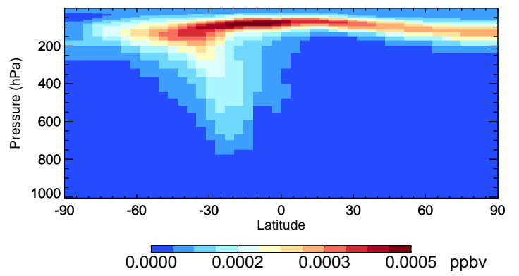
v11-02e-Run1 DHDN - Species Curtain @ -180.000 for Jul
