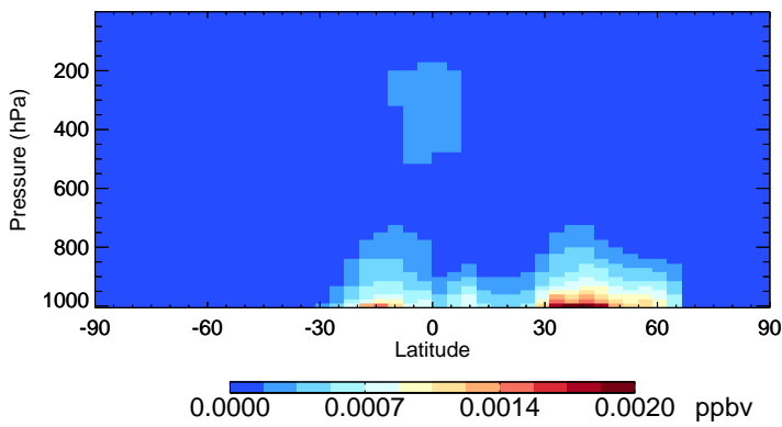
v11-02f-Run0 HONIT - Species Zonal Mean for Jul
