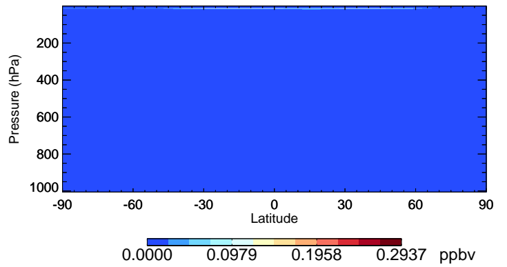
v11-02f-Run0 NO3 - Species Curtain @ -180.000 for Jul
