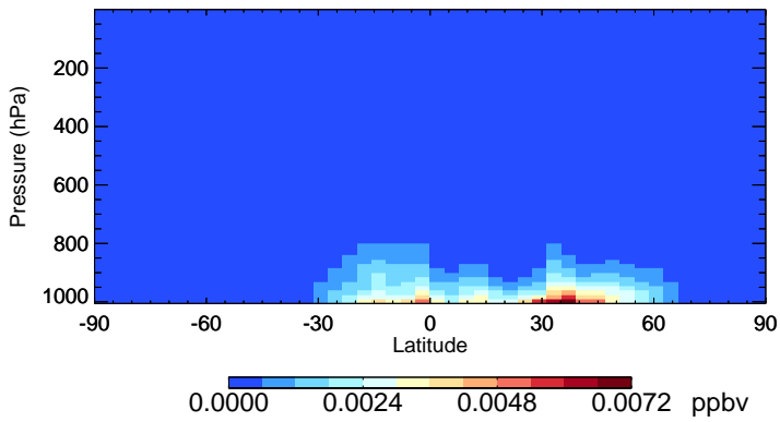
v11-02f-Run0 ISN1 - Species Zonal Mean for Jul
