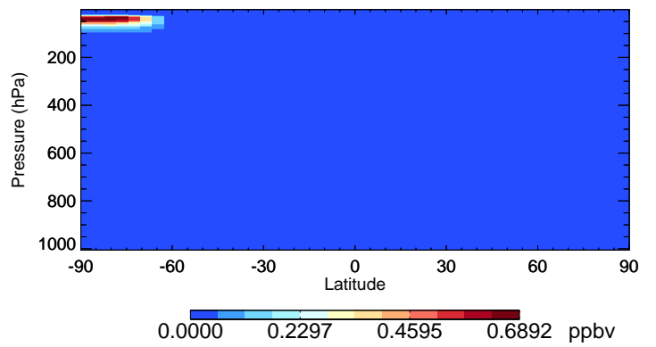
v11-02f-Run0 Cl2O2 - Species Curtain @ -180.000 for Jul
