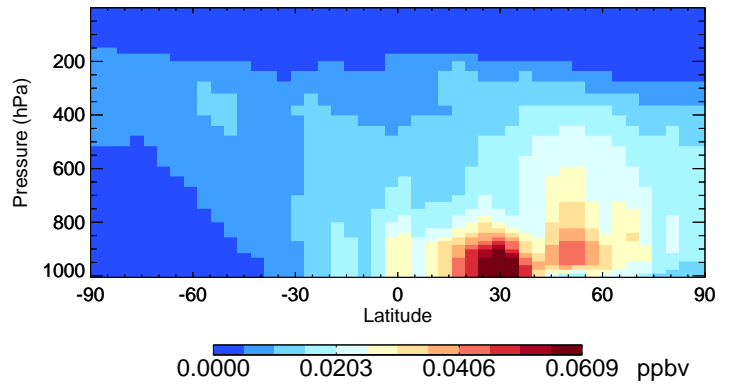
v11-02e-Run0 MAP - Species Curtain @ -180.000 for Jul
