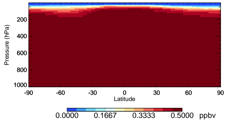
v11-02f-Run0 OCS - Species Curtain @ -180.000 for Jul
