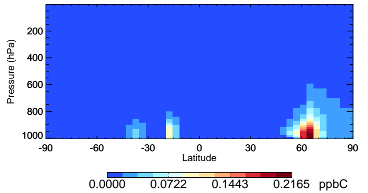
v11-02f-Run0 EOH - Species Curtain @ -180.000 for Jul
