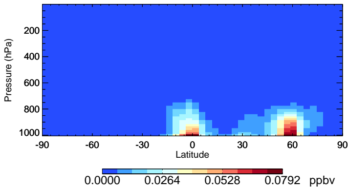
v11-02f-Run0 TSOA2 - Species Zonal Mean for Jul
