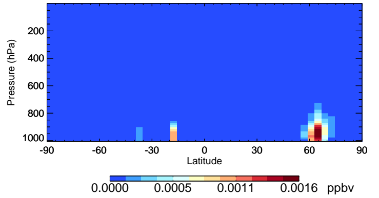
v11-02e-Run1 GLYX - Species Curtain @ -180.000 for Jul
