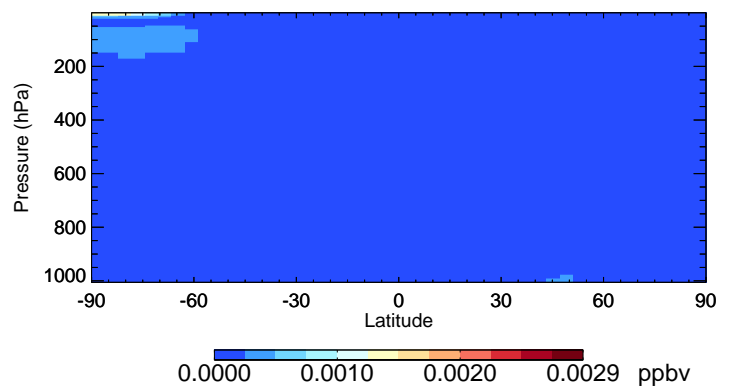
v11-02f-Run0 Br2 - Species Curtain @ -180.000 for Jul
