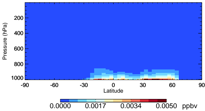
v11-02f-Run0 MONITS - Species Zonal Mean for Jul
