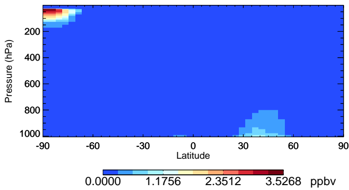
v11-02f-Run0 NIT - Species Zonal Mean for Jul
