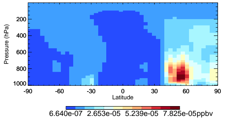
v11-02f-Run0 ISN10A - Species Curtain @ -180.000 for Jul
