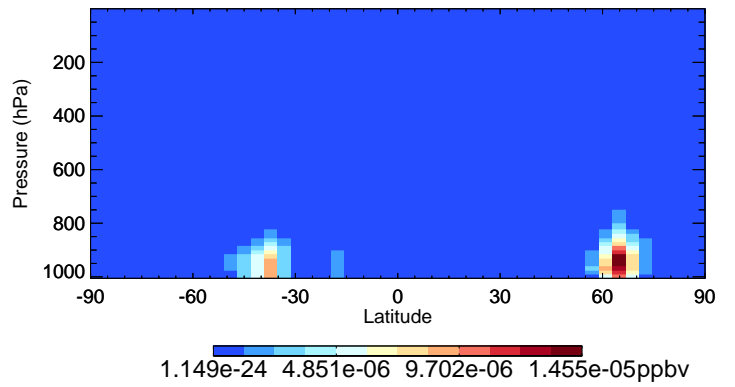
v11-02f-Run0 ETHLN - Species Curtain @ -180.000 for Jul
