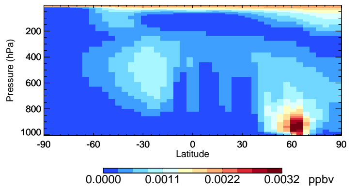
v11-02f-Run0 ISOG1 - Species Curtain @ -180.000 for Jul
