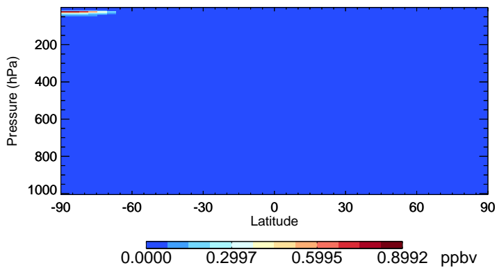
v11-02f-Run0 Cl2 - Species Zonal Mean for Jul
