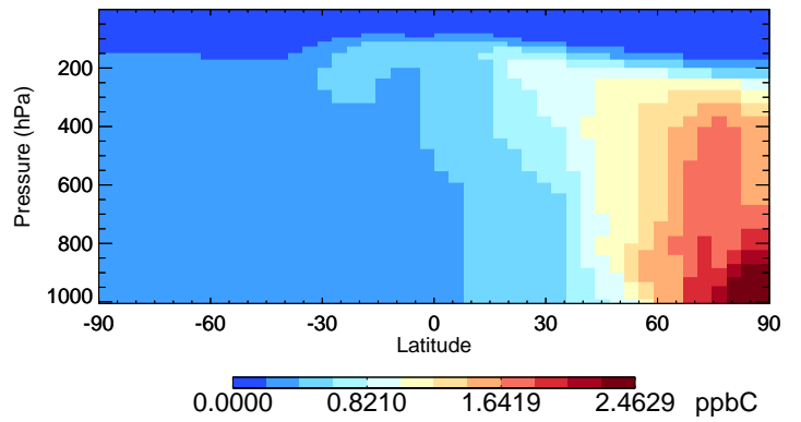
v11-02f-Run0 C2H6 - Species Curtain @ -180.000 for Jul
