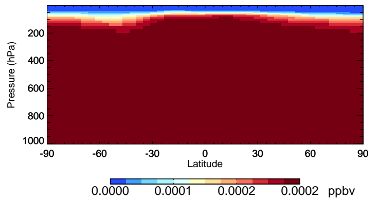
v11-02f-Run0 H2402 - Species Curtain @ -180.000 for Jul
