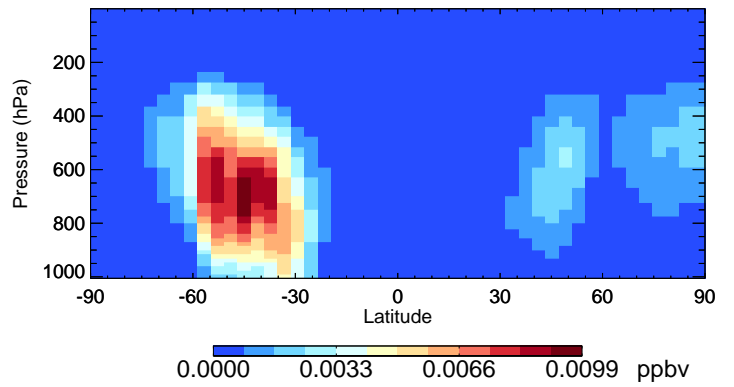
v11-02f-Run0 DST4 - Species Curtain @ -180.000 for Oct
