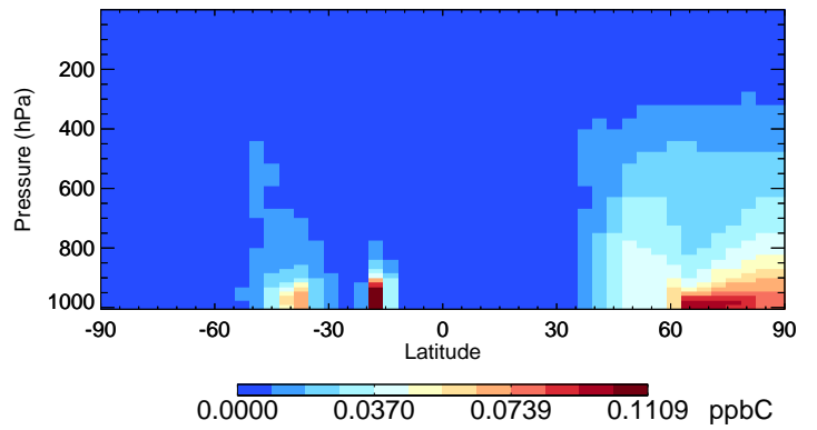
v11-02f-Run0 EOH - Species Curtain @ -180.000 for Oct
