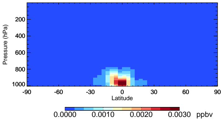
v11-02f-Run0 RIPD - Species Zonal Mean for Oct
