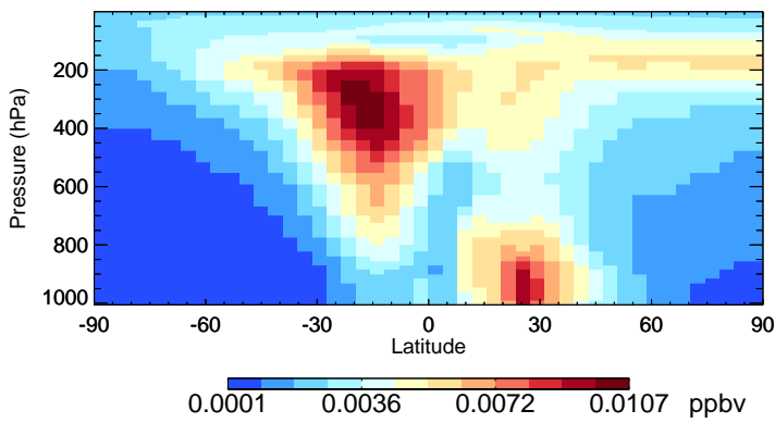
v11-02f-Run0 ASOG3 - Species Zonal Mean for Oct
