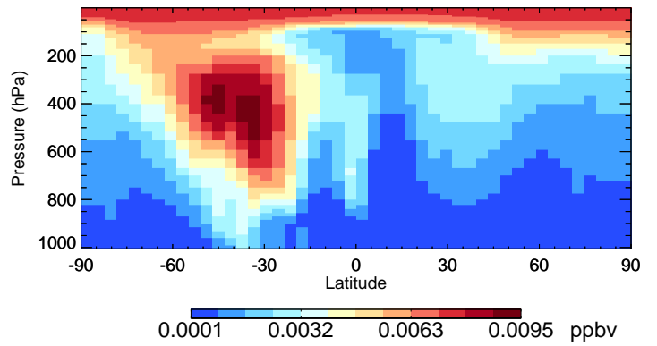
v11-02f-Run0 ISOG3 - Species Curtain @ -180.000 for Oct
