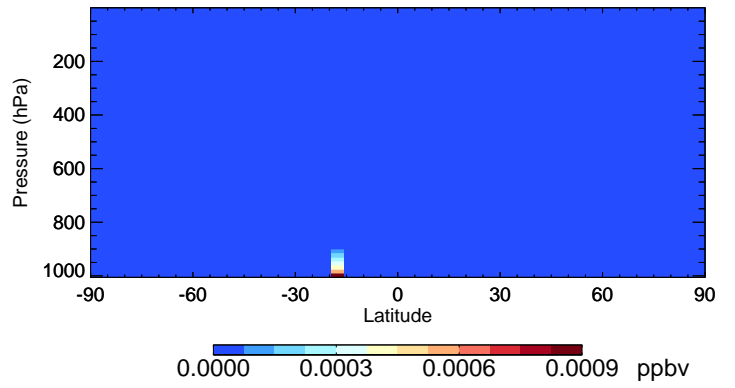
v11-02e-Run0 MTPO - Species Curtain @ -180.000 for Oct
