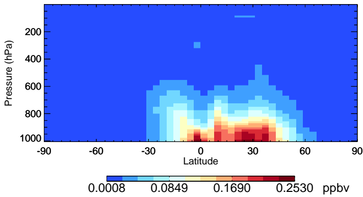
v11-02f-Run0 SOAS - Species Zonal Mean for Oct
