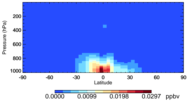
v11-02f-Run0 IPMN - Species Zonal Mean for Oct
