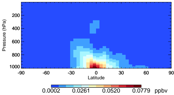
v11-02f-Run0 TSOG2 - Species Zonal Mean for Oct
