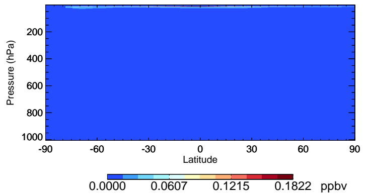
v11-02e-Run0 NO3 - Species Curtain @ -180.000 for Oct
