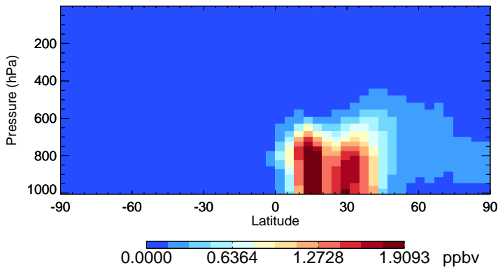
v11-02f-Run0 DST1 - Species Zonal Mean for Oct
