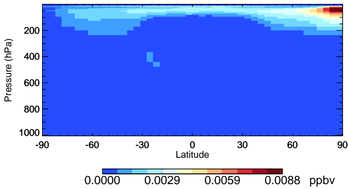
v11-02f-Run0 HOBr - Species Zonal Mean for Oct
