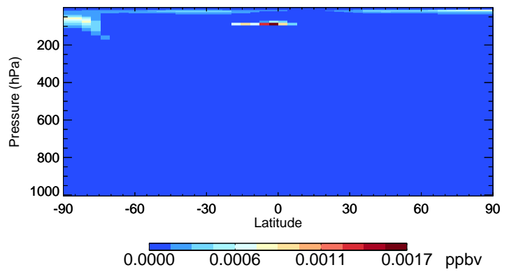
v11-02f-Run0 Cl2 - Species Curtain @ -180.000 for Oct
