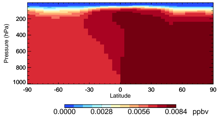
v11-02f-Run0 CH3Br - Species Curtain @ -180.000 for Oct
