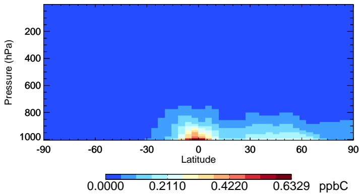
v11-02f-Run0 EOH - Species Zonal Mean for Oct
