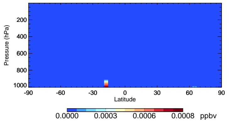
v11-02e-Run1 MTPO - Species Curtain @ -180.000 for Oct
