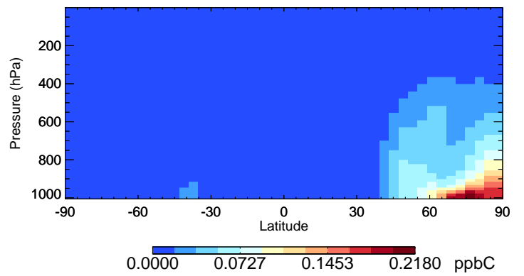
v11-02f-Run0 TOLU - Species Curtain @ -180.000 for Oct
