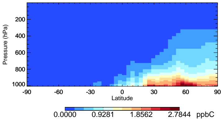
v11-02f-Run0 ALK4 - Species Zonal Mean for Oct
