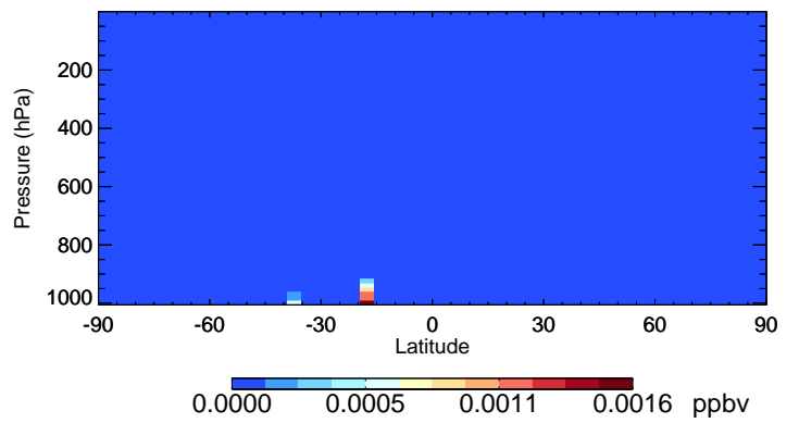
v11-02f-Run0 MTPO - Species Curtain @ -180.000 for Oct
