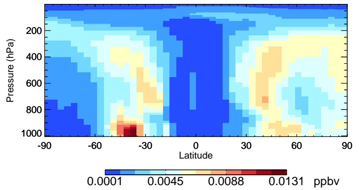
v11-02f-Run0 INDIOL - Species Curtain @ -180.000 for Oct
