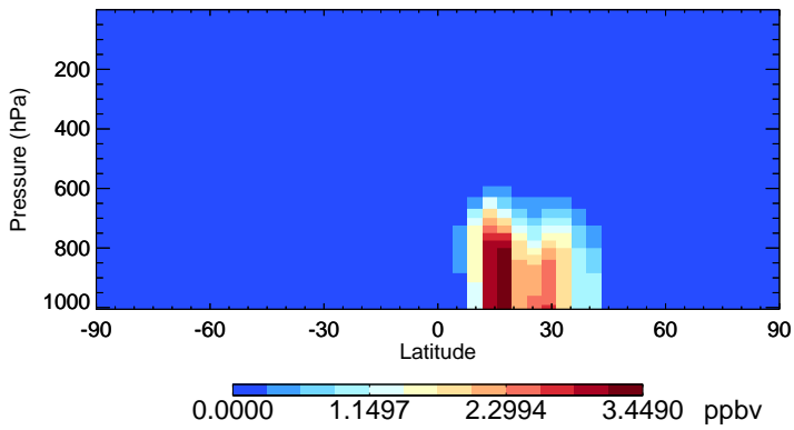
v11-02f-Run0 DST2 - Species Zonal Mean for Oct
