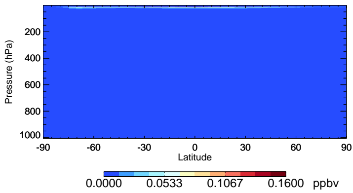
v11-02f-Run0 NO3 - Species Zonal Mean for Oct
