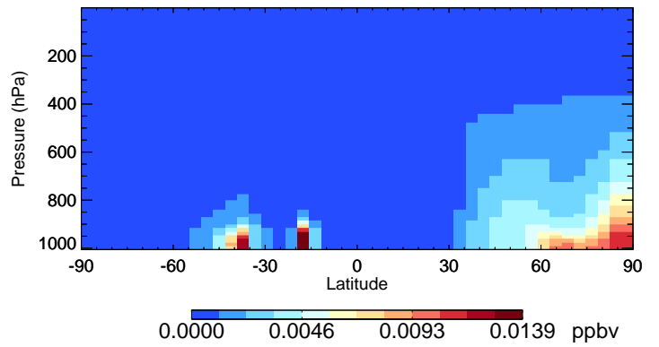
v11-02f-Run0 RCHO - Species Curtain @ -180.000 for Oct
