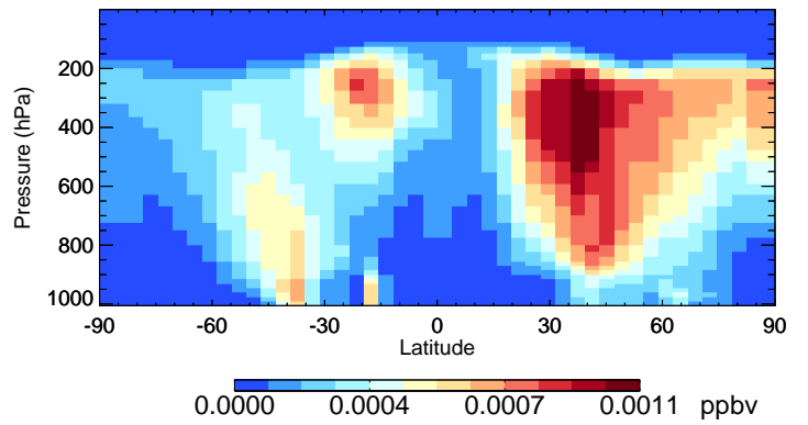
v11-02f-Run0 R4N2 - Species Curtain @ -180.000 for Oct
