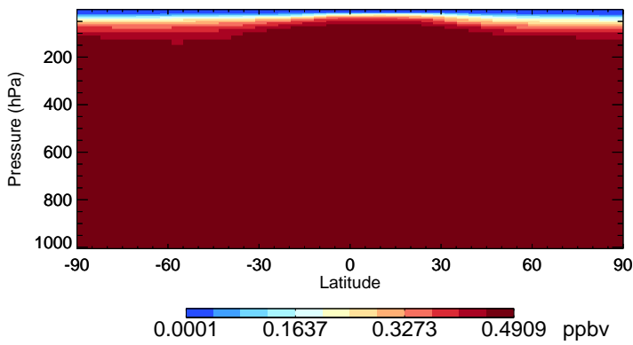
v11-02f-Run0 CFC12 - Species Zonal Mean for Oct
