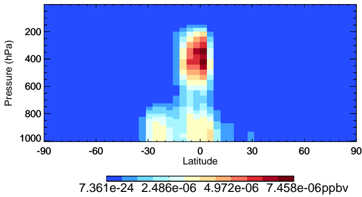
v11-02f-Run0 LVOC - Species Zonal Mean for Oct
