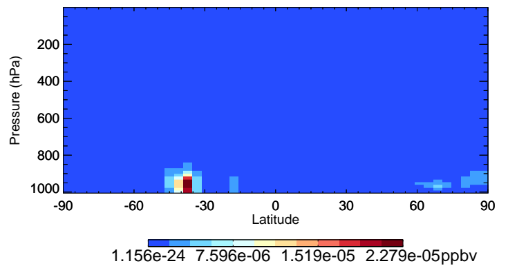
v11-02f-Run0 ETHLN - Species Curtain @ -180.000 for Oct
