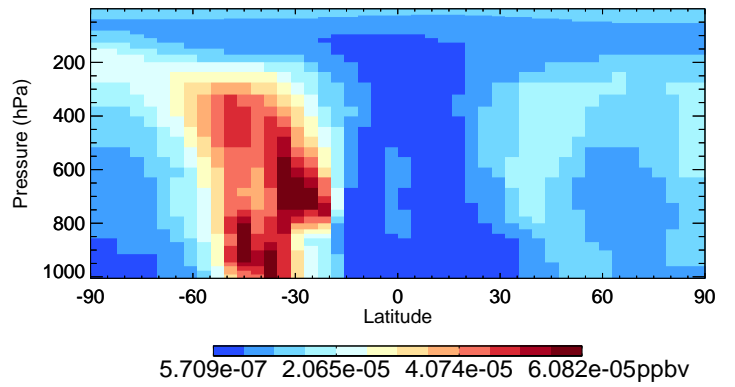
v11-02f-Run0 ISN10A - Species Curtain @ -180.000 for Oct
