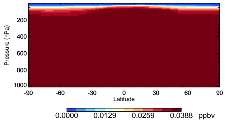
v11-02f-Run0 HCFC141b - Species Curtain @ -180.000 for Oct
