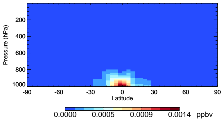
v11-02f-Run0 MOBA - Species Zonal Mean for Oct
