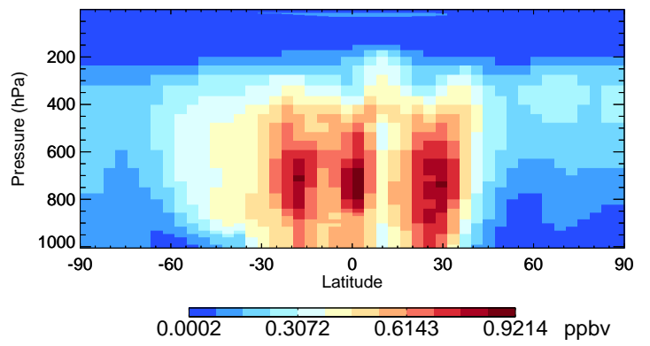
v11-02f-Run0 H2O2 - Species Curtain @ -180.000 for Oct
