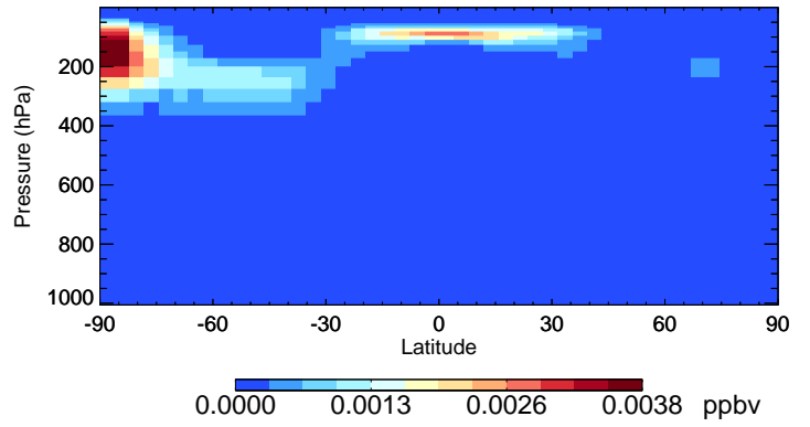
v11-02e-Run1 ISOA3 - Species Curtain @ -180.000 for Oct
