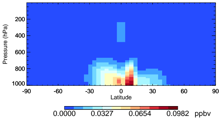
v11-02f-Run0 HAC - Species Zonal Mean for Oct
