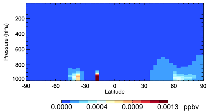
v11-02f-Run0 GLYX - Species Curtain @ -180.000 for Oct
