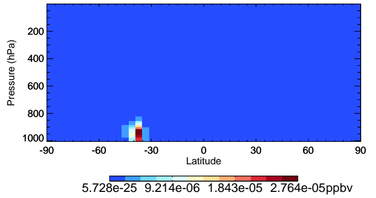
v11-02e-Run0 MACRN - Species Curtain @ -180.000 for Oct
