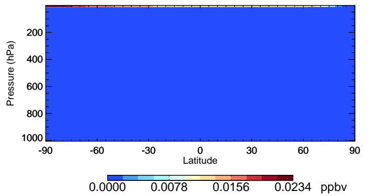
v11-02f-Run0 Br - Species Curtain @ -180.000 for Oct
