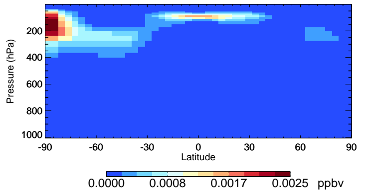
v11-02f-Run0 ISOA3 - Species Curtain @ -180.000 for Oct
