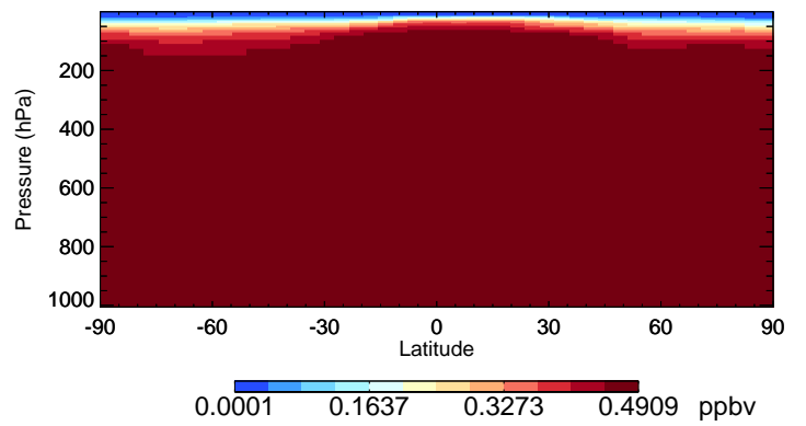
v11-02f-Run0 CFC12 - Species Curtain @ -180.000 for Oct
