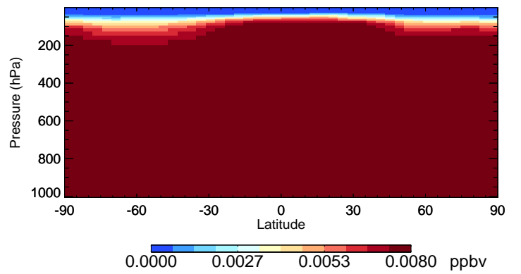
v11-02f-Run0 CH3CCI3 - Species Curtain @ -180.000 for Oct
