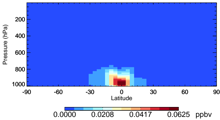
v11-02f-Run0 RIPA - Species Zonal Mean for Oct
