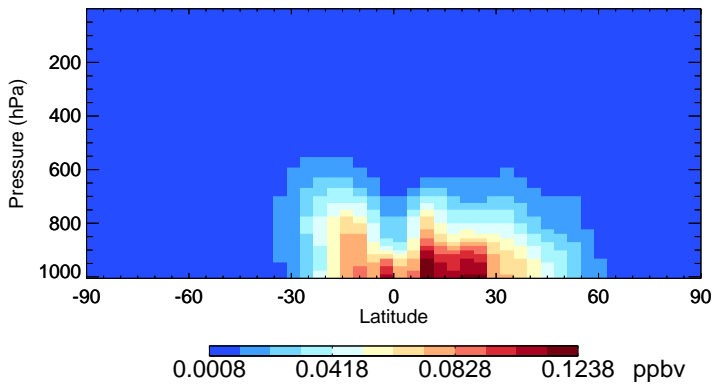
v11-02f-Run0 INDIOL - Species Zonal Mean for Oct
