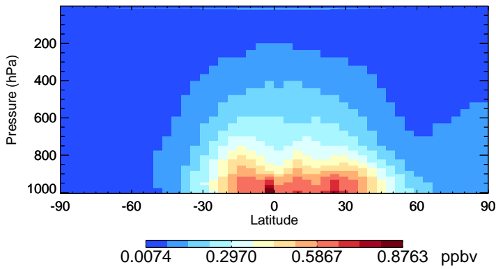
v11-02f-Run0 CH2O - Species Zonal Mean for Oct
