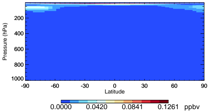
v11-02f-Run0 HOCl - Species Zonal Mean for Oct
