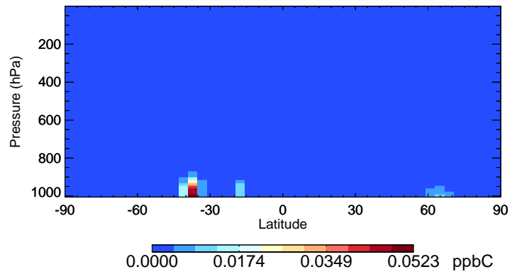
v11-02f-Run0 ISOP - Species Curtain @ -180.000 for Oct
