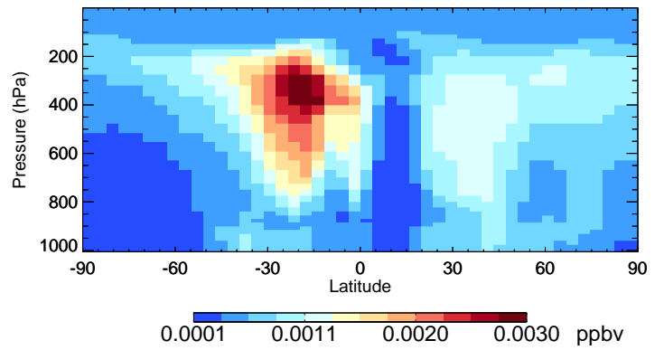
v11-02f-Run0 ASOAN - Species Curtain @ -180.000 for Oct
