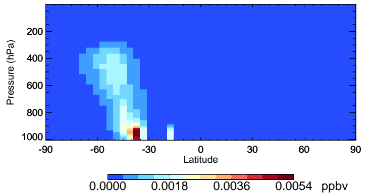
v11-02f-Run0 IEPOXA - Species Curtain @ -180.000 for Oct
