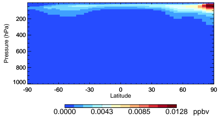
v11-02f-Run0 BrCl - Species Curtain @ -180.000 for Oct
