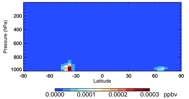
v11-02f-Run0 ISN1 - Species Curtain @ -180.000 for Oct
