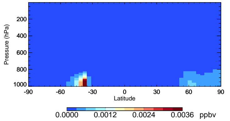
v11-02e-Run0 MACR - Species Curtain @ -180.000 for Oct
