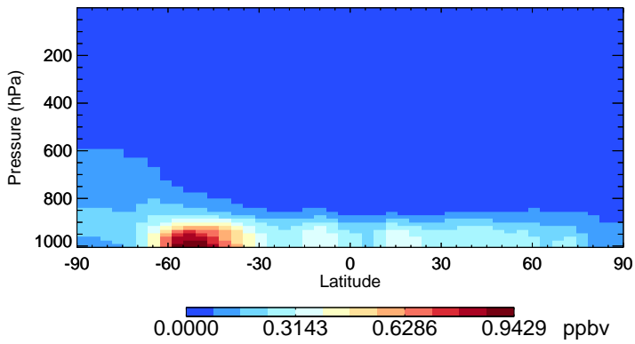
v11-02f-Run0 SALA - Species Zonal Mean for Oct
