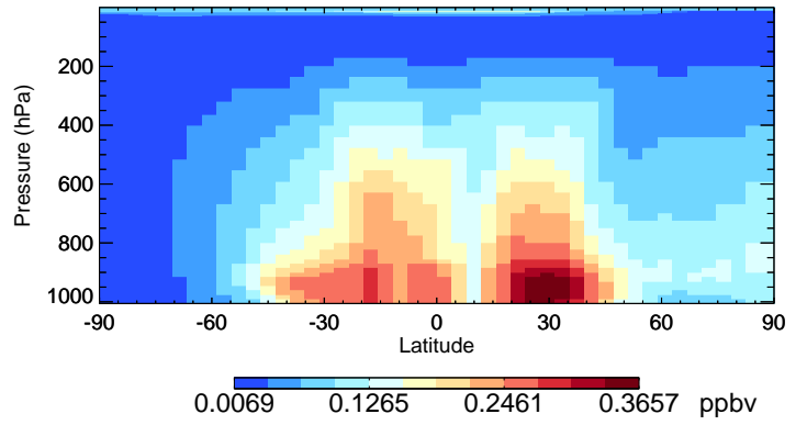
v11-02e-Run1 CH2O - Species Curtain @ -180.000 for Oct
