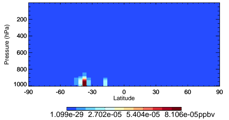
v11-02f-Run0 RIPD - Species Curtain @ -180.000 for Oct
