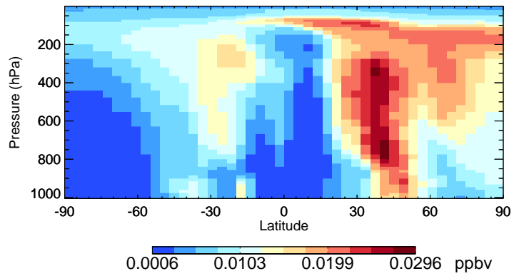
v11-02f-Run0 SOAS - Species Curtain @ -180.000 for Oct
