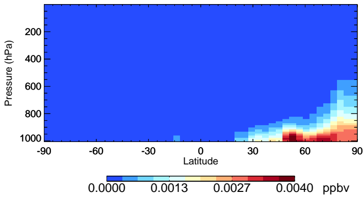
v11-02f-Run0 CINO2 - Species Zonal Mean for Oct
