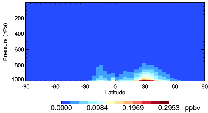
v11-02f-Run0 BCPO - Species Zonal Mean for Oct
