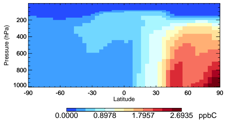
v11-02f-Run0 C2H6 - Species Curtain @ -180.000 for Oct
