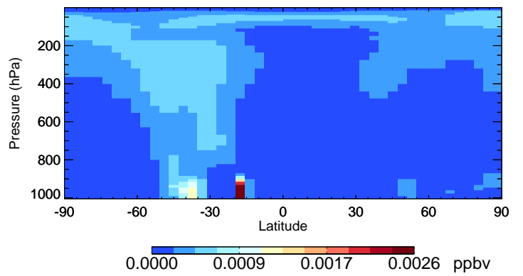
v11-02f-Run0 TSOA0 - Species Curtain @ -180.000 for Oct
