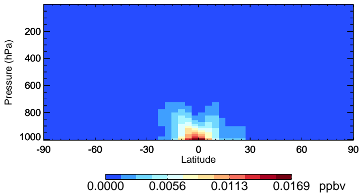
v11-02f-Run0 TSOA1 - Species Zonal Mean for Oct
