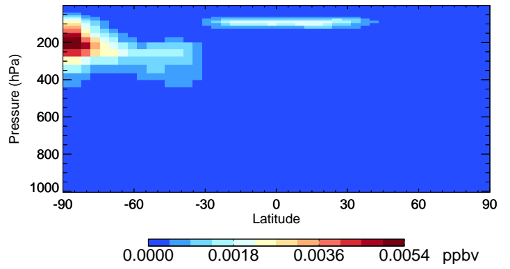
v11-02e-Run0 ISOA3 - Species Curtain @ -180.000 for Oct
