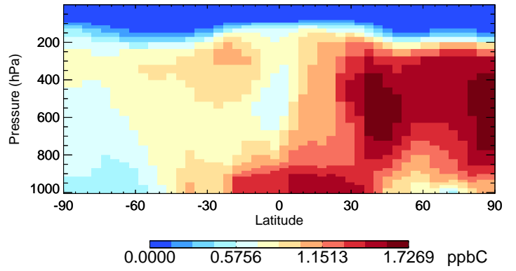
v11-02e-Run1 ACET - Species Curtain @ -180.000 for Oct
