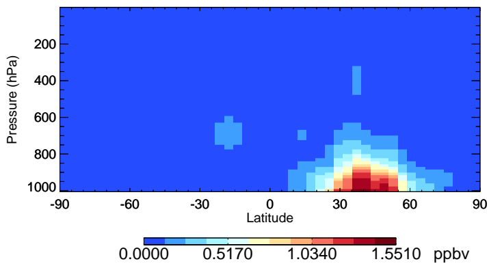
v11-02f-Run0 NIT - Species Zonal Mean for Oct
