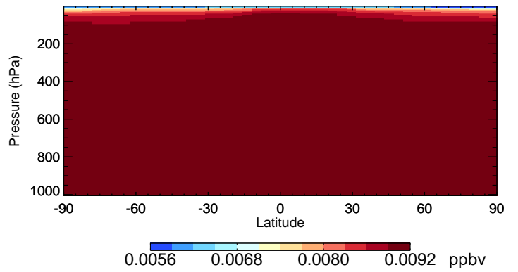
v11-02f-Run0 CFC115 - Species Curtain @ -180.000 for Oct
