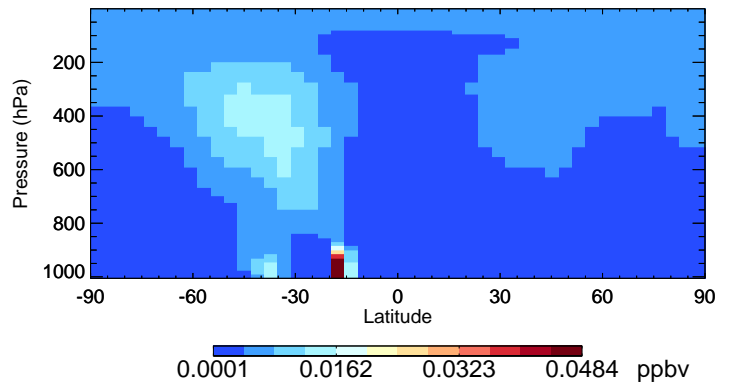
v11-02f-Run0 TSOG3 - Species Curtain @ -180.000 for Oct
