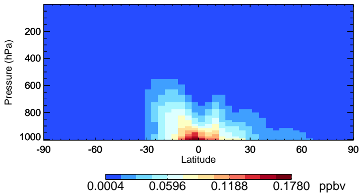
v11-02f-Run0 TSOG3 - Species Zonal Mean for Oct
