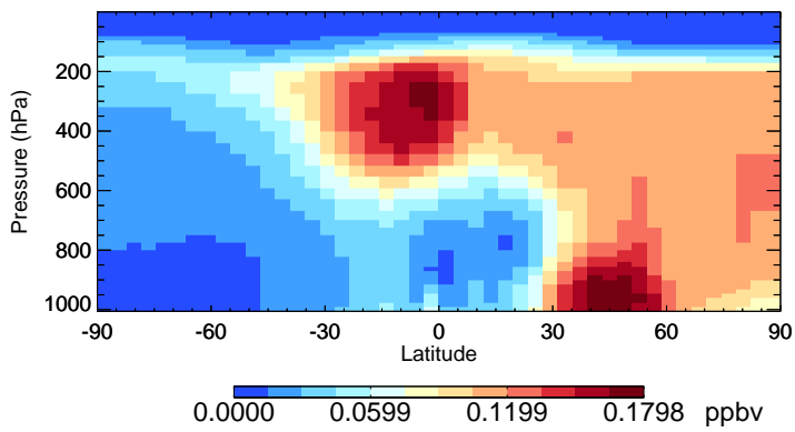
v11-02f-Run0 PAN - Species Zonal Mean for Oct
