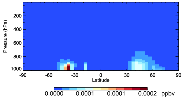
v11-02f-Run0 IONITA - Species Curtain @ -180.000 for Oct
