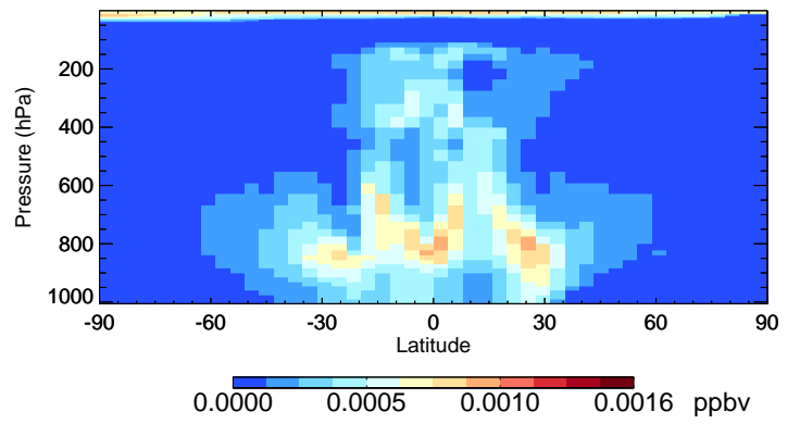
v11-02e-Run1 HBr - Species Curtain @ -180.000 for Oct
