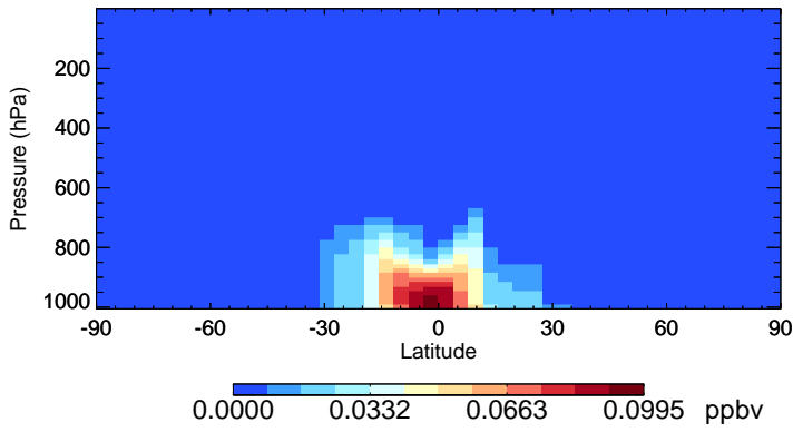
v11-02e-Run0 MACR - Species Zonal Mean for Oct
