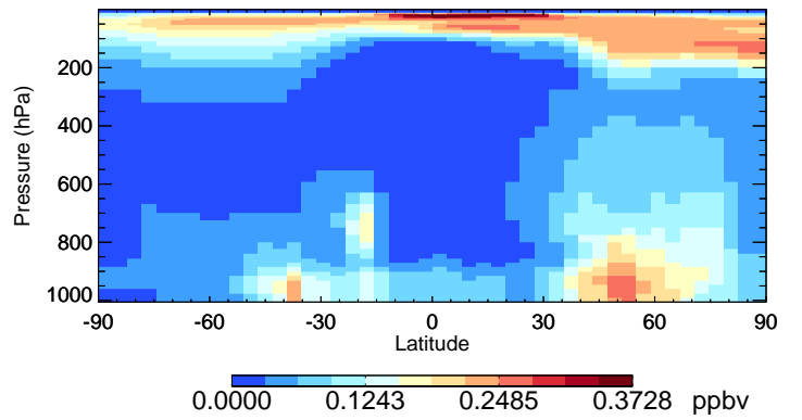
v11-02f-Run0 SO4 - Species Curtain @ -180.000 for Oct
