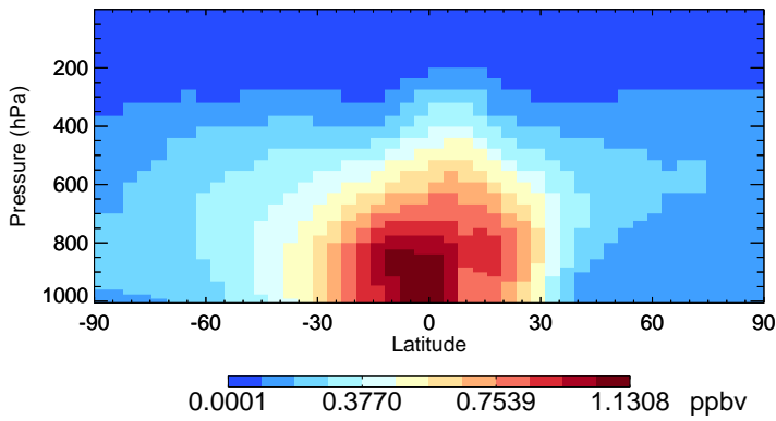
v11-02f-Run0 MP - Species Zonal Mean for Oct
