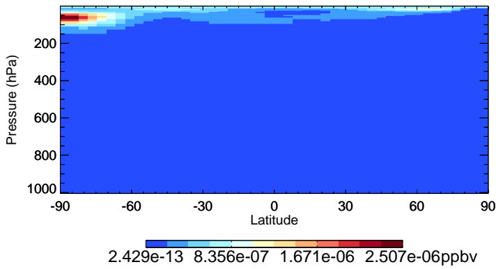
v11-02f-Run0 CIOO - Species Zonal Mean for Oct
