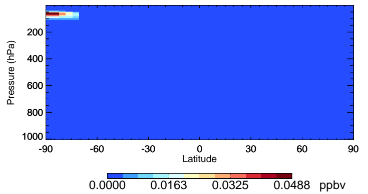
v11-02f-Run0 Cl2O2 - Species Curtain @ -180.000 for Oct
