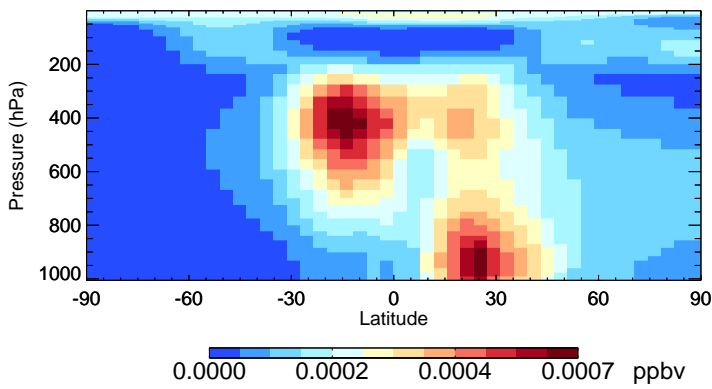
v11-02f-Run0 ASOG1 - Species Zonal Mean for Oct
