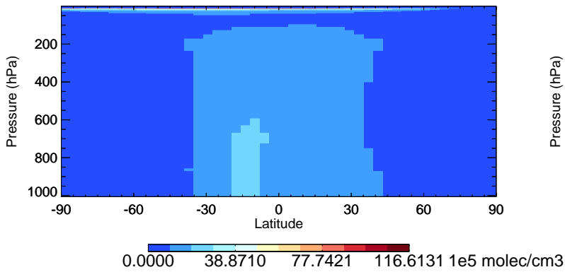
v11-02f-Run0 OH - Species Zonal Mean for Oct
