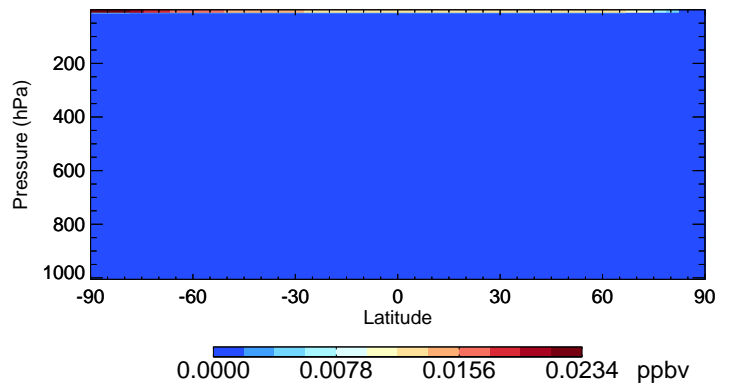
v11-02e-Run0 Br - Species Curtain @ -180.000 for Oct
