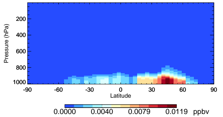
v11-02f-Run0 NITs - Species Curtain @ -180.000 for Oct
