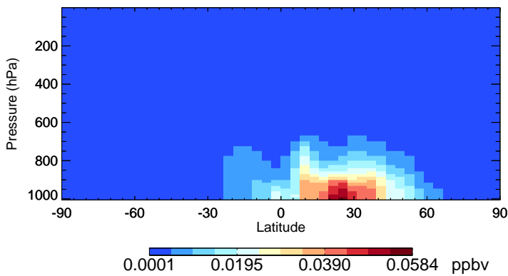
v11-02f-Run0 SOAGX - Species Zonal Mean for Oct
