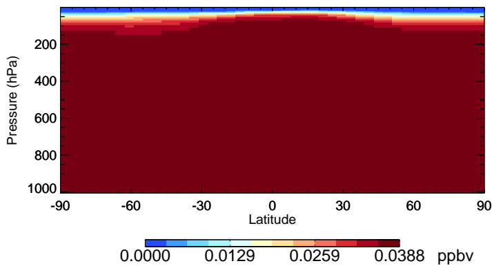
v11-02f-Run0 HCFC141b - Species Zonal Mean for Oct
