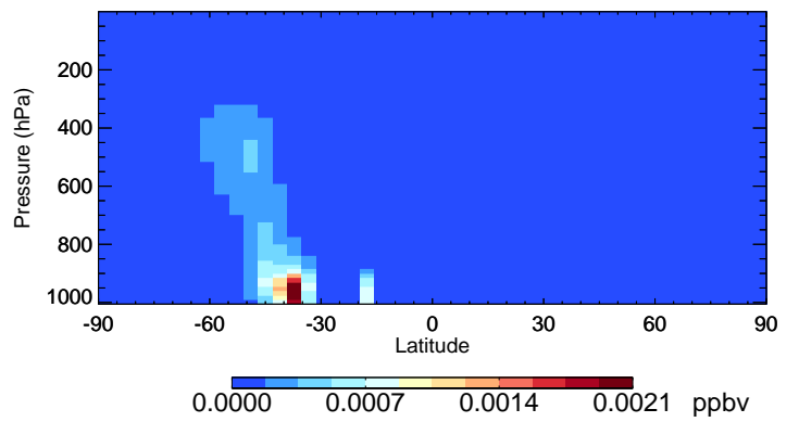
v11-02f-Run0 IEPOXB - Species Curtain @ -180.000 for Oct
