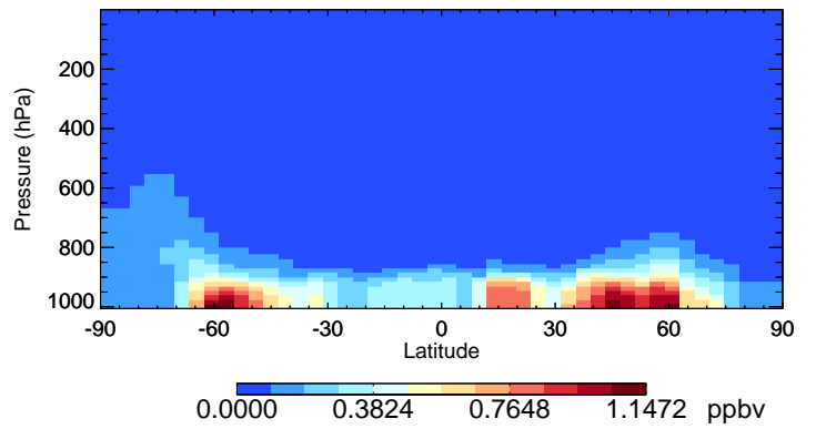
v11-02f-Run0 SALA - Species Curtain @ -180.000 for Oct
