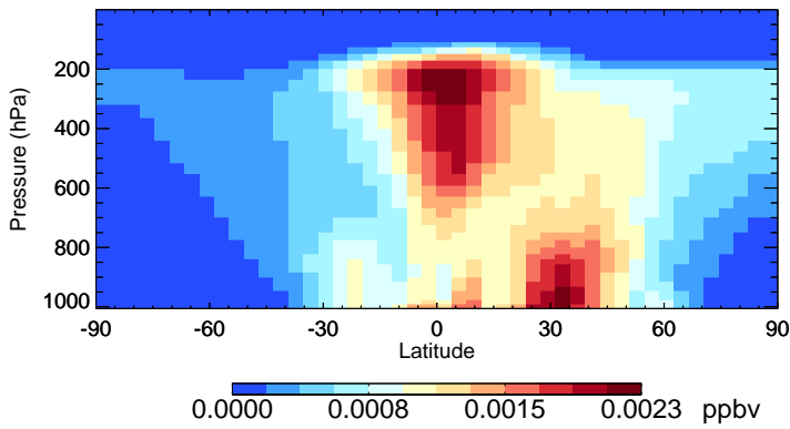
v11-02f-Run0 R4N2 - Species Zonal Mean for Oct
