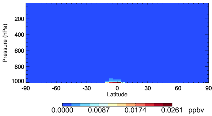
v11-02e-Run1 MTPO - Species Zonal Mean for Oct
