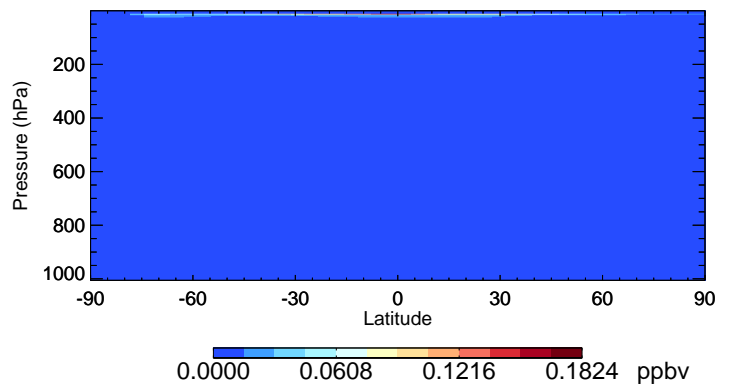
v11-02f-Run0 NO3 - Species Curtain @ -180.000 for Oct
