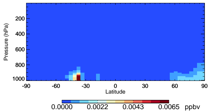
v11-02f-Run0 MACR - Species Curtain @ -180.000 for Oct
