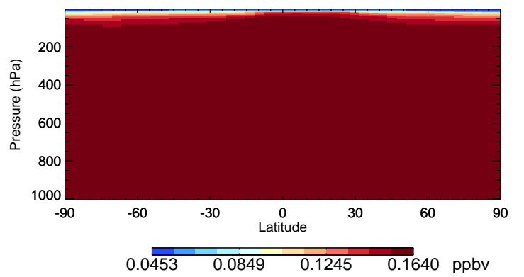
v11-02f-Run0 HCFC22 - Species Curtain @ -180.000 for Oct
