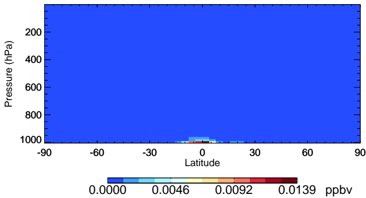
v11-02f-Run0 LIMO - Species Zonal Mean for Oct
