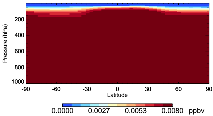
v11-02f-Run0 CH3CCI3 - Species Zonal Mean for Oct
