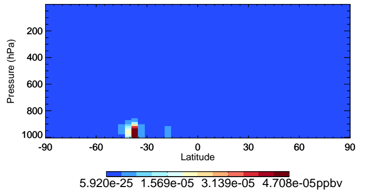
v11-02f-Run0 MACRN - Species Curtain @ -180.000 for Oct
