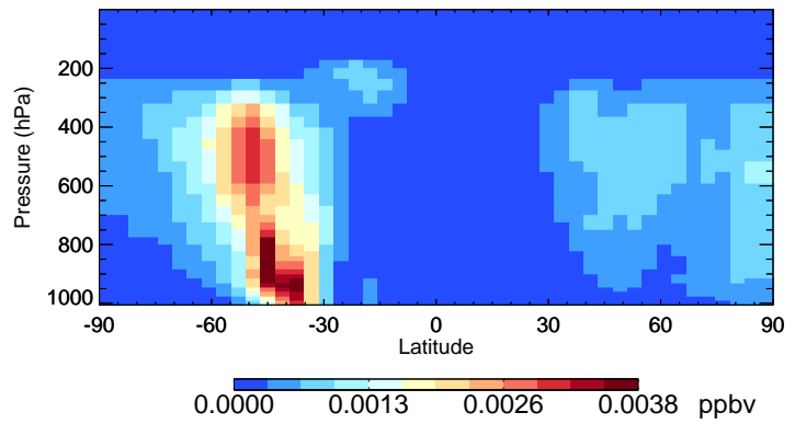
v11-02f-Run0 IMAE - Species Curtain @ -180.000 for Oct
