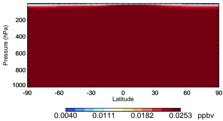
v11-02f-Run0 HCFC142b - Species Zonal Mean for Oct
