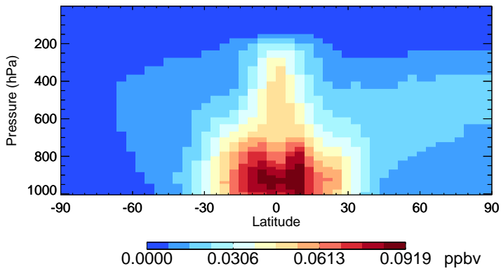
v11-02f-Run0 MAP - Species Zonal Mean for Oct
