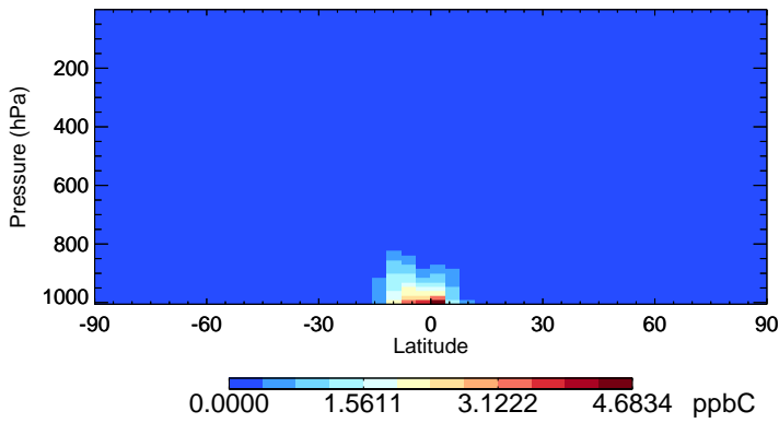
v11-02f-Run0 ISOP - Species Zonal Mean for Oct
