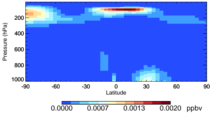
v11-02e-Run1 ASO3 - Species Zonal Mean for Oct
