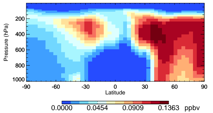
v11-02f-Run0 PAN - Species Curtain @ -180.000 for Oct
