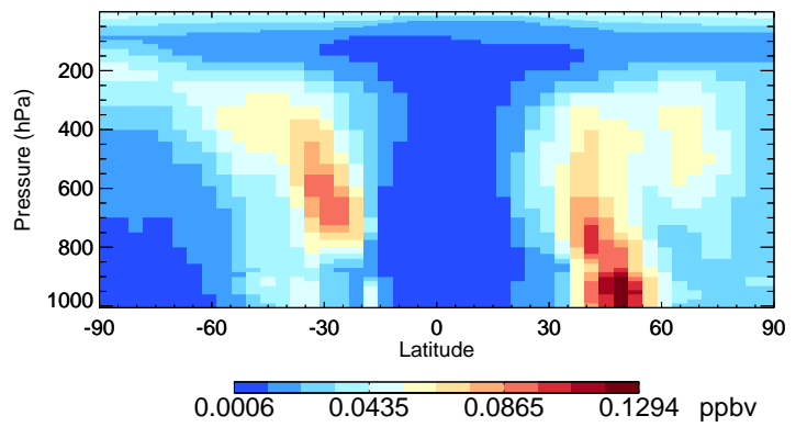
v11-02f-Run0 OCPI - Species Curtain @ -180.000 for Oct
