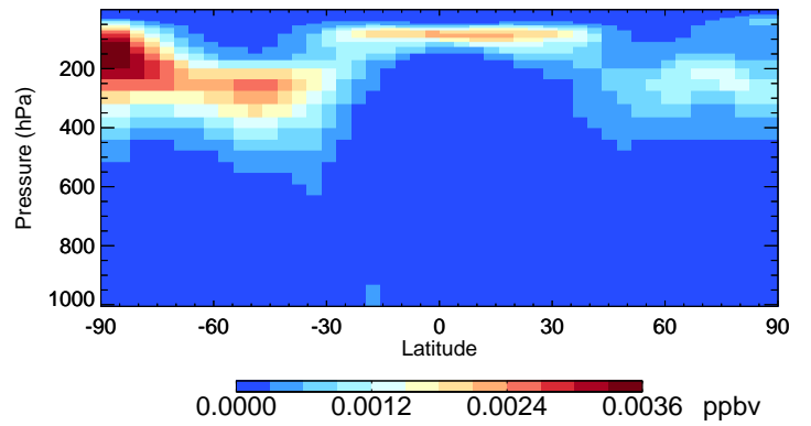
v11-02f-Run0 TSOA2 - Species Curtain @ -180.000 for Oct
