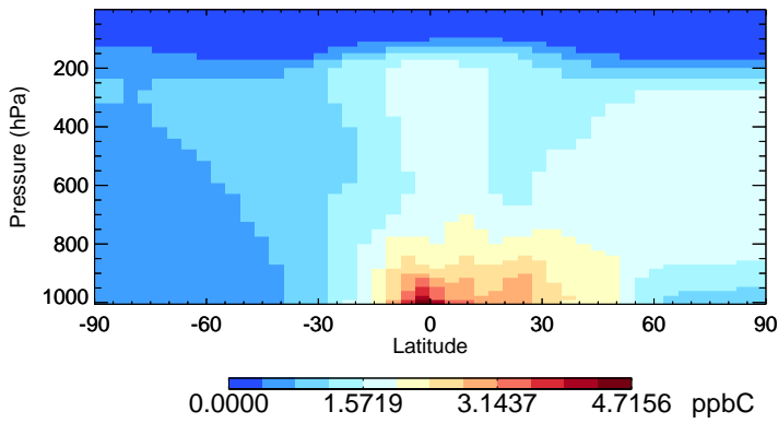
v11-02f-Run0 ACET - Species Zonal Mean for Oct
