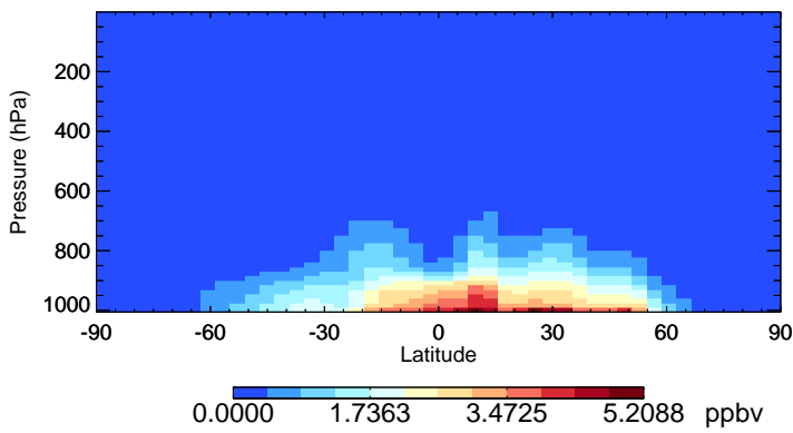
v11-02f-Run0 NH3 - Species Zonal Mean for Oct
