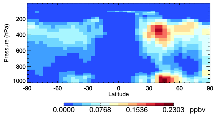
v11-02f-Run0 NIT - Species Curtain @ -180.000 for Oct
