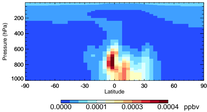
v11-02f-Run0 SOAME - Species Zonal Mean for Oct
