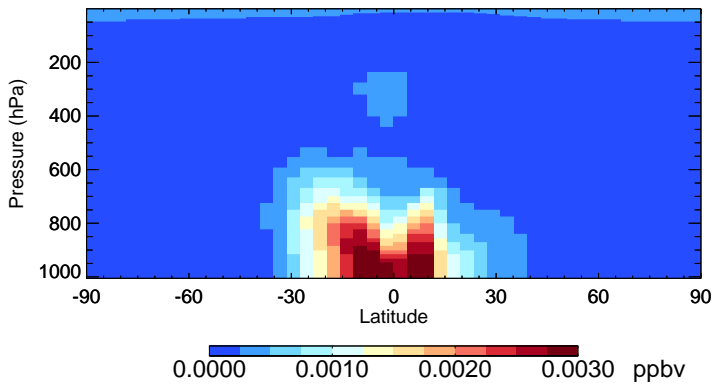
v11-02f-Run0 LVOCOA - Species Zonal Mean for Oct
