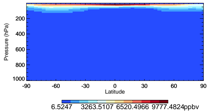
v11-02f-Run0 O3 - Species Curtain @ -180.000 for Oct
