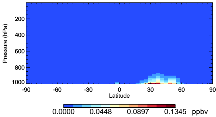
v11-02f-Run0 HNO 2 - Species Zonal Mean for Oct
