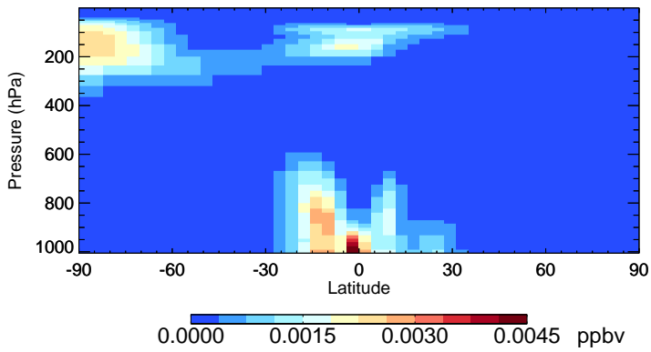
v11-02f-Run0 ISOA3 - Species Zonal Mean for Oct
