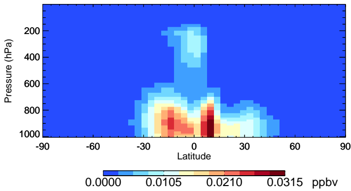
v11-02f-Run0 IMAE - Species Zonal Mean for Oct
