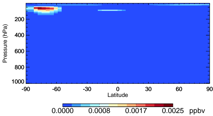
v11-02f-Run0 Cl2 - Species Zonal Mean for Oct
