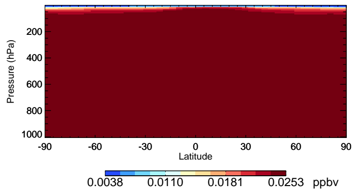
v11-02f-Run0 HCFC142b - Species Curtain @ -180.000 for Oct
