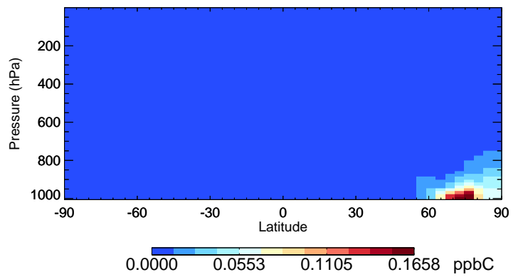
v11-02f-Run0 XYLE - Species Curtain @ -180.000 for Oct
