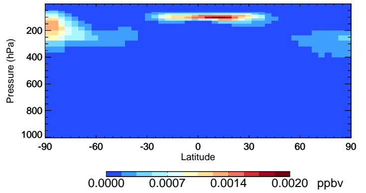
v11-02e-Run0 ASO3 - Species Curtain @ -180.000 for Oct
