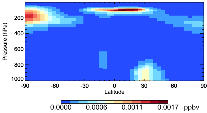
v11-02e-Run0 ASO3 - Species Zonal Mean for Oct
