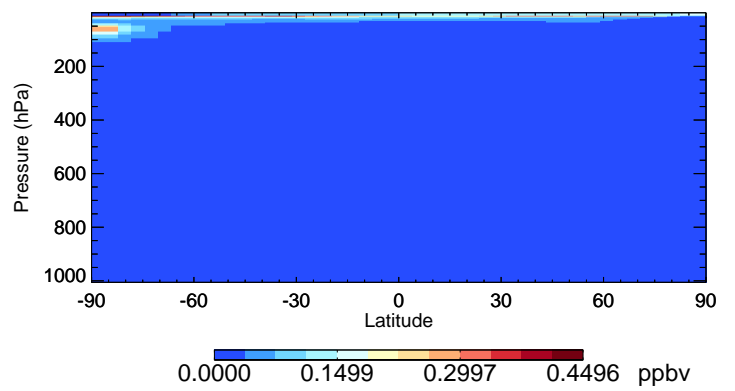
v11-02f-Run0 ClO - Species Curtain @ -180.000 for Oct
