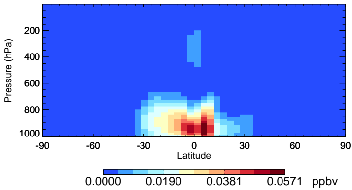
v11-02f-Run0 IEPOXA - Species Zonal Mean for Oct
