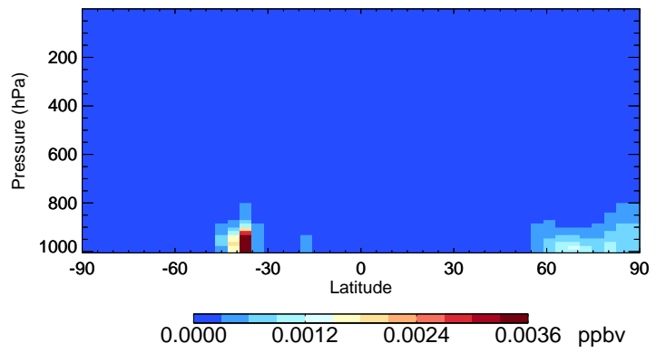
v11-02e-Run1 MACR - Species Curtain @ -180.000 for Oct
