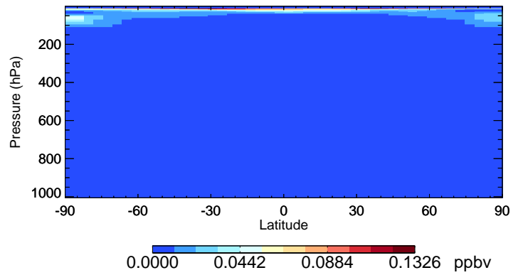
v11-02f-Run0 HOCl - Species Curtain @ -180.000 for Oct
