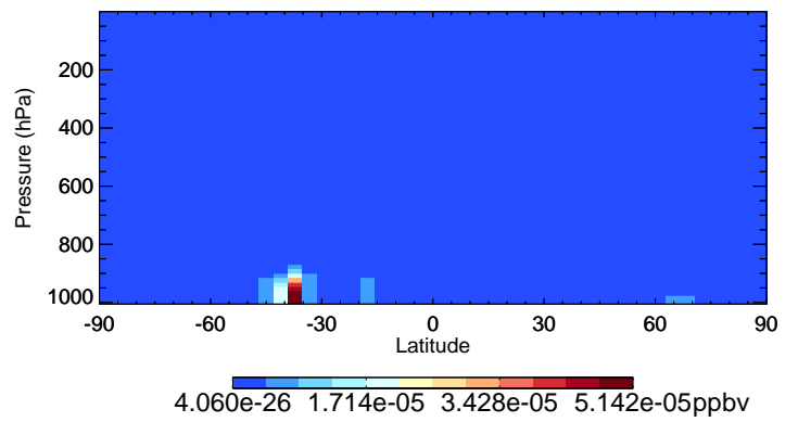
v11-02f-Run0 MOBA - Species Curtain @ -180.000 for Oct
