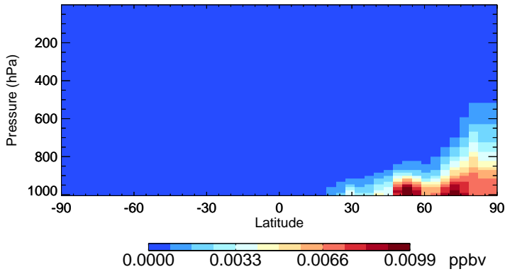
v11-02e-Run1 CINO2 - Species Zonal Mean for Oct
