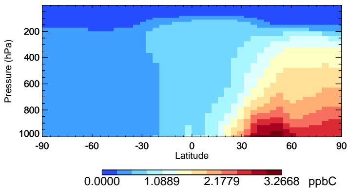
v11-02f-Run0 C2H6 - Species Zonal Mean for Oct
