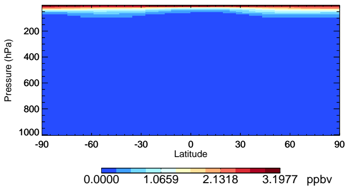
v11-02f-Run0 HCl - Species Zonal Mean for Oct
