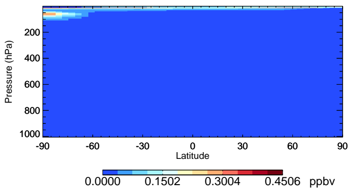
v11-02f-Run0 ClO - Species Zonal Mean for Oct
