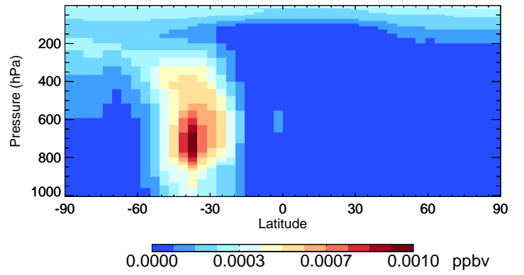
v11-02e-Run0 LVOCOA - Species Curtain @ -180.000 for Oct
