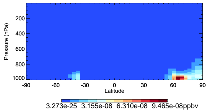
v11-02f-Run0 NPMN - Species Curtain @ -180.000 for Oct
