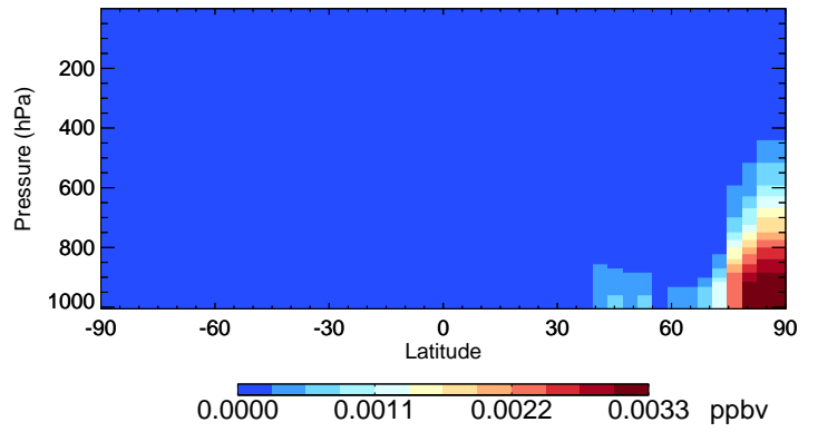
v11-02e-Run0 CINO2 - Species Curtain @ -180.000 for Oct
