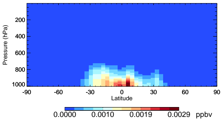
v11-02f-Run0 ISOPNB - Species Zonal Mean for Oct
