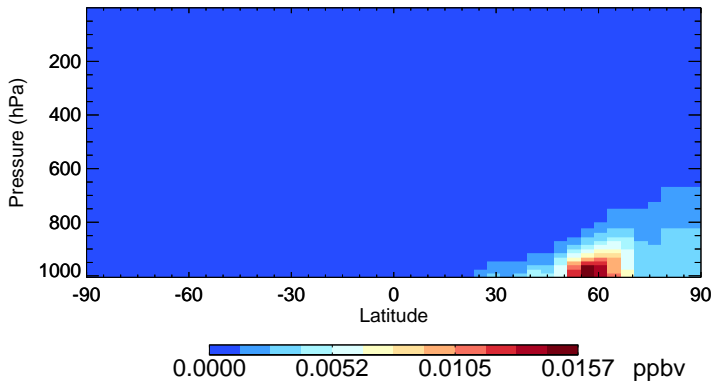
v11-02e-Run0 CINO2 - Species Zonal Mean for Oct
