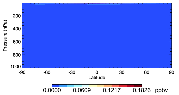
v11-02e-Run1 NO3 - Species Curtain @ -180.000 for Oct
