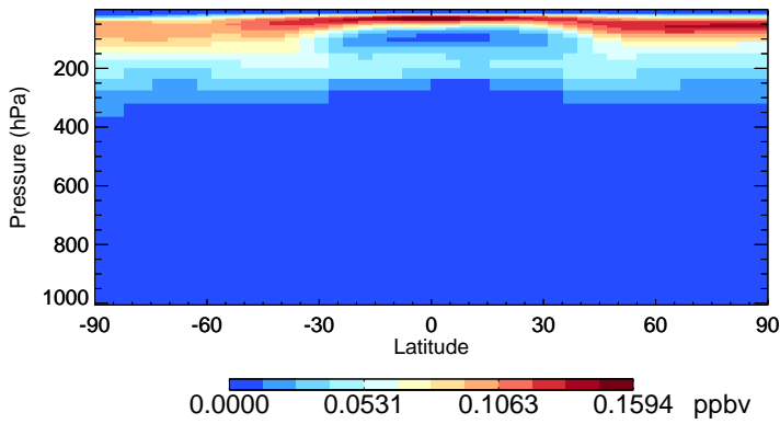
v11-02f-Run0 MPN - Species Zonal Mean for Oct
