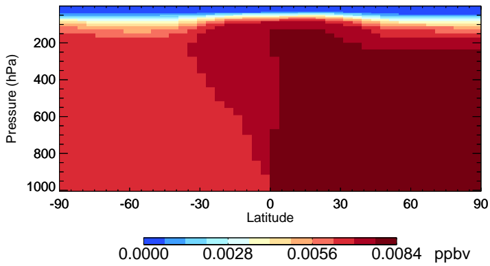
v11-02f-Run0 CH3Br - Species Zonal Mean for Oct
