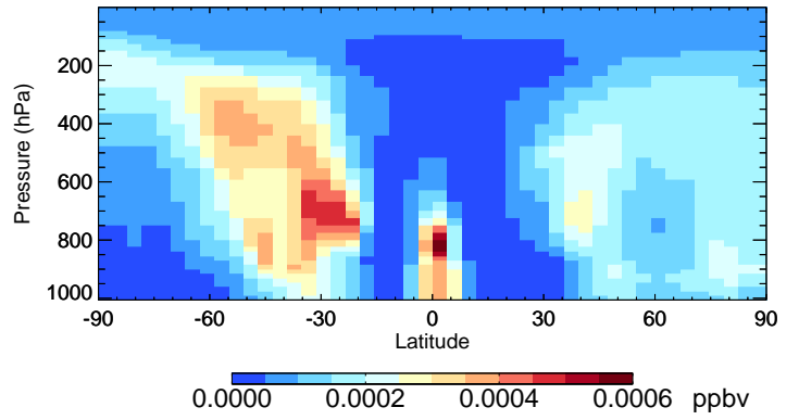
v11-02e-Run1 SOAME - Species Curtain @ -180.000 for Oct
