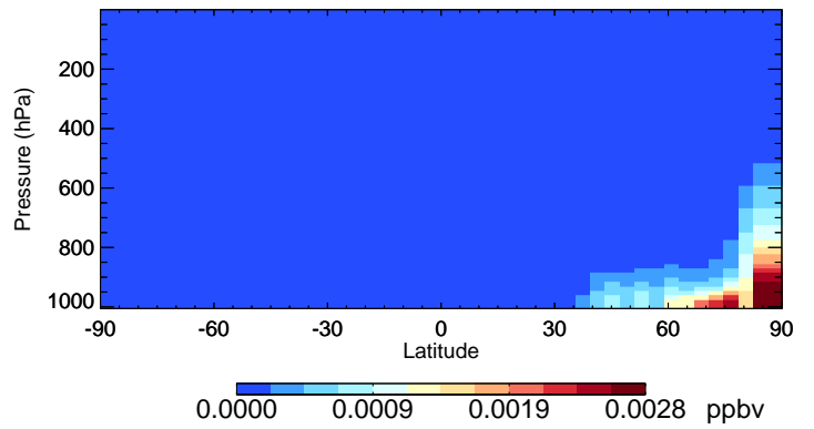
v11-02f-Run0 CINO2 - Species Curtain @ -180.000 for Oct
