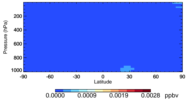
v11-02f-Run0 Br2 - Species Curtain @ -180.000 for Oct
