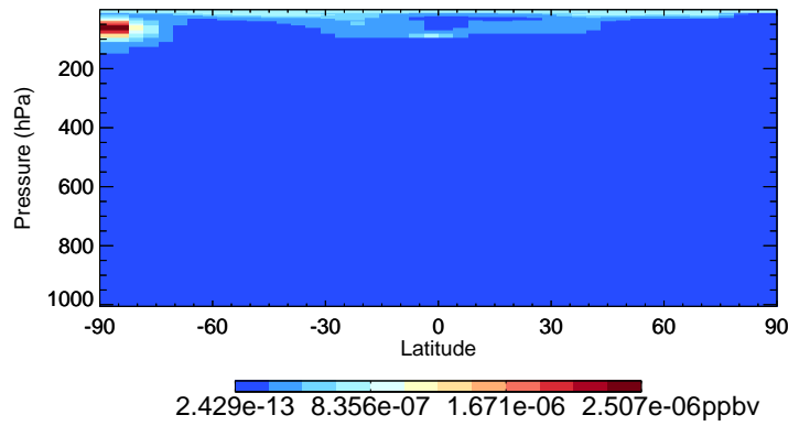
v11-02f-Run0 CIOO - Species Curtain @ -180.000 for Oct
