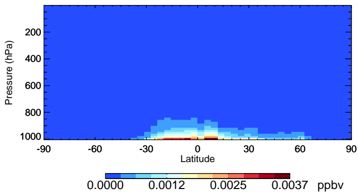
v11-02f-Run0 MONITS - Species Zonal Mean for Oct
