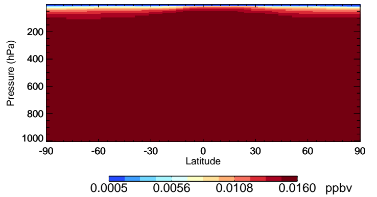
v11-02f-Run0 CFC114 - Species Curtain @ -180.000 for Oct
