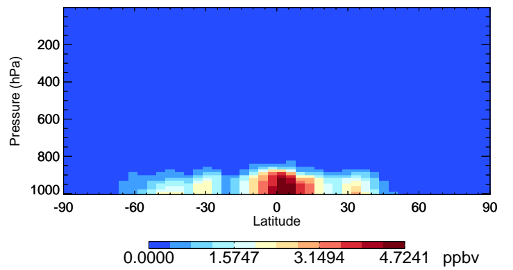
v11-02f-Run0 NH3 - Species Curtain @ -180.000 for Oct
