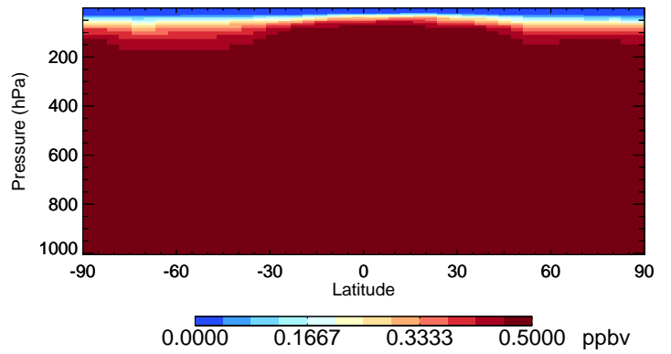
v11-02f-Run0 OCS - Species Curtain @ -180.000 for Oct
