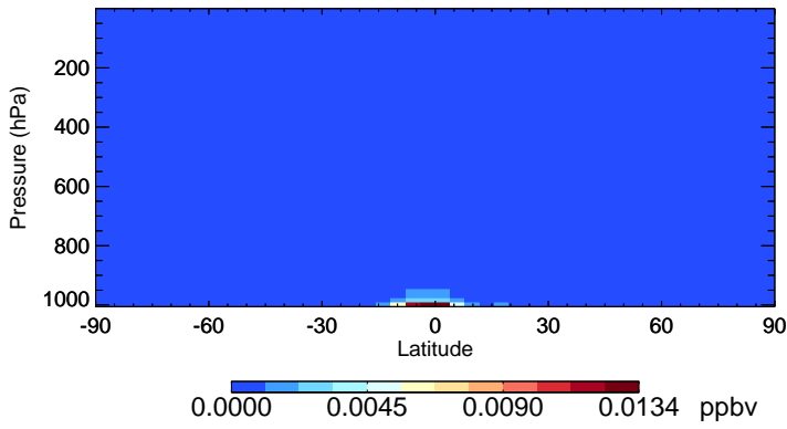
v11-02e-Run0 MTPO - Species Zonal Mean for Oct
