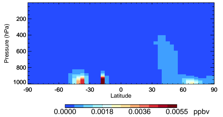
v11-02f-Run0 BCPO - Species Curtain @ -180.000 for Oct
