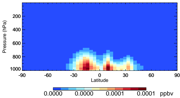
v11-02f-Run0 ETHLN - Species Zonal Mean for Oct
