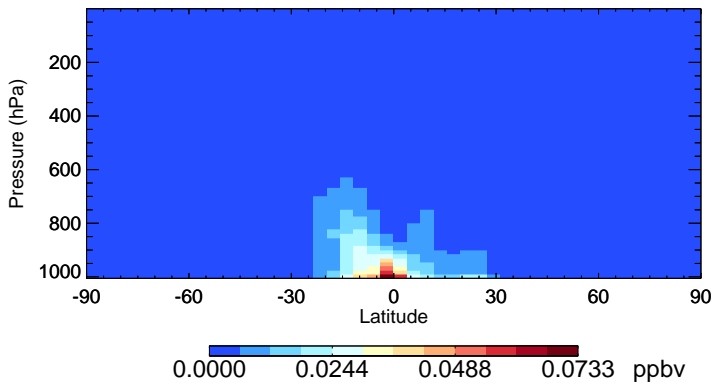
v11-02f-Run0 TSOA2 - Species Zonal Mean for Oct
