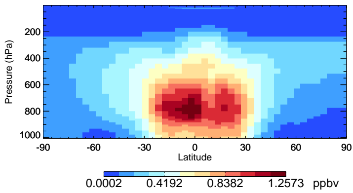
v11-02f-Run0 H2O2 - Species Zonal Mean for Oct
