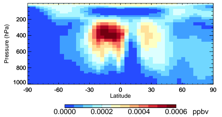
v11-02f-Run0 ASOG1 - Species Curtain @ -180.000 for Oct
