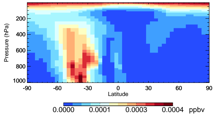
v11-02f-Run0 LVOCOA - Species Curtain @ -180.000 for Oct
