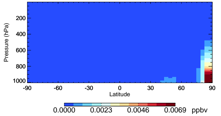
v11-02e-Run1 CINO2 - Species Curtain @ -180.000 for Oct
