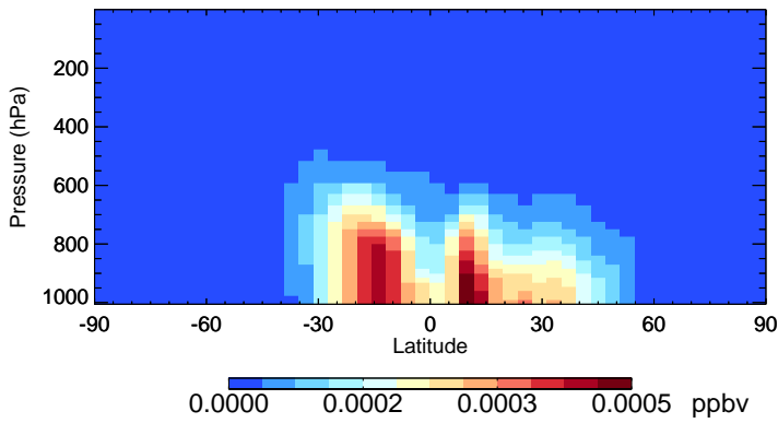
v11-02f-Run0 ISN10A - Species Zonal Mean for Oct
