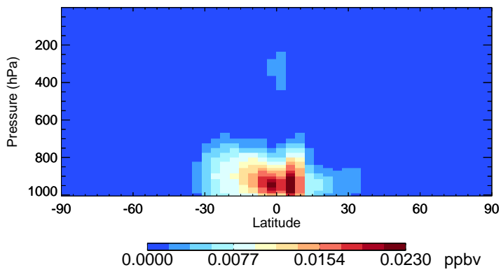
v11-02f-Run0 IEPOXB - Species Zonal Mean for Oct
