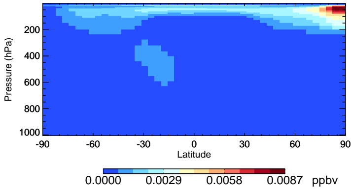
v11-02e-Run1 HOBr - Species Zonal Mean for Oct
