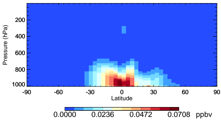
v11-02f-Run0 GLYC - Species Zonal Mean for Oct
