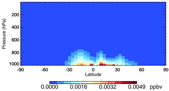
v11-02f-Run0 ISN1 - Species Zonal Mean for Oct
