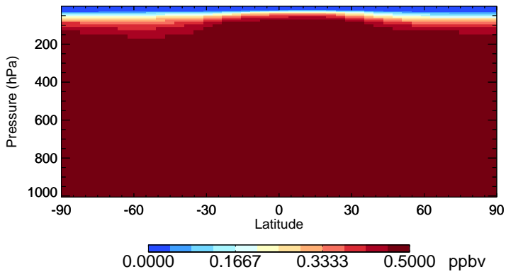
v11-02f-Run0 OCS - Species Zonal Mean for Oct
