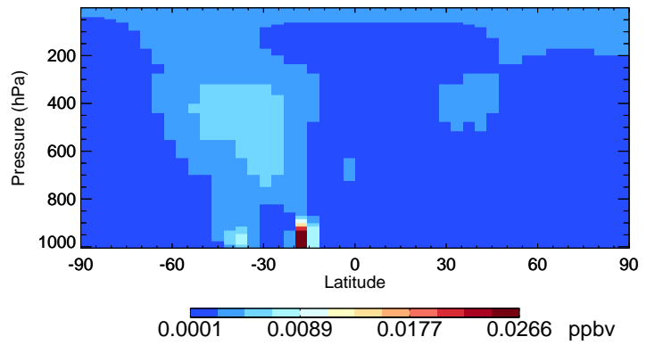
v11-02f-Run0 TSOG2 - Species Curtain @ -180.000 for Oct
