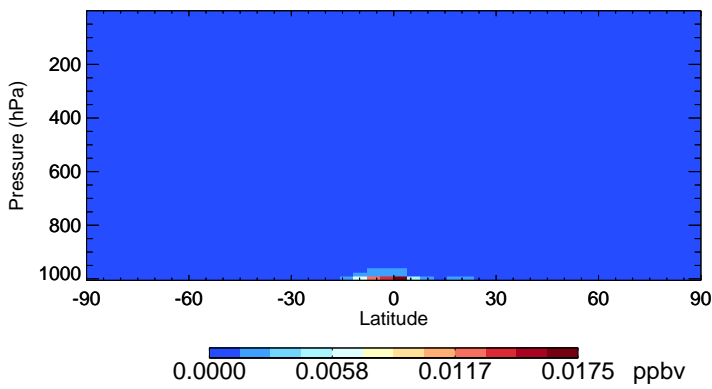
v11-02f-Run0 MTPO - Species Zonal Mean for Oct
