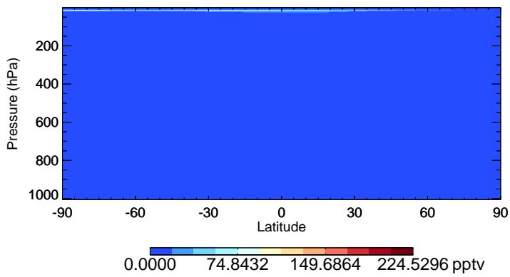
v11-02f-Run0 HO2 - Species Zonal Mean for Oct
