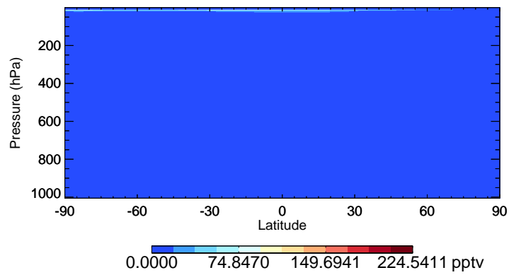
v11-02f-Run0 HO2 - Species Curtain @ -180.000 for Oct
