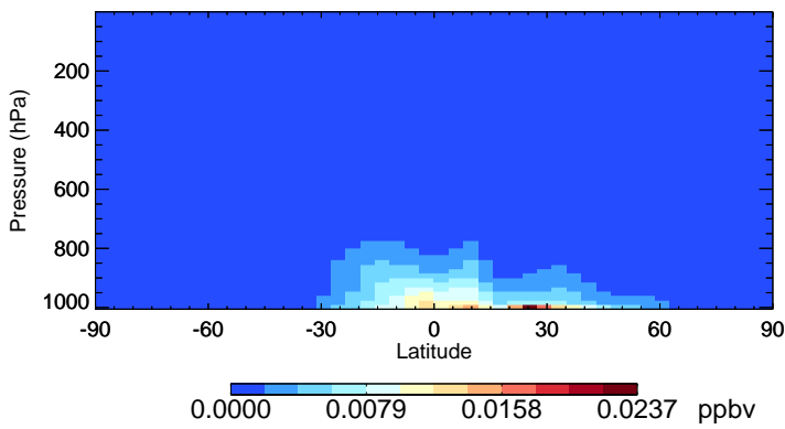
v11-02f-Run0 GLYX - Species Zonal Mean for Oct
