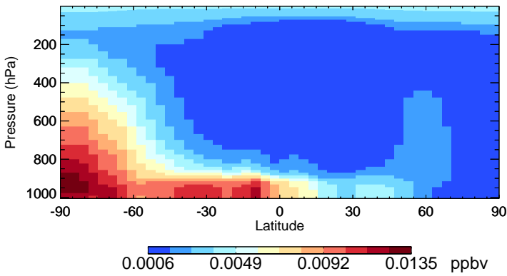
v11-02f-Run0 MSA - Species Zonal Mean for Oct
