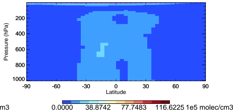
v11-02f-Run0 OH - Species Curtain @ -180.000 for Oct
