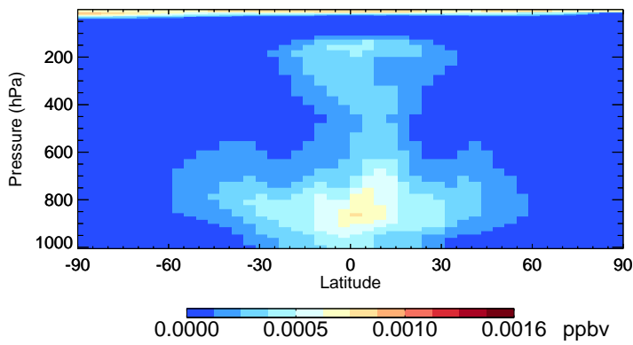
v11-02f-Run0 HBr - Species Zonal Mean for Oct
