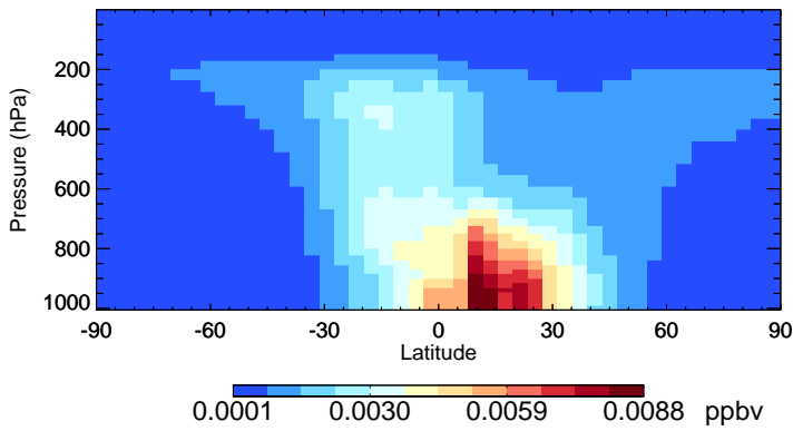
v11-02f-Run0 ASOAN - Species Zonal Mean for Oct
