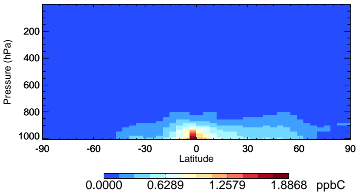
v11-02f-Run0 ALD2 - Species Zonal Mean for Oct
