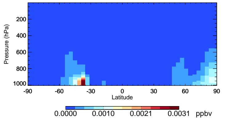
v11-02f-Run0 IPMN - Species Curtain @ -180.000 for Oct
