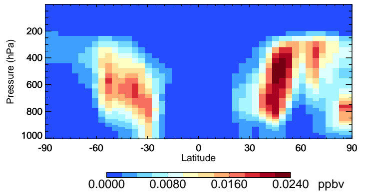
v11-02f-Run0 DST2 - Species Curtain @ -180.000 for Oct
