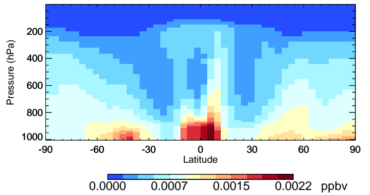
v11-02f-Run0 CHBr3 - Species Curtain @ -180.000 for Oct
