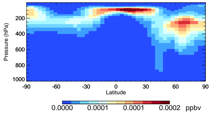
v11-02f-Run0 ASOA2 - Species Curtain @ -180.000 for Oct
