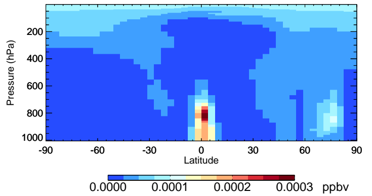
v11-02f-Run0 SOAME - Species Curtain @ -180.000 for Oct
