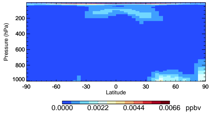
v11-02f-Run0 HNO 2 - Species Curtain @ -180.000 for Oct
