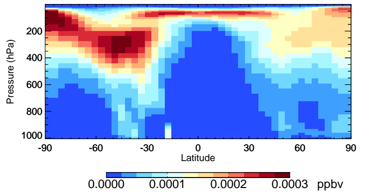
v11-02f-Run0 TSOA1 - Species Curtain @ -180.000 for Oct
