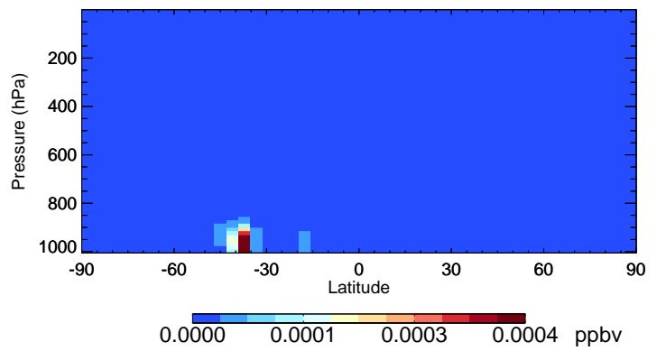
v11-02f-Run0 ISOPNB - Species Curtain @ -180.000 for Oct
