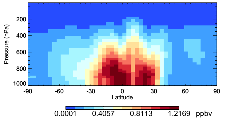
v11-02f-Run0 MP - Species Curtain @ -180.000 for Oct
