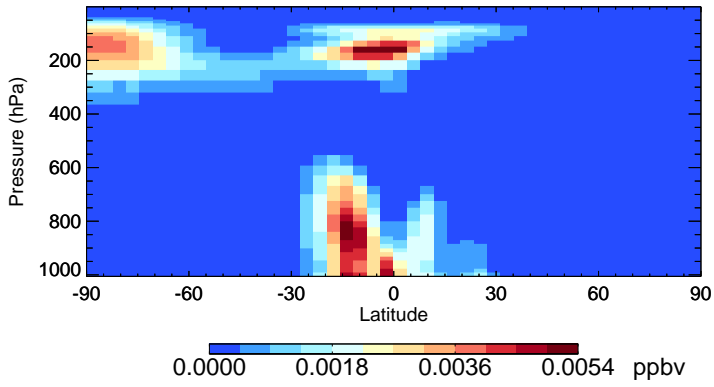
v11-02e-Run1 ISOA3 - Species Zonal Mean for Oct
