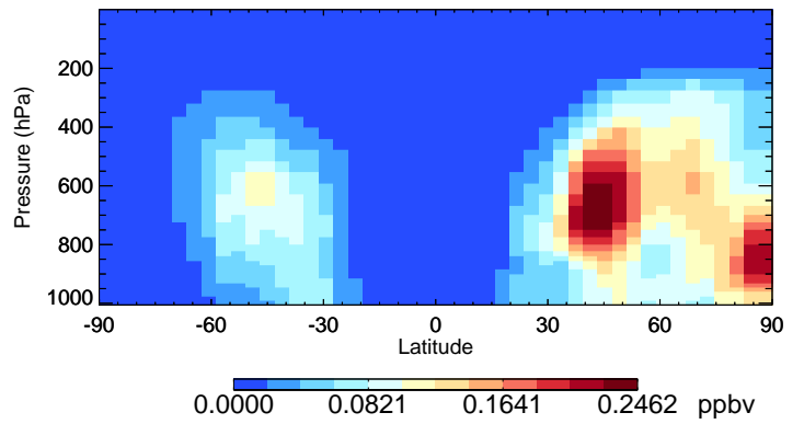
v11-02f-Run0 DST1 - Species Curtain @ -180.000 for Oct
