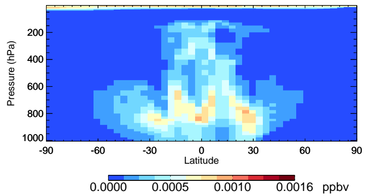
v11-02f-Run0 HBr - Species Curtain @ -180.000 for Oct
