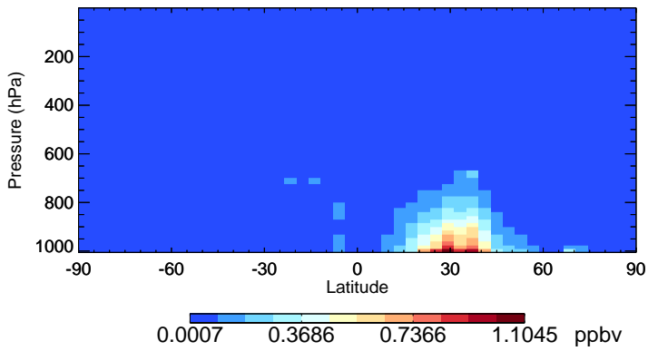
v11-02f-Run0 SO2 - Species Zonal Mean for Oct
