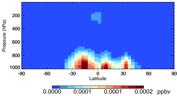
v11-02f-Run0 MACRN - Species Zonal Mean for Oct
