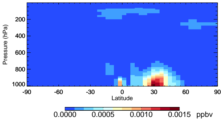
v11-02f-Run0 ASOA2 - Species Zonal Mean for Oct
