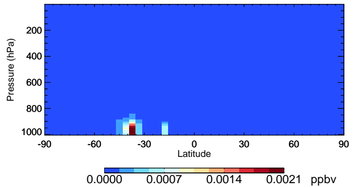
v11-02f-Run0 RIPA - Species Curtain @ -180.000 for Oct
