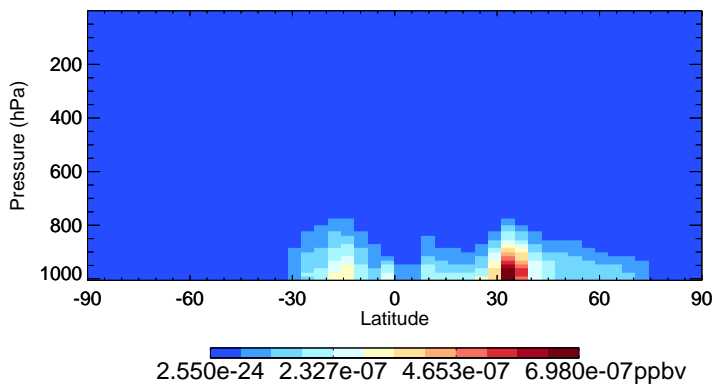
v11-02f-Run0 NPMN - Species Zonal Mean for Oct
