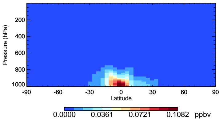
v11-02f-Run0 MACR - Species Zonal Mean for Oct
