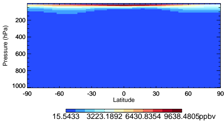
v11-02f-Run0 O3 - Species Zonal Mean for Oct
