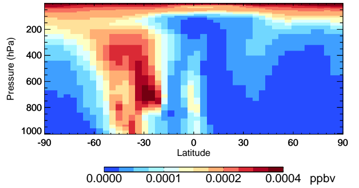
v11-02e-Run1 LVOCOA - Species Curtain @ -180.000 for Oct
