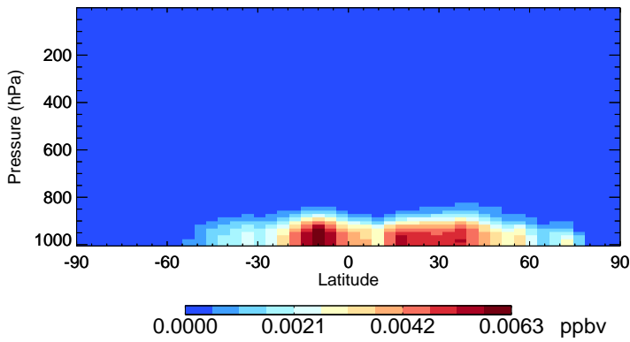
v11-02f-Run0 NITs - Species Zonal Mean for Oct
