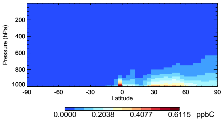
v11-02f-Run0 TOLU - Species Zonal Mean for Oct
