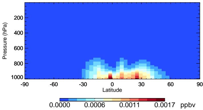
v11-02f-Run0 IONITA - Species Zonal Mean for Oct
