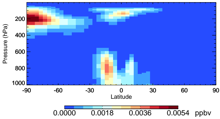
v11-02e-Run0 ISOA3 - Species Zonal Mean for Oct
