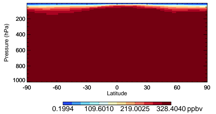
v11-02f-Run0 N2O - Species Curtain @ -180.000 for Oct
