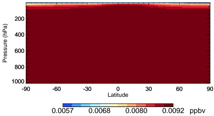
v11-02f-Run0 CFC115 - Species Zonal Mean for Oct
