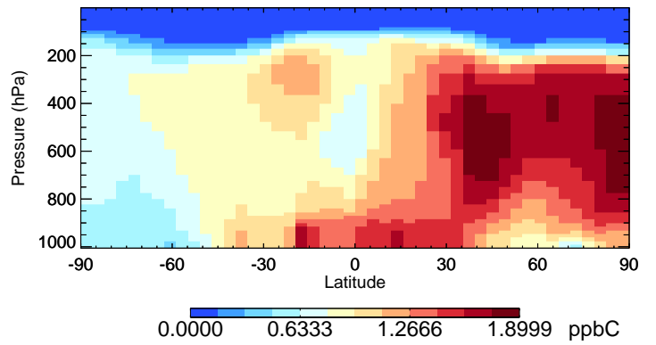
v11-02f-Run0 ACET - Species Curtain @ -180.000 for Oct
