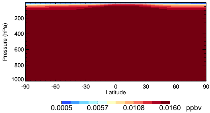
v11-02f-Run0 CFC114 - Species Zonal Mean for Oct
