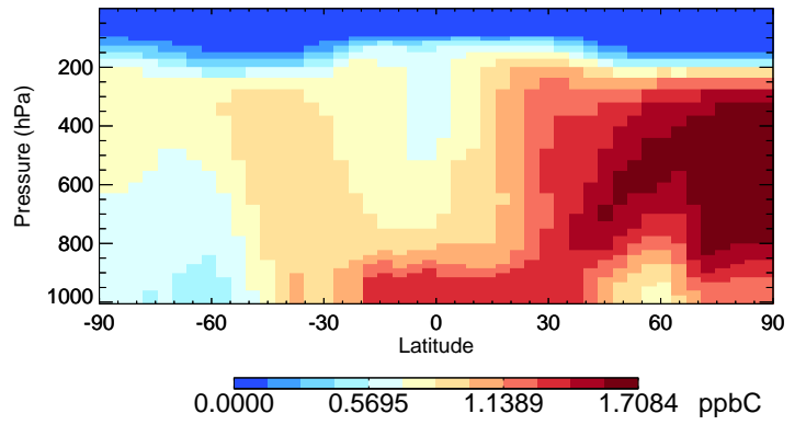
v11-02e-Run0 ACET - Species Curtain @ -180.000 for Oct
