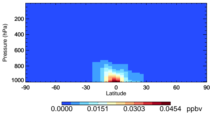
v11-02f-Run0 TSOA0 - Species Zonal Mean for Oct
