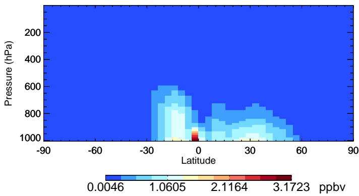
v11-02f-Run0 OCPI - Species Zonal Mean for Oct
