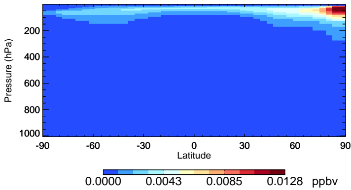
v11-02f-Run0 BrCl - Species Zonal Mean for Oct
