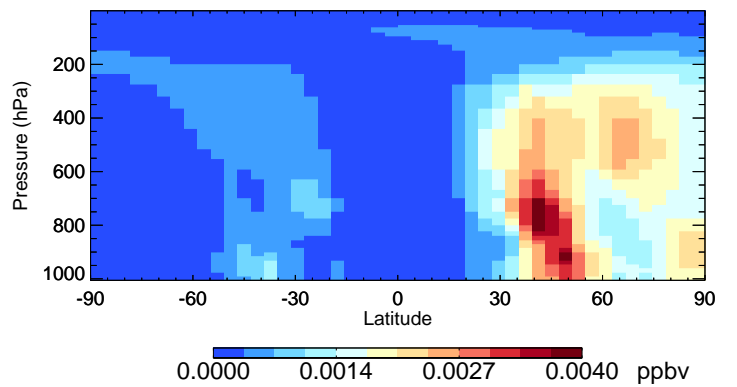
v11-02f-Run0 SOAGX - Species Curtain @ -180.000 for Oct
