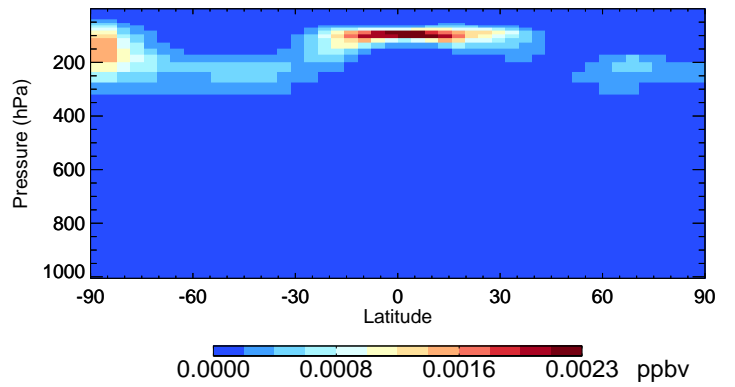
v11-02f-Run0 ASO3 - Species Curtain @ -180.000 for Oct
