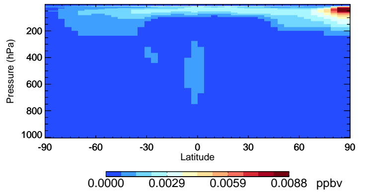
v11-02f-Run0 HOBr - Species Curtain @ -180.000 for Oct
