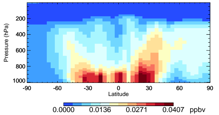
v11-02f-Run0 MAP - Species Curtain @ -180.000 for Oct
