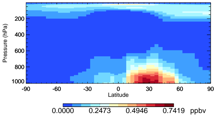
v11-02f-Run0 SO4 - Species Zonal Mean for Oct
