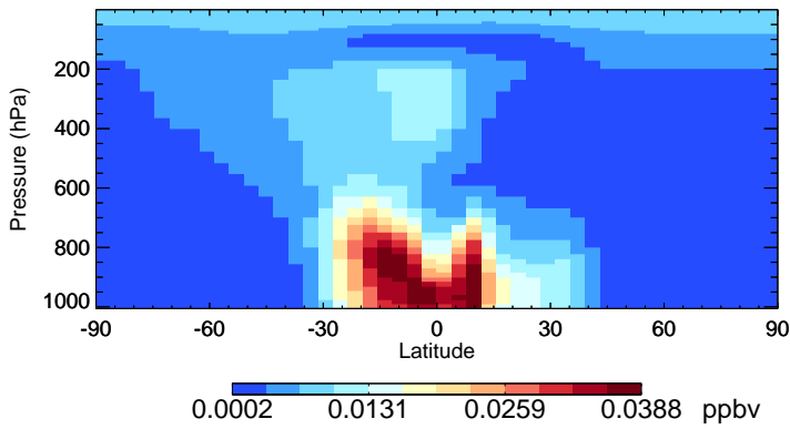
v11-02f-Run0 ISOG3 - Species Zonal Mean for Oct
