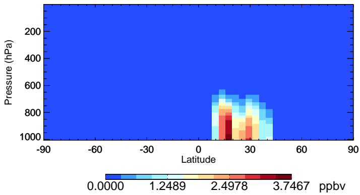
v11-02f-Run0 DST4 - Species Zonal Mean for Oct
