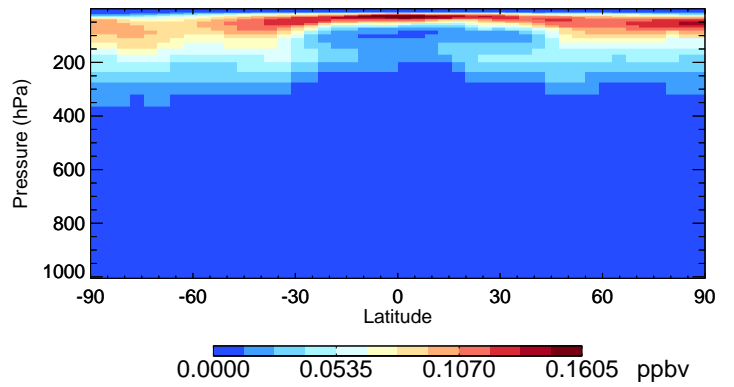
v11-02f-Run0 MPN - Species Curtain @ -180.000 for Oct
