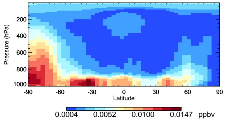
v11-02f-Run0 MSA - Species Curtain @ -180.000 for Oct
