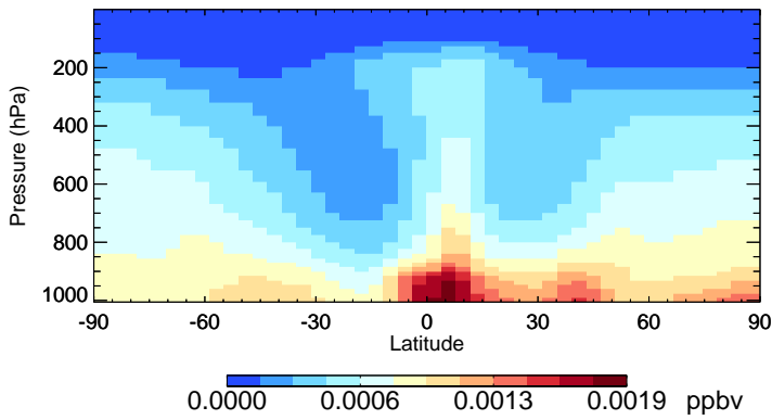
v11-02f-Run0 CHBr3 - Species Zonal Mean for Oct
