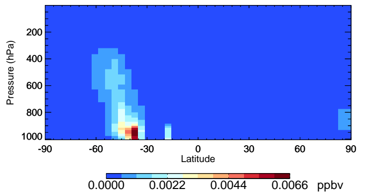
v11-02f-Run0 GLYC - Species Curtain @ -180.000 for Oct
