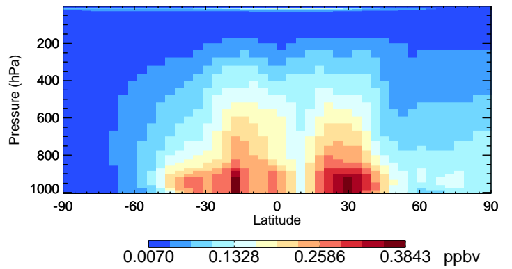
v11-02f-Run0 CH2O - Species Curtain @ -180.000 for Oct
