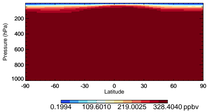
v11-02f-Run0 N2O - Species Zonal Mean for Oct
