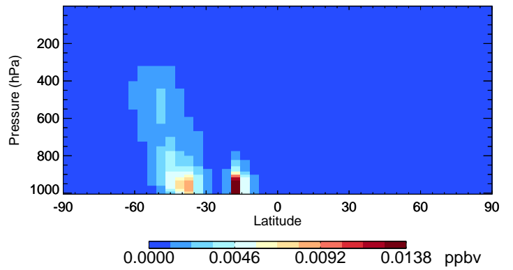
v11-02f-Run0 HAC - Species Curtain @ -180.000 for Oct
