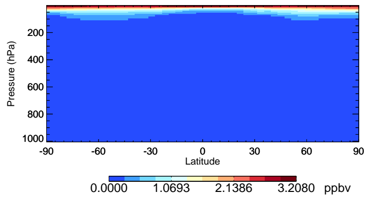
v11-02f-Run0 HCl - Species Curtain @ -180.000 for Oct
