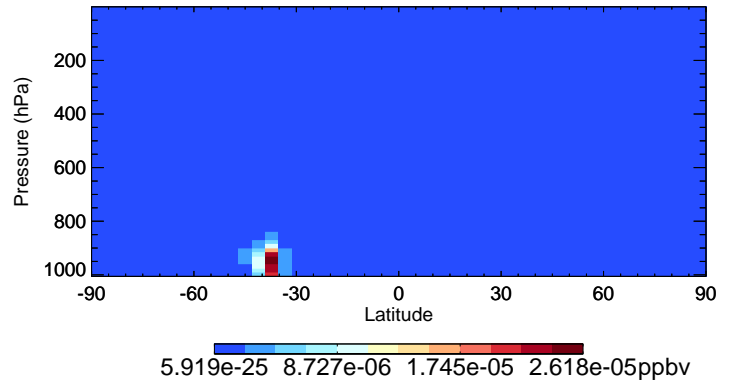
v11-02e-Run1 MACRN - Species Curtain @ -180.000 for Oct
