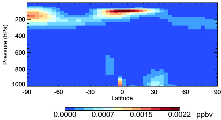
v11-02f-Run0 ASO3 - Species Zonal Mean for Oct
