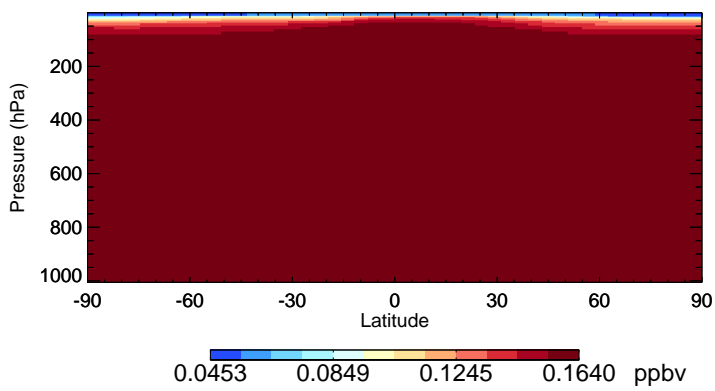
v11-02f-Run0 HCFC22 - Species Zonal Mean for Oct
