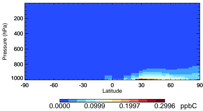
v11-02f-Run0 XYLE - Species Zonal Mean for Oct
