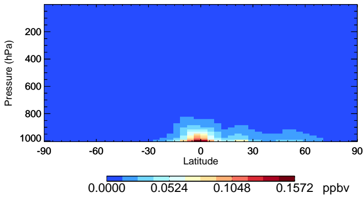
v11-02f-Run0 RCHO - Species Zonal Mean for Oct
