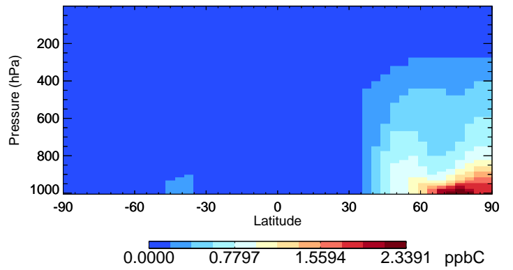
v11-02f-Run0 ALK4 - Species Curtain @ -180.000 for Oct
