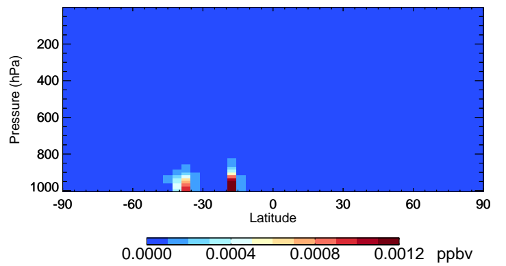
v11-02f-Run0 MONITS - Species Curtain @ -180.000 for Oct
