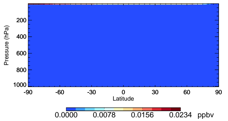
v11-02e-Run1 Br - Species Curtain @ -180.000 for Oct
