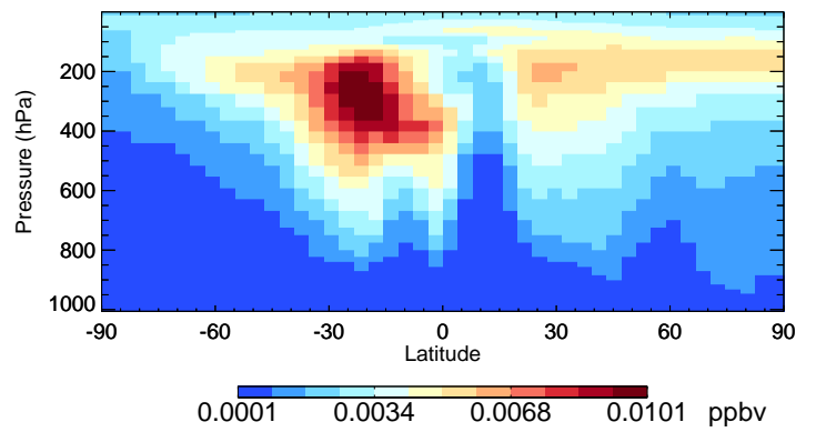
v11-02f-Run0 ASOG3 - Species Curtain @ -180.000 for Oct
