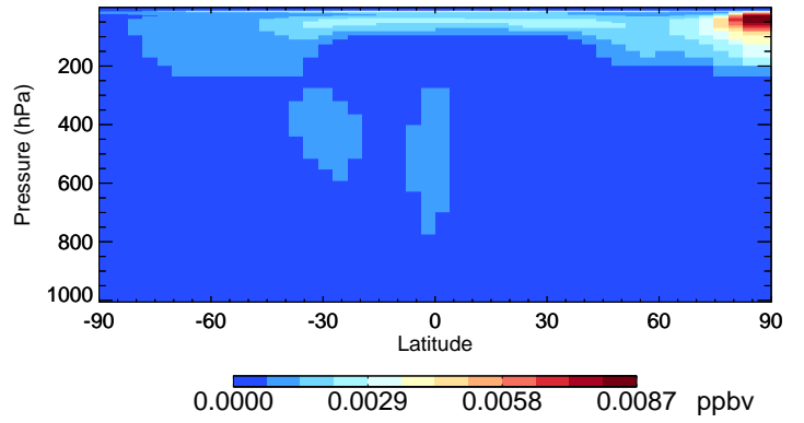
v11-02e-Run1 HOBr - Species Curtain @ -180.000 for Oct
