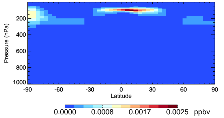
v11-02e-Run1 ASO3 - Species Curtain @ -180.000 for Oct
