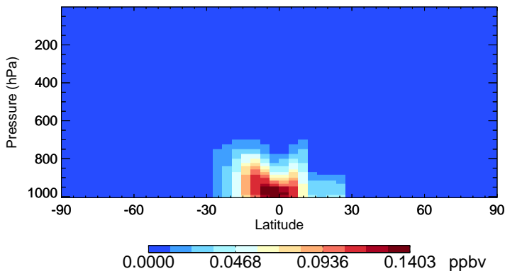
v11-02e-Run1 MACR - Species Zonal Mean for Oct
