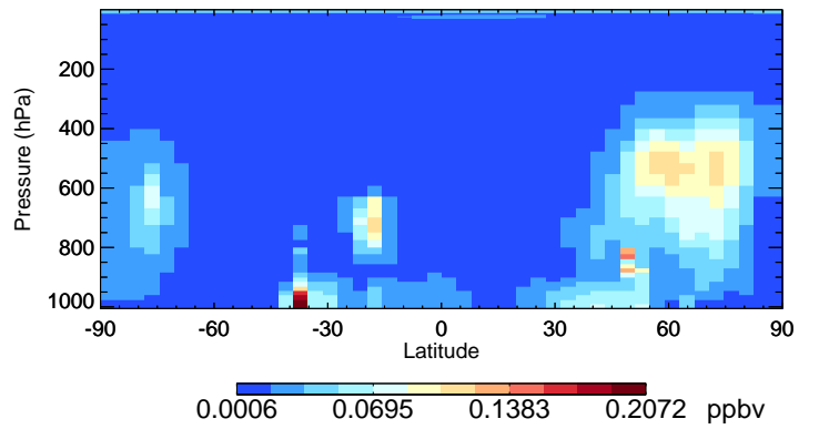
v11-02f-Run0 SO2 - Species Curtain @ -180.000 for Oct
