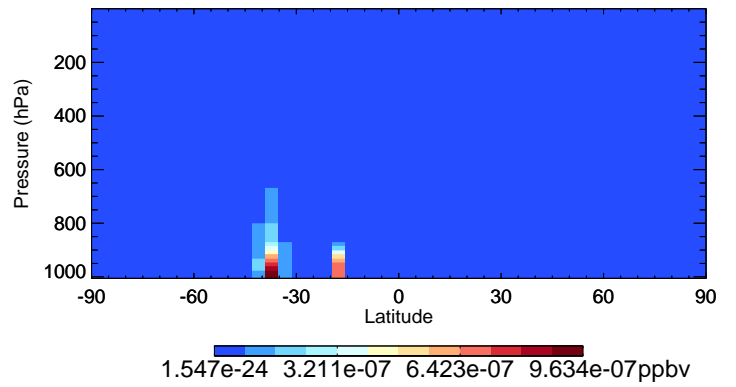
v11-02f-Run0 LVOC - Species Curtain @ -180.000 for Oct
