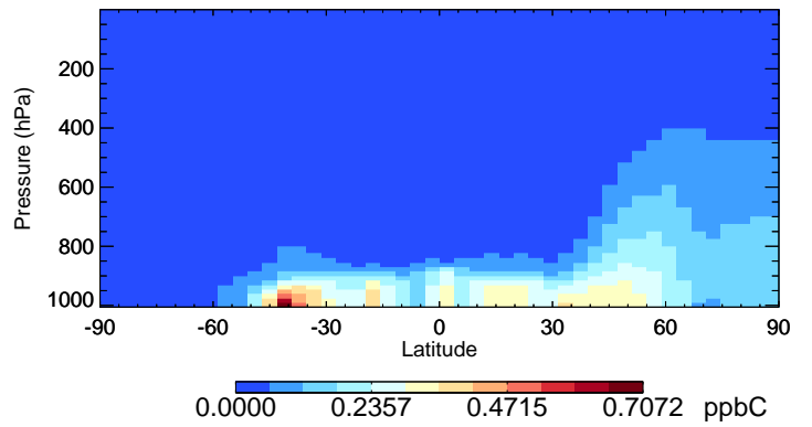
v11-02f-Run0 ALD2 - Species Curtain @ -180.000 for Oct
