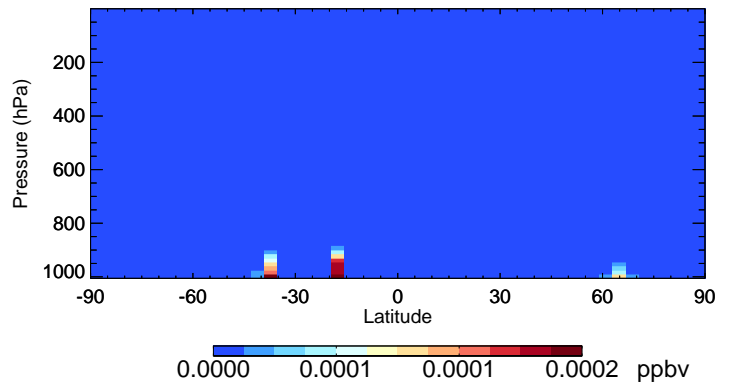
v11-02f-Run0 LIMO - Species Curtain @ -180.000 for Oct
