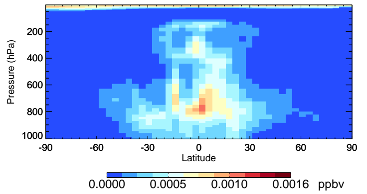
v11-02e-Run0 HBr - Species Curtain @ -180.000 for Oct
