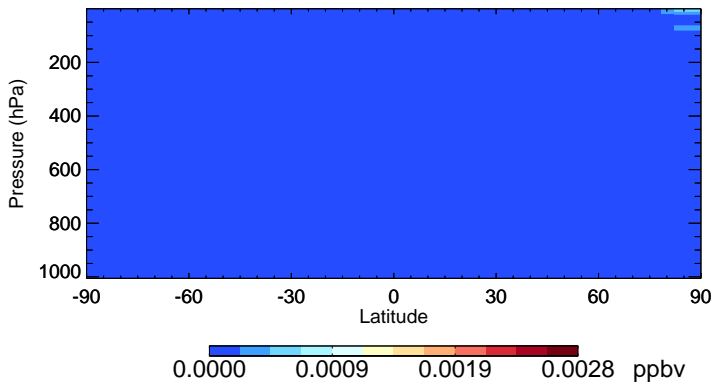
v11-02f-Run0 Br2 - Species Zonal Mean for Oct
