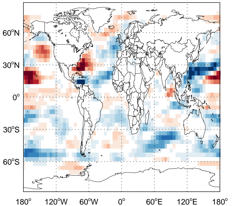
v11-02f-Run1 - v11-02e-Run0 SALC: Column AOD diff for Oct
