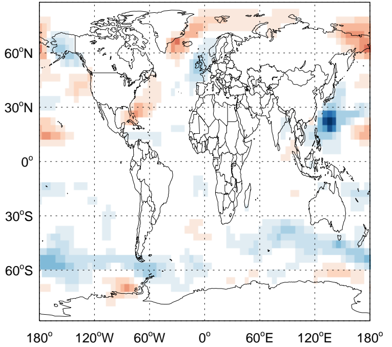
v11-02f-Run1 - v11-02e-Run0 SALA: Column AOD diff for Oct
