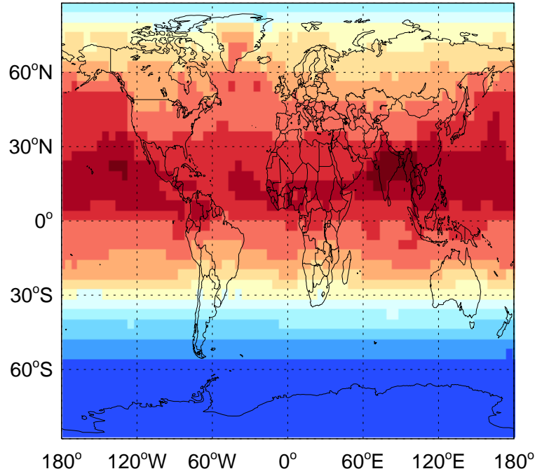
JGLYC - J-Value @ 500 hPa for Jul
