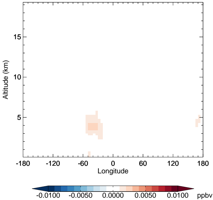
v11-02f-Run1 - v11-02e-Run0 NO3 - Diff along 15S for Apr
