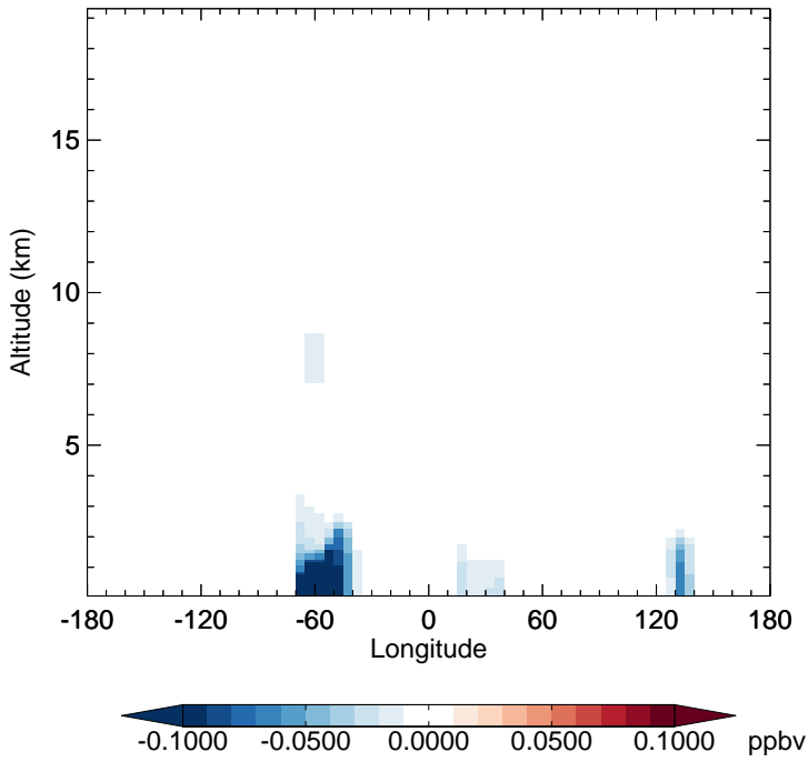
v11-02f-Run1 - v11-02e-Run1 HPALD - Diff along 15S for Apr
