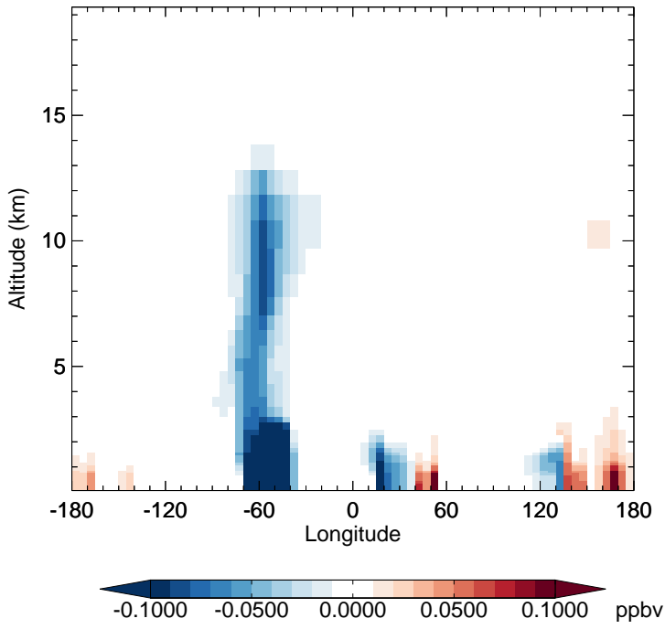
v11-02f-Run1 - v11-02e-Run1 EOH - Diff along 15S for Apr
