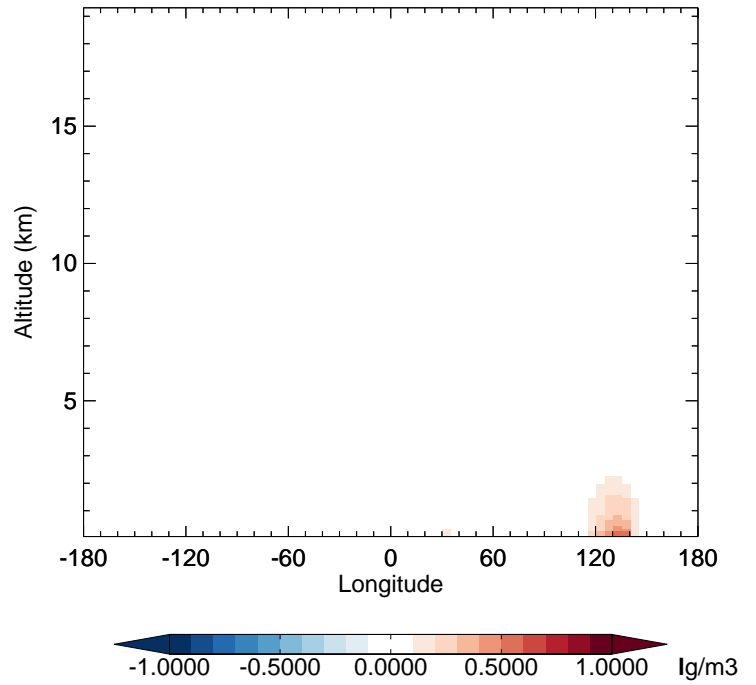
v11-02f-Run1 - v11-02e-Run0 OCPO - Diff along 42N for Apr
