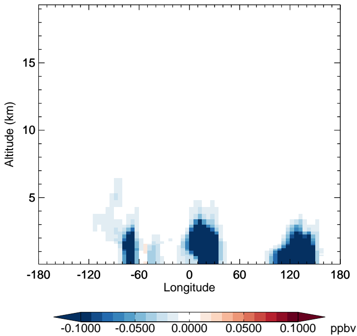
v11-02f-Run1 - v11-02e-Run0 SOAIE - Diff along 15S for Apr
