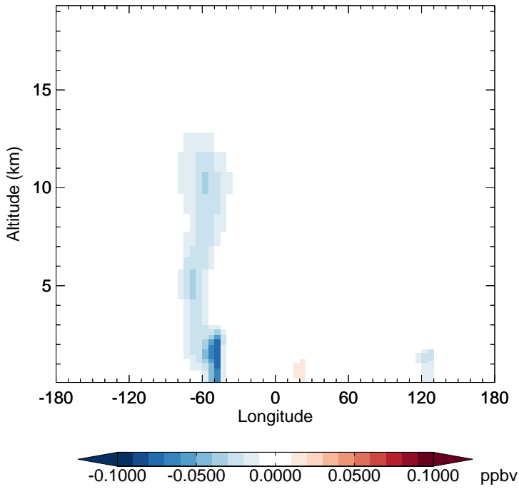
v11-02f-Run1 - v11-02e-Run1 HC187 - Diff along 15S for Apr
