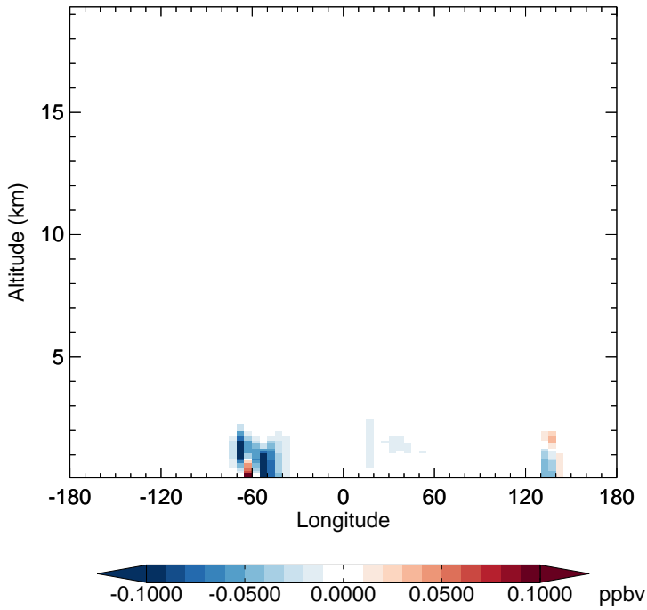
v11-02f-Run1 - v11-02e-Run0 HPALD - Diff along 15S for Apr
