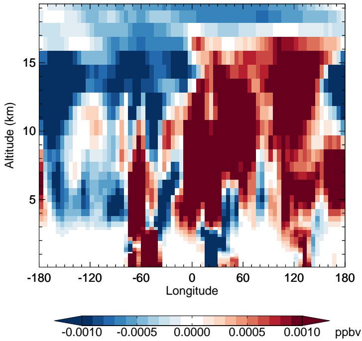
v11-02f-Run1 - v11-02e-Run0 PPN - Diff along 15S for Apr
