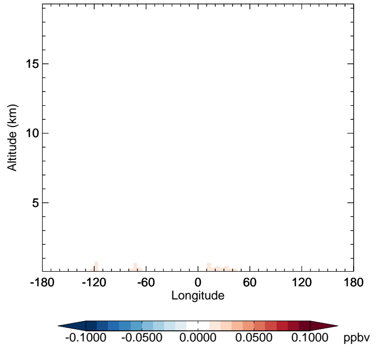
v11-02f-Run1 - v11-02e-Run1 TSOG3 - Diff along 42N for Apr
