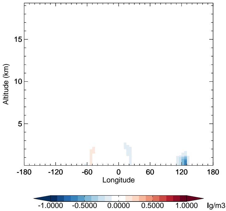
v11-02f-Run1 - v11-02e-Run0 OCPI - Diff along 15S for Apr
