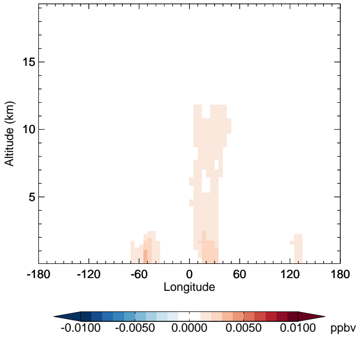
v11-02f-Run1 - v11-02e-Run1 R4N2 - Diff along 15S for Apr
