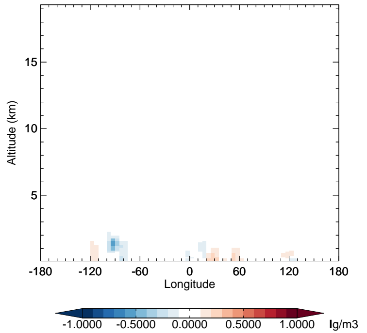
v11-02f-Run1 - v11-02e-Run0 NH3 - Diff along 42N for Apr
