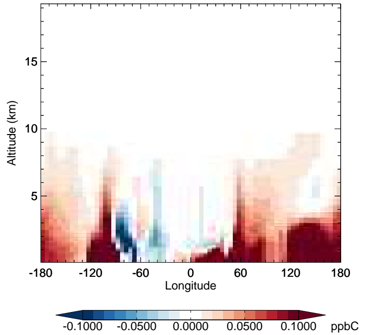
v11-02f-Run1 - v11-02e-Run0 MEK - Diff along 42N for Apr
