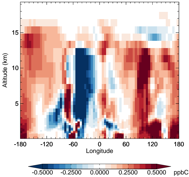
v11-02f-Run1 - v11-02e-Run0 ACET - Diff along 15S for Apr
