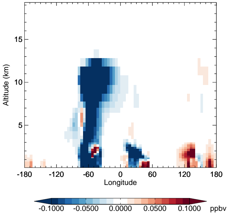
v11-02f-Run1 - v11-02e-Run0 EOH - Diff along 15S for Apr
