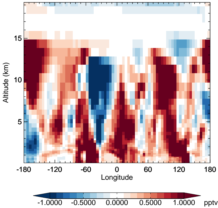
v11-02f-Run1 - v11-02e-Run0 HO2 - Diff along 15S for Apr
