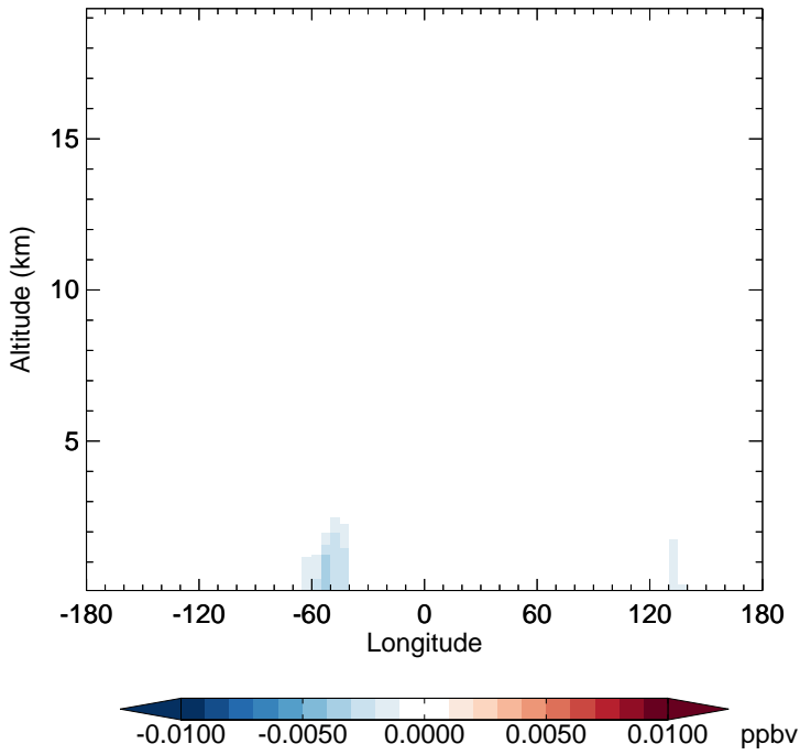
v11-02f-Run1 - v11-02e-Run1 MOBA - Diff along 15S for Apr
