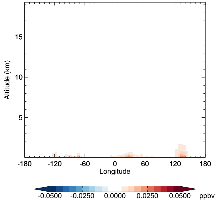
v11-02f-Run1 - v11-02e-Run0 RCHO - Diff along 42N for Apr
