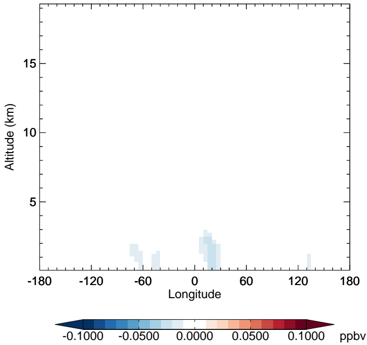
v11-02f-Run1 - v11-02e-Run0 SOAGX - Diff along 15S for Apr
