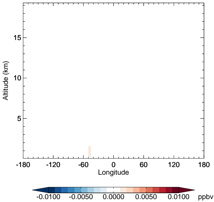
v11-02f-Run1 - v11-02e-Run0 MACRN - Diff along 15S for Apr
