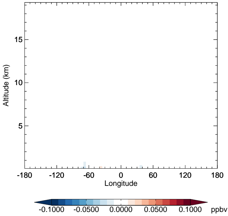
v11-02f-Run1 - v11-02e-Run1 XYLE - Diff along 15S for Apr
