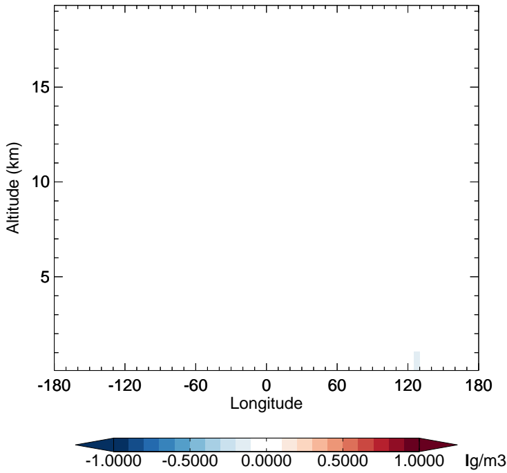
v11-02f-Run1 - v11-02e-Run0 OCPO - Diff along 15S for Apr
