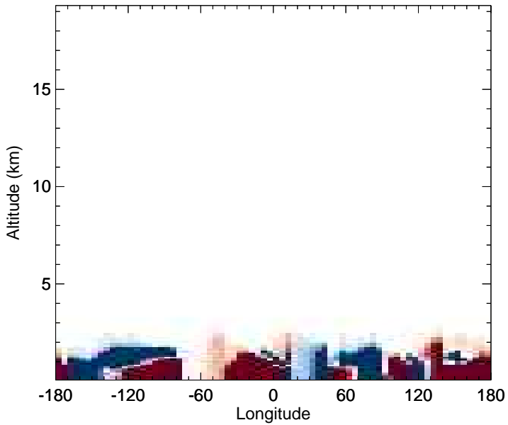
v11-02f-Run1 - v11-02e-Run0 SALC - Diff along 15S for Apr
