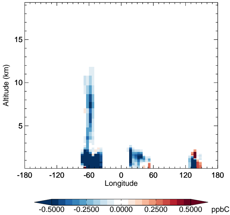
v11-02f-Run1 - v11-02e-Run0 ISOP - Diff along 15S for Apr
