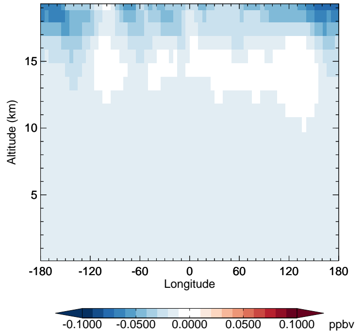
v11-02f-Run1 - v11-02e-Run0 CFC12 - Diff along 42N for Apr
