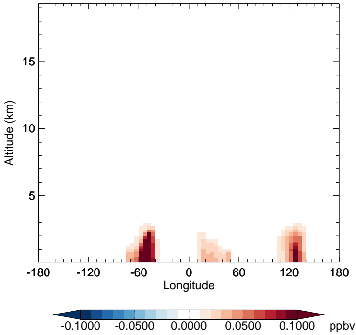
v11-02f-Run1 - v11-02e-Run1 INDIOL - Diff along 15S for Apr
