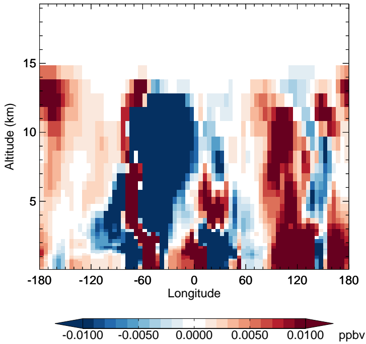
v11-02f-Run1 - v11-02e-Run0 MAP - Diff along 15S for Apr
