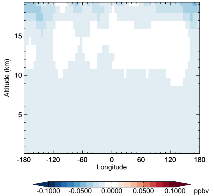
v11-02f-Run1 - v11-02e-Run0 CFC11 - Diff along 42N for Apr
