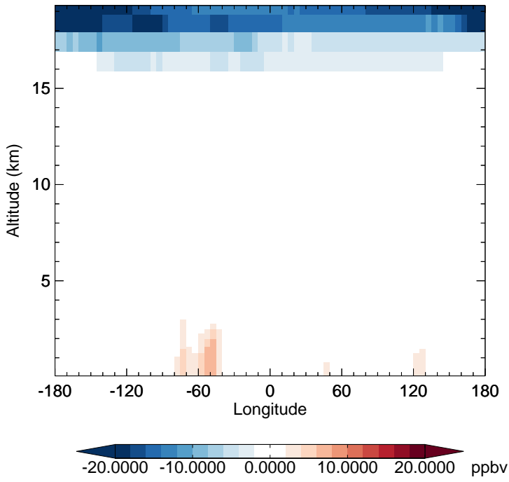
v11-02f-Run1 - v11-02e-Run1 O3 - Diff along 15S for Apr
