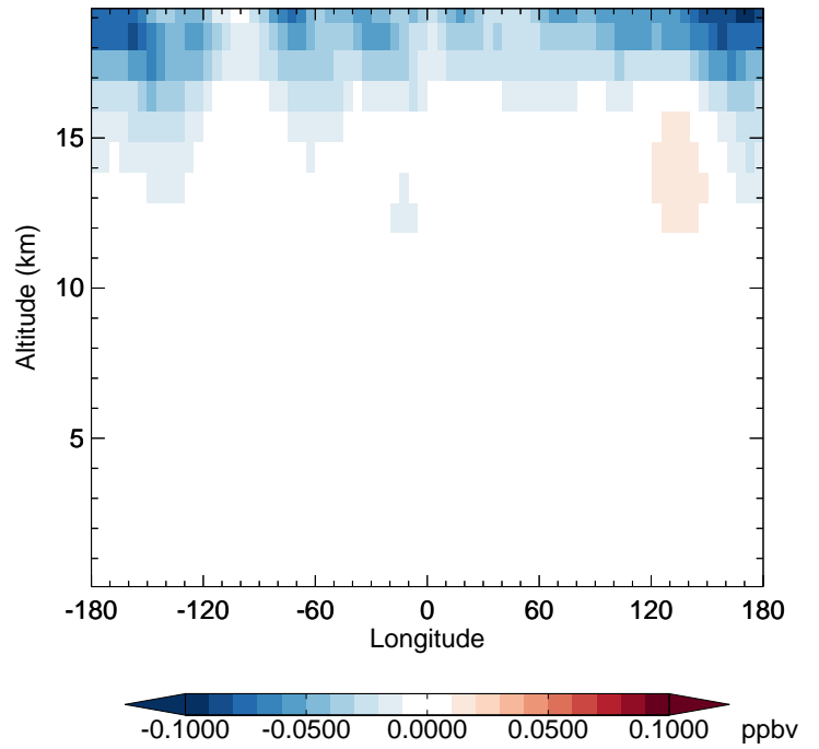
v11-02f-Run1 - v11-02e-Run0 OCS - Diff along 42N for Apr
