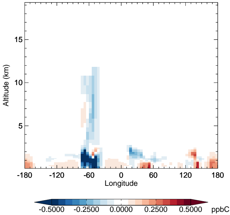
v11-02f-Run1 - v11-02e-Run0 ALD2 - Diff along 15S for Apr
