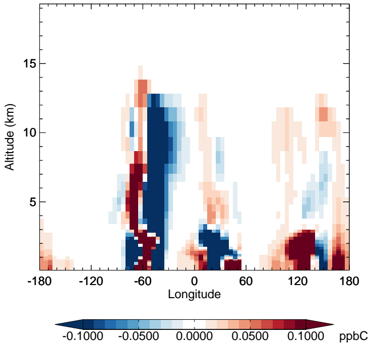
v11-02f-Run1 - v11-02e-Run0 MEK - Diff along 15S for Apr
