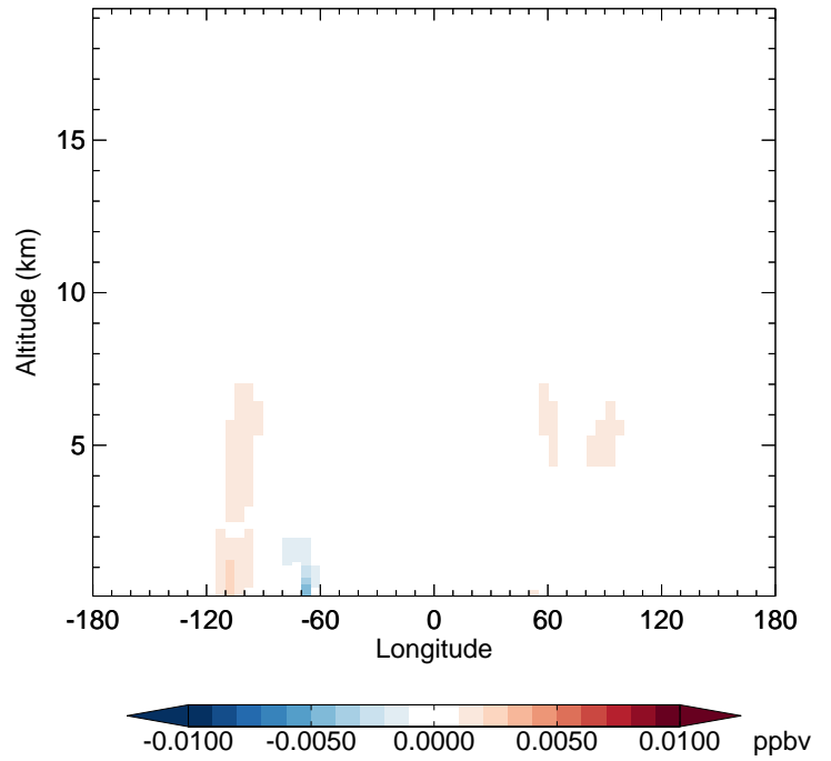
v11-02f-Run1 - v11-02e-Run0 R4N2 - Diff along 42N for Apr
