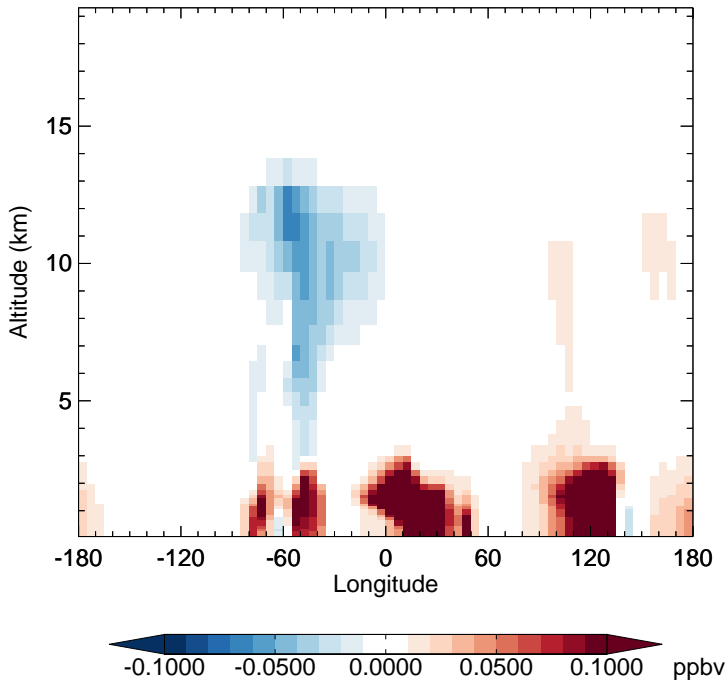
v11-02f-Run1 - v11-02e-Run1 H2O2 - Diff along 15S for Apr
