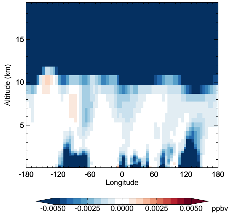
v11-02f-Run1 - v11-02e-Run0 N2O5 - Diff along 42N for Apr
