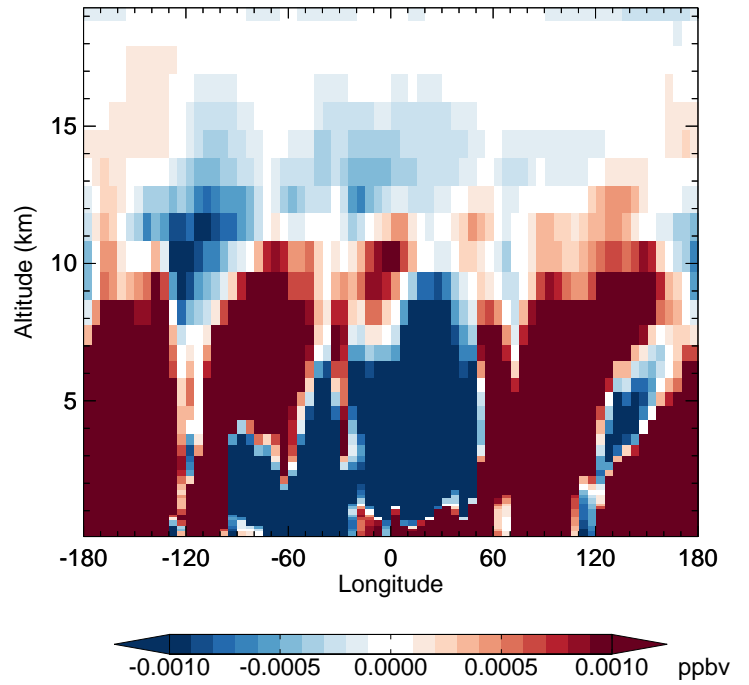
v11-02f-Run1 - v11-02e-Run0 PPN - Diff along 42N for Apr
