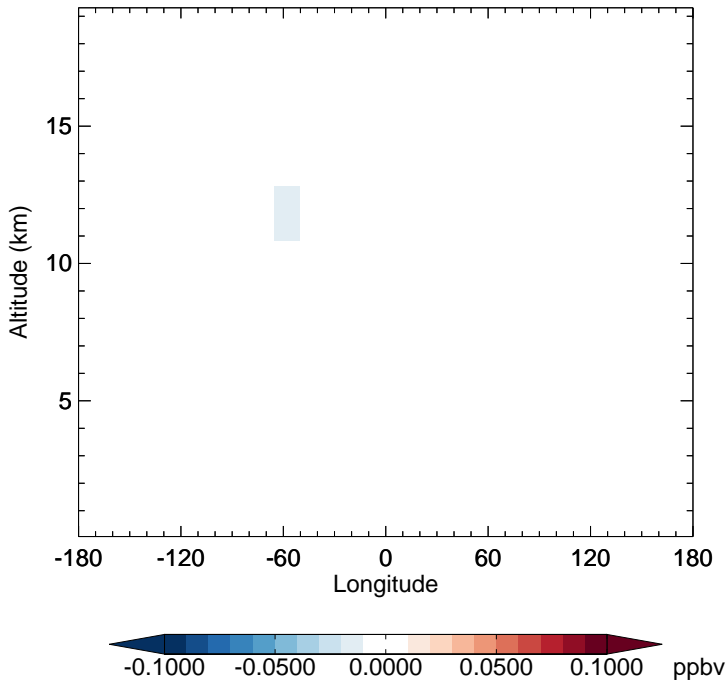
v11-02f-Run1 - v11-02e-Run1 ISOA3 - Diff along 15S for Apr
