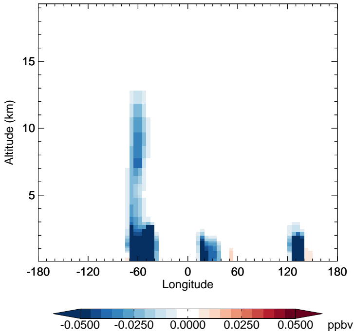
v11-02f-Run1 - v11-02e-Run1 MVK - Diff along 15S for Apr
