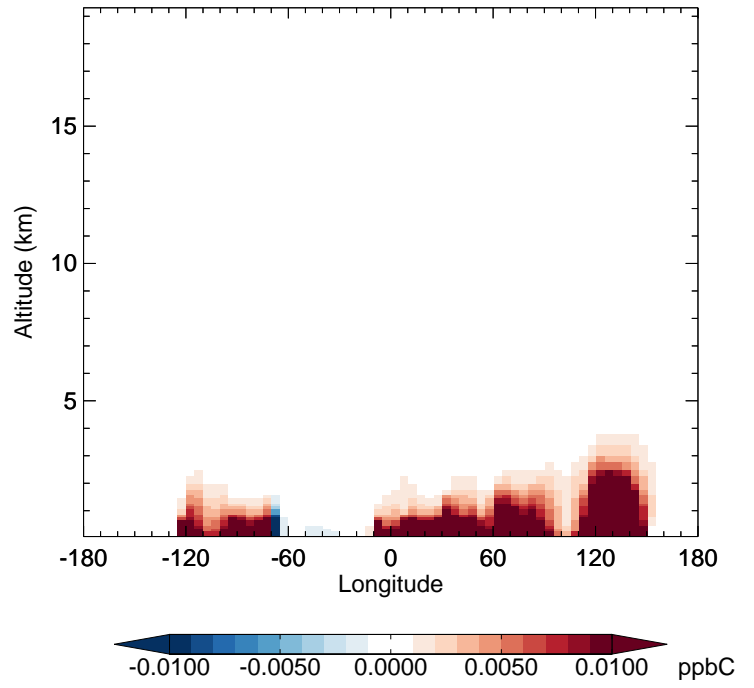
v11-02f-Run1 - v11-02e-Run1 PRPE - Diff along 42N for Apr
