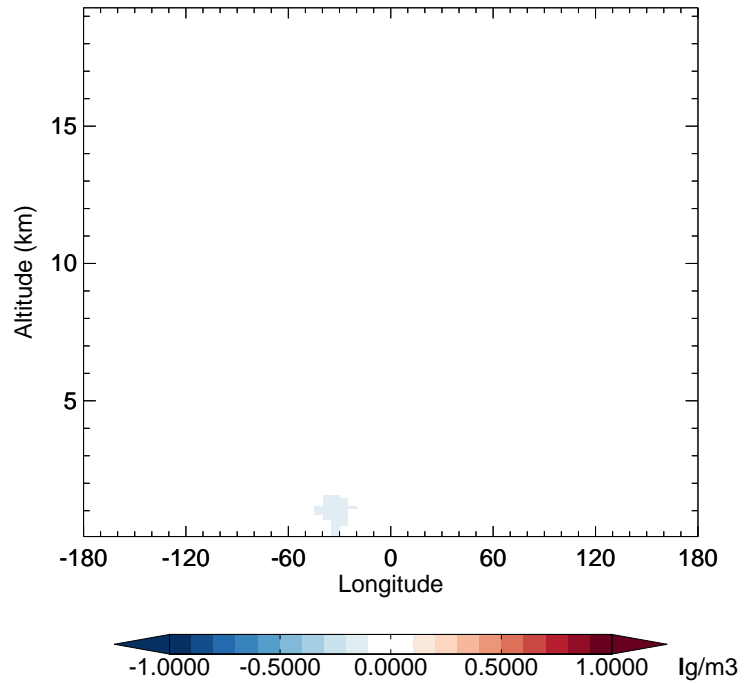
v11-02f-Run1 - v11-02e-Run0 DMS - Diff along 42N for Apr
