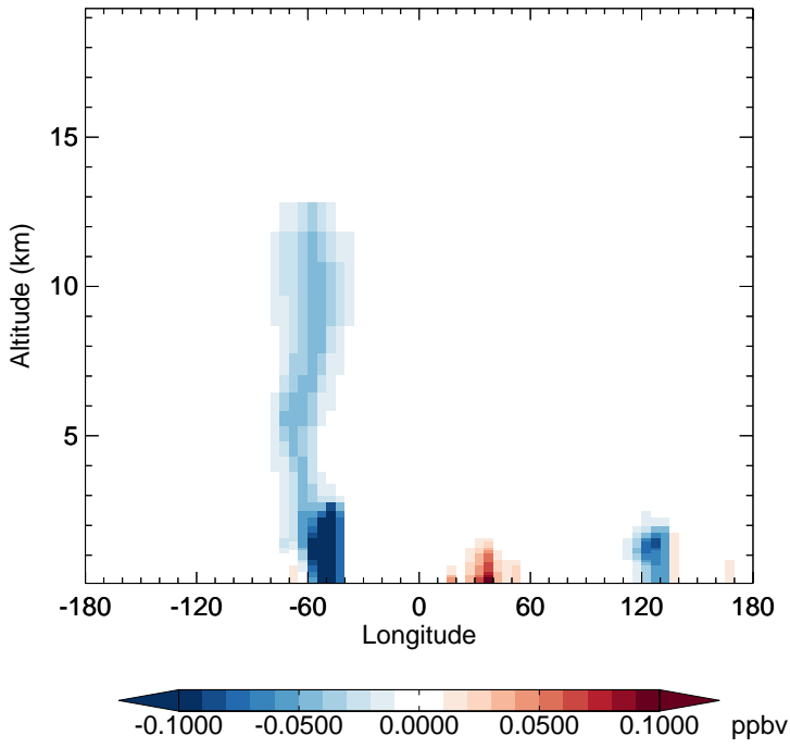
v11-02f-Run1 - v11-02e-Run1 HAC - Diff along 15S for Apr
