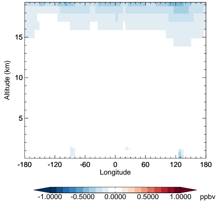
v11-02f-Run1 - v11-02e-Run0 NO 2 - Diff along 42N for Apr
