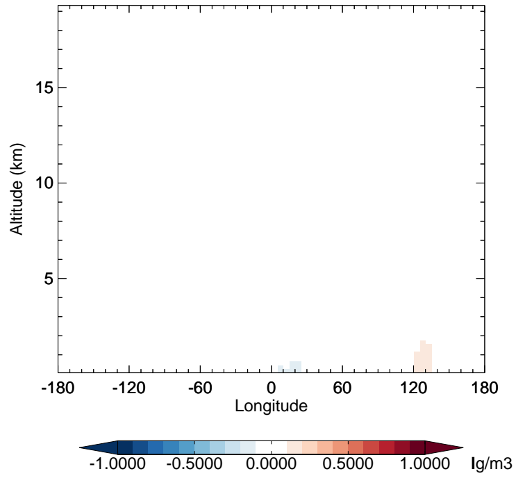
v11-02f-Run1 - v11-02e-Run1 BCPI - Diff along 42N for Apr
