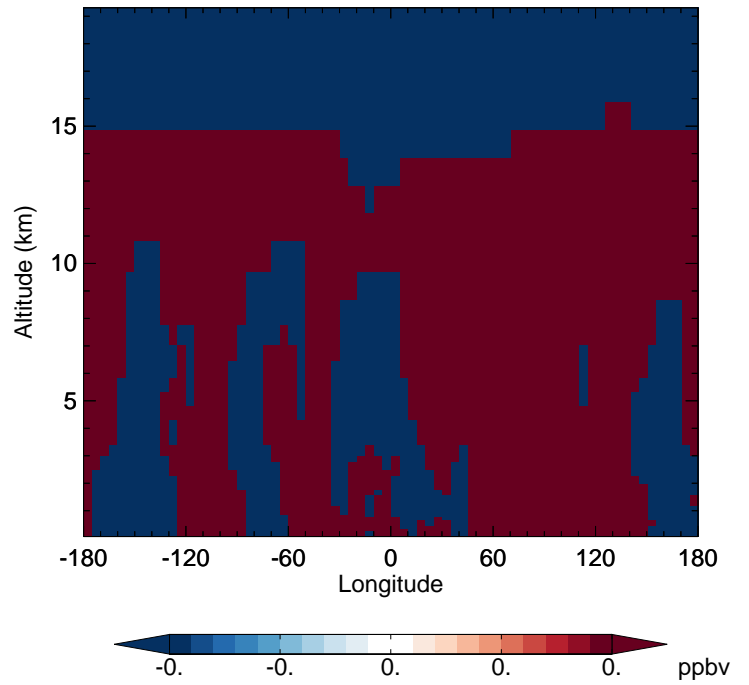
v11-02f-Run1 - v11-02e-Run0 H2O - Diff along 42N for Apr
