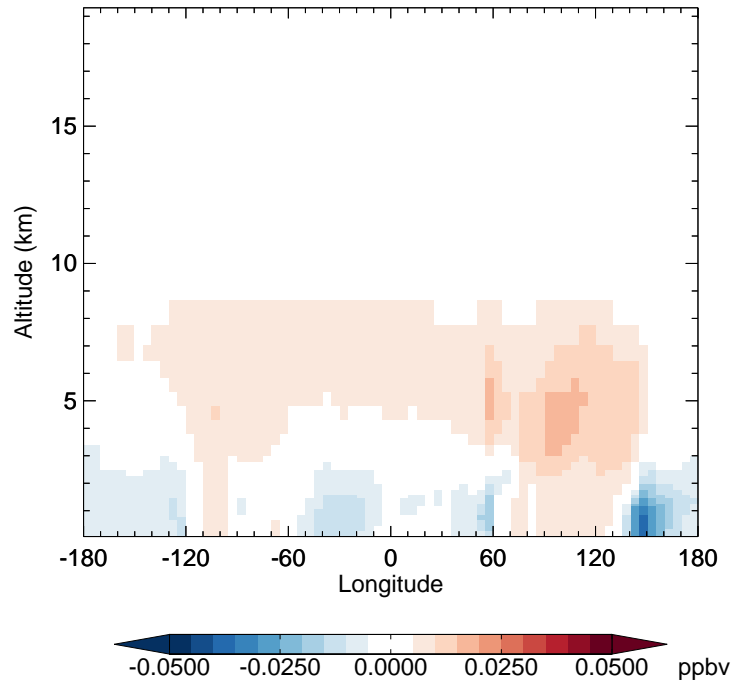
v11-02f-Run1 - v11-02e-Run1 MP - Diff along 42N for Apr
