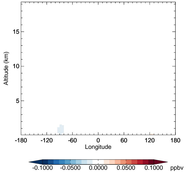
v11-02f-Run1 - v11-02e-Run1 GLYC - Diff along 42N for Apr
