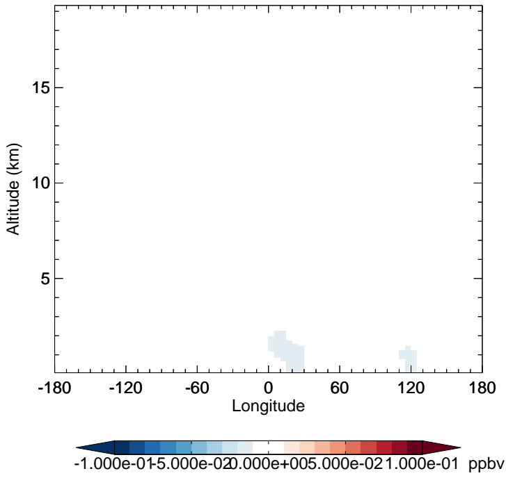
v11-02f-Run1 - v11-02e-Run1 SOAME - Diff along 15S for Apr
