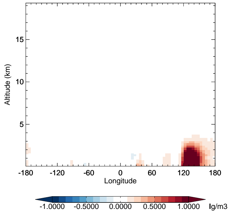
v11-02f-Run1 - v11-02e-Run0 OCPI - Diff along 42N for Apr
