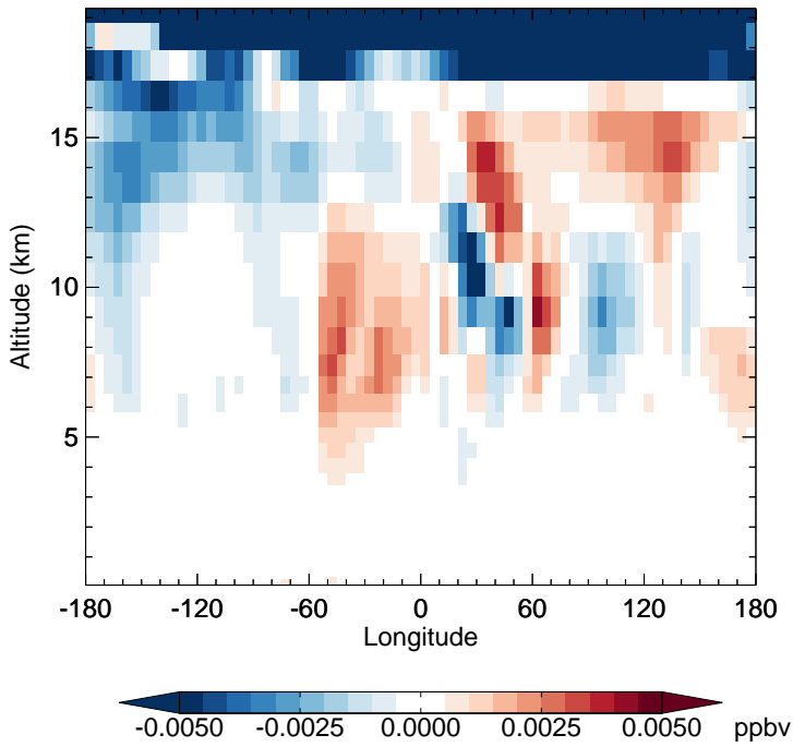
v11-02f-Run1 - v11-02e-Run0 N2O5 - Diff along 15S for Apr
