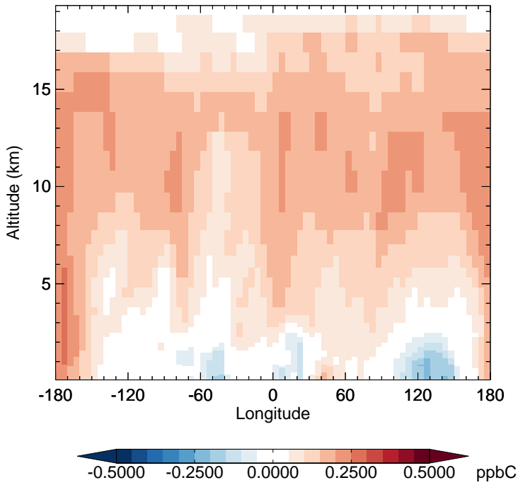
v11-02f-Run1 - v11-02e-Run0 C2H6 - Diff along 15S for Apr
