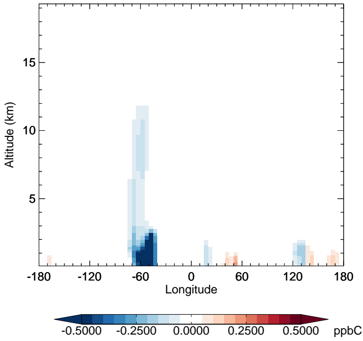
v11-02f-Run1 - v11-02e-Run1 ALD2 - Diff along 15S for Apr
