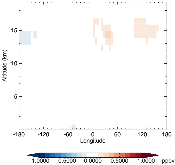
v11-02f-Run1 - v11-02e-Run0 NO 2 - Diff along 15S for Apr
