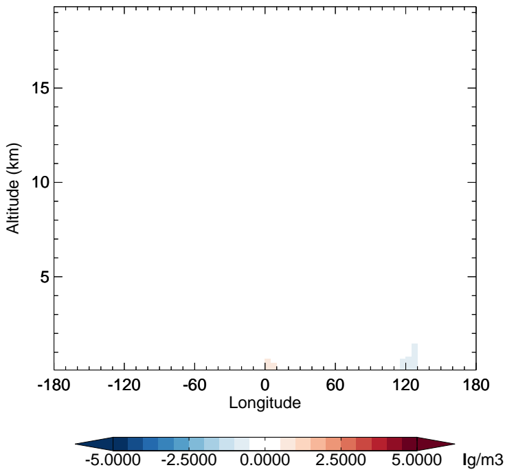
v11-02f-Run1 - v11-02e-Run0 DST3 - Diff along 15S for Apr
