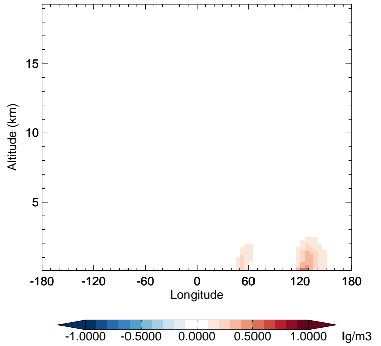
v11-02f-Run1 - v11-02e-Run1 NH4 - Diff along 42N for Apr
