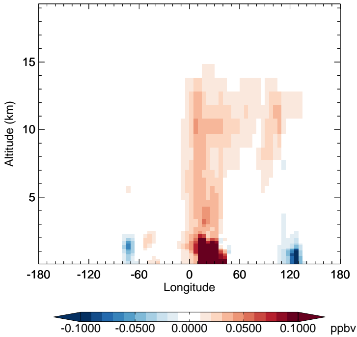
v11-02f-Run1 - v11-02e-Run0 BENZ - Diff along 15S for Apr
