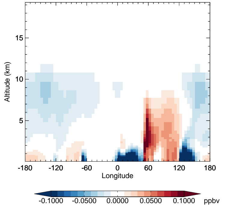
v11-02f-Run1 - v11-02e-Run1 BENZ - Diff along 42N for Apr
