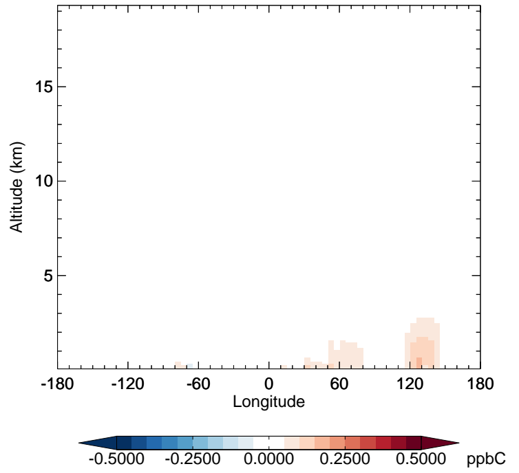
v11-02f-Run1 - v11-02e-Run1 ALD2 - Diff along 42N for Apr
