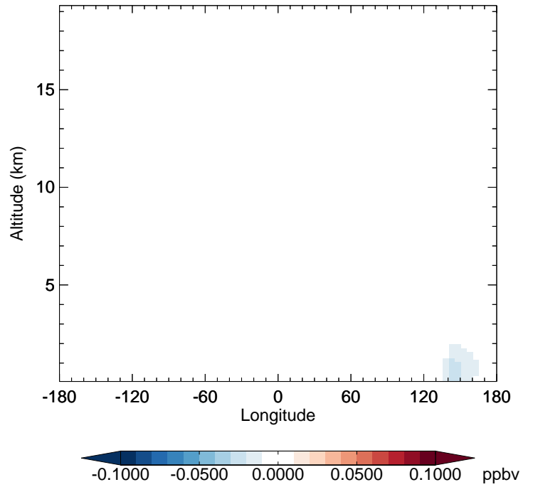
v11-02f-Run1 - v11-02e-Run0 ASOAN - Diff along 42N for Apr
