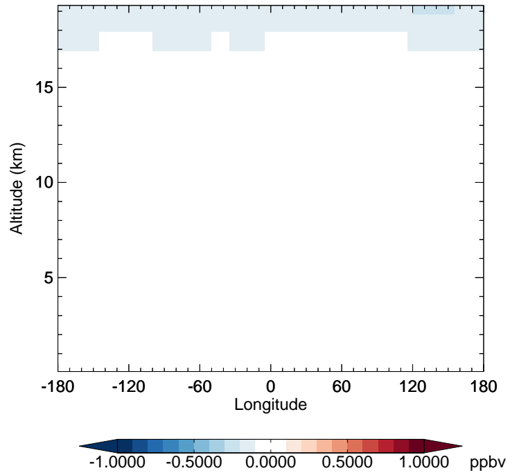
v11-02f-Run1 - v11-02e-Run1 NO - Diff along 42N for Apr
