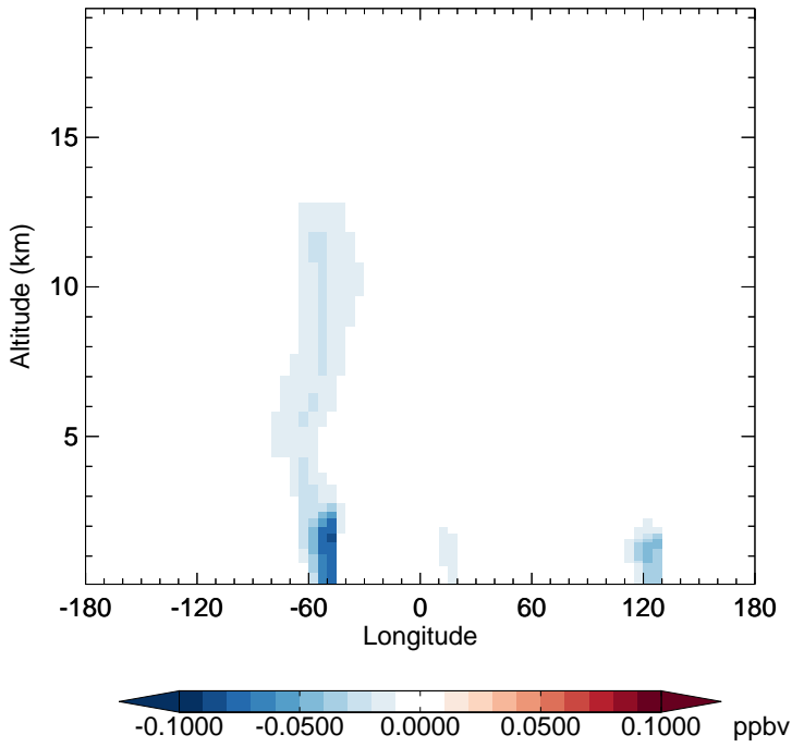
v11-02f-Run1 - v11-02e-Run1 IMAE - Diff along 15S for Apr
