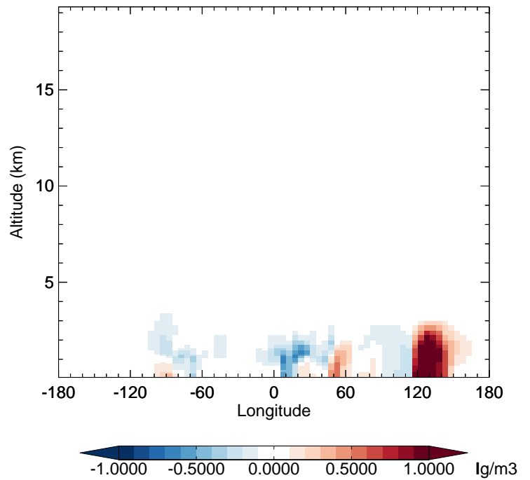
v11-02f-Run1 - v11-02e-Run0 NH4 - Diff along 42N for Apr
