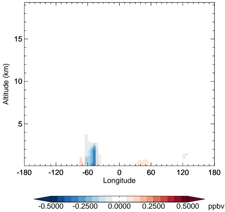
v11-02f-Run1 - v11-02e-Run1 CH 2 O - Diff along 15S for Apr
