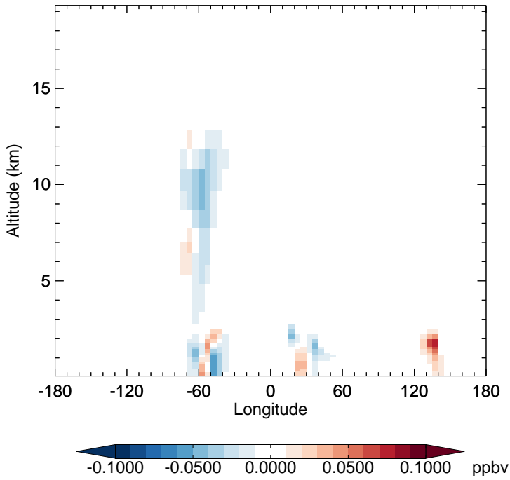
v11-02f-Run1 - v11-02e-Run0 IEPOXB - Diff along 15S for Apr
