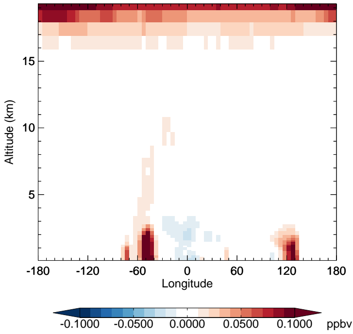
v11-02f-Run1 - v11-02e-Run1 HNO 3 - Diff along 15S for Apr
