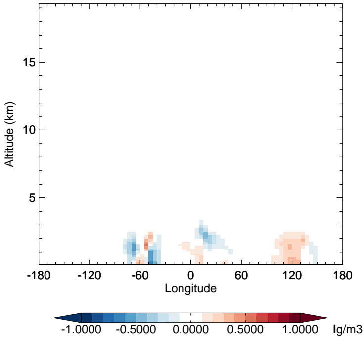
v11-02f-Run1 - v11-02e-Run0 SOAS - Diff along 15S for Apr
