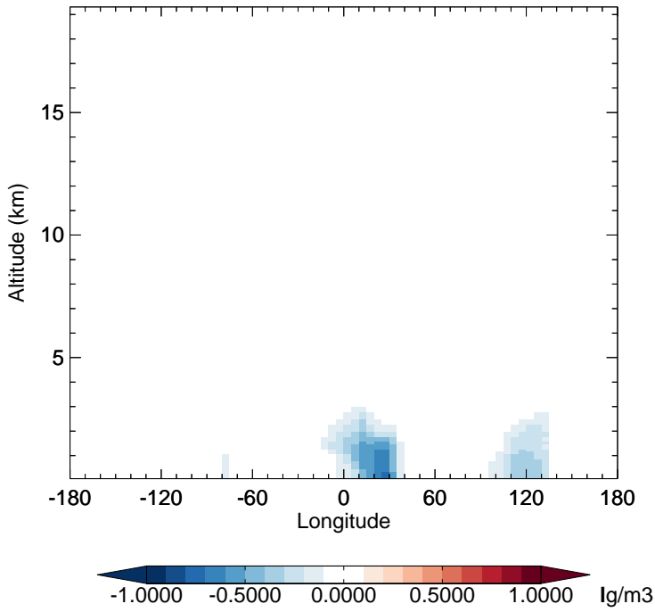
v11-02f-Run1 - v11-02e-Run1 SO4 - Diff along 15S for Apr
