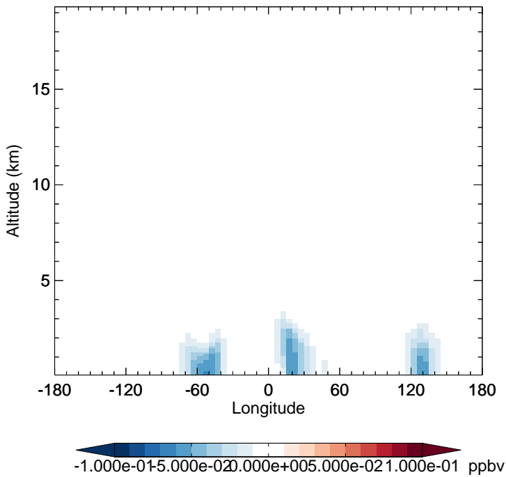
v11-02f-Run1 - v11-02e-Run0 IONITA - Diff along 15S for Apr
