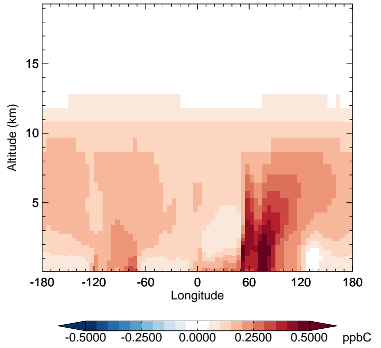
v11-02f-Run1 - v11-02e-Run1 ACET - Diff along 42N for Apr
