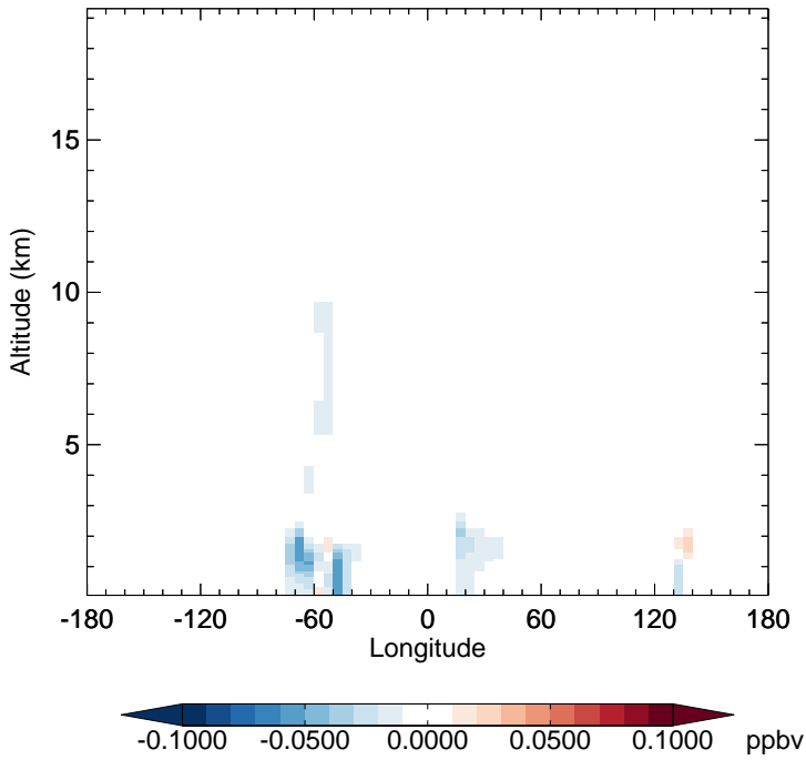
v11-02f-Run1 - v11-02e-Run0 IPMN - Diff along 15S for Apr
