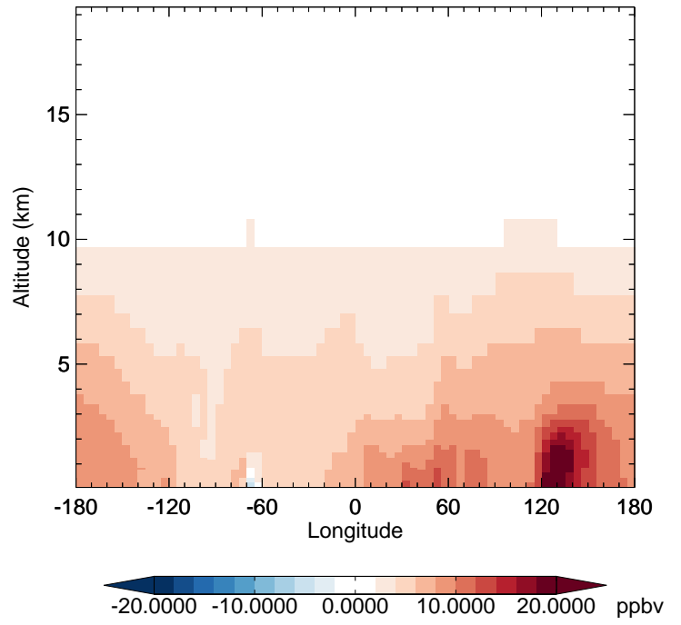
v11-02f-Run1 - v11-02e-Run1 CO - Diff along 42N for Apr
