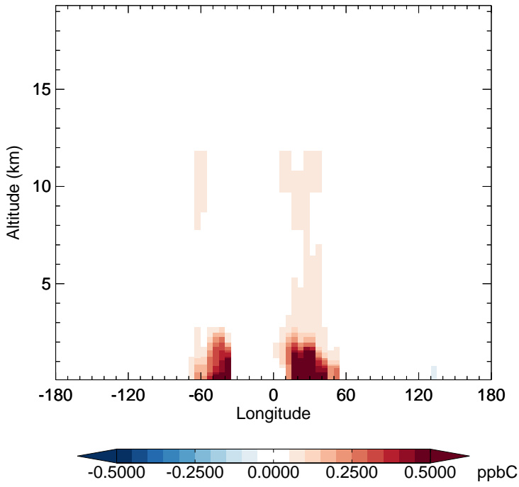
v11-02f-Run1 - v11-02e-Run1 ALK4 - Diff along 15S for Apr
