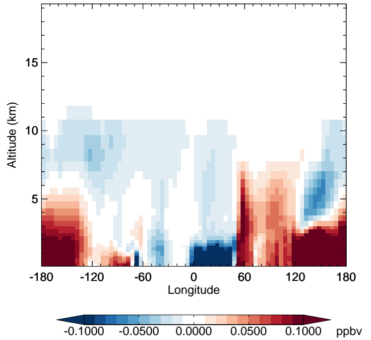
v11-02f-Run1 - v11-02e-Run0 BENZ - Diff along 42N for Apr
