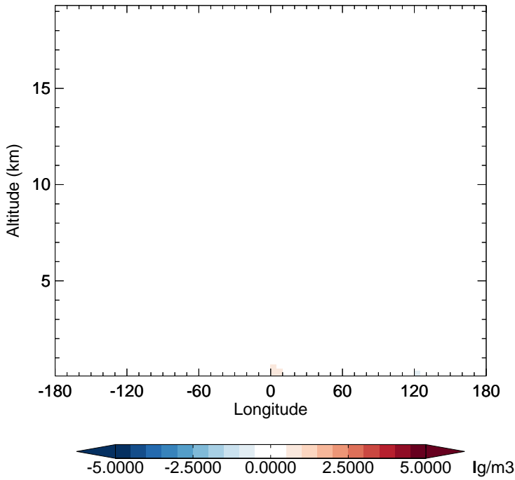
v11-02f-Run1 - v11-02e-Run0 DST2 - Diff along 15S for Apr
