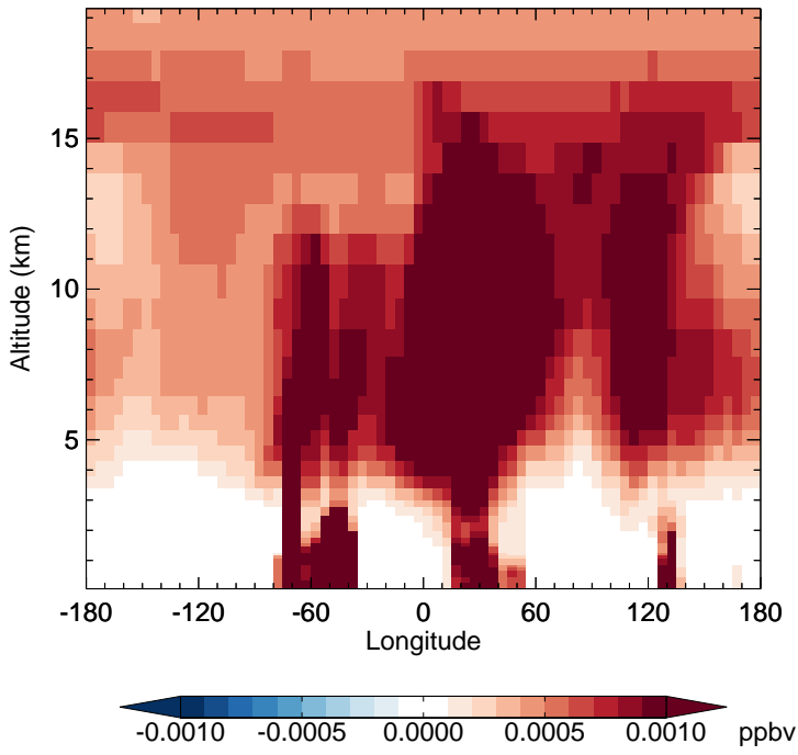
v11-02f-Run1 - v11-02e-Run1 PPN - Diff along 15S for Apr
