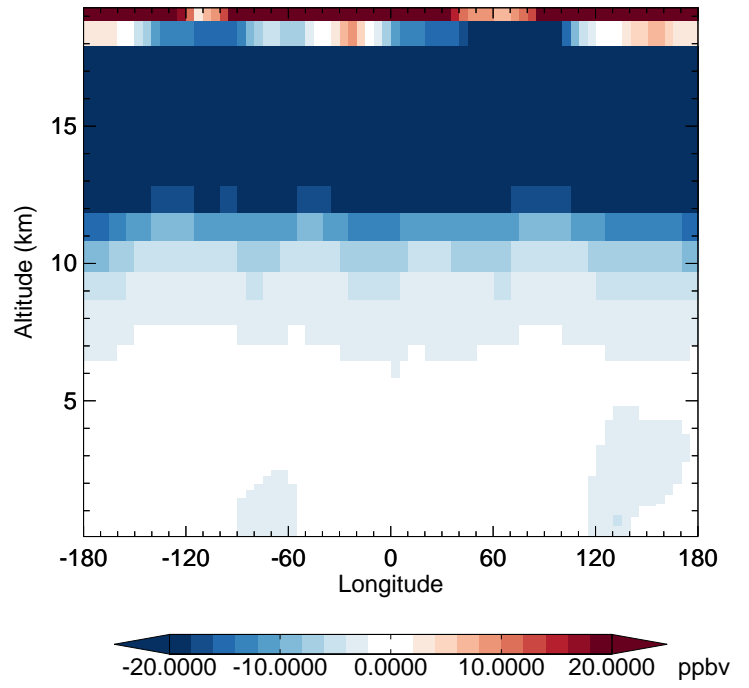
v11-02f-Run1 - v11-02e-Run1 O3 - Diff along 42N for Apr
