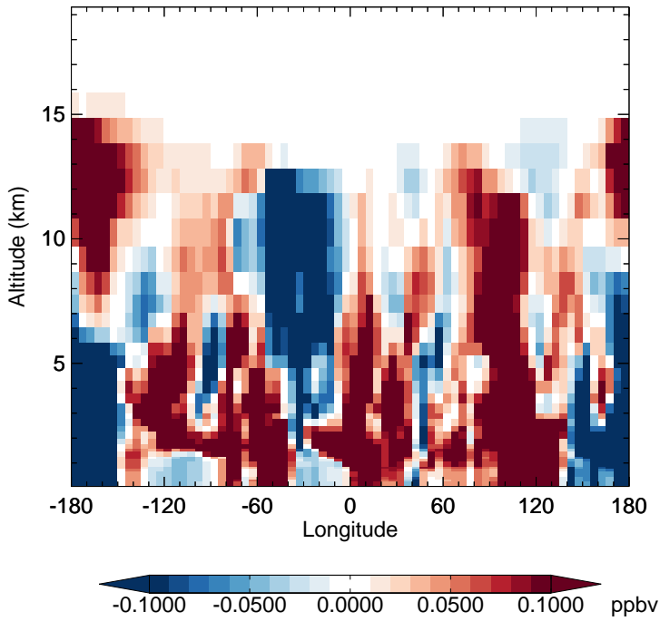
v11-02f-Run1 - v11-02e-Run0 H2O2 - Diff along 15S for Apr
