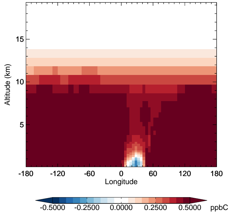
v11-02f-Run1 - v11-02e-Run1 C2H6 - Diff along 42N for Apr
