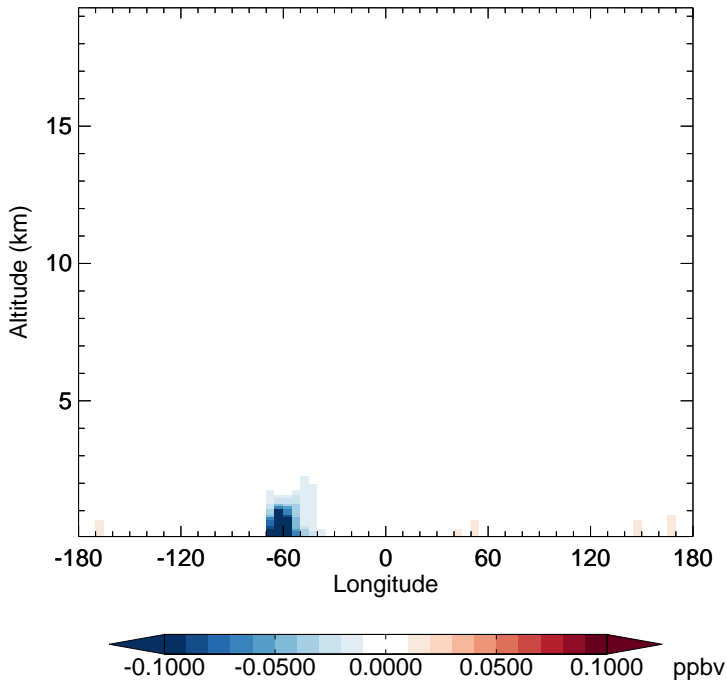
v11-02f-Run1 - v11-02e-Run1 MTPA - Diff along 15S for Apr
