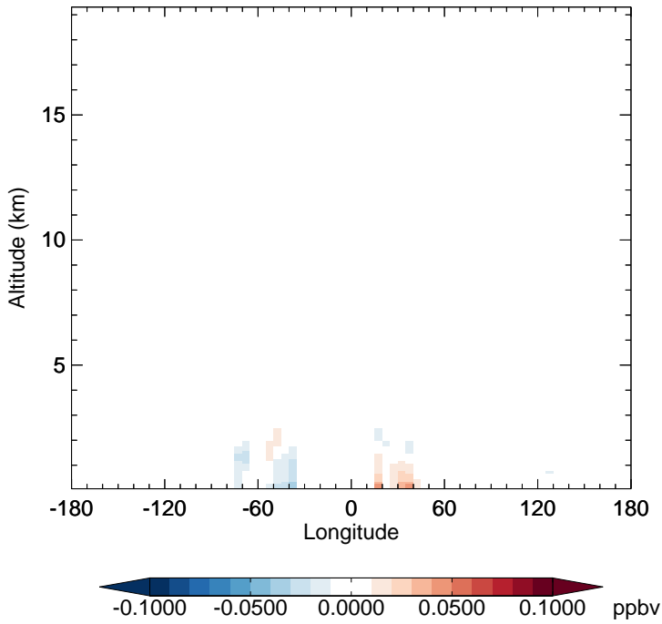
v11-02f-Run1 - v11-02e-Run0 SOAP - Diff along 15S for Apr
