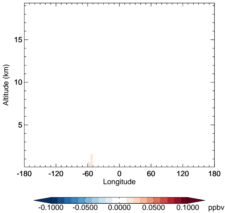
v11-02f-Run1 - v11-02e-Run0 TSOA3 - Diff along 15S for Apr
