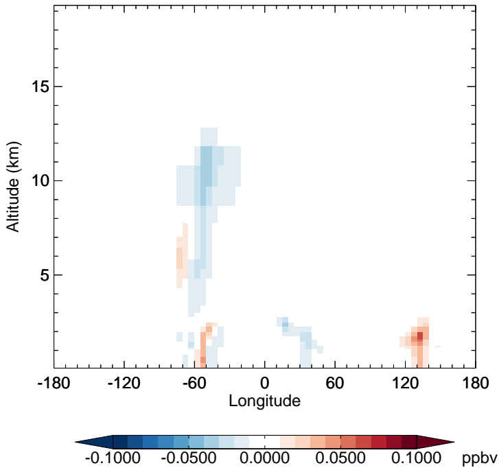
v11-02f-Run1 - v11-02e-Run0 HC187 - Diff along 15S for Apr
