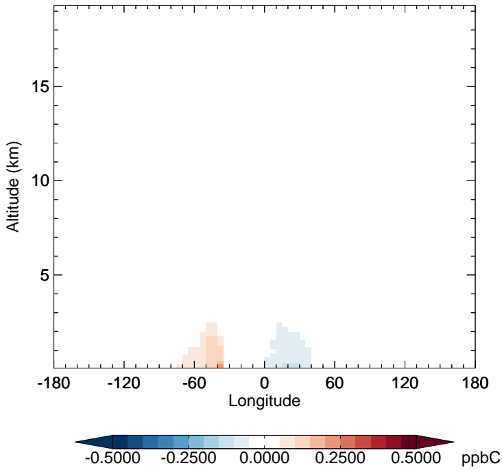
v11-02f-Run1 - v11-02e-Run1 C3H8 - Diff along 15S for Apr
