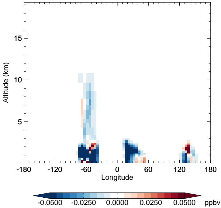
v11-02f-Run1 - v11-02e-Run0 MVK - Diff along 15S for Apr
