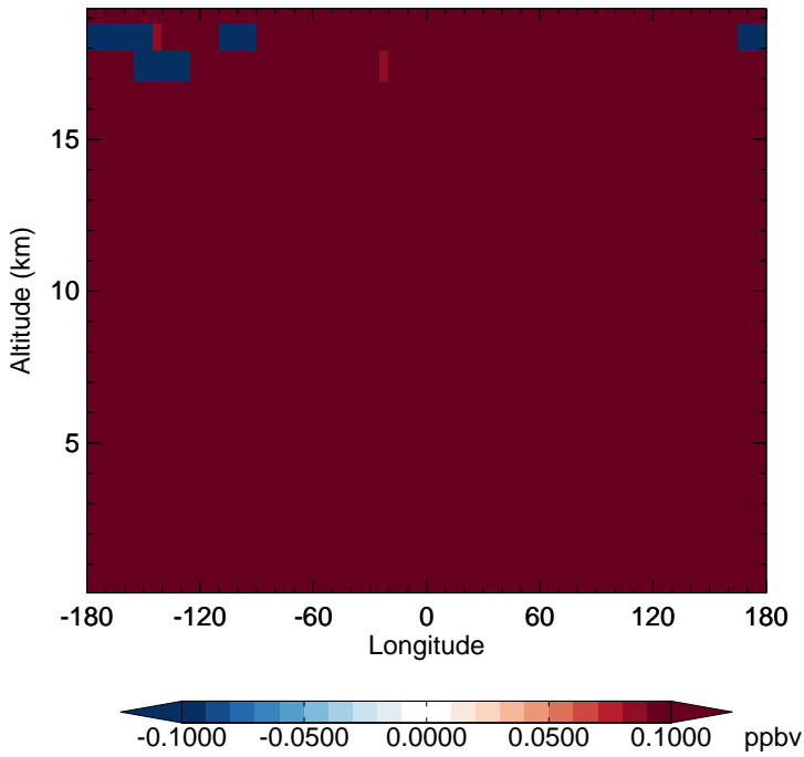
v11-02f-Run1 - v11-02e-Run0 N2O - Diff along 15S for Apr
