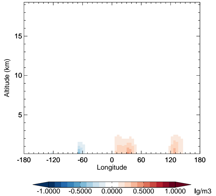
v11-02f-Run1 - v11-02e-Run1 SOAS - Diff along 42N for Apr
