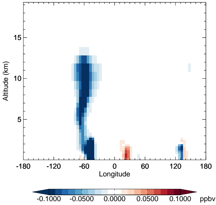
v11-02f-Run1 - v11-02e-Run1 IEPOXA - Diff along 15S for Apr
