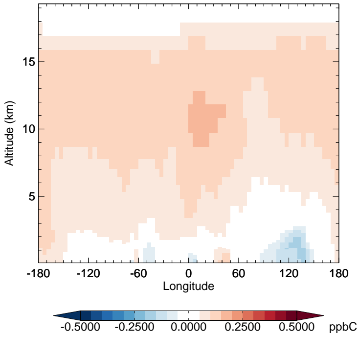
v11-02f-Run1 - v11-02e-Run1 C2H6 - Diff along 15S for Apr
