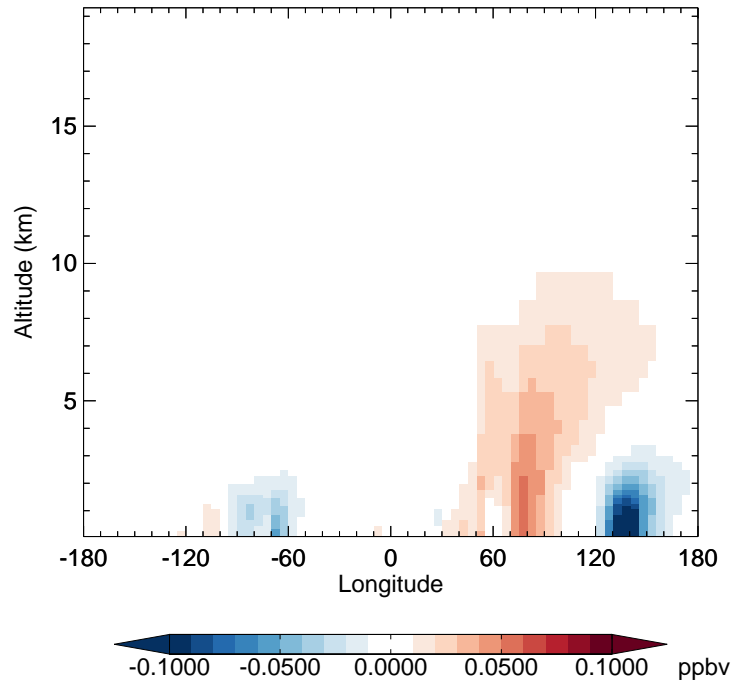
v11-02f-Run1 - v11-02e-Run1 PAN - Diff along 42N for Apr
