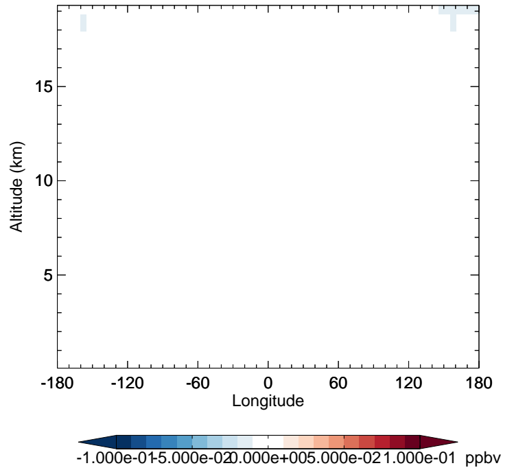
v11-02f-Run1 - v11-02e-Run0 HCFC22 - Diff along 42N for Apr
