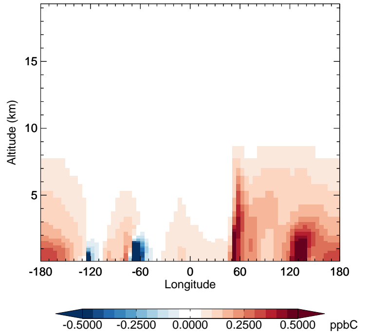
v11-02f-Run1 - v11-02e-Run1 ALK4 - Diff along 42N for Apr
