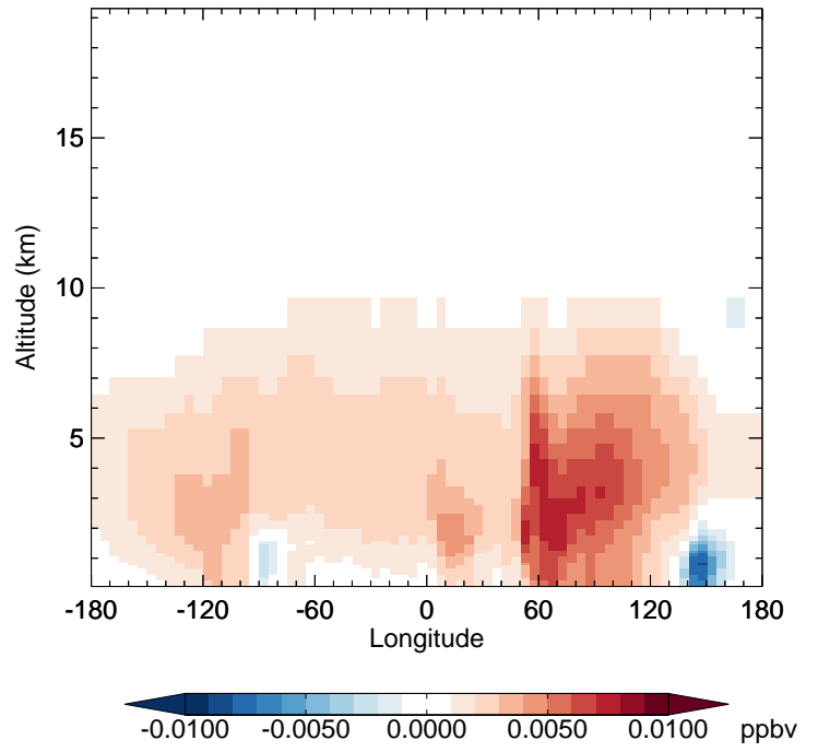
v11-02f-Run1 - v11-02e-Run1 MAP - Diff along 42N for Apr
