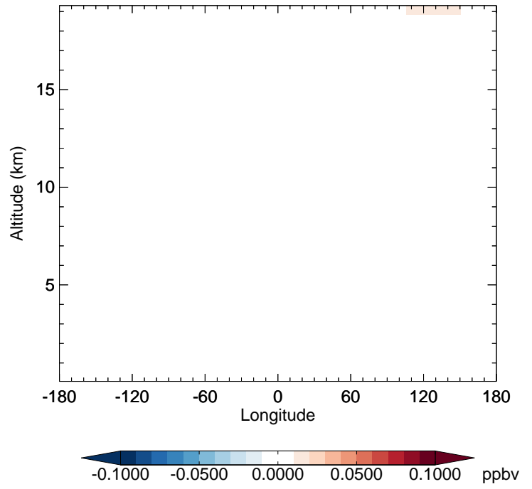
v11-02f-Run1 - v11-02e-Run1 ClO - Diff along 42N for Apr
