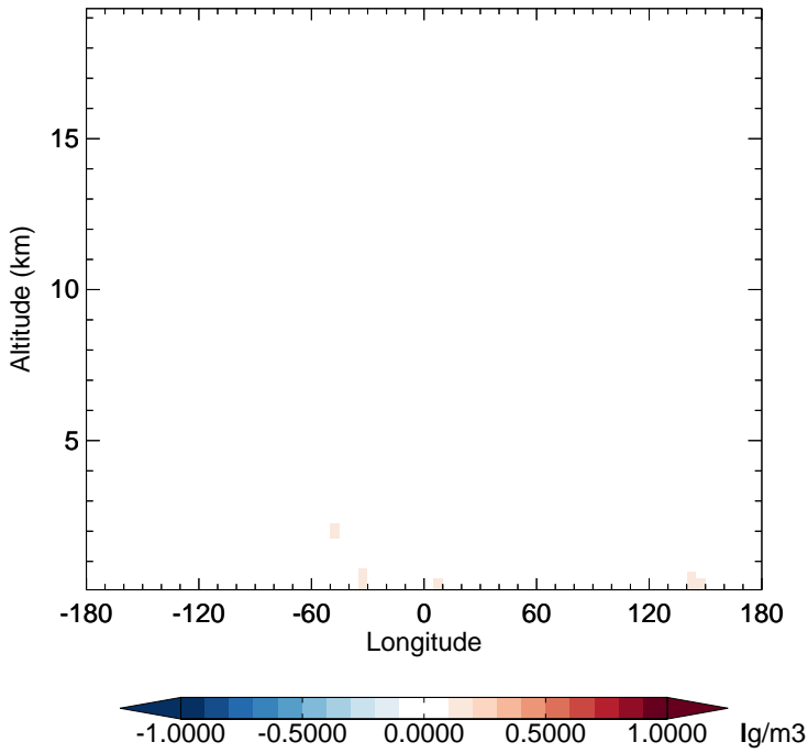
v11-02f-Run1 - v11-02e-Run0 NIT - Diff along 15S for Apr
