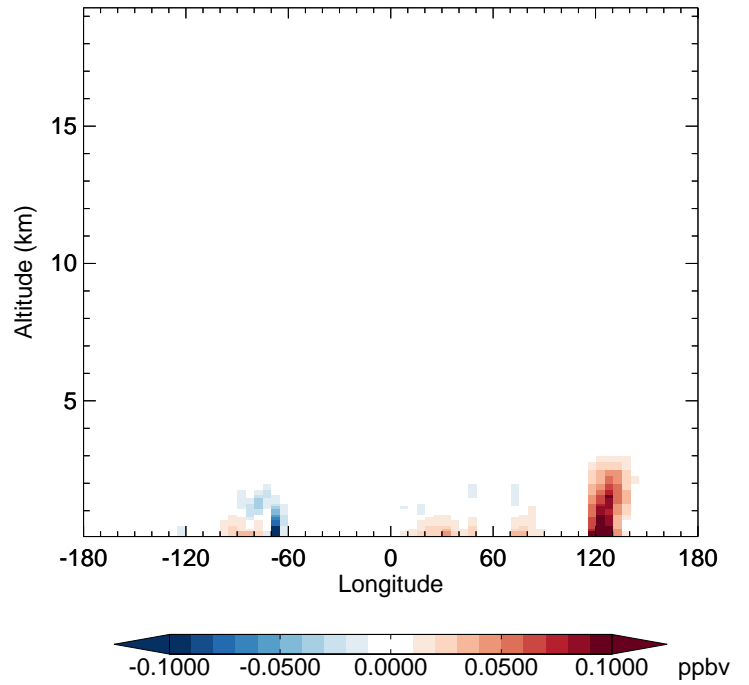
v11-02f-Run1 - v11-02e-Run0 SOAP - Diff along 42N for Apr
