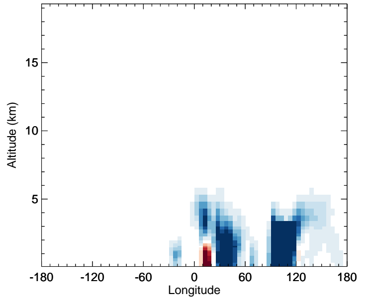
v11-02f-Run1 - v11-02e-Run0 DST4 - Diff along 42N for Apr
