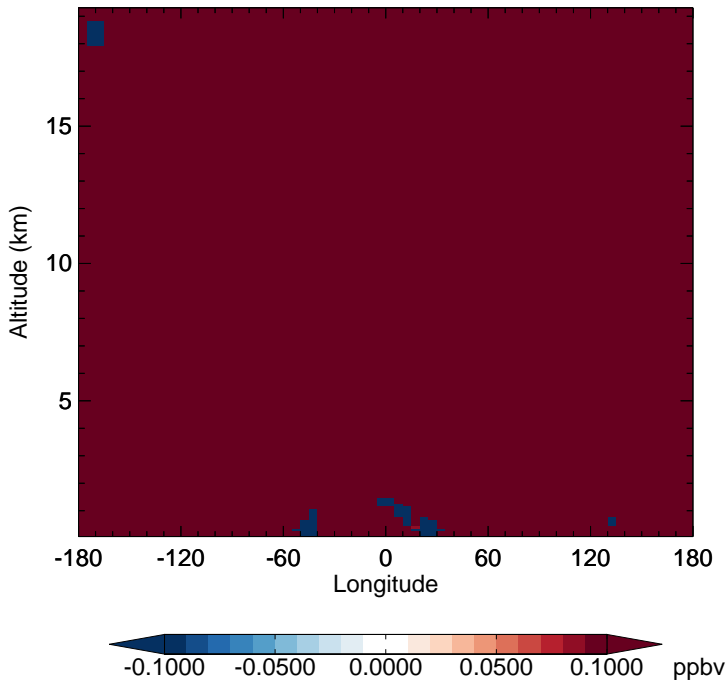
v11-02f-Run1 - v11-02e-Run0 CH4 - Diff along 15S for Apr
