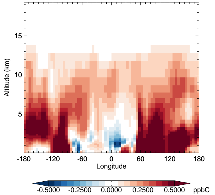
v11-02f-Run1 - v11-02e-Run0 ACET - Diff along 42N for Apr
