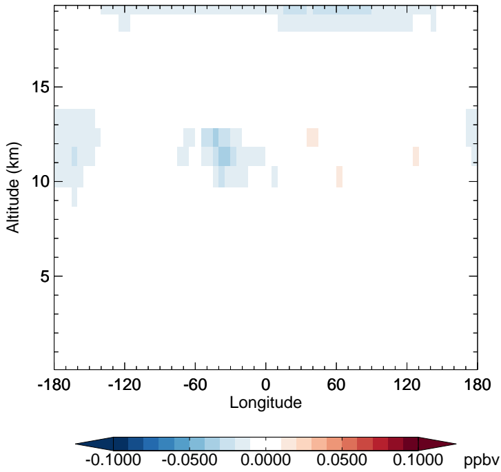
v11-02f-Run1 - v11-02e-Run0 MPN - Diff along 15S for Apr
