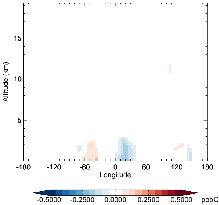
v11-02f-Run1 - v11-02e-Run0 C3H8 - Diff along 15S for Apr
