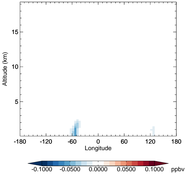
v11-02f-Run1 - v11-02e-Run1 ISOA1 - Diff along 15S for Apr
