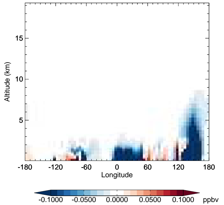
v11-02f-Run1 - v11-02e-Run0 TOLU - Diff along 42N for Apr
