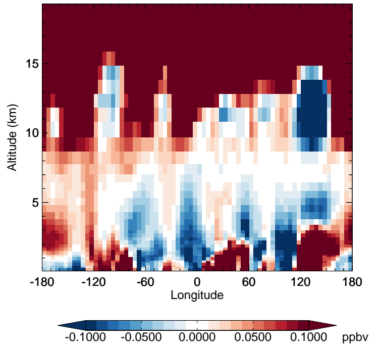
v11-02f-Run1 - v11-02e-Run0 HNO 3 - Diff along 42N for Apr
