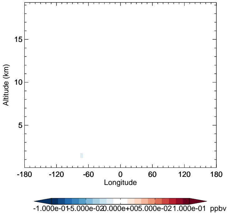
v11-02f-Run1 - v11-02e-Run0 HCFC22 - Diff along 15S for Apr
