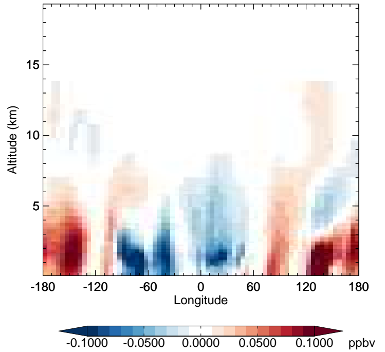
v11-02f-Run1 - v11-02e-Run0 PAN - Diff along 42N for Apr
