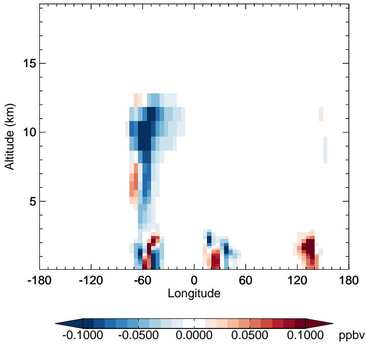
v11-02f-Run1 - v11-02e-Run0 IEPOXA - Diff along 15S for Apr
