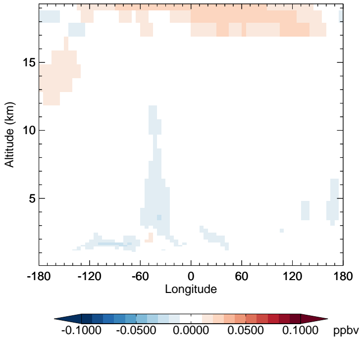
v11-02f-Run1 - v11-02e-Run0 CH3Cl - Diff along 15S for Apr
