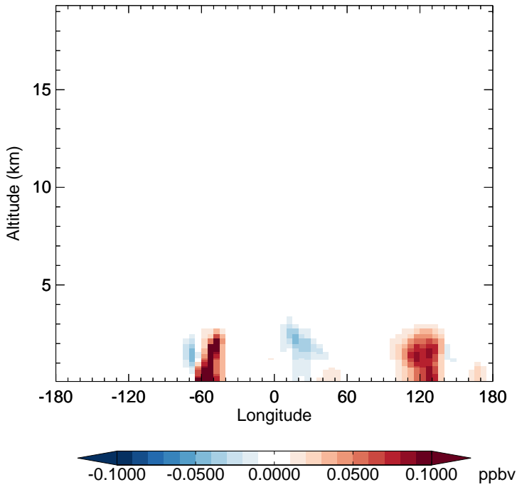
v11-02f-Run1 - v11-02e-Run0 TSOG2 - Diff along 15S for Apr
