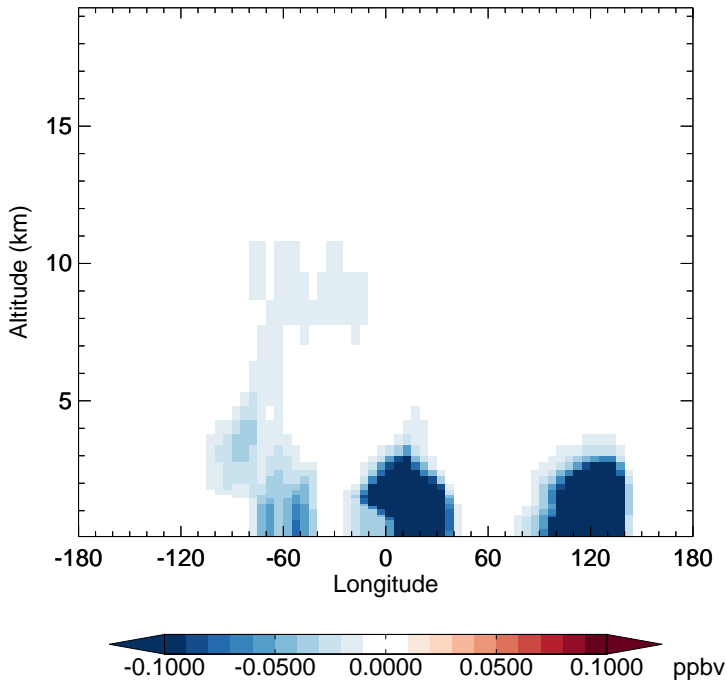
v11-02f-Run1 - v11-02e-Run1 SOAIE - Diff along 15S for Apr
