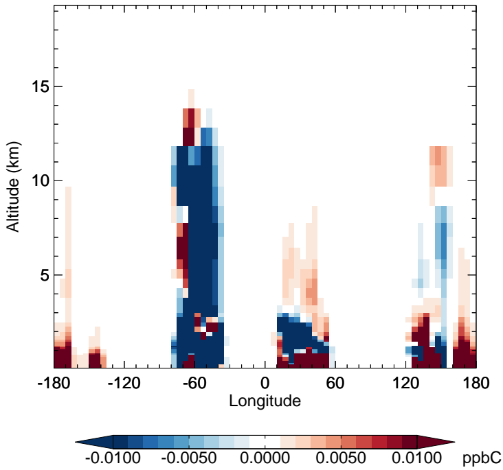
v11-02f-Run1 - v11-02e-Run0 PRPE - Diff along 15S for Apr
