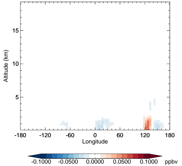
v11-02f-Run1 - v11-02e-Run0 SOAGX - Diff along 42N for Apr
