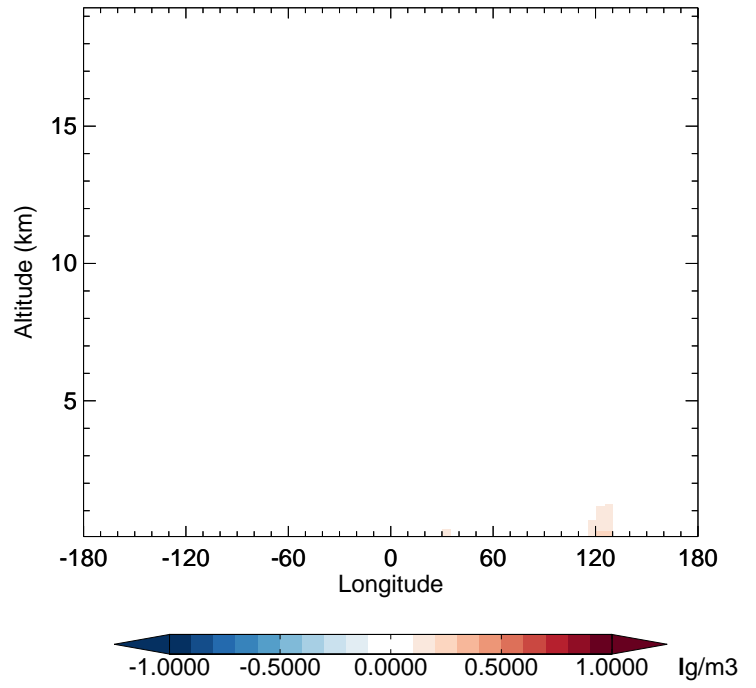
v11-02f-Run1 - v11-02e-Run1 OCPO - Diff along 42N for Apr
