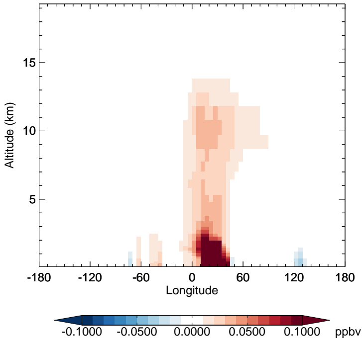
v11-02f-Run1 - v11-02e-Run1 BENZ - Diff along 15S for Apr
