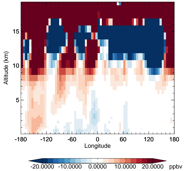
v11-02f-Run1 - v11-02e-Run0 O3 - Diff along 42N for Apr
