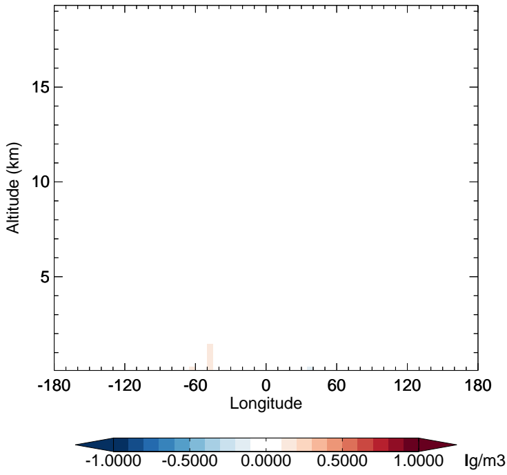
v11-02f-Run1 - v11-02e-Run1 NH3 - Diff along 15S for Apr
