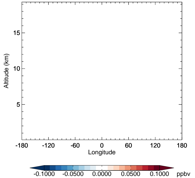
v11-02f-Run1 - v11-02e-Run0 RIPA - Diff along 42N for Apr
