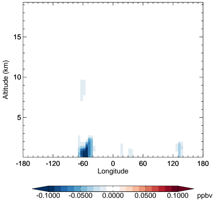
v11-02f-Run1 - v11-02e-Run1 RIPB - Diff along 15S for Apr
