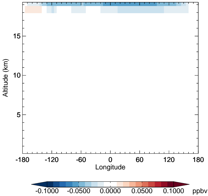
v11-02f-Run1 - v11-02e-Run0 CINO3 - Diff along 15S for Apr
