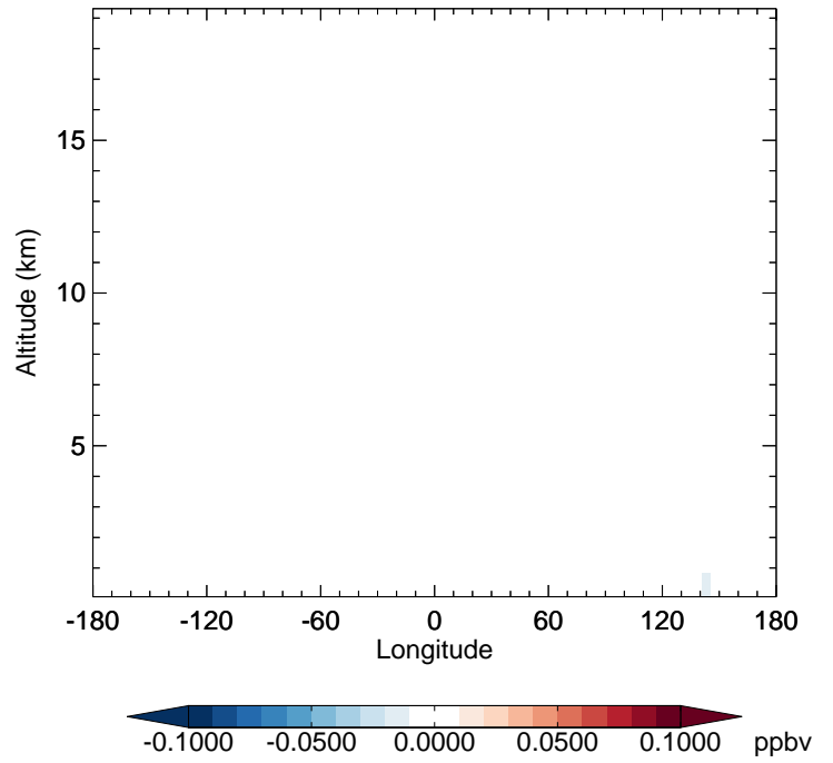
v11-02f-Run1 - v11-02e-Run1 MGLY - Diff along 42N for Apr
