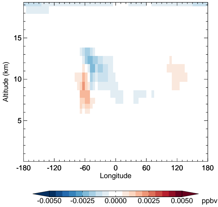
v11-02f-Run1 - v11-02e-Run1 HNO 4 - Diff along 15S for Apr
