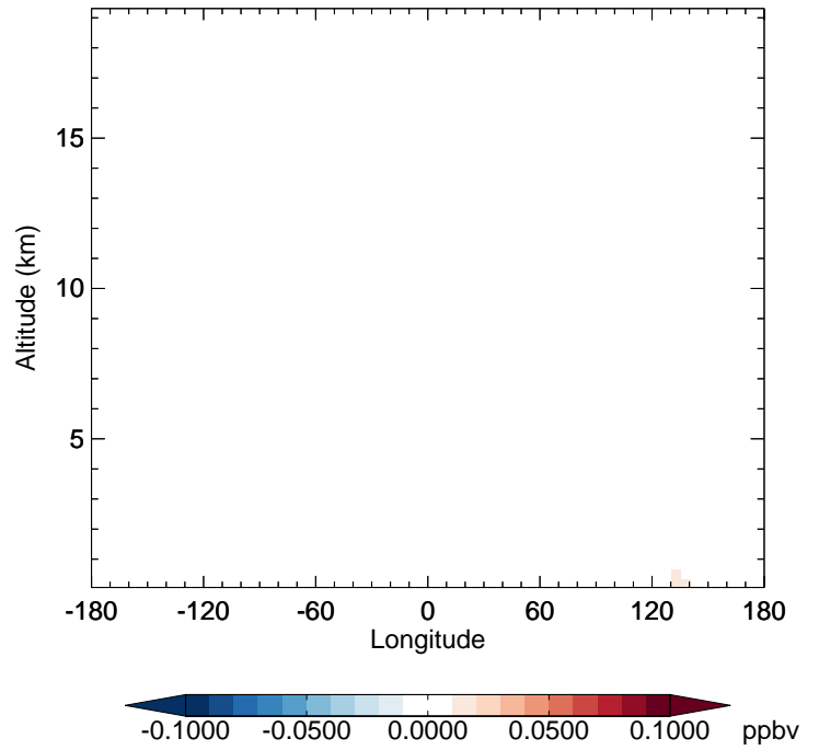
v11-02f-Run1 - v11-02e-Run0 TSOA2 - Diff along 42N for Apr
