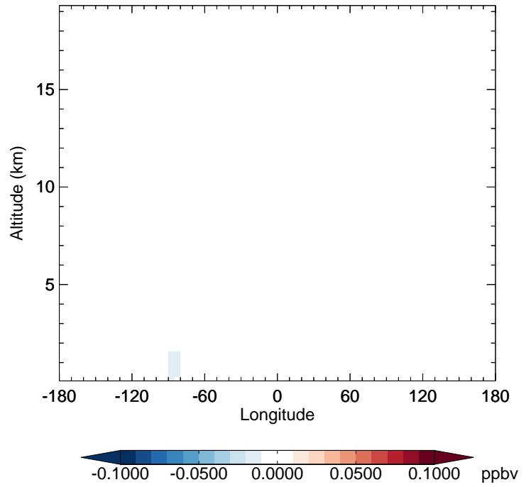
v11-02f-Run1 - v11-02e-Run1 IMAE - Diff along 42N for Apr
