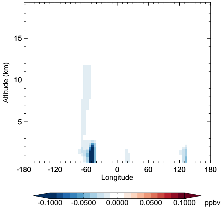
v11-02f-Run1 - v11-02e-Run1 IPMN - Diff along 15S for Apr
