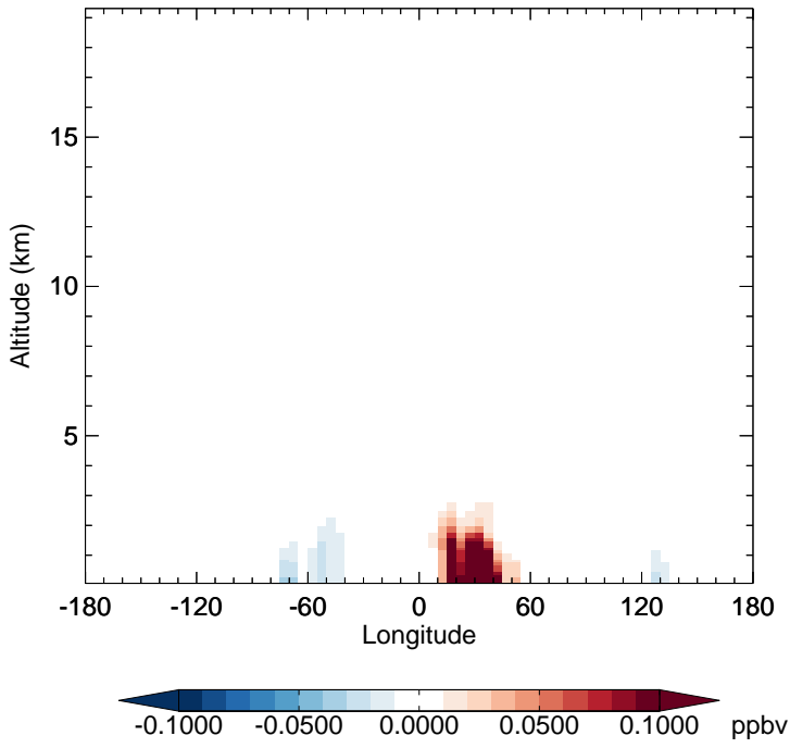
v11-02f-Run1 - v11-02e-Run1 TOLU - Diff along 15S for Apr
