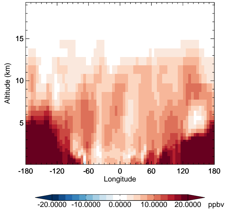
v11-02f-Run1 - v11-02e-Run0 CO - Diff along 42N for Apr
