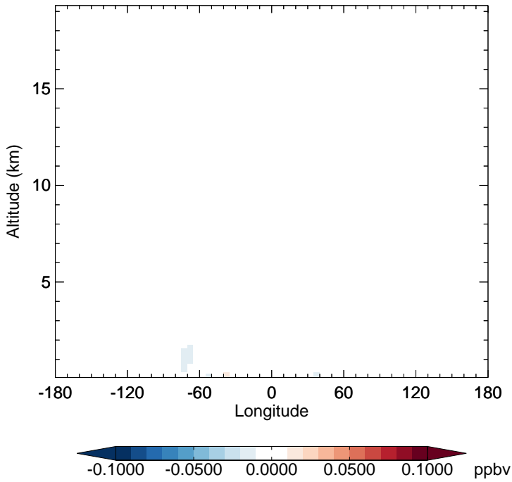
v11-02f-Run1 - v11-02e-Run0 XYLE - Diff along 15S for Apr
