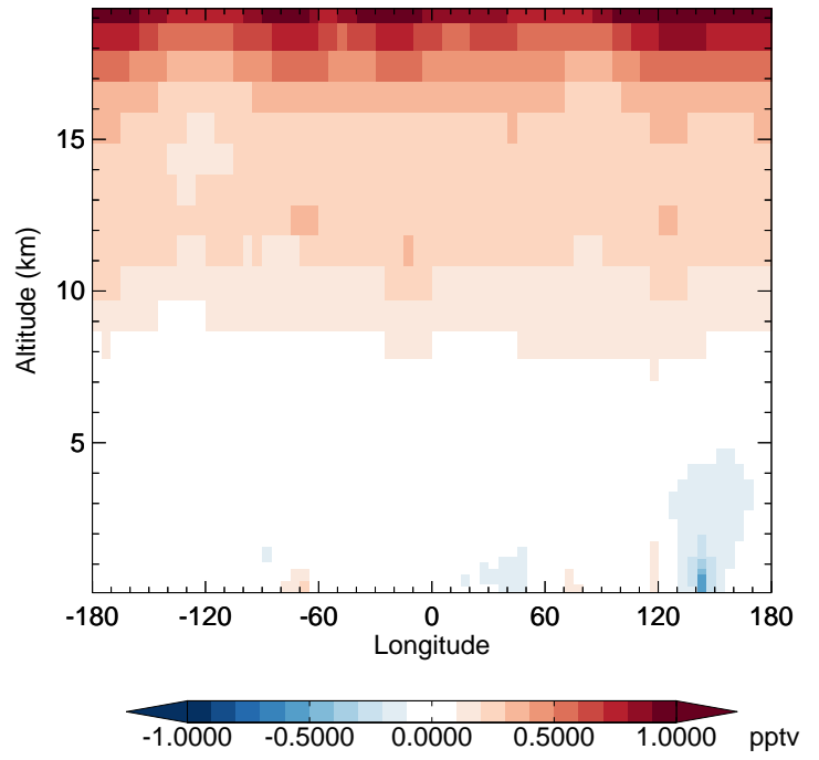
v11-02f-Run1 - v11-02e-Run1 HO2 - Diff along 42N for Apr
