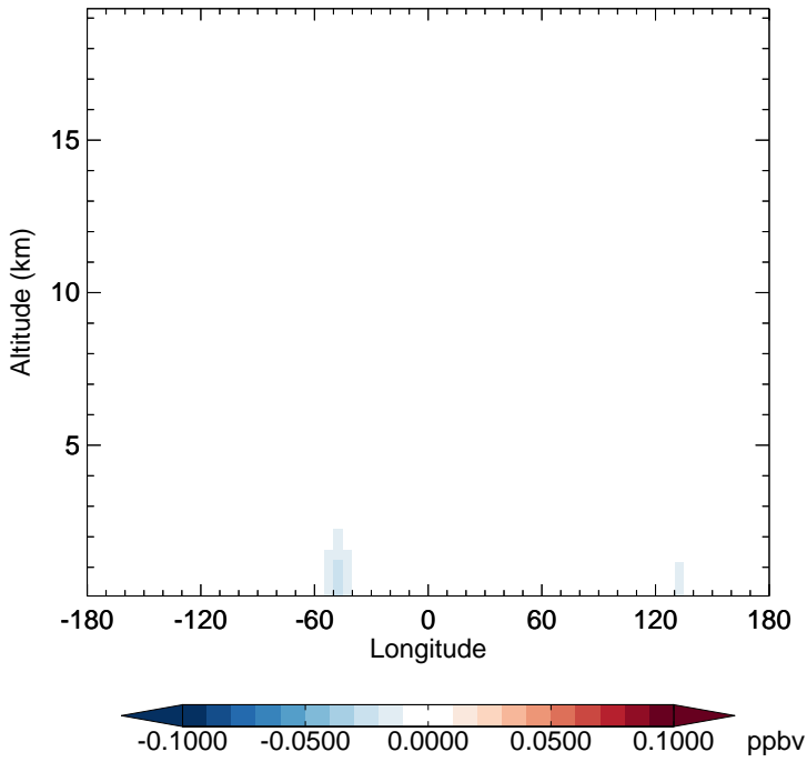
v11-02f-Run1 - v11-02e-Run1 GLYX - Diff along 15S for Apr
