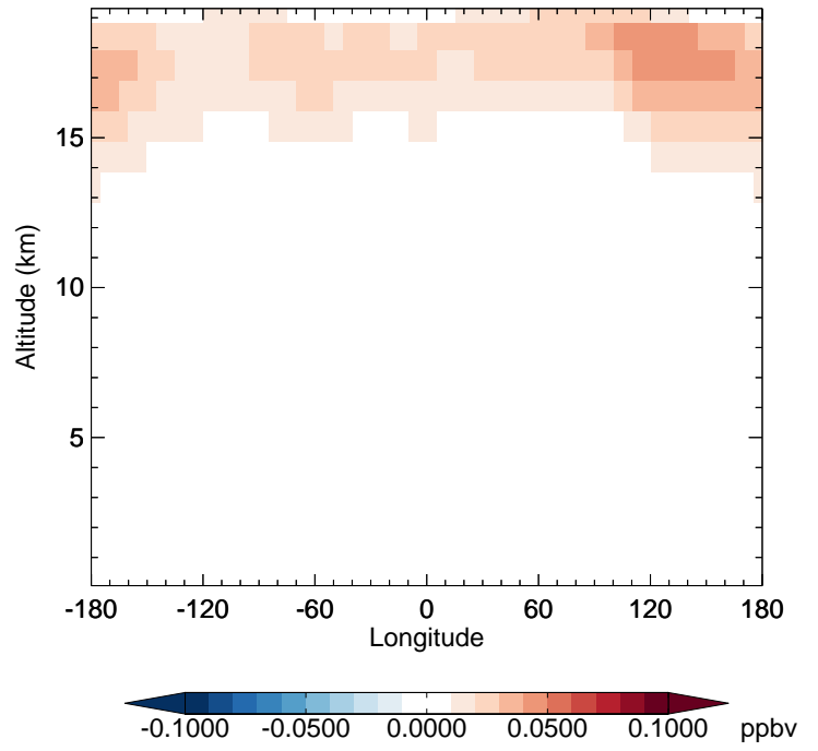
v11-02f-Run1 - v11-02e-Run1 HCl - Diff along 42N for Apr
