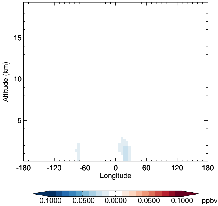
v11-02f-Run1 - v11-02e-Run0 SOAME - Diff along 15S for Apr
