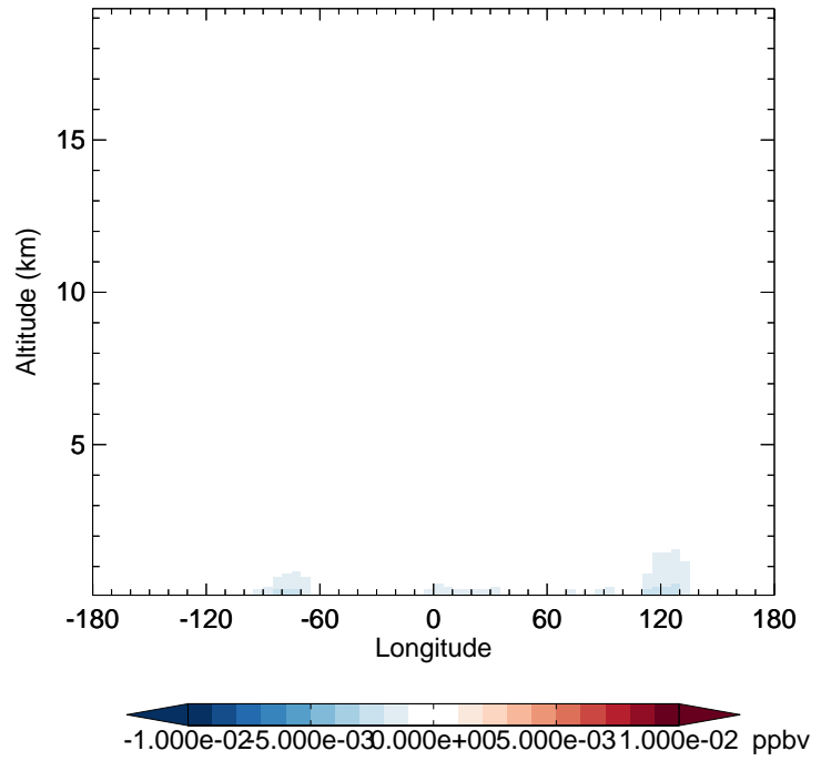
v11-02f-Run1 - v11-02e-Run1 NO3 - Diff along 42N for Apr
