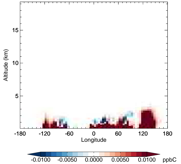
v11-02f-Run1 - v11-02e-Run0 PRPE - Diff along 42N for Apr
