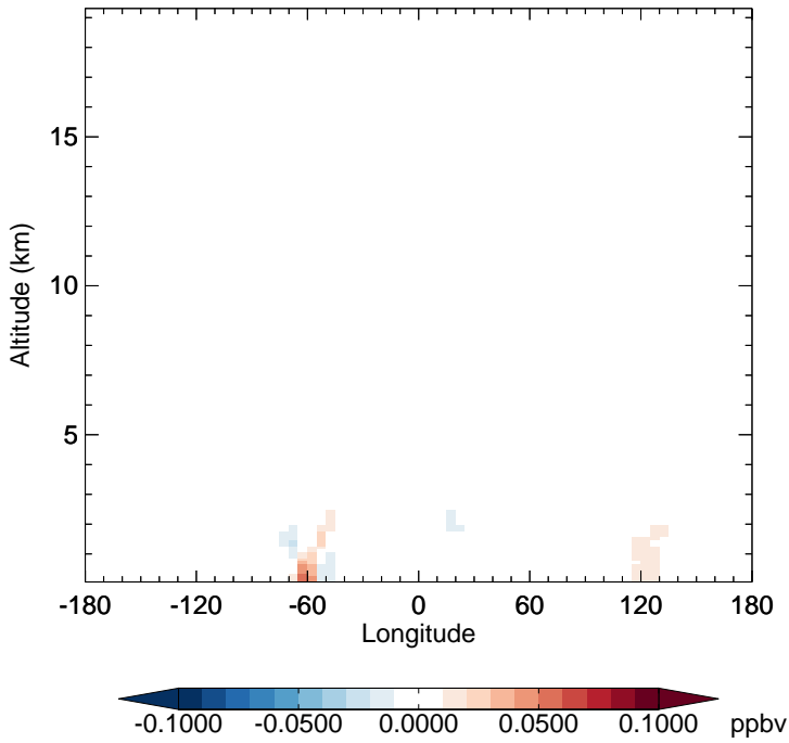
v11-02f-Run1 - v11-02e-Run0 TSOA0 - Diff along 15S for Apr
