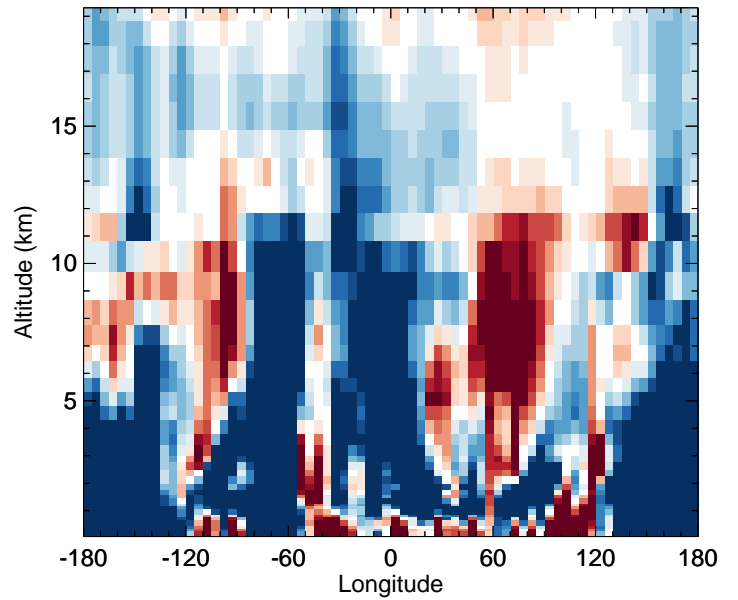
v11-02f-Run1 - v11-02e-Run0 OH - Diff along 42N for Apr
