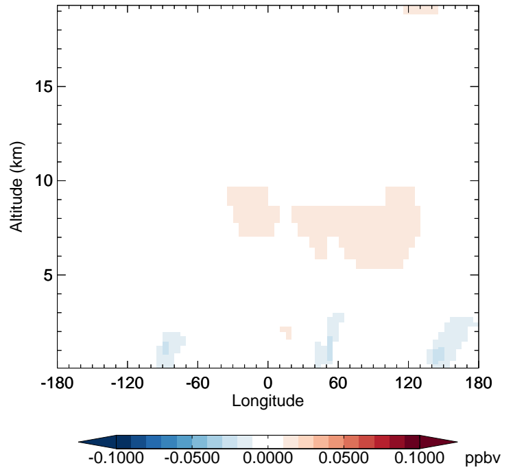
v11-02f-Run1 - v11-02e-Run1 H2O2 - Diff along 42N for Apr
