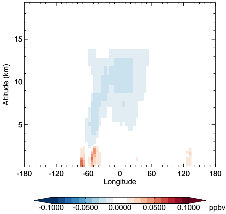
v11-02f-Run1 - v11-02e-Run1 PAN - Diff along 15S for Apr
