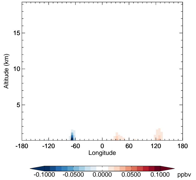
v11-02f-Run1 - v11-02e-Run1 SOAP - Diff along 42N for Apr
