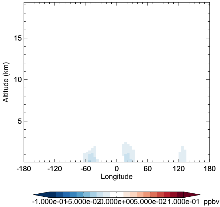
v11-02f-Run1 - v11-02e-Run0 MONITA - Diff along 15S for Apr
