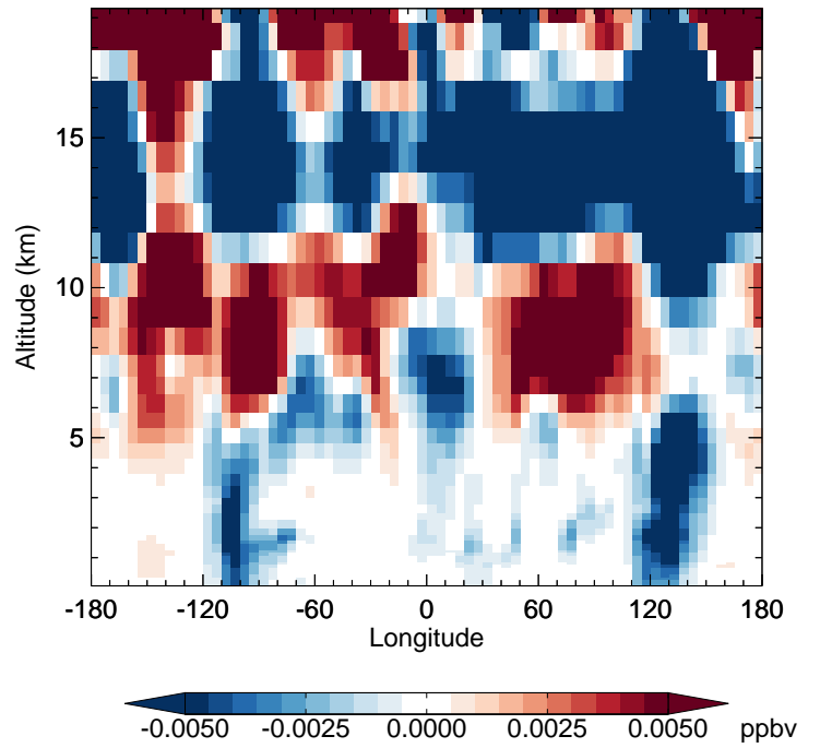
v11-02f-Run1 - v11-02e-Run0 HNO 4 - Diff along 42N for Apr
