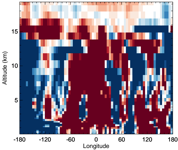
v11-02f-Run1 - v11-02e-Run0 OH - Diff along 15S for Apr
