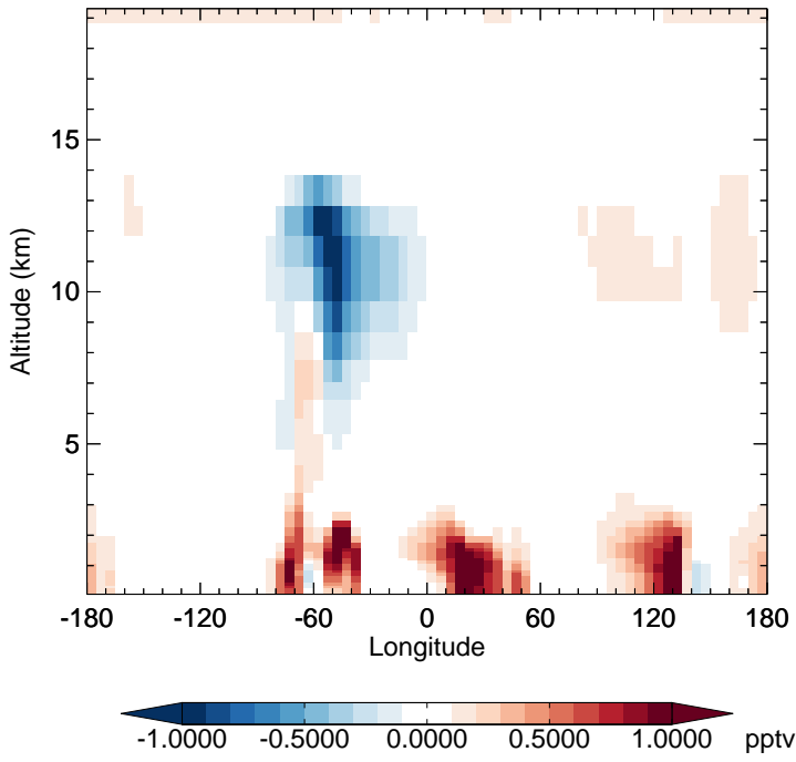
v11-02f-Run1 - v11-02e-Run1 HO2 - Diff along 15S for Apr
