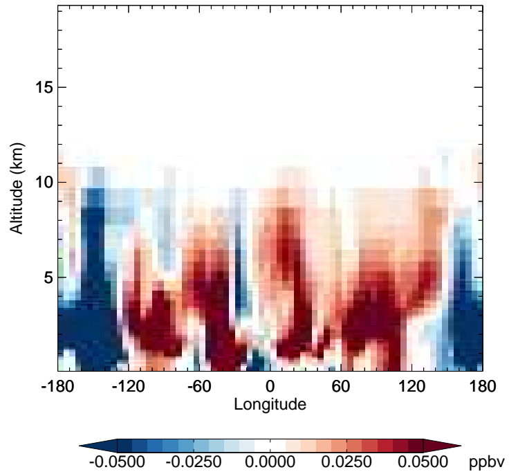
v11-02f-Run1 - v11-02e-Run0 MP - Diff along 42N for Apr
