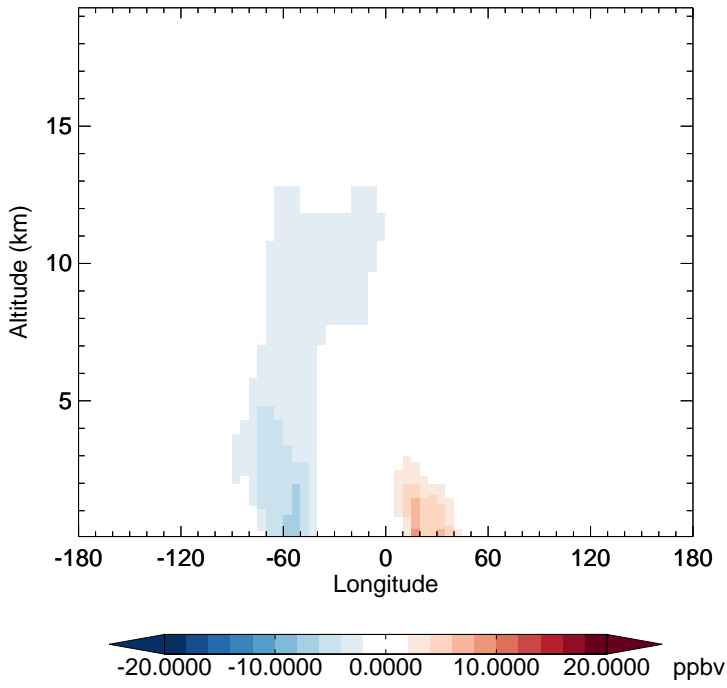
v11-02f-Run1 - v11-02e-Run1 CO - Diff along 15S for Apr
