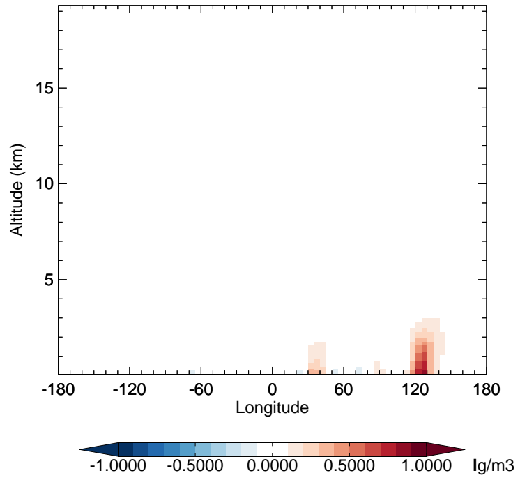
v11-02f-Run1 - v11-02e-Run1 OCPI - Diff along 42N for Apr
