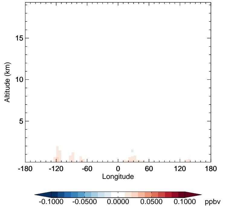
v11-02f-Run1 - v11-02e-Run0 TSOG3 - Diff along 42N for Apr
