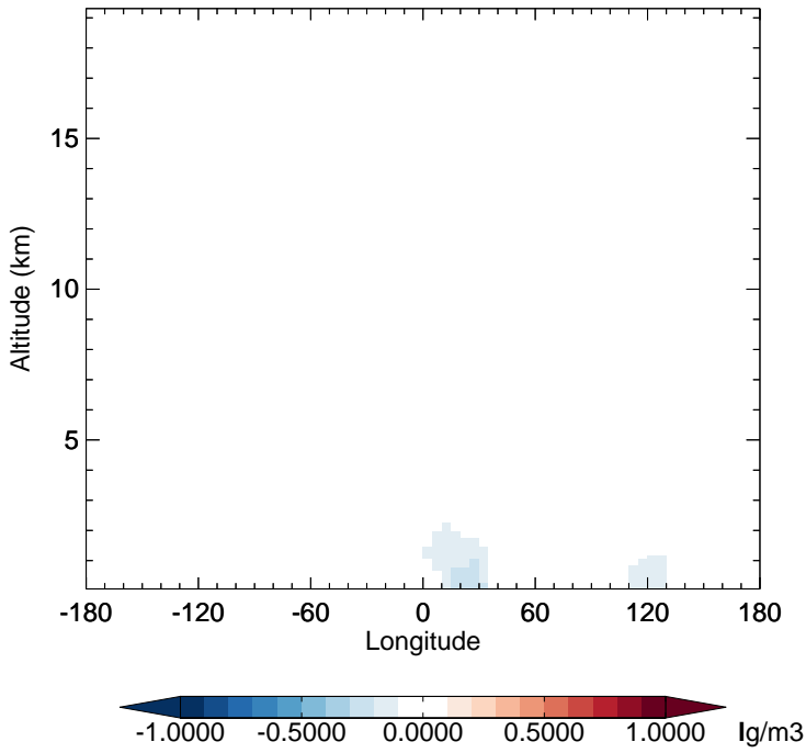
v11-02f-Run1 - v11-02e-Run1 NH4 - Diff along 15S for Apr
