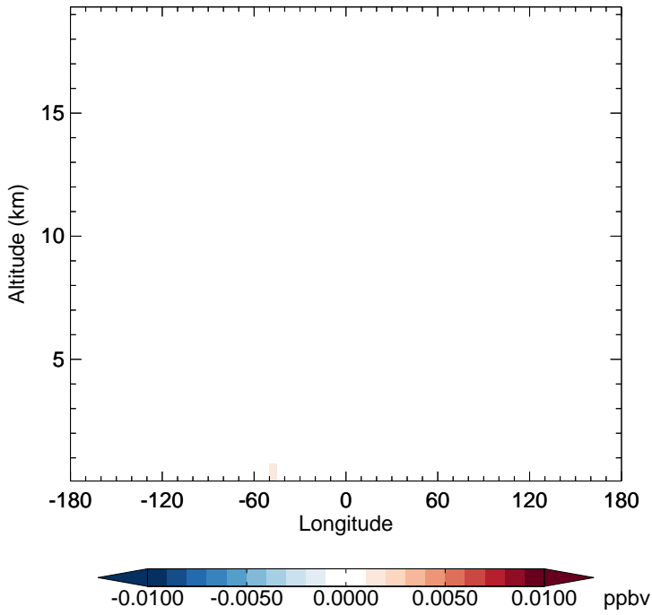
v11-02f-Run1 - v11-02e-Run1 NO3 - Diff along 15S for Apr
