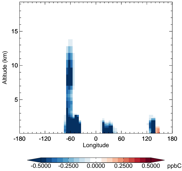
v11-02f-Run1 - v11-02e-Run1 ISOP - Diff along 15S for Apr
