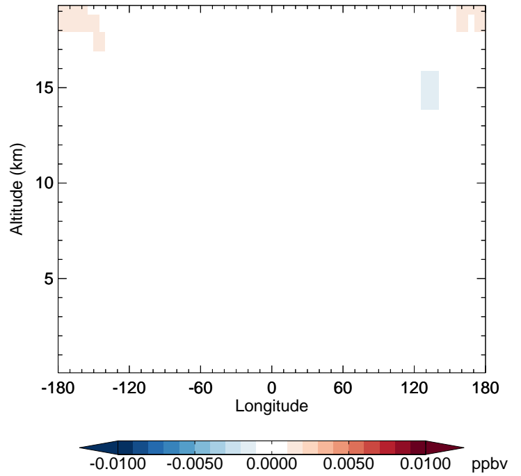
v11-02f-Run1 - v11-02e-Run0 BrNO3 - Diff along 42N for Apr
