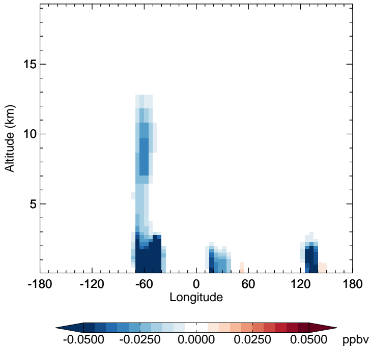
v11-02f-Run1 - v11-02e-Run1 MACR - Diff along 15S for Apr
