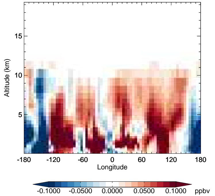
v11-02f-Run1 - v11-02e-Run0 H2O2 - Diff along 42N for Apr
