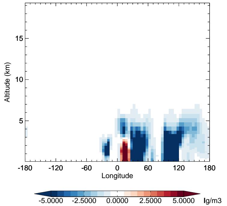
v11-02f-Run1 - v11-02e-Run0 DST3 - Diff along 42N for Apr
