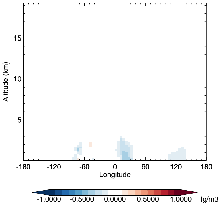
v11-02f-Run1 - v11-02e-Run0 NH4 - Diff along 15S for Apr
