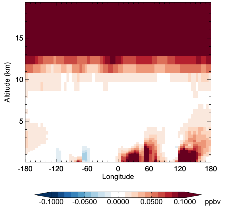
v11-02f-Run1 - v11-02e-Run1 HNO 3 - Diff along 42N for Apr
