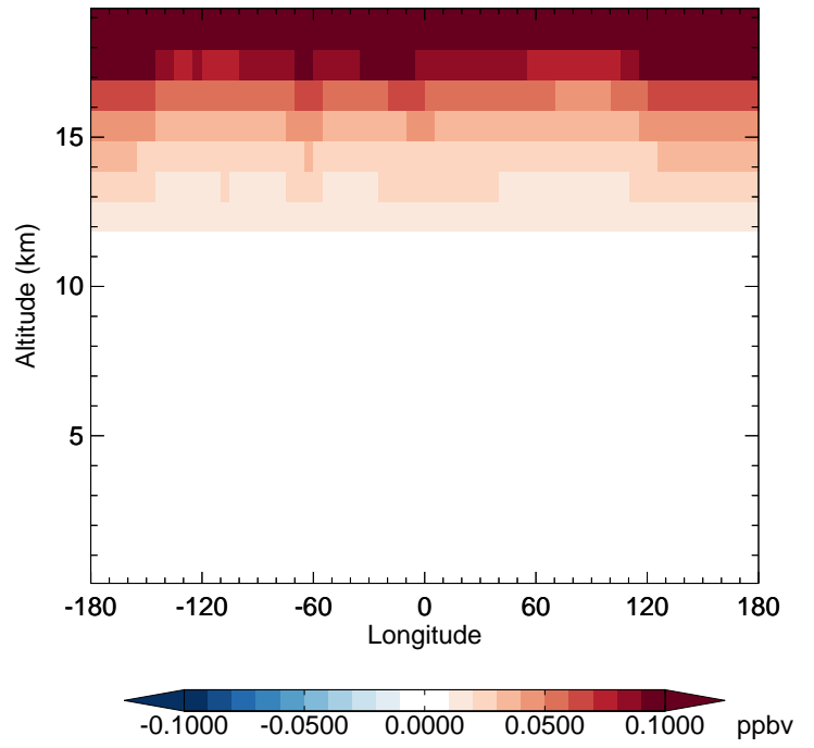
v11-02f-Run1 - v11-02e-Run1 N2O - Diff along 42N for Apr
