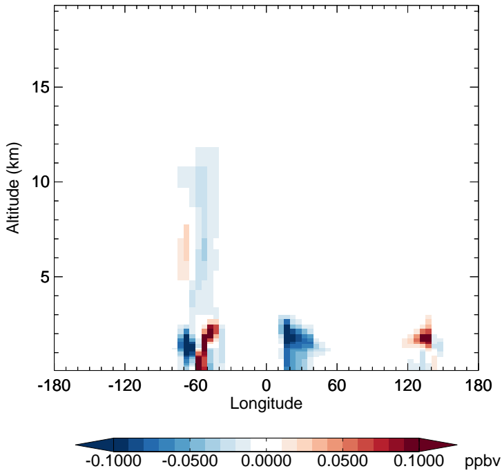
v11-02f-Run1 - v11-02e-Run0 GLYC - Diff along 15S for Apr
