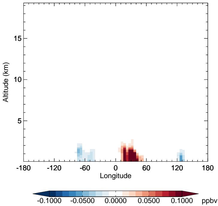
v11-02f-Run1 - v11-02e-Run0 TOLU - Diff along 15S for Apr
