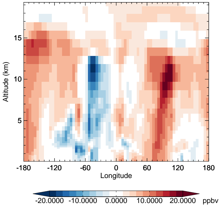
v11-02f-Run1 - v11-02e-Run0 CO - Diff along 15S for Apr
