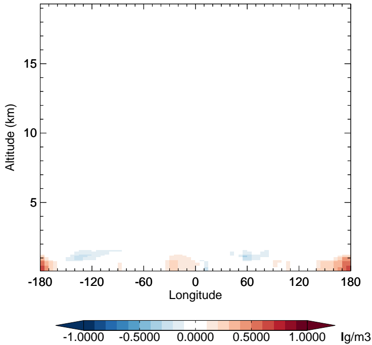
v11-02f-Run1 - v11-02e-Run0 SALA - Diff along 15S for Apr
