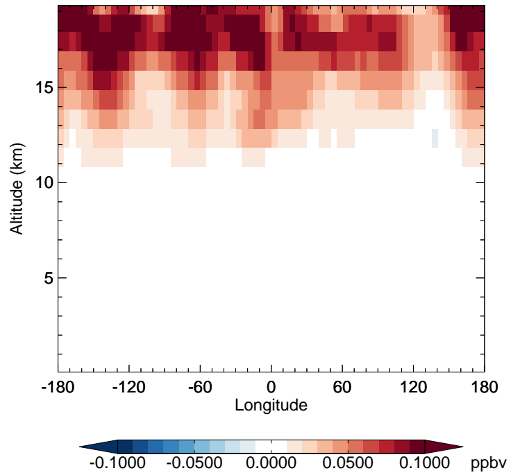
v11-02f-Run1 - v11-02e-Run0 HCl - Diff along 42N for Apr
