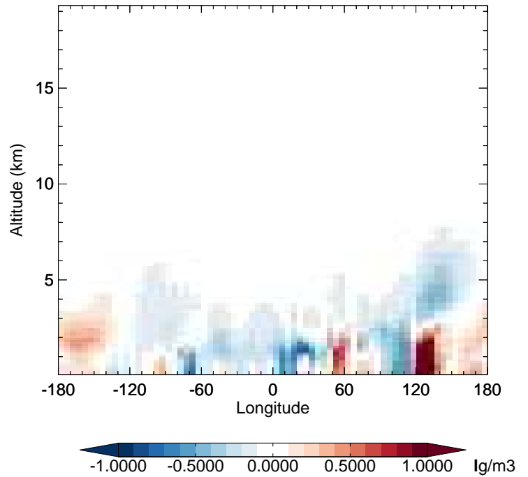
v11-02f-Run1 - v11-02e-Run0 SO4 - Diff along 42N for Apr
