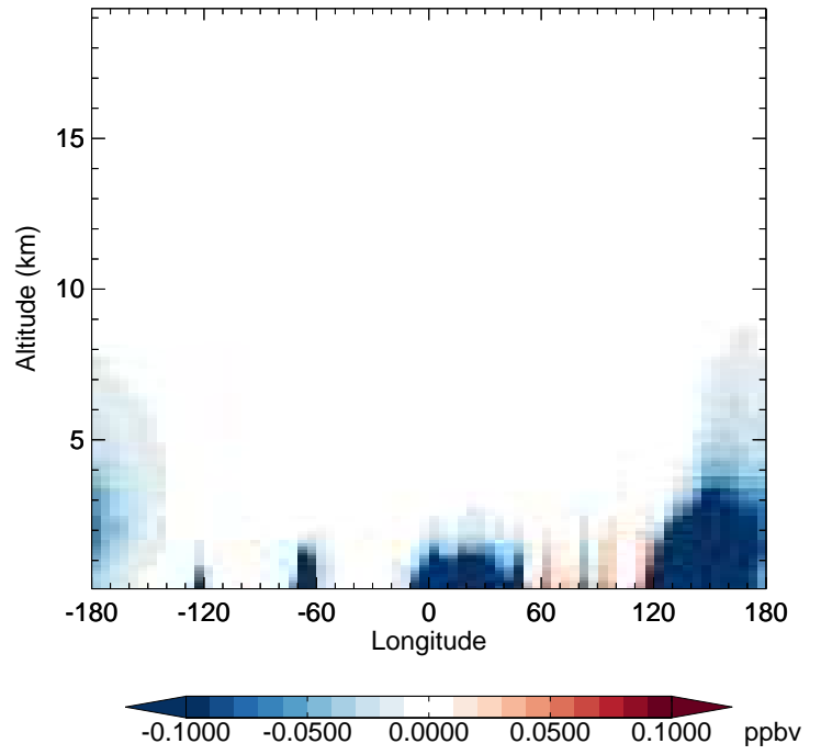
v11-02f-Run1 - v11-02e-Run1 TOLU - Diff along 42N for Apr
