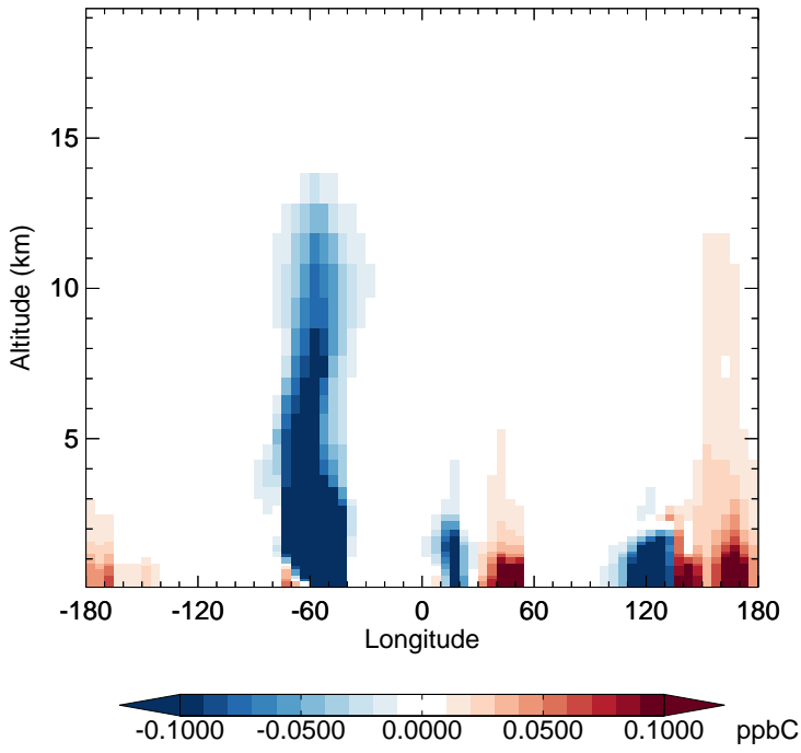
v11-02f-Run1 - v11-02e-Run1 MEK - Diff along 15S for Apr
