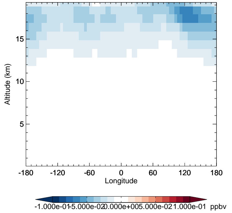
v11-02f-Run1 - v11-02e-Run1 CINO3 - Diff along 42N for Apr
