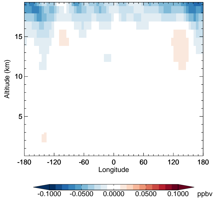
v11-02f-Run1 - v11-02e-Run0 CH3Cl - Diff along 42N for Apr
