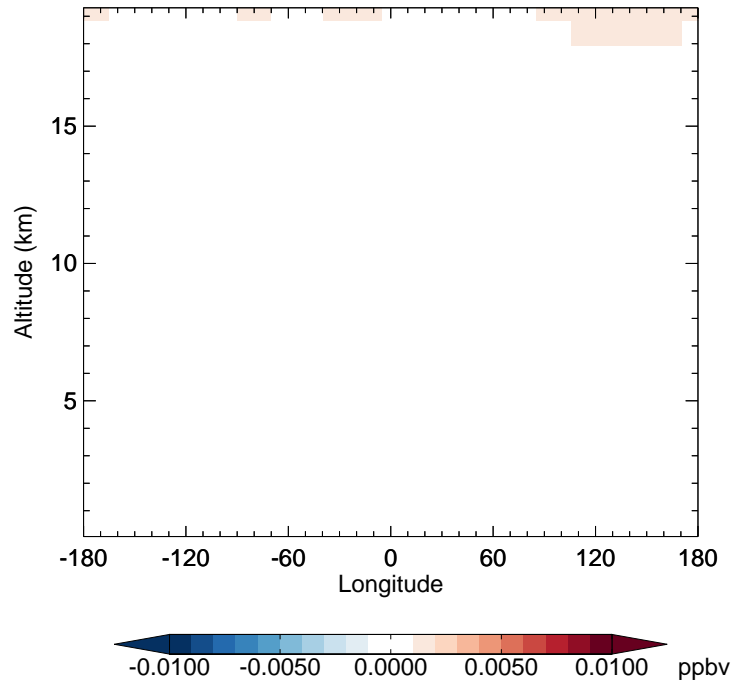
v11-02f-Run1 - v11-02e-Run1 BrO - Diff along 42N for Apr
