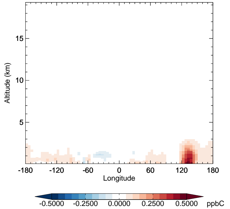
v11-02f-Run1 - v11-02e-Run0 ALD2 - Diff along 42N for Apr
