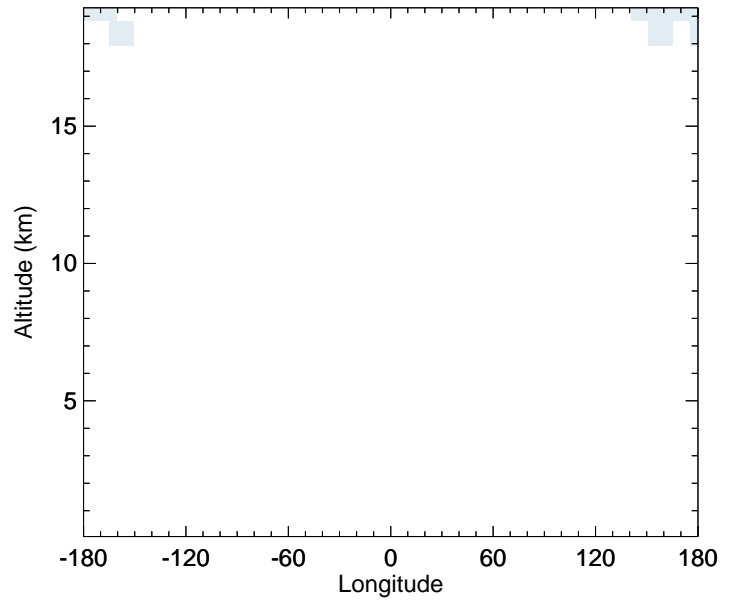
v11-02f-Run1 - v11-02e-Run0 CFC113 - Diff along 42N for Apr
