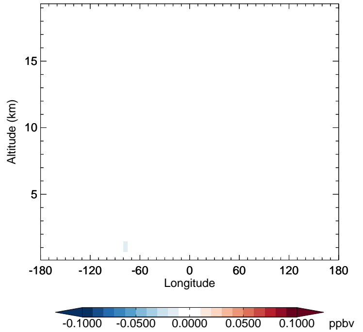
v11-02f-Run1 - v11-02e-Run0 ISO3 - Diff along 42N for Apr
