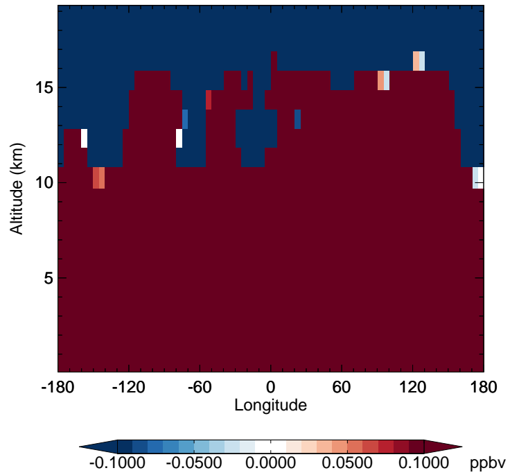
v11-02f-Run1 - v11-02e-Run0 N2O - Diff along 42N for Apr
