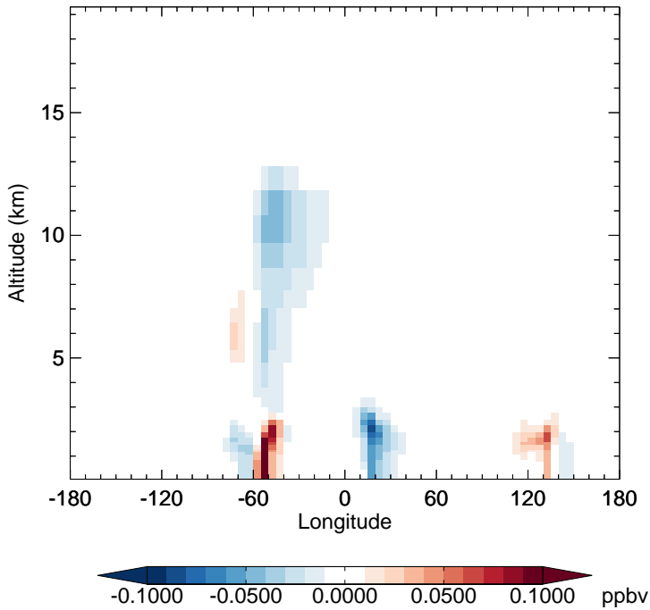
v11-02f-Run1 - v11-02e-Run0 IMAE - Diff along 15S for Apr
