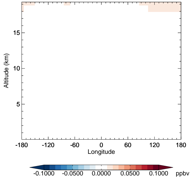
v11-02f-Run1 - v11-02e-Run0 ClO - Diff along 42N for Apr
