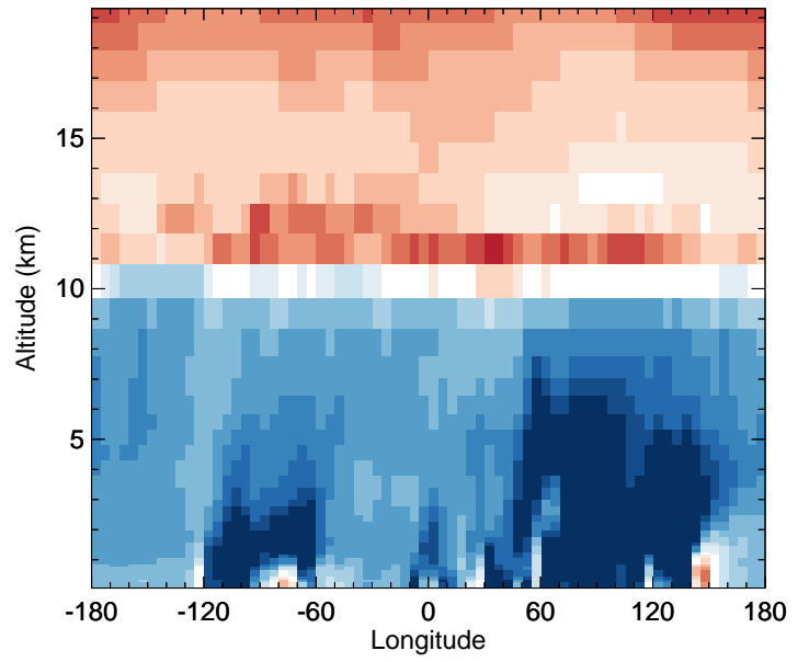
v11-02f-Run1 - v11-02e-Run1 OH - Diff along 42N for Apr
