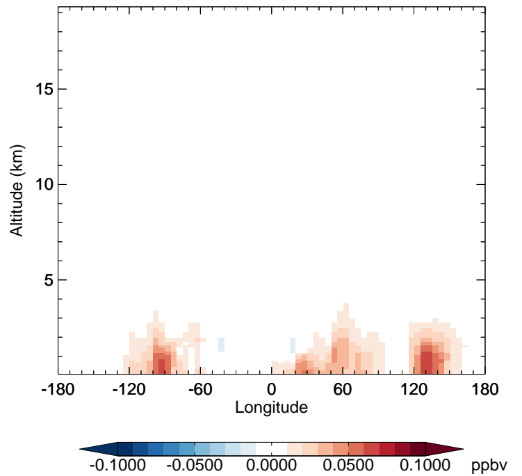
v11-02f-Run1 - v11-02e-Run0 INDIOL - Diff along 42N for Apr
