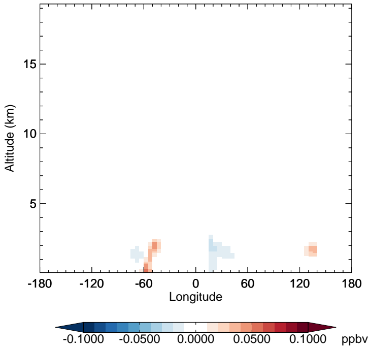
v11-02f-Run1 - v11-02e-Run0 MGLY - Diff along 15S for Apr
