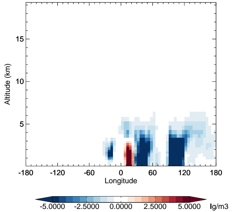
v11-02f-Run1 - v11-02e-Run0 DST2 - Diff along 42N for Apr
