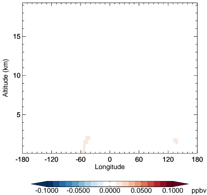
v11-02f-Run1 - v11-02e-Run0 GLYX - Diff along 15S for Apr
