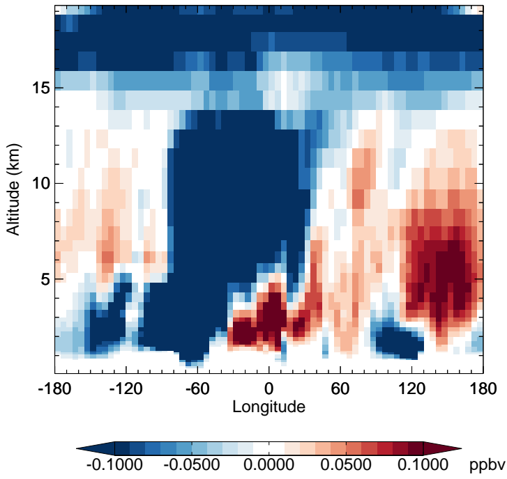
v11-02f-Run1 - v11-02e-Run1 CH4 - Diff along 15S for Apr
