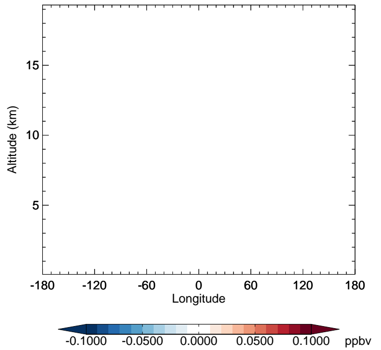
v11-02f-Run1 - v11-02e-Run0 HCFC141b - Diff along 42N for Apr
