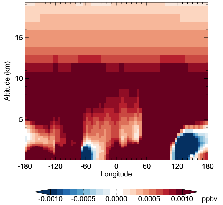
v11-02f-Run1 - v11-02e-Run1 PPN - Diff along 42N for Apr
