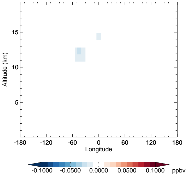
v11-02f-Run1 - v11-02e-Run0 ISOA3 - Diff along 15S for Apr
