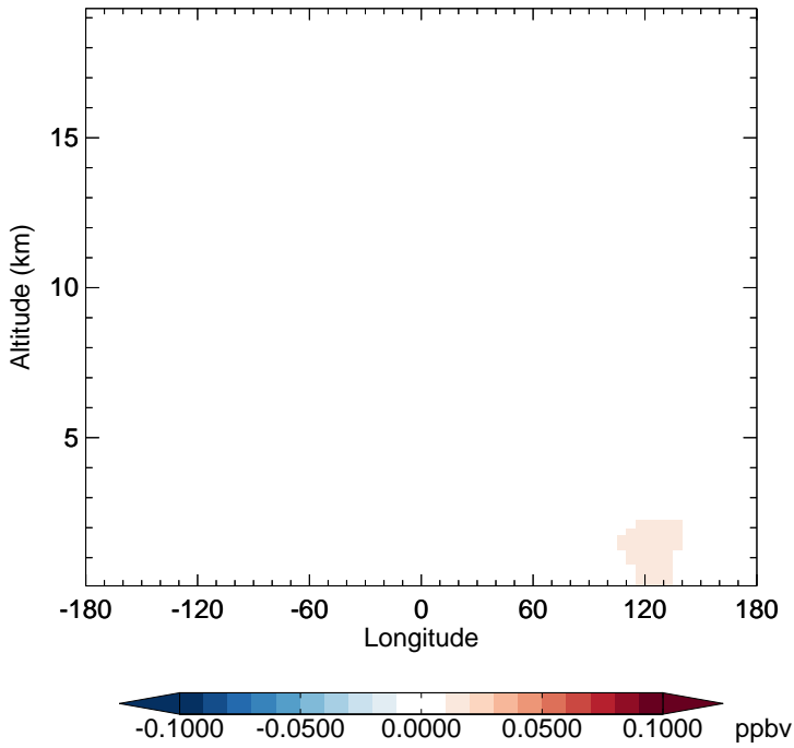
v11-02f-Run1 - v11-02e-Run0 ISOG1 - Diff along 15S for Apr
