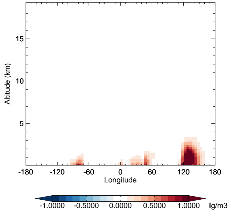
v11-02f-Run1 - v11-02e-Run1 NIT - Diff along 42N for Apr
