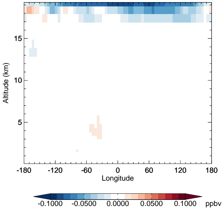
v11-02f-Run1 - v11-02e-Run0 HCl - Diff along 15S for Apr
