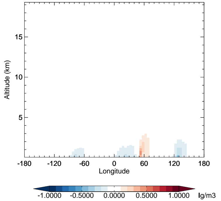
v11-02f-Run1 - v11-02e-Run1 SO4 - Diff along 42N for Apr
