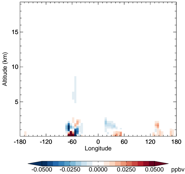
v11-02f-Run1 - v11-02e-Run0 RCHO - Diff along 15S for Apr
