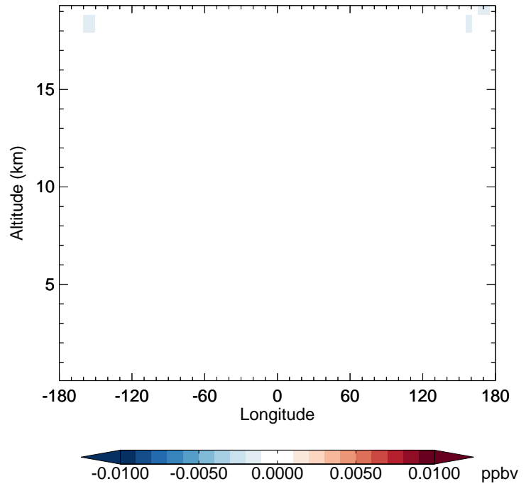
v11-02f-Run1 - v11-02e-Run0 CH3Br - Diff along 42N for Apr
