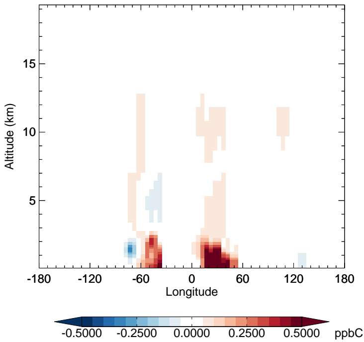
v11-02f-Run1 - v11-02e-Run0 ALK4 - Diff along 15S for Apr
