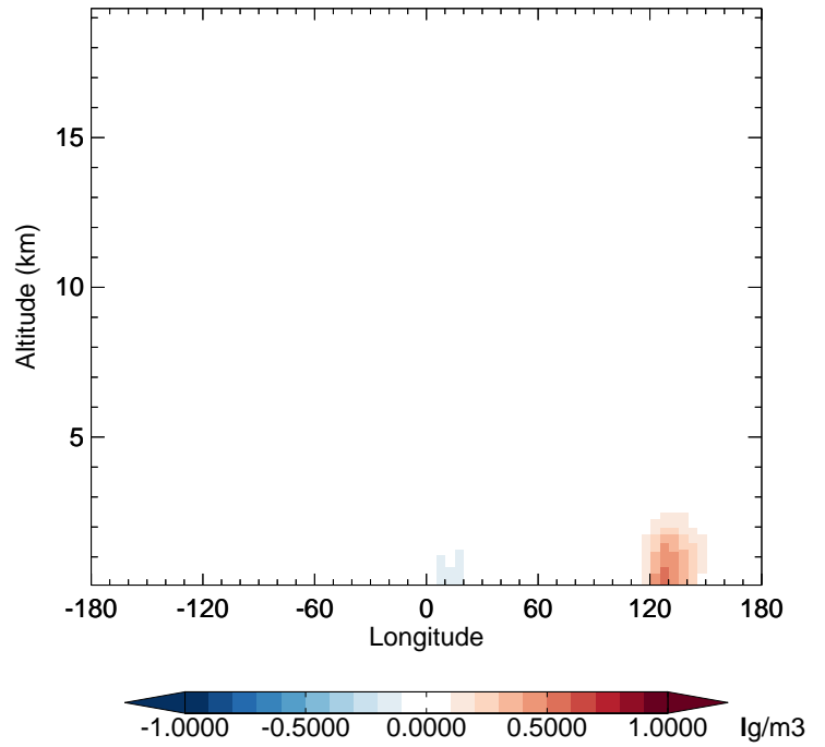
v11-02f-Run1 - v11-02e-Run0 BCPI - Diff along 42N for Apr
