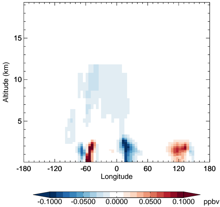
v11-02f-Run1 - v11-02e-Run0 ISO3 - Diff along 15S for Apr
