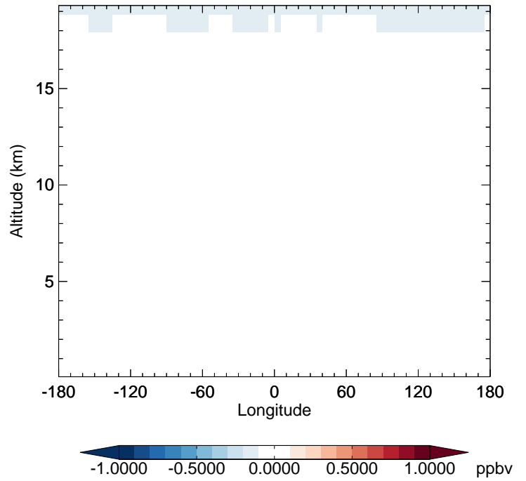
v11-02f-Run1 - v11-02e-Run0 NO - Diff along 42N for Apr
