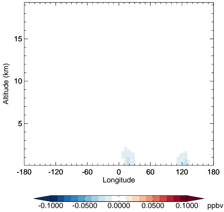
v11-02f-Run1 - v11-02e-Run1 SOAGX - Diff along 15S for Apr
