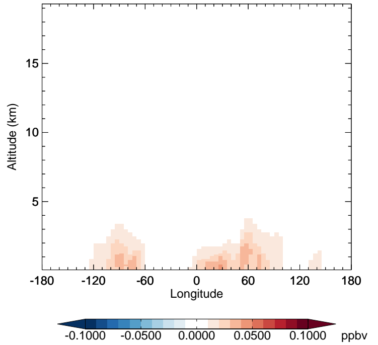
v11-02f-Run1 - v11-02e-Run1 INDIOL - Diff along 42N for Apr
