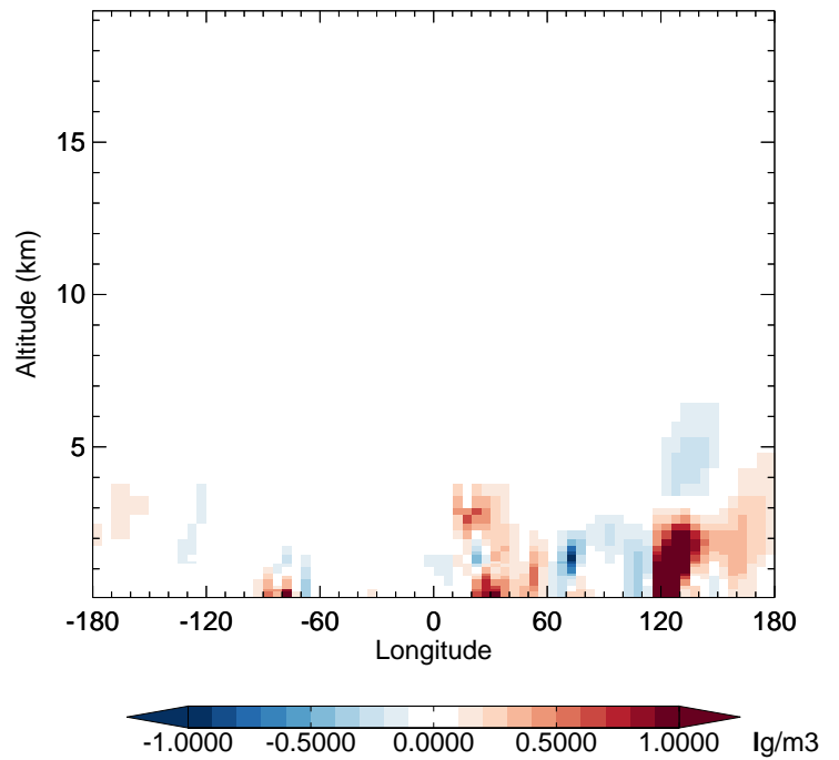
v11-02f-Run1 - v11-02e-Run0 SO 2 - Diff along 42N for Apr
