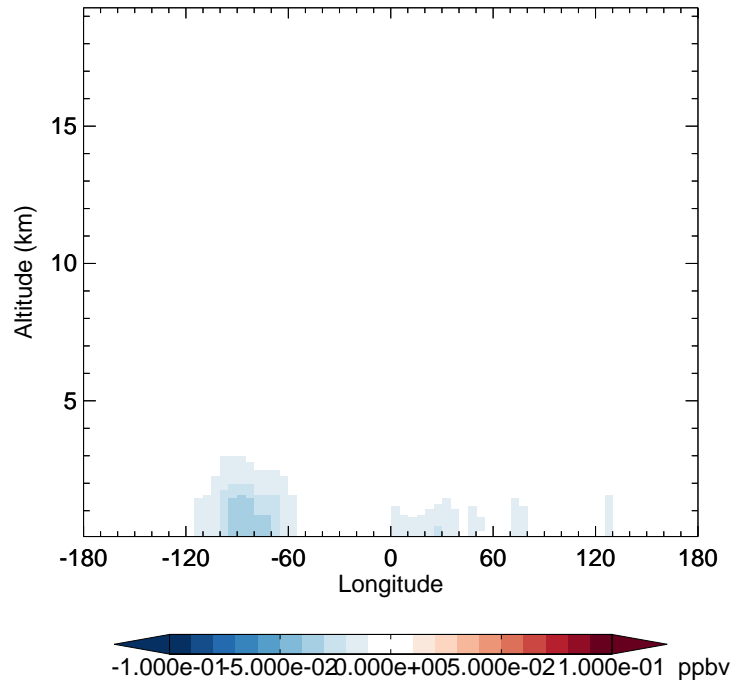
v11-02f-Run1 - v11-02e-Run1 IONITA - Diff along 42N for Apr
