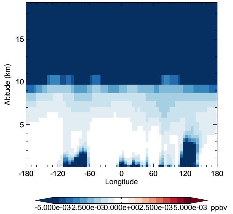
v11-02f-Run1 - v11-02e-Run1 N2O5 - Diff along 42N for Apr
