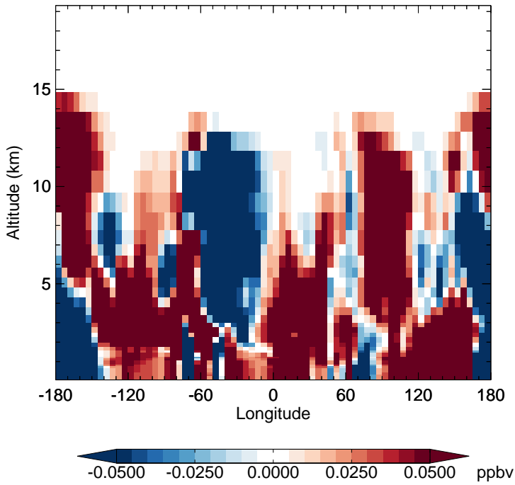
v11-02f-Run1 - v11-02e-Run0 MP - Diff along 15S for Apr
