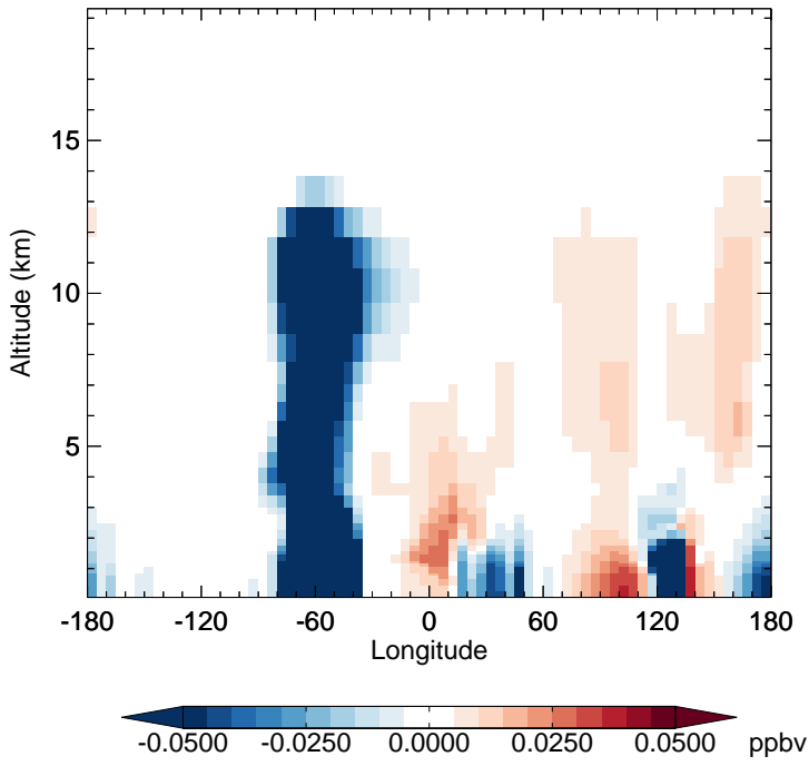
v11-02f-Run1 - v11-02e-Run1 MP - Diff along 15S for Apr
