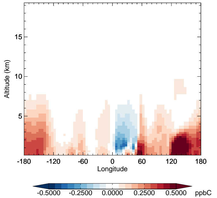
v11-02f-Run1 - v11-02e-Run0 C3H8 - Diff along 42N for Apr
