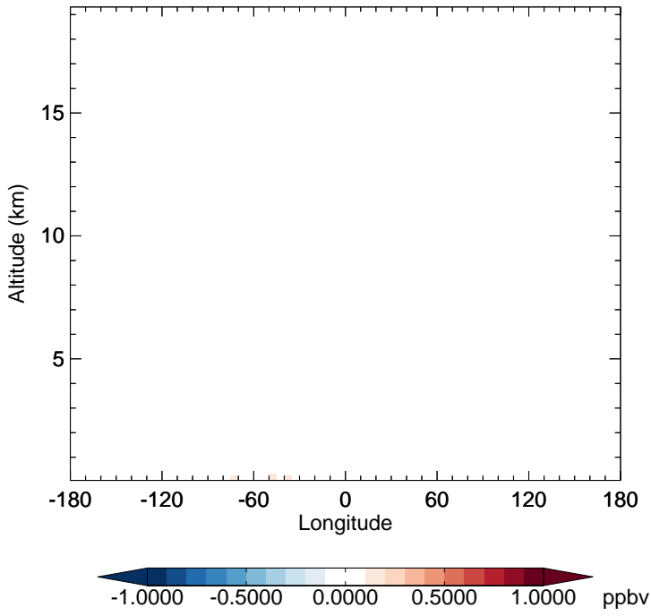
v11-02f-Run1 - v11-02e-Run1 NO 2 - Diff along 15S for Apr
