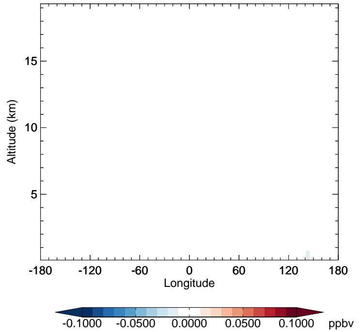
v11-02f-Run1 - v11-02e-Run0 MGLY - Diff along 42N for Apr
