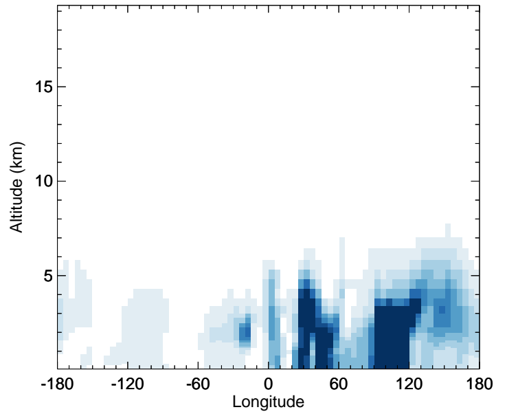
v11-02f-Run1 - v11-02e-Run0 DST1 - Diff along 42N for Apr
