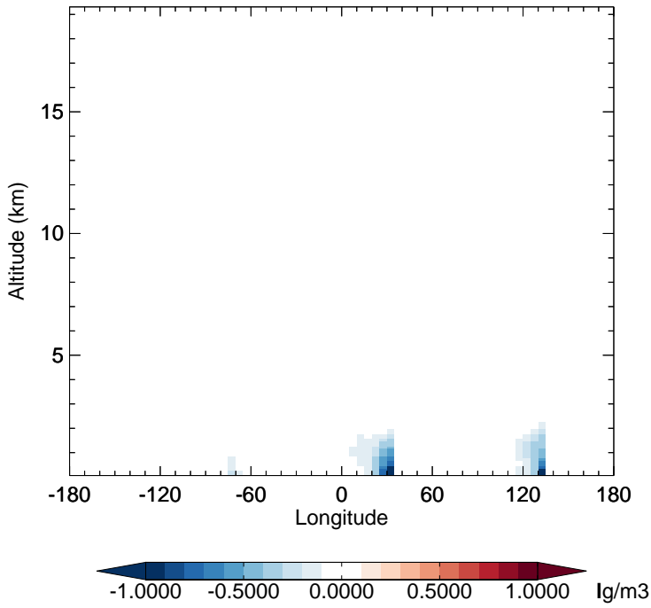
v11-02f-Run1 - v11-02e-Run1 SO 2 - Diff along 15S for Apr
