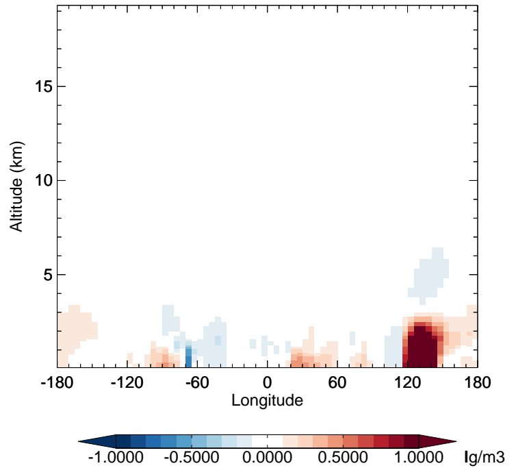
v11-02f-Run1 - v11-02e-Run0 SOAS - Diff along 42N for Apr
