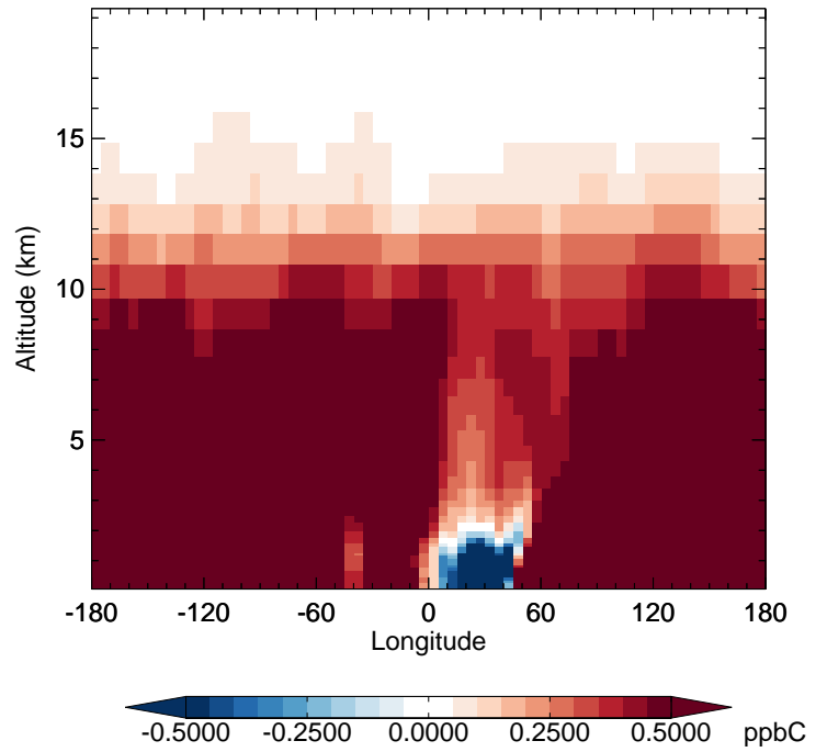
v11-02f-Run1 - v11-02e-Run0 C2H6 - Diff along 42N for Apr
