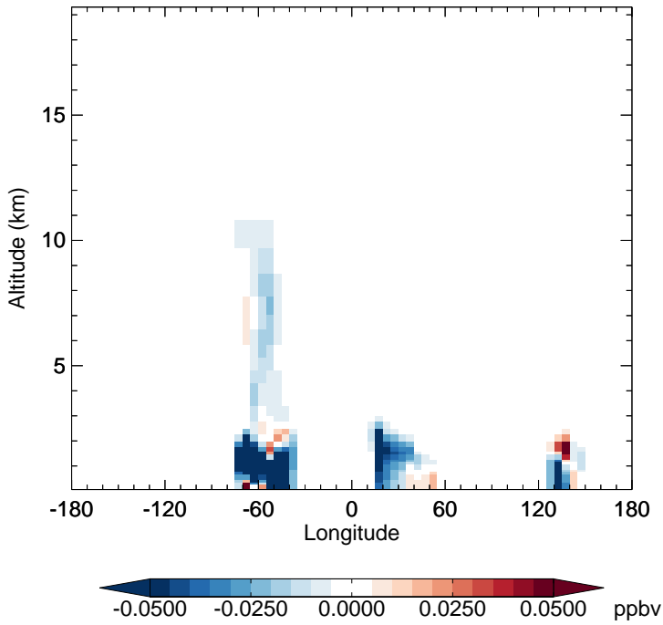
v11-02f-Run1 - v11-02e-Run0 MACR - Diff along 15S for Apr
