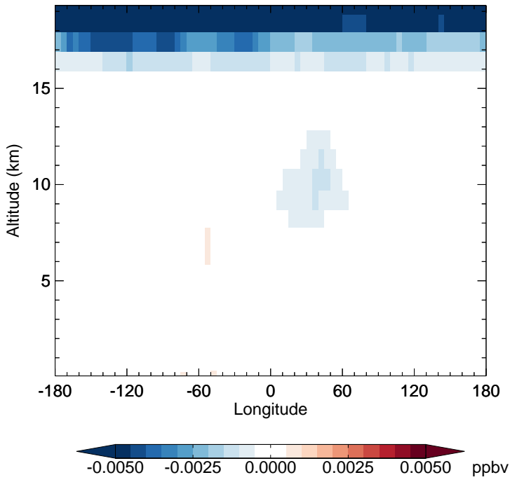
v11-02f-Run1 - v11-02e-Run1 N2O5 - Diff along 15S for Apr
