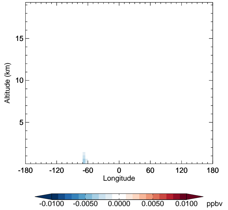
v11-02f-Run1 - v11-02e-Run1 R4N2 - Diff along 42N for Apr
