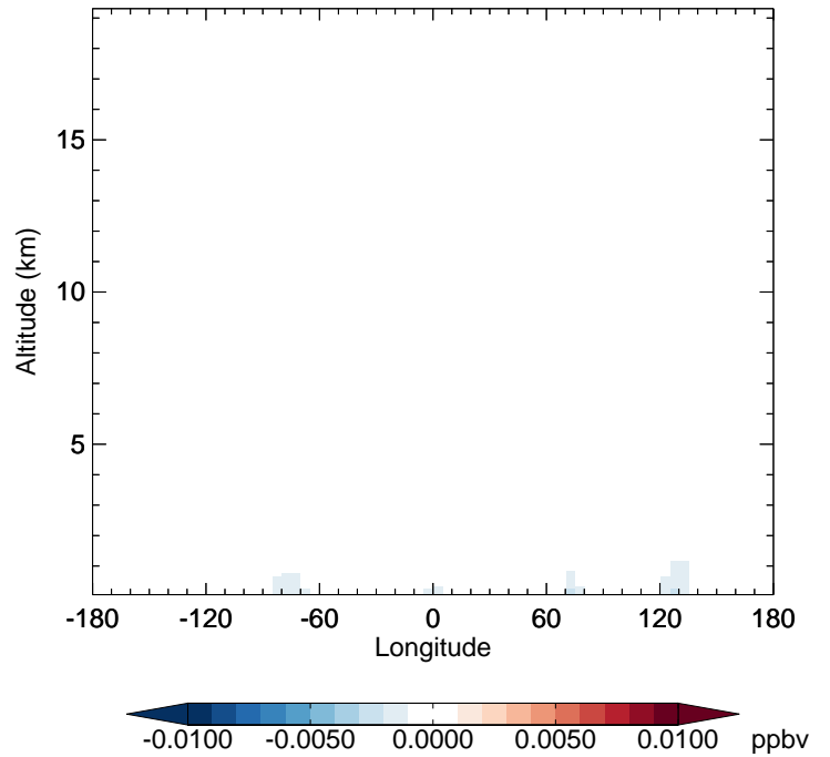
v11-02f-Run1 - v11-02e-Run0 NO3 - Diff along 42N for Apr
