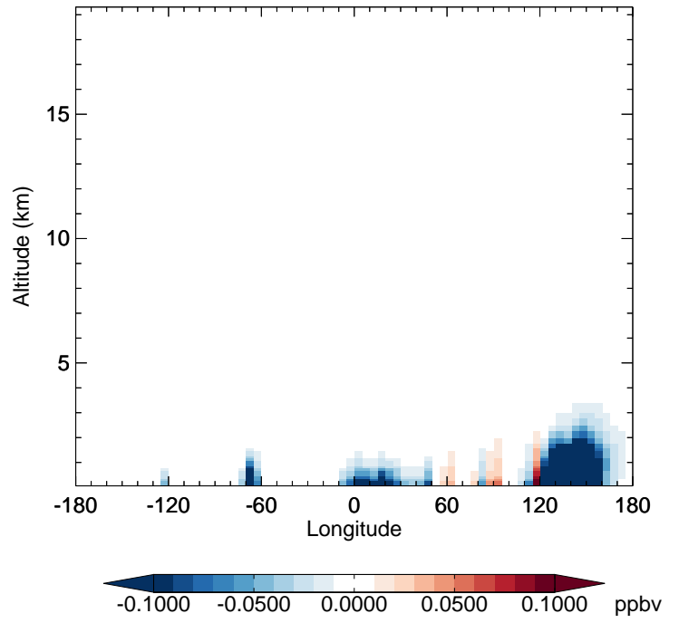
v11-02f-Run1 - v11-02e-Run1 XYLE - Diff along 42N for Apr
