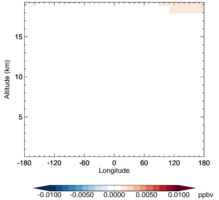
v11-02f-Run1 - v11-02e-Run0 BrO - Diff along 42N for Apr
