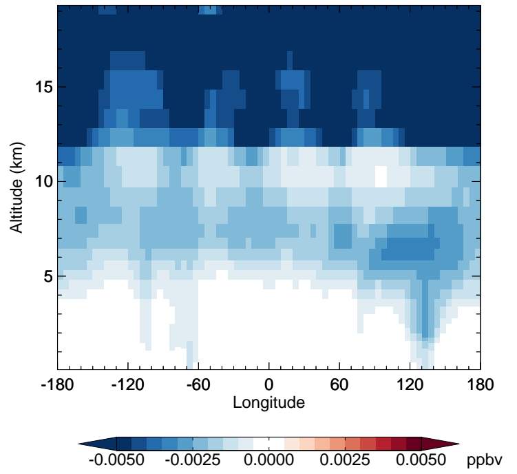
v11-02f-Run1 - v11-02e-Run1 HNO 4 - Diff along 42N for Apr
