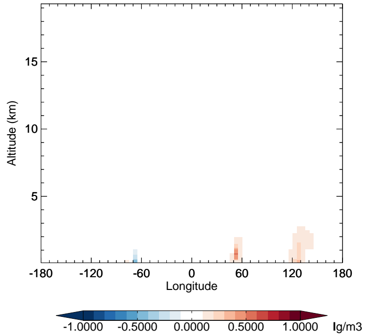
v11-02f-Run1 - v11-02e-Run1 SO 2 - Diff along 42N for Apr
