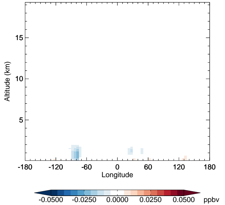
v11-02f-Run1 - v11-02e-Run0 MVK - Diff along 42N for Apr
