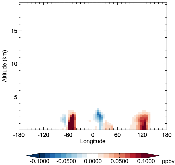
v11-02f-Run1 - v11-02e-Run0 INDIOL - Diff along 15S for Apr
