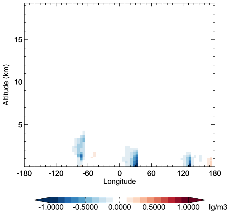
v11-02f-Run1 - v11-02e-Run0 SO 2 - Diff along 15S for Apr
