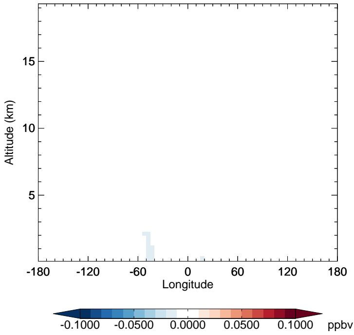
v11-02f-Run1 - v11-02e-Run1 ISOG1 - Diff along 15S for Apr
