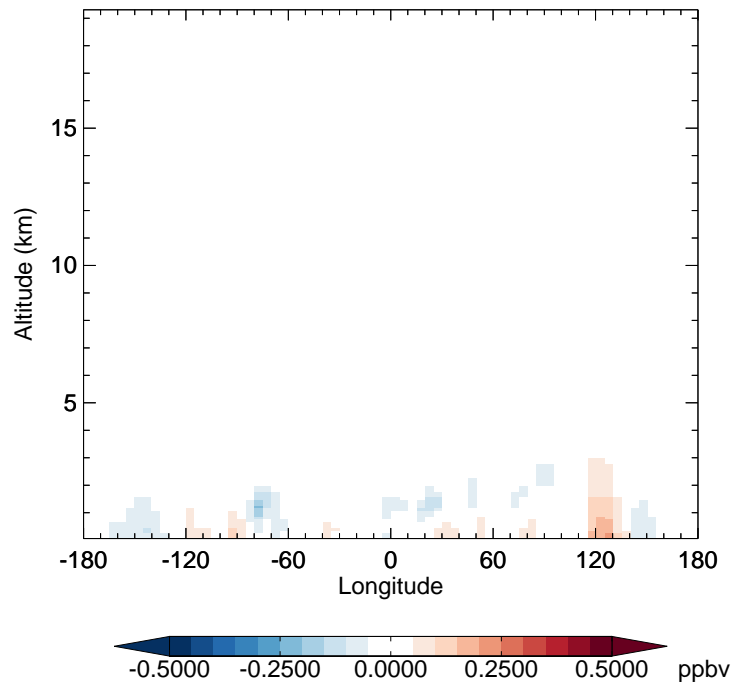
v11-02f-Run1 - v11-02e-Run0 CH 2 O - Diff along 42N for Apr
