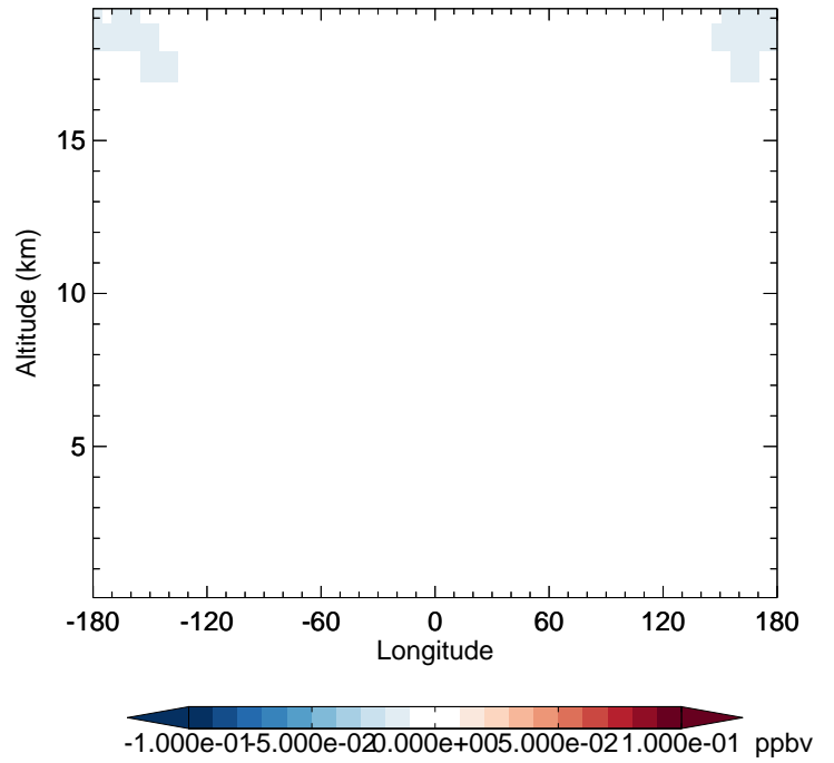
v11-02f-Run1 - v11-02e-Run0 CCI4 - Diff along 42N for Apr
