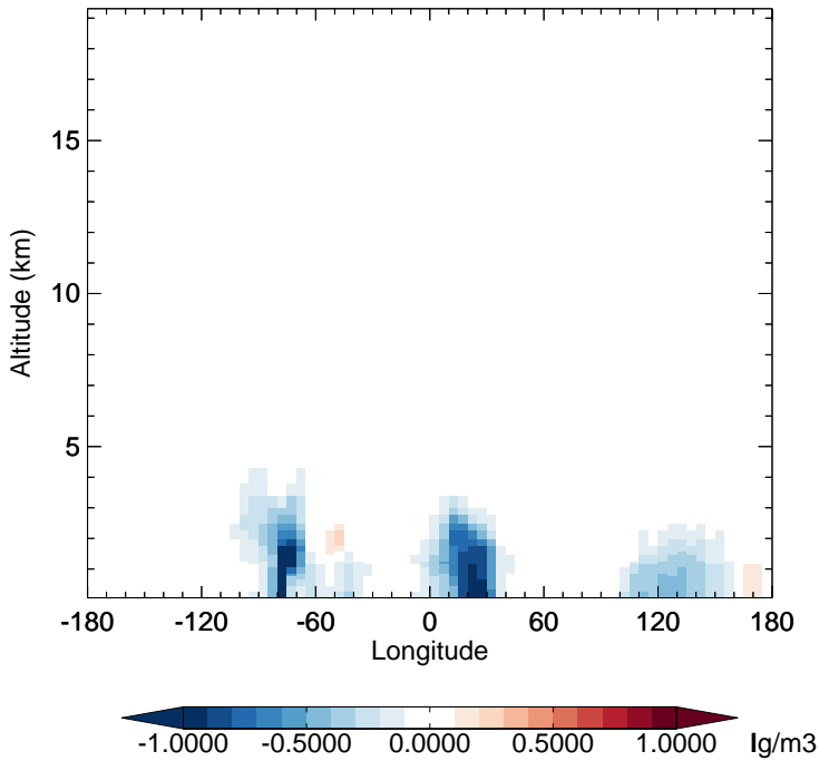
v11-02f-Run1 - v11-02e-Run0 SO4 - Diff along 15S for Apr
