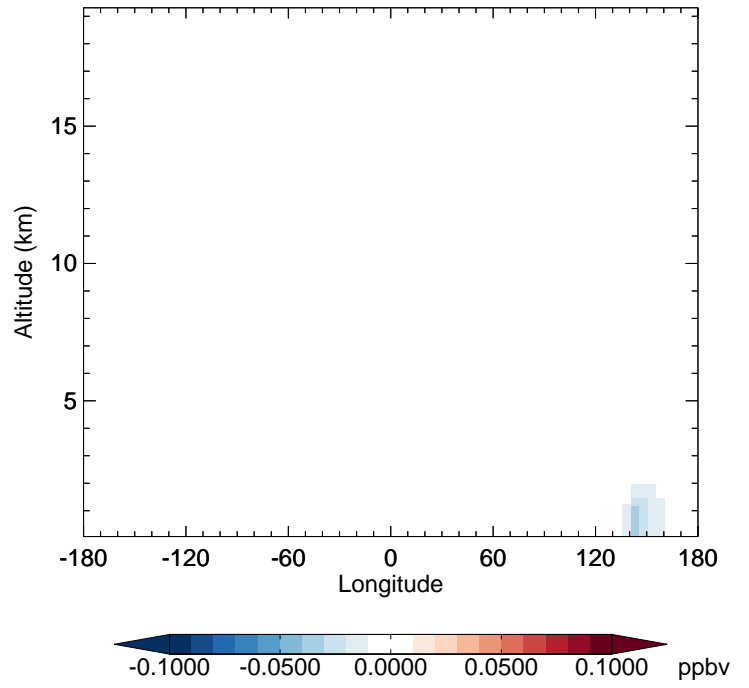
v11-02f-Run1 - v11-02e-Run1 ASOAN - Diff along 42N for Apr
