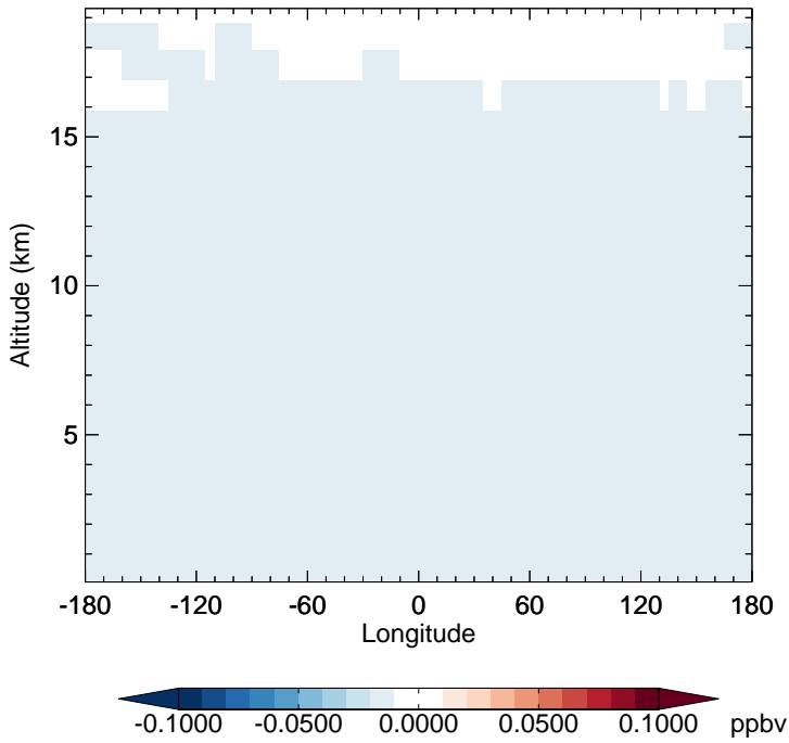
v11-02f-Run1 - v11-02e-Run0 CFC12 - Diff along 15S for Apr
