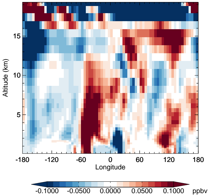
v11-02f-Run1 - v11-02e-Run0 HNO 3 - Diff along 15S for Apr
