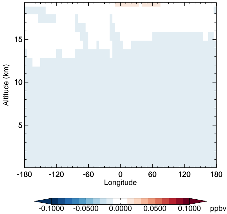
v11-02f-Run1 - v11-02e-Run0 CFC11 - Diff along 15S for Apr
