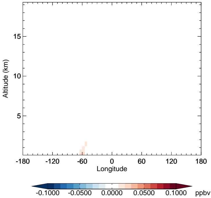
v11-02f-Run1 - v11-02e-Run0 TSOA1 - Diff along 15S for Apr
