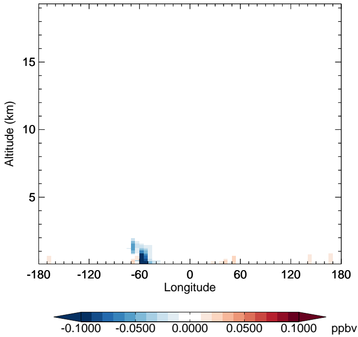
v11-02f-Run1 - v11-02e-Run0 MTPA - Diff along 15S for Apr
