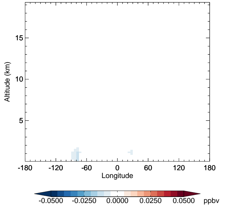
v11-02f-Run1 - v11-02e-Run0 MACR - Diff along 42N for Apr
