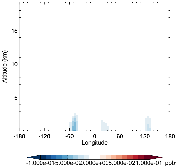
v11-02f-Run1 - v11-02e-Run1 MONITA - Diff along 15S for Apr
