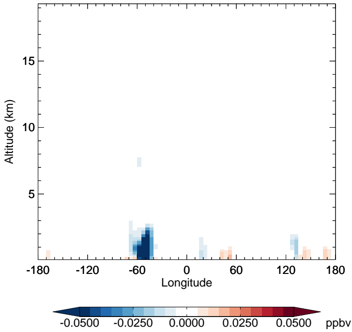
v11-02f-Run1 - v11-02e-Run1 RCHO - Diff along 15S for Apr
