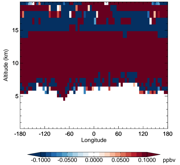
v11-02f-Run1 - v11-02e-Run1 H2O - Diff along 42N for Apr
