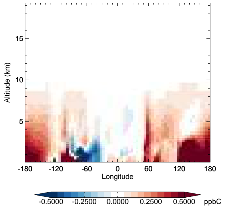
v11-02f-Run1 - v11-02e-Run0 ALK4 - Diff along 42N for Apr
