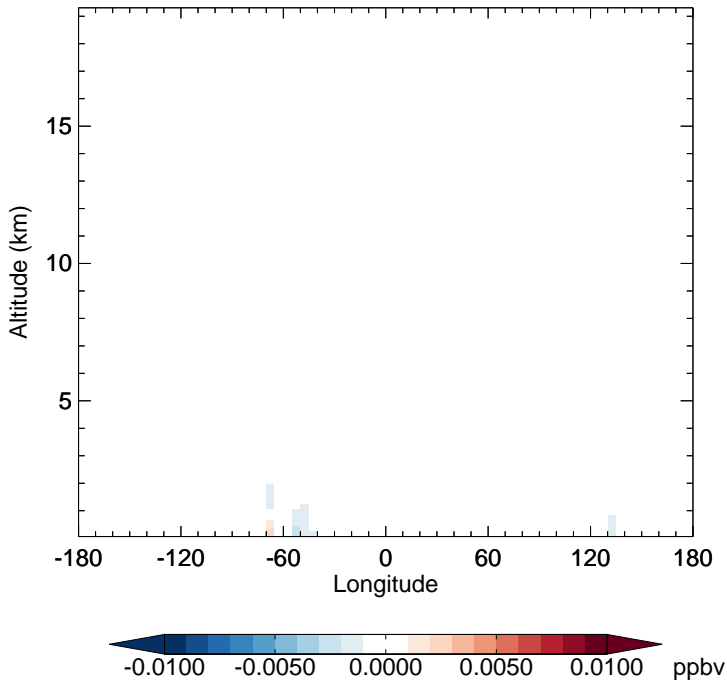
v11-02f-Run1 - v11-02e-Run0 MOBA - Diff along 15S for Apr
