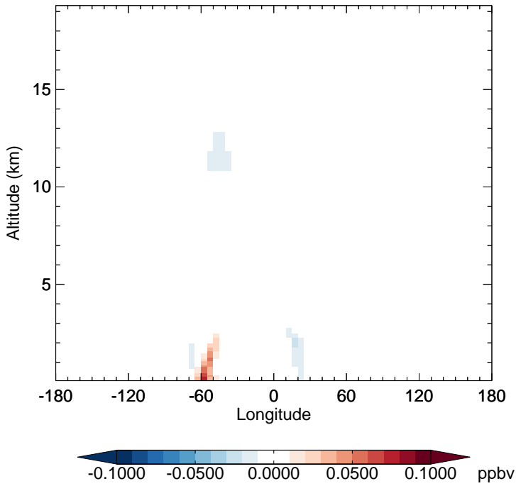
v11-02f-Run1 - v11-02e-Run0 TSOA2 - Diff along 15S for Apr
