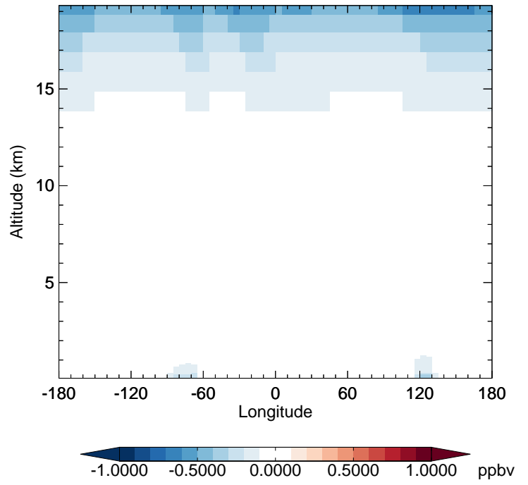
v11-02f-Run1 - v11-02e-Run1 NO 2 - Diff along 42N for Apr
