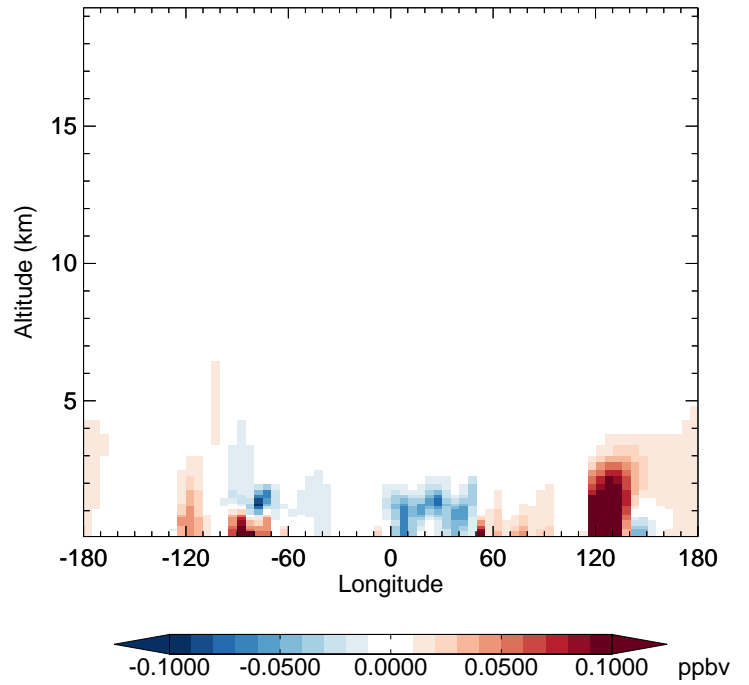
v11-02f-Run1 - v11-02e-Run0 EOH - Diff along 42N for Apr
