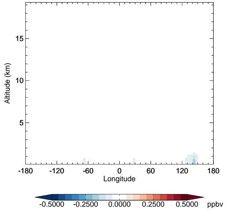
v11-02f-Run1 - v11-02e-Run1 CH 2 O - Diff along 42N for Apr
