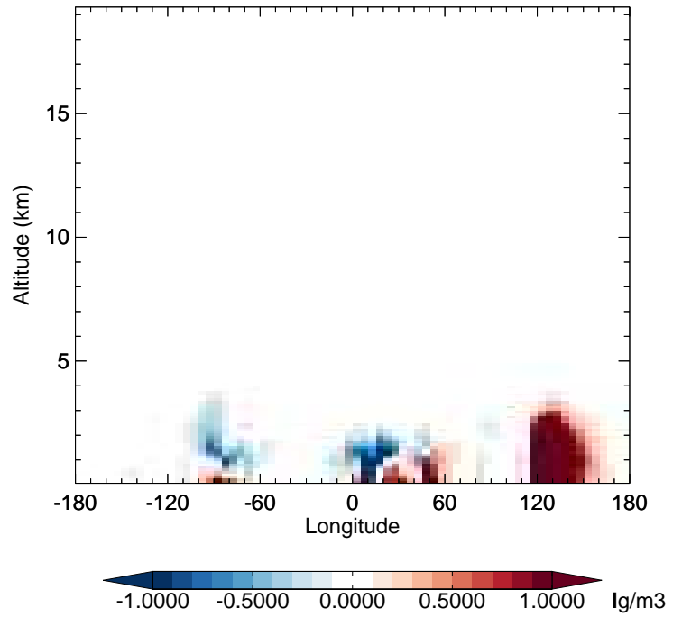
v11-02f-Run1 - v11-02e-Run0 NIT - Diff along 42N for Apr
