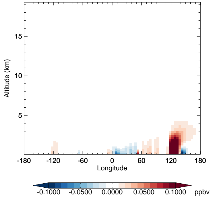
v11-02f-Run1 - v11-02e-Run1 EOH - Diff along 42N for Apr
