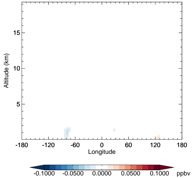
v11-02f-Run1 - v11-02e-Run0 GLYC - Diff along 42N for Apr
