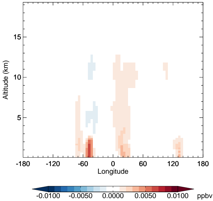
v11-02f-Run1 - v11-02e-Run0 R4N2 - Diff along 15S for Apr
