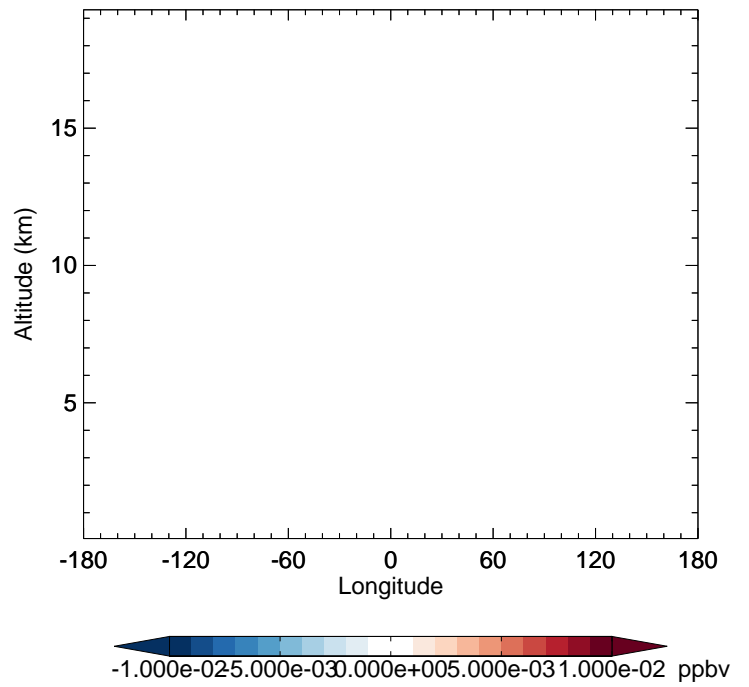
v11-02f-Run1 - v11-02e-Run0 Br - Diff along 42N for Apr
