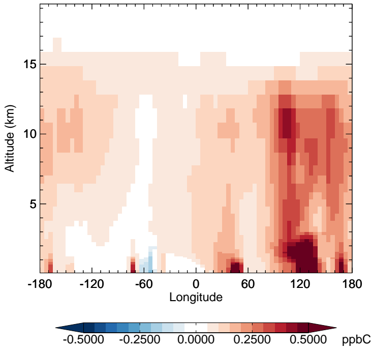
v11-02f-Run1 - v11-02e-Run1 ACET - Diff along 15S for Apr
