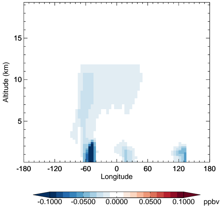
v11-02f-Run1 - v11-02e-Run1 ISO3 - Diff along 15S for Apr
