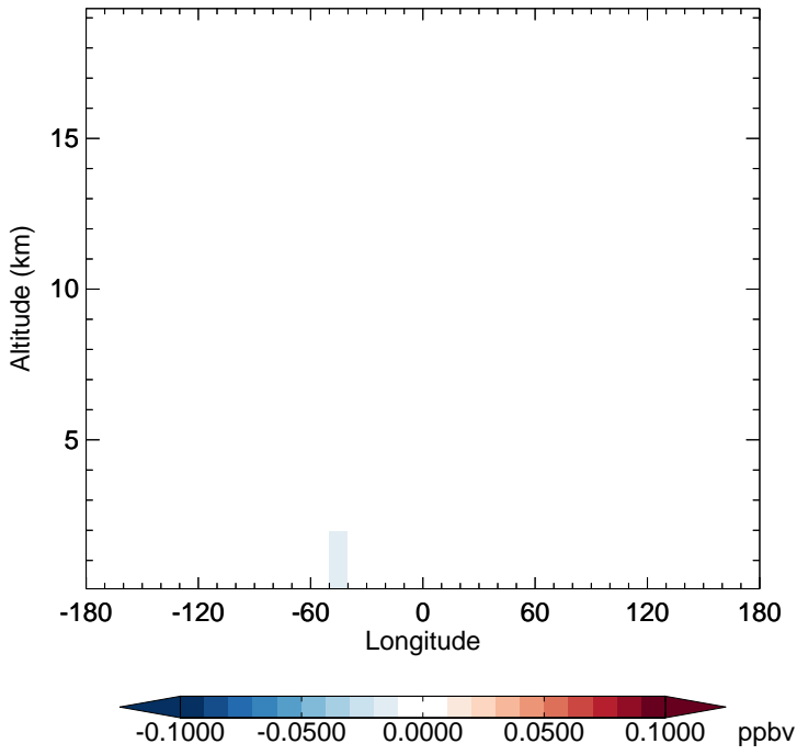
v11-02f-Run1 - v11-02e-Run1 ISOPNB - Diff along 15S for Apr
