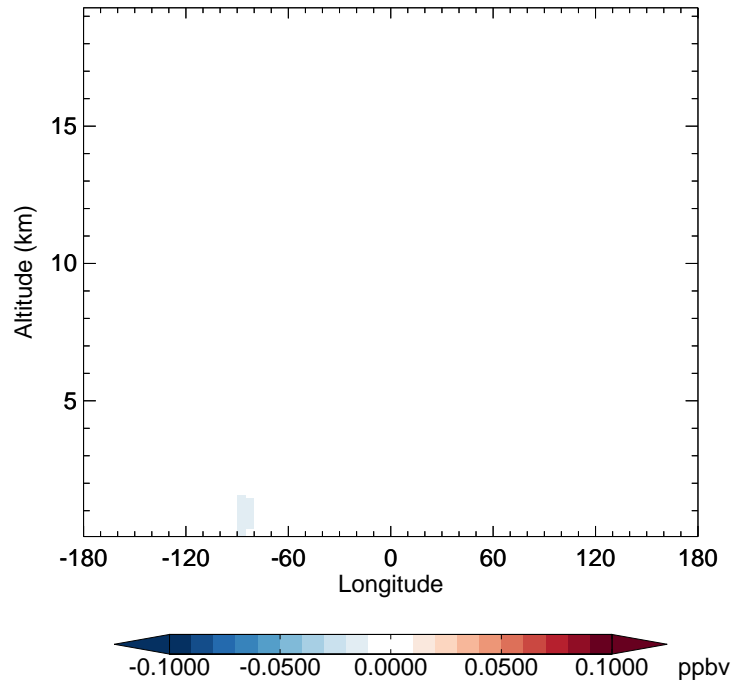
v11-02f-Run1 - v11-02e-Run1 HAC - Diff along 42N for Apr
