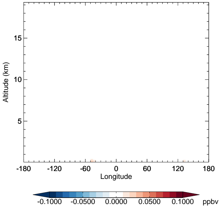
v11-02f-Run1 - v11-02e-Run0 MONITS - Diff along 15S for Apr
