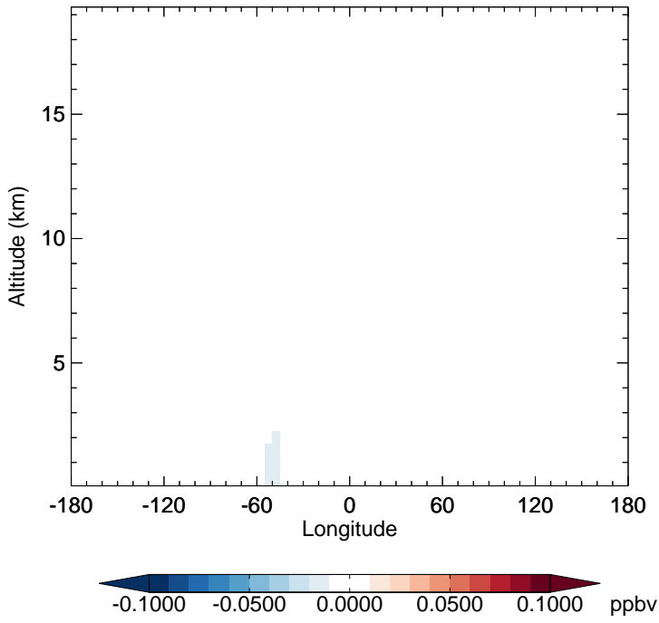
v11-02f-Run1 - v11-02e-Run1 IEPOXD - Diff along 15S for Apr
