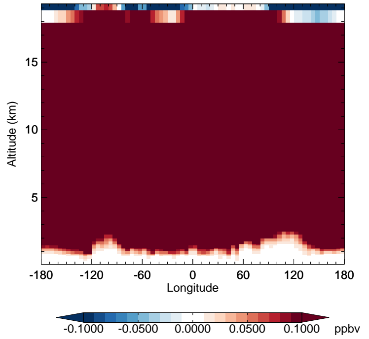
v11-02f-Run1 - v11-02e-Run1 CH4 - Diff along 42N for Apr
