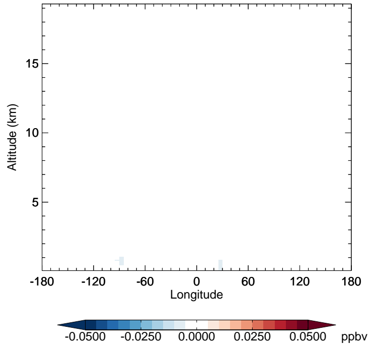
v11-02f-Run1 - v11-02e-Run1 MACR - Diff along 42N for Apr
