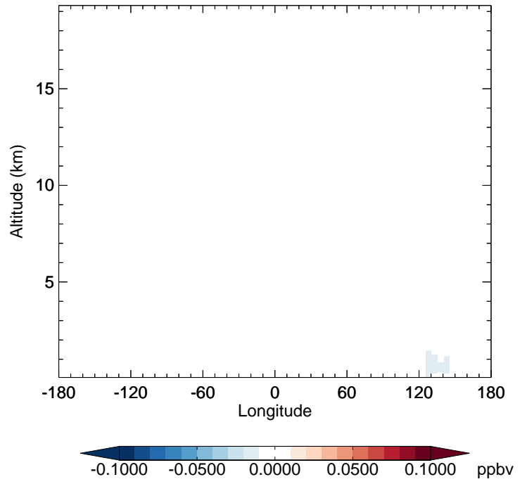
v11-02f-Run1 - v11-02e-Run1 ASOG3 - Diff along 42N for Apr
