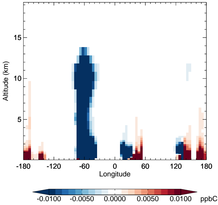
v11-02f-Run1 - v11-02e-Run1 PRPE - Diff along 15S for Apr
