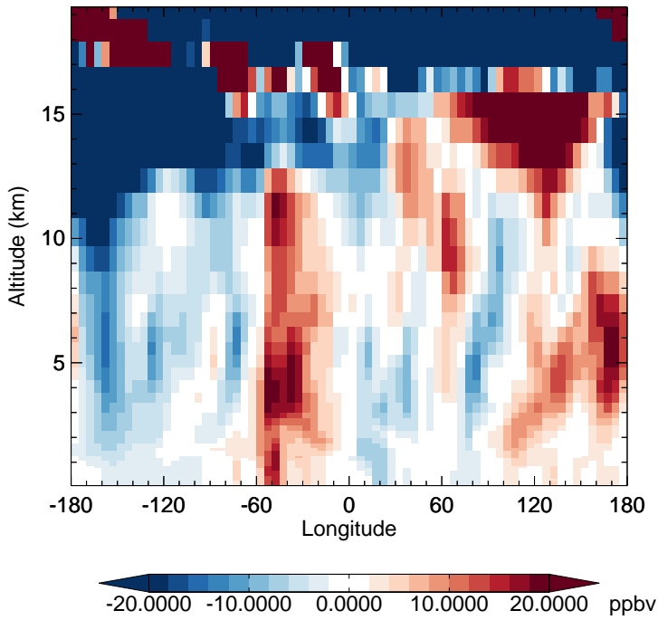
v11-02f-Run1 - v11-02e-Run0 O3 - Diff along 15S for Apr
