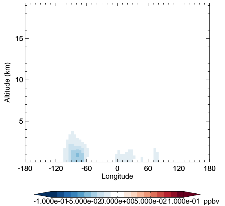
v11-02f-Run1 - v11-02e-Run0 IONITA - Diff along 42N for Apr
