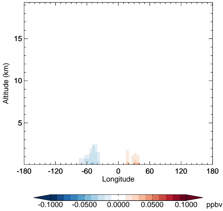
v11-02f-Run1 - v11-02e-Run1 SOAP - Diff along 15S for Apr
