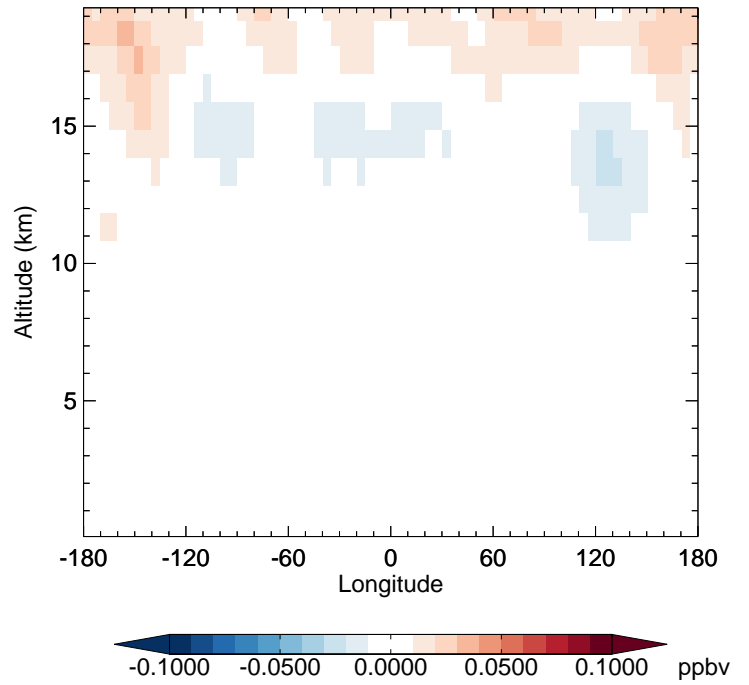
v11-02f-Run1 - v11-02e-Run0 MPN - Diff along 42N for Apr
