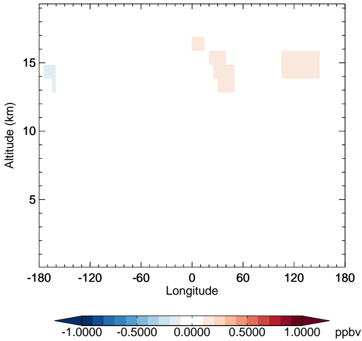
v11-02f-Run1 - v11-02e-Run0 NO - Diff along 15S for Apr
