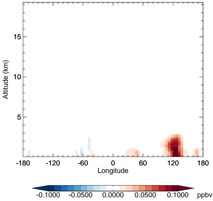
v11-02f-Run1 - v11-02e-Run1 TSOG3 - Diff along 15S for Apr
