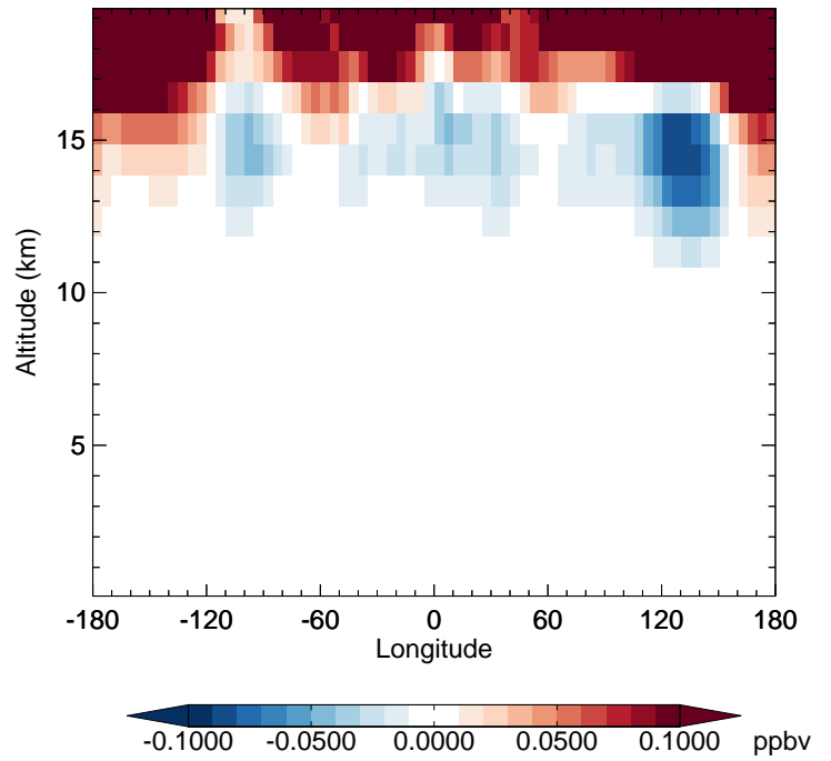
v11-02f-Run1 - v11-02e-Run0 CINO3 - Diff along 42N for Apr
