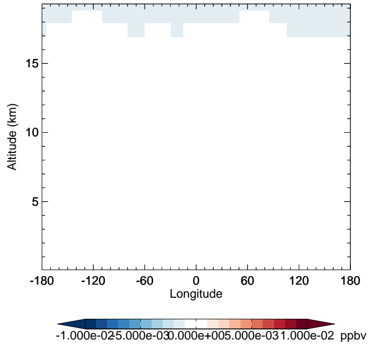
v11-02f-Run1 - v11-02e-Run1 BrNO3 - Diff along 42N for Apr
