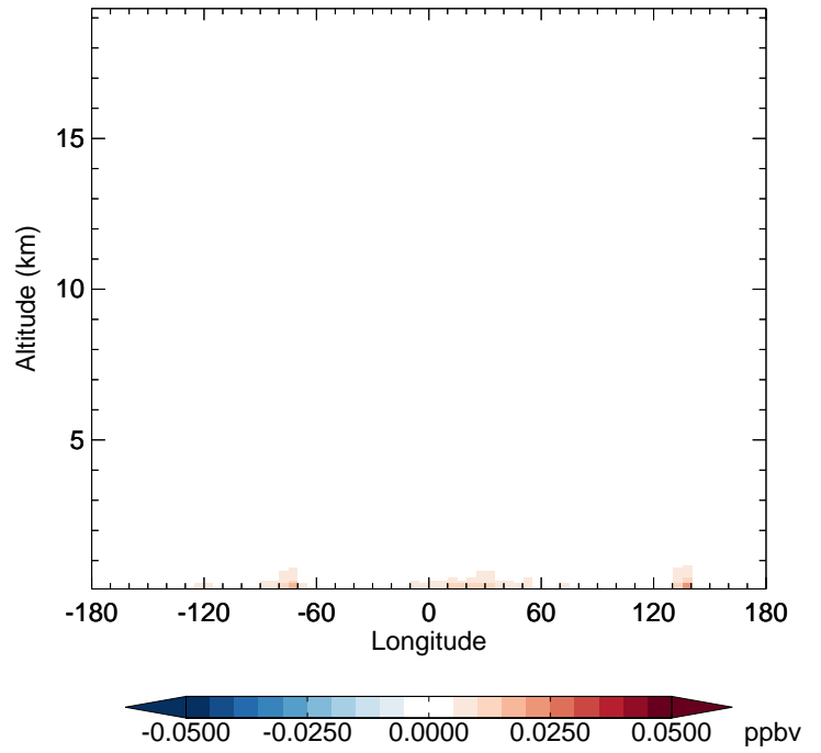
v11-02f-Run1 - v11-02e-Run1 RCHO - Diff along 42N for Apr
