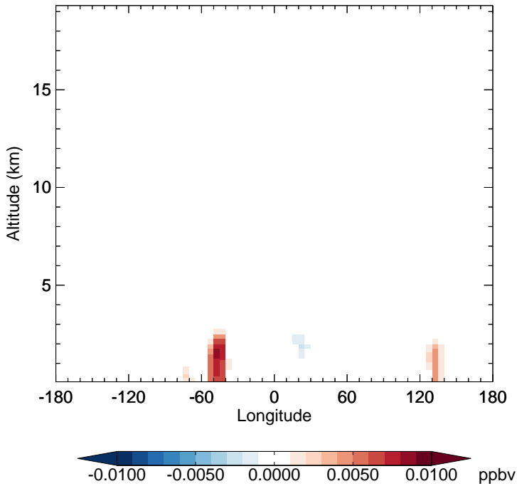
v11-02f-Run1 - v11-02e-Run0 MVKN - Diff along 15S for Apr
