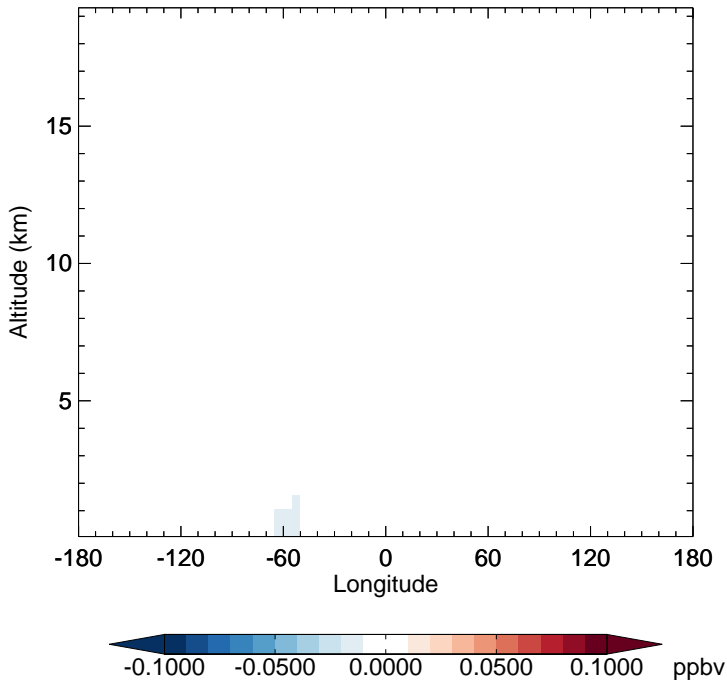
v11-02f-Run1 - v11-02e-Run1 RIPD - Diff along 15S for Apr
