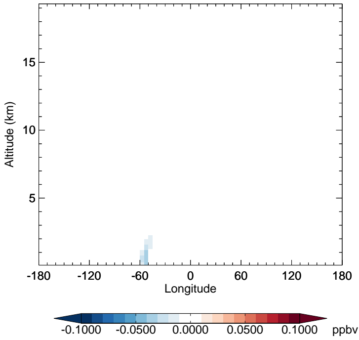
v11-02f-Run1 - v11-02e-Run1 TSOA2 - Diff along 15S for Apr
