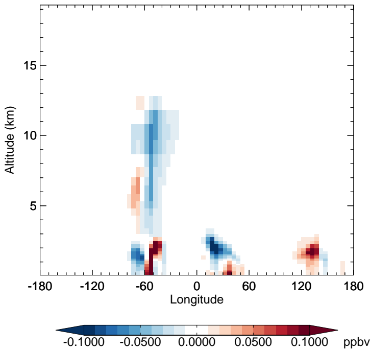
v11-02f-Run1 - v11-02e-Run0 HAC - Diff along 15S for Apr
