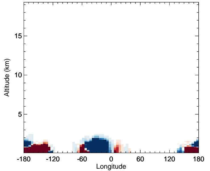
v11-02f-Run1 - v11-02e-Run0 SALC - Diff along 42N for Apr
