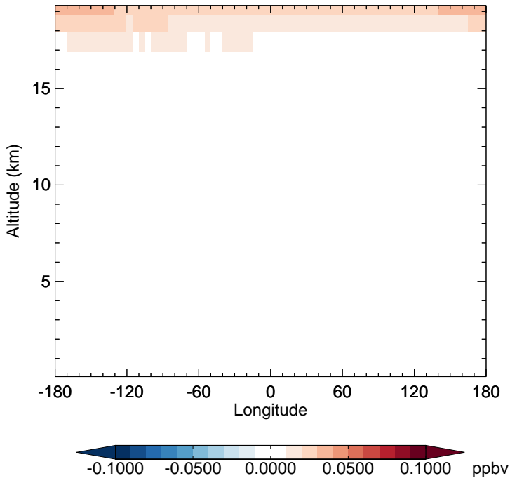
v11-02f-Run1 - v11-02e-Run1 N2O - Diff along 15S for Apr
