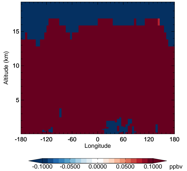
v11-02f-Run1 - v11-02e-Run0 CH4 - Diff along 42N for Apr
