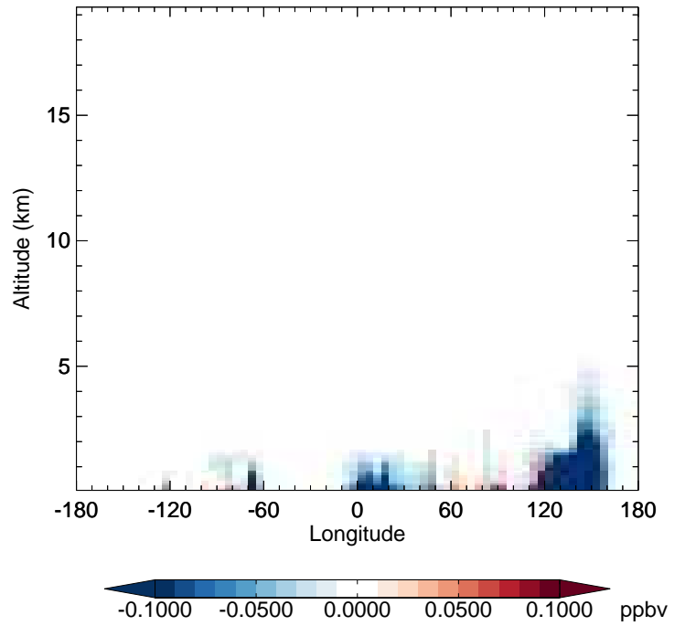
v11-02f-Run1 - v11-02e-Run0 XYLE - Diff along 42N for Apr
