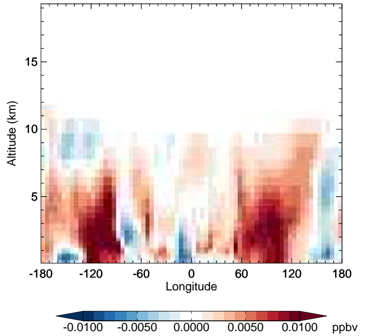
v11-02f-Run1 - v11-02e-Run0 MAP - Diff along 42N for Apr
