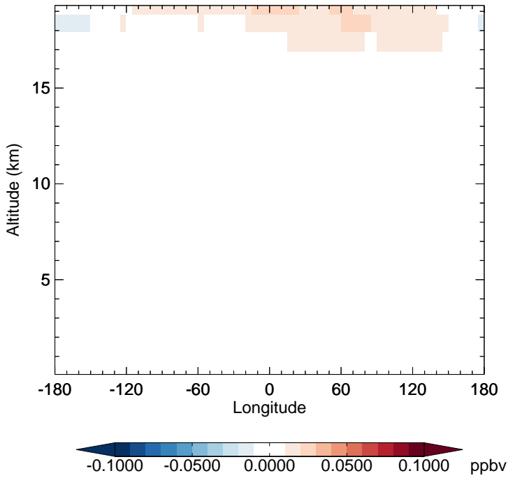
v11-02f-Run1 - v11-02e-Run0 OCS - Diff along 15S for Apr
