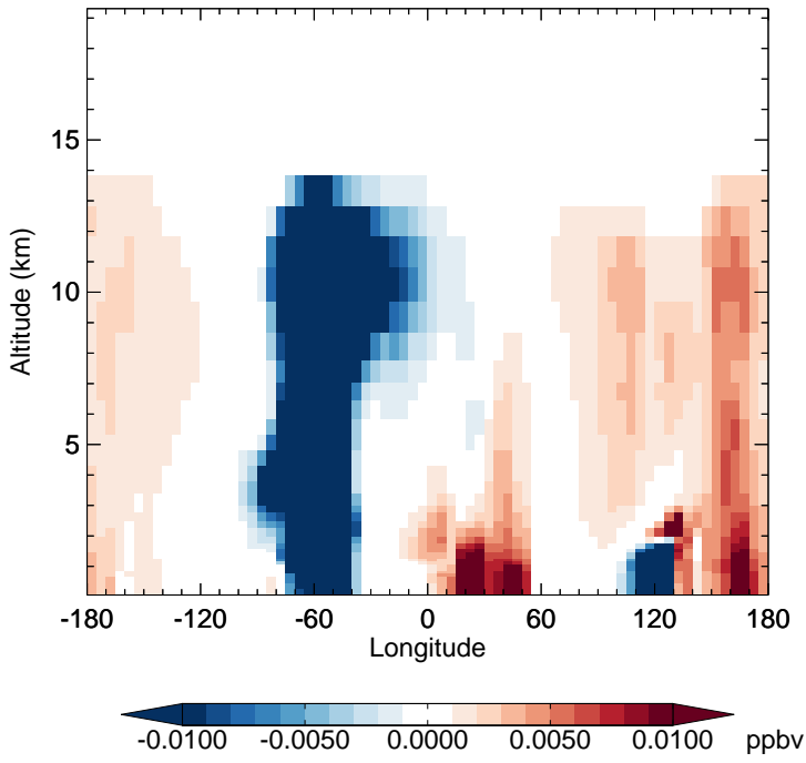
v11-02f-Run1 - v11-02e-Run1 MAP - Diff along 15S for Apr
