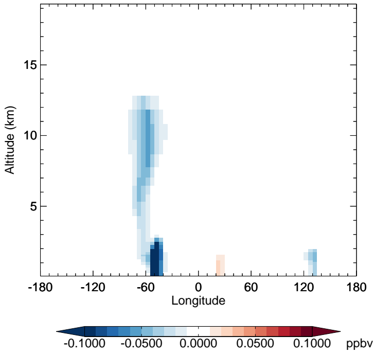
v11-02f-Run1 - v11-02e-Run1 IEPOXB - Diff along 15S for Apr
