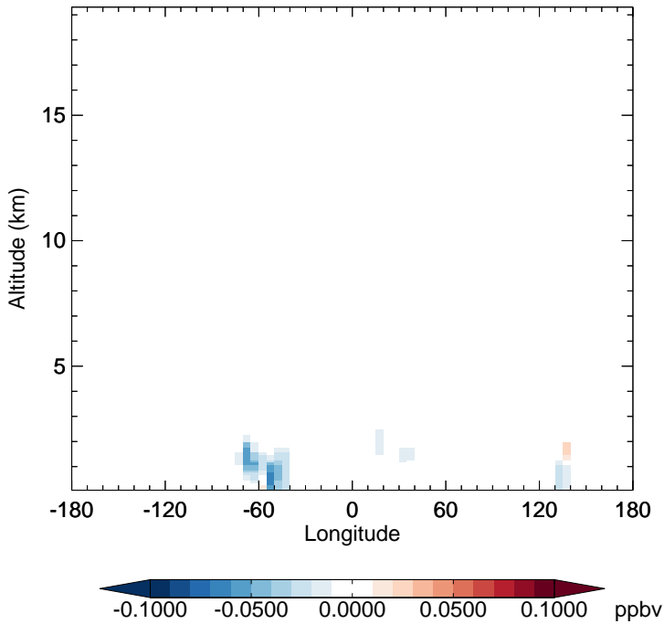
v11-02f-Run1 - v11-02e-Run0 RIPB - Diff along 15S for Apr
