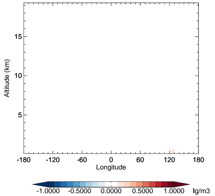
v11-02f-Run1 - v11-02e-Run0 BCPO - Diff along 42N for Apr
