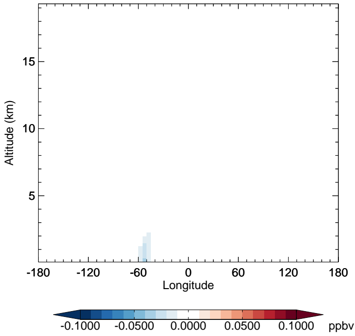
v11-02f-Run1 - v11-02e-Run1 TSOA0 - Diff along 15S for Apr
