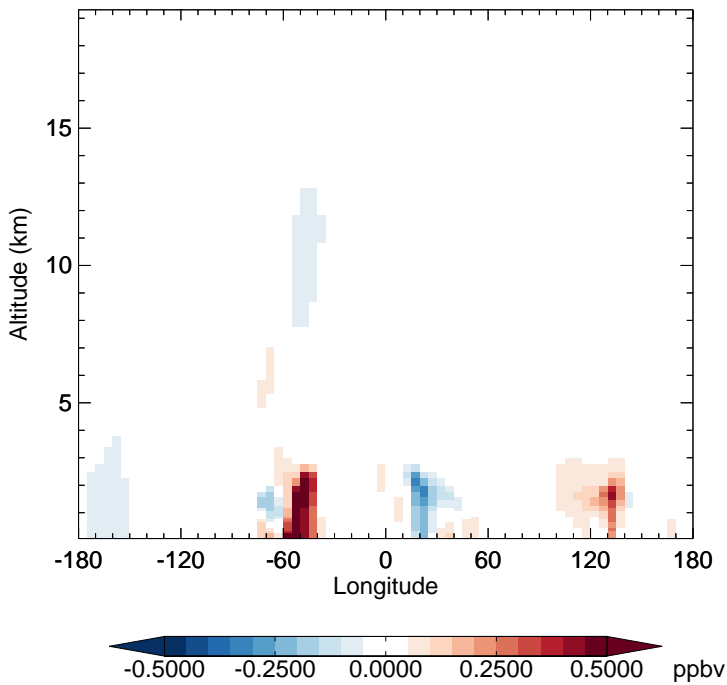
v11-02f-Run1 - v11-02e-Run0 CH 2 O - Diff along 15S for Apr
