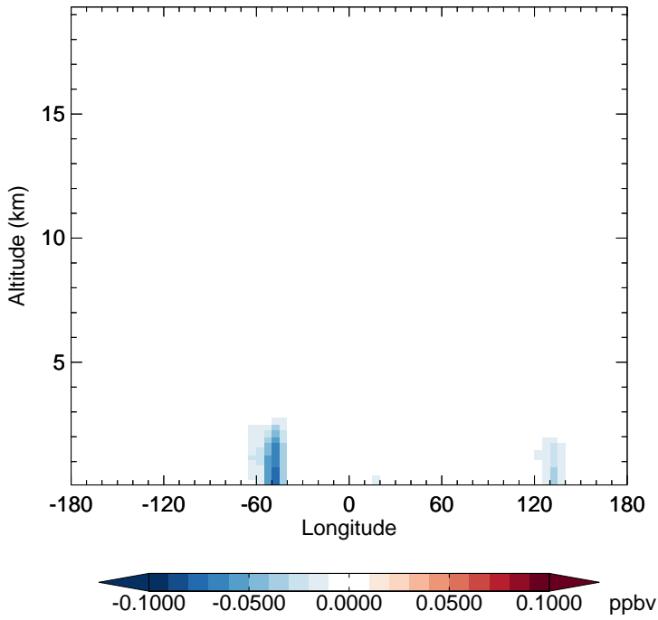
v11-02f-Run1 - v11-02e-Run1 MGLY - Diff along 15S for Apr
