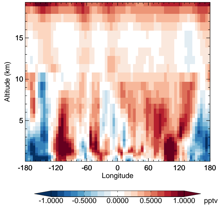
v11-02f-Run1 - v11-02e-Run0 HO2 - Diff along 42N for Apr
