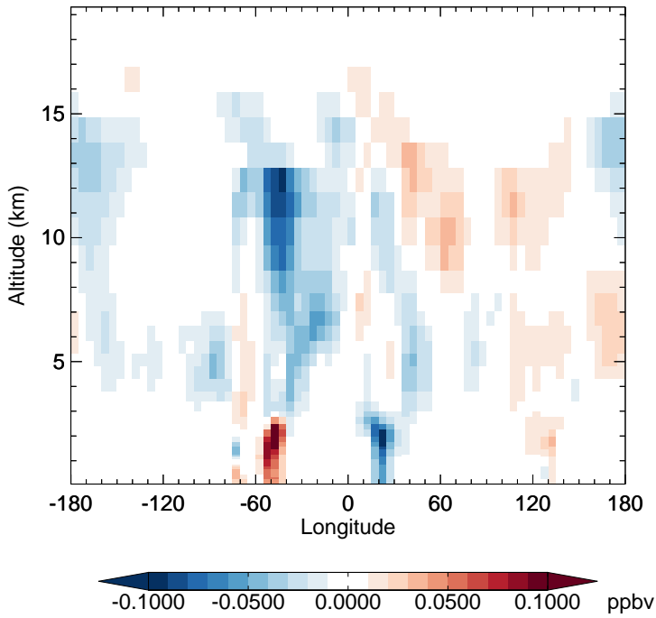
v11-02f-Run1 - v11-02e-Run0 PAN - Diff along 15S for Apr
