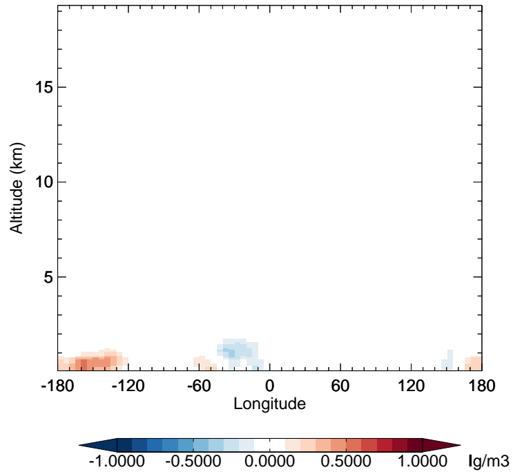
v11-02f-Run1 - v11-02e-Run0 SALA - Diff along 42N for Apr
