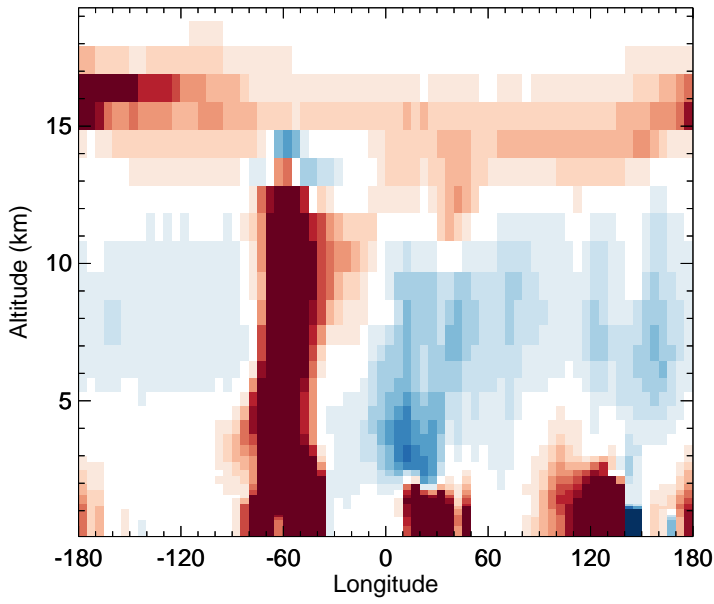
v11-02f-Run1 - v11-02e-Run1 OH - Diff along 15S for Apr
