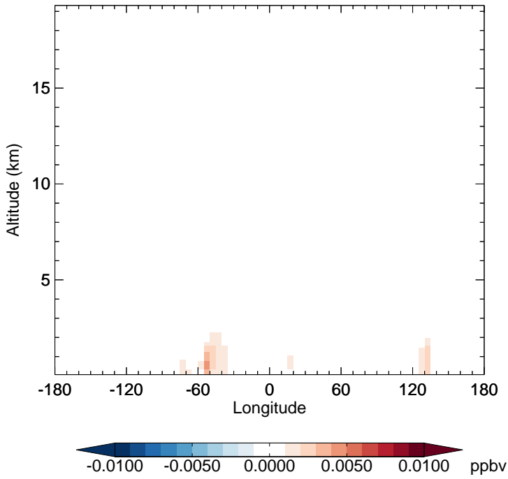
v11-02f-Run1 - v11-02e-Run1 MVKN - Diff along 15S for Apr
