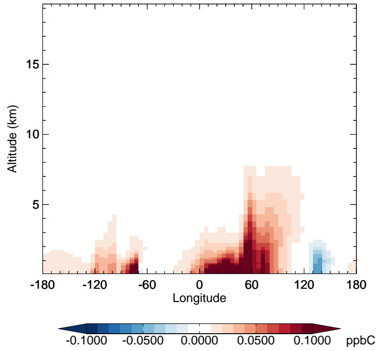
v11-02f-Run1 - v11-02e-Run1 MEK - Diff along 42N for Apr
