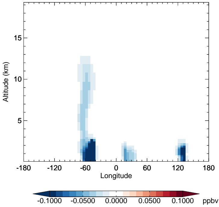
v11-02f-Run1 - v11-02e-Run1 GLYC - Diff along 15S for Apr
