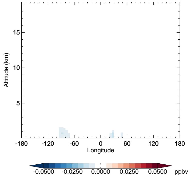
v11-02f-Run1 - v11-02e-Run1 MVK - Diff along 42N for Apr
