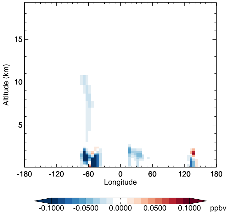
v11-02f-Run1 - v11-02e-Run0 RIPA - Diff along 15S for Apr
