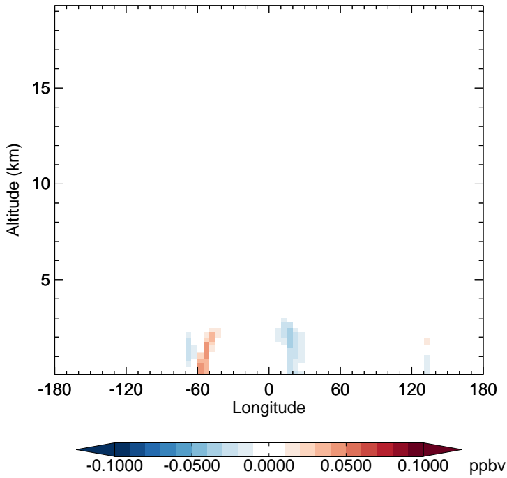
v11-02f-Run1 - v11-02e-Run0 ISOA1 - Diff along 15S for Apr
