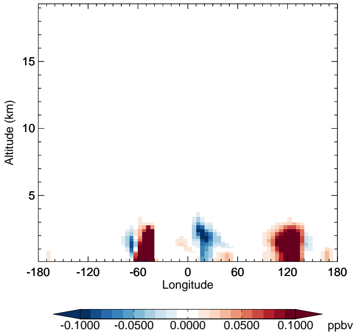
v11-02f-Run1 - v11-02e-Run0 TSOG3 - Diff along 15S for Apr
