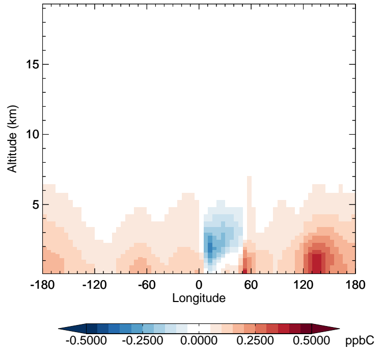
v11-02f-Run1 - v11-02e-Run1 C3H8 - Diff along 42N for Apr
