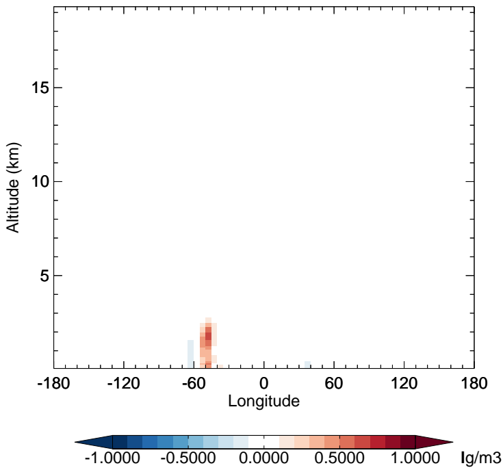
v11-02f-Run1 - v11-02e-Run0 NH3 - Diff along 15S for Apr
