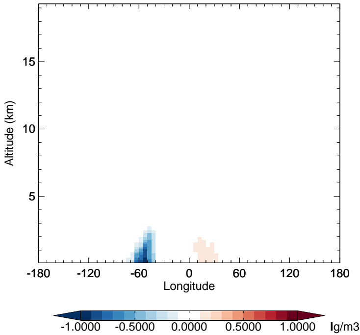
v11-02f-Run1 - v11-02e-Run1 SOAS - Diff along 15S for Apr
