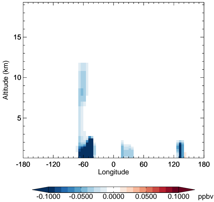
v11-02f-Run1 - v11-02e-Run1 RIPA - Diff along 15S for Apr
