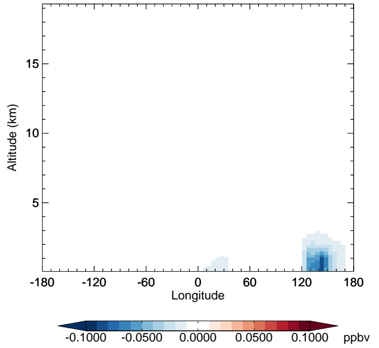
v11-02f-Run1 - v11-02e-Run1 SOAGX - Diff along 42N for Apr
