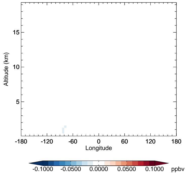
v11-02f-Run1 - v11-02e-Run0 SOAIE - Diff along 42N for Apr
