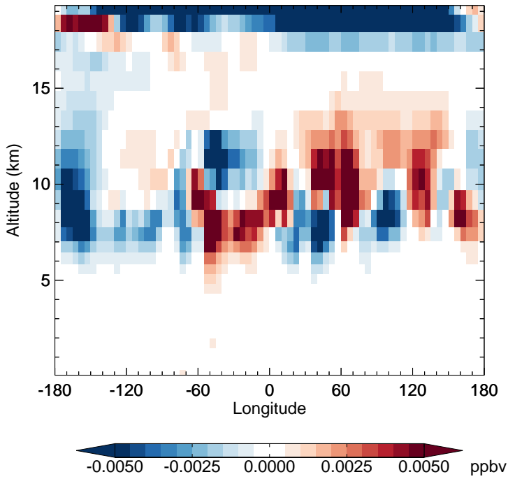
v11-02f-Run1 - v11-02e-Run0 HNO 4 - Diff along 15S for Apr
