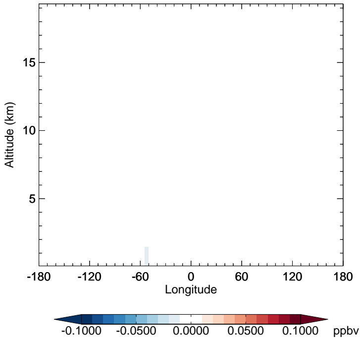
v11-02f-Run1 - v11-02e-Run1 TSOA1 - Diff along 15S for Apr
