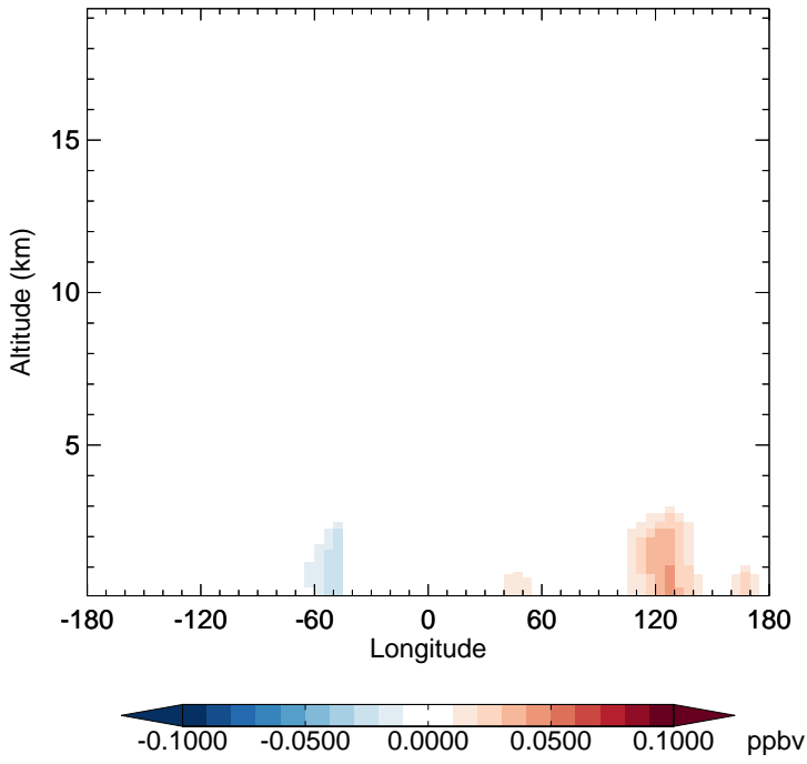
v11-02f-Run1 - v11-02e-Run1 TSOG2 - Diff along 15S for Apr
