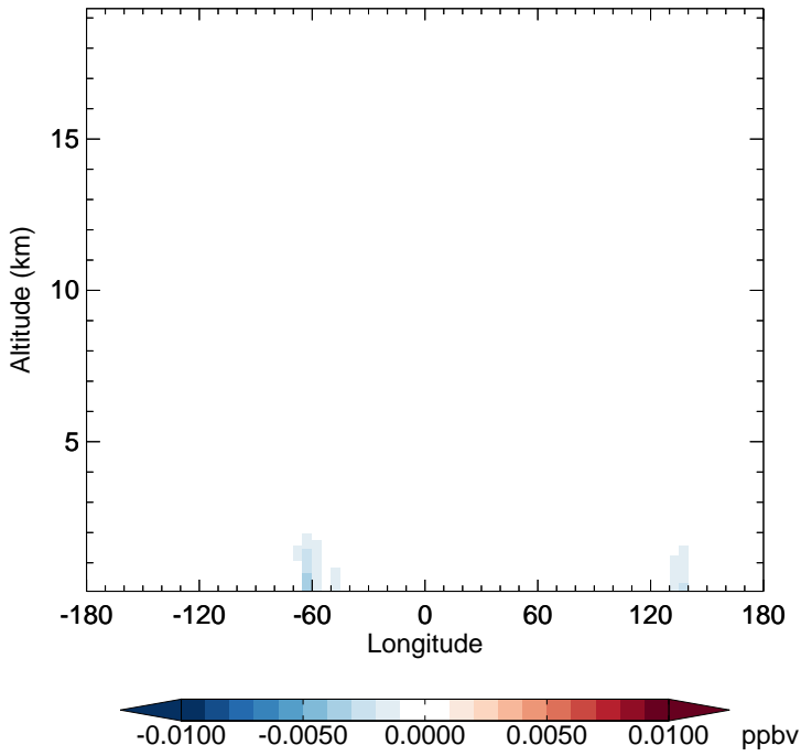
v11-02f-Run1 - v11-02e-Run1 MOBA - Diff along 15S for Jan
