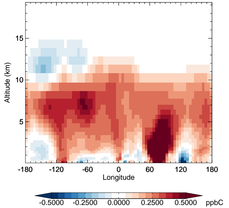
v11-02f-Run1 - v11-02e-Run0 ACET - Diff along 42N for Jan
