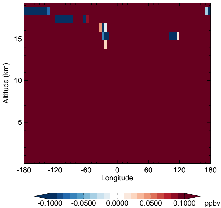
v11-02f-Run1 - v11-02e-Run0 N2O - Diff along 15S for Jan
