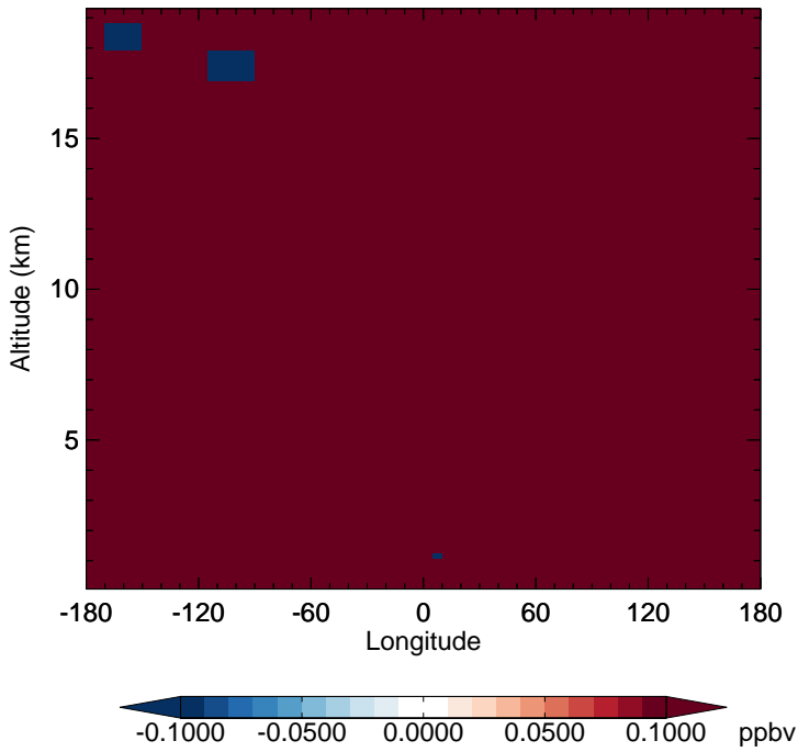
v11-02f-Run1 - v11-02e-Run0 CH4 - Diff along 15S for Jan
