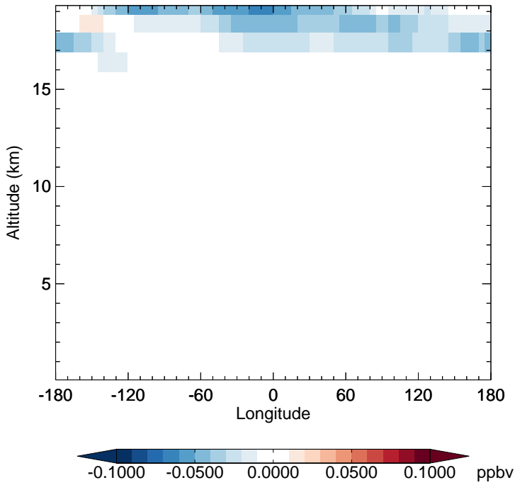
v11-02f-Run1 - v11-02e-Run0 CINO3 - Diff along 15S for Jan
