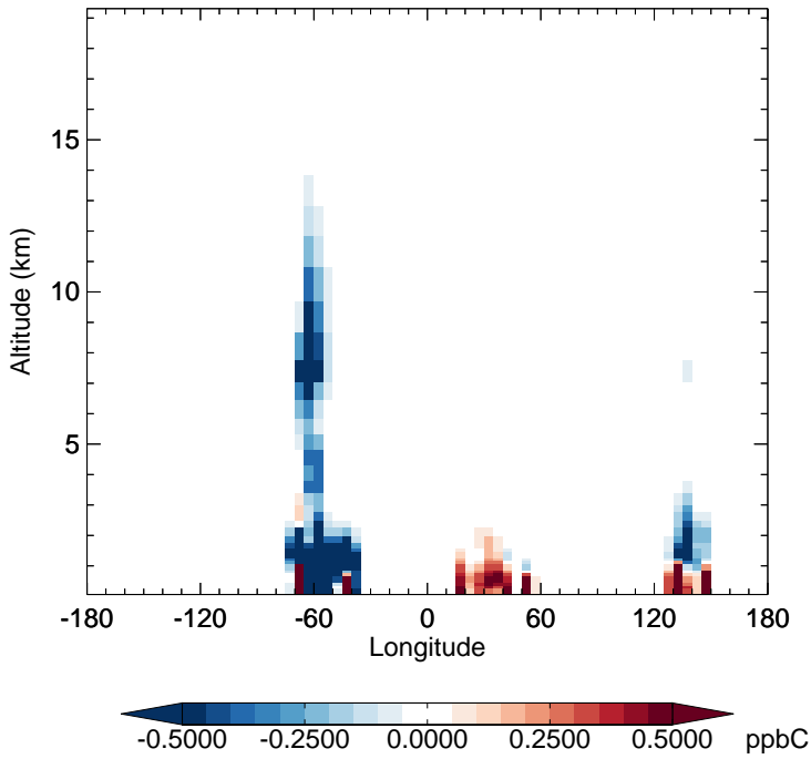
v11-02f-Run1 - v11-02e-Run0 ISOP - Diff along 15S for Jan
