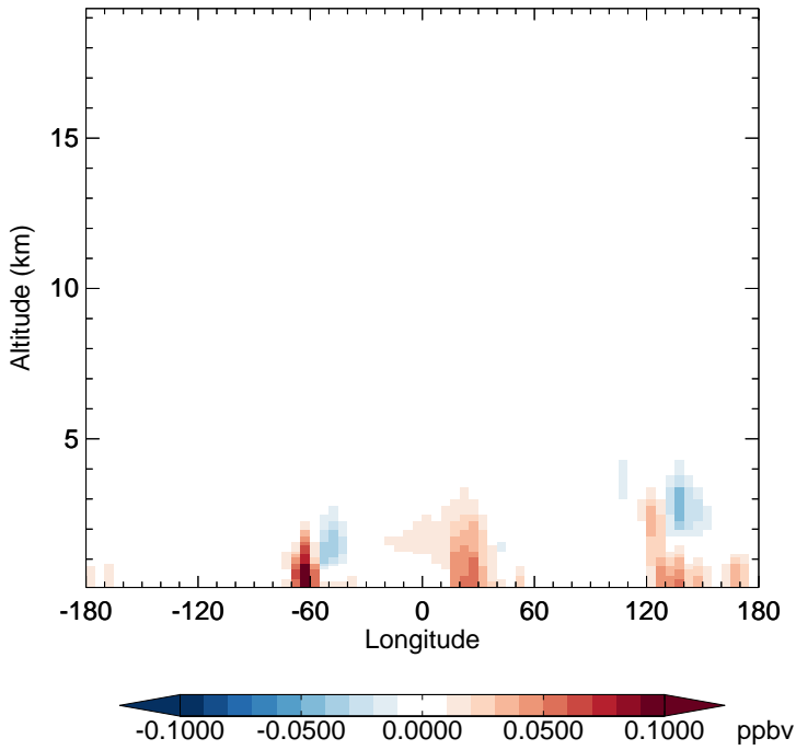
v11-02f-Run1 - v11-02e-Run0 TSOG2 - Diff along 15S for Jan
