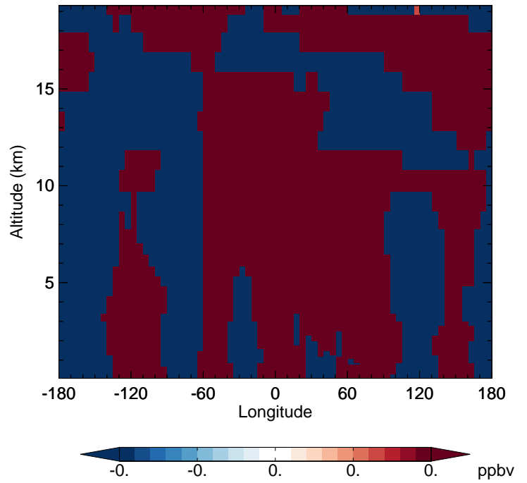
v11-02f-Run1 - v11-02e-Run0 H2O - Diff along 42N for Jan
