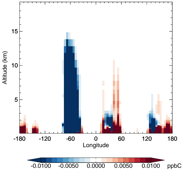
v11-02f-Run1 - v11-02e-Run1 PRPE - Diff along 15S for Jan
