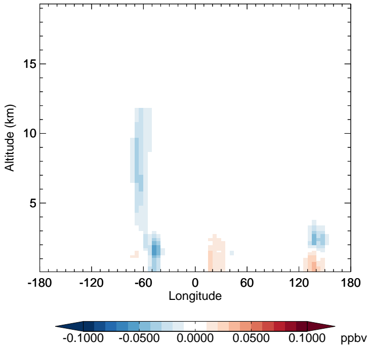
v11-02f-Run1 - v11-02e-Run0 HC187 - Diff along 15S for Jan
