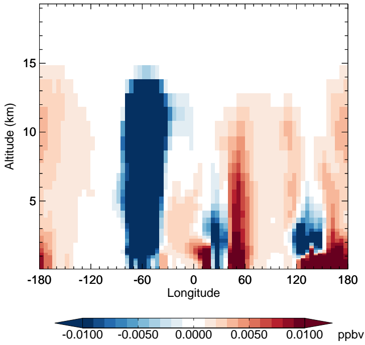
v11-02f-Run1 - v11-02e-Run1 MAP - Diff along 15S for Jan
