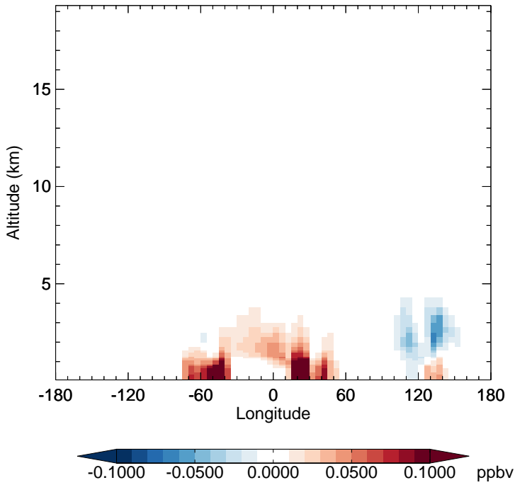
v11-02f-Run1 - v11-02e-Run0 INDIOL - Diff along 15S for Jan
