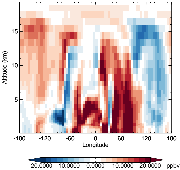
v11-02f-Run1 - v11-02e-Run0 CO - Diff along 15S for Jan
