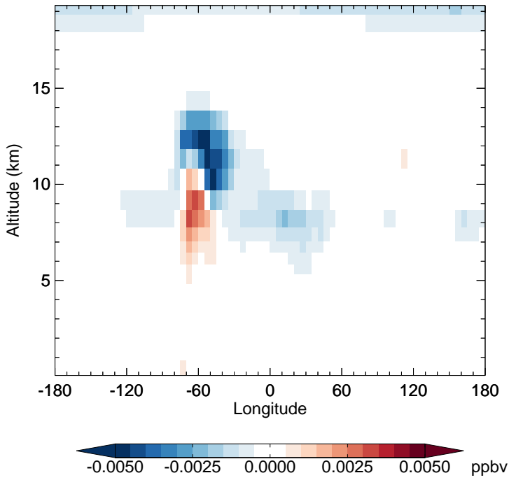
v11-02f-Run1 - v11-02e-Run1 HNO 4 - Diff along 15S for Jan
