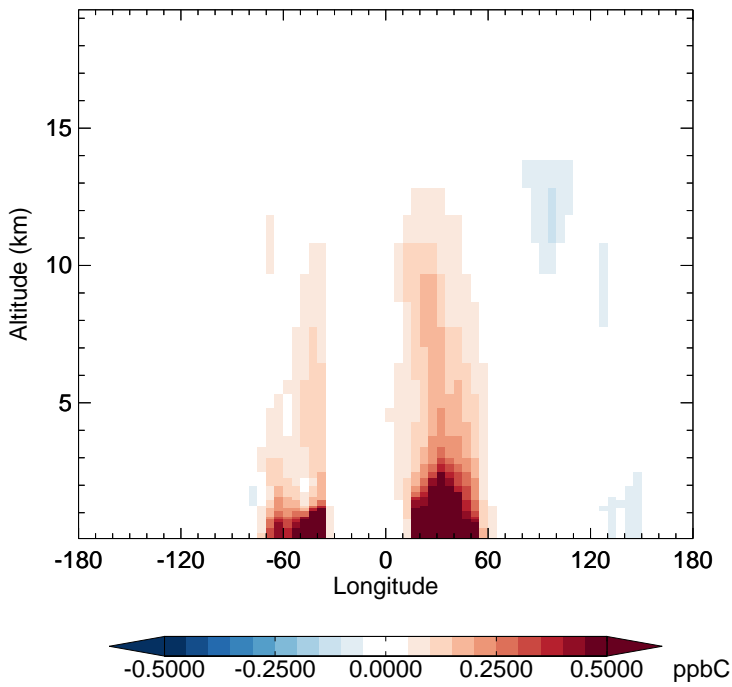
v11-02f-Run1 - v11-02e-Run0 ALK4 - Diff along 15S for Jan
