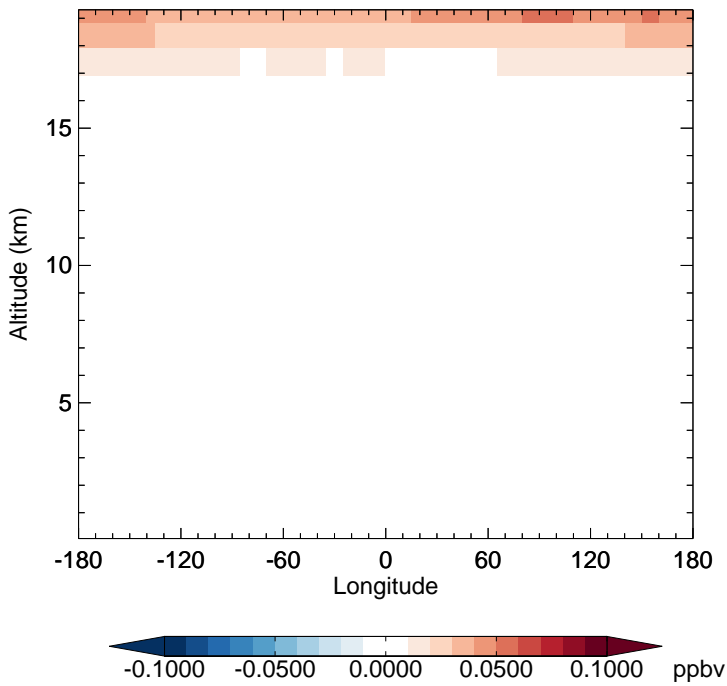
v11-02f-Run1 - v11-02e-Run1 N2O - Diff along 15S for Jan
