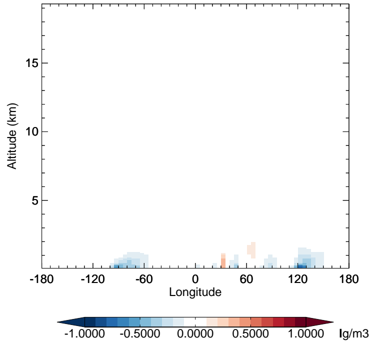
v11-02f-Run1 - v11-02e-Run1 SO4 - Diff along 42N for Jan
