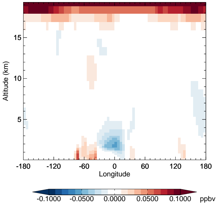
v11-02f-Run1 - v11-02e-Run1 HNO 3 - Diff along 15S for Jan
