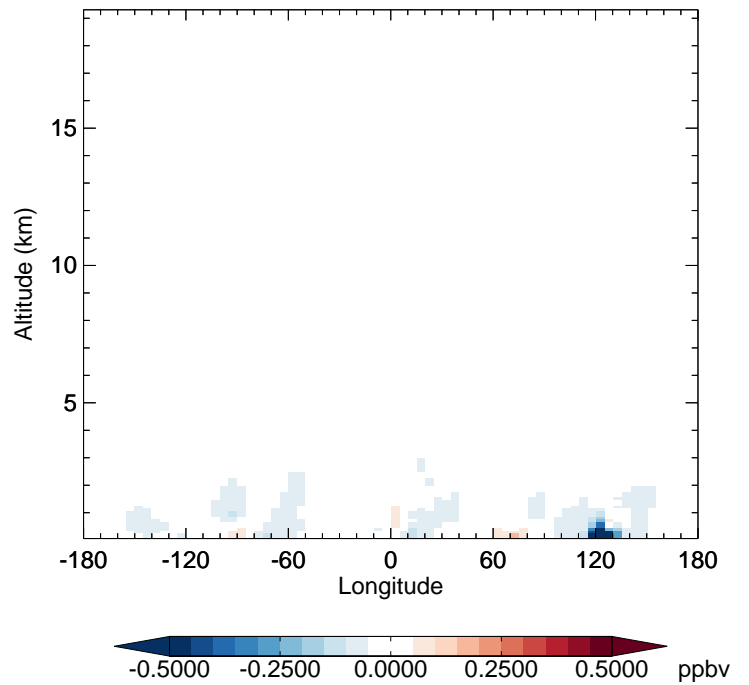
v11-02f-Run1 - v11-02e-Run0 CH 2 O - Diff along 42N for Jan
