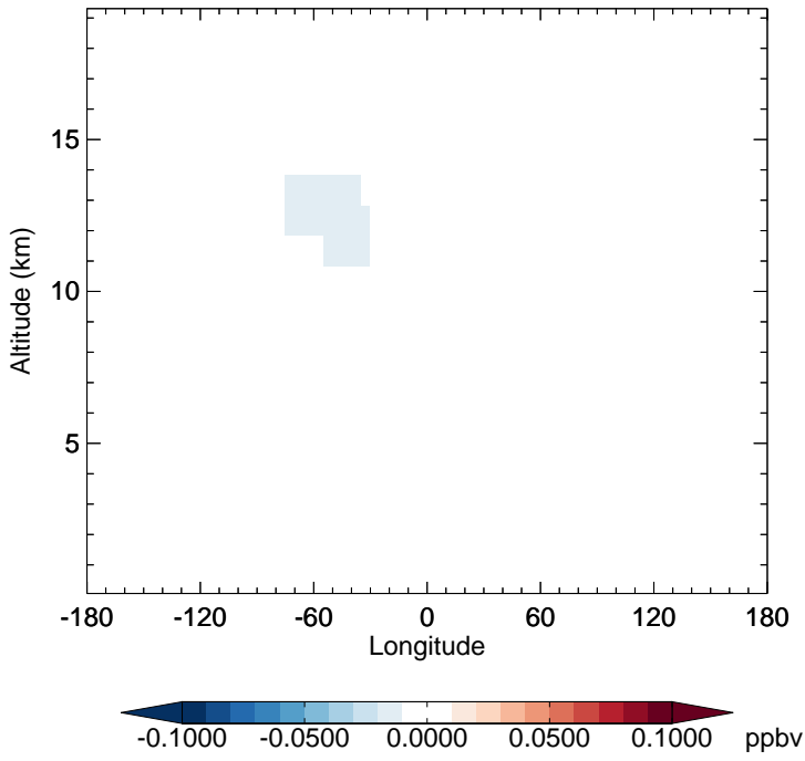
v11-02f-Run1 - v11-02e-Run1 MPN - Diff along 15S for Jan
