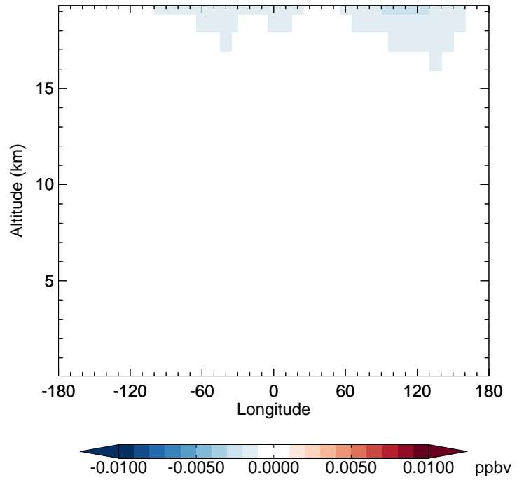
v11-02f-Run1 - v11-02e-Run0 BrNO3 - Diff along 42N for Jan
