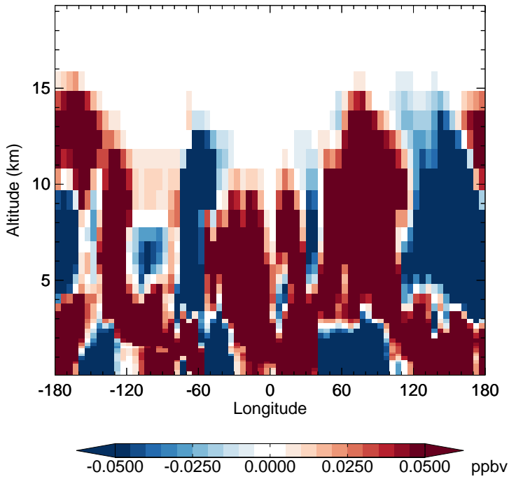
v11-02f-Run1 - v11-02e-Run0 MP - Diff along 15S for Jan
