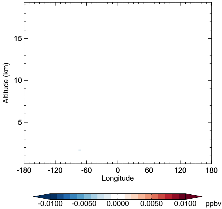
v11-02f-Run1 - v11-02e-Run0 CHBr3 - Diff along 15S for Jan
