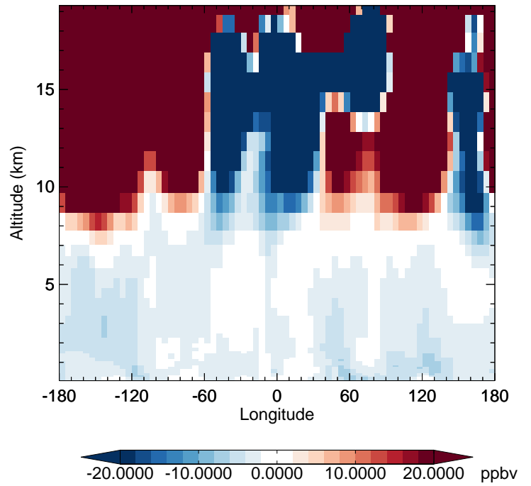
v11-02f-Run1 - v11-02e-Run0 O3 - Diff along 42N for Jan
