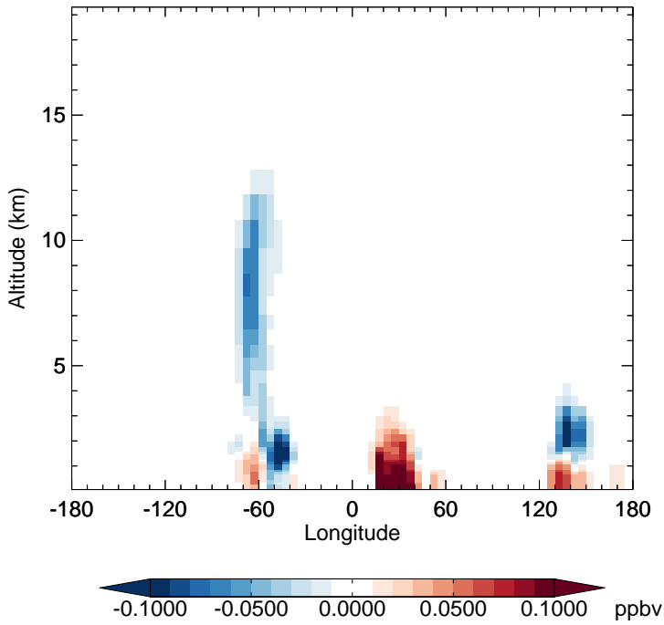
v11-02f-Run1 - v11-02e-Run0 HAC - Diff along 15S for Jan
