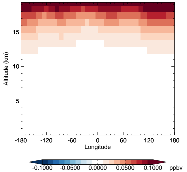
v11-02f-Run1 - v11-02e-Run1 N2O - Diff along 42N for Jan
