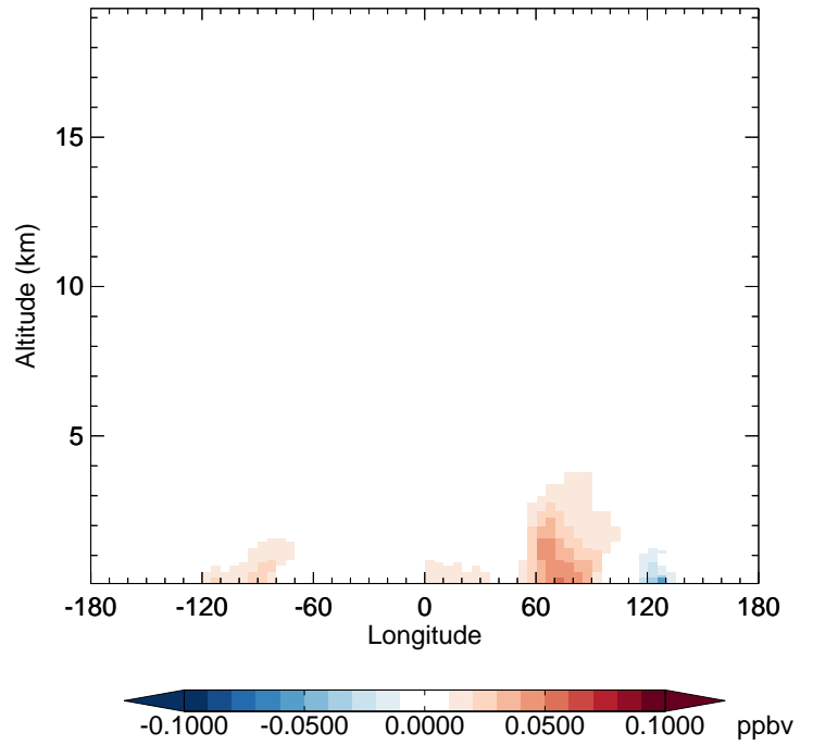
v11-02f-Run1 - v11-02e-Run0 INDIOL - Diff along 42N for Jan
