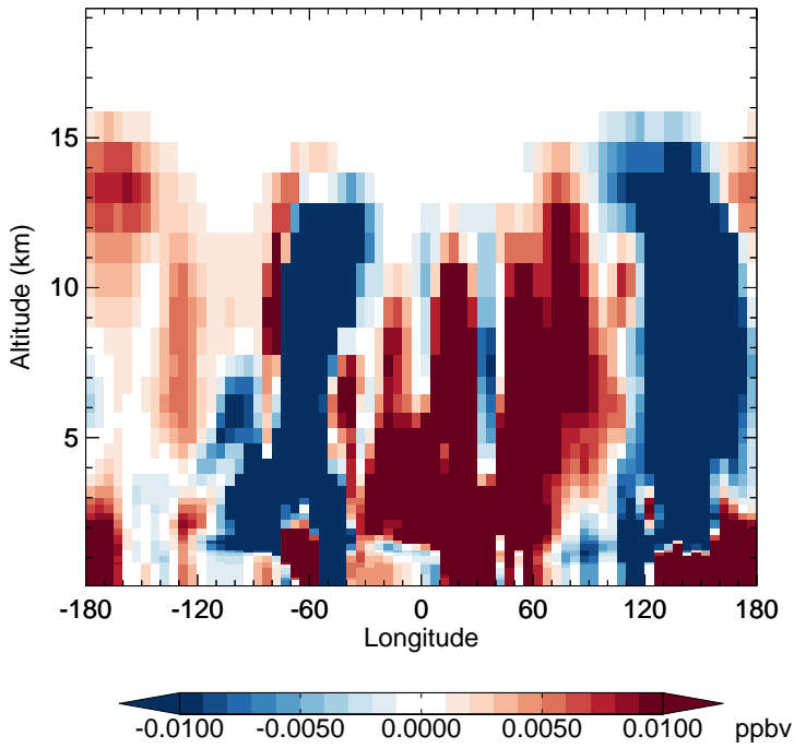
v11-02f-Run1 - v11-02e-Run0 MAP - Diff along 15S for Jan
