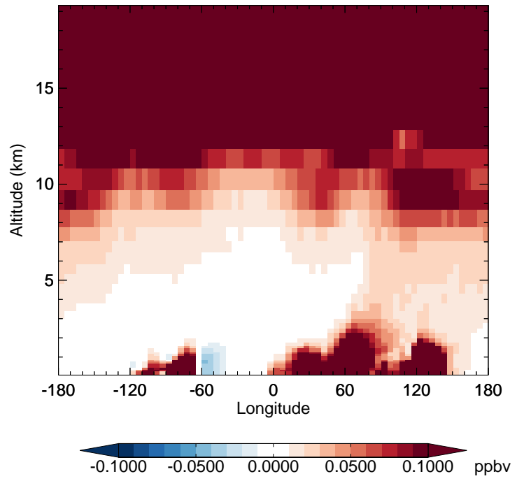
v11-02f-Run1 - v11-02e-Run1 HNO 3 - Diff along 42N for Jan
