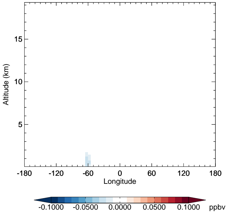
v11-02f-Run1 - v11-02e-Run1 TSOA2 - Diff along 15S for Jan
