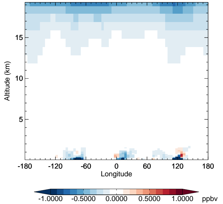
v11-02f-Run1 - v11-02e-Run0 NO2 - Diff along 42N for Jan
