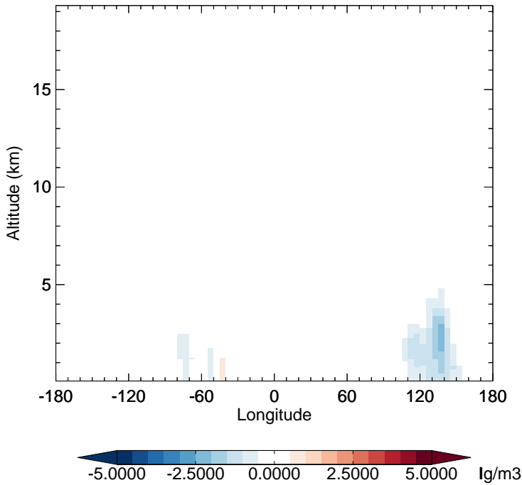
v11-02f-Run1 - v11-02e-Run0 DST1 - Diff along 15S for Jan
