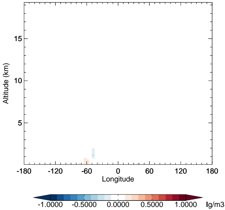
v11-02f-Run1 - v11-02e-Run0 NH3 - Diff along 15S for Jan
