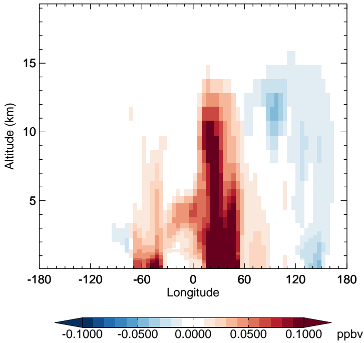
v11-02f-Run1 - v11-02e-Run0 BENZ - Diff along 15S for Jan
