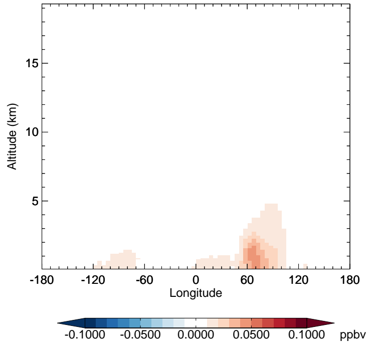
v11-02f-Run1 - v11-02e-Run1 INDIOL - Diff along 42N for Jan
