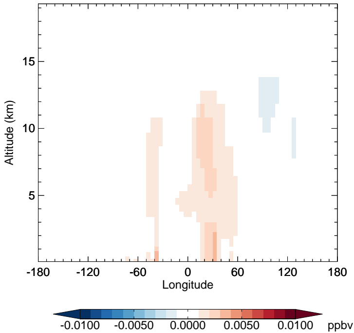
v11-02f-Run1 - v11-02e-Run0 R4N2 - Diff along 15S for Jan
