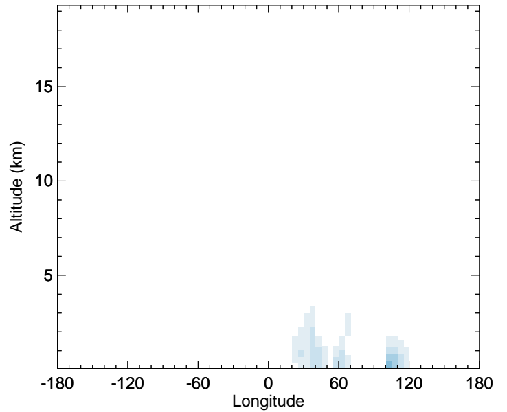
v11-02f-Run1 - v11-02e-Run0 DST2 - Diff along 42N for Jan
