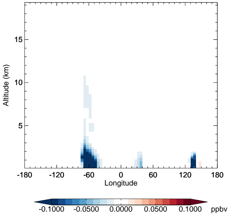
v11-02f-Run1 - v11-02e-Run1 HPALD - Diff along 15S for Jan
