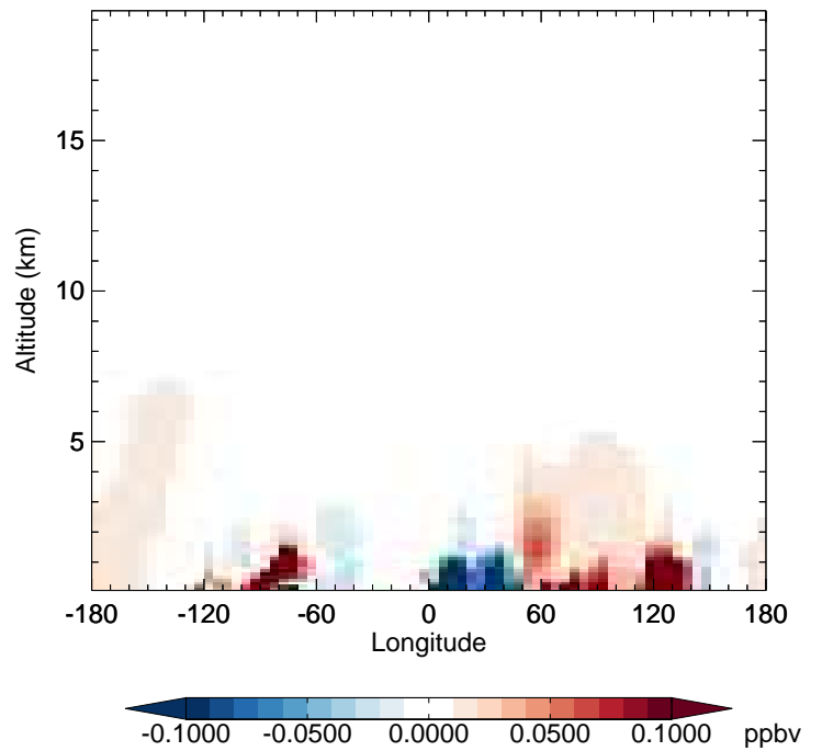
v11-02f-Run1 - v11-02e-Run0 EOH - Diff along 42N for Jan
