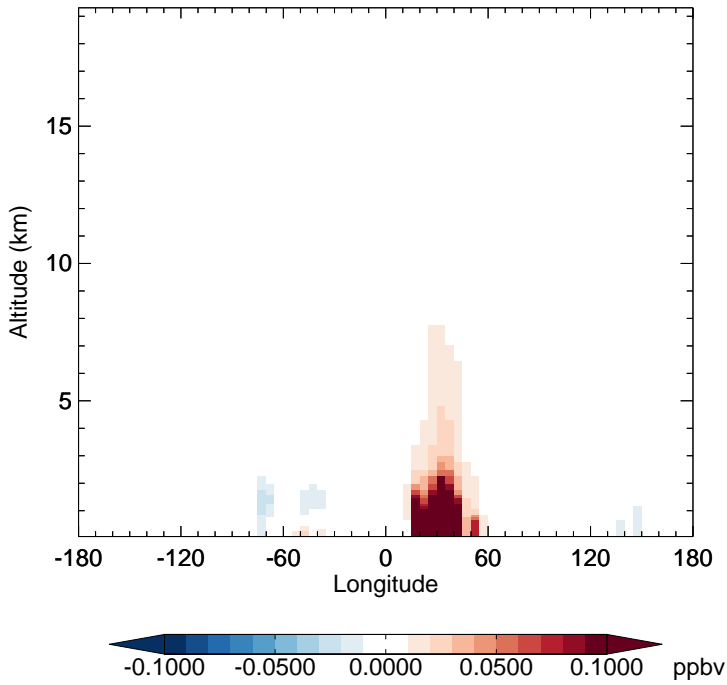
v11-02f-Run1 - v11-02e-Run0 TOLU - Diff along 15S for Jan
