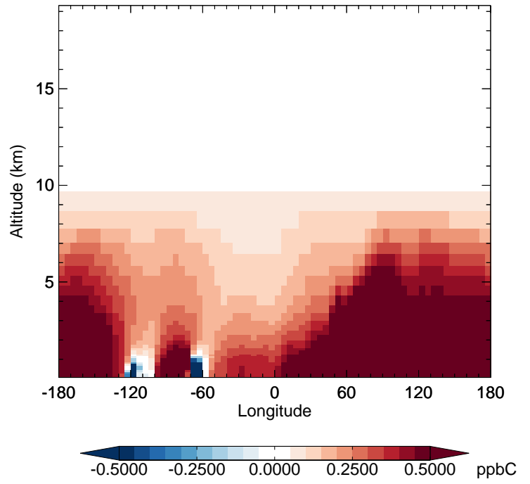
v11-02f-Run1 - v11-02e-Run1 ALK4 - Diff along 42N for Jan
