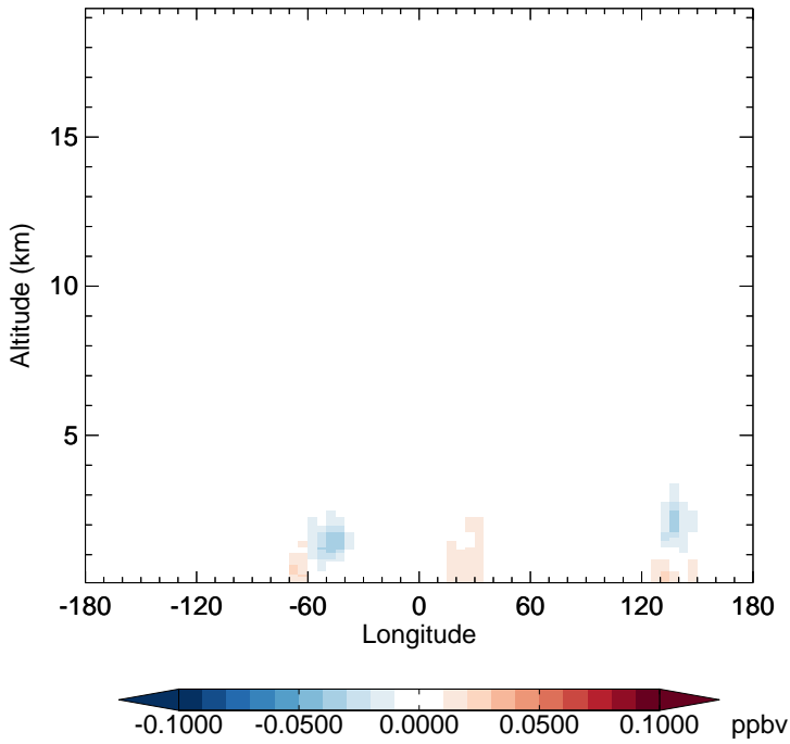
v11-02f-Run1 - v11-02e-Run0 MGLY - Diff along 15S for Jan
