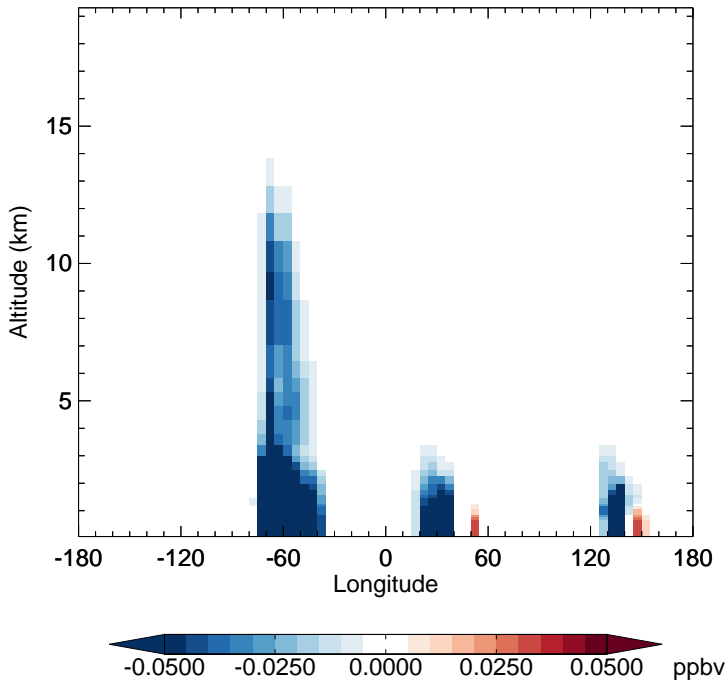
v11-02f-Run1 - v11-02e-Run1 MVK - Diff along 15S for Jan
