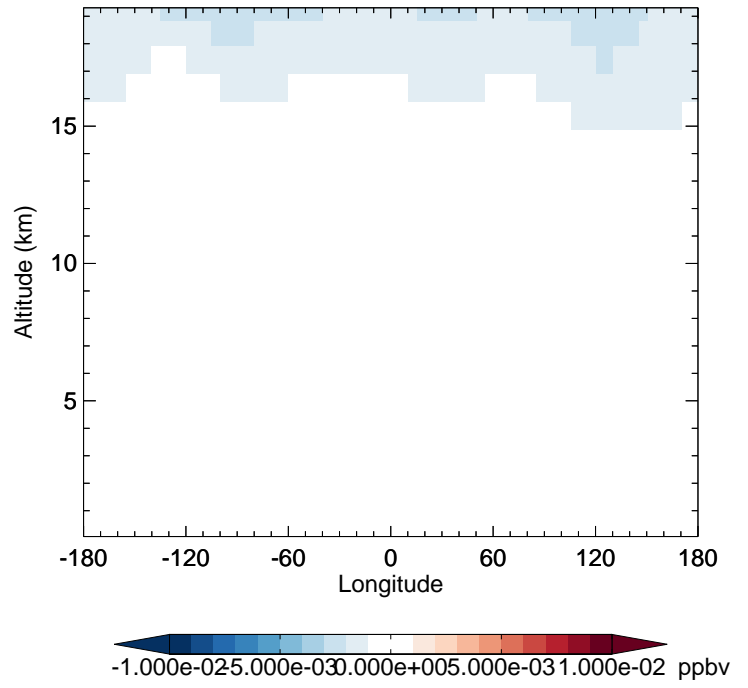
v11-02f-Run1 - v11-02e-Run1 BrNO3 - Diff along 42N for Jan
