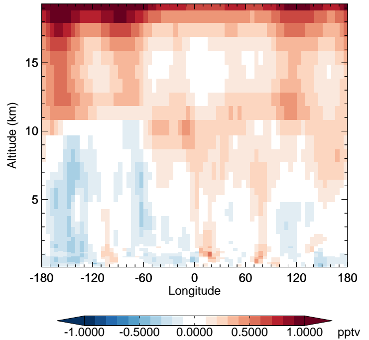
v11-02f-Run1 - v11-02e-Run0 HO2 - Diff along 42N for Jan
