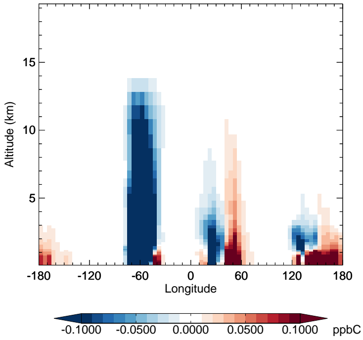
v11-02f-Run1 - v11-02e-Run1 MEK - Diff along 15S for Jan
