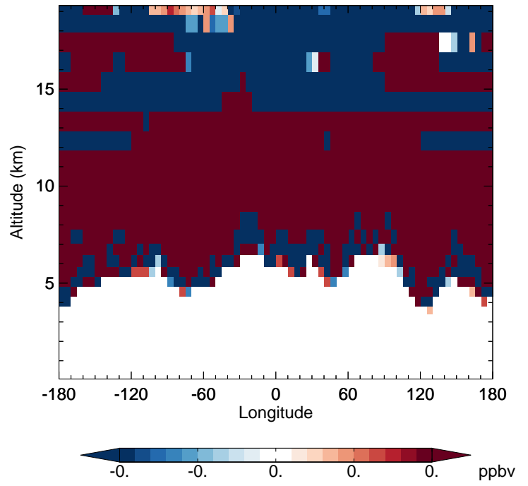
v11-02f-Run1 - v11-02e-Run1 H2O - Diff along 42N for Jan
