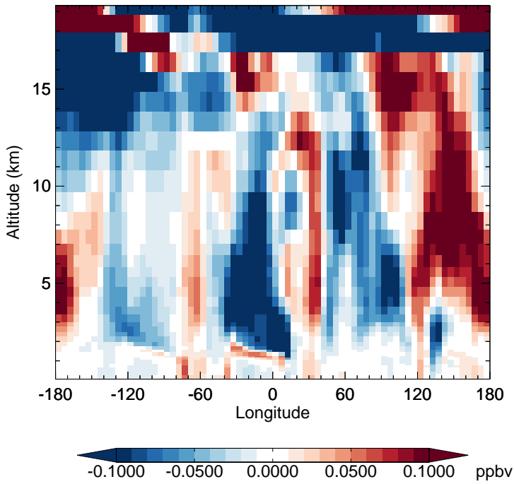
v11-02f-Run1 - v11-02e-Run0 HNO 3 - Diff along 15S for Jan
