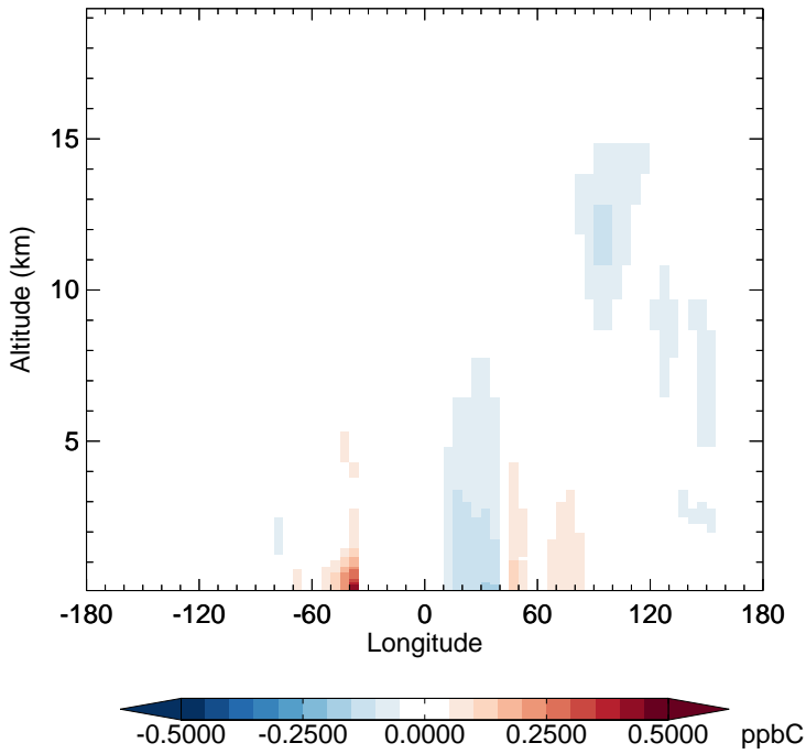
v11-02f-Run1 - v11-02e-Run0 C3H8 - Diff along 15S for Jan
