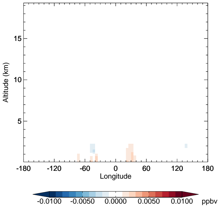
v11-02f-Run1 - v11-02e-Run0 MVKN - Diff along 15S for Jan
