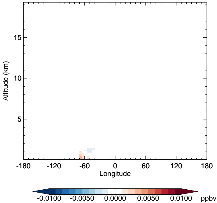
v11-02f-Run1 - v11-02e-Run0 MOBA - Diff along 15S for Jan
