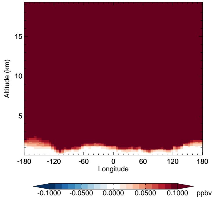
v11-02f-Run1 - v11-02e-Run1 CH4 - Diff along 42N for Jan
