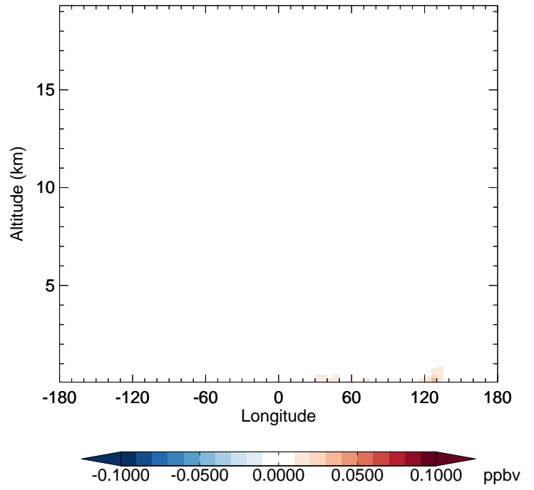
v11-02f-Run1 - v11-02e-Run1 GLYC - Diff along 42N for Jan
