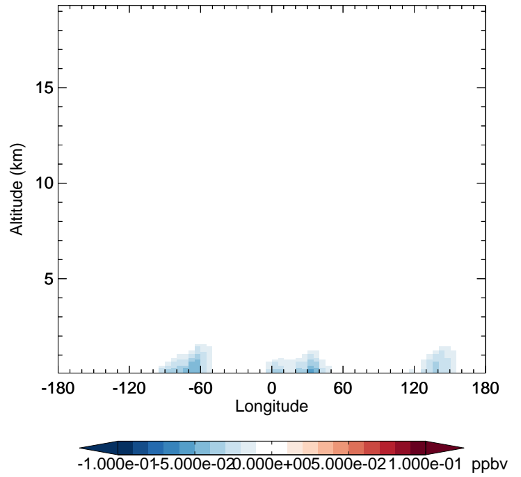
v11-02f-Run1 - v11-02e-Run1 CINO2 - Diff along 42N for Jan
