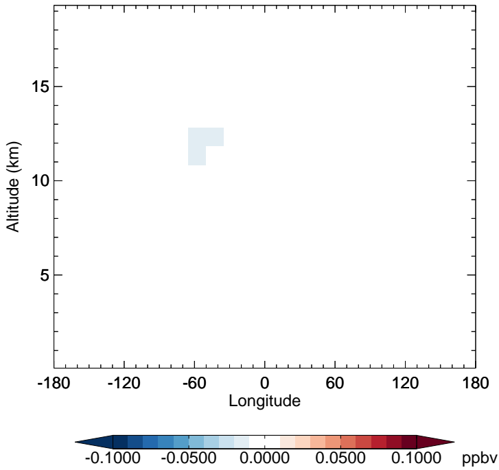
v11-02f-Run1 - v11-02e-Run0 ISOA3 - Diff along 15S for Jan
