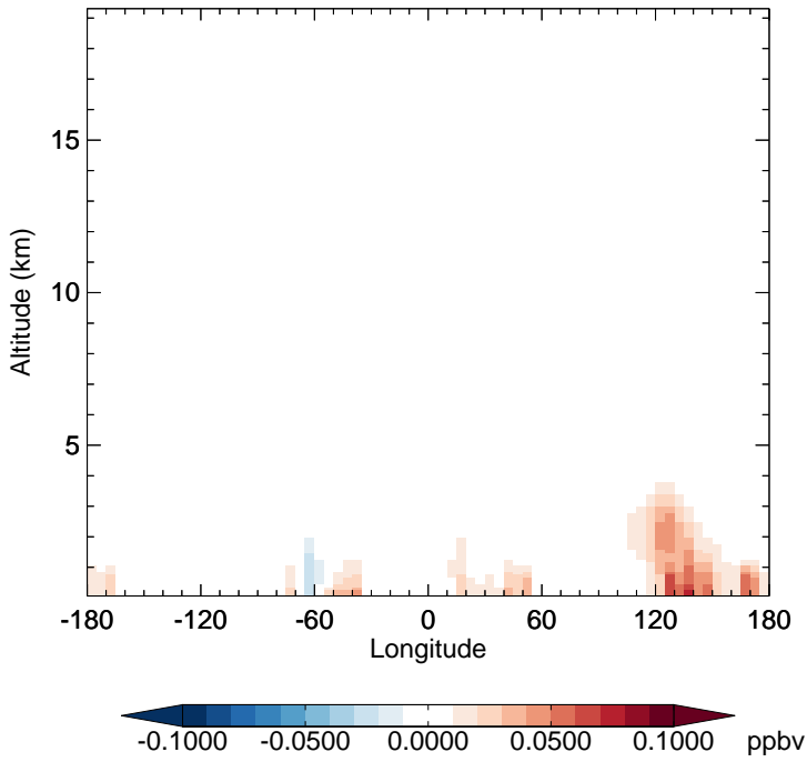
v11-02f-Run1 - v11-02e-Run1 TSOG3 - Diff along 15S for Jan
