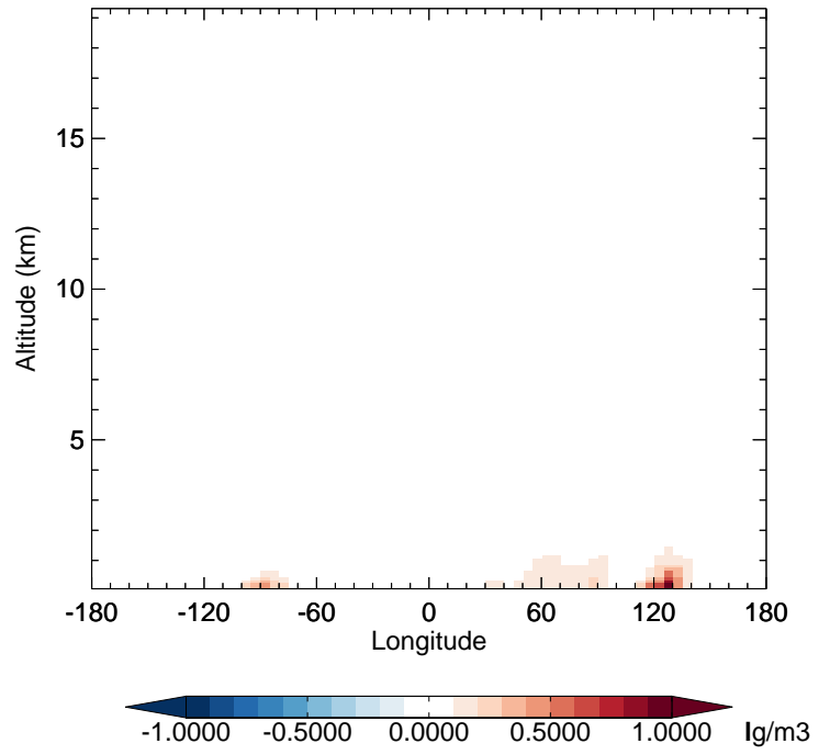
v11-02f-Run1 - v11-02e-Run1 NH4 - Diff along 42N for Jan
