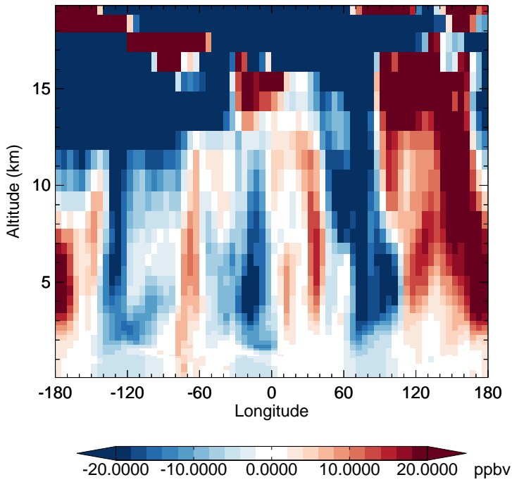
v11-02f-Run1 - v11-02e-Run0 O3 - Diff along 15S for Jan
