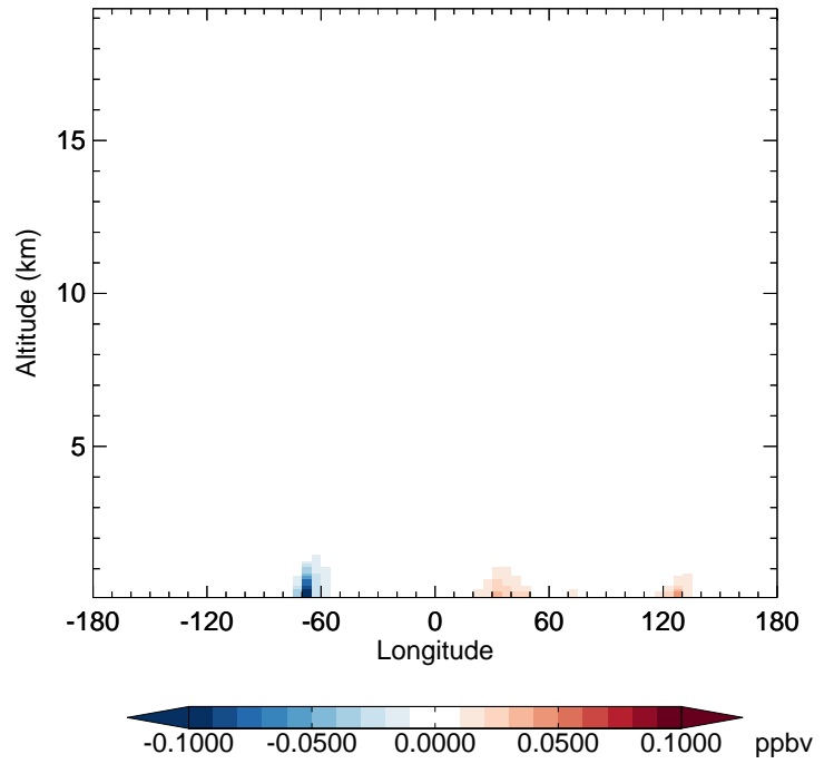
v11-02f-Run1 - v11-02e-Run1 SOAP - Diff along 42N for Jan
