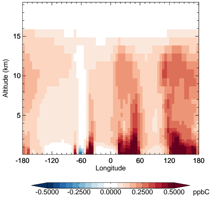
v11-02f-Run1 - v11-02e-Run1 ACET - Diff along 15S for Jan
