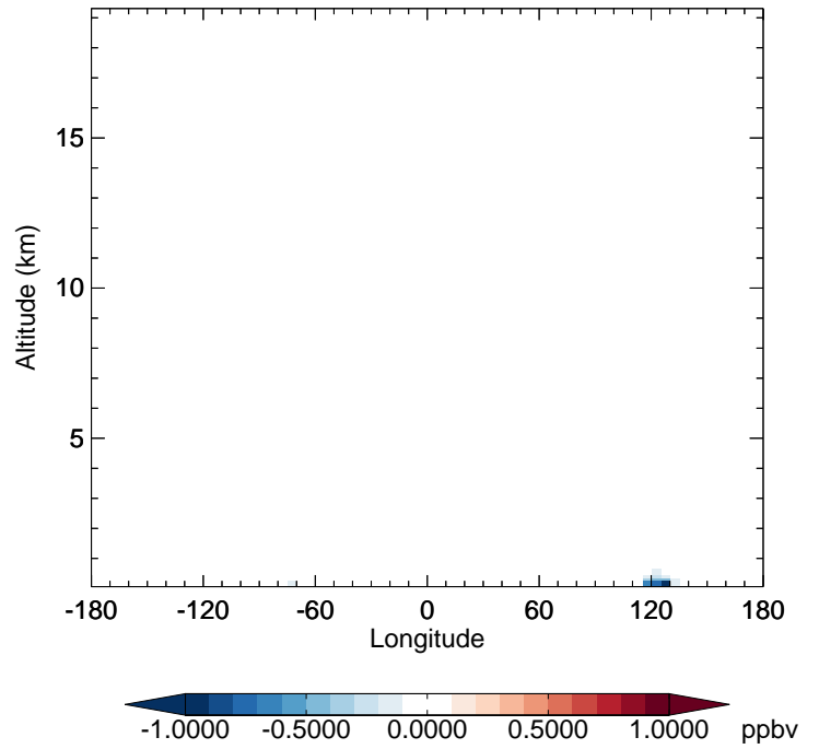
v11-02f-Run1 - v11-02e-Run0 HNO 2 - Diff along 42N for Jan
