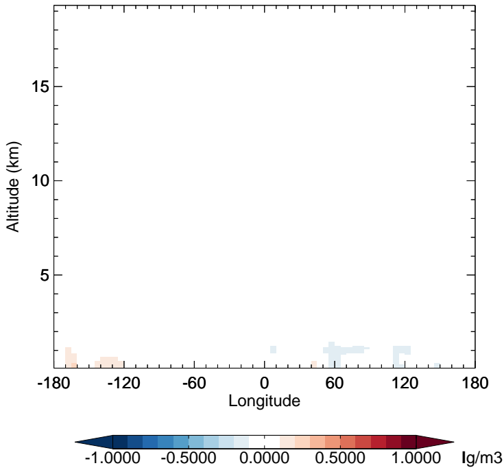
v11-02f-Run1 - v11-02e-Run0 DMS - Diff along 15S for Jan
