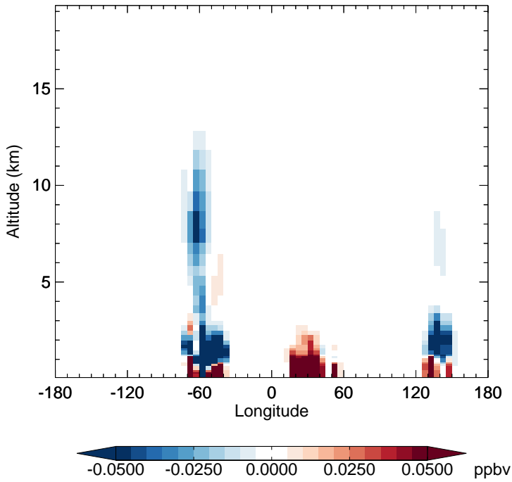
v11-02f-Run1 - v11-02e-Run0 MVK - Diff along 15S for Jan
