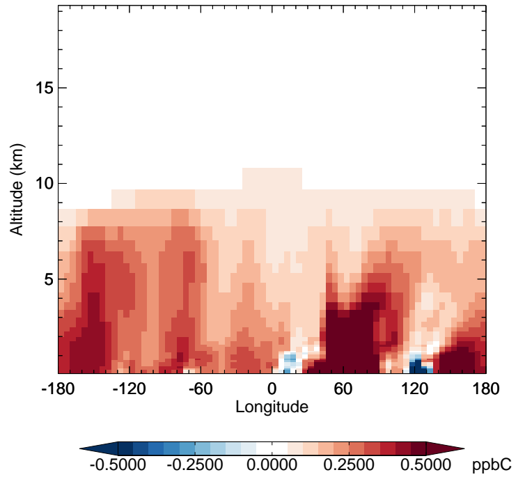
v11-02f-Run1 - v11-02e-Run0 C3H8 - Diff along 42N for Jan
