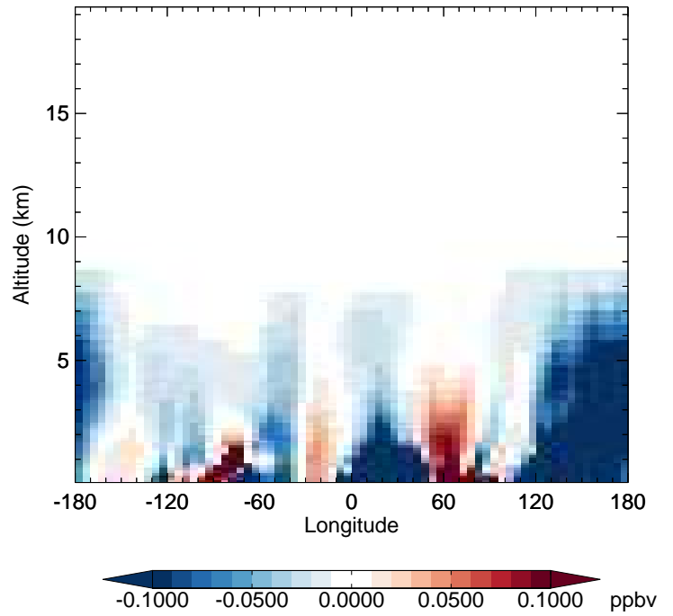
v11-02f-Run1 - v11-02e-Run0 TOLU - Diff along 42N for Jan
