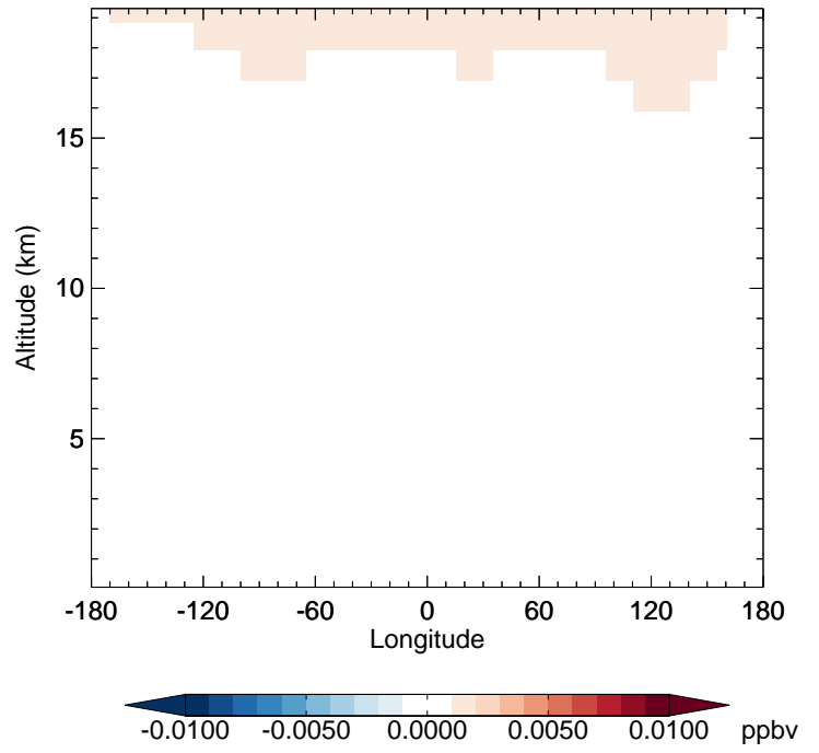
v11-02f-Run1 - v11-02e-Run1 BrO - Diff along 42N for Jan
