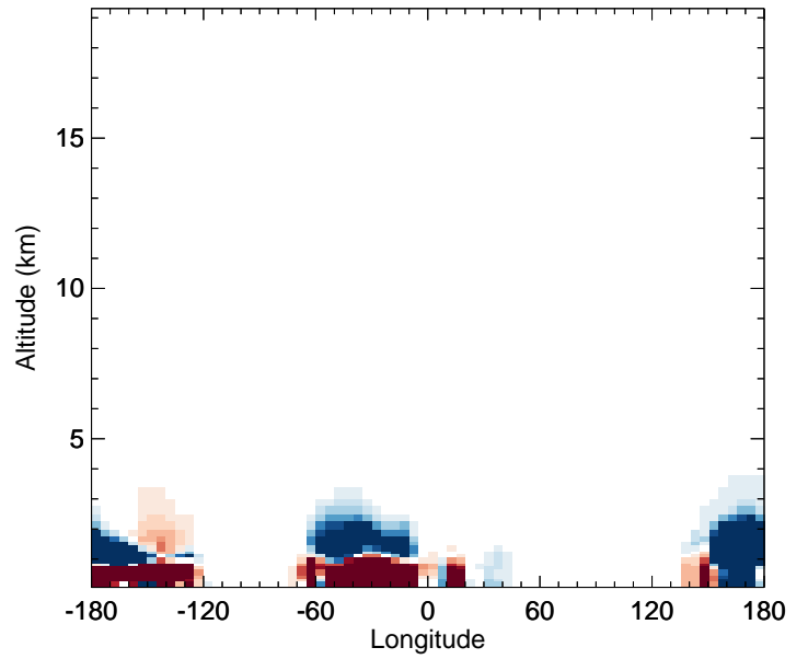
v11-02f-Run1 - v11-02e-Run0 SALC - Diff along 42N for Jan
