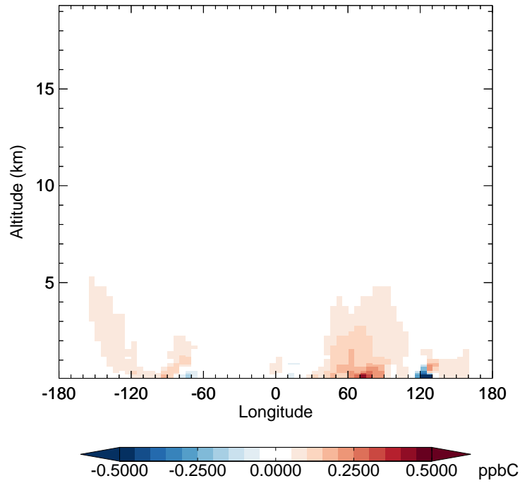
v11-02f-Run1 - v11-02e-Run0 ALD2 - Diff along 42N for Jan
