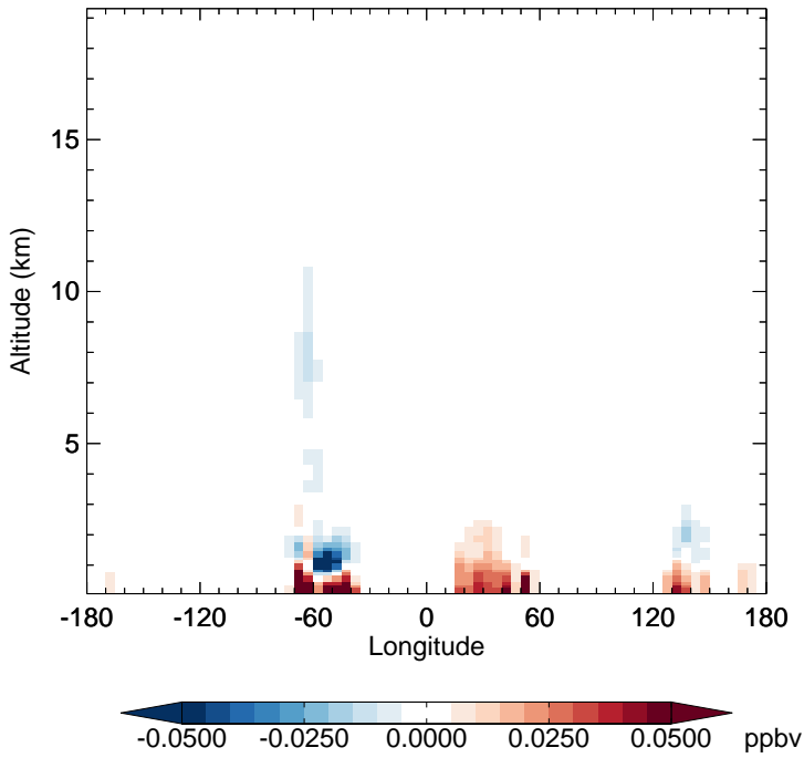
v11-02f-Run1 - v11-02e-Run0 RCHO - Diff along 15S for Jan
