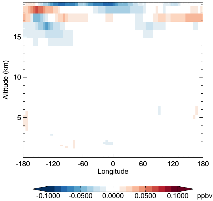
v11-02f-Run1 - v11-02e-Run0 HCl - Diff along 15S for Jan
