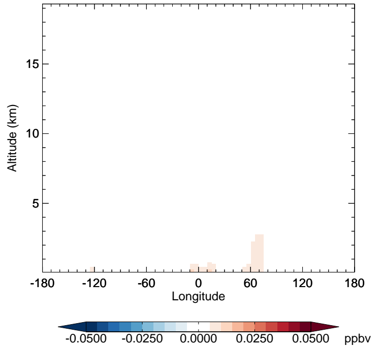
v11-02f-Run1 - v11-02e-Run1 RCHO - Diff along 42N for Jan
