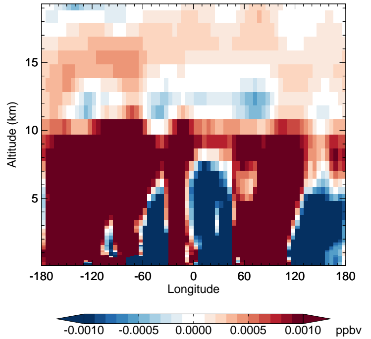
v11-02f-Run1 - v11-02e-Run0 PPN - Diff along 42N for Jan
