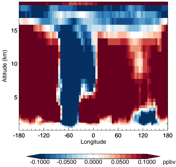
v11-02f-Run1 - v11-02e-Run1 CH4 - Diff along 15S for Jan
