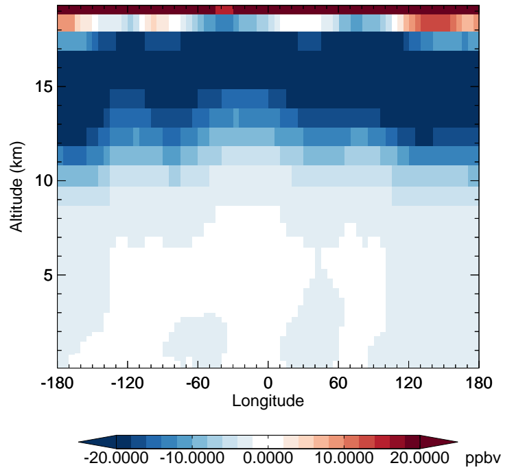
v11-02f-Run1 - v11-02e-Run1 O3 - Diff along 42N for Jan
