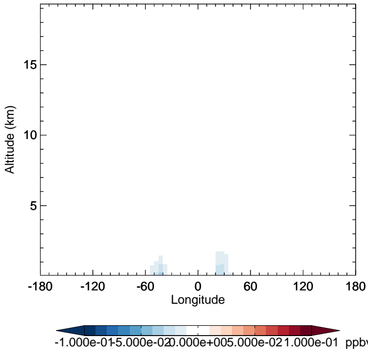
v11-02f-Run1 - v11-02e-Run1 MONITA - Diff along 15S for Jan
