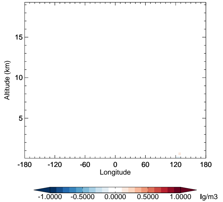
v11-02f-Run1 - v11-02e-Run0 BCPO - Diff along 42N for Jan
