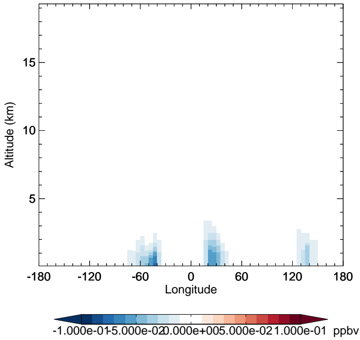
v11-02f-Run1 - v11-02e-Run1 IONITA - Diff along 15S for Jan
