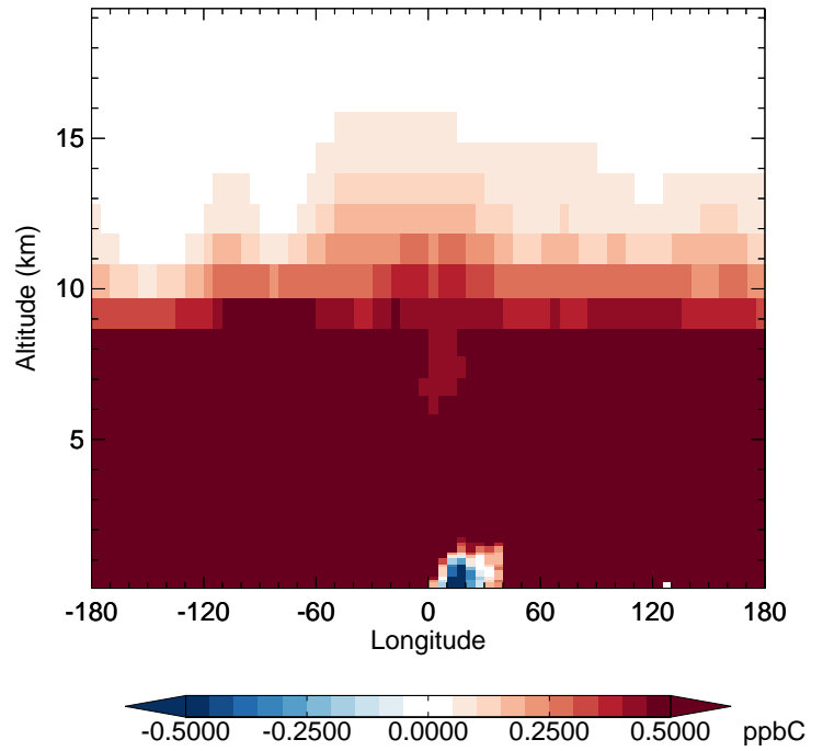
v11-02f-Run1 - v11-02e-Run0 C2H6 - Diff along 42N for Jan
