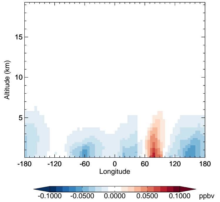
v11-02f-Run1 - v11-02e-Run1 PAN - Diff along 42N for Jan
