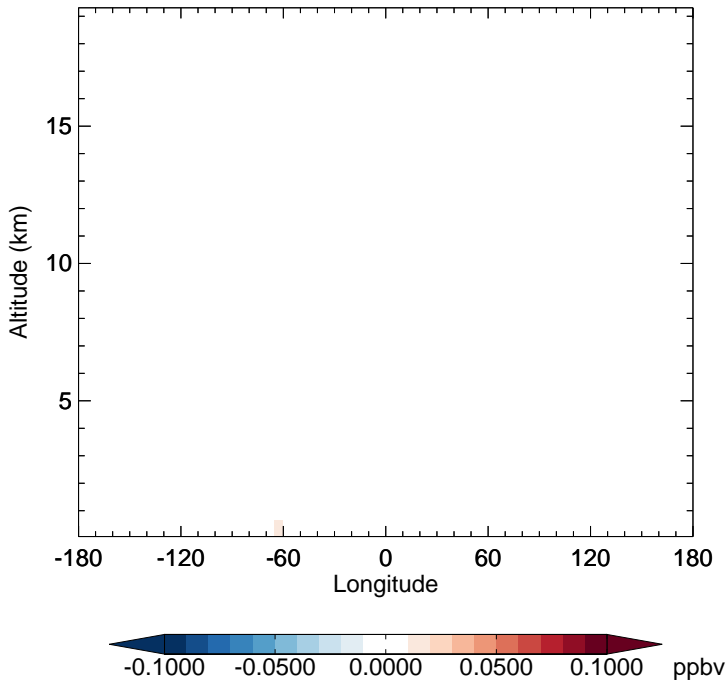
v11-02f-Run1 - v11-02e-Run0 TSOA3 - Diff along 15S for Jan
