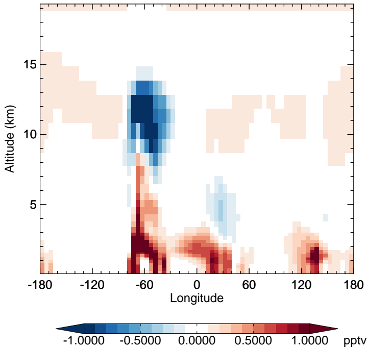
v11-02f-Run1 - v11-02e-Run1 HO2 - Diff along 15S for Jan
