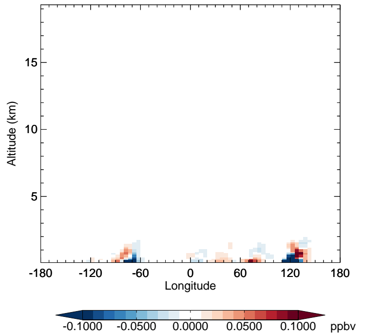
v11-02f-Run1 - v11-02e-Run0 SOAP - Diff along 42N for Jan
