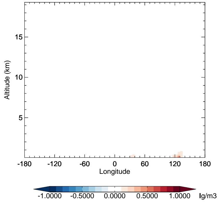
v11-02f-Run1 - v11-02e-Run1 OCPO - Diff along 42N for Jan
