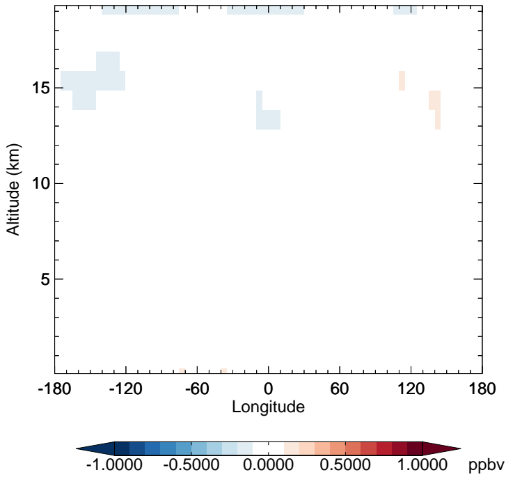
v11-02f-Run1 - v11-02e-Run0 NO2 - Diff along 15S for Jan
