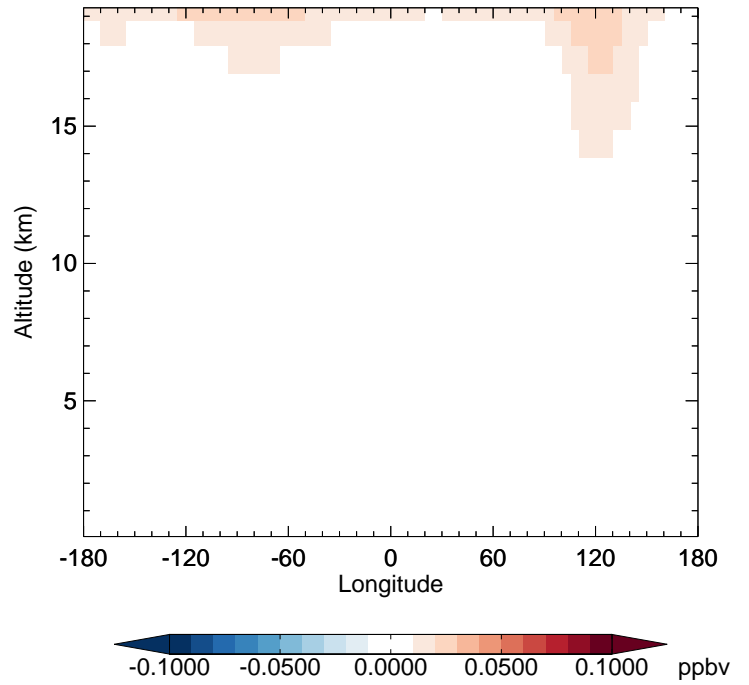
v11-02f-Run1 - v11-02e-Run0 ClO - Diff along 42N for Jan
