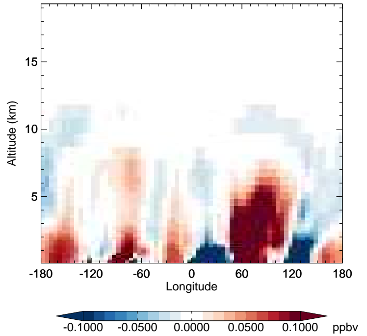
v11-02f-Run1 - v11-02e-Run0 BENZ - Diff along 42N for Jan
