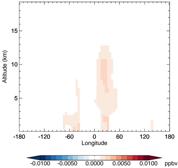
v11-02f-Run1 - v11-02e-Run1 R4N2 - Diff along 15S for Jan
