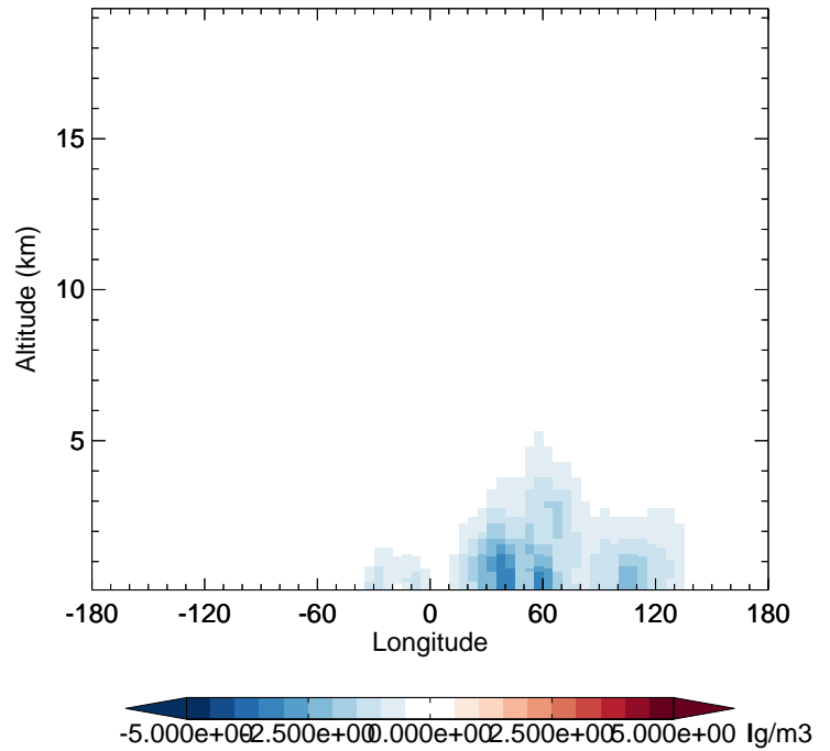
v11-02f-Run1 - v11-02e-Run0 DST1 - Diff along 42N for Jan
