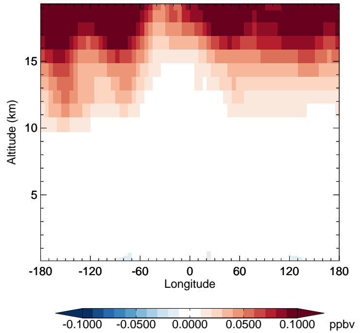
v11-02f-Run1 - v11-02e-Run0 HCl - Diff along 42N for Jan
