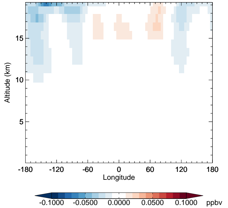
v11-02f-Run1 - v11-02e-Run0 OCS - Diff along 42N for Jan
