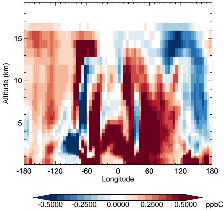
v11-02f-Run1 - v11-02e-Run0 ACET - Diff along 15S for Jan
