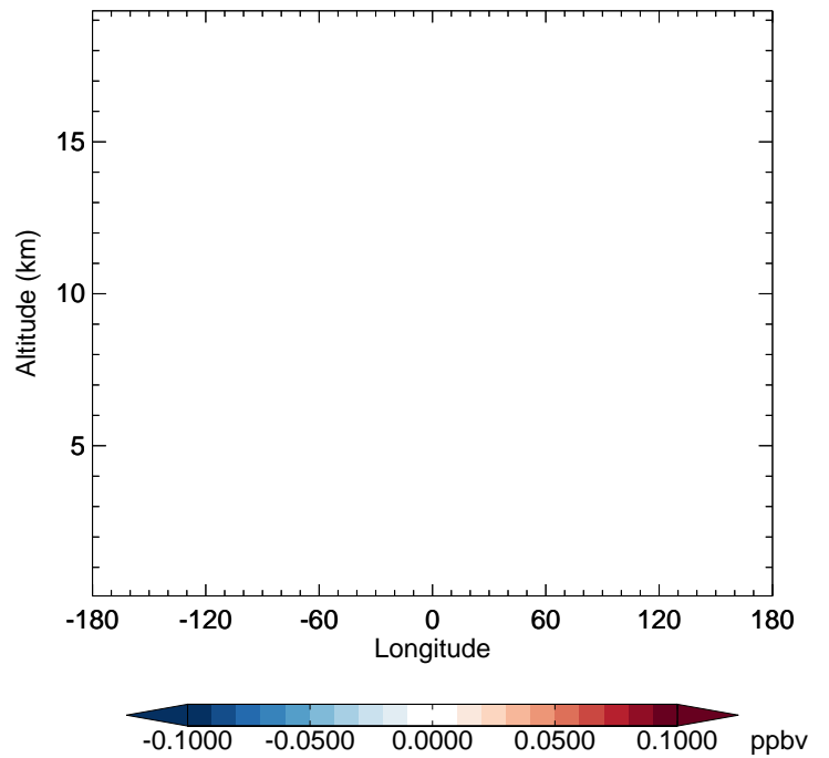
v11-02f-Run1 - v11-02e-Run0 MTPA - Diff along 42N for Jan
