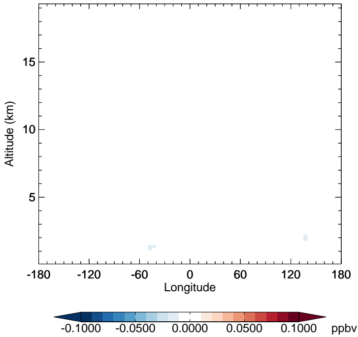
v11-02f-Run1 - v11-02e-Run0 GLYX - Diff along 15S for Jan
