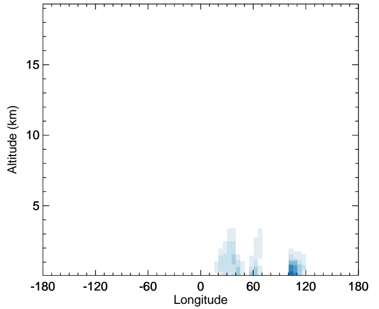
v11-02f-Run1 - v11-02e-Run0 DST3 - Diff along 42N for Jan
