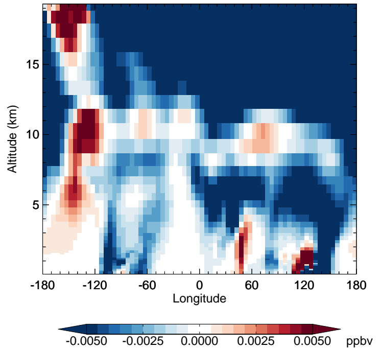
v11-02f-Run1 - v11-02e-Run0 HNO 4 - Diff along 42N for Jan
