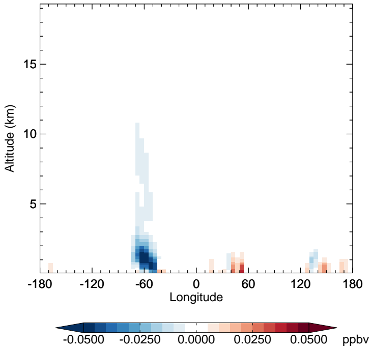
v11-02f-Run1 - v11-02e-Run1 RCHO - Diff along 15S for Jan
