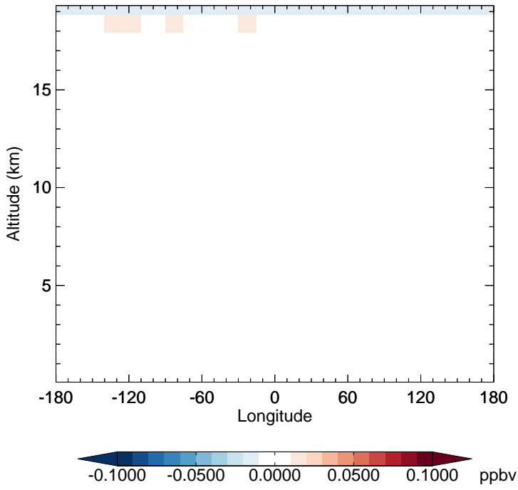
v11-02f-Run1 - v11-02e-Run1 HCl - Diff along 15S for Jan
