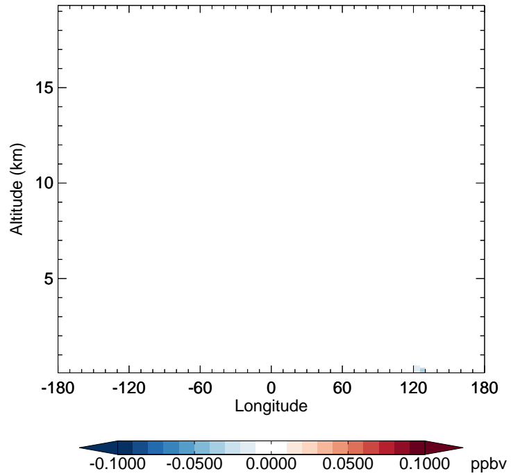
v11-02f-Run1 - v11-02e-Run0 ASOA3 - Diff along 42N for Jan
