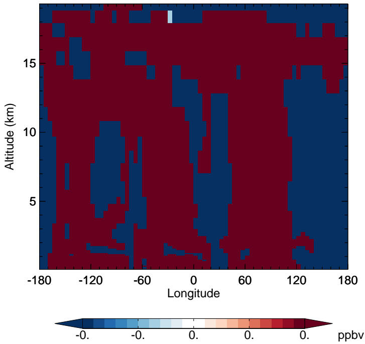
v11-02f-Run1 - v11-02e-Run0 H2O - Diff along 15S for Jan
