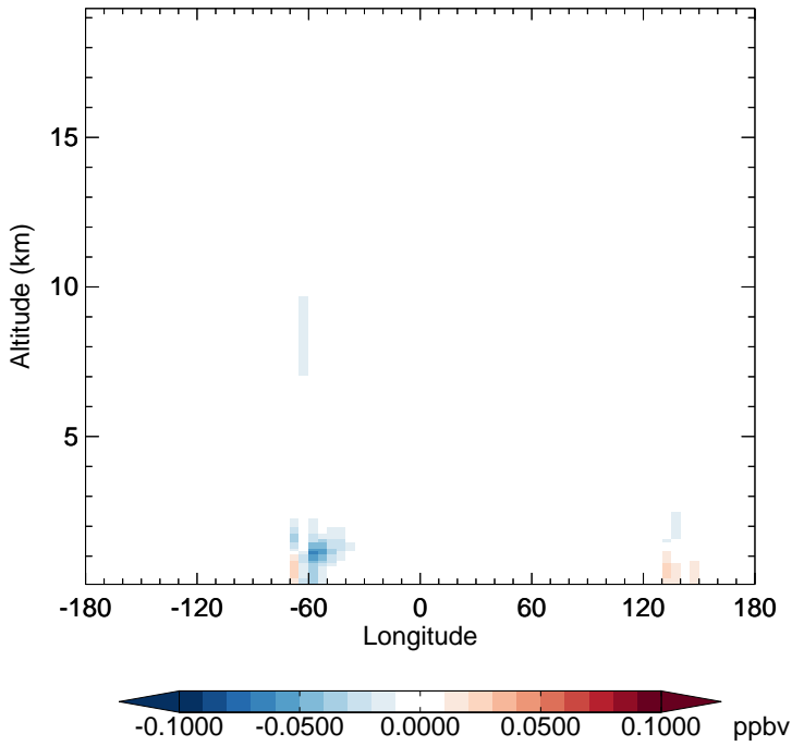
v11-02f-Run1 - v11-02e-Run0 RIPB - Diff along 15S for Jan
