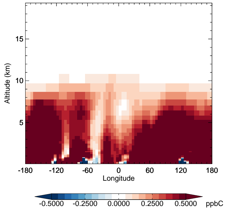
v11-02f-Run1 - v11-02e-Run0 ALK4 - Diff along 42N for Jan
