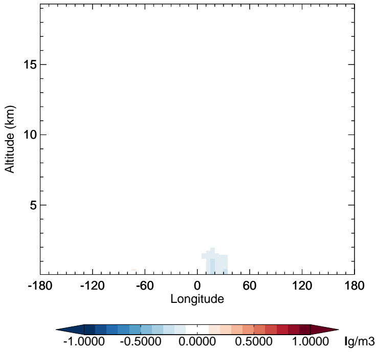
v11-02f-Run1 - v11-02e-Run1 NH4 - Diff along 15S for Jan
