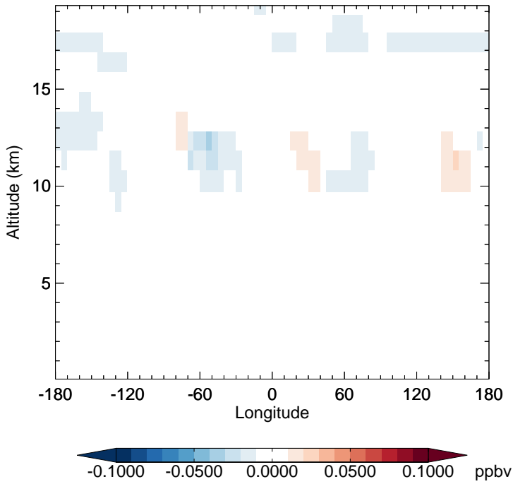
v11-02f-Run1 - v11-02e-Run0 MPN - Diff along 15S for Jan
