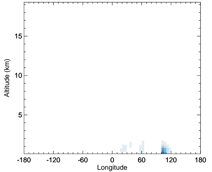
v11-02f-Run1 - v11-02e-Run0 DST4 - Diff along 42N for Jan
