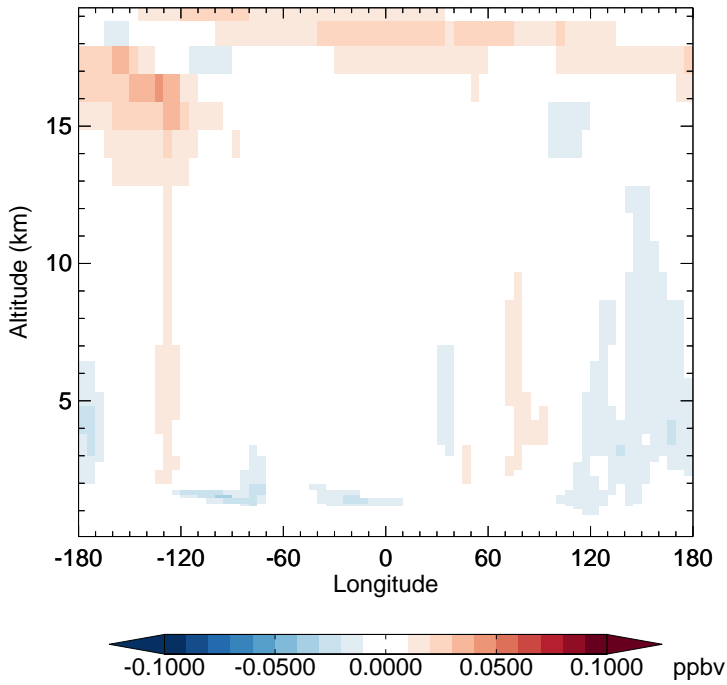
v11-02f-Run1 - v11-02e-Run0 CH3Cl - Diff along 15S for Jan
