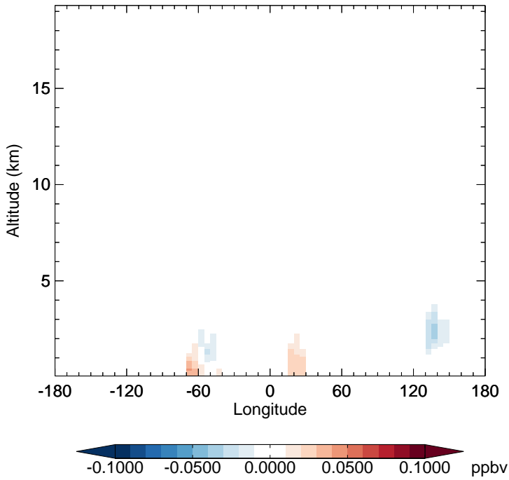
v11-02f-Run1 - v11-02e-Run0 ISOA1 - Diff along 15S for Jan
