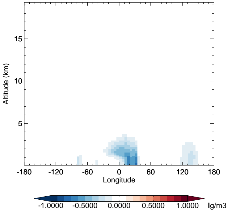
v11-02f-Run1 - v11-02e-Run1 SO4 - Diff along 15S for Jan
