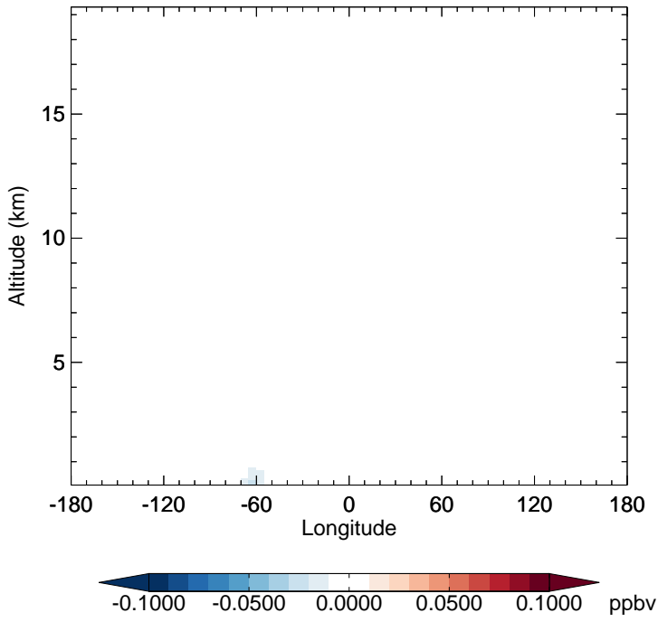
v11-02f-Run1 - v11-02e-Run1 LIMO - Diff along 15S for Jan
