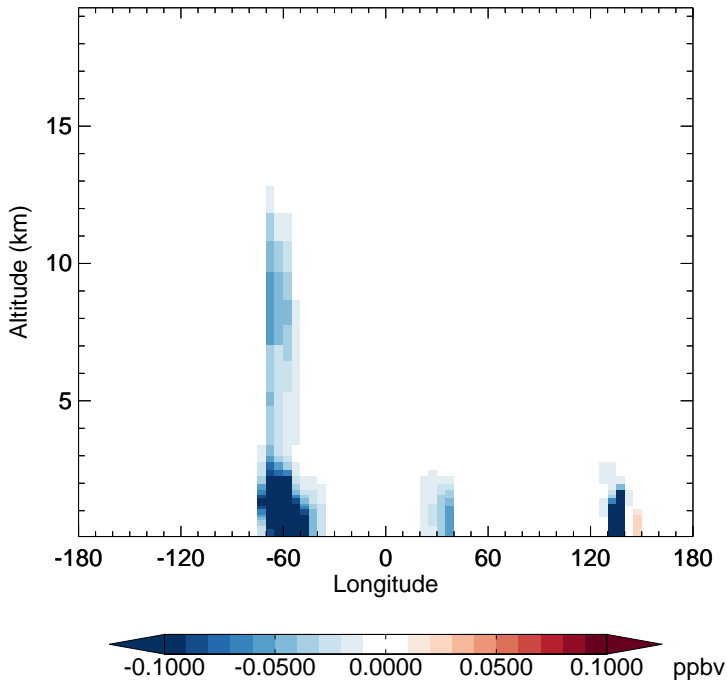
v11-02f-Run1 - v11-02e-Run1 RIPA - Diff along 15S for Jan
