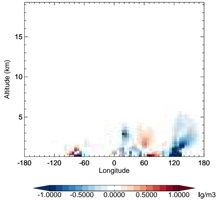
v11-02f-Run1 - v11-02e-Run0 SO 2 - Diff along 42N for Jan
