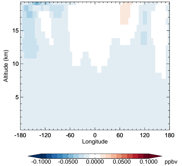
v11-02f-Run1 - v11-02e-Run0 CFC12 - Diff along 42N for Jan
