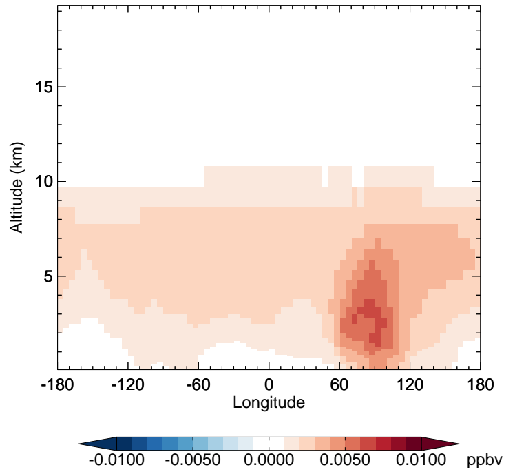
v11-02f-Run1 - v11-02e-Run1 MAP - Diff along 42N for Jan
