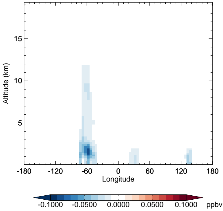
v11-02f-Run1 - v11-02e-Run1 IPMN - Diff along 15S for Jan
