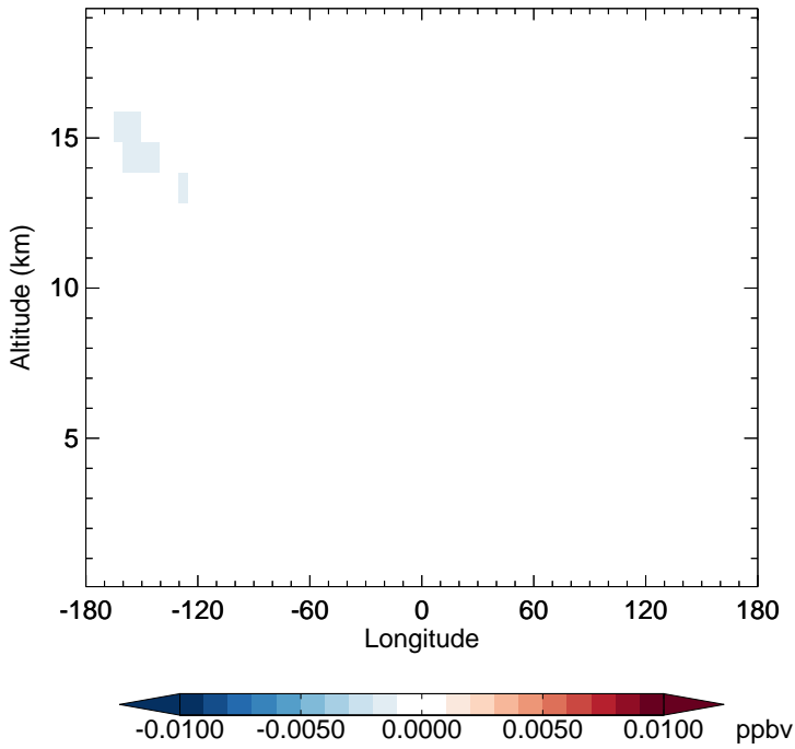
v11-02f-Run1 - v11-02e-Run0 BrNO3 - Diff along 15S for Jan
