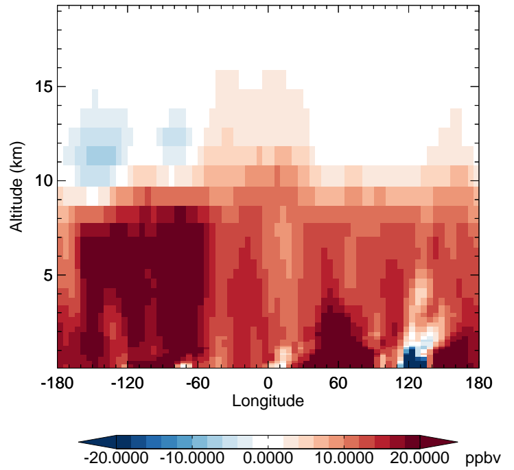
v11-02f-Run1 - v11-02e-Run0 CO - Diff along 42N for Jan
