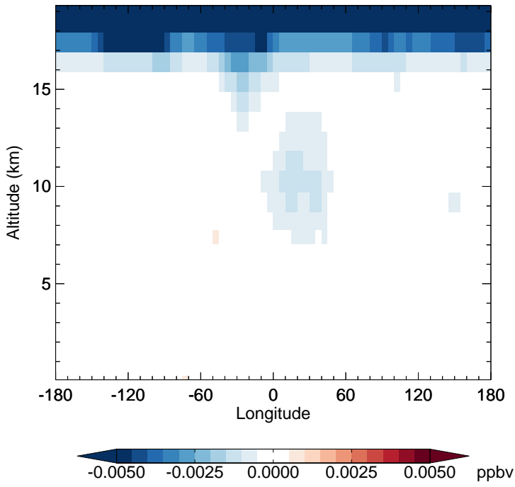
v11-02f-Run1 - v11-02e-Run1 N2O5 - Diff along 15S for Jan
