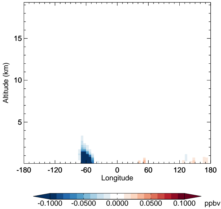
v11-02f-Run1 - v11-02e-Run1 MTPA - Diff along 15S for Jan
