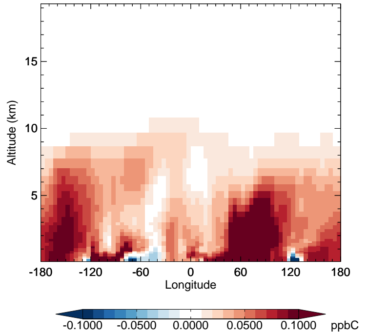
v11-02f-Run1 - v11-02e-Run0 MEK - Diff along 42N for Jan
