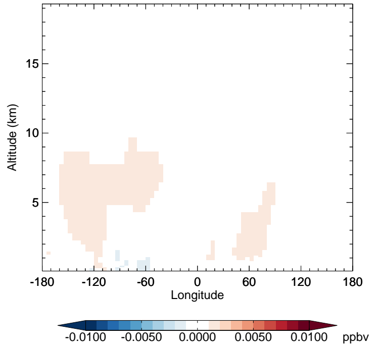
v11-02f-Run1 - v11-02e-Run0 R4N2 - Diff along 42N for Jan
