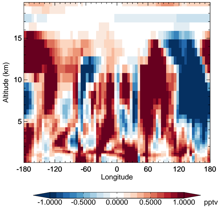
v11-02f-Run1 - v11-02e-Run0 HO2 - Diff along 15S for Jan
