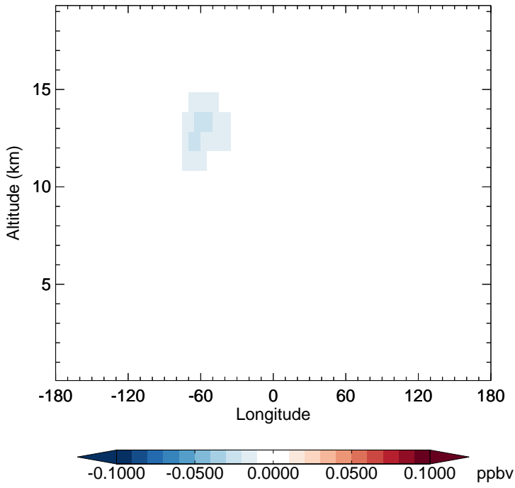
v11-02f-Run1 - v11-02e-Run1 ISOA3 - Diff along 15S for Jan
