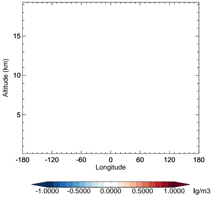
v11-02f-Run1 - v11-02e-Run1 NH3 - Diff along 15S for Jan
