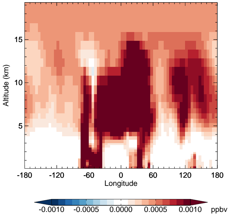
v11-02f-Run1 - v11-02e-Run1 PPN - Diff along 15S for Jan
