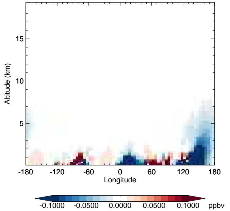
v11-02f-Run1 - v11-02e-Run0 XYLE - Diff along 42N for Jan
