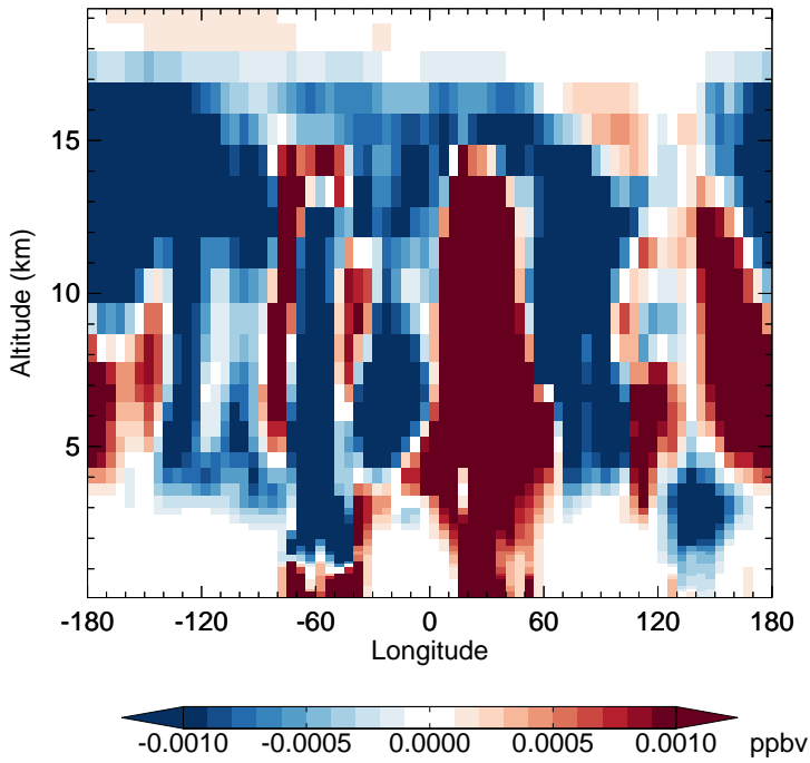
v11-02f-Run1 - v11-02e-Run0 PPN - Diff along 15S for Jan
