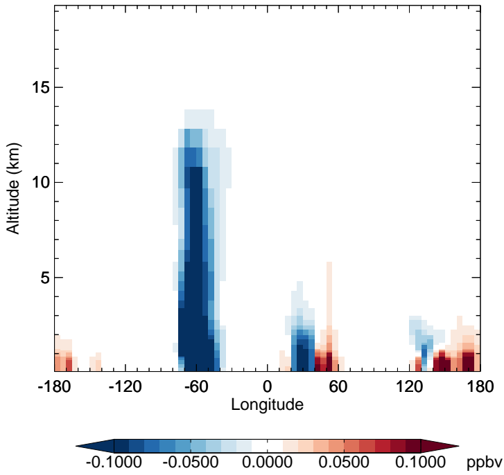
v11-02f-Run1 - v11-02e-Run1 EOH - Diff along 15S for Jan
