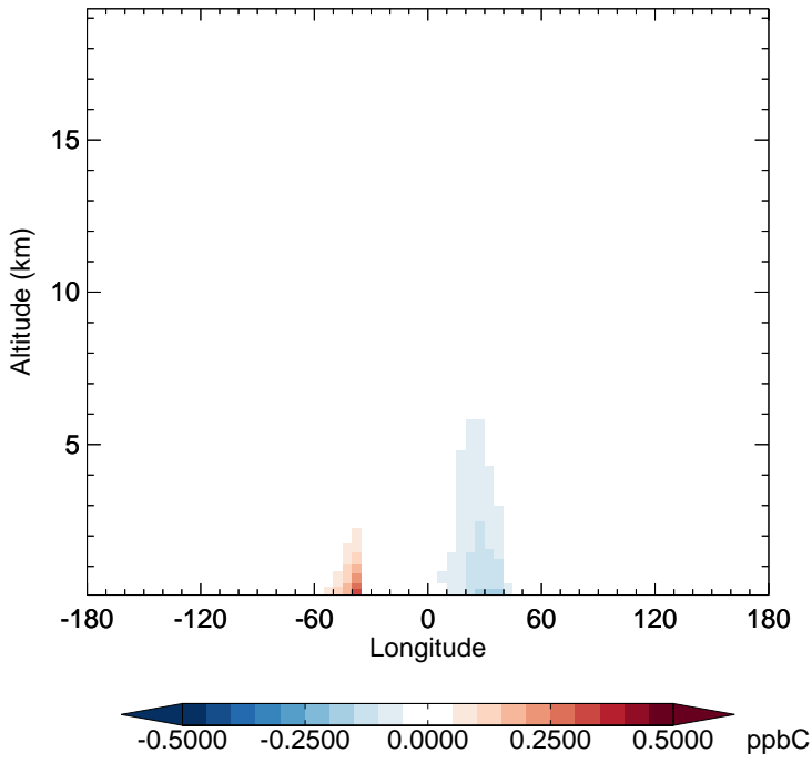
v11-02f-Run1 - v11-02e-Run1 C3H8 - Diff along 15S for Jan
