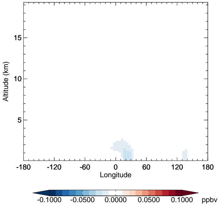
v11-02f-Run1 - v11-02e-Run1 SOAGX - Diff along 15S for Jan
