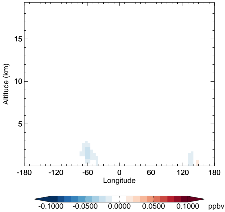
v11-02f-Run1 - v11-02e-Run1 MGLY - Diff along 15S for Jan
