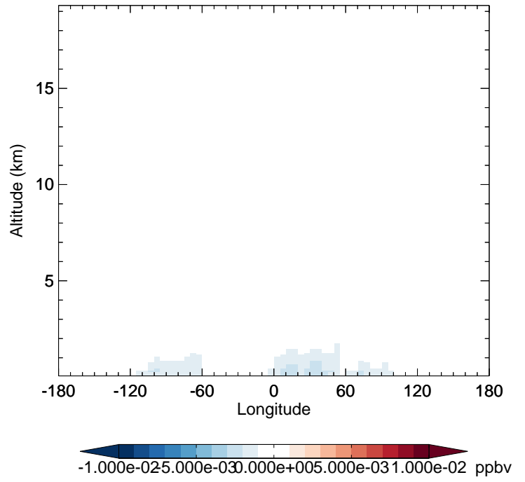
v11-02f-Run1 - v11-02e-Run1 NO3 - Diff along 42N for Jan
