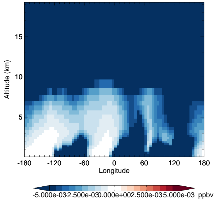
v11-02f-Run1 - v11-02e-Run1 N2O5 - Diff along 42N for Jan
