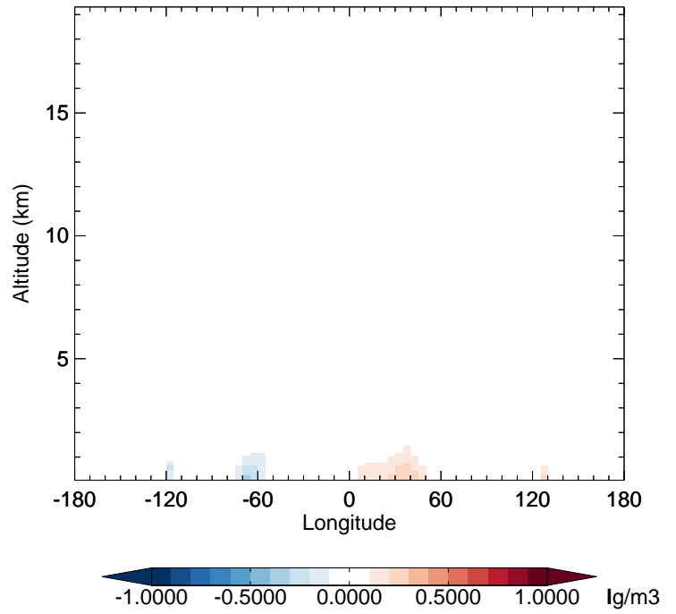
v11-02f-Run1 - v11-02e-Run1 SOAS - Diff along 42N for Jan
