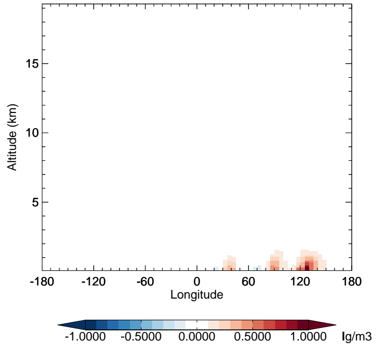
v11-02f-Run1 - v11-02e-Run1 OCPI - Diff along 42N for Jan
