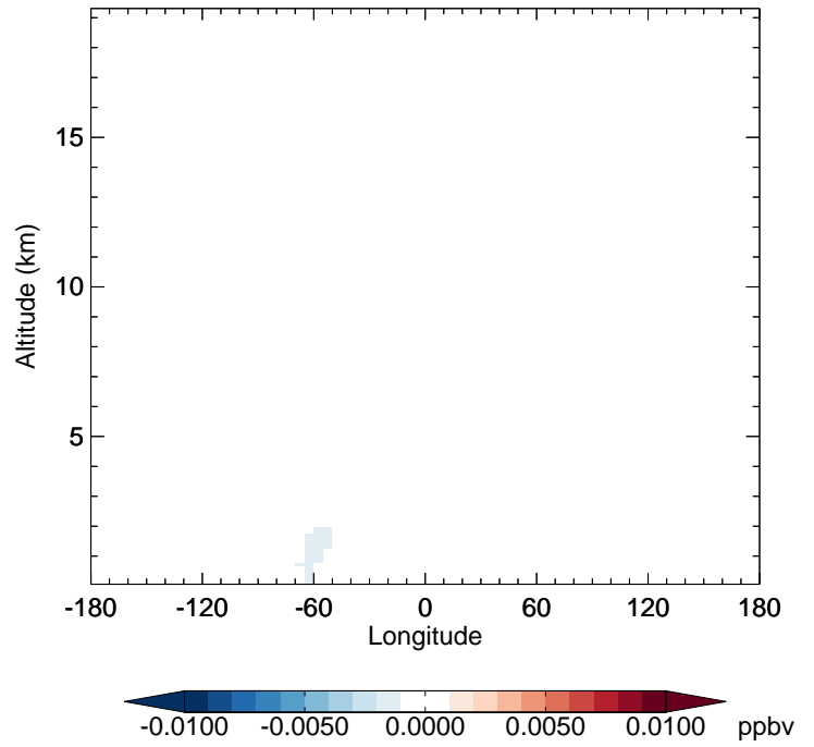
v11-02f-Run1 - v11-02e-Run1 R4N2 - Diff along 42N for Jan
