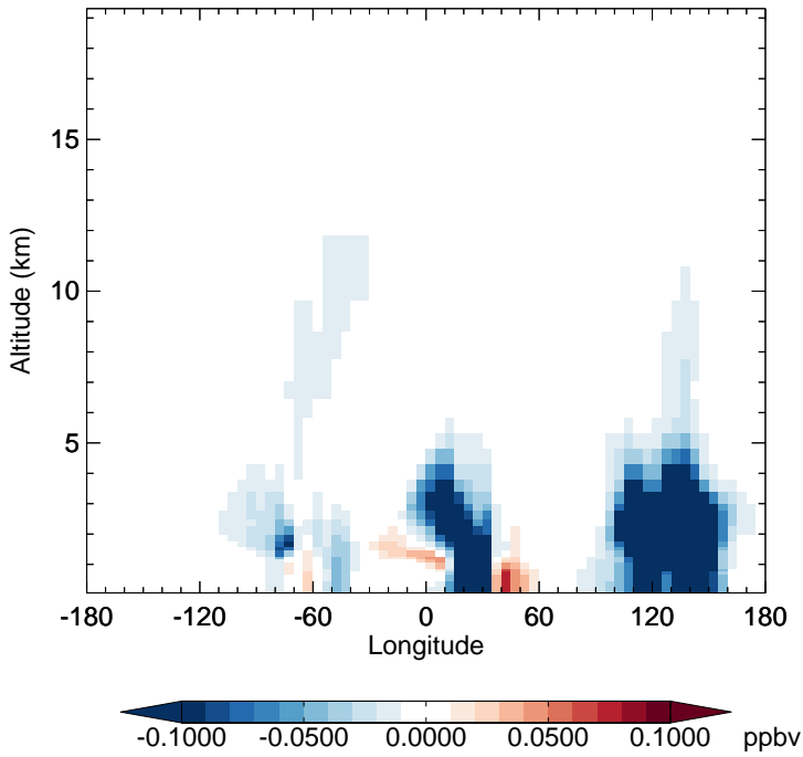
v11-02f-Run1 - v11-02e-Run0 SOAIE - Diff along 15S for Jan
