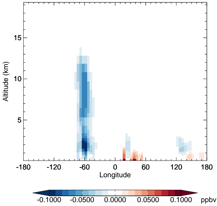
v11-02f-Run1 - v11-02e-Run1 HAC - Diff along 15S for Jan
