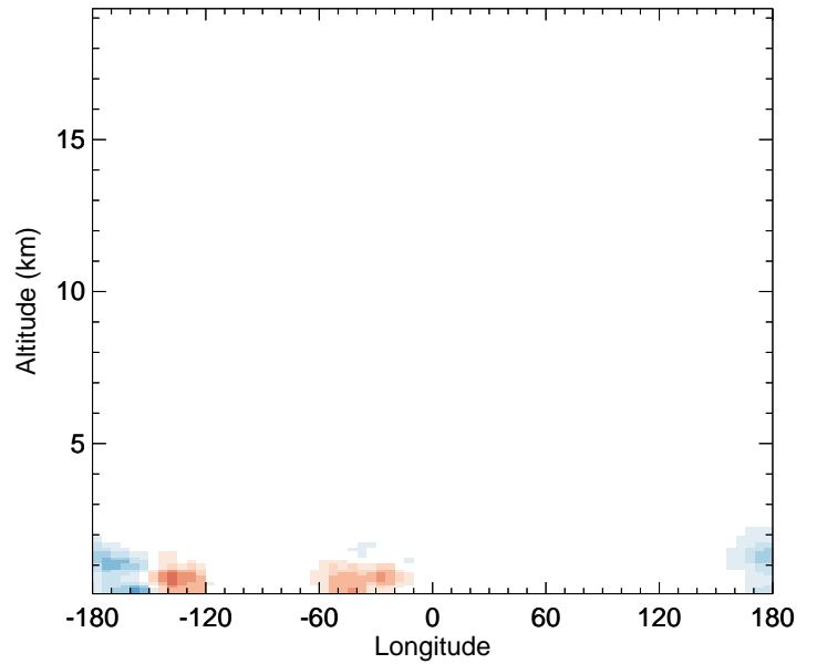
v11-02f-Run1 - v11-02e-Run0 SALA - Diff along 42N for Jan
