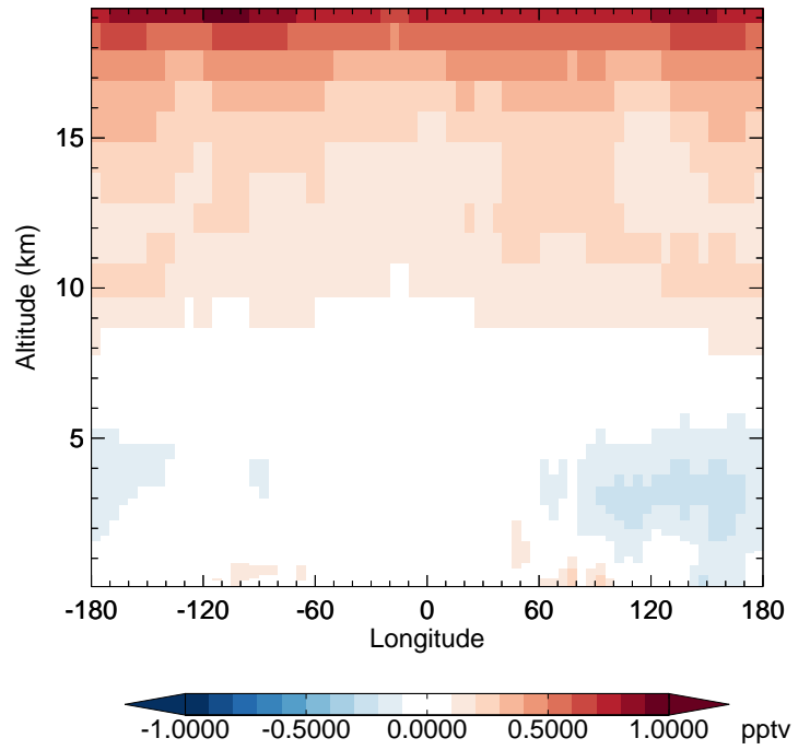
v11-02f-Run1 - v11-02e-Run1 HO2 - Diff along 42N for Jan
