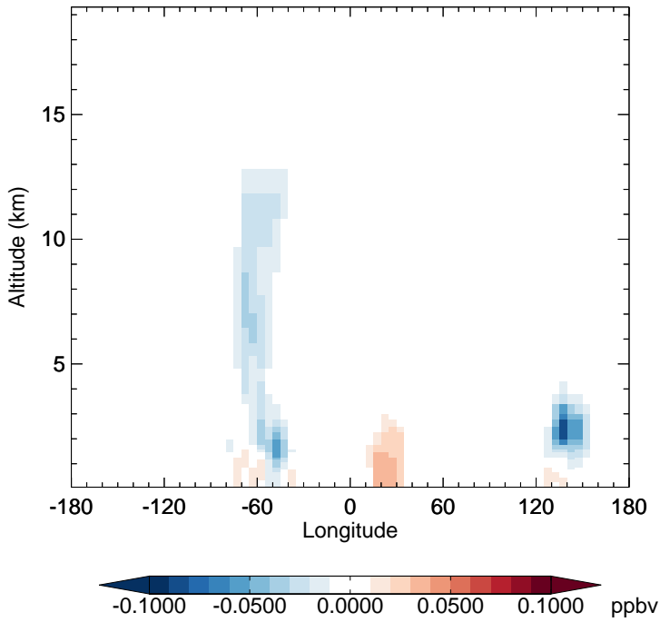
v11-02f-Run1 - v11-02e-Run0 IMAE - Diff along 15S for Jan
