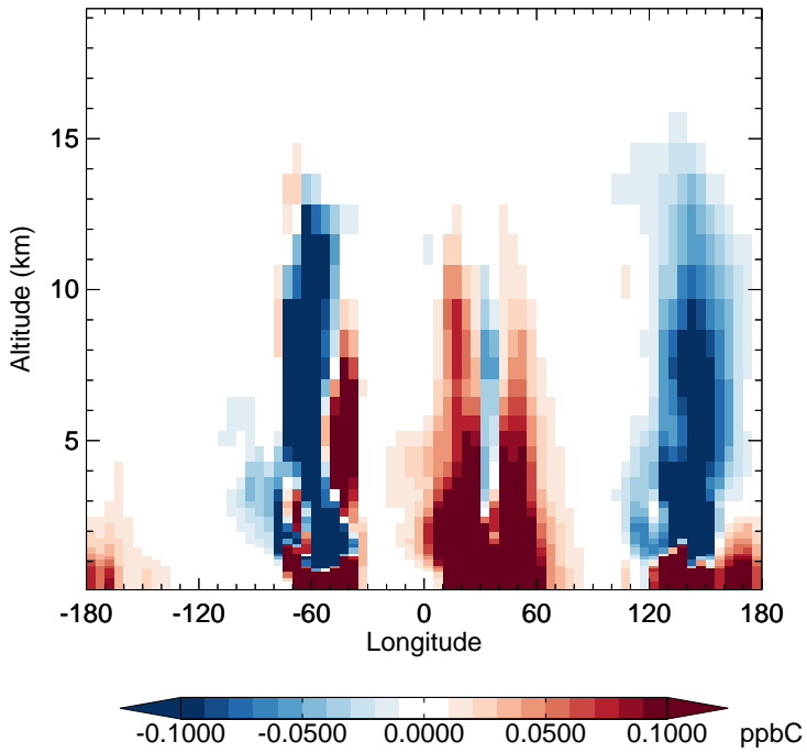
v11-02f-Run1 - v11-02e-Run0 MEK - Diff along 15S for Jan
