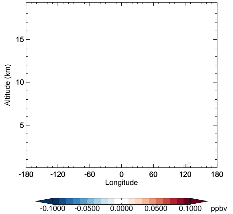
v11-02f-Run1 - v11-02e-Run0 HAC - Diff along 42N for Jan
