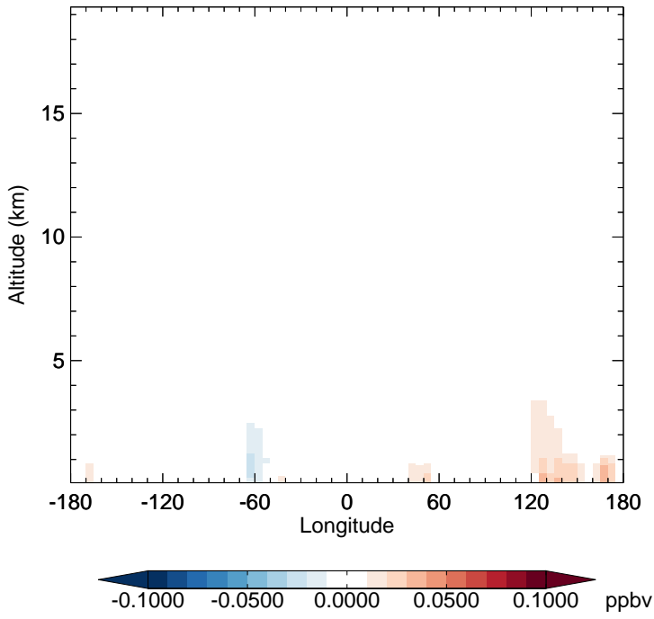
v11-02f-Run1 - v11-02e-Run1 TSOG2 - Diff along 15S for Jan
