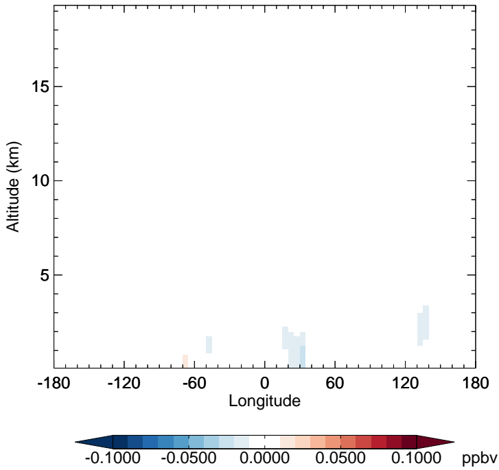
v11-02f-Run1 - v11-02e-Run0 SOAGX - Diff along 15S for Jan
