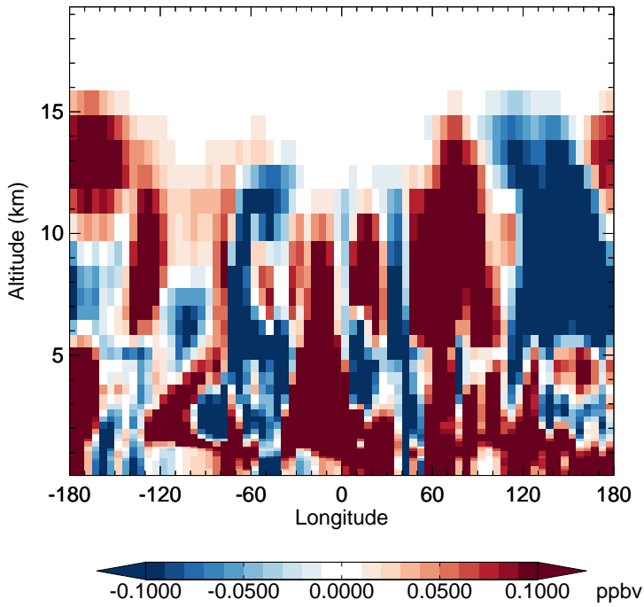
v11-02f-Run1 - v11-02e-Run0 H2O2 - Diff along 15S for Jan
