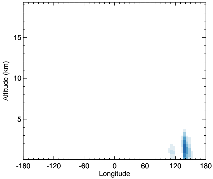
v11-02f-Run1 - v11-02e-Run0 DST3 - Diff along 15S for Jan
