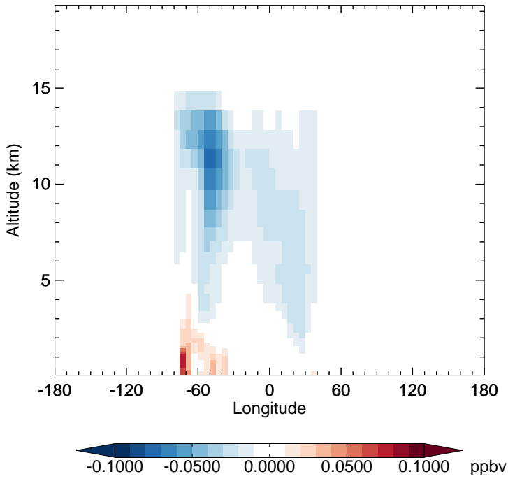
v11-02f-Run1 - v11-02e-Run1 PAN - Diff along 15S for Jan
