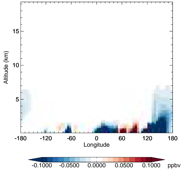
v11-02f-Run1 - v11-02e-Run1 XYLE - Diff along 42N for Jan
