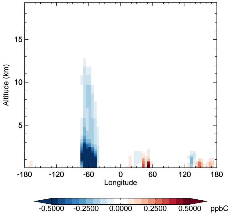
v11-02f-Run1 - v11-02e-Run1 ALD2 - Diff along 15S for Jan
