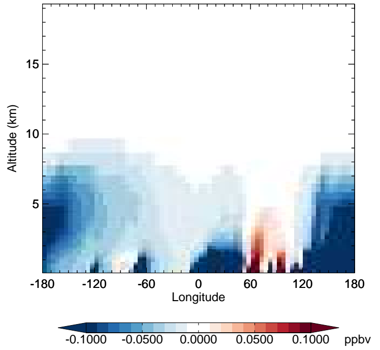
v11-02f-Run1 - v11-02e-Run1 TOLU - Diff along 42N for Jan
