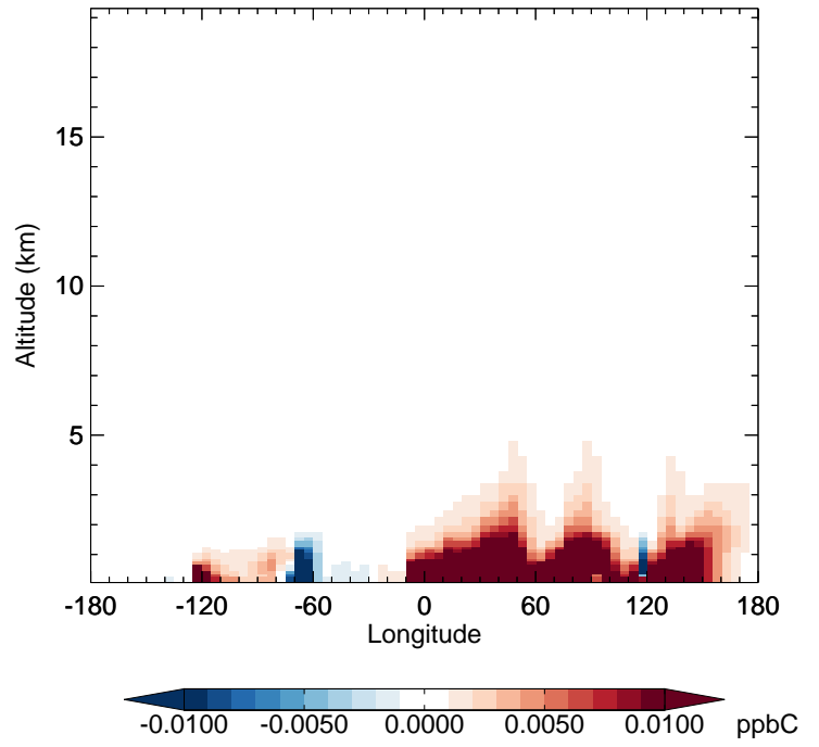
v11-02f-Run1 - v11-02e-Run1 PRPE - Diff along 42N for Jan
