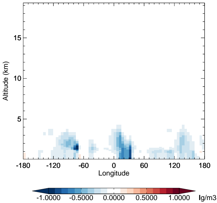
v11-02f-Run1 - v11-02e-Run0 SO4 - Diff along 15S for Jan
