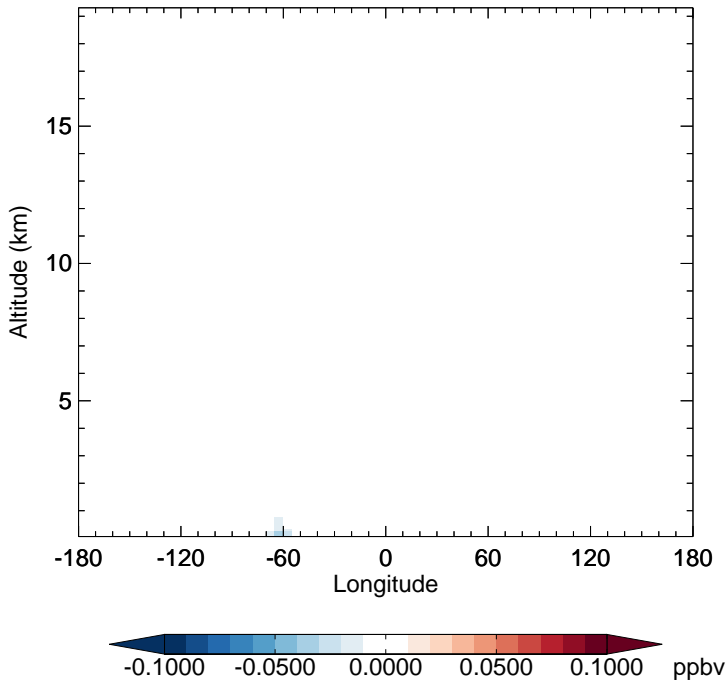
v11-02f-Run1 - v11-02e-Run1 MTPO - Diff along 15S for Jan
