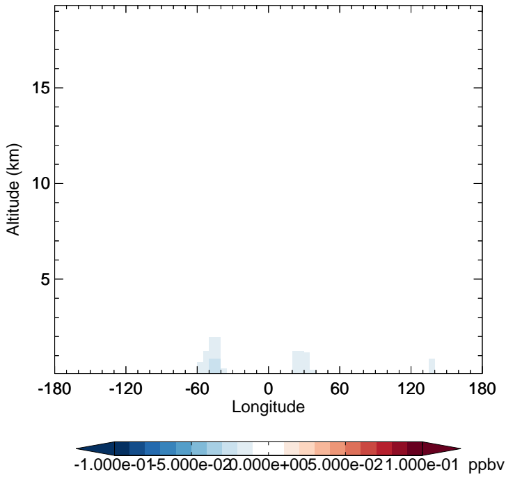
v11-02f-Run1 - v11-02e-Run0 MONITA - Diff along 15S for Jan
