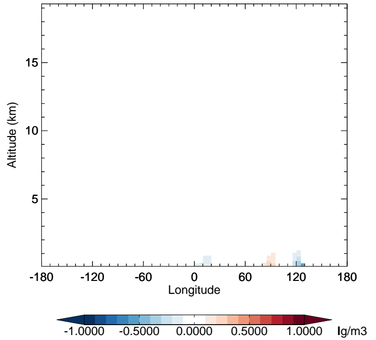
v11-02f-Run1 - v11-02e-Run0 BCPI - Diff along 42N for Jan
