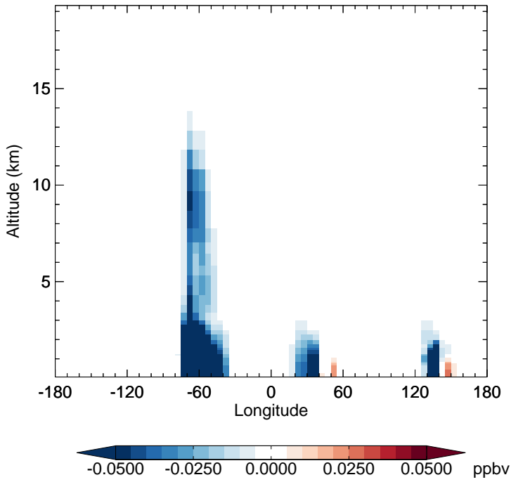
v11-02f-Run1 - v11-02e-Run1 MACR - Diff along 15S for Jan
