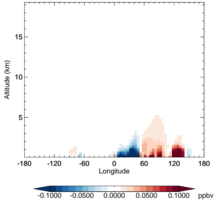
v11-02f-Run1 - v11-02e-Run1 EOH - Diff along 42N for Jan
