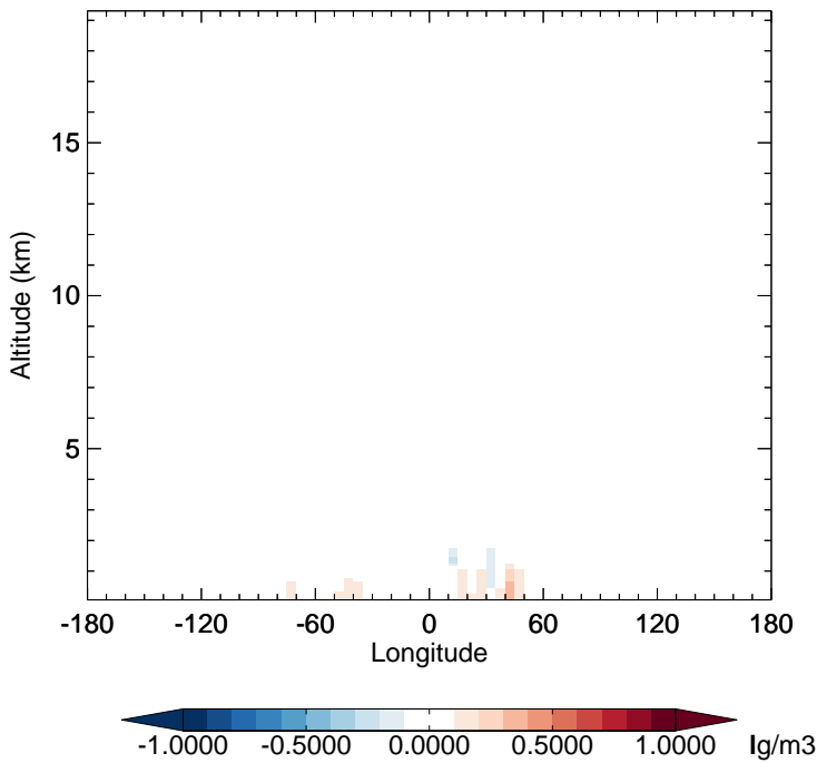
v11-02f-Run1 - v11-02e-Run0 OCPI - Diff along 15S for Jan
