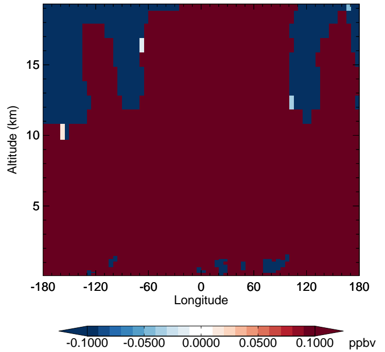
v11-02f-Run1 - v11-02e-Run0 CH4 - Diff along 42N for Jan
