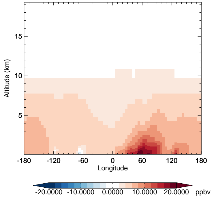
v11-02f-Run1 - v11-02e-Run1 CO - Diff along 42N for Jan
