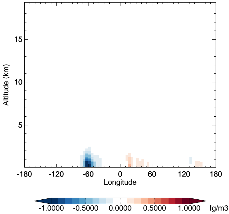
v11-02f-Run1 - v11-02e-Run1 SOAS - Diff along 15S for Jan
