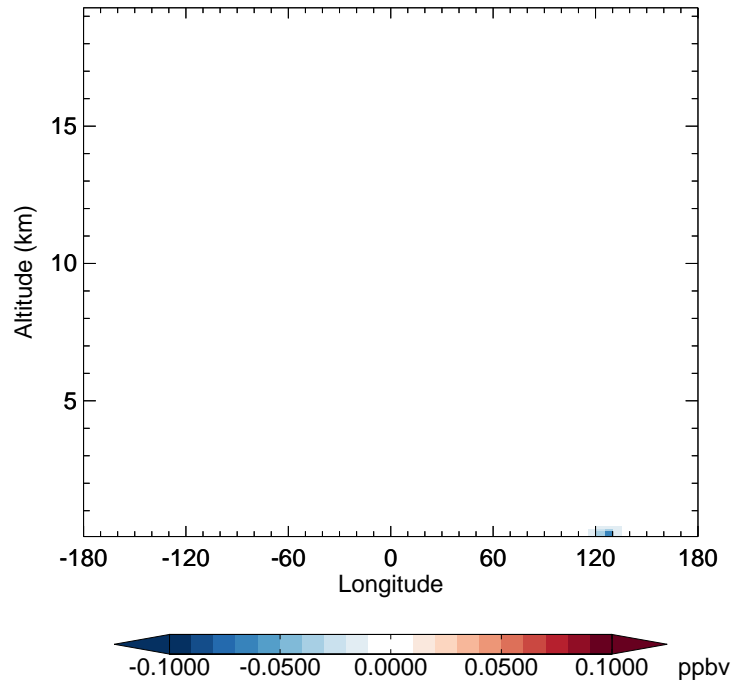
v11-02f-Run1 - v11-02e-Run0 MGLY - Diff along 42N for Jan
