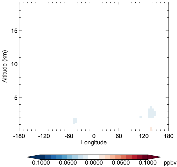
v11-02f-Run1 - v11-02e-Run0 ISOG1 - Diff along 15S for Jan
