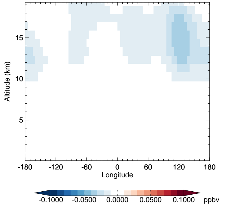
v11-02f-Run1 - v11-02e-Run1 MPN - Diff along 42N for Jan
