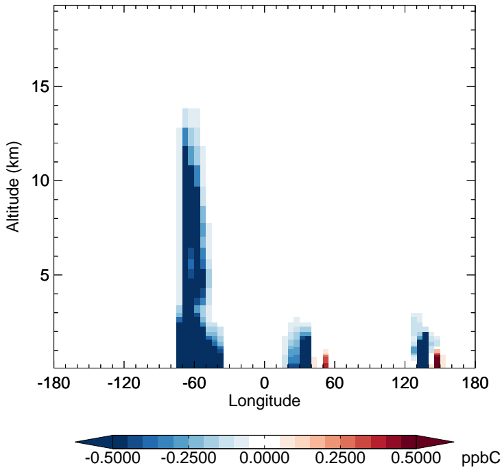
v11-02f-Run1 - v11-02e-Run1 ISOP - Diff along 15S for Jan
