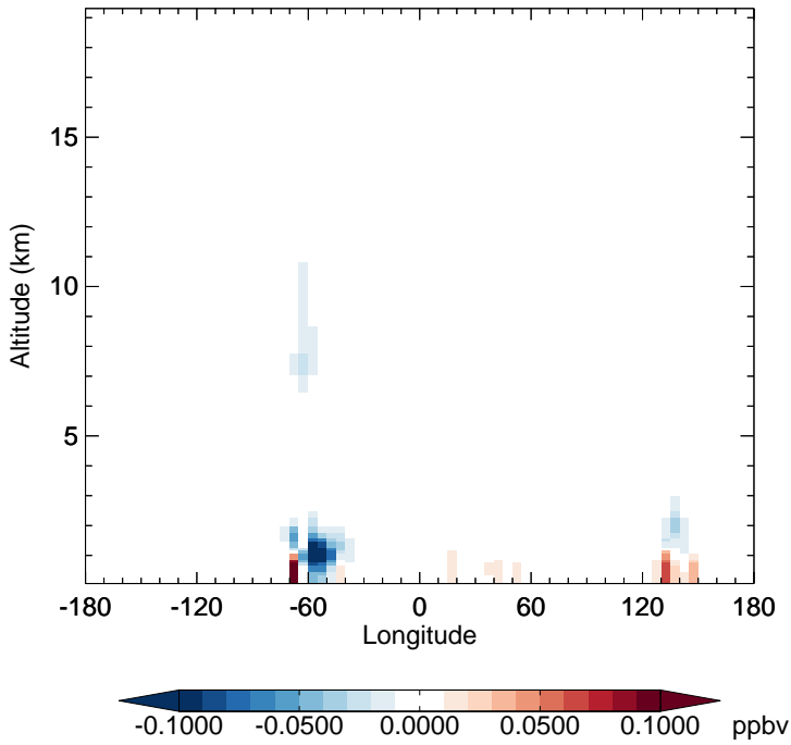
v11-02f-Run1 - v11-02e-Run0 HPALD - Diff along 15S for Jan
