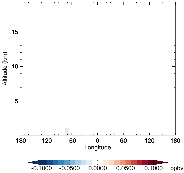
v11-02f-Run1 - v11-02e-Run1 XYLE - Diff along 15S for Jan
