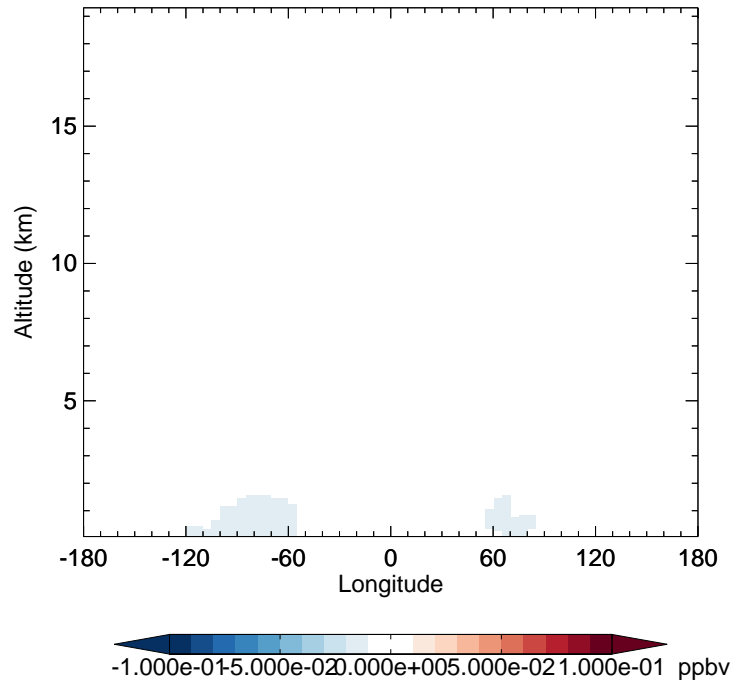
v11-02f-Run1 - v11-02e-Run1 IONITA - Diff along 42N for Jan
