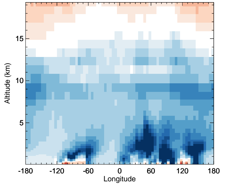
v11-02f-Run1 - v11-02e-Run1 OH - Diff along 42N for Jan
