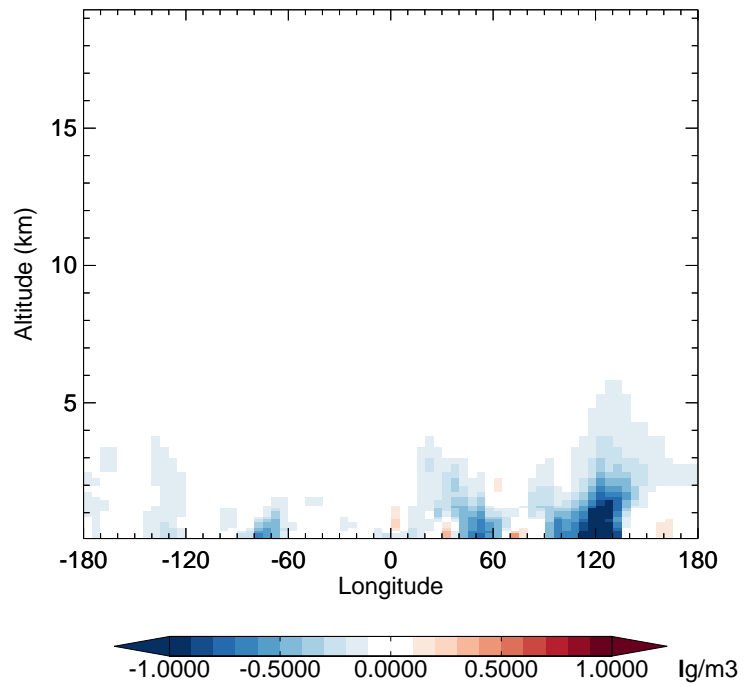
v11-02f-Run1 - v11-02e-Run0 SO4 - Diff along 42N for Jan
