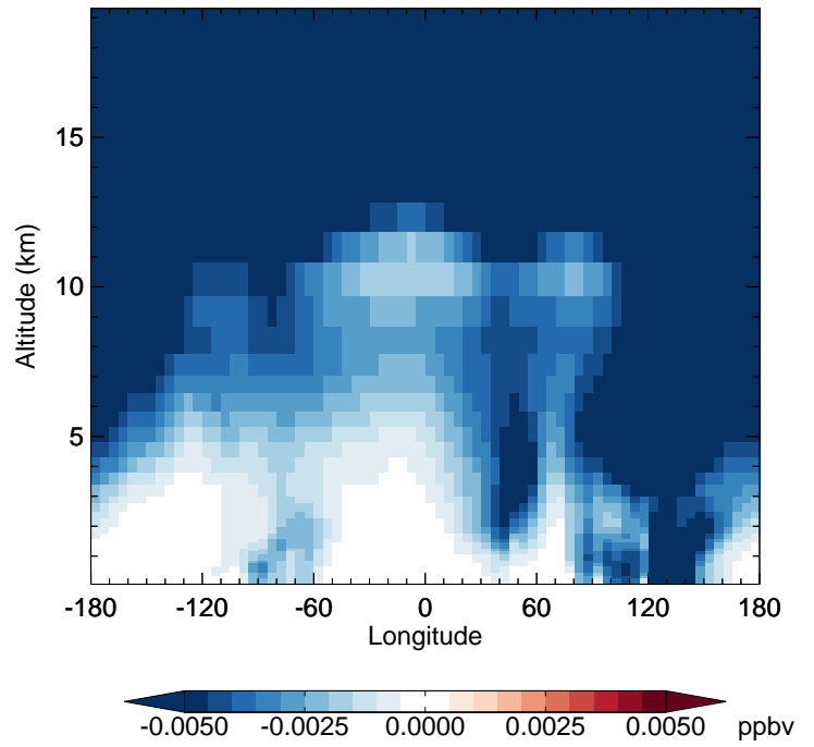
v11-02f-Run1 - v11-02e-Run1 HNO 4 - Diff along 42N for Jan
