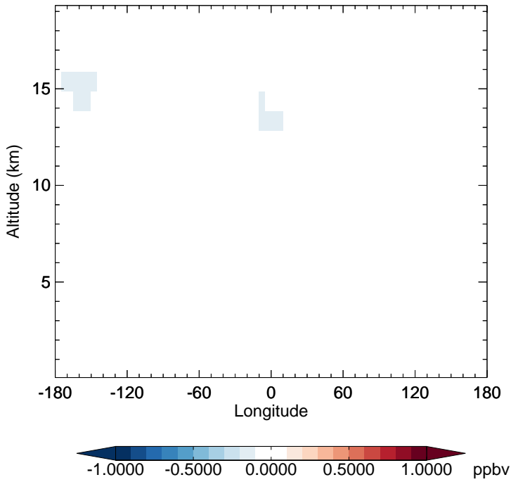
v11-02f-Run1 - v11-02e-Run0 NO - Diff along 15S for Jan
