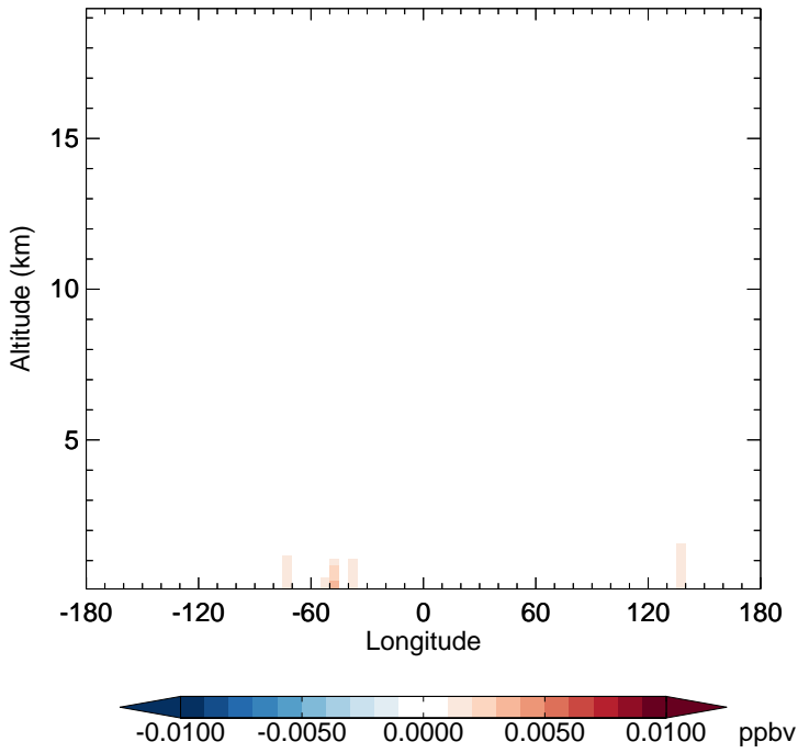
v11-02f-Run1 - v11-02e-Run1 MVKN - Diff along 15S for Jan
