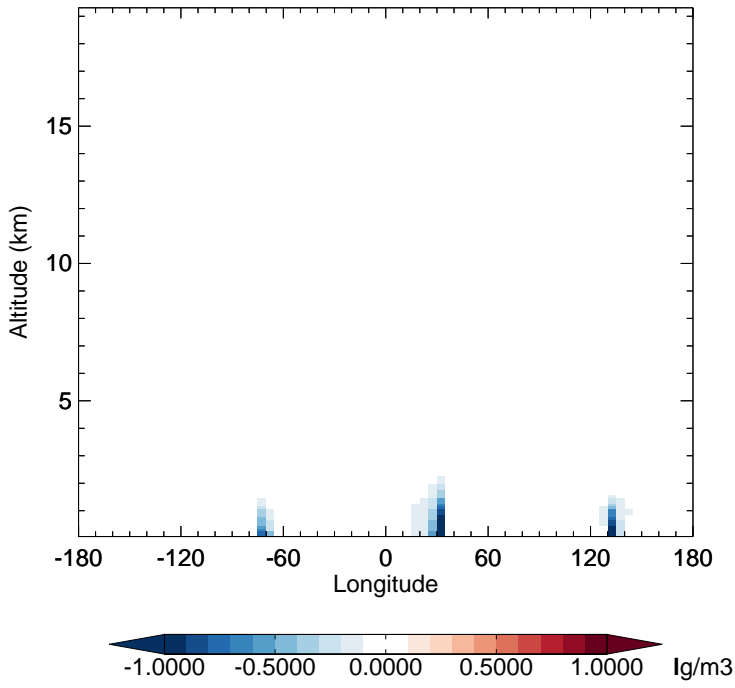
v11-02f-Run1 - v11-02e-Run1 SO 2 - Diff along 15S for Jan
