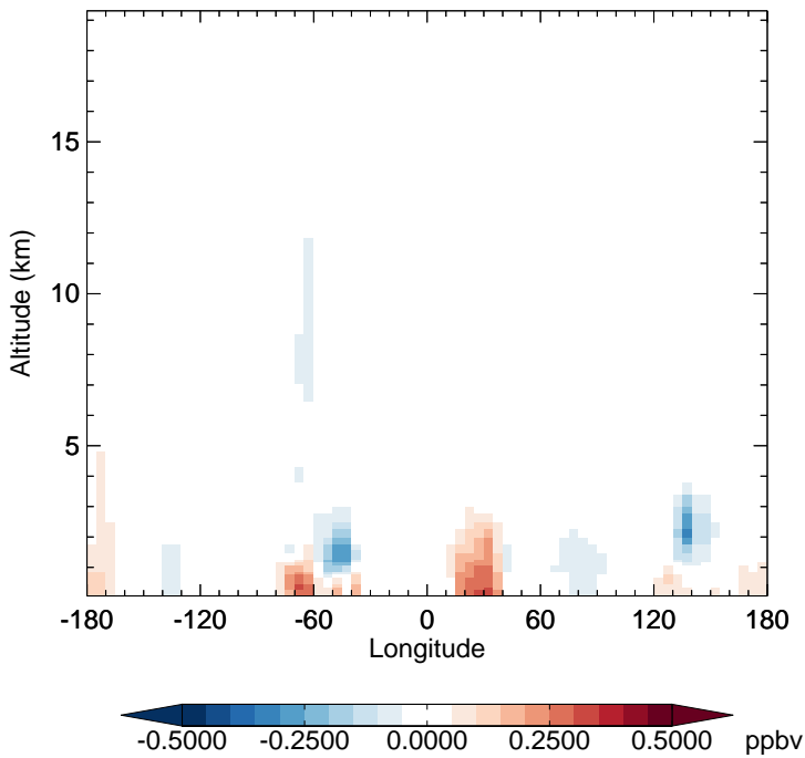
v11-02f-Run1 - v11-02e-Run0 CH 2 O - Diff along 15S for Jan
