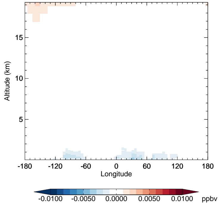
v11-02f-Run1 - v11-02e-Run0 NO3 - Diff along 42N for Jan
