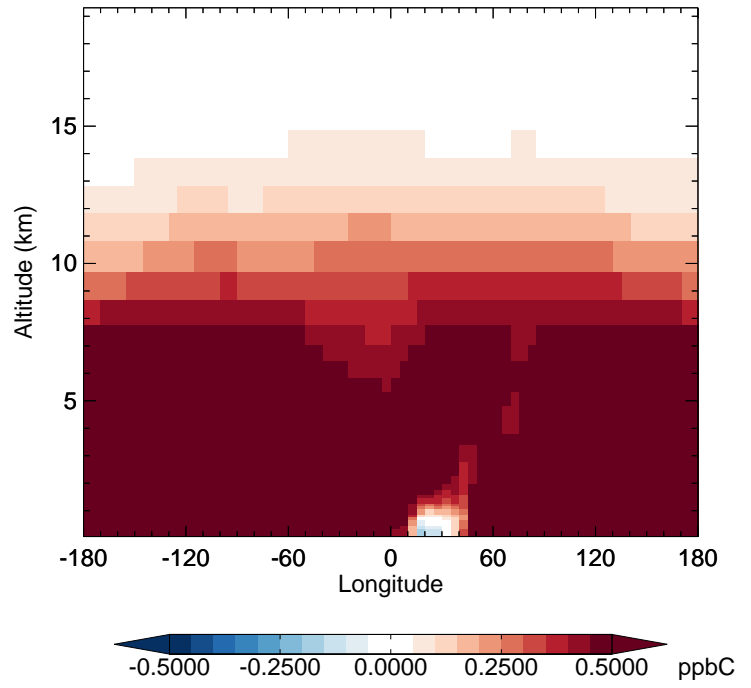
v11-02f-Run1 - v11-02e-Run1 C2H6 - Diff along 42N for Jan
