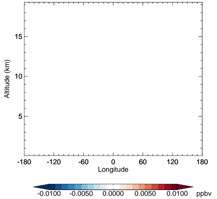
v11-02f-Run1 - v11-02e-Run1 MVKN - Diff along 42N for Jan
