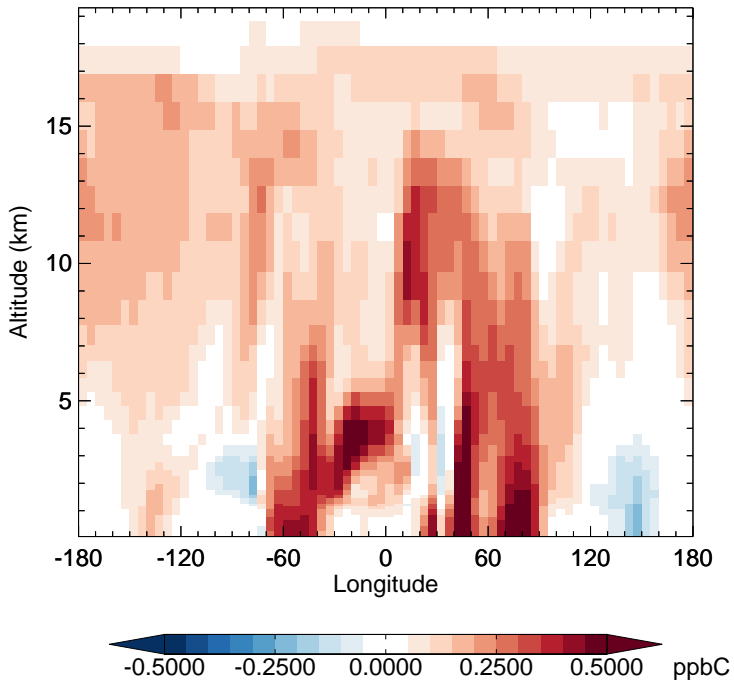
v11-02f-Run1 - v11-02e-Run0 C2H6 - Diff along 15S for Jan
