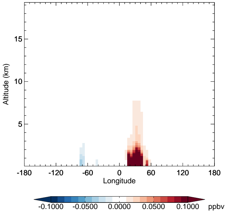
v11-02f-Run1 - v11-02e-Run1 TOLU - Diff along 15S for Jan
