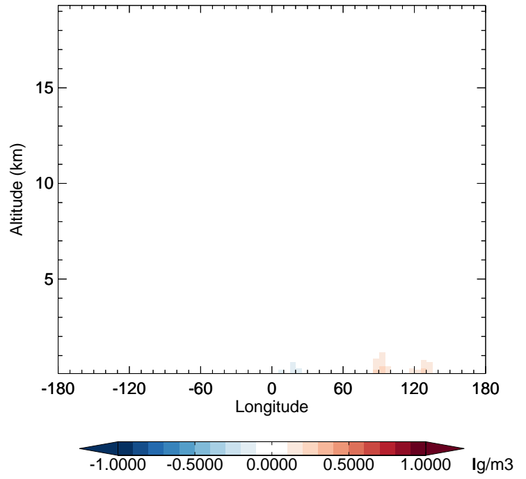
v11-02f-Run1 - v11-02e-Run1 BCPI - Diff along 42N for Jan
