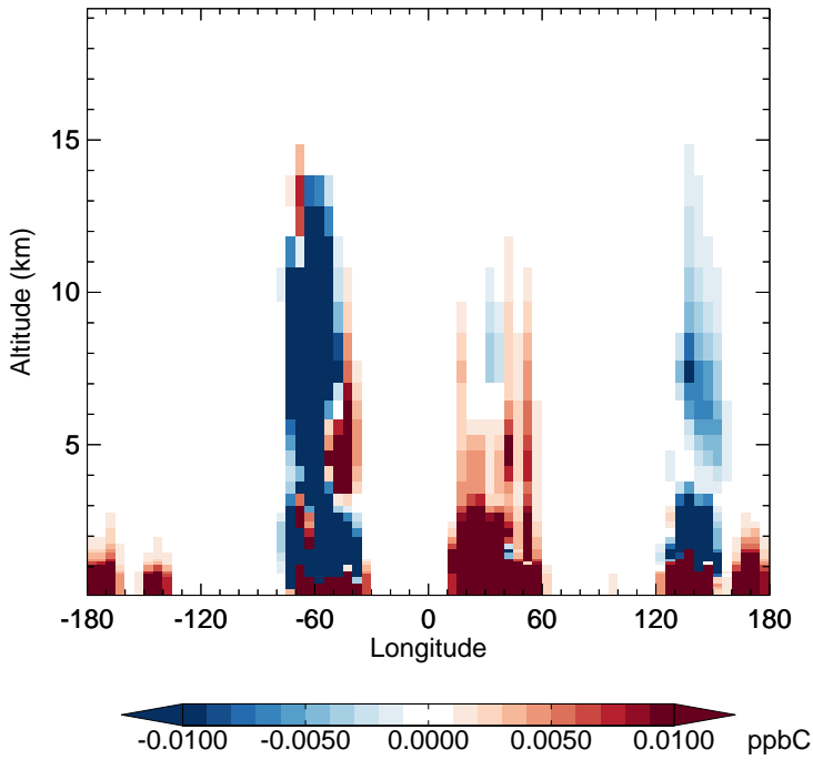
v11-02f-Run1 - v11-02e-Run0 PRPE - Diff along 15S for Jan
