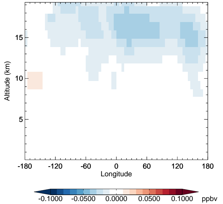
v11-02f-Run1 - v11-02e-Run0 MPN - Diff along 42N for Jan
