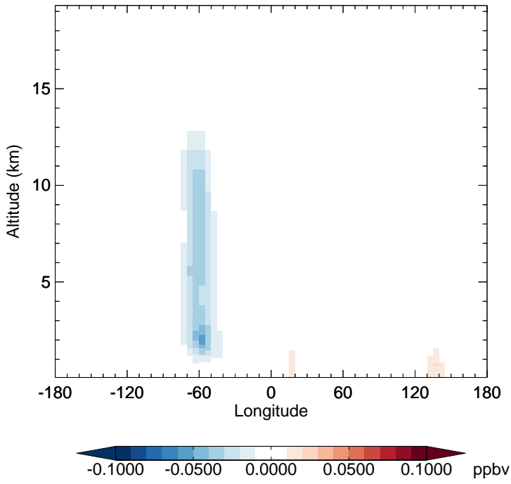
v11-02f-Run1 - v11-02e-Run1 HC187 - Diff along 15S for Jan
