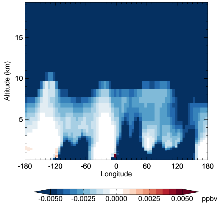
v11-02f-Run1 - v11-02e-Run0 N2O5 - Diff along 42N for Jan
