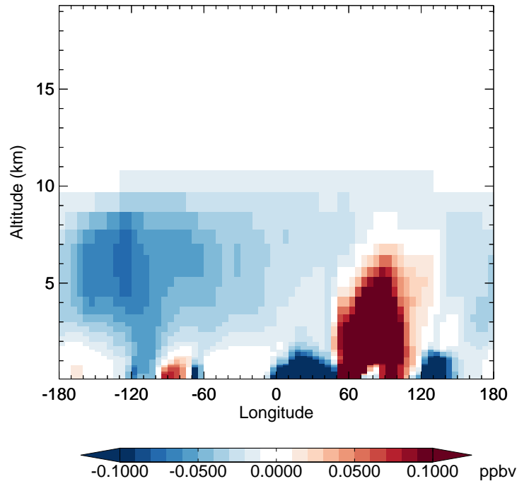
v11-02f-Run1 - v11-02e-Run1 BENZ - Diff along 42N for Jan
