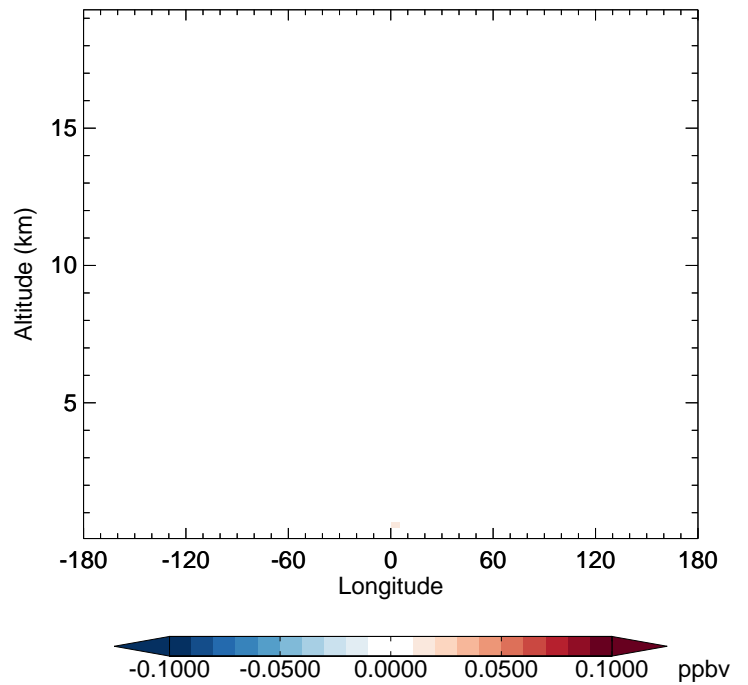
v11-02f-Run1 - v11-02e-Run0 TSOG3 - Diff along 42N for Jan
