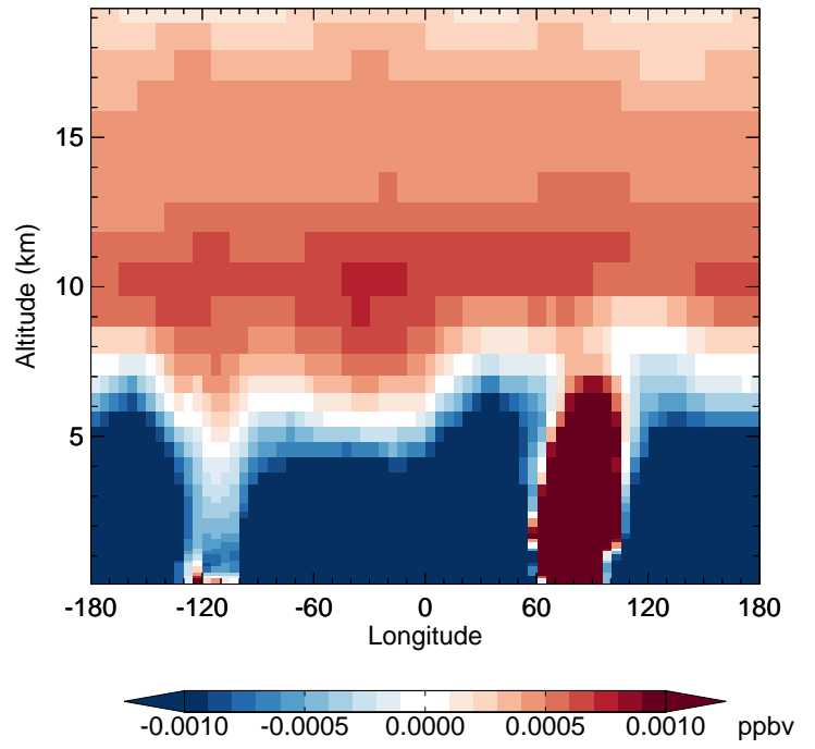
v11-02f-Run1 - v11-02e-Run1 PPN - Diff along 42N for Jan
