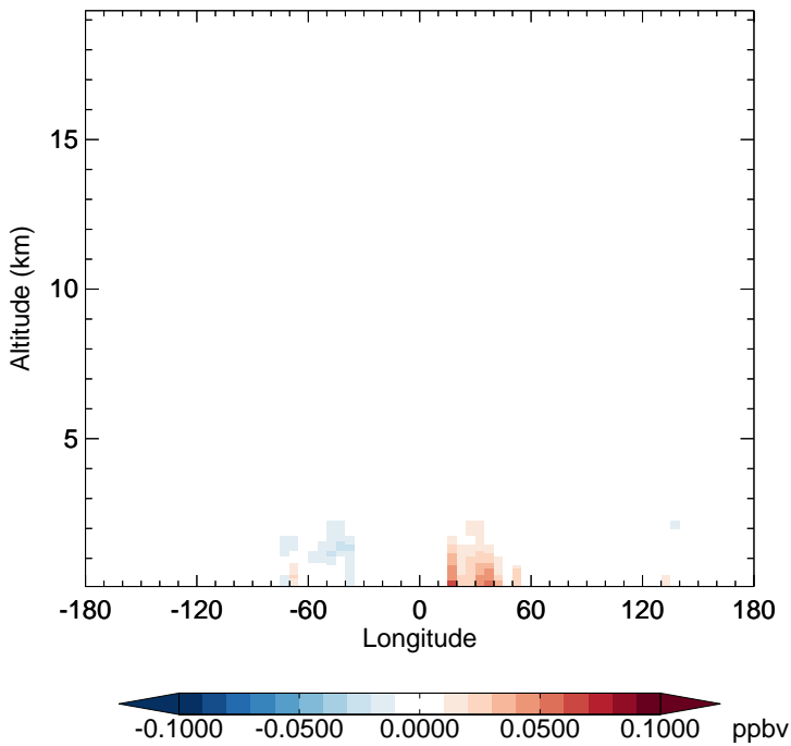
v11-02f-Run1 - v11-02e-Run0 SOAP - Diff along 15S for Jan
