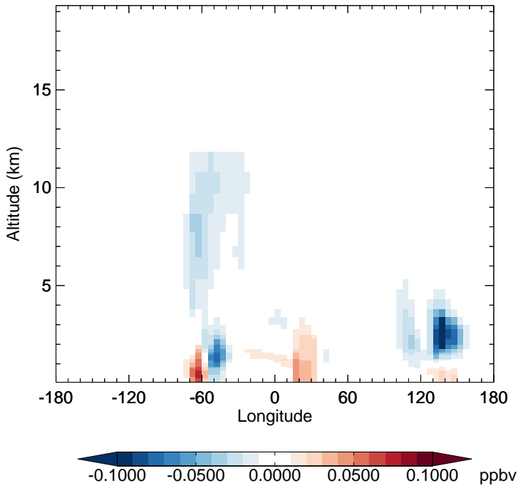
v11-02f-Run1 - v11-02e-Run0 ISO3 - Diff along 15S for Jan
