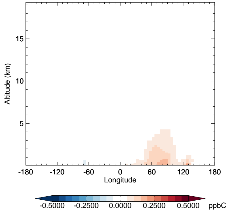
v11-02f-Run1 - v11-02e-Run1 ALD2 - Diff along 42N for Jan
