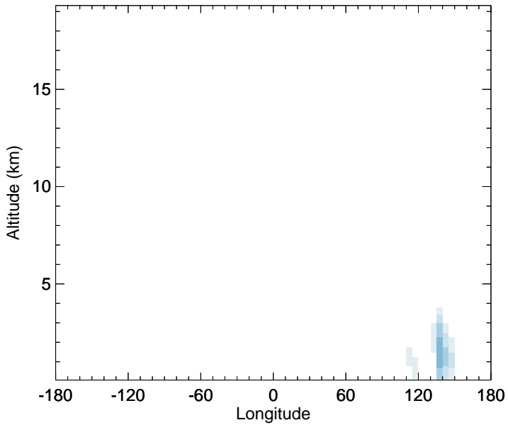
v11-02f-Run1 - v11-02e-Run0 DST2 - Diff along 15S for Jan
