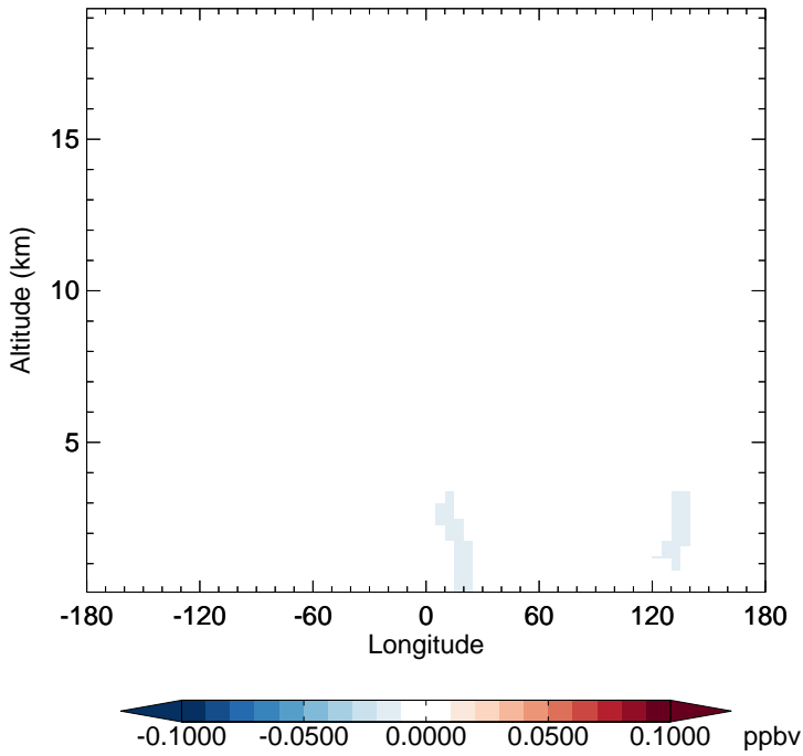
v11-02f-Run1 - v11-02e-Run0 SOAME - Diff along 15S for Jan
