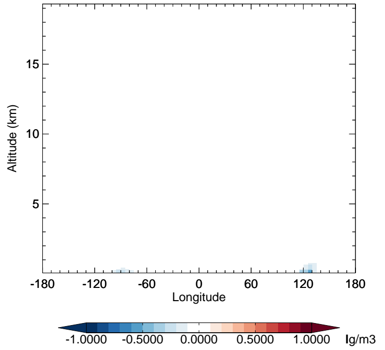
v11-02f-Run1 - v11-02e-Run1 NH3 - Diff along 42N for Jan
