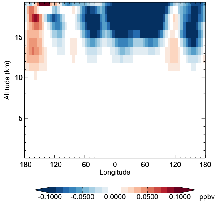
v11-02f-Run1 - v11-02e-Run0 CINO3 - Diff along 42N for Jan
