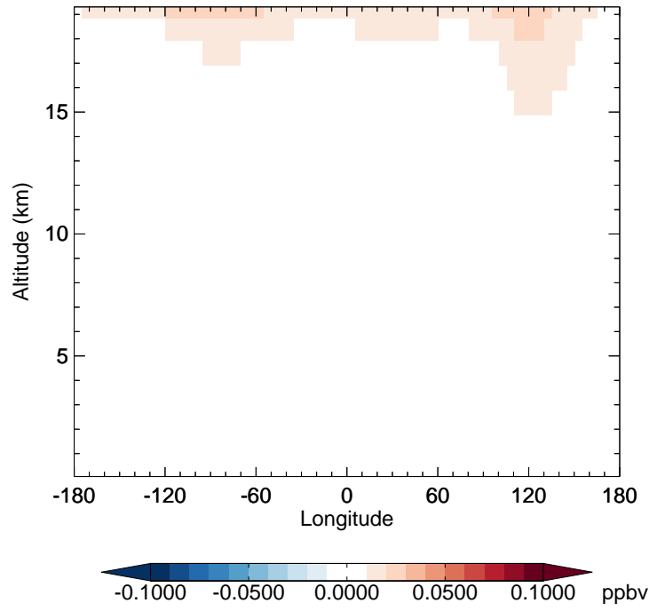
v11-02f-Run1 - v11-02e-Run1 ClO - Diff along 42N for Jan
