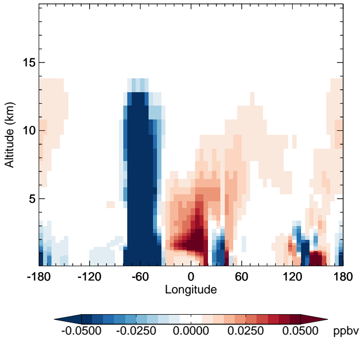
v11-02f-Run1 - v11-02e-Run1 MP - Diff along 15S for Jan
