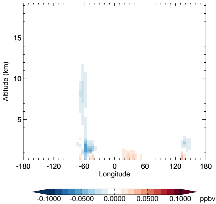
v11-02f-Run1 - v11-02e-Run0 IPMN - Diff along 15S for Jan
