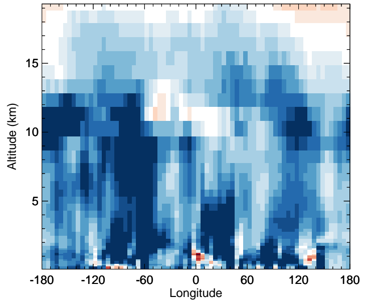
v11-02f-Run1 - v11-02e-Run0 OH - Diff along 42N for Jan
