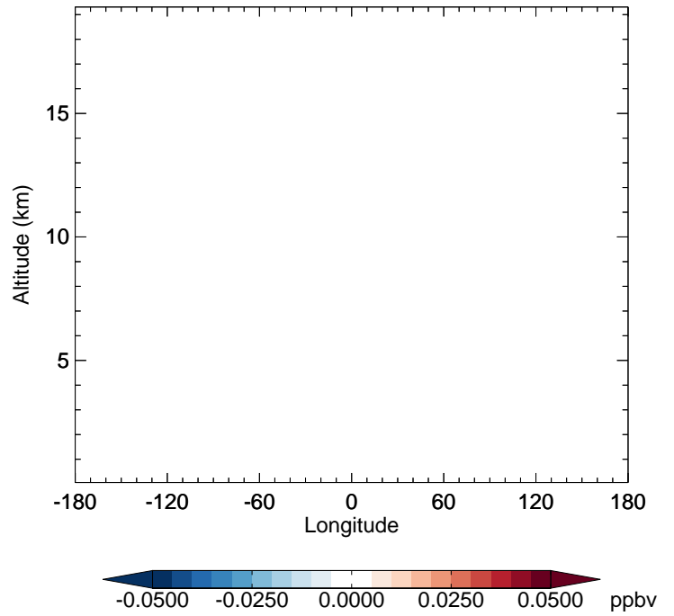
v11-02f-Run1 - v11-02e-Run0 MACR - Diff along 42N for Jan
