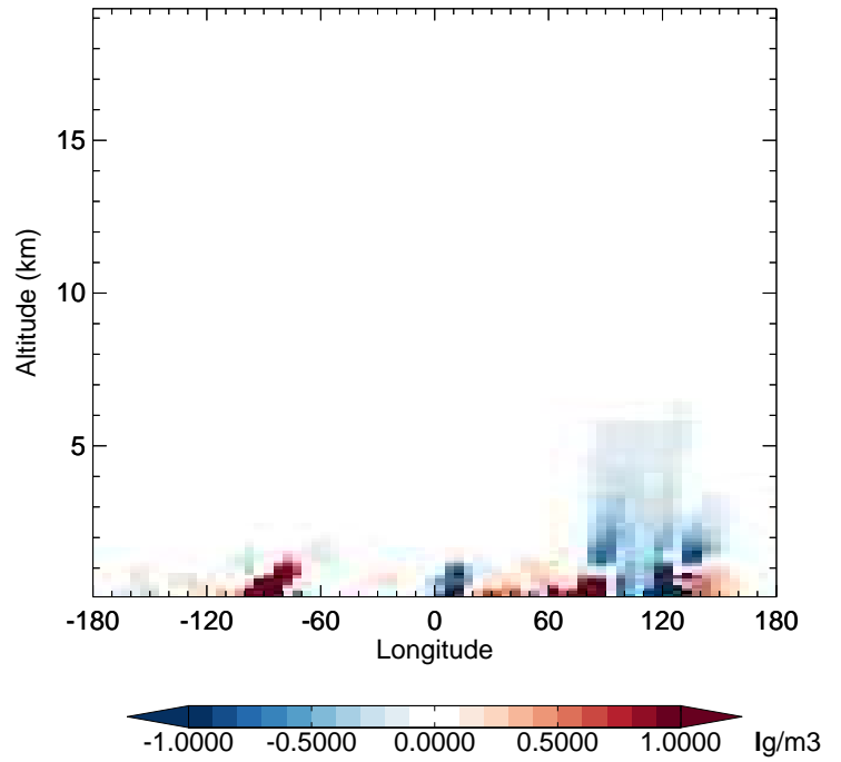
v11-02f-Run1 - v11-02e-Run0 NIT - Diff along 42N for Jan
