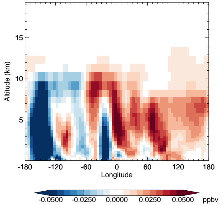
v11-02f-Run1 - v11-02e-Run0 MP - Diff along 42N for Jan
