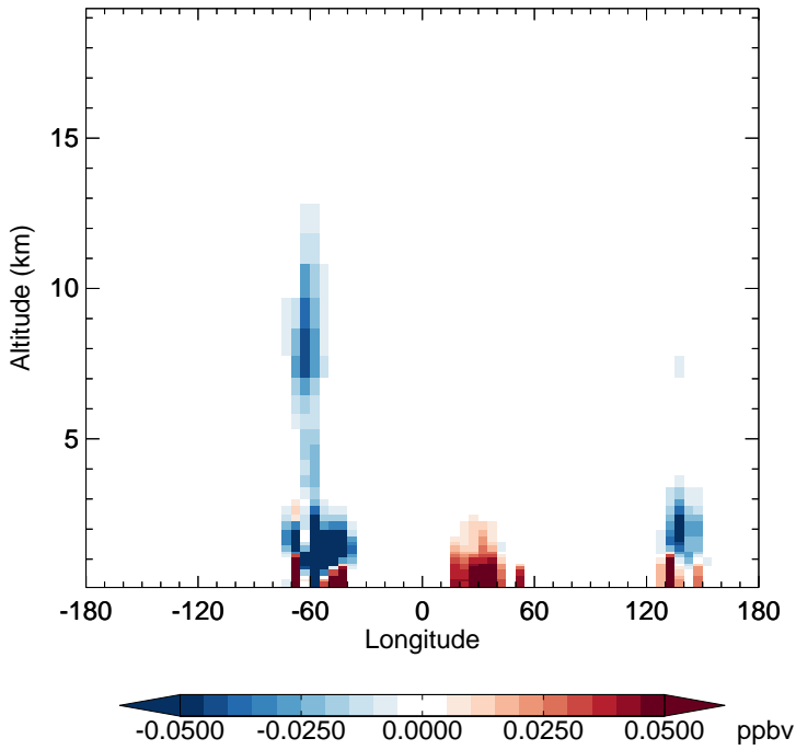
v11-02f-Run1 - v11-02e-Run0 MACR - Diff along 15S for Jan
