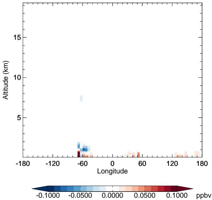
v11-02f-Run1 - v11-02e-Run0 MTPA - Diff along 15S for Jan
