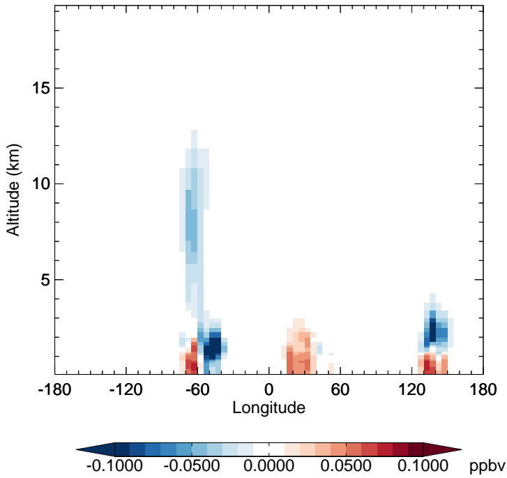
v11-02f-Run1 - v11-02e-Run0 GLYC - Diff along 15S for Jan
