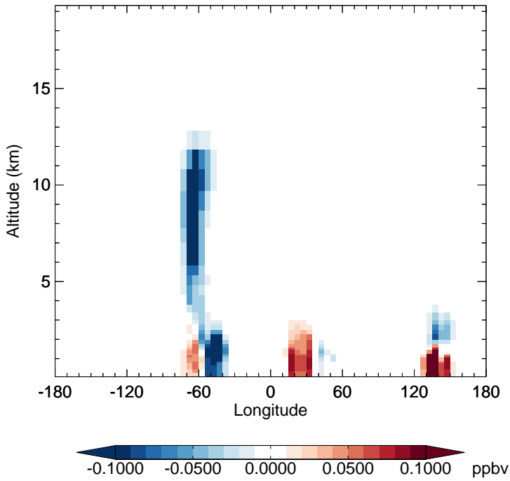
v11-02f-Run1 - v11-02e-Run0 IEPOXA - Diff along 15S for Jan
