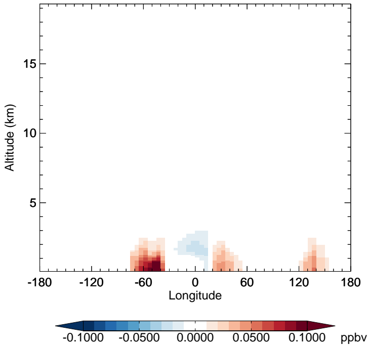
v11-02f-Run1 - v11-02e-Run1 INDIOL - Diff along 15S for Jan
