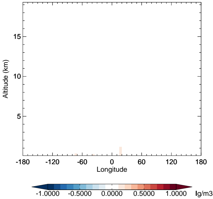
v11-02f-Run1 - v11-02e-Run1 OCPI - Diff along 15S for Jan
