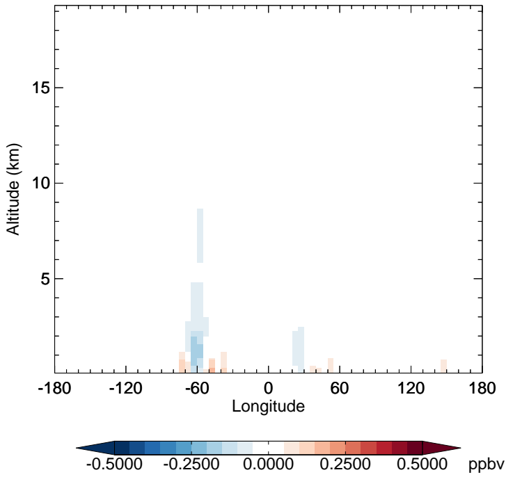
v11-02f-Run1 - v11-02e-Run1 CH 2 O - Diff along 15S for Jan
