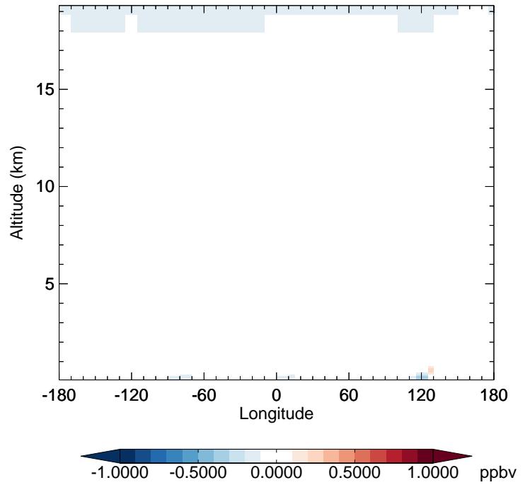
v11-02f-Run1 - v11-02e-Run0 NO - Diff along 42N for Jan
