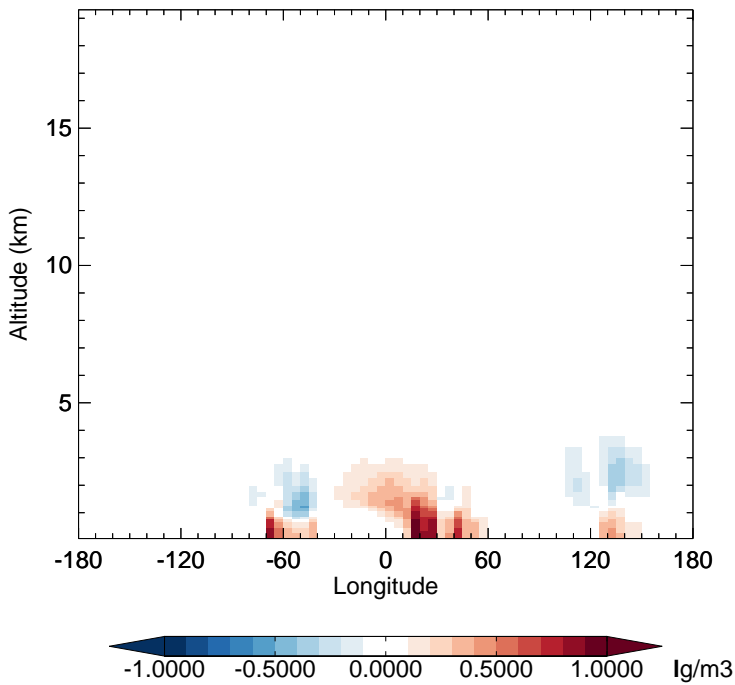
v11-02f-Run1 - v11-02e-Run0 SOAS - Diff along 15S for Jan
