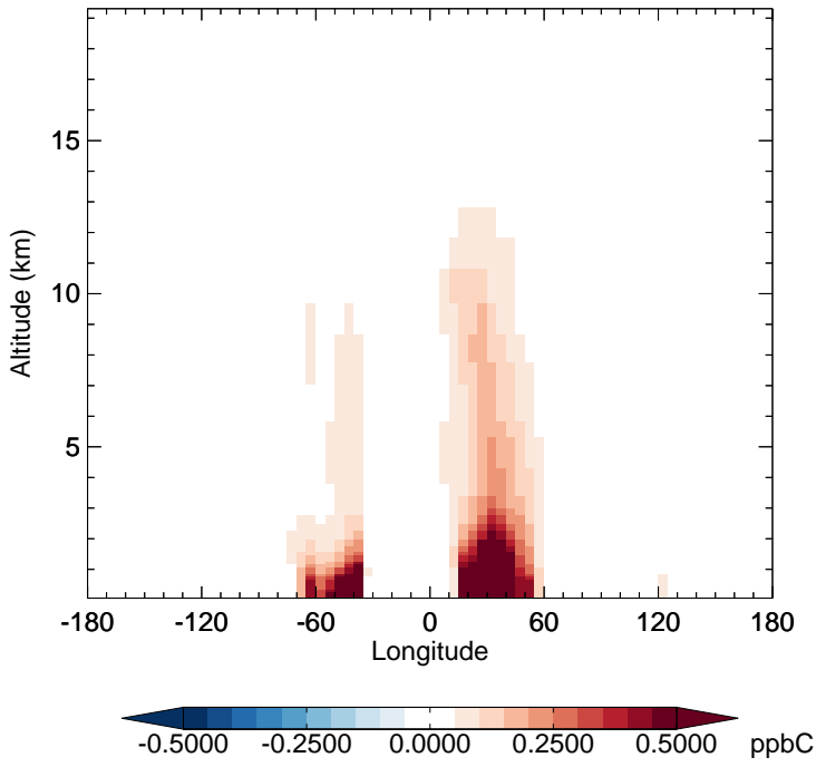
v11-02f-Run1 - v11-02e-Run1 ALK4 - Diff along 15S for Jan
