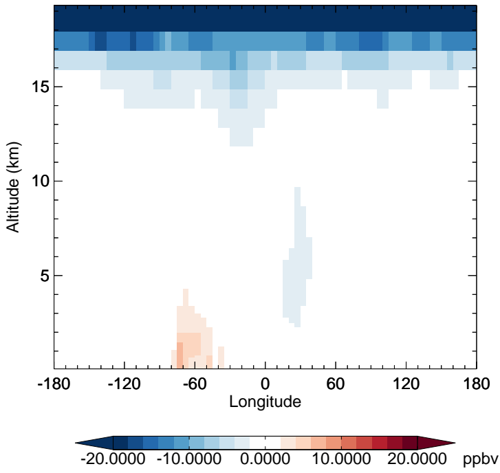
v11-02f-Run1 - v11-02e-Run1 O3 - Diff along 15S for Jan
