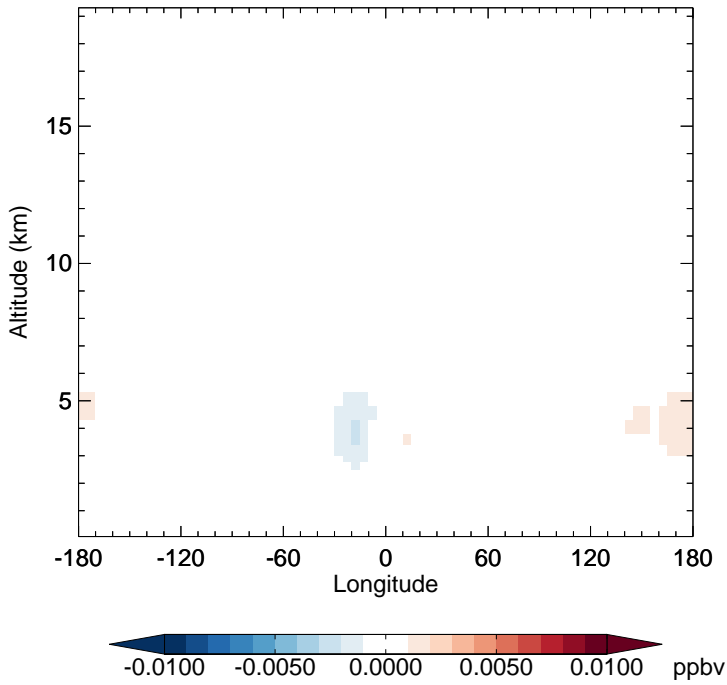
v11-02f-Run1 - v11-02e-Run0 NO3 - Diff along 15S for Jan
