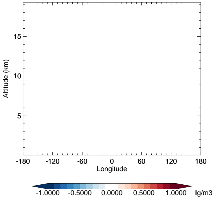
v11-02f-Run1 - v11-02e-Run0 MSA - Diff along 15S for Jan
