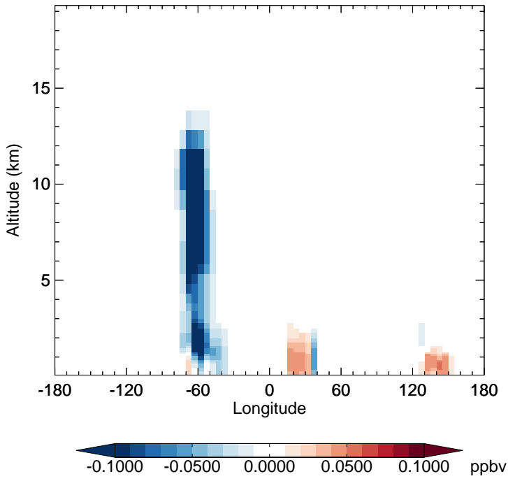
v11-02f-Run1 - v11-02e-Run1 IEPOXA - Diff along 15S for Jan
