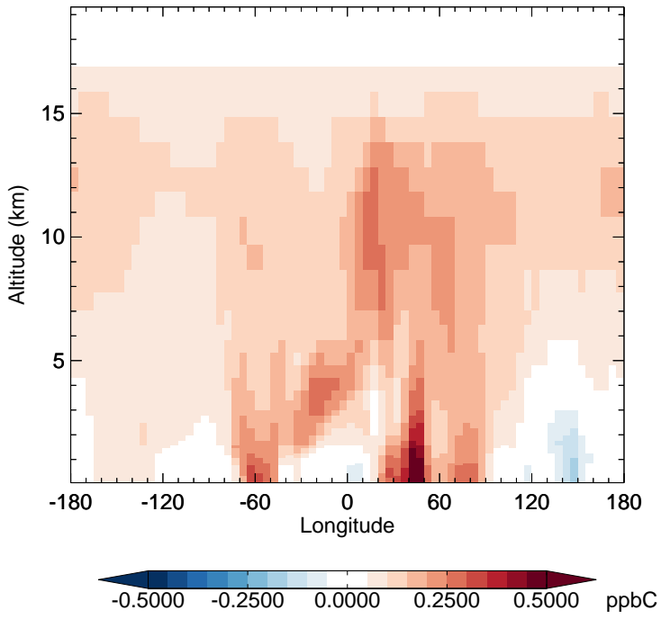
v11-02f-Run1 - v11-02e-Run1 C2H6 - Diff along 15S for Jan
