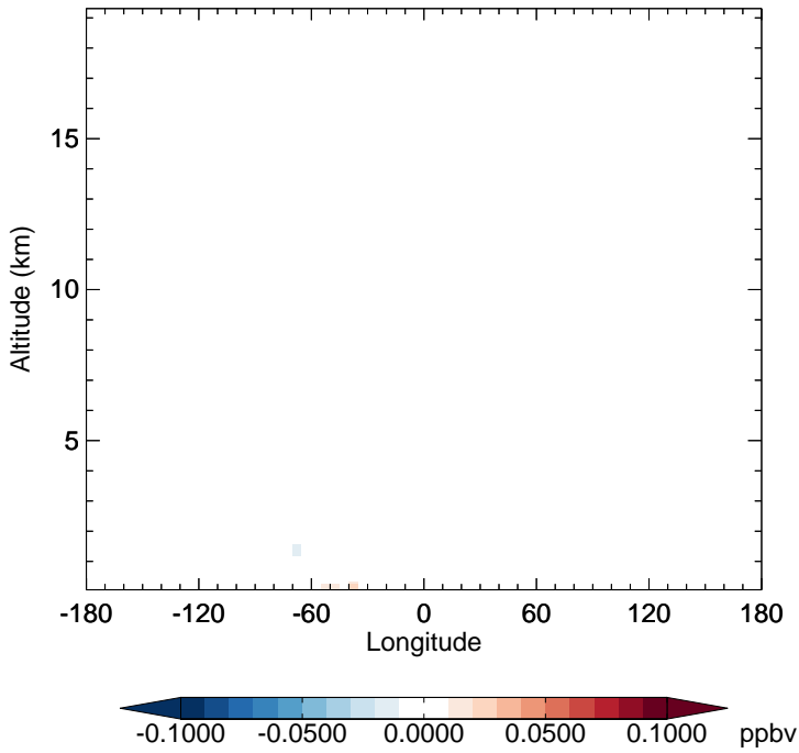
v11-02f-Run1 - v11-02e-Run0 XYLE - Diff along 15S for Jan
