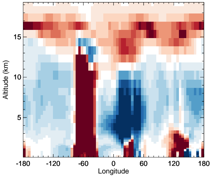
v11-02f-Run1 - v11-02e-Run1 OH - Diff along 15S for Jan
