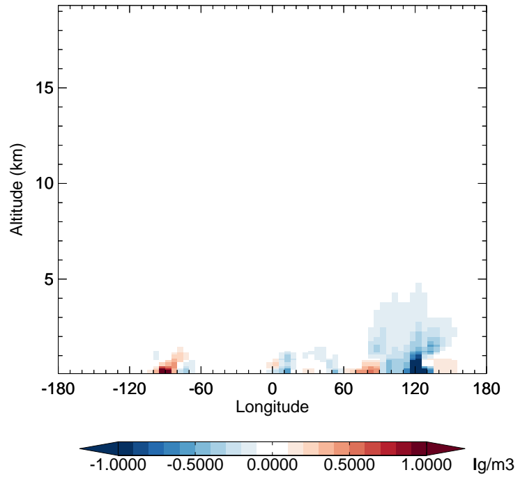
v11-02f-Run1 - v11-02e-Run0 NH4 - Diff along 42N for Jan
