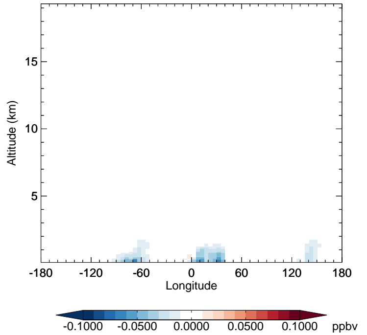
v11-02f-Run1 - v11-02e-Run0 CINO2 - Diff along 42N for Jan
