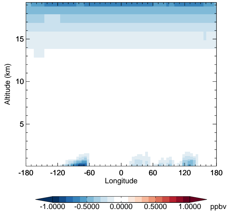
v11-02f-Run1 - v11-02e-Run1 NO2 - Diff along 42N for Jan
