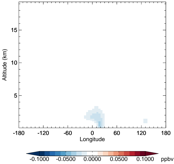
v11-02f-Run1 - v11-02e-Run1 SOAME - Diff along 15S for Jan
