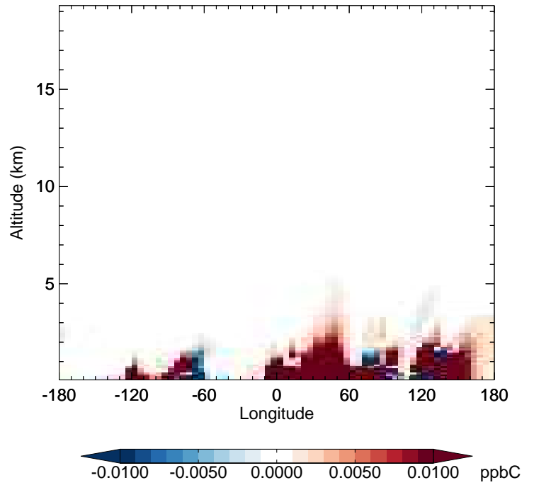
v11-02f-Run1 - v11-02e-Run0 PRPE - Diff along 42N for Jan
