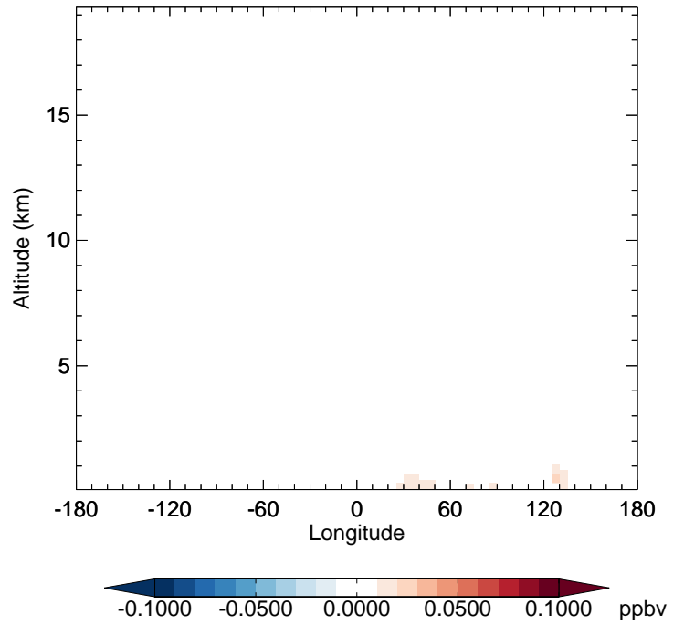
v11-02f-Run1 - v11-02e-Run0 GLYC - Diff along 42N for Jan
