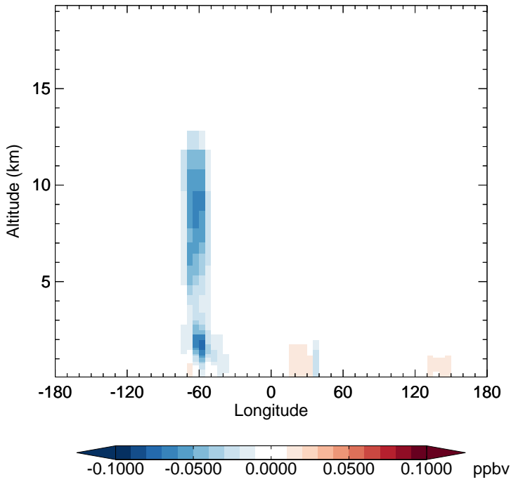
v11-02f-Run1 - v11-02e-Run1 IEPOXB - Diff along 15S for Jan
