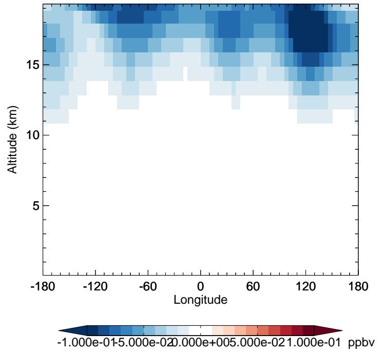
v11-02f-Run1 - v11-02e-Run1 CINO3 - Diff along 42N for Jan
