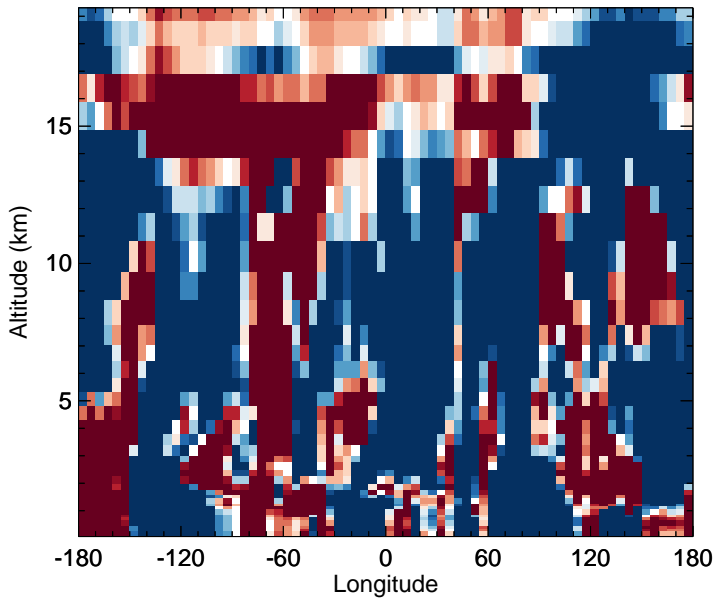
v11-02f-Run1 - v11-02e-Run0 OH - Diff along 15S for Jan
