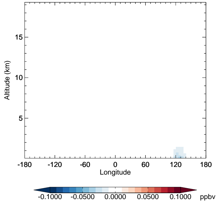
v11-02f-Run1 - v11-02e-Run0 ASOG3 - Diff along 42N for Jan
