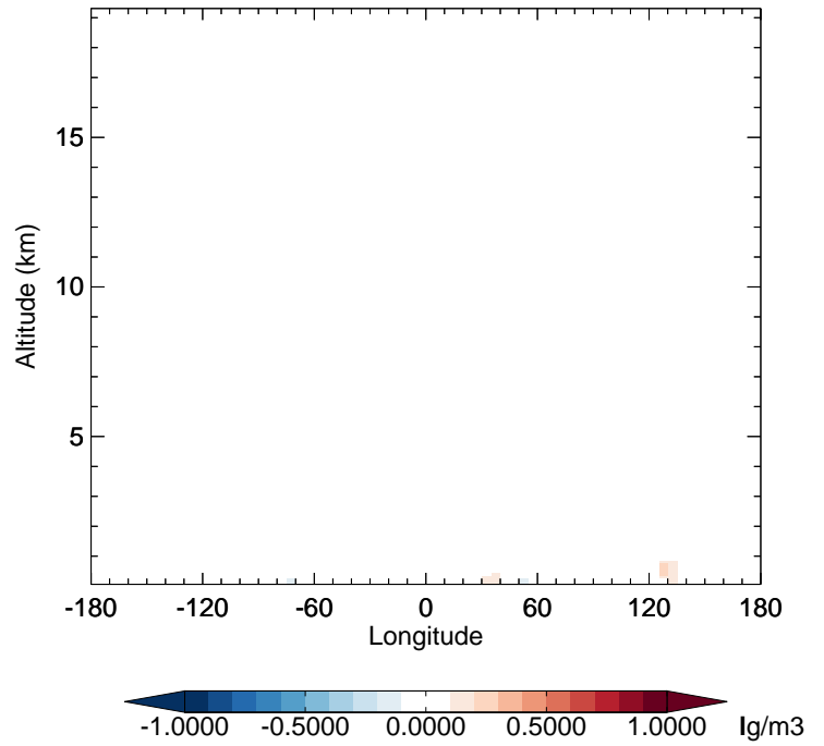
v11-02f-Run1 - v11-02e-Run0 OCPO - Diff along 42N for Jan
