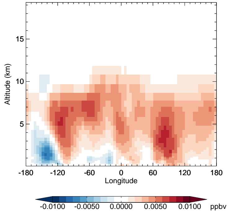
v11-02f-Run1 - v11-02e-Run0 MAP - Diff along 42N for Jan
