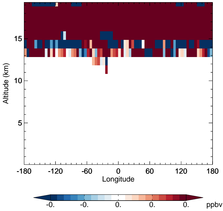
v11-02f-Run1 - v11-02e-Run1 H2O - Diff along 15S for Jan
