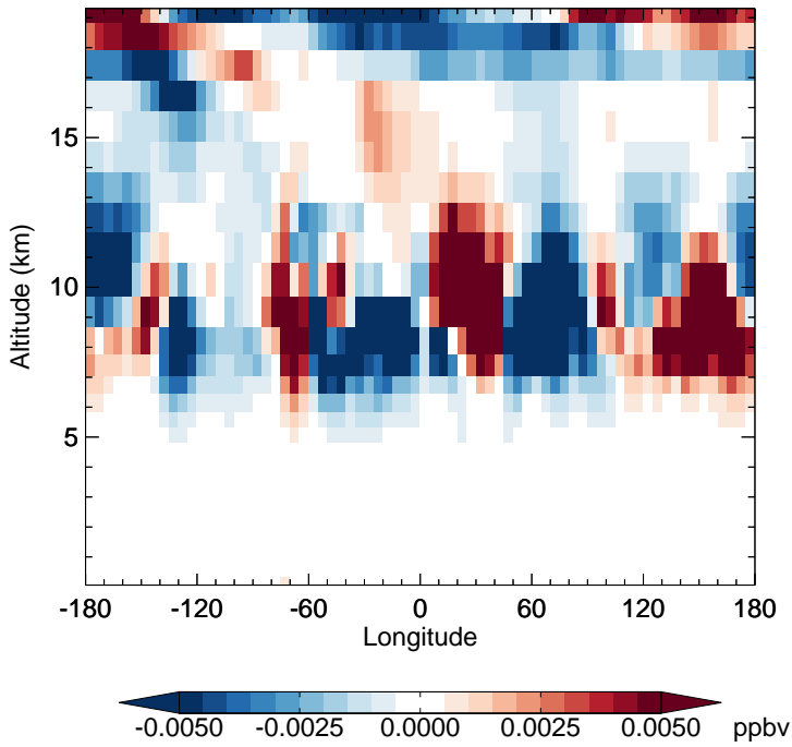
v11-02f-Run1 - v11-02e-Run0 HNO 4 - Diff along 15S for Jan
