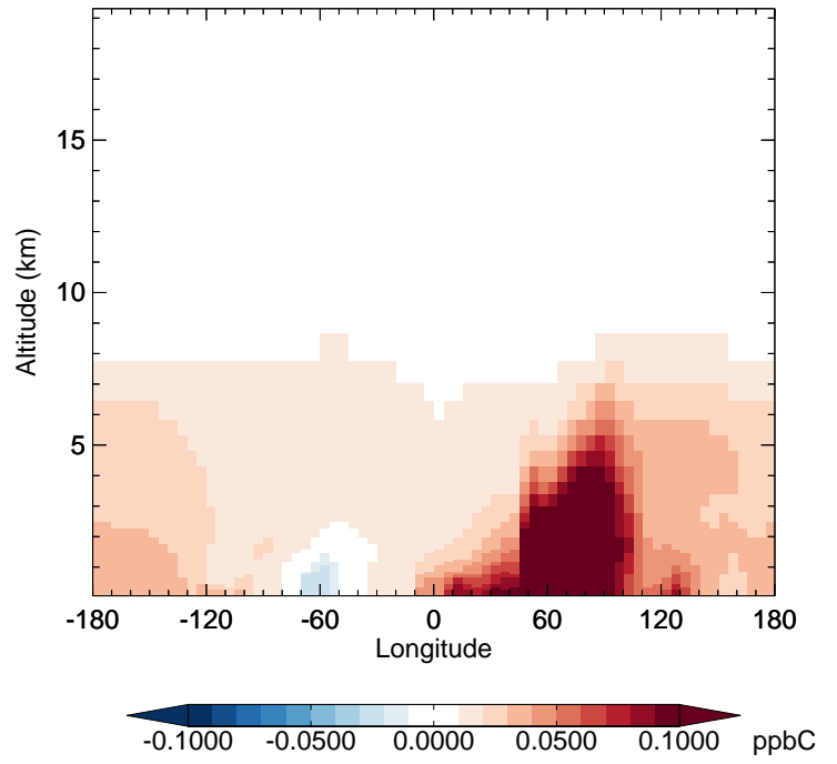
v11-02f-Run1 - v11-02e-Run1 MEK - Diff along 42N for Jan
