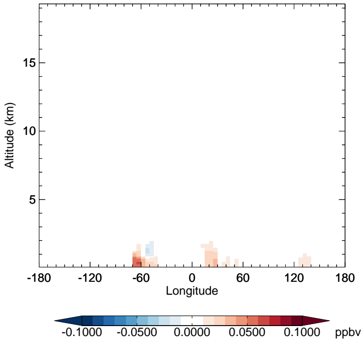
v11-02f-Run1 - v11-02e-Run0 TSOA0 - Diff along 15S for Jan
