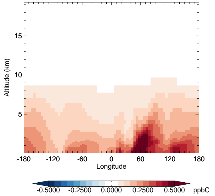
v11-02f-Run1 - v11-02e-Run1 C3H8 - Diff along 42N for Jan
