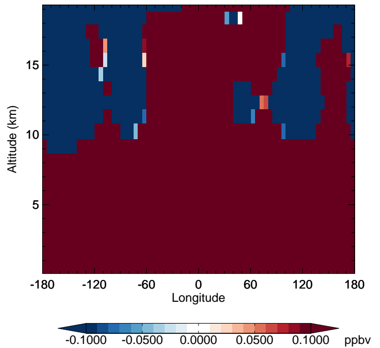
v11-02f-Run1 - v11-02e-Run0 N2O - Diff along 42N for Jan
