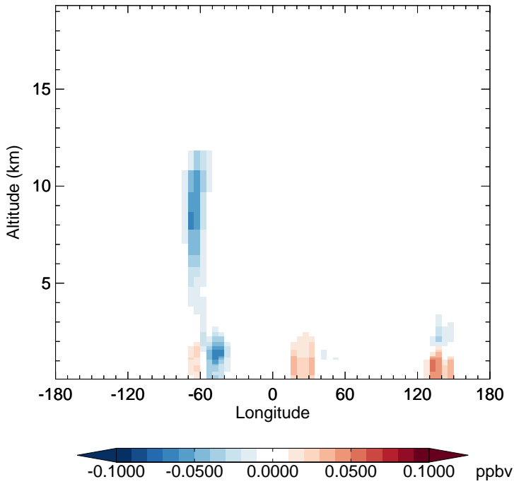
v11-02f-Run1 - v11-02e-Run0 IEPOXB - Diff along 15S for Jan
