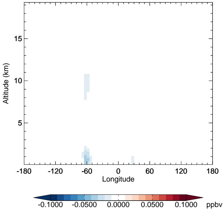
v11-02f-Run1 - v11-02e-Run1 ISOA1 - Diff along 15S for Jan
