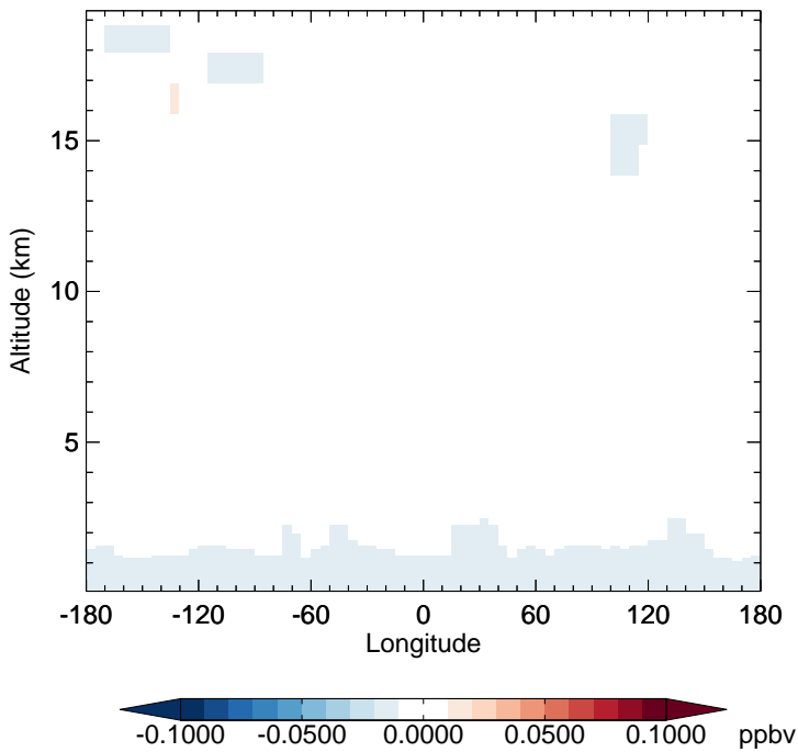
v11-02f-Run1 - v11-02e-Run0 CFC11 - Diff along 15S for Jan
