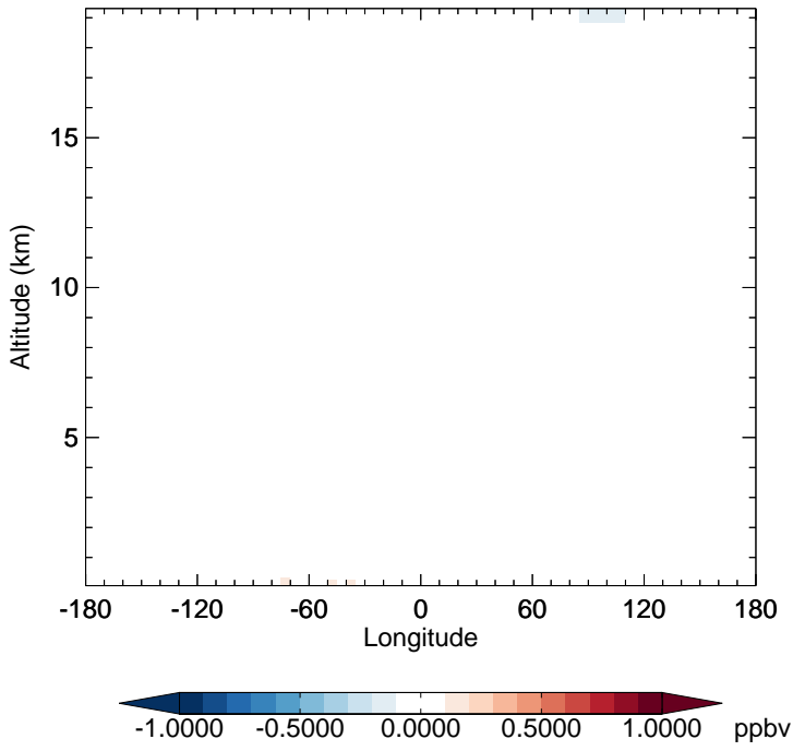
v11-02f-Run1 - v11-02e-Run1 NO2 - Diff along 15S for Jan
