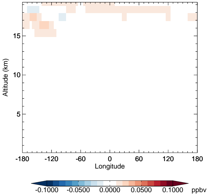
v11-02f-Run1 - v11-02e-Run0 OCS - Diff along 15S for Jan
