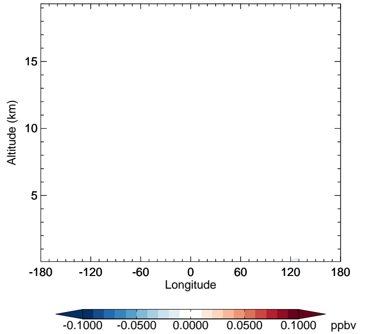
v11-02f-Run1 - v11-02e-Run0 ASOA1 - Diff along 42N for Jan
