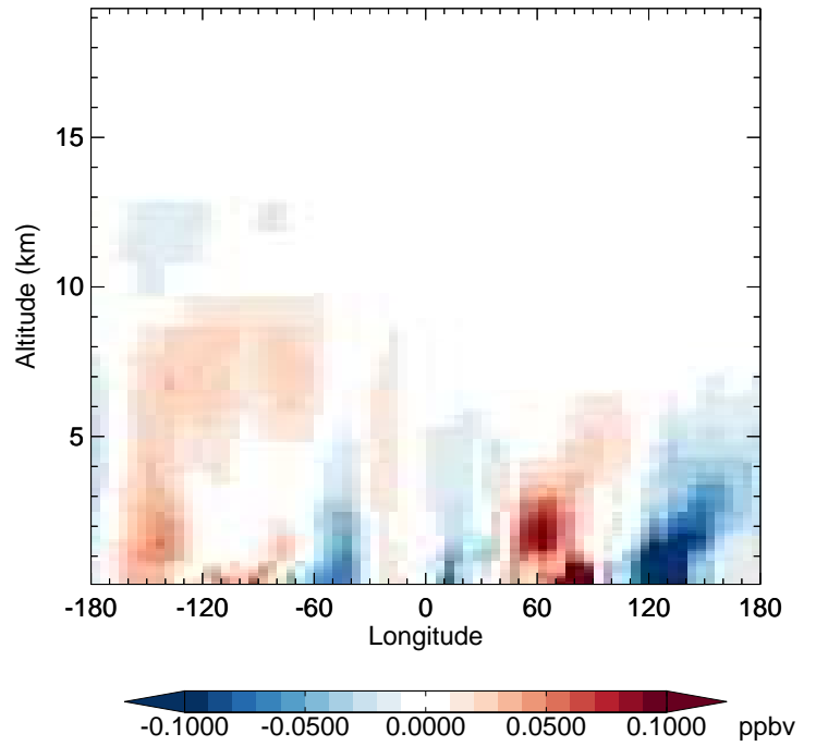
v11-02f-Run1 - v11-02e-Run0 PAN - Diff along 42N for Jan
