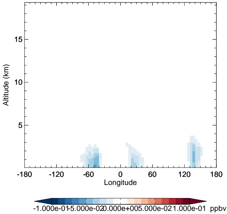
v11-02f-Run1 - v11-02e-Run0 IONITA - Diff along 15S for Jan
