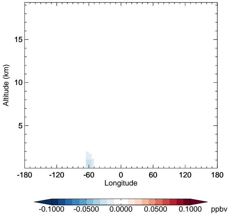
v11-02f-Run1 - v11-02e-Run1 TSOA0 - Diff along 15S for Jan
