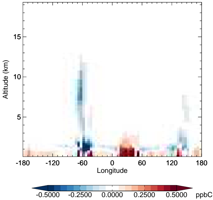
v11-02f-Run1 - v11-02e-Run0 ALD2 - Diff along 15S for Jan
