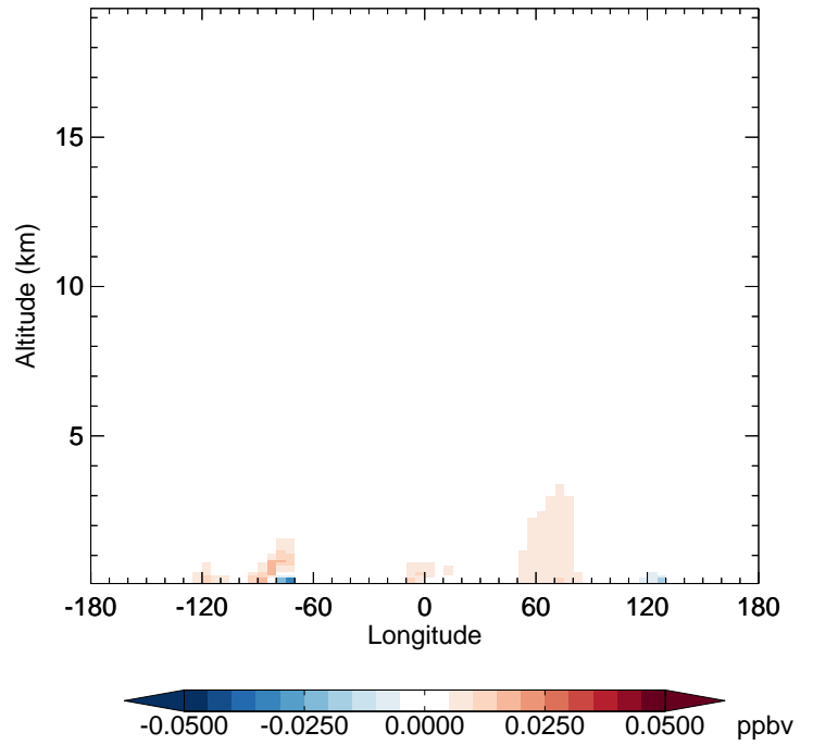
v11-02f-Run1 - v11-02e-Run0 RCHO - Diff along 42N for Jan
