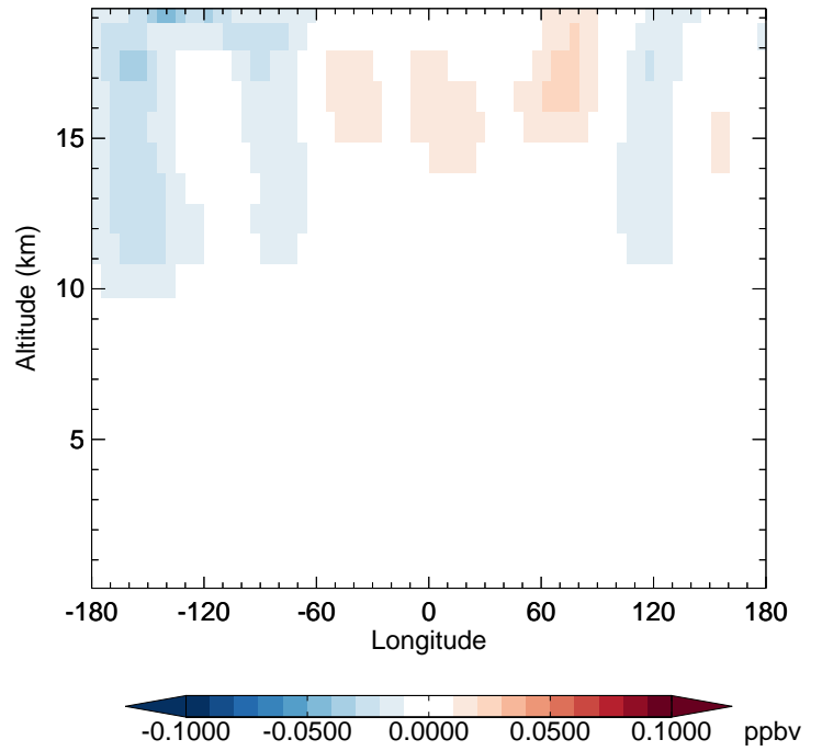
v11-02f-Run1 - v11-02e-Run0 CH3Cl - Diff along 42N for Jan
