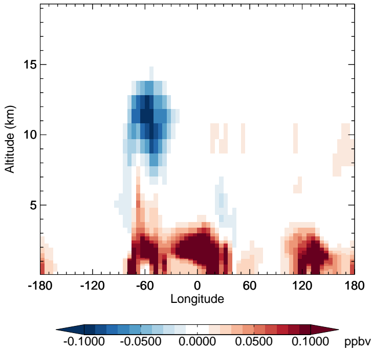
v11-02f-Run1 - v11-02e-Run1 H2O2 - Diff along 15S for Jan
