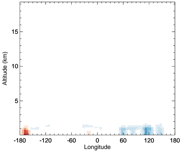
v11-02f-Run1 - v11-02e-Run0 SALA - Diff along 15S for Jan
