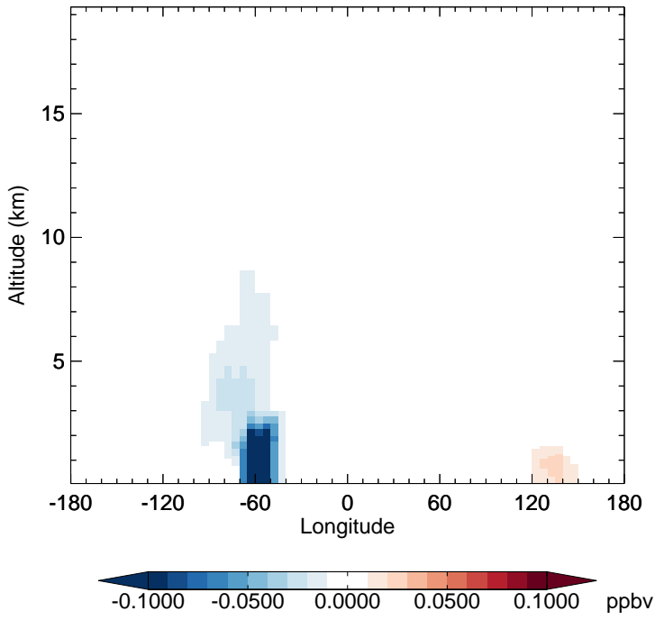
v11-02f-Run1 - v11-02e-Run1 ISO3 - Diff along 15S for Jul
