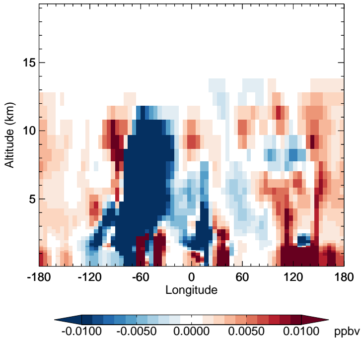
v11-02f-Run1 - v11-02e-Run0 MAP - Diff along 15S for Jul
