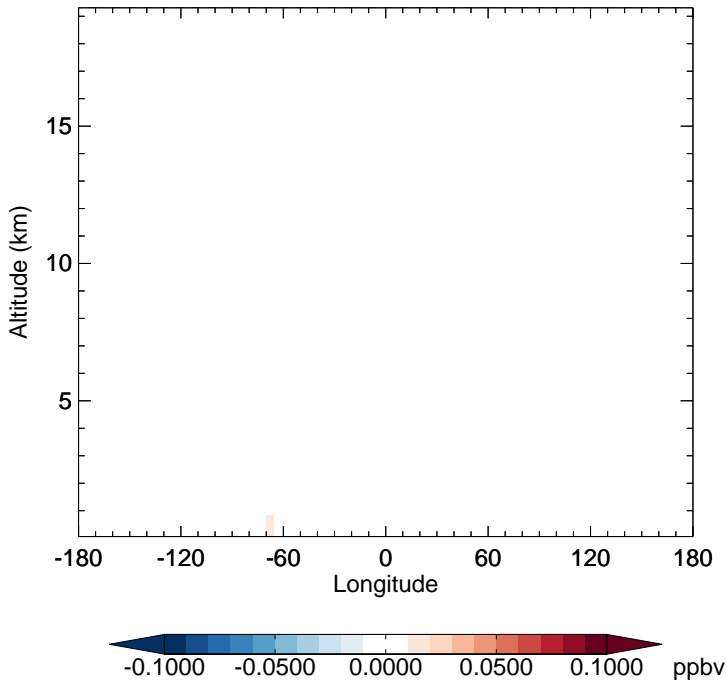
v11-02f-Run1 - v11-02e-Run1 TSOA0 - Diff along 15S for Jul
