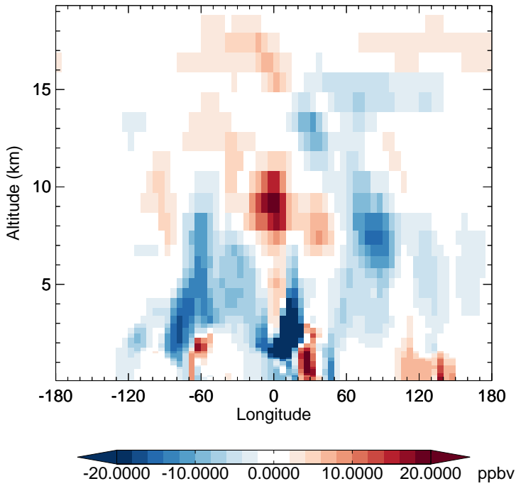
v11-02f-Run1 - v11-02e-Run0 CO - Diff along 15S for Jul
