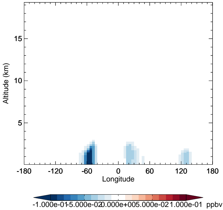
v11-02f-Run1 - v11-02e-Run0 IONITA - Diff along 15S for Jul
