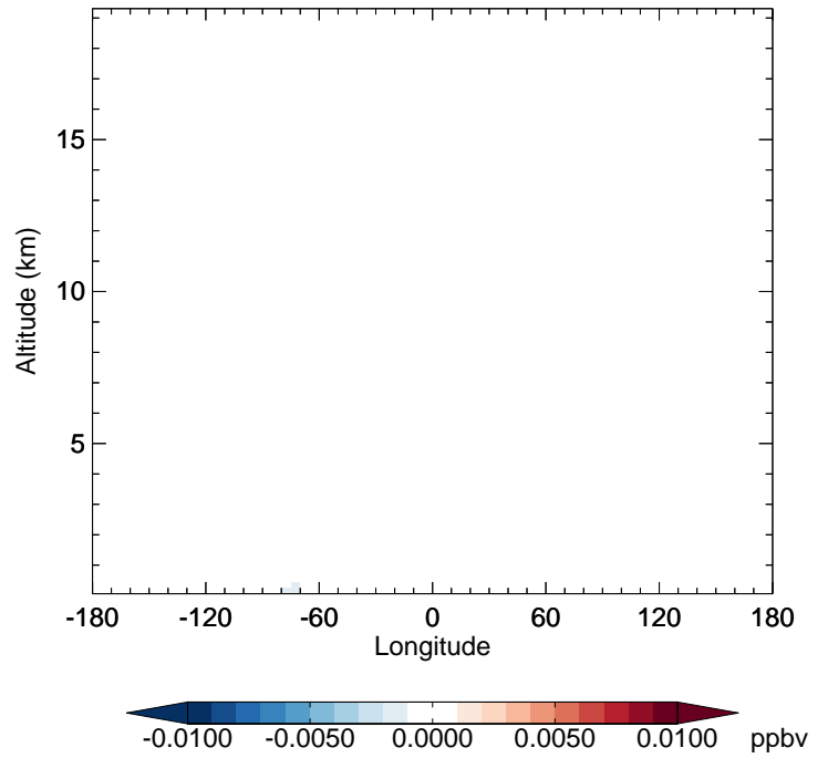
v11-02f-Run1 - v11-02e-Run0 MACRN - Diff along 42N for Jul
