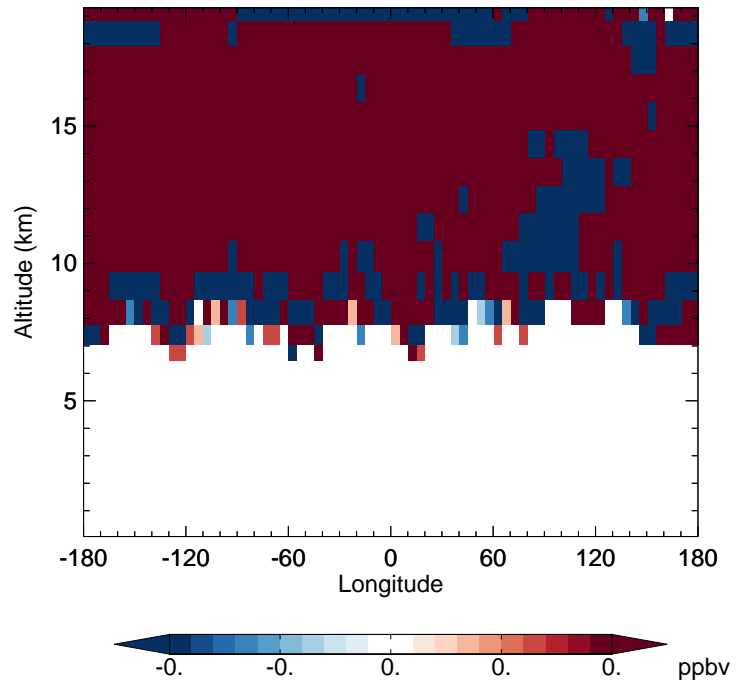
v11-02f-Run1 - v11-02e-Run1 H2O - Diff along 42N for Jul
