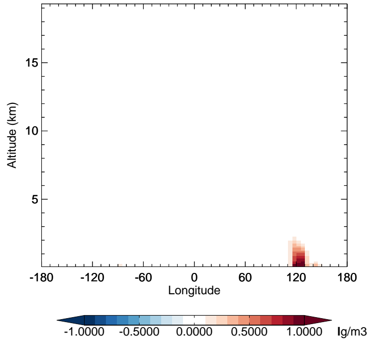
v11-02f-Run1 - v11-02e-Run1 NIT - Diff along 42N for Jul
