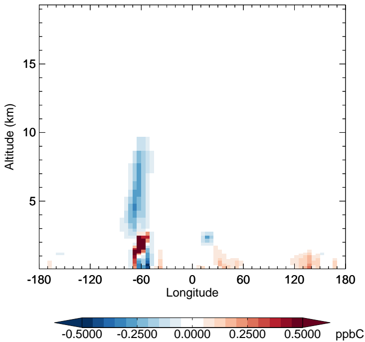
v11-02f-Run1 - v11-02e-Run0 ALD2 - Diff along 15S for Jul
