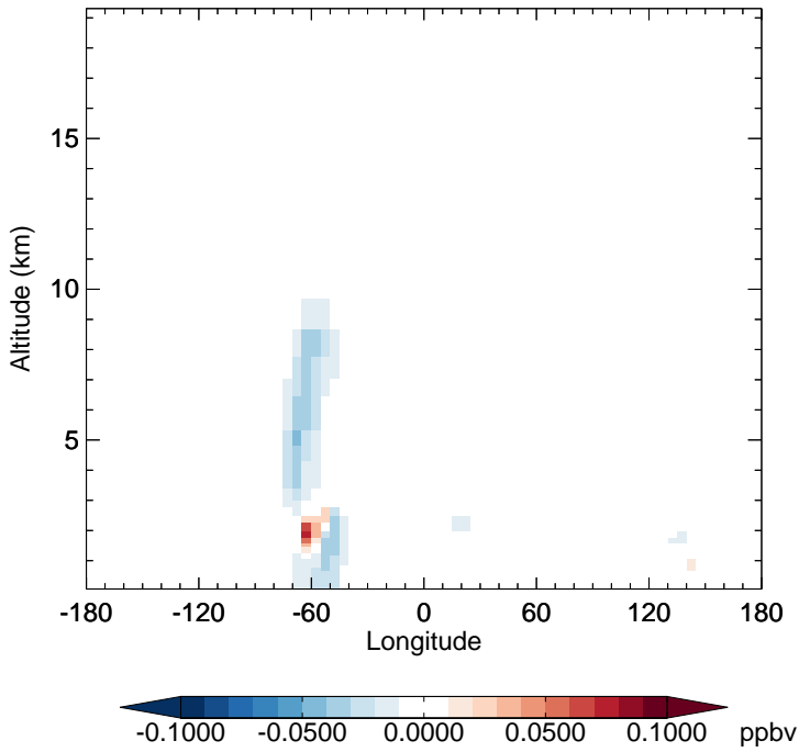
v11-02f-Run1 - v11-02e-Run0 IEPOXB - Diff along 15S for Jul
