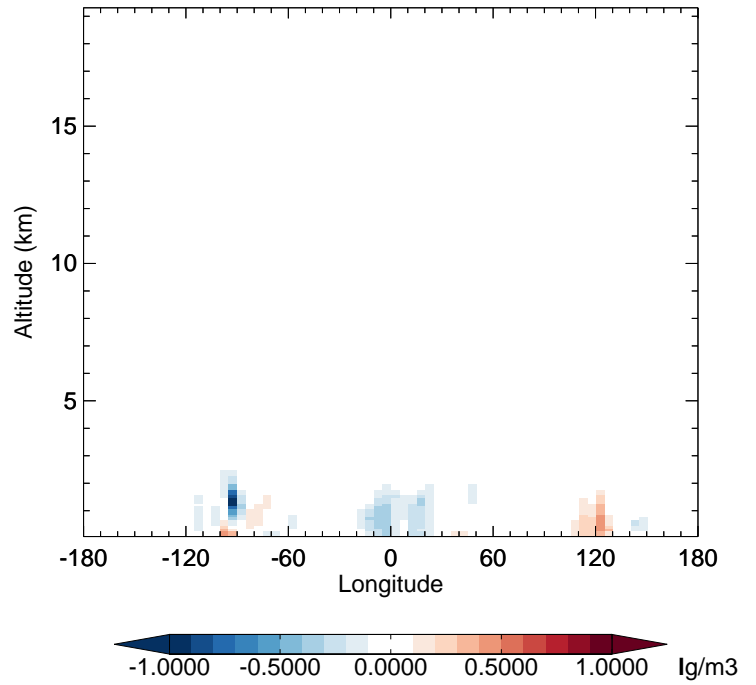
v11-02f-Run1 - v11-02e-Run0 NH3 - Diff along 42N for Jul
