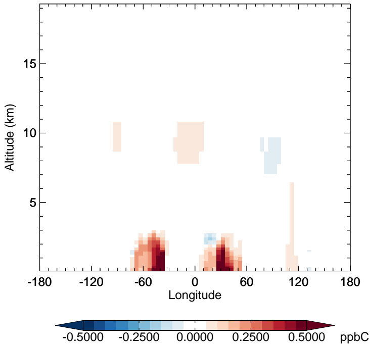
v11-02f-Run1 - v11-02e-Run0 ALK4 - Diff along 15S for Jul
