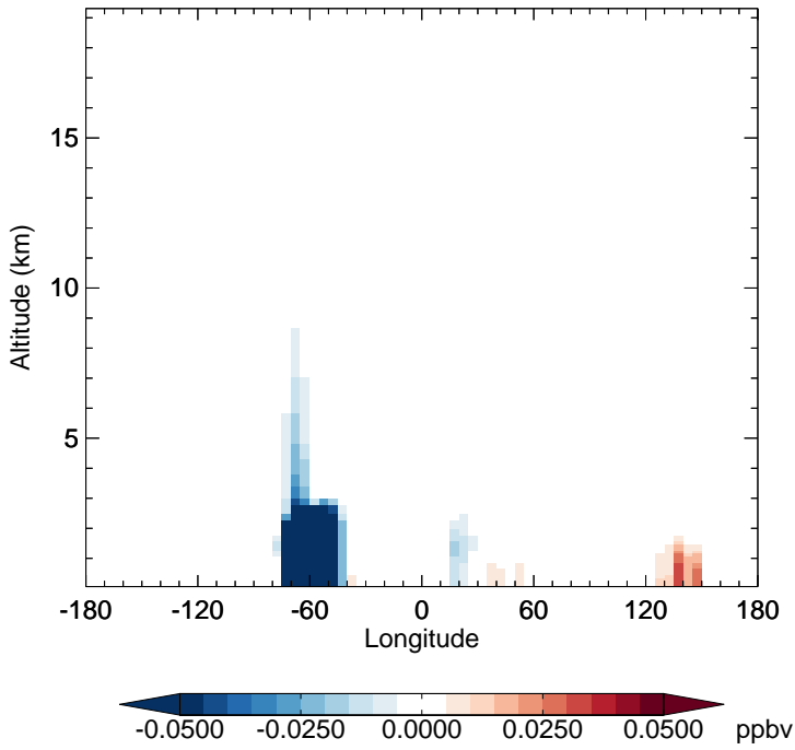
v11-02f-Run1 - v11-02e-Run1 MACR - Diff along 15S for Jul
