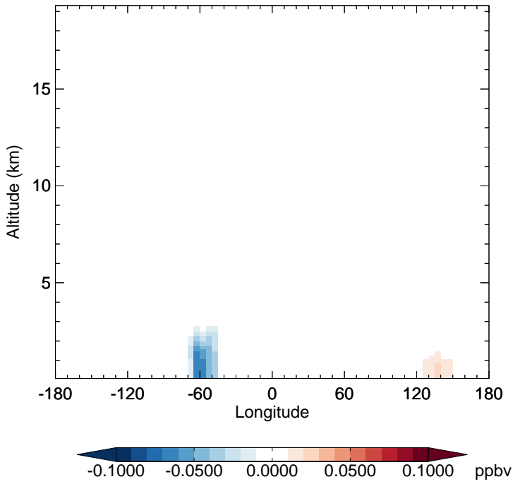
v11-02f-Run1 - v11-02e-Run1 MGLY - Diff along 15S for Jul
