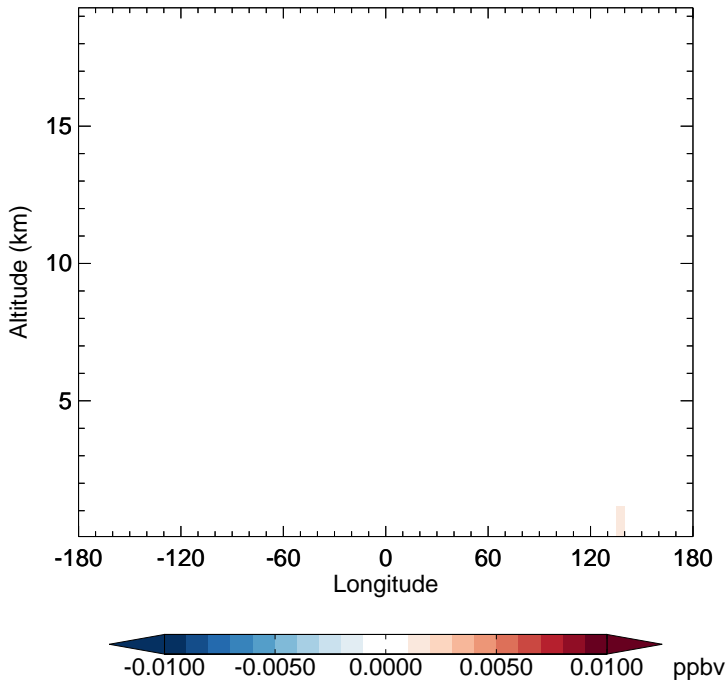
v11-02f-Run1 - v11-02e-Run0 MACRN - Diff along 15S for Jul
