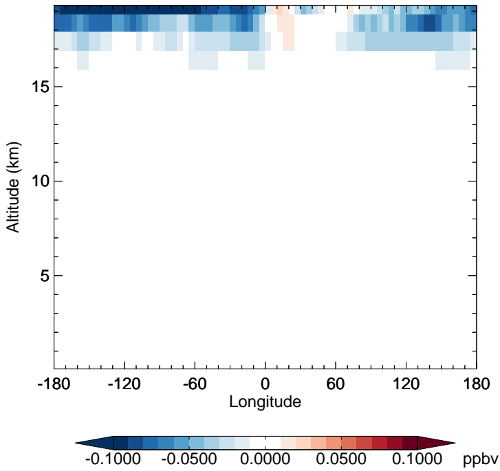
v11-02f-Run1 - v11-02e-Run0 ClNO 3 - Diff along 15S for Jul
