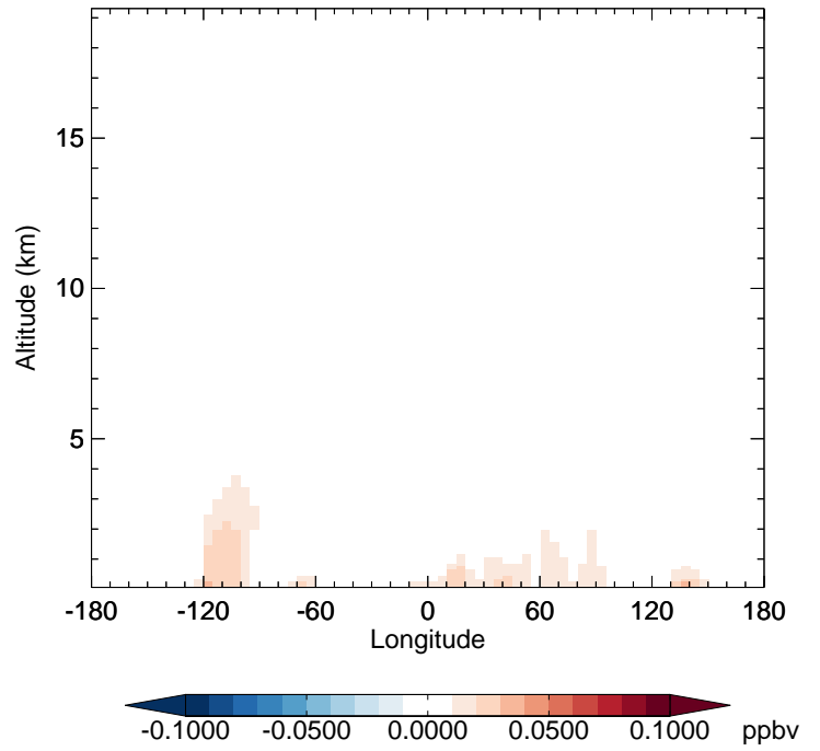
v11-02f-Run1 - v11-02e-Run1 TSOG2 - Diff along 42N for Jul
