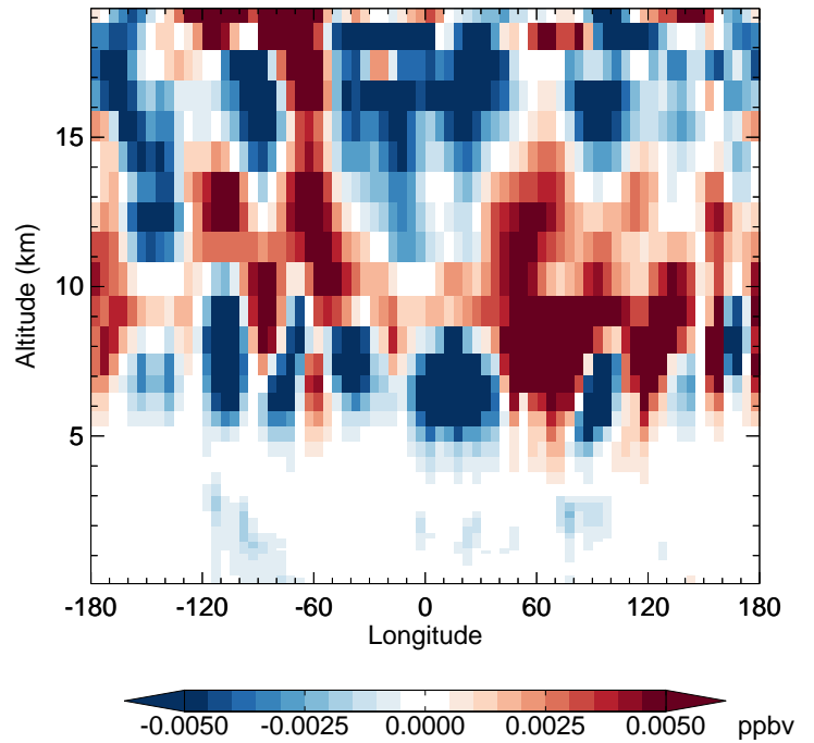
v11-02f-Run1 - v11-02e-Run0 HNO 4 - Diff along 42N for Jul
