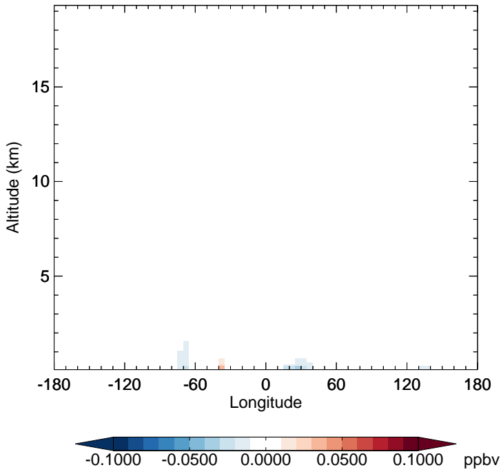
v11-02f-Run1 - v11-02e-Run1 XYLE - Diff along 15S for Jul
