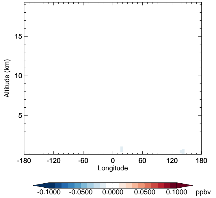
v11-02f-Run1 - v11-02e-Run1 ASOG3 - Diff along 42N for Jul
