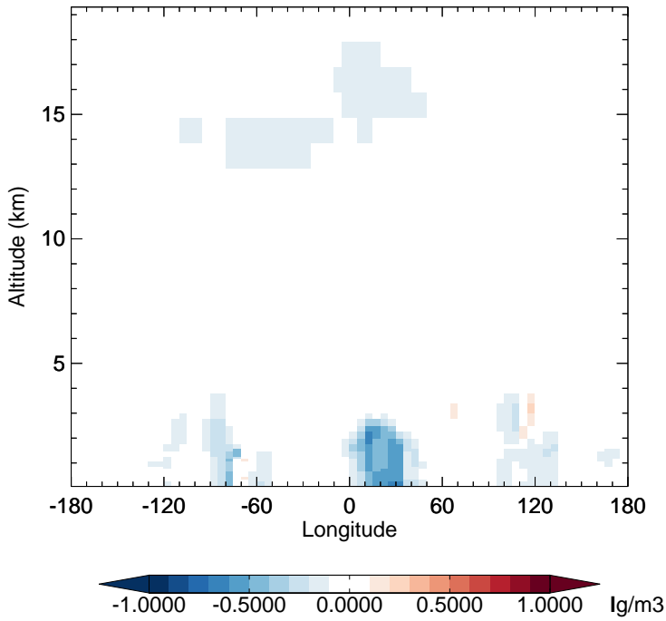
v11-02f-Run1 - v11-02e-Run0 SO4 - Diff along 15S for Jul
