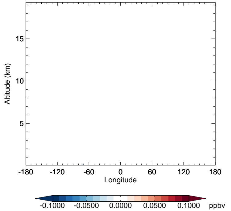
v11-02f-Run1 - v11-02e-Run0 ISOPNB - Diff along 42N for Jul
