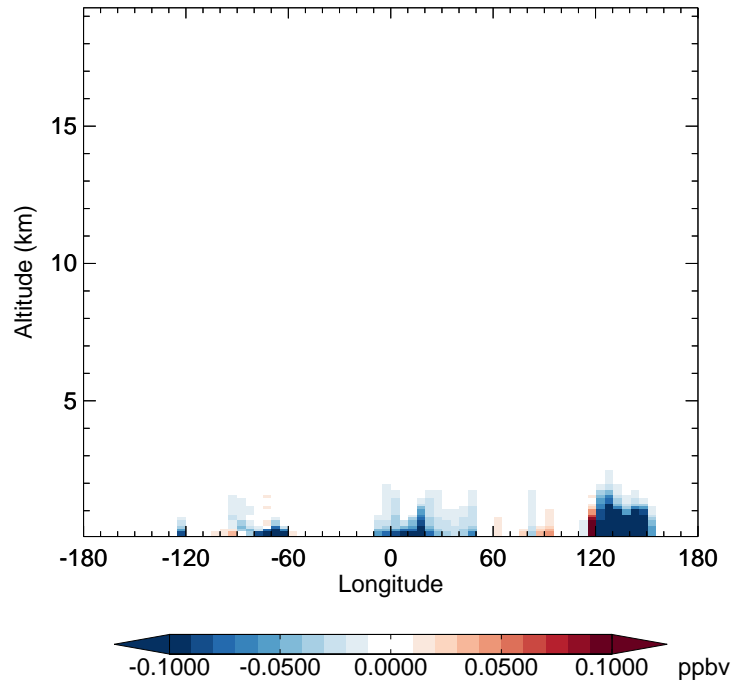
v11-02f-Run1 - v11-02e-Run0 XYLE - Diff along 42N for Jul
