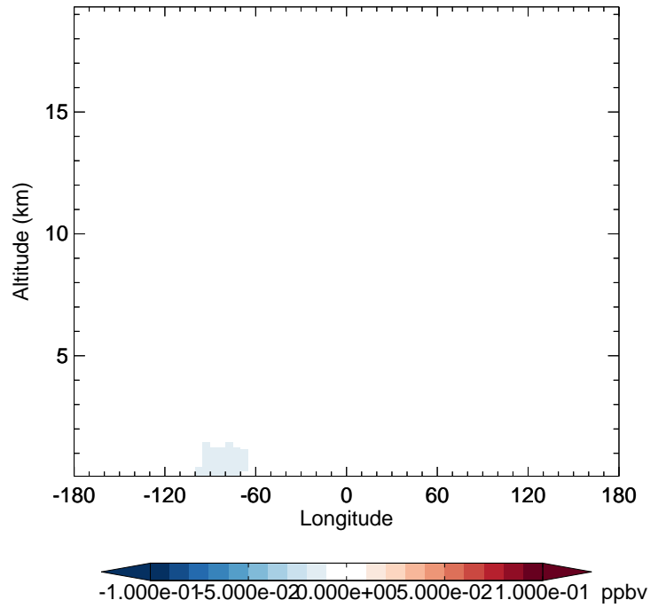
v11-02f-Run1 - v11-02e-Run0 ISO G 1 - Diff along 42N for Jul
