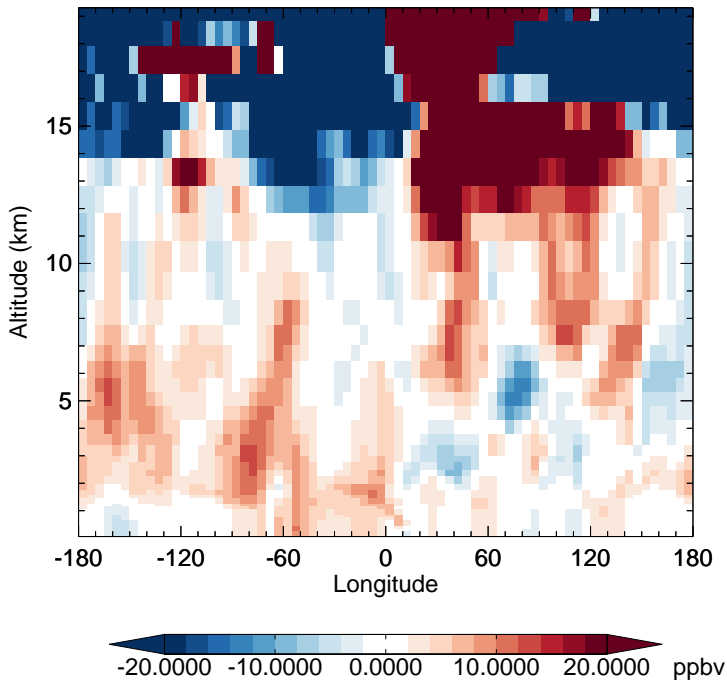
v11-02f-Run1 - v11-02e-Run0 O3 - Diff along 15S for Jul
