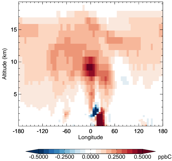
v11-02f-Run1 - v11-02e-Run0 C2H6 - Diff along 15S for Jul
