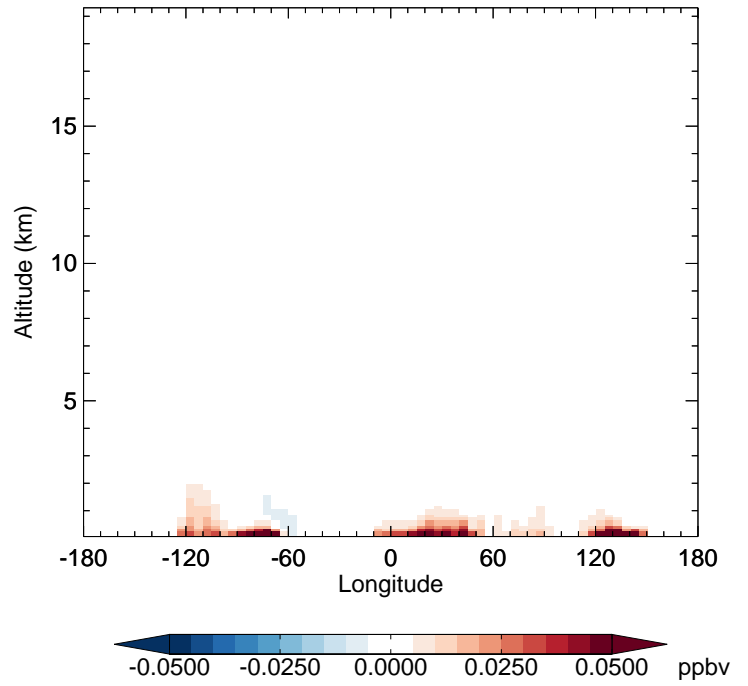
v11-02f-Run1 - v11-02e-Run1 RCHO - Diff along 42N for Jul
