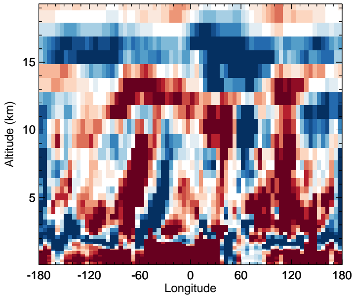
v11-02f-Run1 - v11-02e-Run0 OH - Diff along 15S for Jul
