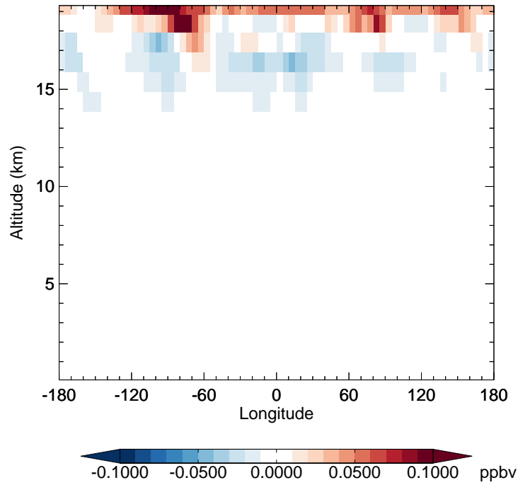
v11-02f-Run1 - v11-02e-Run0 ClNO 3 - Diff along 42N for Jul
