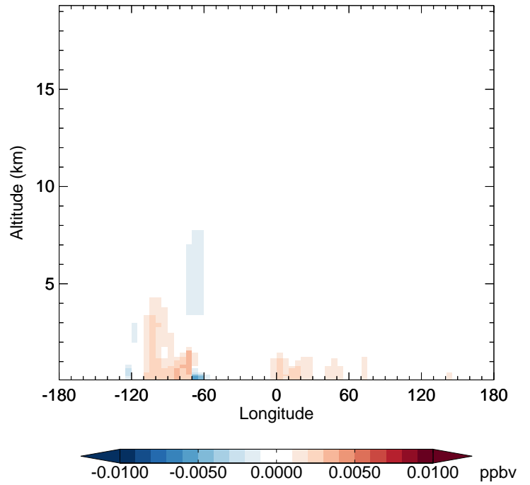
v11-02f-Run1 - v11-02e-Run0 R4N2 - Diff along 42N for Jul
