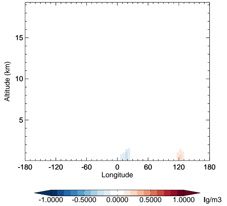
v11-02f-Run1 - v11-02e-Run1 BCPI - Diff along 42N for Jul
