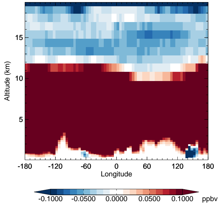
v11-02f-Run1 - v11-02e-Run1 CH4 - Diff along 42N for Jul
