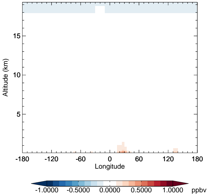
v11-02f-Run1 - v11-02e-Run1 NO2 - Diff along 15S for Jul
