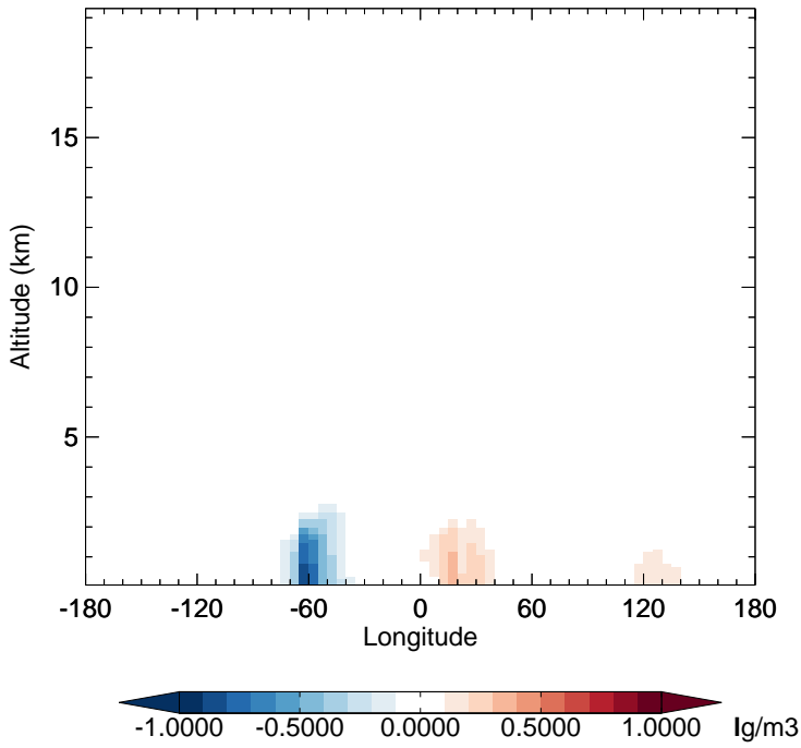
v11-02f-Run1 - v11-02e-Run1 SOAS - Diff along 15S for Jul
