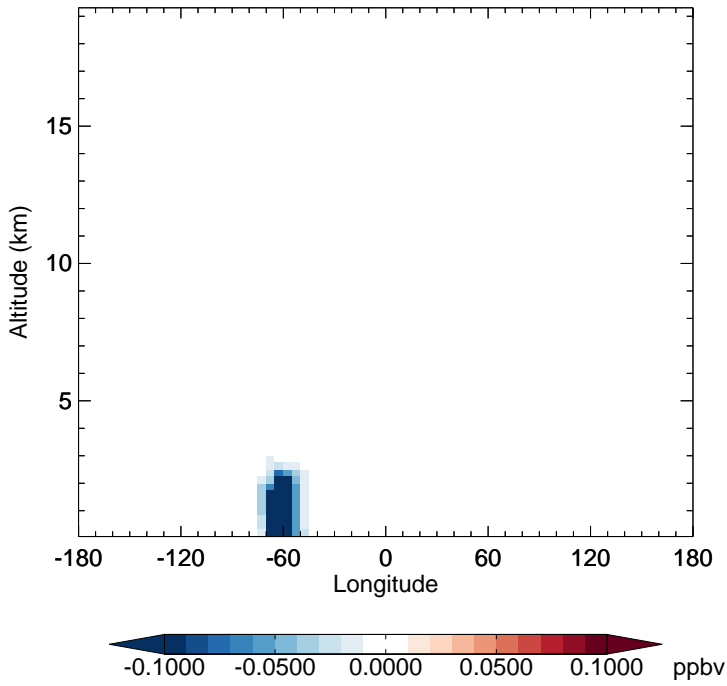
v11-02f-Run1 - v11-02e-Run1 HPALD - Diff along 15S for Jul
