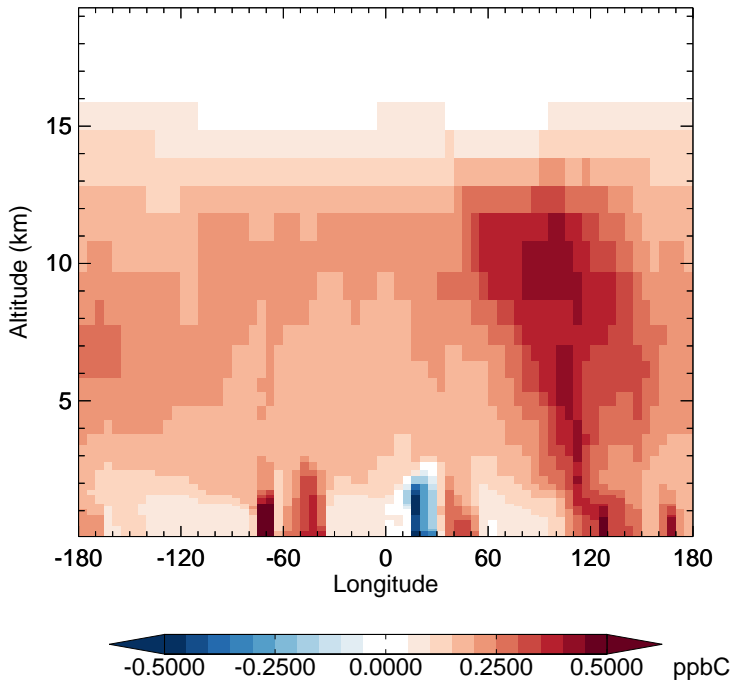
v11-02f-Run1 - v11-02e-Run1 ACET - Diff along 15S for Jul
