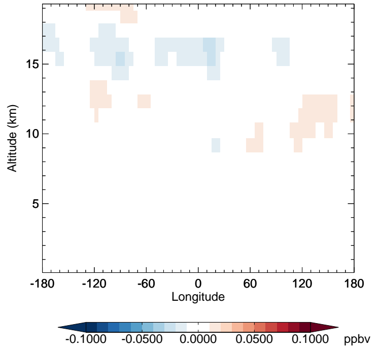
v11-02f-Run1 - v11-02e-Run0 MPN - Diff along 42N for Jul
