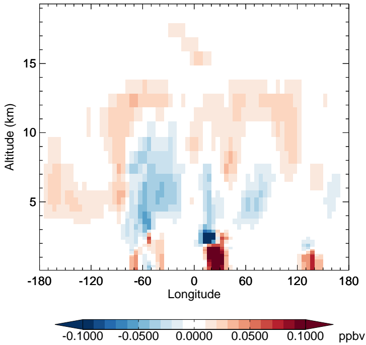
v11-02f-Run1 - v11-02e-Run0 PAN - Diff along 15S for Jul
