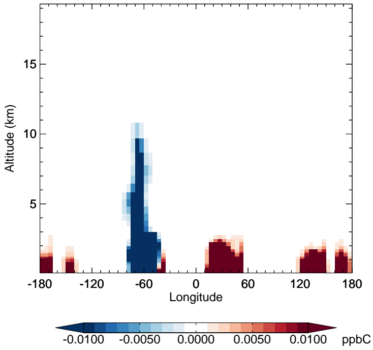
v11-02f-Run1 - v11-02e-Run1 PRPE - Diff along 15S for Jul
