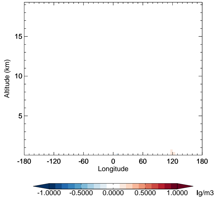
v11-02f-Run1 - v11-02e-Run0 BCPO - Diff along 42N for Jul
