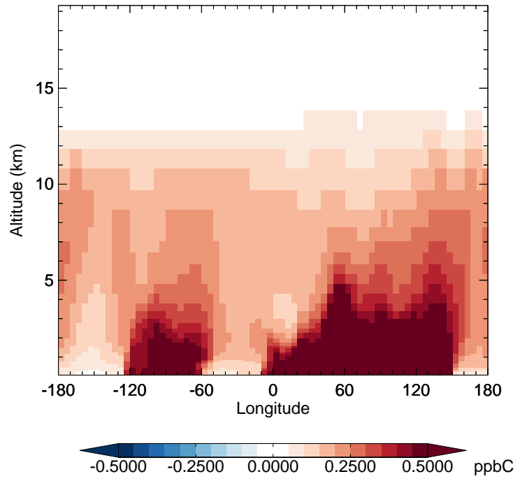
v11-02f-Run1 - v11-02e-Run1 ACET - Diff along 42N for Jul
