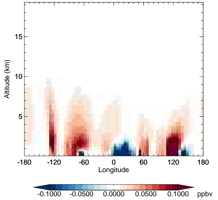
v11-02f-Run1 - v11-02e-Run1 BENZ - Diff along 42N for Jul
