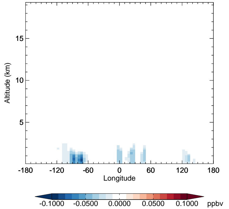
v11-02f-Run1 - v11-02e-Run0 IEPOXA - Diff along 42N for Jul
