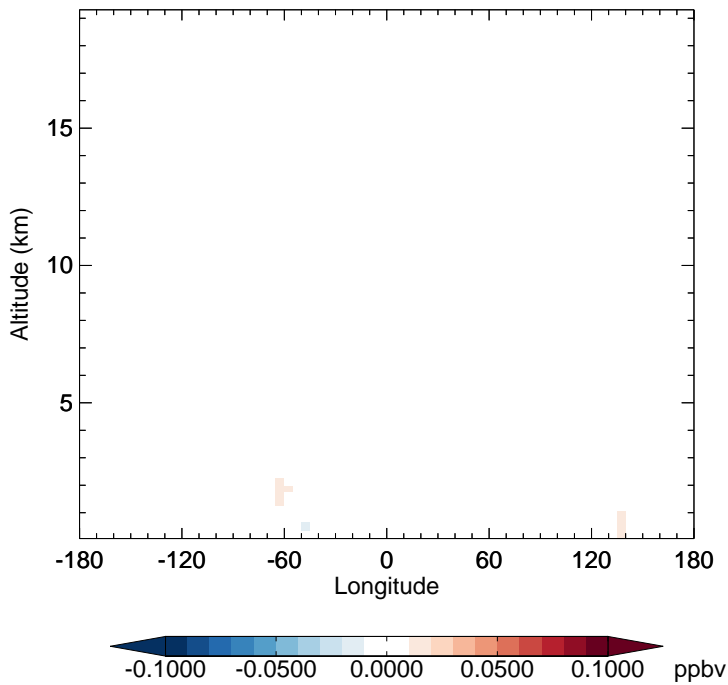
v11-02f-Run1 - v11-02e-Run0 GLYX - Diff along 15S for Jul
