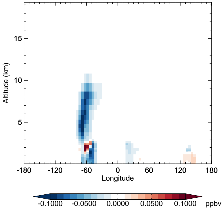
v11-02f-Run1 - v11-02e-Run0 IEPOXA - Diff along 15S for Jul
