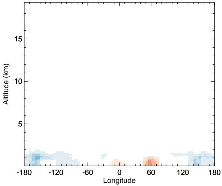
v11-02f-Run1 - v11-02e-Run0 SALA - Diff along 15S for Jul
