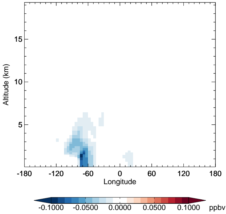
v11-02f-Run1 - v11-02e-Run1 SOAIE - Diff along 15S for Jul
