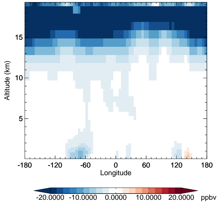
v11-02f-Run1 - v11-02e-Run1 O3 - Diff along 42N for Jul
