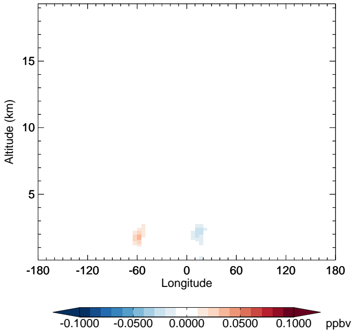
v11-02f-Run1 - v11-02e-Run0 TSOA3 - Diff along 15S for Jul
