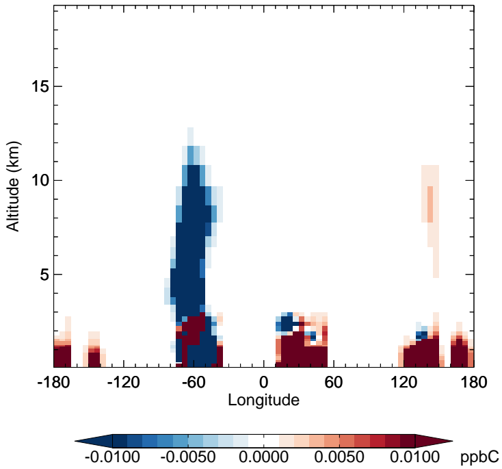
v11-02f-Run1 - v11-02e-Run0 PRPE - Diff along 15S for Jul
