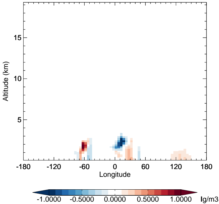
v11-02f-Run1 - v11-02e-Run0 SOAS - Diff along 15S for Jul
