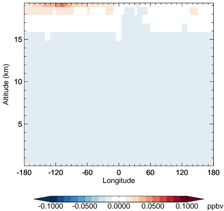
v11-02f-Run1 - v11-02e-Run0 CFC12 - Diff along 15S for Jul
