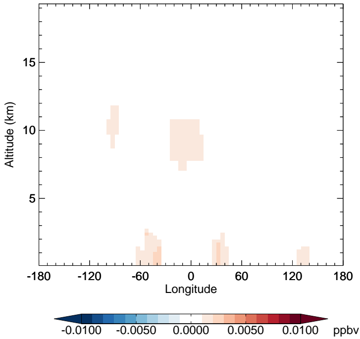
v11-02f-Run1 - v11-02e-Run0 R4N2 - Diff along 15S for Jul
