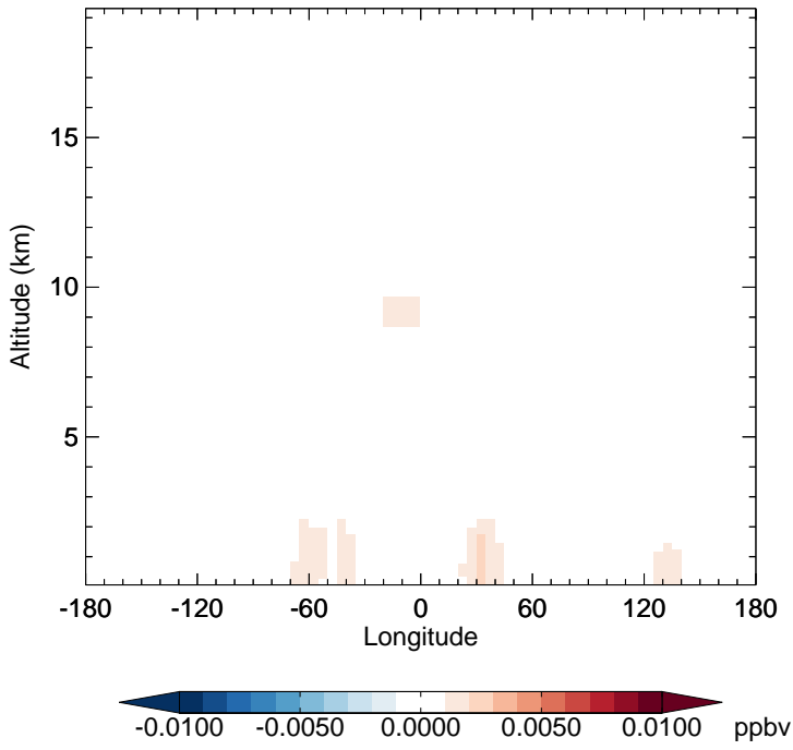
v11-02f-Run1 - v11-02e-Run1 R4N2 - Diff along 15S for Jul
