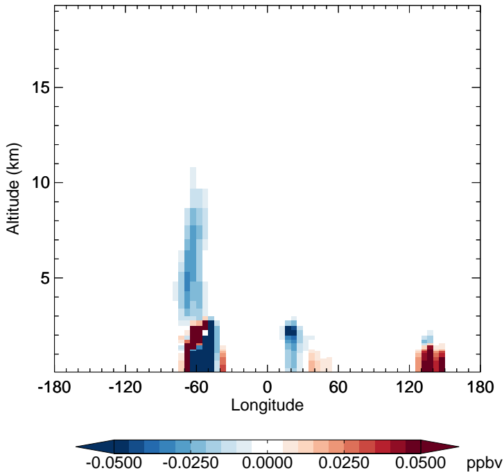
v11-02f-Run1 - v11-02e-Run0 MVK - Diff along 15S for Jul
