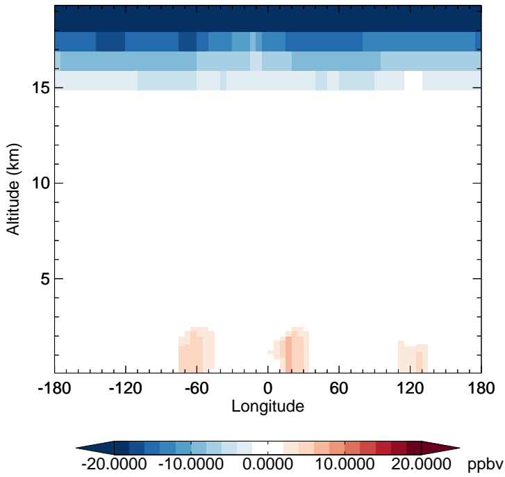
v11-02f-Run1 - v11-02e-Run1 O3 - Diff along 15S for Jul
