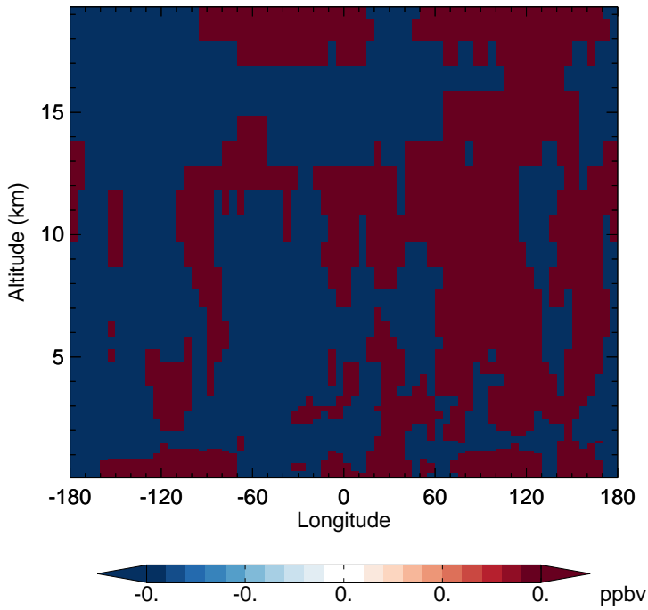
v11-02f-Run1 - v11-02e-Run0 H2O - Diff along 15S for Jul
