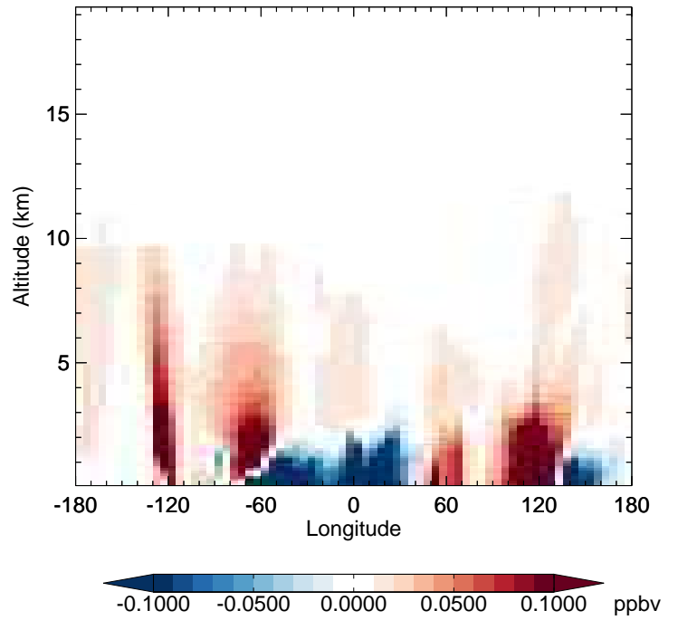
v11-02f-Run1 - v11-02e-Run0 BENZ - Diff along 42N for Jul
