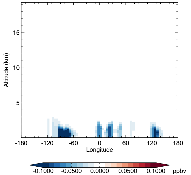
v11-02f-Run1 - v11-02e-Run0 GLYC - Diff along 42N for Jul
