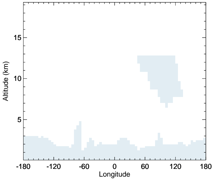
v11-02f-Run1 - v11-02e-Run0 HCFC22 - Diff along 15S for Jul
