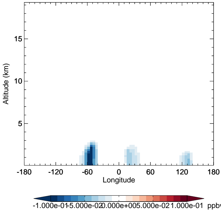
v11-02f-Run1 - v11-02e-Run1 IONITA - Diff along 15S for Jul
