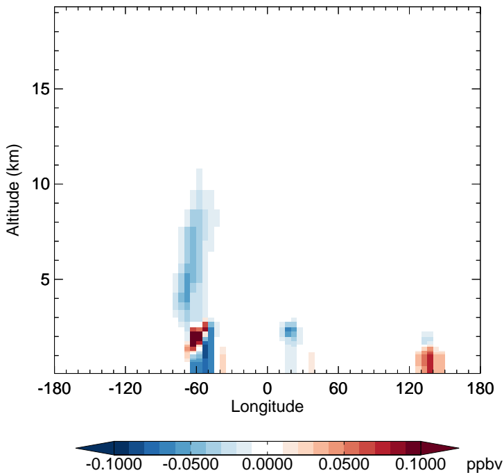
v11-02f-Run1 - v11-02e-Run0 GLYC - Diff along 15S for Jul
