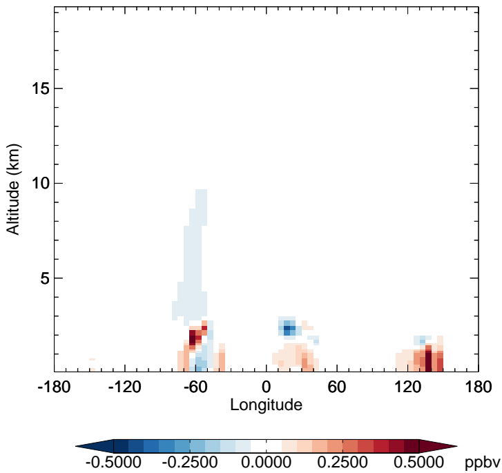
v11-02f-Run1 - v11-02e-Run0 CH 2 O - Diff along 15S for Jul
