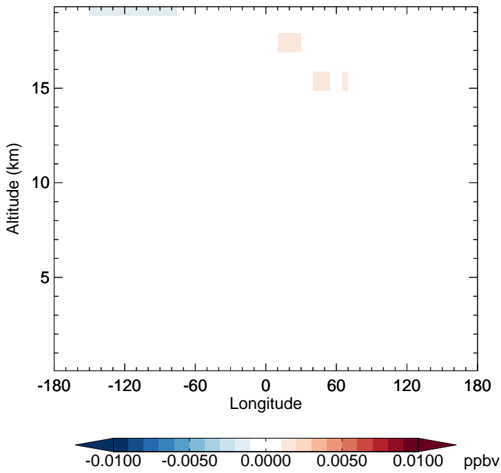
v11-02f-Run1 - v11-02e-Run0 BrNO 3 - Diff along 15S for Jul
