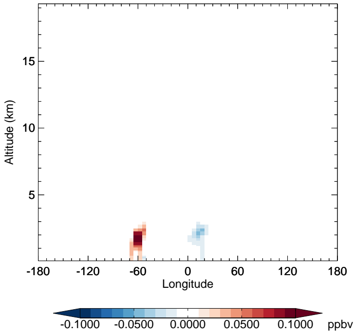
v11-02f-Run1 - v11-02e-Run0 TSOA2 - Diff along 15S for Jul
