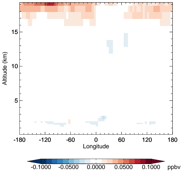
v11-02f-Run1 - v11-02e-Run0 CH3Cl - Diff along 15S for Jul
