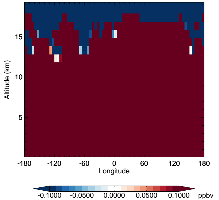
v11-02f-Run1 - v11-02e-Run0 N2O - Diff along 42N for Jul
