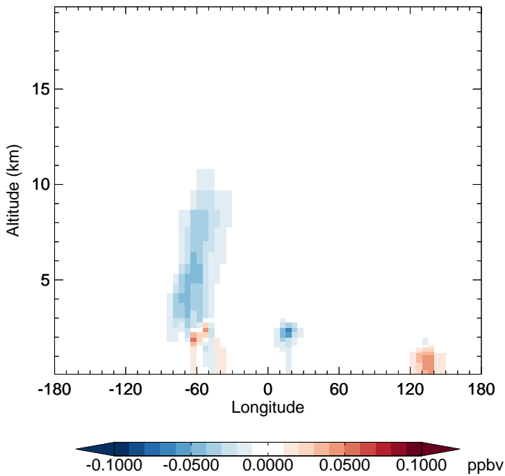
v11-02f-Run1 - v11-02e-Run0 IMAE - Diff along 15S for Jul
