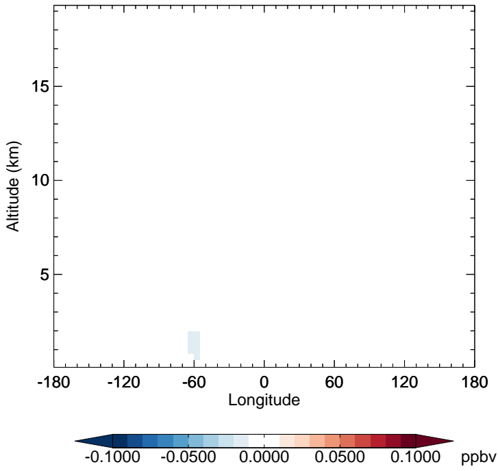
v11-02f-Run1 - v11-02e-Run1 ISOA3 - Diff along 15S for Jul
