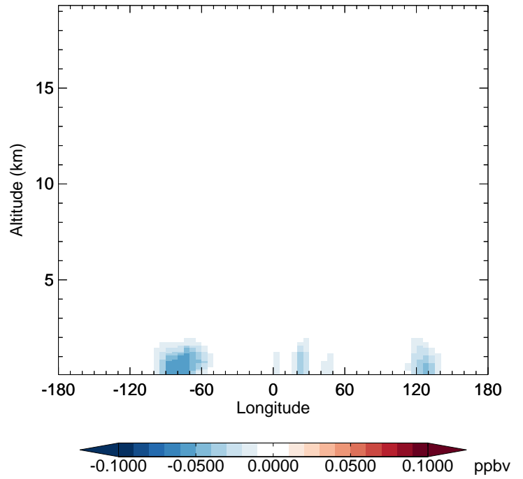
v11-02f-Run1 - v11-02e-Run1 ISOA1 - Diff along 42N for Jul
