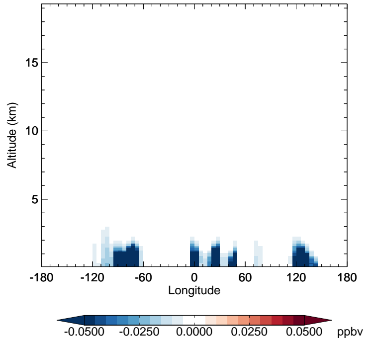
v11-02f-Run1 - v11-02e-Run1 MVK - Diff along 42N for Jul
