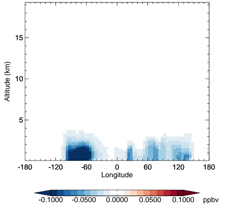
v11-02f-Run1 - v11-02e-Run1 SOAIE - Diff along 42N for Jul
