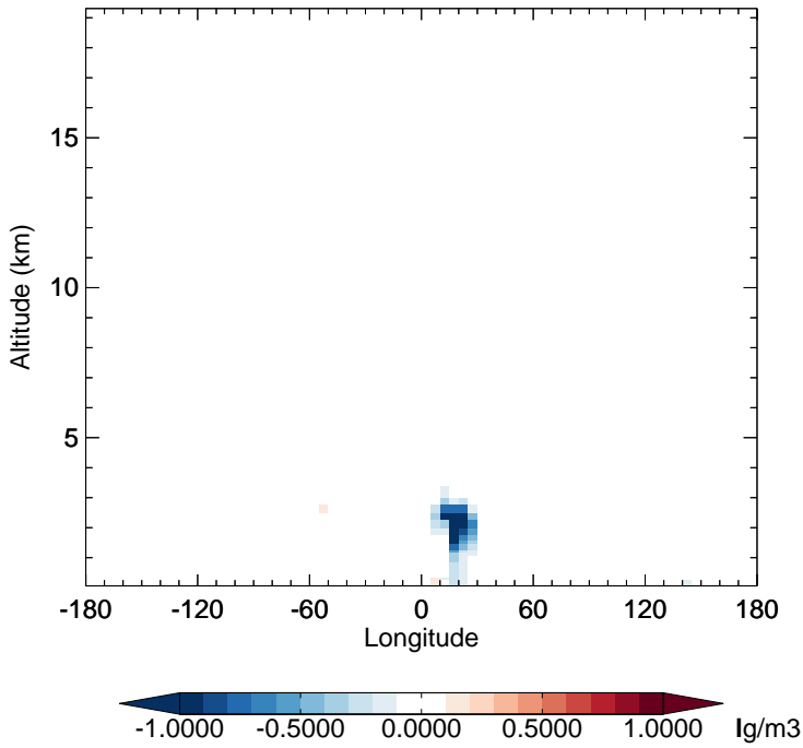
v11-02f-Run1 - v11-02e-Run0 NIT - Diff along 15S for Jul
