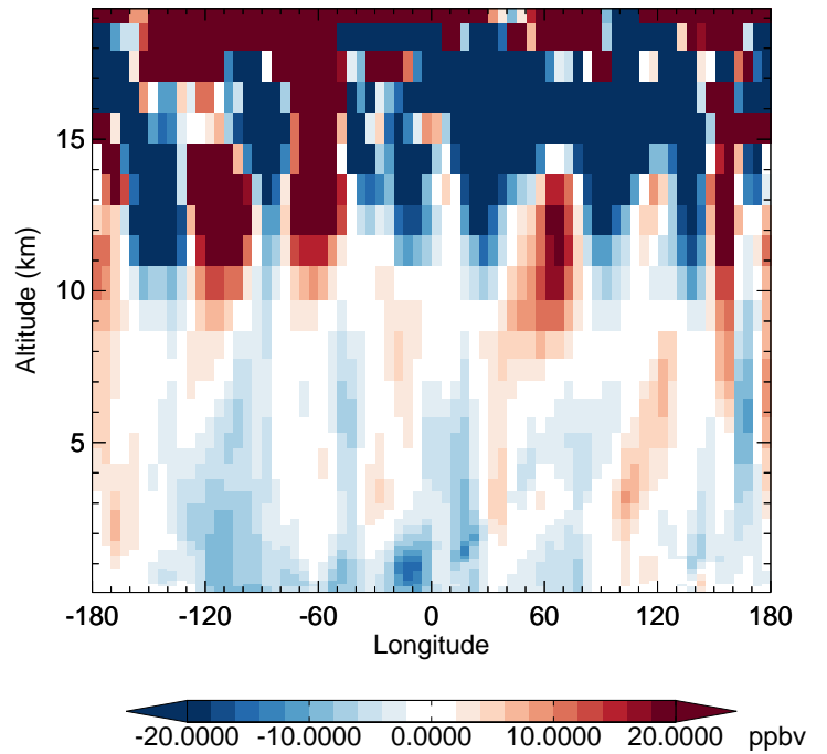
v11-02f-Run1 - v11-02e-Run0 O3 - Diff along 42N for Jul
