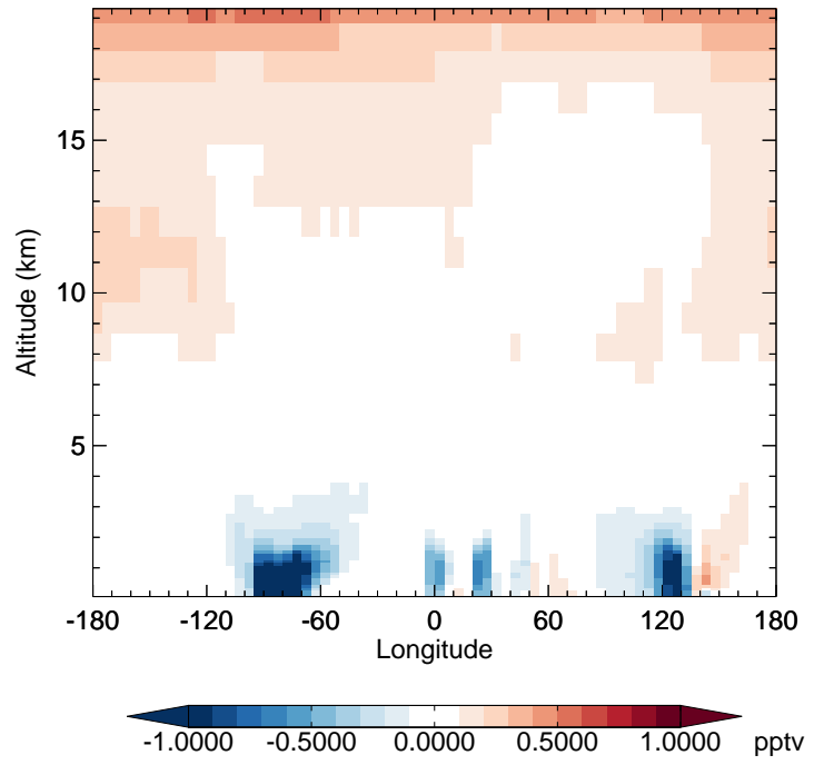
v11-02f-Run1 - v11-02e-Run1 HO2 - Diff along 42N for Jul
