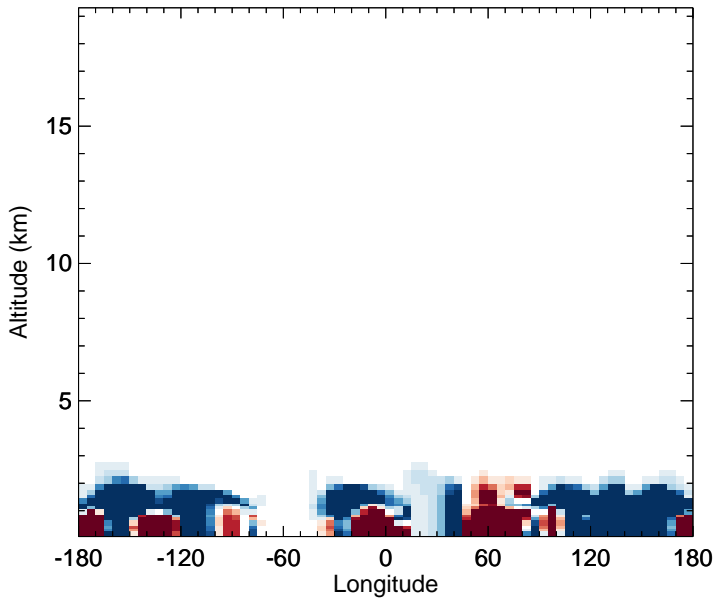
v11-02f-Run1 - v11-02e-Run0 SALC - Diff along 15S for Jul
