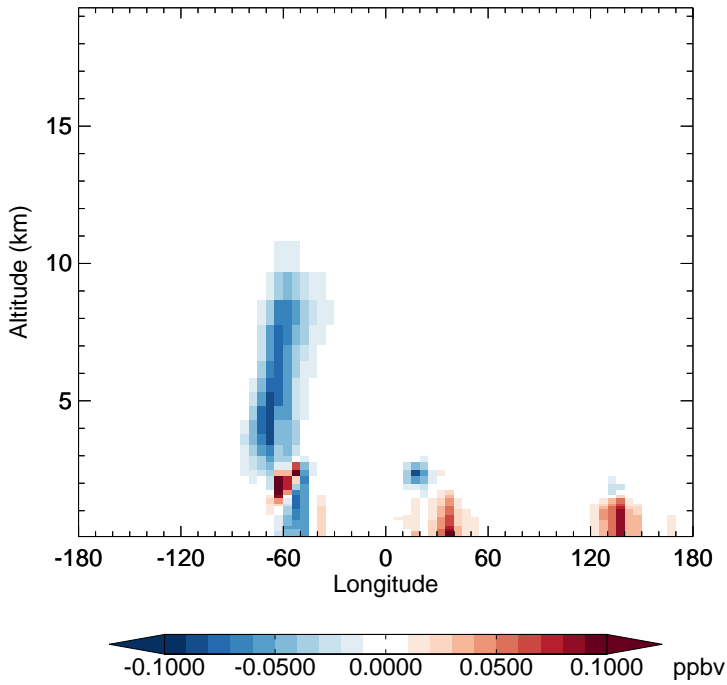
v11-02f-Run1 - v11-02e-Run0 HAC - Diff along 15S for Jul
