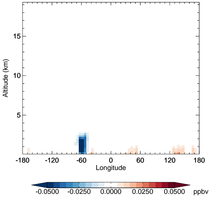
v11-02f-Run1 - v11-02e-Run1 RCHO - Diff along 15S for Jul
