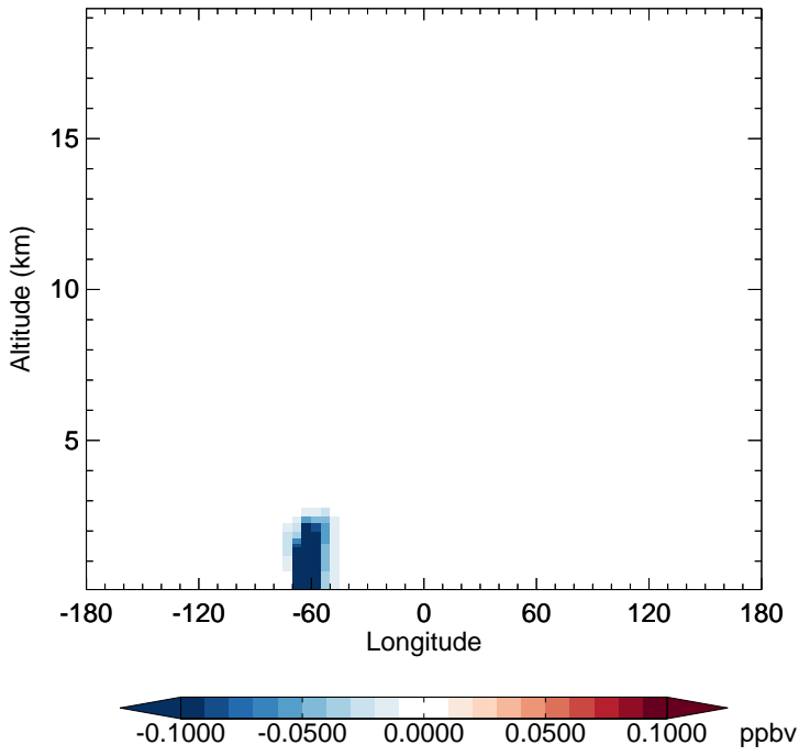
v11-02f-Run1 - v11-02e-Run1 RIPB - Diff along 15S for Jul
