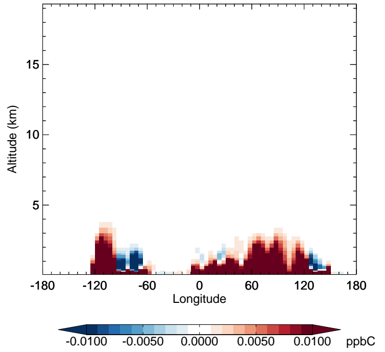
v11-02f-Run1 - v11-02e-Run1 PRPE - Diff along 42N for Jul
