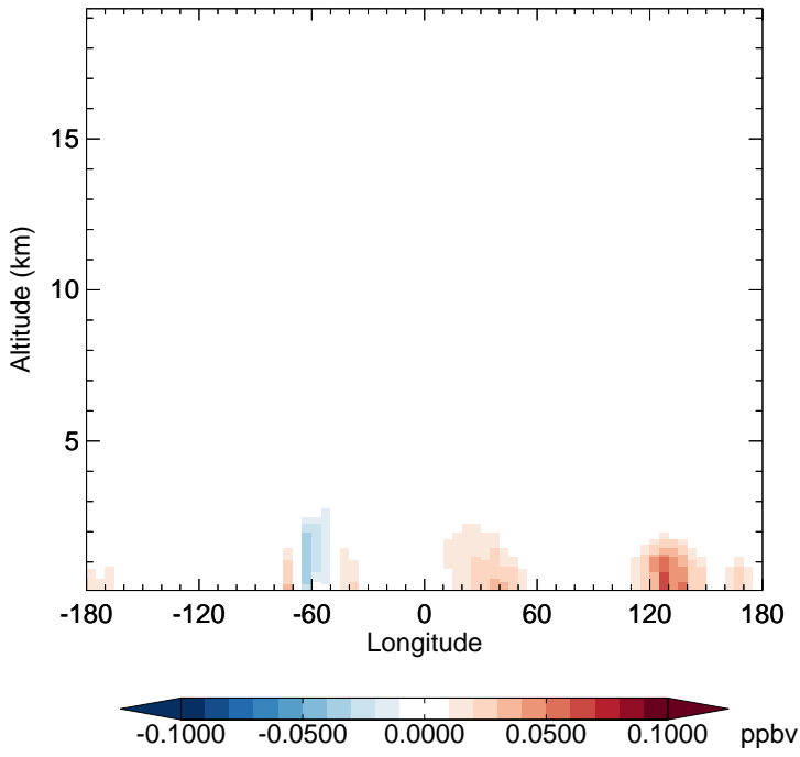
v11-02f-Run1 - v11-02e-Run1 TSOG3 - Diff along 15S for Jul
