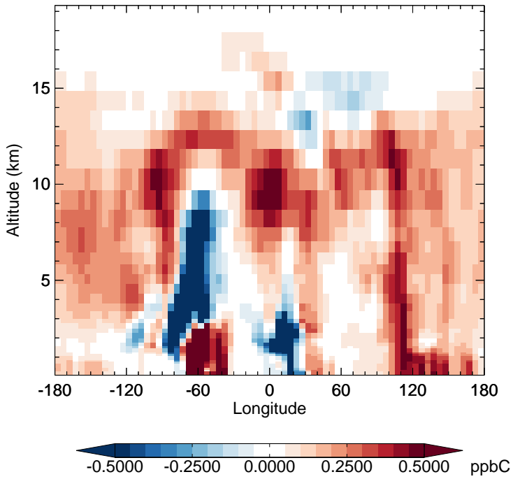
v11-02f-Run1 - v11-02e-Run0 ACET - Diff along 15S for Jul
