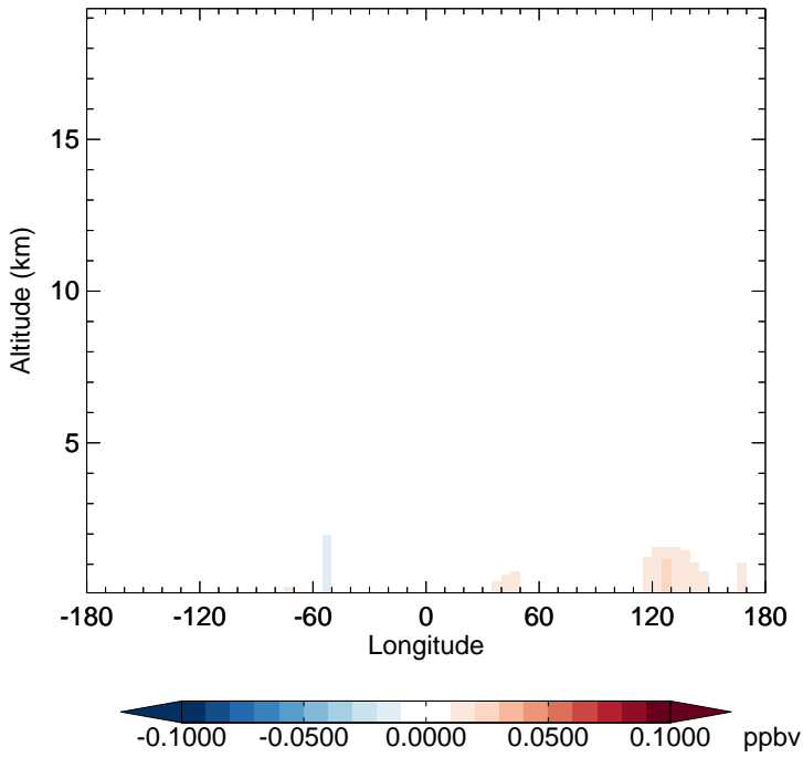
v11-02f-Run1 - v11-02e-Run1 TSOG2 - Diff along 15S for Jul
