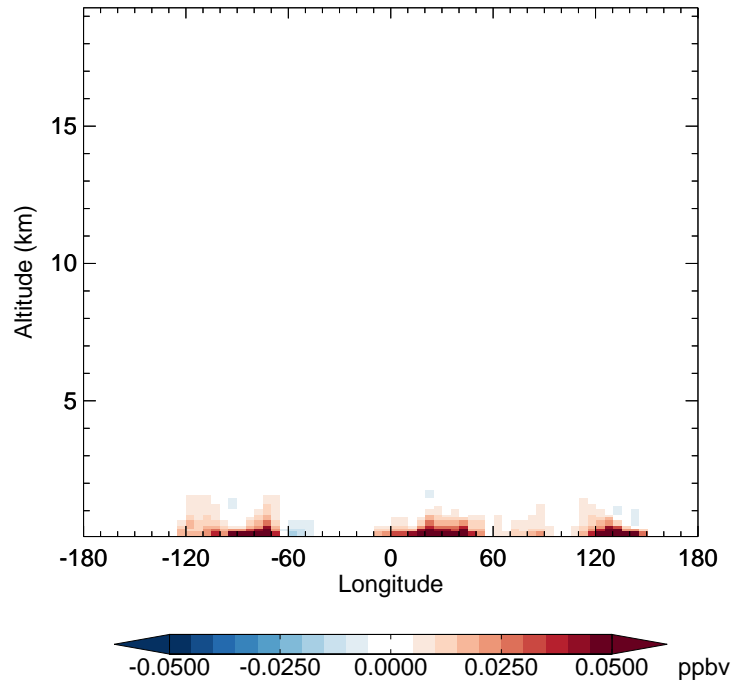
v11-02f-Run1 - v11-02e-Run0 RCHO - Diff along 42N for Jul
