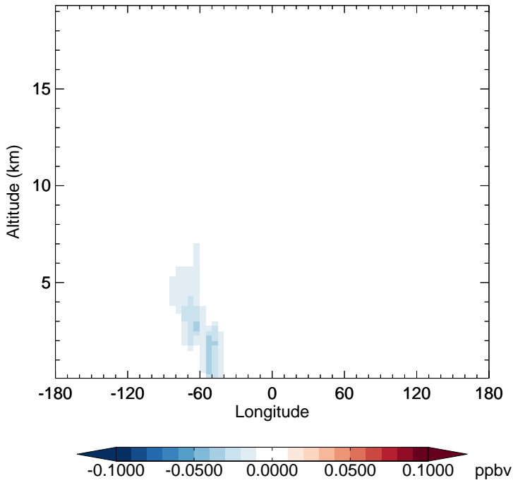
v11-02f-Run1 - v11-02e-Run1 HC187 - Diff along 15S for Jul
