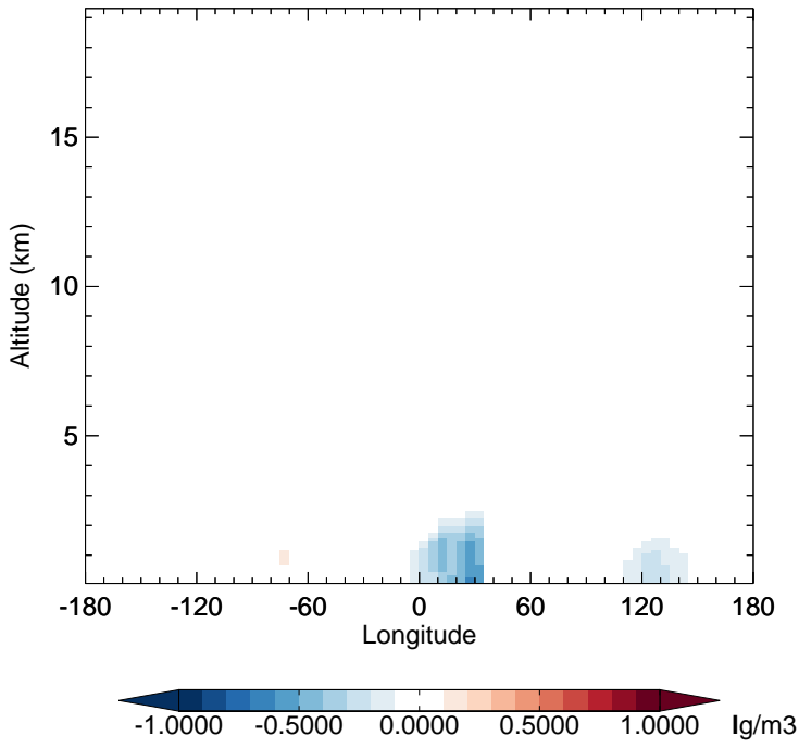
v11-02f-Run1 - v11-02e-Run1 SO4 - Diff along 15S for Jul
