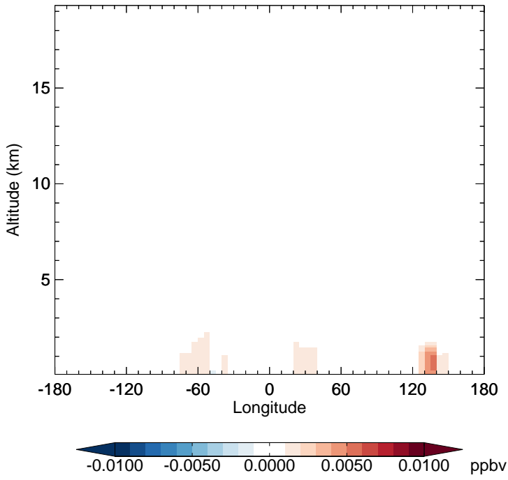
v11-02f-Run1 - v11-02e-Run1 MVKN - Diff along 15S for Jul
