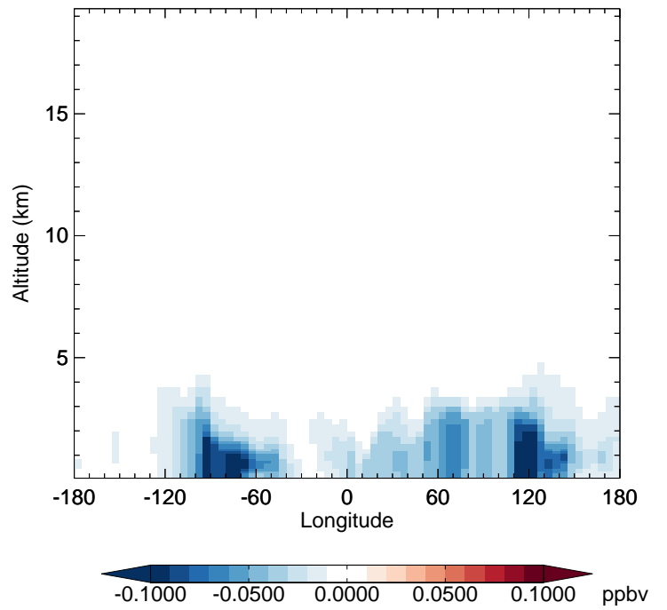
v11-02f-Run1 - v11-02e-Run0 SOAIE - Diff along 42N for Jul
