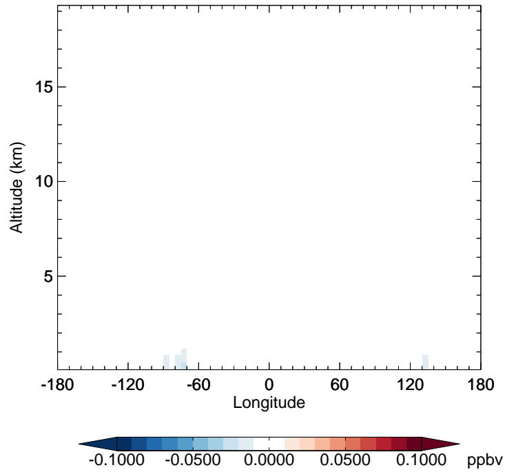
v11-02f-Run1 - v11-02e-Run0 RIPA - Diff along 42N for Jul
