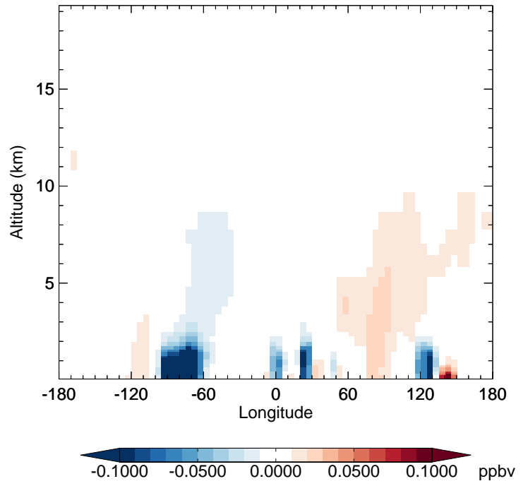
v11-02f-Run1 - v11-02e-Run1 PAN - Diff along 42N for Jul
