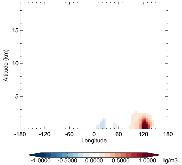
v11-02f-Run1 - v11-02e-Run1 OCPI - Diff along 42N for Jul
