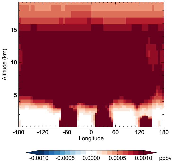
v11-02f-Run1 - v11-02e-Run1 PPN - Diff along 15S for Jul
