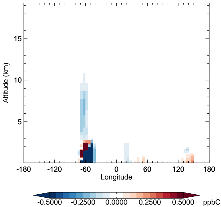
v11-02f-Run1 - v11-02e-Run0 ISOP - Diff along 15S for Jul
