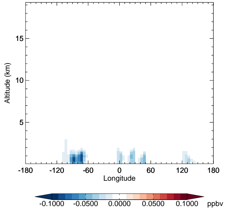
v11-02f-Run1 - v11-02e-Run1 IEPOXA - Diff along 42N for Jul
