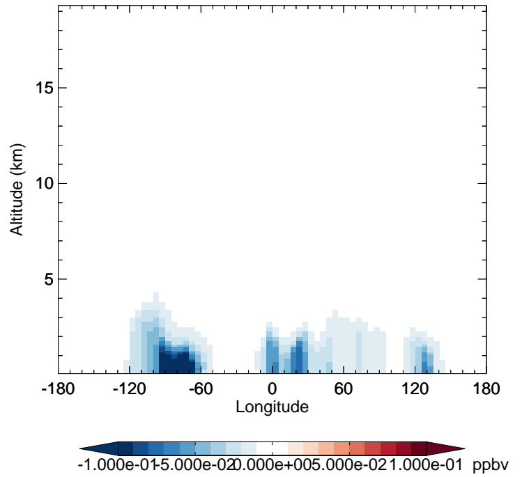
v11-02f-Run1 - v11-02e-Run0 IONITA - Diff along 42N for Jul
