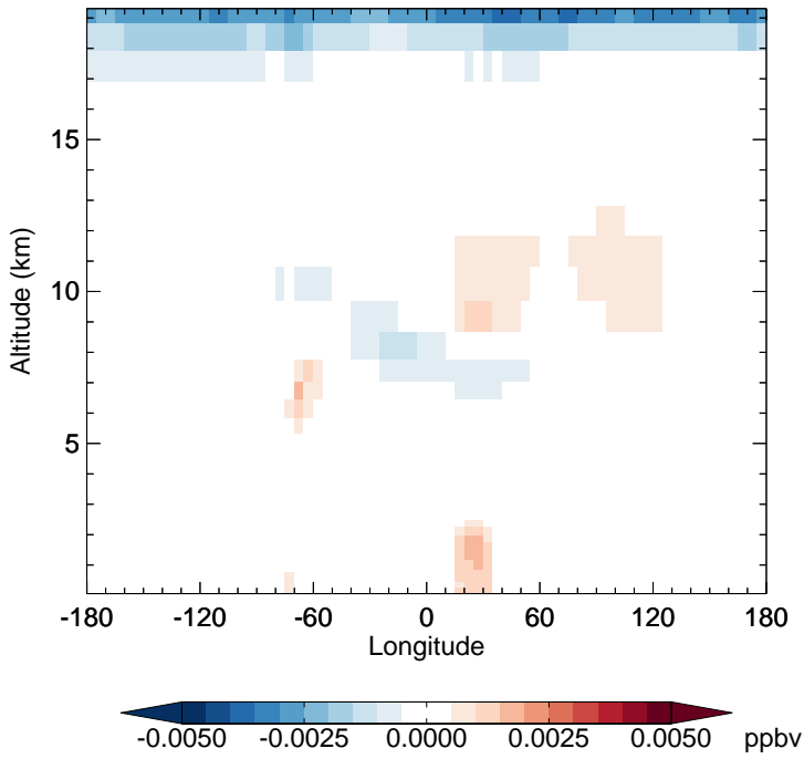
v11-02f-Run1 - v11-02e-Run1 HNO 4 - Diff along 15S for Jul
