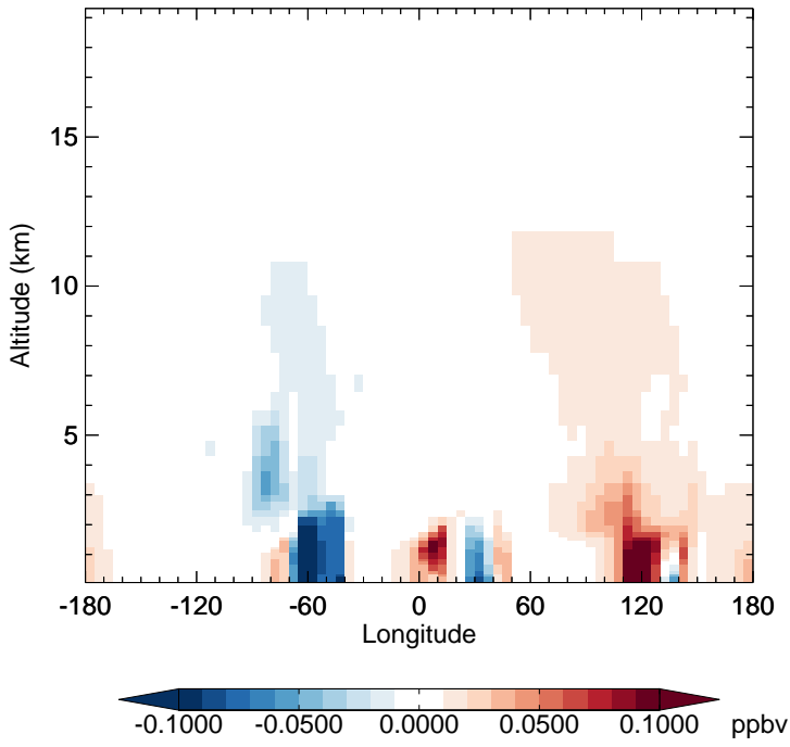
v11-02f-Run1 - v11-02e-Run1 H2O2 - Diff along 15S for Jul
