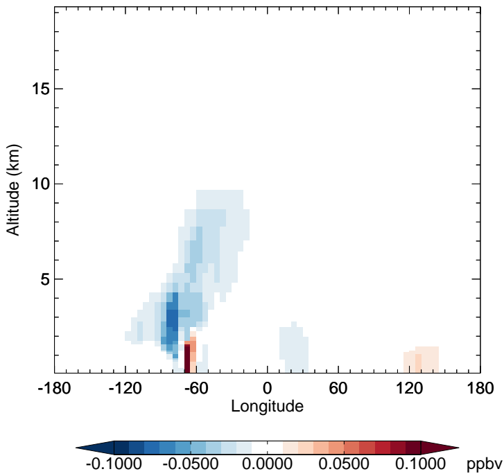
v11-02f-Run1 - v11-02e-Run0 SOAIE - Diff along 15S for Jul
