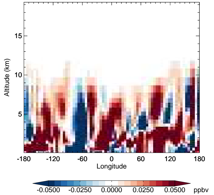
v11-02f-Run1 - v11-02e-Run0 MP - Diff along 42N for Jul
