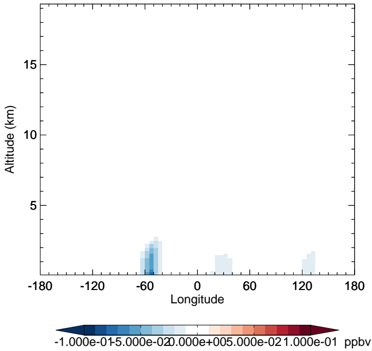
v11-02f-Run1 - v11-02e-Run0 MONITA - Diff along 15S for Jul
