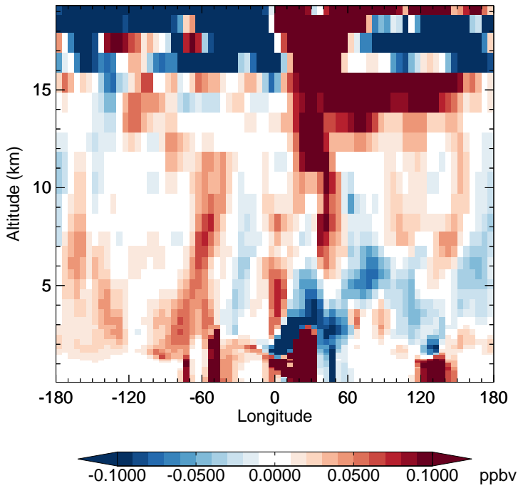
v11-02f-Run1 - v11-02e-Run0 HNO 3 - Diff along 15S for Jul
