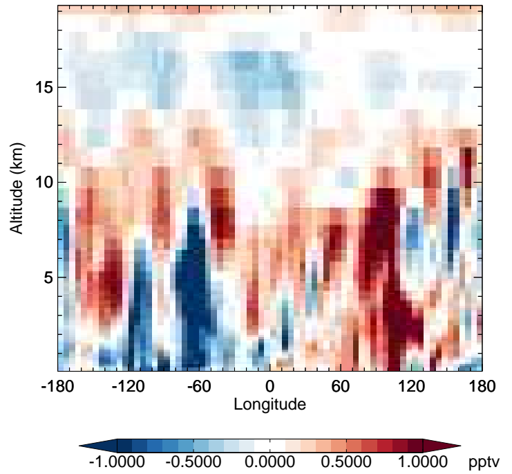
v11-02f-Run1 - v11-02e-Run0 HO2 - Diff along 42N for Jul
