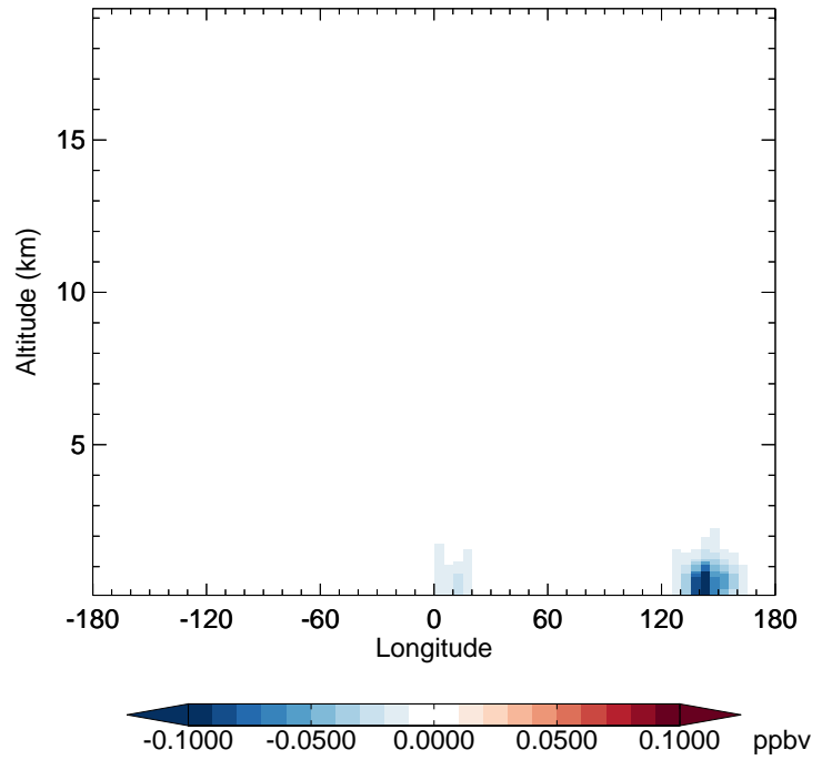
v11-02f-Run1 - v11-02e-Run0 ASOAN - Diff along 42N for Jul
