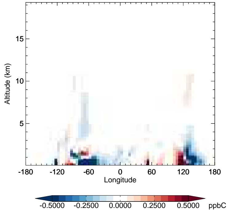
v11-02f-Run1 - v11-02e-Run0 ALK4 - Diff along 42N for Jul
