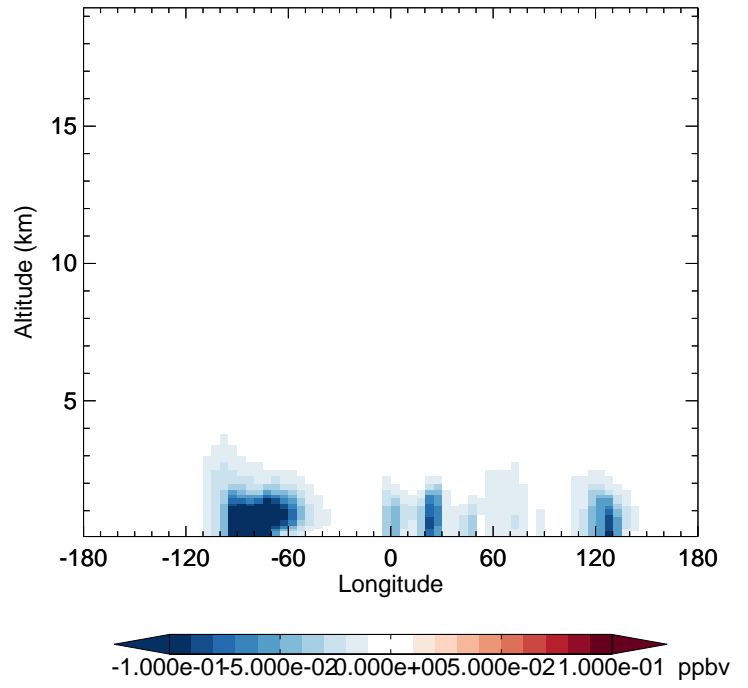
v11-02f-Run1 - v11-02e-Run1 ISO3 - Diff along 42N for Jul
