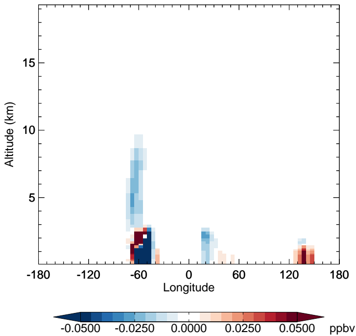
v11-02f-Run1 - v11-02e-Run0 MACR - Diff along 15S for Jul
