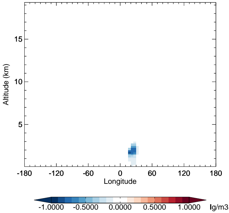
v11-02f-Run1 - v11-02e-Run1 NIT - Diff along 15S for Jul
