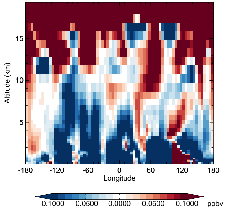
v11-02f-Run1 - v11-02e-Run0 HNO 3 - Diff along 42N for Jul
