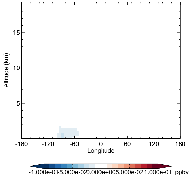
v11-02f-Run1 - v11-02e-Run1 ISO G 1 - Diff along 42N for Jul
