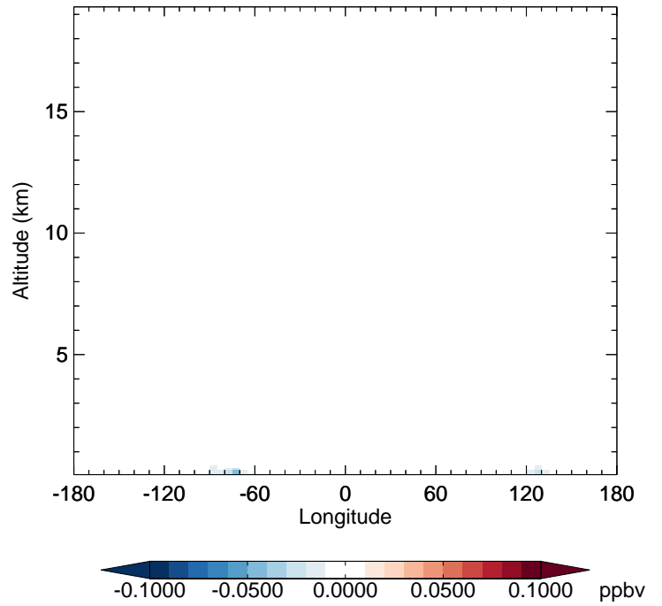
v11-02f-Run1 - v11-02e-Run0 ISN1 - Diff along 42N for Jul
