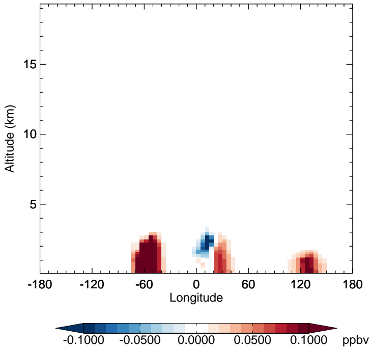
v11-02f-Run1 - v11-02e-Run0 INDIOL - Diff along 15S for Jul
