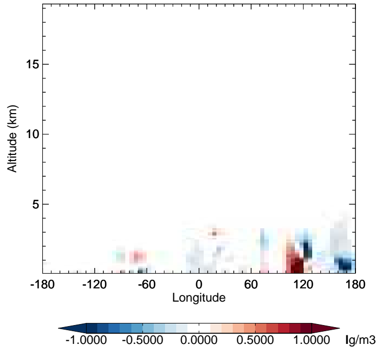
v11-02f-Run1 - v11-02e-Run0 SO 2 - Diff along 42N for Jul
