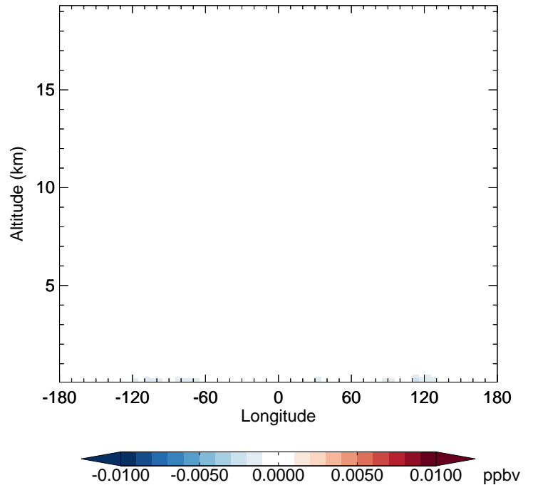
v11-02f-Run1 - v11-02e-Run1 NO3 - Diff along 42N for Jul
