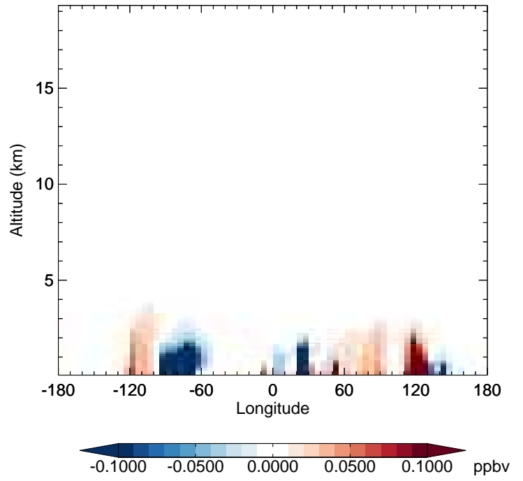
v11-02f-Run1 - v11-02e-Run1 EOH - Diff along 42N for Jul
