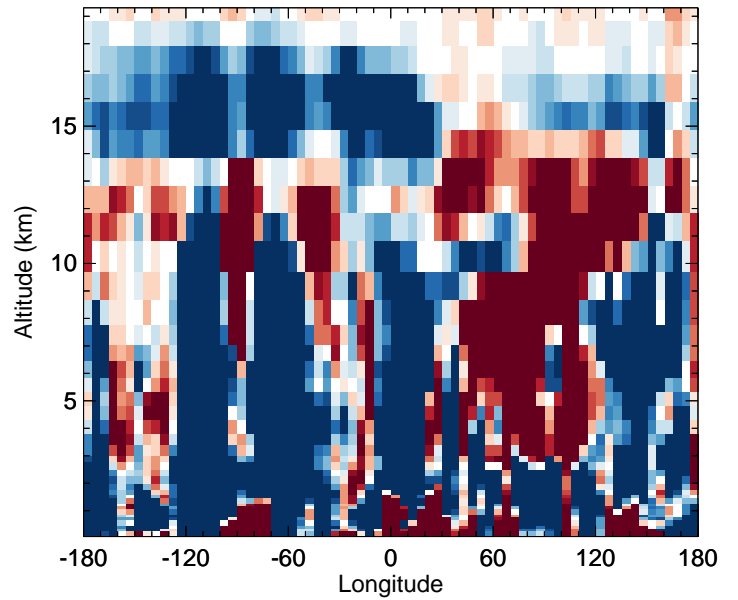
v11-02f-Run1 - v11-02e-Run0 OH - Diff along 42N for Jul
