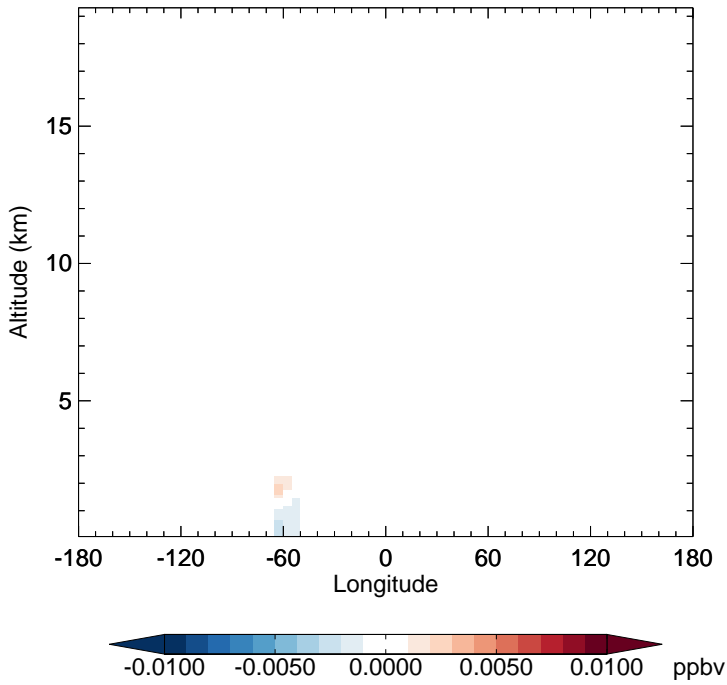
v11-02f-Run1 - v11-02e-Run0 MOBA - Diff along 15S for Jul
