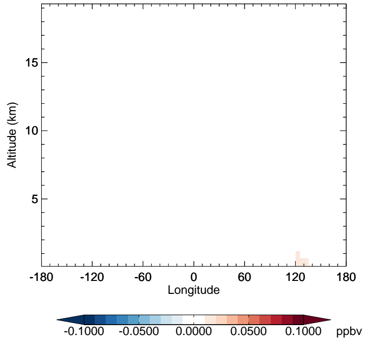
v11-02f-Run1 - v11-02e-Run0 TSOA1 - Diff along 42N for Jul
