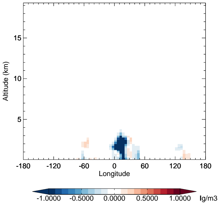
v11-02f-Run1 - v11-02e-Run0 OCPI - Diff along 15S for Jul
