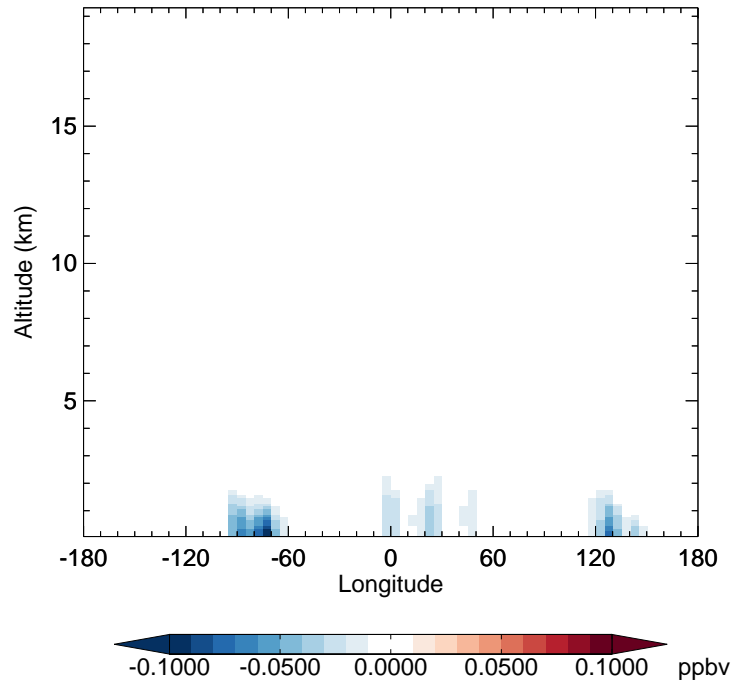
v11-02f-Run1 - v11-02e-Run0 MGLY - Diff along 42N for Jul
