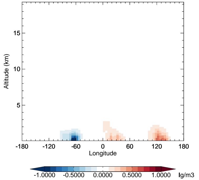
v11-02f-Run1 - v11-02e-Run1 SOAS - Diff along 42N for Jul
