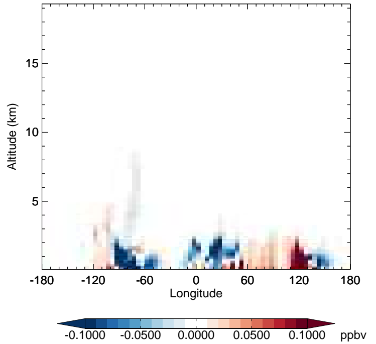
v11-02f-Run1 - v11-02e-Run0 EOH - Diff along 42N for Jul
