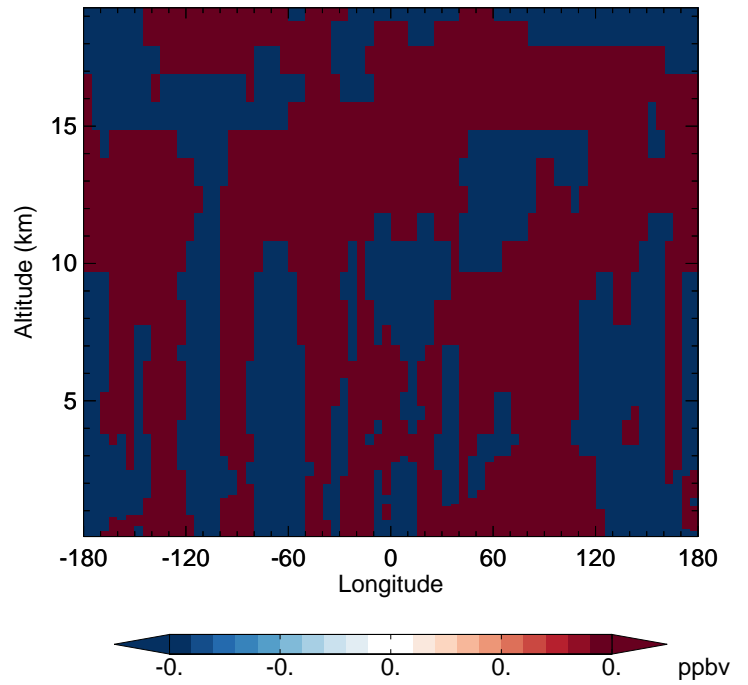
v11-02f-Run1 - v11-02e-Run0 H2O - Diff along 42N for Jul
