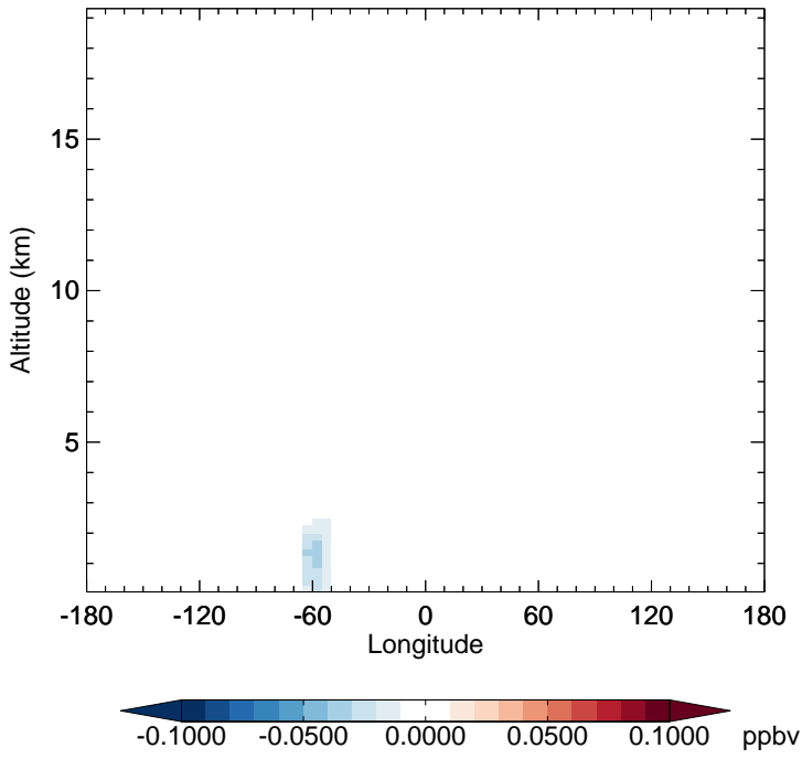
v11-02f-Run1 - v11-02e-Run1 TSOA2 - Diff along 15S for Jul
