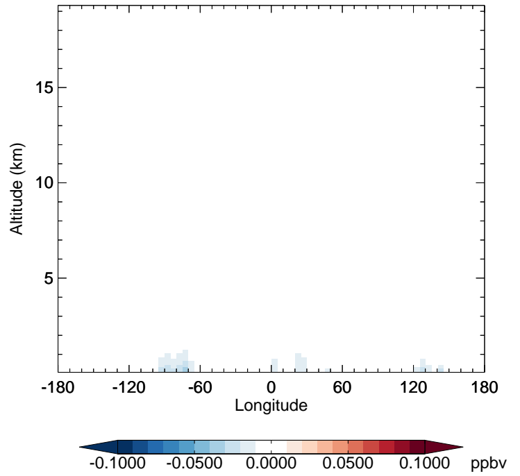
v11-02f-Run1 - v11-02e-Run1 GLYX - Diff along 42N for Jul
