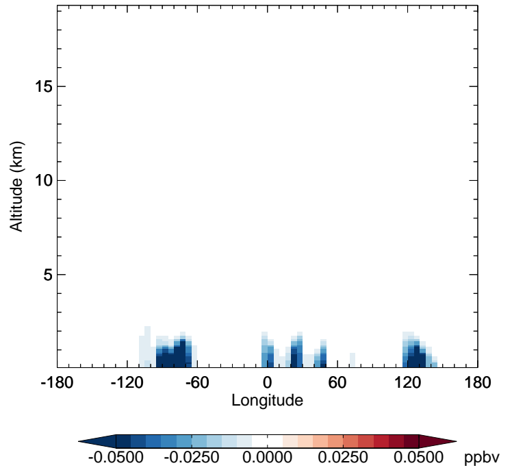
v11-02f-Run1 - v11-02e-Run1 MACR - Diff along 42N for Jul
