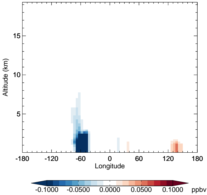
v11-02f-Run1 - v11-02e-Run1 GLYC - Diff along 15S for Jul
