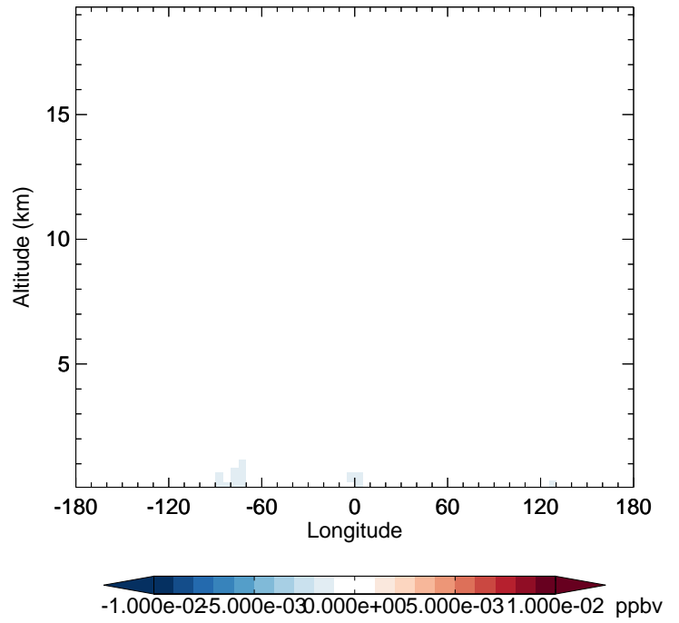
v11-02f-Run1 - v11-02e-Run1 MACRN - Diff along 42N for Jul
