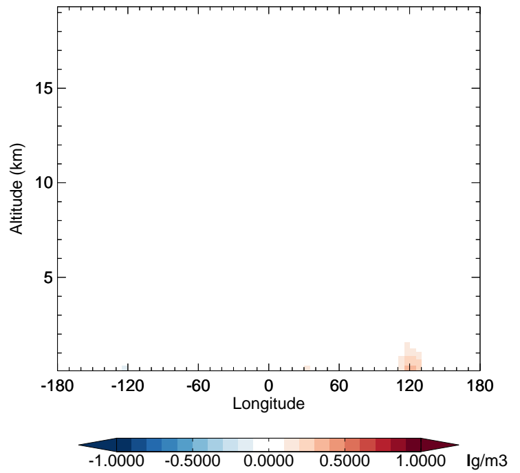
v11-02f-Run1 - v11-02e-Run0 OCPO - Diff along 42N for Jul
