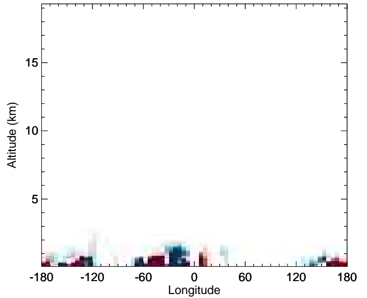
v11-02f-Run1 - v11-02e-Run0 SALC - Diff along 42N for Jul
