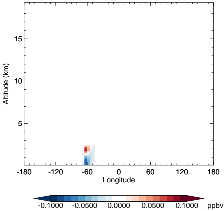
v11-02f-Run1 - v11-02e-Run0 RIPB - Diff along 15S for Jul
