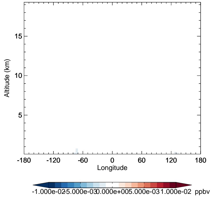
v11-02f-Run1 - v11-02e-Run1 MOBA - Diff along 42N for Jul
