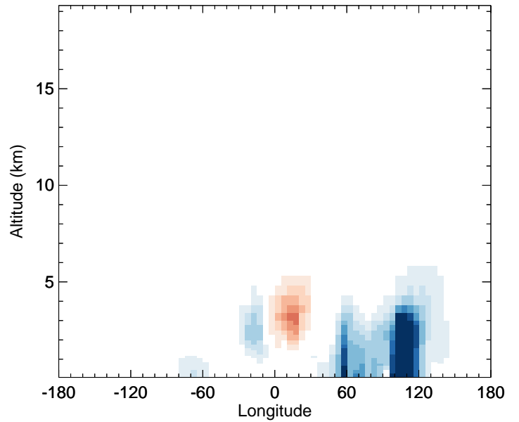
v11-02f-Run1 - v11-02e-Run0 DST1 - Diff along 42N for Jul
