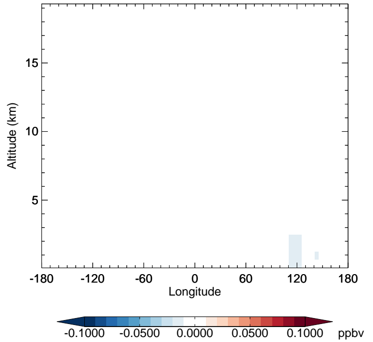
v11-02f-Run1 - v11-02e-Run0 SOAME - Diff along 42N for Jul
