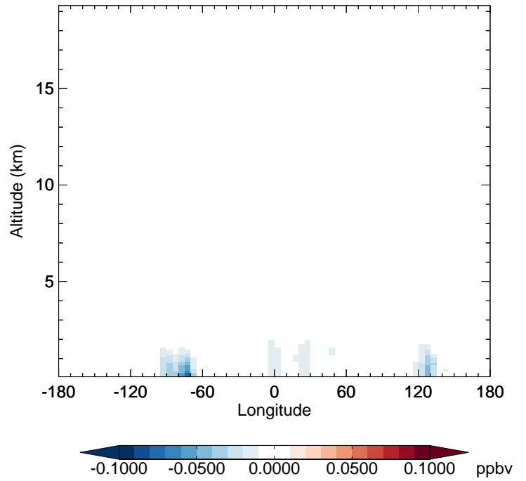
v11-02f-Run1 - v11-02e-Run0 IPMN - Diff along 42N for Jul
