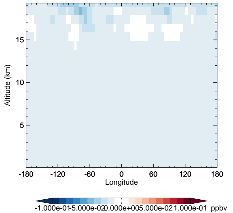
v11-02f-Run1 - v11-02e-Run0 CFC12 - Diff along 42N for Jul
