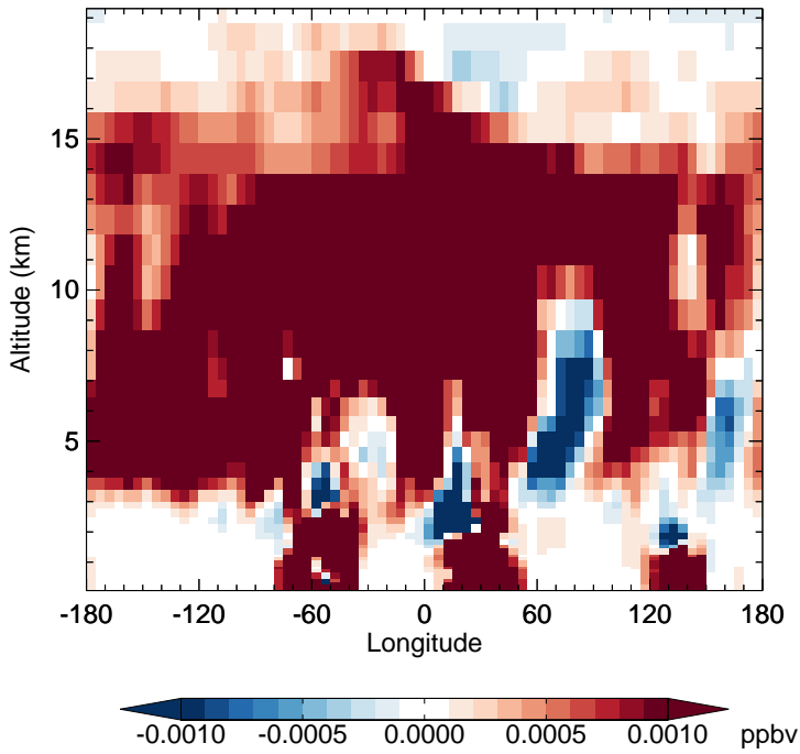
v11-02f-Run1 - v11-02e-Run0 PPN - Diff along 15S for Jul
