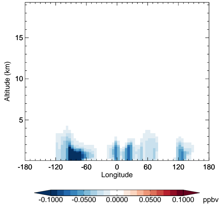
v11-02f-Run1 - v11-02e-Run0 ISO3 - Diff along 42N for Jul
