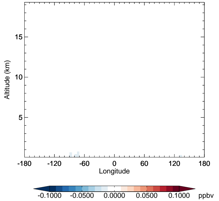
v11-02f-Run1 - v11-02e-Run1 HPALD - Diff along 42N for Jul
