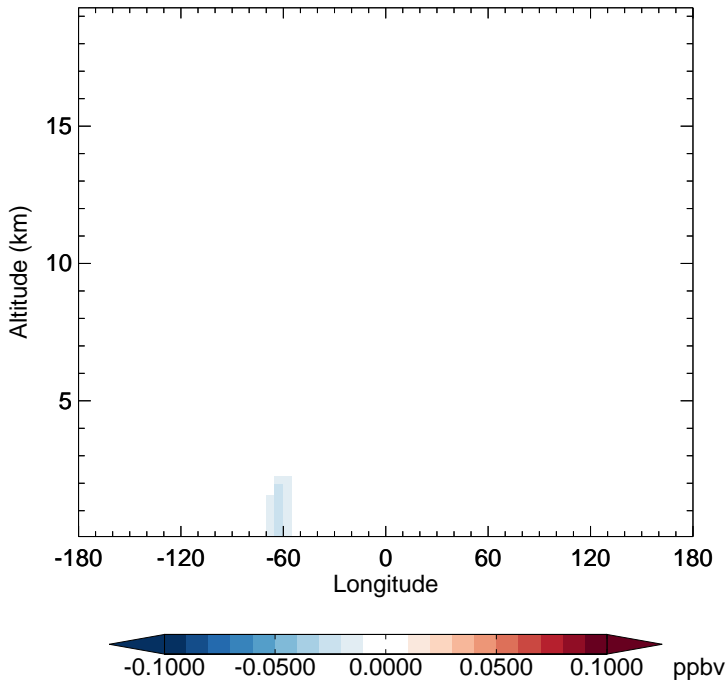
v11-02f-Run1 - v11-02e-Run1 RIPD - Diff along 15S for Jul
