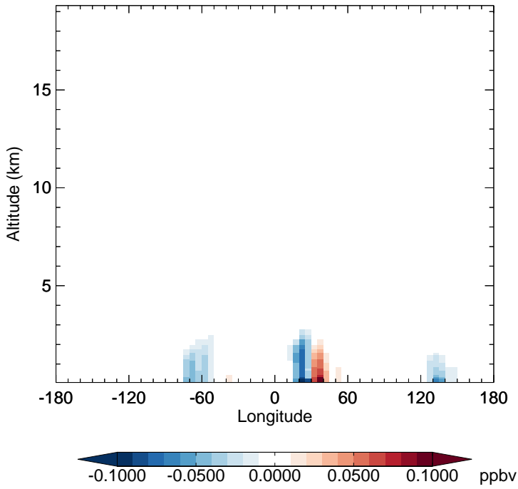
v11-02f-Run1 - v11-02e-Run1 TOLU - Diff along 15S for Jul
