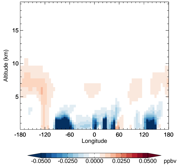
v11-02f-Run1 - v11-02e-Run1 MP - Diff along 42N for Jul
