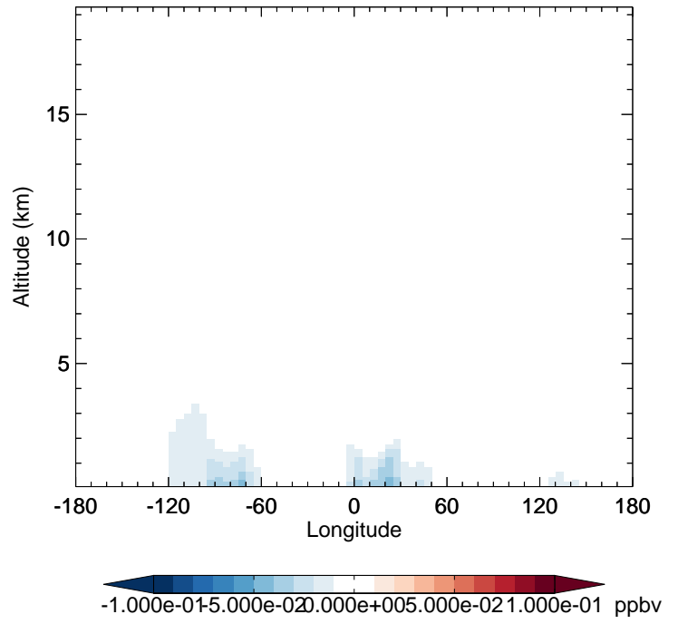
v11-02f-Run1 - v11-02e-Run1 MONITA - Diff along 42N for Jul
