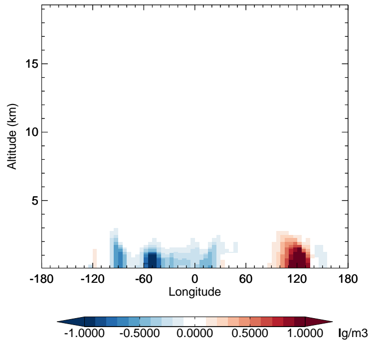
v11-02f-Run1 - v11-02e-Run0 OCPI - Diff along 42N for Jul
