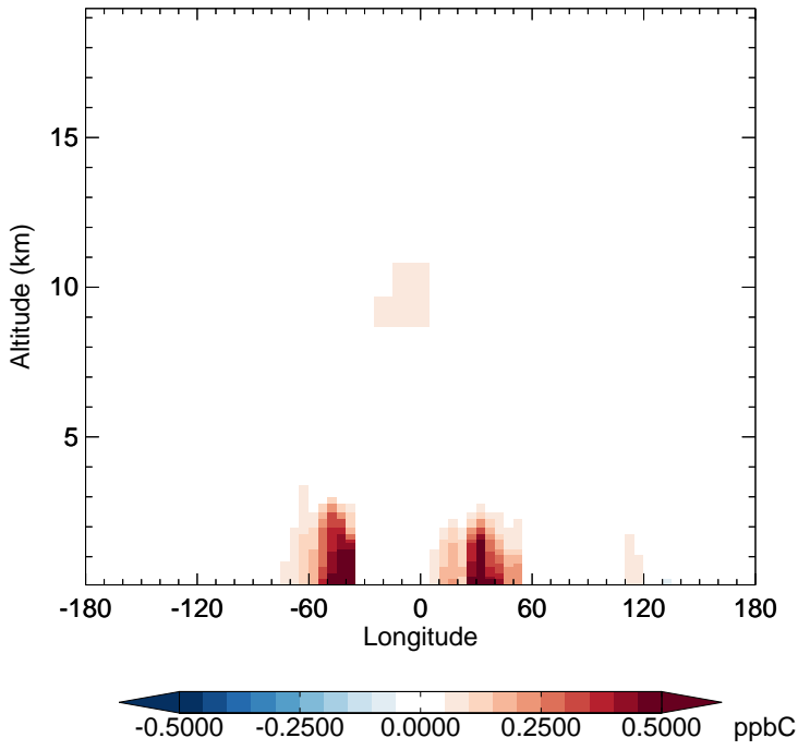
v11-02f-Run1 - v11-02e-Run1 ALK4 - Diff along 15S for Jul
