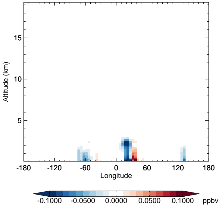
v11-02f-Run1 - v11-02e-Run0 TOLU - Diff along 15S for Jul
