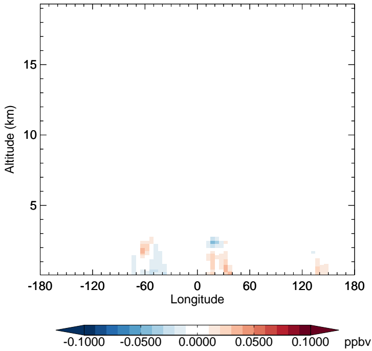
v11-02f-Run1 - v11-02e-Run0 SOAP - Diff along 15S for Jul
