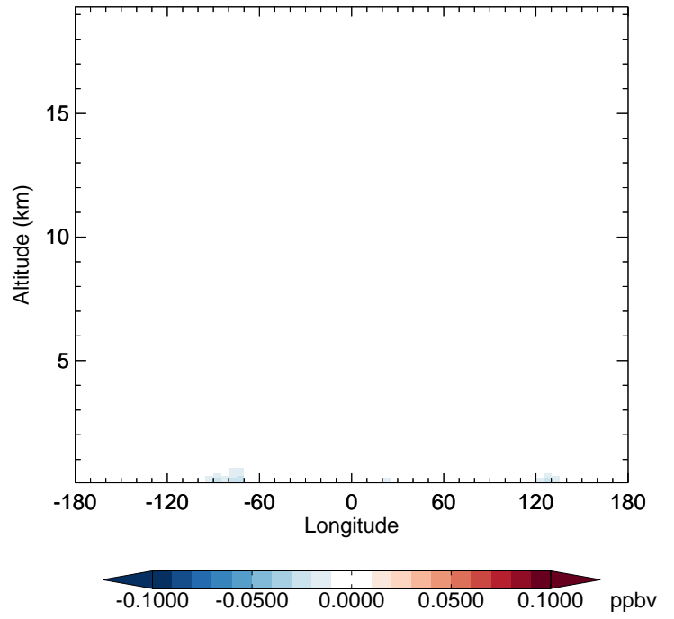
v11-02f-Run1 - v11-02e-Run1 ISN1 - Diff along 42N for Jul
