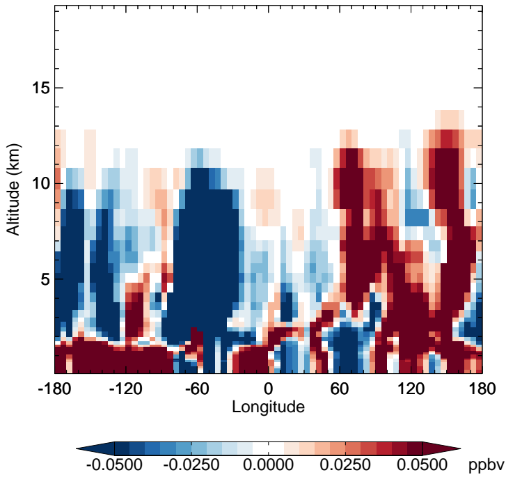
v11-02f-Run1 - v11-02e-Run0 MP - Diff along 15S for Jul
