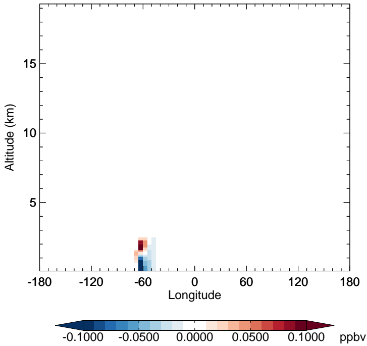
v11-02f-Run1 - v11-02e-Run0 HPALD - Diff along 15S for Jul
