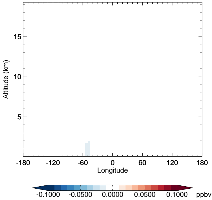
v11-02f-Run1 - v11-02e-Run1 GLYX - Diff along 15S for Jul
