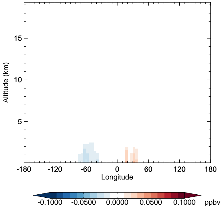
v11-02f-Run1 - v11-02e-Run1 SOAP - Diff along 15S for Jul
