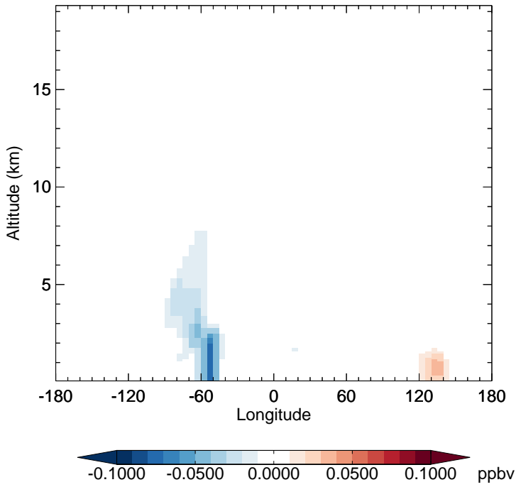
v11-02f-Run1 - v11-02e-Run1 IMAE - Diff along 15S for Jul
