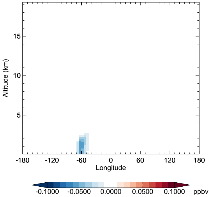
v11-02f-Run1 - v11-02e-Run1 ISOA1 - Diff along 15S for Jul
