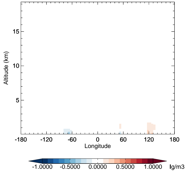
v11-02f-Run1 - v11-02e-Run1 SO 2 - Diff along 42N for Jul
