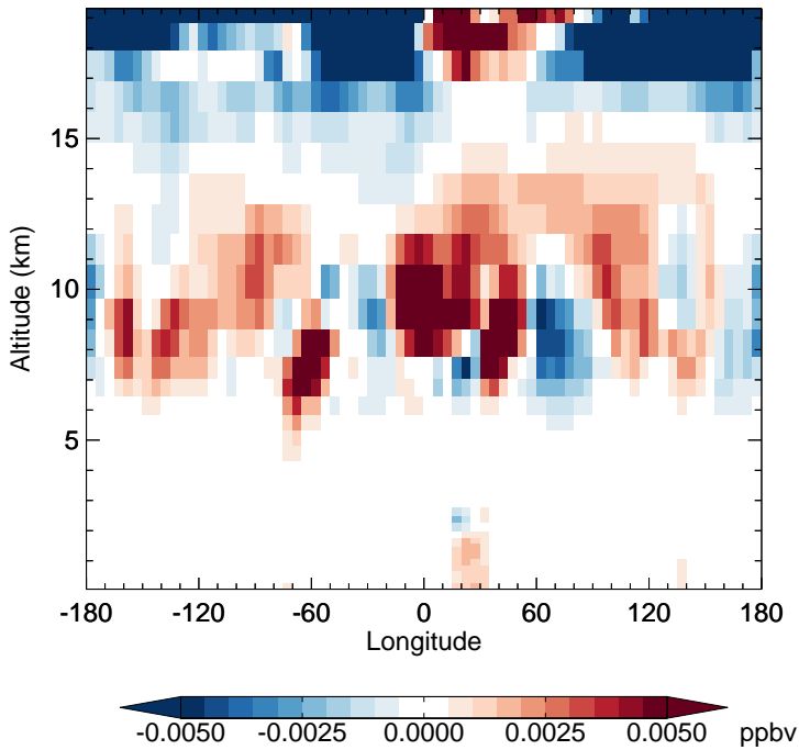
v11-02f-Run1 - v11-02e-Run0 HNO 4 - Diff along 15S for Jul
