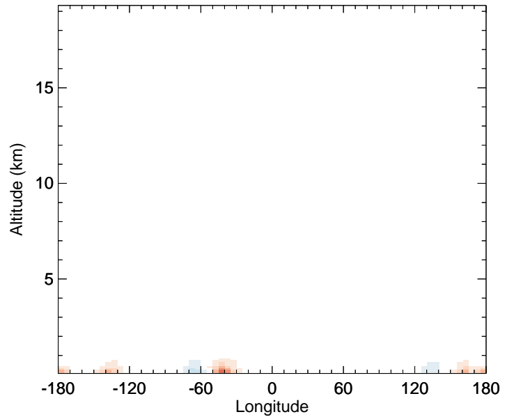
v11-02f-Run1 - v11-02e-Run0 SALA - Diff along 42N for Jul
