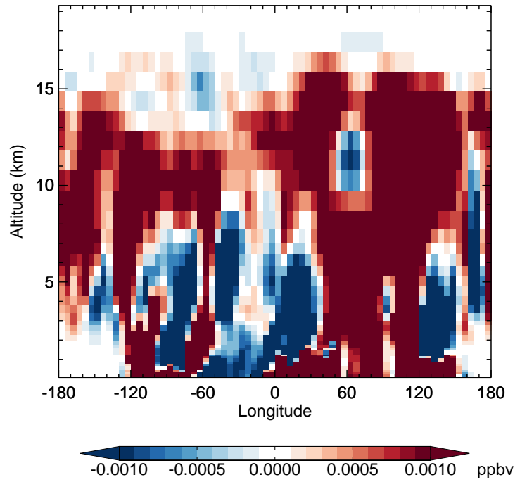
v11-02f-Run1 - v11-02e-Run0 PPN - Diff along 42N for Jul
