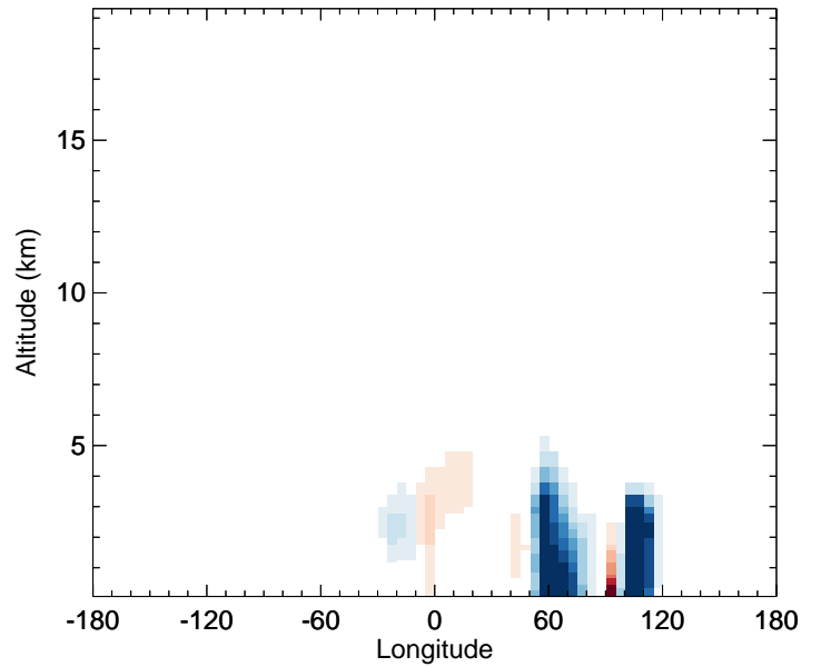
v11-02f-Run1 - v11-02e-Run0 DST2 - Diff along 42N for Jul
