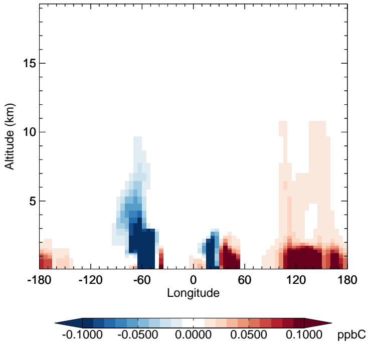
v11-02f-Run1 - v11-02e-Run1 MEK - Diff along 15S for Jul
