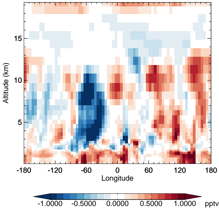
v11-02f-Run1 - v11-02e-Run0 HO2 - Diff along 15S for Jul
