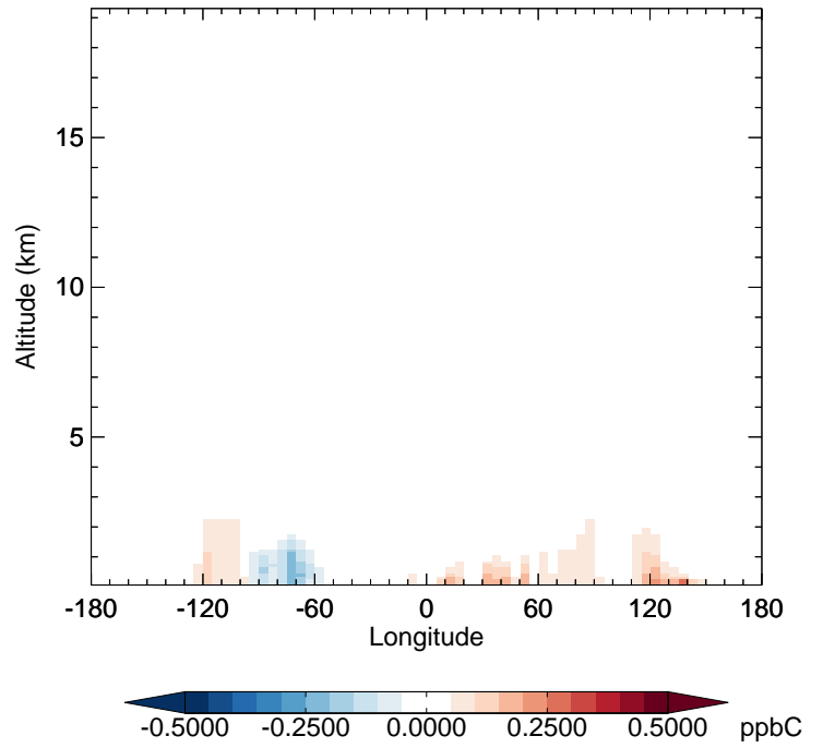
v11-02f-Run1 - v11-02e-Run1 ALD2 - Diff along 42N for Jul
