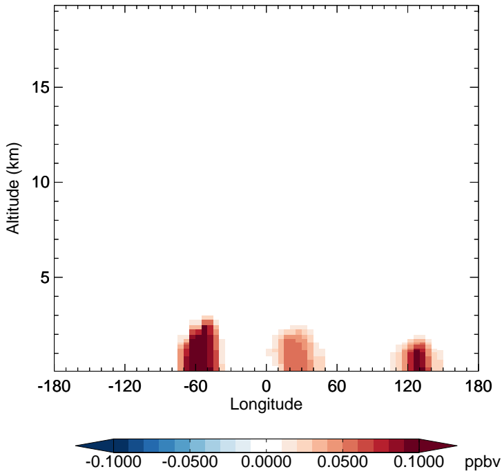
v11-02f-Run1 - v11-02e-Run1 INDIOL - Diff along 15S for Jul
