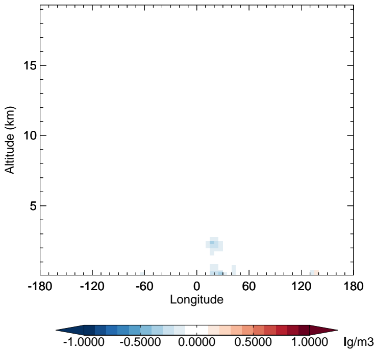
v11-02f-Run1 - v11-02e-Run0 OCPO - Diff along 15S for Jul
