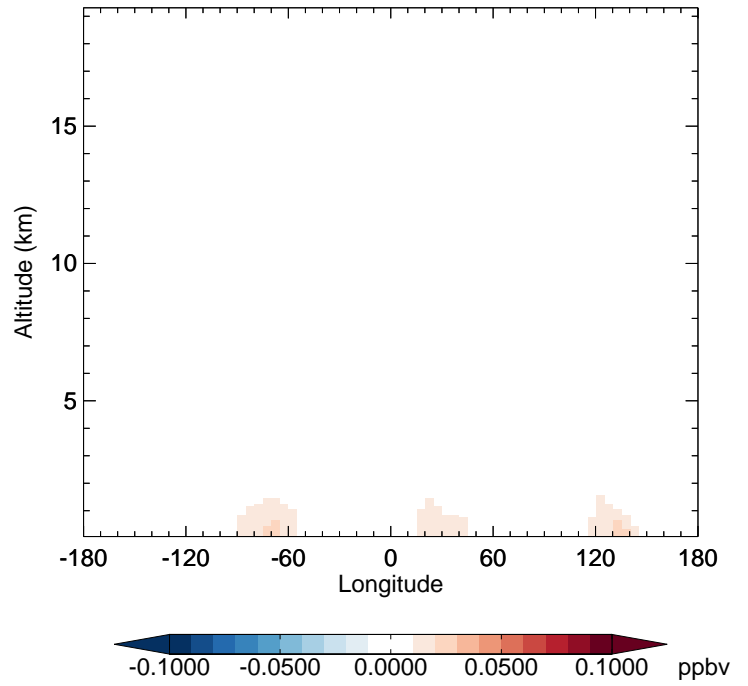
v11-02f-Run1 - v11-02e-Run1 TSOA0 - Diff along 42N for Jul
