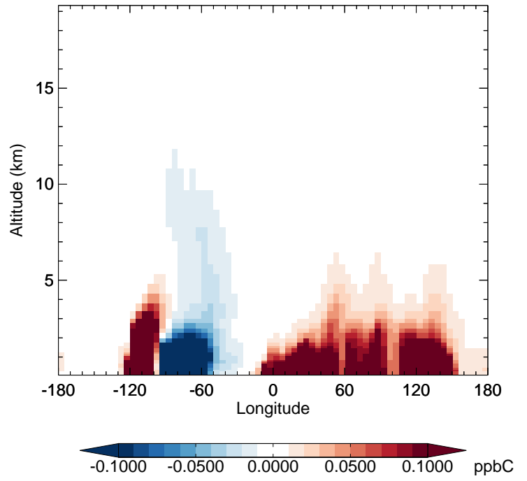
v11-02f-Run1 - v11-02e-Run1 MEK - Diff along 42N for Jul
