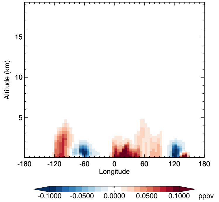
v11-02f-Run1 - v11-02e-Run1 INDIOL - Diff along 42N for Jul
