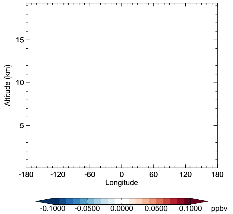
v11-02f-Run1 - v11-02e-Run0 ClNO 2 - Diff along 42N for Jul
