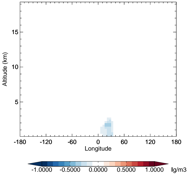
v11-02f-Run1 - v11-02e-Run1 NH4 - Diff along 15S for Jul
