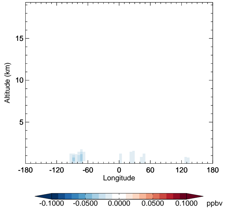
v11-02f-Run1 - v11-02e-Run1 IEPOXB - Diff along 42N for Jul
