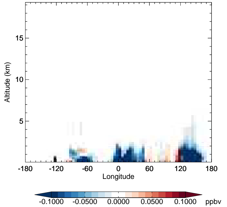
v11-02f-Run1 - v11-02e-Run0 TOLU - Diff along 42N for Jul
