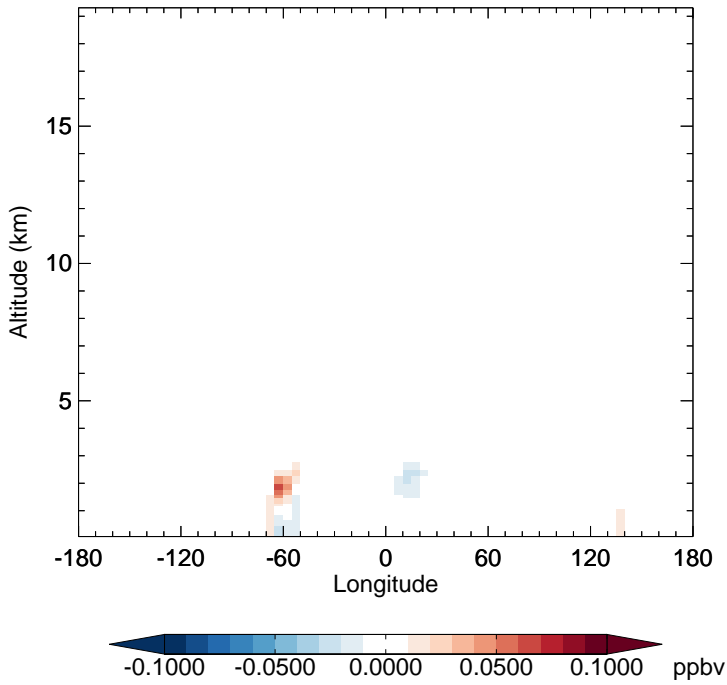
v11-02f-Run1 - v11-02e-Run0 ISOA1 - Diff along 15S for Jul
