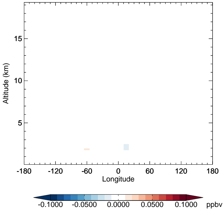
v11-02f-Run1 - v11-02e-Run0 ISOA3 - Diff along 15S for Jul
