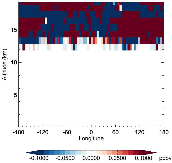
v11-02f-Run1 - v11-02e-Run1 H2O - Diff along 15S for Jul
