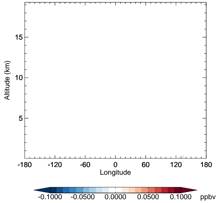
v11-02f-Run1 - v11-02e-Run1 TSOA1 - Diff along 42N for Jul
