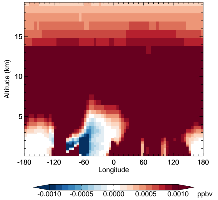
v11-02f-Run1 - v11-02e-Run1 PPN - Diff along 42N for Jul
