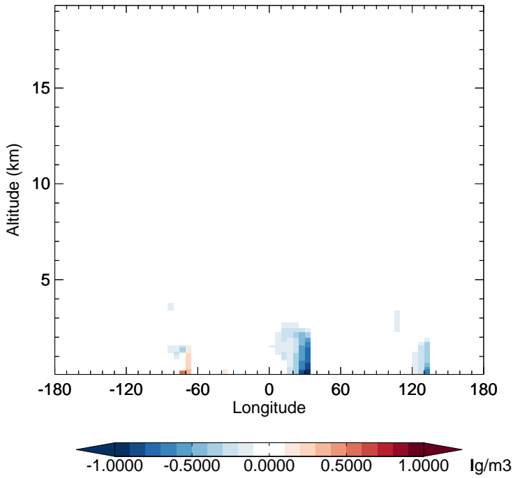
v11-02f-Run1 - v11-02e-Run0 SO 2 - Diff along 15S for Jul
