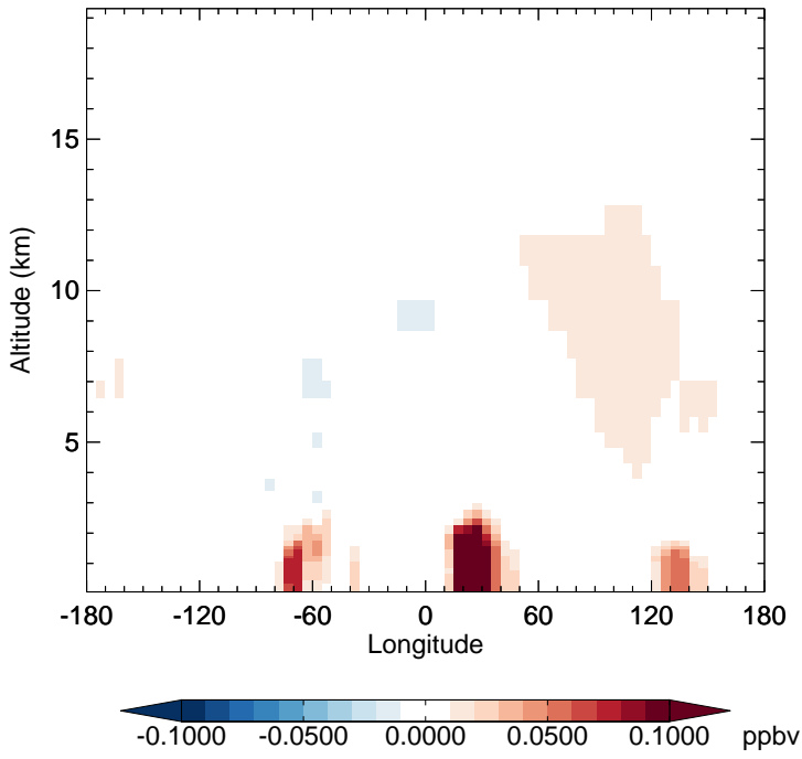
v11-02f-Run1 - v11-02e-Run1 PAN - Diff along 15S for Jul
