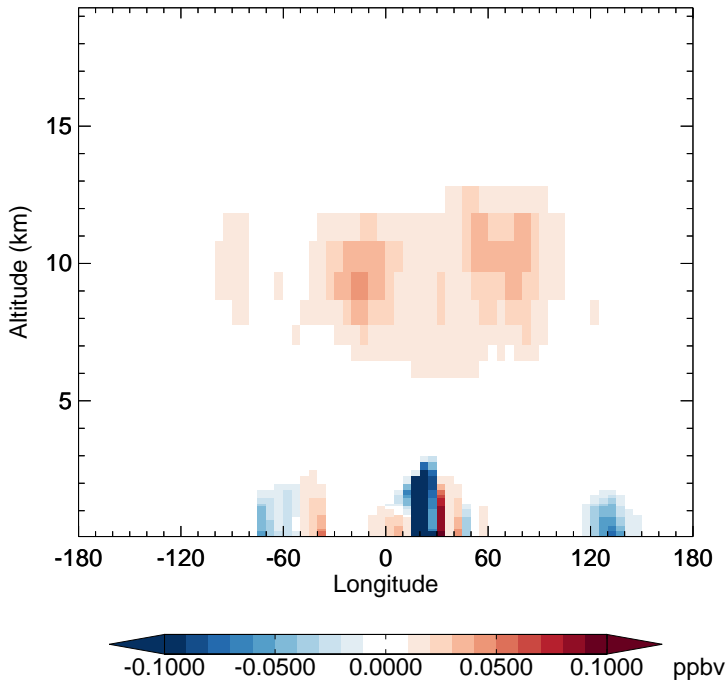
v11-02f-Run1 - v11-02e-Run1 BENZ - Diff along 15S for Jul
