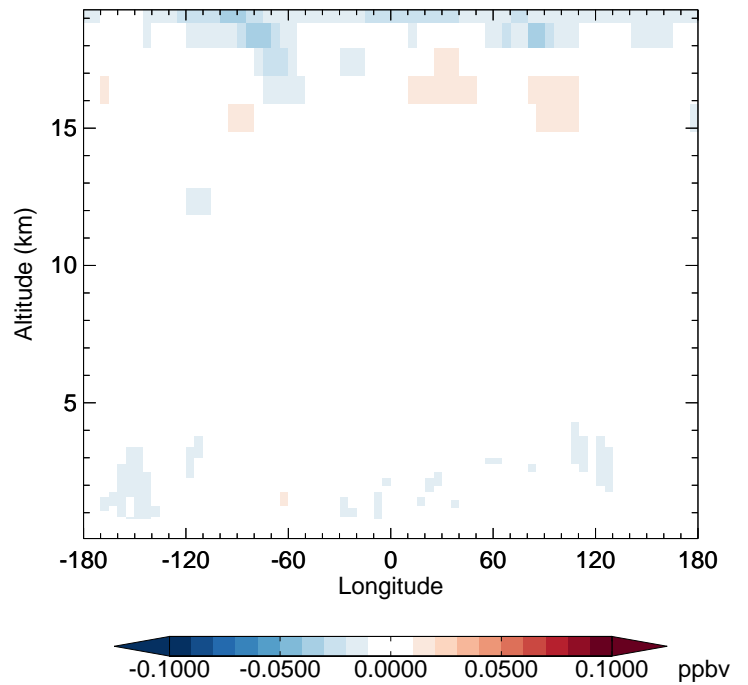
v11-02f-Run1 - v11-02e-Run0 CH3Cl - Diff along 42N for Jul
