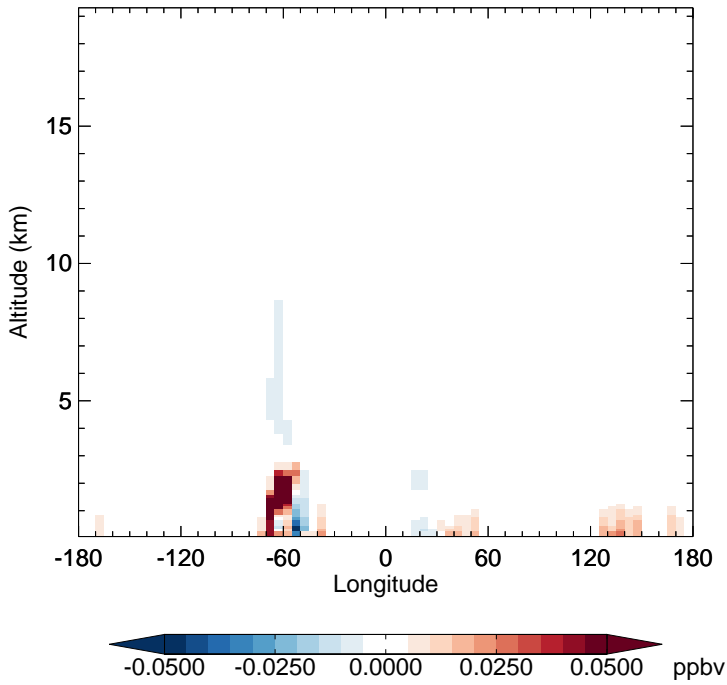
v11-02f-Run1 - v11-02e-Run0 RCHO - Diff along 15S for Jul
