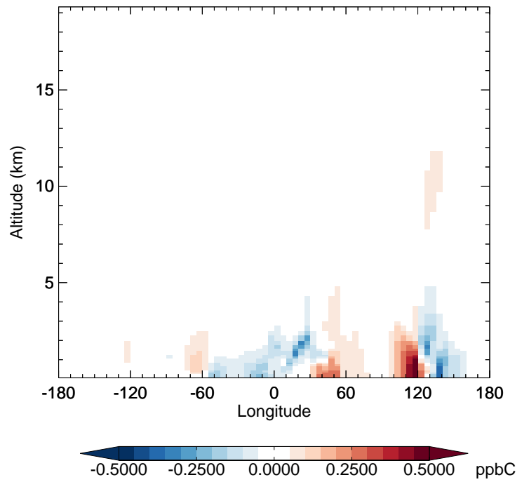
v11-02f-Run1 - v11-02e-Run0 C3H8 - Diff along 42N for Jul
