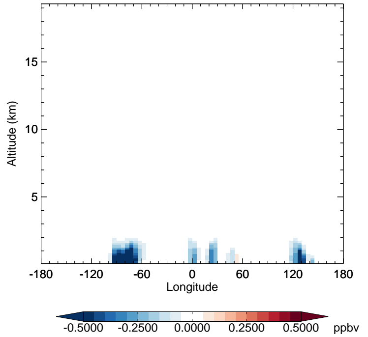
v11-02f-Run1 - v11-02e-Run1 CH 2 O - Diff along 42N for Jul
