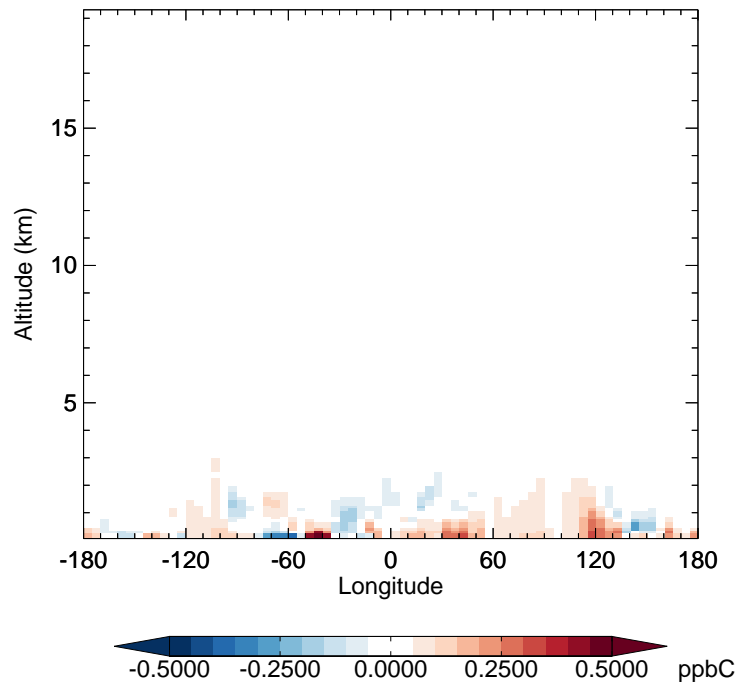
v11-02f-Run1 - v11-02e-Run0 ALD2 - Diff along 42N for Jul
