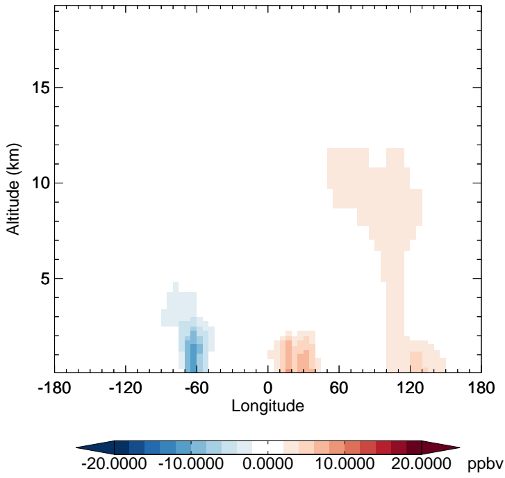
v11-02f-Run1 - v11-02e-Run1 CO - Diff along 15S for Jul
