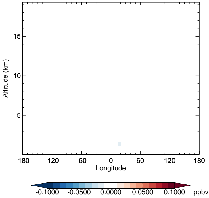
v11-02f-Run1 - v11-02e-Run1 SOAGX - Diff along 15S for Jul
