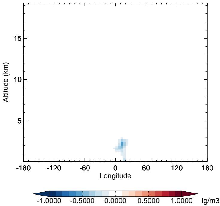
v11-02f-Run1 - v11-02e-Run0 BCPI - Diff along 15S for Jul
