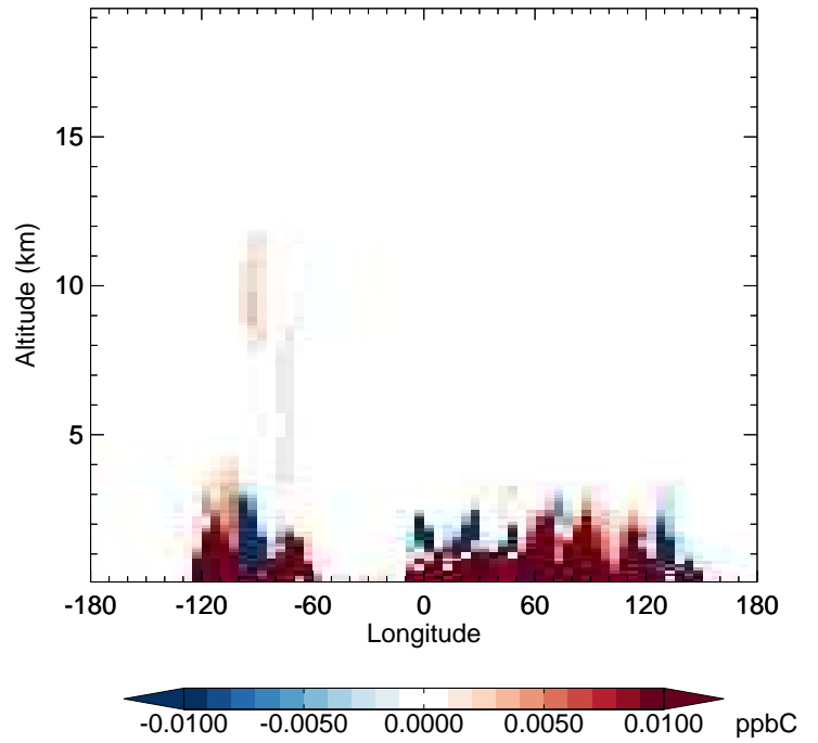
v11-02f-Run1 - v11-02e-Run0 PRPE - Diff along 42N for Jul
