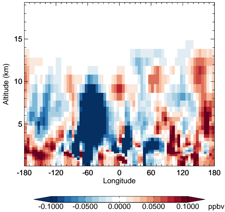
v11-02f-Run1 - v11-02e-Run0 H2O2 - Diff along 15S for Jul
