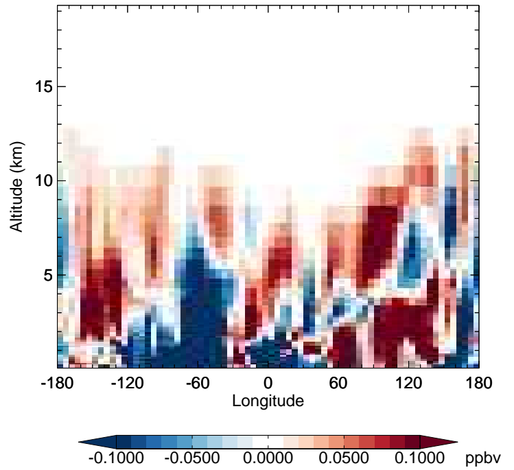
v11-02f-Run1 - v11-02e-Run0 H2O2 - Diff along 42N for Jul
