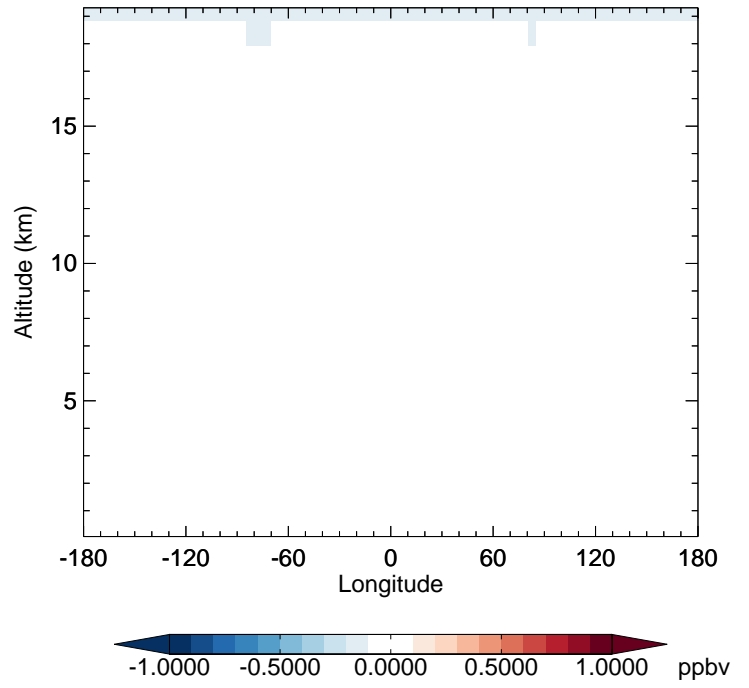
v11-02f-Run1 - v11-02e-Run1 NO - Diff along 42N for Jul
