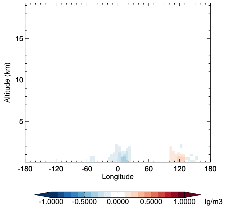
v11-02f-Run1 - v11-02e-Run0 BCPI - Diff along 42N for Jul
