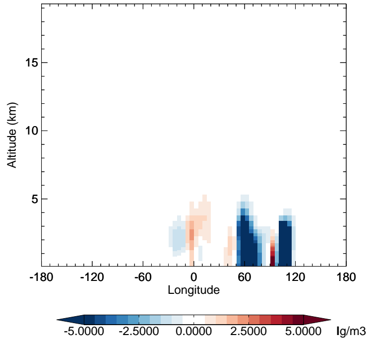
v11-02f-Run1 - v11-02e-Run0 DST3 - Diff along 42N for Jul
