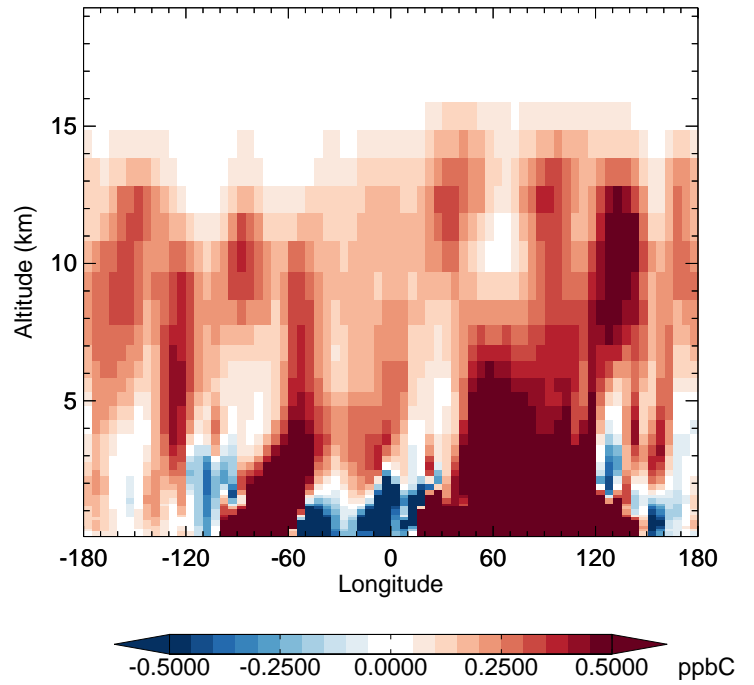
v11-02f-Run1 - v11-02e-Run0 ACET - Diff along 42N for Jul
