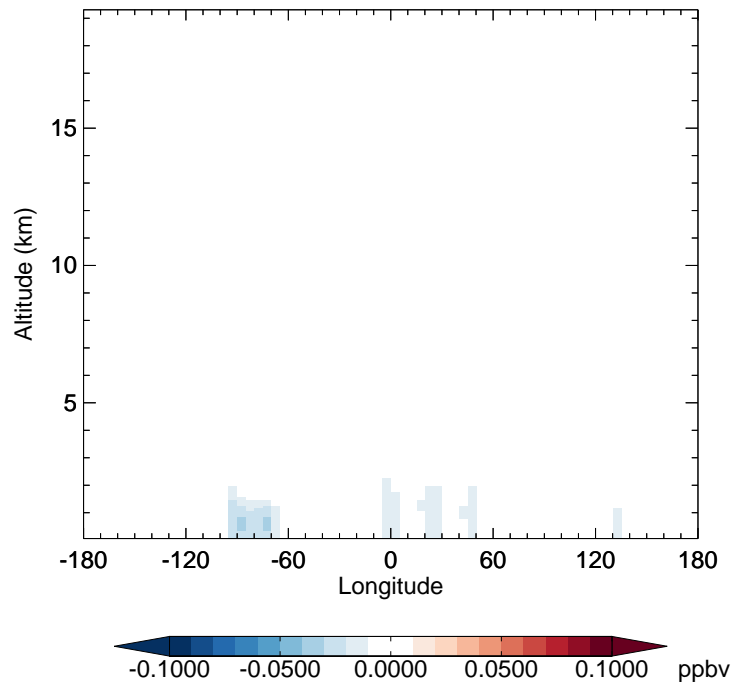
v11-02f-Run1 - v11-02e-Run0 HC187 - Diff along 42N for Jul
