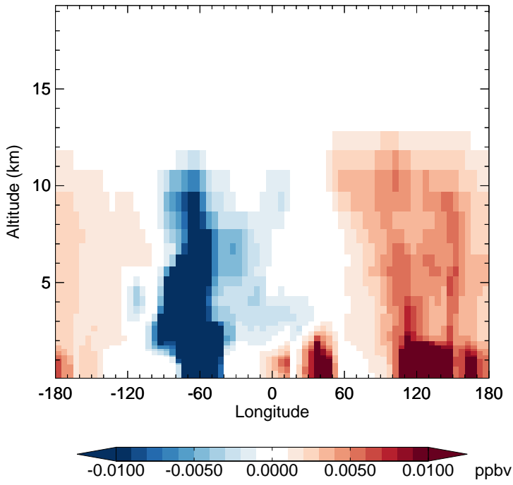
v11-02f-Run1 - v11-02e-Run1 MAP - Diff along 15S for Jul
