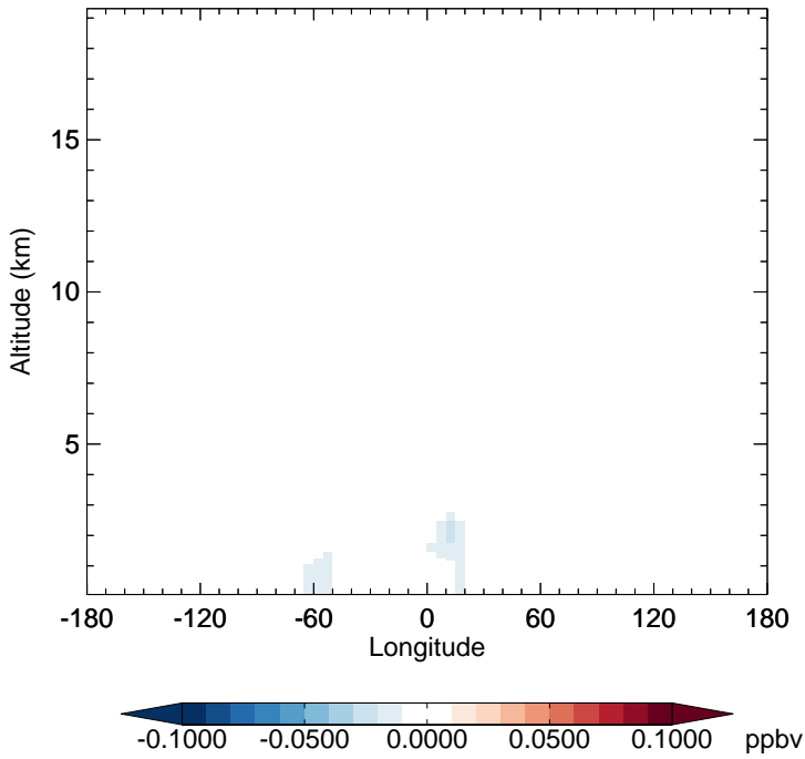
v11-02f-Run1 - v11-02e-Run0 SOAGX - Diff along 15S for Jul
