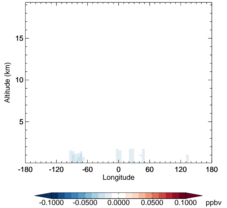
v11-02f-Run1 - v11-02e-Run0 IEPOXB - Diff along 42N for Jul
