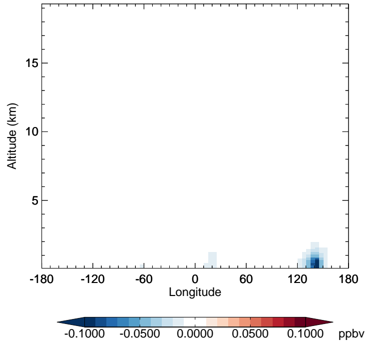
v11-02f-Run1 - v11-02e-Run1 ASOAN - Diff along 42N for Jul
