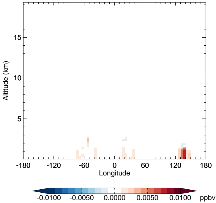
v11-02f-Run1 - v11-02e-Run0 MVKN - Diff along 15S for Jul
