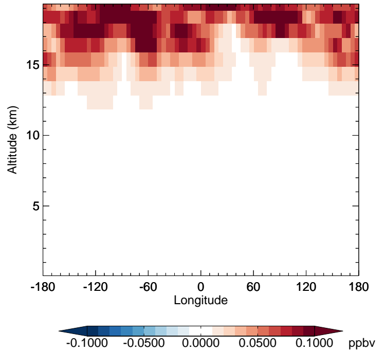
v11-02f-Run1 - v11-02e-Run0 HCl - Diff along 42N for Jul
