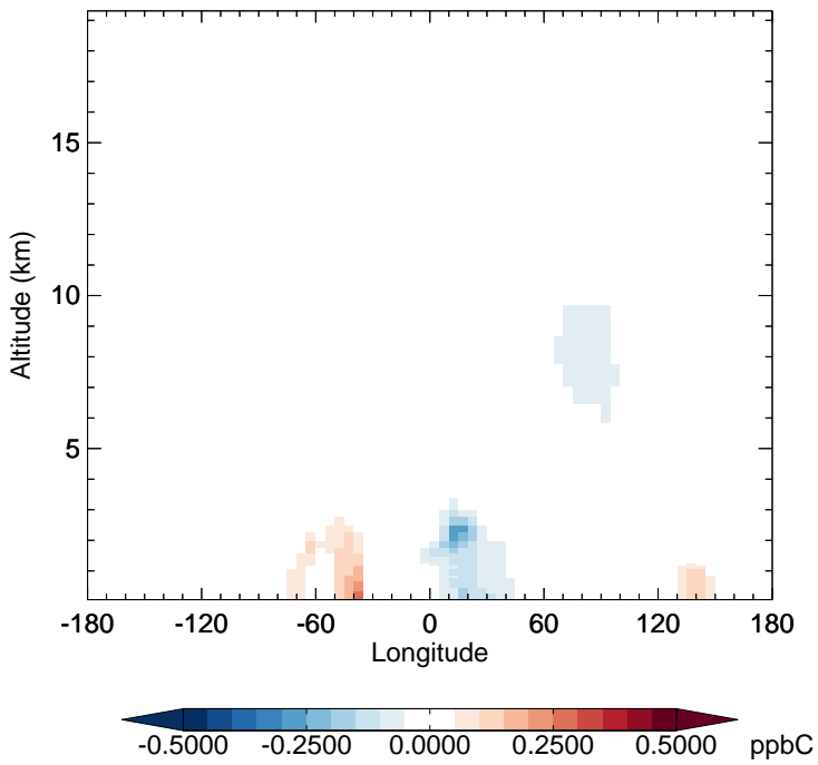
v11-02f-Run1 - v11-02e-Run0 C3H8 - Diff along 15S for Jul
