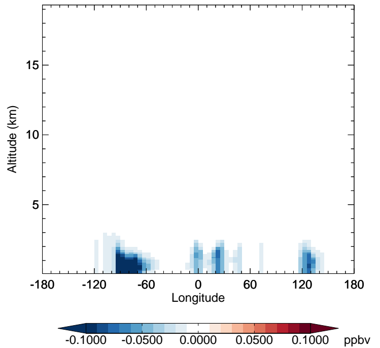
v11-02f-Run1 - v11-02e-Run0 IMAE - Diff along 42N for Jul
