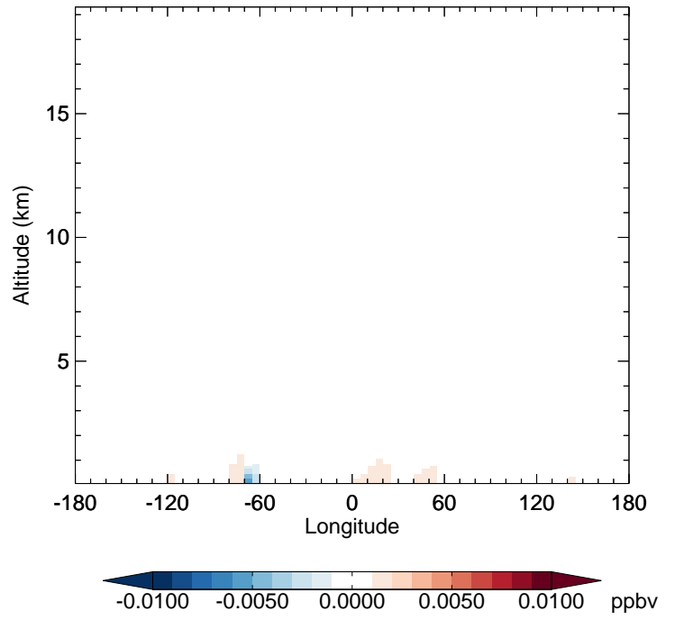
v11-02f-Run1 - v11-02e-Run1 R4N2 - Diff along 42N for Jul
