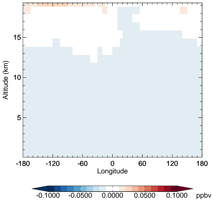
v11-02f-Run1 - v11-02e-Run0 CFC11 - Diff along 15S for Jul
