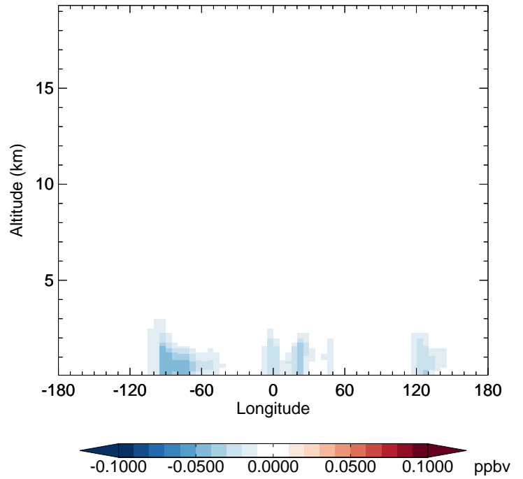
v11-02f-Run1 - v11-02e-Run0 ISOA1 - Diff along 42N for Jul
