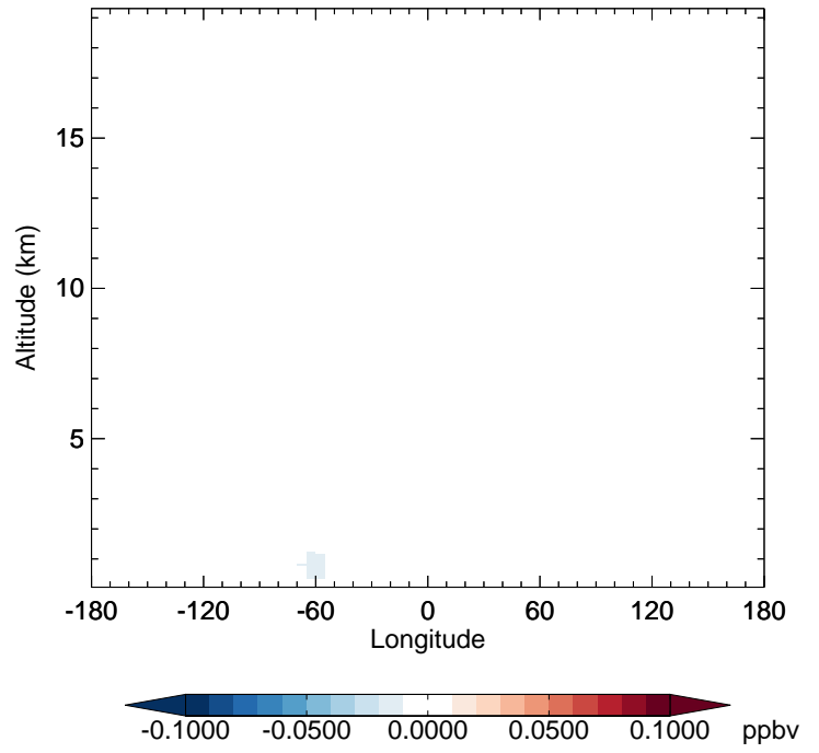
v11-02f-Run1 - v11-02e-Run1 SOAME - Diff along 42N for Jul
