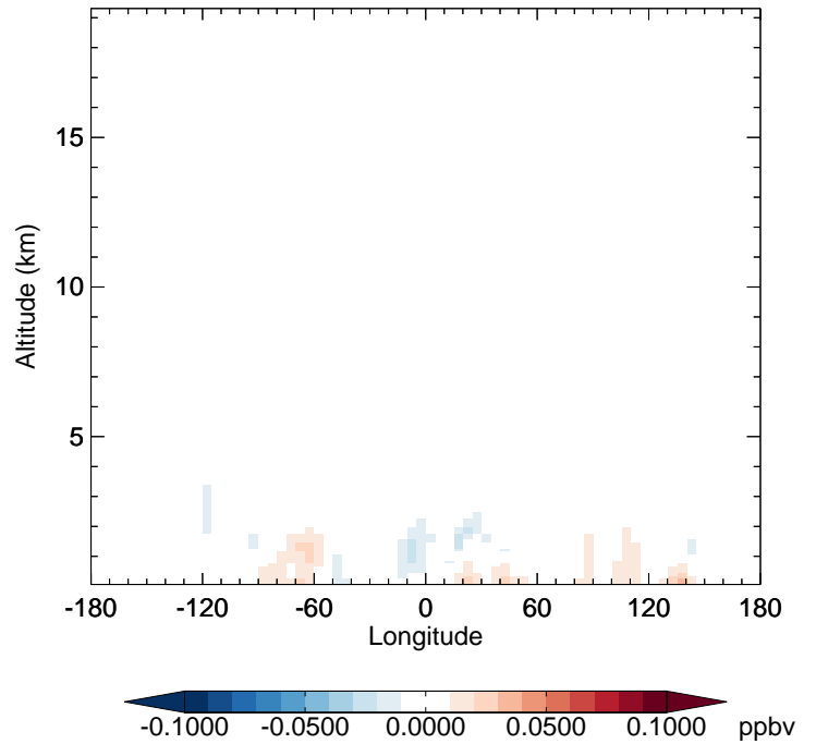
v11-02f-Run1 - v11-02e-Run0 TSOG2 - Diff along 42N for Jul
