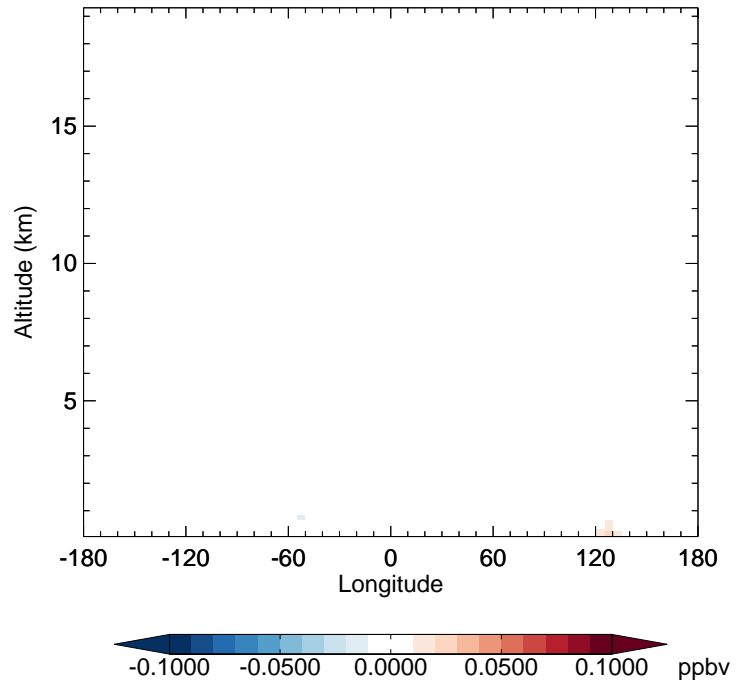
v11-02f-Run1 - v11-02e-Run0 TSOA3 - Diff along 42N for Jul
