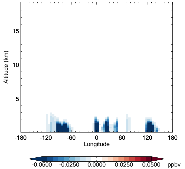
v11-02f-Run1 - v11-02e-Run0 MVK - Diff along 42N for Jul
