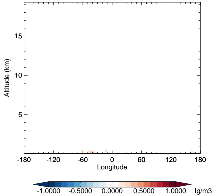
v11-02f-Run1 - v11-02e-Run0 DMS - Diff along 42N for Jul
