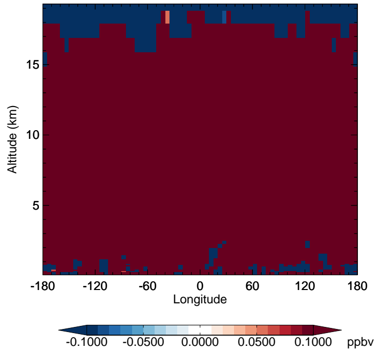
v11-02f-Run1 - v11-02e-Run0 CH4 - Diff along 42N for Jul
