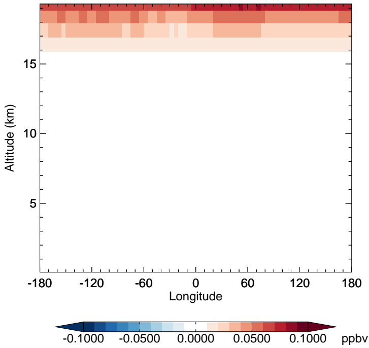
v11-02f-Run1 - v11-02e-Run1 N2O - Diff along 15S for Jul
