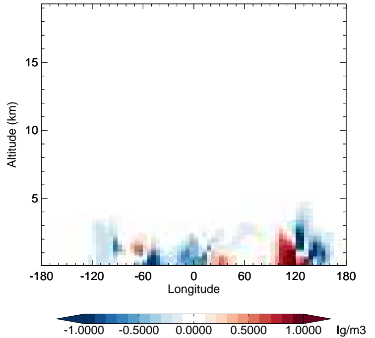
v11-02f-Run1 - v11-02e-Run0 SOAS - Diff along 42N for Jul
