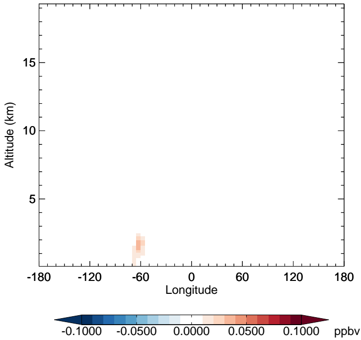
v11-02f-Run1 - v11-02e-Run0 TSOA1 - Diff along 15S for Jul
