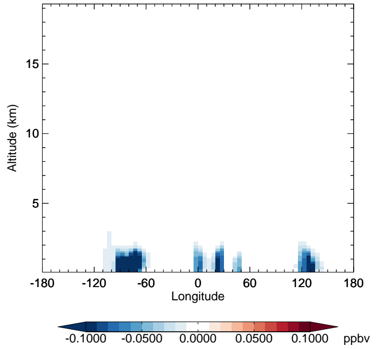
v11-02f-Run1 - v11-02e-Run1 HAC - Diff along 42N for Jul
