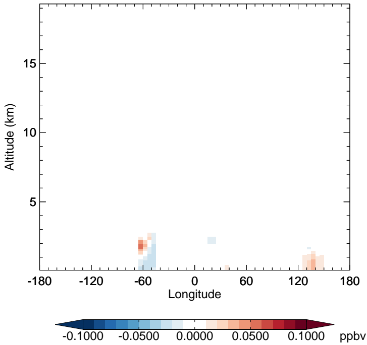
v11-02f-Run1 - v11-02e-Run0 MGLY - Diff along 15S for Jul
