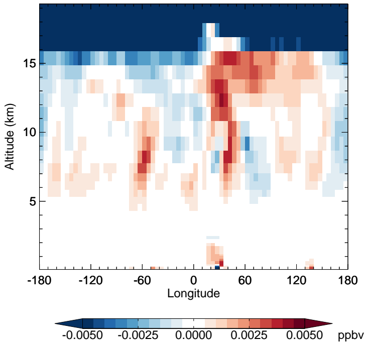
v11-02f-Run1 - v11-02e-Run0 N2O5 - Diff along 15S for Jul
