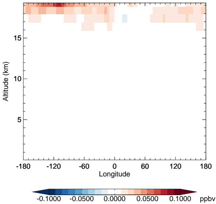
v11-02f-Run1 - v11-02e-Run0 OCS - Diff along 15S for Jul
