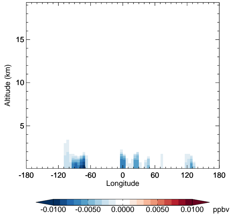
v11-02f-Run1 - v11-02e-Run1 MVKN - Diff along 42N for Jul
