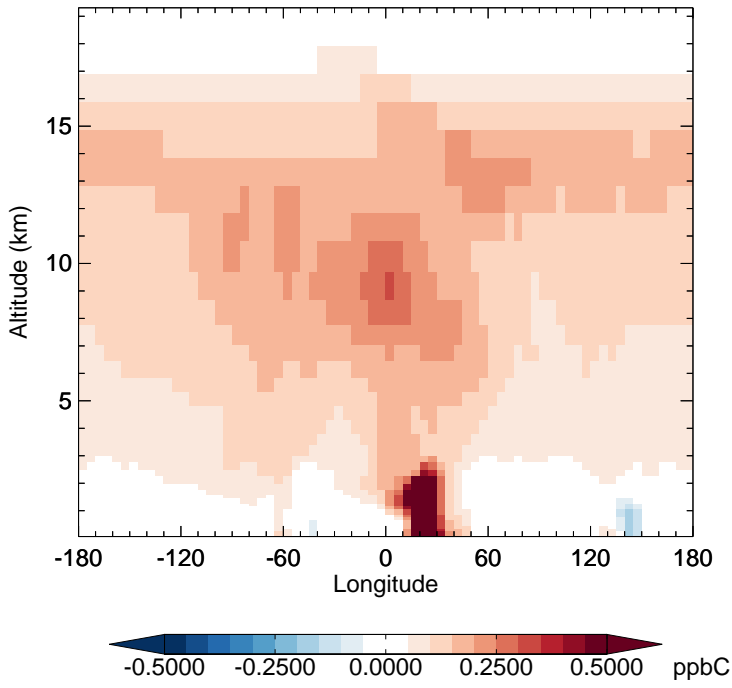
v11-02f-Run1 - v11-02e-Run1 C2H6 - Diff along 15S for Jul
