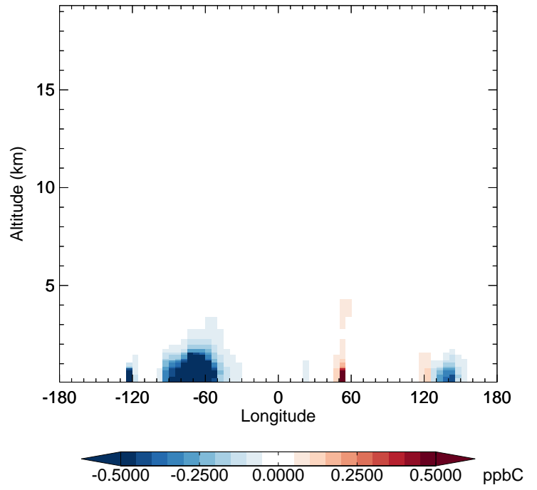
v11-02f-Run1 - v11-02e-Run1 ALK4 - Diff along 42N for Jul
