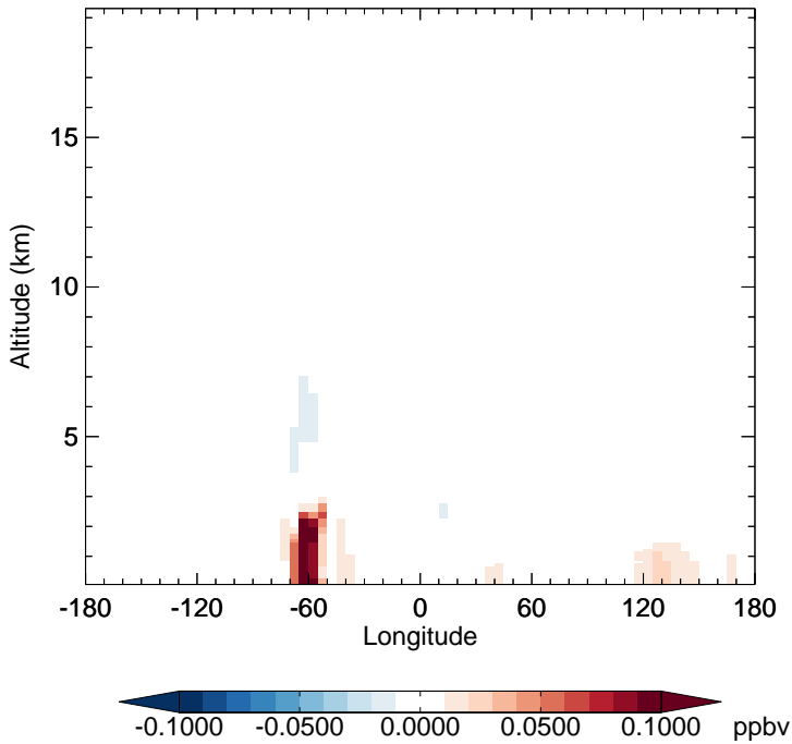
v11-02f-Run1 - v11-02e-Run0 TSOG2 - Diff along 15S for Jul
