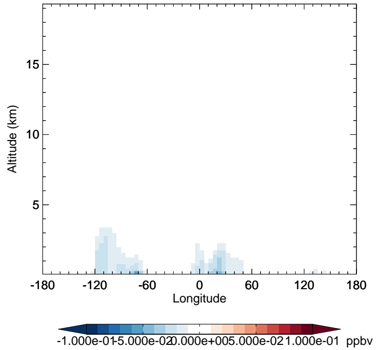
v11-02f-Run1 - v11-02e-Run0 MONITA - Diff along 42N for Jul
