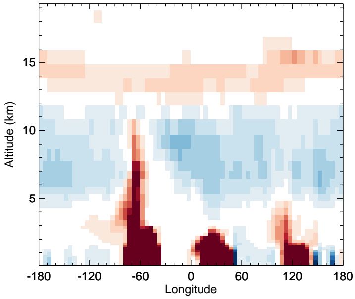
v11-02f-Run1 - v11-02e-Run1 OH - Diff along 15S for Jul
