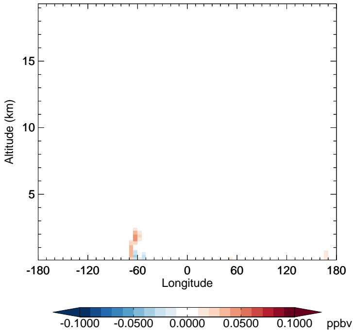
v11-02f-Run1 - v11-02e-Run0 MTPA - Diff along 15S for Jul
