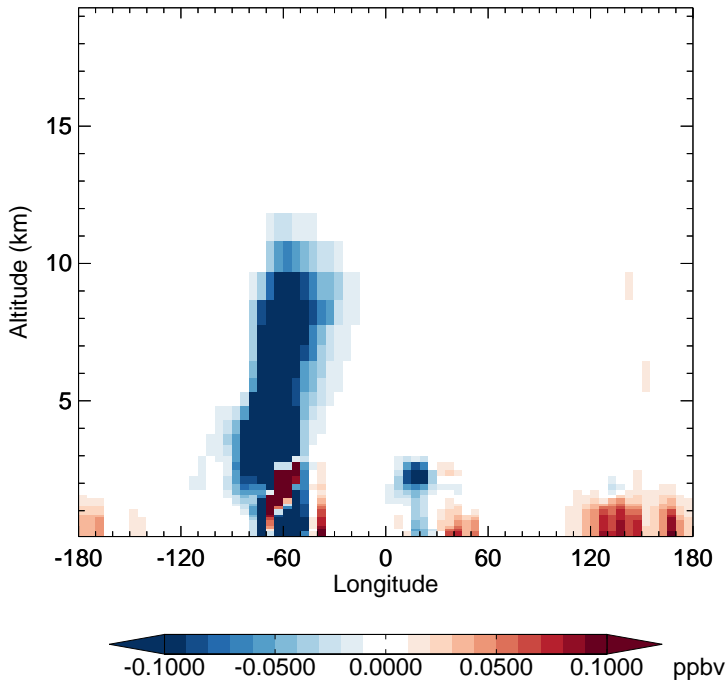
v11-02f-Run1 - v11-02e-Run0 EOH - Diff along 15S for Jul
