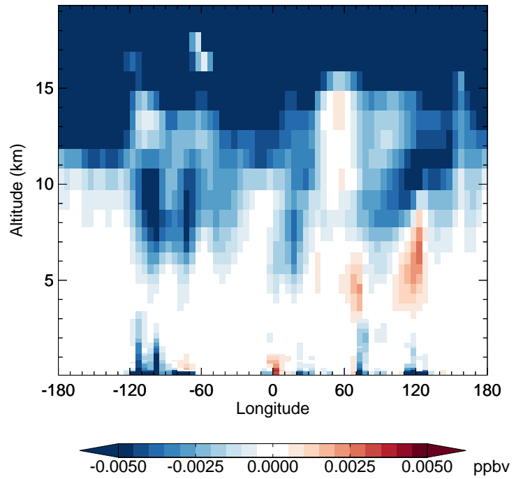
v11-02f-Run1 - v11-02e-Run0 N2O5 - Diff along 42N for Jul
