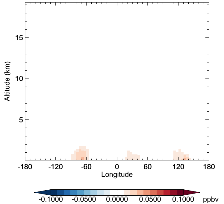
v11-02f-Run1 - v11-02e-Run0 TSOA0 - Diff along 42N for Jul
