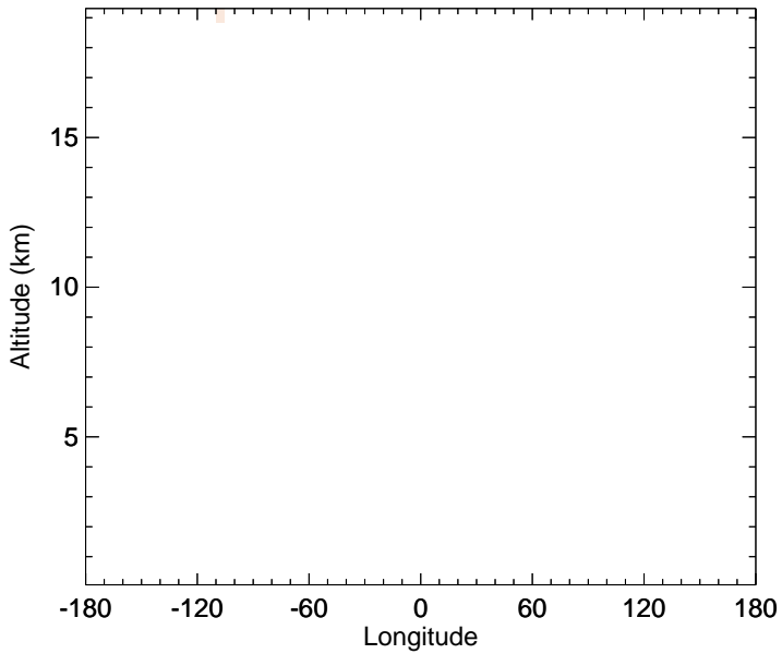
v11-02f-Run1 - v11-02e-Run0 CH3Br - Diff along 15S for Jul
