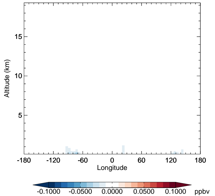
v11-02f-Run1 - v11-02e-Run0 GLYX - Diff along 42N for Jul
