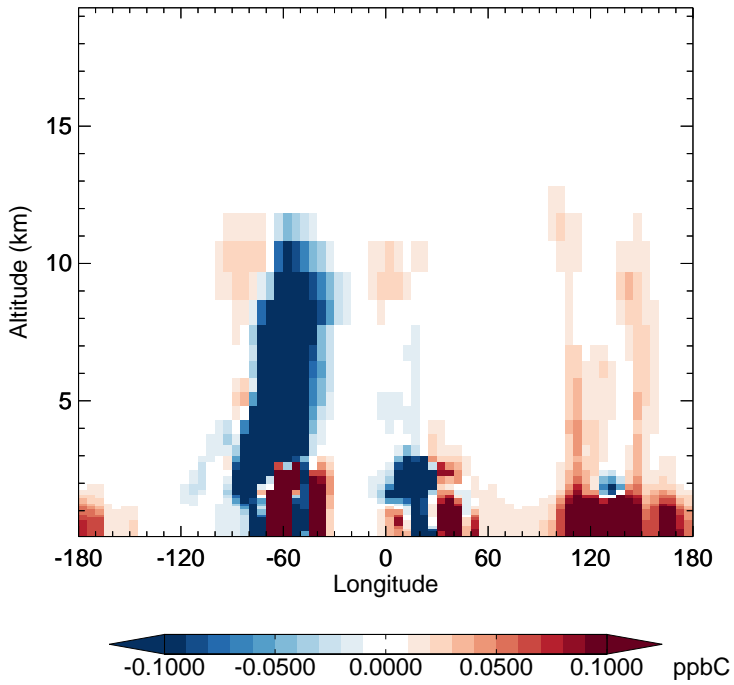
v11-02f-Run1 - v11-02e-Run0 MEK - Diff along 15S for Jul
