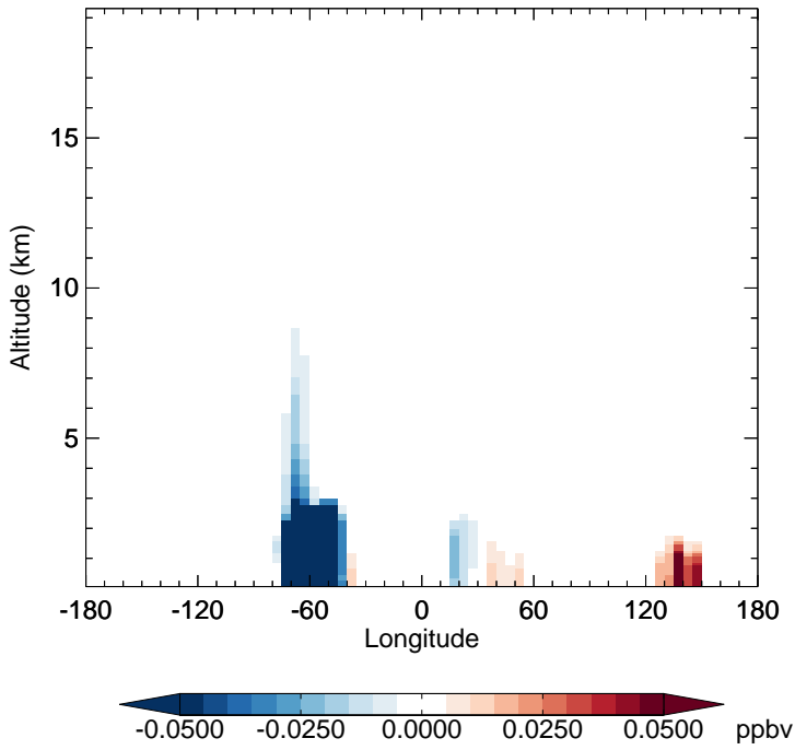
v11-02f-Run1 - v11-02e-Run1 MVK - Diff along 15S for Jul
