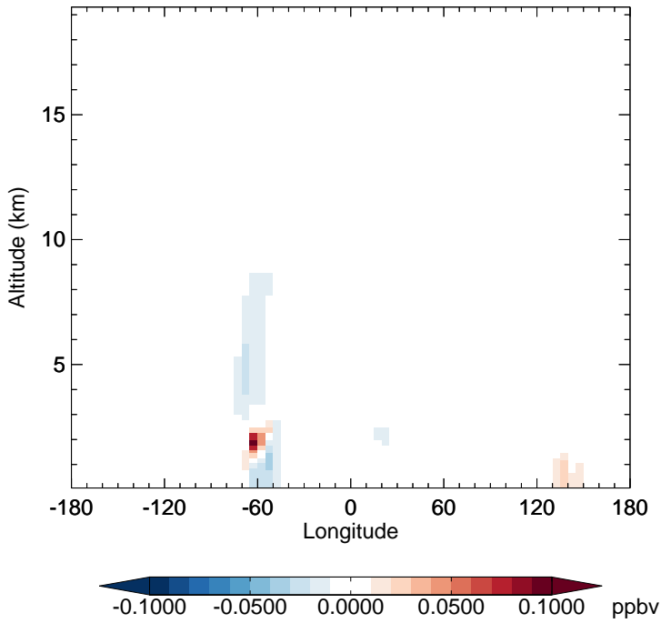
v11-02f-Run1 - v11-02e-Run0 IPMN - Diff along 15S for Jul
