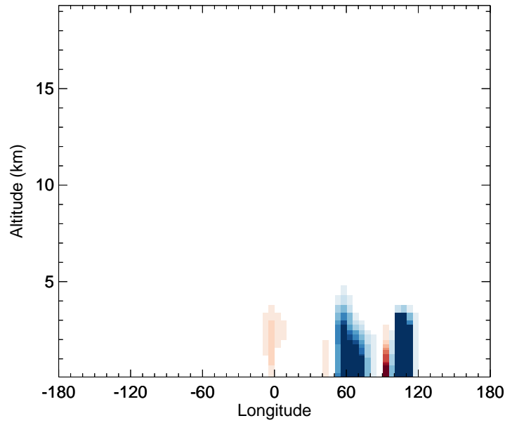
v11-02f-Run1 - v11-02e-Run0 DST4 - Diff along 42N for Jul
