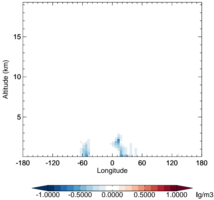
v11-02f-Run1 - v11-02e-Run0 NH3 - Diff along 15S for Jul
