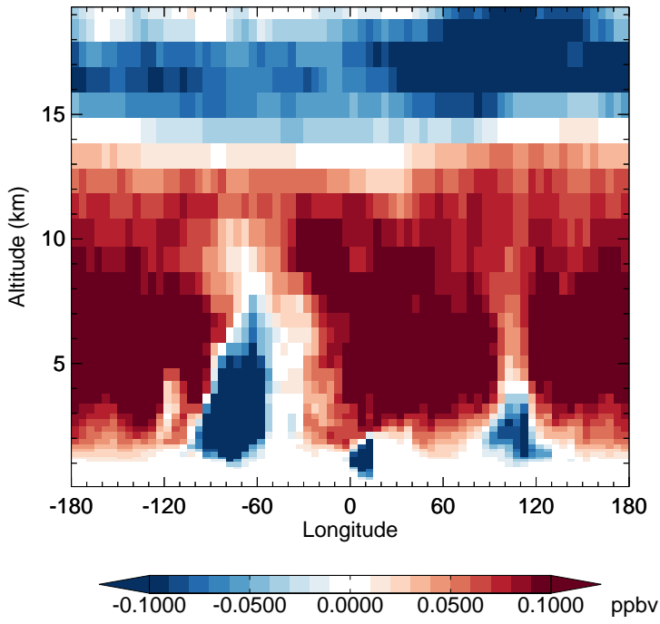
v11-02f-Run1 - v11-02e-Run1 CH4 - Diff along 15S for Jul
