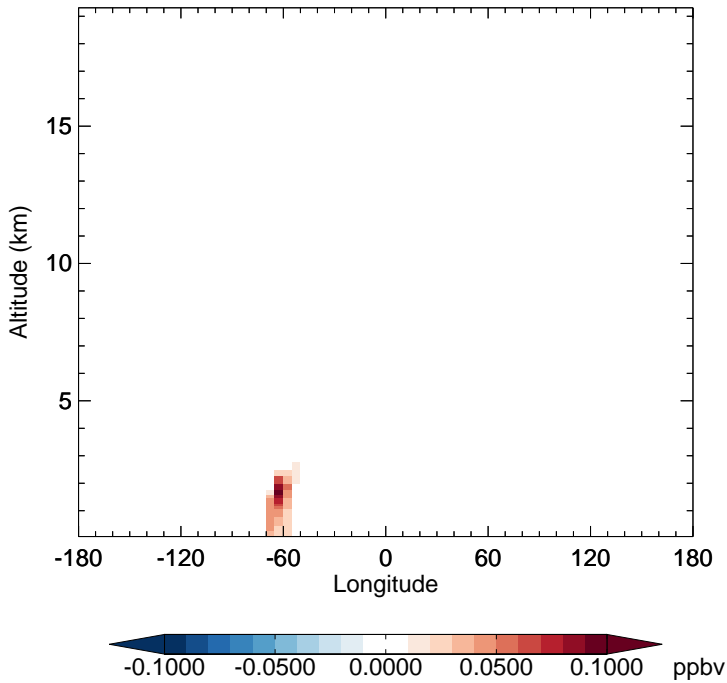
v11-02f-Run1 - v11-02e-Run0 TSOA0 - Diff along 15S for Jul
