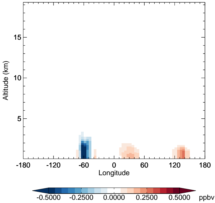
v11-02f-Run1 - v11-02e-Run1 CH 2 O - Diff along 15S for Jul
