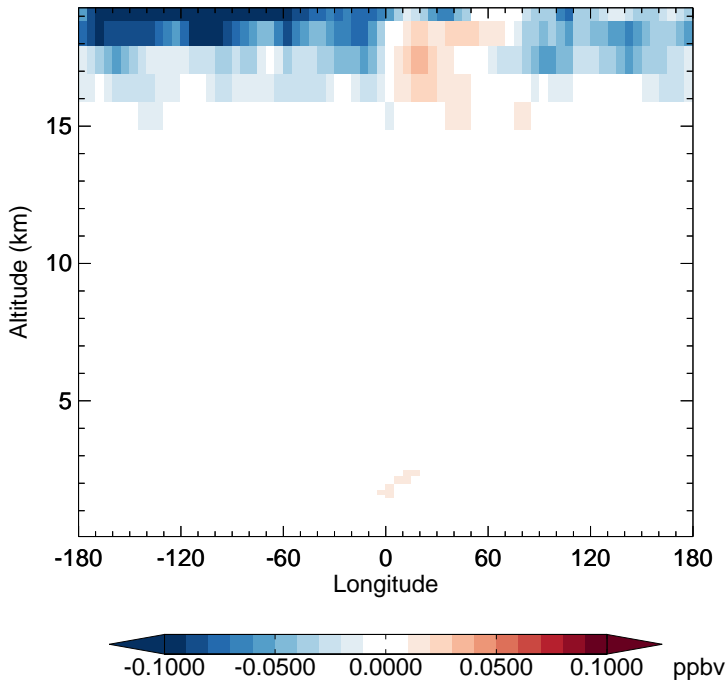
v11-02f-Run1 - v11-02e-Run0 HCl - Diff along 15S for Jul
