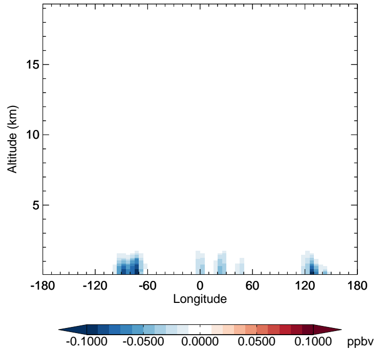
v11-02f-Run1 - v11-02e-Run1 MGLY - Diff along 42N for Jul
