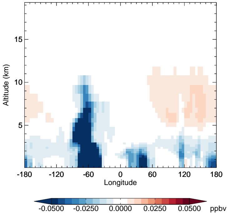
v11-02f-Run1 - v11-02e-Run1 MP - Diff along 15S for Jul
