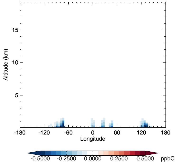
v11-02f-Run1 - v11-02e-Run1 ISOP - Diff along 42N for Jul
