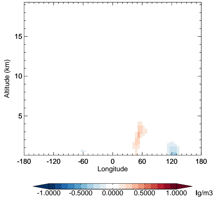
v11-02f-Run1 - v11-02e-Run1 SO4 - Diff along 42N for Jul
