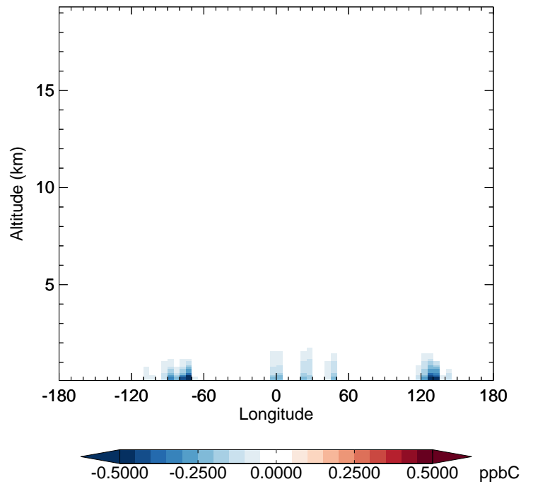
v11-02f-Run1 - v11-02e-Run0 ISOP - Diff along 42N for Jul
