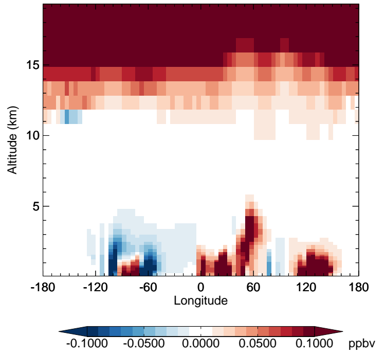
v11-02f-Run1 - v11-02e-Run1 HNO 3 - Diff along 42N for Jul
