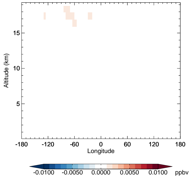
v11-02f-Run1 - v11-02e-Run0 BrNO 3 - Diff along 42N for Jul
