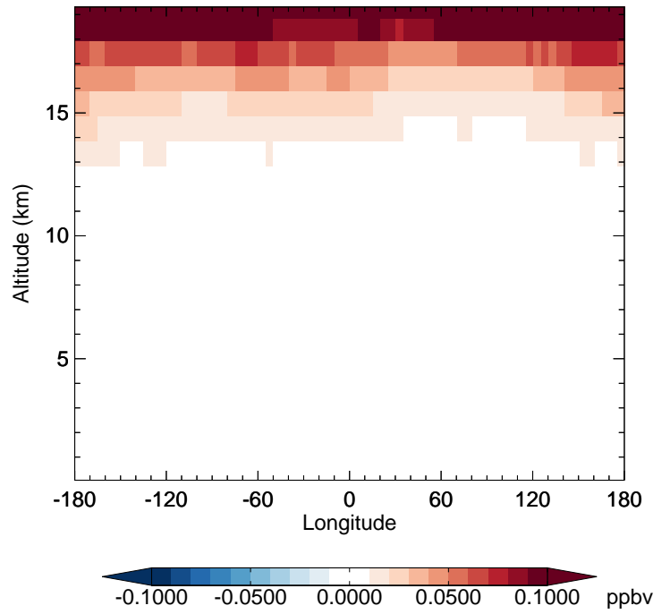
v11-02f-Run1 - v11-02e-Run1 N2O - Diff along 42N for Jul
