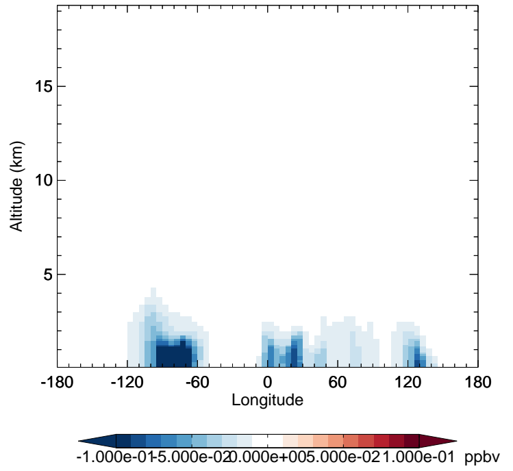
v11-02f-Run1 - v11-02e-Run1 IONITA - Diff along 42N for Jul
