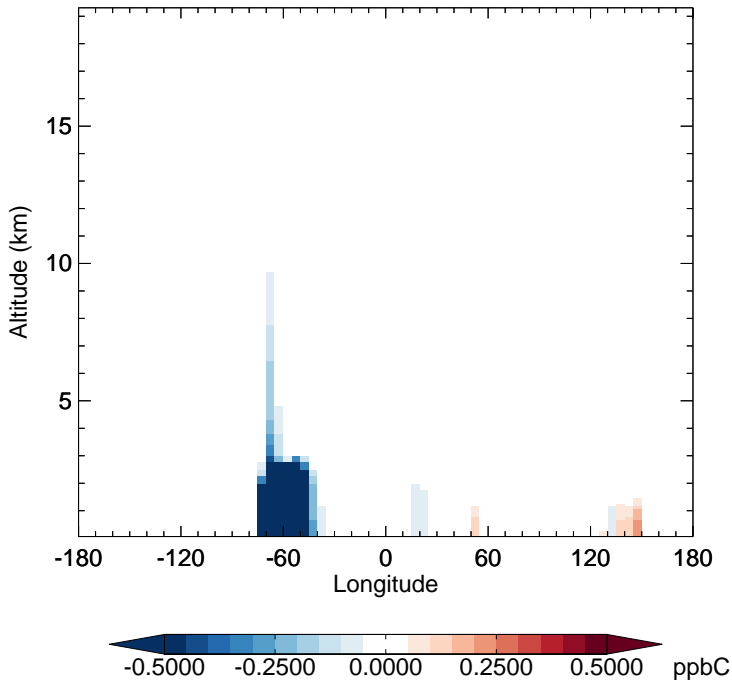
v11-02f-Run1 - v11-02e-Run1 ISOP - Diff along 15S for Jul
