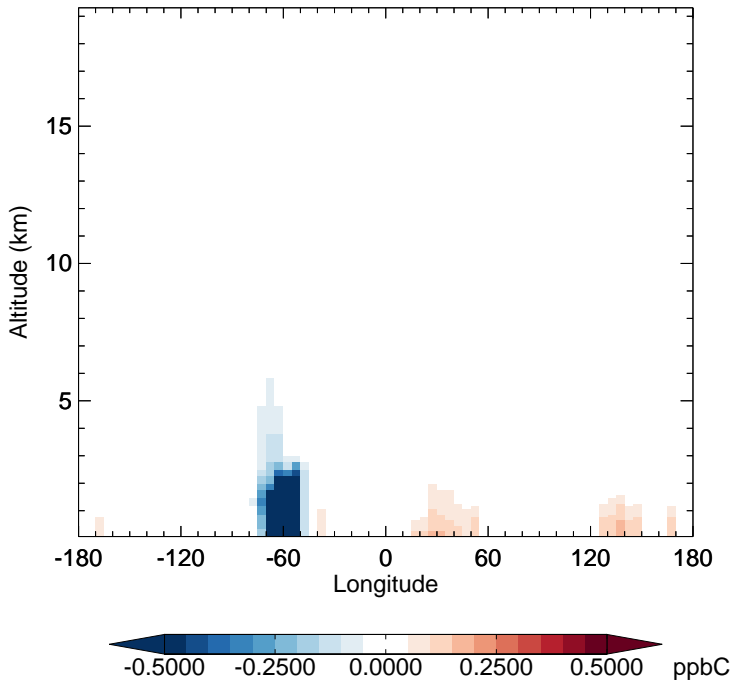
v11-02f-Run1 - v11-02e-Run1 ALD2 - Diff along 15S for Jul
