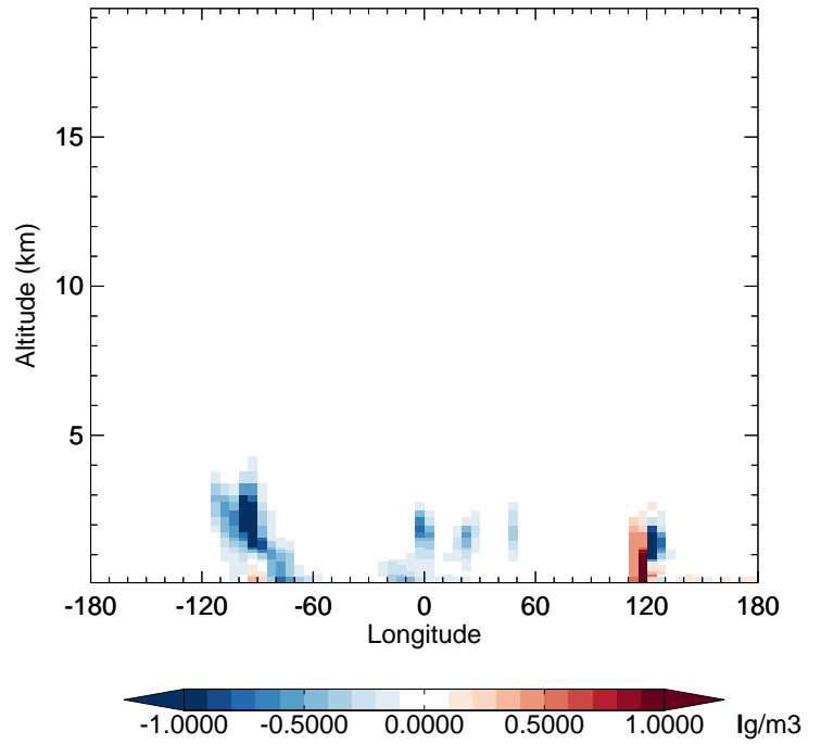
v11-02f-Run1 - v11-02e-Run0 NIT - Diff along 42N for Jul
