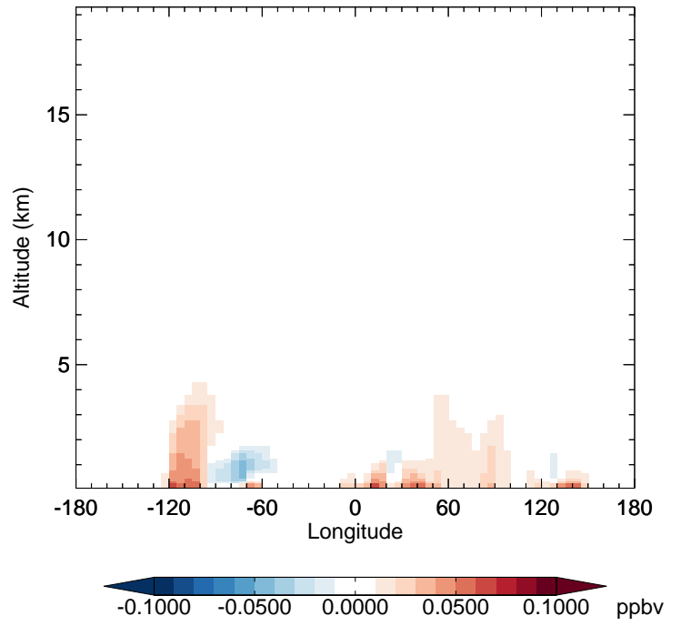
v11-02f-Run1 - v11-02e-Run1 TSOG3 - Diff along 42N for Jul
