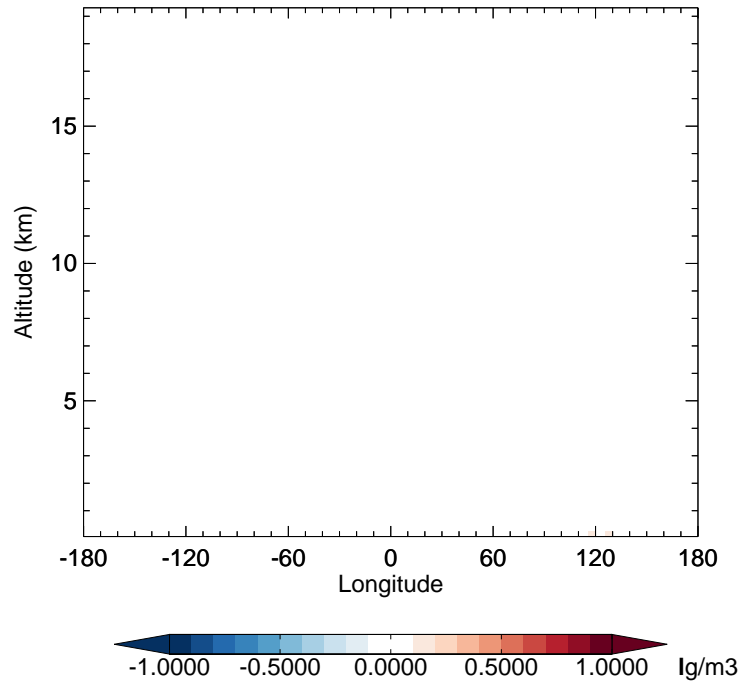
v11-02f-Run1 - v11-02e-Run1 BCPO - Diff along 42N for Oct
