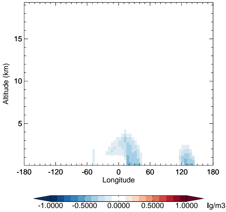
v11-02f-Run1 - v11-02e-Run1 OCPI - Diff along 15S for Oct
