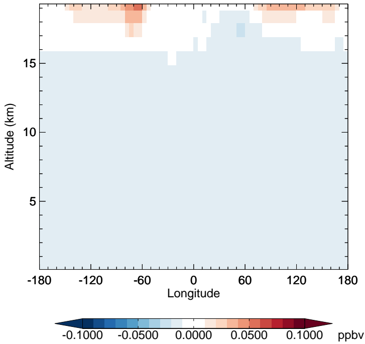
v11-02f-Run1 - v11-02e-Run0 CFC12 - Diff along 15S for Oct
