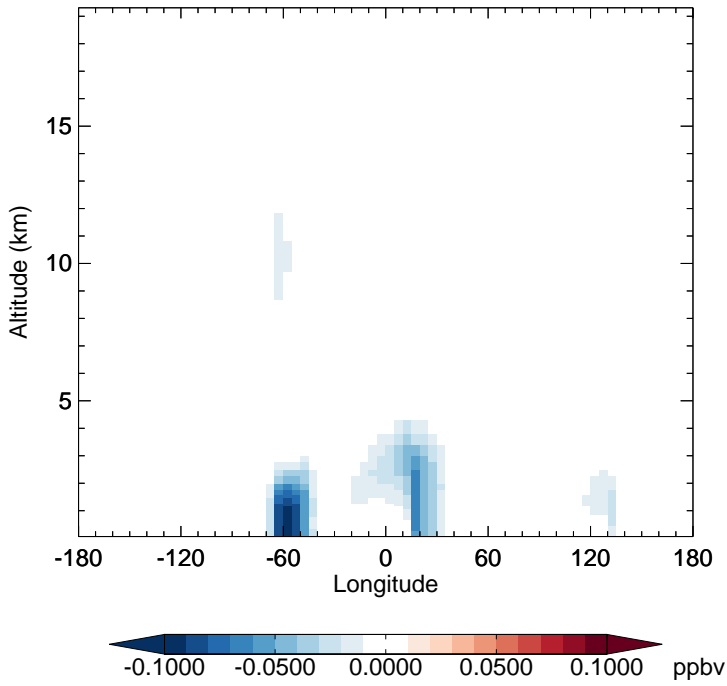
v11-02f-Run1 - v11-02e-Run1 ISOA1 - Diff along 15S for Oct
