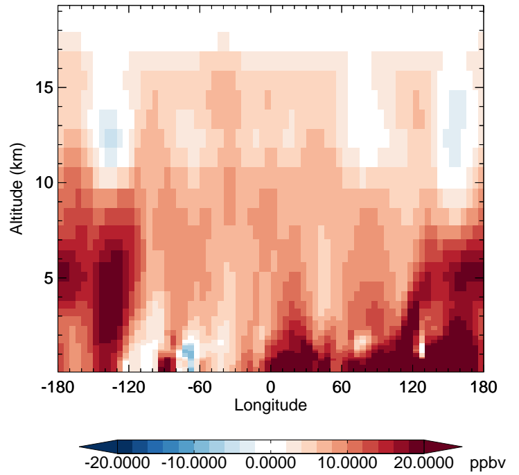
v11-02f-Run1 - v11-02e-Run0 CO - Diff along 42N for Oct
