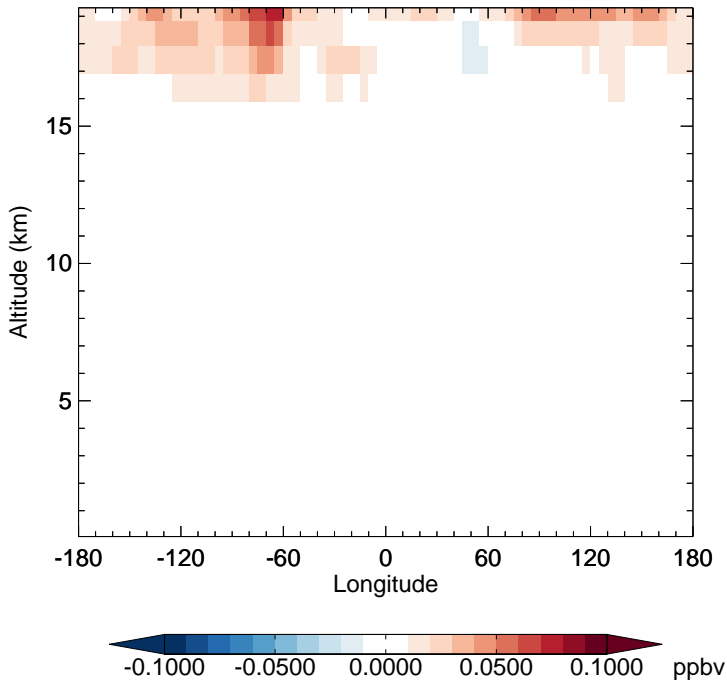
v11-02f-Run1 - v11-02e-Run0 OCS - Diff along 15S for Oct
