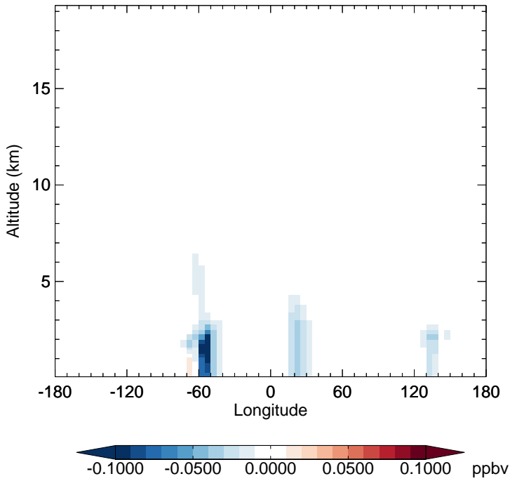
v11-02f-Run1 - v11-02e-Run0 IPMN - Diff along 15S for Oct
