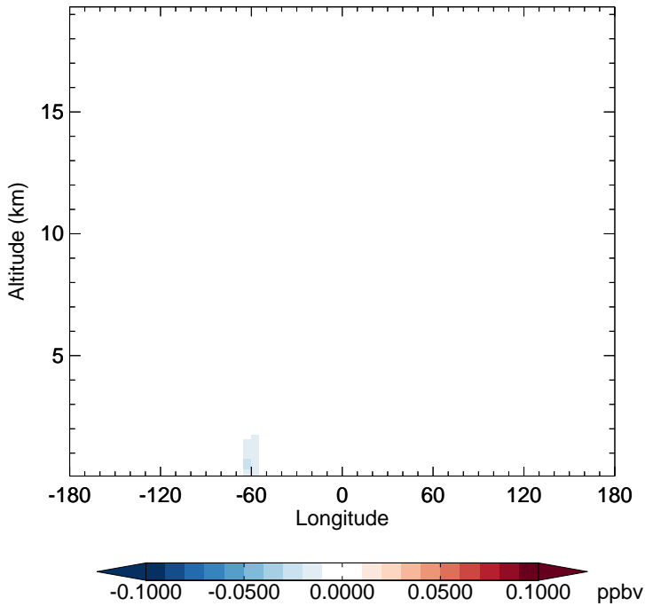
v11-02f-Run1 - v11-02e-Run0 RIPD - Diff along 15S for Oct
