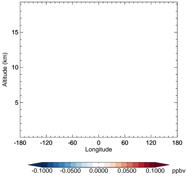
v11-02f-Run1 - v11-02e-Run1 PROPNN - Diff along 15S for Oct
