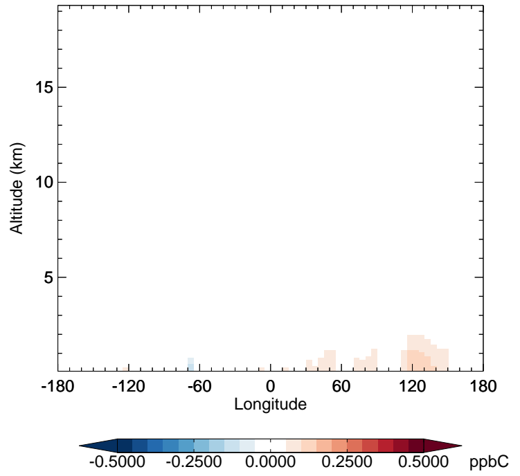
v11-02f-Run1 - v11-02e-Run1 ALD2 - Diff along 42N for Oct
