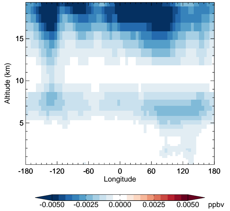
v11-02f-Run1 - v11-02e-Run1 HNO 4 - Diff along 42N for Oct
