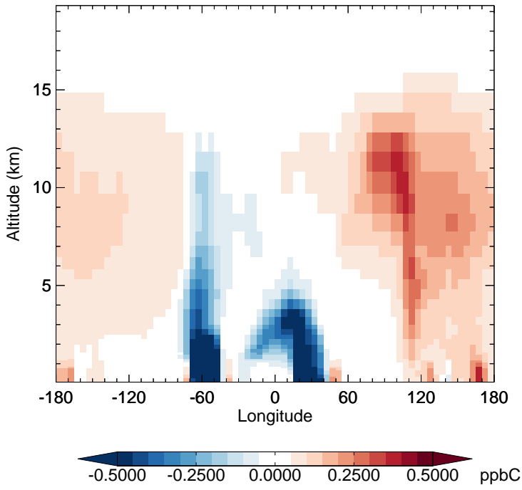
v11-02f-Run1 - v11-02e-Run1 ACET - Diff along 15S for Oct
