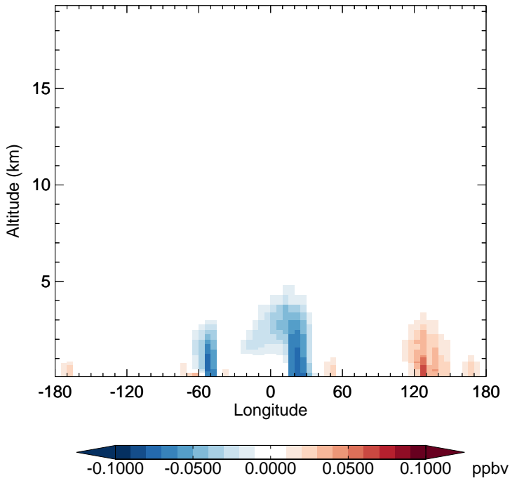
v11-02f-Run1 - v11-02e-Run1 TSOG3 - Diff along 15S for Oct
