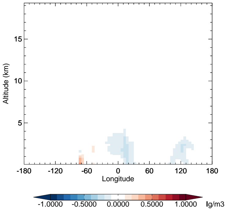
v11-02f-Run1 - v11-02e-Run0 NH4 - Diff along 15S for Oct
