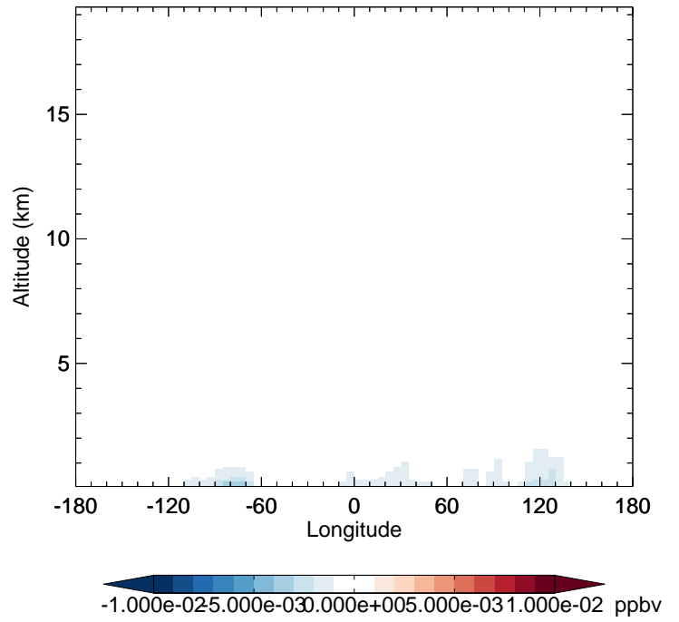
v11-02f-Run1 - v11-02e-Run1 NO3 - Diff along 42N for Oct
