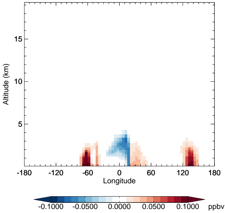
v11-02f-Run1 - v11-02e-Run1 INDIOL - Diff along 15S for Oct
