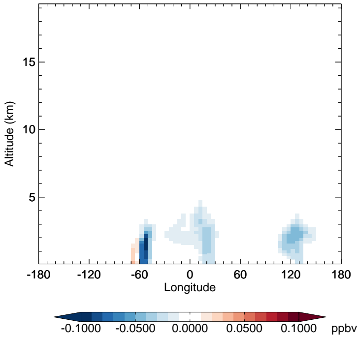
v11-02f-Run1 - v11-02e-Run0 ISOA1 - Diff along 15S for Oct
