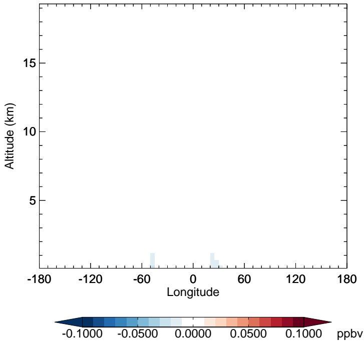
v11-02f-Run1 - v11-02e-Run1 ISN1 - Diff along 15S for Oct
