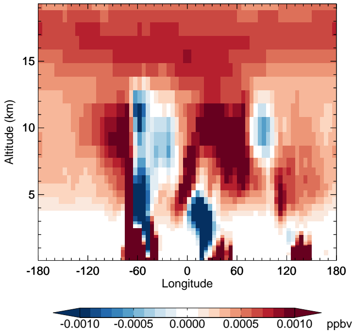
v11-02f-Run1 - v11-02e-Run1 PPN - Diff along 15S for Oct
