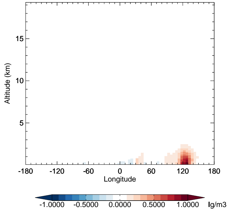
v11-02f-Run1 - v11-02e-Run1 OCPI - Diff along 42N for Oct
