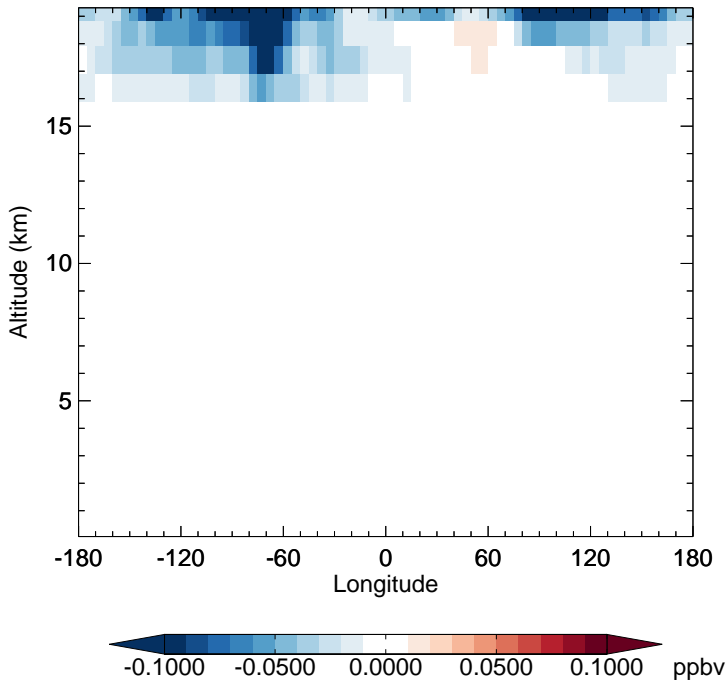
v11-02f-Run1 - v11-02e-Run0 CINO3 - Diff along 15S for Oct
