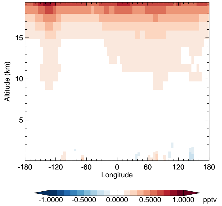
v11-02f-Run1 - v11-02e-Run1 HO2 - Diff along 42N for Oct
