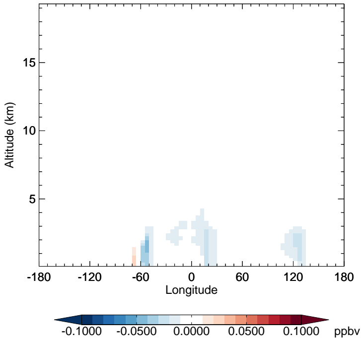
v11-02f-Run1 - v11-02e-Run0 SOAGX - Diff along 15S for Oct
