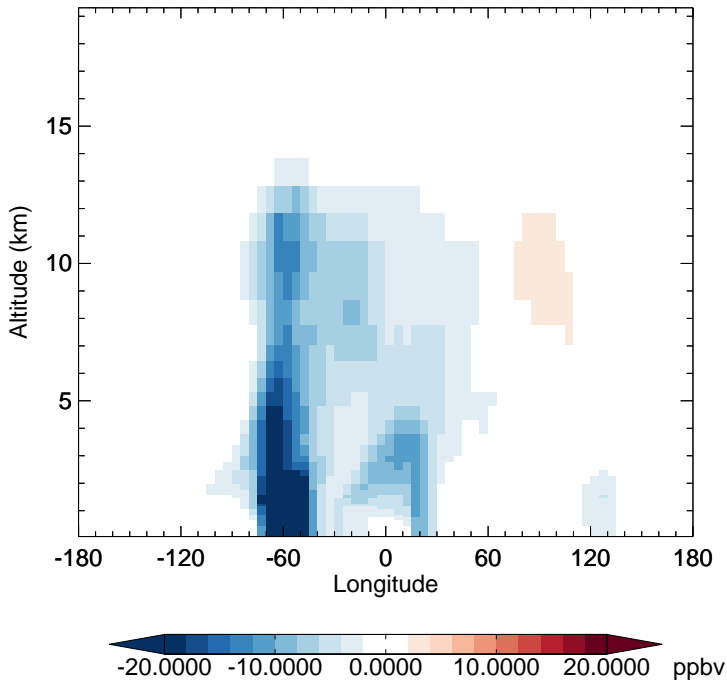
v11-02f-Run1 - v11-02e-Run1 CO - Diff along 15S for Oct
