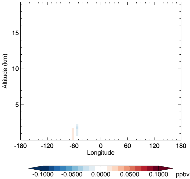
v11-02f-Run1 - v11-02e-Run0 ISOA3 - Diff along 15S for Oct
