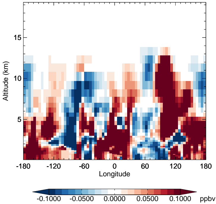
v11-02f-Run1 - v11-02e-Run0 H2O2 - Diff along 15S for Oct
