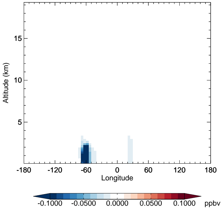
v11-02f-Run1 - v11-02e-Run1 RIPB - Diff along 15S for Oct
