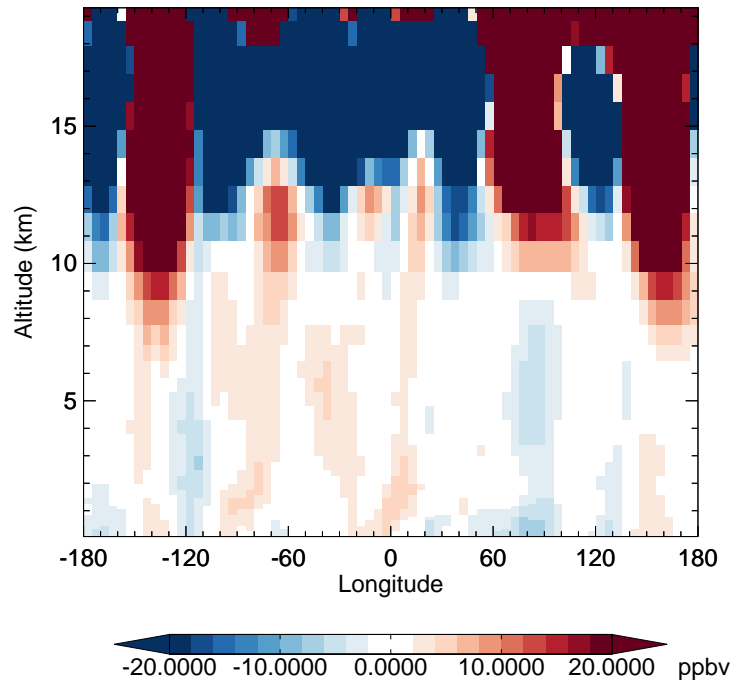
v11-02f-Run1 - v11-02e-Run0 O3 - Diff along 42N for Oct
