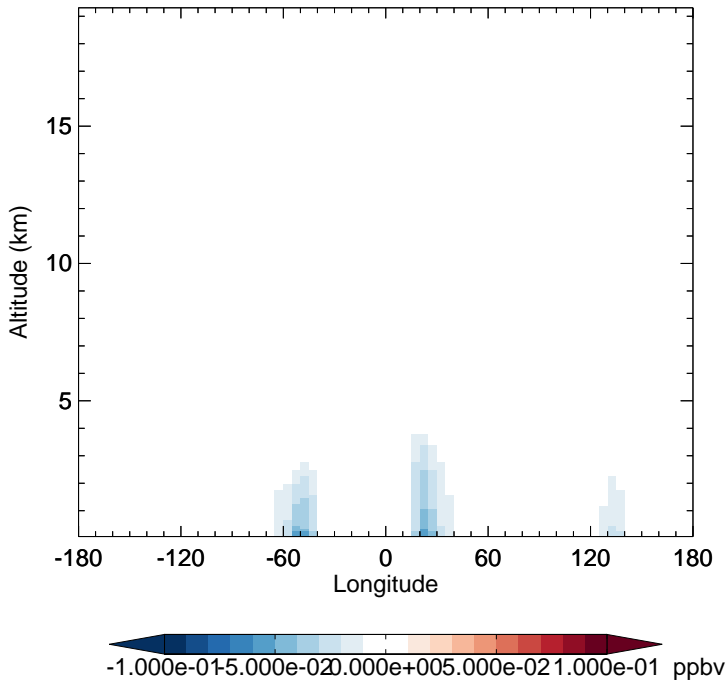
v11-02f-Run1 - v11-02e-Run1 MONITA - Diff along 15S for Oct
