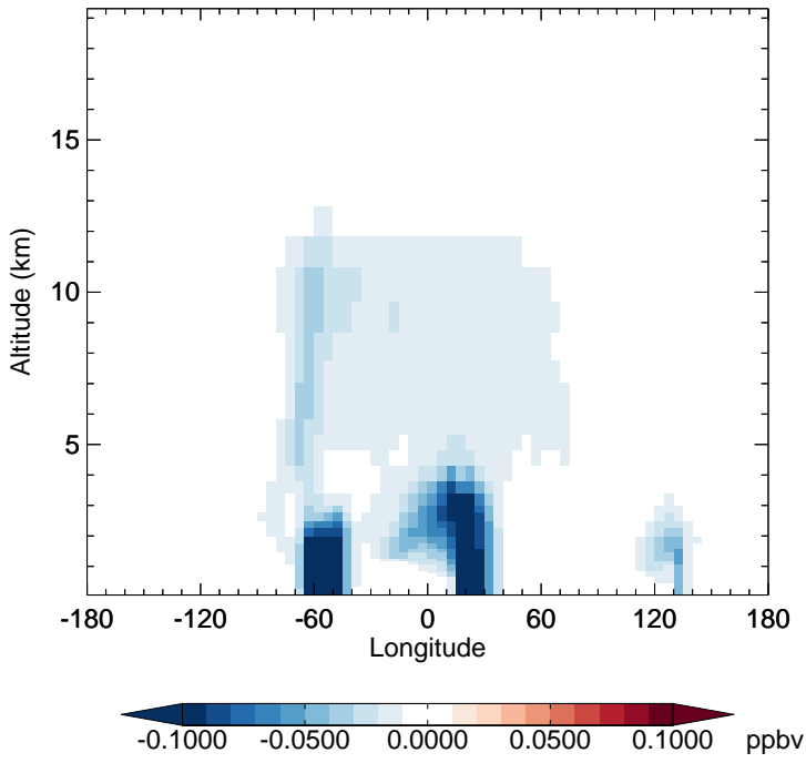
v11-02f-Run1 - v11-02e-Run1 ISO3 - Diff along 15S for Oct
