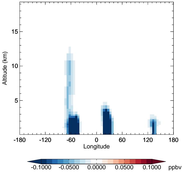
v11-02f-Run1 - v11-02e-Run1 GLYC - Diff along 15S for Oct
