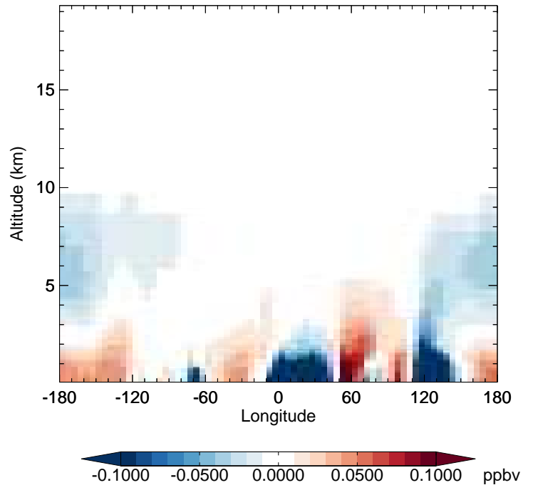
v11-02f-Run1 - v11-02e-Run1 BENZ - Diff along 42N for Oct
