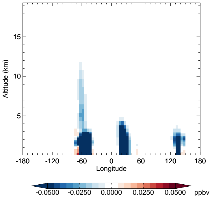
v11-02f-Run1 - v11-02e-Run0 MVK - Diff along 15S for Oct
