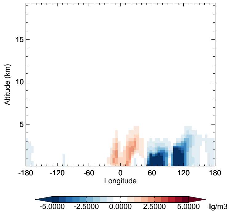
v11-02f-Run1 - v11-02e-Run0 DST1 - Diff along 42N for Oct
