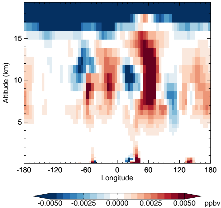
v11-02f-Run1 - v11-02e-Run0 N2O5 - Diff along 15S for Oct
