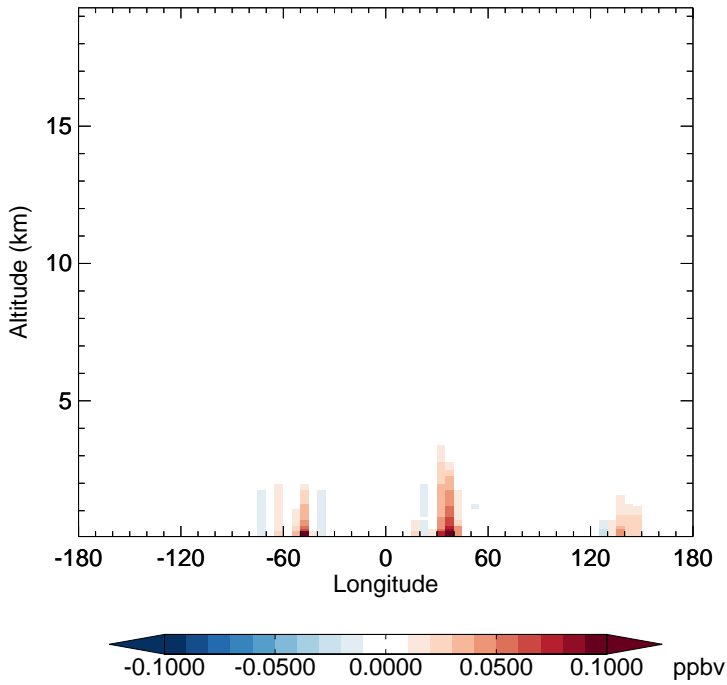
v11-02f-Run1 - v11-02e-Run0 SOAP - Diff along 15S for Oct
