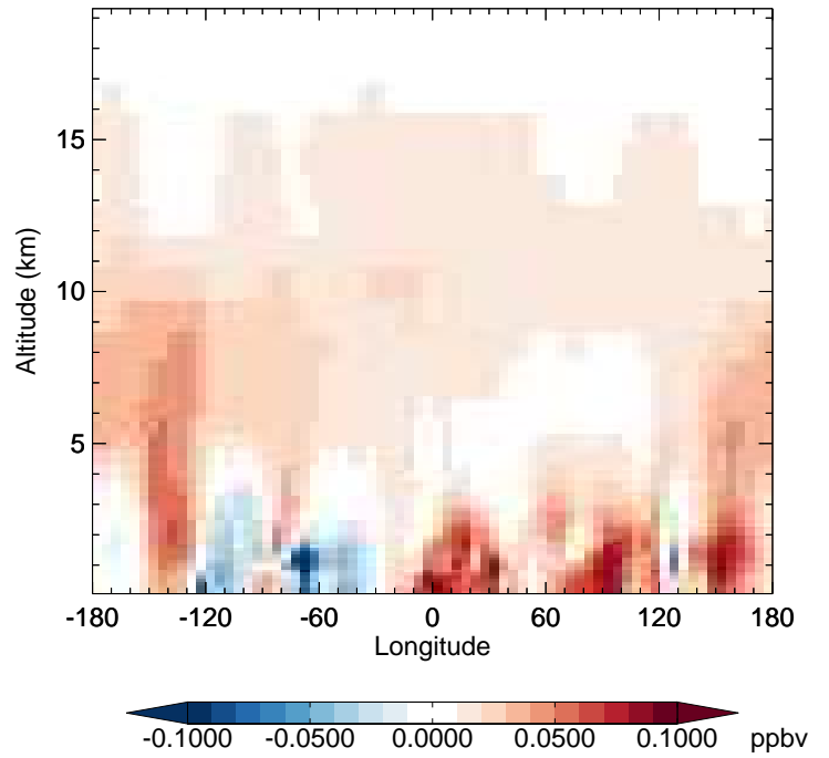
v11-02f-Run1 - v11-02e-Run0 PAN - Diff along 42N for Oct
