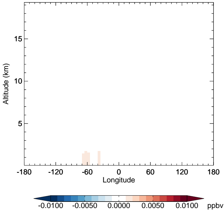
v11-02f-Run1 - v11-02e-Run1 R4N2 - Diff along 15S for Oct
