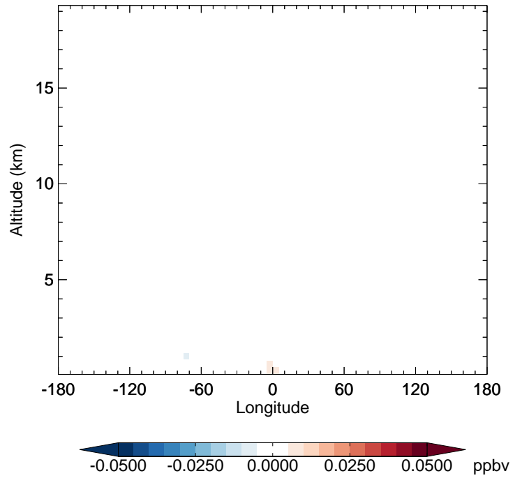
v11-02f-Run1 - v11-02e-Run0 MACR - Diff along 42N for Oct
