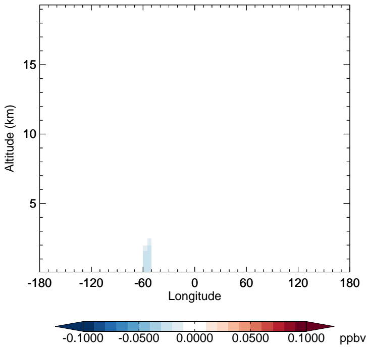
v11-02f-Run1 - v11-02e-Run0 TSOA1 - Diff along 15S for Oct
