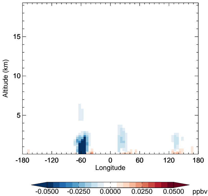
v11-02f-Run1 - v11-02e-Run0 RCHO - Diff along 15S for Oct
