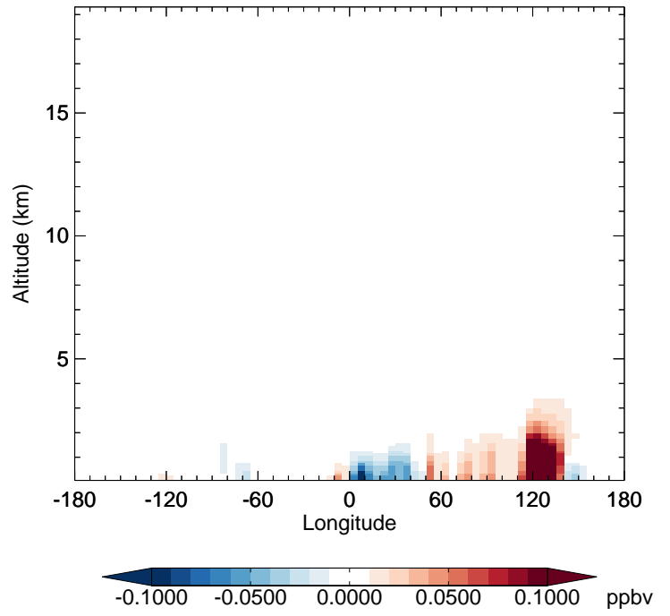
v11-02f-Run1 - v11-02e-Run1 EOH - Diff along 42N for Oct
