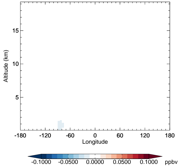
v11-02f-Run1 - v11-02e-Run1 IMAE - Diff along 42N for Oct
