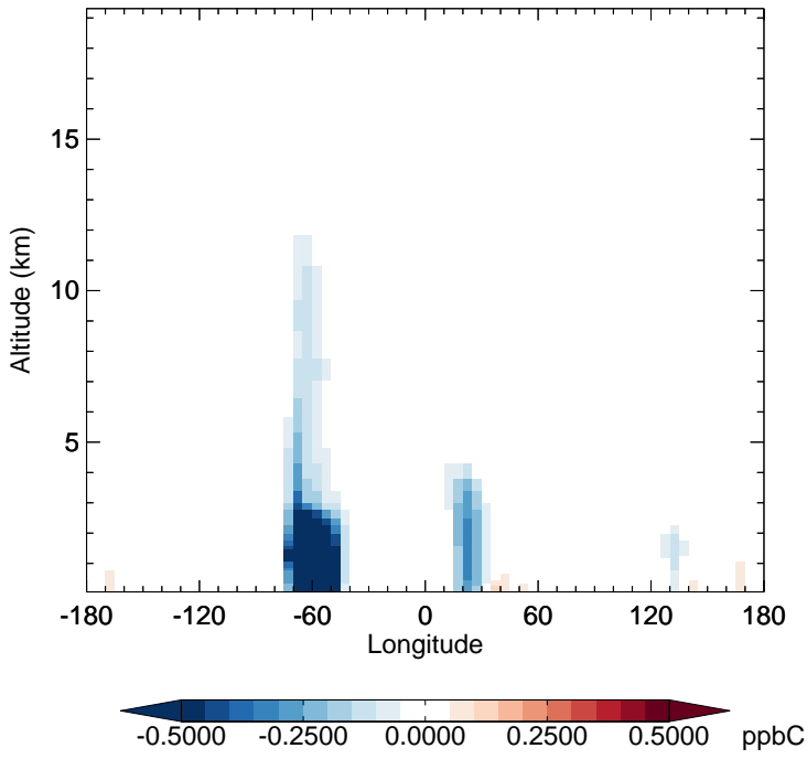
v11-02f-Run1 - v11-02e-Run1 ALD2 - Diff along 15S for Oct
