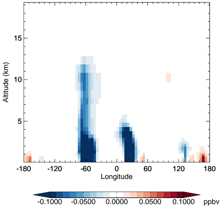
v11-02f-Run1 - v11-02e-Run1 EOH - Diff along 15S for Oct
