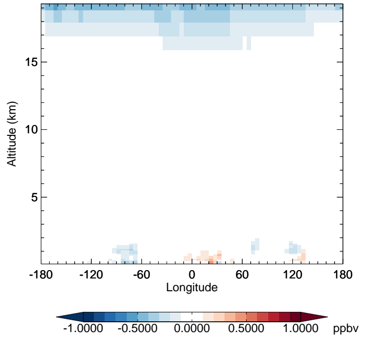
v11-02f-Run1 - v11-02e-Run0 NO 2 - Diff along 42N for Oct
