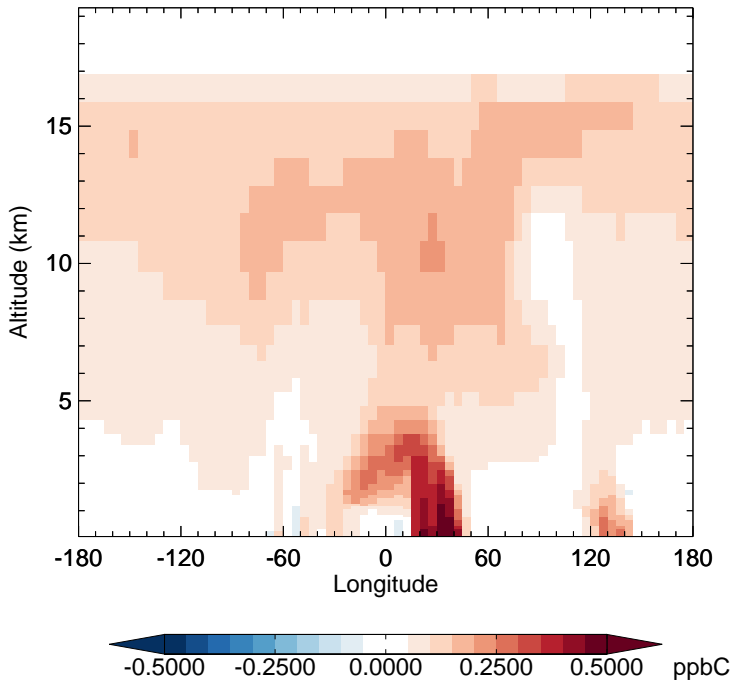
v11-02f-Run1 - v11-02e-Run1 C2H6 - Diff along 15S for Oct
