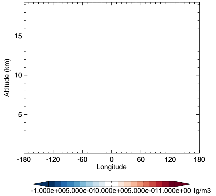
v11-02f-Run1 - v11-02e-Run1 SO4s - Diff along 42N for Oct
