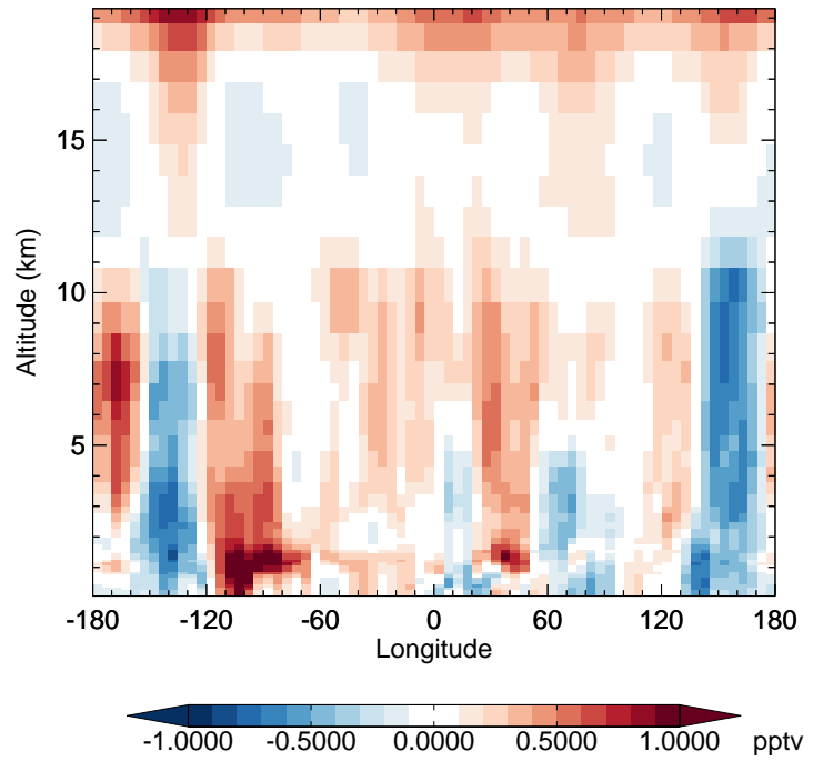
v11-02f-Run1 - v11-02e-Run0 HO2 - Diff along 42N for Oct
