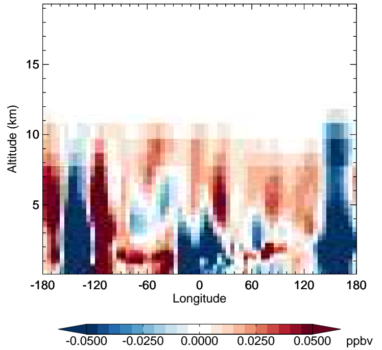
v11-02f-Run1 - v11-02e-Run0 MP - Diff along 42N for Oct
