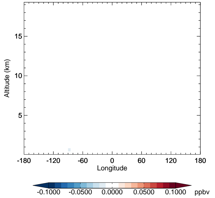
v11-02f-Run1 - v11-02e-Run1 ISO3 - Diff along 42N for Oct
