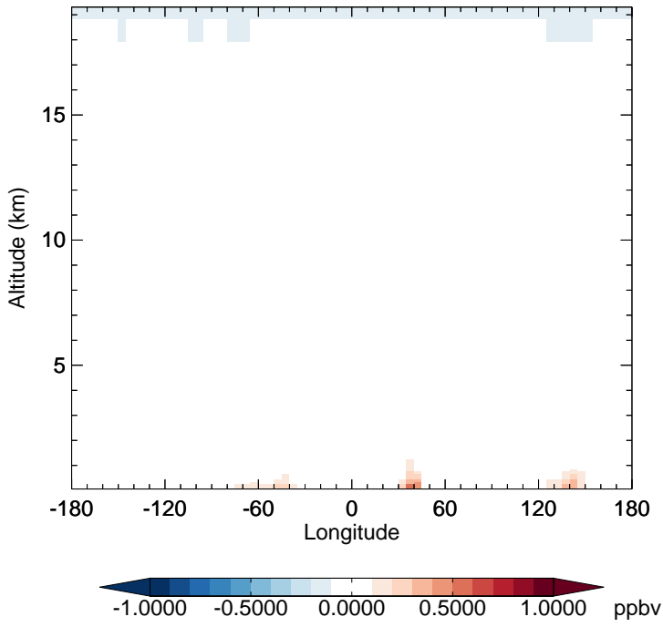
v11-02f-Run1 - v11-02e-Run1 NO 2 - Diff along 15S for Oct
