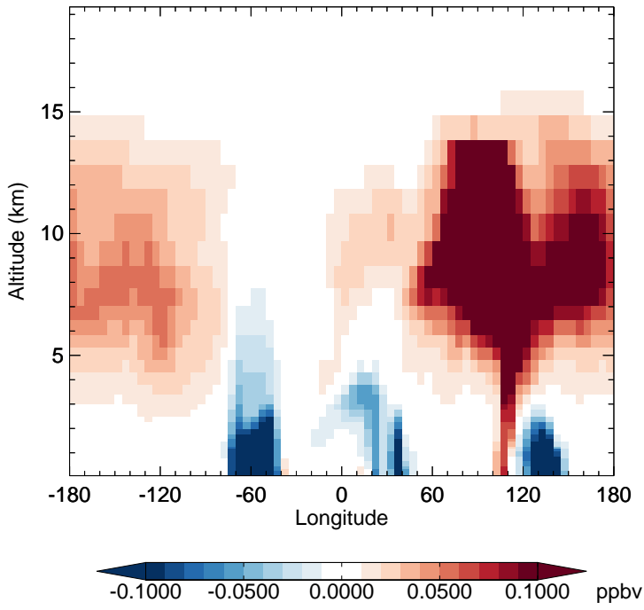
v11-02f-Run1 - v11-02e-Run1 BENZ - Diff along 15S for Oct
