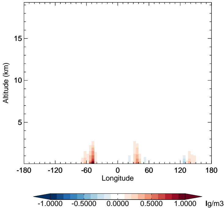
v11-02f-Run1 - v11-02e-Run0 OCPO - Diff along 15S for Oct
