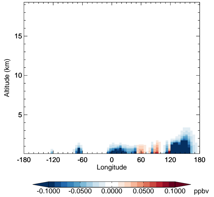
v11-02f-Run1 - v11-02e-Run1 XYLE - Diff along 42N for Oct
