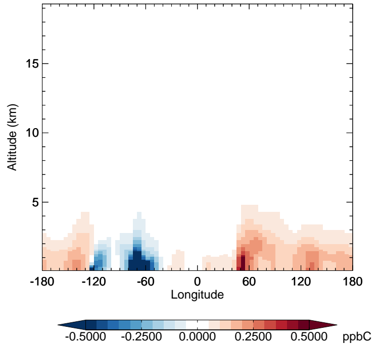
v11-02f-Run1 - v11-02e-Run1 ALK4 - Diff along 42N for Oct
