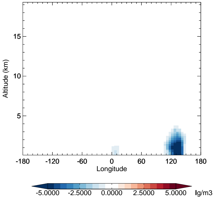
v11-02f-Run1 - v11-02e-Run0 DST3 - Diff along 15S for Oct
