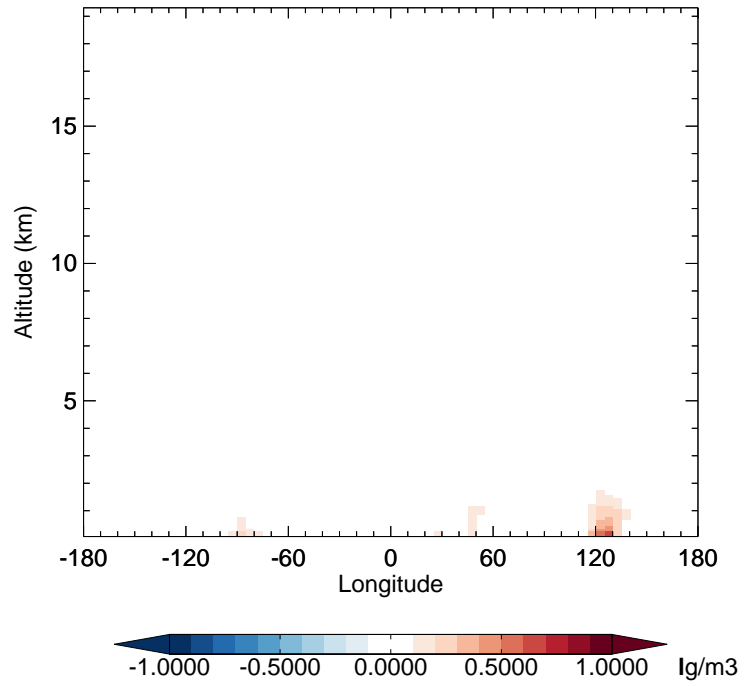
v11-02f-Run1 - v11-02e-Run1 NH4 - Diff along 42N for Oct
