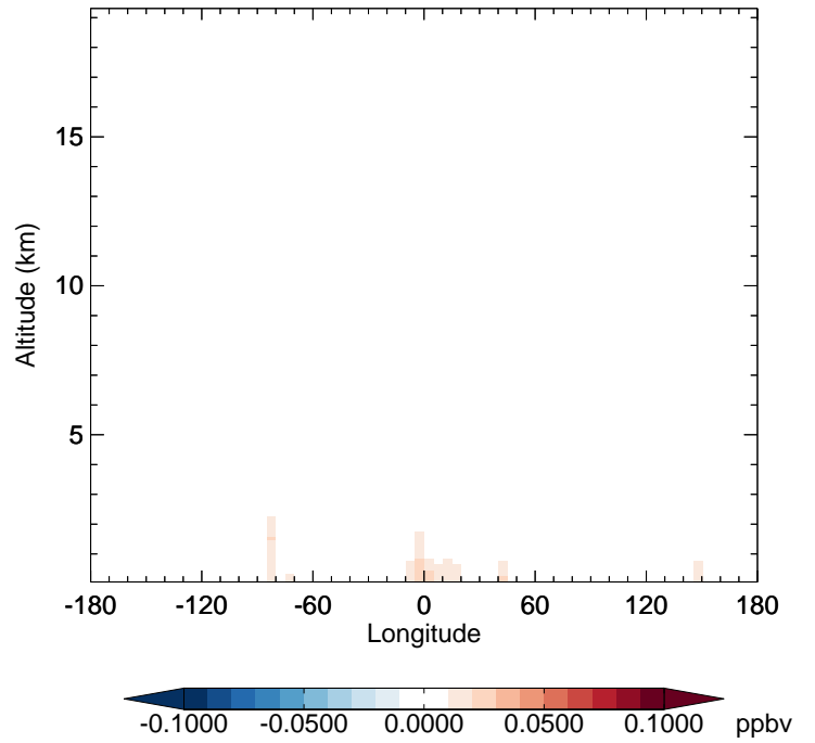
v11-02f-Run1 - v11-02e-Run0 TSOG3 - Diff along 42N for Oct
