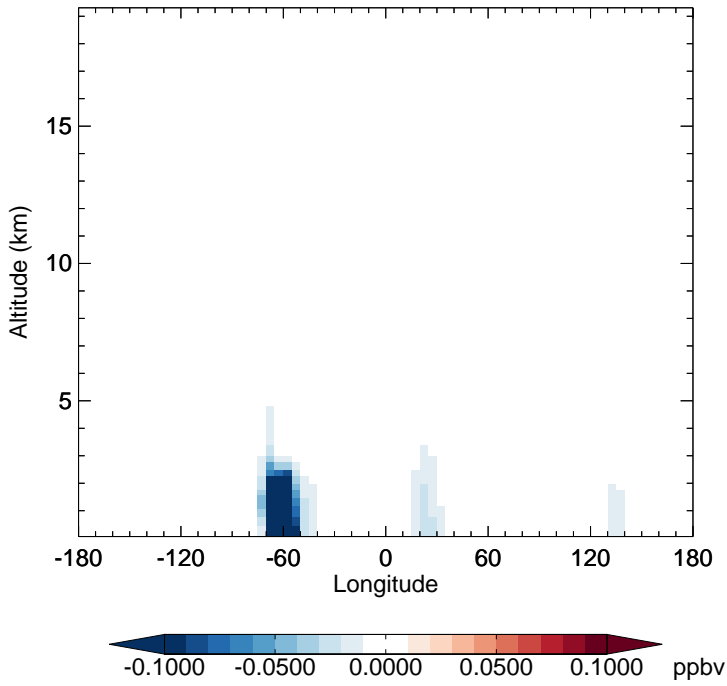
v11-02f-Run1 - v11-02e-Run1 HPALD - Diff along 15S for Oct
