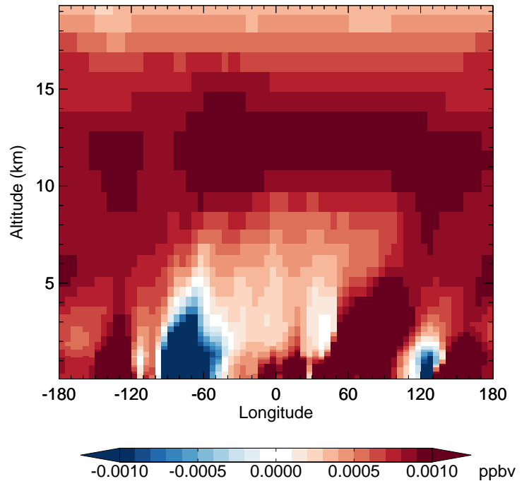
v11-02f-Run1 - v11-02e-Run1 PPN - Diff along 42N for Oct
