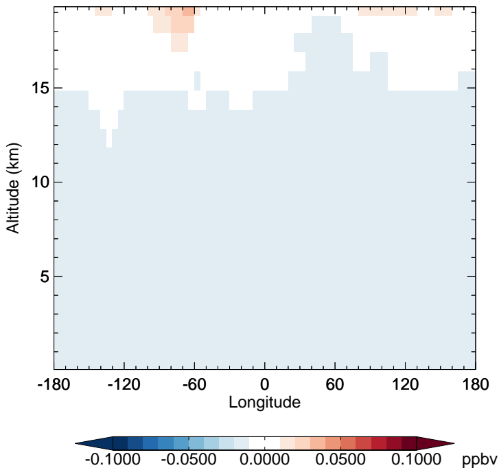
v11-02f-Run1 - v11-02e-Run0 CFC11 - Diff along 15S for Oct
