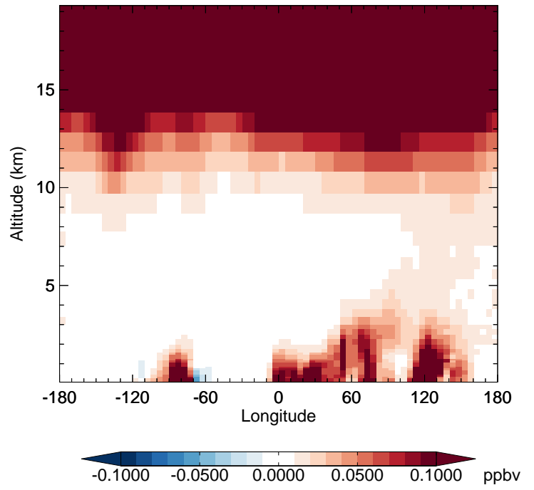
v11-02f-Run1 - v11-02e-Run1 HNO 3 - Diff along 42N for Oct
