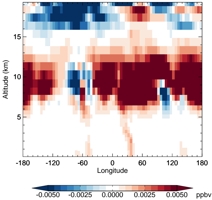
v11-02f-Run1 - v11-02e-Run0 HNO 4 - Diff along 15S for Oct
