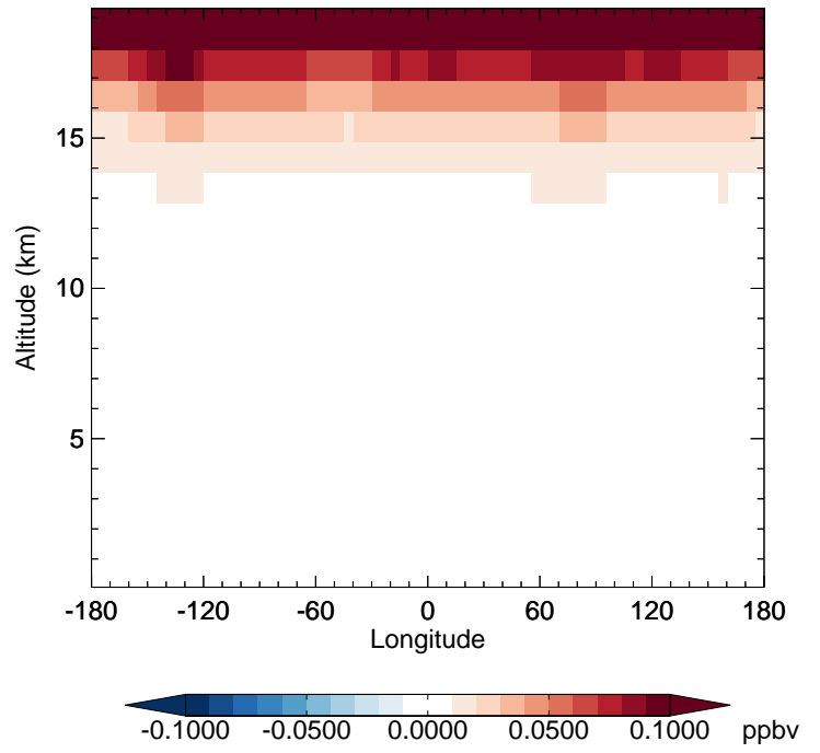
v11-02f-Run1 - v11-02e-Run1 N2O - Diff along 42N for Oct
