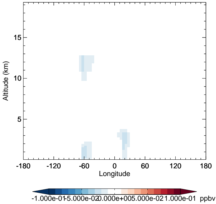
v11-02f-Run1 - v11-02e-Run1 ISOA3 - Diff along 15S for Oct
