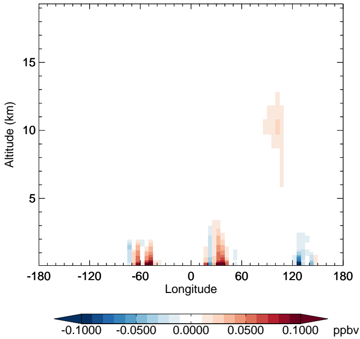
v11-02f-Run1 - v11-02e-Run0 TOLU - Diff along 15S for Oct
