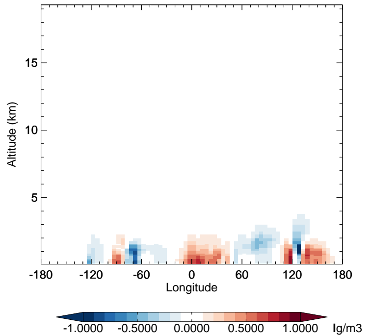
v11-02f-Run1 - v11-02e-Run0 SOAS - Diff along 42N for Oct
