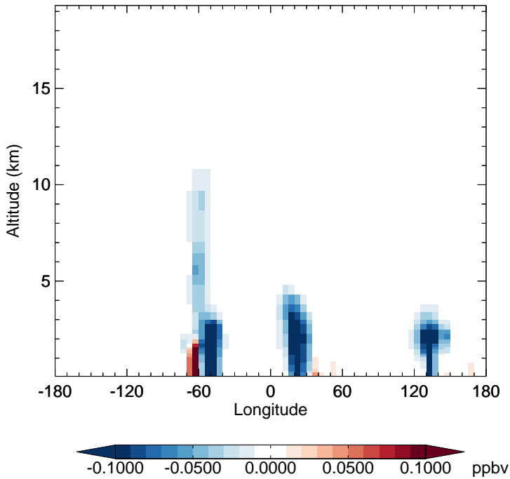
v11-02f-Run1 - v11-02e-Run0 HAC - Diff along 15S for Oct
