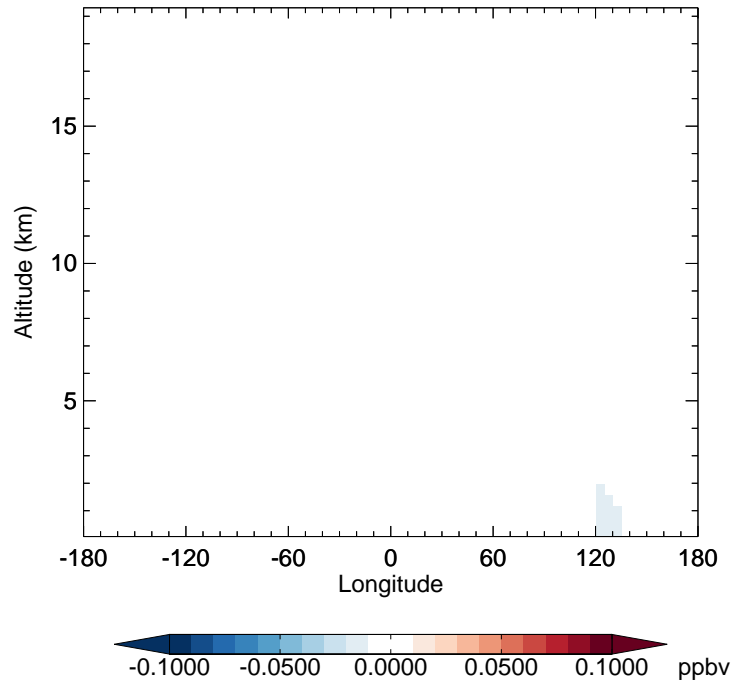
v11-02f-Run1 - v11-02e-Run0 ASOG3 - Diff along 42N for Oct
