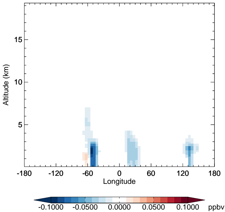
v11-02f-Run1 - v11-02e-Run0 HC187 - Diff along 15S for Oct
