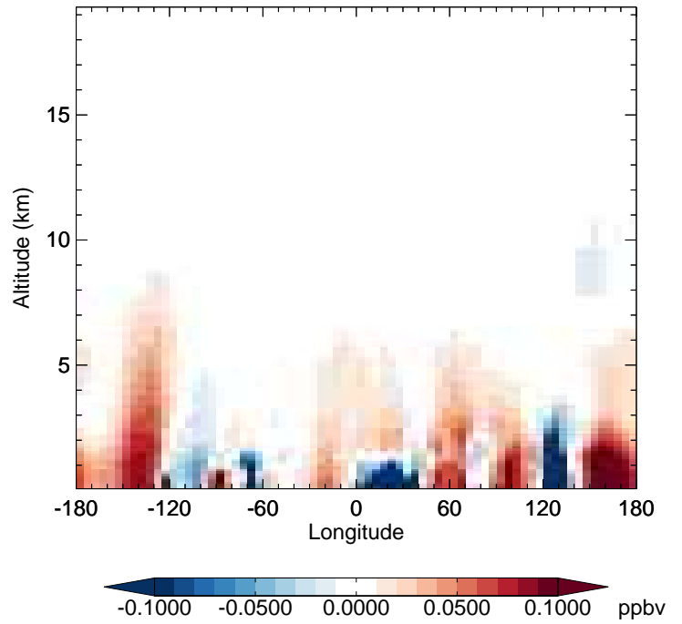
v11-02f-Run1 - v11-02e-Run0 BENZ - Diff along 42N for Oct
