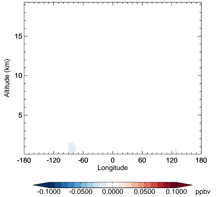
v11-02f-Run1 - v11-02e-Run1 GLYC - Diff along 42N for Oct
