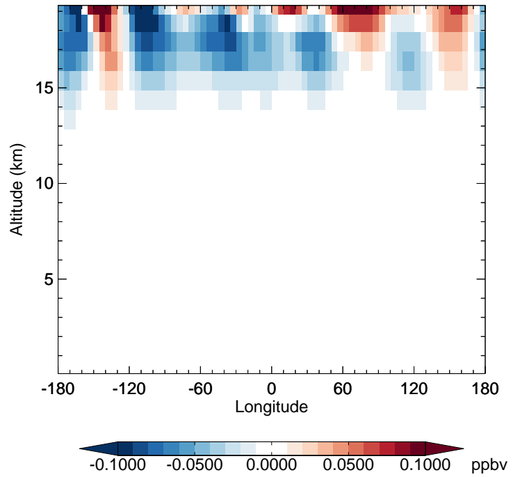
v11-02f-Run1 - v11-02e-Run0 CINO3 - Diff along 42N for Oct
