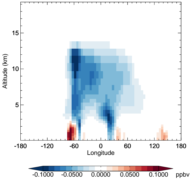
v11-02f-Run1 - v11-02e-Run1 PAN - Diff along 15S for Oct
