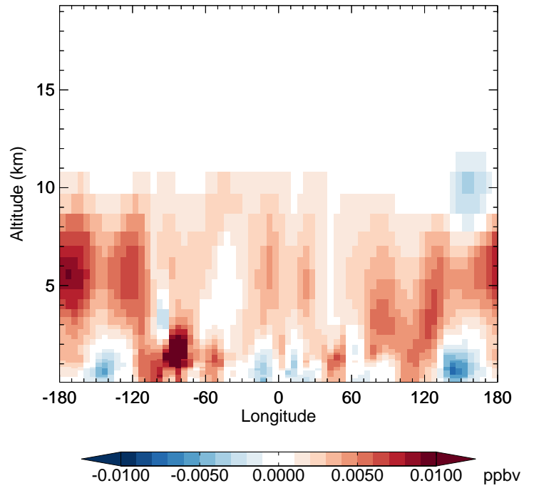
v11-02f-Run1 - v11-02e-Run0 MAP - Diff along 42N for Oct
