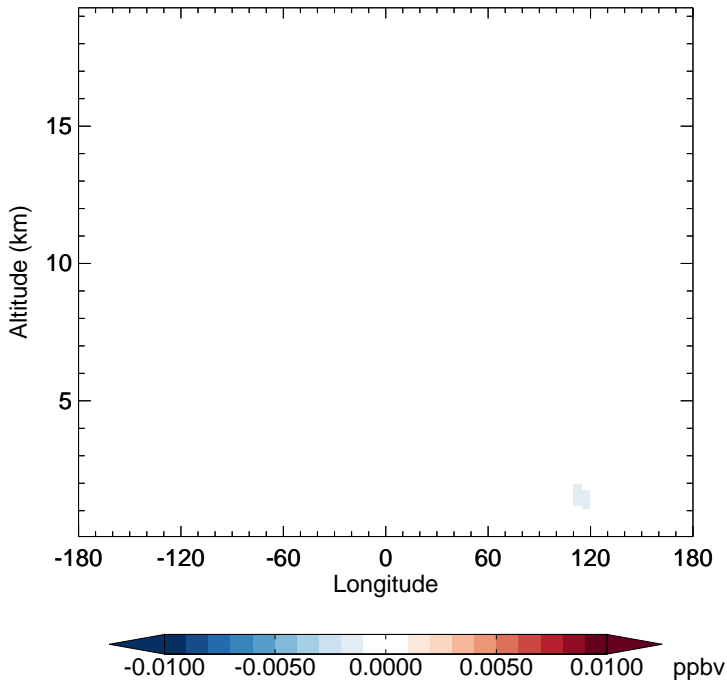
v11-02f-Run1 - v11-02e-Run0 HOBr - Diff along 15S for Oct
