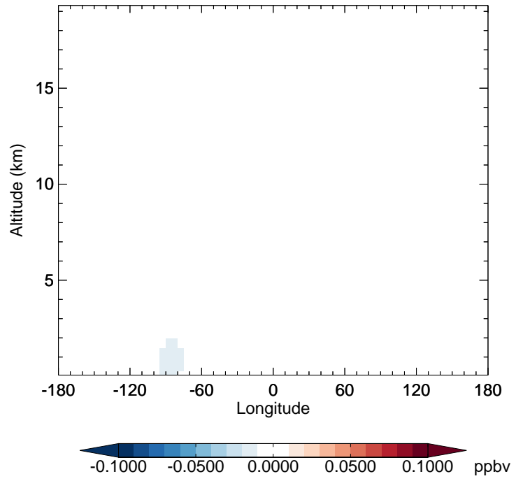
v11-02f-Run1 - v11-02e-Run1 SOAIE - Diff along 42N for Oct
