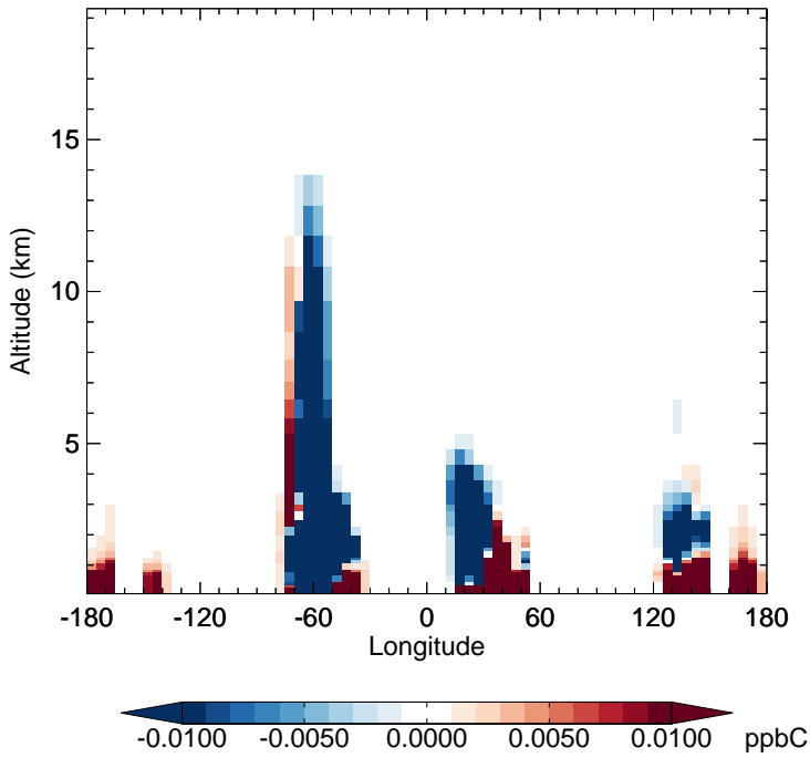
v11-02f-Run1 - v11-02e-Run0 PRPE - Diff along 15S for Oct
