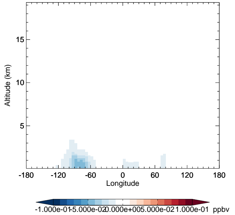
v11-02f-Run1 - v11-02e-Run0 IONITA - Diff along 42N for Oct
