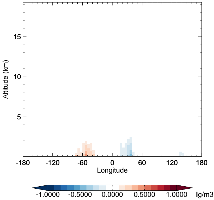
v11-02f-Run1 - v11-02e-Run1 NH3 - Diff along 15S for Oct
