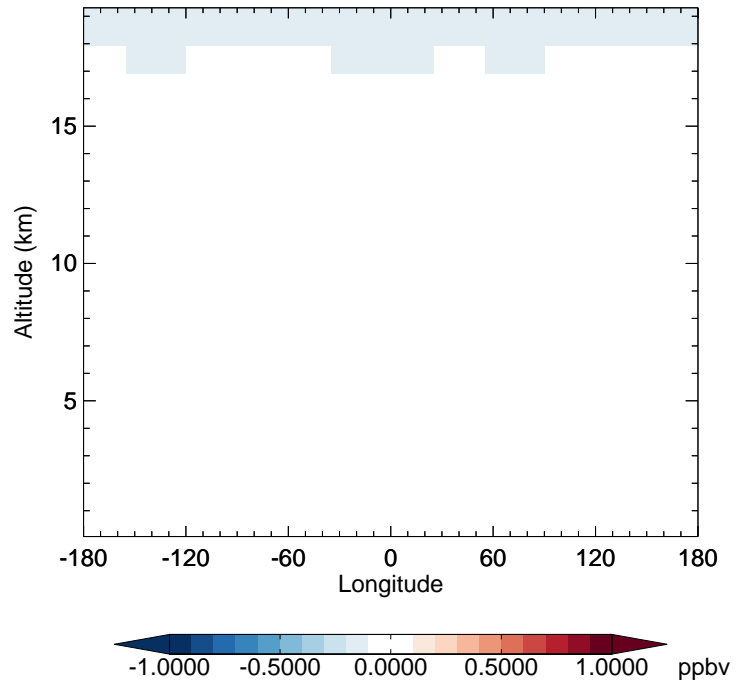
v11-02f-Run1 - v11-02e-Run1 NO - Diff along 42N for Oct
