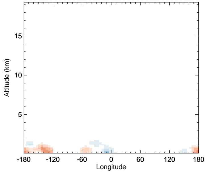
v11-02f-Run1 - v11-02e-Run0 SALA - Diff along 42N for Oct
