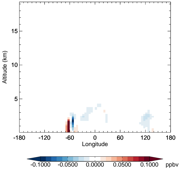
v11-02f-Run1 - v11-02e-Run0 TSOA2 - Diff along 15S for Oct
