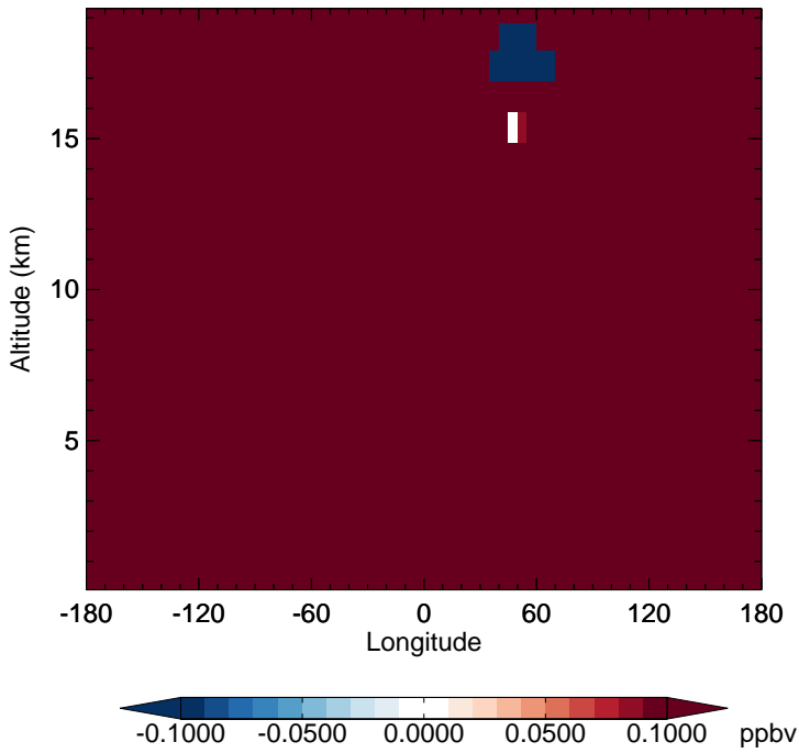
v11-02f-Run1 - v11-02e-Run0 N2O - Diff along 15S for Oct
