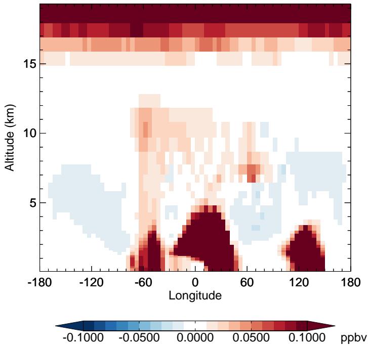
v11-02f-Run1 - v11-02e-Run1 HNO 3 - Diff along 15S for Oct
