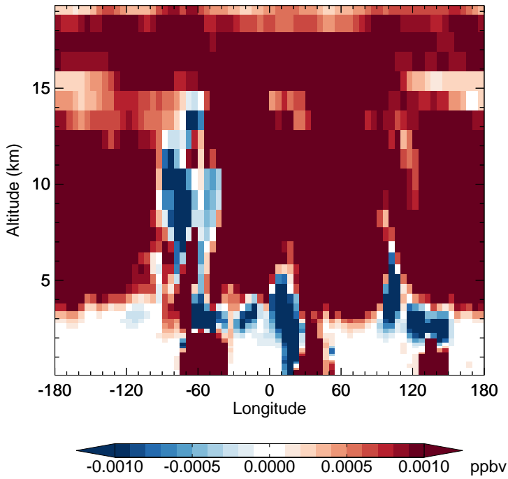
v11-02f-Run1 - v11-02e-Run0 PPN - Diff along 15S for Oct
