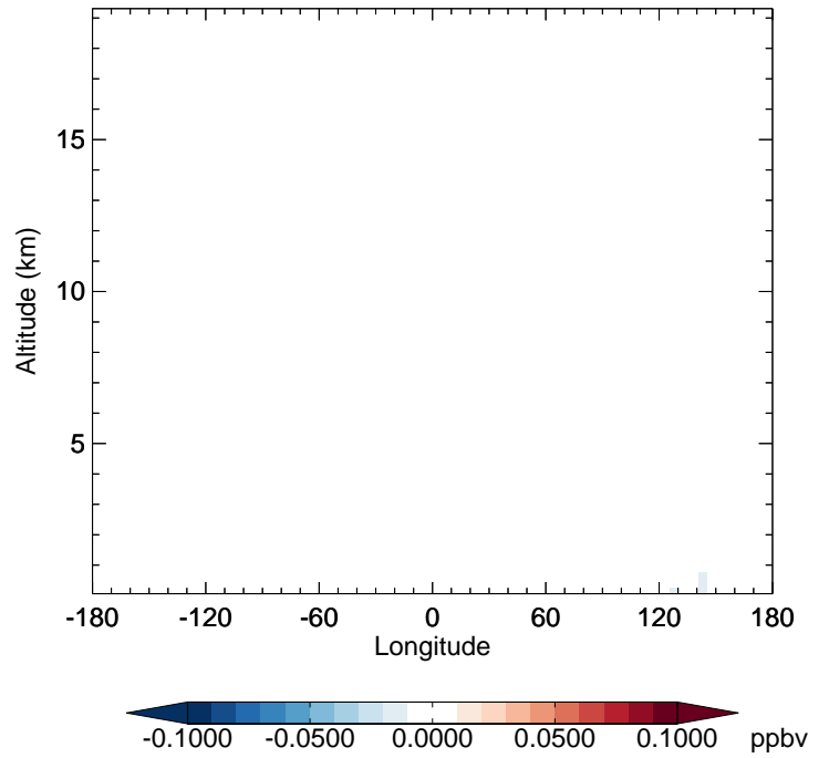
v11-02f-Run1 - v11-02e-Run0 MGLY - Diff along 42N for Oct
