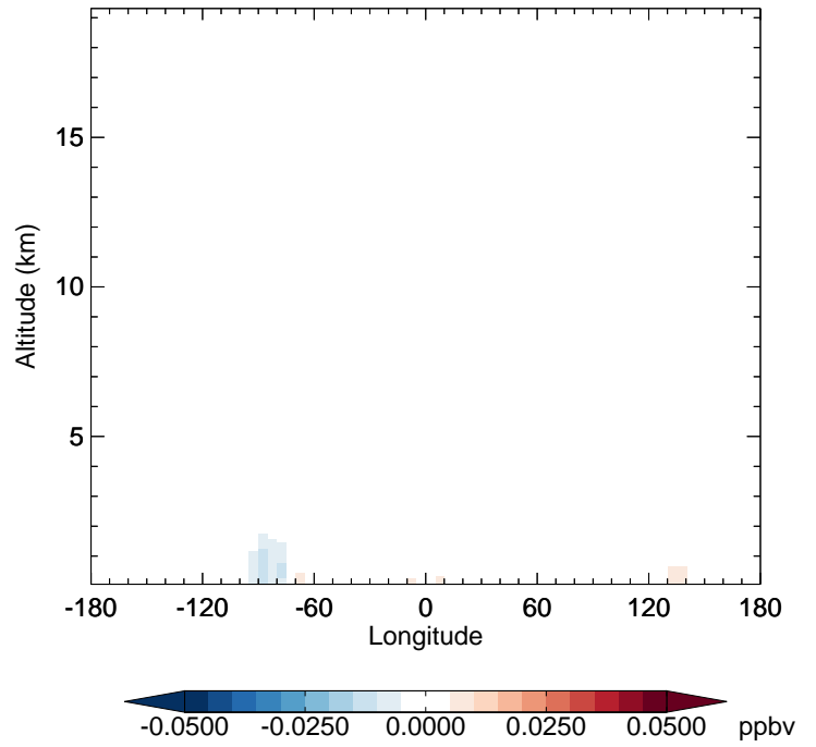
v11-02f-Run1 - v11-02e-Run1 MVK - Diff along 42N for Oct
