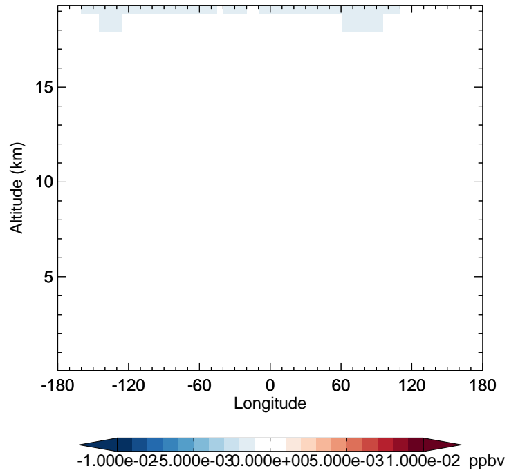
v11-02f-Run1 - v11-02e-Run1 BrNO3 - Diff along 42N for Oct
