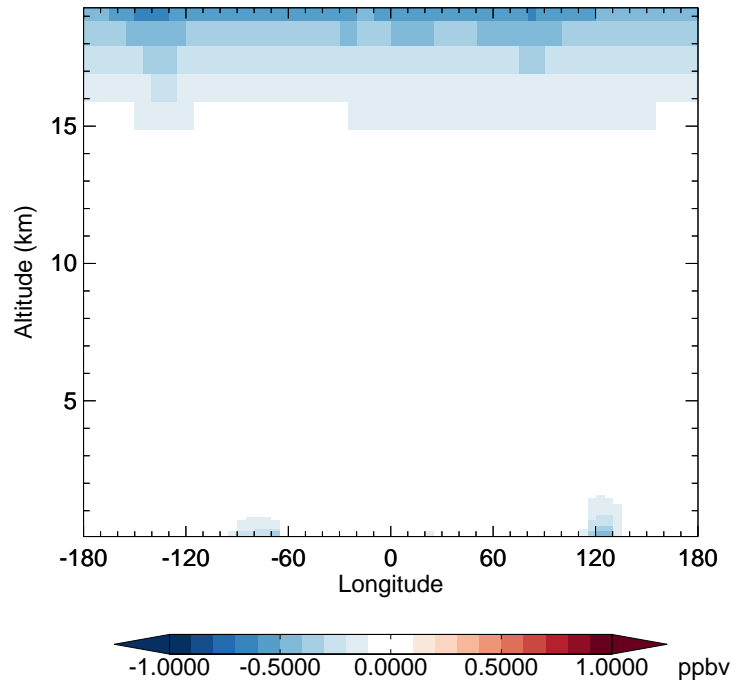
v11-02f-Run1 - v11-02e-Run1 NO 2 - Diff along 42N for Oct
