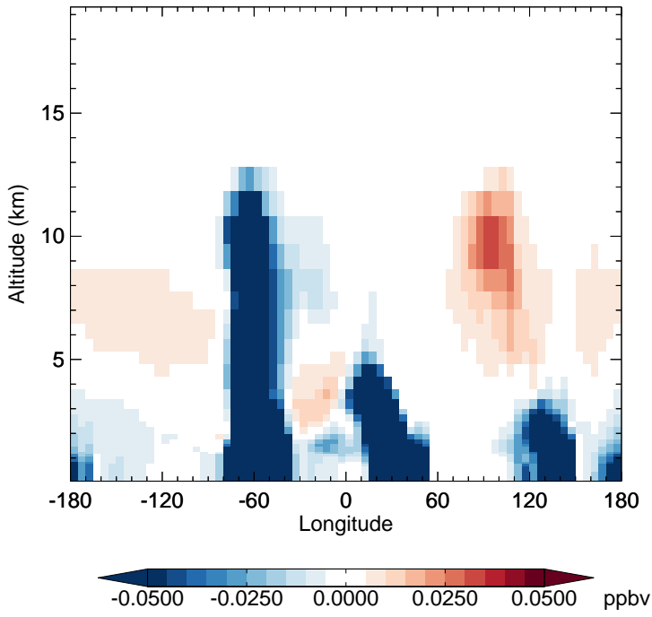
v11-02f-Run1 - v11-02e-Run1 MP - Diff along 15S for Oct
