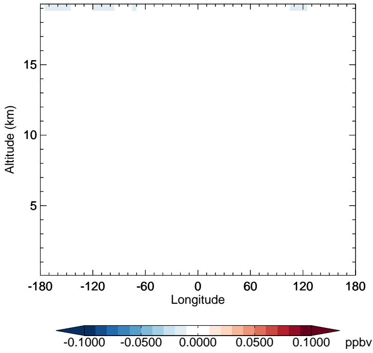
v11-02f-Run1 - v11-02e-Run1 CINO3 - Diff along 15S for Oct
