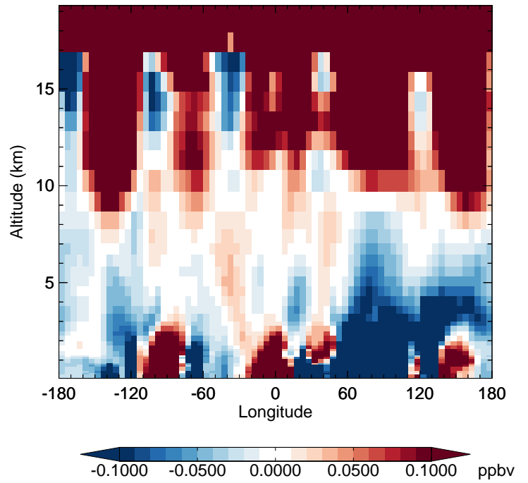
v11-02f-Run1 - v11-02e-Run0 HNO 3 - Diff along 42N for Oct
