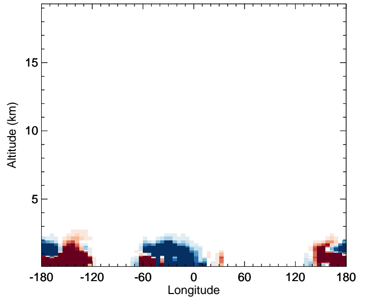
v11-02f-Run1 - v11-02e-Run0 SALC - Diff along 42N for Oct
