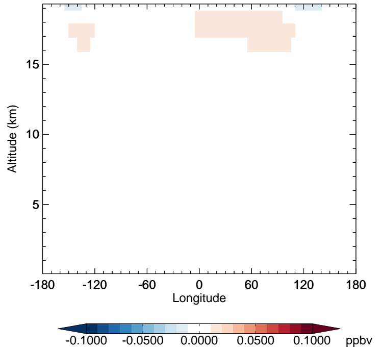
v11-02f-Run1 - v11-02e-Run1 HCl - Diff along 42N for Oct
