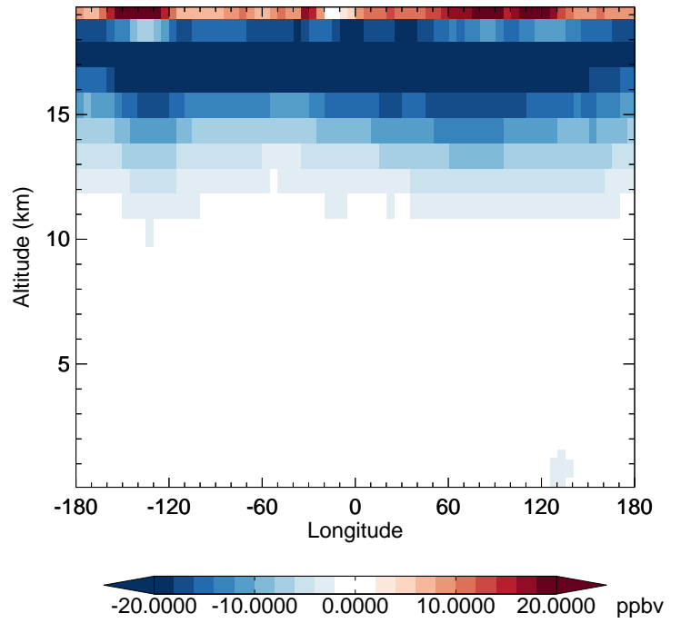
v11-02f-Run1 - v11-02e-Run1 O3 - Diff along 42N for Oct
