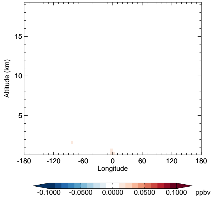
v11-02f-Run1 - v11-02e-Run0 HAC - Diff along 42N for Oct
