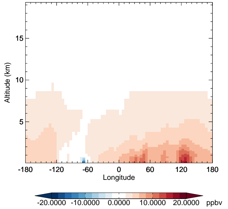
v11-02f-Run1 - v11-02e-Run1 CO - Diff along 42N for Oct
