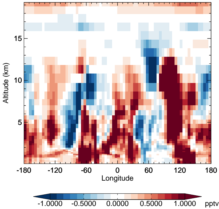
v11-02f-Run1 - v11-02e-Run0 HO2 - Diff along 15S for Oct
