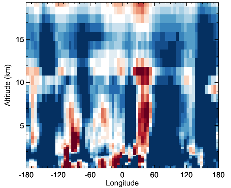
v11-02f-Run1 - v11-02e-Run0 OH - Diff along 42N for Oct
