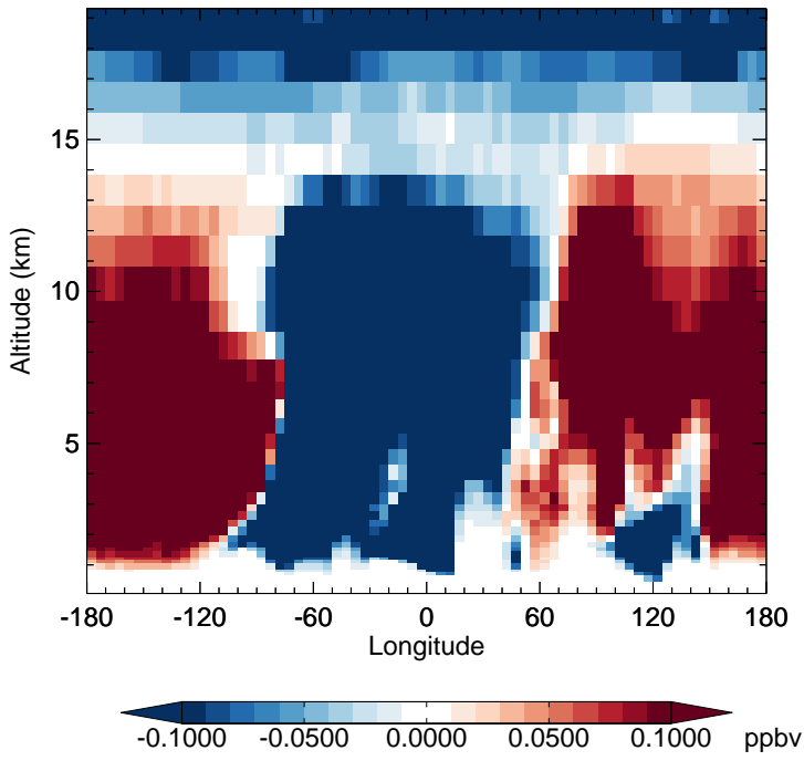
v11-02f-Run1 - v11-02e-Run1 CH4 - Diff along 15S for Oct
