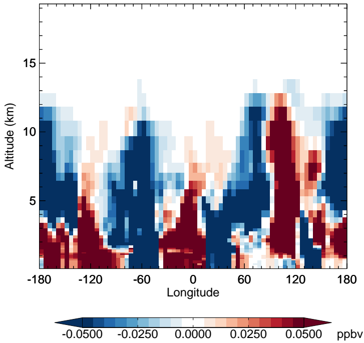
v11-02f-Run1 - v11-02e-Run0 MP - Diff along 15S for Oct
