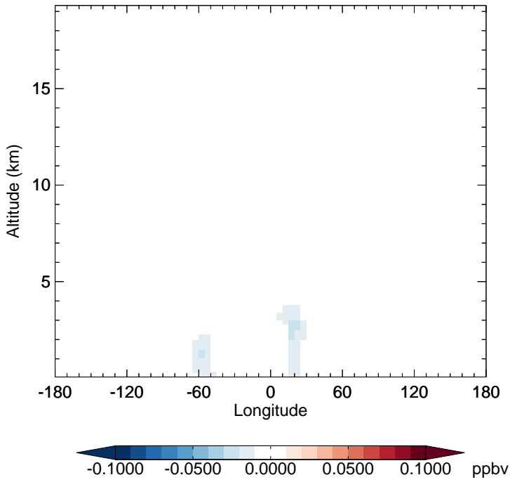
v11-02f-Run1 - v11-02e-Run1 TSOA3 - Diff along 15S for Oct
