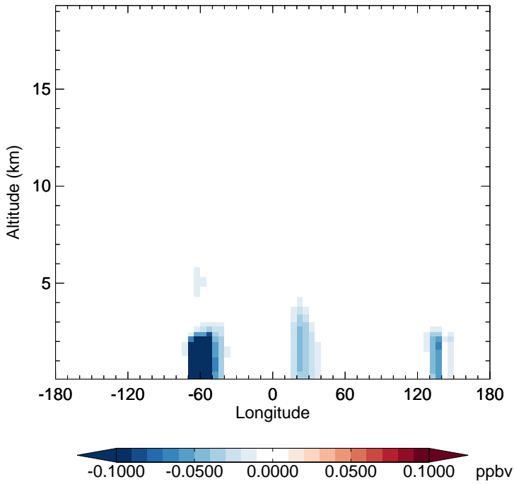
v11-02f-Run1 - v11-02e-Run0 RIPA - Diff along 15S for Oct
