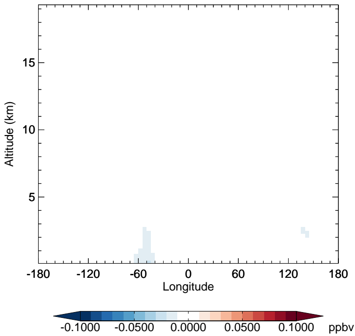
v11-02f-Run1 - v11-02e-Run0 ISOG1 - Diff along 15S for Oct
