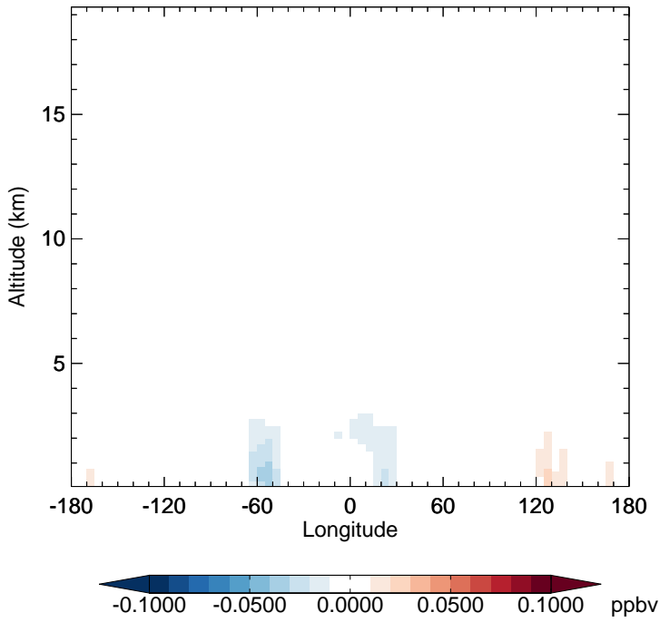
v11-02f-Run1 - v11-02e-Run1 TSOG2 - Diff along 15S for Oct
