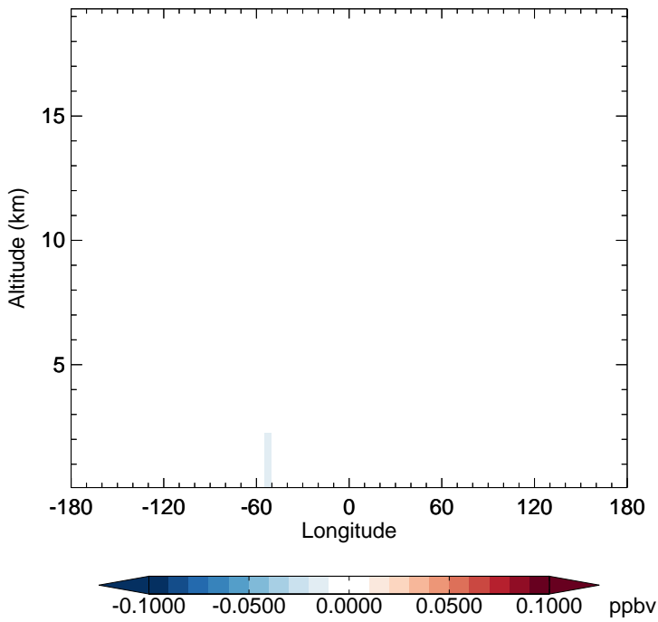
v11-02f-Run1 - v11-02e-Run0 IEPOXD - Diff along 15S for Oct
