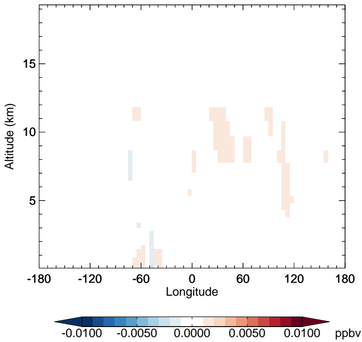
v11-02f-Run1 - v11-02e-Run0 R4N2 - Diff along 15S for Oct
