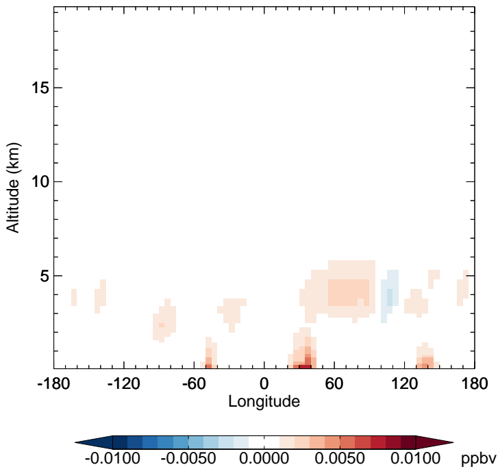
v11-02f-Run1 - v11-02e-Run0 NO3 - Diff along 15S for Oct
