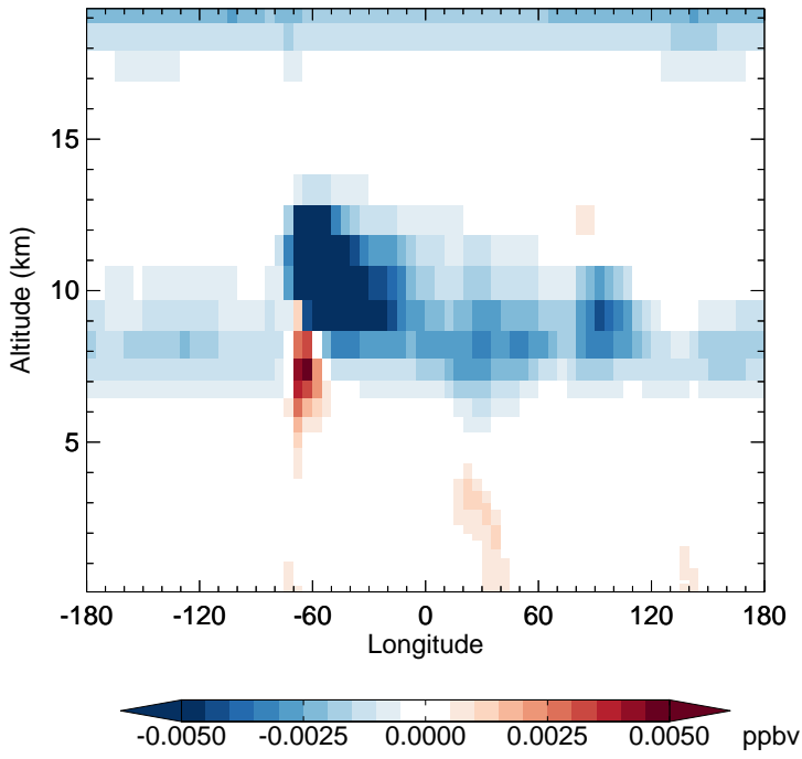
v11-02f-Run1 - v11-02e-Run1 HNO 4 - Diff along 15S for Oct
