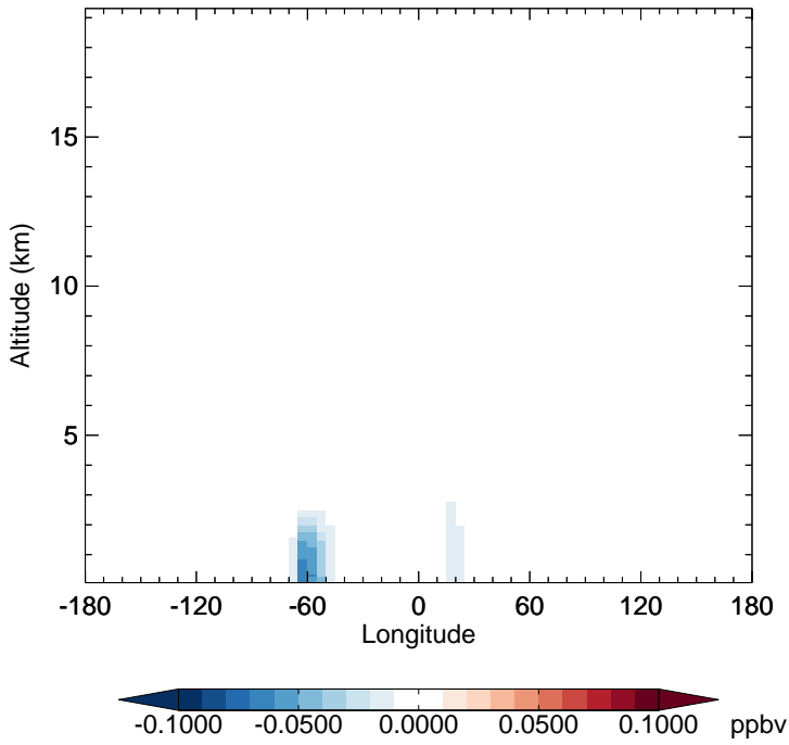
v11-02f-Run1 - v11-02e-Run1 TSOA0 - Diff along 15S for Oct
