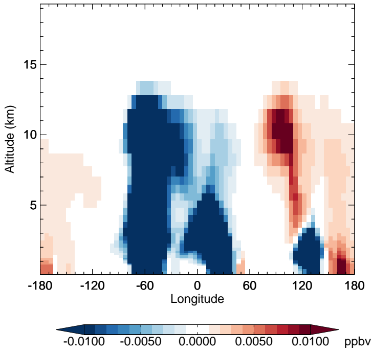
v11-02f-Run1 - v11-02e-Run1 MAP - Diff along 15S for Oct
