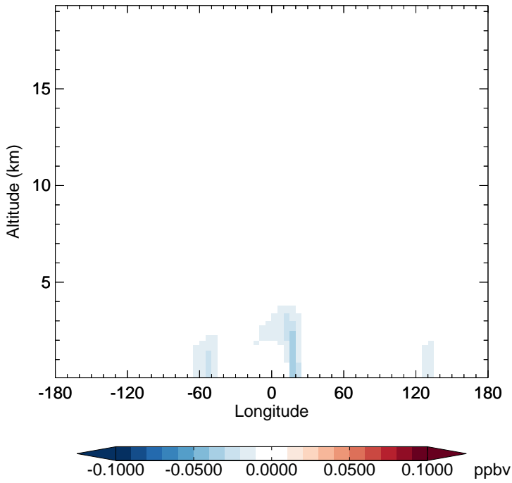
v11-02f-Run1 - v11-02e-Run1 SOAGX - Diff along 15S for Oct
