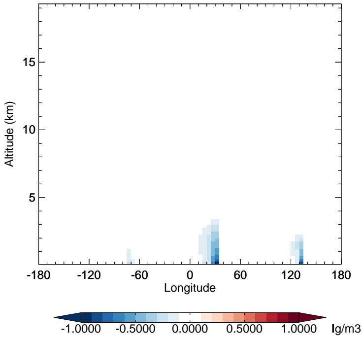
v11-02f-Run1 - v11-02e-Run1 SO 2 - Diff along 15S for Oct
