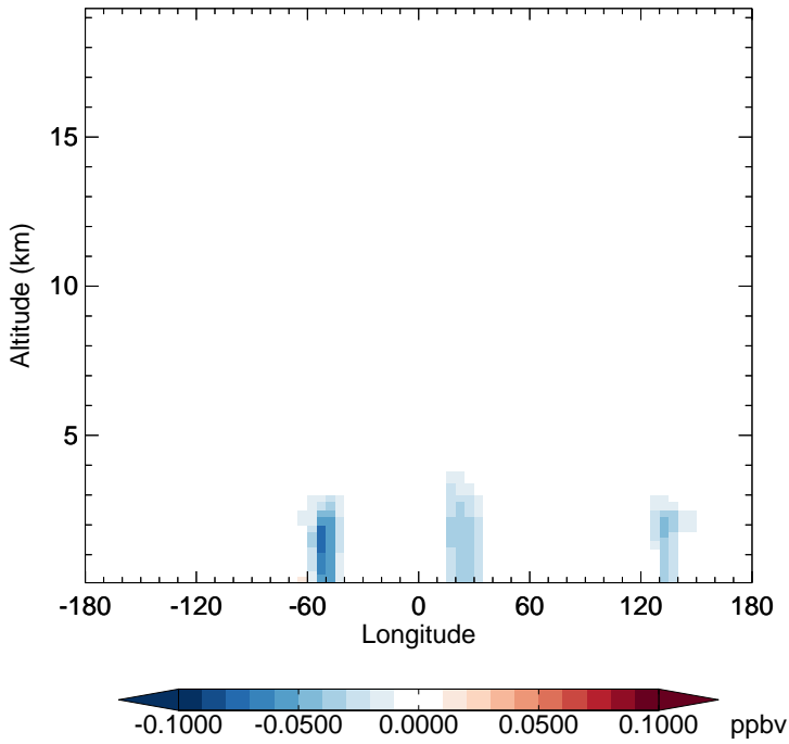
v11-02f-Run1 - v11-02e-Run0 MGLY - Diff along 15S for Oct
