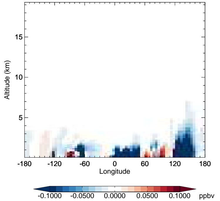
v11-02f-Run1 - v11-02e-Run0 TOLU - Diff along 42N for Oct
