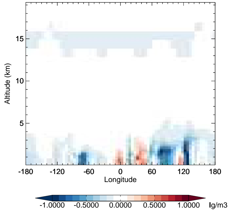
v11-02f-Run1 - v11-02e-Run0 SO4 - Diff along 42N for Oct
