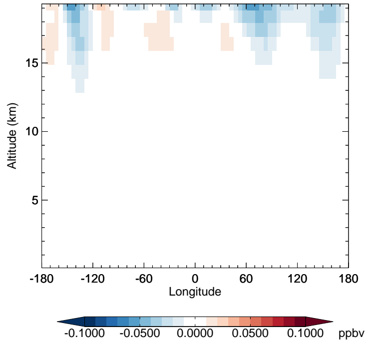
v11-02f-Run1 - v11-02e-Run0 OCS - Diff along 42N for Oct
