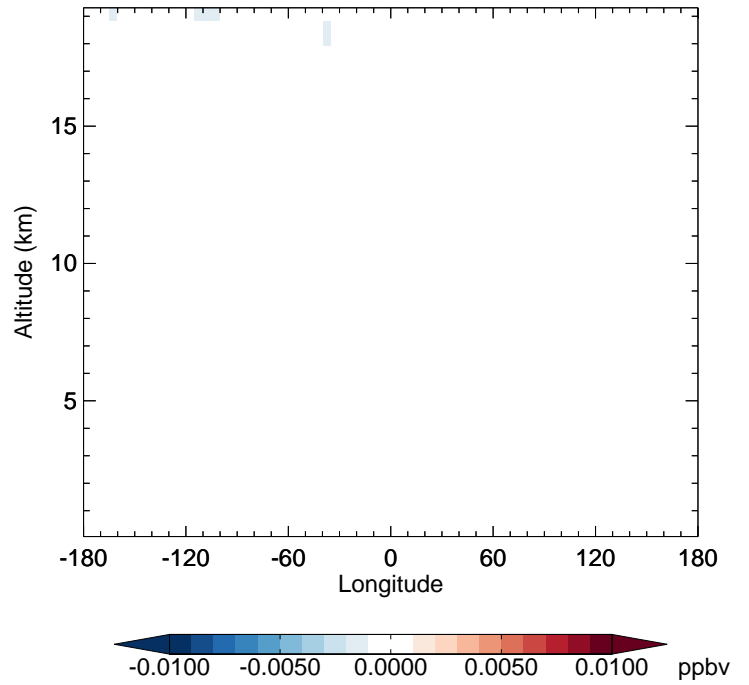
v11-02f-Run1 - v11-02e-Run0 BrNO3 - Diff along 42N for Oct
