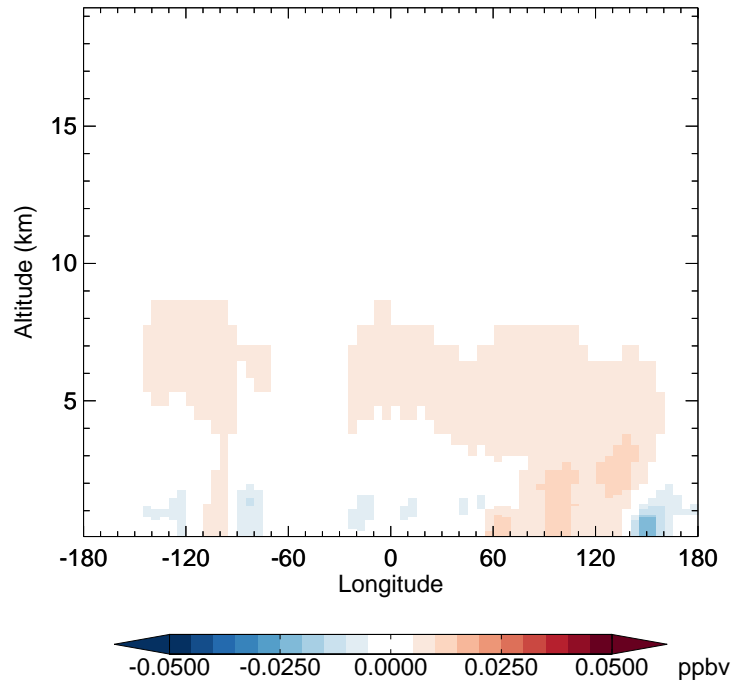
v11-02f-Run1 - v11-02e-Run1 MP - Diff along 42N for Oct
