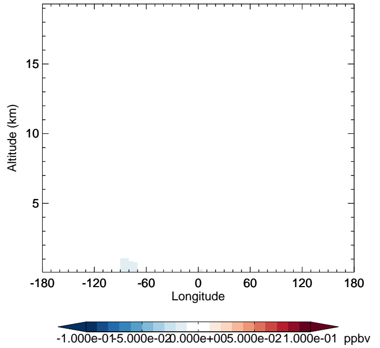
v11-02f-Run1 - v11-02e-Run1 MONITA - Diff along 42N for Oct
