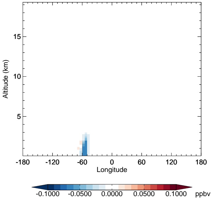
v11-02f-Run1 - v11-02e-Run0 TSOA0 - Diff along 15S for Oct
