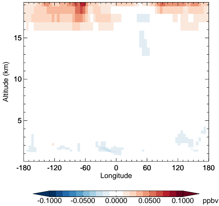
v11-02f-Run1 - v11-02e-Run0 CH3Cl - Diff along 15S for Oct
