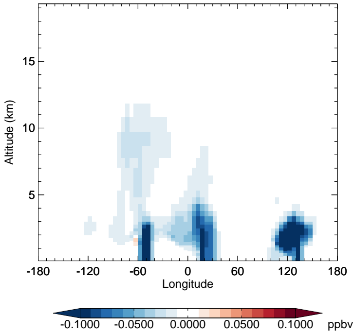
v11-02f-Run1 - v11-02e-Run0 ISO3 - Diff along 15S for Oct
