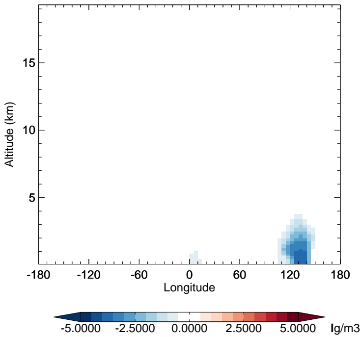
v11-02f-Run1 - v11-02e-Run0 DST2 - Diff along 15S for Oct
