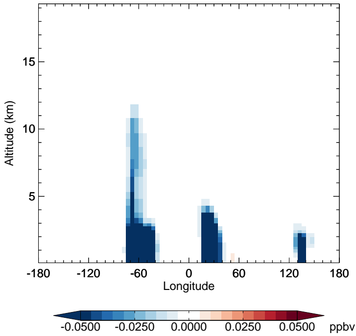
v11-02f-Run1 - v11-02e-Run1 MVK - Diff along 15S for Oct
