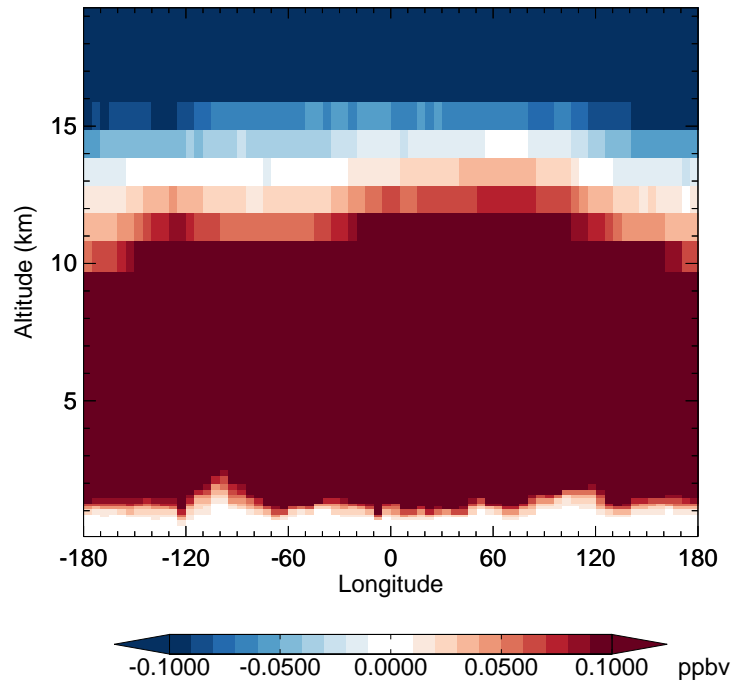
v11-02f-Run1 - v11-02e-Run1 CH4 - Diff along 42N for Oct
