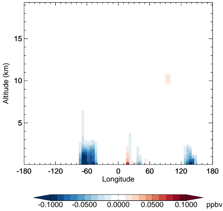
v11-02f-Run1 - v11-02e-Run1 TOLU - Diff along 15S for Oct
