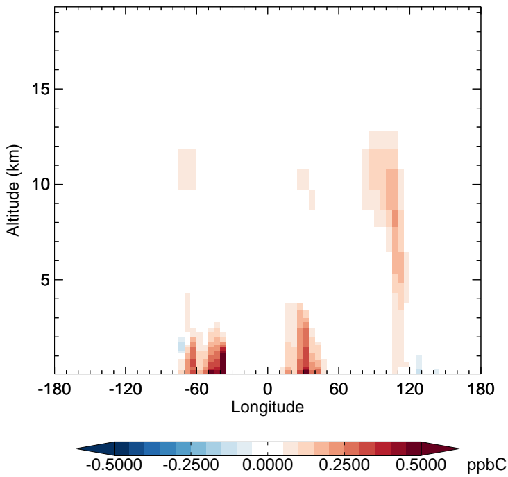
v11-02f-Run1 - v11-02e-Run0 ALK4 - Diff along 15S for Oct
