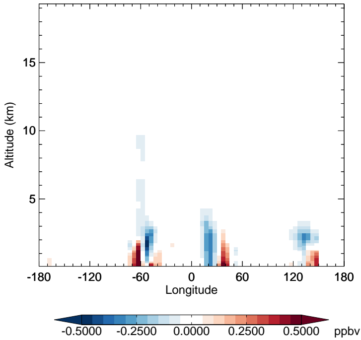
v11-02f-Run1 - v11-02e-Run0 CH 2 O - Diff along 15S for Oct
