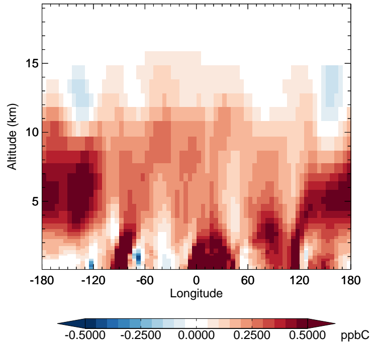
v11-02f-Run1 - v11-02e-Run0 ACET - Diff along 42N for Oct
