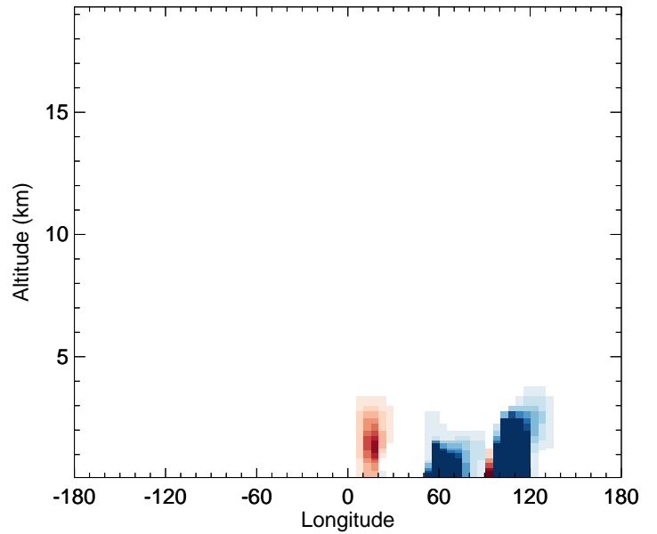
v11-02f-Run1 - v11-02e-Run0 DST4 - Diff along 42N for Oct
