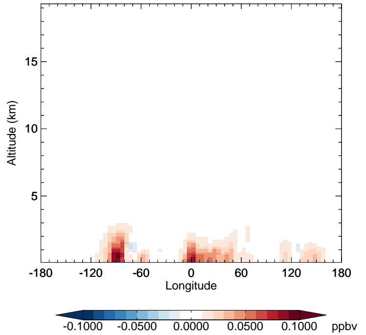
v11-02f-Run1 - v11-02e-Run0 INDIOL - Diff along 42N for Oct
