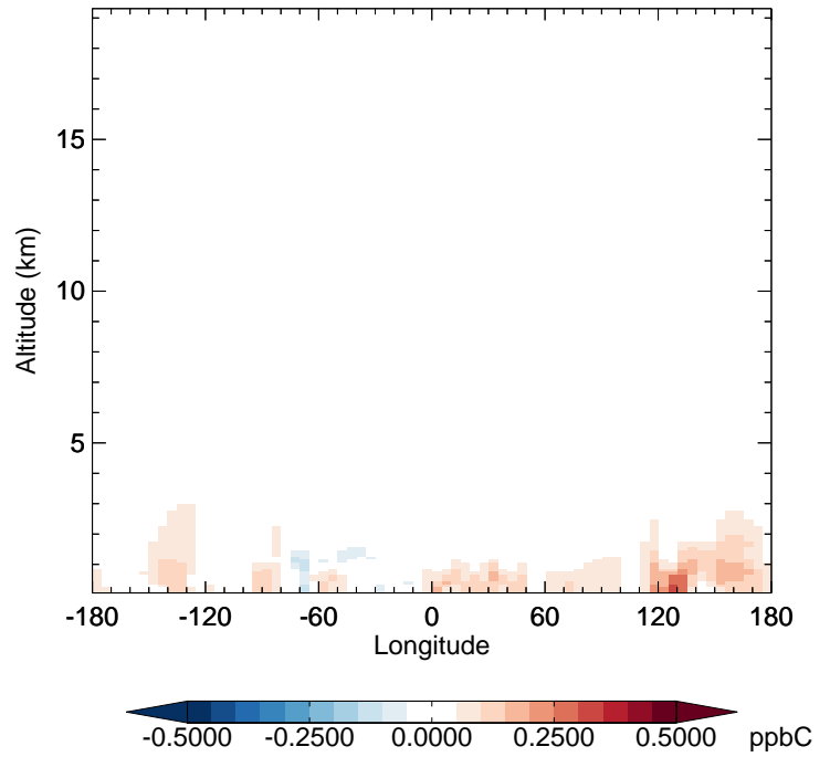
v11-02f-Run1 - v11-02e-Run0 ALD2 - Diff along 42N for Oct
