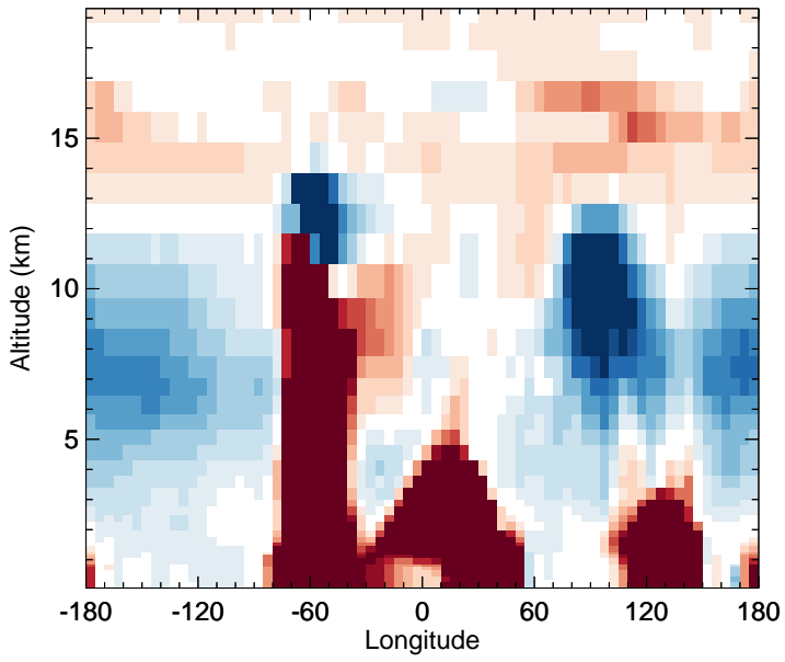
v11-02f-Run1 - v11-02e-Run1 OH - Diff along 15S for Oct
