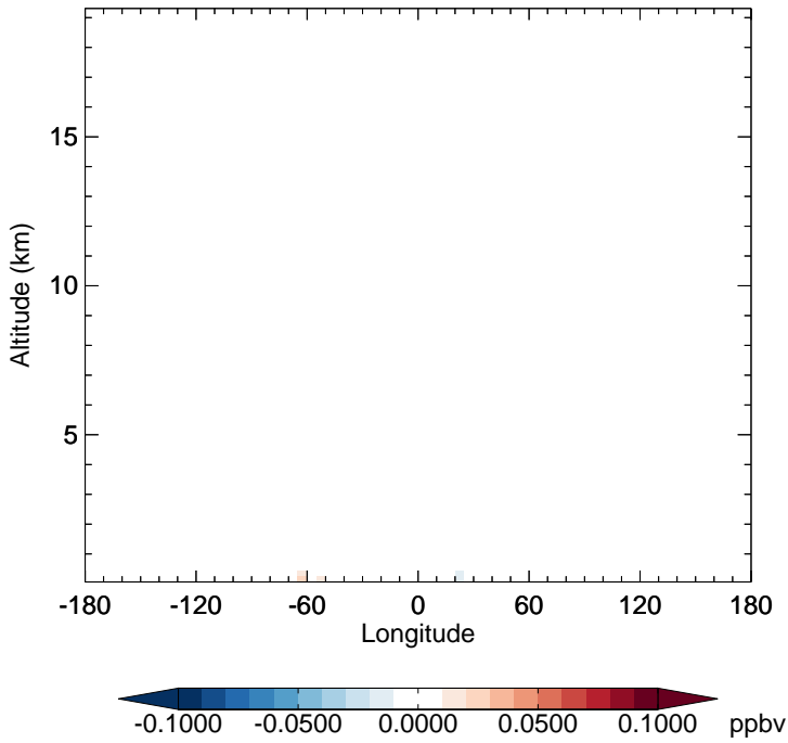
v11-02f-Run1 - v11-02e-Run0 ISN1 - Diff along 15S for Oct
