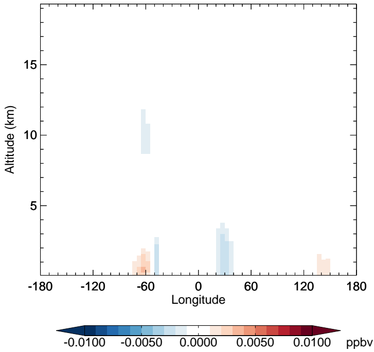
v11-02f-Run1 - v11-02e-Run1 MVKN - Diff along 15S for Oct
