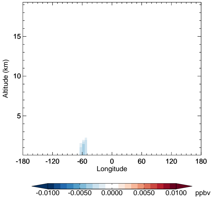
v11-02f-Run1 - v11-02e-Run0 MOBA - Diff along 15S for Oct
