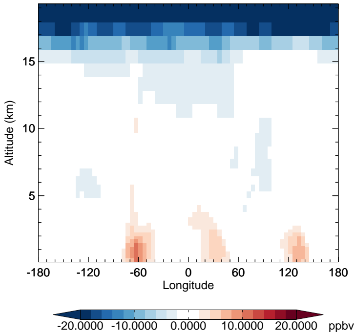
v11-02f-Run1 - v11-02e-Run1 O3 - Diff along 15S for Oct
