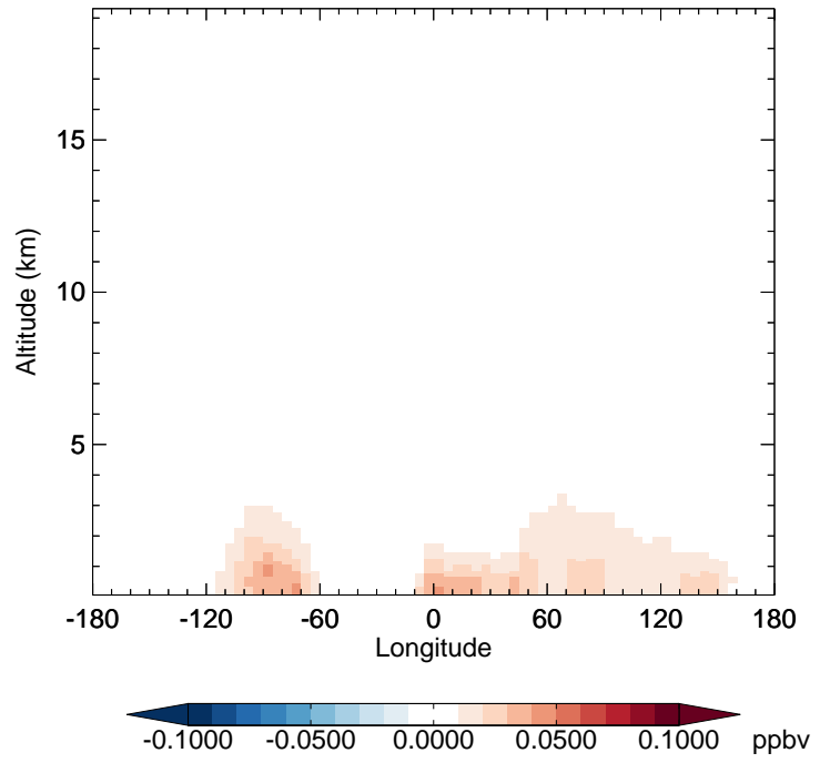
v11-02f-Run1 - v11-02e-Run1 INDIOL - Diff along 42N for Oct
