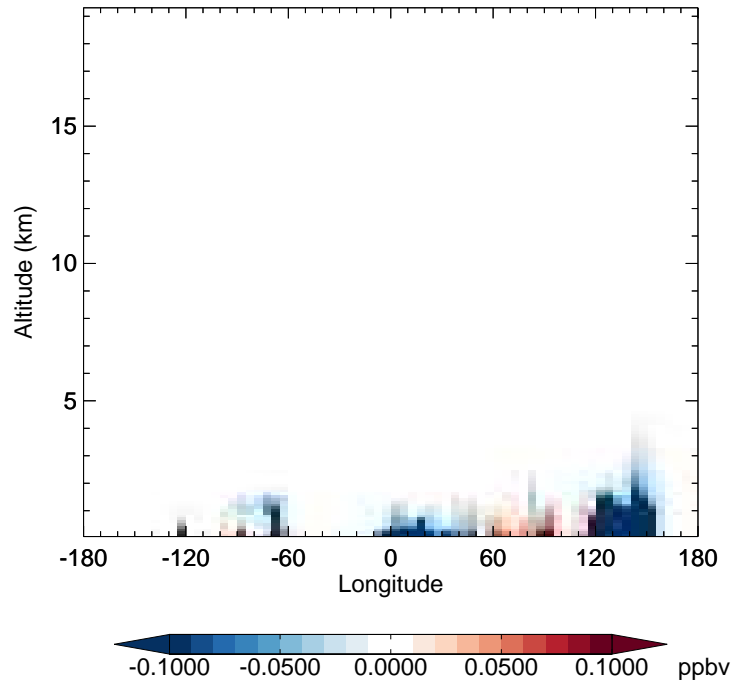
v11-02f-Run1 - v11-02e-Run0 XYLE - Diff along 42N for Oct
