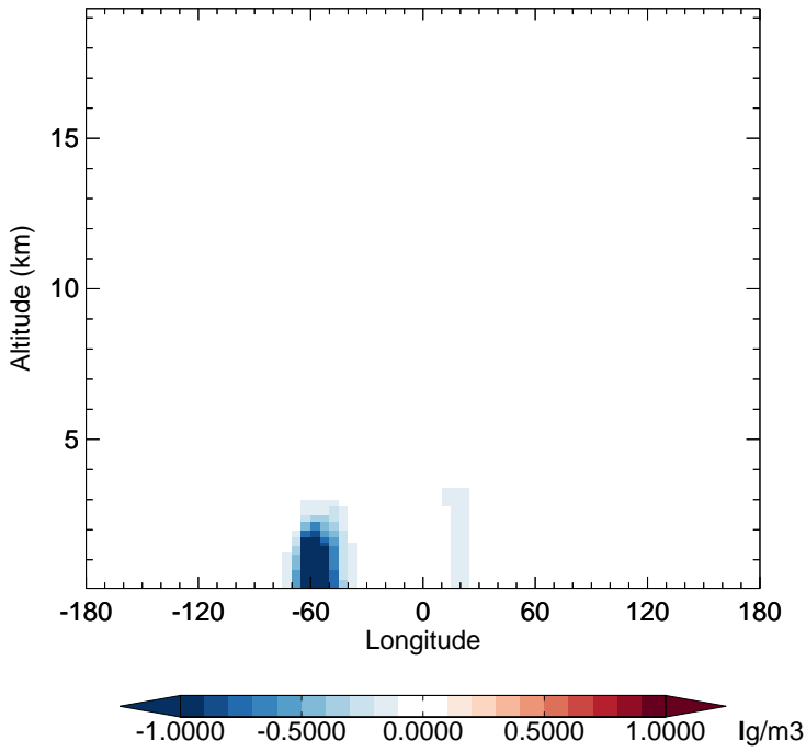
v11-02f-Run1 - v11-02e-Run1 SOAS - Diff along 15S for Oct
