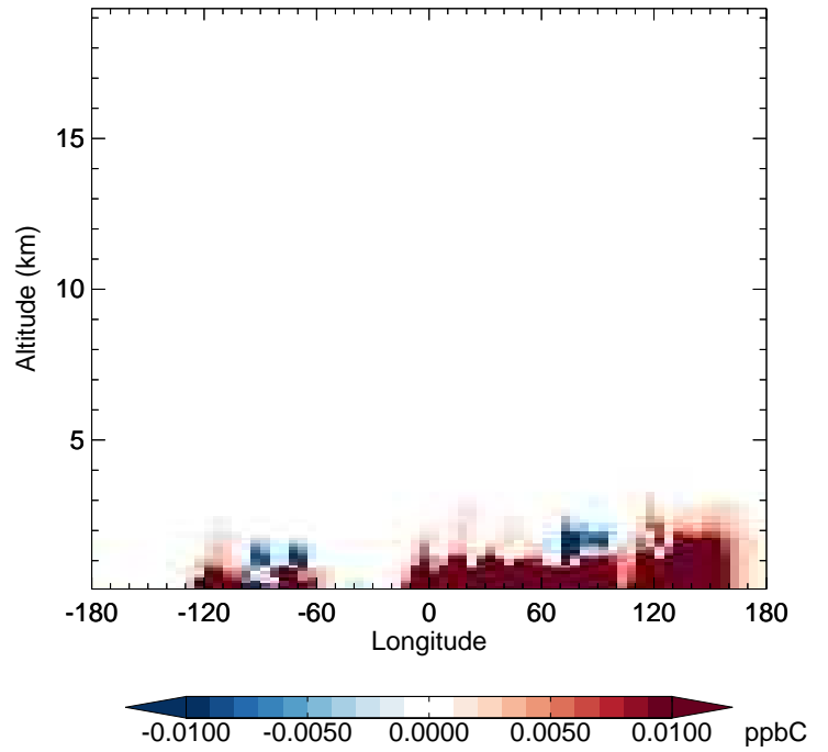
v11-02f-Run1 - v11-02e-Run0 PRPE - Diff along 42N for Oct
