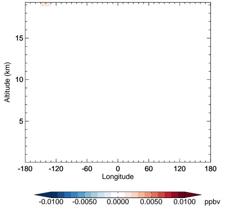
v11-02f-Run1 - v11-02e-Run1 BrO - Diff along 42N for Oct
