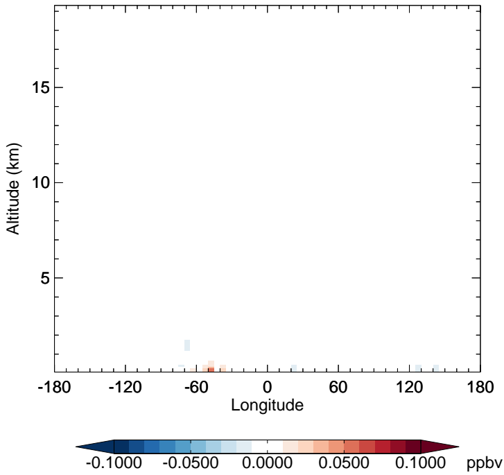
v11-02f-Run1 - v11-02e-Run0 XYLE - Diff along 15S for Oct
