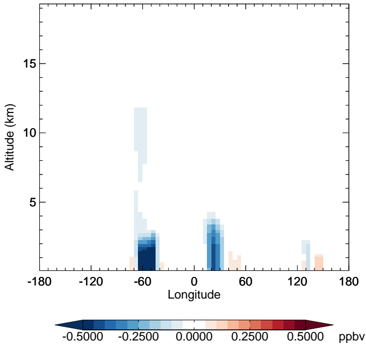
v11-02f-Run1 - v11-02e-Run1 CH 2 O - Diff along 15S for Oct
