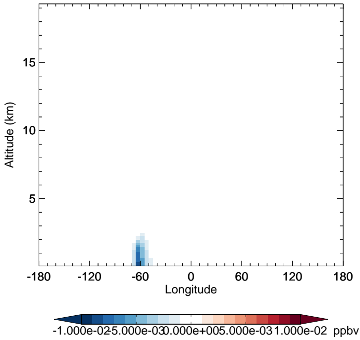
v11-02f-Run1 - v11-02e-Run1 MOBA - Diff along 15S for Oct
