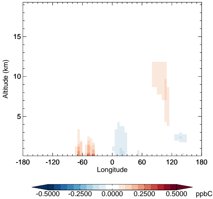
v11-02f-Run1 - v11-02e-Run0 C3H8 - Diff along 15S for Oct
