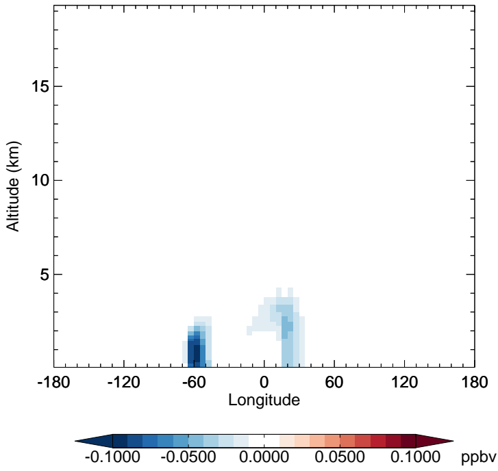
v11-02f-Run1 - v11-02e-Run1 TSOA2 - Diff along 15S for Oct
