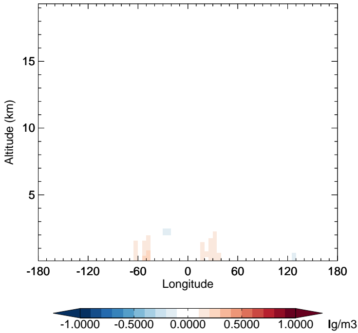
v11-02f-Run1 - v11-02e-Run0 BCPI - Diff along 15S for Oct
