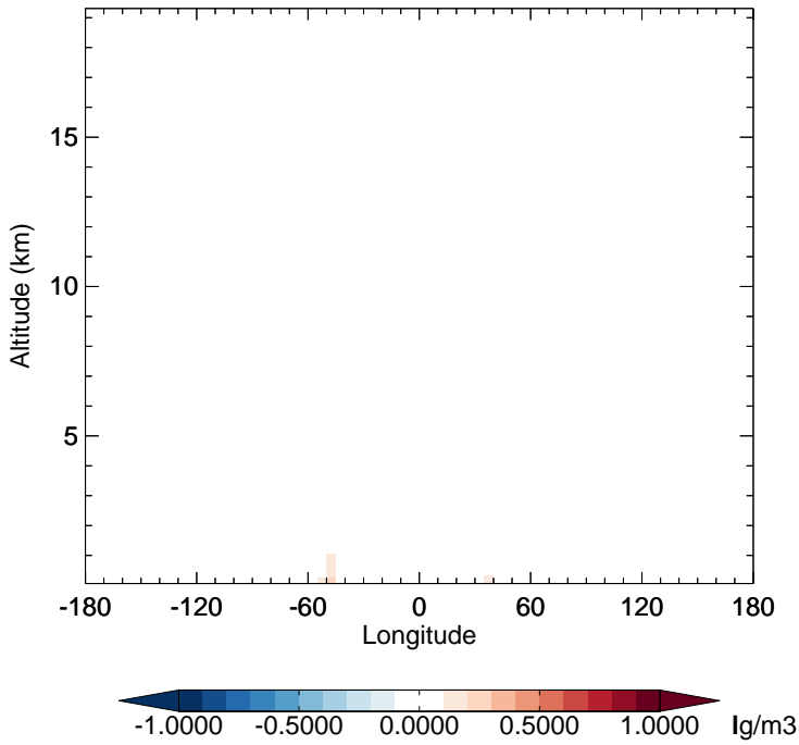
v11-02f-Run1 - v11-02e-Run0 BCPO - Diff along 15S for Oct
