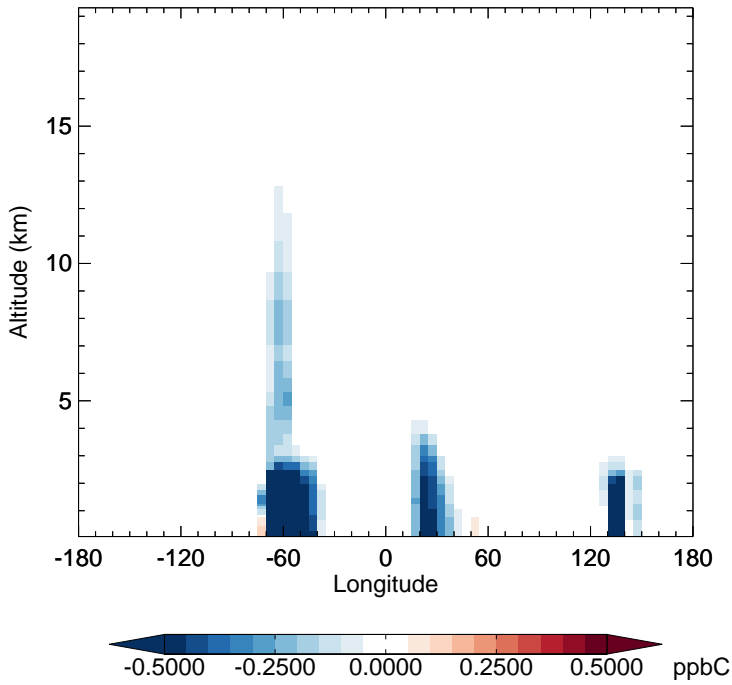
v11-02f-Run1 - v11-02e-Run0 ISOP - Diff along 15S for Oct
