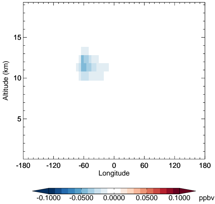
v11-02f-Run1 - v11-02e-Run1 MPN - Diff along 15S for Oct
