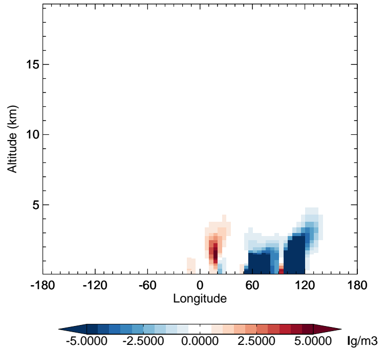
v11-02f-Run1 - v11-02e-Run0 DST3 - Diff along 42N for Oct
