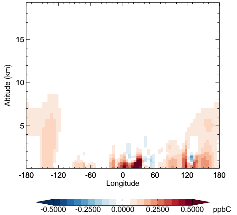
v11-02f-Run1 - v11-02e-Run0 C3H8 - Diff along 42N for Oct
