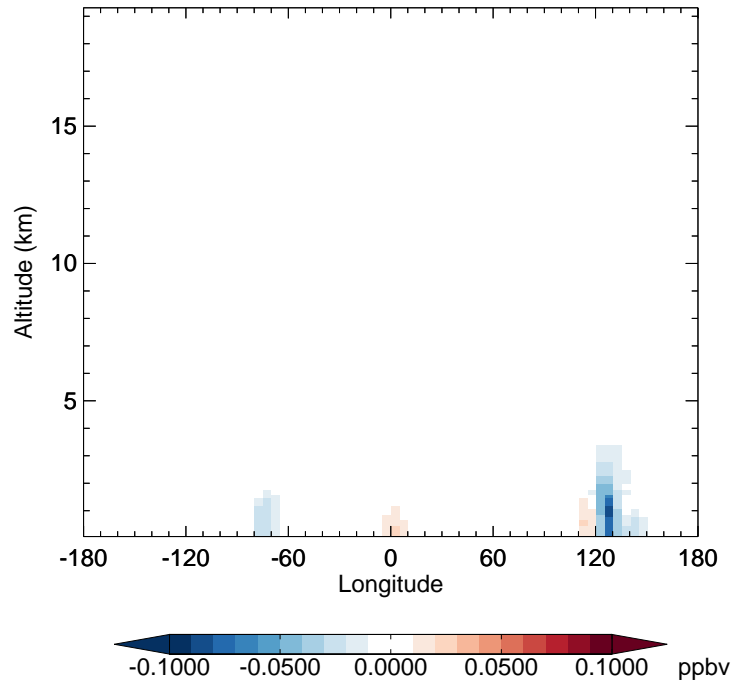
v11-02f-Run1 - v11-02e-Run0 SOAGX - Diff along 42N for Oct
