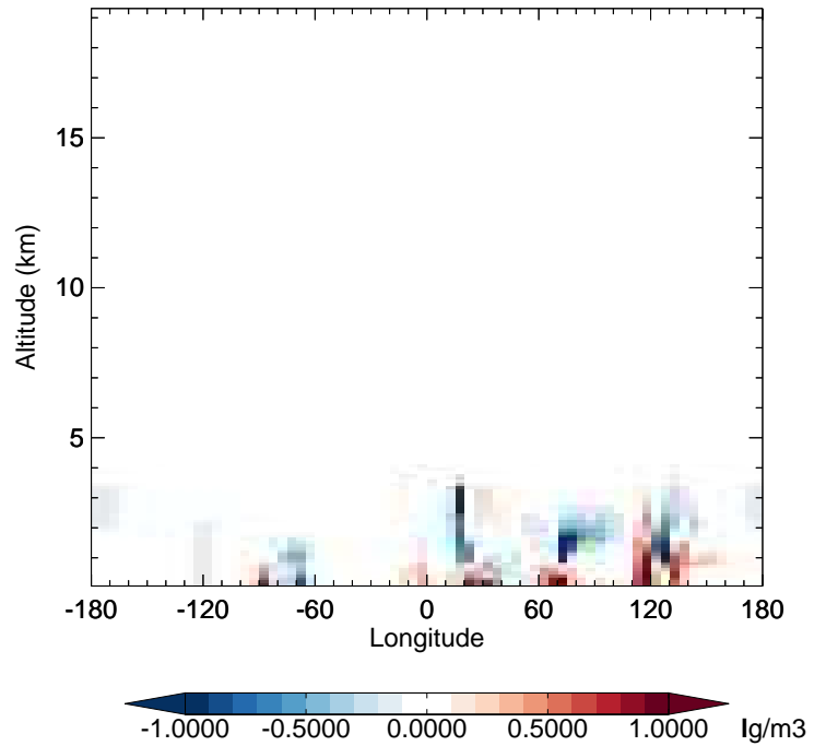
v11-02f-Run1 - v11-02e-Run0 SO 2 - Diff along 42N for Oct
