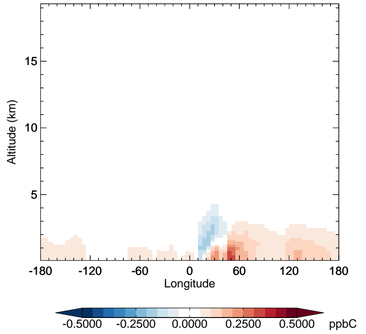
v11-02f-Run1 - v11-02e-Run1 C3H8 - Diff along 42N for Oct
