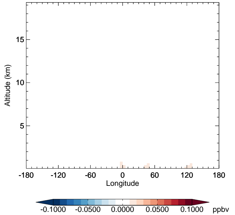
v11-02f-Run1 - v11-02e-Run0 GLYC - Diff along 42N for Oct
