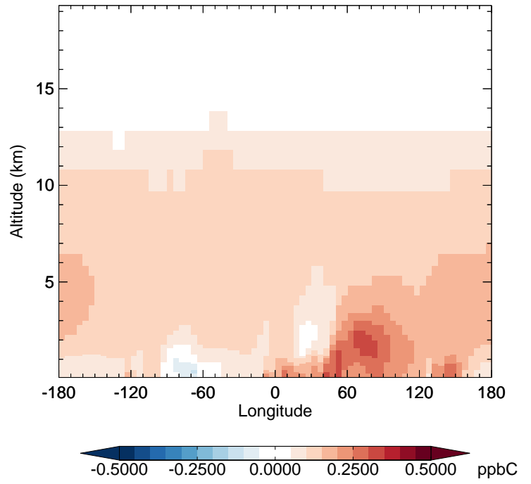
v11-02f-Run1 - v11-02e-Run1 ACET - Diff along 42N for Oct
