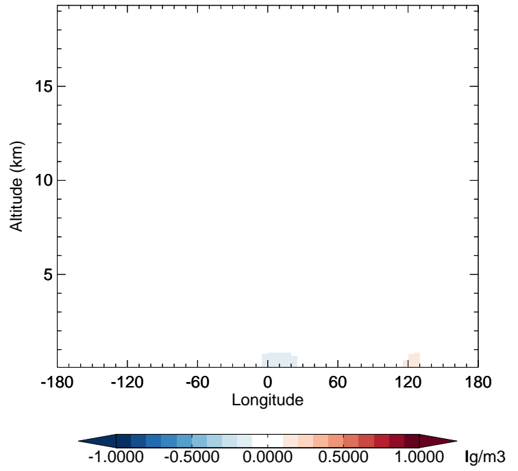
v11-02f-Run1 - v11-02e-Run1 BCPI - Diff along 42N for Oct
