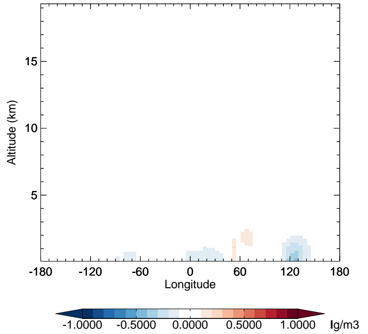
v11-02f-Run1 - v11-02e-Run1 SO4 - Diff along 42N for Oct
