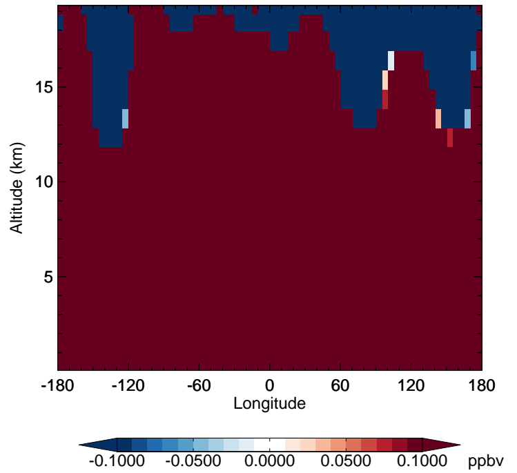
v11-02f-Run1 - v11-02e-Run0 N2O - Diff along 42N for Oct
