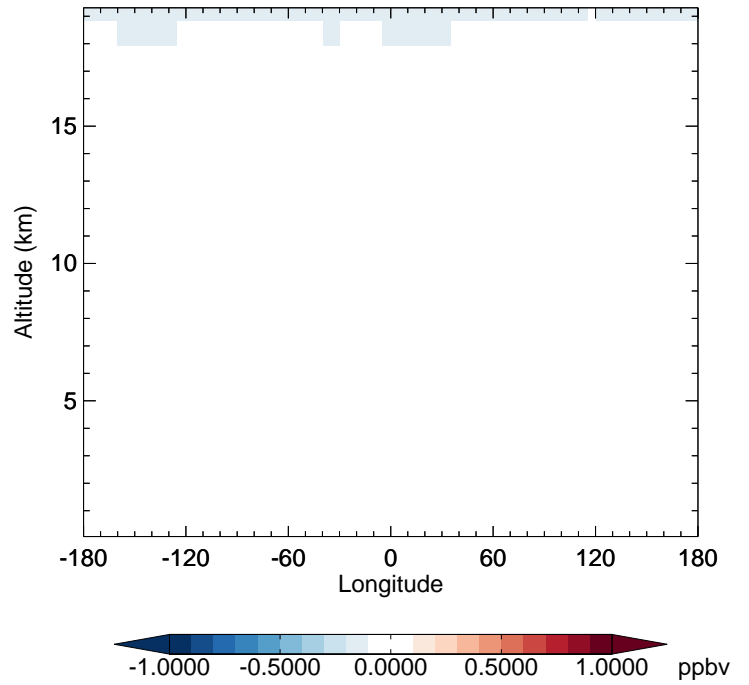
v11-02f-Run1 - v11-02e-Run0 NO - Diff along 42N for Oct
