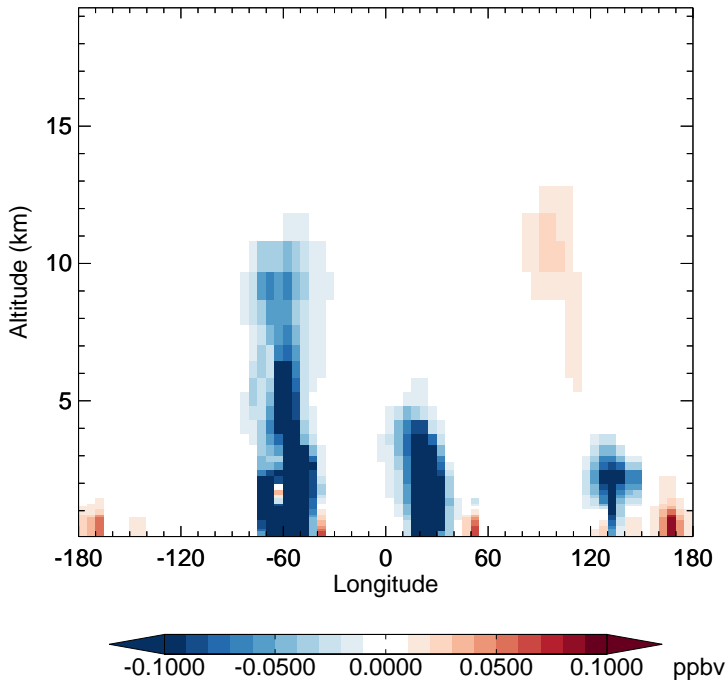
v11-02f-Run1 - v11-02e-Run0 EOH - Diff along 15S for Oct
