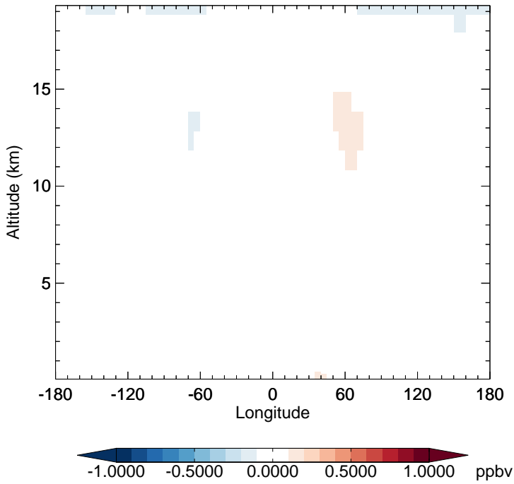
v11-02f-Run1 - v11-02e-Run0 NO - Diff along 15S for Oct
