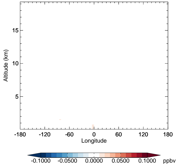
v11-02f-Run1 - v11-02e-Run0 IMAE - Diff along 42N for Oct
