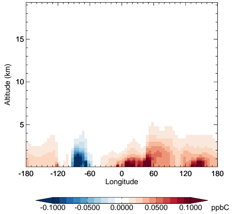
v11-02f-Run1 - v11-02e-Run1 MEK - Diff along 42N for Oct
