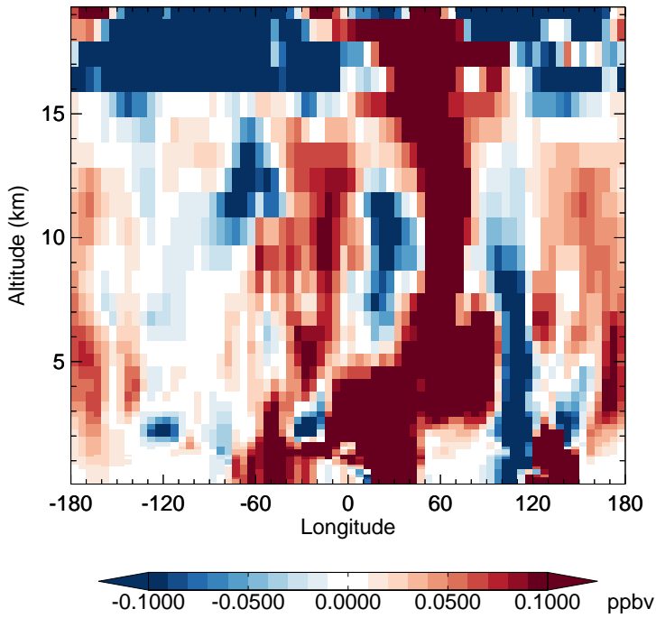
v11-02f-Run1 - v11-02e-Run0 HNO 3 - Diff along 15S for Oct
