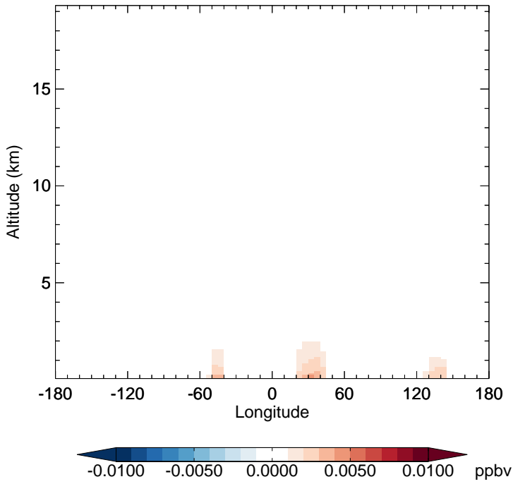
v11-02f-Run1 - v11-02e-Run1 NO3 - Diff along 15S for Oct
