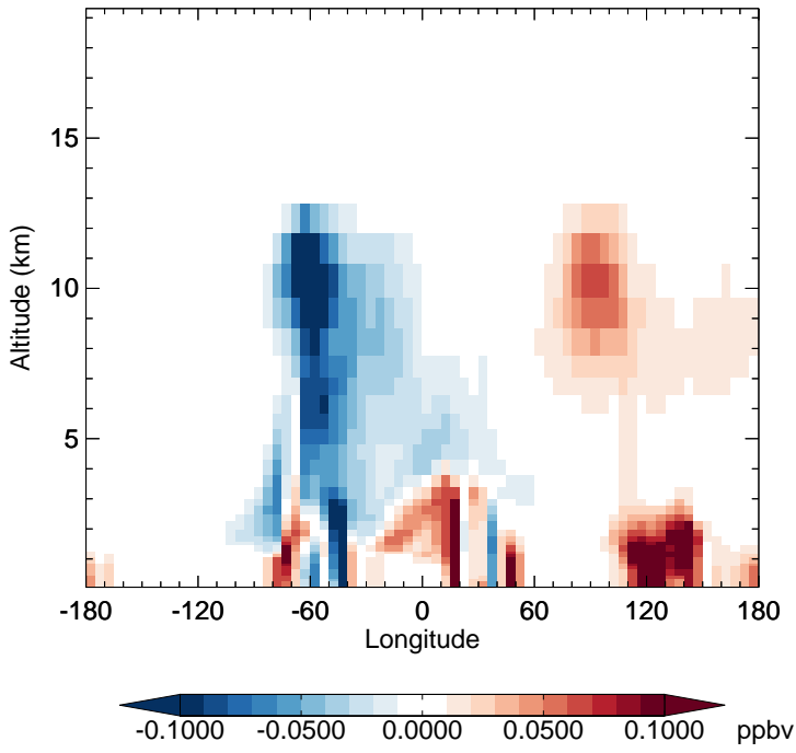
v11-02f-Run1 - v11-02e-Run1 H2O2 - Diff along 15S for Oct
