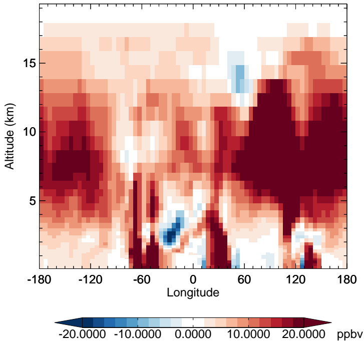
v11-02f-Run1 - v11-02e-Run0 CO - Diff along 15S for Oct
