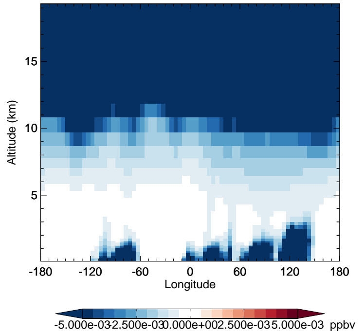
v11-02f-Run1 - v11-02e-Run1 N2O5 - Diff along 42N for Oct
