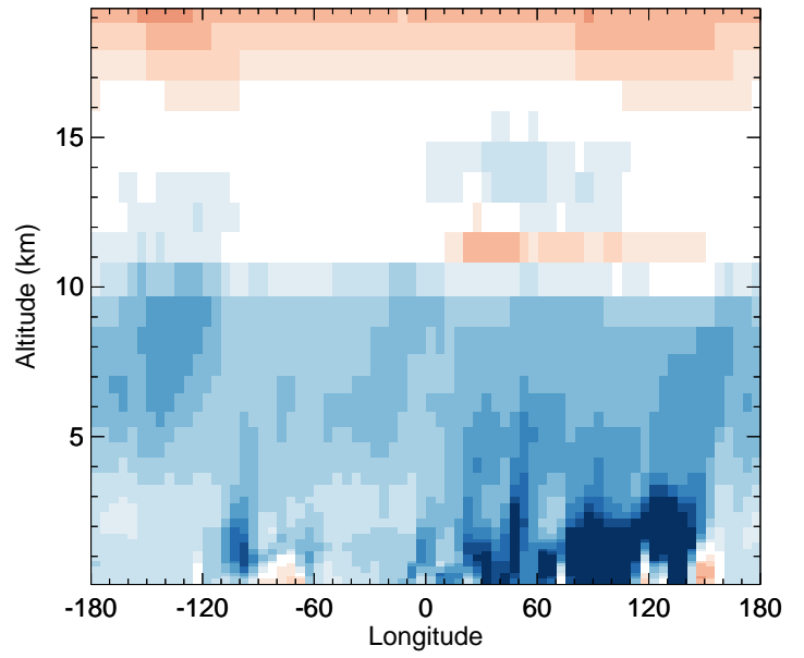
v11-02f-Run1 - v11-02e-Run1 OH - Diff along 42N for Oct
