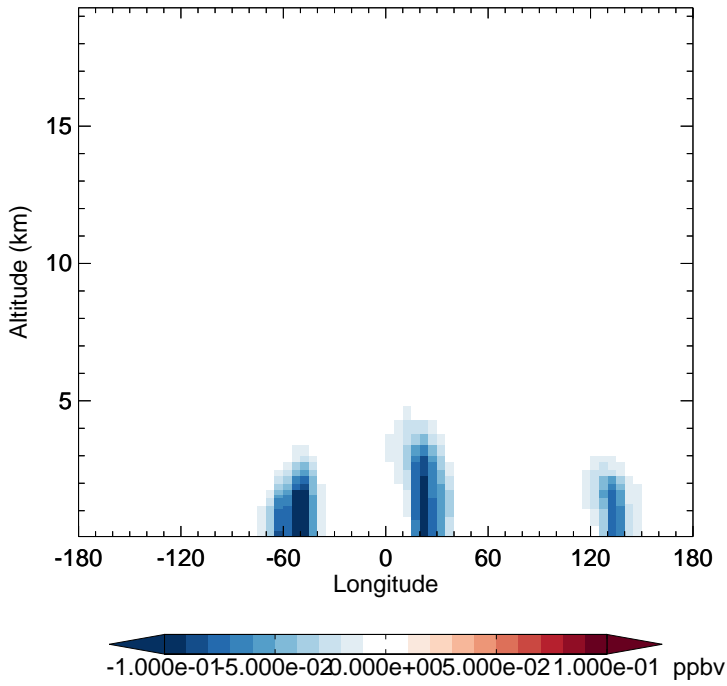
v11-02f-Run1 - v11-02e-Run1 IONITA - Diff along 15S for Oct
