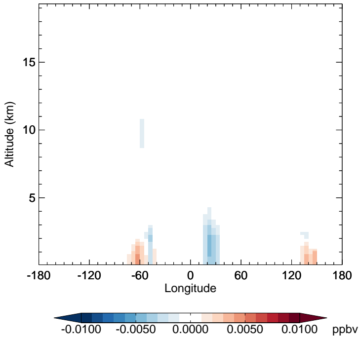
v11-02f-Run1 - v11-02e-Run0 MVKN - Diff along 15S for Oct
