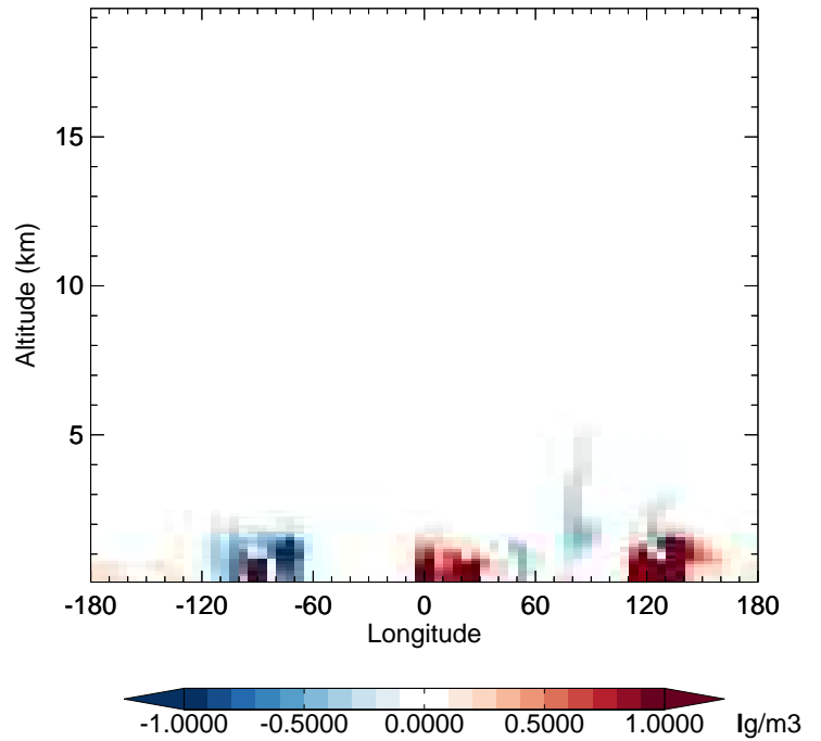
v11-02f-Run1 - v11-02e-Run0 NIT - Diff along 42N for Oct
