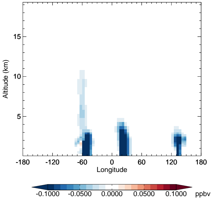
v11-02f-Run1 - v11-02e-Run0 GLYC - Diff along 15S for Oct
