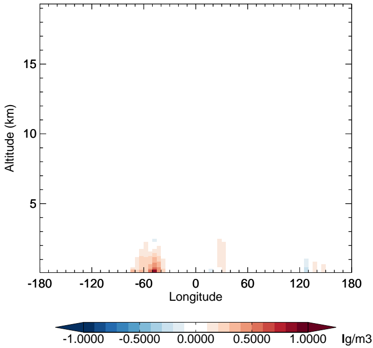
v11-02f-Run1 - v11-02e-Run0 NH3 - Diff along 15S for Oct
