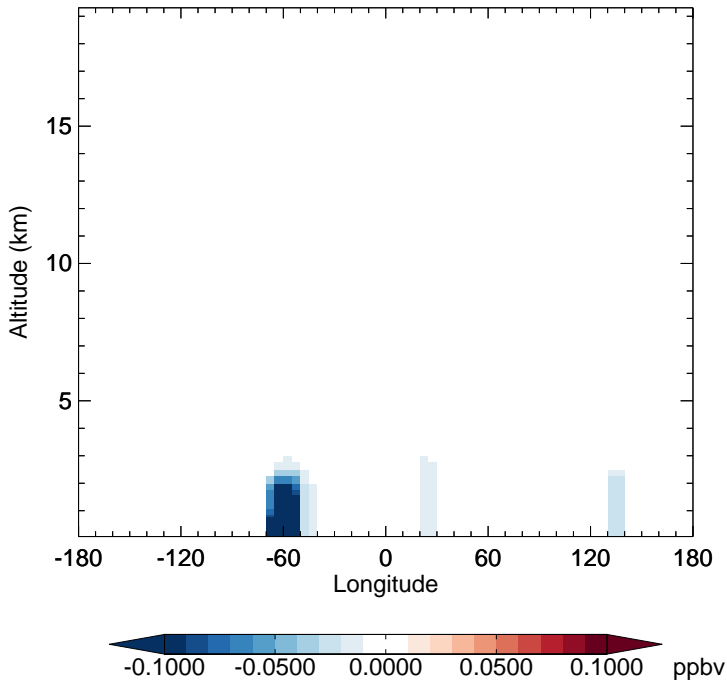
v11-02f-Run1 - v11-02e-Run0 HPALD - Diff along 15S for Oct
