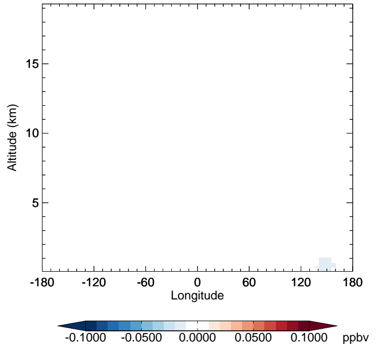
v11-02f-Run1 - v11-02e-Run1 ASOAN - Diff along 42N for Oct
