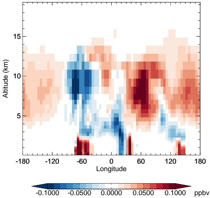
v11-02f-Run1 - v11-02e-Run0 PAN - Diff along 15S for Oct
