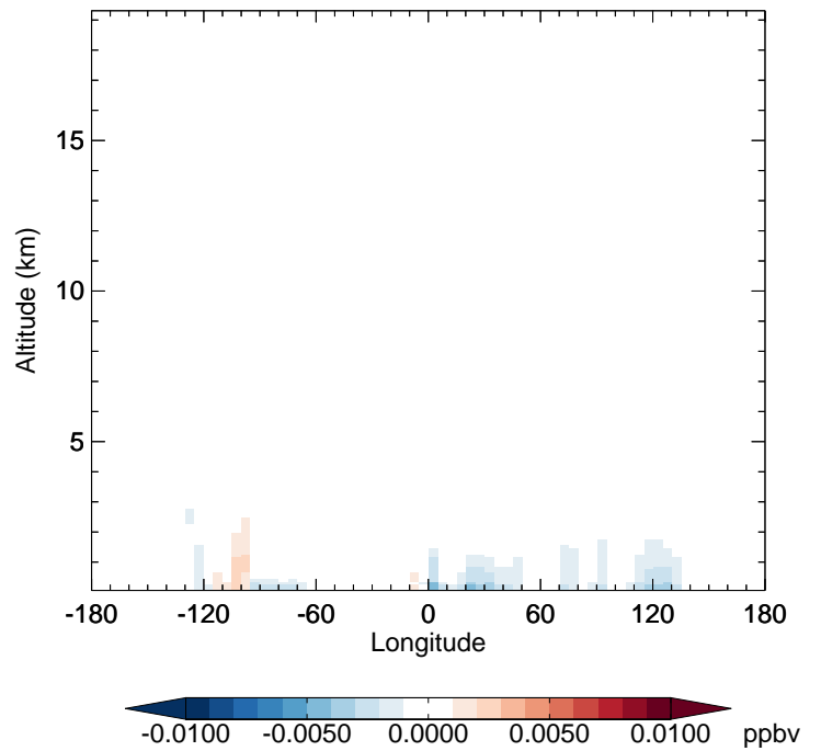
v11-02f-Run1 - v11-02e-Run0 NO3 - Diff along 42N for Oct
