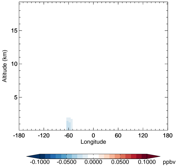
v11-02f-Run1 - v11-02e-Run1 TSOA1 - Diff along 15S for Oct
