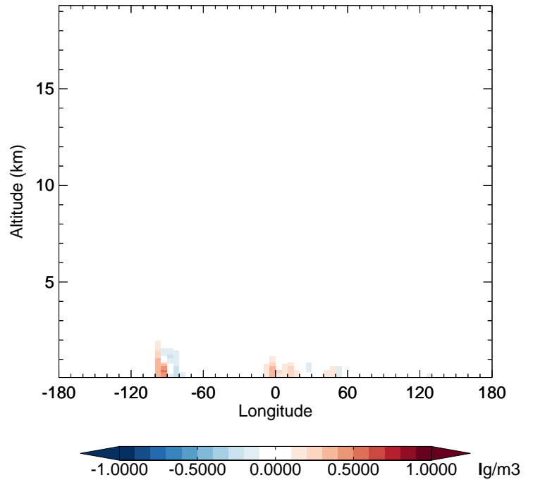
v11-02f-Run1 - v11-02e-Run0 NH3 - Diff along 42N for Oct
