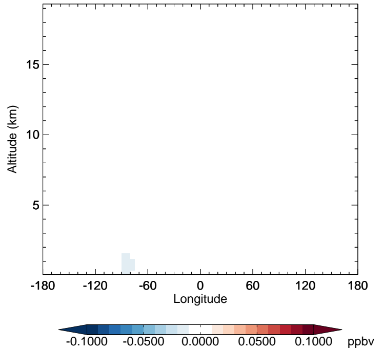
v11-02f-Run1 - v11-02e-Run1 HAC - Diff along 42N for Oct
