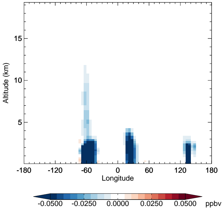
v11-02f-Run1 - v11-02e-Run0 MACR - Diff along 15S for Oct
