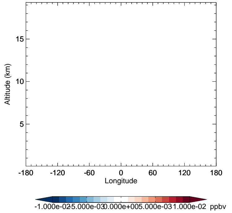
v11-02f-Run1 - v11-02e-Run1 HBr - Diff along 42N for Oct
