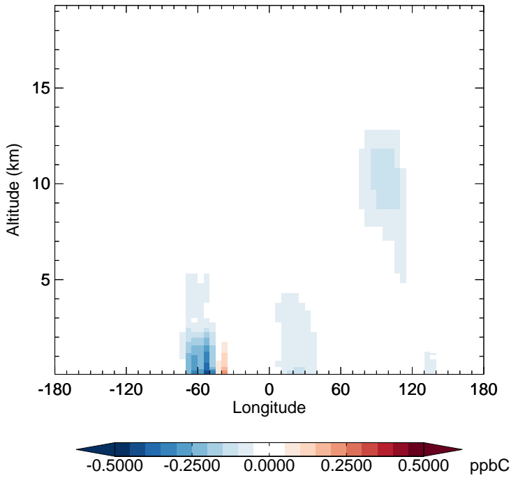
v11-02f-Run1 - v11-02e-Run1 C3H8 - Diff along 15S for Oct
