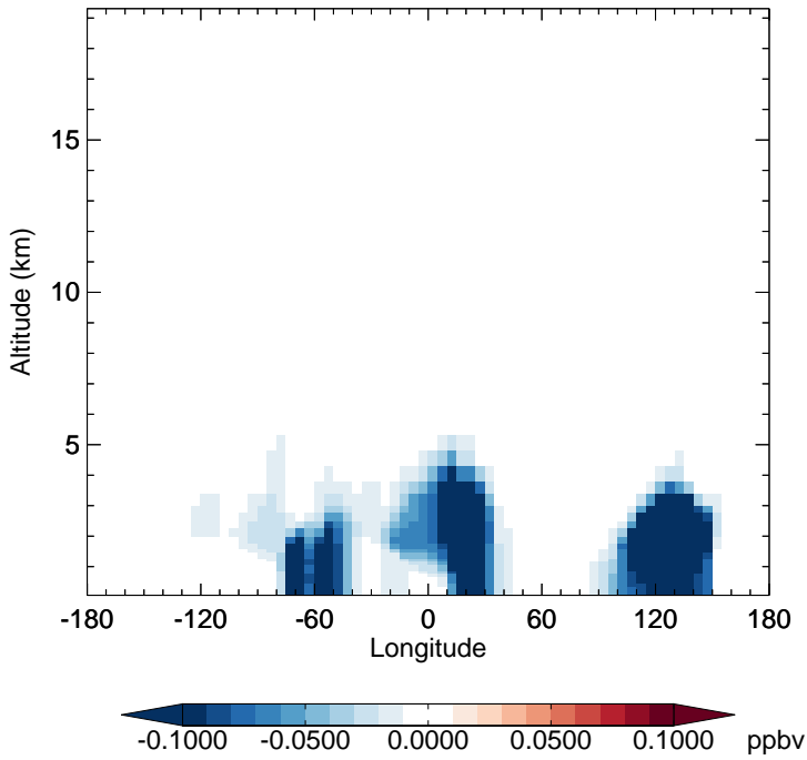
v11-02f-Run1 - v11-02e-Run0 SOAIE - Diff along 15S for Oct
