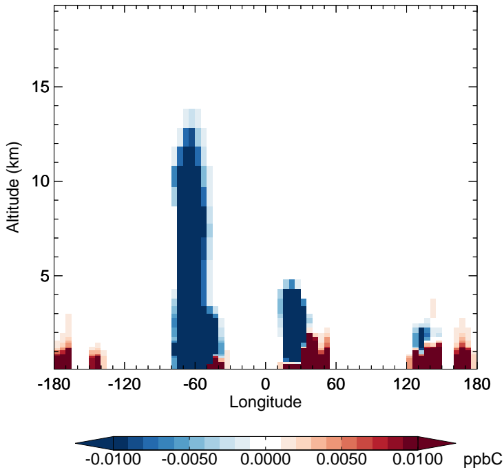
v11-02f-Run1 - v11-02e-Run1 PRPE - Diff along 15S for Oct
