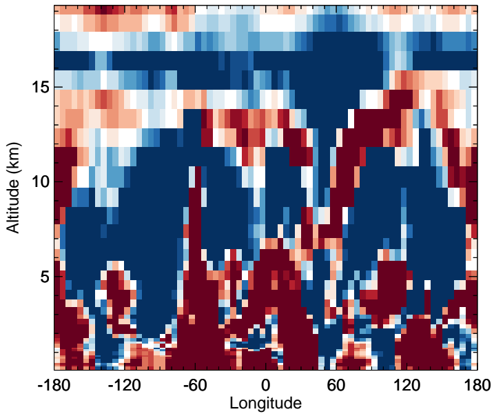
v11-02f-Run1 - v11-02e-Run0 OH - Diff along 15S for Oct
