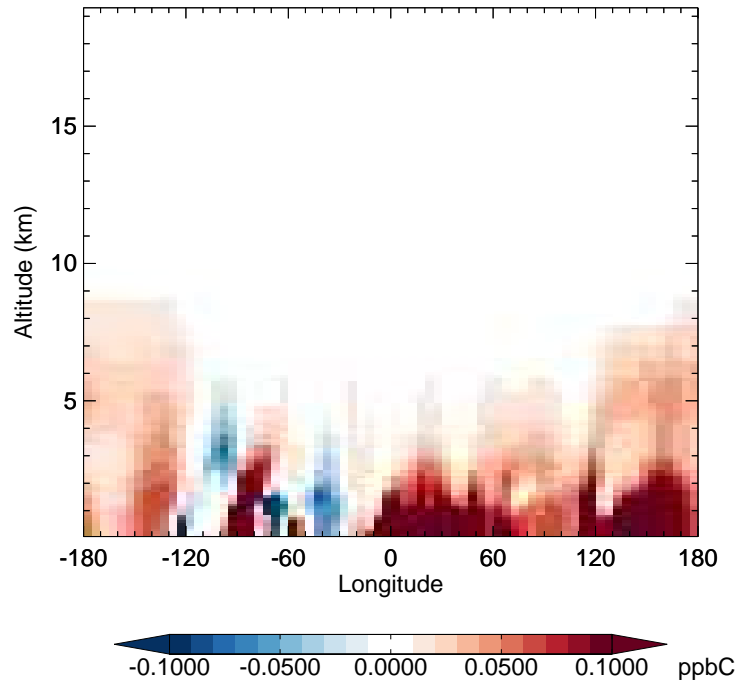
v11-02f-Run1 - v11-02e-Run0 MEK - Diff along 42N for Oct
