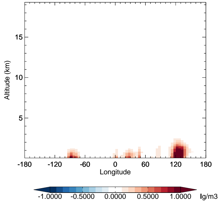
v11-02f-Run1 - v11-02e-Run1 NIT - Diff along 42N for Oct
