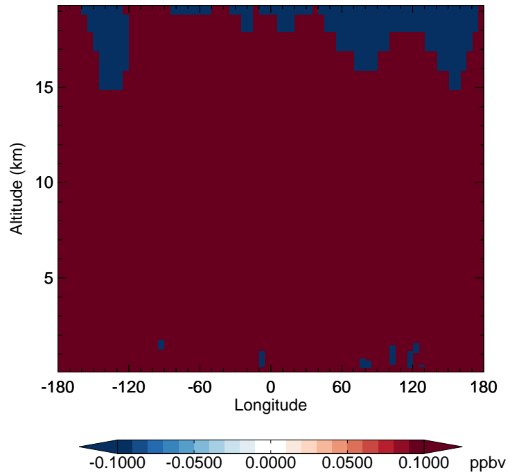
v11-02f-Run1 - v11-02e-Run0 CH4 - Diff along 42N for Oct
