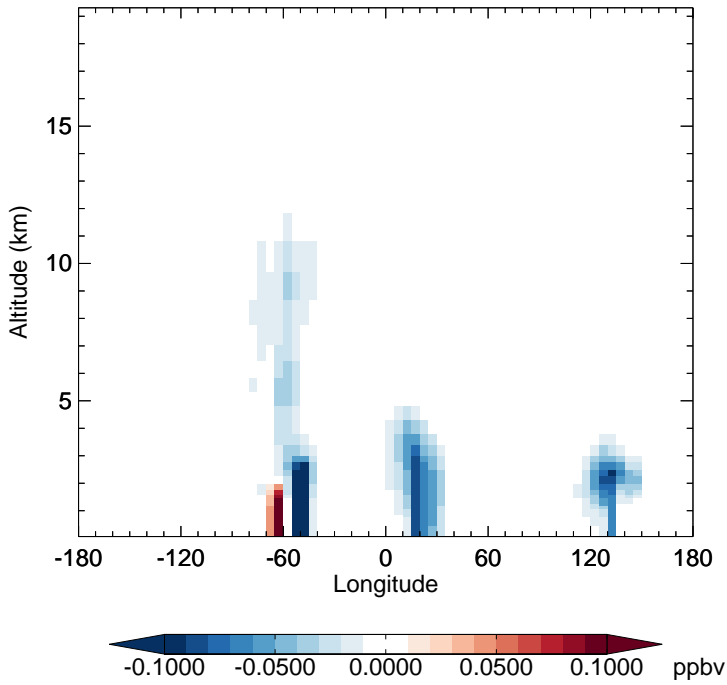
v11-02f-Run1 - v11-02e-Run0 IMAE - Diff along 15S for Oct
