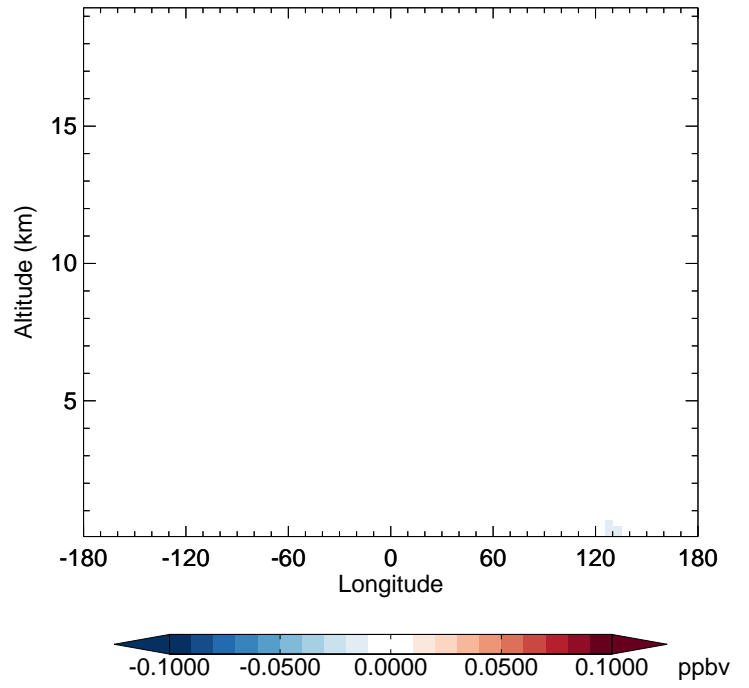
v11-02f-Run1 - v11-02e-Run1 MGLY - Diff along 42N for Oct
