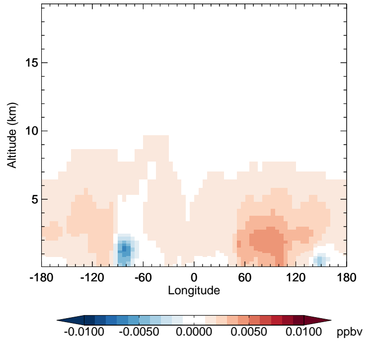
v11-02f-Run1 - v11-02e-Run1 MAP - Diff along 42N for Oct
