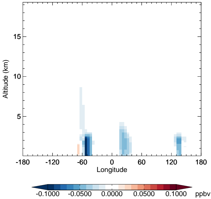
v11-02f-Run1 - v11-02e-Run0 IEPOXB - Diff along 15S for Oct
