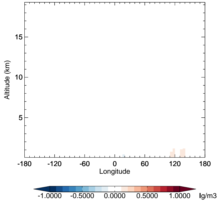
v11-02f-Run1 - v11-02e-Run0 BCPI - Diff along 42N for Oct
