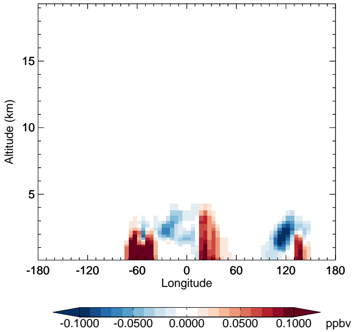
v11-02f-Run1 - v11-02e-Run0 INDIOL - Diff along 15S for Oct
