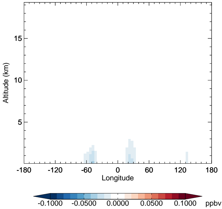
v11-02f-Run1 - v11-02e-Run1 GLYX - Diff along 15S for Oct
