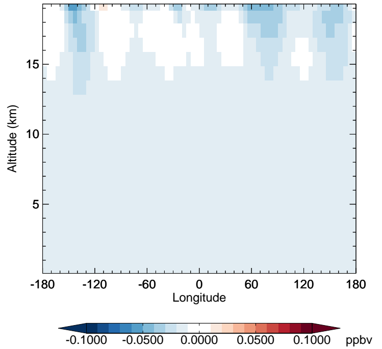
v11-02f-Run1 - v11-02e-Run0 CFC12 - Diff along 42N for Oct
