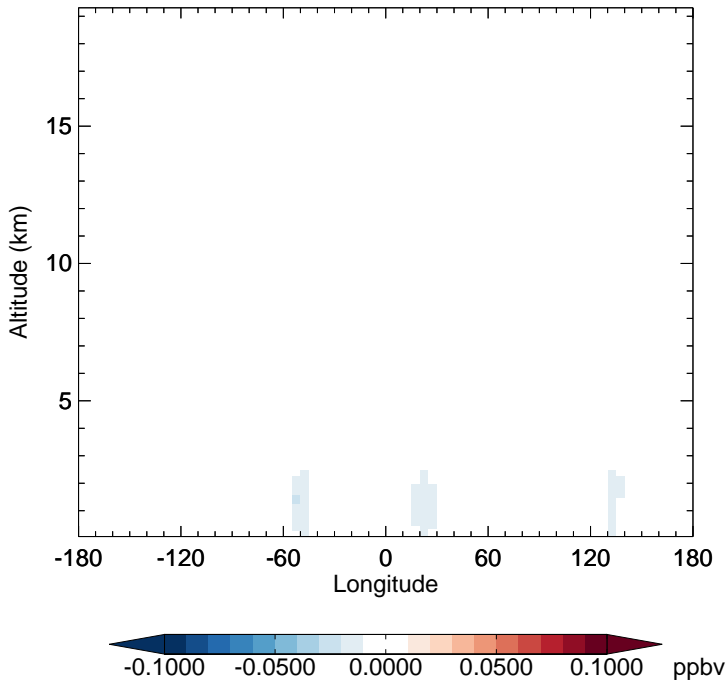
v11-02f-Run1 - v11-02e-Run0 GLYX - Diff along 15S for Oct
