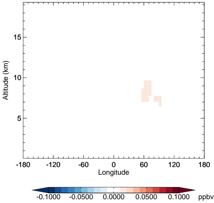
v11-02f-Run1 - v11-02e-Run1 ASOG3 - Diff along 15S for Oct
