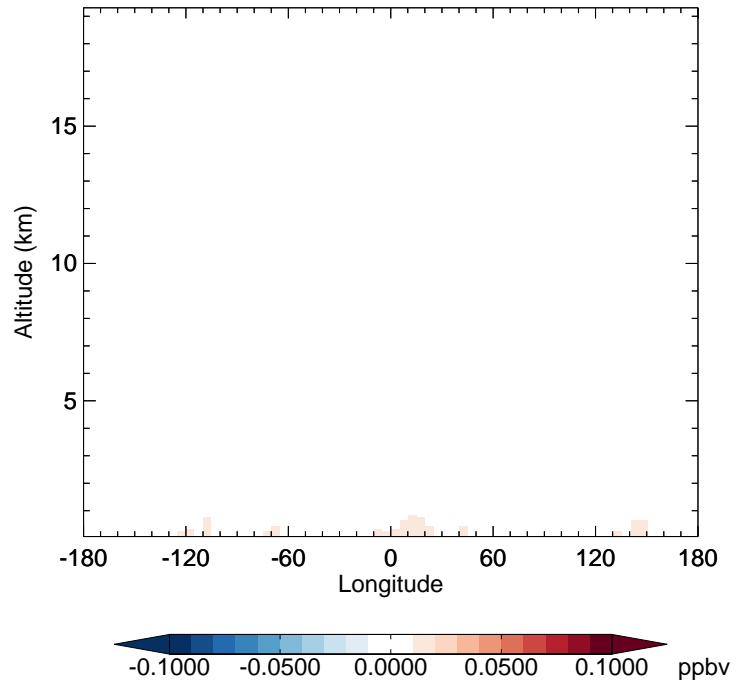
v11-02f-Run1 - v11-02e-Run1 TSOG3 - Diff along 42N for Oct
