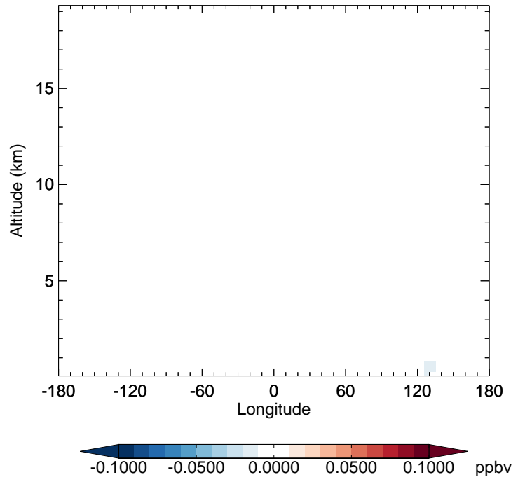
v11-02f-Run1 - v11-02e-Run1 ASOG3 - Diff along 42N for Oct
