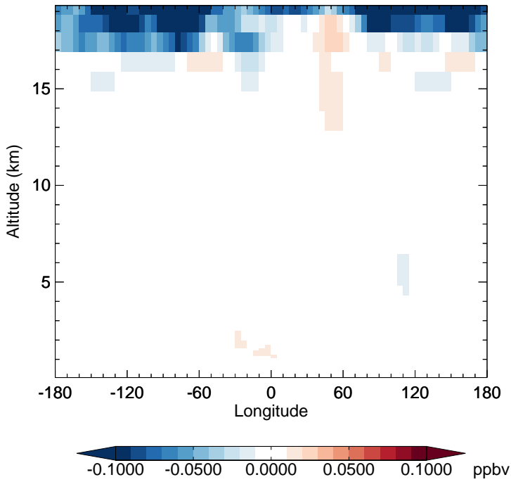
v11-02f-Run1 - v11-02e-Run0 HCl - Diff along 15S for Oct
