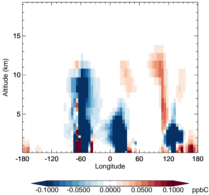
v11-02f-Run1 - v11-02e-Run0 MEK - Diff along 15S for Oct
