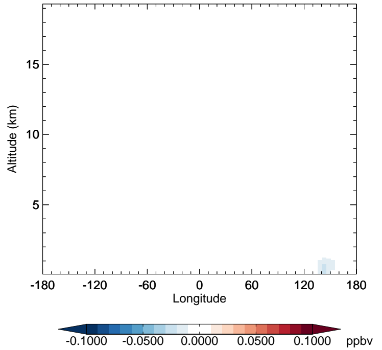
v11-02f-Run1 - v11-02e-Run0 ASOAN - Diff along 42N for Oct
