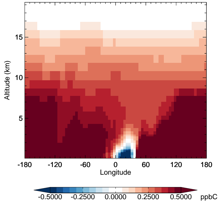
v11-02f-Run1 - v11-02e-Run1 C2H6 - Diff along 42N for Oct
