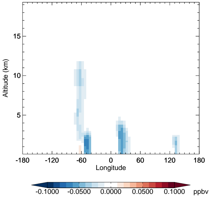
v11-02f-Run1 - v11-02e-Run1 HC187 - Diff along 15S for Oct
