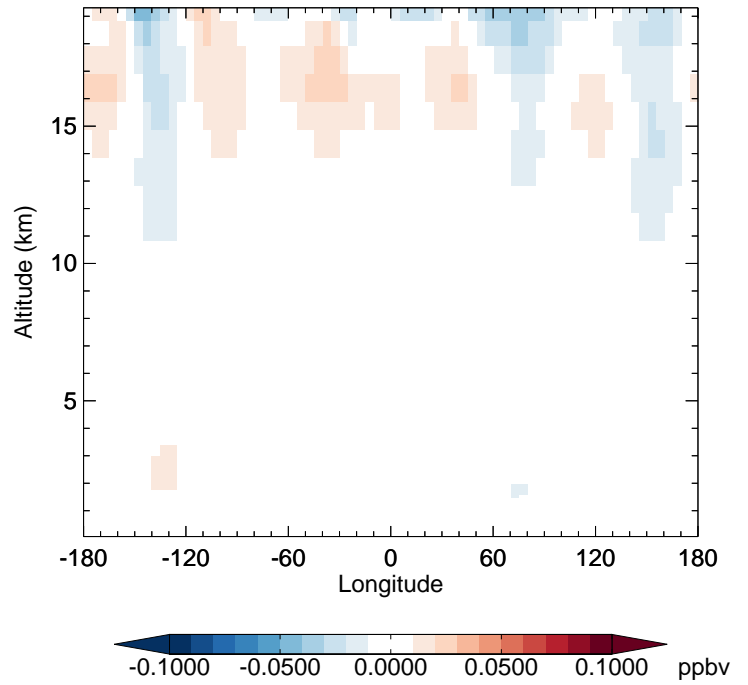
v11-02f-Run1 - v11-02e-Run0 CH3Cl - Diff along 42N for Oct
