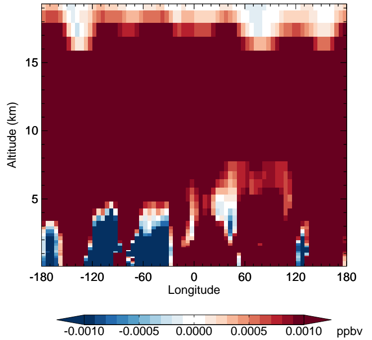
v11-02f-Run1 - v11-02e-Run0 PPN - Diff along 42N for Oct
