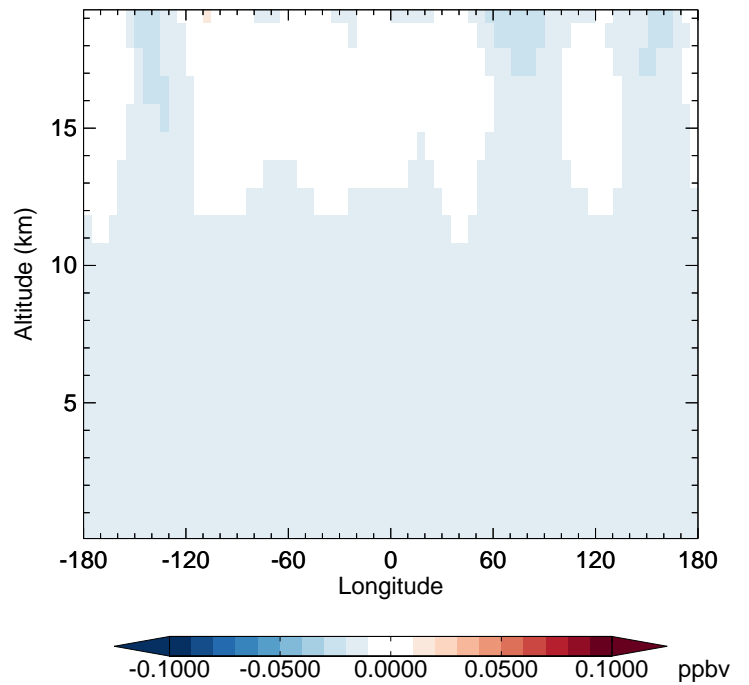
v11-02f-Run1 - v11-02e-Run0 CFC11 - Diff along 42N for Oct
