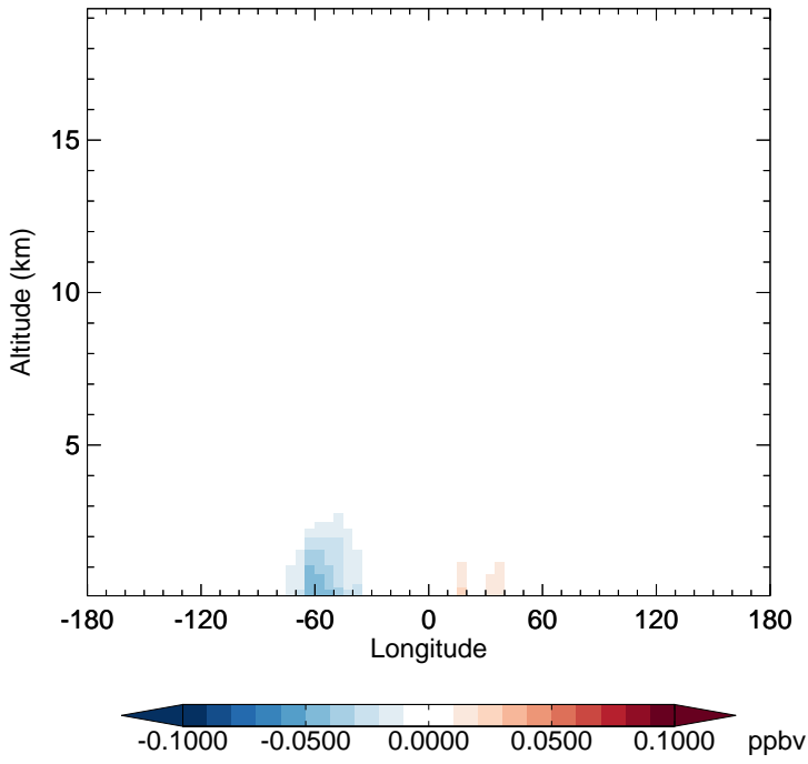
v11-02f-Run1 - v11-02e-Run1 SOAP - Diff along 15S for Oct
