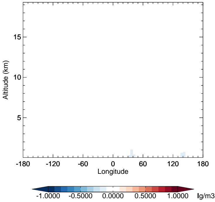
v11-02f-Run1 - v11-02e-Run1 OCPO - Diff along 15S for Oct
