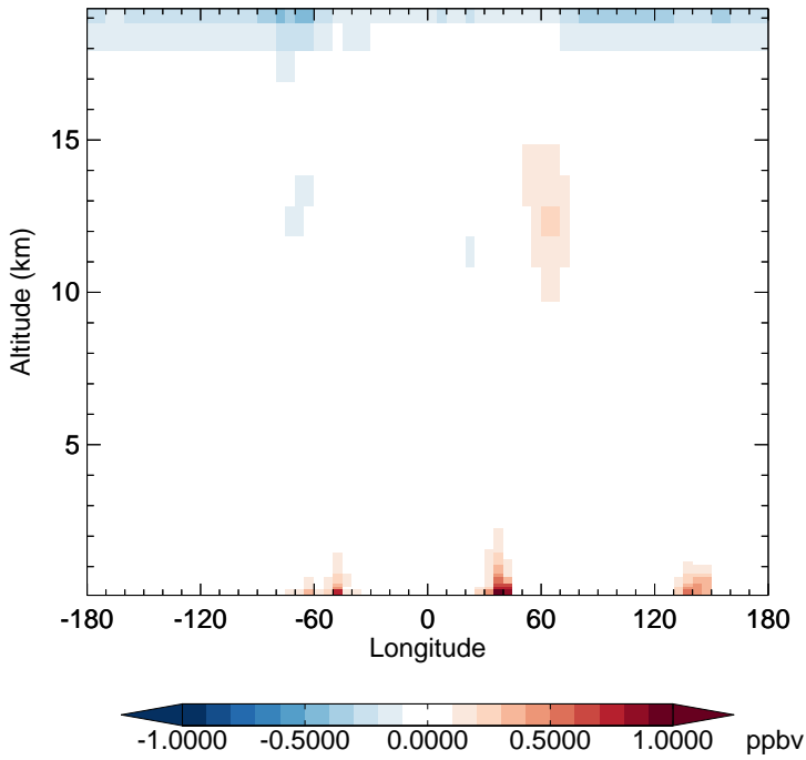
v11-02f-Run1 - v11-02e-Run0 NO 2 - Diff along 15S for Oct
