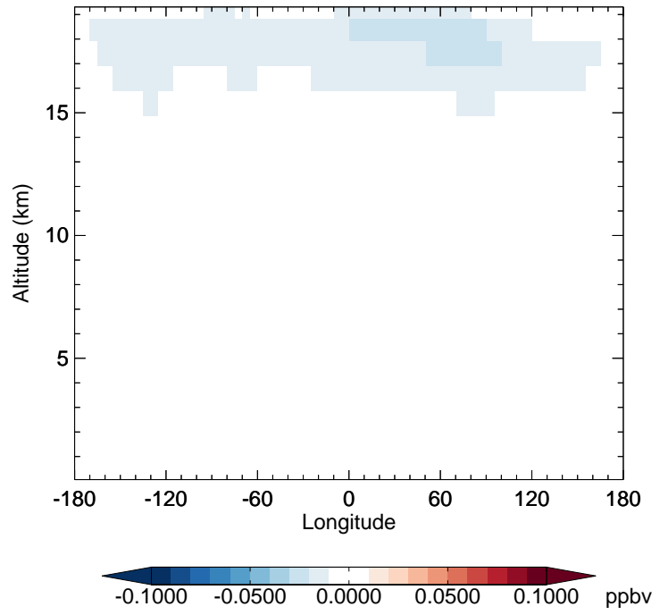
v11-02f-Run1 - v11-02e-Run1 CINO3 - Diff along 42N for Oct
