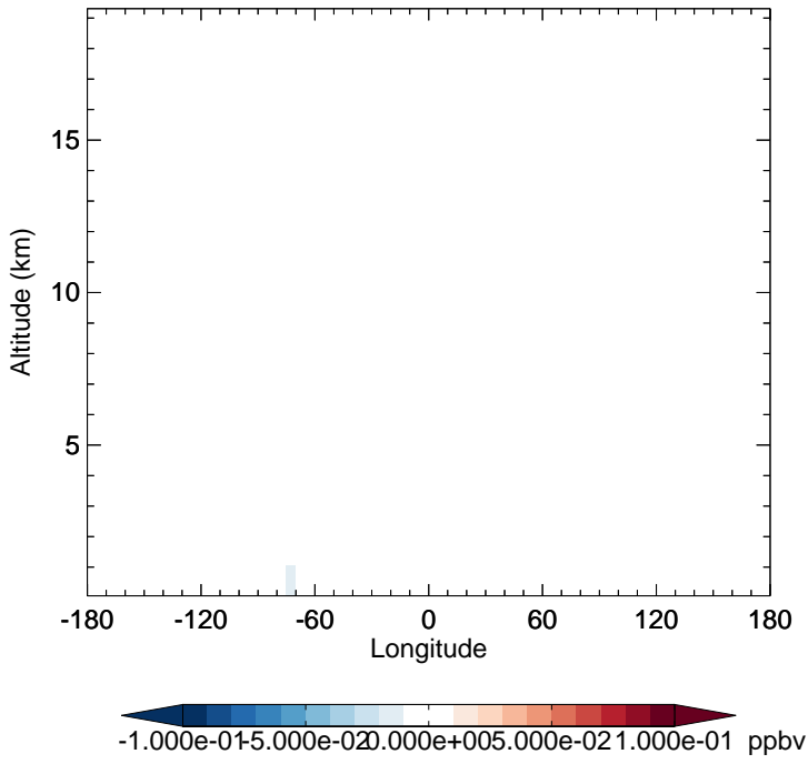
v11-02f-Run1 - v11-02e-Run1 SOAME - Diff along 15S for Oct
