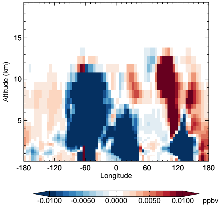
v11-02f-Run1 - v11-02e-Run0 MAP - Diff along 15S for Oct
