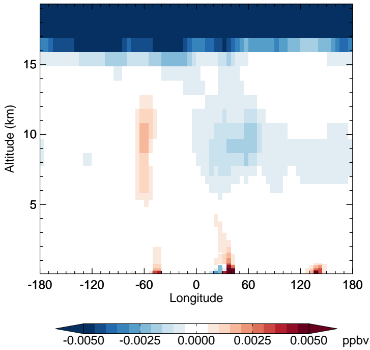
v11-02f-Run1 - v11-02e-Run1 N2O5 - Diff along 15S for Oct
