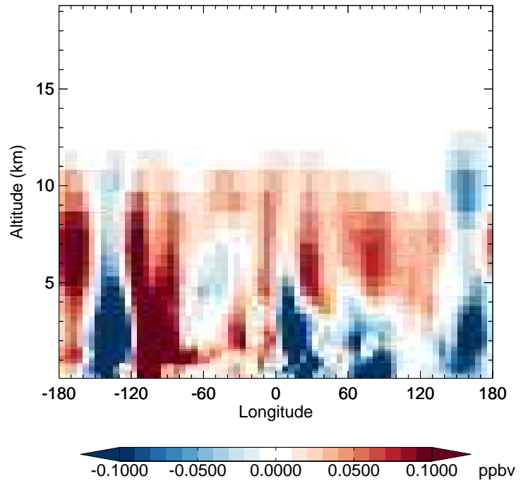
v11-02f-Run1 - v11-02e-Run0 H2O2 - Diff along 42N for Oct
