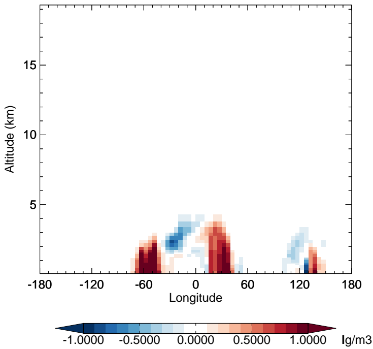
v11-02f-Run1 - v11-02e-Run0 OCPI - Diff along 15S for Oct
