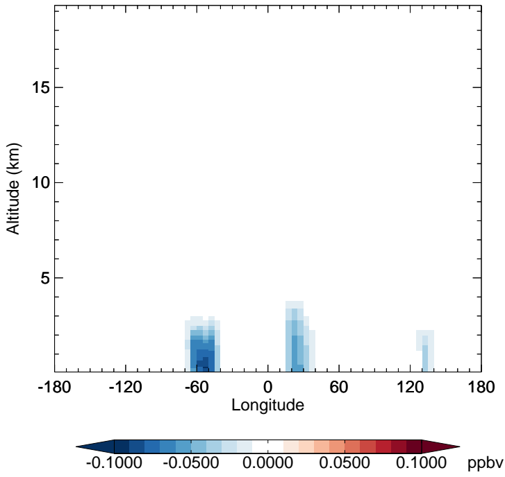
v11-02f-Run1 - v11-02e-Run1 MGLY - Diff along 15S for Oct
