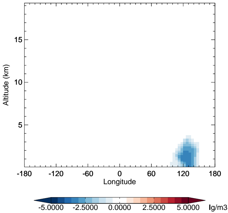
v11-02f-Run1 - v11-02e-Run0 DST1 - Diff along 15S for Oct
