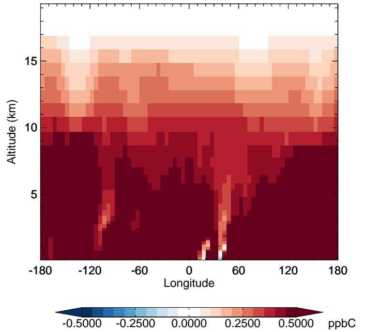
v11-02f-Run1 - v11-02e-Run0 C2H6 - Diff along 42N for Oct
