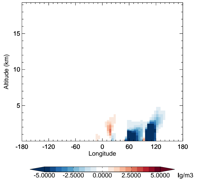
v11-02f-Run1 - v11-02e-Run0 DST2 - Diff along 42N for Oct
