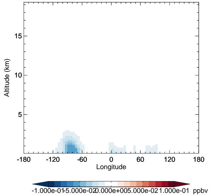
v11-02f-Run1 - v11-02e-Run1 IONITA - Diff along 42N for Oct
