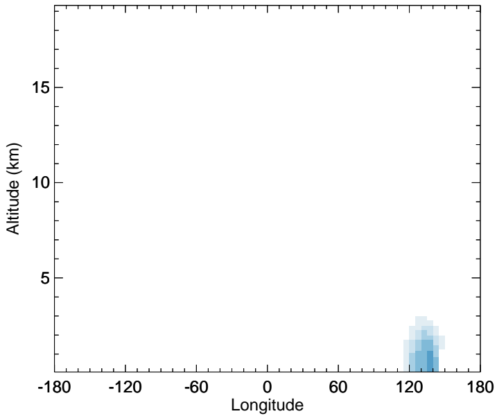
v11-02f-Run1 - v11-02e-Run0 DST4 - Diff along 15S for Oct
