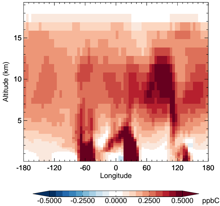
v11-02f-Run1 - v11-02e-Run0 C2H6 - Diff along 15S for Oct
