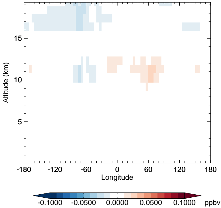
v11-02f-Run1 - v11-02e-Run0 MPN - Diff along 15S for Oct
