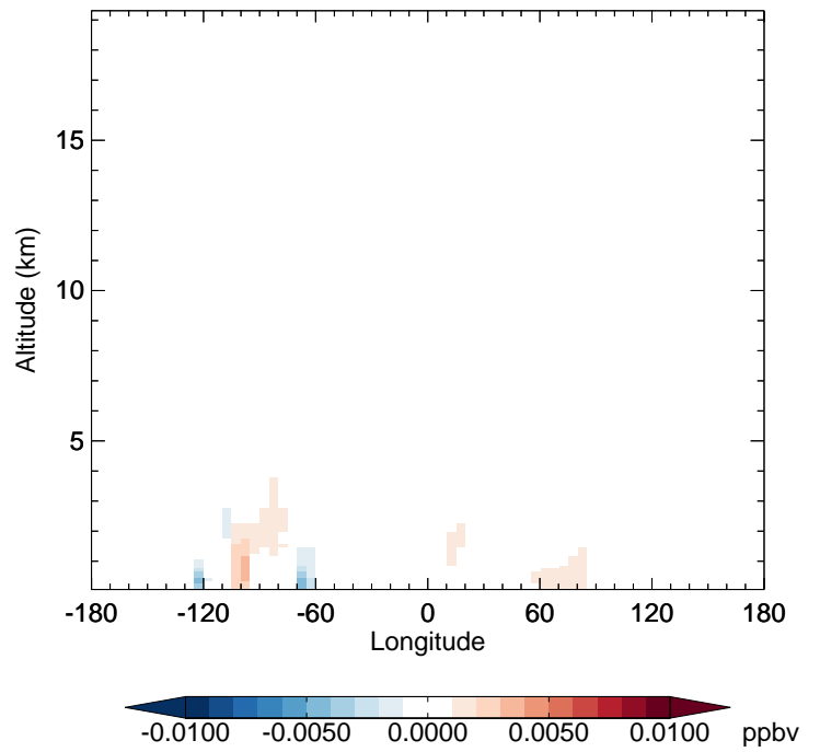
v11-02f-Run1 - v11-02e-Run0 R4N2 - Diff along 42N for Oct
