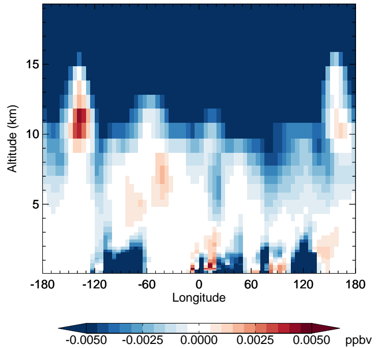
v11-02f-Run1 - v11-02e-Run0 N2O5 - Diff along 42N for Oct
