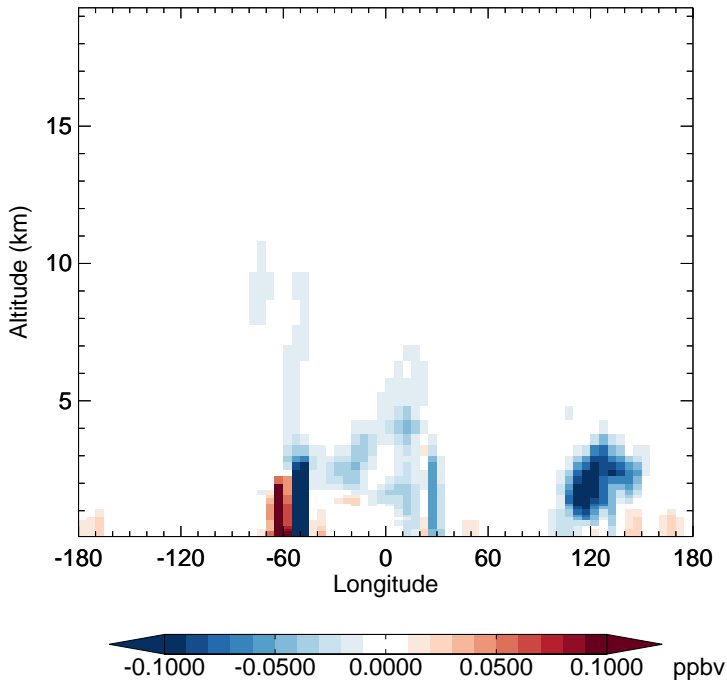
v11-02f-Run1 - v11-02e-Run0 TSOG3 - Diff along 15S for Oct
