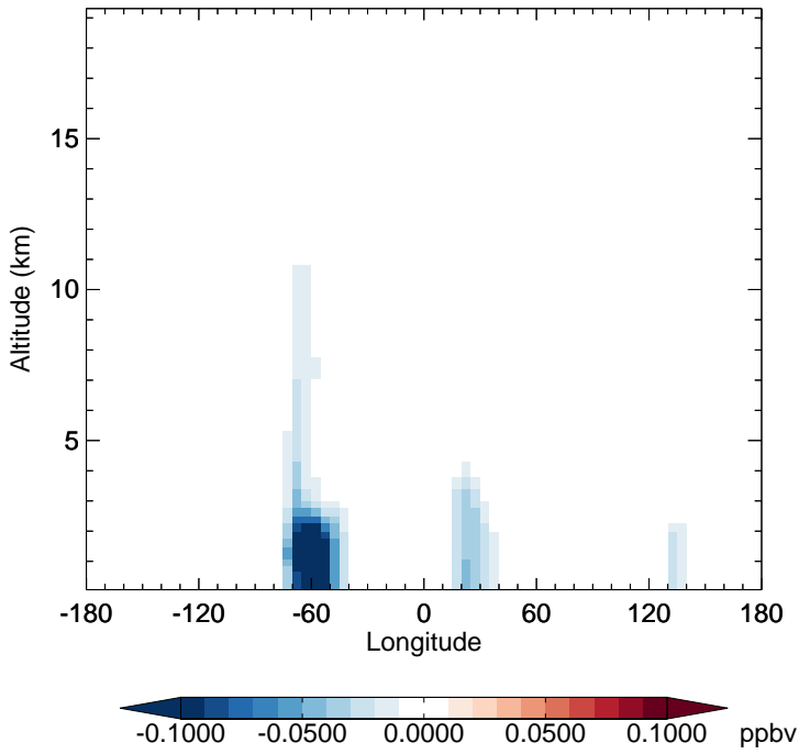
v11-02f-Run1 - v11-02e-Run1 IPMN - Diff along 15S for Oct
