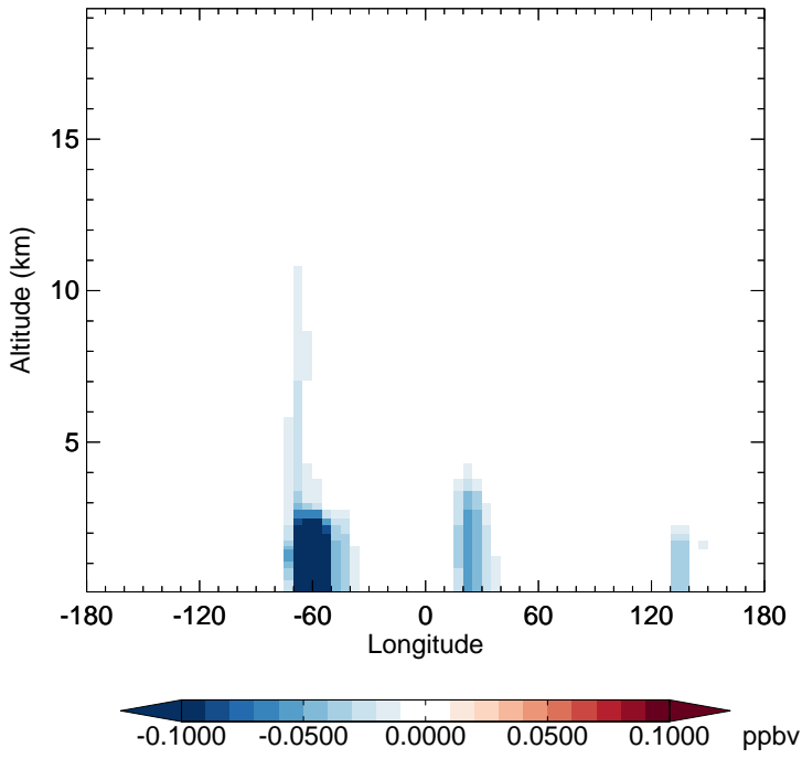
v11-02f-Run1 - v11-02e-Run1 RIPA - Diff along 15S for Oct
