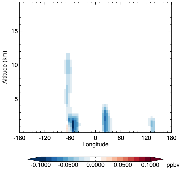
v11-02f-Run1 - v11-02e-Run1 IEPOXB - Diff along 15S for Oct
