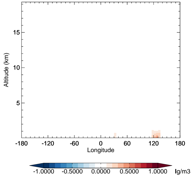
v11-02f-Run1 - v11-02e-Run0 OCPO - Diff along 42N for Oct
