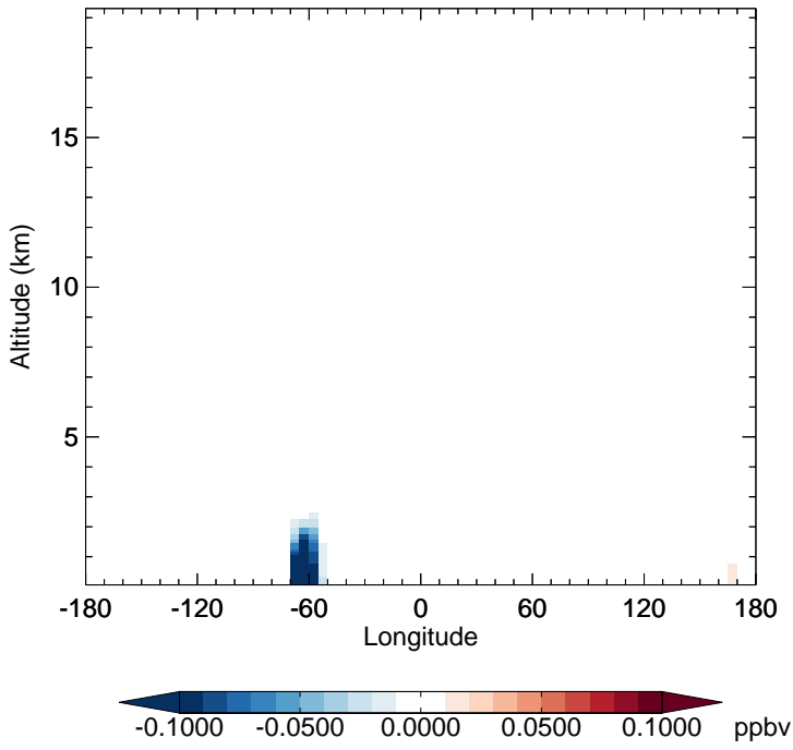
v11-02f-Run1 - v11-02e-Run1 MTPA - Diff along 15S for Oct
