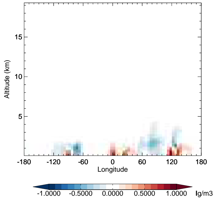
v11-02f-Run1 - v11-02e-Run0 NH4 - Diff along 42N for Oct
