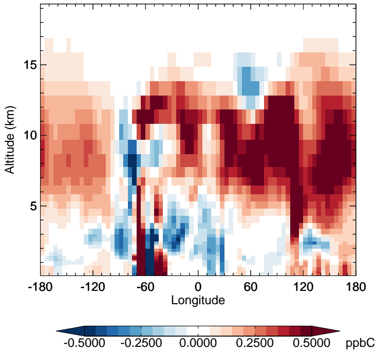
v11-02f-Run1 - v11-02e-Run0 ACET - Diff along 15S for Oct
