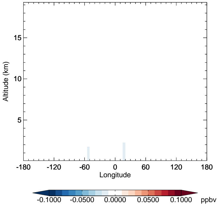
v11-02f-Run1 - v11-02e-Run1 LVOCOA - Diff along 15S for Oct
