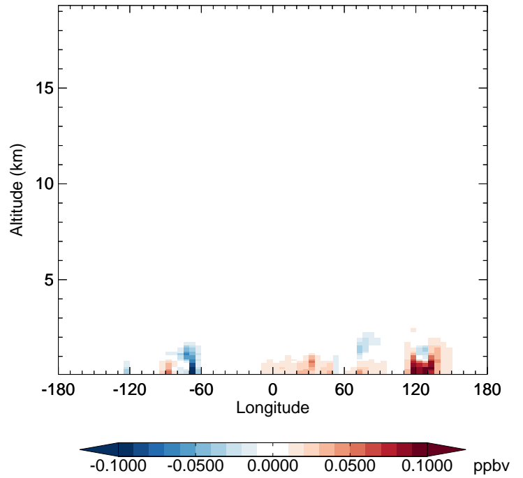
v11-02f-Run1 - v11-02e-Run0 SOAP - Diff along 42N for Oct
