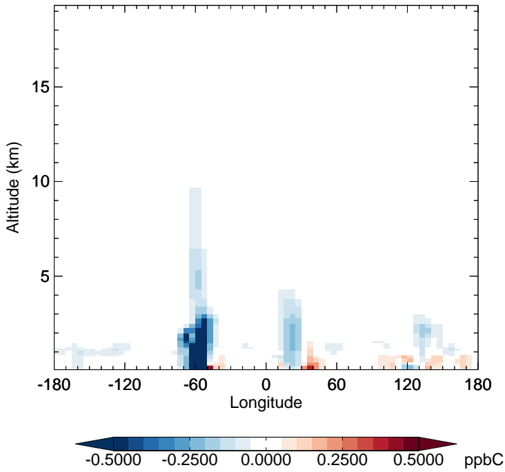
v11-02f-Run1 - v11-02e-Run0 ALD2 - Diff along 15S for Oct
