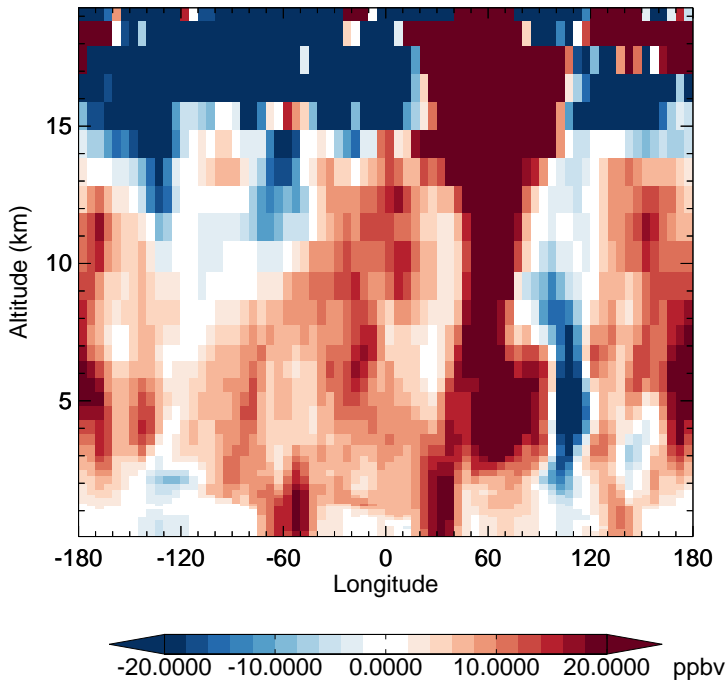
v11-02f-Run1 - v11-02e-Run0 O3 - Diff along 15S for Oct
