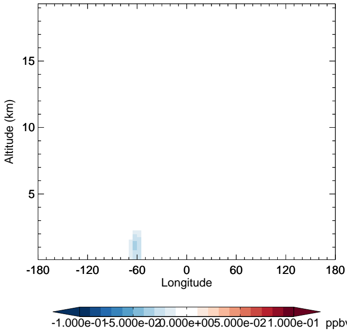
v11-02f-Run1 - v11-02e-Run1 RIPD - Diff along 15S for Oct
