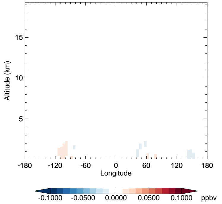
v11-02f-Run1 - v11-02e-Run1 H2O2 - Diff along 42N for Oct
