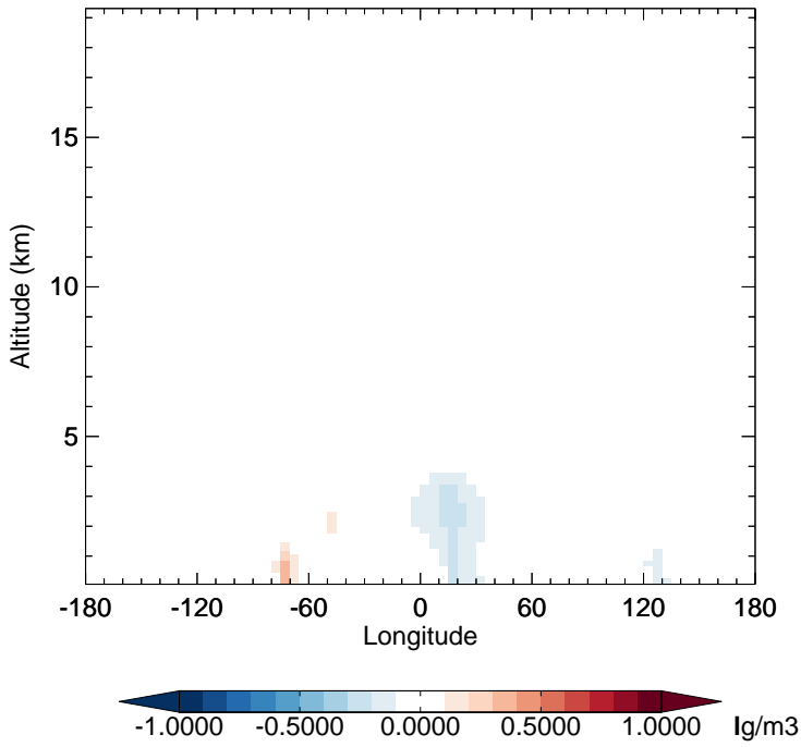
v11-02f-Run1 - v11-02e-Run1 NH4 - Diff along 15S for Oct
