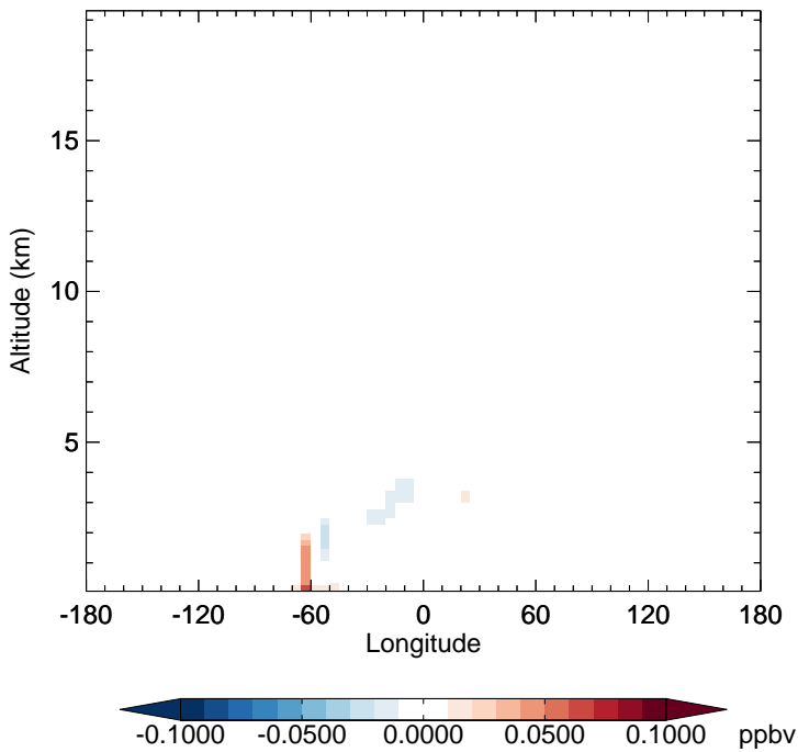
v11-02f-Run1 - v11-02e-Run0 TSOA3 - Diff along 15S for Oct
