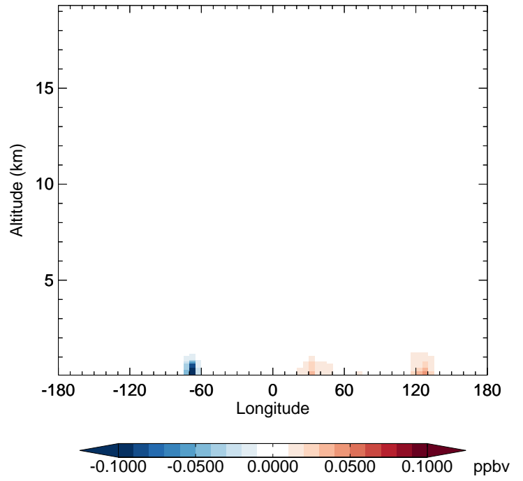
v11-02f-Run1 - v11-02e-Run1 SOAP - Diff along 42N for Oct
