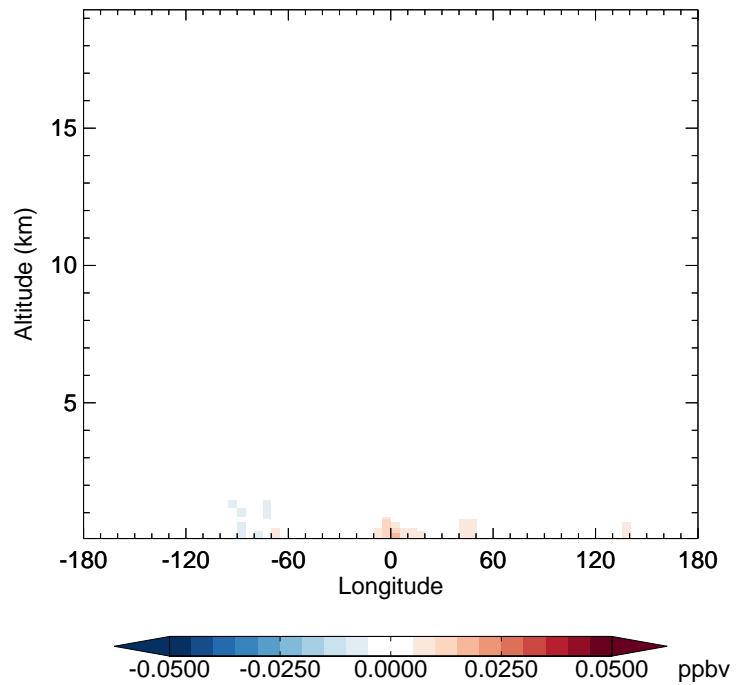
v11-02f-Run1 - v11-02e-Run0 MVK - Diff along 42N for Oct
