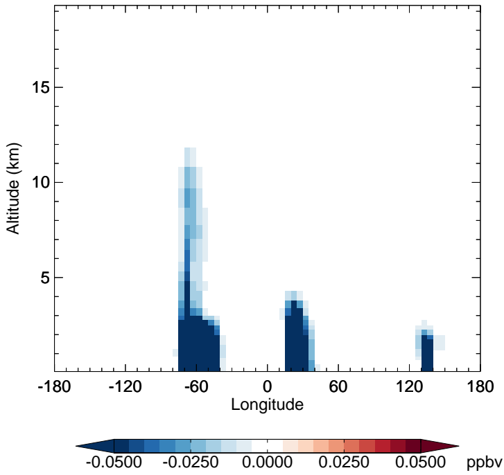
v11-02f-Run1 - v11-02e-Run1 MACR - Diff along 15S for Oct
