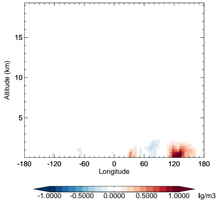
v11-02f-Run1 - v11-02e-Run0 OCPI - Diff along 42N for Oct
