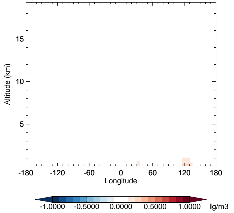
v11-02f-Run1 - v11-02e-Run1 OCPO - Diff along 42N for Oct
