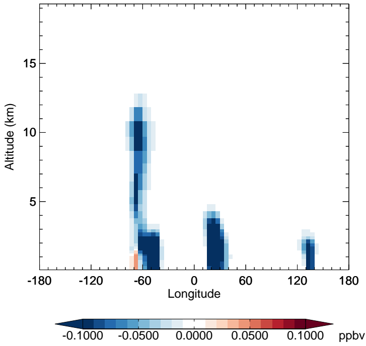
v11-02f-Run1 - v11-02e-Run1 IEPOXA - Diff along 15S for Oct
