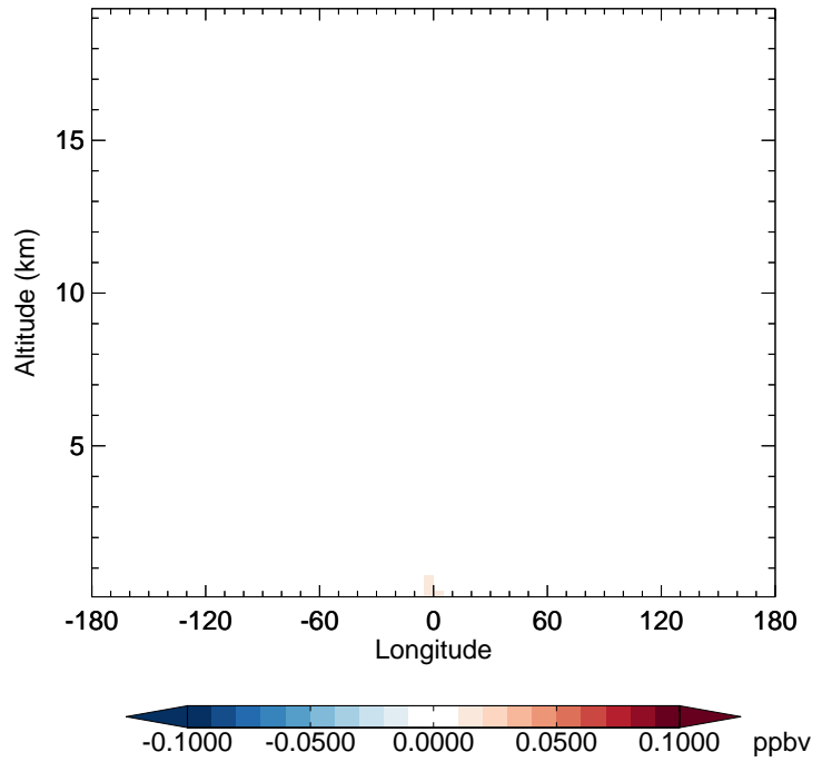
v11-02f-Run1 - v11-02e-Run0 TSOG2 - Diff along 42N for Oct
