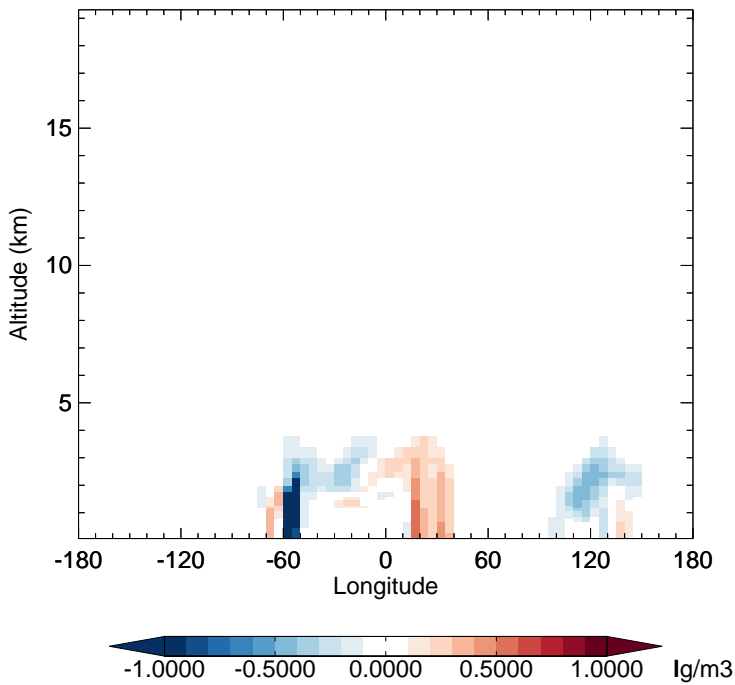
v11-02f-Run1 - v11-02e-Run0 SOAS - Diff along 15S for Oct
