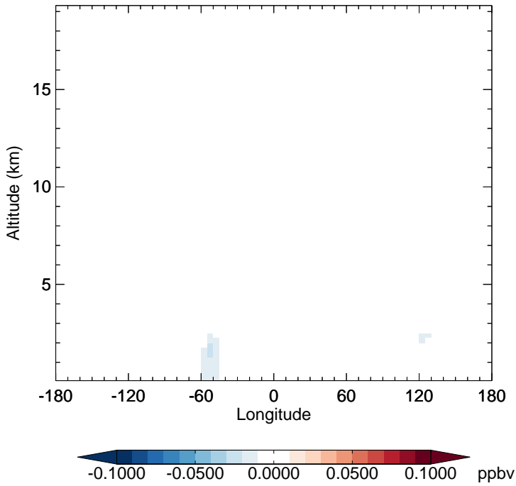
v11-02f-Run1 - v11-02e-Run0 LVOCOA - Diff along 15S for Oct
