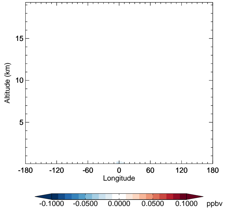
v11-02f-Run1 - v11-02e-Run0 CINO2 - Diff along 42N for Oct
