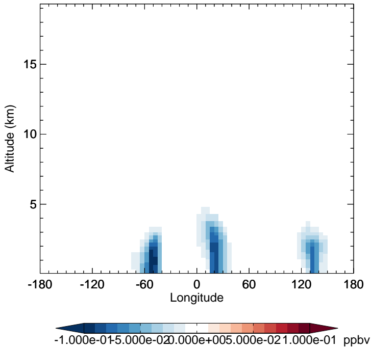
v11-02f-Run1 - v11-02e-Run0 IONITA - Diff along 15S for Oct
