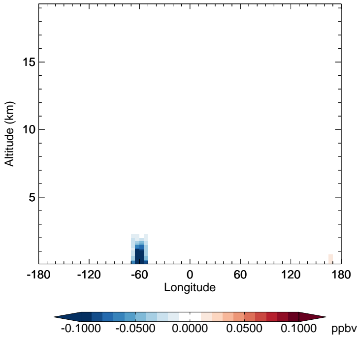
v11-02f-Run1 - v11-02e-Run0 MTPA - Diff along 15S for Oct
