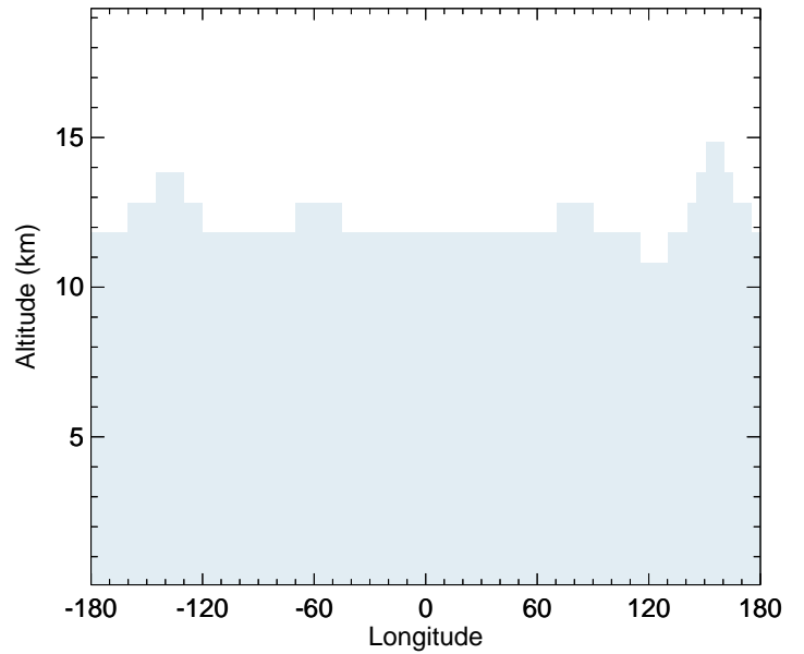
v11-02f-Run1 - v11-02e-Run0 HCFC22 - Diff along 42N for Oct
