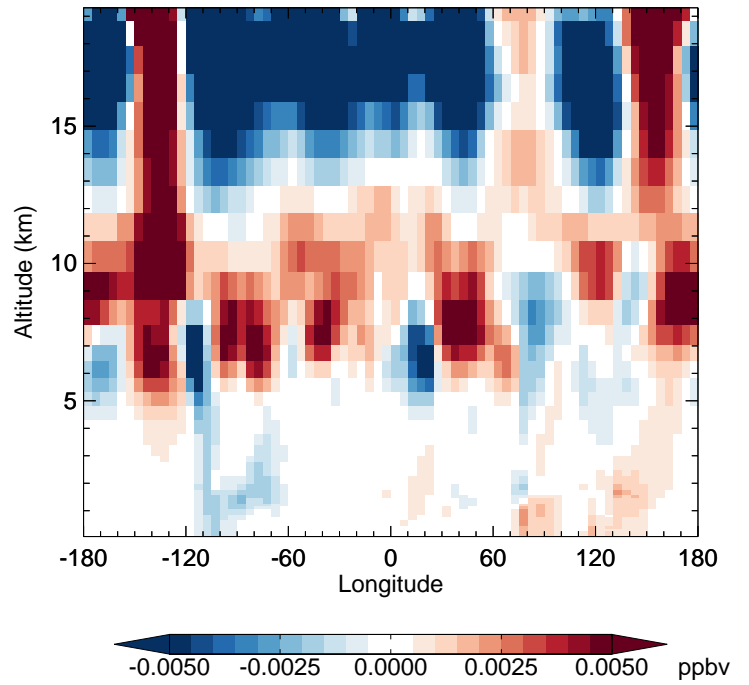
v11-02f-Run1 - v11-02e-Run0 HNO 4 - Diff along 42N for Oct
