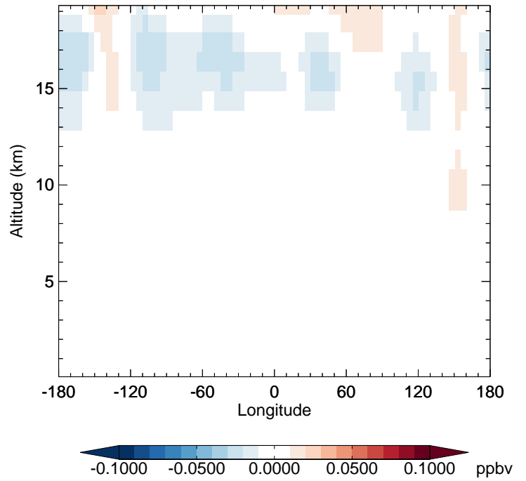
v11-02f-Run1 - v11-02e-Run0 MPN - Diff along 42N for Oct
