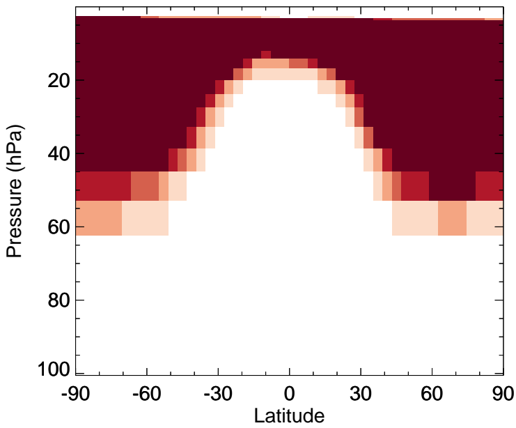
HNO 3 - Strat zonal mean abs diff for Apr
