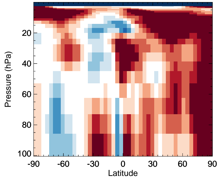
HNO 3 - Strat zonal mean % diff for Apr
