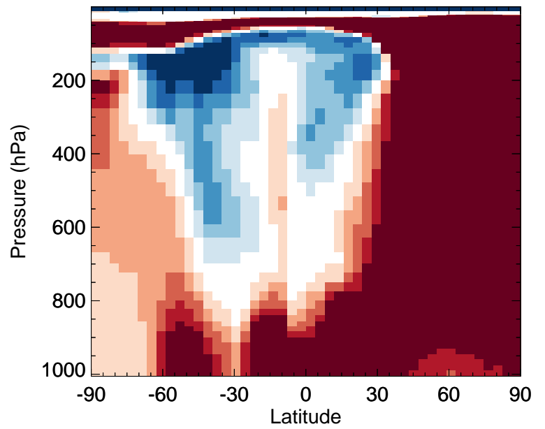
v11-02f-Run1 / v11-02e-Run1 HAC - Zonal mean % diff for Jan
