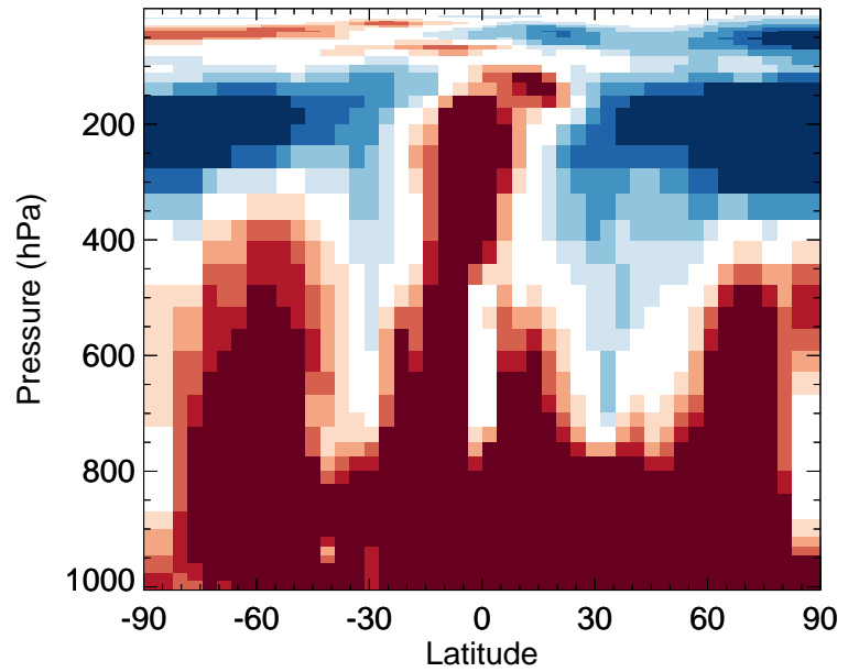
v11-02f-Run1 / v11-02e-Run0 DHDN - Zonal mean % diff for Jan
