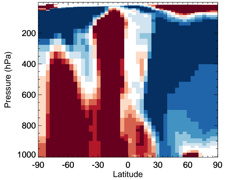
v11-02f-Run1 / v11-02e-Run1 TOLU - Zonal mean % diff for Jan
