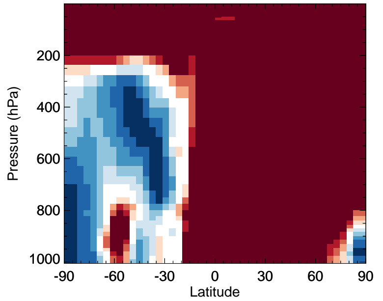
v11-02f-Run1 / v11-02e-Run0 INDIOL - Zonal mean % diff for Jan
