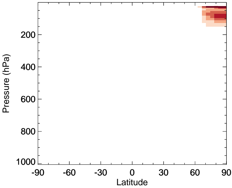
v11-02f-Run1 - v11-02e-Run0 Cl2 - Zonal mean abs diff for Jan
