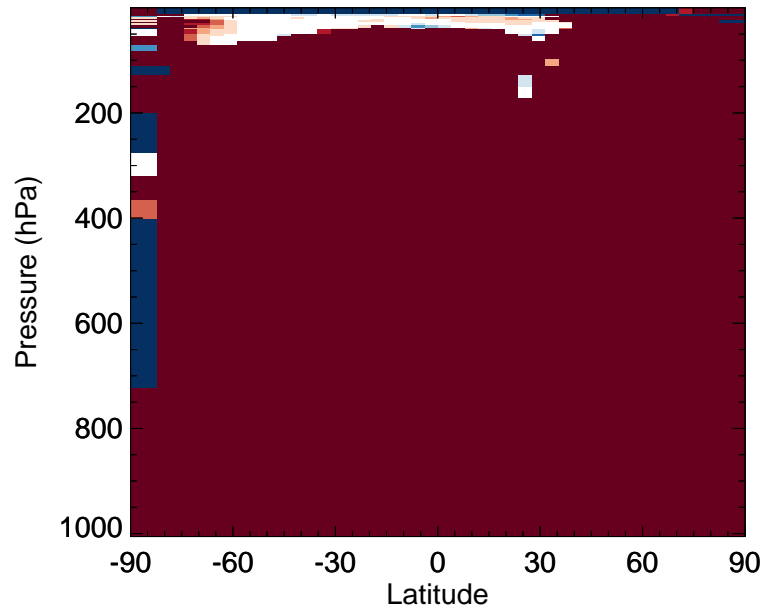
v11-02f-Run1 / v11-02e-Run0 ISOP - Zonal mean % diff for Jan
