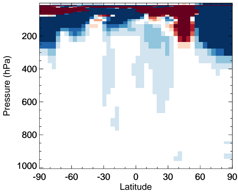
v11-02f-Run1 - v11-02e-Run0 O3 - Zonal mean abs diff for Jan
