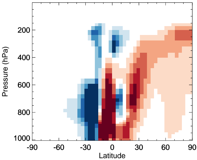
v11-02f-Run1 - v11-02e-Run0 MAP - Zonal mean abs diff for Jan
