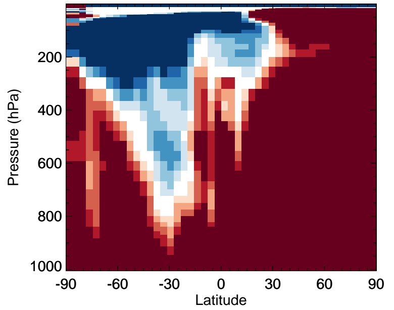
v11-02f-Run1 / v11-02e-Run1 IPMN - Zonal mean % diff for Jan
