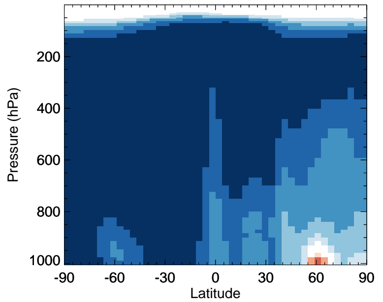
v11-02f-Run1 / v11-02e-Run1 SOAGX - Zonal mean % diff for Jan
