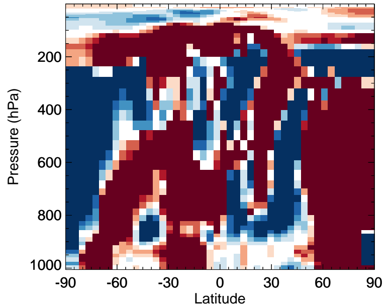
v11-02f-Run1 / v11-02e-Run0 NH3 - Zonal mean % diff for Jan
