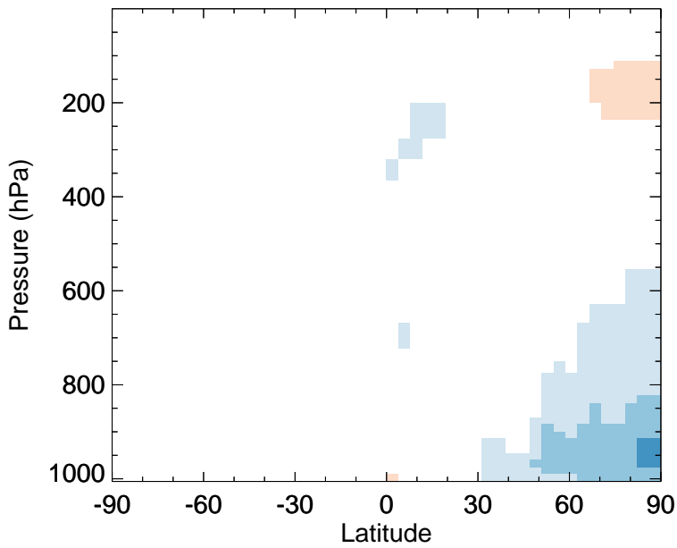
v11-02f-Run1 - v11-02e-Run0 PAN - Zonal mean abs diff for Jan
