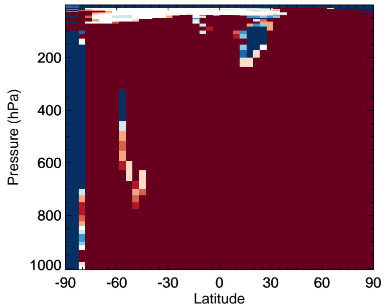
v11-02f-Run1 / v11-02e-Run0 ISN1 - Zonal mean % diff for Jan
