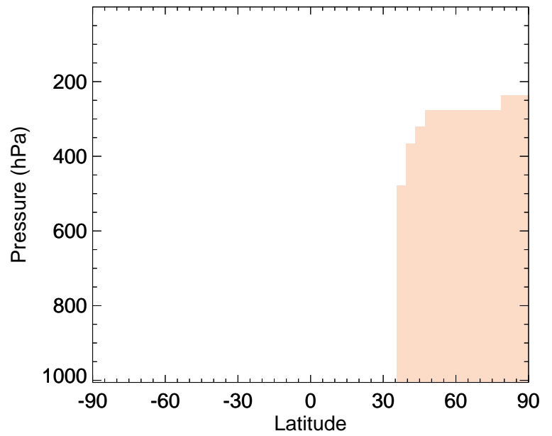
v11-02f-Run1 / v11-02e-Run1 MSA - Zonal mean % diff for Jan
