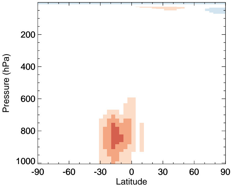
v11-02f-Run1 - v11-02e-Run1 H2O2 - Zonal mean abs diff for Jan
