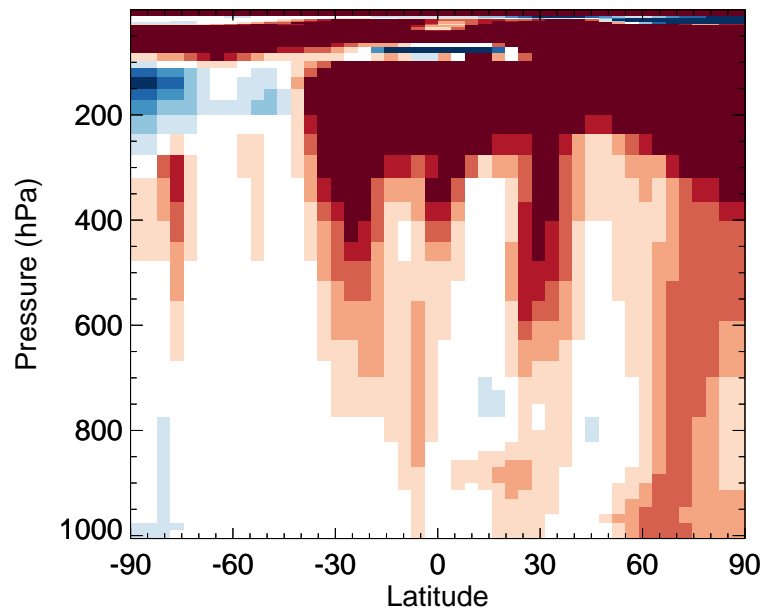
v11-02f-Run1 / v11-02e-Run0 MP - Zonal mean % diff for Jan
