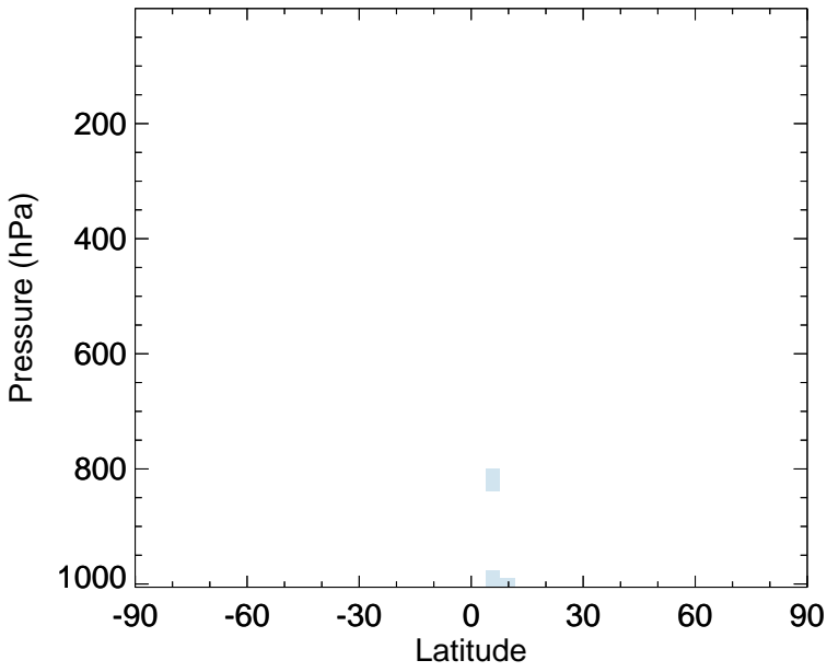
v11-02f-Run1 - v11-02e-Run1 NH3 - Zonal mean abs diff for Jan
