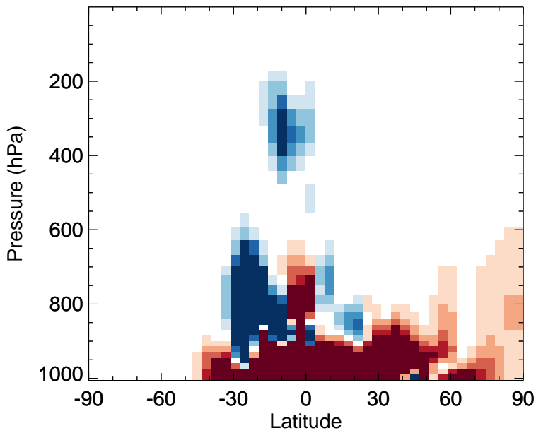
v11-02f-Run1 - v11-02e-Run0 PRPE - Zonal mean abs diff for Jan
