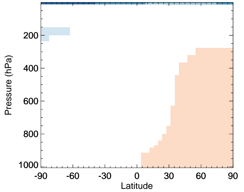
v11-02f-Run1 / v11-02e-Run1 CO - Zonal mean % diff for Jan
