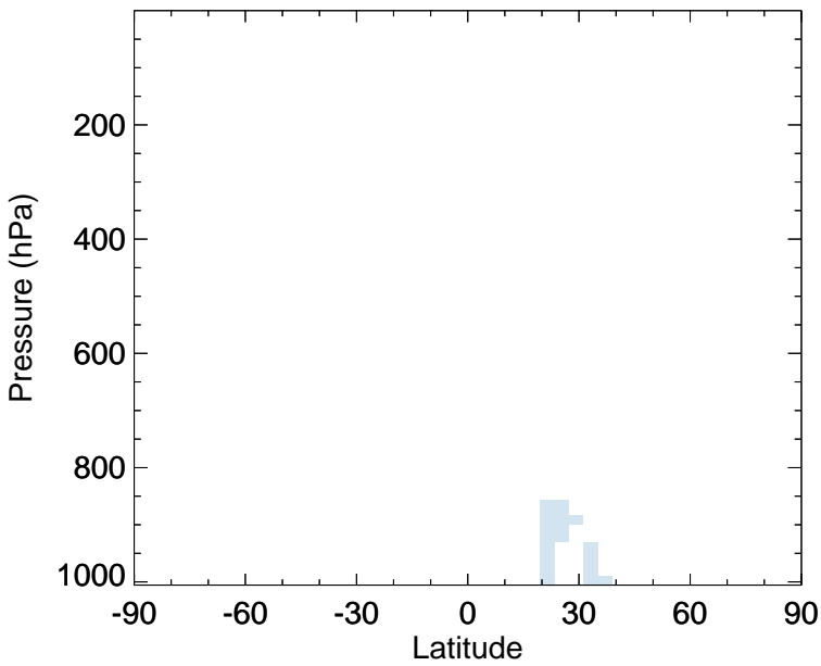
v11-02f-Run1 - v11-02e-Run0 SOAGX - Zonal mean abs diff for Jan
