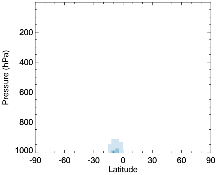
v11-02f-Run1 - v11-02e-Run1 MTPA - Zonal mean abs diff for Jan
