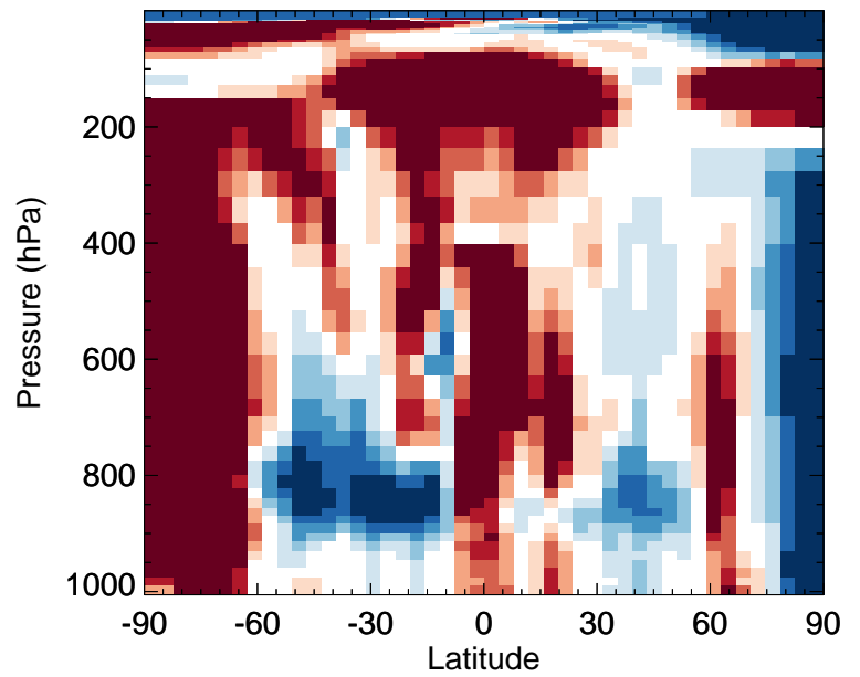
v11-02f-Run1 / v11-02e-Run0 SO 2 - Zonal mean % diff for Jan
