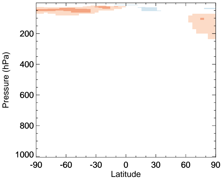
v11-02f-Run1 - v11-02e-Run0 CH3Cl - Zonal mean abs diff for Jan
