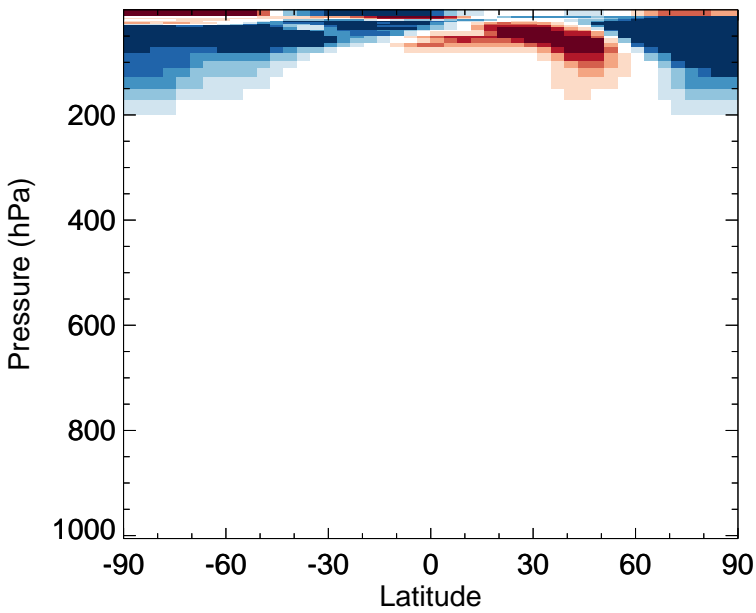
v11-02f-Run1 - v11-02e-Run0 HCl - Zonal mean abs diff for Jan
