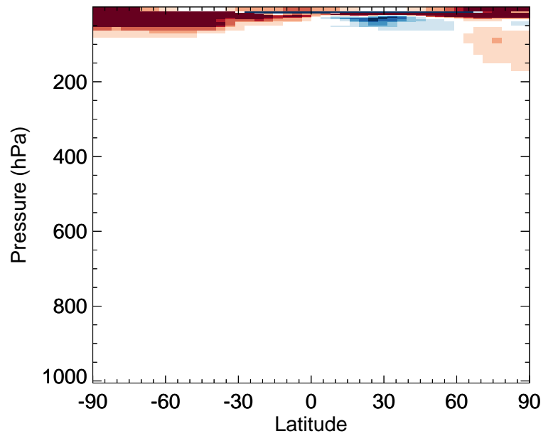
v11-02f-Run1 / v11-02e-Run0 OCS - Zonal mean % diff for Jan
