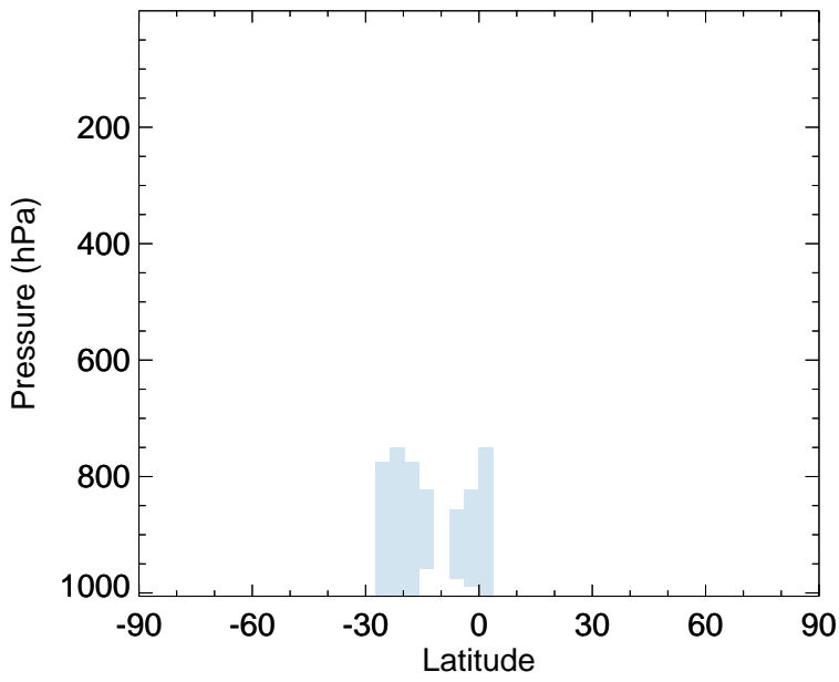
v11-02f-Run1 - v11-02e-Run1 RIPA - Zonal mean abs diff for Jan
