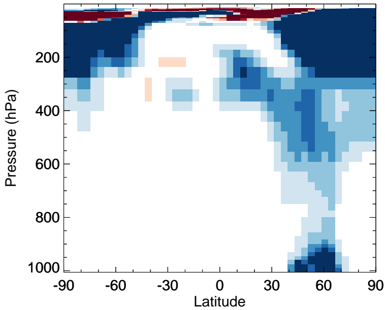
v11-02f-Run1 - v11-02e-Run0 HNO 4 - Zonal mean abs diff for Jan
