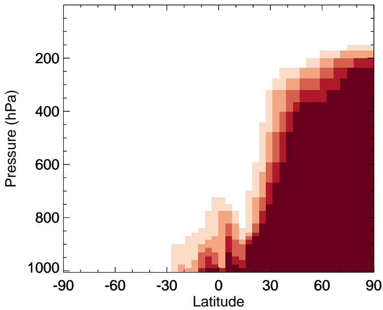
v11-02f-Run1 - v11-02e-Run0 ALK4 - Zonal mean abs diff for Jan
