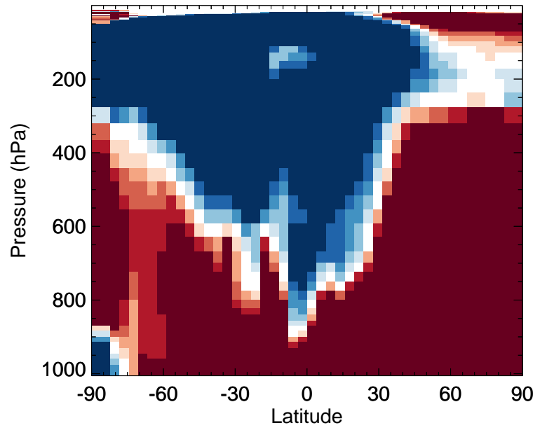
v11-02f-Run1 / v11-02e-Run1 IEPOXA - Zonal mean % diff for Jan
