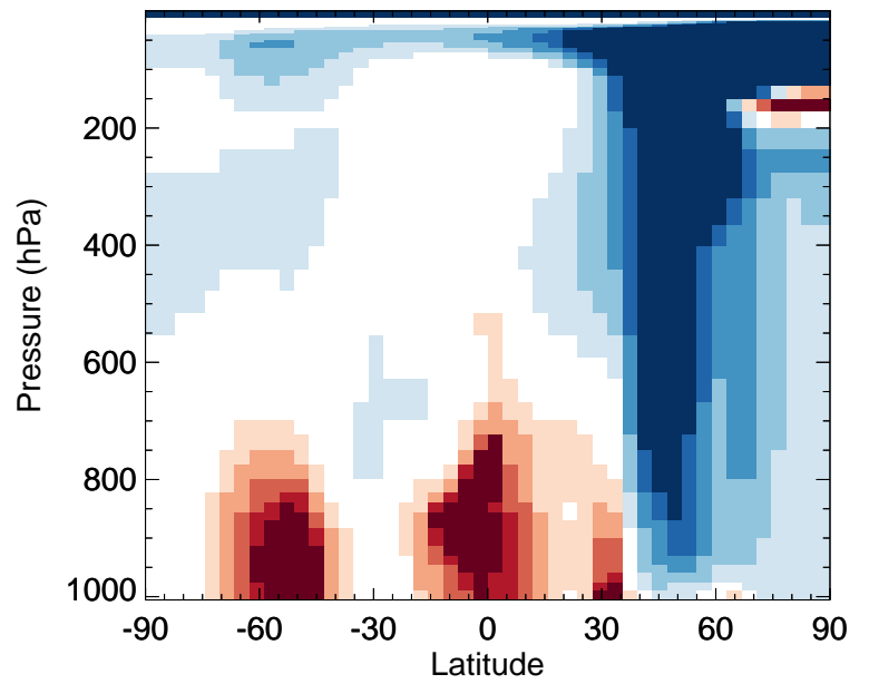
v11-02f-Run1 / v11-02e-Run1 HNO 2 - Zonal mean % diff for Jan
