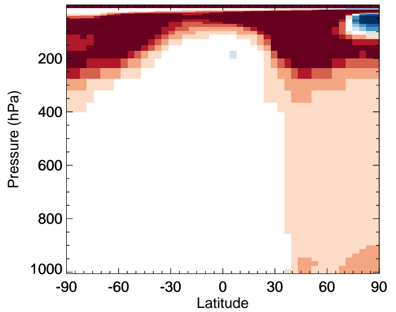
v11-02f-Run1 / v11-02e-Run1 MP - Zonal mean % diff for Jan
