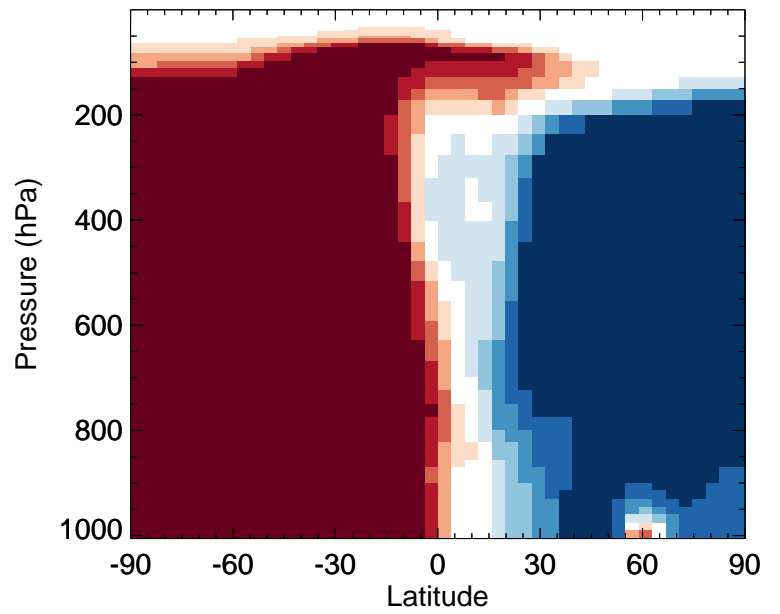
v11-02f-Run1 / v11-02e-Run1 ASOA1 - Zonal mean % diff for Jan
