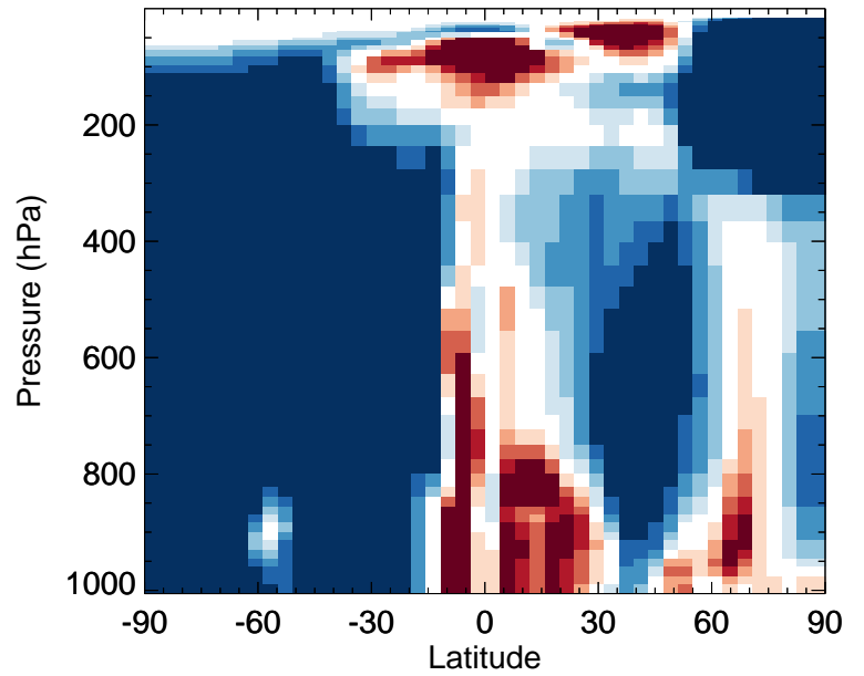
v11-02f-Run1 / v11-02e-Run0 ISOG1 - Zonal mean % diff for Jan
