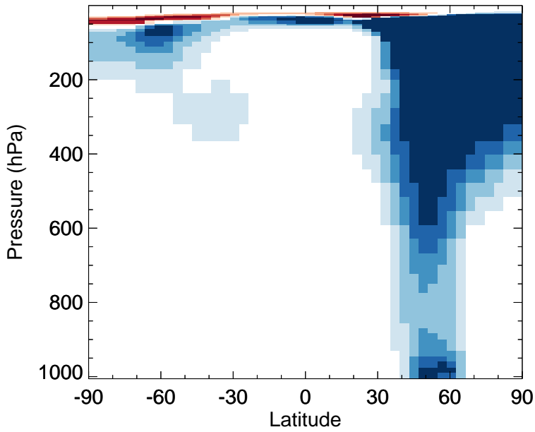
v11-02f-Run1 - v11-02e-Run1 HNO 4 - Zonal mean abs diff for Jan
