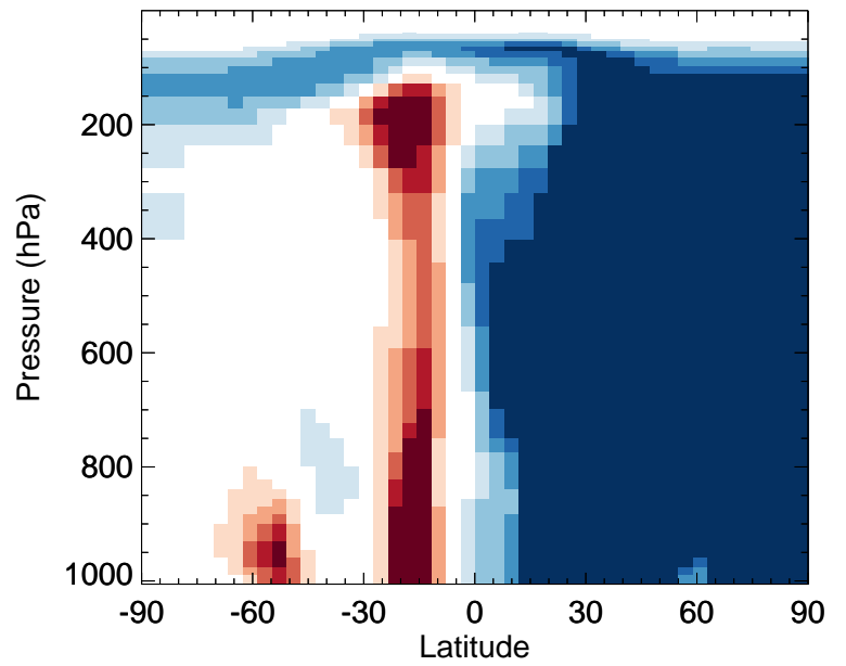
v11-02f-Run1 / v11-02e-Run1 ASOG2 - Zonal mean % diff for Jan
