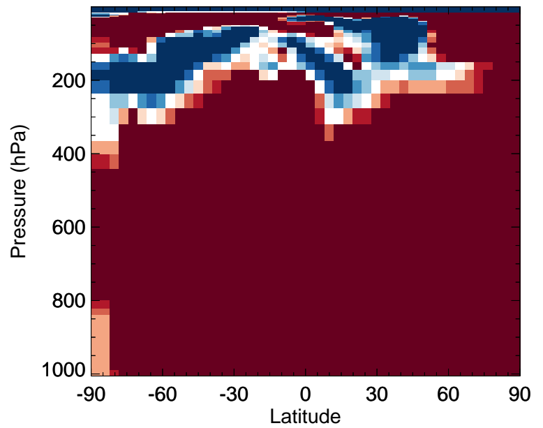
v11-02f-Run1 / v11-02e-Run0 HONIT - Zonal mean % diff for Jan
