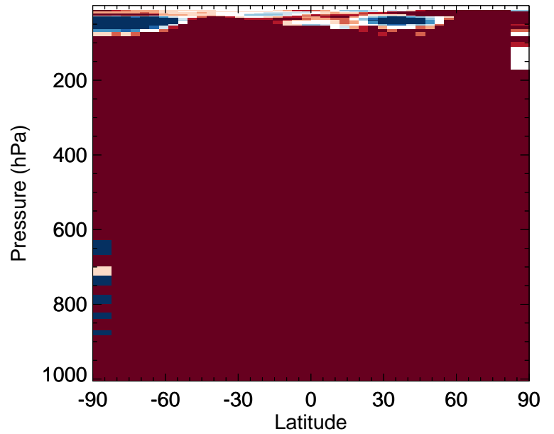
v11-02f-Run1 / v11-02e-Run0 MTPO - Zonal mean % diff for Jan
