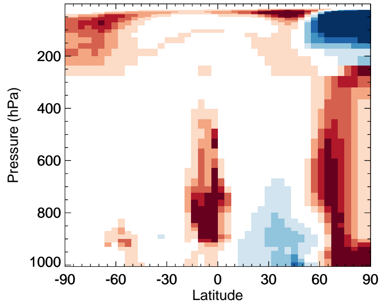
v11-02f-Run1 / v11-02e-Run1 HOBr - Zonal mean % diff for Jan
