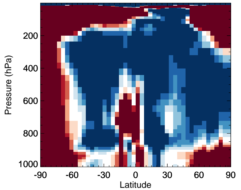
v11-02f-Run1 / v11-02e-Run0 SALC - Zonal mean % diff for Jan
