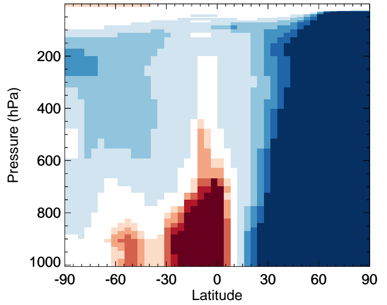
v11-02f-Run1 / v11-02e-Run1 CINO3 - Zonal mean % diff for Jan
