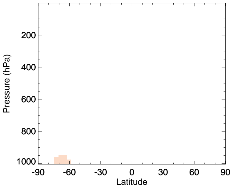
v11-02f-Run1 - v11-02e-Run0 DMS - Zonal mean abs diff for Jan
