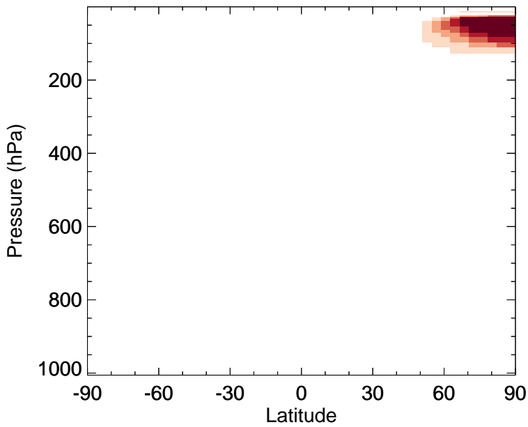
v11-02f-Run1 - v11-02e-Run0 OCIO - Zonal mean abs diff for Jan
