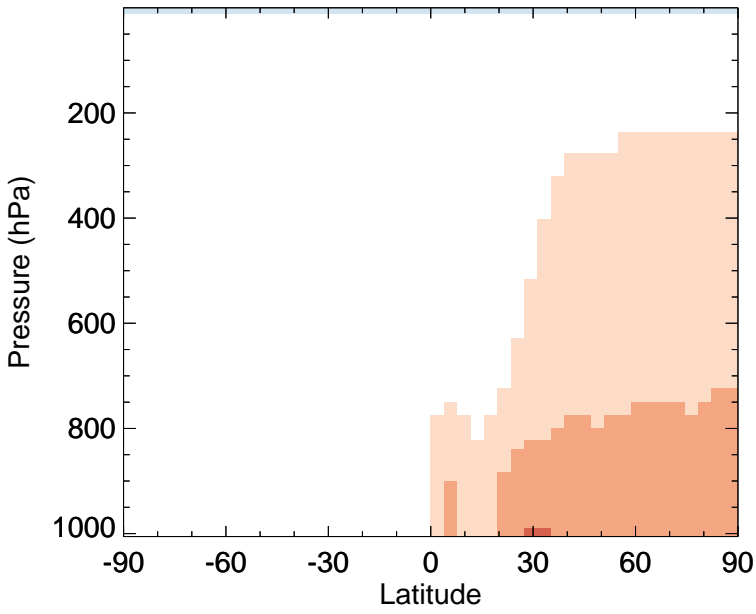
v11-02f-Run1 - v11-02e-Run1 CO - Zonal mean abs diff for Jan
