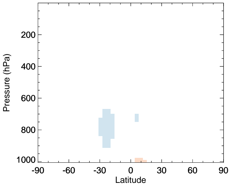
v11-02f-Run1 - v11-02e-Run0 HAC - Zonal mean abs diff for Jan
