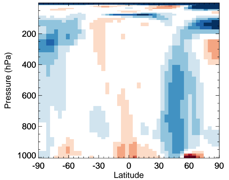
v11-02f-Run1 / v11-02e-Run0 CH 2 O - Zonal mean % diff for Jan
