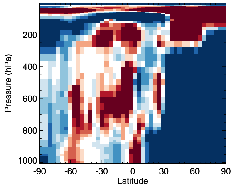
v11-02f-Run1 / v11-02e-Run0 HOCl - Zonal mean % diff for Jan
