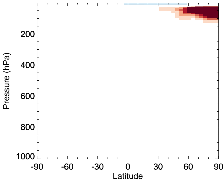
v11-02f-Run1 - v11-02e-Run0 HOCl - Zonal mean abs diff for Jan
