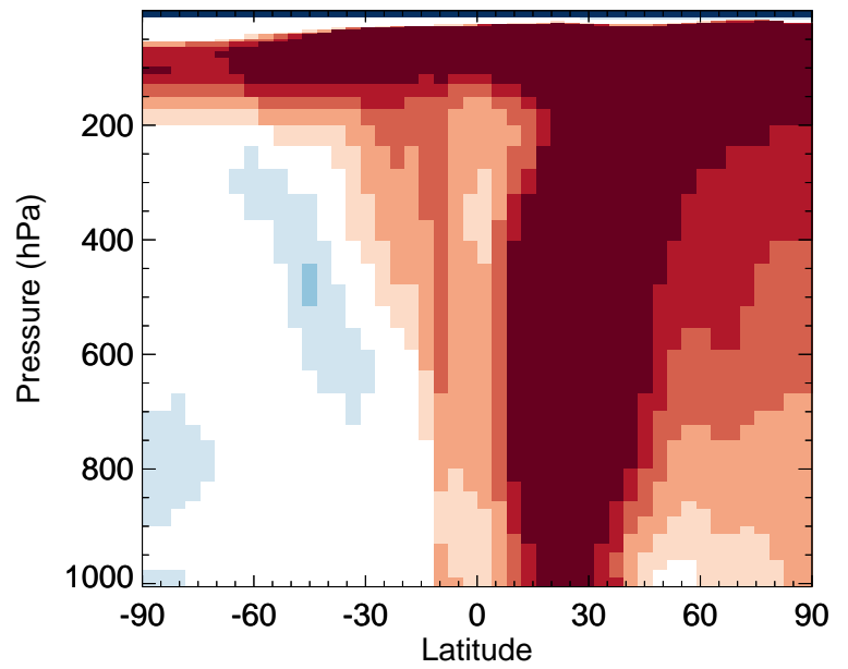
v11-02f-Run1 / v11-02e-Run1 ALD2 - Zonal mean % diff for Jan
