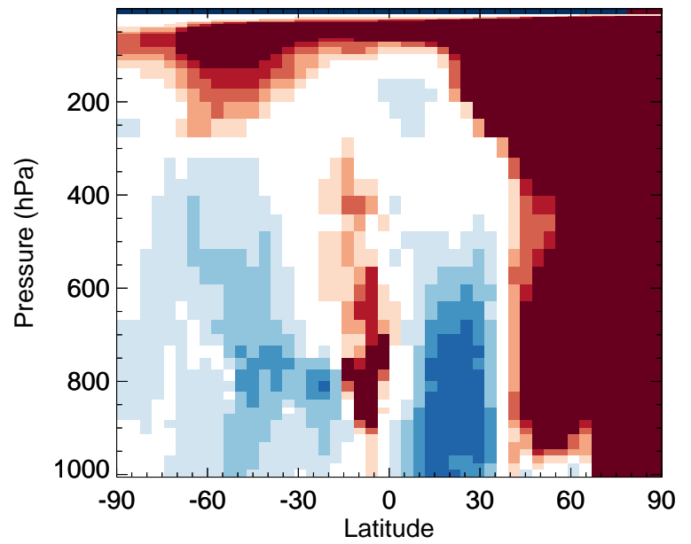
v11-02f-Run1 / v11-02e-Run1 OCIO - Zonal mean % diff for Jan
