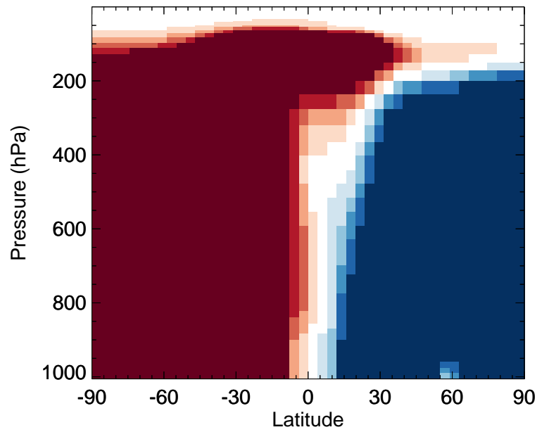
v11-02f-Run1 / v11-02e-Run1 ASOG1 - Zonal mean % diff for Jan
