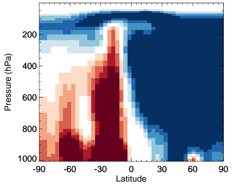
v11-02f-Run1 / v11-02e-Run1 ASOA2 - Zonal mean % diff for Jan
