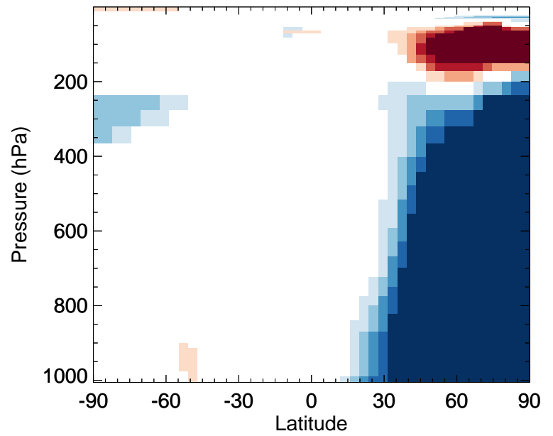
v11-02f-Run1 / v11-02e-Run1 HCl - Zonal mean % diff for Jan
