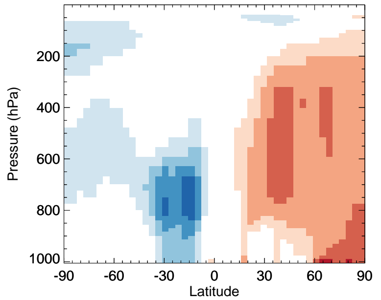
v11-02f-Run1 / v11-02e-Run1 SO 2 - Zonal mean % diff for Jan
