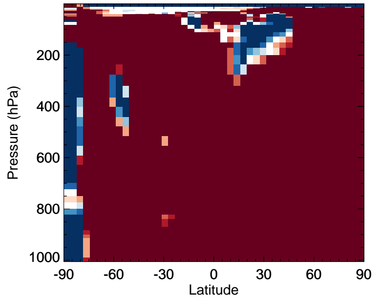
v11-02f-Run1 / v11-02e-Run0 IPMN - Zonal mean % diff for Jan
