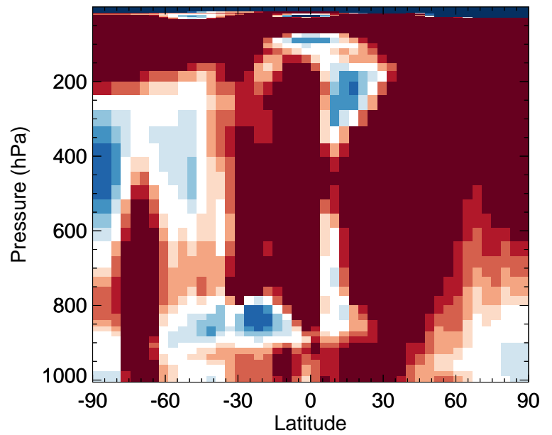
v11-02f-Run1 / v11-02e-Run0 ALD2 - Zonal mean % diff for Jan
