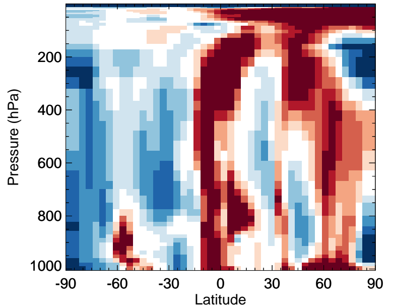
v11-02f-Run1 / v11-02e-Run0 HNO 3 - Zonal mean % diff for Jan
