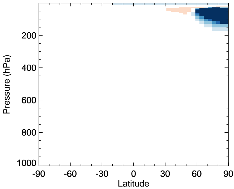
v11-02f-Run1 - v11-02e-Run1 HOCl - Zonal mean abs diff for Jan
