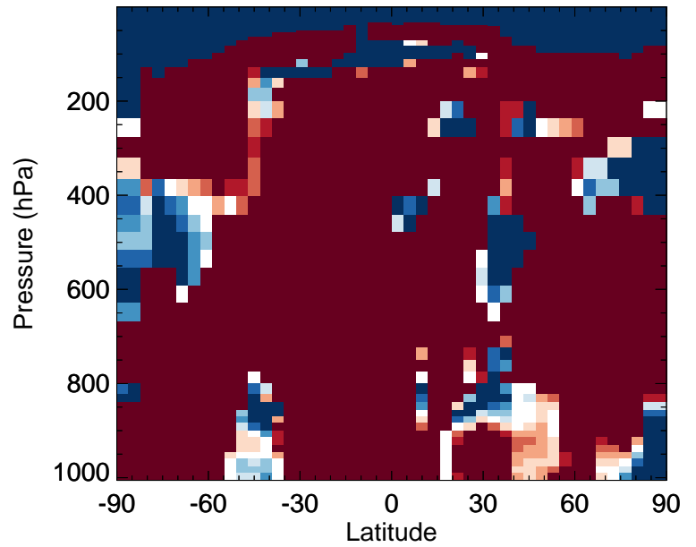
v11-02f-Run1 / v11-02e-Run0 NIT - Zonal mean % diff for Jan
