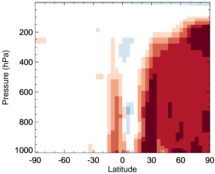
v11-02f-Run1 - v11-02e-Run0 CO - Zonal mean abs diff for Jan
