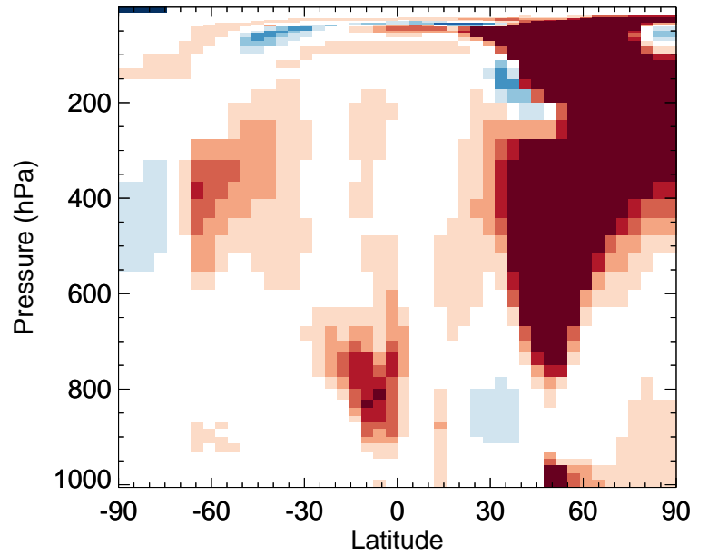
v11-02f-Run1 / v11-02e-Run1 Br2 - Zonal mean % diff for Jan
