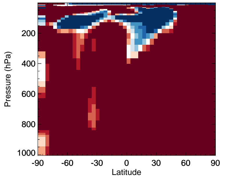
v11-02f-Run1 / v11-02e-Run0 ALK4 - Zonal mean % diff for Jan
