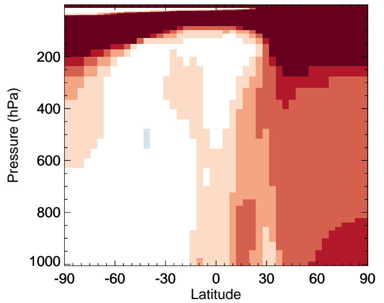
v11-02f-Run1 / v11-02e-Run1 MAP - Zonal mean % diff for Jan
