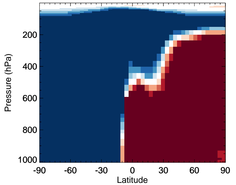
v11-02f-Run1 / v11-02e-Run0 SOAME - Zonal mean % diff for Jan
