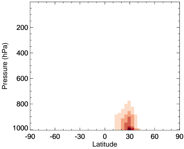
v11-02f-Run1 - v11-02e-Run1 OCPI - Zonal mean abs diff for Jan
