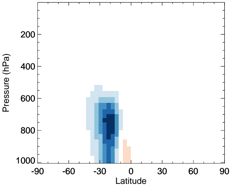
v11-02f-Run1 - v11-02e-Run0 SOAIE - Zonal mean abs diff for Jan
