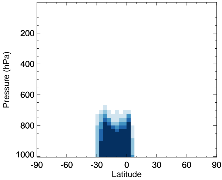
v11-02f-Run1 - v11-02e-Run1 ISOP - Zonal mean abs diff for Jan
