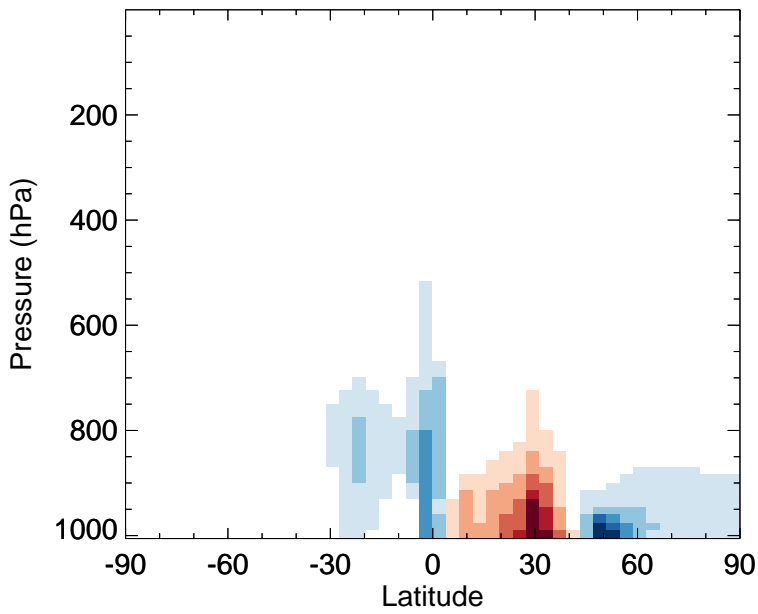
v11-02f-Run1 - v11-02e-Run1 EOH - Zonal mean abs diff for Jan
