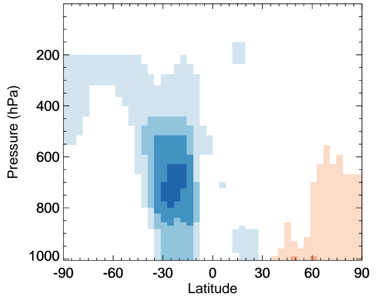
v11-02f-Run1 / v11-02e-Run1 NH4 - Zonal mean % diff for Jan
