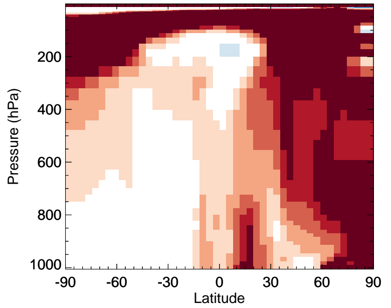
v11-02f-Run1 / v11-02e-Run1 ACTA - Zonal mean % diff for Jan
