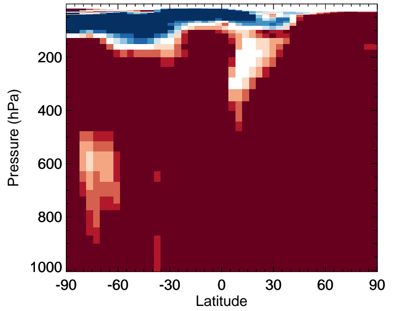
v11-02f-Run1 / v11-02e-Run1 ISN1OG - Zonal mean % diff for Jan
