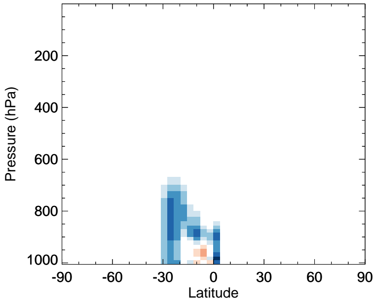
v11-02f-Run1 - v11-02e-Run0 ISOP - Zonal mean abs diff for Jan
