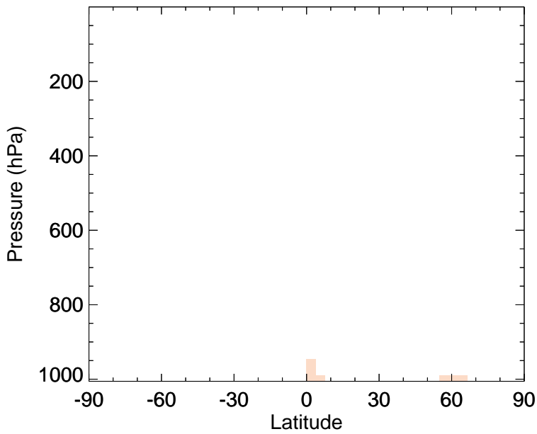
v11-02f-Run1 - v11-02e-Run0 CH 2 O - Zonal mean abs diff for Jan
