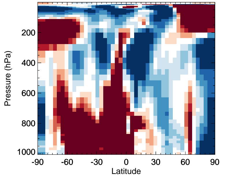
v11-02f-Run1 / v11-02e-Run0 ISOA2 - Zonal mean % diff for Jan
