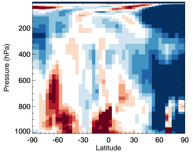
v11-02f-Run1 / v11-02e-Run0 HNO 4 - Zonal mean % diff for Jan
