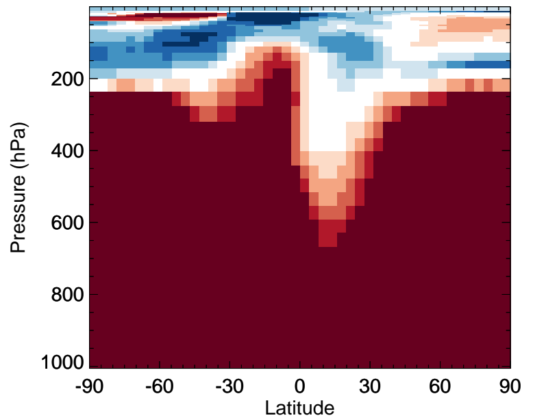
v11-02f-Run1 / v11-02e-Run1 HONIT - Zonal mean % diff for Jan
