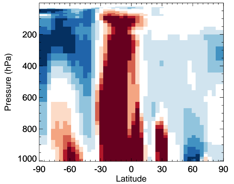
v11-02f-Run1 / v11-02e-Run1 SOAP - Zonal mean % diff for Jan
