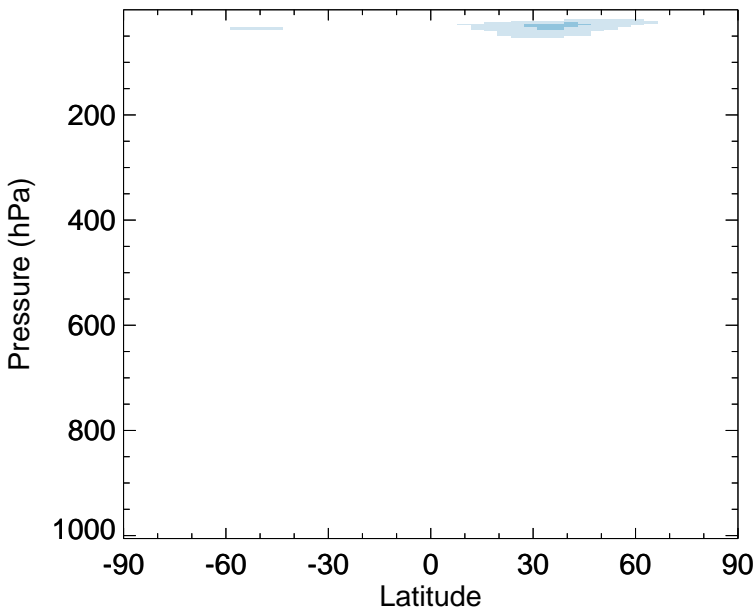
v11-02f-Run1 - v11-02e-Run1 NO - Zonal mean abs diff for Jan
