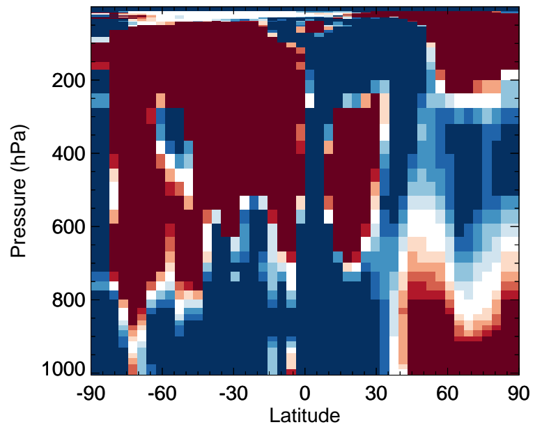
v11-02f-Run1 / v11-02e-Run0 XYLE - Zonal mean % diff for Jan
