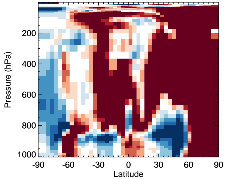
v11-02f-Run1 / v11-02e-Run0 Br2 - Zonal mean % diff for Jan
