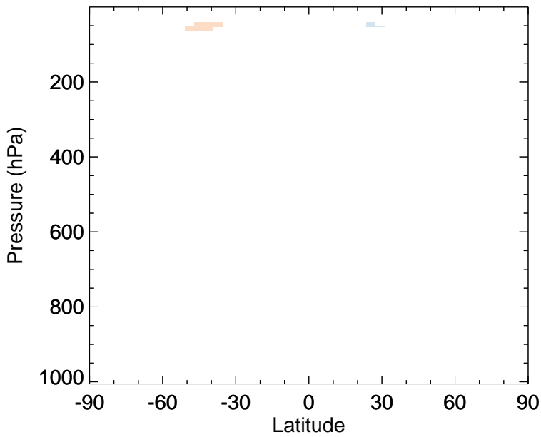
v11-02f-Run1 - v11-02e-Run0 CFC11 - Zonal mean abs diff for Jan
