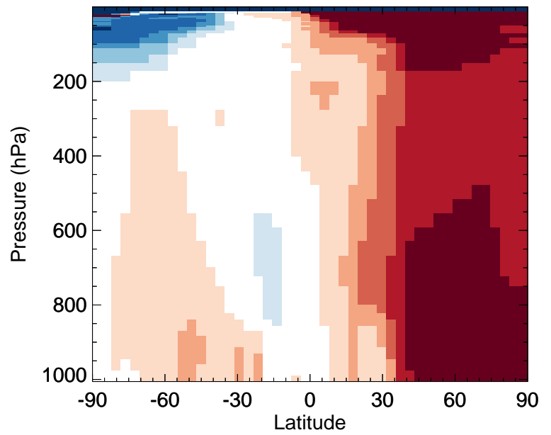
v11-02f-Run1 / v11-02e-Run1 C3H8 - Zonal mean % diff for Jan
