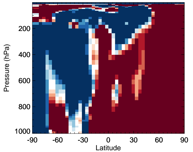
v11-02f-Run1 / v11-02e-Run0 IMAE - Zonal mean % diff for Jan
