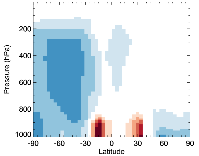
v11-02f-Run1 / v11-02e-Run1 SOAS - Zonal mean % diff for Jan
