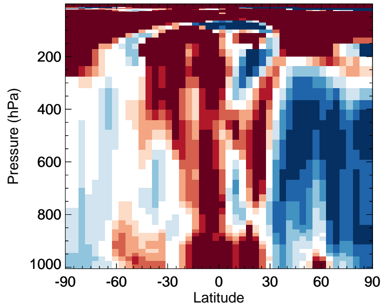
v11-02f-Run1 / v11-02e-Run0 MGLY - Zonal mean % diff for Jan
