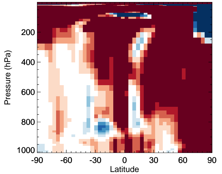
v11-02f-Run1 / v11-02e-Run0 ACTA - Zonal mean % diff for Jan
