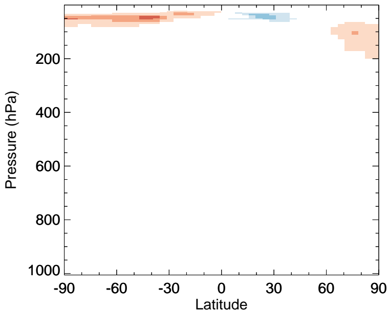
v11-02f-Run1 - v11-02e-Run0 OCS - Zonal mean abs diff for Jan
