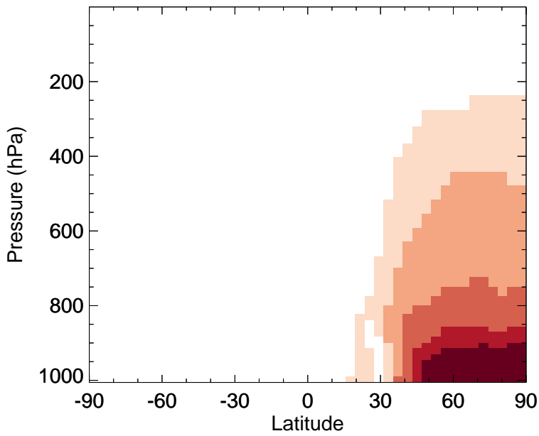
v11-02f-Run1 - v11-02e-Run1 C3H8 - Zonal mean abs diff for Jan
