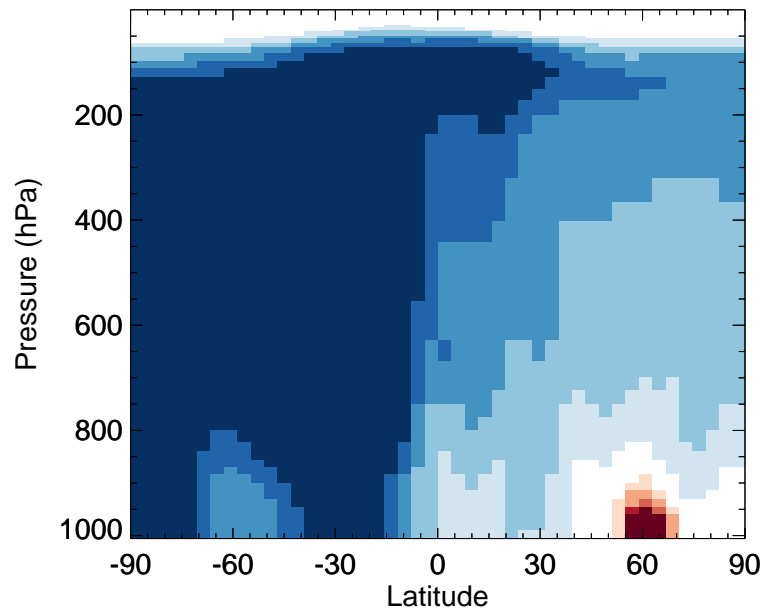
v11-02f-Run1 / v11-02e-Run1 SOAMG - Zonal mean % diff for Jan
