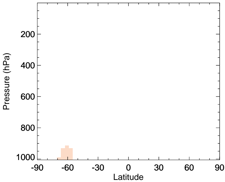
v11-02f-Run1 - v11-02e-Run0 SALA - Zonal mean abs diff for Jan
