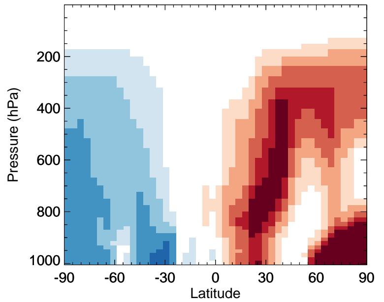
v11-02f-Run1 / v11-02e-Run1 BCPI - Zonal mean % diff for Jan
