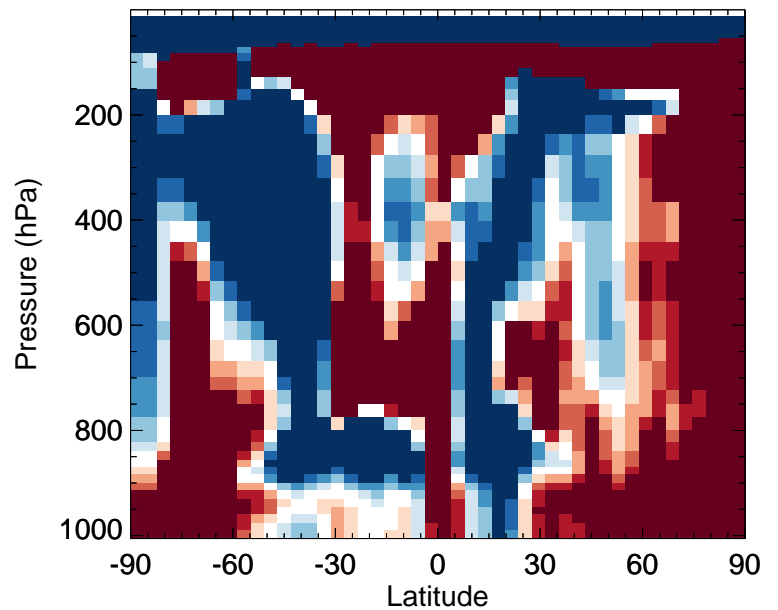
v11-02f-Run1 / v11-02e-Run0 SO4s - Zonal mean % diff for Jan
