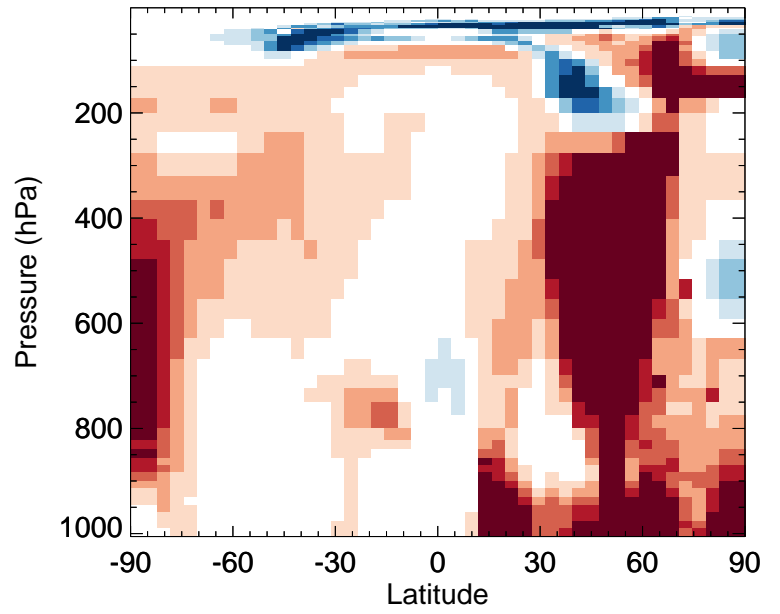
v11-02f-Run1 / v11-02e-Run1 HBr - Zonal mean % diff for Jan
