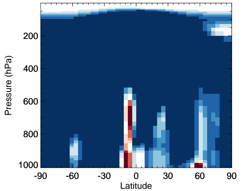
v11-02f-Run1 / v11-02e-Run0 SOAGX - Zonal mean % diff for Jan
