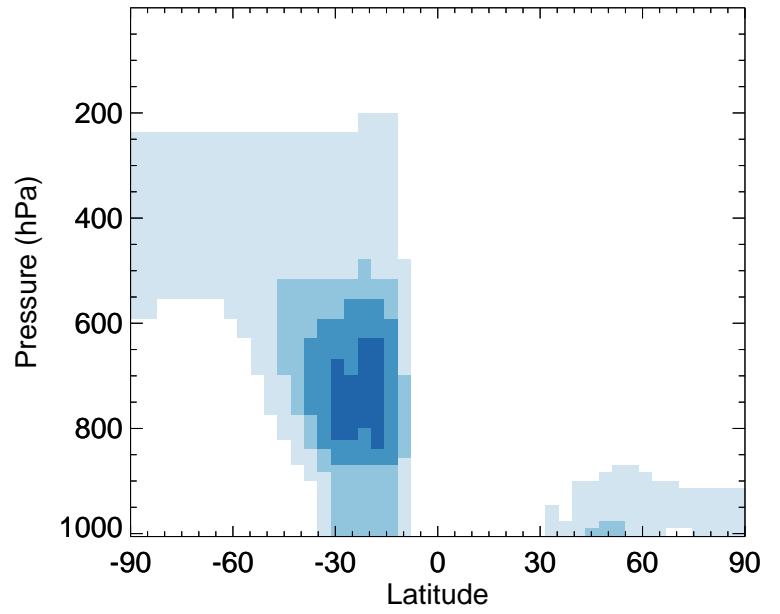
v11-02f-Run1 / v11-02e-Run1 SO4 - Zonal mean % diff for Jan
