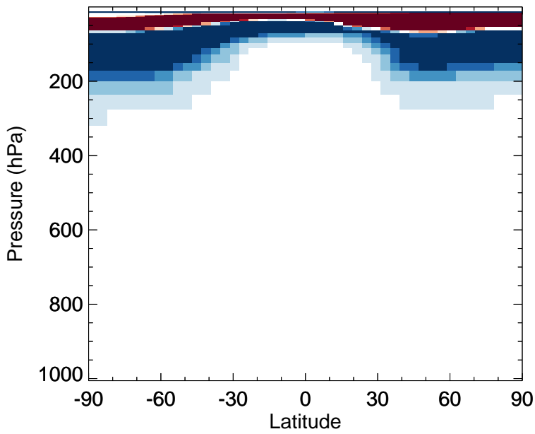
v11-02f-Run1 - v11-02e-Run1 O3 - Zonal mean abs diff for Jan
