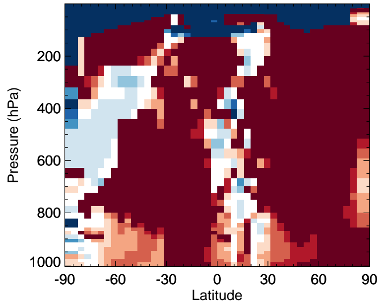
v11-02f-Run1 / v11-02e-Run1 NIT - Zonal mean % diff for Jan
