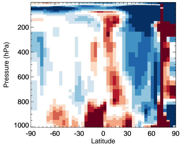
v11-02f-Run1 / v11-02e-Run0 NO - Zonal mean % diff for Jan
