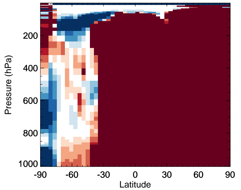
v11-02f-Run1 / v11-02e-Run1 RIPD - Zonal mean % diff for Jan
