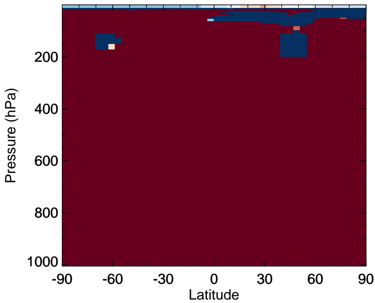
v11-02f-Run1 - v11-02e-Run0 N2O - Zonal mean abs diff for Jan
