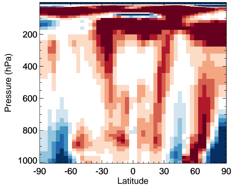
v11-02f-Run1 / v11-02e-Run0 H2O2 - Zonal mean % diff for Jan
