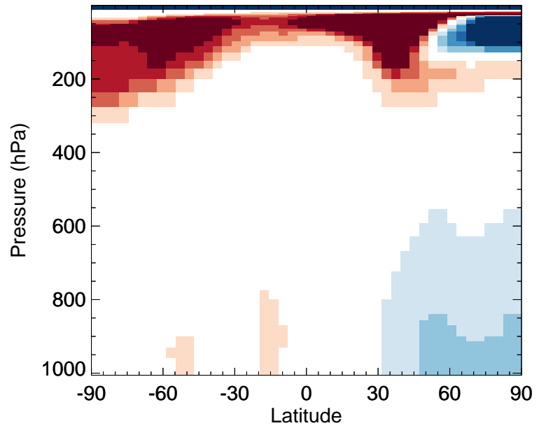
v11-02f-Run1 / v11-02e-Run1 H2O2 - Zonal mean % diff for Jan
