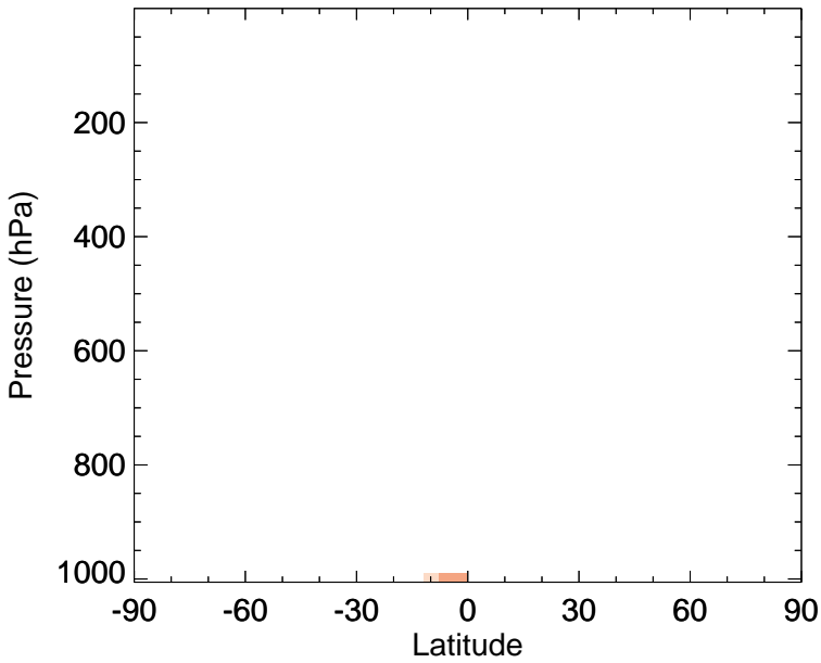
v11-02f-Run1 - v11-02e-Run0 MTPA - Zonal mean abs diff for Jan
