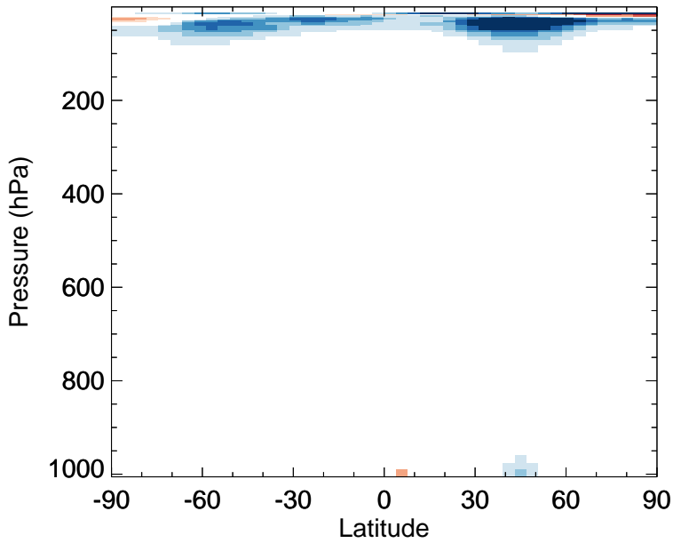
v11-02f-Run1 - v11-02e-Run0 NO 2 - Zonal mean abs diff for Jan
