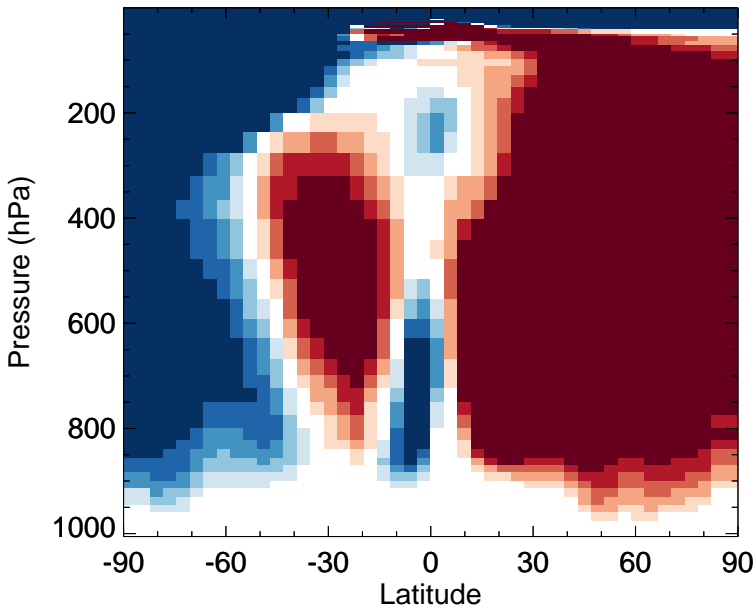
v11-02f-Run1 - v11-02e-Run1 CH4 - Zonal mean abs diff for Jan
