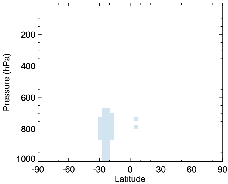
v11-02f-Run1 - v11-02e-Run0 GLYC - Zonal mean abs diff for Jan
