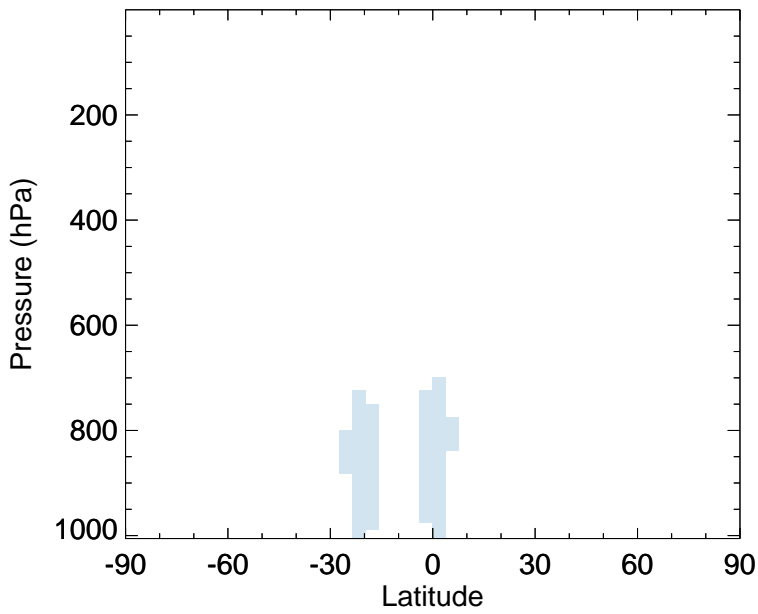
v11-02f-Run1 - v11-02e-Run1 GLYC - Zonal mean abs diff for Jan
