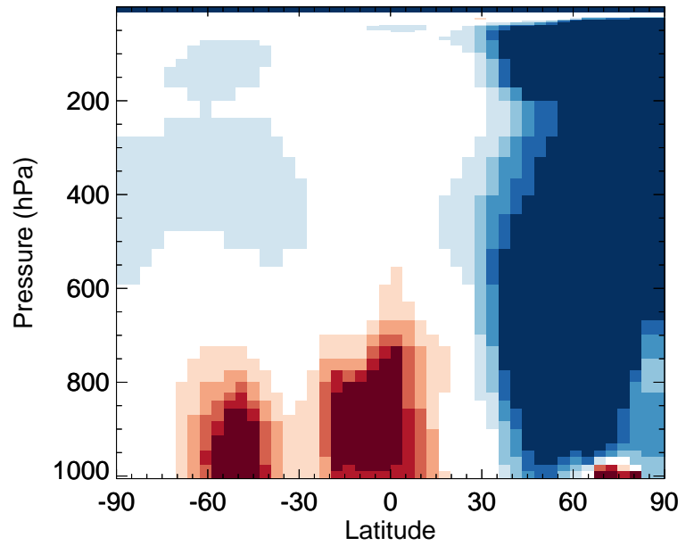
v11-02f-Run1 / v11-02e-Run1 HNO 4 - Zonal mean % diff for Jan
