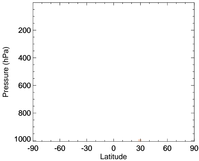
v11-02f-Run1 - v11-02e-Run0 BCPI - Zonal mean abs diff for Jan
