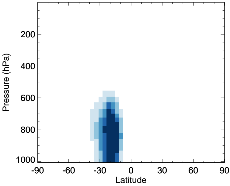
v11-02f-Run1 - v11-02e-Run1 SOAIE - Zonal mean abs diff for Jan
