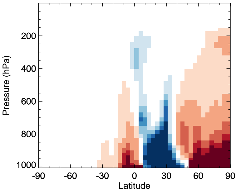
v11-02f-Run1 - v11-02e-Run0 BENZ - Zonal mean abs diff for Jan
