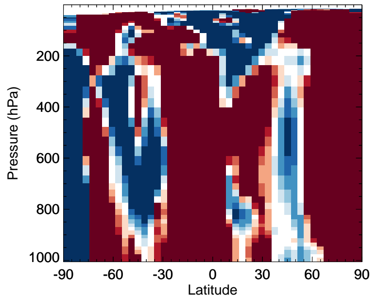
v11-02f-Run1 / v11-02e-Run0 SOAP - Zonal mean % diff for Jan
