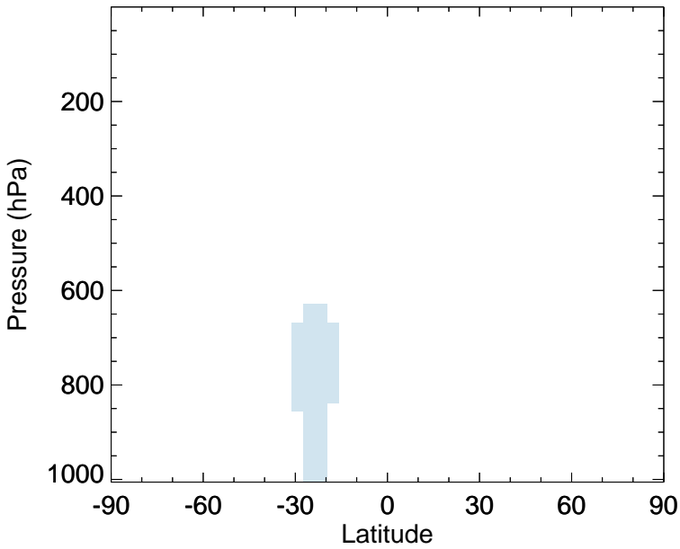
v11-02f-Run1 - v11-02e-Run0 ISO3 - Zonal mean abs diff for Jan
