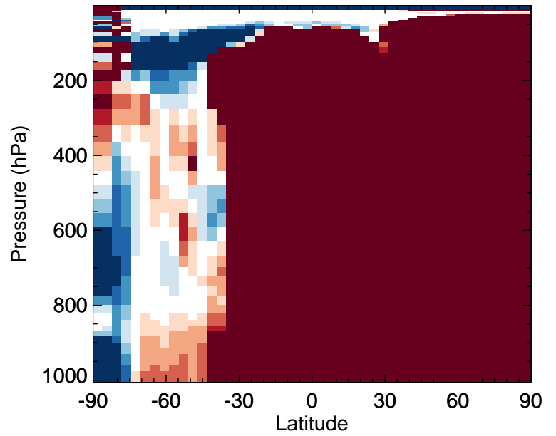
v11-02f-Run1 / v11-02e-Run1 RIPB - Zonal mean % diff for Jan
