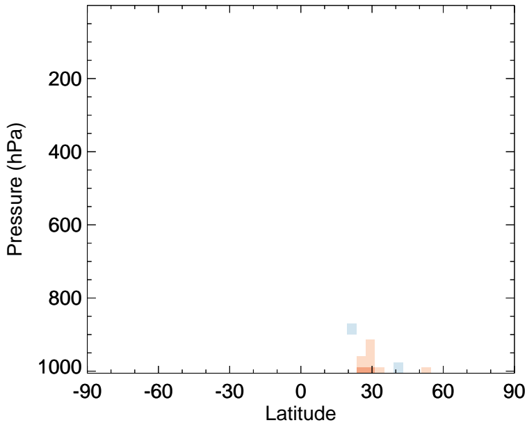
v11-02f-Run1 - v11-02e-Run0 NH4 - Zonal mean abs diff for Jan
