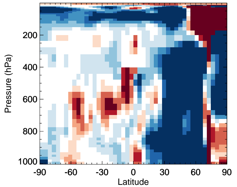
v11-02f-Run1 / v11-02e-Run0 ClOO - Zonal mean % diff for Jan
