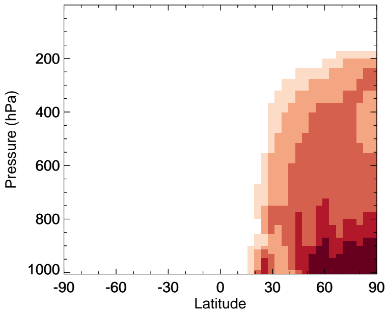
v11-02f-Run1 - v11-02e-Run0 C3H8 - Zonal mean abs diff for Jan
