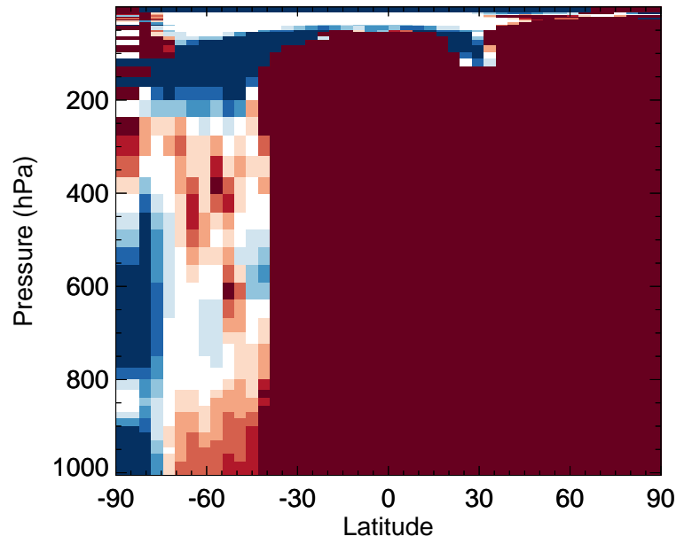
v11-02f-Run1 / v11-02e-Run1 ISOP - Zonal mean % diff for Jan
