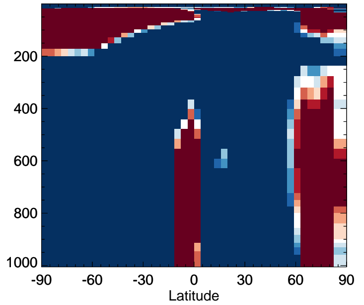
v11-02f-Run1 / v11-02e-Run0 DST2 - Zonal mean % diff for Jan
