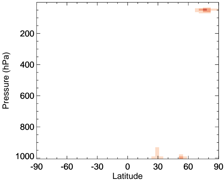
v11-02f-Run1 - v11-02e-Run0 NIT - Zonal mean abs diff for Jan
