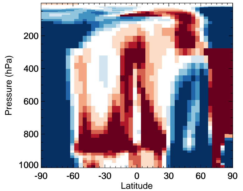
v11-02f-Run1 / v11-02e-Run0 HCl - Zonal mean % diff for Jan
