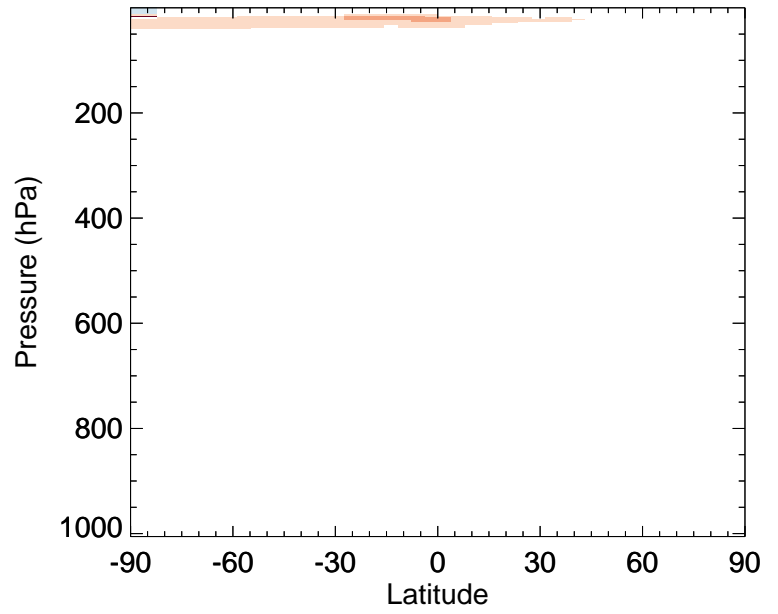
v11-02f-Run1 / v11-02e-Run1 CH2Br2 - Zonal mean % diff for Jan
