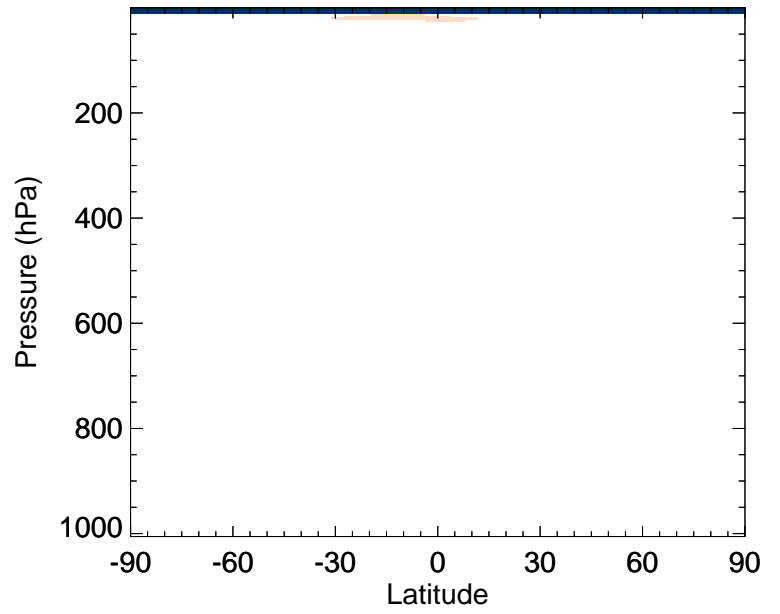
v11-02f-Run1 / v11-02e-Run1 CCI4 - Zonal mean % diff for Jan
