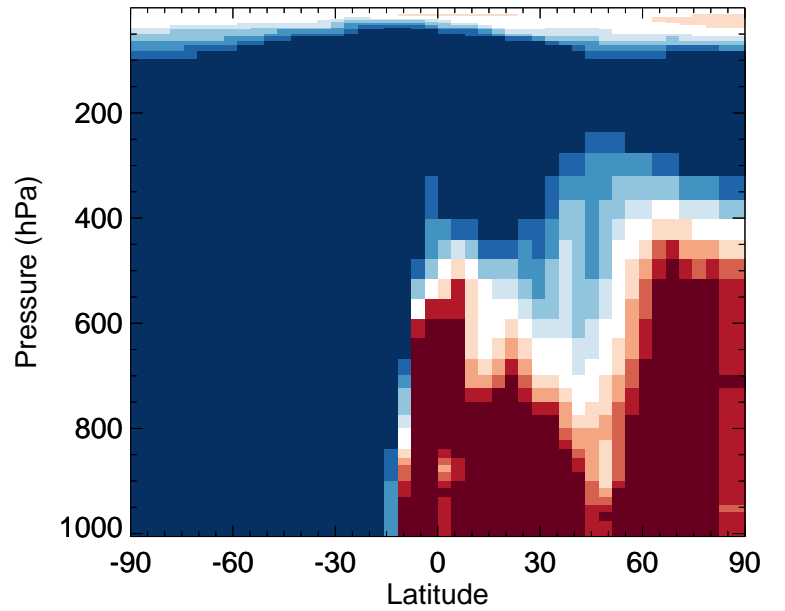
v11-02f-Run1 / v11-02e-Run0 SOAIE - Zonal mean % diff for Jan
