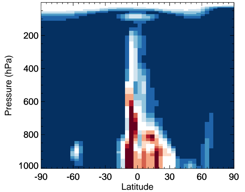
v11-02f-Run1 / v11-02e-Run0 ISO3 - Zonal mean % diff for Jan
