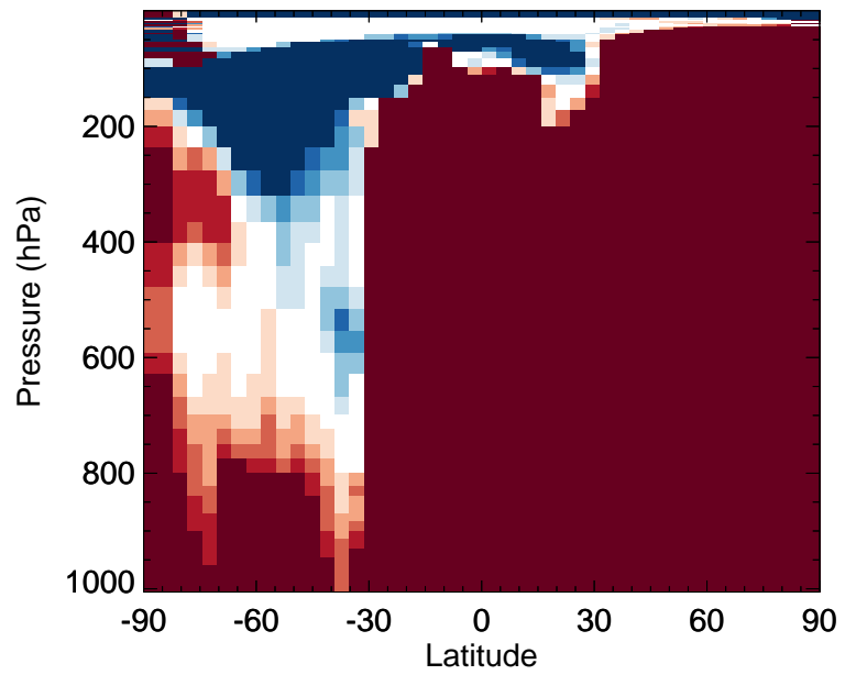
v11-02f-Run1 / v11-02e-Run1 ISN1 - Zonal mean % diff for Jan
