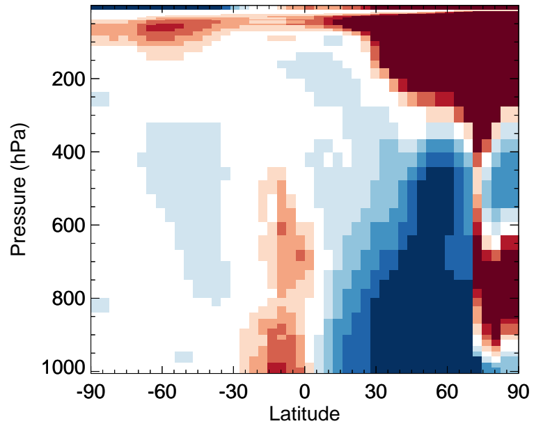
v11-02f-Run1 / v11-02e-Run1 ClO - Zonal mean % diff for Jan
