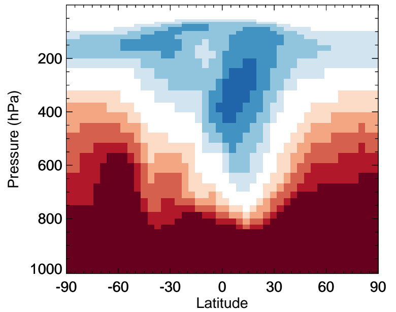
v11-02f-Run1 / v11-02e-Run1 TSOA0 - Zonal mean % diff for Jan
