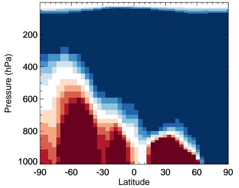
v11-02f-Run1 / v11-02e-Run1 DHDN - Zonal mean % diff for Jan
