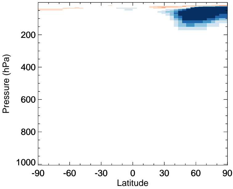
v11-02f-Run1 - v11-02e-Run1 CINO3 - Zonal mean abs diff for Jan
