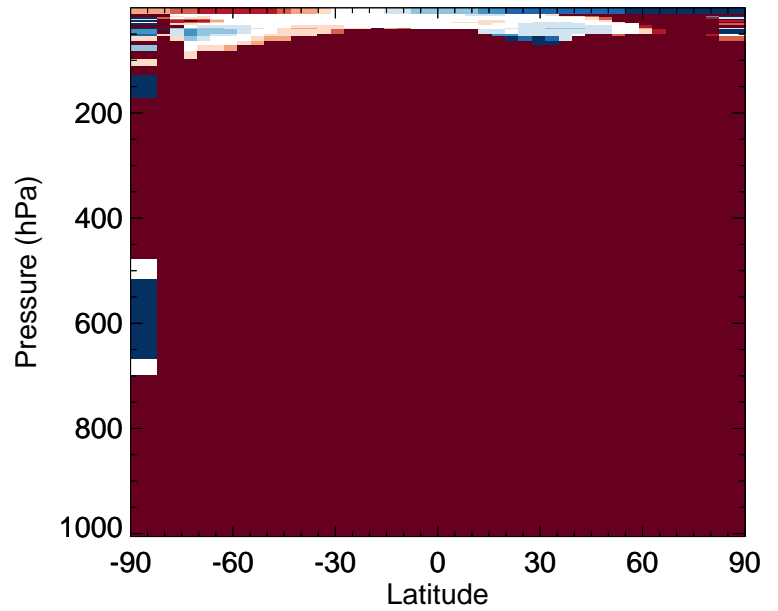
v11-02f-Run1 / v11-02e-Run0 MTPA - Zonal mean % diff for Jan
