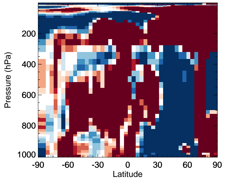
v11-02f-Run1 / v11-02e-Run0 Cl2O2 - Zonal mean % diff for Jan
