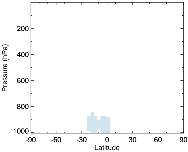
v11-02f-Run1 - v11-02e-Run1 HPALD - Zonal mean abs diff for Jan
