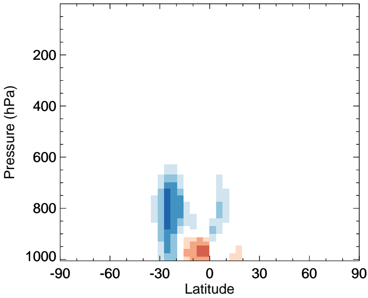
v11-02f-Run1 - v11-02e-Run0 MVK - Zonal mean abs diff for Jan
