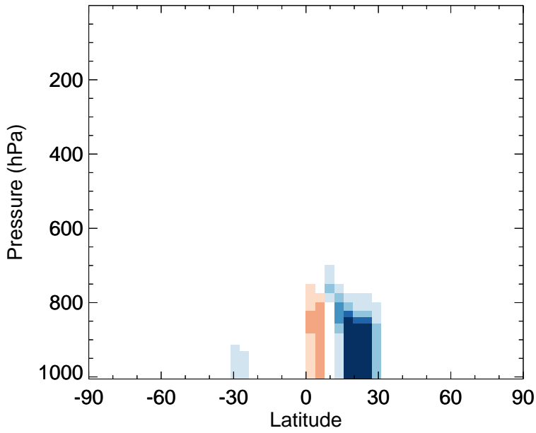
v11-02f-Run1 - v11-02e-Run0 DST2 - Zonal mean abs diff for Jan
