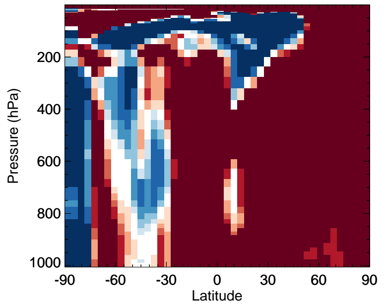
v11-02f-Run1 / v11-02e-Run0 MEK - Zonal mean % diff for Jan
