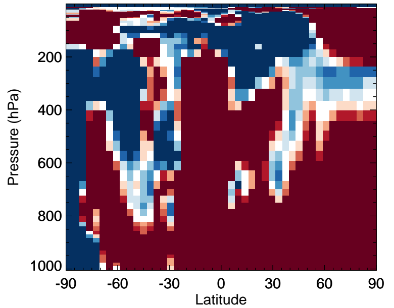
v11-02f-Run1 / v11-02e-Run0 IEPOXA - Zonal mean % diff for Jan
