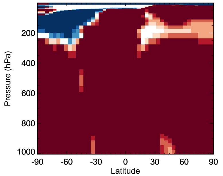
v11-02f-Run1 / v11-02e-Run1 PRPE - Zonal mean % diff for Jan
