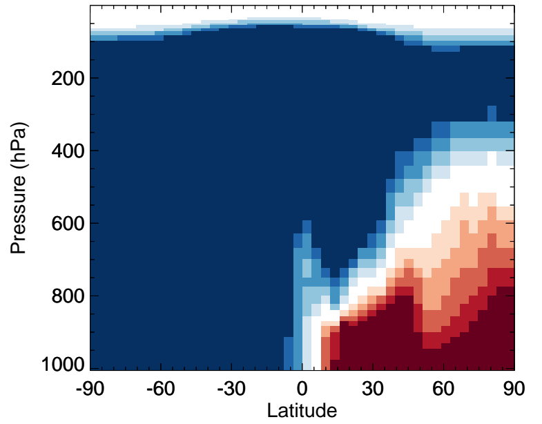
v11-02f-Run1 / v11-02e-Run1 SOAIE - Zonal mean % diff for Jan
