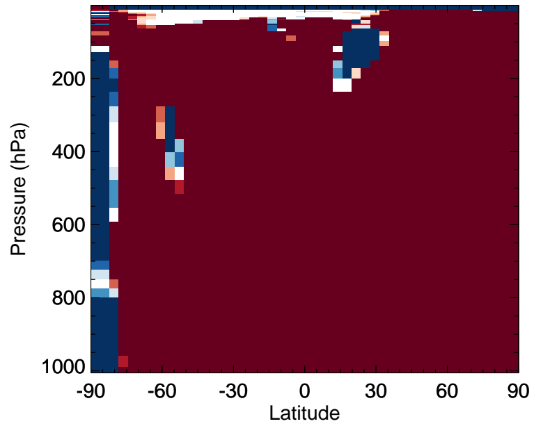
v11-02f-Run1 / v11-02e-Run0 MVK - Zonal mean % diff for Jan
