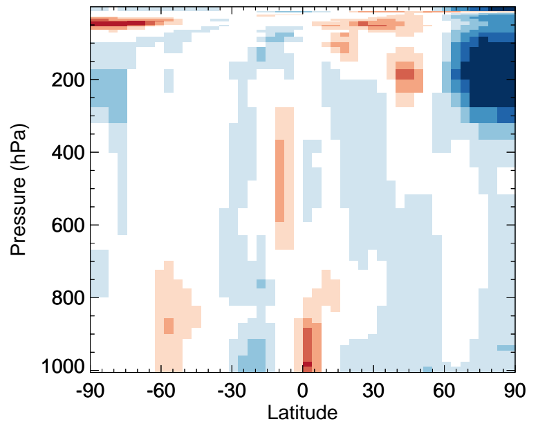
v11-02f-Run1 / v11-02e-Run0 O3 - Zonal mean % diff for Jan
