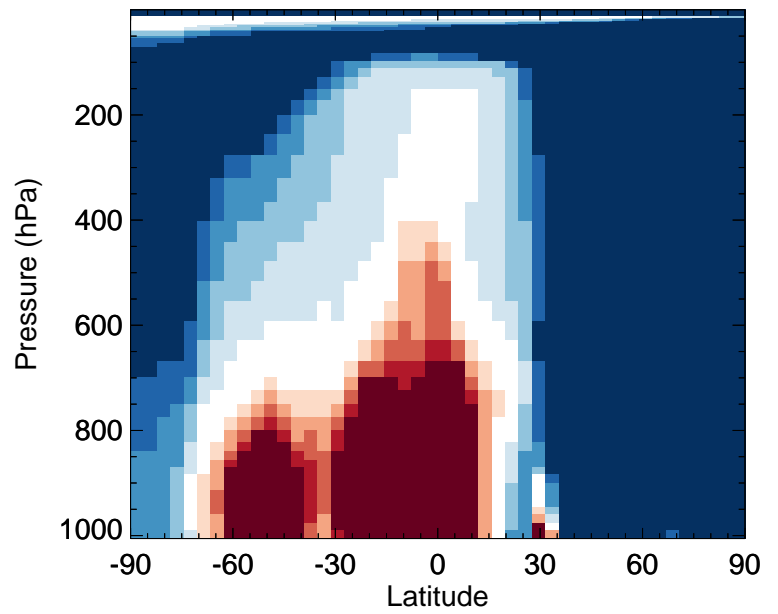
v11-02f-Run1 / v11-02e-Run1 N2O5 - Zonal mean % diff for Jan
