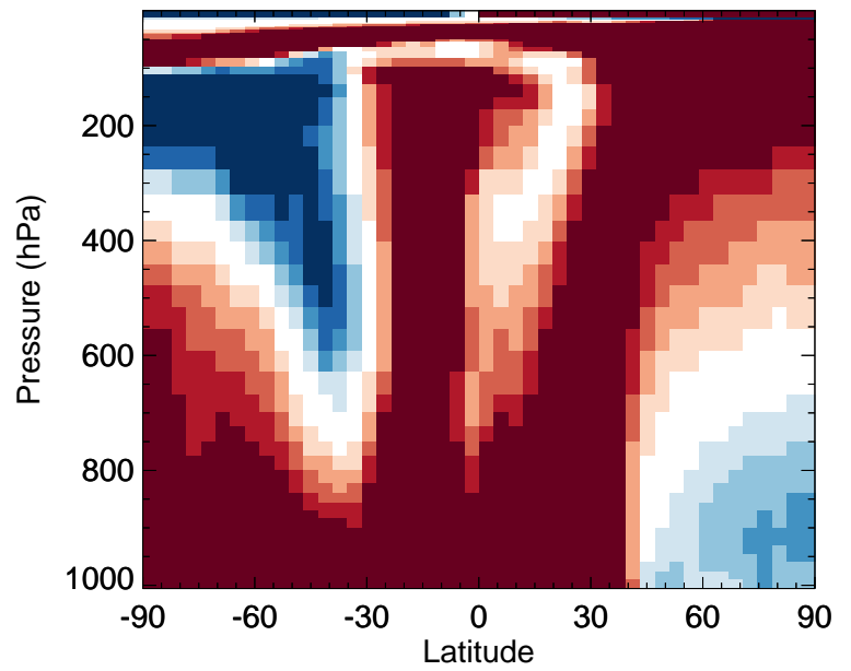
v11-02f-Run1 / v11-02e-Run1 EOH - Zonal mean % diff for Jan
