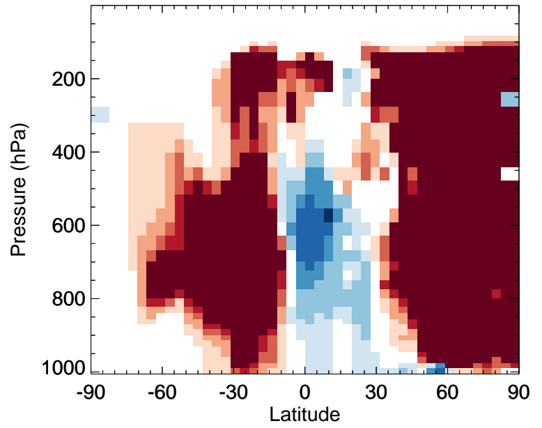
v11-02f-Run1 / v11-02e-Run1 NH3 - Zonal mean % diff for Jan
