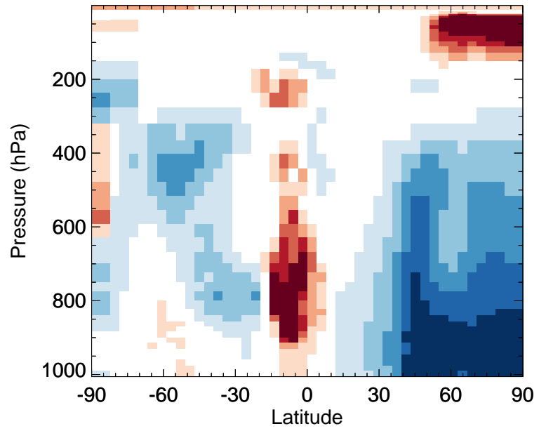
v11-02f-Run1 / v11-02e-Run1 BrCl - Zonal mean % diff for Jan
