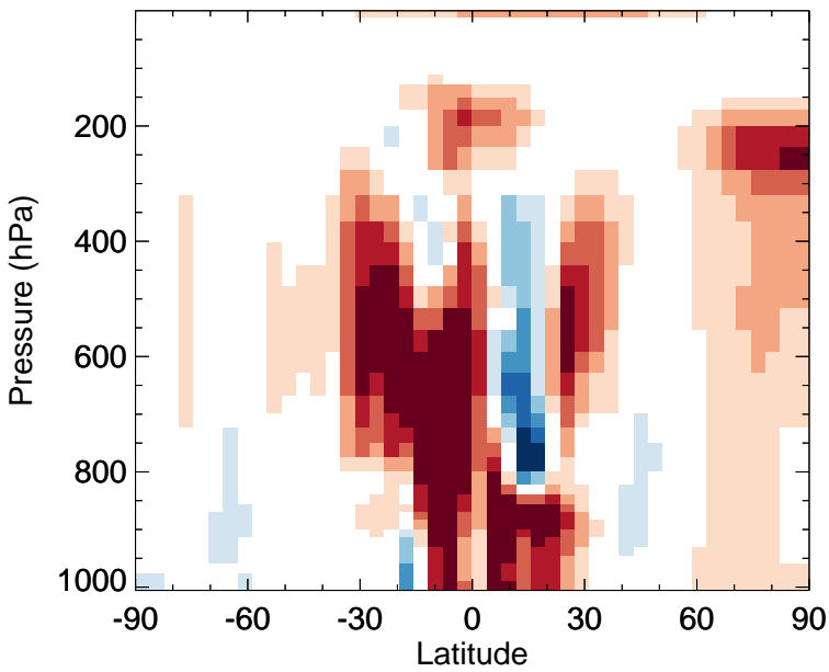
v11-02f-Run1 - v11-02e-Run0 MP - Zonal mean abs diff for Jan
