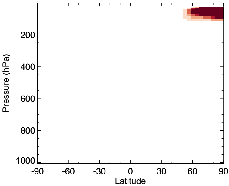
v11-02f-Run1 - v11-02e-Run0 Cl2O2 - Zonal mean abs diff for Jan
