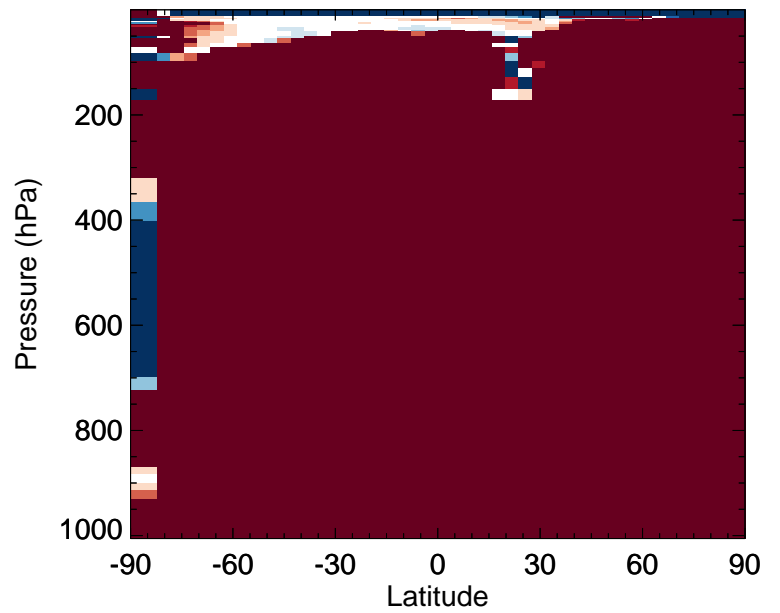
v11-02f-Run1 / v11-02e-Run0 RIPA - Zonal mean % diff for Jan
