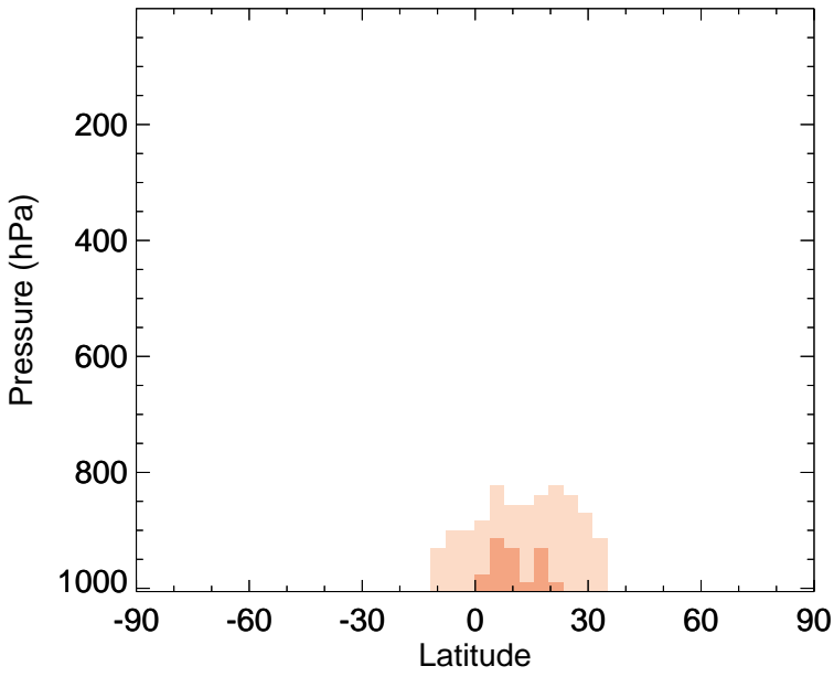
v11-02f-Run1 - v11-02e-Run1 INDIOL - Zonal mean abs diff for Jan
