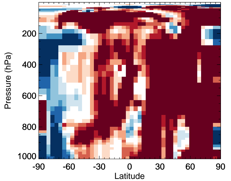
v11-02f-Run1 / v11-02e-Run0 HBr - Zonal mean % diff for Jan
