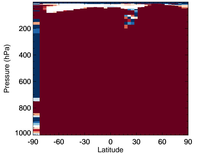
v11-02f-Run1 / v11-02e-Run0 MOBA - Zonal mean % diff for Jan
