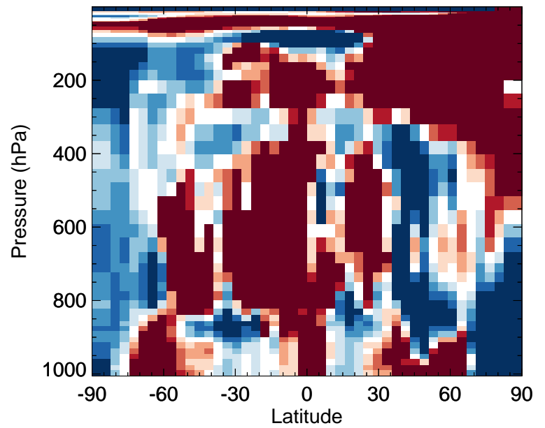
v11-02f-Run1 / v11-02e-Run0 OCIO - Zonal mean % diff for Jan
