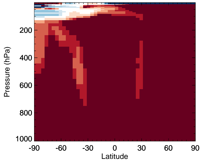
v11-02f-Run1 / v11-02e-Run1 ALK4 - Zonal mean % diff for Jan
