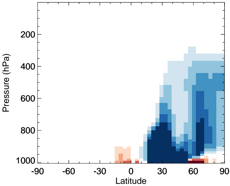
v11-02f-Run1 - v11-02e-Run0 TOLU - Zonal mean abs diff for Jan
