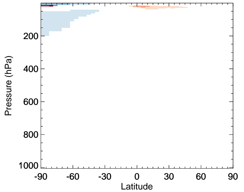
v11-02f-Run1 / v11-02e-Run1 CHBr3 - Zonal mean % diff for Jan
