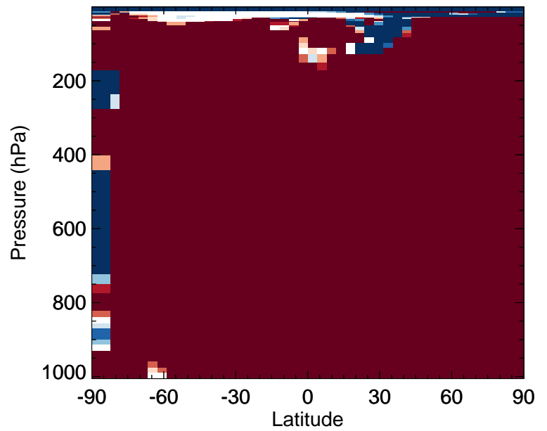
v11-02f-Run1 / v11-02e-Run0 LVOC - Zonal mean % diff for Jan
