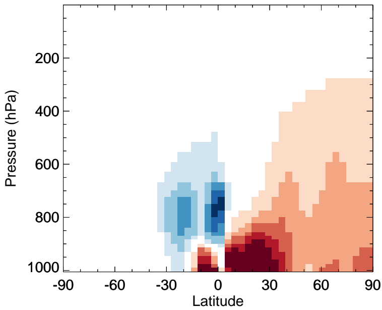
v11-02f-Run1 - v11-02e-Run1 MEK - Zonal mean abs diff for Jan
