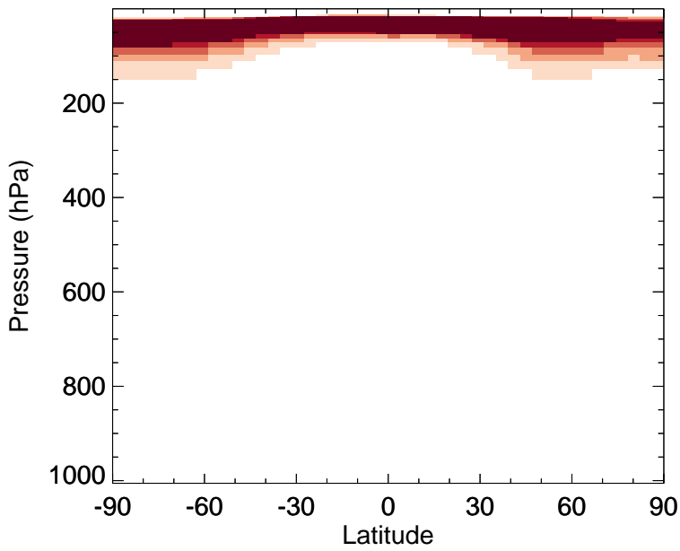
v11-02f-Run1 - v11-02e-Run1 N2O - Zonal mean abs diff for Jan
