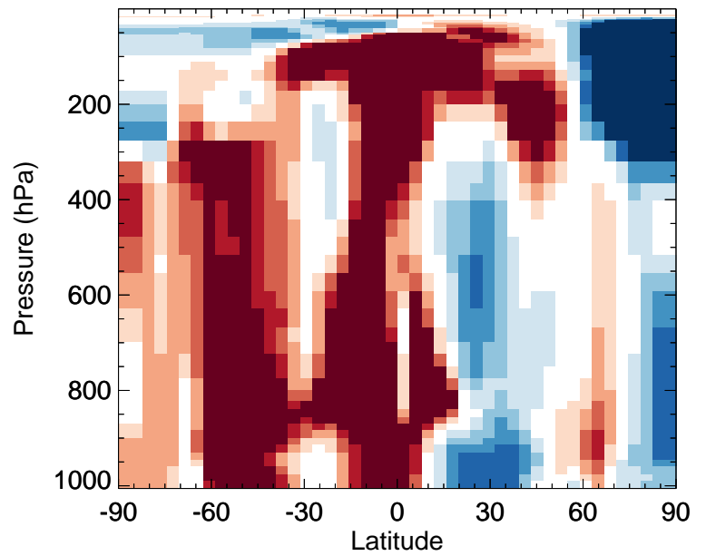
v11-02f-Run1 / v11-02e-Run0 ISO2 - Zonal mean % diff for Jan
