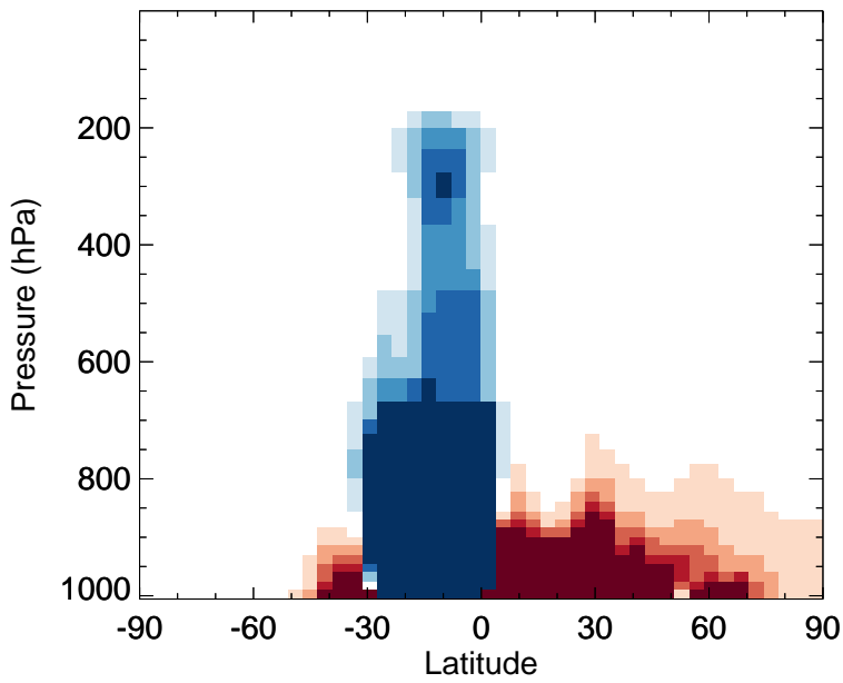
v11-02f-Run1 - v11-02e-Run1 PRPE - Zonal mean abs diff for Jan
