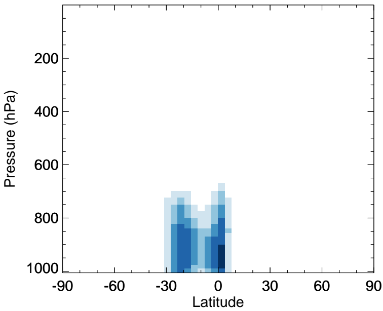
v11-02f-Run1 - v11-02e-Run1 MACR - Zonal mean abs diff for Jan
