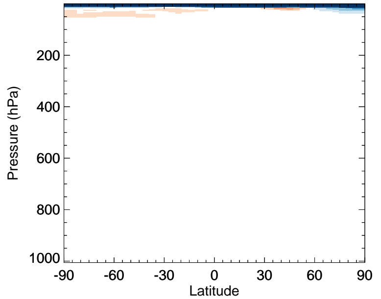
v11-02f-Run1 / v11-02e-Run0 CH4 - Zonal mean % diff for Jan
