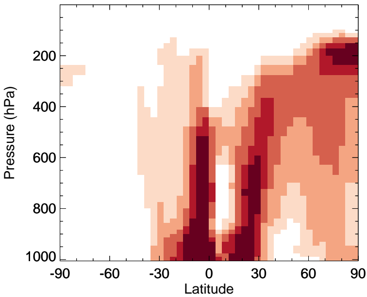
v11-02f-Run1 - v11-02e-Run0 ACET - Zonal mean abs diff for Jan
