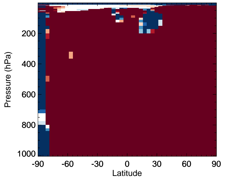
v11-02f-Run1 / v11-02e-Run0 HPALD - Zonal mean % diff for Jan
