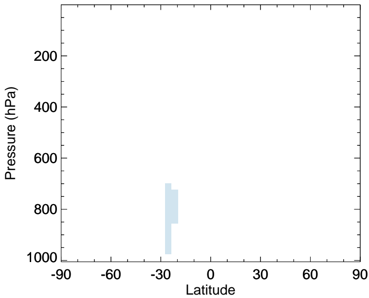
v11-02f-Run1 - v11-02e-Run0 RIPA - Zonal mean abs diff for Jan
