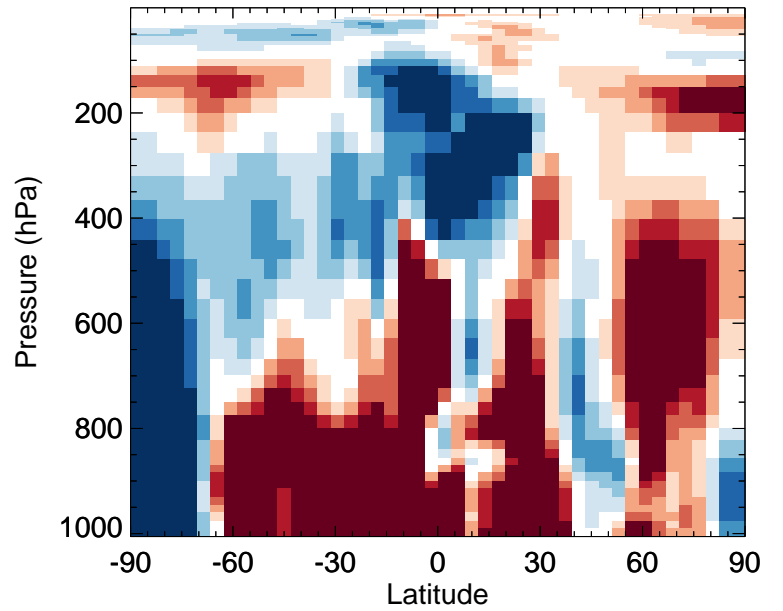
v11-02f-Run1 / v11-02e-Run0 OCPI - Zonal mean % diff for Jan
