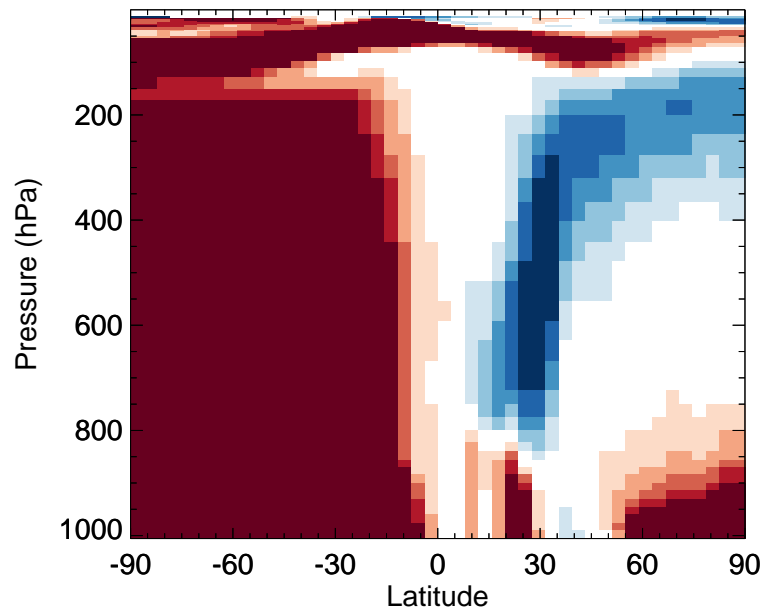
v11-02f-Run1 / v11-02e-Run1 BENZ - Zonal mean % diff for Jan
