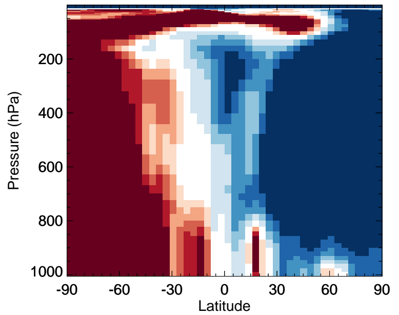
v11-02f-Run1 / v11-02e-Run1 GLYX - Zonal mean % diff for Jan
