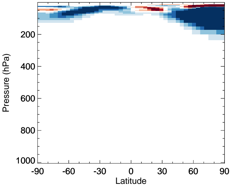
v11-02f-Run1 - v11-02e-Run0 CINO3 - Zonal mean abs diff for Jan
