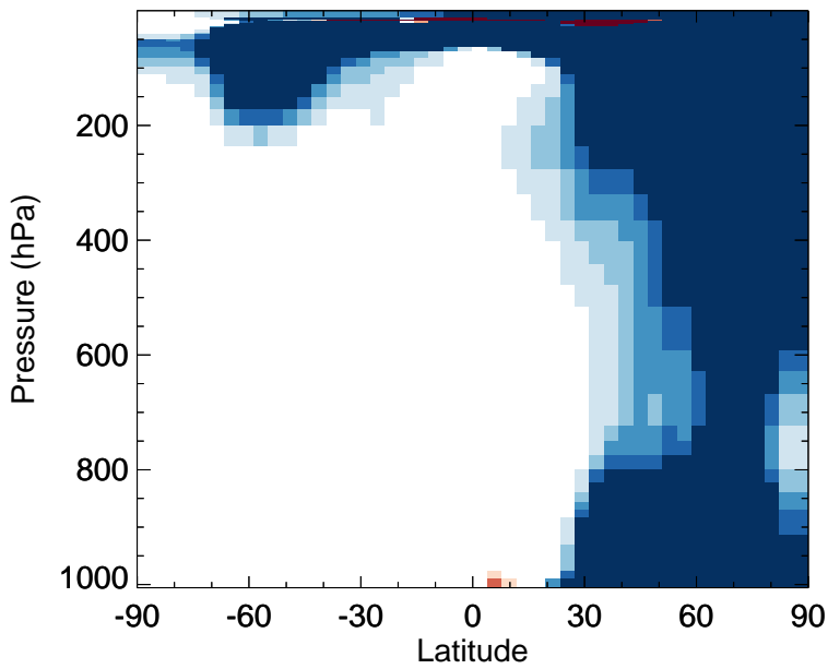
v11-02f-Run1 - v11-02e-Run0 N2O5 - Zonal mean abs diff for Jan
