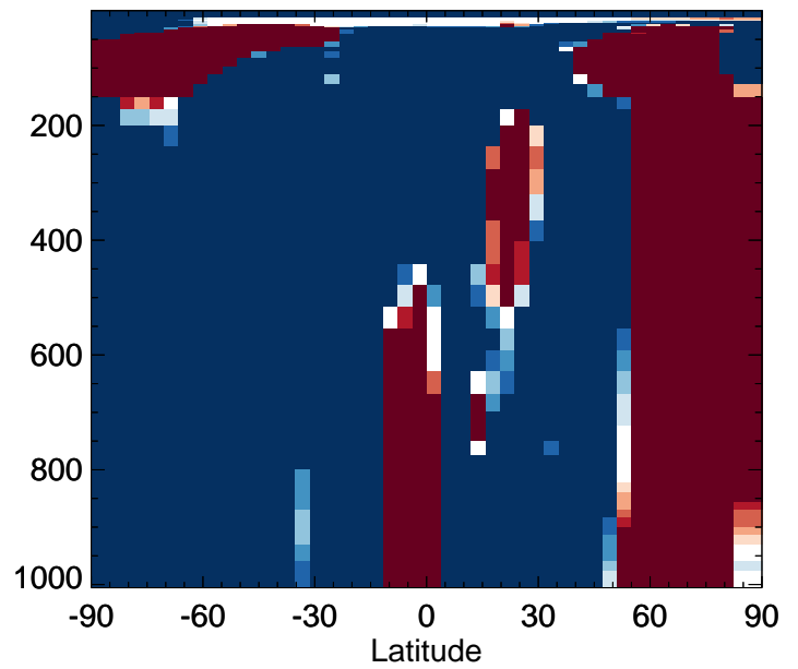
v11-02f-Run1 / v11-02e-Run0 DST4 - Zonal mean % diff for Jan
