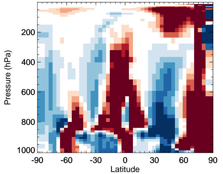
v11-02f-Run1 / v11-02e-Run0 BrO - Zonal mean % diff for Jan
