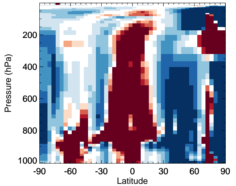
v11-02f-Run1 / v11-02e-Run0 BrNO3 - Zonal mean % diff for Jan
