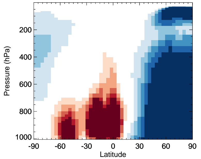
v11-02f-Run1 / v11-02e-Run1 NO 3 - Zonal mean % diff for Jan
