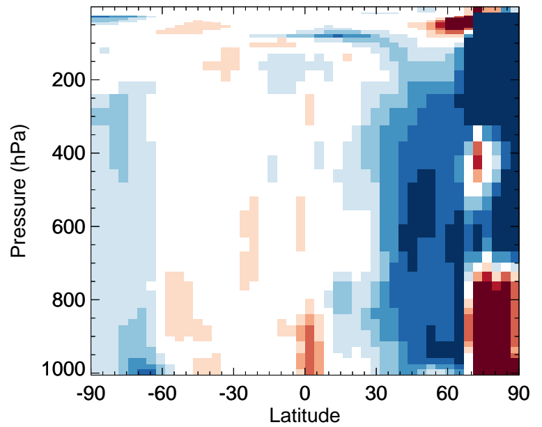
v11-02f-Run1 / v11-02e-Run0 OH - Zonal mean % diff for Jan
