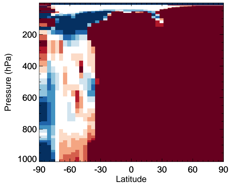
v11-02f-Run1 / v11-02e-Run1 RIPA - Zonal mean % diff for Jan
