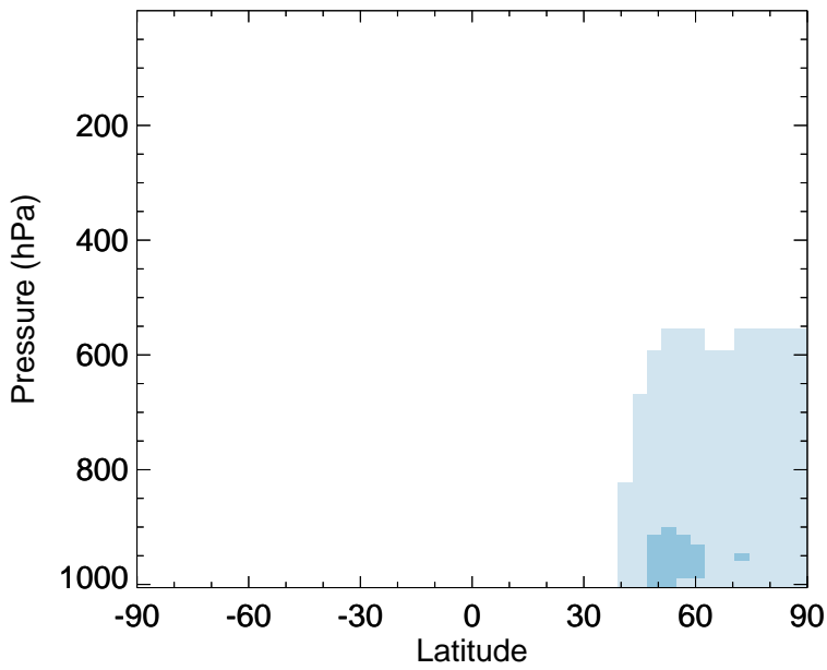
v11-02f-Run1 - v11-02e-Run1 PAN - Zonal mean abs diff for Jan
