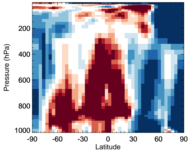
v11-02f-Run1 / v11-02e-Run0 NO 3 - Zonal mean % diff for Jan
