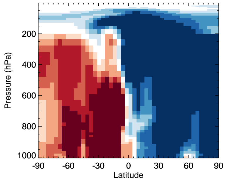
v11-02f-Run1 / v11-02e-Run0 ASOAN - Zonal mean % diff for Jan
