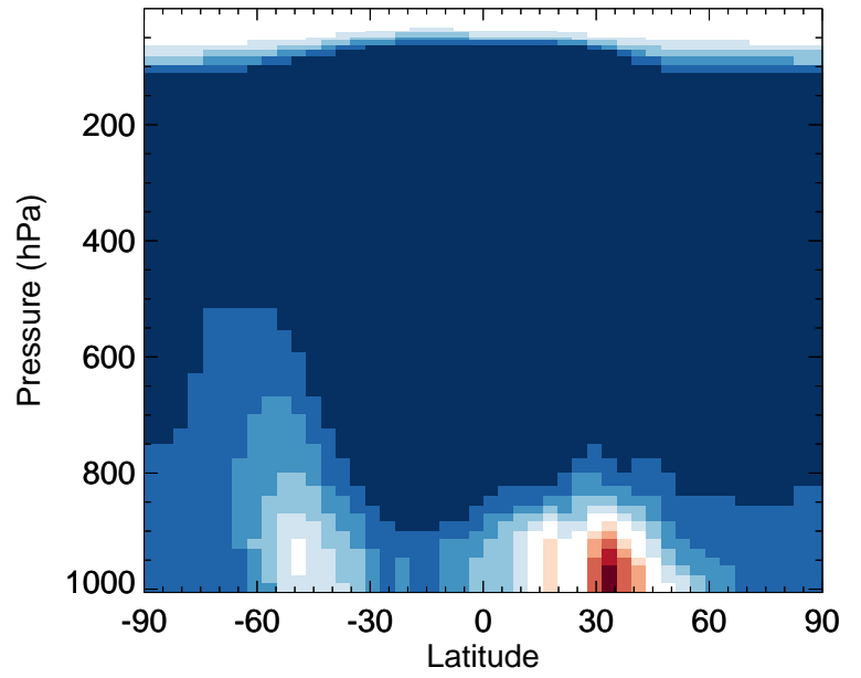
v11-02f-Run1 / v11-02e-Run1 ISO3 - Zonal mean % diff for Jan
