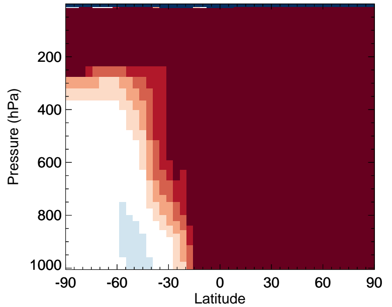
v11-02f-Run1 / v11-02e-Run0 C2H6 - Zonal mean % diff for Jan
