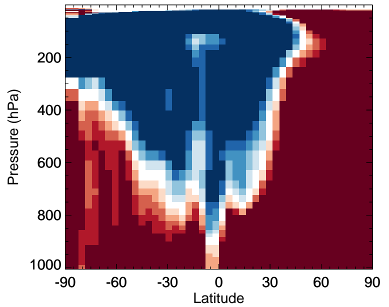
v11-02f-Run1 / v11-02e-Run1 HC187 - Zonal mean % diff for Jan
