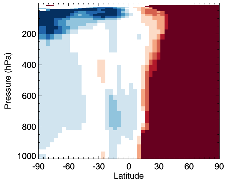
v11-02f-Run1 / v11-02e-Run1 DMS - Zonal mean % diff for Jan
