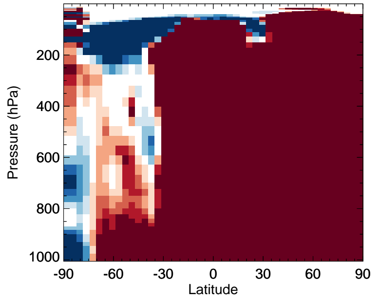
v11-02f-Run1 / v11-02e-Run1 MOBA - Zonal mean % diff for Jan
