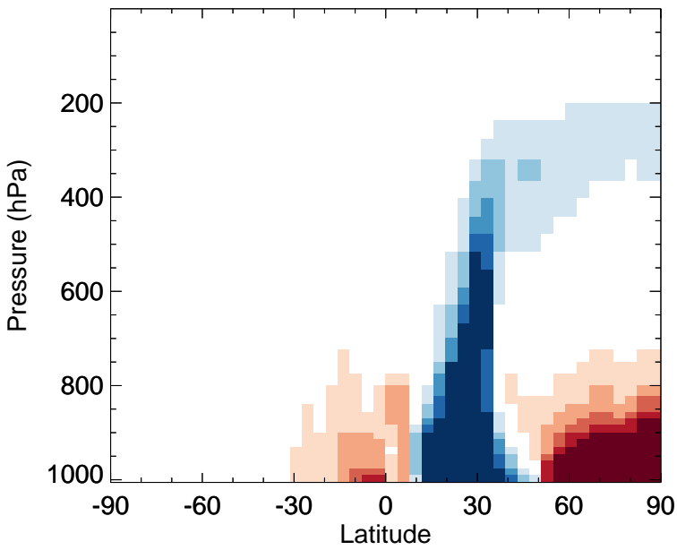
v11-02f-Run1 - v11-02e-Run1 BENZ - Zonal mean abs diff for Jan
