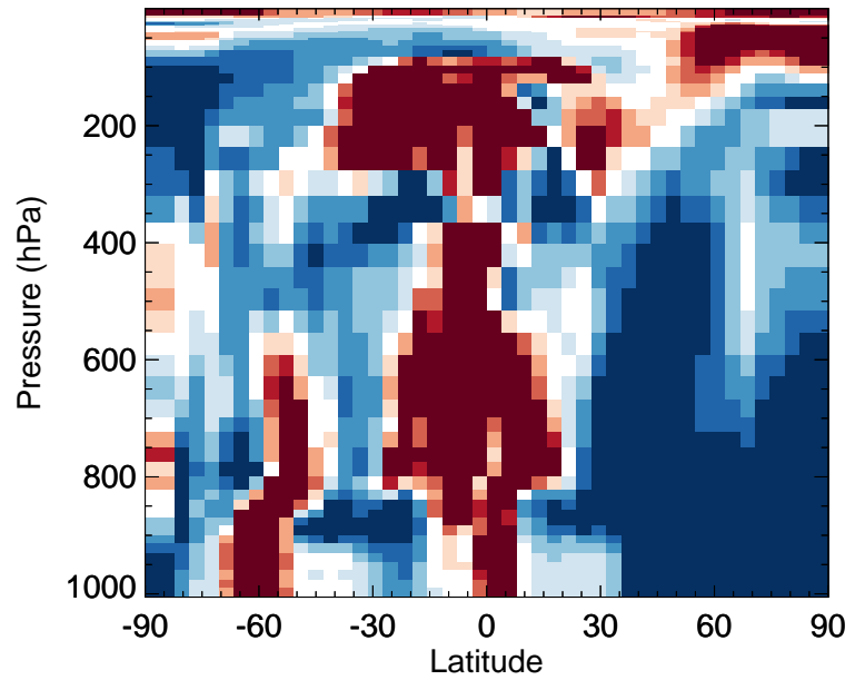
v11-02f-Run1 / v11-02e-Run0 BrCl - Zonal mean % diff for Jan
