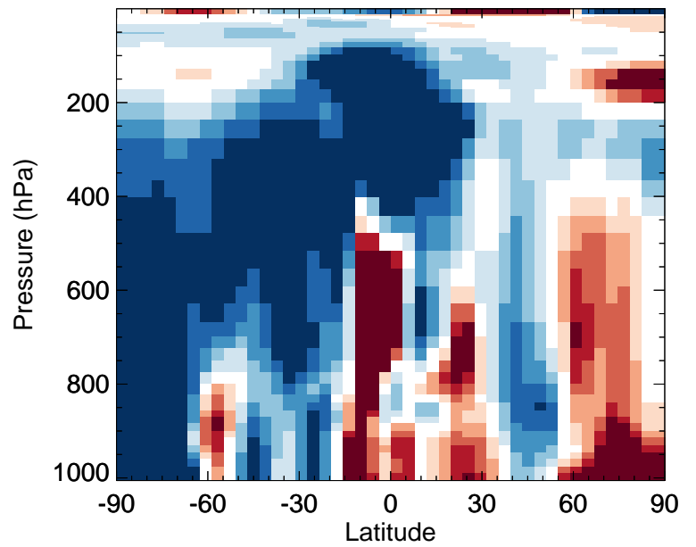
v11-02f-Run1 / v11-02e-Run0 BCPI - Zonal mean % diff for Jan
