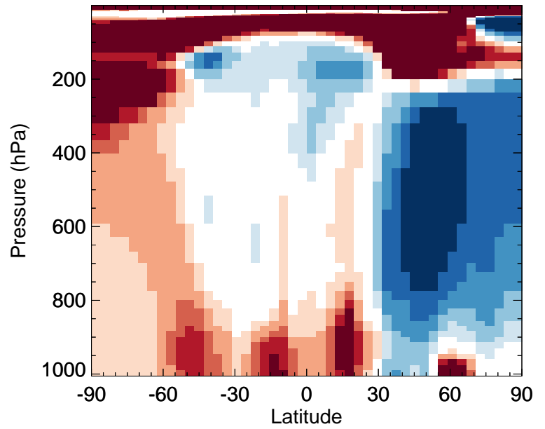
v11-02f-Run1 / v11-02e-Run1 MGLY - Zonal mean % diff for Jan
