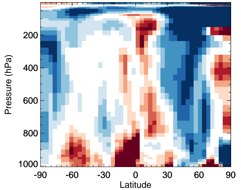
v11-02f-Run1 / v11-02e-Run0 NO 2 - Zonal mean % diff for Jan
