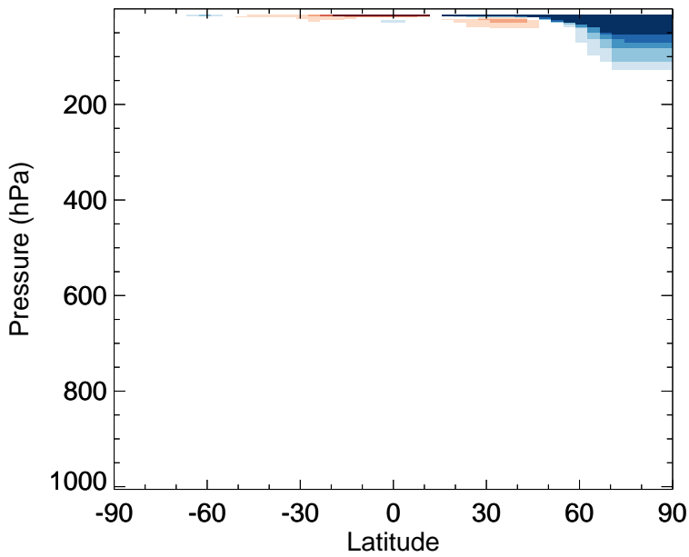
v11-02f-Run1 - v11-02e-Run0 NO 3 - Zonal mean abs diff for Jan
