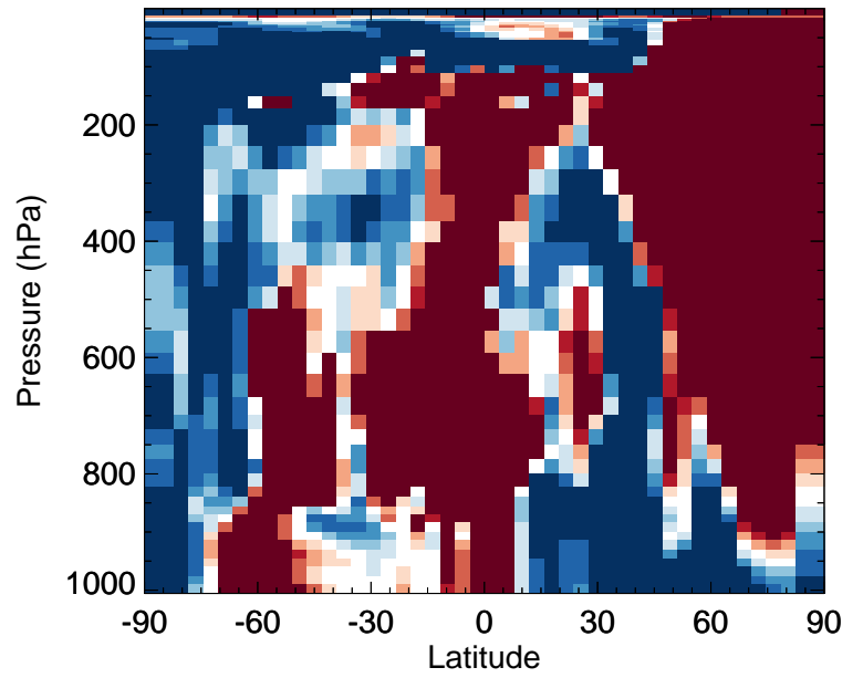
v11-02f-Run1 / v11-02e-Run0 Cl2 - Zonal mean % diff for Jan
