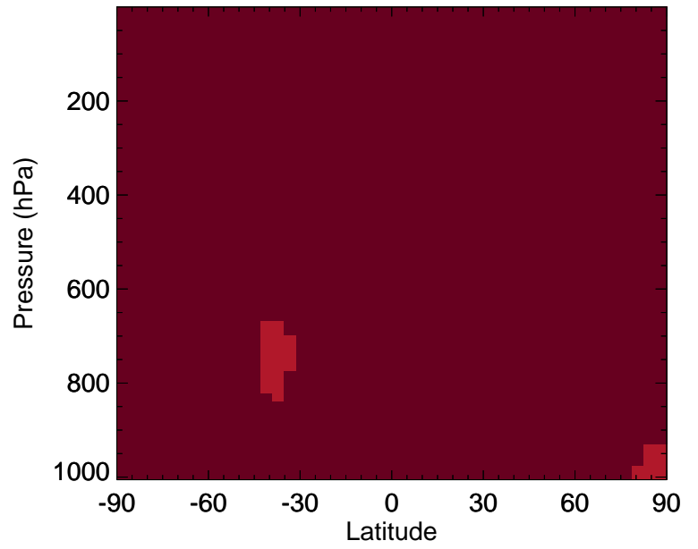
v11-02f-Run1 / v11-02e-Run1 INDIOL - Zonal mean % diff for Jan
