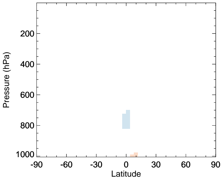
v11-02f-Run1 - v11-02e-Run1 HAC - Zonal mean abs diff for Jan
