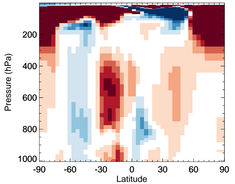
v11-02f-Run1 / v11-02e-Run0 CHBr3 - Zonal mean % diff for Jan
