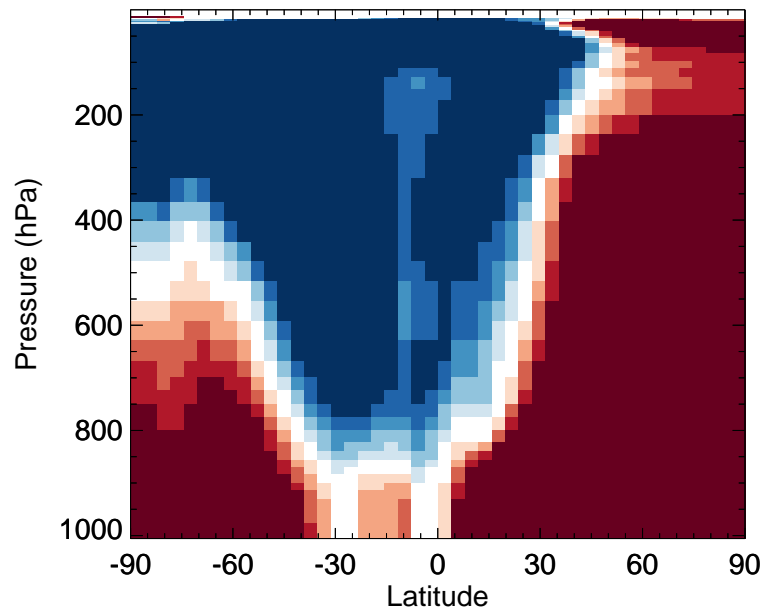
v11-02f-Run1 / v11-02e-Run1 IMAE - Zonal mean % diff for Jan
