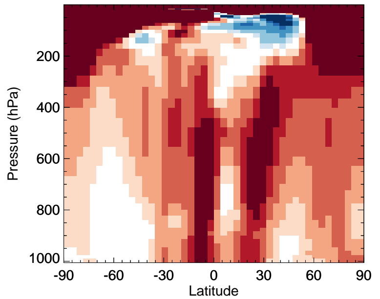
v11-02f-Run1 / v11-02e-Run0 ACET - Zonal mean % diff for Jan
