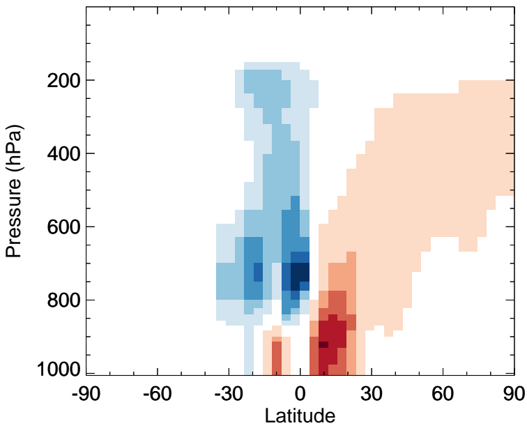
v11-02f-Run1 - v11-02e-Run1 MAP - Zonal mean abs diff for Jan
