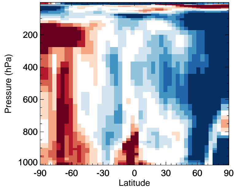
v11-02f-Run1 / v11-02e-Run0 MPN - Zonal mean % diff for Jan
