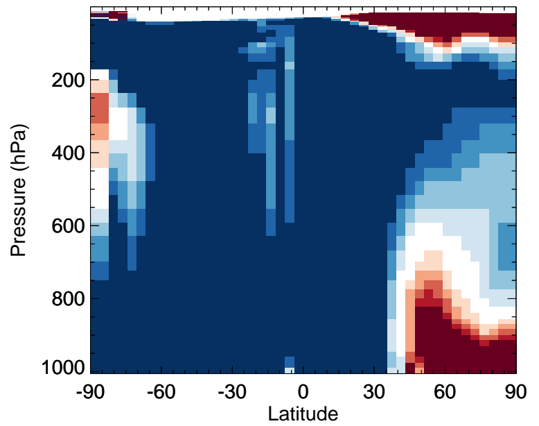
v11-02f-Run1 / v11-02e-Run1 XYLE - Zonal mean % diff for Jan
