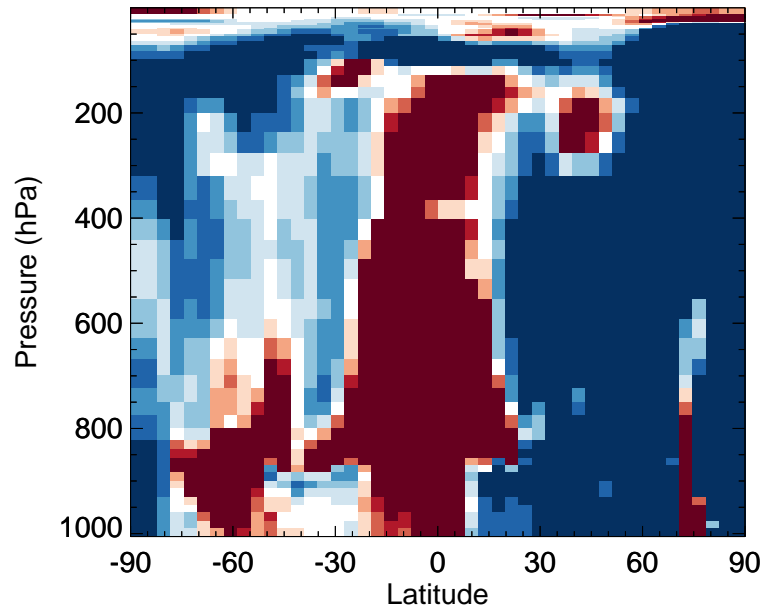
v11-02f-Run1 / v11-02e-Run0 CINO3 - Zonal mean % diff for Jan
