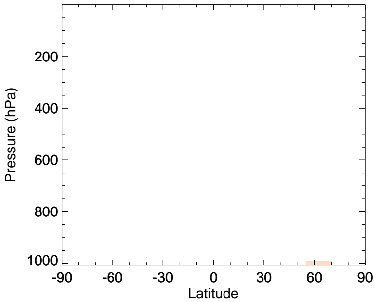
v11-02f-Run1 - v11-02e-Run1 CH 2 O - Zonal mean abs diff for Jan
