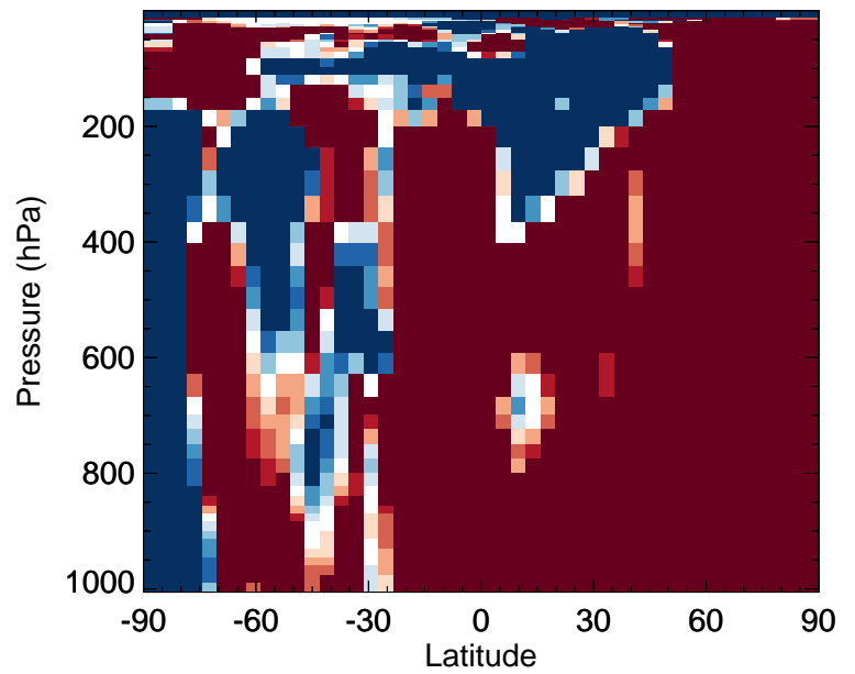
v11-02f-Run1 / v11-02e-Run0 HC187 - Zonal mean % diff for Jan
