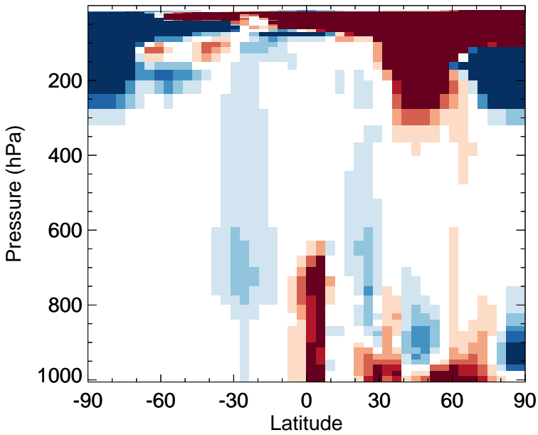
v11-02f-Run1 - v11-02e-Run0 HNO 3 - Zonal mean abs diff for Jan
