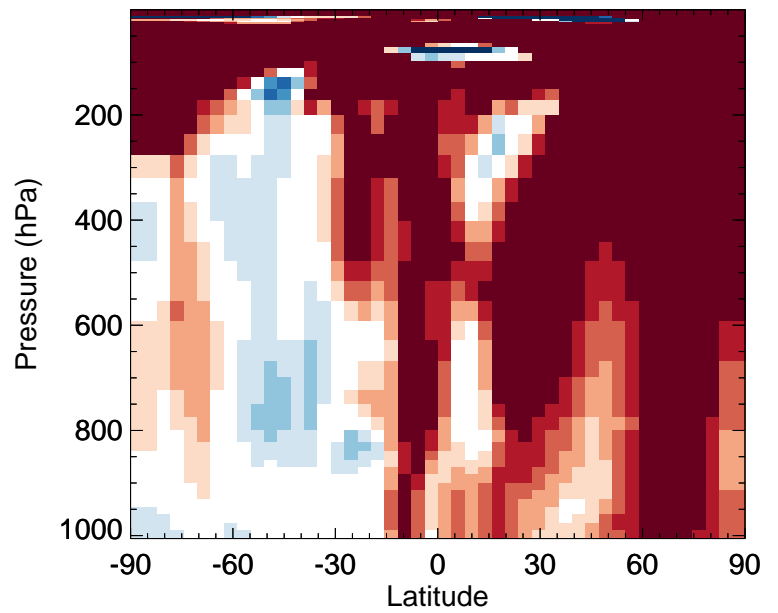
v11-02f-Run1 / v11-02e-Run0 MAP - Zonal mean % diff for Jan
