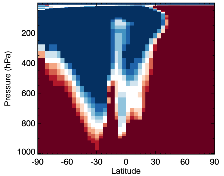
v11-02f-Run1 / v11-02e-Run1 GLYC - Zonal mean % diff for Jan
