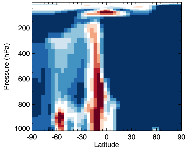
v11-02f-Run1 / v11-02e-Run0 ASOG2 - Zonal mean % diff for Jan
