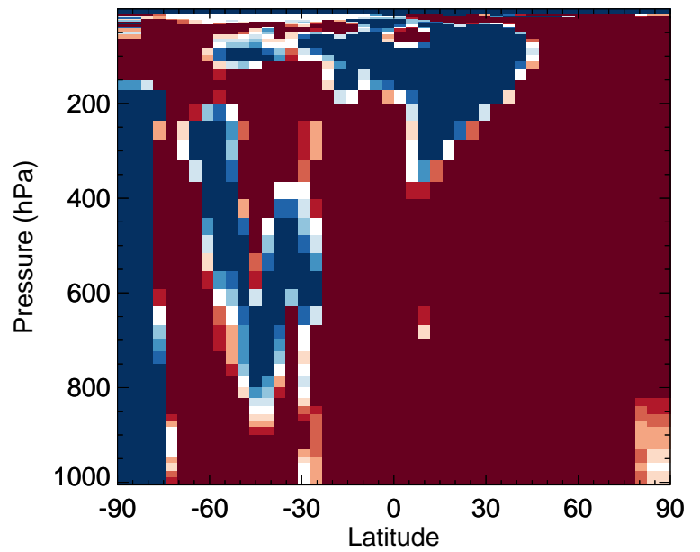
v11-02f-Run1 / v11-02e-Run0 GLYC - Zonal mean % diff for Jan
