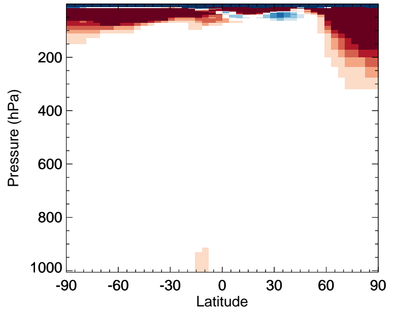
v11-02f-Run1 / v11-02e-Run0 CH2Br2 - Zonal mean % diff for Jan
