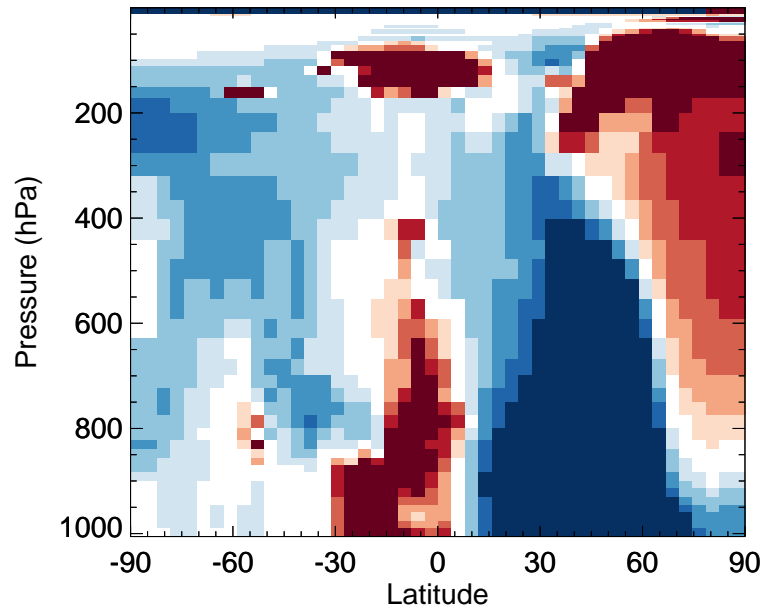
v11-02f-Run1 / v11-02e-Run1 Cl2 - Zonal mean % diff for Jan
