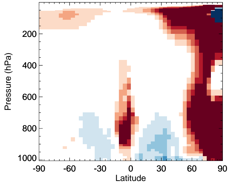
v11-02f-Run1 / v11-02e-Run1 BrO - Zonal mean % diff for Jan
