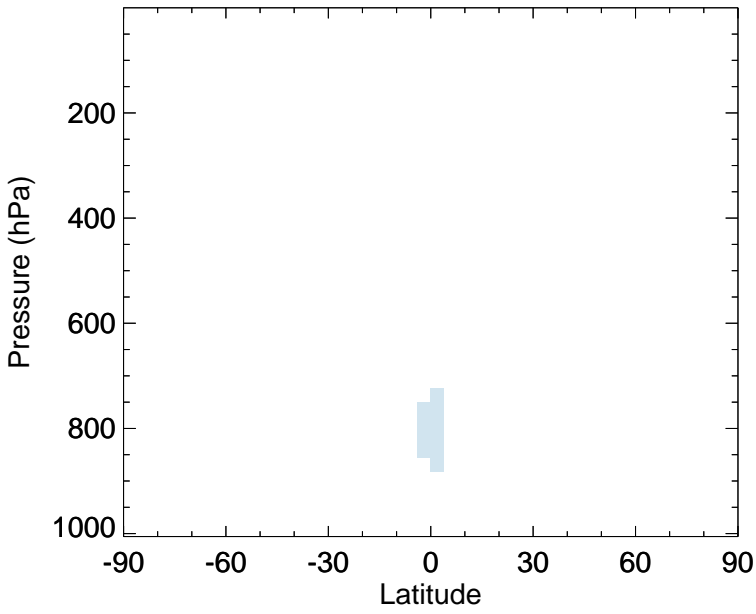
v11-02f-Run1 - v11-02e-Run1 IEPOXA - Zonal mean abs diff for Jan
