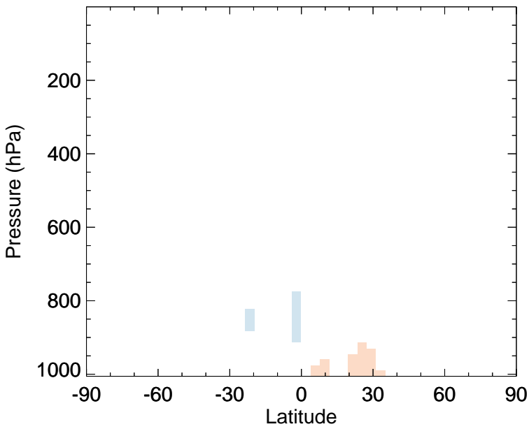
v11-02f-Run1 - v11-02e-Run1 ALD2 - Zonal mean abs diff for Jan
