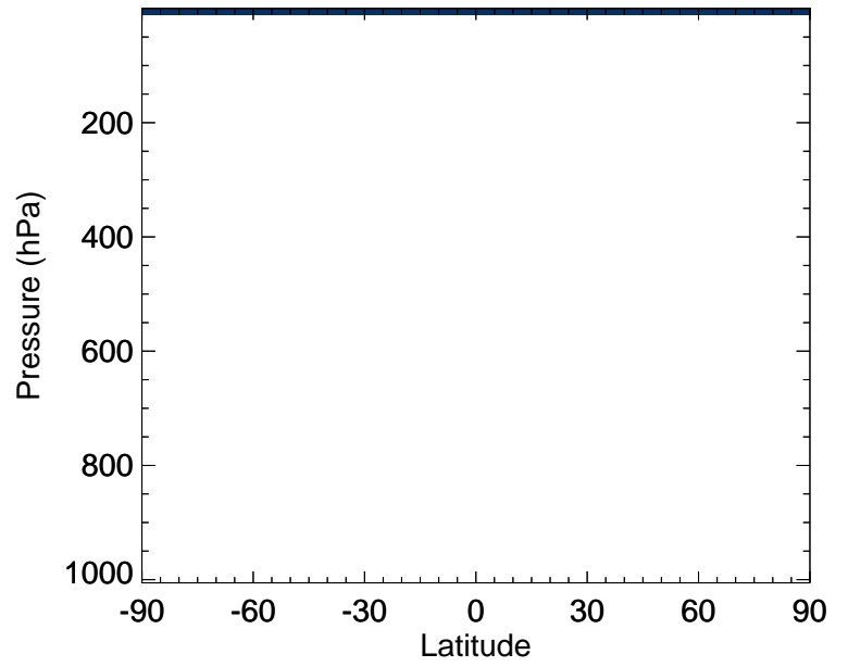
v11-02f-Run1 / v11-02e-Run1 CFC113 - Zonal mean % diff for Jan
