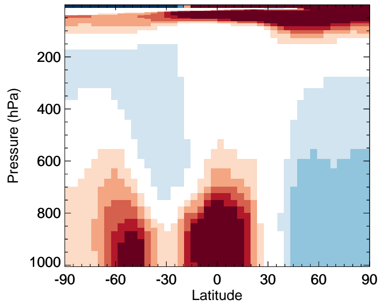
v11-02f-Run1 / v11-02e-Run1 PAN - Zonal mean % diff for Jan
