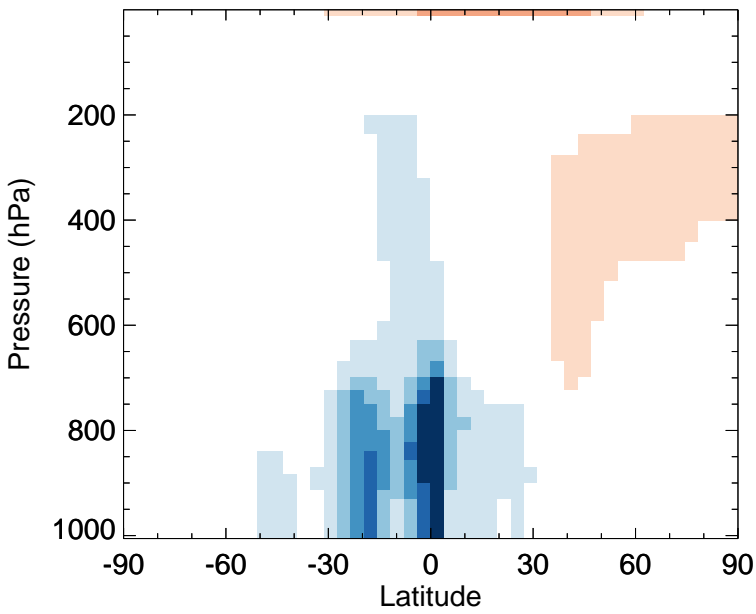
v11-02f-Run1 - v11-02e-Run1 MP - Zonal mean abs diff for Jan
