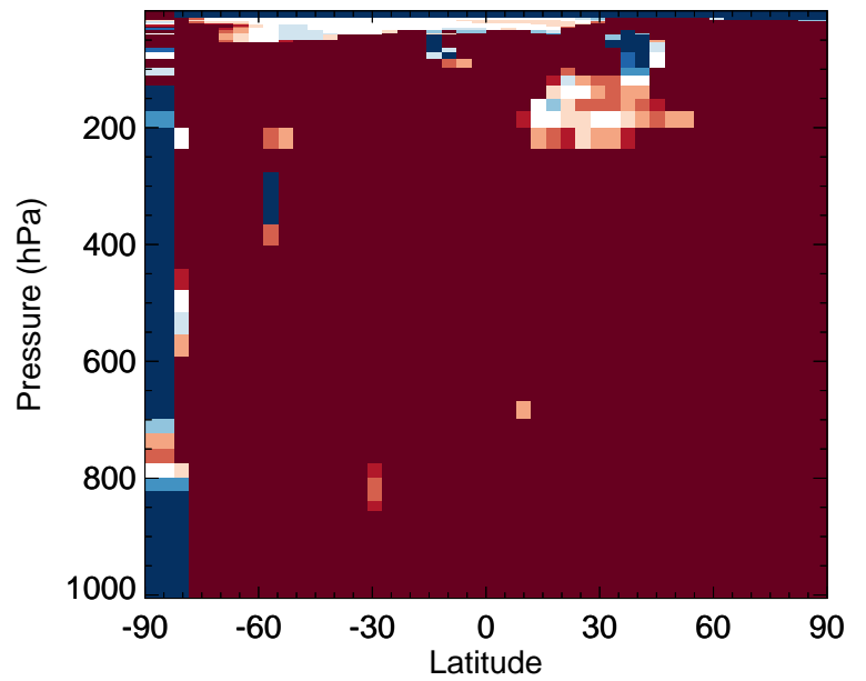
v11-02f-Run1 / v11-02e-Run0 MACR - Zonal mean % diff for Jan
