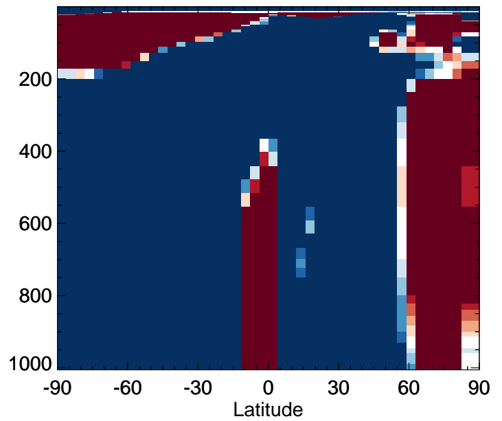
v11-02f-Run1 / v11-02e-Run0 DST3 - Zonal mean % diff for Jan
