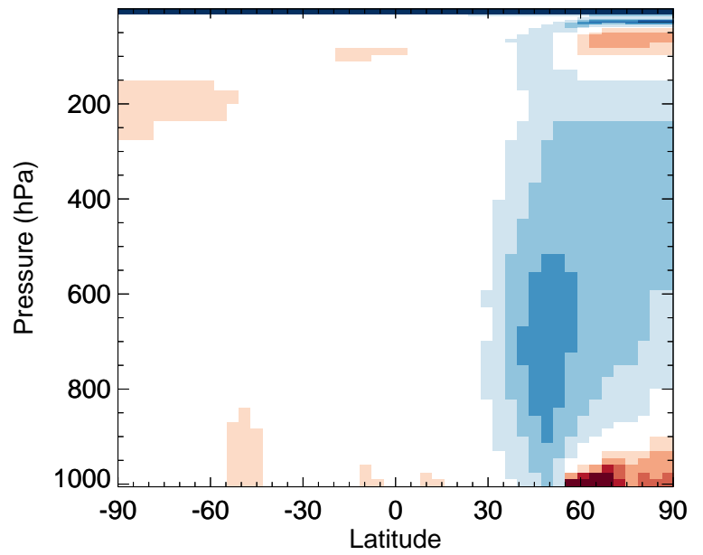
v11-02f-Run1 / v11-02e-Run1 CH 2 O - Zonal mean % diff for Jan
