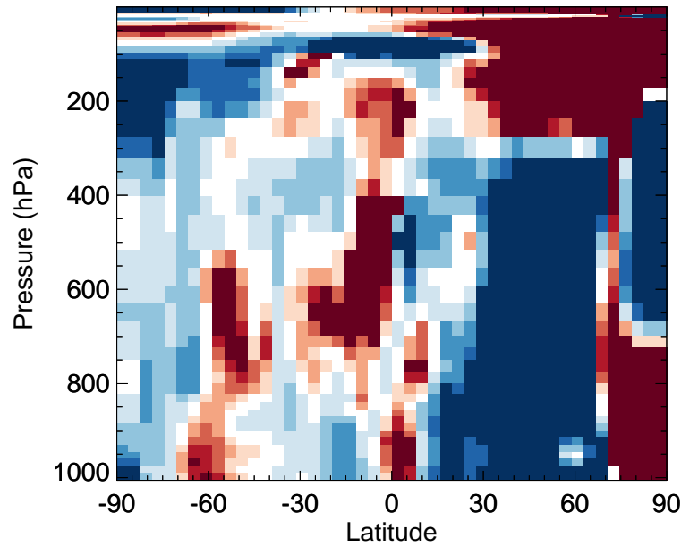
v11-02f-Run1 / v11-02e-Run0 ClO - Zonal mean % diff for Jan
