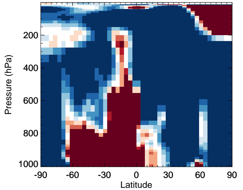
v11-02f-Run1 / v11-02e-Run0 ASOA2 - Zonal mean % diff for Jan
