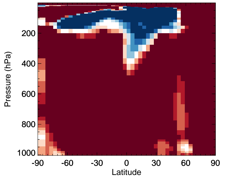
v11-02f-Run1 / v11-02e-Run0 R4N2 - Zonal mean % diff for Jan
