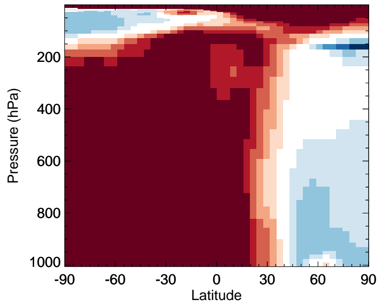
v11-02f-Run1 / v11-02e-Run1 R4N2 - Zonal mean % diff for Jan
