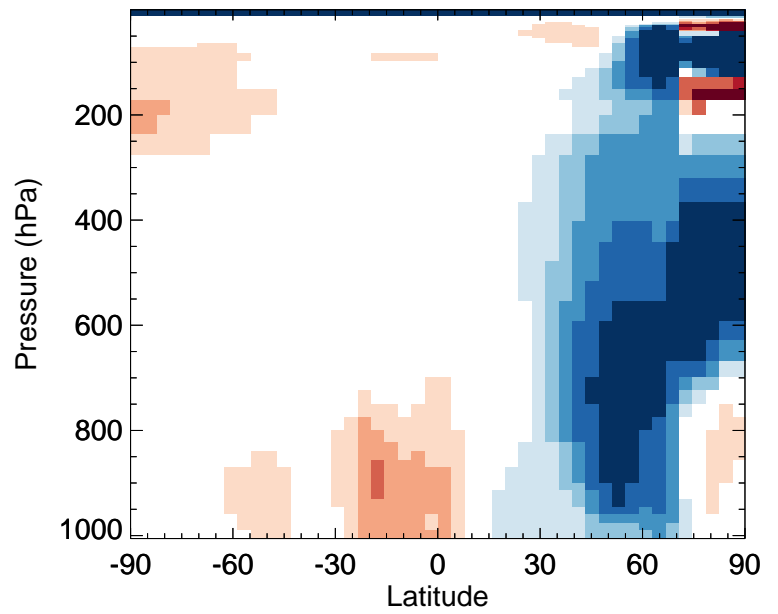
v11-02f-Run1 / v11-02e-Run1 OH - Zonal mean % diff for Jan
