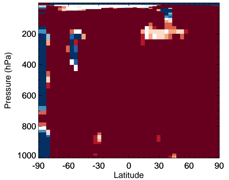
v11-02f-Run1 / v11-02e-Run0 PRPE - Zonal mean % diff for Jan
