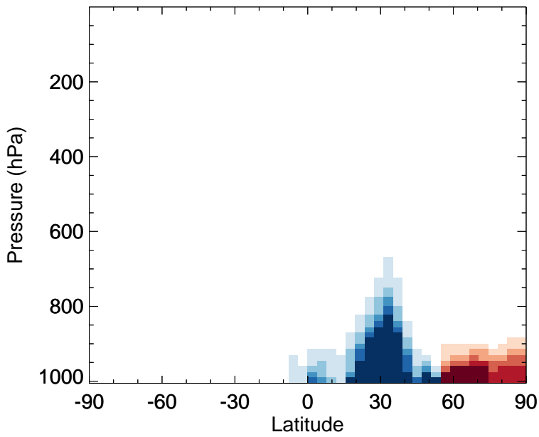
v11-02f-Run1 - v11-02e-Run1 XYLE - Zonal mean abs diff for Jan
