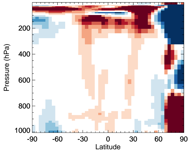
v11-02f-Run1 / v11-02e-Run0 HO2 - Zonal mean % diff for Jan
