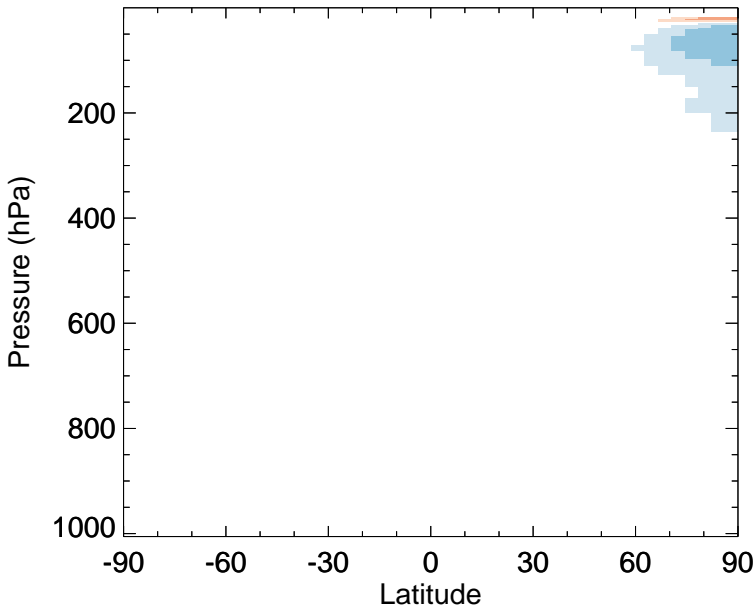
v11-02f-Run1 - v11-02e-Run0 HOBr - Zonal mean abs diff for Jan
