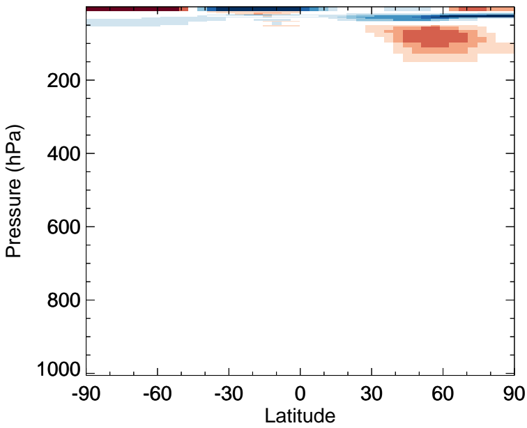
v11-02f-Run1 - v11-02e-Run1 HCl - Zonal mean abs diff for Jan
