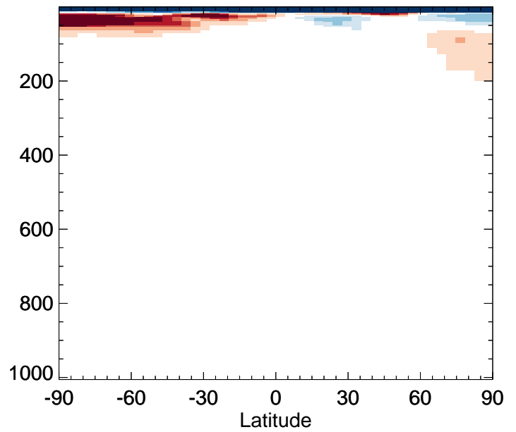
v11-02f-Run1 / v11-02e-Run0 CH3Cl - Zonal mean % diff for Jan
