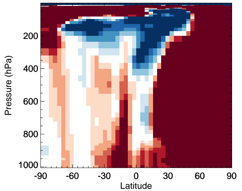
v11-02f-Run1 / v11-02e-Run0 C3H8 - Zonal mean % diff for Jan
