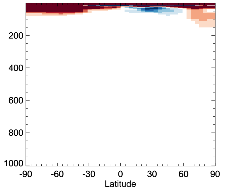
v11-02f-Run1 / v11-02e-Run0 CFC11 - Zonal mean % diff for Jan
