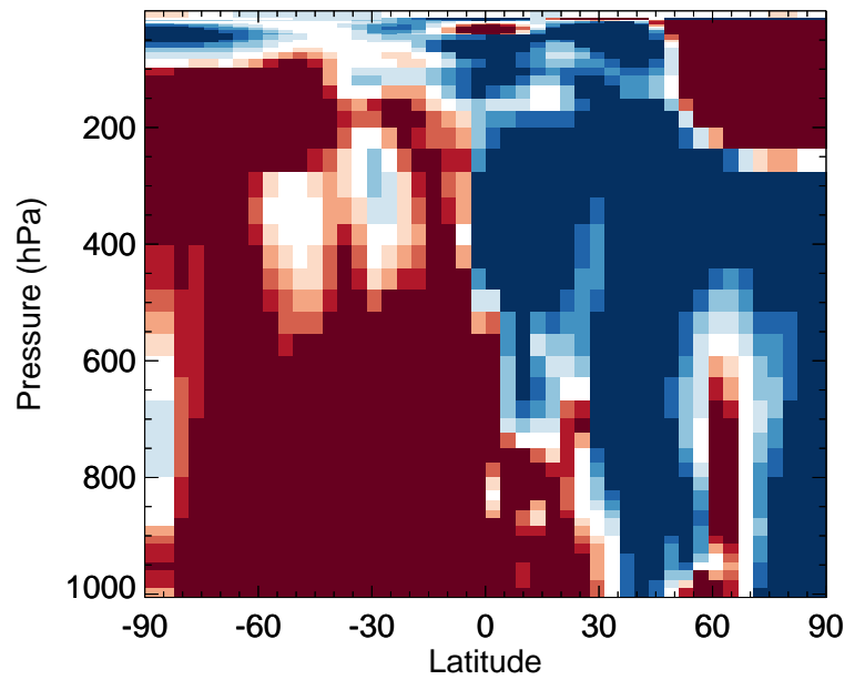
v11-02f-Run1 / v11-02e-Run0 ASOA3 - Zonal mean % diff for Jan
