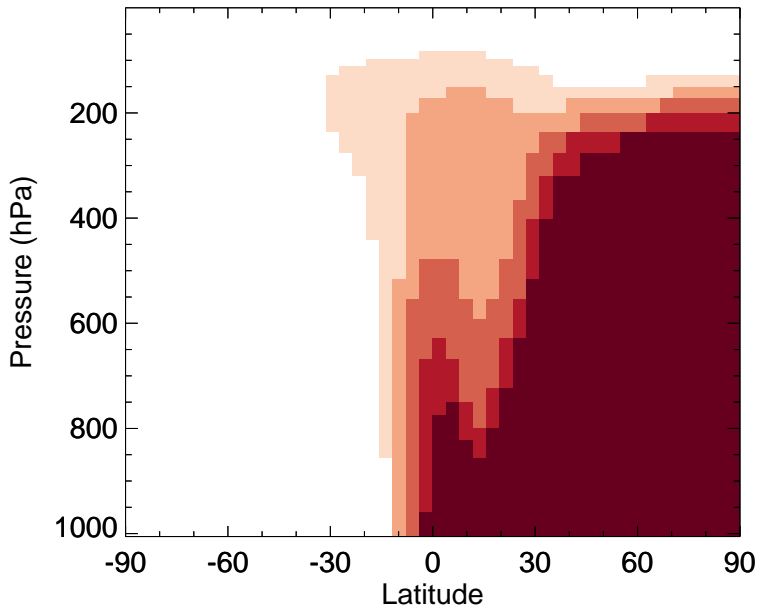
v11-02f-Run1 - v11-02e-Run1 C2H6 - Zonal mean abs diff for Jan
