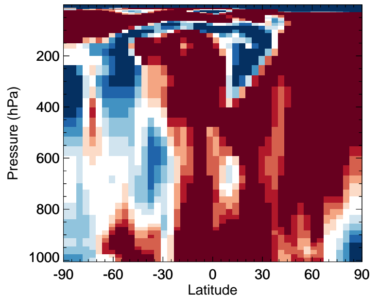
v11-02f-Run1 / v11-02e-Run0 HAC - Zonal mean % diff for Jan
