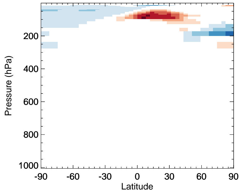
v11-02f-Run1 / v11-02e-Run1 SALC - Zonal mean % diff for Jan
