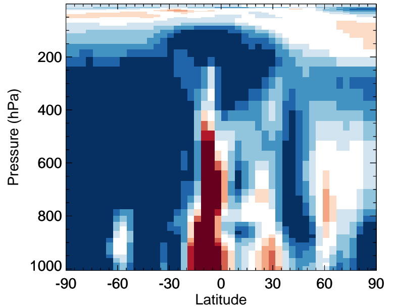
v11-02f-Run1 / v11-02e-Run0 SOAS - Zonal mean % diff for Jan
