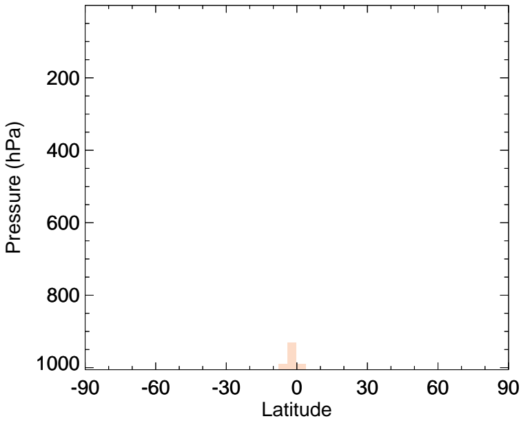
v11-02f-Run1 - v11-02e-Run0 TSOA2 - Zonal mean abs diff for Jan
