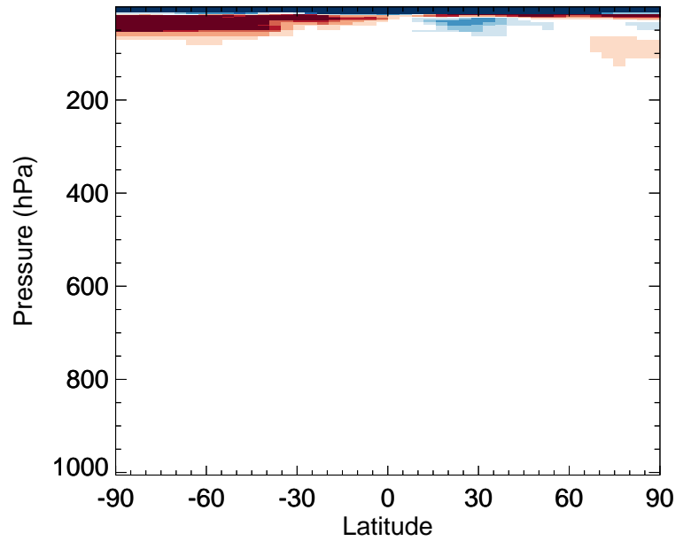
v11-02f-Run1 / v11-02e-Run0 CFC113 - Zonal mean % diff for Jan
