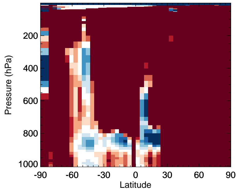
v11-02f-Run1 / v11-02e-Run0 DMS - Zonal mean % diff for Jan
