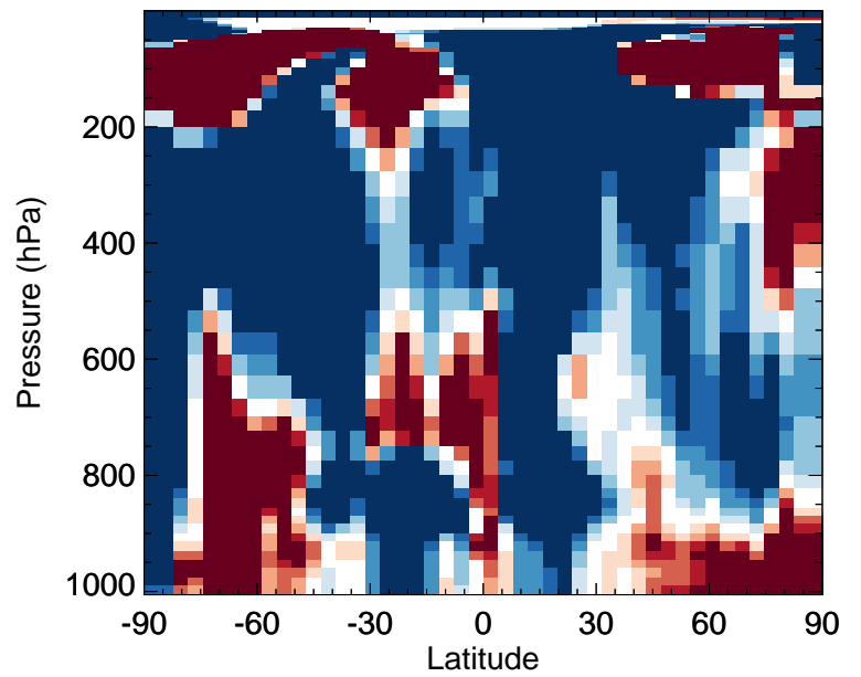
v11-02f-Run1 / v11-02e-Run0 NITs - Zonal mean % diff for Jan
