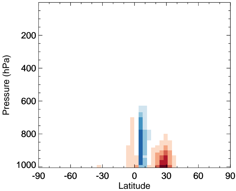
v11-02f-Run1 - v11-02e-Run0 OCPI - Zonal mean abs diff for Jan
