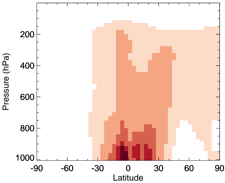
v11-02f-Run1 - v11-02e-Run1 ACET - Zonal mean abs diff for Jan
