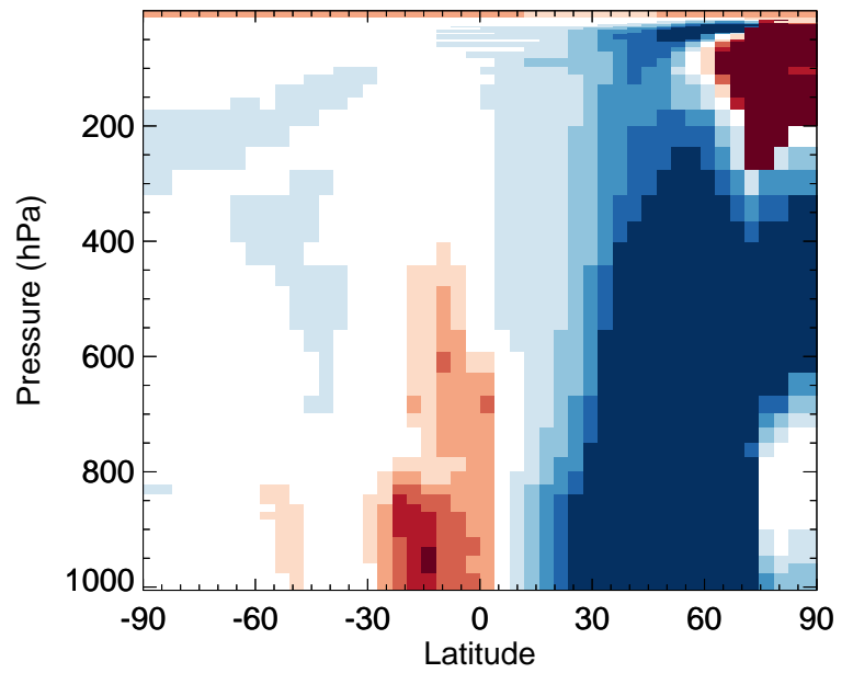
v11-02f-Run1 / v11-02e-Run1 ClOO - Zonal mean % diff for Jan
