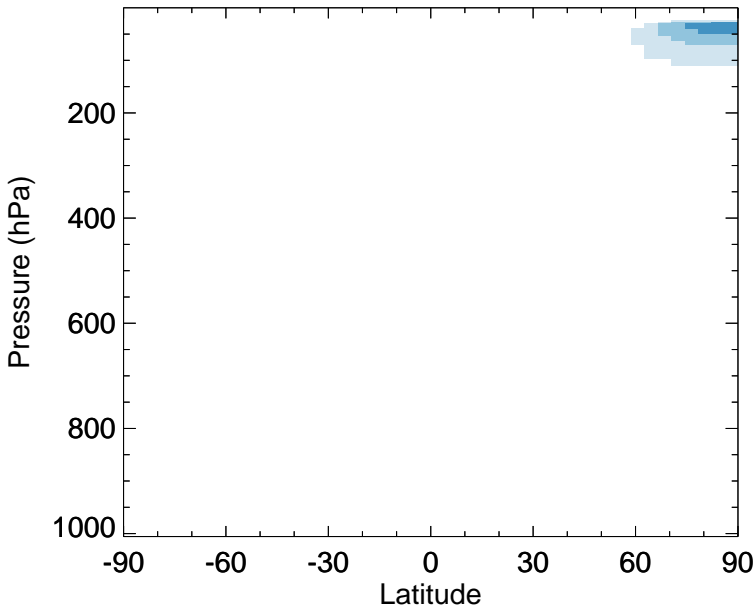
v11-02f-Run1 - v11-02e-Run1 HOBr - Zonal mean abs diff for Jan
