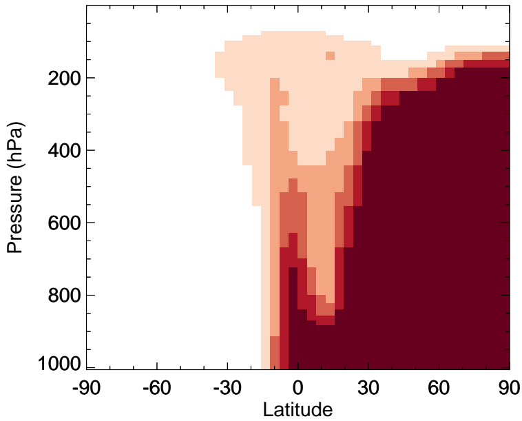
v11-02f-Run1 - v11-02e-Run0 C2H6 - Zonal mean abs diff for Jan
