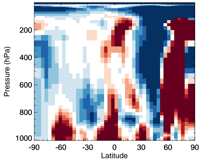
v11-02f-Run1 / v11-02e-Run0 HNO 2 - Zonal mean % diff for Jan
