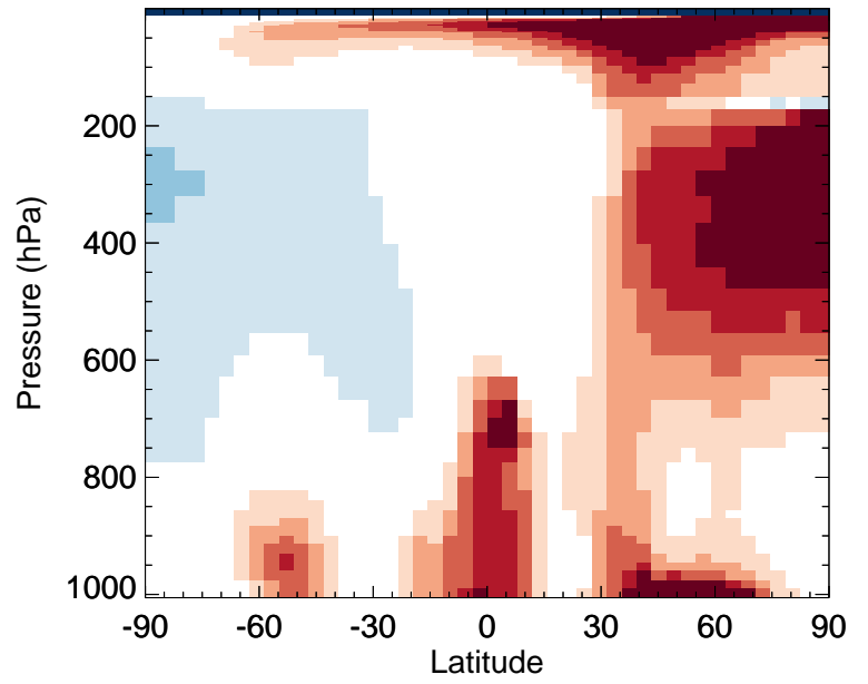
v11-02f-Run1 / v11-02e-Run1 HNO 3 - Zonal mean % diff for Jan
