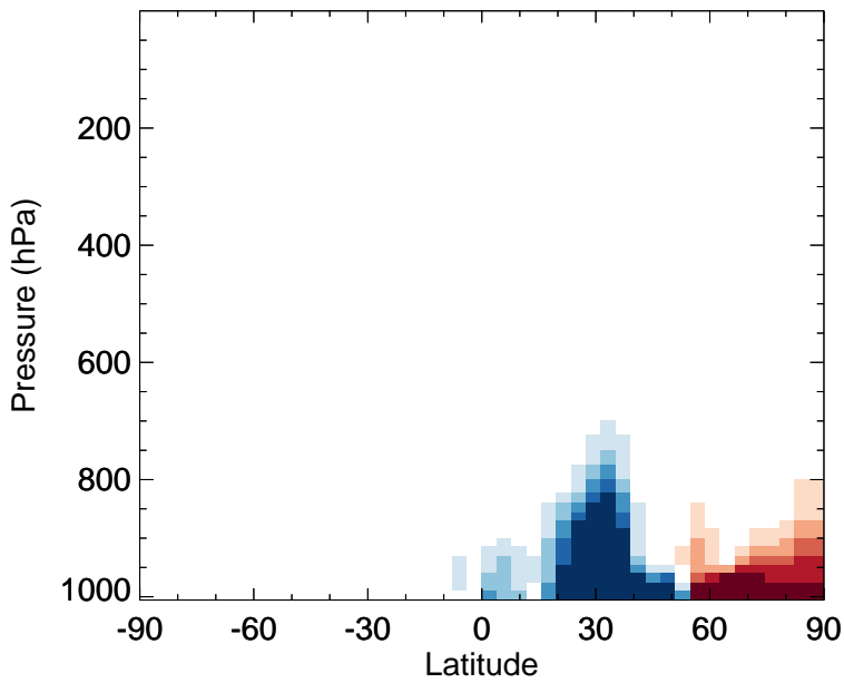
v11-02f-Run1 - v11-02e-Run0 XYLE - Zonal mean abs diff for Jan
