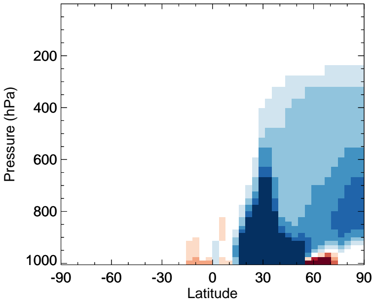
v11-02f-Run1 - v11-02e-Run1 TOLU - Zonal mean abs diff for Jan
