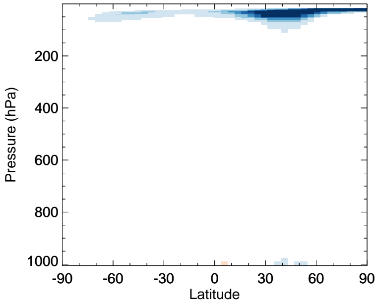
v11-02f-Run1 - v11-02e-Run1 NO 2 - Zonal mean abs diff for Jan
