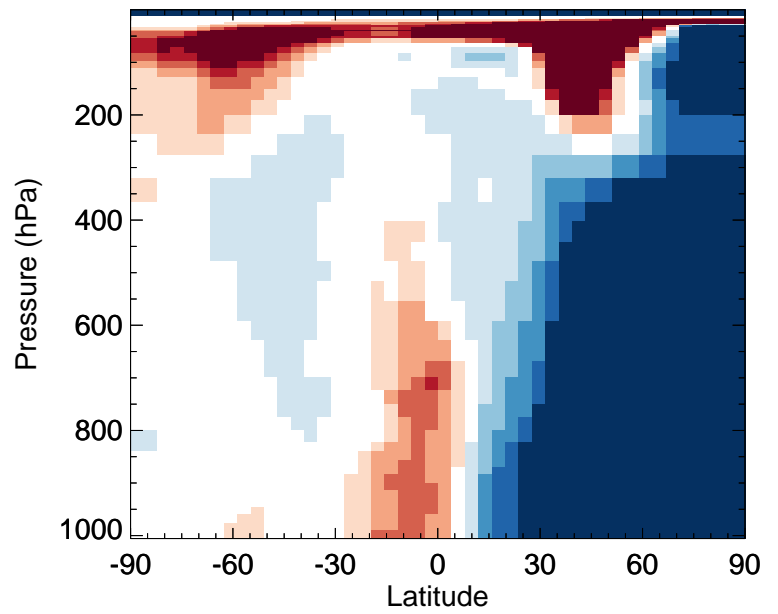
v11-02f-Run1 / v11-02e-Run1 HOCl - Zonal mean % diff for Jan
