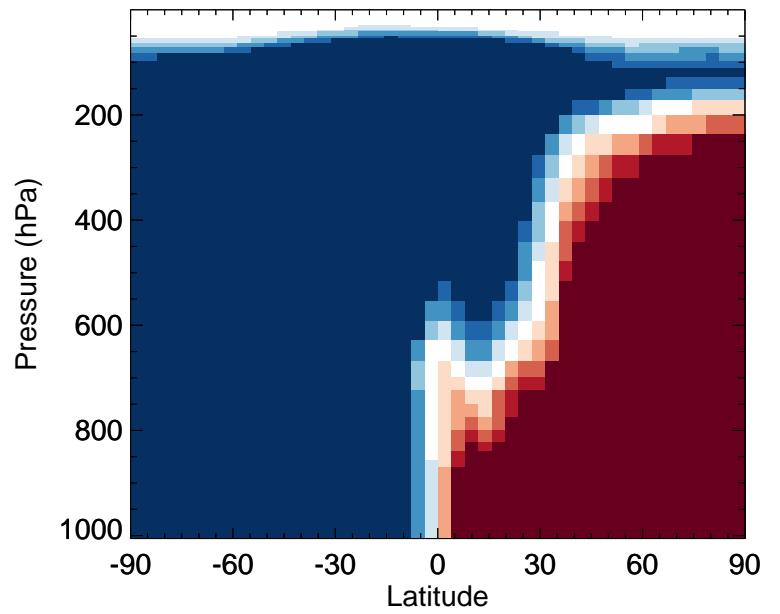
v11-02f-Run1 / v11-02e-Run1 SOAME - Zonal mean % diff for Jan
