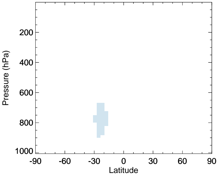
v11-02f-Run1 - v11-02e-Run0 IEPOXA - Zonal mean abs diff for Jan
