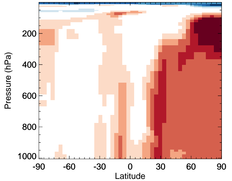
v11-02f-Run1 / v11-02e-Run0 CO - Zonal mean % diff for Jan
