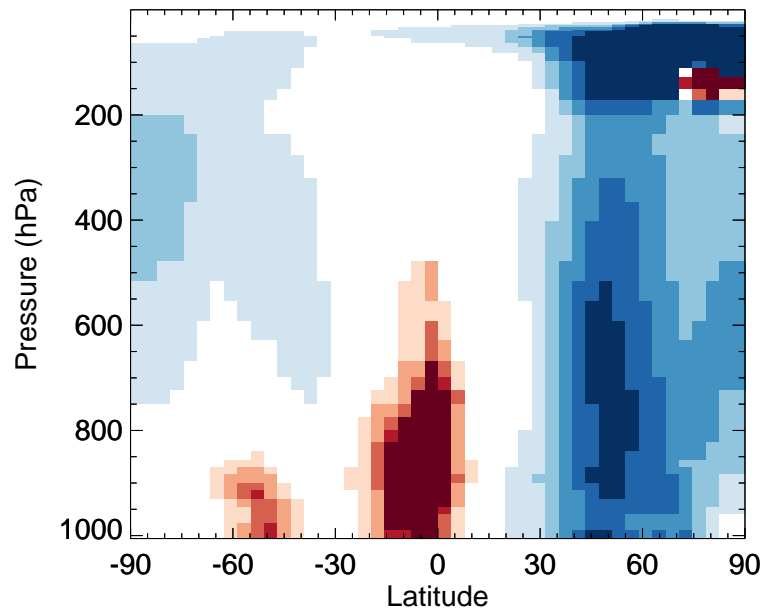
v11-02f-Run1 / v11-02e-Run1 BrNO3 - Zonal mean % diff for Jan
