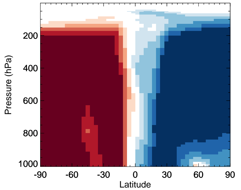
v11-02f-Run1 / v11-02e-Run1 ASOAN - Zonal mean % diff for Jan
