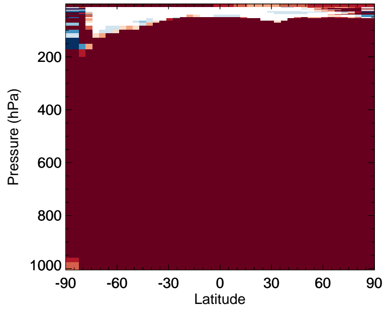
v11-02f-Run1 / v11-02e-Run1 MTPA - Zonal mean % diff for Jan
