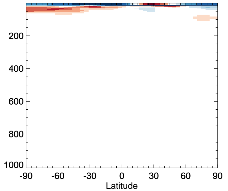
v11-02f-Run1 / v11-02e-Run0 N2O - Zonal mean % diff for Jan
