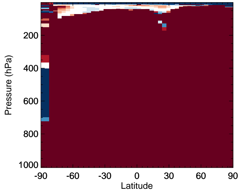
v11-02f-Run1 / v11-02e-Run0 RIPB - Zonal mean % diff for Jan
