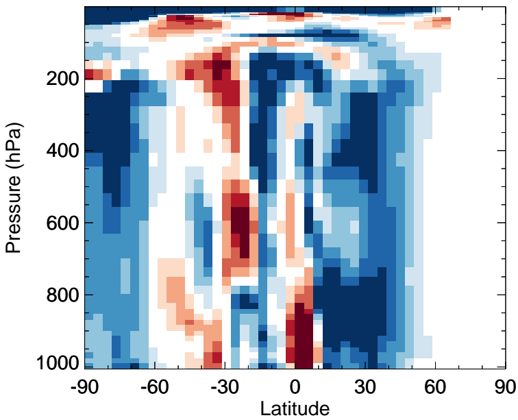
v11-02f-Run1 - v11-02e-Run0 OH - Zonal mean abs diff for Jan
