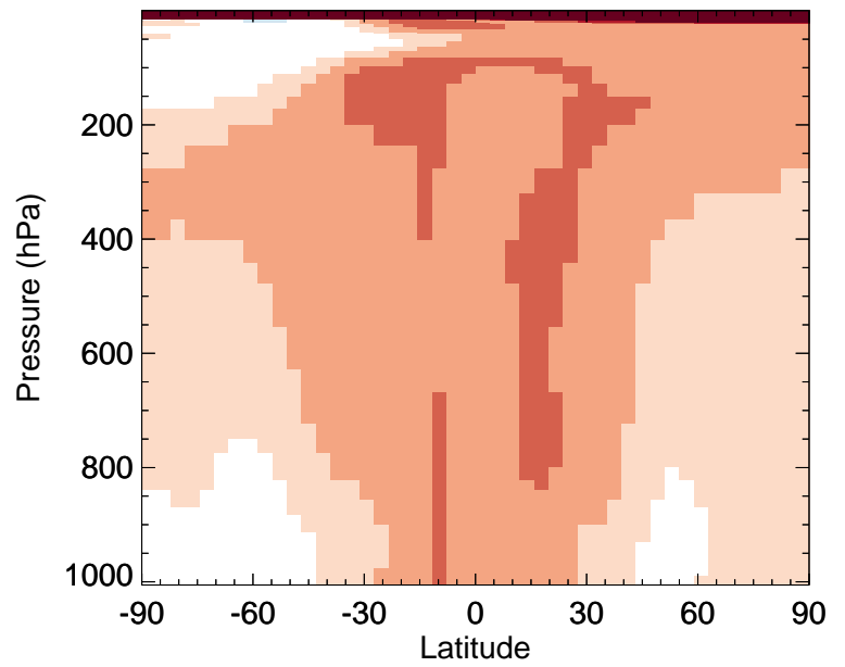
v11-02f-Run1 / v11-02e-Run1 ACET - Zonal mean % diff for Jan
