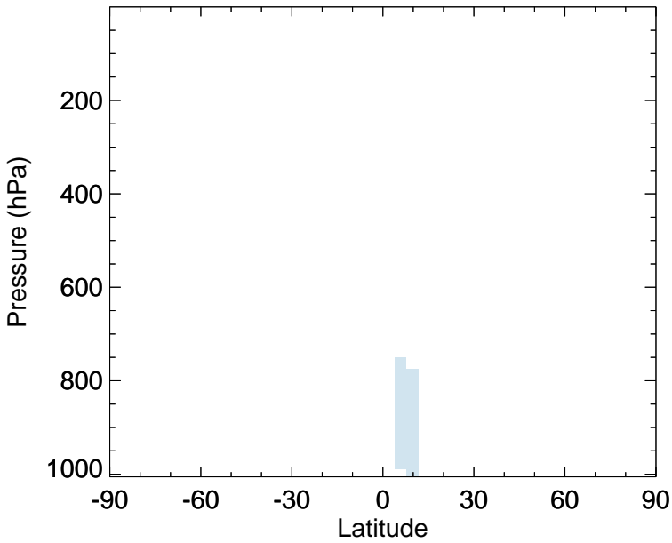
v11-02f-Run1 - v11-02e-Run0 NH3 - Zonal mean abs diff for Jan
