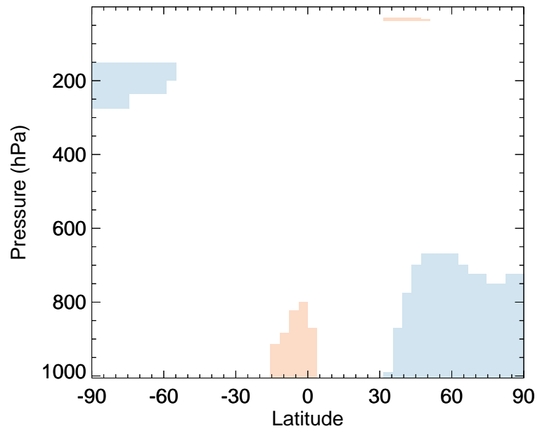
v11-02f-Run1 / v11-02e-Run1 O3 - Zonal mean % diff for Jan
