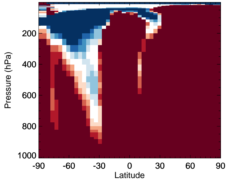
v11-02f-Run1 / v11-02e-Run1 MVK - Zonal mean % diff for Jan
