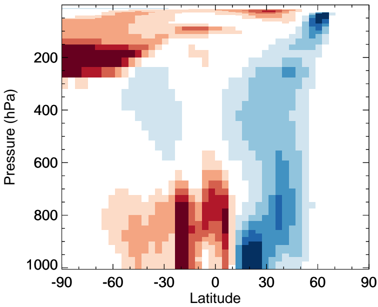
v11-02f-Run1 - v11-02e-Run1 OH - Zonal mean abs diff for Jan
