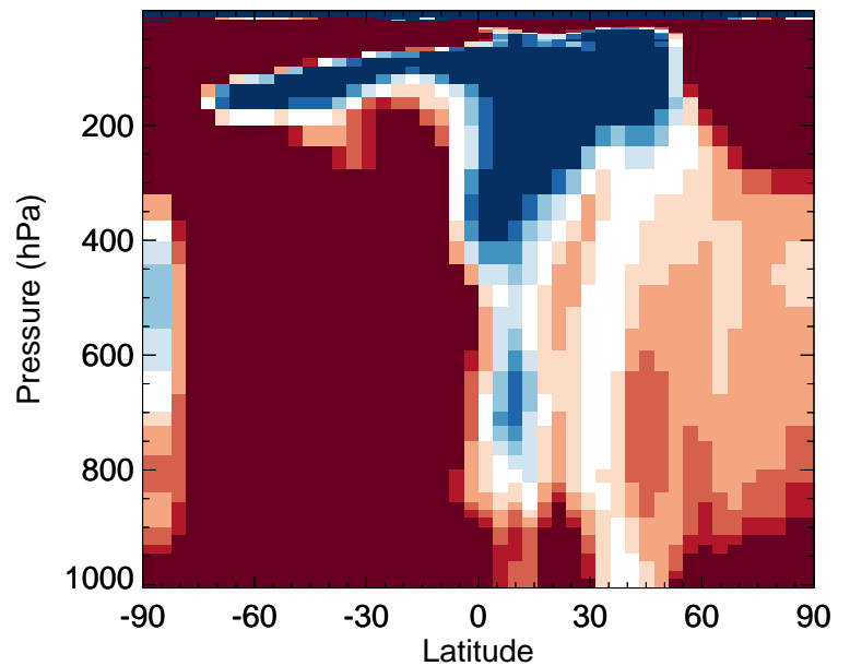
v11-02f-Run1 / v11-02e-Run0 BENZ - Zonal mean % diff for Jan
