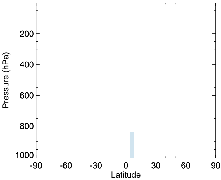
v11-02f-Run1 - v11-02e-Run1 IONITA - Zonal mean abs diff for Jan
