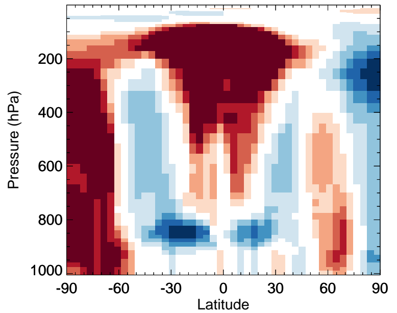
v11-02f-Run1 / v11-02e-Run0 MSA - Zonal mean % diff for Jan
