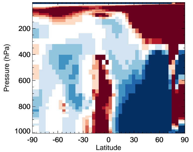
v11-02f-Run1 / v11-02e-Run1 Cl2O2 - Zonal mean % diff for Jan
