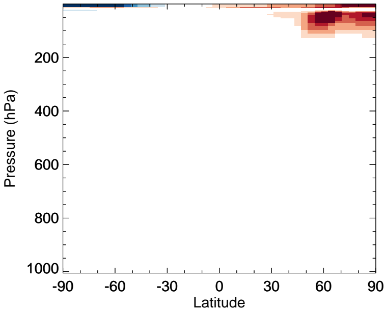
v11-02f-Run1 - v11-02e-Run0 ClO - Zonal mean abs diff for Jan
