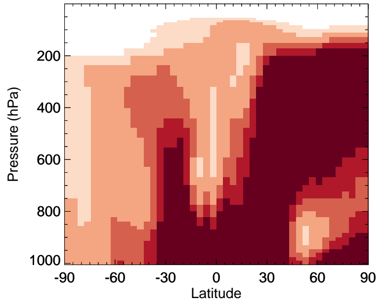
v11-02f-Run1 / v11-02e-Run1 OCPI - Zonal mean % diff for Jan
