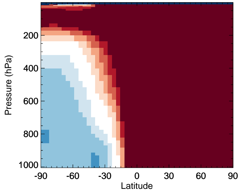
v11-02f-Run1 / v11-02e-Run1 C2H6 - Zonal mean % diff for Jan
