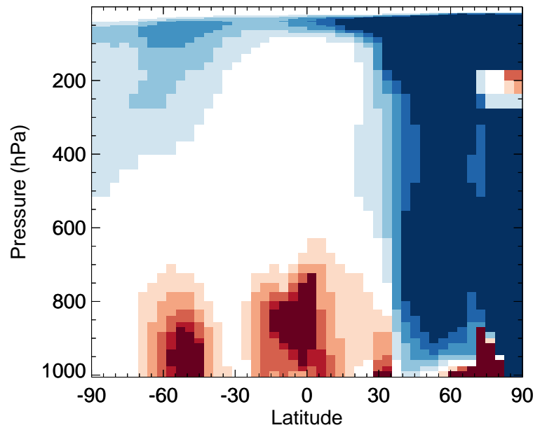
v11-02f-Run1 / v11-02e-Run1 NO - Zonal mean % diff for Jan
