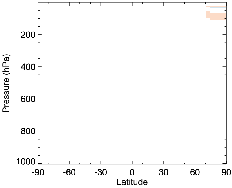
v11-02f-Run1 - v11-02e-Run1 Cl2 - Zonal mean abs diff for Jan
