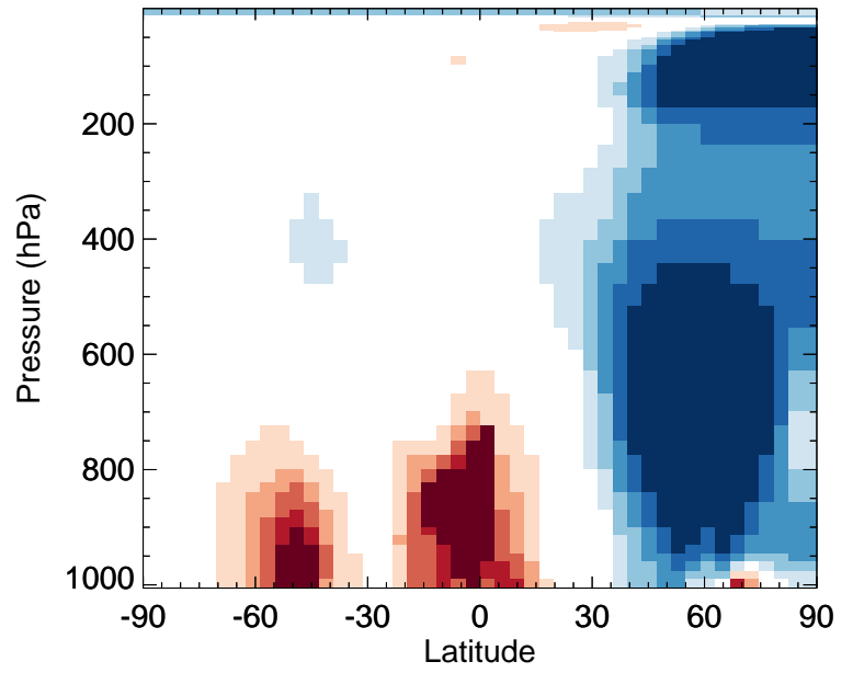
v11-02f-Run1 / v11-02e-Run1 MPN - Zonal mean % diff for Jan
