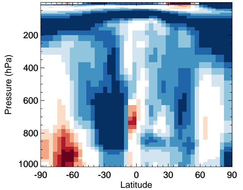
v11-02f-Run1 / v11-02e-Run0 SO4 - Zonal mean % diff for Jan
