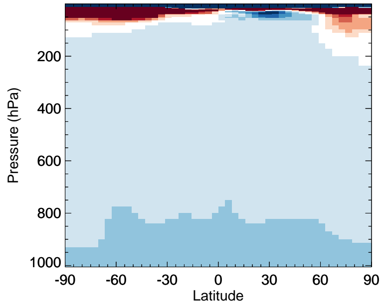
v11-02f-Run1 / v11-02e-Run0 CCI4 - Zonal mean % diff for Jan
