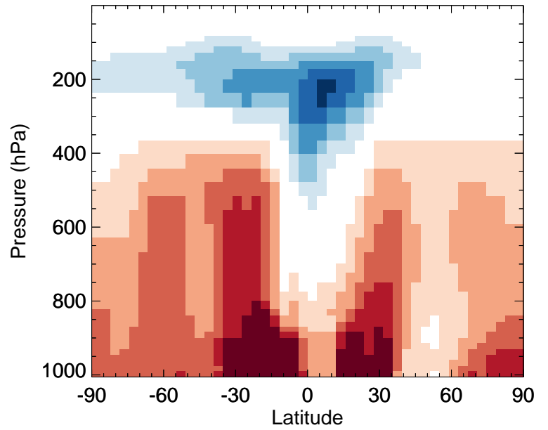
v11-02f-Run1 / v11-02e-Run1 ISOA2 - Zonal mean % diff for Jan
