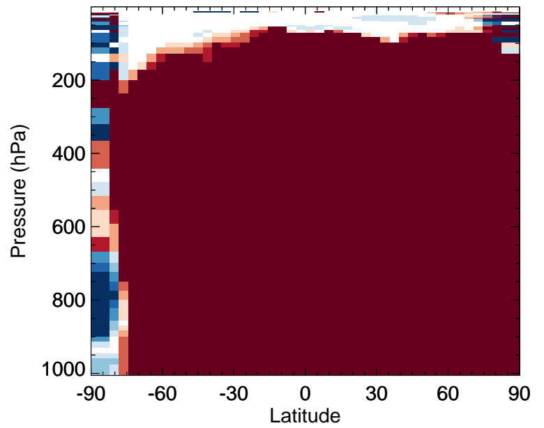
v11-02f-Run1 / v11-02e-Run1 LIMO - Zonal mean % diff for Jan
