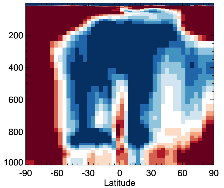
v11-02f-Run1 / v11-02e-Run0 SALA - Zonal mean % diff for Jan
