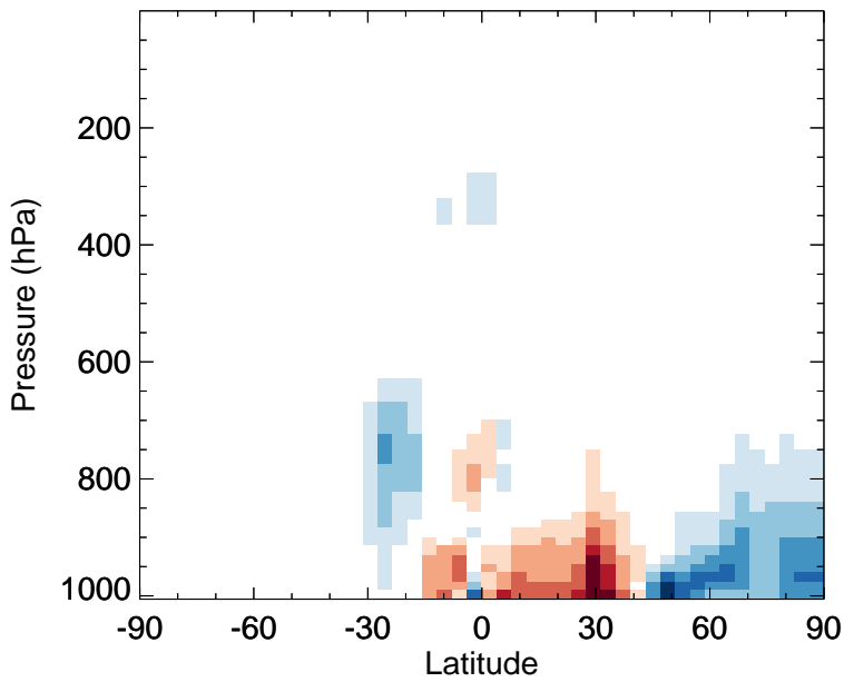
v11-02f-Run1 - v11-02e-Run0 EOH - Zonal mean abs diff for Jan
