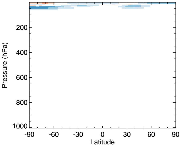
v11-02f-Run1 - v11-02e-Run0 NO - Zonal mean abs diff for Jan
