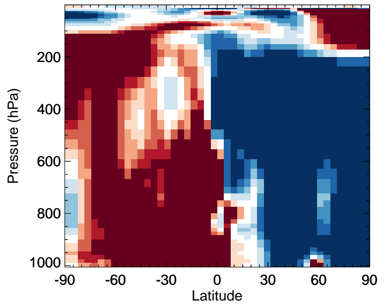
v11-02f-Run1 / v11-02e-Run0 ASOA1 - Zonal mean % diff for Jan
