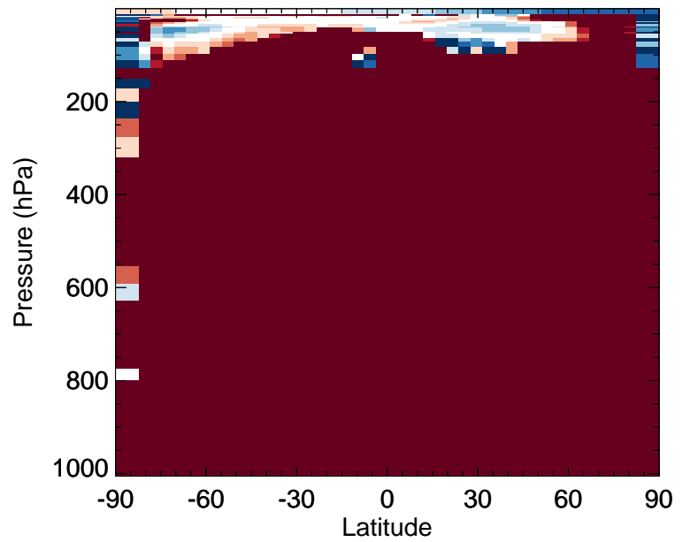
v11-02f-Run1 / v11-02e-Run0 LIMO - Zonal mean % diff for Jan
