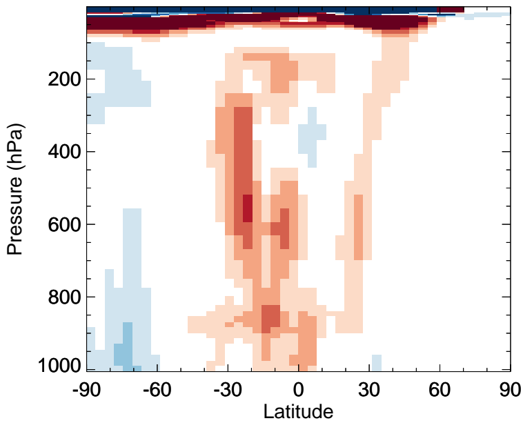
v11-02f-Run1 - v11-02e-Run0 HO2 - Zonal mean abs diff for Jan
