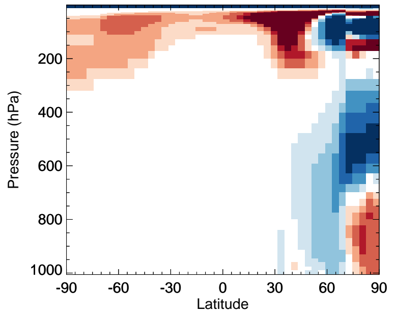
v11-02f-Run1 / v11-02e-Run1 HO2 - Zonal mean % diff for Jan
