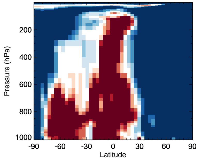
v11-02f-Run1 / v11-02e-Run0 N2O5 - Zonal mean % diff for Jan
