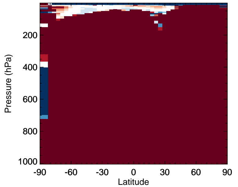
v11-02f-Run1 / v11-02e-Run0 RIPD - Zonal mean % diff for Jan
