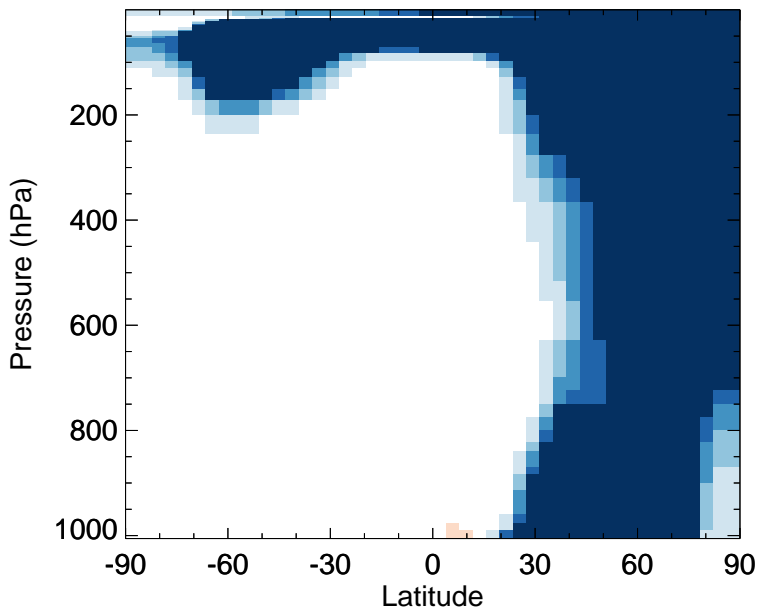
v11-02f-Run1 - v11-02e-Run1 N2O5 - Zonal mean abs diff for Jan
