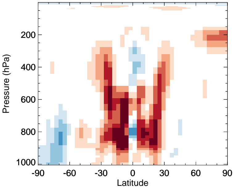
v11-02f-Run1 - v11-02e-Run0 H2O2 - Zonal mean abs diff for Jan
