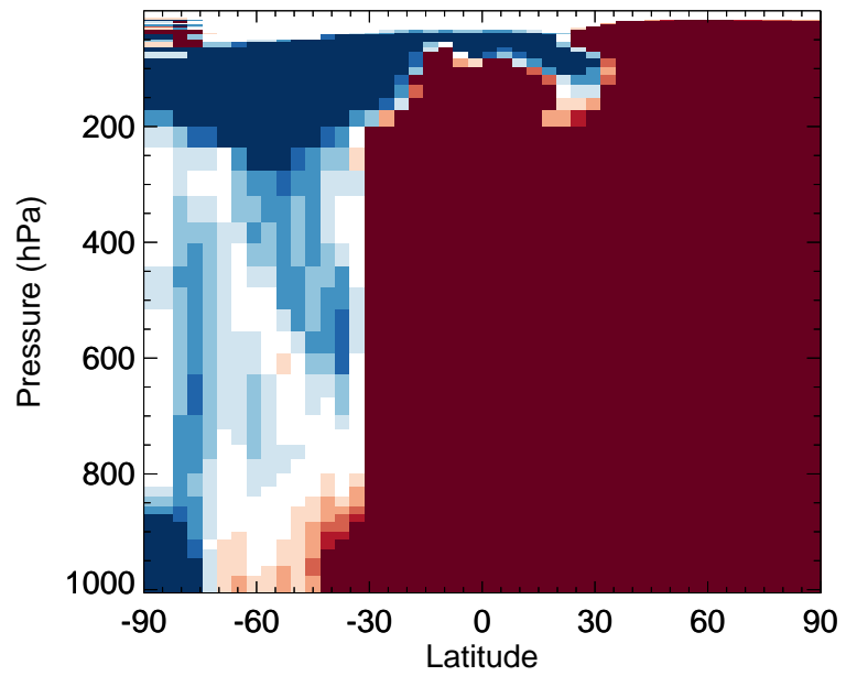
v11-02f-Run1 / v11-02e-Run1 HPALD - Zonal mean % diff for Jan
