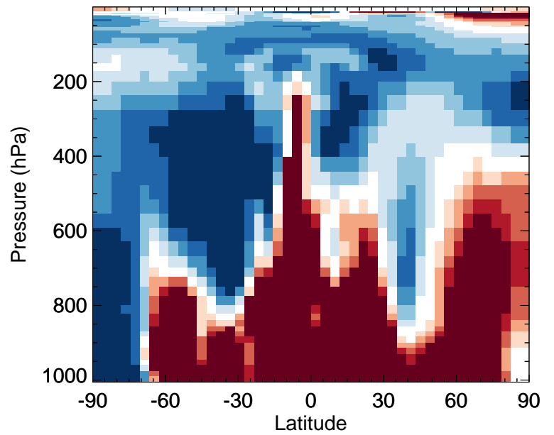
v11-02f-Run1 / v11-02e-Run0 TSOA0 - Zonal mean % diff for Jan
