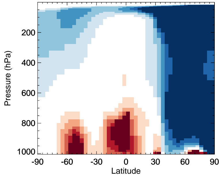
v11-02f-Run1 / v11-02e-Run1 NO 2 - Zonal mean % diff for Jan
