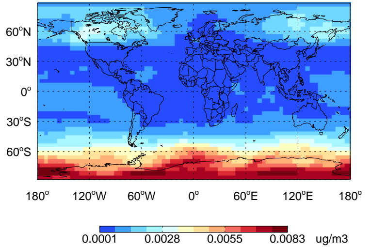
MSA - Species map @ 500 hPa for Oct
