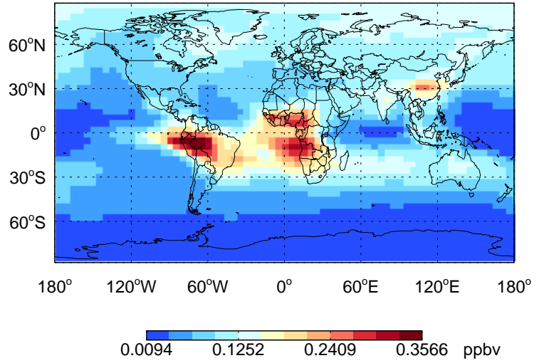
PAN - Species map @ 500 hPa for Oct
