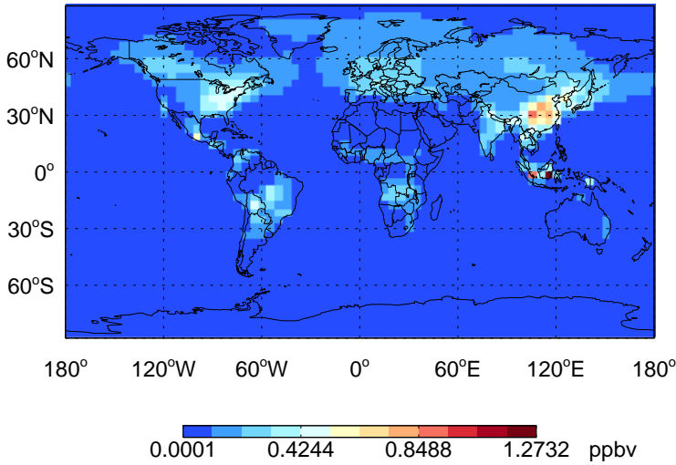
PAN - Species map @ surface for Oct
