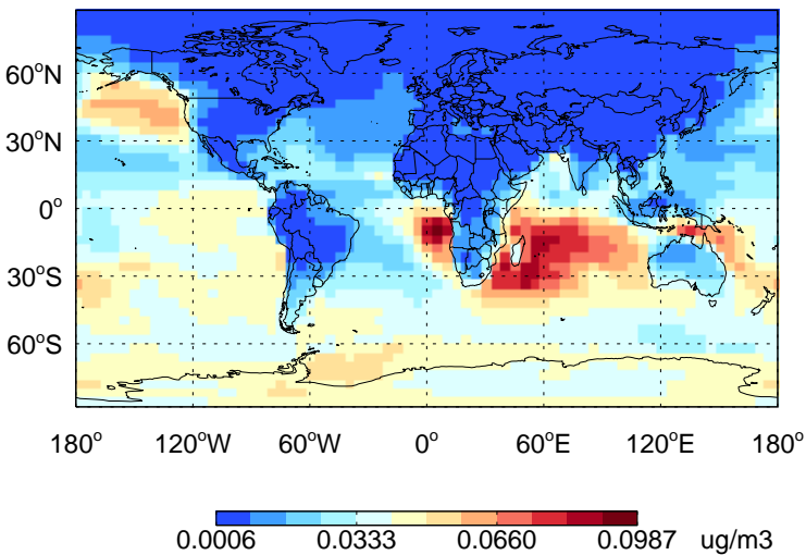
MSA - Species map @ surface for Oct
