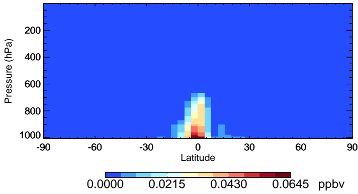
v11-02e-Run1 TSOA2 - Species Zonal Mean for Jan
