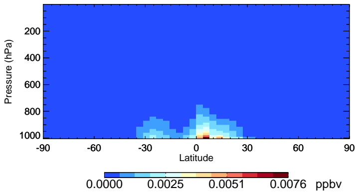
v11-02f-Run1 ISN1 - Species Zonal Mean for Jan
