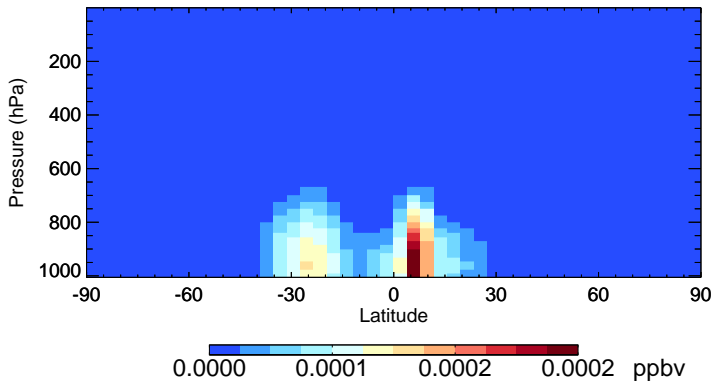
v11-02e-Run0 ETHLN - Species Zonal Mean for Jan
