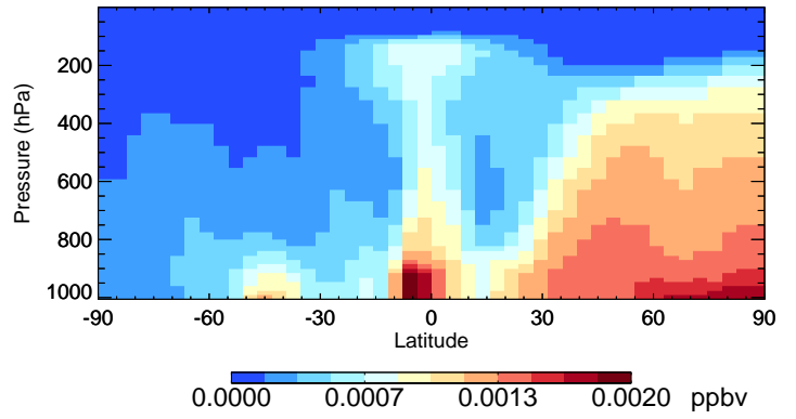
v11-02e-Run1 CHBr3 - Species Curtain @ -180.000 for Jan
