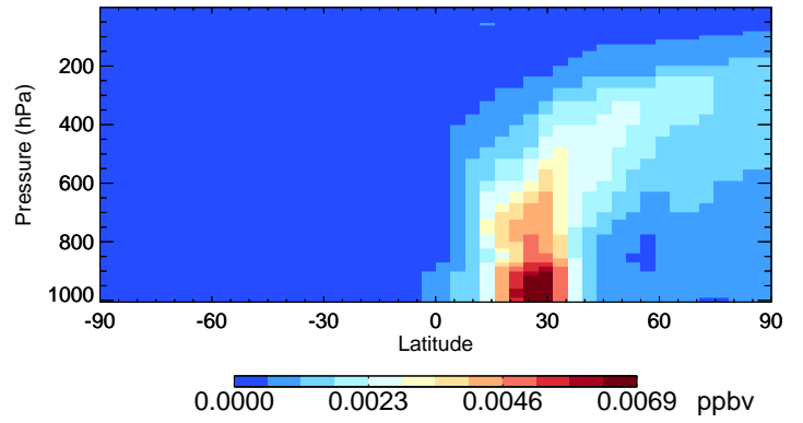
v11-02e-Run1 ASOAN - Species Curtain @ -180.000 for Jan
