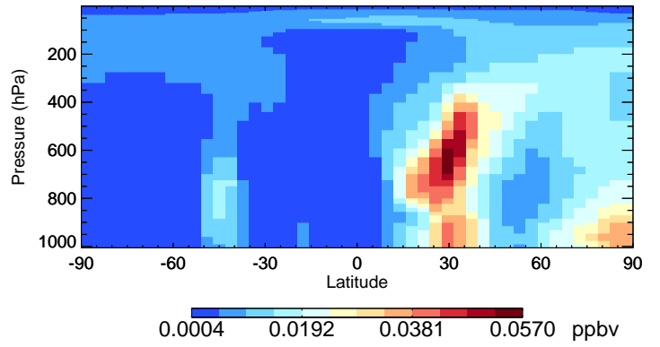
v11-02e-Run1 SOAS - Species Curtain @ -180.000 for Jan
