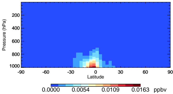
v11-02f-Run1 TSOA1 - Species Zonal Mean for Jan
