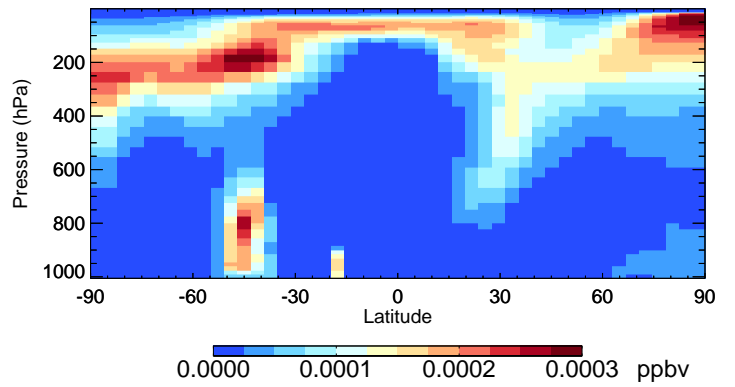
v11-02f-Run1 TSOA1 - Species Curtain @ -180.000 for Jan
