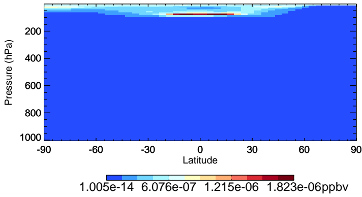
v11-02e-Run0 CIOO - Species Zonal Mean for Jan
