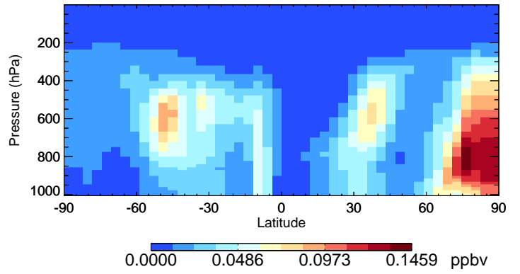
v11-02e-Run1 DST1 - Species Curtain @ -180.000 for Jan
