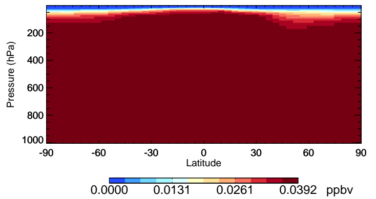
v11-02f-Run1 HCFC141b - Species Curtain @ -180.000 for Jan
