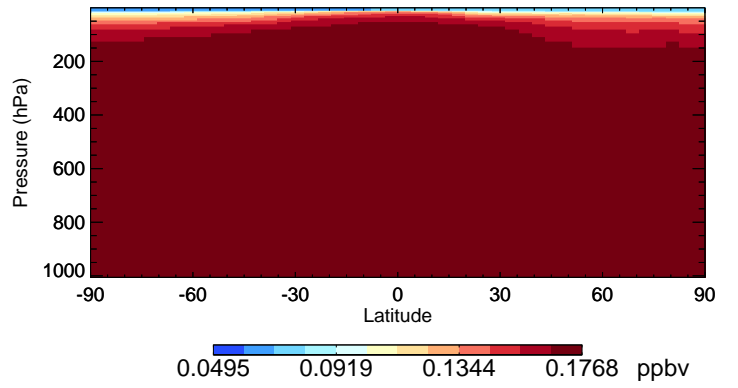
v11-02e-Run0 HCFC22 - Species Curtain @ -180.000 for Jan
