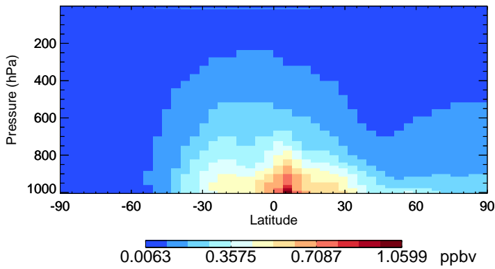
v11-02f-Run1 CH2O - Species Zonal Mean for Jan
