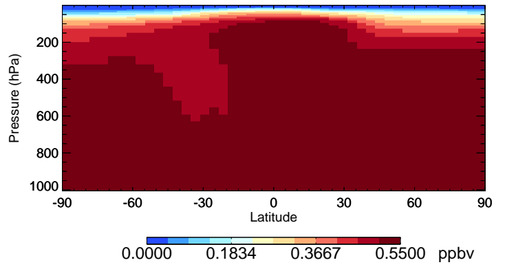
v11-02e-Run0 CH3Cl - Species Curtain @ -180.000 for Jan
