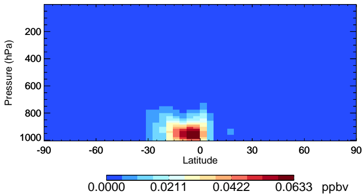
v11-02f-Run1 RIPA - Species Zonal Mean for Jan
