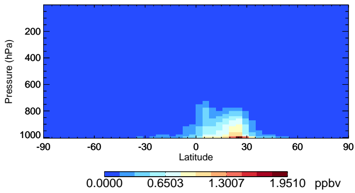
v11-02e-Run1 NH3 - Species Zonal Mean for Jan
