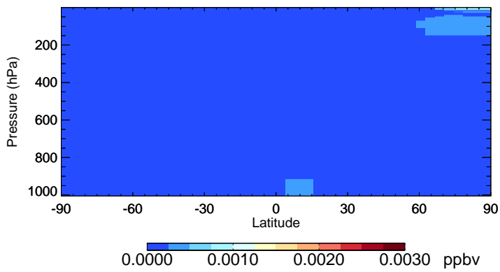
v11-02f-Run1 Br2 - Species Zonal Mean for Jan
