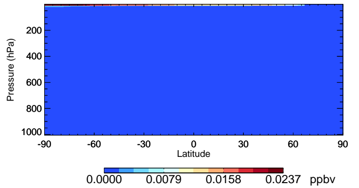
v11-02f-Run1 Br - Species Curtain @ -180.000 for Jan
