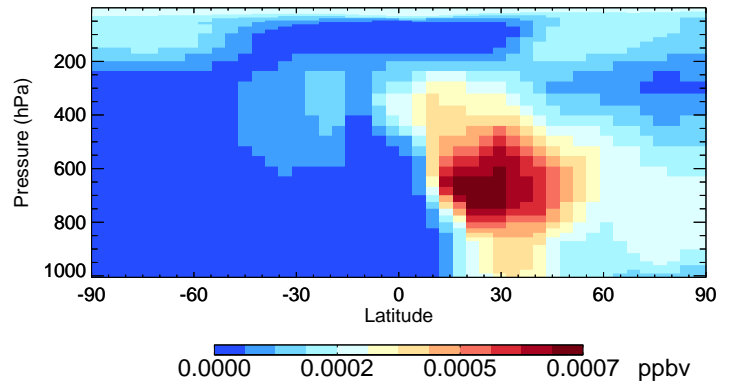
v11-02e-Run0 ASOG1 - Species Curtain @ -180.000 for Jan
