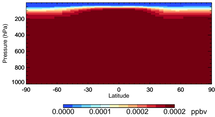
v11-02f-Run1 H2402 - Species Zonal Mean for Jan
