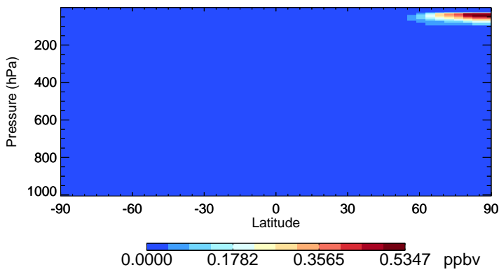
v11-02f-Run1 Cl2O2 - Species Zonal Mean for Jan
