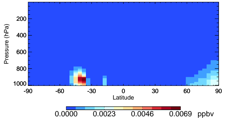
v11-02e-Run1 GLYC - Species Curtain @ -180.000 for Jan
