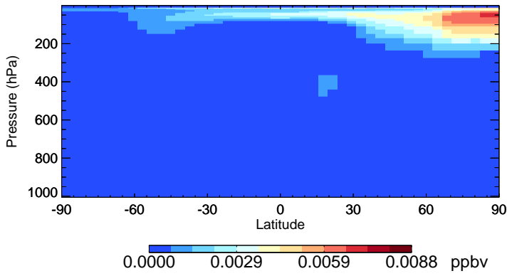
v11-02e-Run0 HOBr - Species Zonal Mean for Jan
