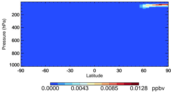
v11-02e-Run0 Cl2O2 - Species Zonal Mean for Jan
