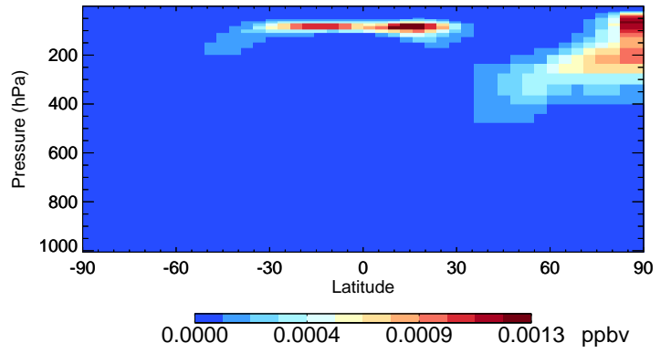
v11-02e-Run1 ASOA3 - Species Curtain @ -180.000 for Jan
