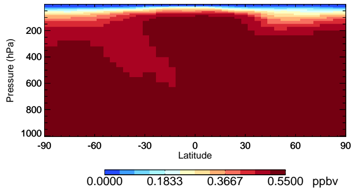
v11-02f-Run1 CH3Cl - Species Curtain @ -180.000 for Jan
