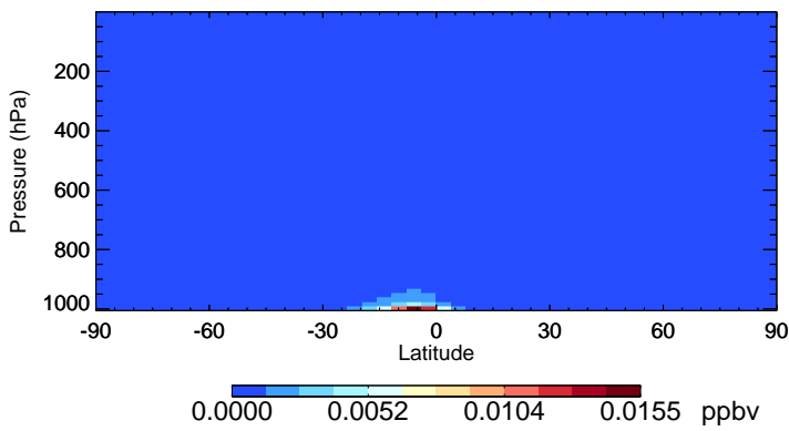
v11-02f-Run1 LIMO - Species Zonal Mean for Jan
