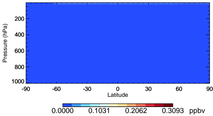
v11-02f-Run1 NO3 - Species Zonal Mean for Jan
