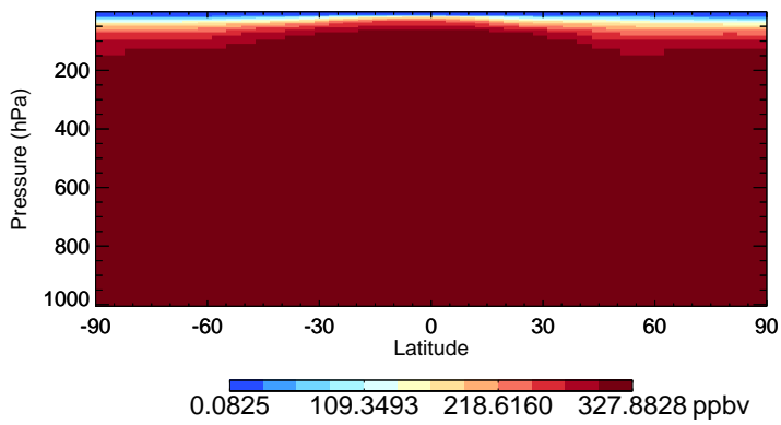
v11-02f-Run1 N2O - Species Zonal Mean for Jan
