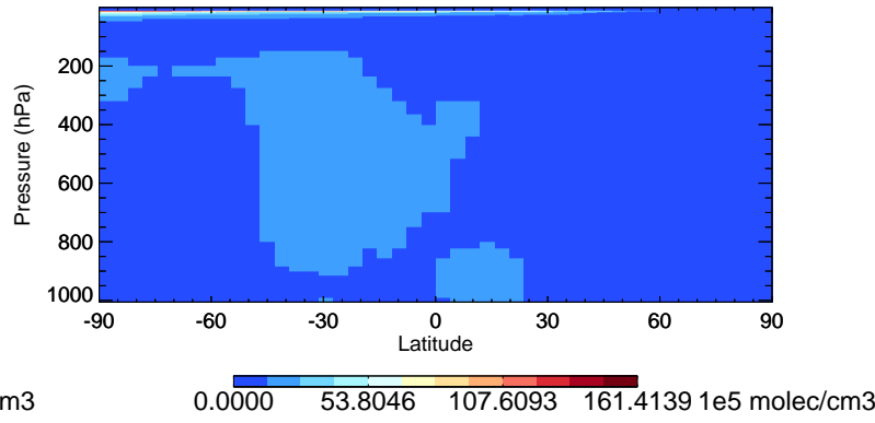
v11-02e-Run1 OH - Species Curtain @ -180.000 for Jan
