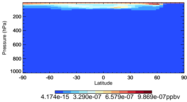
v11-02e-Run1 CIOO - Species Zonal Mean for Jan
