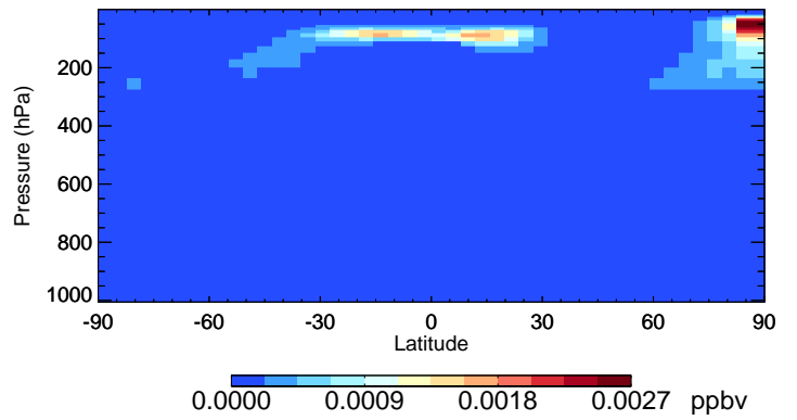
v11-02f-Run1 ISOA3 - Species Curtain @ -180.000 for Jan
