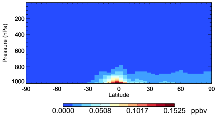
v11-02f-Run1 RCHO - Species Zonal Mean for Jan
