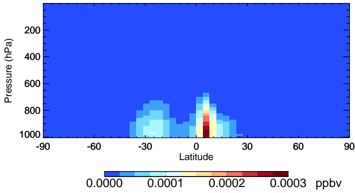
v11-02e-Run1 ETHLN - Species Zonal Mean for Jan
