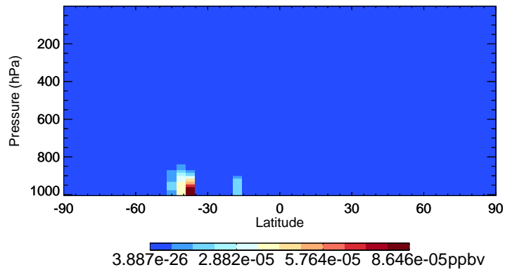
v11-02f-Run1 MOBA - Species Curtain @ -180.000 for Jan
