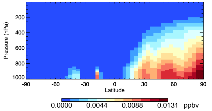
v11-02e-Run1 RCHO - Species Curtain @ -180.000 for Jan
