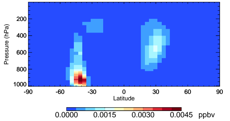
v11-02e-Run1 IMAE - Species Curtain @ -180.000 for Jan
