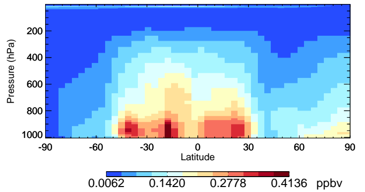
v11-02f-Run1 CH2O - Species Curtain @ -180.000 for Jan
