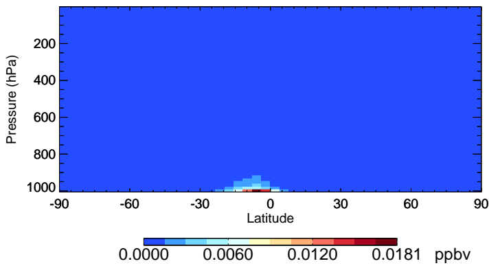
v11-02e-Run1 LIMO - Species Zonal Mean for Jan
