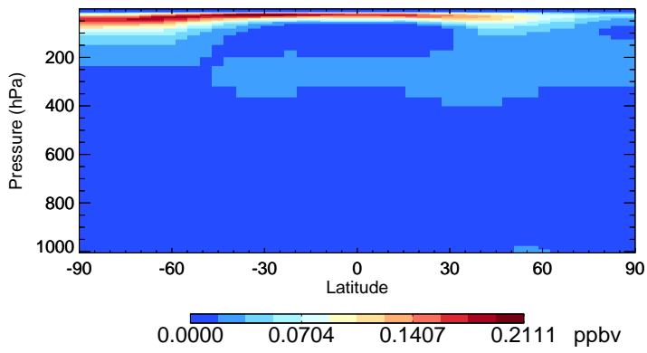
v11-02e-Run1 HNO4 - Species Zonal Mean for Jan
