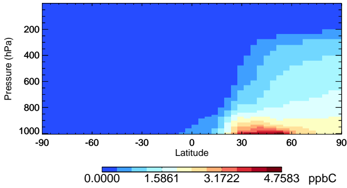
v11-02e-Run1 ALK4 - Species Zonal Mean for Jan
