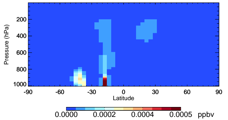
v11-02f-Run1 HONIT - Species Curtain @ -180.000 for Jan
