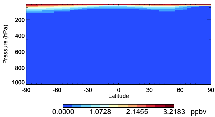
v11-02f-Run1 HCl - Species Zonal Mean for Jan
