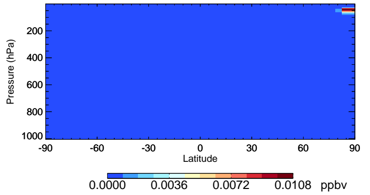
v11-02e-Run0 Cl2O2 - Species Curtain @ -180.000 for Jan
