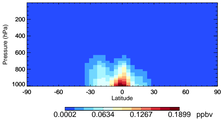
v11-02f-Run1 TSOG3 - Species Zonal Mean for Jan
