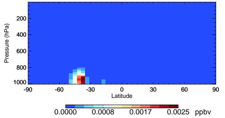
v11-02e-Run1 IPMN - Species Curtain @ -180.000 for Jan
