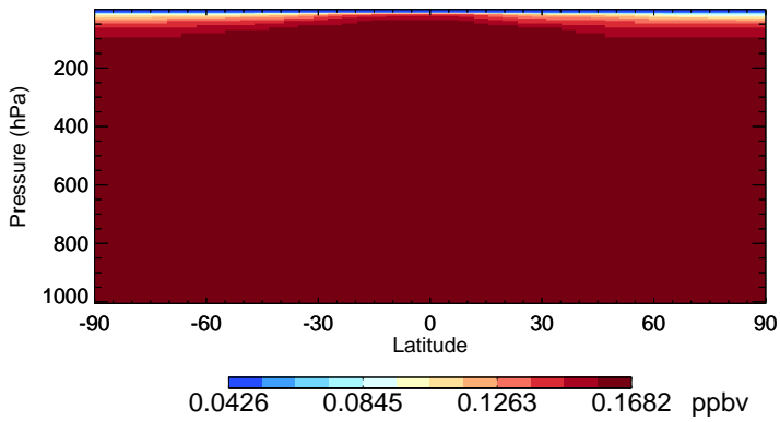
v11-02f-Run1 HCFC22 - Species Zonal Mean for Jan
