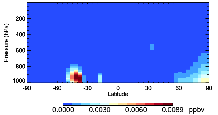
v11-02f-Run1 GLYC - Species Curtain @ -180.000 for Jan
