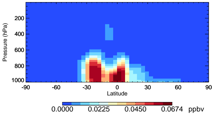
v11-02e-Run0 GLYC - Species Zonal Mean for Jan
