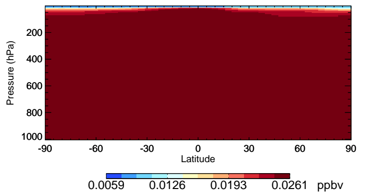
v11-02e-Run1 HCFC142b - Species Curtain @ -180.000 for Jan
