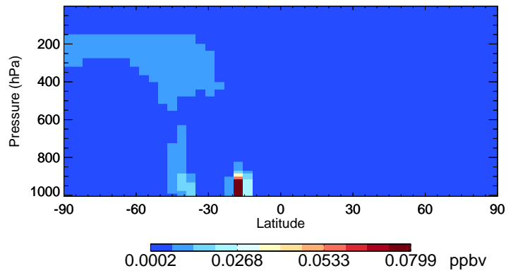
v11-02f-Run1 TSOG3 - Species Curtain @ -180.000 for Jan
