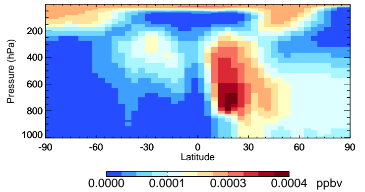
v11-02f-Run1 ASOG1 - Species Curtain @ -180.000 for Jan
