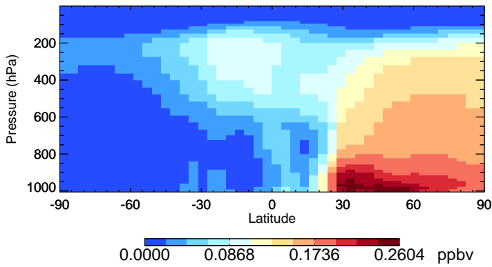
v11-02f-Run1 PAN - Species Zonal Mean for Jan
