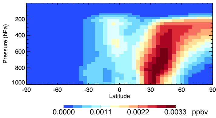
v11-02e-Run1 R4N2 - Species Zonal Mean for Jan
