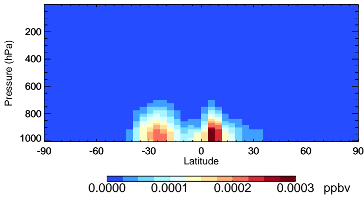
v11-02f-Run1 MACRN - Species Zonal Mean for Jan
