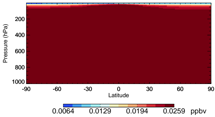
v11-02e-Run0 HCFC142b - Species Zonal Mean for Jan
