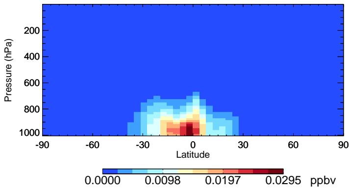
v11-02f-Run1 IPMN - Species Zonal Mean for Jan
