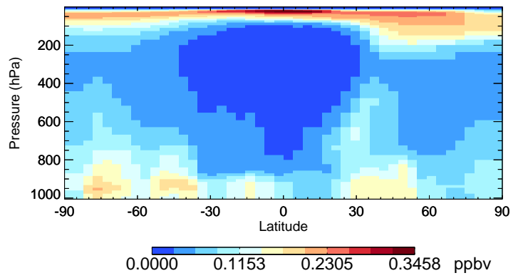
v11-02e-Run1 SO4 - Species Curtain @ -180.000 for Jan
