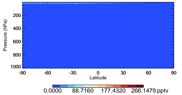
v11-02f-Run1 HO2 - Species Curtain @ -180.000 for Jan
