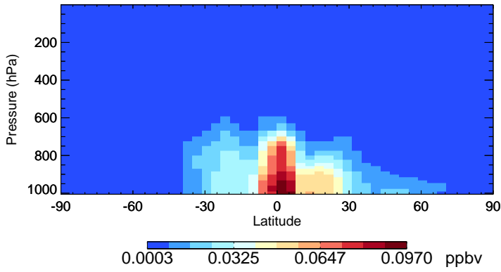
v11-02e-Run1 INDIOL - Species Zonal Mean for Jan
