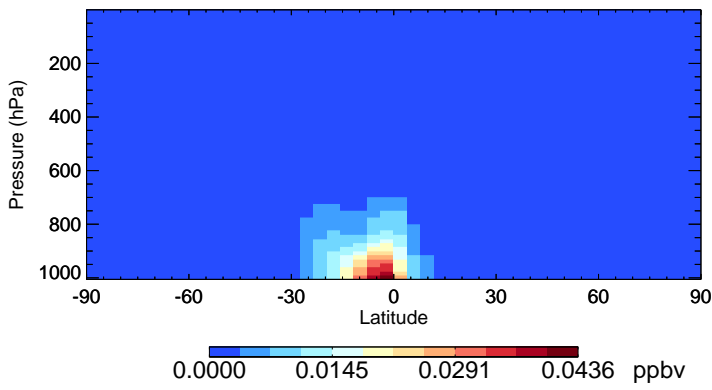
v11-02e-Run1 TSOA0 - Species Zonal Mean for Jan
