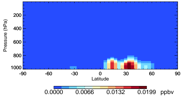
v11-02e-Run1 NITs - Species Curtain @ -180.000 for Jan
