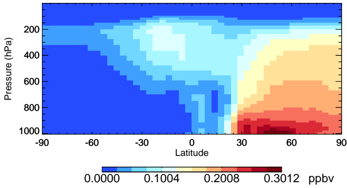
v11-02e-Run1 PAN - Species Zonal Mean for Jan
