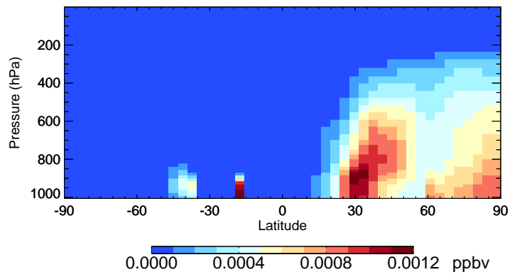
v11-02e-Run1 GLYX - Species Curtain @ -180.000 for Jan
