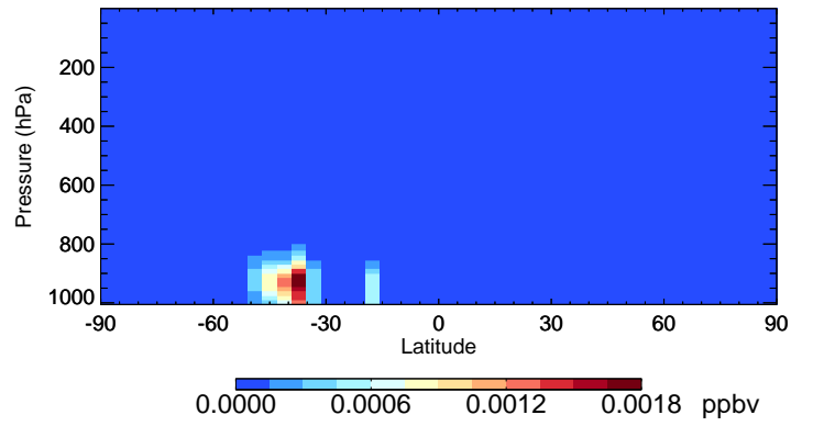
v11-02e-Run0 RIPA - Species Curtain @ -180.000 for Jan
