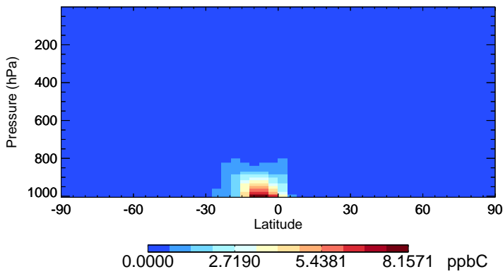
v11-02e-Run1 ISOP - Species Zonal Mean for Jan
