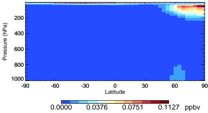
v11-02e-Run0 HOCl - Species Zonal Mean for Jan
