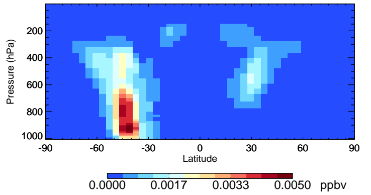
v11-02e-Run0 IMAE - Species Curtain @ -180.000 for Jan
