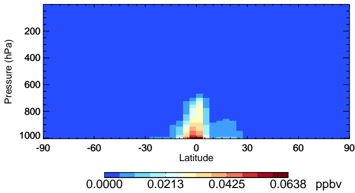
v11-02f-Run1 TSOA2 - Species Zonal Mean for Jan
