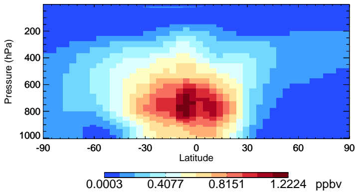
v11-02f-Run1 H2O2 - Species Zonal Mean for Jan
