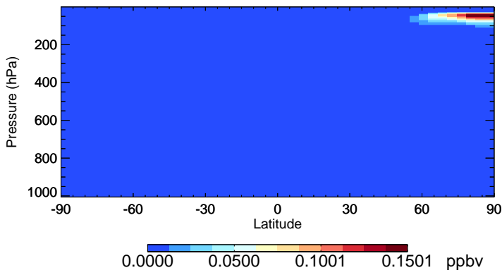
v11-02e-Run1 Cl2O2 - Species Zonal Mean for Jan
