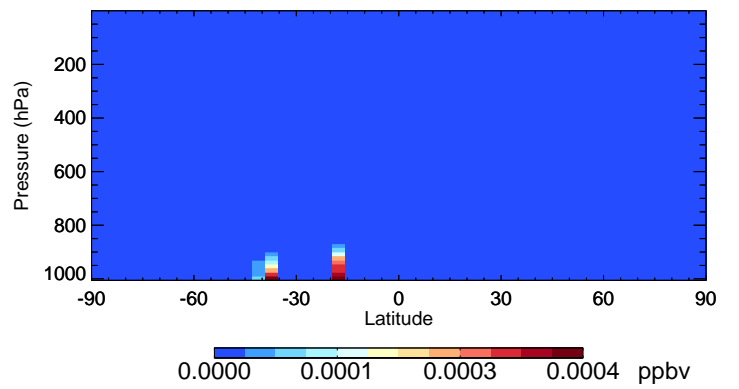
v11-02f-Run1 LIMO - Species Curtain @ -180.000 for Jan
