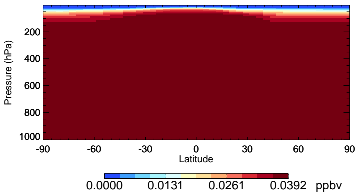
v11-02f-Run1 HCFC141b - Species Zonal Mean for Jan
