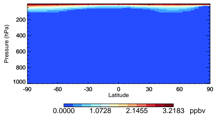
v11-02f-Run1 HCl - Species Curtain @ -180.000 for Jan
