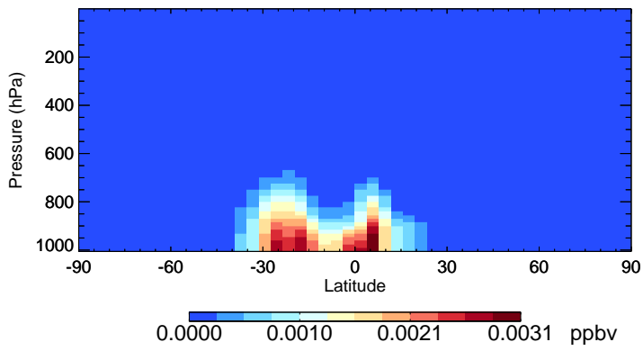
v11-02e-Run1 ISOPNB - Species Zonal Mean for Jan
