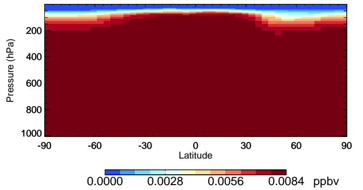
v11-02f-Run1 CH3CCI3 - Species Curtain @ -180.000 for Jan
