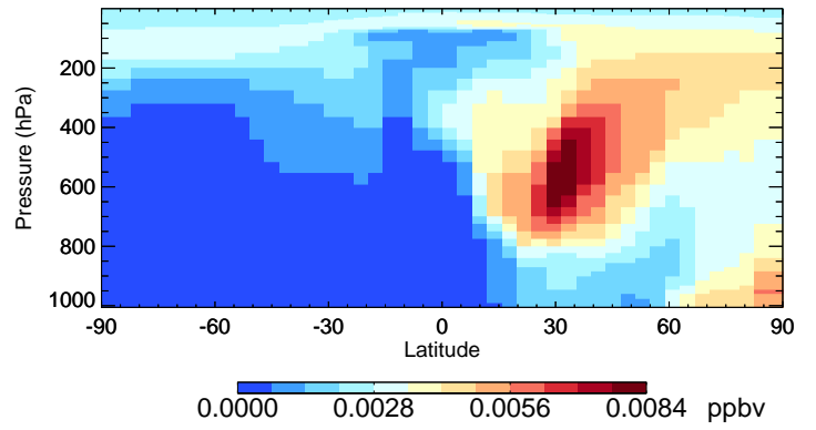
v11-02e-Run0 ASOG3 - Species Curtain @ -180.000 for Jan
