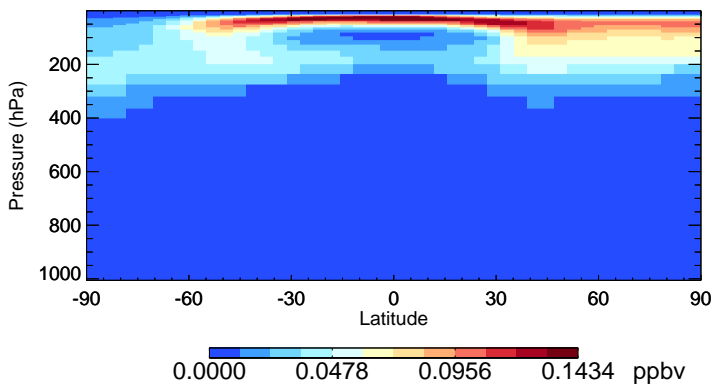
v11-02f-Run1 MPN - Species Zonal Mean for Jan
