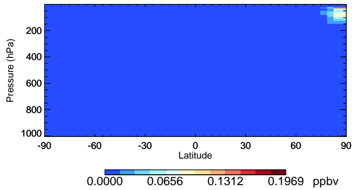
v11-02f-Run1 Cl2 - Species Curtain @ -180.000 for Jan
