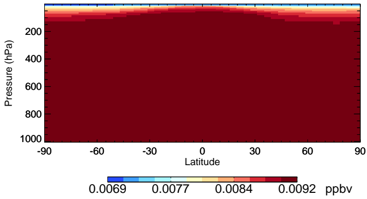
v11-02e-Run0 CFC115 - Species Zonal Mean for Jan
