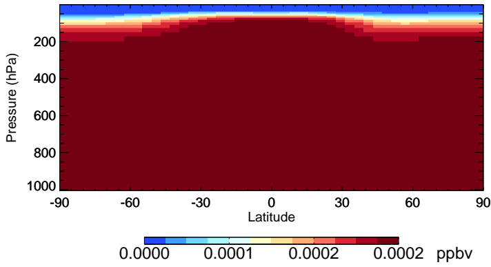
v11-02e-Run1 H2402 - Species Zonal Mean for Jan
