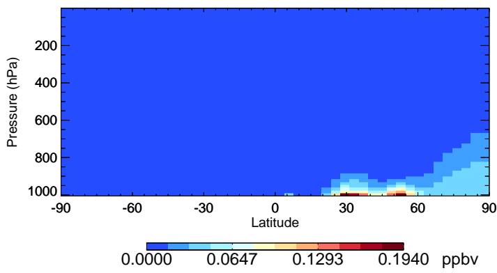
v11-02e-Run1 HNO 2 - Species Zonal Mean for Jan
