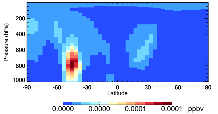
v11-02f-Run1 ISN10A - Species Curtain @ -180.000 for Jan
