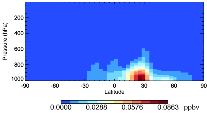
v11-02e-Run1 SOAGX - Species Zonal Mean for Jan
