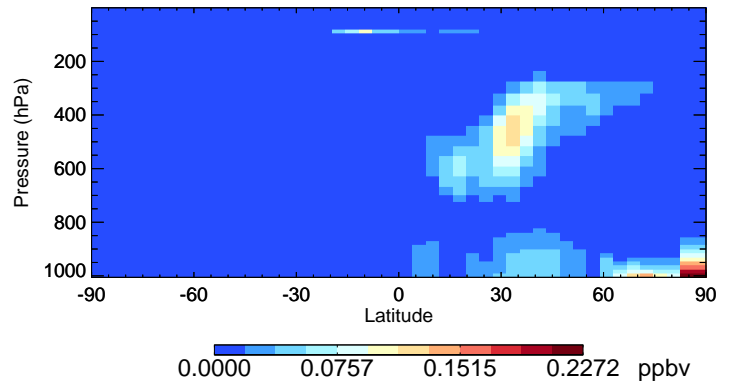
v11-02e-Run0 NIT - Species Curtain @ -180.000 for Jan
