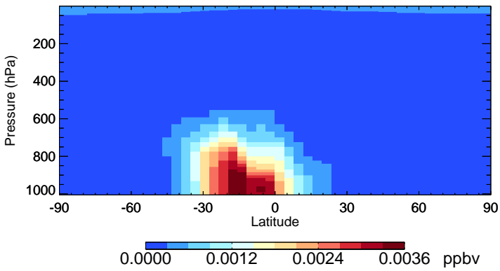
v11-02f-Run1 LVOCOA - Species Zonal Mean for Jan
