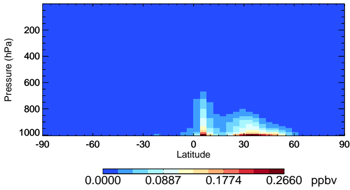
v11-02e-Run0 BCPO - Species Zonal Mean for Jan
