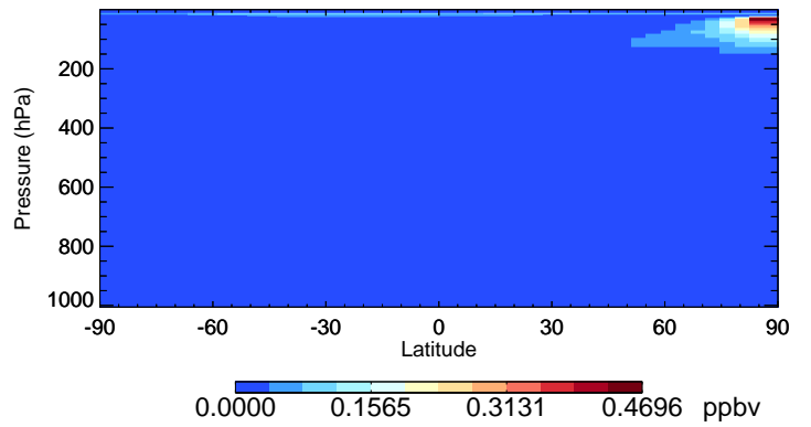
v11-02f-Run1 HOCl - Species Curtain @ -180.000 for Jan
