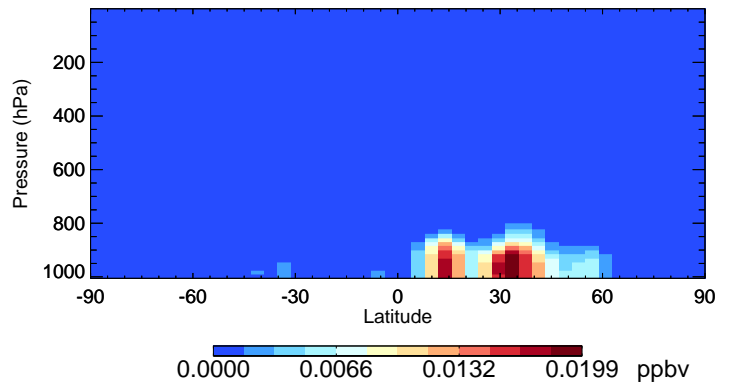
v11-02f-Run1 NITs - Species Curtain @ -180.000 for Jan
