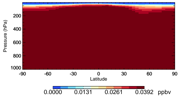
v11-02e-Run1 HCFC141b - Species Curtain @ -180.000 for Jan
