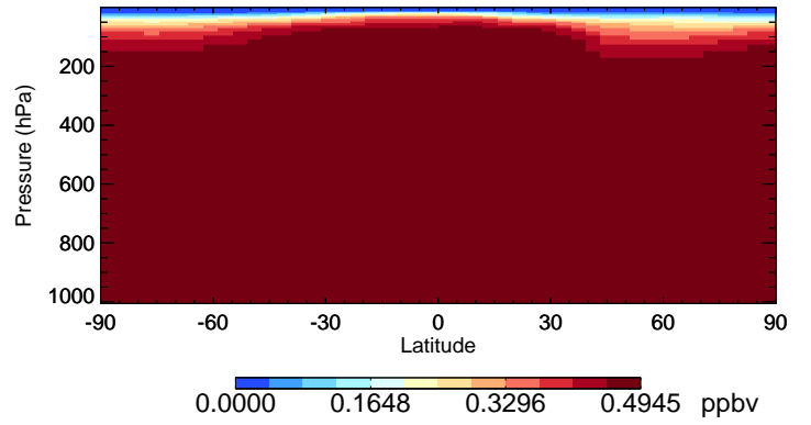
v11-02e-Run1 CFC12 - Species Curtain @ -180.000 for Jan
