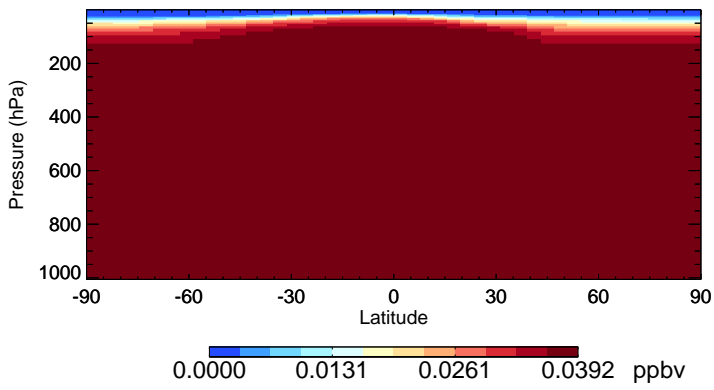
v11-02e-Run1 HCFC141b - Species Zonal Mean for Jan
