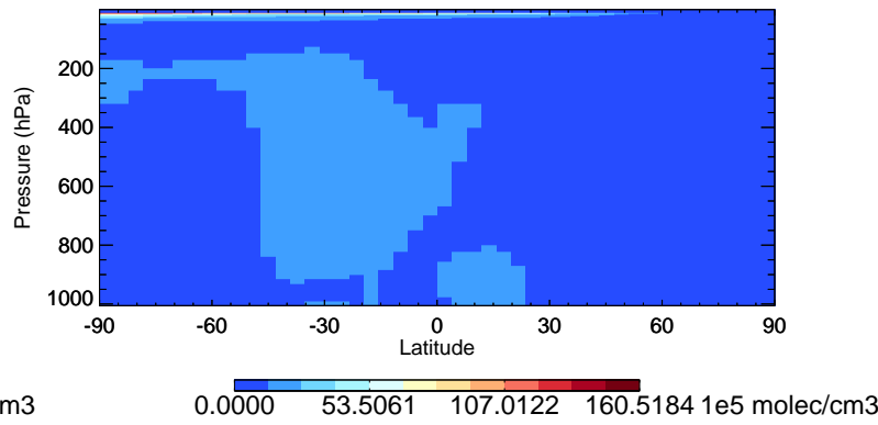
v11-02f-Run1 OH - Species Curtain @ -180.000 for Jan
