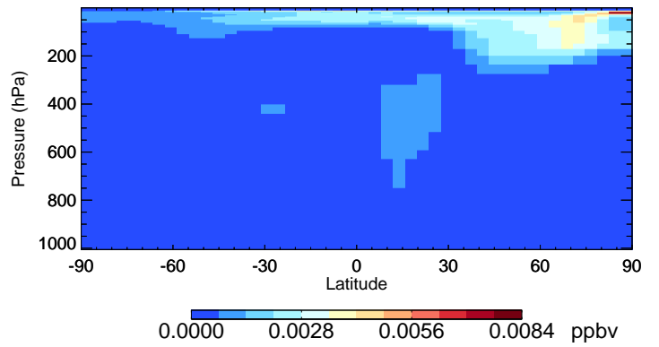
v11-02f-Run1 HOBr - Species Curtain @ -180.000 for Jan
