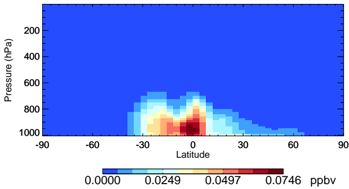
v11-02f-Run1 GLYC - Species Zonal Mean for Jan
