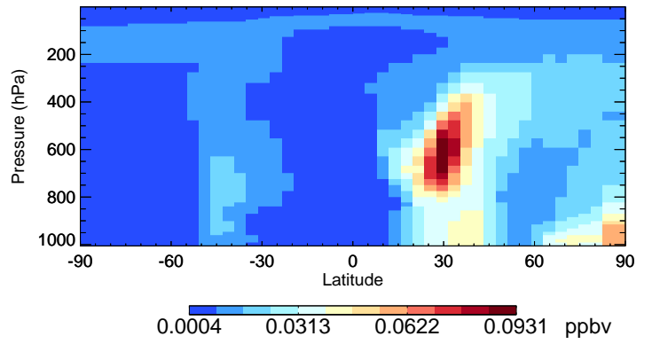
v11-02e-Run0 SOAS - Species Curtain @ -180.000 for Jan
