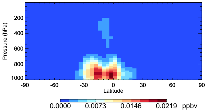
v11-02f-Run1 IEPOXB - Species Zonal Mean for Jan
