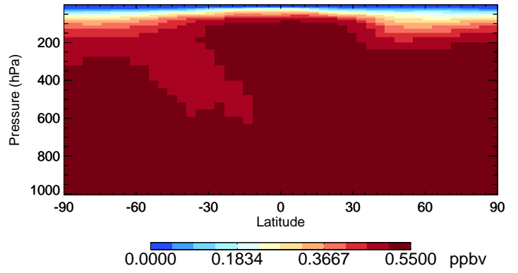
v11-02e-Run1 CH3Cl - Species Curtain @ -180.000 for Jan
