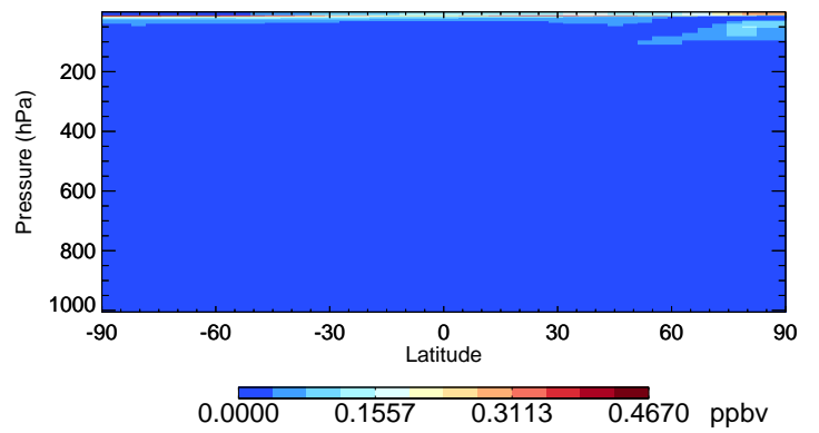
v11-02f-Run1 CIO - Species Curtain @ -180.000 for Jan
