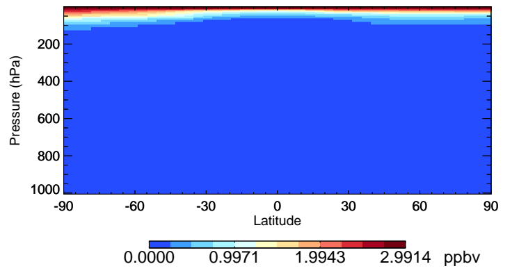
v11-02e-Run0 HCl - Species Curtain @ -180.000 for Jan
