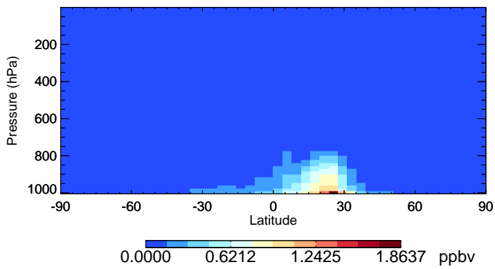
v11-02f-Run1 NH3 - Species Zonal Mean for Jan
