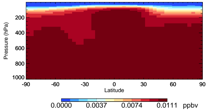
v11-02e-Run0 CH3CCI3 - Species Curtain @ -180.000 for Jan
