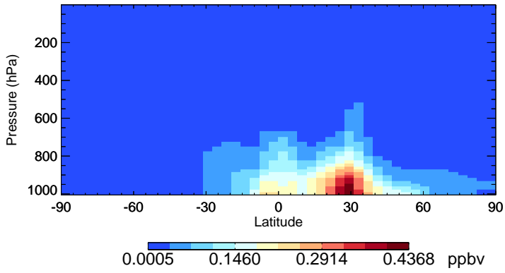
v11-02e-Run1 SOAS - Species Zonal Mean for Jan
