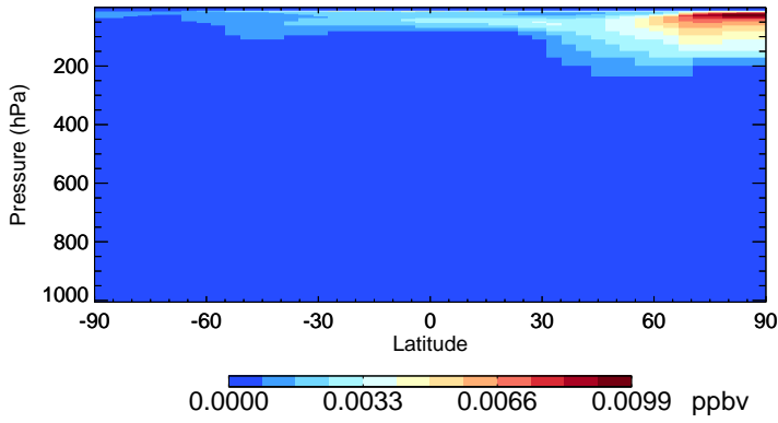
v11-02e-Run1 HOBr - Species Zonal Mean for Jan
