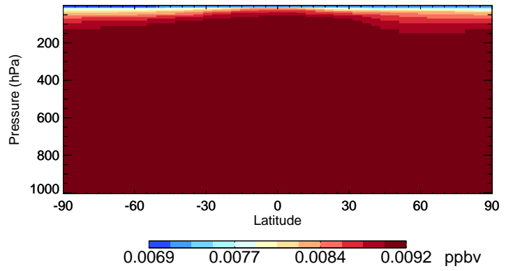
v11-02e-Run0 CFC115 - Species Curtain @ -180.000 for Jan
