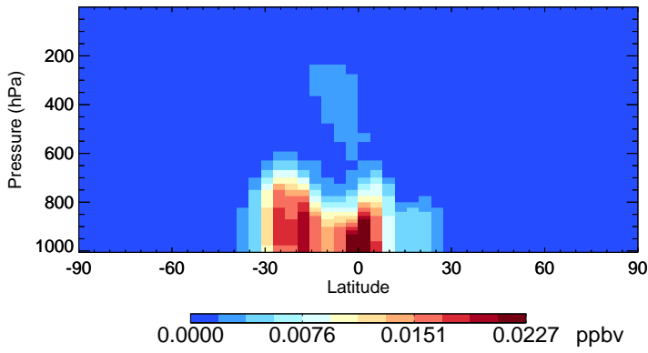
v11-02e-Run0 IPMN - Species Zonal Mean for Jan
