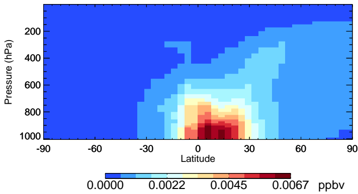
v11-02f-Run1 ASOAN - Species Zonal Mean for Jan
