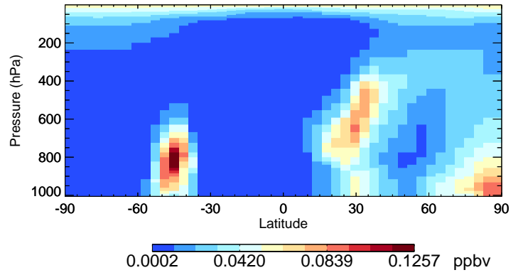
v11-02e-Run1 OCPI - Species Curtain @ -180.000 for Jan
