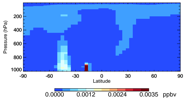
v11-02f-Run1 TSOA0 - Species Curtain @ -180.000 for Jan
