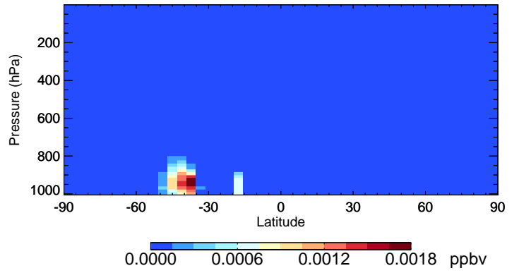
v11-02e-Run1 IEPOXB - Species Curtain @ -180.000 for Jan
