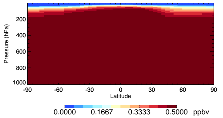
v11-02e-Run0 OCS - Species Curtain @ -180.000 for Jan
