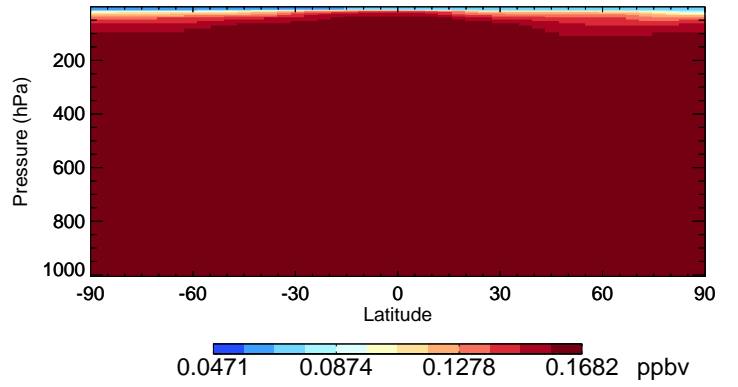
v11-02e-Run1 HCFC22 - Species Curtain @ -180.000 for Jan
