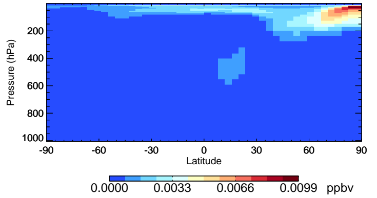
v11-02e-Run1 HOBr - Species Curtain @ -180.000 for Jan
