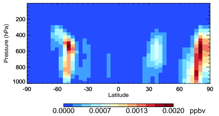
v11-02f-Run1 DST4 - Species Curtain @ -180.000 for Jan
