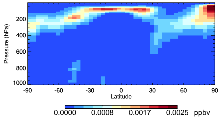
v11-02f-Run1 TSOA2 - Species Curtain @ -180.000 for Jan
