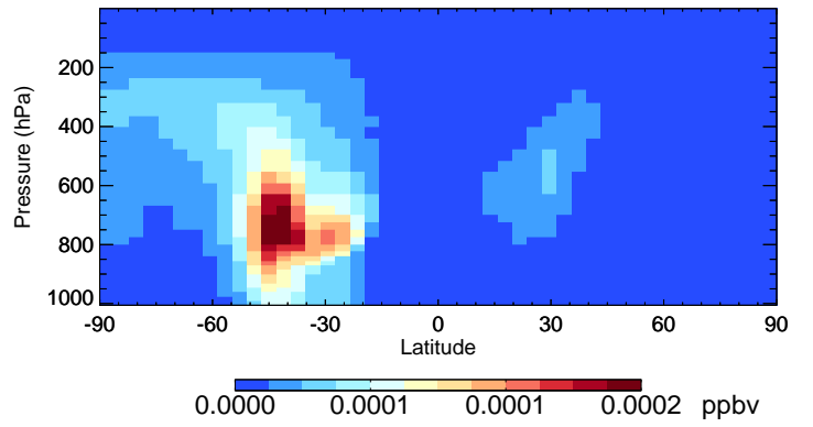
v11-02e-Run0 ISN10A - Species Curtain @ -180.000 for Jan
