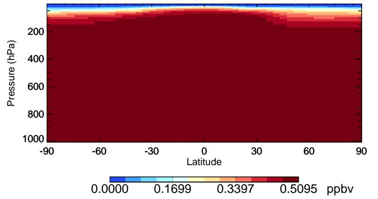
v11-02e-Run0 CFC12 - Species Curtain @ -180.000 for Jan
