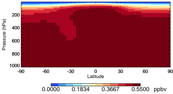
v11-02e-Run0 CH3Cl - Species Zonal Mean for Jan
