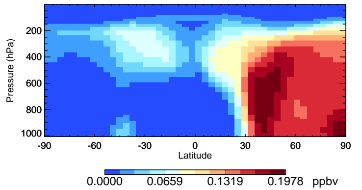
v11-02f-Run1 PAN - Species Curtain @ -180.000 for Jan
