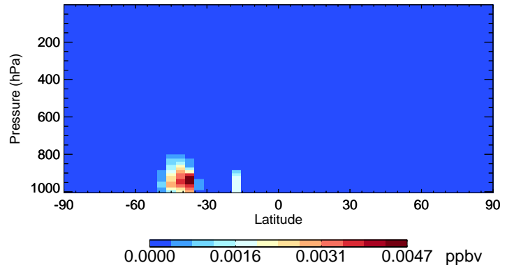
v11-02e-Run1 IEPOXA - Species Curtain @ -180.000 for Jan
