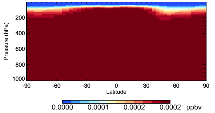
v11-02e-Run1 H2402 - Species Curtain @ -180.000 for Jan
