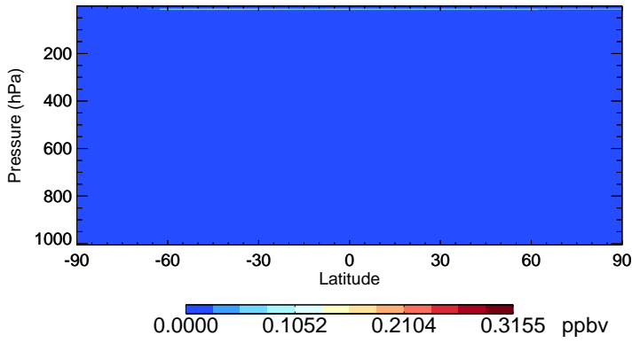
v11-02e-Run1 NO3 - Species Zonal Mean for Jan
