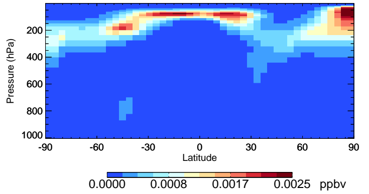
v11-02e-Run1 TSOA2 - Species Curtain @ -180.000 for Jan
