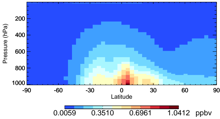
v11-02e-Run1 CH2O - Species Zonal Mean for Jan
