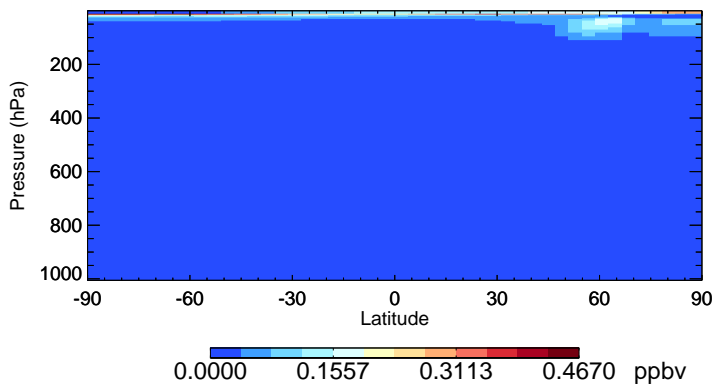
v11-02f-Run1 CIO - Species Zonal Mean for Jan
