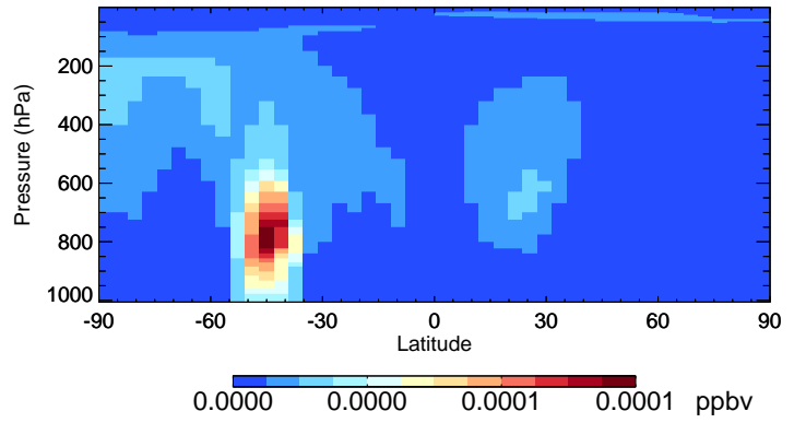
v11-02e-Run1 ISN10A - Species Curtain @ -180.000 for Jan
