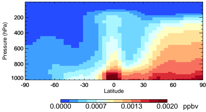
v11-02e-Run1 CHBr3 - Species Zonal Mean for Jan
