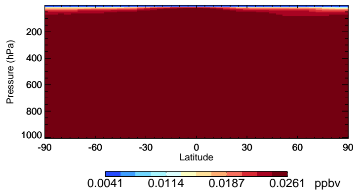
v11-02f-Run1 HCFC142b - Species Curtain @ -180.000 for Jan
