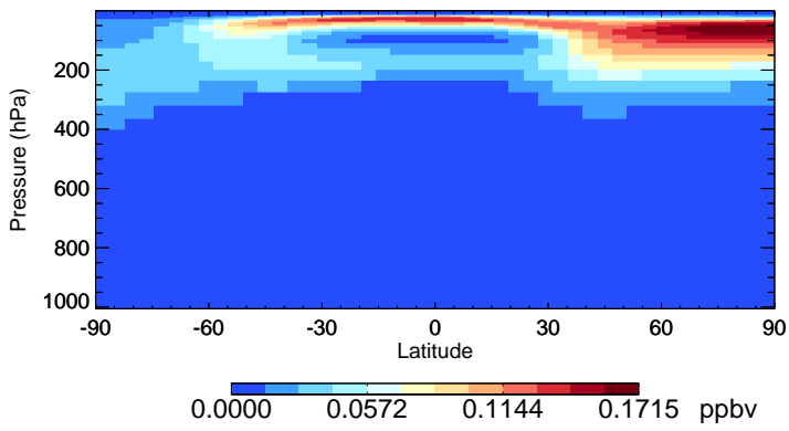
v11-02e-Run1 MPN - Species Zonal Mean for Jan
