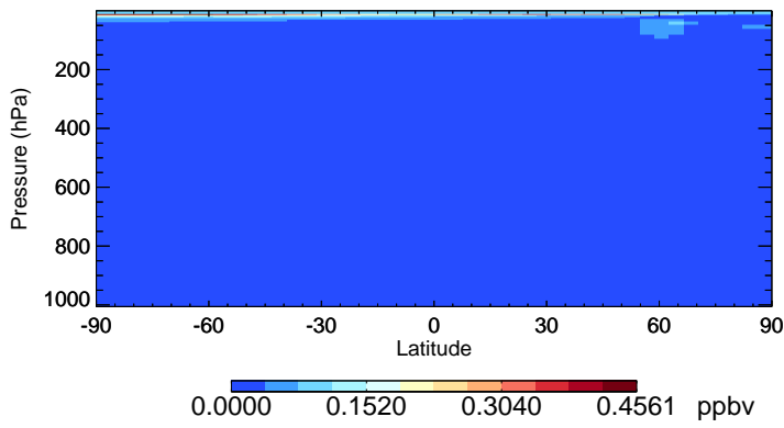
v11-02e-Run1 CIO - Species Zonal Mean for Jan
