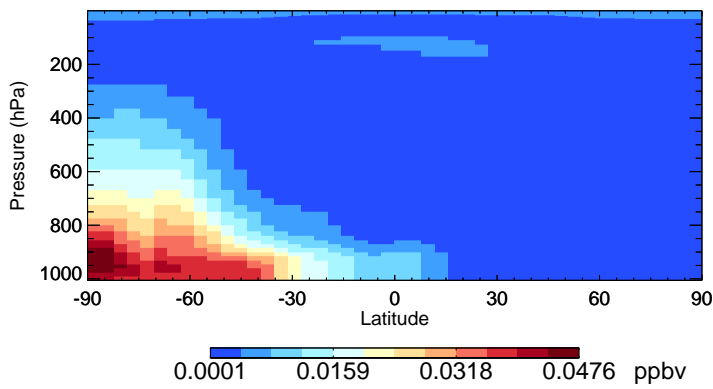
v11-02f-Run1 MSA - Species Zonal Mean for Jan
