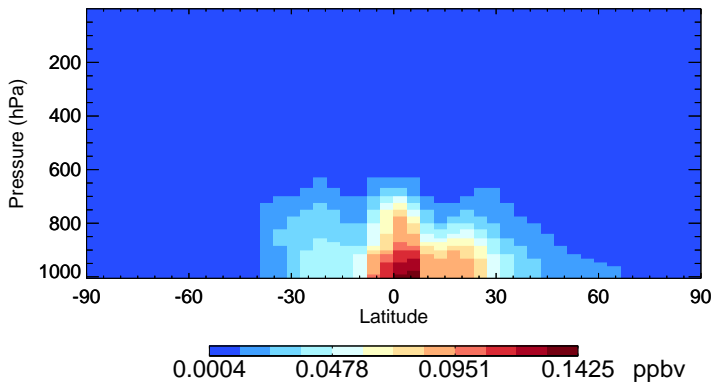
v11-02f-Run1 INDIOL - Species Zonal Mean for Jan
