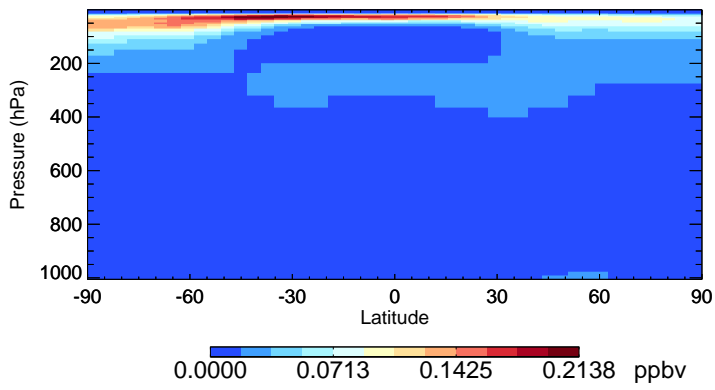
v11-02e-Run0 HNO4 - Species Zonal Mean for Jan
