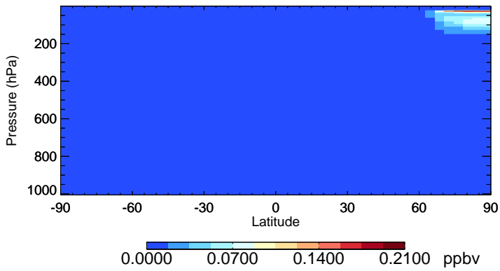
v11-02f-Run1 Cl2 - Species Zonal Mean for Jan
