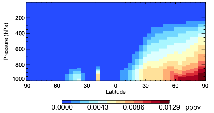
v11-02e-Run0 RCHO - Species Curtain @ -180.000 for Jan
