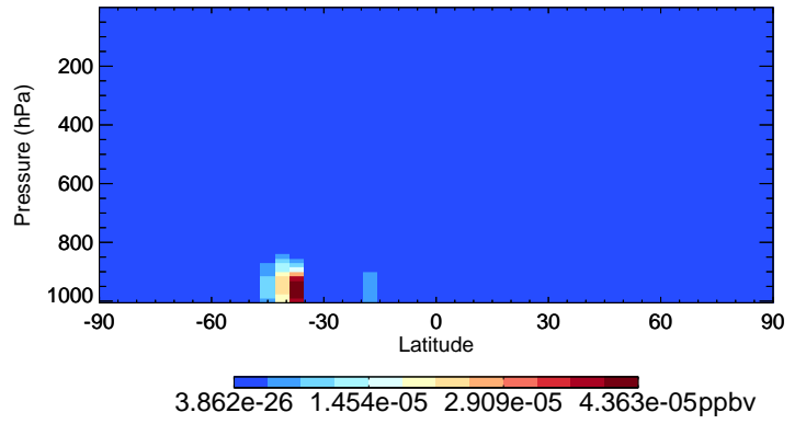
v11-02e-Run1 MOBA - Species Curtain @ -180.000 for Jan
