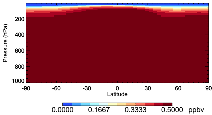
v11-02f-Run1 OCS - Species Zonal Mean for Jan
