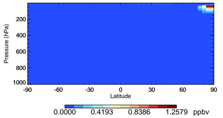
v11-02e-Run1 HOCl - Species Curtain @ -180.000 for Jan
