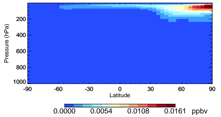
v11-02e-Run1 BrCl - Species Curtain @ -180.000 for Jan
