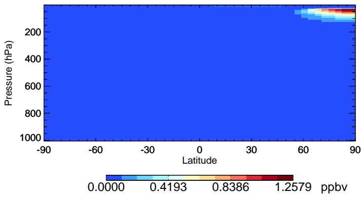
v11-02e-Run1 HOCl - Species Zonal Mean for Jan
