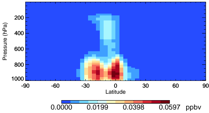
v11-02e-Run1 IEPOXA - Species Zonal Mean for Jan
