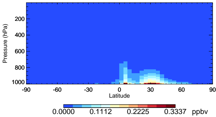
v11-02f-Run1 BCPO - Species Zonal Mean for Jan
