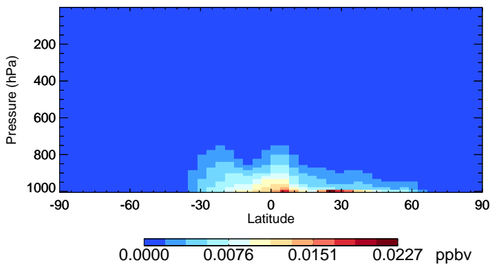
v11-02f-Run1 GLYX - Species Zonal Mean for Jan
