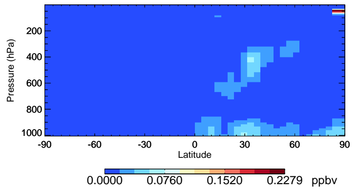
v11-02e-Run1 NIT - Species Curtain @ -180.000 for Jan
