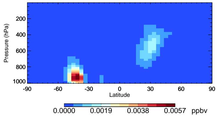
v11-02f-Run1 IMAE - Species Curtain @ -180.000 for Jan
