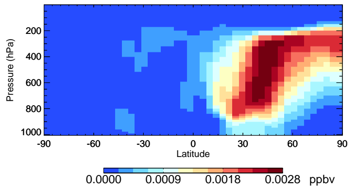
v11-02e-Run1 R4N2 - Species Curtain @ -180.000 for Jan
