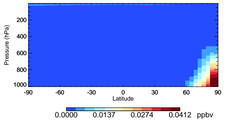
v11-02f-Run1 HNO 2 - Species Curtain @ -180.000 for Jan
