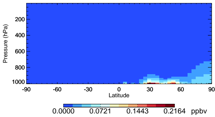
v11-02f-Run1 HNO 2 - Species Zonal Mean for Jan
