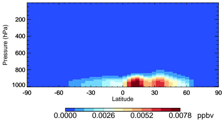
v11-02f-Run1 NITs - Species Zonal Mean for Jan
