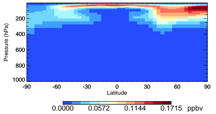
v11-02e-Run1 MPN - Species Curtain @ -180.000 for Jan
