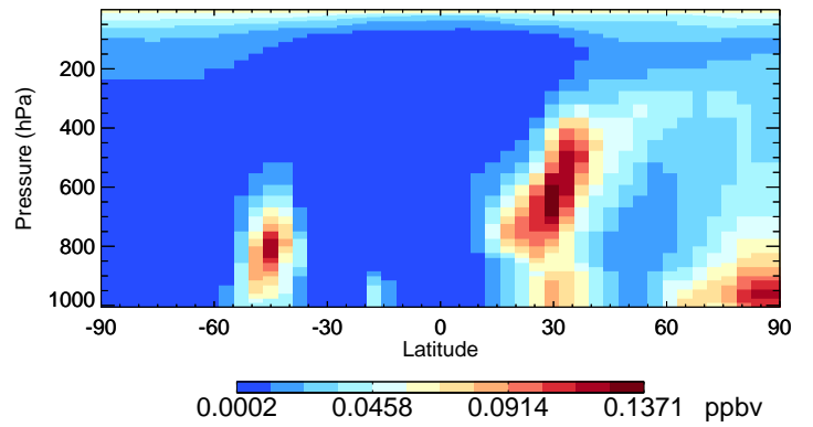
v11-02f-Run1 OCPI - Species Curtain @ -180.000 for Jan
