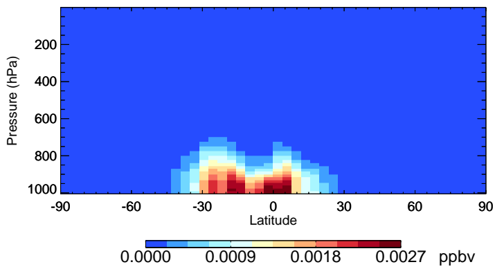
v11-02f-Run1 ISOPNB - Species Zonal Mean for Jan
