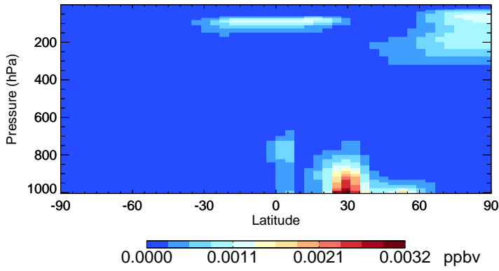
v11-02e-Run1 ASOA3 - Species Zonal Mean for Jan
