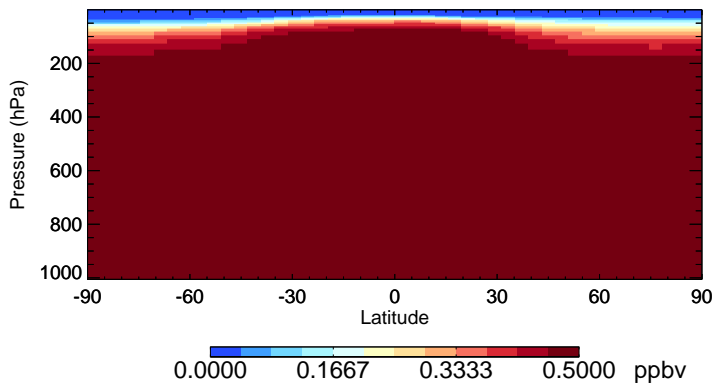
v11-02e-Run0 OCS - Species Zonal Mean for Jan
