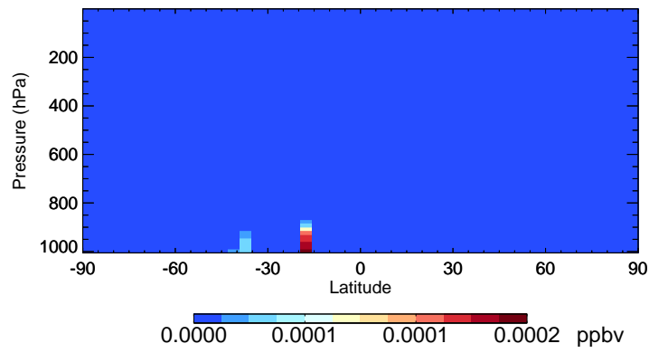
v11-02e-Run1 LIMO - Species Curtain @ -180.000 for Jan
