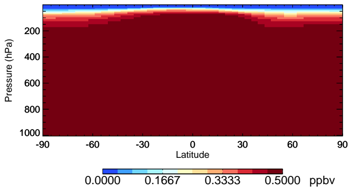
v11-02e-Run1 OCS - Species Zonal Mean for Jan
