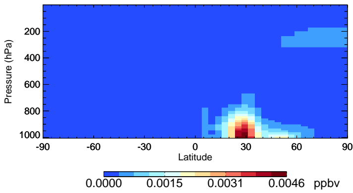
v11-02e-Run1 ASOA2 - Species Zonal Mean for Jan
