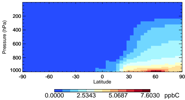
v11-02f-Run1 ALK4 - Species Zonal Mean for Jan
