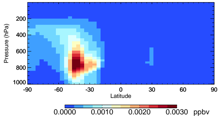
v11-02e-Run0 SOAME - Species Curtain @ -180.000 for Jan
