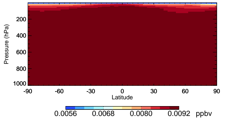
v11-02f-Run1 CFC115 - Species Curtain @ -180.000 for Jan
