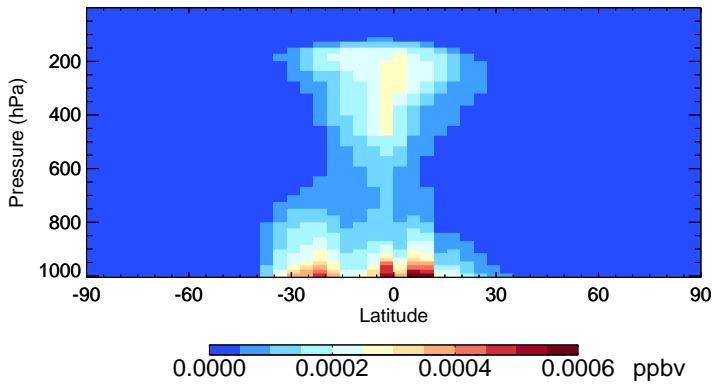
v11-02e-Run0 HONIT - Species Zonal Mean for Jan
