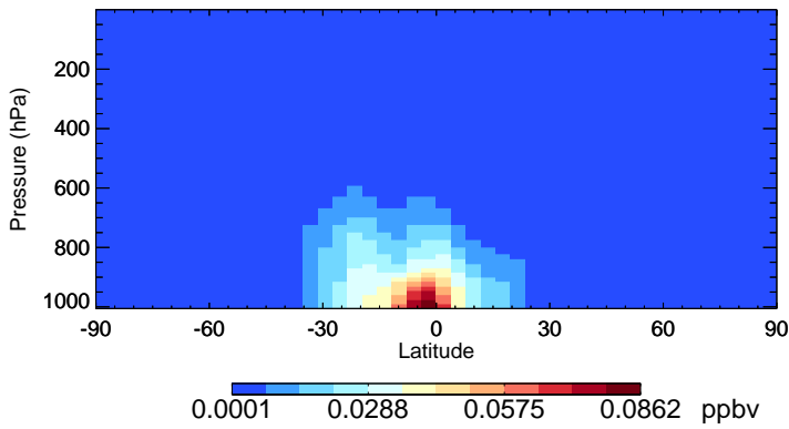
v11-02f-Run1 TSOG2 - Species Zonal Mean for Jan
