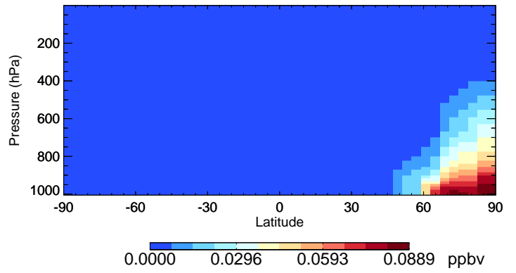
v11-02e-Run0 ClNO 2 - Species Curtain @ -180.000 for Jan
