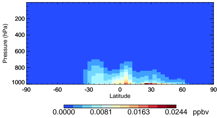
v11-02e-Run0 GLYX - Species Zonal Mean for Jan
