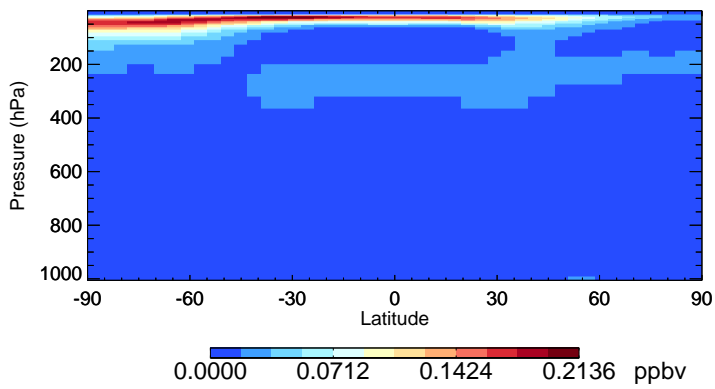
v11-02f-Run1 HNO4 - Species Zonal Mean for Jan
