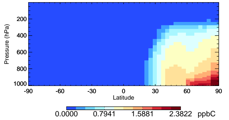
v11-02e-Run0 ALK4 - Species Curtain @ -180.000 for Jan
