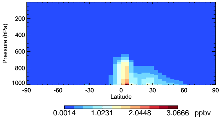
v11-02e-Run1 OCPI - Species Zonal Mean for Jan
