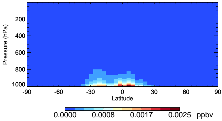
v11-02e-Run0 MONITS - Species Zonal Mean for Jan
