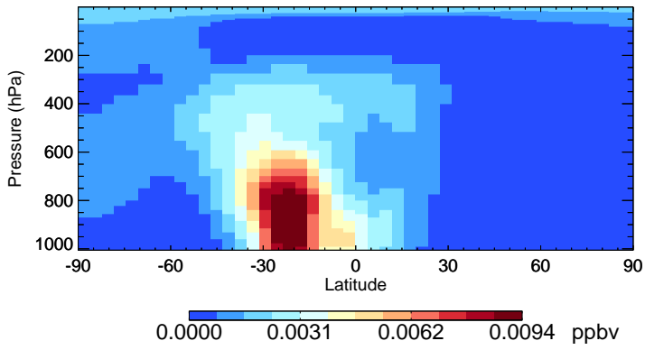
v11-02e-Run0 ISOG1 - Species Zonal Mean for Jan
