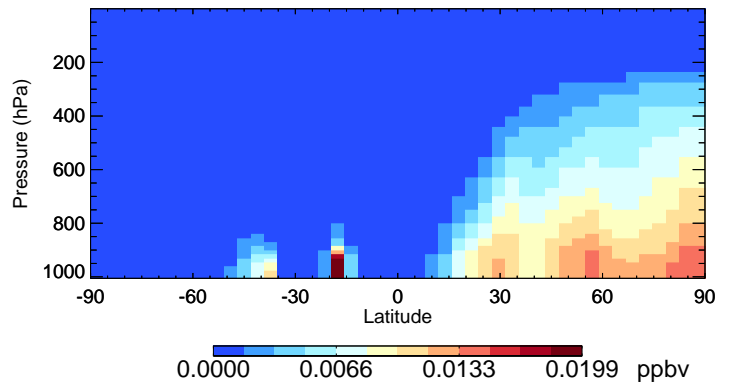
v11-02f-Run1 RCHO - Species Curtain @ -180.000 for Jan
