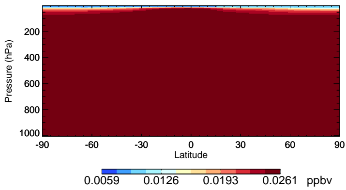
v11-02e-Run1 HCFC142b - Species Zonal Mean for Jan
