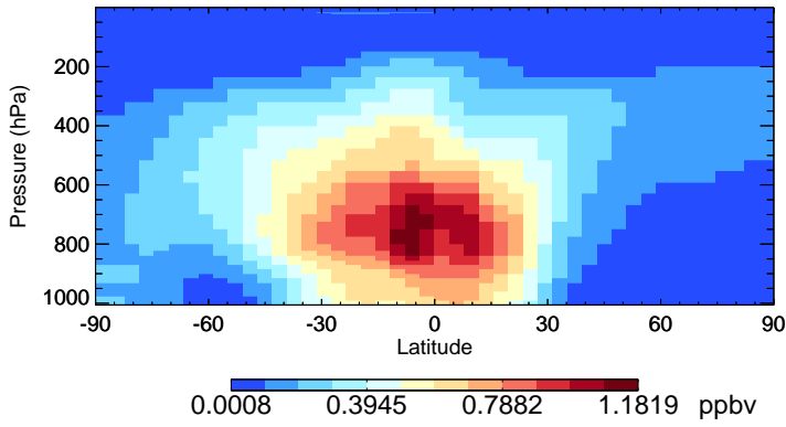
v11-02e-Run1 H2O2 - Species Zonal Mean for Jan
