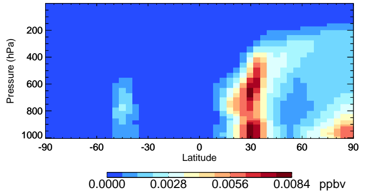
v11-02e-Run1 SOAGX - Species Curtain @ -180.000 for Jan
