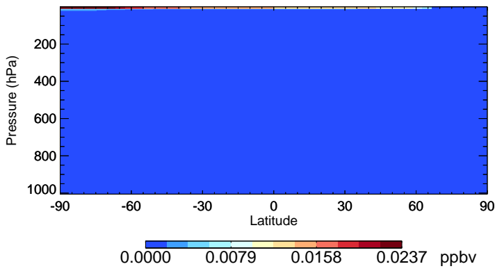
v11-02e-Run1 Br - Species Zonal Mean for Jan
