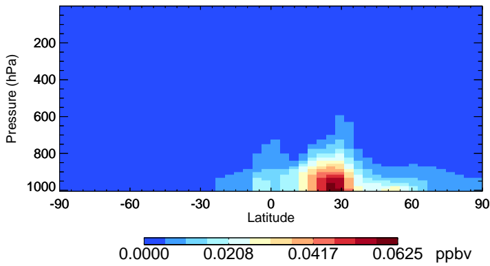
v11-02f-Run1 SOAGX - Species Zonal Mean for Jan
