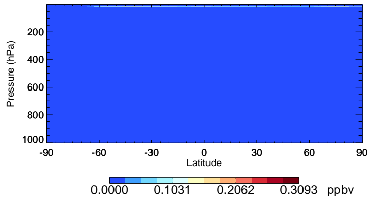
v11-02f-Run1 NO3 - Species Curtain @ -180.000 for Jan
