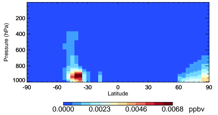
v11-02e-Run0 GLYC - Species Curtain @ -180.000 for Jan
