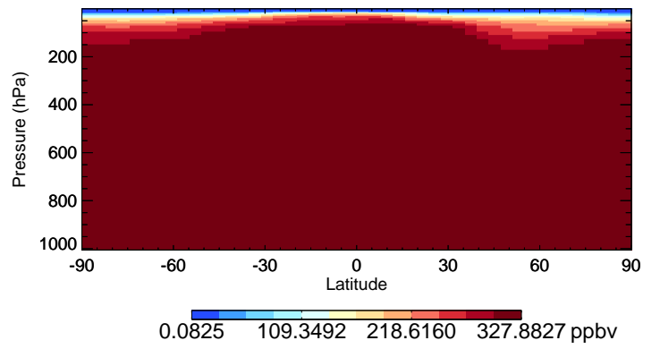
v11-02e-Run1 N2O - Species Curtain @ -180.000 for Jan
