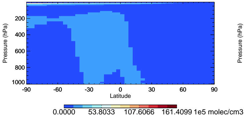
v11-02e-Run1 OH - Species Zonal Mean for Jan
