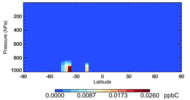
v11-02e-Run1 ISOP - Species Curtain @ -180.000 for Jan
