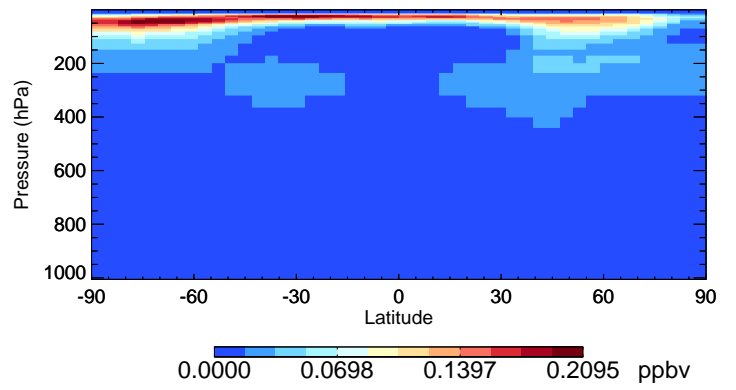
v11-02e-Run1 HNO4 - Species Curtain @ -180.000 for Jan
