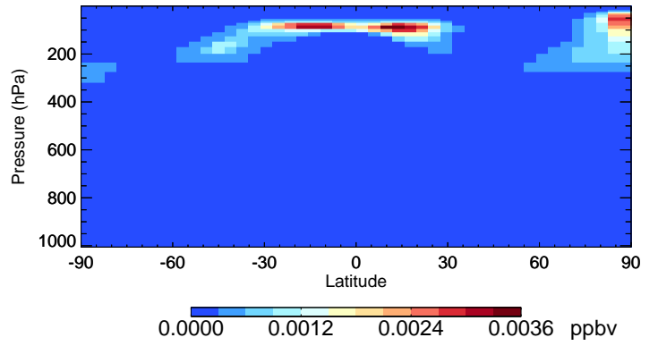
v11-02e-Run1 ISOA3 - Species Curtain @ -180.000 for Jan
