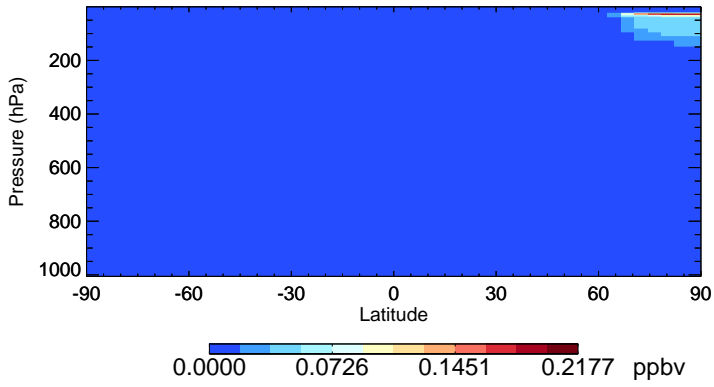
v11-02e-Run1 Cl2 - Species Zonal Mean for Jan
