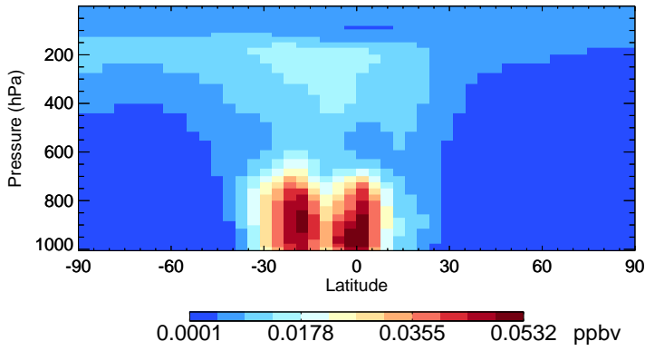
v11-02e-Run1 ISO3 - Species Zonal Mean for Jan
