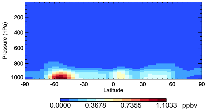
v11-02e-Run1 SALA - Species Zonal Mean for Jan
