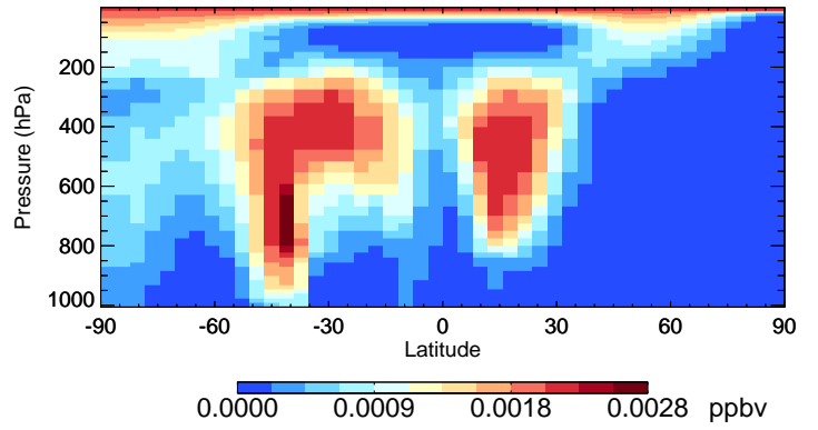
v11-02e-Run1 ISOG1 - Species Curtain @ -180.000 for Jan
