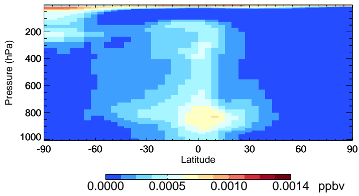
v11-02e-Run1 HBr - Species Zonal Mean for Jan
