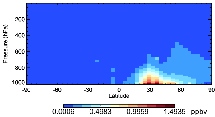
v11-02f-Run1 SO2 - Species Zonal Mean for Jan
