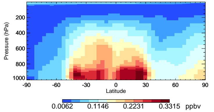
v11-02e-Run1 CH2O - Species Curtain @ -180.000 for Jan
