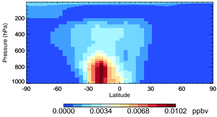
v11-02e-Run1 ISOG1 - Species Zonal Mean for Jan
