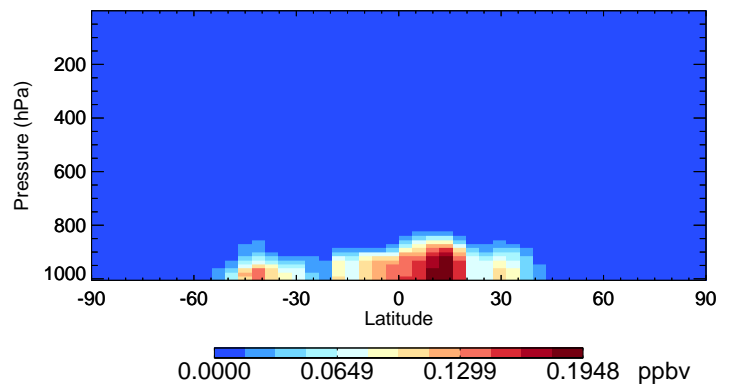
v11-02f-Run1 NH3 - Species Curtain @ -180.000 for Jan
