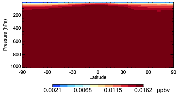
v11-02e-Run0 CFC114 - Species Curtain @ -180.000 for Jan
