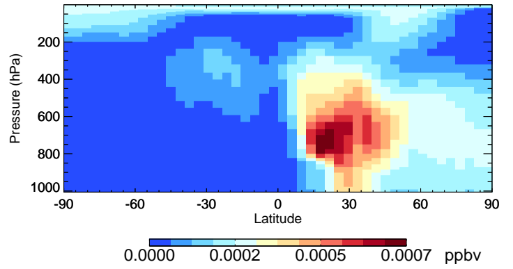
v11-02e-Run1 ASOG1 - Species Curtain @ -180.000 for Jan
