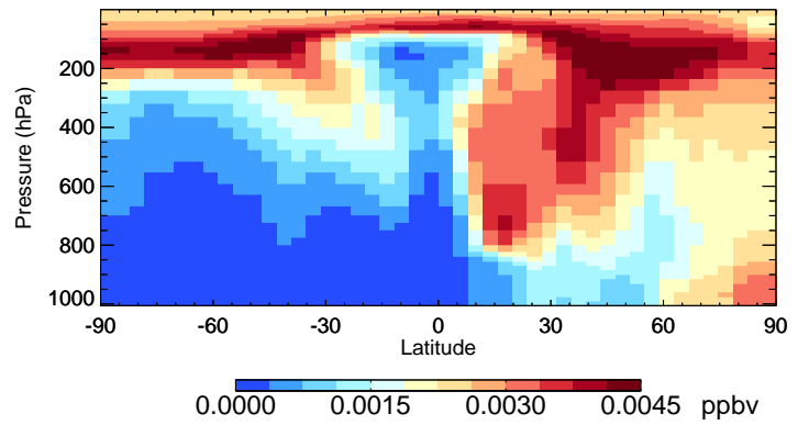
v11-02f-Run1 ASOG3 - Species Curtain @ -180.000 for Jan
