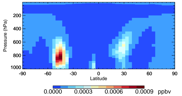
v11-02f-Run1 SOAME - Species Curtain @ -180.000 for Jan
