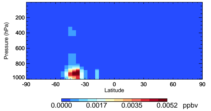
v11-02e-Run0 IEPOXA - Species Curtain @ -180.000 for Jan
