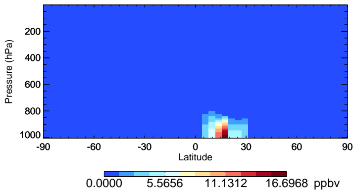
v11-02e-Run1 DST4 - Species Zonal Mean for Jan
