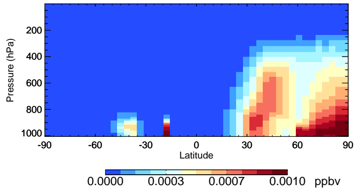
v11-02e-Run0 GLYX - Species Curtain @ -180.000 for Jan
