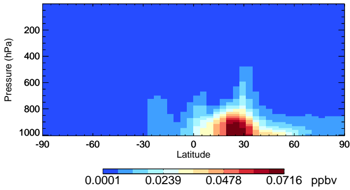
v11-02e-Run0 SOAGX - Species Zonal Mean for Jan
