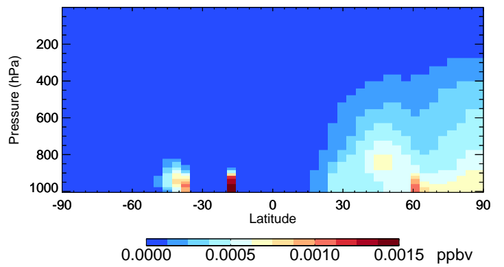
v11-02f-Run1 GLYX - Species Curtain @ -180.000 for Jan
