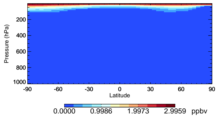
v11-02e-Run1 HCl - Species Curtain @ -180.000 for Jan
