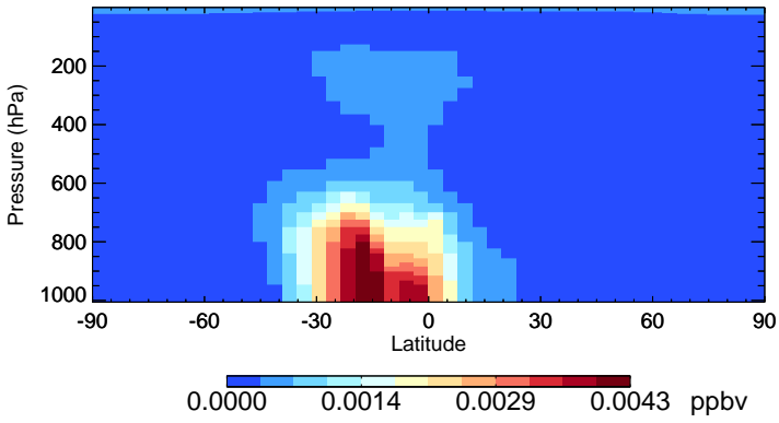
v11-02e-Run1 LVOCOA - Species Zonal Mean for Jan
