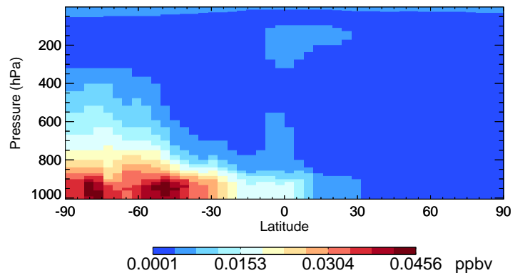
v11-02e-Run0 MSA - Species Curtain @ -180.000 for Jan
