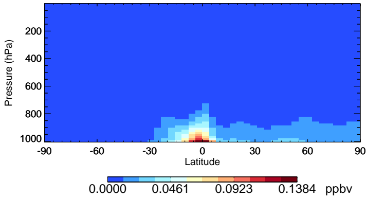
v11-02e-Run1 RCHO - Species Zonal Mean for Jan
