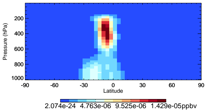
v11-02f-Run1 LVOC - Species Zonal Mean for Jan
