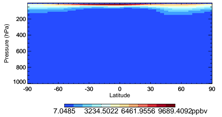
v11-02e-Run1 O3 - Species Curtain @ -180.000 for Jan
