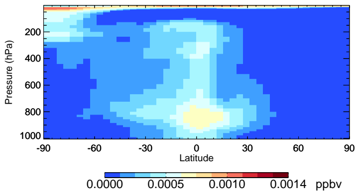
v11-02f-Run1 HBr - Species Zonal Mean for Jan
