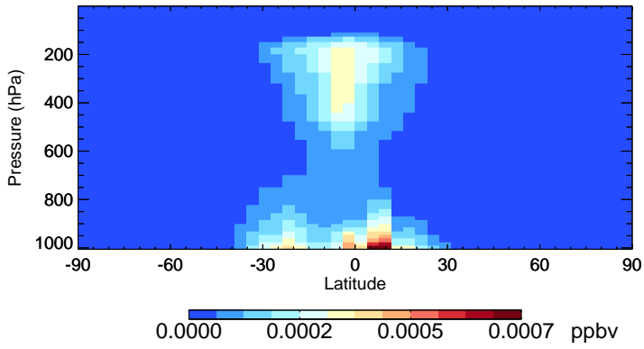
v11-02e-Run1 HONIT - Species Zonal Mean for Jan
