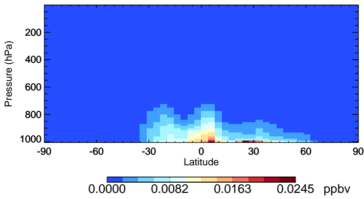
v11-02e-Run1 GLYX - Species Zonal Mean for Jan
