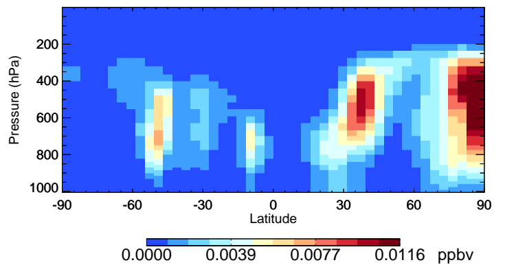
v11-02f-Run1 DST2 - Species Curtain @ -180.000 for Jan
