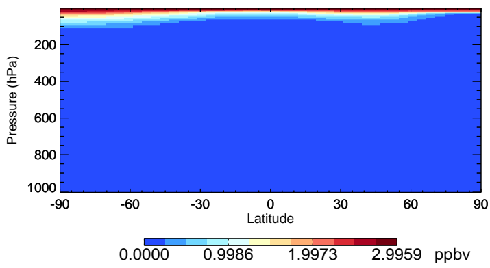
v11-02e-Run1 HCl - Species Zonal Mean for Jan
