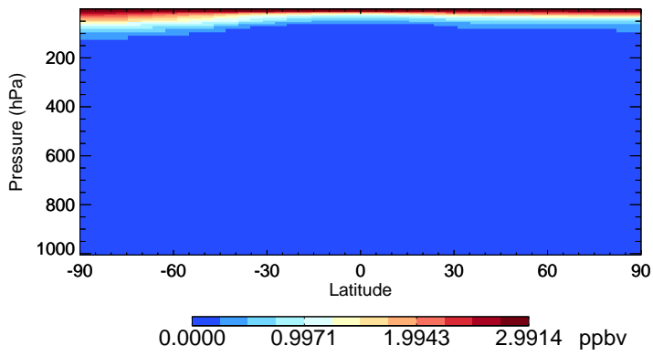
v11-02e-Run0 HCl - Species Zonal Mean for Jan
