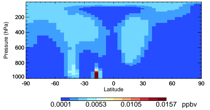
v11-02e-Run1 TSOG2 - Species Curtain @ -180.000 for Jan
