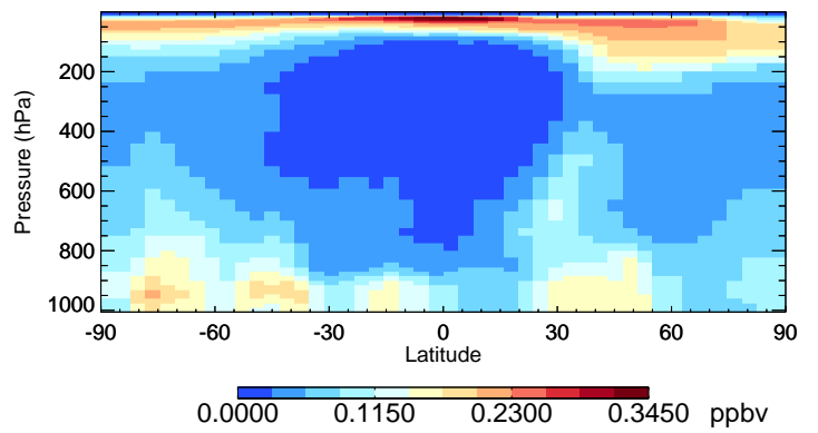
v11-02f-Run1 SO4 - Species Curtain @ -180.000 for Jan
