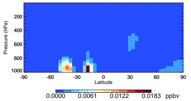
v11-02f-Run1 HAC - Species Curtain @ -180.000 for Jan
