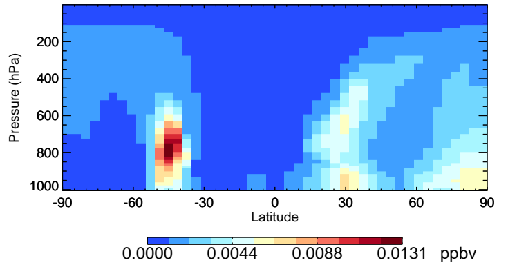
v11-02e-Run1 INDIOL - Species Curtain @ -180.000 for Jan
