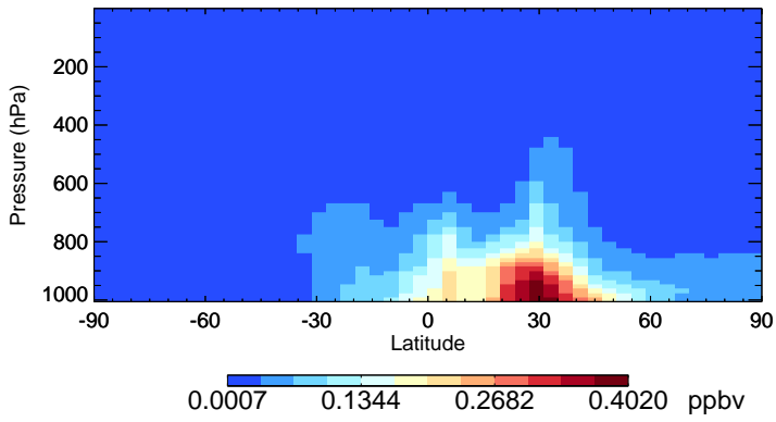
v11-02e-Run0 SOAS - Species Zonal Mean for Jan
