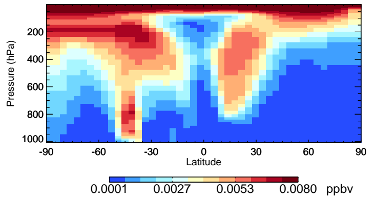
v11-02f-Run1 ISO3 - Species Curtain @ -180.000 for Jan
