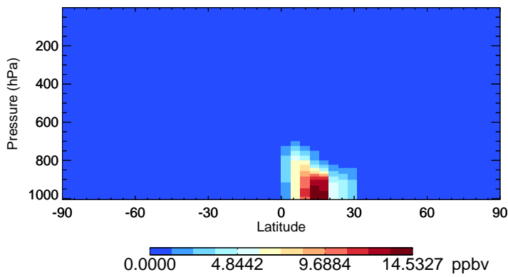
v11-02f-Run1 DST2 - Species Zonal Mean for Jan
