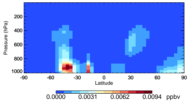
v11-02e-Run0 HAC - Species Curtain @ -180.000 for Jan
