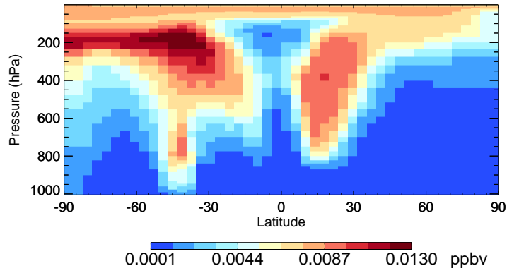
v11-02e-Run1 ISO3 - Species Curtain @ -180.000 for Jan
