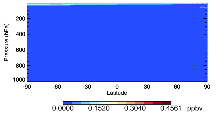
v11-02e-Run1 CIO - Species Curtain @ -180.000 for Jan
