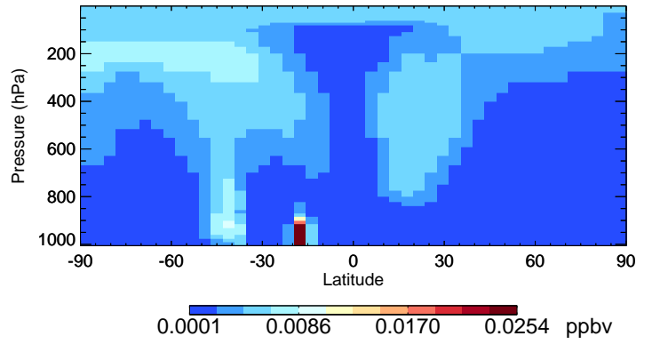
v11-02e-Run1 TSOG3 - Species Curtain @ -180.000 for Jan
