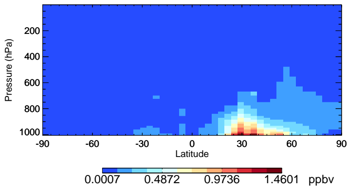
v11-02e-Run1 SO2 - Species Zonal Mean for Jan
