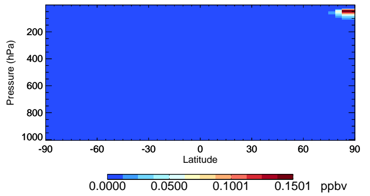
v11-02e-Run1 Cl2O2 - Species Curtain @ -180.000 for Jan
