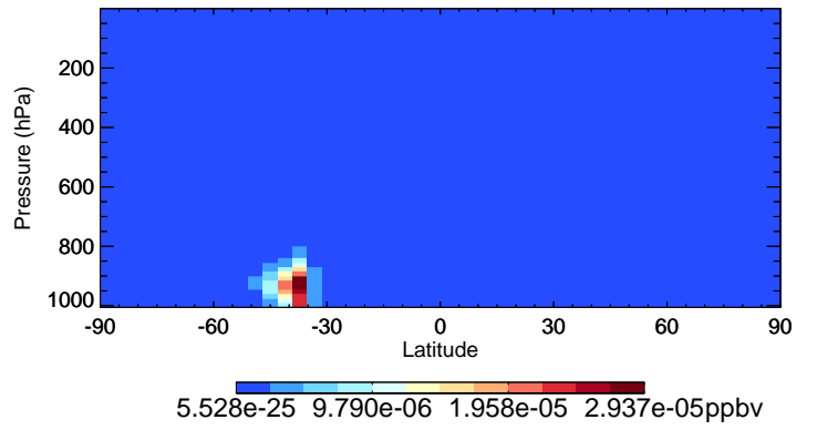
v11-02e-Run0 MACRN - Species Curtain @ -180.000 for Jan
