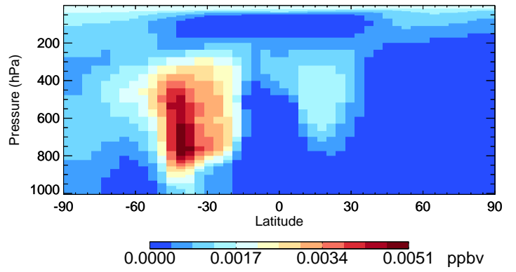
v11-02e-Run0 ISOG1 - Species Curtain @ -180.000 for Jan
