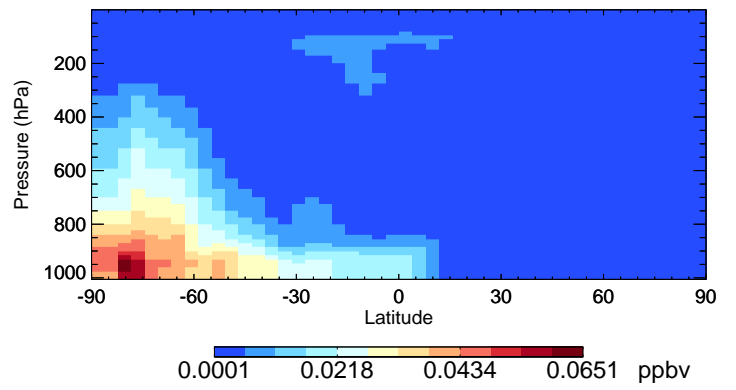
v11-02e-Run1 MSA - Species Curtain @ -180.000 for Jan
