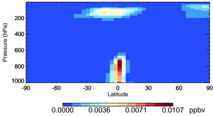
v11-02e-Run1 ISOA3 - Species Zonal Mean for Jan
