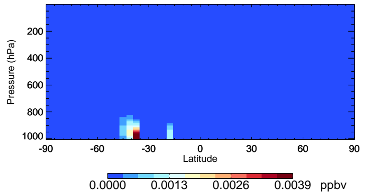
v11-02f-Run1 RIPA - Species Curtain @ -180.000 for Jan
