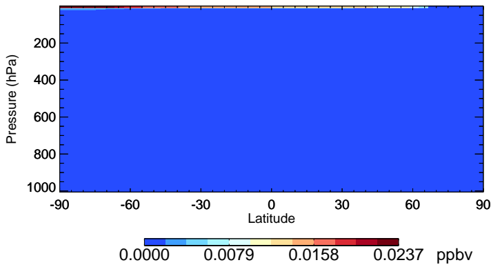
v11-02f-Run1 Br - Species Zonal Mean for Jan
