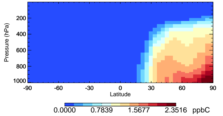
v11-02e-Run1 ALK4 - Species Curtain @ -180.000 for Jan
