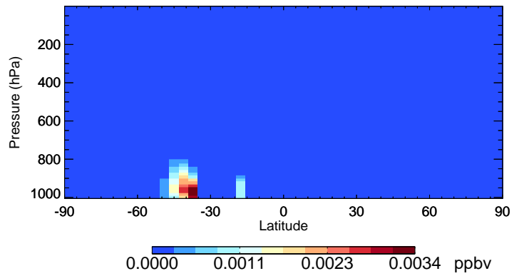
v11-02f-Run1 IEPOXB - Species Curtain @ -180.000 for Jan
