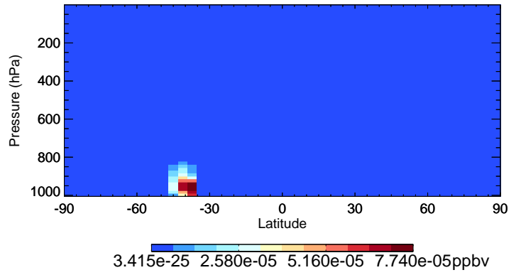
v11-02e-Run1 ISN1 - Species Curtain @ -180.000 for Jan
