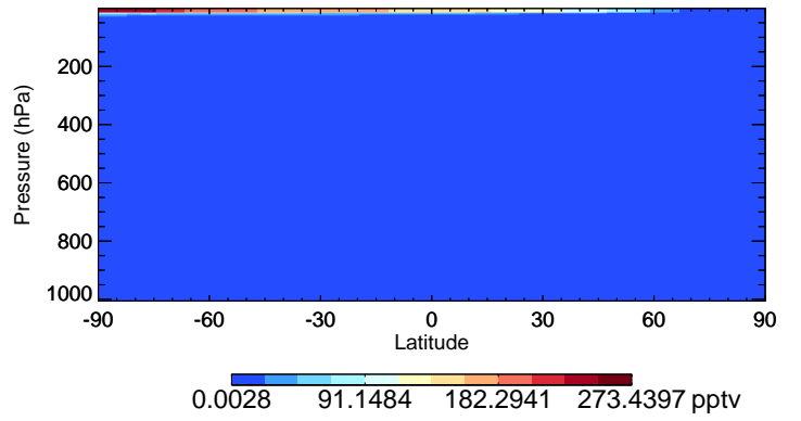
v11-02e-Run0 HO2 - Species Curtain @ -180.000 for Jan
