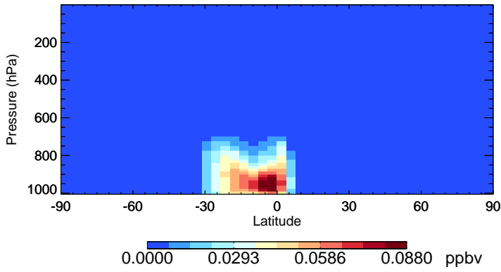
v11-02e-Run1 RIPA - Species Zonal Mean for Jan
