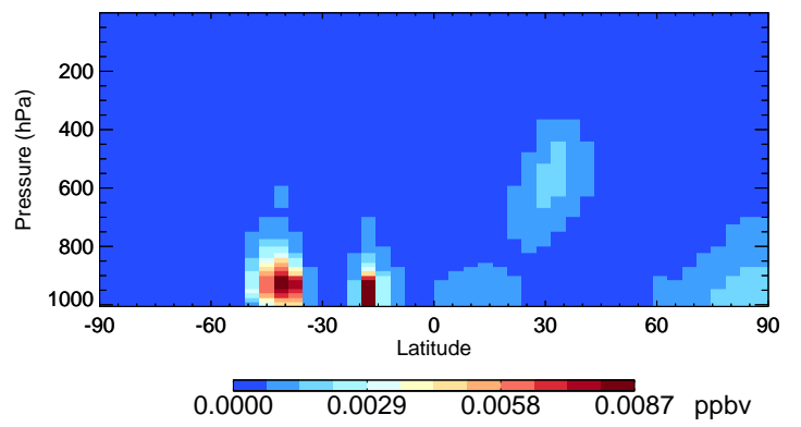
v11-02e-Run1 HAC - Species Curtain @ -180.000 for Jan
