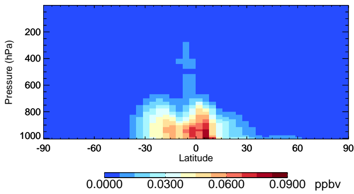
v11-02f-Run1 HAC - Species Zonal Mean for Jan
