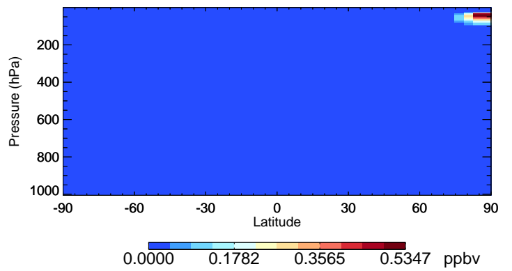
v11-02f-Run1 Cl2O2 - Species Curtain @ -180.000 for Jan
