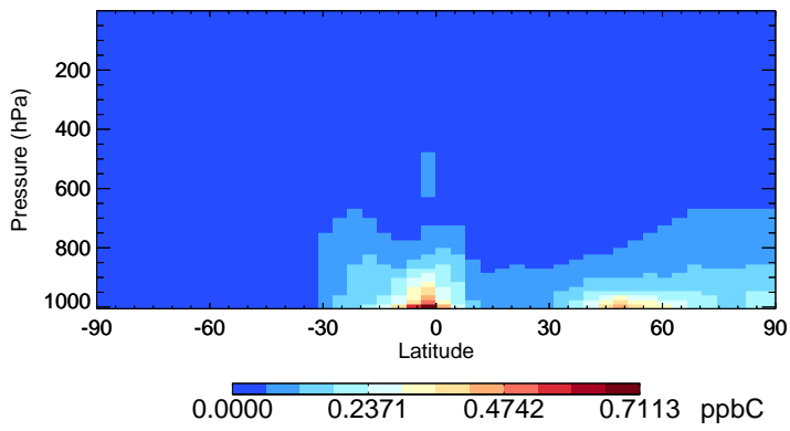
v11-02e-Run0 EOH - Species Zonal Mean for Jan
