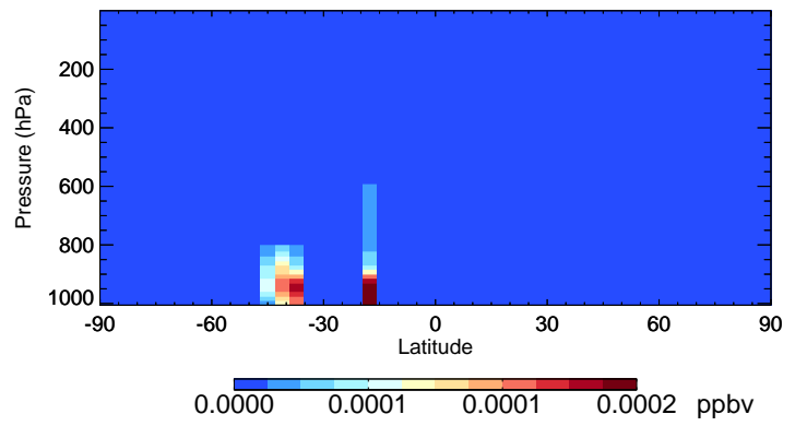
v11-02e-Run1 MONITS - Species Curtain @ -180.000 for Jan
