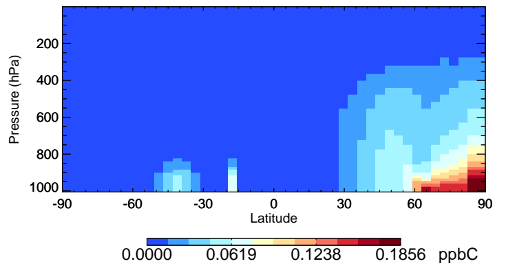
v11-02e-Run0 EOH - Species Curtain @ -180.000 for Jan
