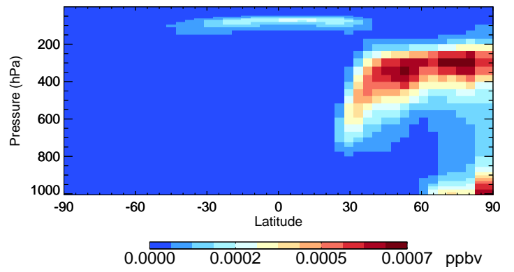
v11-02e-Run0 ASOA2 - Species Curtain @ -180.000 for Jan
