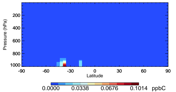
v11-02f-Run1 ISOP - Species Curtain @ -180.000 for Jan
