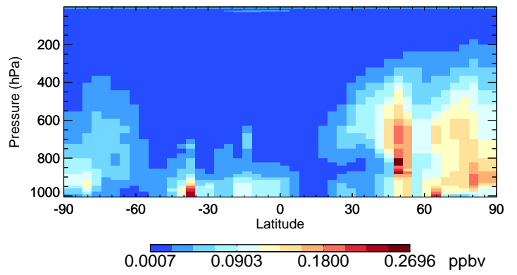
v11-02e-Run1 SO2 - Species Curtain @ -180.000 for Jan
