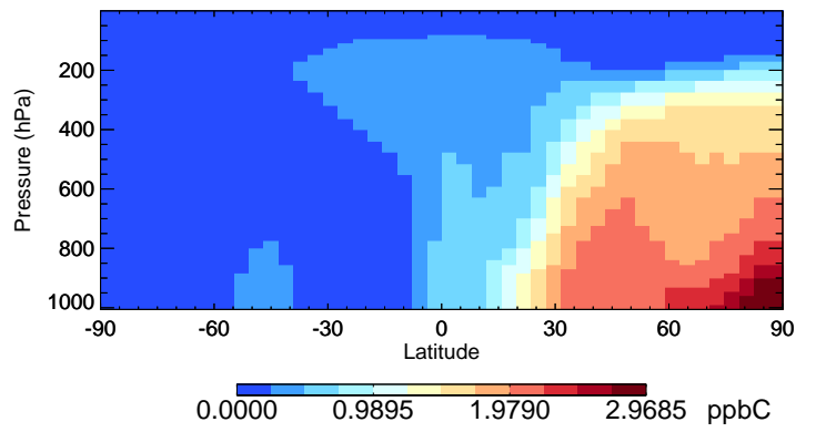
v11-02e-Run1 C2H6 - Species Curtain @ -180.000 for Jan
