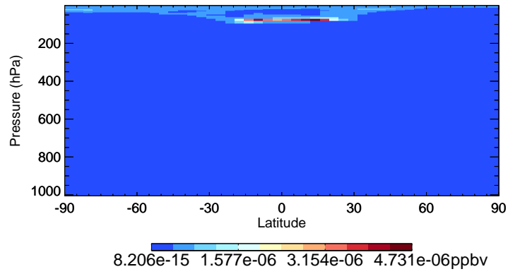
v11-02e-Run0 CIOO - Species Curtain @ -180.000 for Jan
