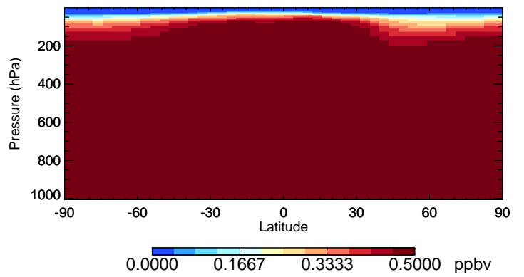
v11-02f-Run1 OCS - Species Curtain @ -180.000 for Jan
