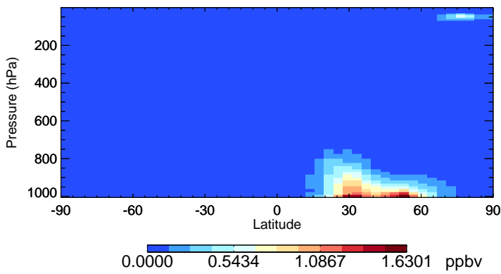
v11-02f-Run1 NIT - Species Zonal Mean for Jan
