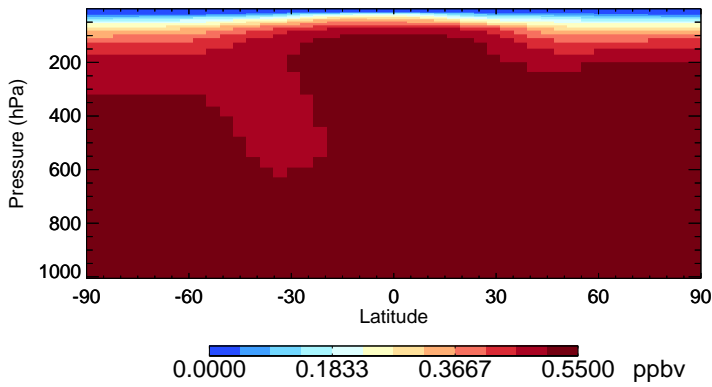
v11-02f-Run1 CH3Cl - Species Zonal Mean for Jan
