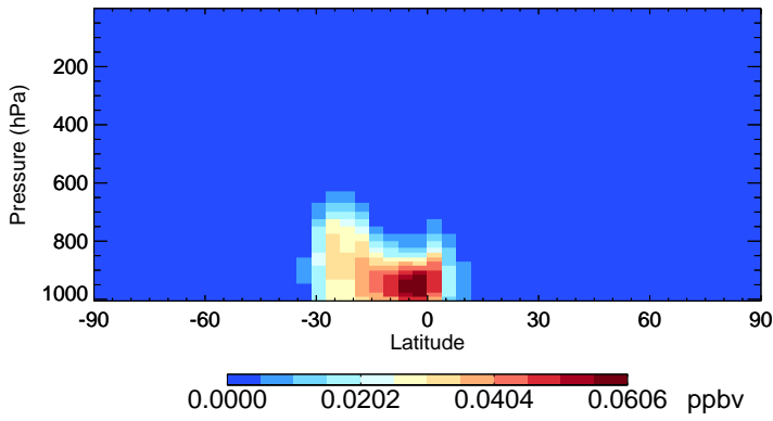
v11-02e-Run0 RIPA - Species Zonal Mean for Jan
