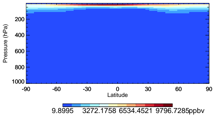
v11-02f-Run1 O3 - Species Zonal Mean for Jan
