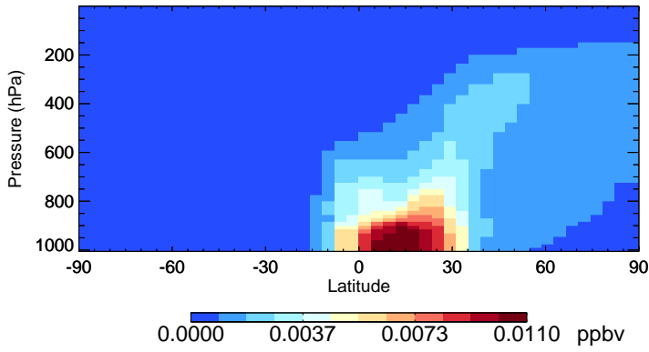
v11-02e-Run1 ASOAN - Species Zonal Mean for Jan
