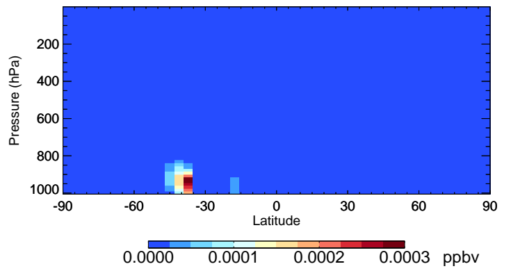
v11-02e-Run1 ISOPNB - Species Curtain @ -180.000 for Jan
