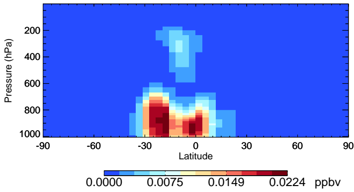
v11-02e-Run0 IEPOXB - Species Zonal Mean for Jan
