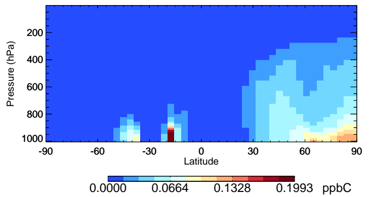
v11-02f-Run1 EOH - Species Curtain @ -180.000 for Jan
