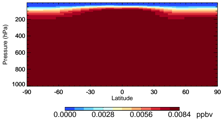
v11-02f-Run1 CH3CCI3 - Species Zonal Mean for Jan
