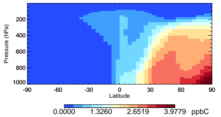
v11-02f-Run1 C2H6 - Species Curtain @ -180.000 for Jan
