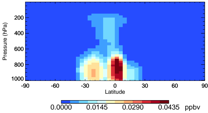
v11-02e-Run1 IMAE - Species Zonal Mean for Jan
