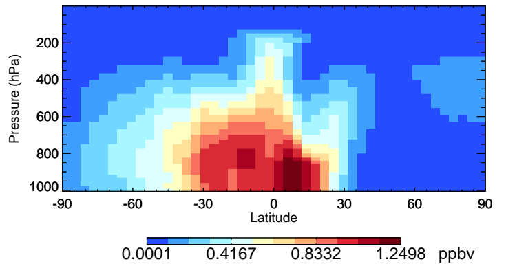
v11-02f-Run1 MP - Species Curtain @ -180.000 for Jan
