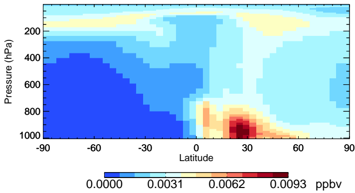
v11-02f-Run1 ASOG3 - Species Zonal Mean for Jan
