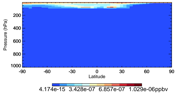
v11-02e-Run1 CIOO - Species Curtain @ -180.000 for Jan
