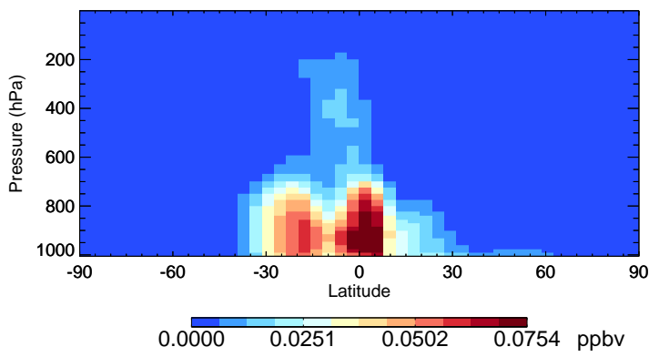
v11-02e-Run1 HAC - Species Zonal Mean for Jan
