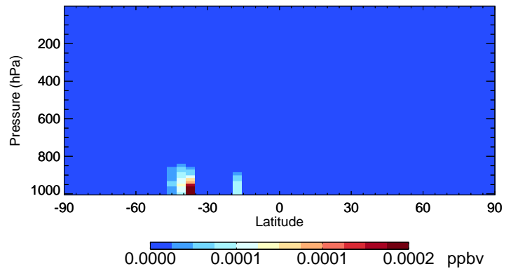
v11-02f-Run1 RIPD - Species Curtain @ -180.000 for Jan
