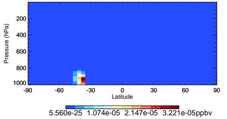
v11-02e-Run1 MACRN - Species Curtain @ -180.000 for Jan
