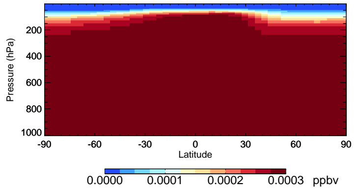
v11-02e-Run0 H2402 - Species Curtain @ -180.000 for Jan
