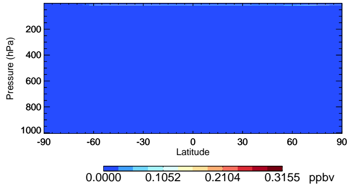
v11-02e-Run1 NO3 - Species Curtain @ -180.000 for Jan
