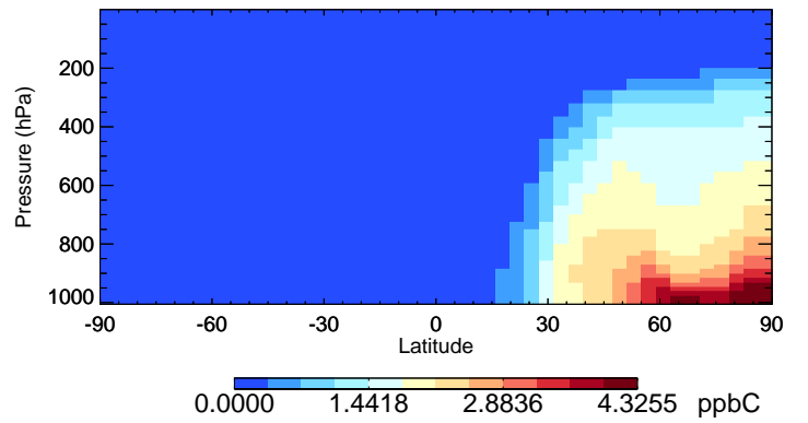
v11-02f-Run1 ALK4 - Species Curtain @ -180.000 for Jan
