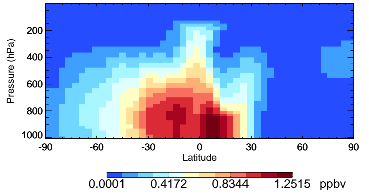
v11-02e-Run1 MP - Species Curtain @ -180.000 for Jan
