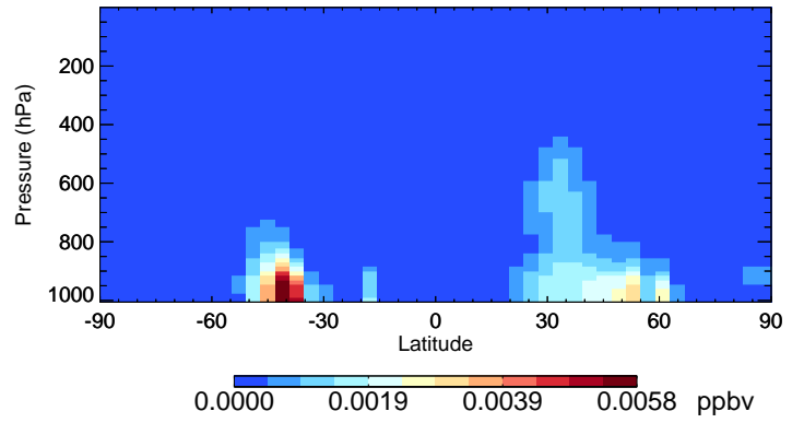
v11-02e-Run1 BCPO - Species Curtain @ -180.000 for Jan
