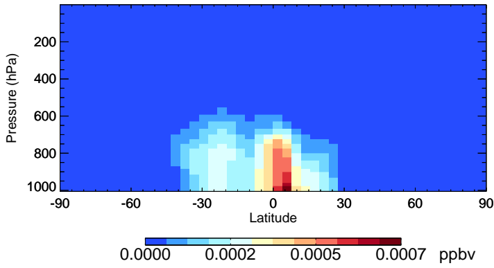
v11-02e-Run1 ISN10A - Species Zonal Mean for Jan
