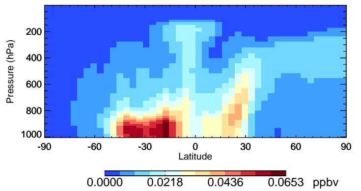
v11-02f-Run1 MAP - Species Curtain @ -180.000 for Jan
