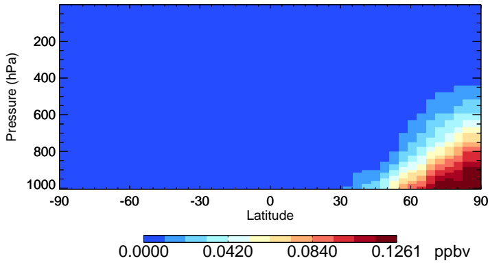
v11-02e-Run1 ClNO 2 - Species Zonal Mean for Jan
