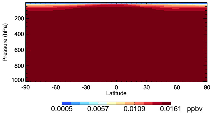
v11-02f-Run1 CFC114 - Species Zonal Mean for Jan
