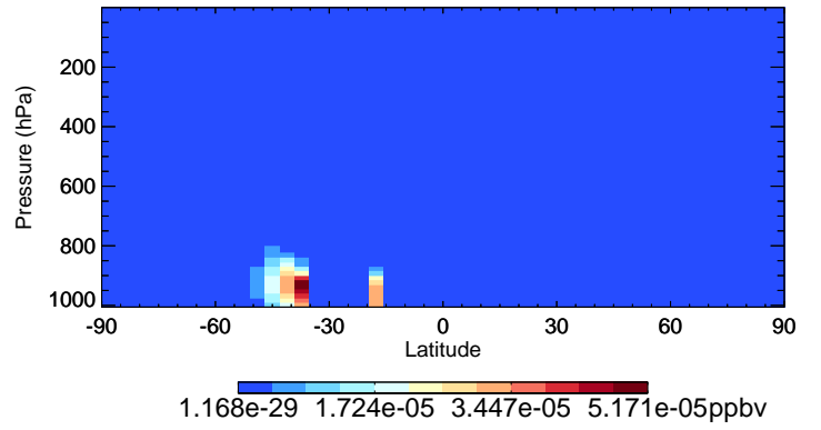
v11-02e-Run1 RIPD - Species Curtain @ -180.000 for Jan
