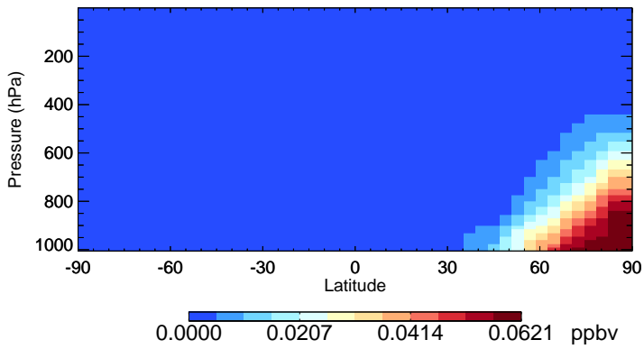
v11-02f-Run1 ClNO 2 - Species Zonal Mean for Jan
