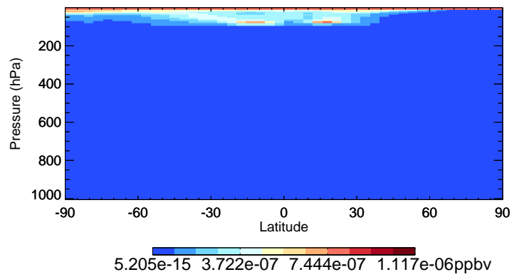
v11-02f-Run1 CIOO - Species Curtain @ -180.000 for Jan
