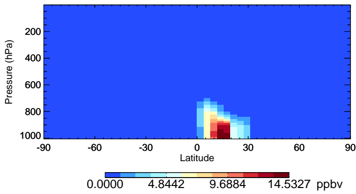
v11-02e-Run1 DST2 - Species Zonal Mean for Jan
