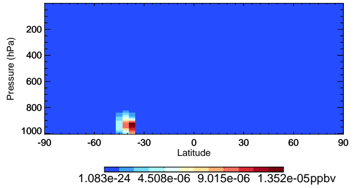
v11-02e-Run1 ETHLN - Species Curtain @ -180.000 for Jan
