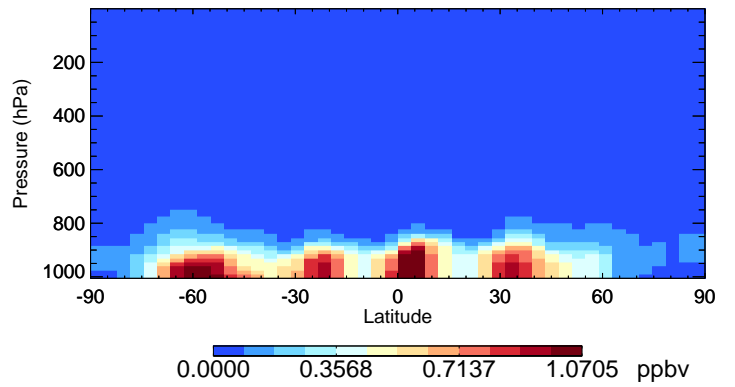
v11-02f-Run1 SALA - Species Curtain @ -180.000 for Jan
