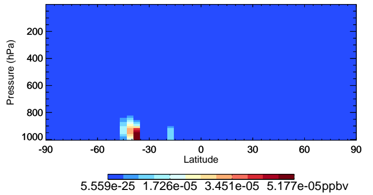
v11-02f-Run1 MACRN - Species Curtain @ -180.000 for Jan
