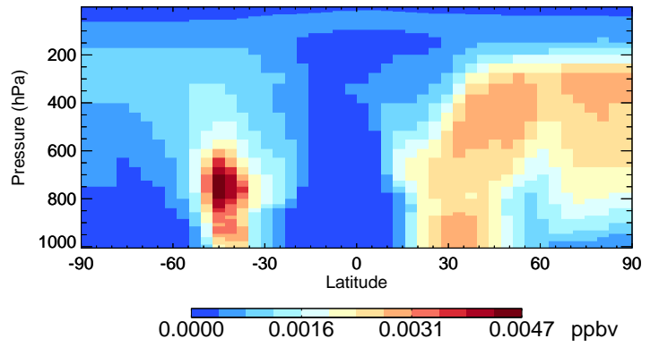
v11-02e-Run0 IONITA - Species Curtain @ -180.000 for Jan
