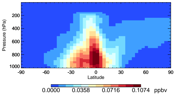
v11-02e-Run1 MAP - Species Zonal Mean for Jan
