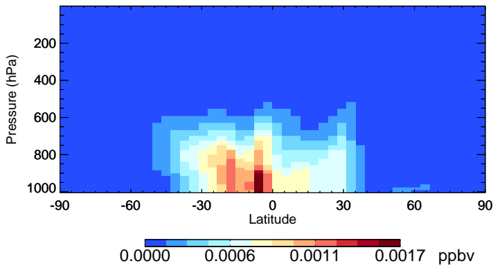
v11-02f-Run1 SOAME - Species Zonal Mean for Jan
