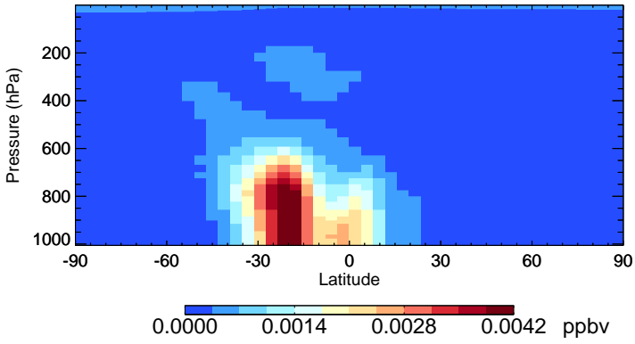
v11-02e-Run0 LVOCOA - Species Zonal Mean for Jan
