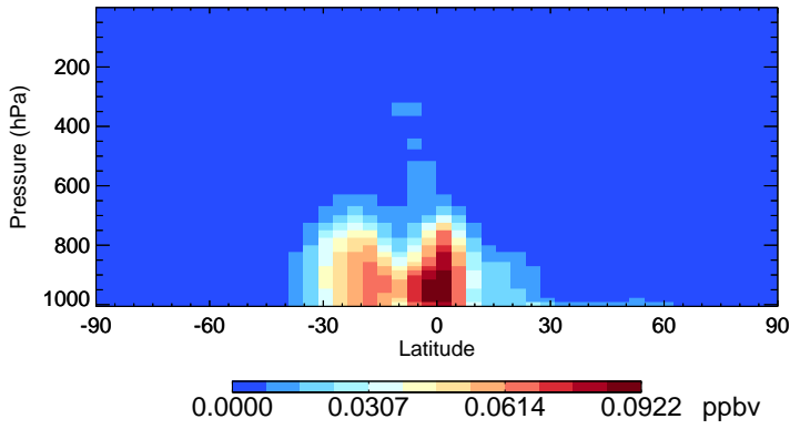
v11-02e-Run1 GLYC - Species Zonal Mean for Jan
