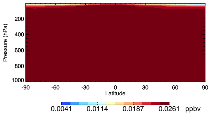
v11-02f-Run1 HCFC142b - Species Zonal Mean for Jan
