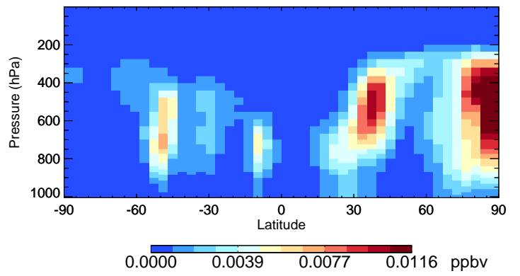
v11-02e-Run1 DST2 - Species Curtain @ -180.000 for Jan
