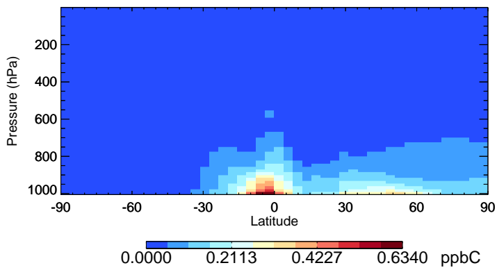
v11-02f-Run1 EOH - Species Zonal Mean for Jan
