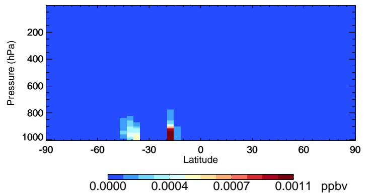
v11-02f-Run1 MONITS - Species Curtain @ -180.000 for Jan
