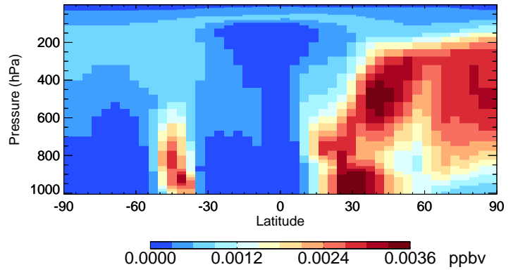
v11-02e-Run1 IONITA - Species Curtain @ -180.000 for Jan
