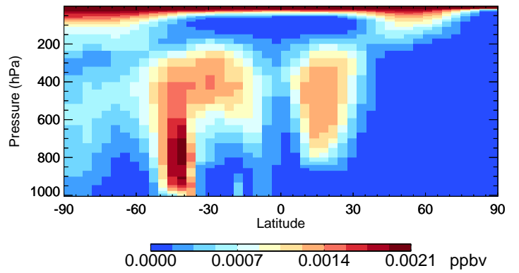
v11-02f-Run1 ISOG1 - Species Curtain @ -180.000 for Jan
