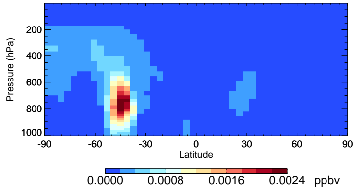
v11-02e-Run1 SOAME - Species Curtain @ -180.000 for Jan
