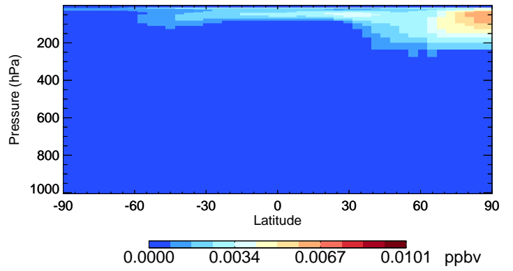
v11-02e-Run0 HOBr - Species Curtain @ -180.000 for Jan
