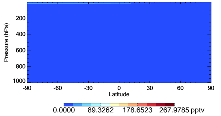
v11-02e-Run1 HO2 - Species Curtain @ -180.000 for Jan
