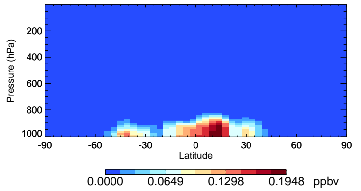
v11-02e-Run1 NH3 - Species Curtain @ -180.000 for Jan
