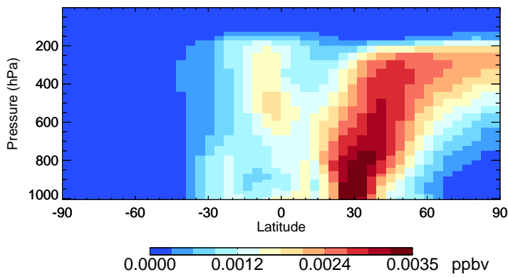
v11-02f-Run1 R4N2 - Species Zonal Mean for Jan
