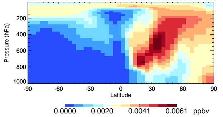
v11-02e-Run1 ASOG3 - Species Curtain @ -180.000 for Jan
