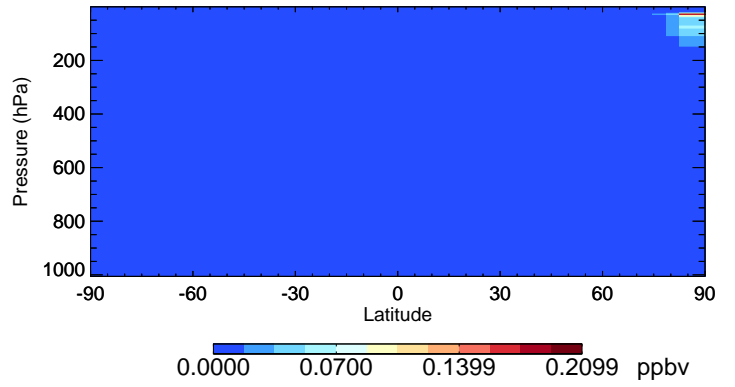
v11-02e-Run1 Cl2 - Species Curtain @ -180.000 for Jan
