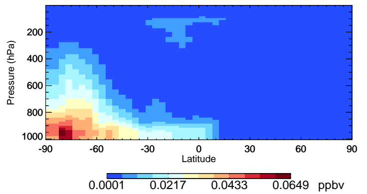
v11-02f-Run1 MSA - Species Curtain @ -180.000 for Jan
