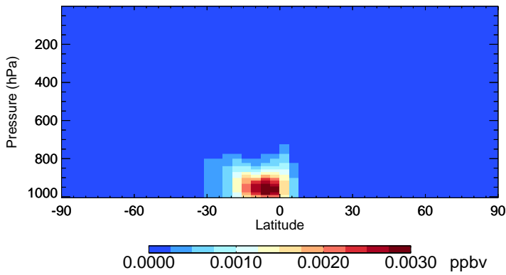
v11-02f-Run1 RIPD - Species Zonal Mean for Jan
