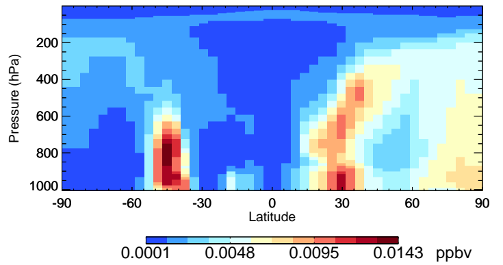
v11-02f-Run1 INDIOL - Species Curtain @ -180.000 for Jan
