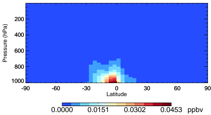
v11-02f-Run1 TSOA0 - Species Zonal Mean for Jan
