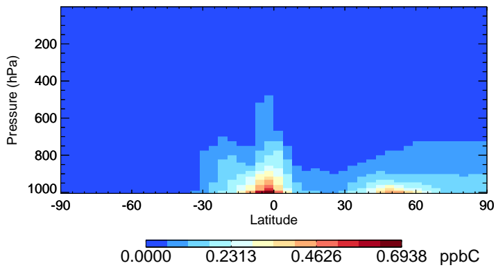
v11-02e-Run1 EOH - Species Zonal Mean for Jan
