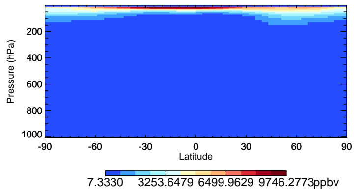
v11-02f-Run1 O3 - Species Curtain @ -180.000 for Jan
