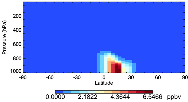
v11-02e-Run1 DST1 - Species Zonal Mean for Jan
