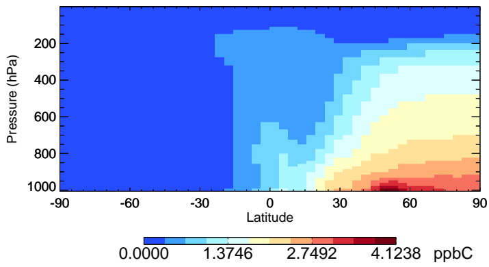
v11-02e-Run1 C2H6 - Species Zonal Mean for Jan
