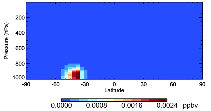
v11-02e-Run0 IPMN - Species Curtain @ -180.000 for Jan
