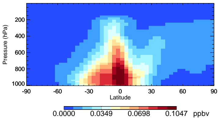
v11-02f-Run1 MAP - Species Zonal Mean for Jan
