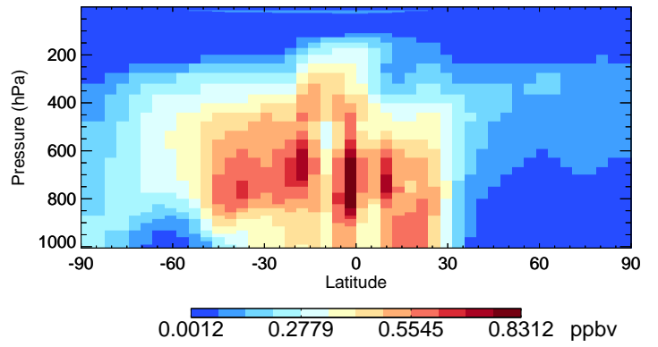
v11-02e-Run0 H2O2 - Species Curtain @ -180.000 for Jan
