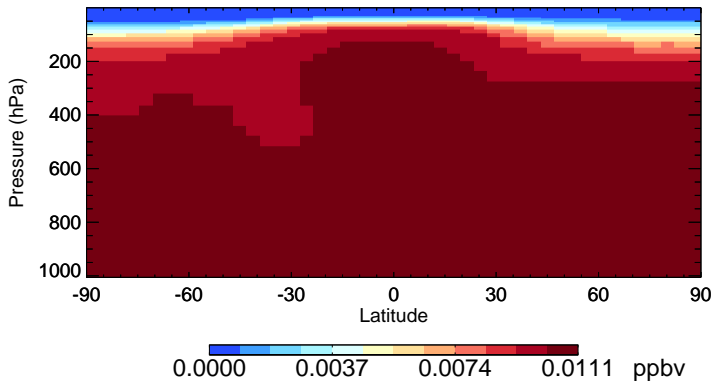
v11-02e-Run0 CH3CCI3 - Species Zonal Mean for Jan
