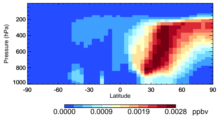
v11-02f-Run1 R4N2 - Species Curtain @ -180.000 for Jan
