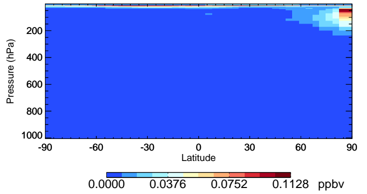
v11-02e-Run0 HOCl - Species Curtain @ -180.000 for Jan
