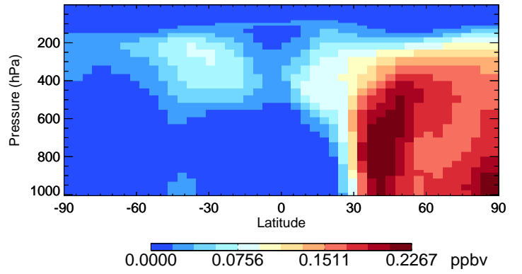
v11-02e-Run1 PAN - Species Curtain @ -180.000 for Jan
