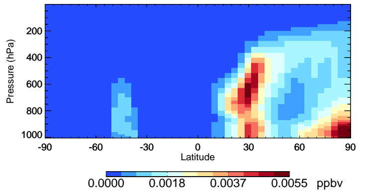
v11-02f-Run1 SOAGX - Species Curtain @ -180.000 for Jan
