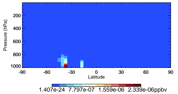
v11-02f-Run1 LVOC - Species Curtain @ -180.000 for Jan
