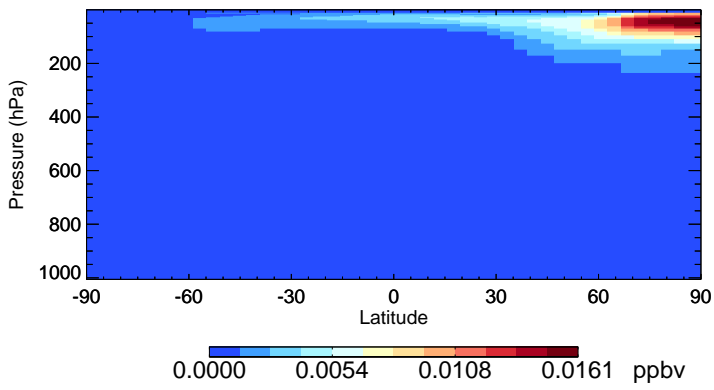
v11-02e-Run1 BrCl - Species Zonal Mean for Jan
