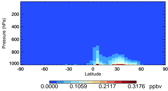
v11-02e-Run1 BCPO - Species Zonal Mean for Jan
