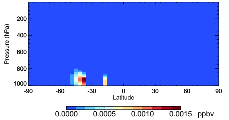
v11-02e-Run1 RIPA - Species Curtain @ -180.000 for Jan
