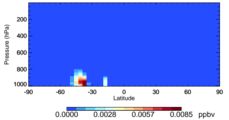
v11-02f-Run1 IEPOXA - Species Curtain @ -180.000 for Jan
