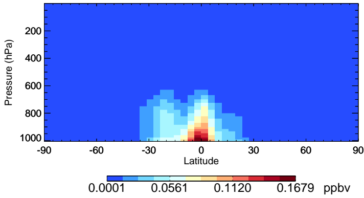
v11-02e-Run1 TSOG3 - Species Zonal Mean for Jan
