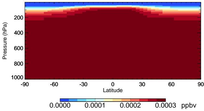
v11-02e-Run0 H2402 - Species Zonal Mean for Jan
