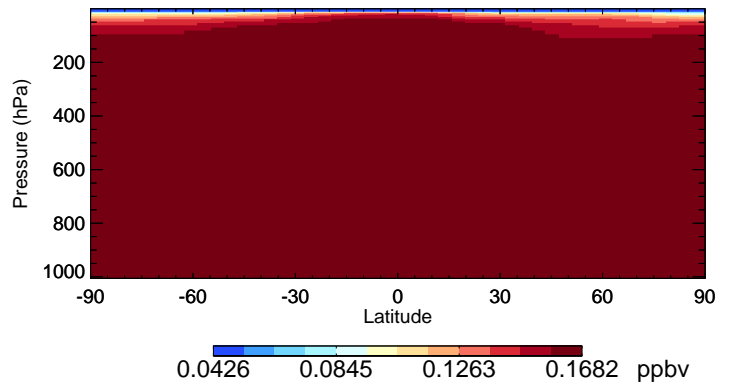
v11-02f-Run1 HCFC22 - Species Curtain @ -180.000 for Jan
