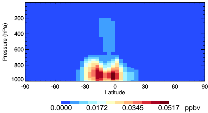
v11-02f-Run1 IEPOXA - Species Zonal Mean for Jan
