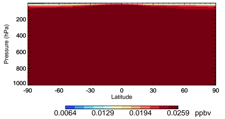
v11-02e-Run0 HCFC142b - Species Curtain @ -180.000 for Jan
