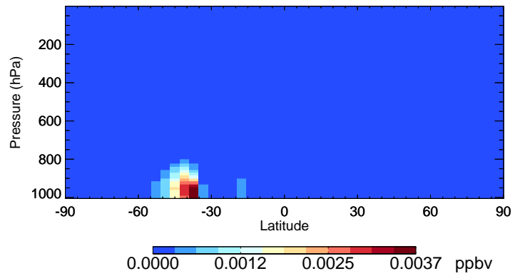
v11-02f-Run1 IPMN - Species Curtain @ -180.000 for Jan
