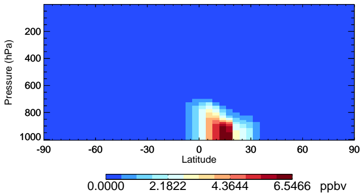
v11-02f-Run1 DST1 - Species Zonal Mean for Jan
