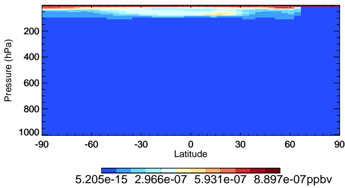
v11-02f-Run1 CIOO - Species Zonal Mean for Jan
