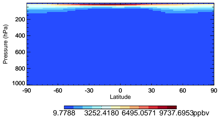
v11-02e-Run1 O3 - Species Zonal Mean for Jan
