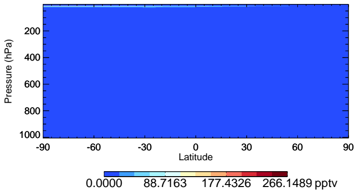
v11-02f-Run1 HO2 - Species Zonal Mean for Jan
