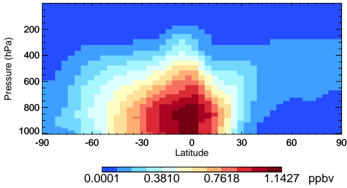
v11-02e-Run1 MP - Species Zonal Mean for Jan
