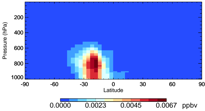
v11-02e-Run1 SOAME - Species Zonal Mean for Jan
