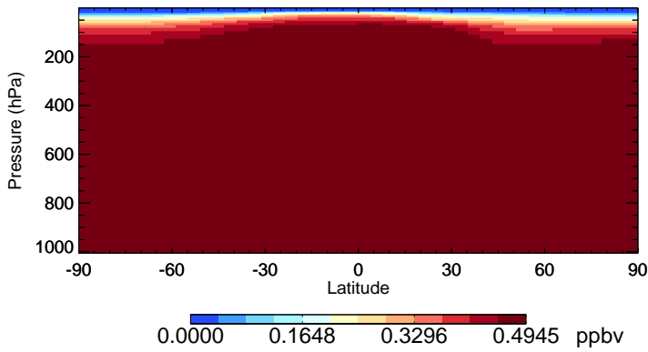
v11-02f-Run1 CFC12 - Species Zonal Mean for Jan
