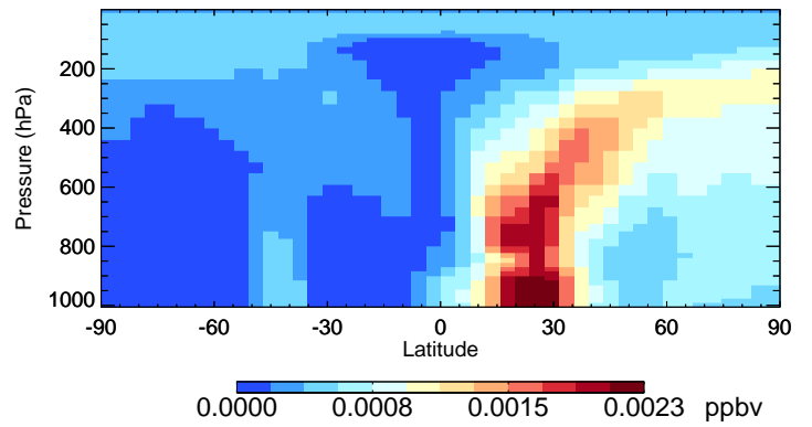
v11-02f-Run1 ASOAN - Species Curtain @ -180.000 for Jan
