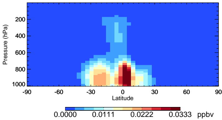
v11-02f-Run1 IMAE - Species Zonal Mean for Jan
