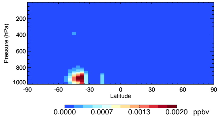
v11-02e-Run0 IEPOXB - Species Curtain @ -180.000 for Jan
