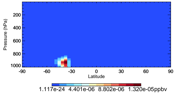
v11-02e-Run0 ETHLN - Species Curtain @ -180.000 for Jan
