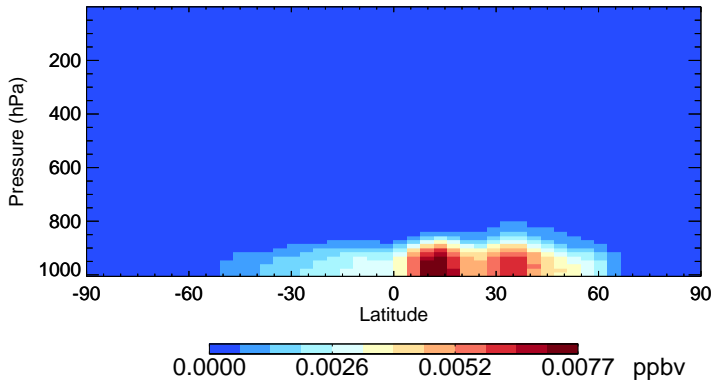
v11-02e-Run1 NITs - Species Zonal Mean for Jan
