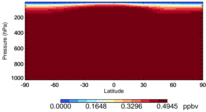
v11-02e-Run1 CFC12 - Species Zonal Mean for Jan
