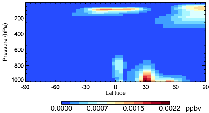
v11-02f-Run1 ASOA3 - Species Zonal Mean for Jan
