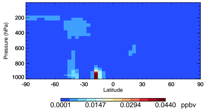
v11-02f-Run1 TSOG2 - Species Curtain @ -180.000 for Jan
