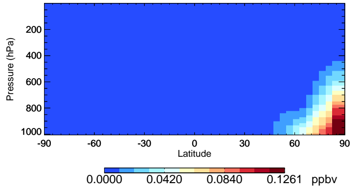
v11-02e-Run1 ClNO 2 - Species Curtain @ -180.000 for Jan
