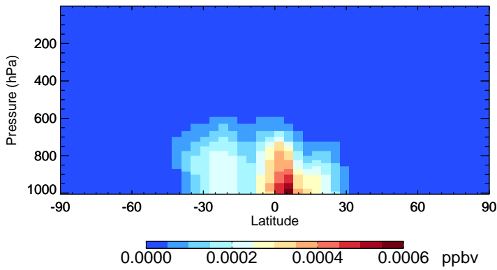
v11-02f-Run1 ISN10A - Species Zonal Mean for Jan
