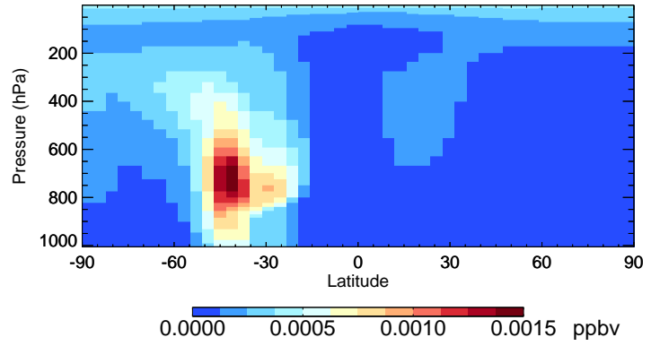
v11-02e-Run0 LVOCOA - Species Curtain @ -180.000 for Jan
