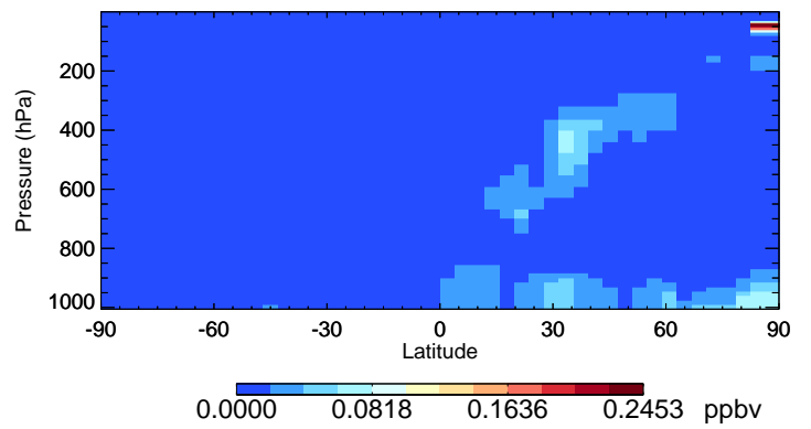
v11-02f-Run1 NIT - Species Curtain @ -180.000 for Jan
