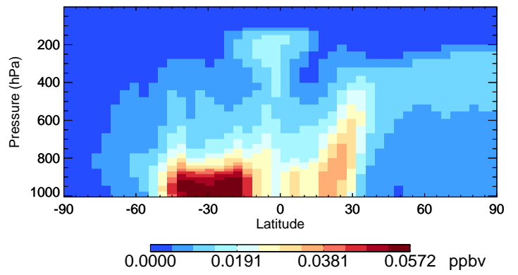
v11-02e-Run1 MAP - Species Curtain @ -180.000 for Jan
