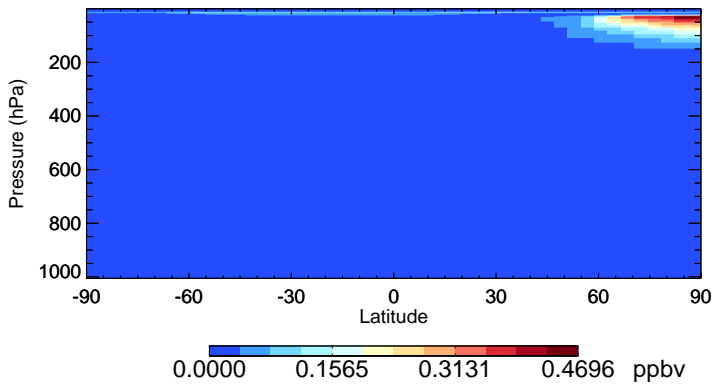
v11-02f-Run1 HOCl - Species Zonal Mean for Jan
