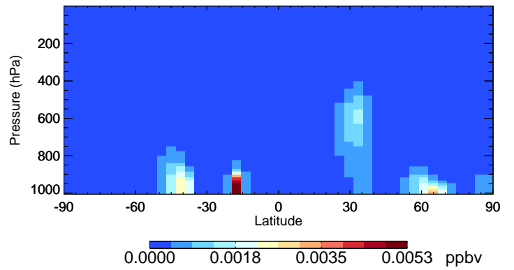
v11-02f-Run1 BCPO - Species Curtain @ -180.000 for Jan
