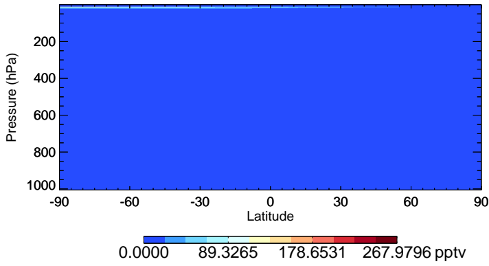
v11-02e-Run1 HO2 - Species Zonal Mean for Jan
