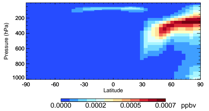
v11-02e-Run1 ASOA2 - Species Curtain @ -180.000 for Jan
