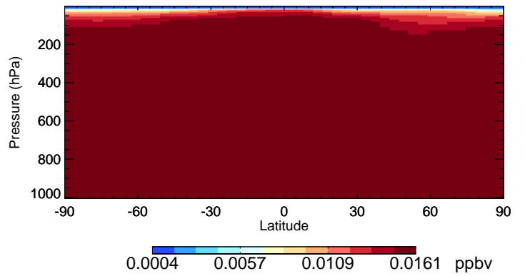
v11-02f-Run1 CFC114 - Species Curtain @ -180.000 for Jan
