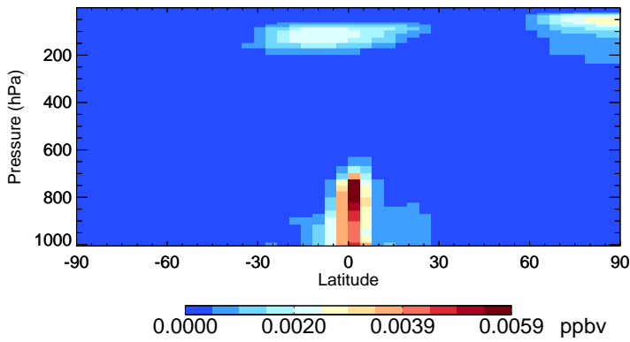
v11-02f-Run1 ISOA3 - Species Zonal Mean for Jan
