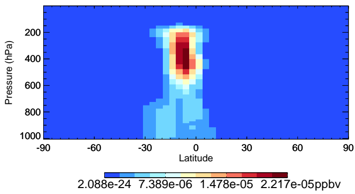
v11-02e-Run1 LVOC - Species Zonal Mean for Jan
