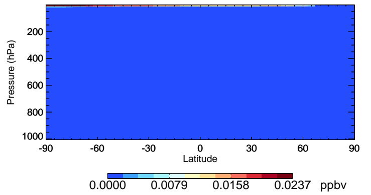
v11-02e-Run1 Br - Species Curtain @ -180.000 for Jan
