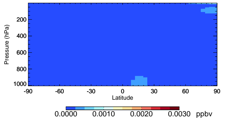
v11-02e-Run1 Br2 - Species Curtain @ -180.000 for Jan
