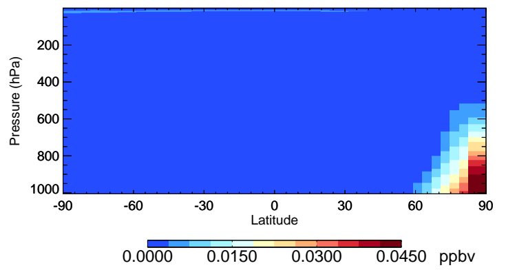
v11-02e-Run1 HNO 2 - Species Curtain @ -180.000 for Jan
