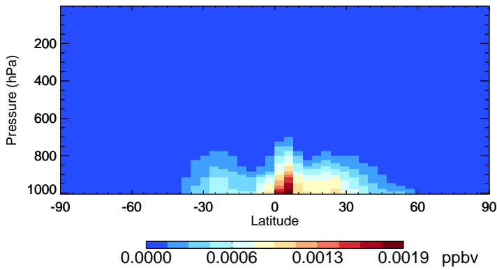
v11-02f-Run1 IONITA - Species Zonal Mean for Jan
