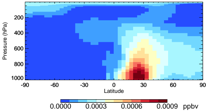
v11-02e-Run1 ASOG1 - Species Zonal Mean for Jan
