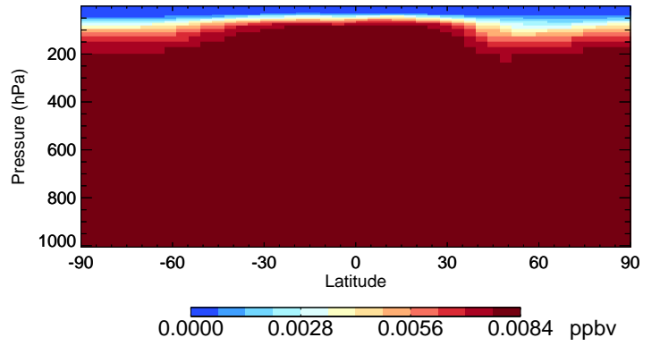
v11-02e-Run1 CH3CCI3 - Species Curtain @ -180.000 for Jan
