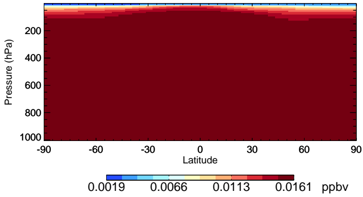
v11-02e-Run1 CFC114 - Species Zonal Mean for Jan
