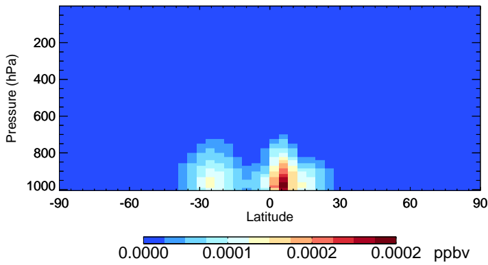
v11-02f-Run1 ETHLN - Species Zonal Mean for Jan
