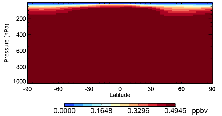
v11-02f-Run1 CFC12 - Species Curtain @ -180.000 for Jan
