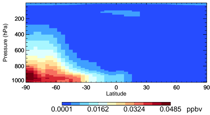
v11-02e-Run1 MSA - Species Zonal Mean for Jan
