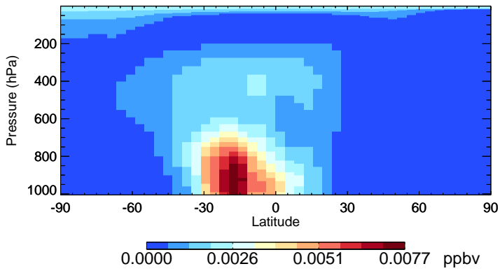
v11-02f-Run1 ISOG1 - Species Zonal Mean for Jan
