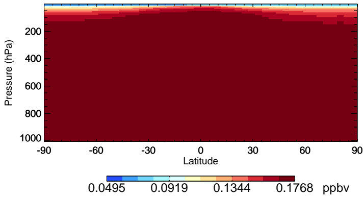
v11-02e-Run0 HCFC22 - Species Zonal Mean for Jan
