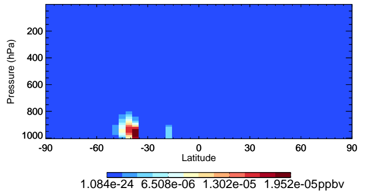
v11-02f-Run1 ETHLN - Species Curtain @ -180.000 for Jan
