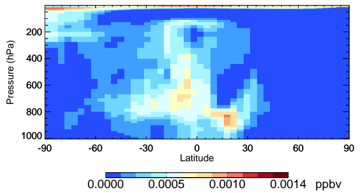
v11-02f-Run1 HBr - Species Curtain @ -180.000 for Jan
