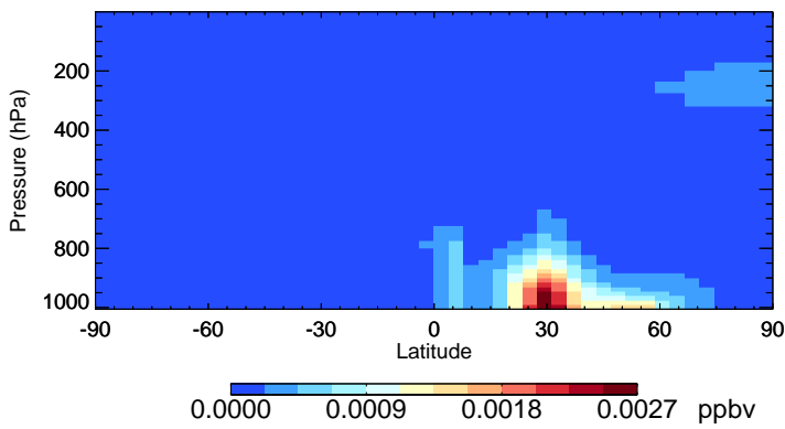
v11-02f-Run1 ASOA2 - Species Zonal Mean for Jan
