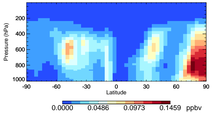
v11-02f-Run1 DST1 - Species Curtain @ -180.000 for Jan
