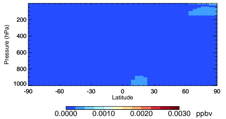
v11-02f-Run1 Br2 - Species Curtain @ -180.000 for Jan
