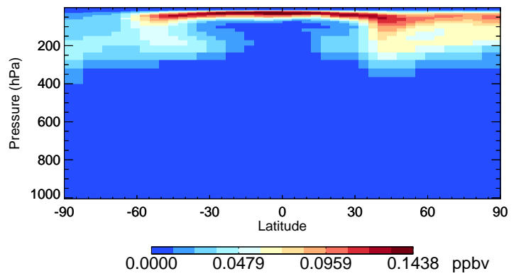
v11-02f-Run1 MPN - Species Curtain @ -180.000 for Jan
