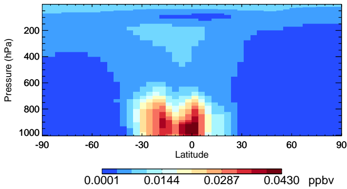
v11-02f-Run1 ISO3 - Species Zonal Mean for Jan
