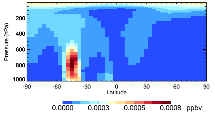
v11-02f-Run1 LVOCOA - Species Curtain @ -180.000 for Jan
