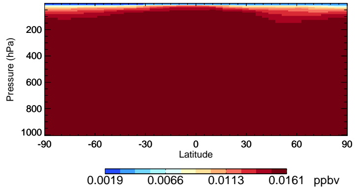
v11-02e-Run1 CFC114 - Species Curtain @ -180.000 for Jan
