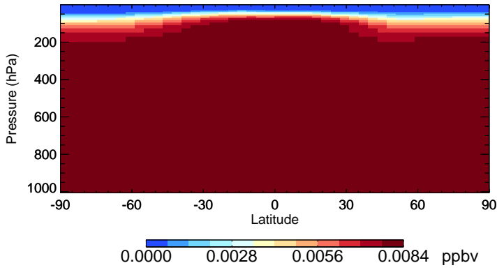
v11-02e-Run1 CH3CCI3 - Species Zonal Mean for Jan
