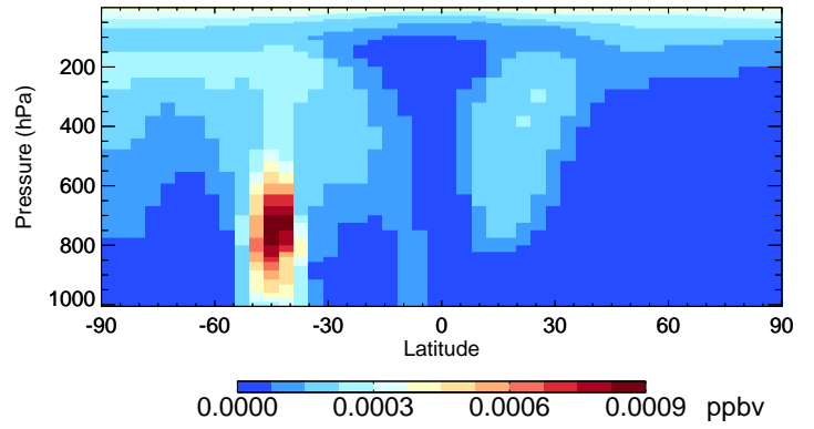
v11-02e-Run1 LVOCOA - Species Curtain @ -180.000 for Jan
