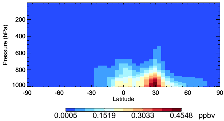
v11-02f-Run1 SOAS - Species Zonal Mean for Jan
