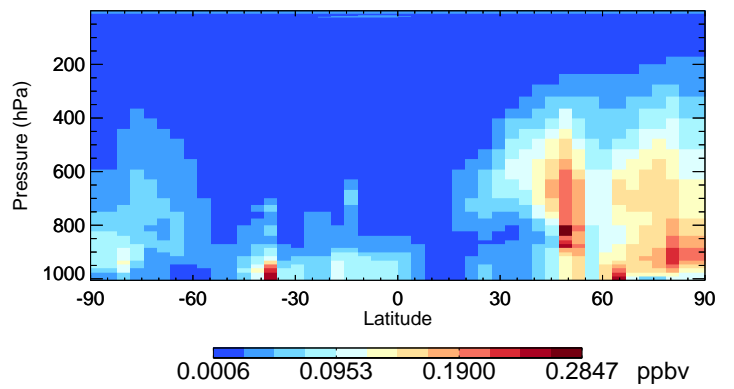
v11-02f-Run1 SO2 - Species Curtain @ -180.000 for Jan
