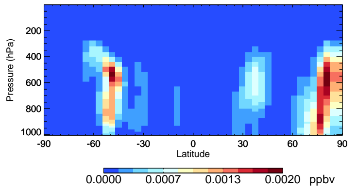
v11-02e-Run1 DST4 - Species Curtain @ -180.000 for Jan
