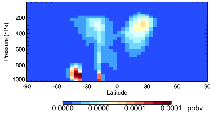
v11-02e-Run1 HONIT - Species Curtain @ -180.000 for Jan
