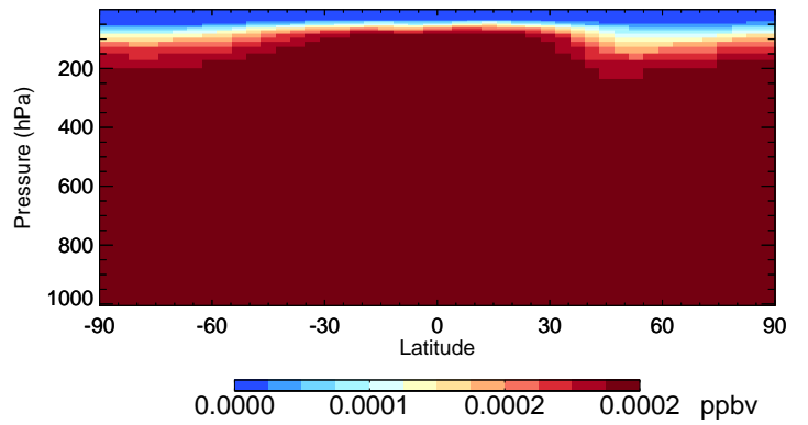
v11-02f-Run1 H2402 - Species Curtain @ -180.000 for Jan
