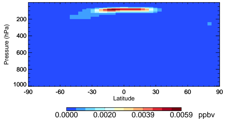
v11-02e-Run0 ISOA3 - Species Curtain @ -180.000 for Jan
