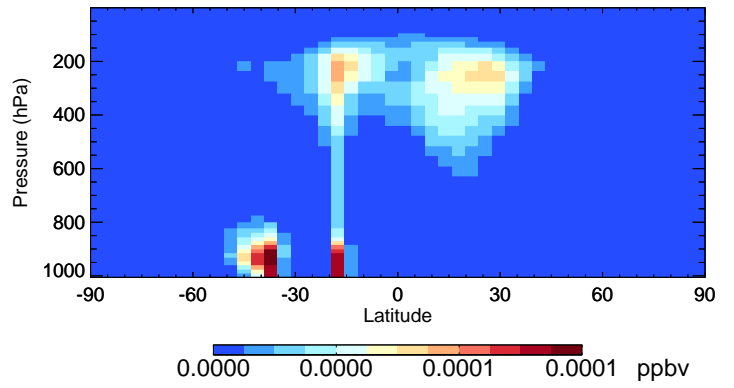
v11-02e-Run0 HONIT - Species Curtain @ -180.000 for Jan
