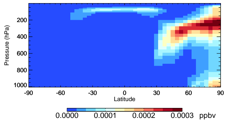
v11-02f-Run1 ASOA2 - Species Curtain @ -180.000 for Jan
