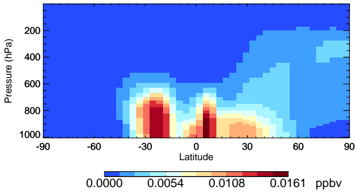
v11-02e-Run0 IONITA - Species Zonal Mean for Jan
