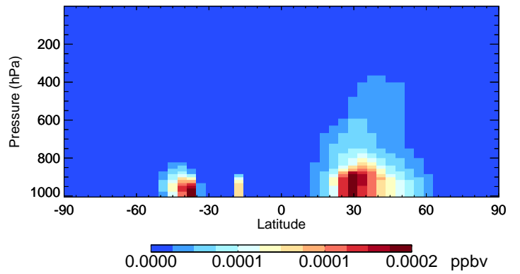
v11-02f-Run1 IONITA - Species Curtain @ -180.000 for Jan
