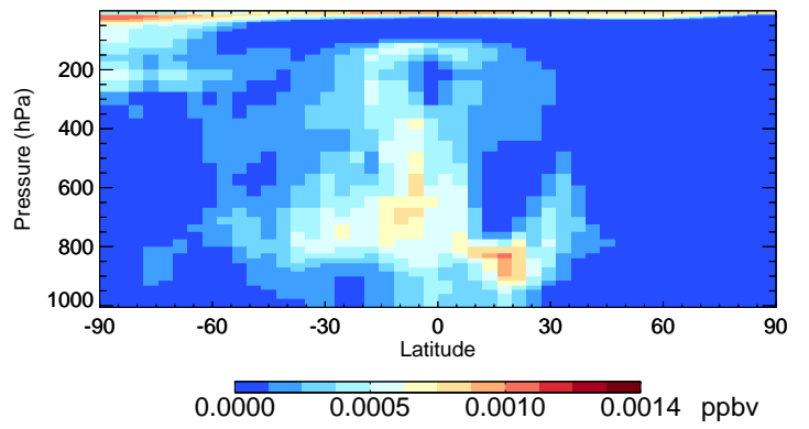
v11-02e-Run1 HBr - Species Curtain @ -180.000 for Jan
