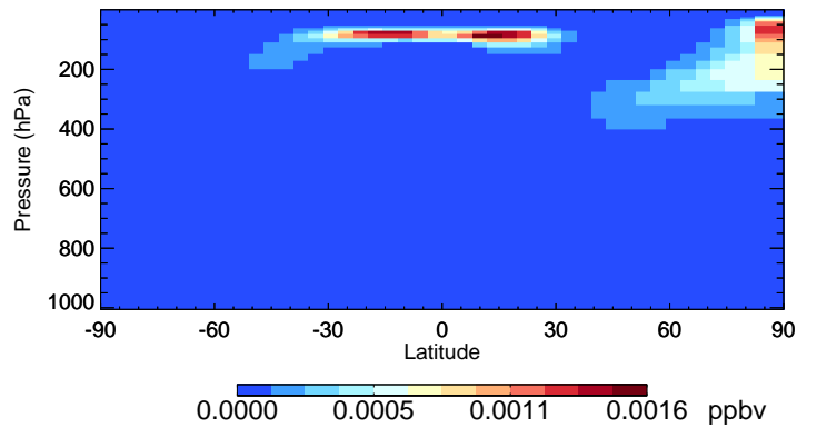
v11-02f-Run1 ASOA3 - Species Curtain @ -180.000 for Jan
