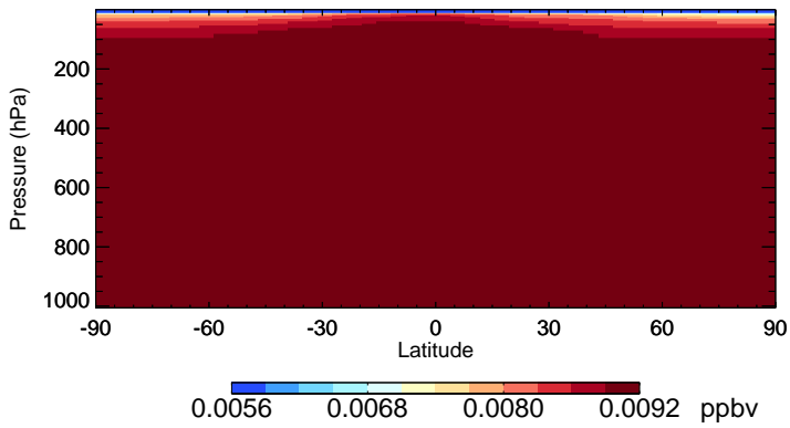
v11-02f-Run1 CFC115 - Species Zonal Mean for Jan
