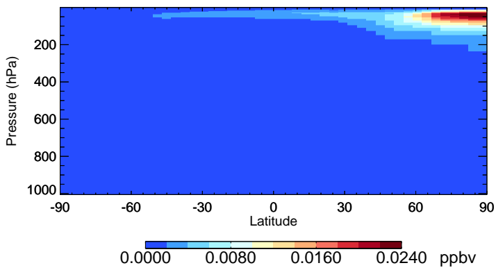
v11-02f-Run1 BrCl - Species Zonal Mean for Jan
