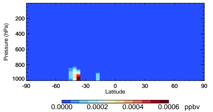
v11-02f-Run1 ISOPNB - Species Curtain @ -180.000 for Jan
