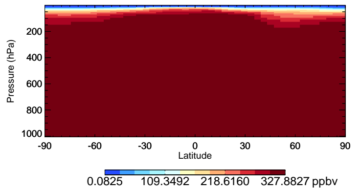
v11-02f-Run1 N2O - Species Curtain @ -180.000 for Jan
