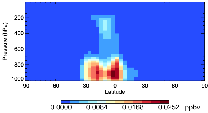
v11-02e-Run1 IEPOXB - Species Zonal Mean for Jan
