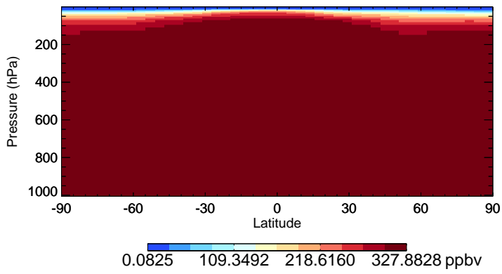
v11-02e-Run1 N2O - Species Zonal Mean for Jan
