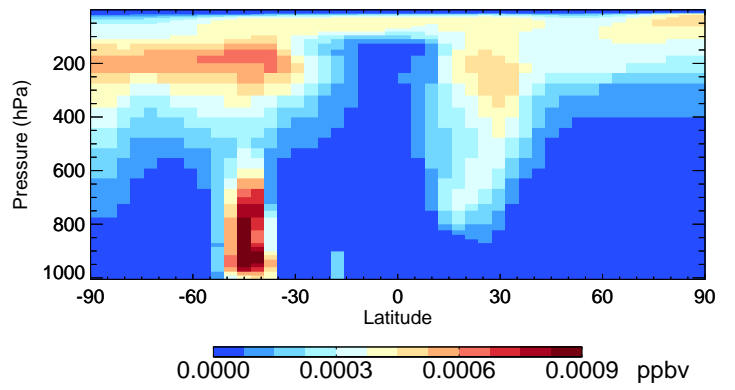
v11-02e-Run1 TSOA0 - Species Curtain @ -180.000 for Jan
