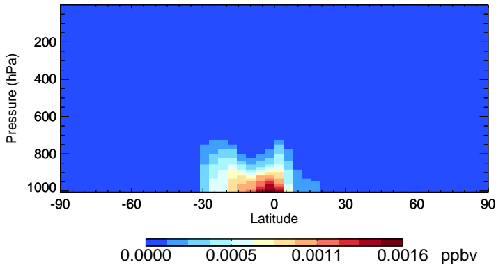
v11-02e-Run1 MOBA - Species Zonal Mean for Jan
