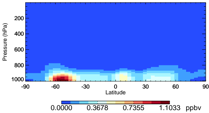
v11-02f-Run1 SALA - Species Zonal Mean for Jan
