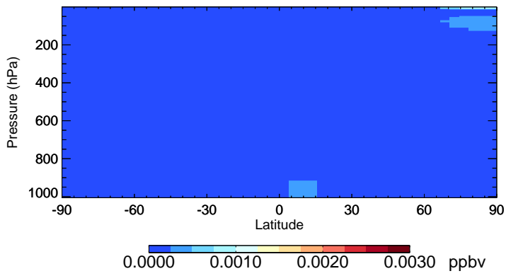
v11-02e-Run1 Br2 - Species Zonal Mean for Jan
