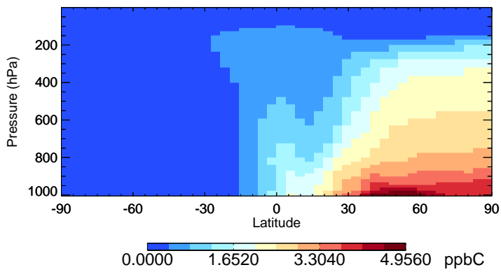
v11-02f-Run1 C2H6 - Species Zonal Mean for Jan
