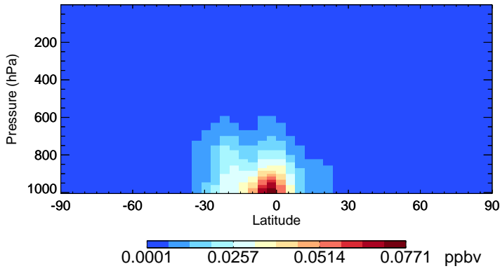
v11-02e-Run1 TSOG2 - Species Zonal Mean for Jan
