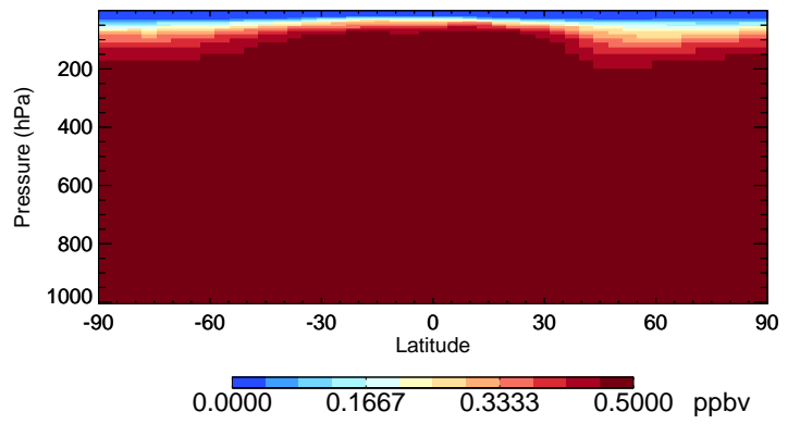
v11-02e-Run1 OCS - Species Curtain @ -180.000 for Jan
