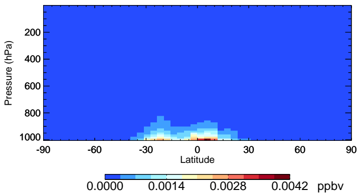
v11-02f-Run1 MONITS - Species Zonal Mean for Jan
