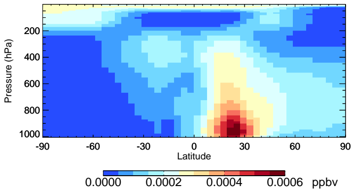
v11-02f-Run1 ASOG1 - Species Zonal Mean for Jan
