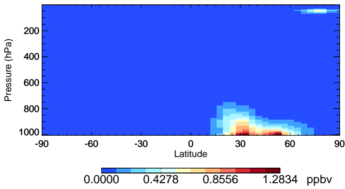
v11-02e-Run1 NIT - Species Zonal Mean for Jan
