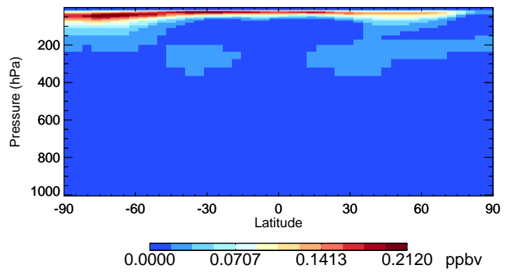
v11-02f-Run1 HNO4 - Species Curtain @ -180.000 for Jan
