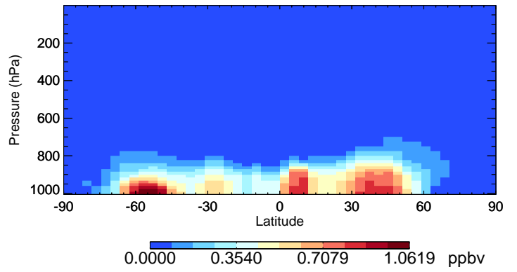
v11-02e-Run0 SALA - Species Curtain @ -180.000 for Jan
