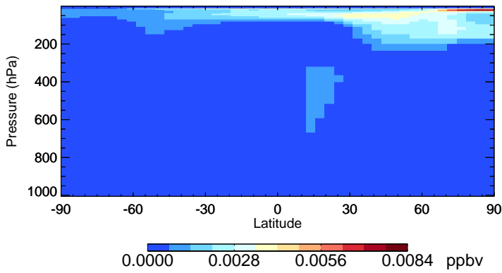
v11-02f-Run1 HOBr - Species Zonal Mean for Jan
