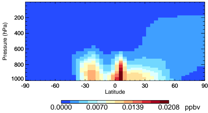
v11-02e-Run1 IONITA - Species Zonal Mean for Jan
