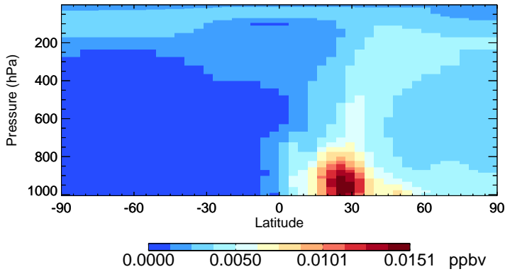
v11-02e-Run1 ASOG3 - Species Zonal Mean for Jan
