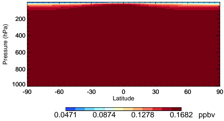
v11-02e-Run1 HCFC22 - Species Zonal Mean for Jan
