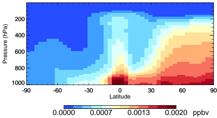
v11-02f-Run1 CHBr3 - Species Zonal Mean for Jan
