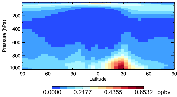
v11-02e-Run1 SO4 - Species Zonal Mean for Jan
