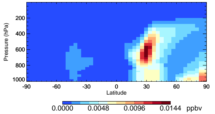
v11-02e-Run0 SOAGX - Species Curtain @ -180.000 for Jan
