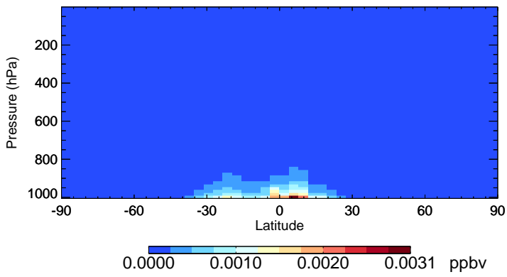
v11-02e-Run1 MONITS - Species Zonal Mean for Jan
