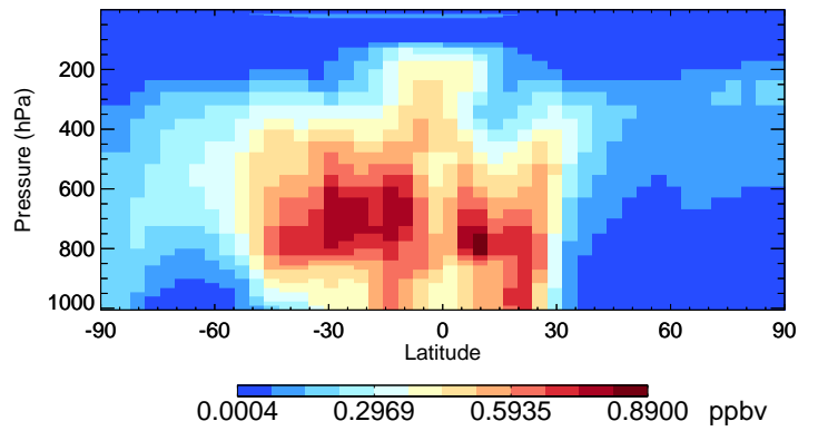
v11-02f-Run1 H2O2 - Species Curtain @ -180.000 for Jan
