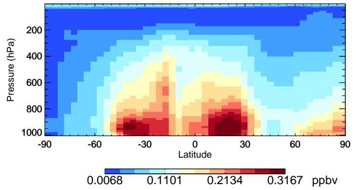
v11-02e-Run0 CH2O - Species Curtain @ -180.000 for Jan
