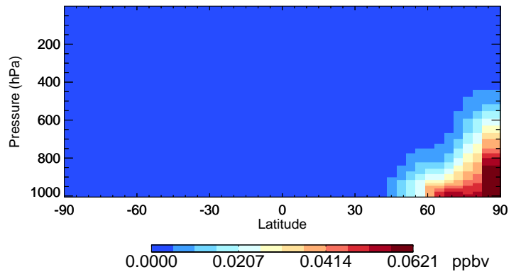
v11-02f-Run1 ClNO 2 - Species Curtain @ -180.000 for Jan
