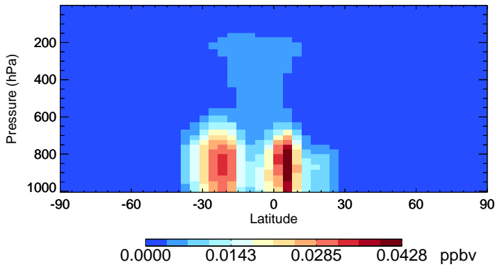
v11-02e-Run0 IMAE - Species Zonal Mean for Jan
