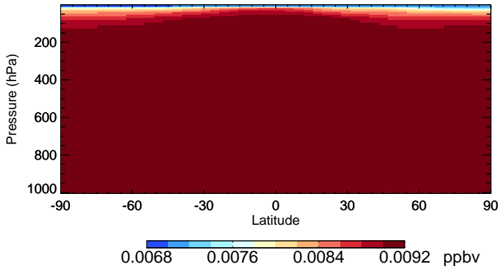
v11-02e-Run1 CFC115 - Species Zonal Mean for Jan
