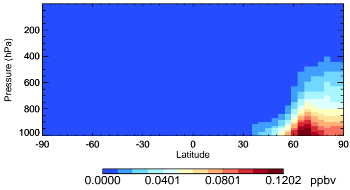
v11-02e-Run0 ClNO 2 - Species Zonal Mean for Jan
