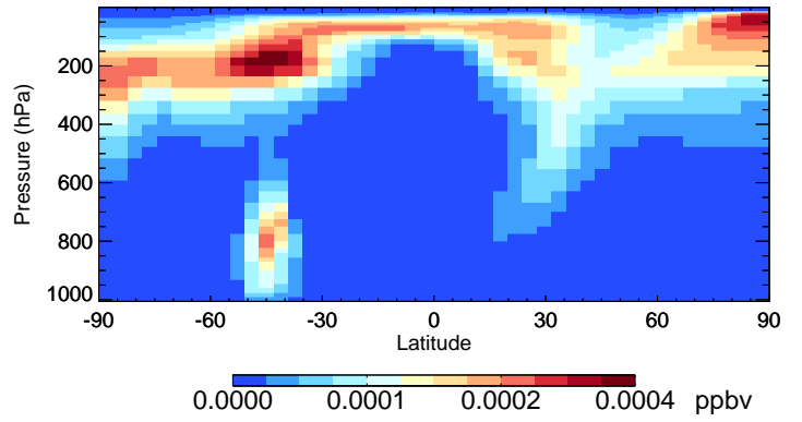
v11-02e-Run1 TSOA1 - Species Curtain @ -180.000 for Jan
