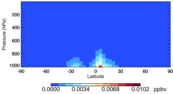
v11-02e-Run1 ISN1 - Species Zonal Mean for Jan
