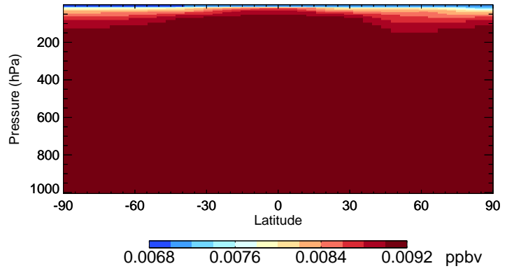
v11-02e-Run1 CFC115 - Species Curtain @ -180.000 for Jan
