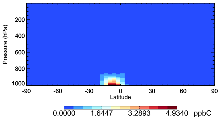
v11-02f-Run1 ISOP - Species Zonal Mean for Jan
