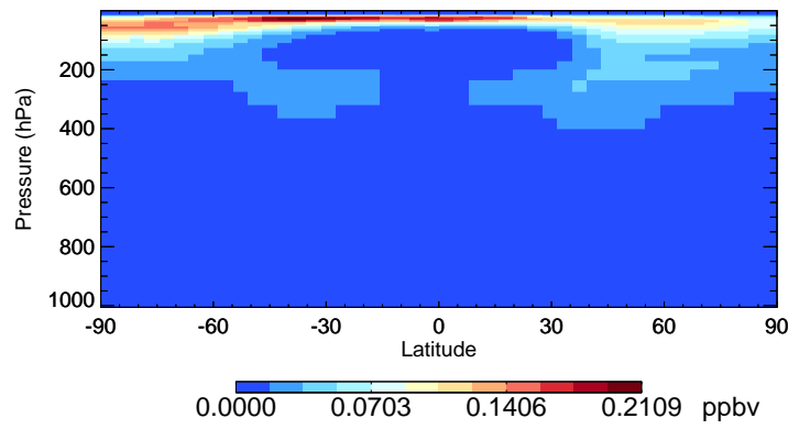
v11-02e-Run0 HNO4 - Species Curtain @ -180.000 for Jan
