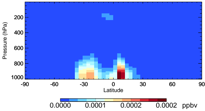
v11-02e-Run1 MACRN - Species Zonal Mean for Jan
