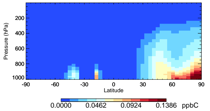
v11-02e-Run1 EOH - Species Curtain @ -180.000 for Jan
