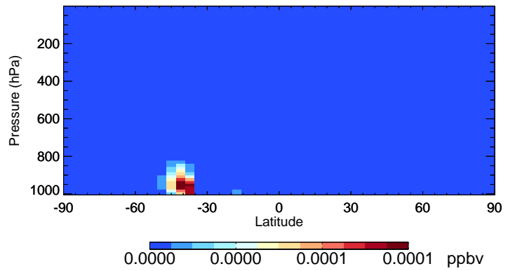
v11-02f-Run1 ISN1 - Species Curtain @ -180.000 for Jan
