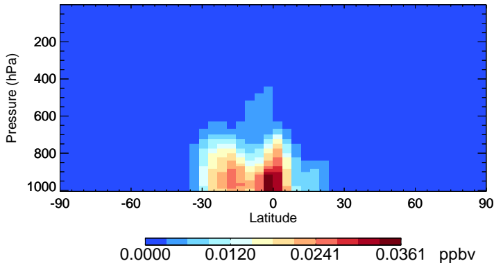
v11-02e-Run1 IPMN - Species Zonal Mean for Jan
