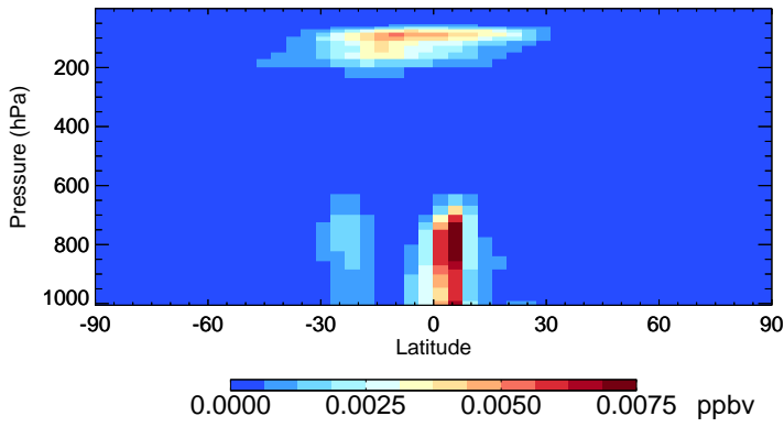
v11-02e-Run0 ISOA3 - Species Zonal Mean for Jan
