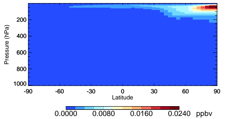
v11-02f-Run1 BrCl - Species Curtain @ -180.000 for Jan
