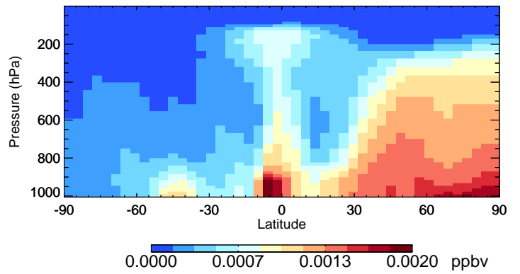
v11-02f-Run1 CHBr3 - Species Curtain @ -180.000 for Jan
