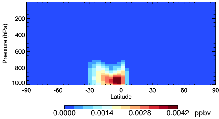
v11-02e-Run1 RIPD - Species Zonal Mean for Jan
