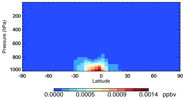
v11-02f-Run1 MOBA - Species Zonal Mean for Jan
