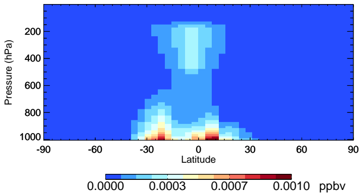
v11-02f-Run1 HONIT - Species Zonal Mean for Jan
