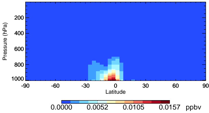
v11-02e-Run1 TSOA1 - Species Zonal Mean for Jan
