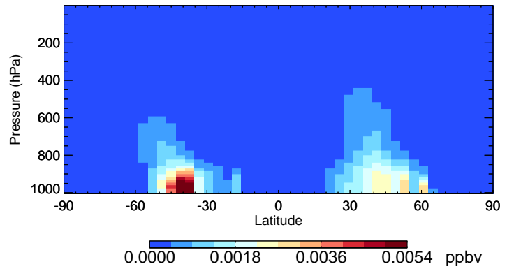
v11-02e-Run0 BCPO - Species Curtain @ -180.000 for Jan
