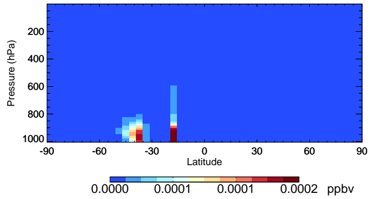
v11-02e-Run0 MONITS - Species Curtain @ -180.000 for Jan
