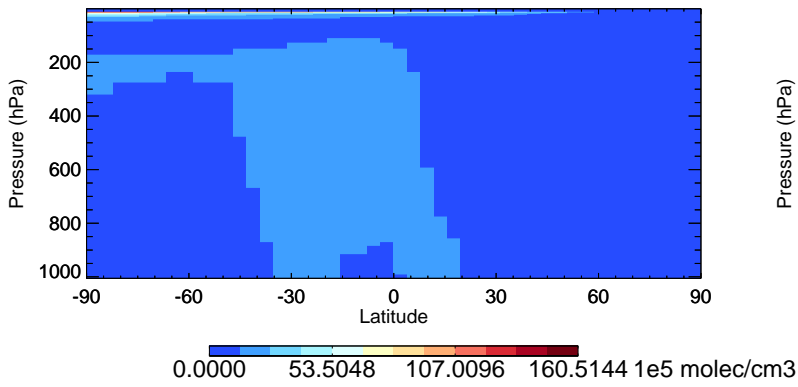
v11-02f-Run1 OH - Species Zonal Mean for Jan
