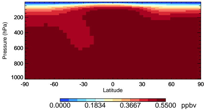
v11-02e-Run1 CH3Cl - Species Zonal Mean for Jan
