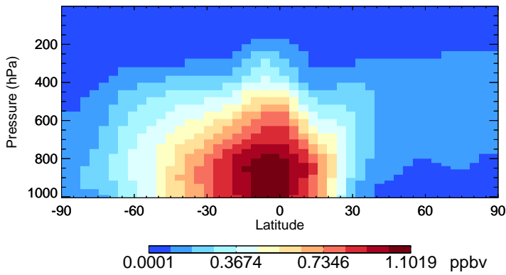
v11-02f-Run1 MP - Species Zonal Mean for Jan
