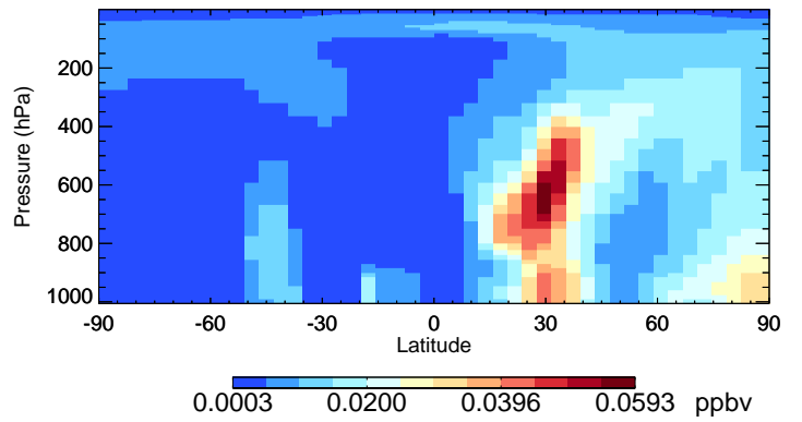
v11-02f-Run1 SOAS - Species Curtain @ -180.000 for Jan
