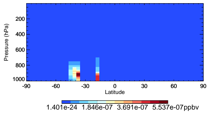
v11-02e-Run1 LVOC - Species Curtain @ -180.000 for Jan
