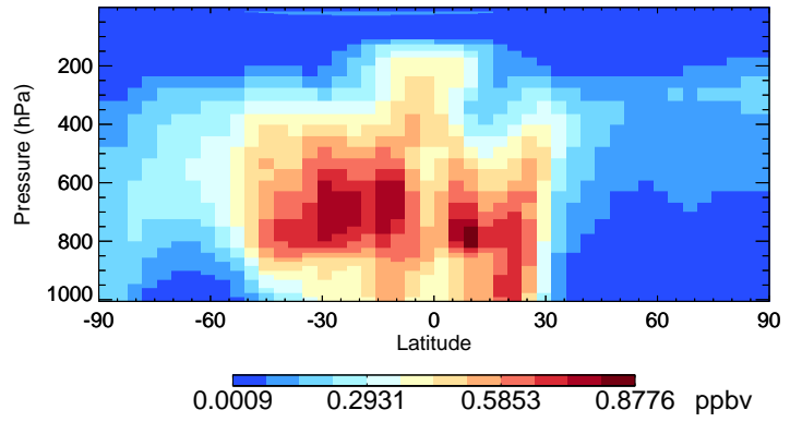
v11-02e-Run1 H2O2 - Species Curtain @ -180.000 for Jan
