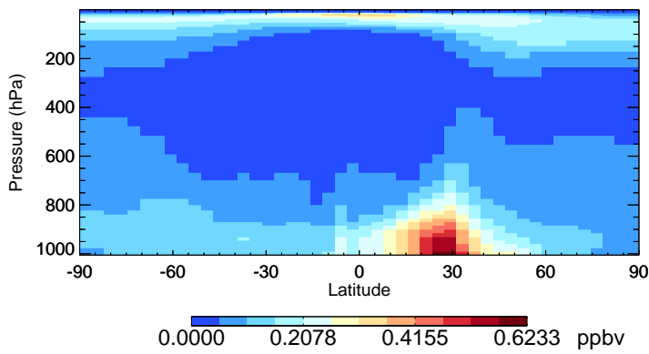
v11-02f-Run1 SO4 - Species Zonal Mean for Jan
