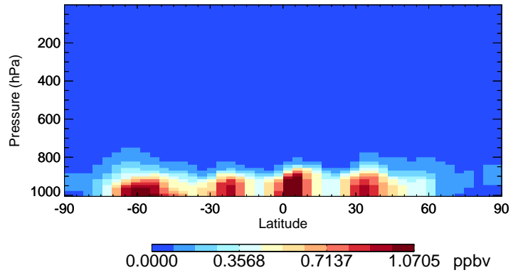
v11-02e-Run1 SALA - Species Curtain @ -180.000 for Jan
