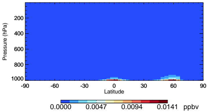
v11-02f-Run1 LIMO - Species Zonal Mean for Jul
