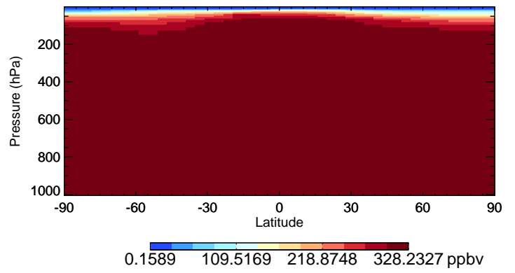
v11-02e-Run1 N2O - Species Curtain @ -180.000 for Jul
