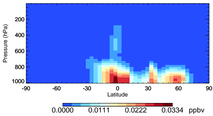
v11-02e-Run1 IPMN - Species Zonal Mean for Jul
