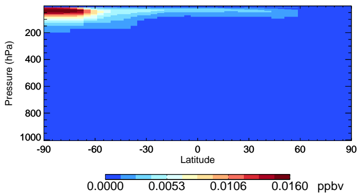
v11-02e-Run1 BrCl - Species Zonal Mean for Jul
