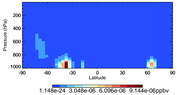
v11-02f-Run1 ETHLN - Species Curtain @ -180.000 for Jul
