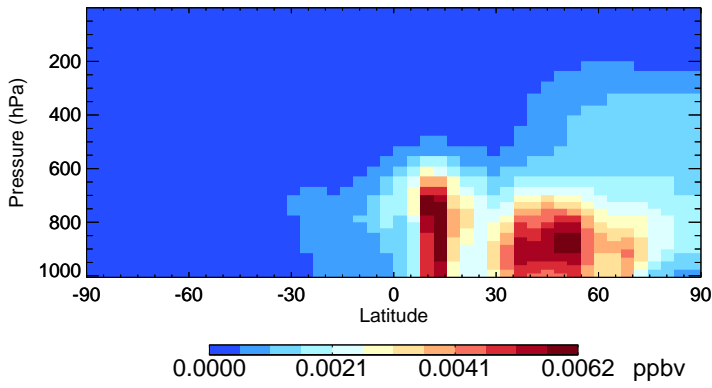
v11-02e-Run0 SOAME - Species Zonal Mean for Jul
