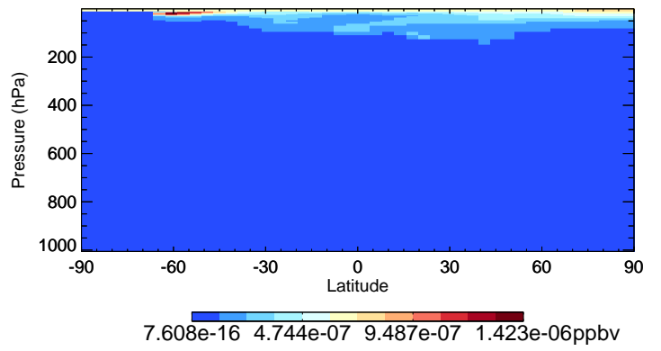
v11-02e-Run1 CIOO - Species Curtain @ -180.000 for Jul
