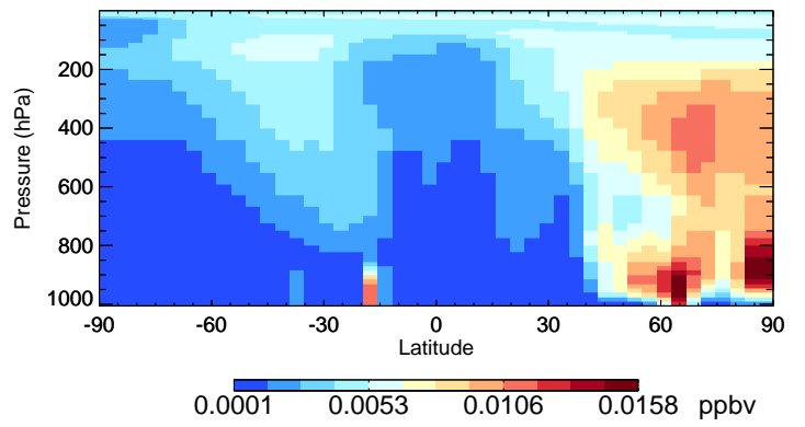
v11-02e-Run1 TSOG3 - Species Curtain @ -180.000 for Jul
