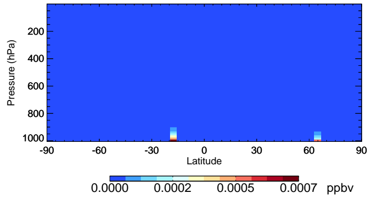
v11-02e-Run0 MTPO - Species Curtain @ -180.000 for Jul
