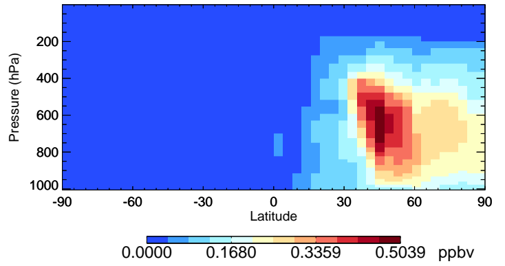
v11-02e-Run1 DST1 - Species Curtain @ -180.000 for Jul
