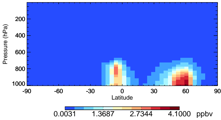
v11-02e-Run0 OCPI - Species Zonal Mean for Jul
