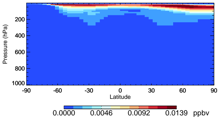
v11-02e-Run0 BrNO3 - Species Zonal Mean for Jul
