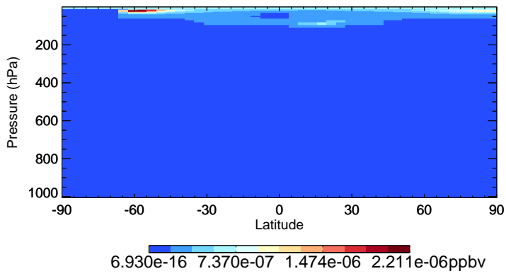
v11-02e-Run0 CIOO - Species Zonal Mean for Jul
