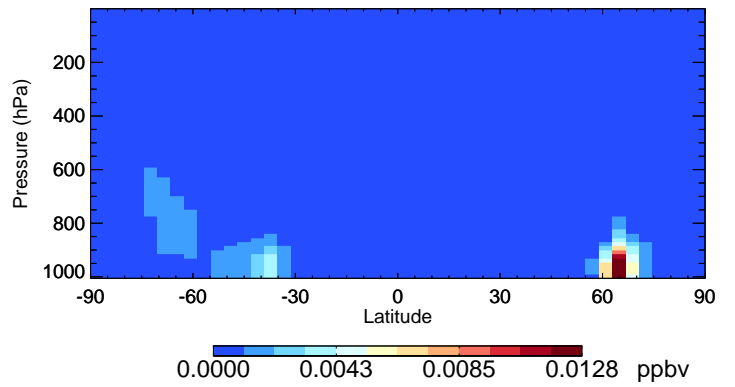
v11-02f-Run1 MACR - Species Curtain @ -180.000 for Jul
