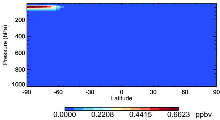
v11-02f-Run1 Cl2O2 - Species Zonal Mean for Jul
