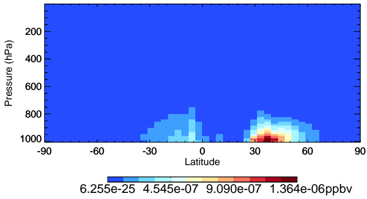
v11-02e-Run0 NPMN - Species Zonal Mean for Jul
