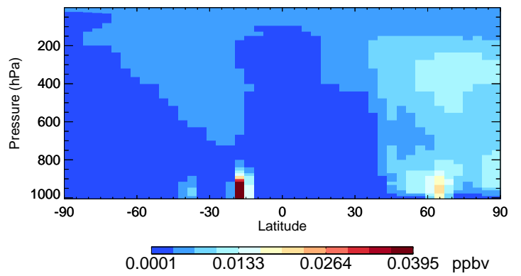
v11-02f-Run1 TSOG3 - Species Curtain @ -180.000 for Jul
