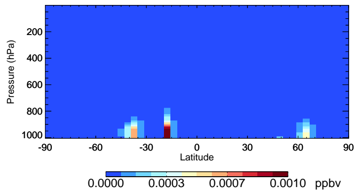
v11-02f-Run1 MONITS - Species Curtain @ -180.000 for Jul
