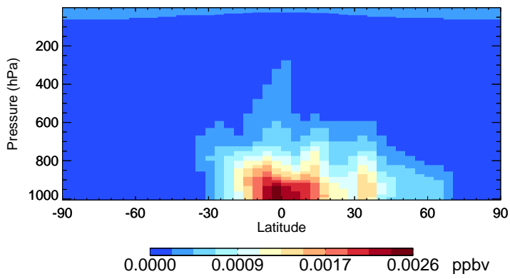
v11-02f-Run1 LVOCOA - Species Zonal Mean for Jul
