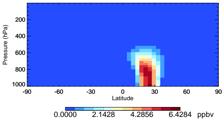
v11-02e-Run1 DST2 - Species Zonal Mean for Jul
