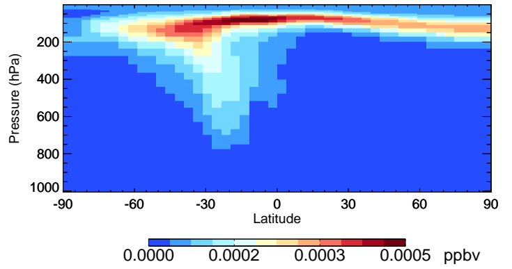
v11-02e-Run1 DHDN - Species Curtain @ -180.000 for Jul
