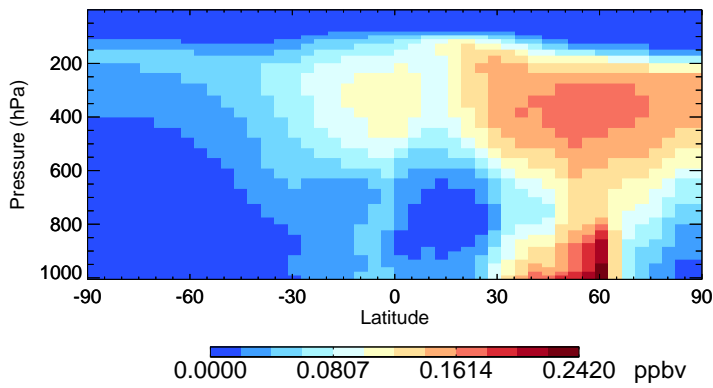
v11-02e-Run1 PAN - Species Zonal Mean for Jul
