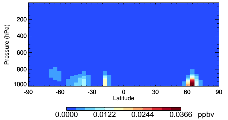
v11-02f-Run1 RCHO - Species Curtain @ -180.000 for Jul
