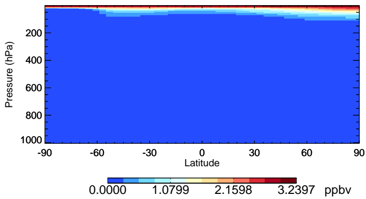
v11-02f-Run1 HCl - Species Zonal Mean for Jul
