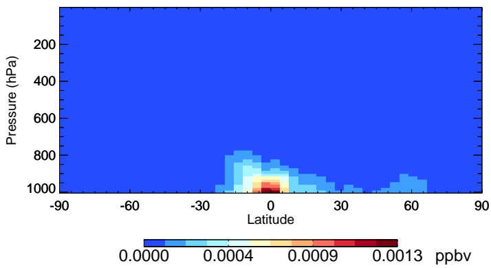
v11-02f-Run1 MOBA - Species Zonal Mean for Jul
