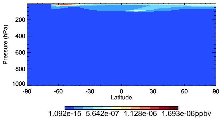
v11-02f-Run1 CIOO - Species Zonal Mean for Jul
