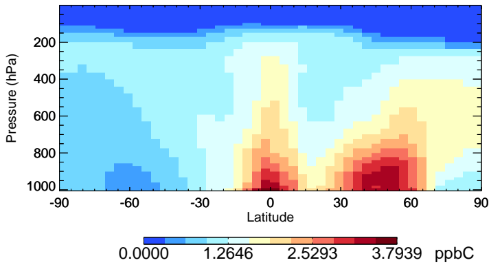
v11-02e-Run0 ACET - Species Zonal Mean for Jul
