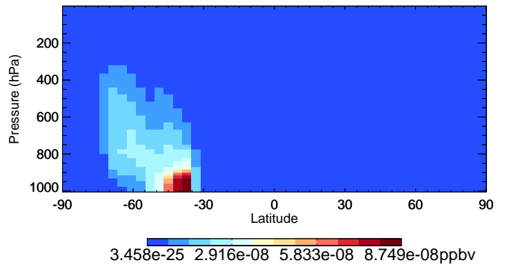
v11-02f-Run1 NPMN - Species Curtain @ -180.000 for Jul
