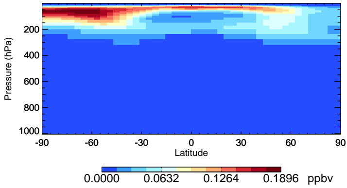
v11-02e-Run1 MPN - Species Zonal Mean for Jul
