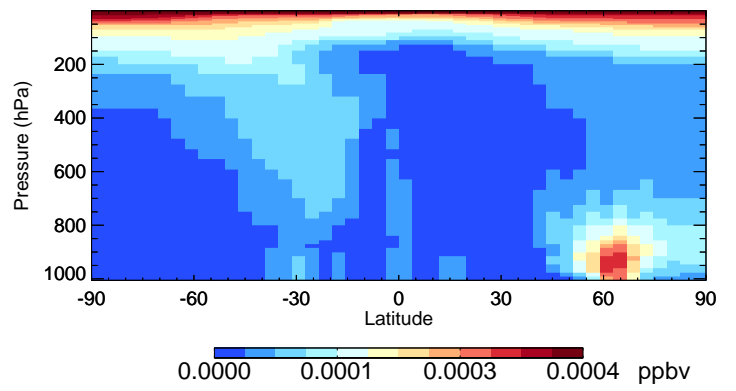
v11-02f-Run1 LVOCOA - Species Curtain @ -180.000 for Jul
