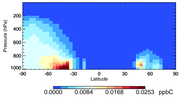
v11-02e-Run0 TOLU - Species Curtain @ -180.000 for Jul
