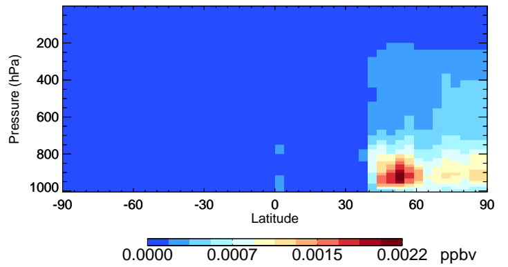
v11-02f-Run1 SOAME - Species Curtain @ -180.000 for Jul
