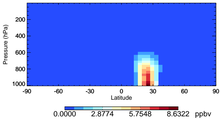
v11-02e-Run1 DST4 - Species Zonal Mean for Jul
