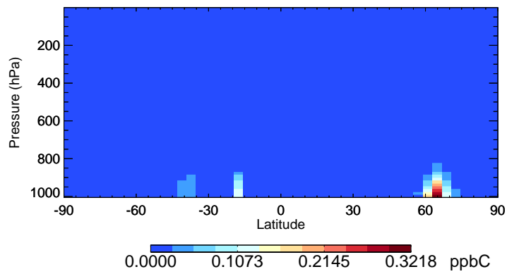
v11-02f-Run1 PRPE - Species Curtain @ -180.000 for Jul
