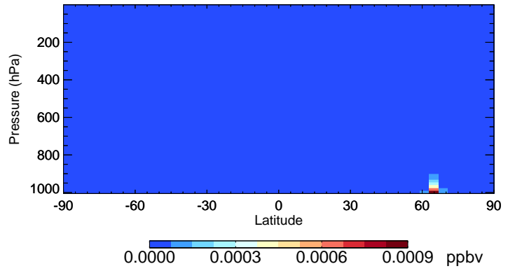
v11-02e-Run1 LIMO - Species Curtain @ -180.000 for Jul
