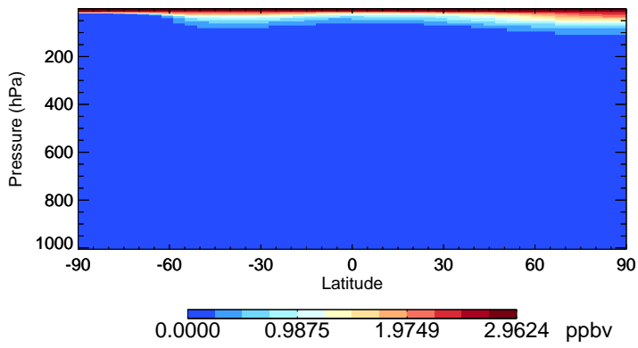
v11-02e-Run0 HCl - Species Zonal Mean for Jul
