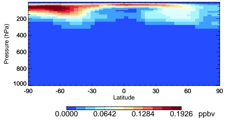
v11-02e-Run1 MPN - Species Curtain @ -180.000 for Jul
