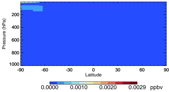
v11-02e-Run0 Br2 - Species Zonal Mean for Jul
