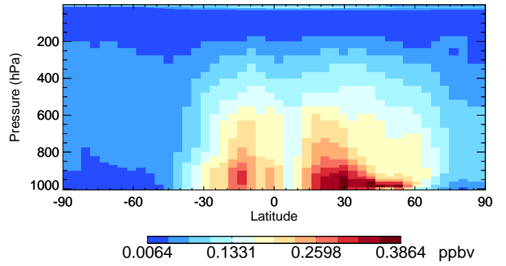
v11-02e-Run1 CH2O - Species Curtain @ -180.000 for Jul
