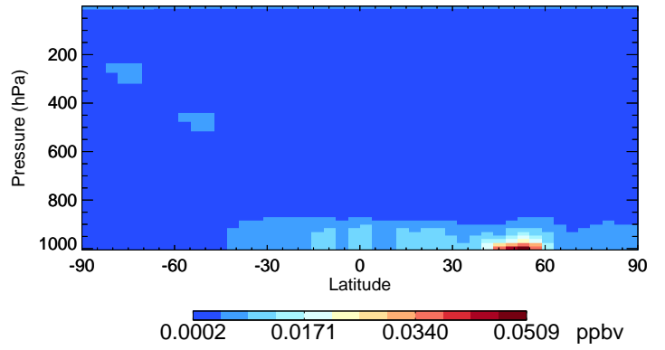
v11-02e-Run1 MSA - Species Curtain @ -180.000 for Jul
