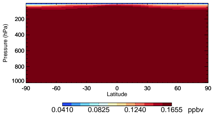
v11-02f-Run1 HCFC22 - Species Zonal Mean for Jul
