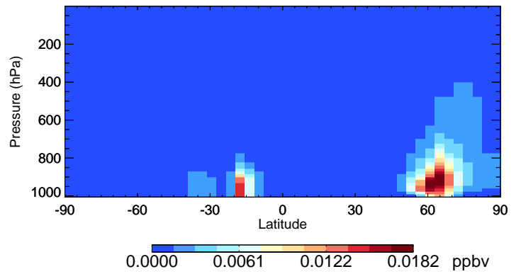
v11-02f-Run1 HAC - Species Curtain @ -180.000 for Jul
