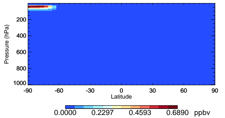
v11-02f-Run1 Cl2O2 - Species Curtain @ -180.000 for Jul
