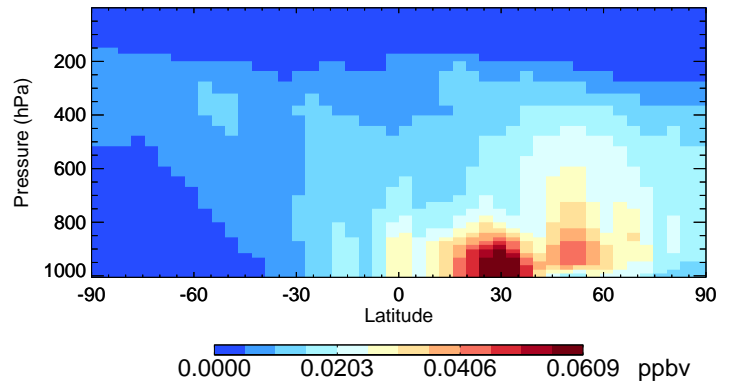
v11-02e-Run0 MAP - Species Curtain @ -180.000 for Jul
