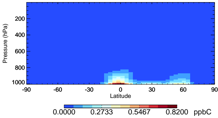
v11-02e-Run0 PRPE - Species Zonal Mean for Jul
