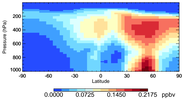
v11-02e-Run0 PAN - Species Zonal Mean for Jul
