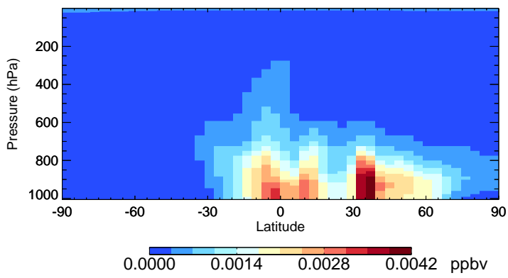
v11-02e-Run1 LVOCOA - Species Zonal Mean for Jul
