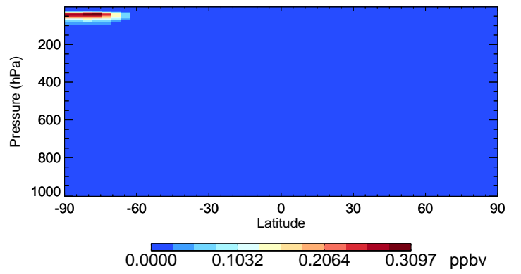
v11-02e-Run1 Cl2O2 - Species Curtain @ -180.000 for Jul
