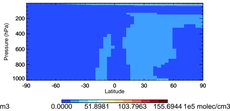
v11-02f-Run1 OH - Species Curtain @ -180.000 for Jul
