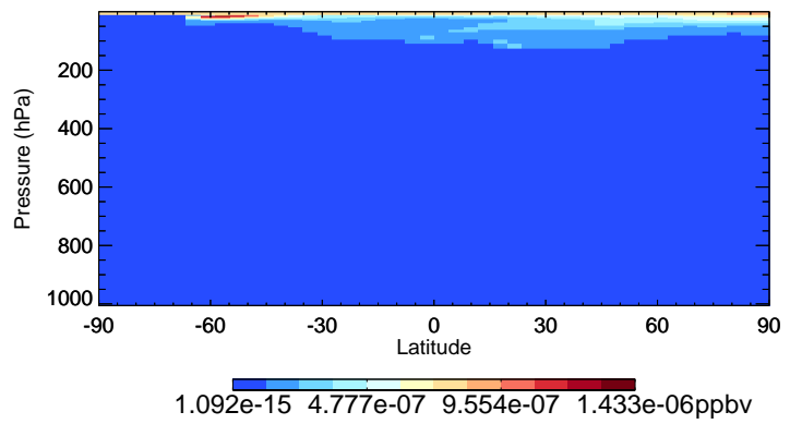
v11-02f-Run1 CIOO - Species Curtain @ -180.000 for Jul
