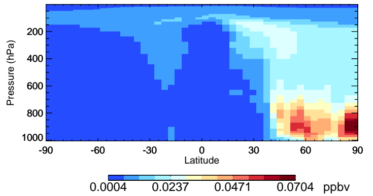
v11-02f-Run1 SOAS - Species Curtain @ -180.000 for Jul
