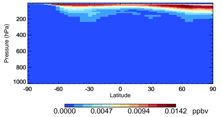
v11-02e-Run0 BrNO3 - Species Curtain @ -180.000 for Jul
