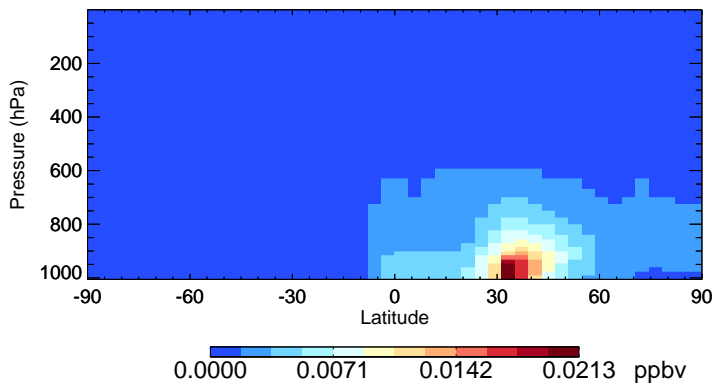
v11-02e-Run1 ASOAN - Species Zonal Mean for Jul
