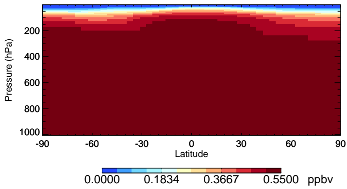
v11-02e-Run0 CH3Cl - Species Zonal Mean for Jul
