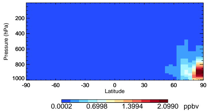
v11-02e-Run1 OCPI - Species Curtain @ -180.000 for Jul
