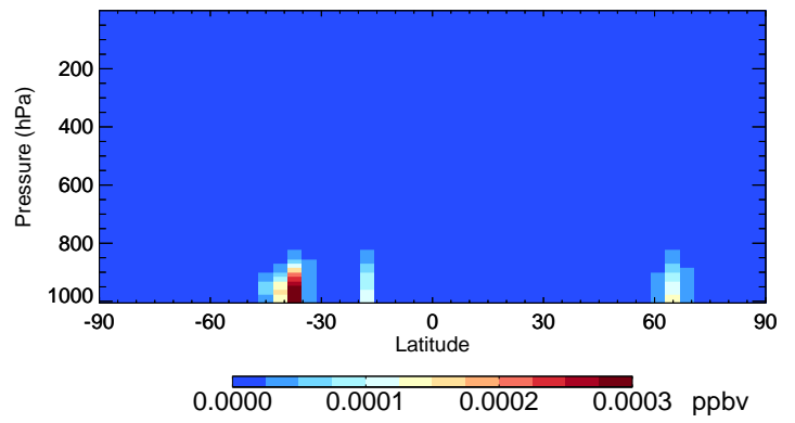
v11-02e-Run0 MONITS - Species Curtain @ -180.000 for Jul
