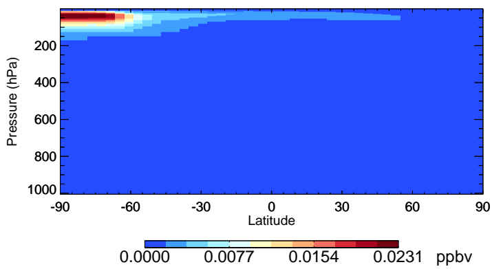
v11-02f-Run1 BrCl - Species Zonal Mean for Jul
