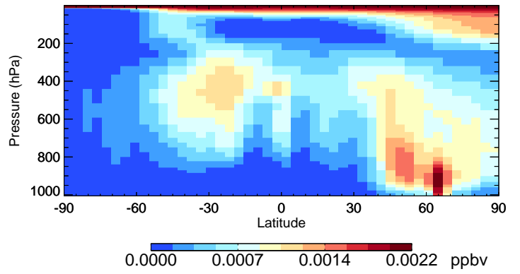
v11-02e-Run0 ISOG1 - Species Curtain @ -180.000 for Jul
