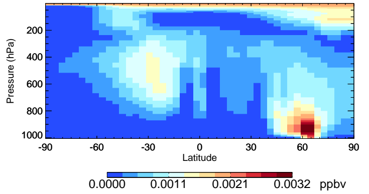
v11-02e-Run1 ISOG1 - Species Curtain @ -180.000 for Jul
