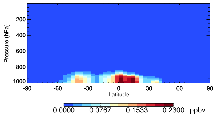
v11-02e-Run1 NH3 - Species Curtain @ -180.000 for Jul
