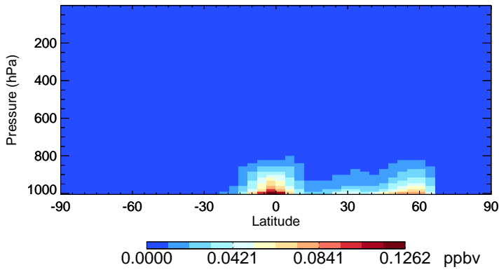
v11-02e-Run0 RCHO - Species Zonal Mean for Jul
