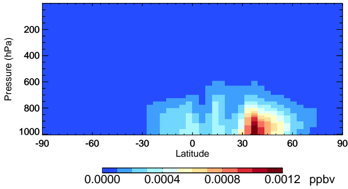
v11-02e-Run1 ISN10A - Species Zonal Mean for Jul
