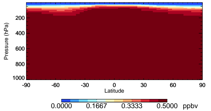
v11-02f-Run1 OCS - Species Curtain @ -180.000 for Jul
