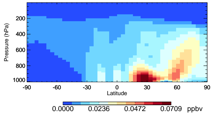
v11-02f-Run1 MAP - Species Curtain @ -180.000 for Jul
