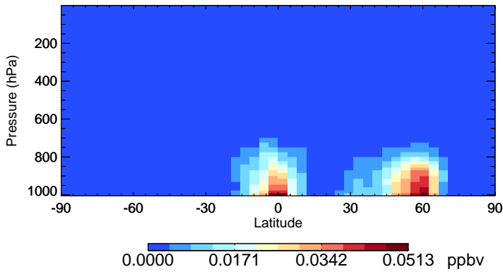
v11-02e-Run0 TSOA2 - Species Zonal Mean for Jul
