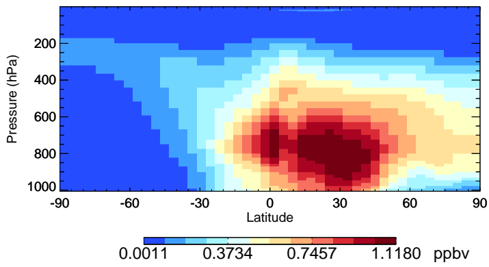
v11-02e-Run0 H2O2 - Species Zonal Mean for Jul
