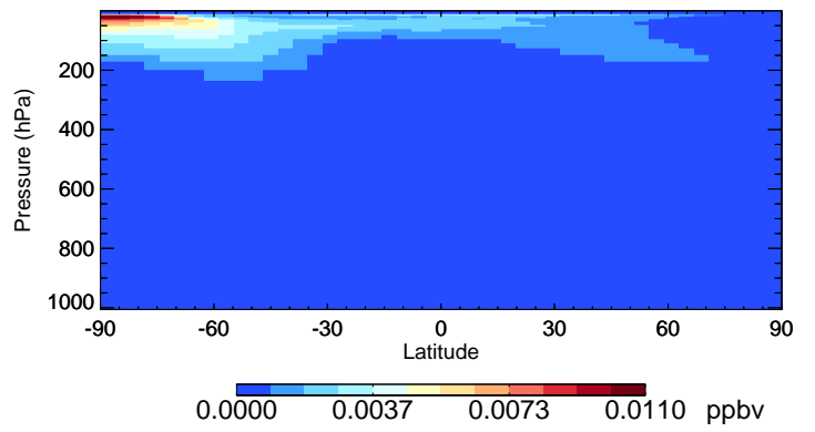
v11-02e-Run1 HOBr - Species Curtain @ -180.000 for Jul
