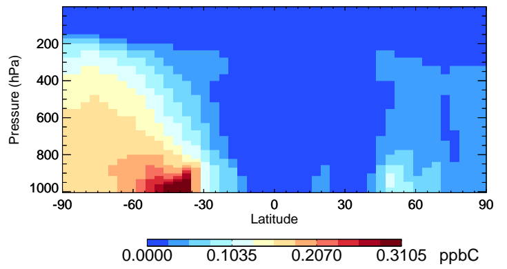
v11-02e-Run0 ALK4 - Species Curtain @ -180.000 for Jul
