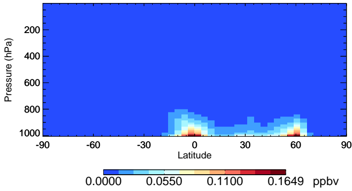
v11-02e-Run1 RCHO - Species Zonal Mean for Jul
