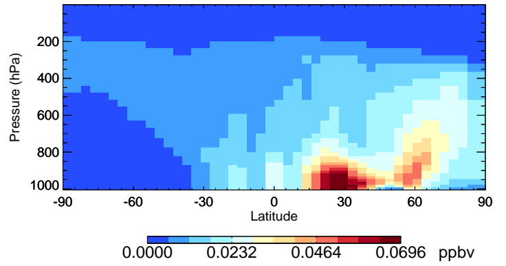
v11-02e-Run1 MAP - Species Curtain @ -180.000 for Jul
