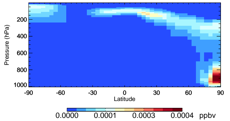
v11-02f-Run1 ASOA2 - Species Curtain @ -180.000 for Jul
