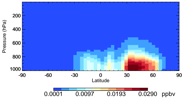
v11-02e-Run0 IONITA - Species Zonal Mean for Jul
