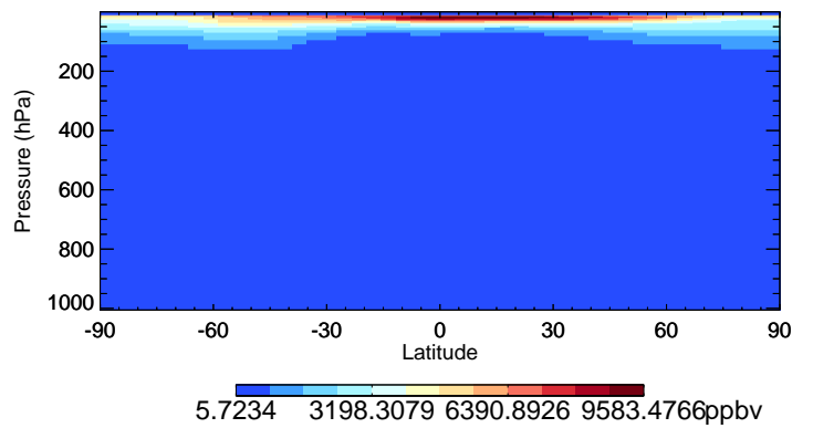
v11-02f-Run1 O3 - Species Curtain @ -180.000 for Jul
