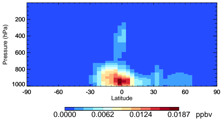
v11-02f-Run1 IEPOXB - Species Zonal Mean for Jul
