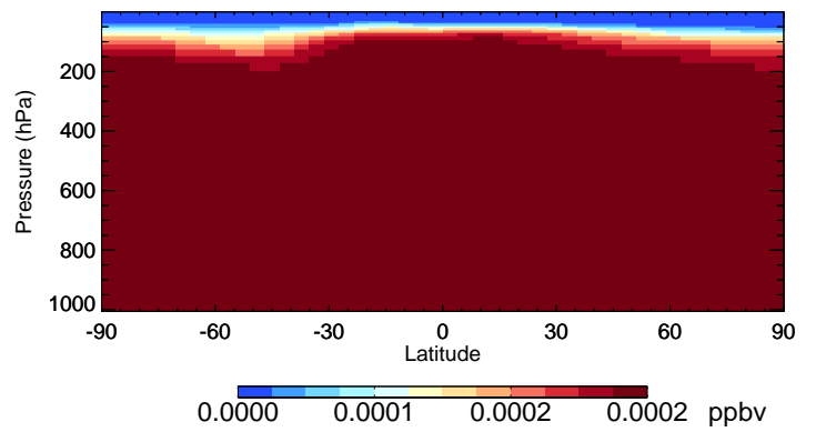
v11-02f-Run1 H2402 - Species Curtain @ -180.000 for Jul
