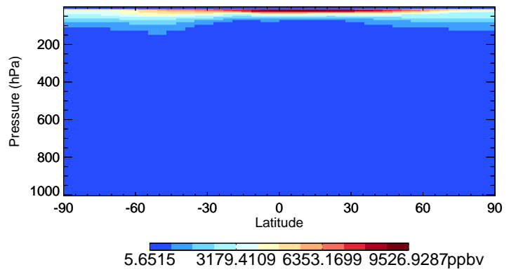
v11-02e-Run1 O3 - Species Curtain @ -180.000 for Jul
