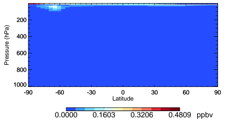
v11-02f-Run1 CIO - Species Curtain @ -180.000 for Jul
