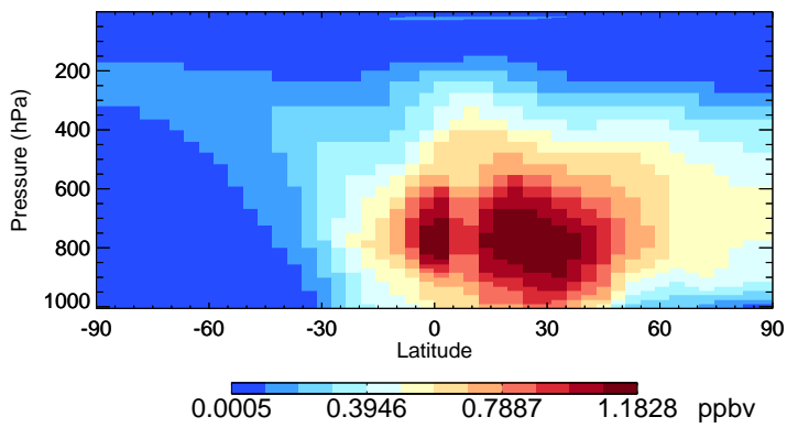
v11-02f-Run1 H2O2 - Species Zonal Mean for Jul
