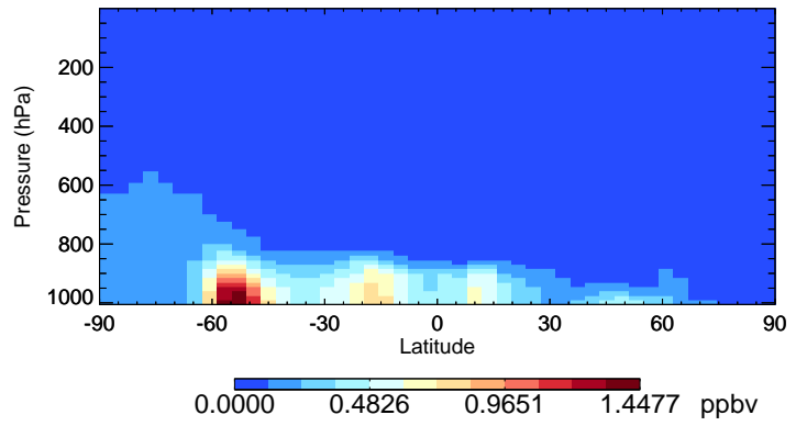
v11-02e-Run0 SALA - Species Curtain @ -180.000 for Jul
