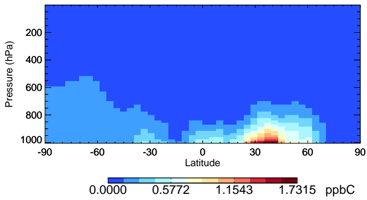
v11-02e-Run1 ALK4 - Species Zonal Mean for Jul
