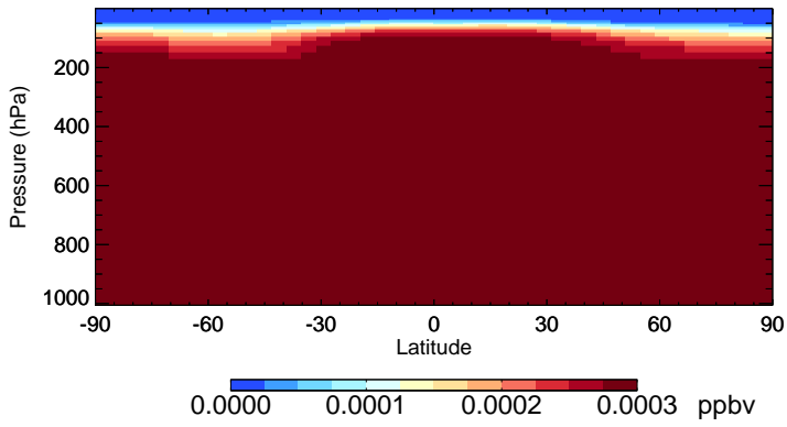
v11-02e-Run0 H2402 - Species Zonal Mean for Jul
