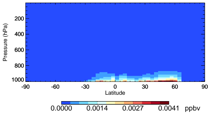
v11-02e-Run1 MONITS - Species Zonal Mean for Jul
