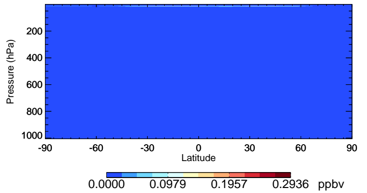
v11-02f-Run1 NO3 - Species Curtain @ -180.000 for Jul
