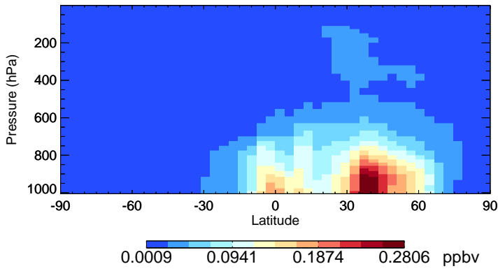
v11-02e-Run0 SOAS - Species Zonal Mean for Jul
