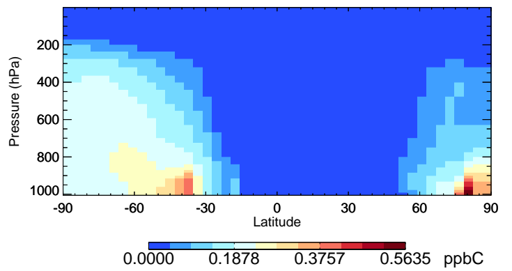
v11-02f-Run1 ALK4 - Species Curtain @ -180.000 for Jul
