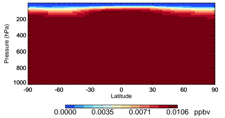
v11-02e-Run0 CH3CCI3 - Species Curtain @ -180.000 for Jul
