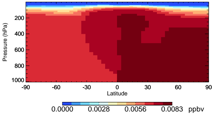
v11-02e-Run1 CH3Br - Species Zonal Mean for Jul
