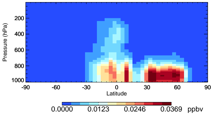
v11-02e-Run0 IMAE - Species Zonal Mean for Jul
