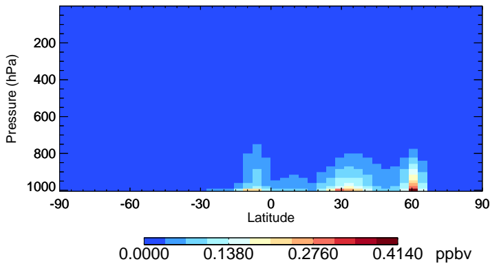
v11-02f-Run1 BCPO - Species Zonal Mean for Jul
