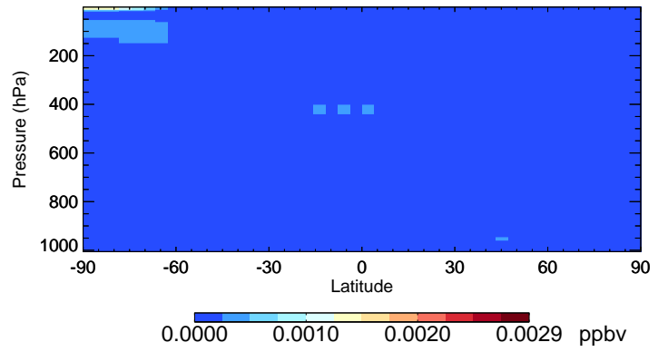
v11-02e-Run0 Br2 - Species Curtain @ -180.000 for Jul
