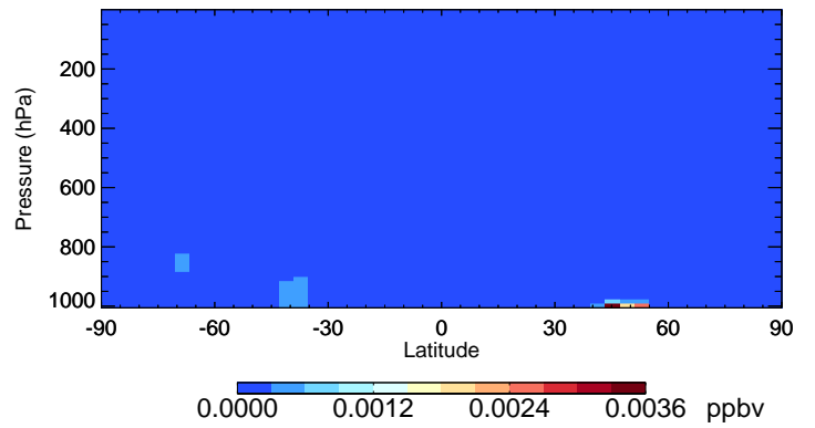
v11-02f-Run1 ClNO2 - Species Curtain @ -180.000 for Jul
