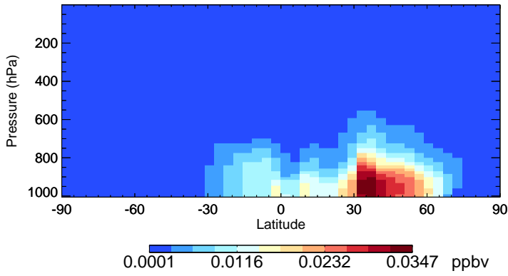
v11-02e-Run1 IONITA - Species Zonal Mean for Jul
