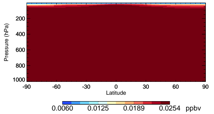
v11-02e-Run1 HCFC142b - Species Curtain @ -180.000 for Jul
