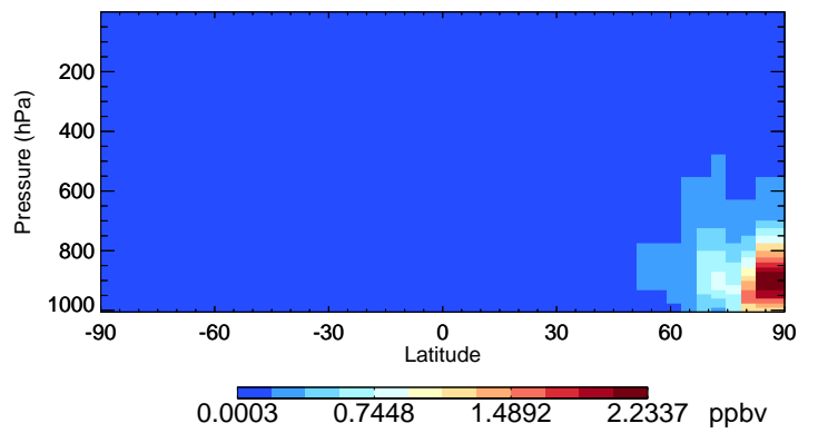
v11-02f-Run1 OCPI - Species Curtain @ -180.000 for Jul
