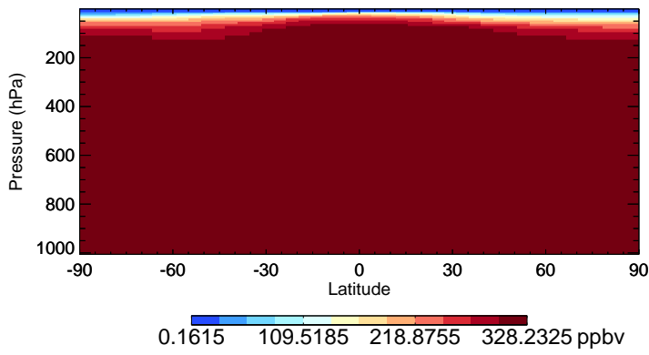
v11-02e-Run1 N2O - Species Zonal Mean for Jul
