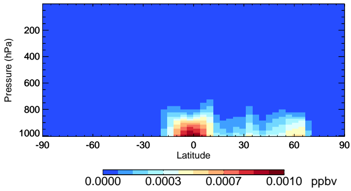
v11-02e-Run0 MOBA - Species Zonal Mean for Jul
