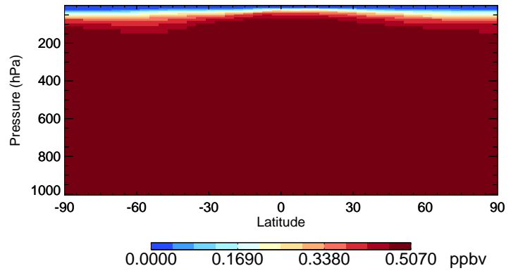
v11-02e-Run0 CFC12 - Species Curtain @ -180.000 for Jul
