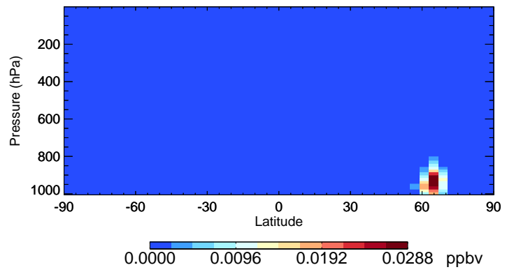
v11-02e-Run1 RIPA - Species Curtain @ -180.000 for Jul
