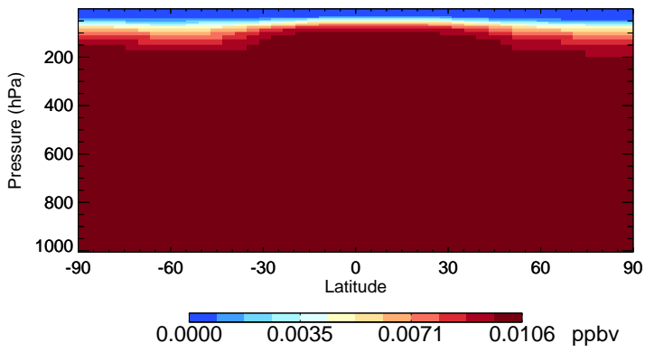
v11-02e-Run0 CH3CCI3 - Species Zonal Mean for Jul
