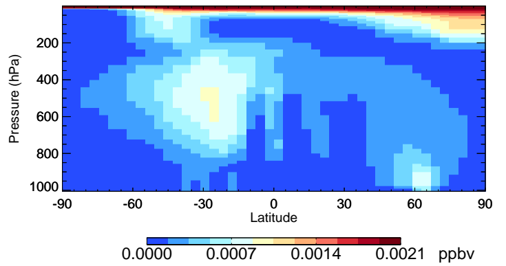
v11-02f-Run1 ISOG1 - Species Curtain @ -180.000 for Jul
