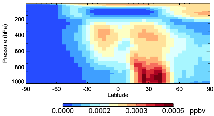
v11-02f-Run1 ASOG1 - Species Zonal Mean for Jul
