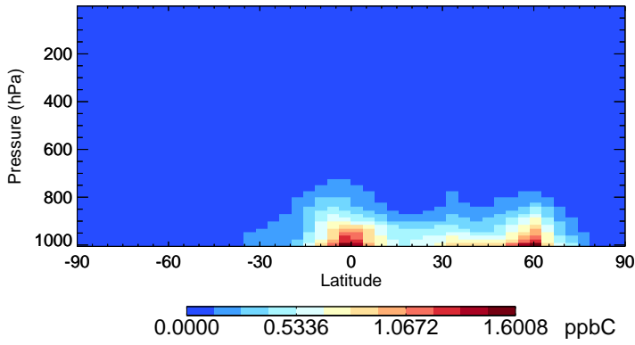
v11-02e-Run1 ALD2 - Species Zonal Mean for Jul
