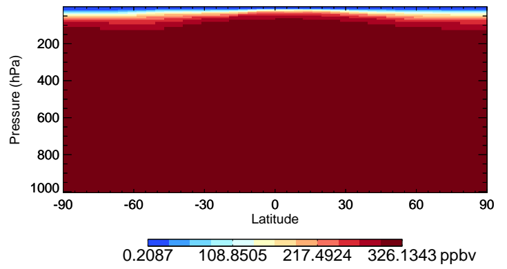
v11-02e-Run0 N2O - Species Curtain @ -180.000 for Jul
