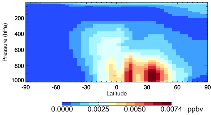
v11-02e-Run0 ISOG1 - Species Zonal Mean for Jul
