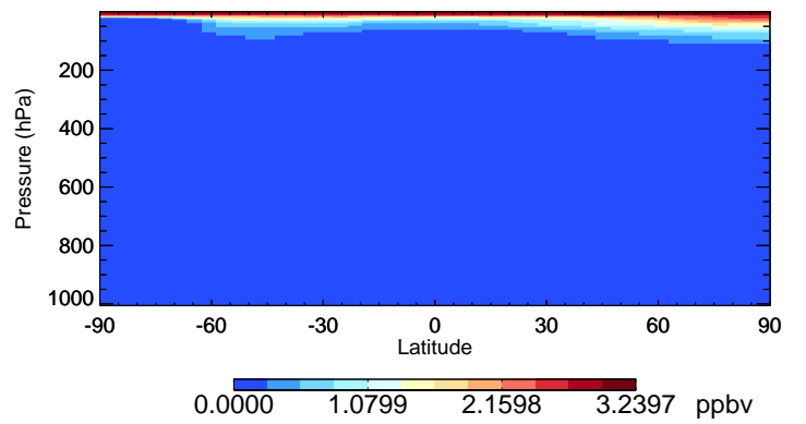
v11-02f-Run1 HCl - Species Curtain @ -180.000 for Jul
