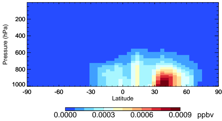
v11-02e-Run0 ISN10A - Species Zonal Mean for Jul
