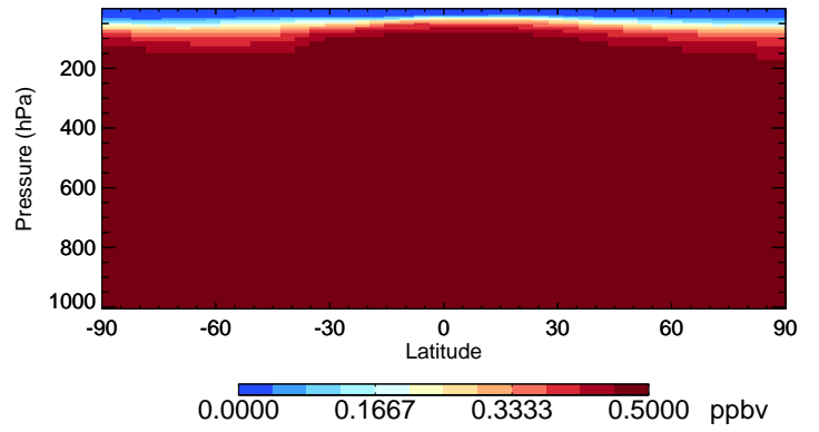
v11-02e-Run0 OCS - Species Curtain @ -180.000 for Jul
