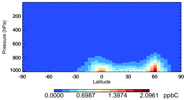
v11-02f-Run1 ALD2 - Species Zonal Mean for Jul
