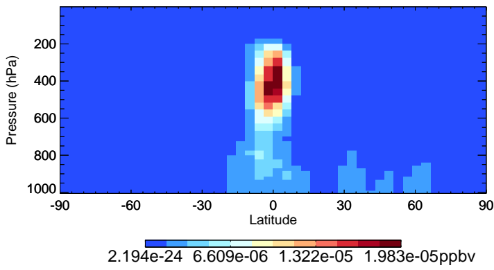
v11-02e-Run1 LVOC - Species Zonal Mean for Jul
