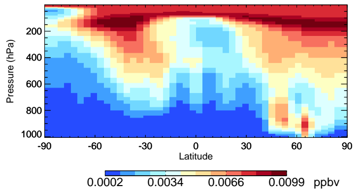
v11-02e-Run0 ISO3 - Species Curtain @ -180.000 for Jul
