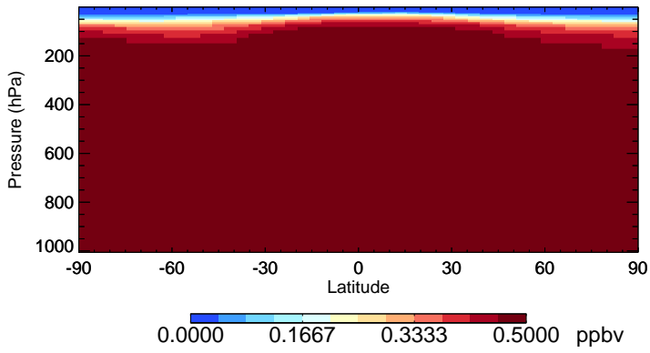
v11-02e-Run0 OCS - Species Zonal Mean for Jul
