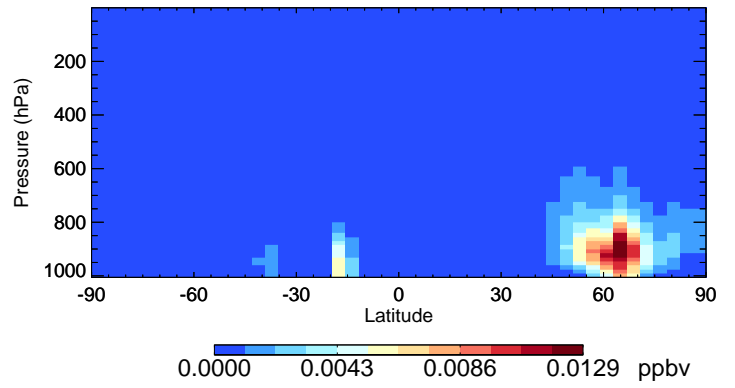
v11-02e-Run0 HAC - Species Curtain @ -180.000 for Jul
