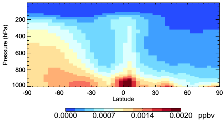
v11-02f-Run1 CHBr3 - Species Zonal Mean for Jul
