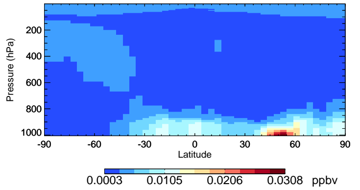
v11-02e-Run0 MSA - Species Curtain @ -180.000 for Jul
