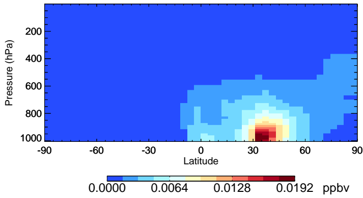
v11-02e-Run0 ASOAN - Species Zonal Mean for Jul
