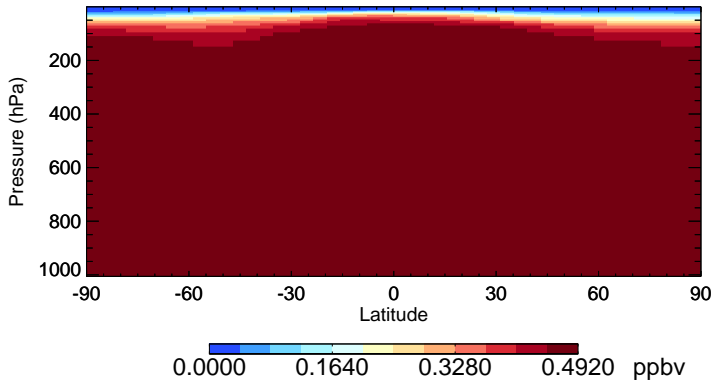
v11-02e-Run1 CFC12 - Species Zonal Mean for Jul
