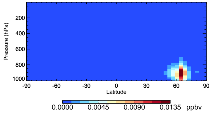
v11-02e-Run0 GLYC - Species Curtain @ -180.000 for Jul
