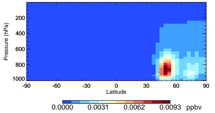
v11-02e-Run0 SOAME - Species Curtain @ -180.000 for Jul
