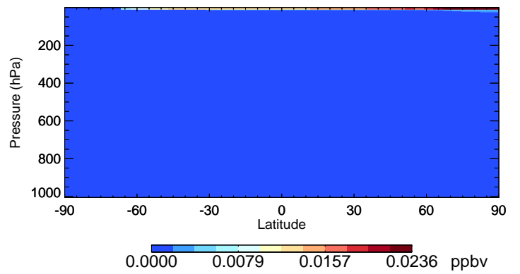
v11-02f-Run1 Br - Species Curtain @ -180.000 for Jul
