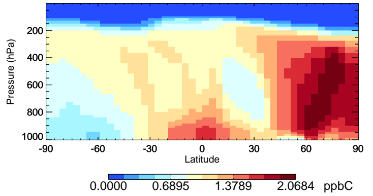
v11-02e-Run1 ACET - Species Curtain @ -180.000 for Jul
