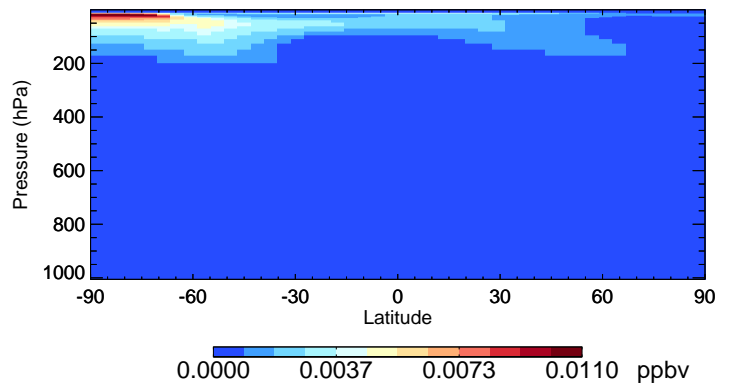
v11-02e-Run0 HOBr - Species Curtain @ -180.000 for Jul
