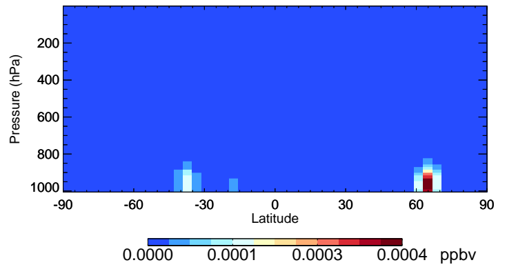
v11-02f-Run1 ISOPNB - Species Curtain @ -180.000 for Jul
