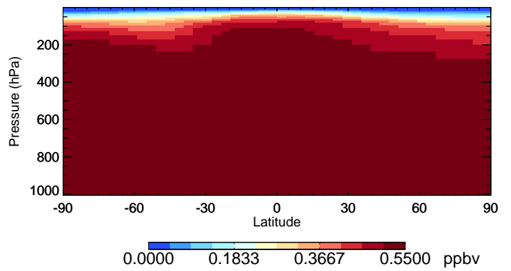
v11-02f-Run1 CH3Cl - Species Curtain @ -180.000 for Jul
