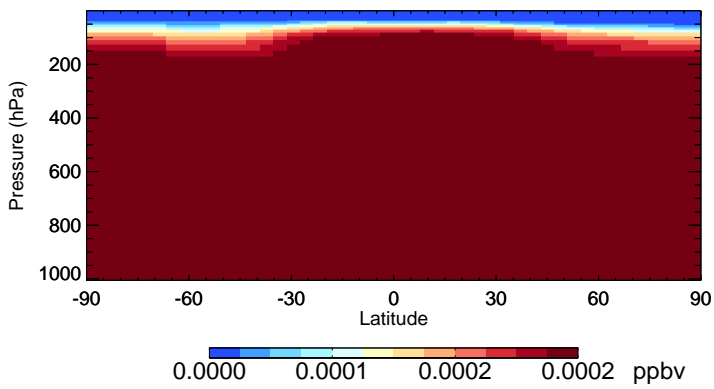
v11-02f-Run1 H2402 - Species Zonal Mean for Jul
