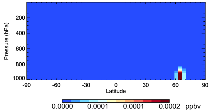
v11-02e-Run0 MOBA - Species Curtain @ -180.000 for Jul
