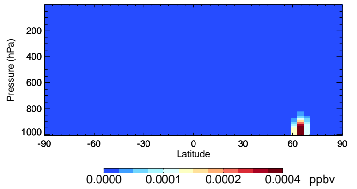
v11-02e-Run1 MOBA - Species Curtain @ -180.000 for Jul
