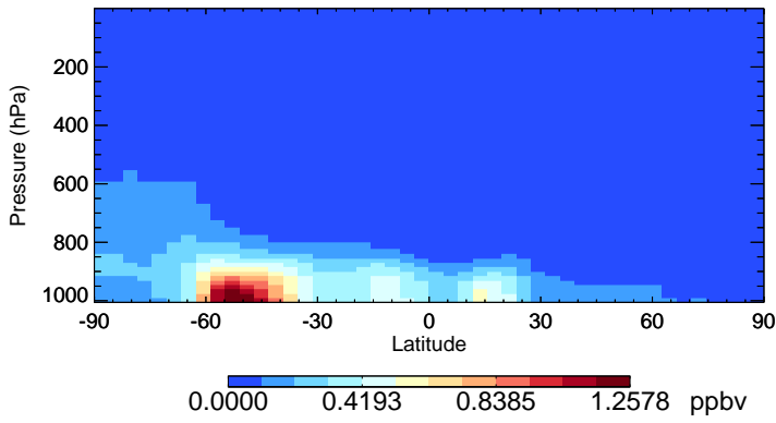
v11-02e-Run0 SALA - Species Zonal Mean for Jul
