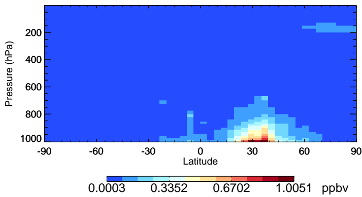
v11-02f-Run1 SO2 - Species Zonal Mean for Jul
