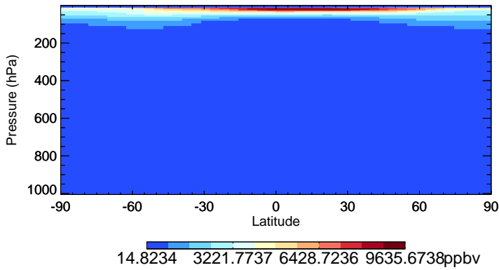
v11-02e-Run0 O3 - Species Zonal Mean for Jul
