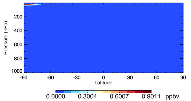
v11-02f-Run1 Cl2 - Species Curtain @ -180.000 for Jul
