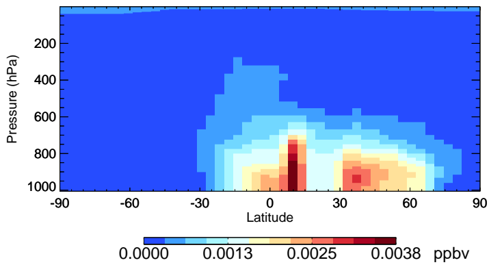
v11-02e-Run0 LVOCOA - Species Zonal Mean for Jul
