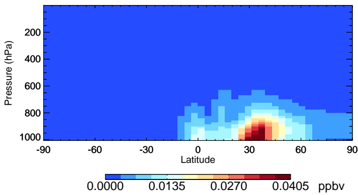
v11-02f-Run1 SOAGX - Species Zonal Mean for Jul
