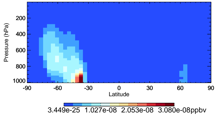
v11-02e-Run1 NPMN - Species Curtain @ -180.000 for Jul
