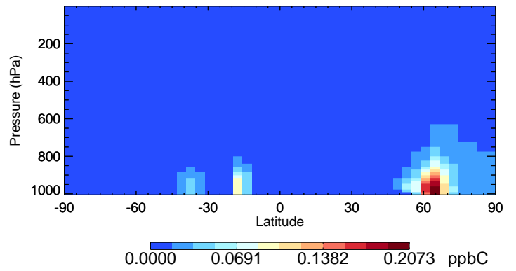
v11-02f-Run1 EOH - Species Curtain @ -180.000 for Jul
