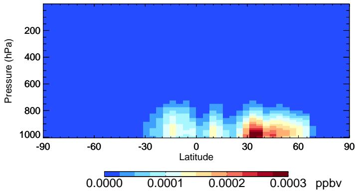
v11-02e-Run0 ETHLN - Species Zonal Mean for Jul
