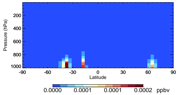
v11-02e-Run1 MONITS - Species Curtain @ -180.000 for Jul
