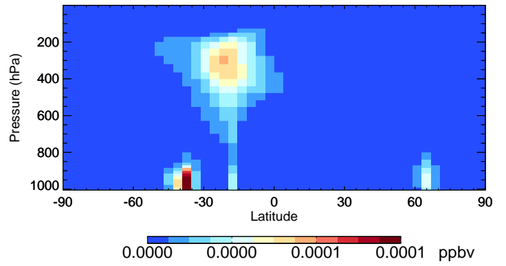
v11-02e-Run0 HONIT - Species Curtain @ -180.000 for Jul
