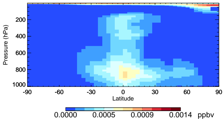
v11-02e-Run1 HBr - Species Zonal Mean for Jul
