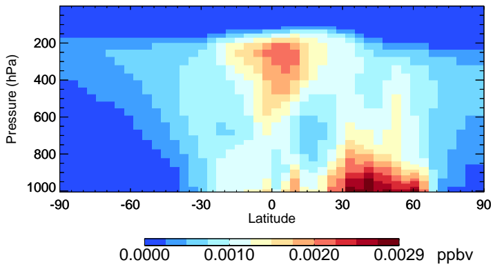
v11-02f-Run1 R4N2 - Species Zonal Mean for Jul
