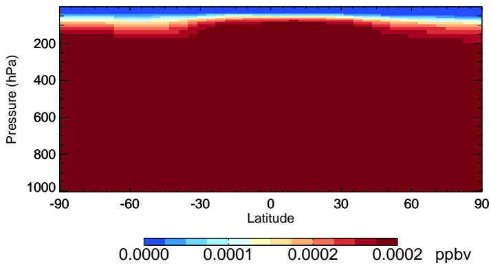
v11-02e-Run1 H2402 - Species Zonal Mean for Jul
