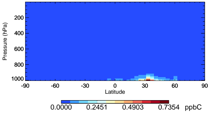
v11-02e-Run1 XYLE - Species Zonal Mean for Jul
