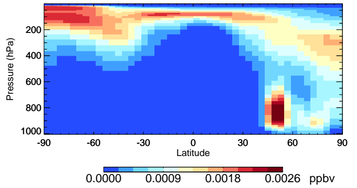
v11-02e-Run0 ISOA1 - Species Curtain @ -180.000 for Jul
