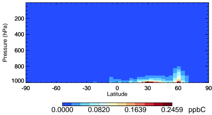
v11-02f-Run1 XYLE - Species Zonal Mean for Jul
