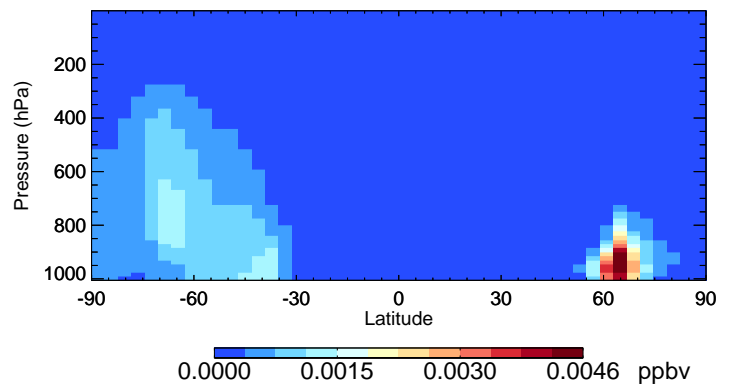
v11-02f-Run1 IPMN - Species Curtain @ -180.000 for Jul
