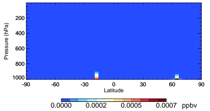
v11-02e-Run1 MTPO - Species Curtain @ -180.000 for Jul
