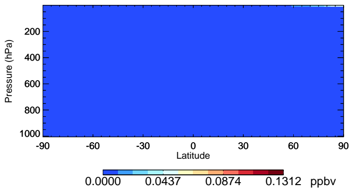
v11-02f-Run1 ACTA - Species Zonal Mean for Jul
