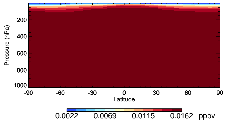
v11-02e-Run0 CFC114 - Species Curtain @ -180.000 for Jul
