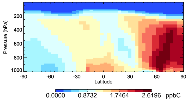
v11-02f-Run1 ACET - Species Curtain @ -180.000 for Jul
