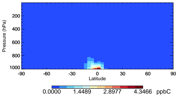
v11-02f-Run1 ISOP - Species Zonal Mean for Jul
