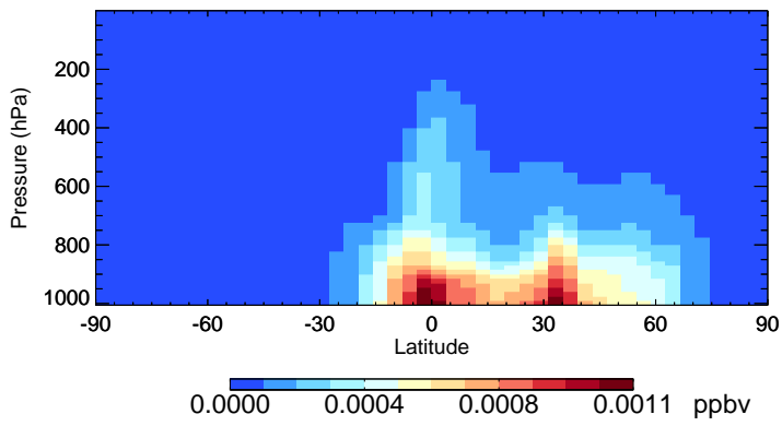
v11-02e-Run1 ACTA - Species Zonal Mean for Jul
