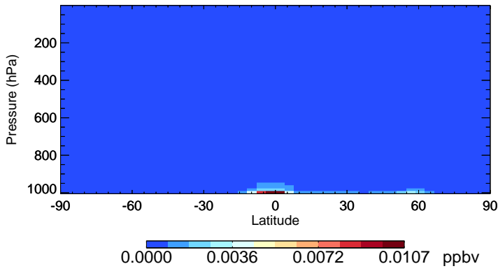
v11-02e-Run0 MTPO - Species Zonal Mean for Jul
