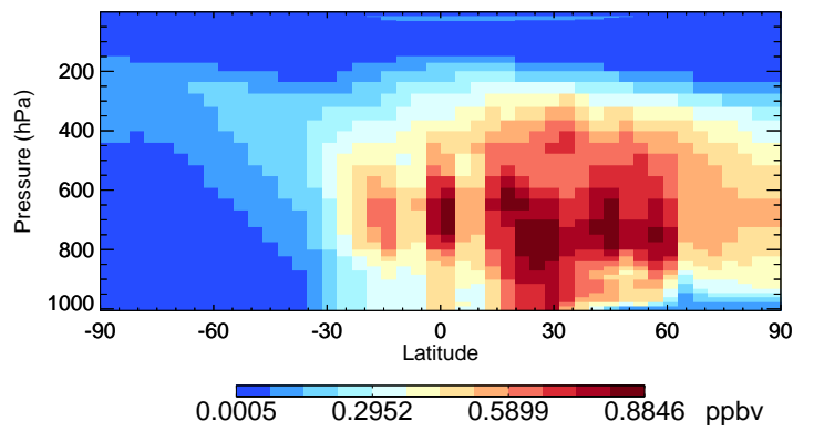
v11-02f-Run1 H2O2 - Species Curtain @ -180.000 for Jul
