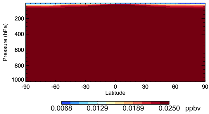
v11-02e-Run0 HCFC142b - Species Zonal Mean for Jul
