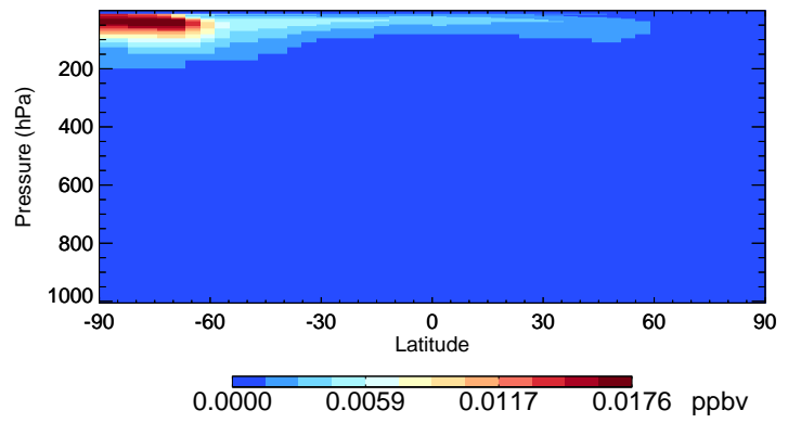
v11-02e-Run0 BrCl - Species Curtain @ -180.000 for Jul
