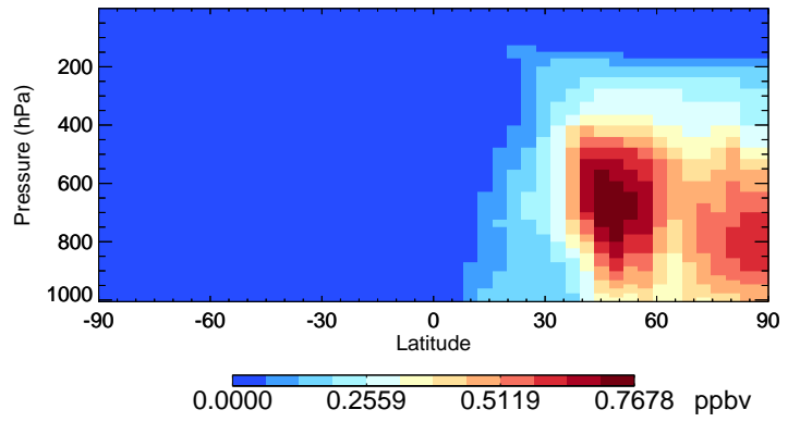
v11-02e-Run0 DST1 - Species Curtain @ -180.000 for Jul
