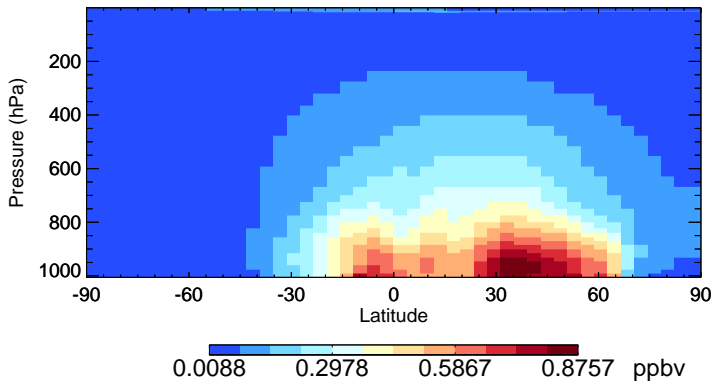
v11-02e-Run0 CH2O - Species Zonal Mean for Jul
