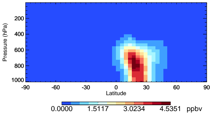
v11-02f-Run1 DST1 - Species Zonal Mean for Jul
