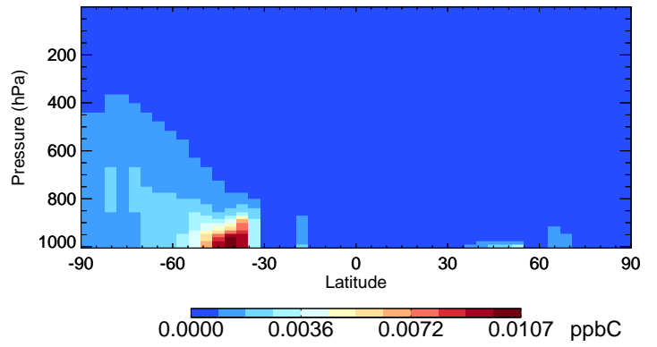
v11-02e-Run0 XYLE - Species Curtain @ -180.000 for Jul
