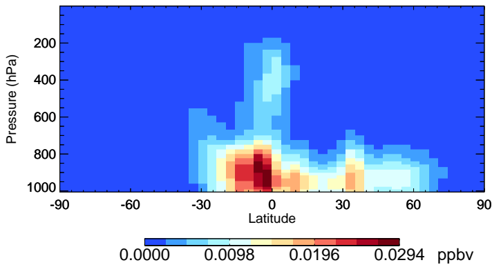
v11-02f-Run1 IMAE - Species Zonal Mean for Jul
