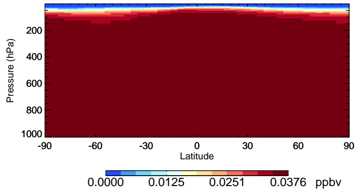
v11-02e-Run0 HCFC141b - Species Curtain @ -180.000 for Jul
