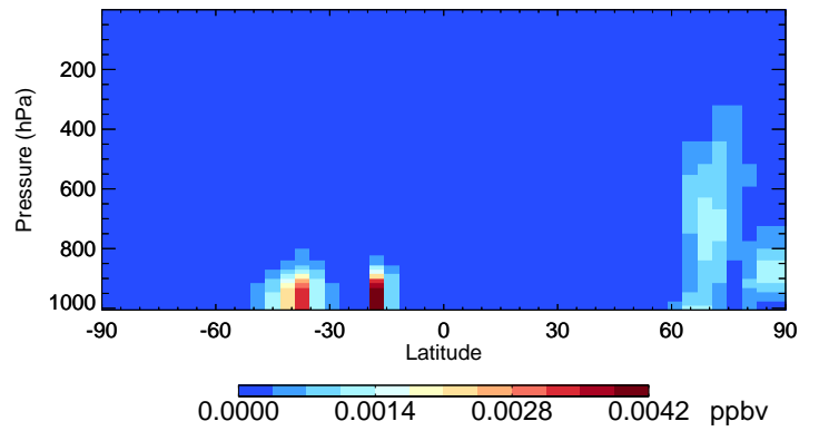
v11-02f-Run1 BCPO - Species Curtain @ -180.000 for Jul
