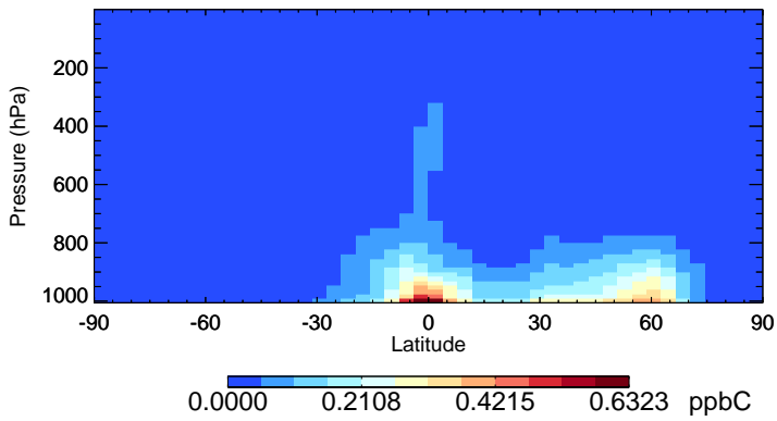
v11-02f-Run1 EOH - Species Zonal Mean for Jul
