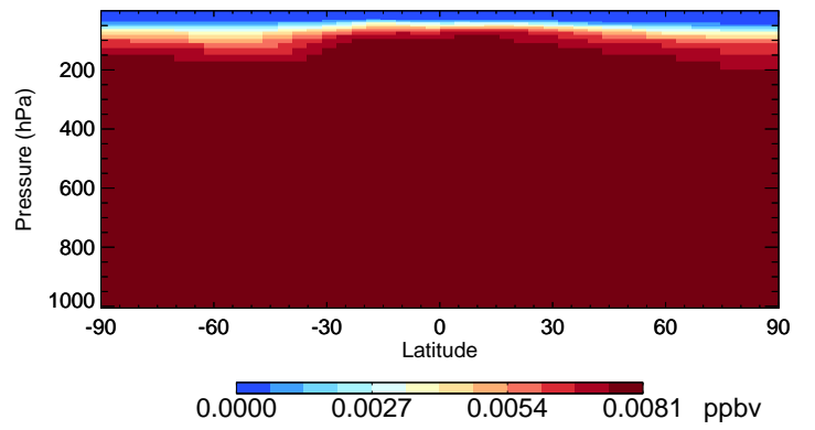
v11-02e-Run1 CH3CCI3 - Species Curtain @ -180.000 for Jul
