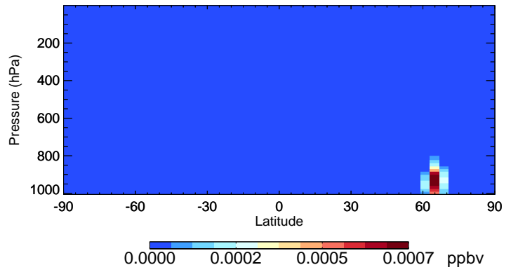
v11-02e-Run0 RIPD - Species Curtain @ -180.000 for Jul
