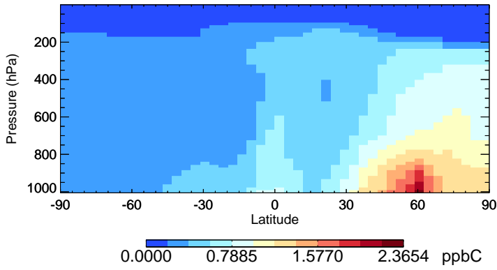
v11-02e-Run1 C2H6 - Species Zonal Mean for Jul
