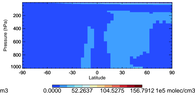
v11-02e-Run1 OH - Species Curtain @ -180.000 for Jul
