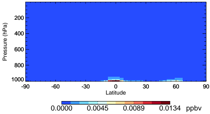
v11-02e-Run1 LIMO - Species Zonal Mean for Jul
