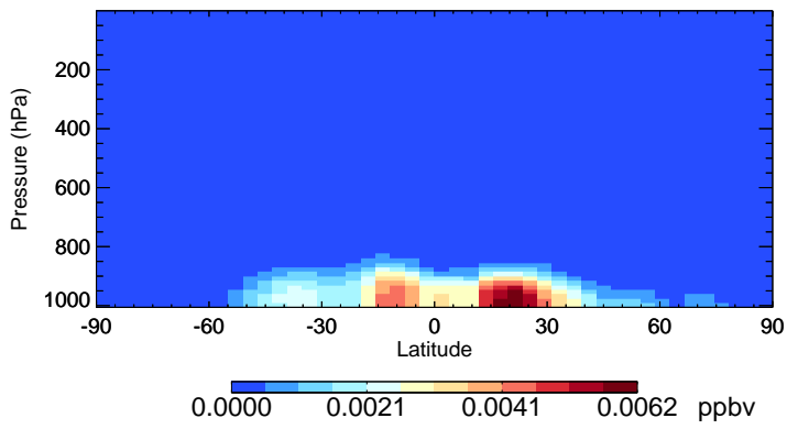
v11-02e-Run1 NITs - Species Zonal Mean for Jul
