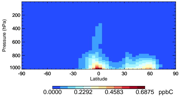
v11-02e-Run1 EOH - Species Zonal Mean for Jul
