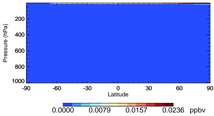
v11-02e-Run1 Br - Species Zonal Mean for Jul
