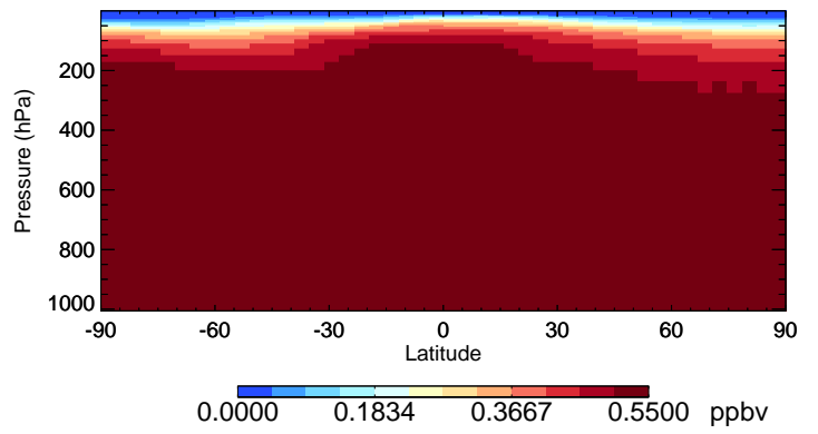
v11-02e-Run0 CH3Cl - Species Curtain @ -180.000 for Jul
