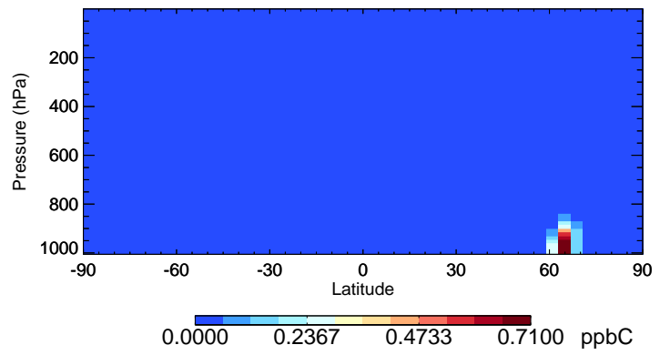
v11-02e-Run1 ISOP - Species Curtain @ -180.000 for Jul
