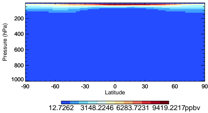
v11-02e-Run1 O3 - Species Zonal Mean for Jul
