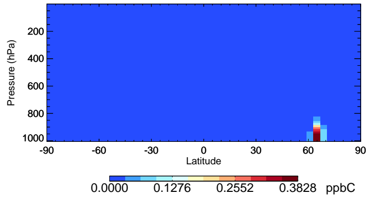
v11-02e-Run0 ISOP - Species Curtain @ -180.000 for Jul
