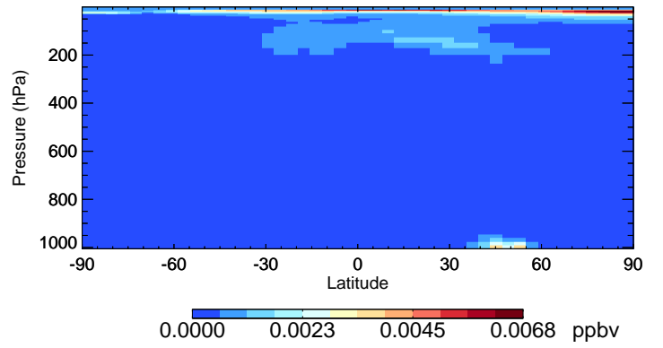
v11-02e-Run0 HNO 2 - Species Curtain @ -180.000 for Jul
