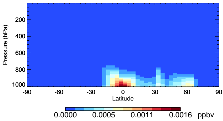
v11-02e-Run1 MOBA - Species Zonal Mean for Jul
