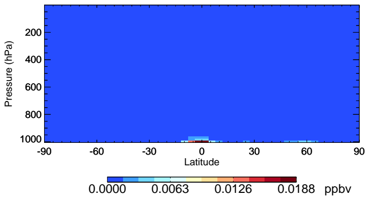
v11-02e-Run1 MTPO - Species Zonal Mean for Jul
