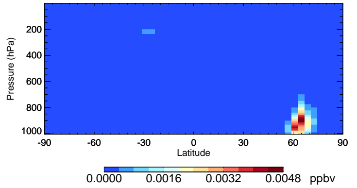
v11-02e-Run1 IEPOXB - Species Curtain @ -180.000 for Jul
