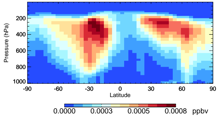
v11-02e-Run1 R4N2 - Species Curtain @ -180.000 for Jul
