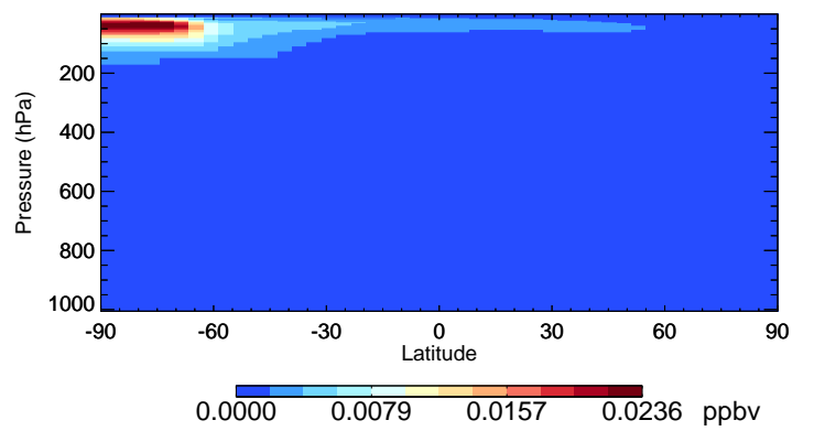
v11-02f-Run1 BrCl - Species Curtain @ -180.000 for Jul
