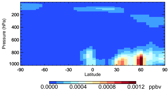
v11-02f-Run1 ASOA2 - Species Zonal Mean for Jul
