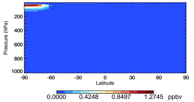
v11-02e-Run1 HOCl - Species Curtain @ -180.000 for Jul
