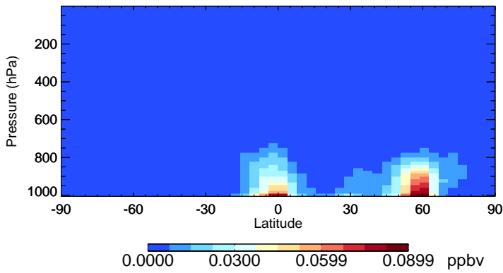
v11-02f-Run1 TSOA2 - Species Zonal Mean for Jul
