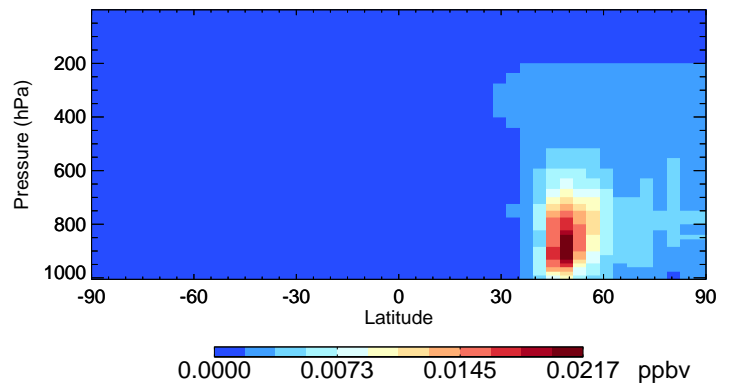
v11-02e-Run0 SOAGX - Species Curtain @ -180.000 for Jul
