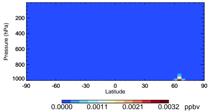
v11-02f-Run1 LIMO - Species Curtain @ -180.000 for Jul
