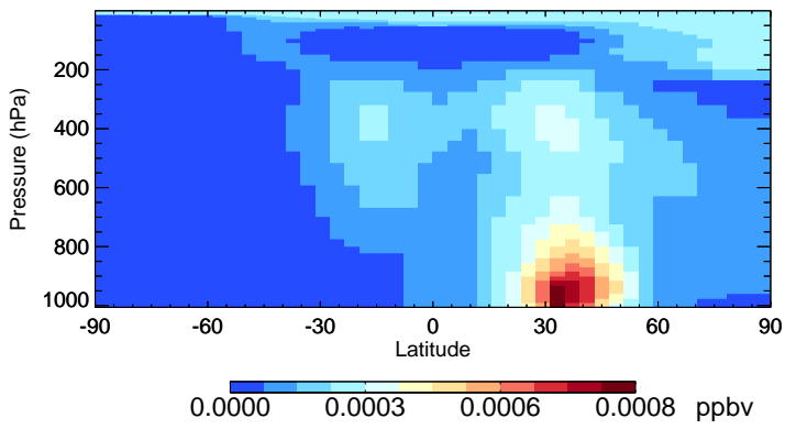
v11-02e-Run1 ASOG1 - Species Zonal Mean for Jul
