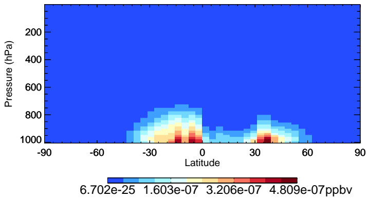
v11-02f-Run1 NPMN - Species Zonal Mean for Jul
