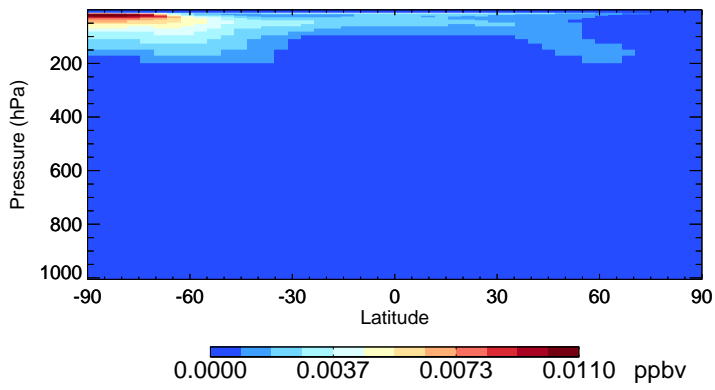
v11-02e-Run1 HOBr - Species Zonal Mean for Jul
