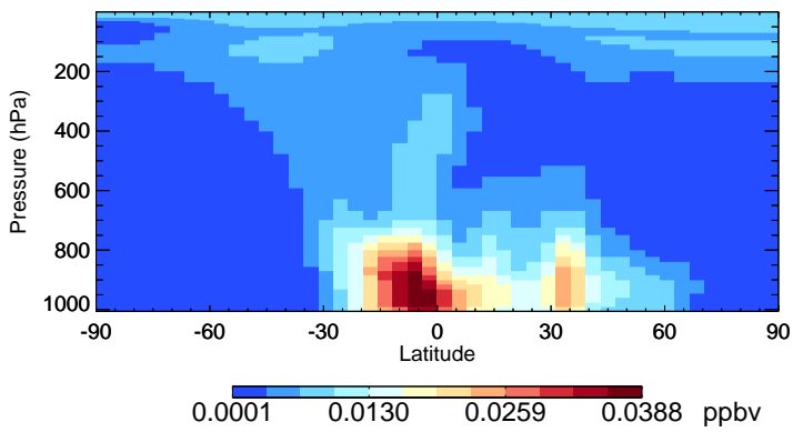
v11-02f-Run1 ISO3 - Species Zonal Mean for Jul
