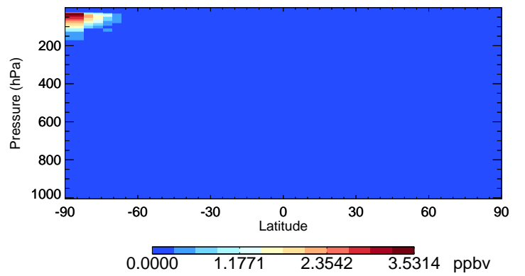
v11-02f-Run1 NIT - Species Curtain @ -180.000 for Jul
