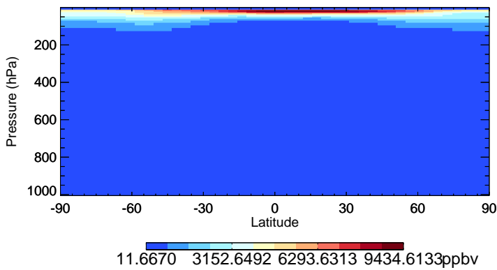
v11-02f-Run1 O3 - Species Zonal Mean for Jul
