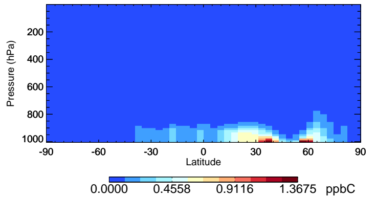
v11-02f-Run1 ALD2 - Species Curtain @ -180.000 for Jul
