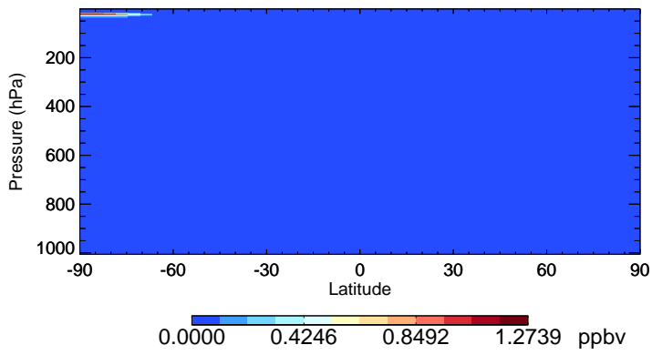
v11-02e-Run0 Cl2 - Species Zonal Mean for Jul
