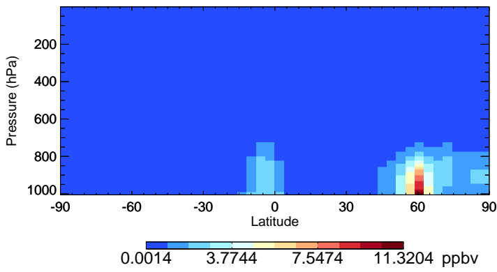
v11-02e-Run1 OCPI - Species Zonal Mean for Jul
