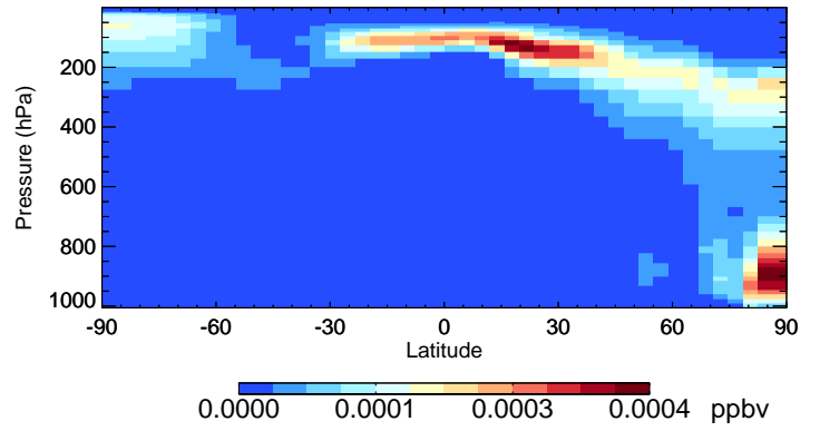
v11-02e-Run1 ASOA2 - Species Curtain @ -180.000 for Jul
