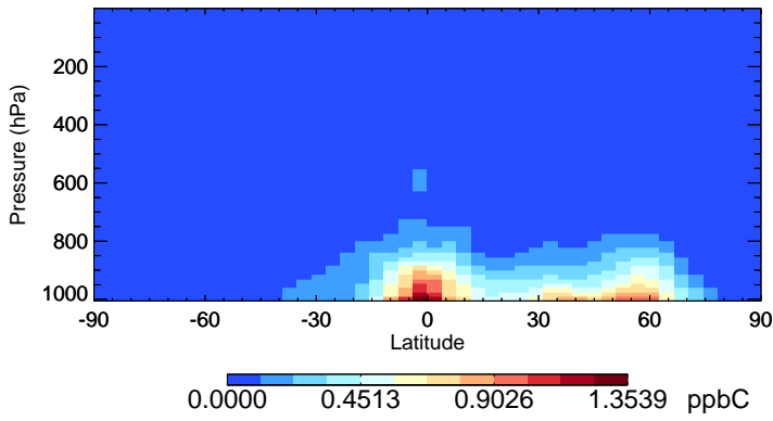
v11-02e-Run0 ALD2 - Species Zonal Mean for Jul
