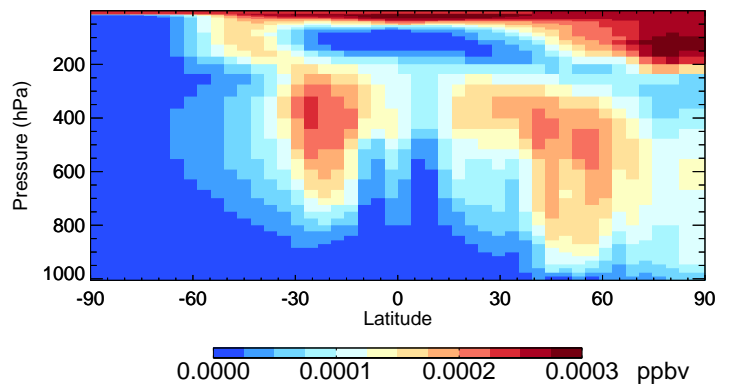
v11-02f-Run1 ASOG1 - Species Curtain @ -180.000 for Jul
