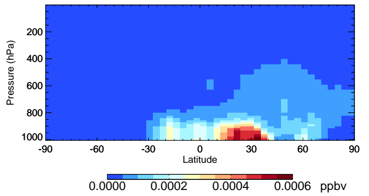
v11-02e-Run0 ACTA - Species Curtain @ -180.000 for Jul
