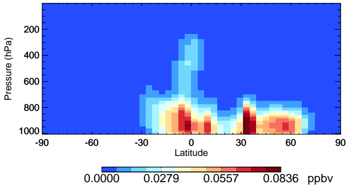
v11-02e-Run1 HAC - Species Zonal Mean for Jul
