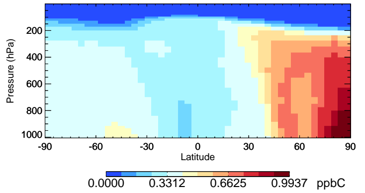
v11-02e-Run0 C2H6 - Species Curtain @ -180.000 for Jul
