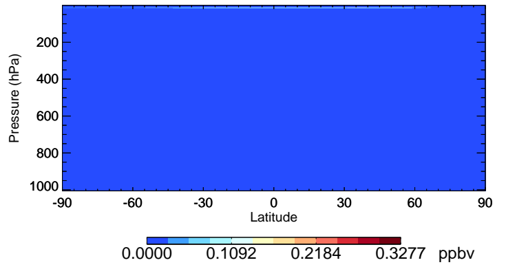
v11-02e-Run0 NO3 - Species Curtain @ -180.000 for Jul
