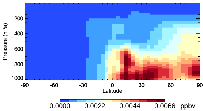
v11-02f-Run1 ASOAN - Species Zonal Mean for Jul
