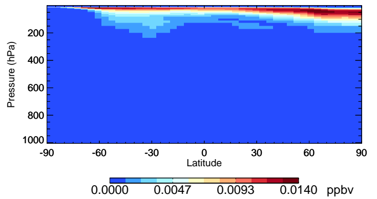
v11-02f-Run1 BrNO3 - Species Curtain @ -180.000 for Jul
