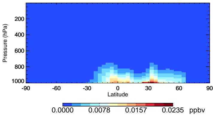
v11-02e-Run1 GLYX - Species Zonal Mean for Jul
