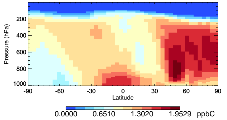
v11-02e-Run0 ACET - Species Curtain @ -180.000 for Jul
