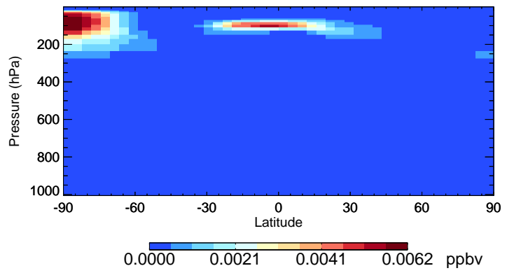
v11-02e-Run1 ISOA3 - Species Curtain @ -180.000 for Jul
