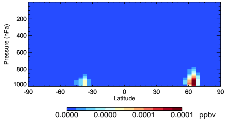
v11-02e-Run1 ISN1 - Species Curtain @ -180.000 for Jul
