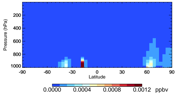
v11-02f-Run1 GLYX - Species Curtain @ -180.000 for Jul
