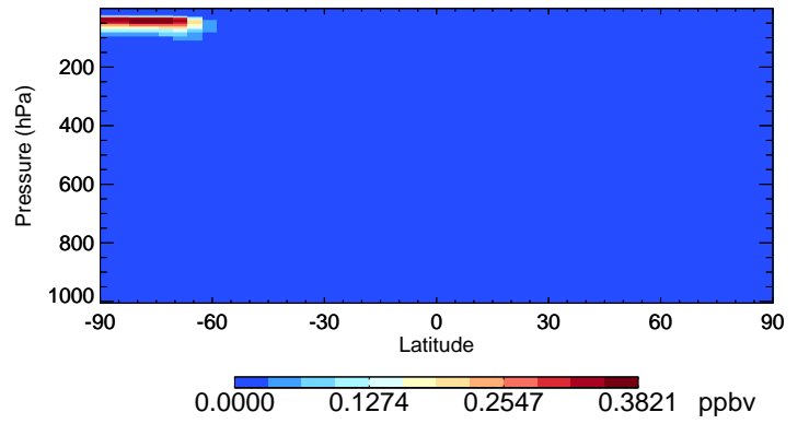
v11-02e-Run0 Cl2O2 - Species Curtain @ -180.000 for Jul
