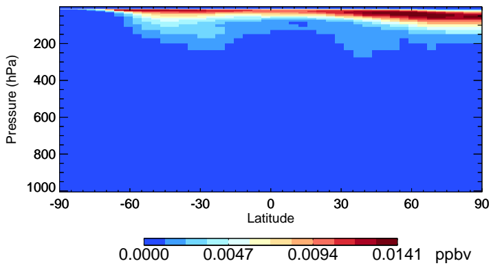
v11-02e-Run1 BrNO3 - Species Zonal Mean for Jul
