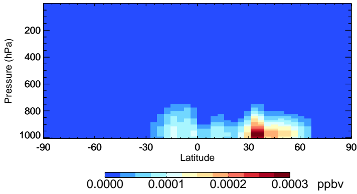
v11-02e-Run1 ETHLN - Species Zonal Mean for Jul
