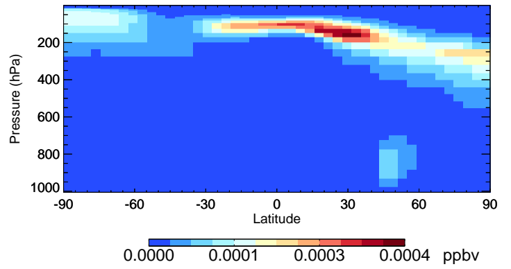
v11-02e-Run0 ASOA2 - Species Curtain @ -180.000 for Jul
