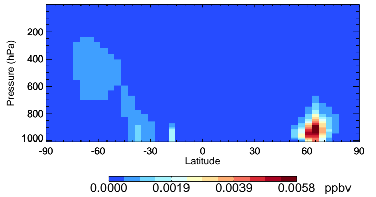
v11-02f-Run1 GLYC - Species Curtain @ -180.000 for Jul
