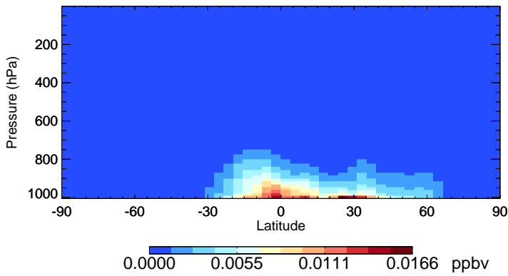
v11-02f-Run1 GLYX - Species Zonal Mean for Jul
