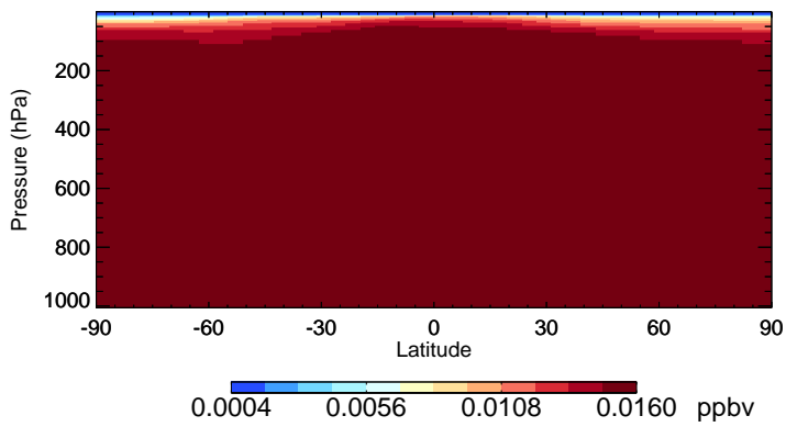
v11-02f-Run1 CFC114 - Species Zonal Mean for Jul
