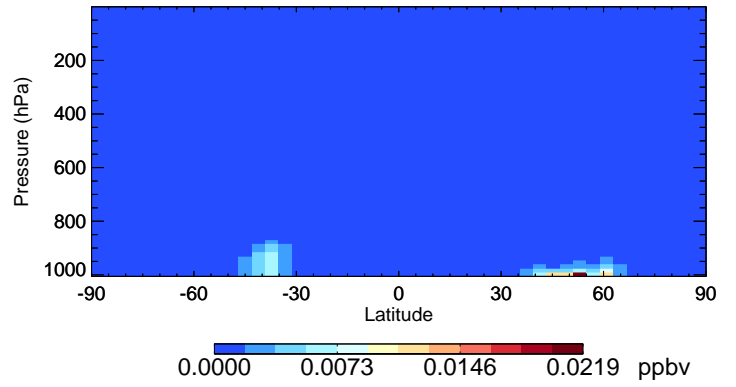
v11-02e-Run1 BCPO - Species Curtain @ -180.000 for Jul
