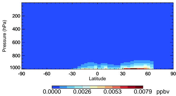
v11-02f-Run1 MONITS - Species Zonal Mean for Jul
