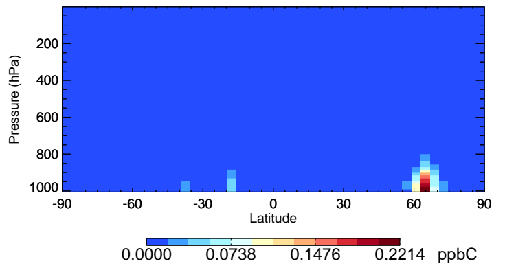
v11-02e-Run1 PRPE - Species Curtain @ -180.000 for Jul
