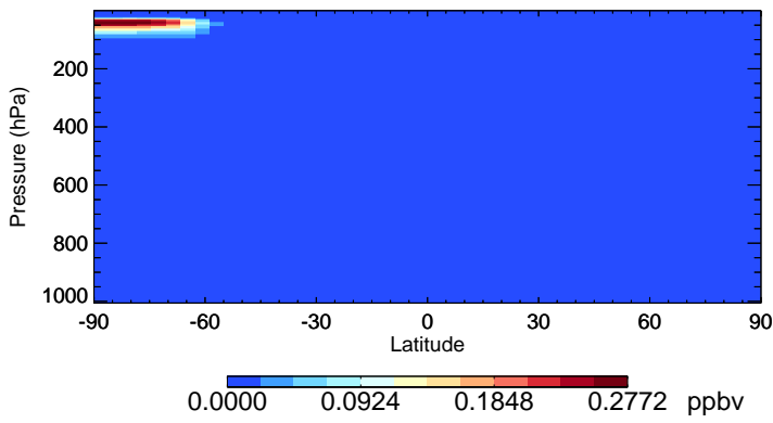
v11-02e-Run1 Cl2O2 - Species Zonal Mean for Jul
