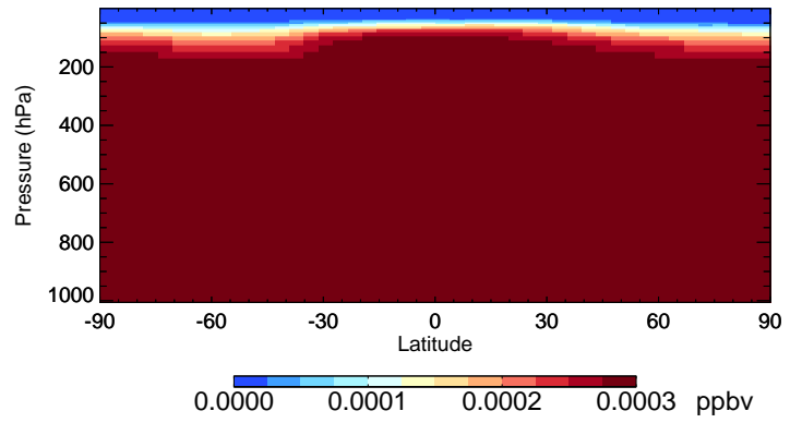
v11-02e-Run0 H2402 - Species Curtain @ -180.000 for Jul
