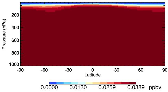
v11-02e-Run1 HCFC141b - Species Zonal Mean for Jul
