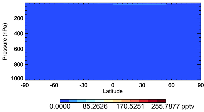
v11-02e-Run1 HO2 - Species Zonal Mean for Jul
