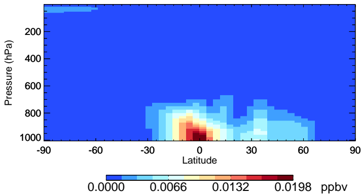
v11-02f-Run1 ISOA1 - Species Zonal Mean for Jul
