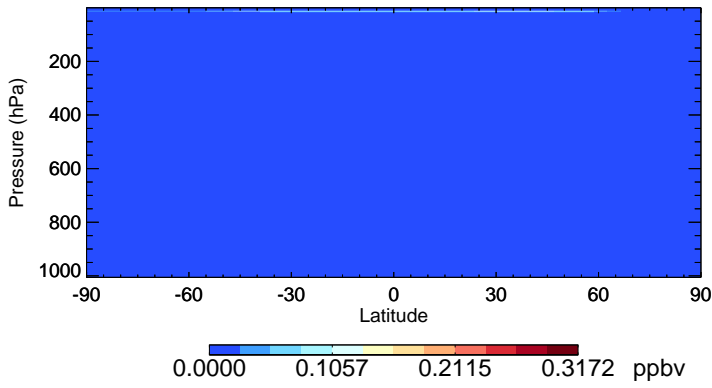
v11-02e-Run0 NO3 - Species Zonal Mean for Jul
