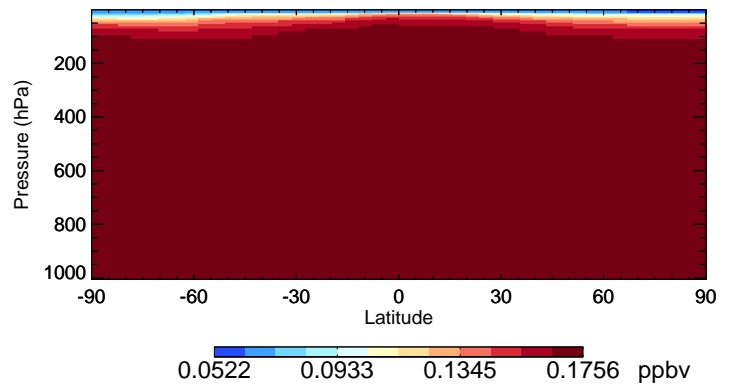
v11-02e-Run0 HCFC22 - Species Curtain @ -180.000 for Jul
