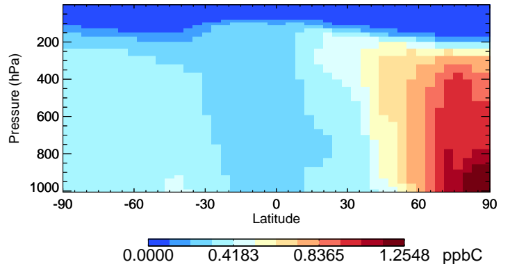
v11-02e-Run1 C2H6 - Species Curtain @ -180.000 for Jul
