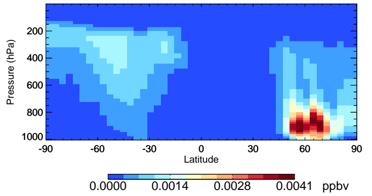
v11-02e-Run0 IMAE - Species Curtain @ -180.000 for Jul
