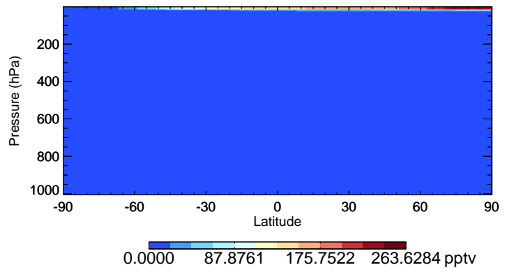
v11-02e-Run0 HO2 - Species Curtain @ -180.000 for Jul
