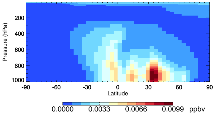
v11-02e-Run1 ISOG1 - Species Zonal Mean for Jul
