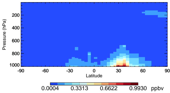
v11-02e-Run1 SO2 - Species Zonal Mean for Jul
