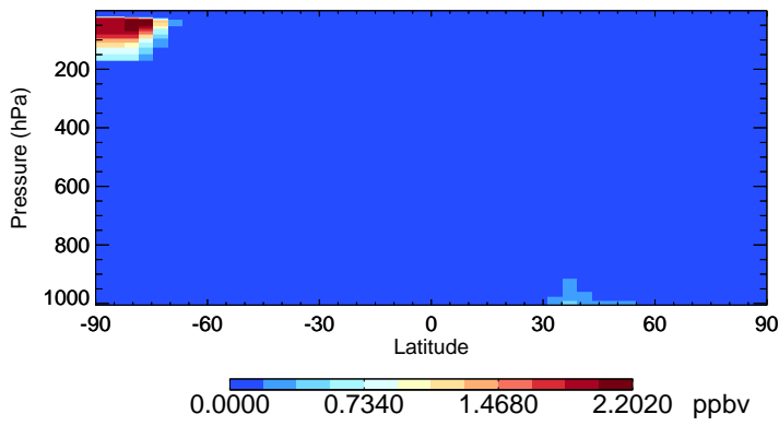
v11-02e-Run0 NIT - Species Zonal Mean for Jul
