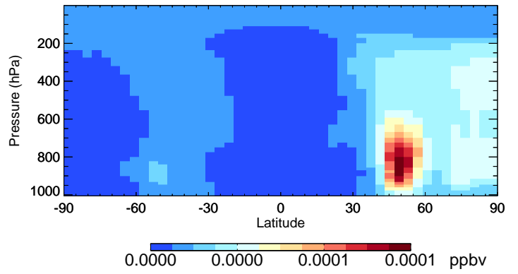
v11-02e-Run0 ISN10A - Species Curtain @ -180.000 for Jul
