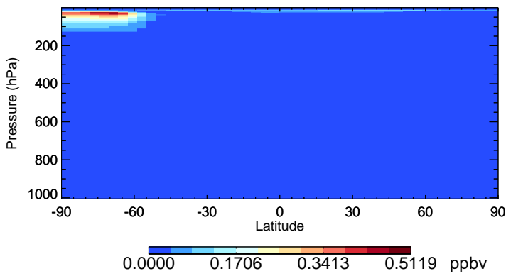
v11-02f-Run1 HOCl - Species Zonal Mean for Jul
