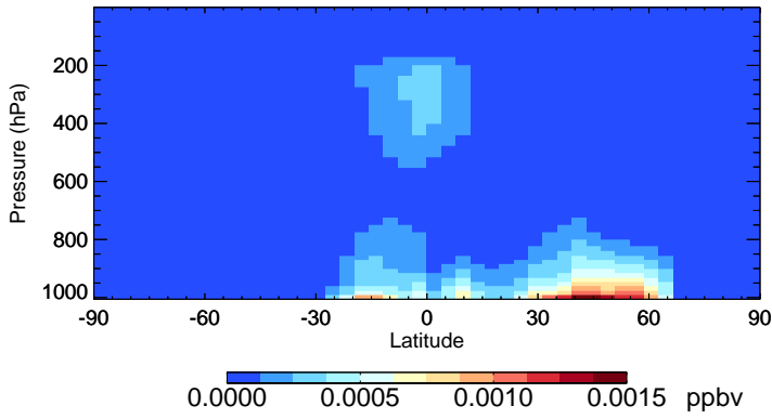
v11-02e-Run1 HONIT - Species Zonal Mean for Jul
