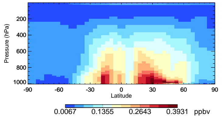
v11-02f-Run1 CH2O - Species Curtain @ -180.000 for Jul
