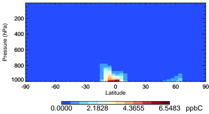
v11-02e-Run1 ISOP - Species Zonal Mean for Jul
