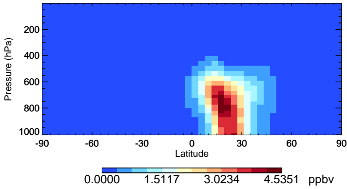
v11-02e-Run1 DST1 - Species Zonal Mean for Jul
