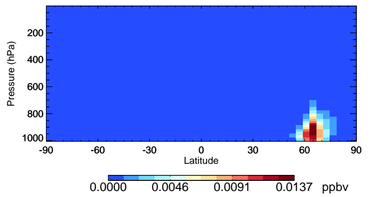
v11-02e-Run1 IPMN - Species Curtain @ -180.000 for Jul
