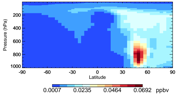
v11-02e-Run0 SOAS - Species Curtain @ -180.000 for Jul
