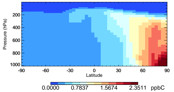
v11-02f-Run1 C2H6 - Species Curtain @ -180.000 for Jul
