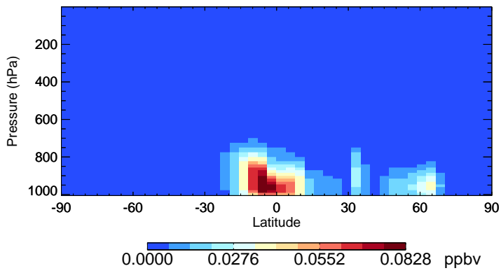
v11-02e-Run1 RIPA - Species Zonal Mean for Jul
