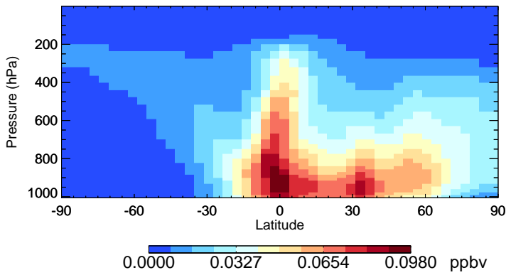
v11-02f-Run1 MAP - Species Zonal Mean for Jul
