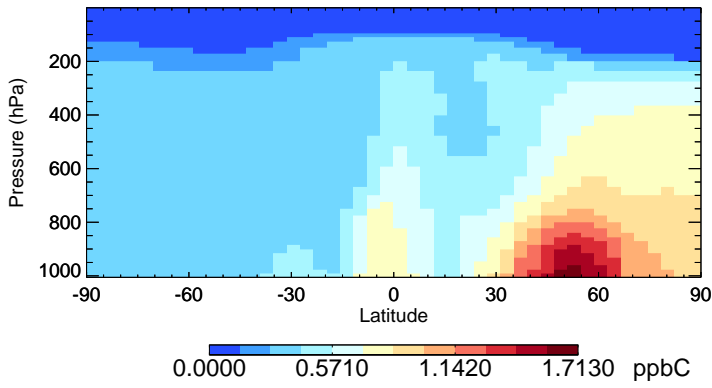
v11-02e-Run0 C2H6 - Species Zonal Mean for Jul
