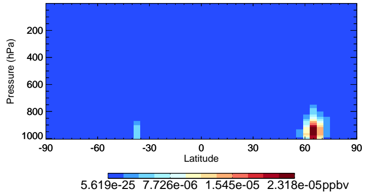
v11-02e-Run1 MACRN - Species Curtain @ -180.000 for Jul
