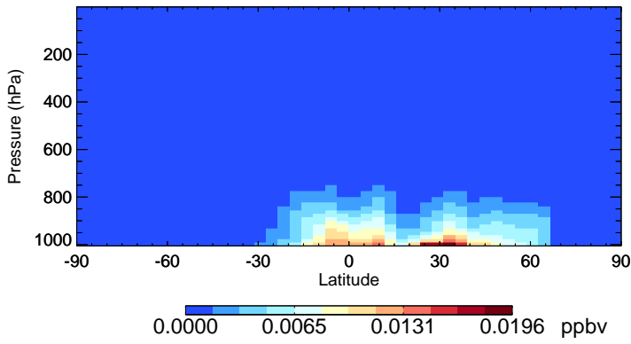
v11-02e-Run0 GLYX - Species Zonal Mean for Jul
