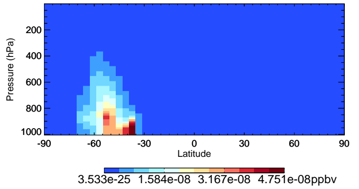
v11-02e-Run0 NPMN - Species Curtain @ -180.000 for Jul
