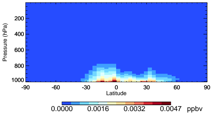
v11-02f-Run1 ISN1 - Species Zonal Mean for Jul
