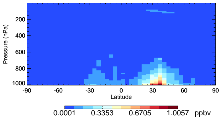
v11-02e-Run0 SO2 - Species Zonal Mean for Jul
