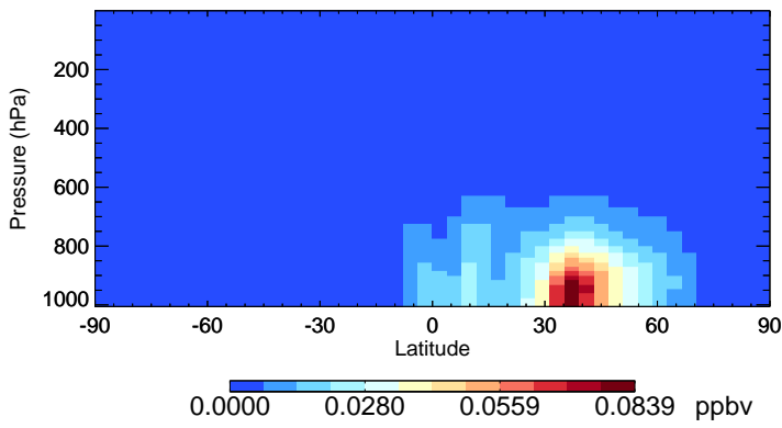
v11-02e-Run0 SOAGX - Species Zonal Mean for Jul
