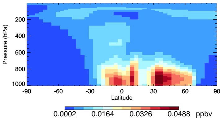
v11-02e-Run0 ISO3 - Species Zonal Mean for Jul
