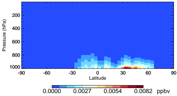
v11-02e-Run0 ISN1 - Species Zonal Mean for Jul
