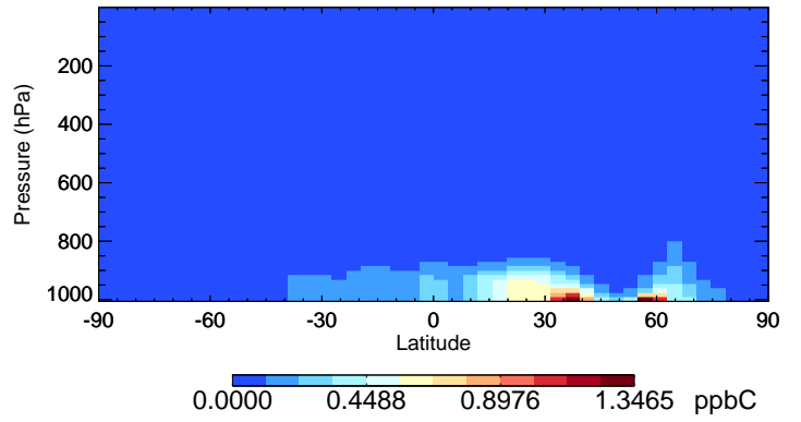
v11-02e-Run1 ALD2 - Species Curtain @ -180.000 for Jul
