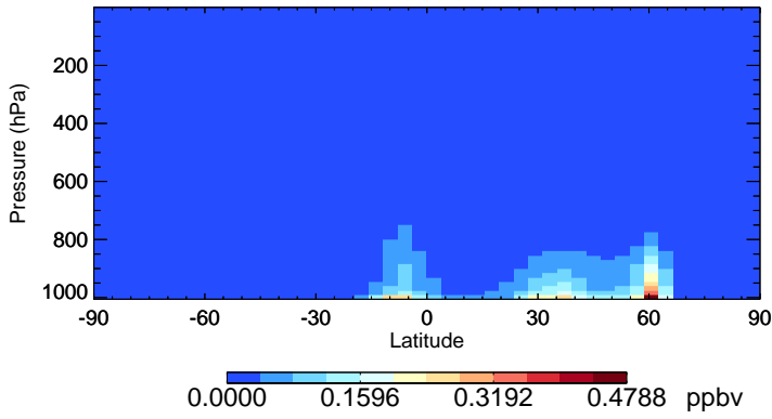
v11-02e-Run1 BCPO - Species Zonal Mean for Jul
