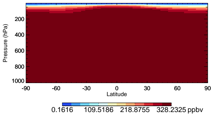
v11-02f-Run1 N2O - Species Zonal Mean for Jul
