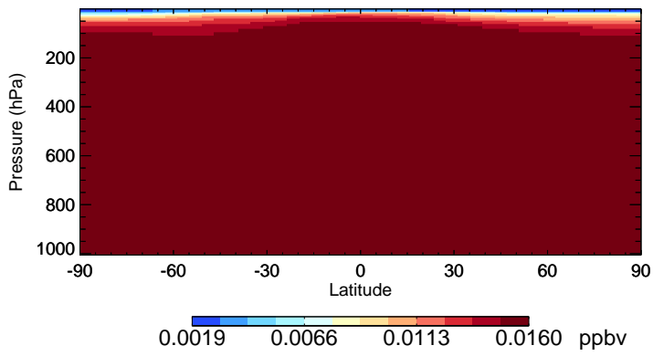
v11-02e-Run1 CFC114 - Species Zonal Mean for Jul
