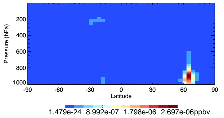
v11-02e-Run1 LVOC - Species Curtain @ -180.000 for Jul
