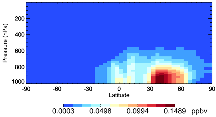
v11-02e-Run0 INDIOL - Species Zonal Mean for Jul
