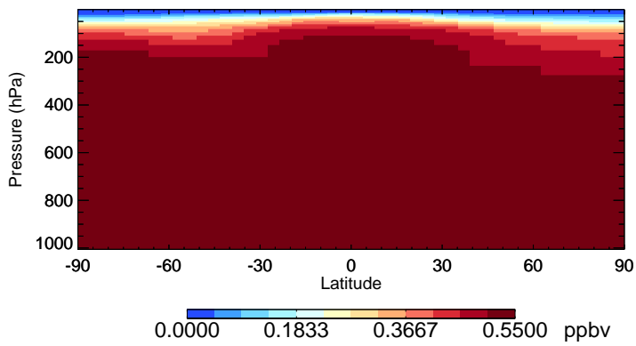
v11-02f-Run1 CH3Cl - Species Zonal Mean for Jul
