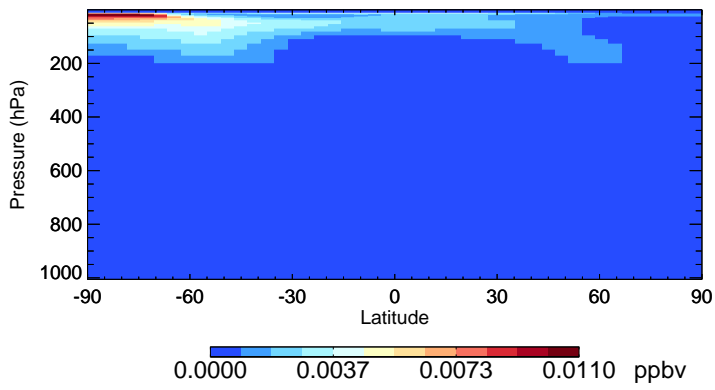
v11-02e-Run0 HOBr - Species Zonal Mean for Jul
