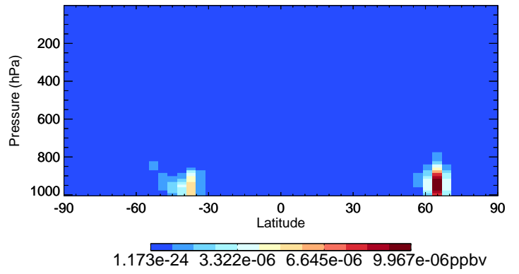
v11-02e-Run0 ETHLN - Species Curtain @ -180.000 for Jul
