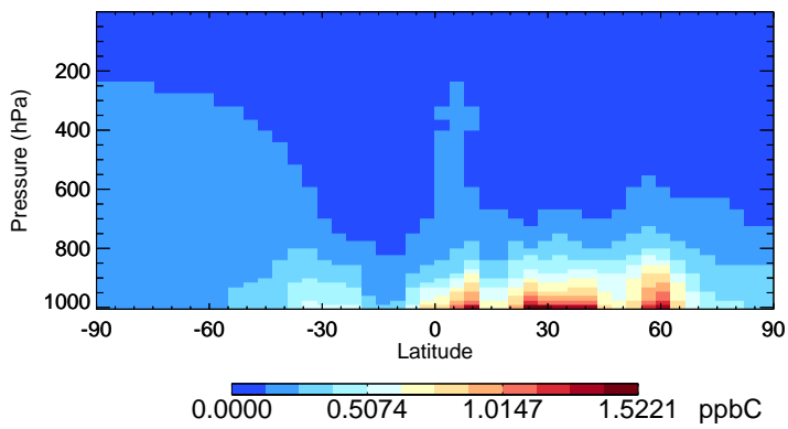
v11-02f-Run1 ALK4 - Species Zonal Mean for Jul
