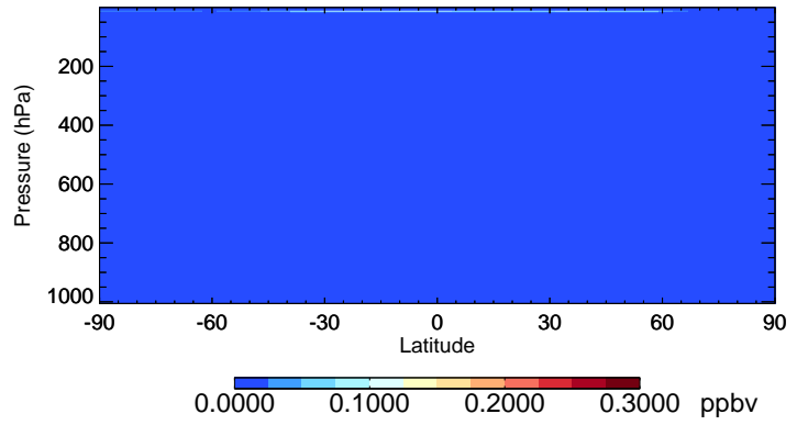
v11-02e-Run1 NO3 - Species Curtain @ -180.000 for Jul
