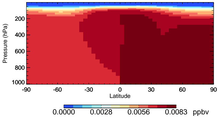
v11-02e-Run0 CH3Br - Species Zonal Mean for Jul
