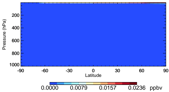
v11-02f-Run1 Br - Species Zonal Mean for Jul
