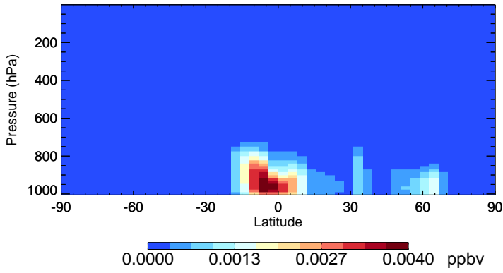
v11-02e-Run1 RIPD - Species Zonal Mean for Jul
