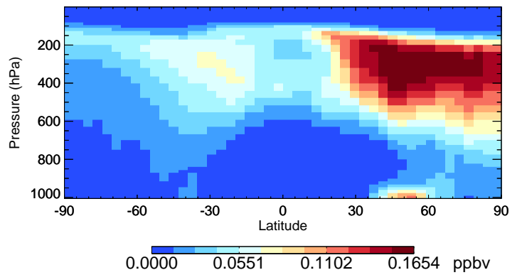
v11-02e-Run0 PAN - Species Curtain @ -180.000 for Jul
