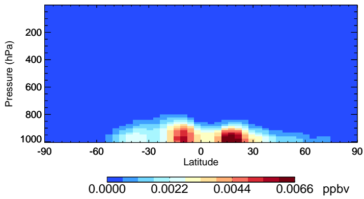
v11-02e-Run0 NITs - Species Zonal Mean for Jul
