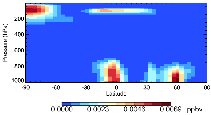
v11-02e-Run1 ISOA3 - Species Zonal Mean for Jul
