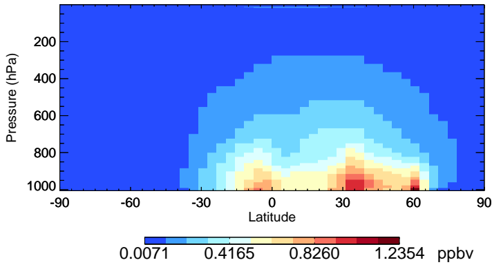
v11-02e-Run1 CH2O - Species Zonal Mean for Jul
