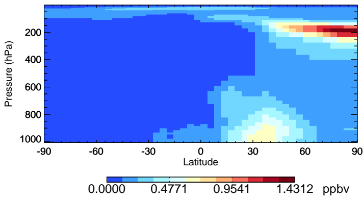
v11-02e-Run1 SO4 - Species Zonal Mean for Jul
