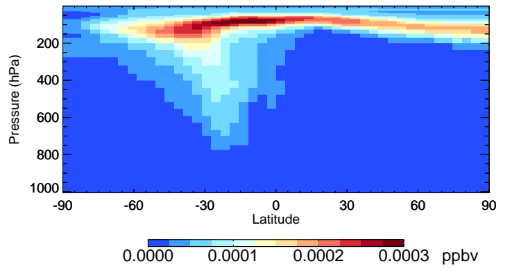
v11-02f-Run1 DHDN - Species Curtain @ -180.000 for Jul
