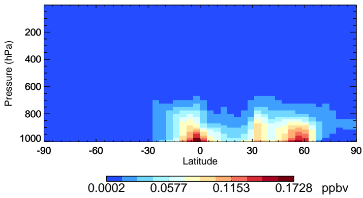
v11-02e-Run1 TSOG3 - Species Zonal Mean for Jul
