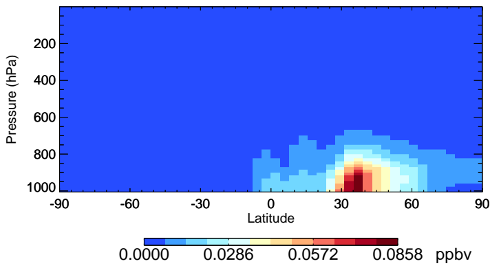
v11-02e-Run1 SOAGX - Species Zonal Mean for Jul
