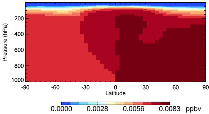
v11-02f-Run1 CH3Br - Species Zonal Mean for Jul
