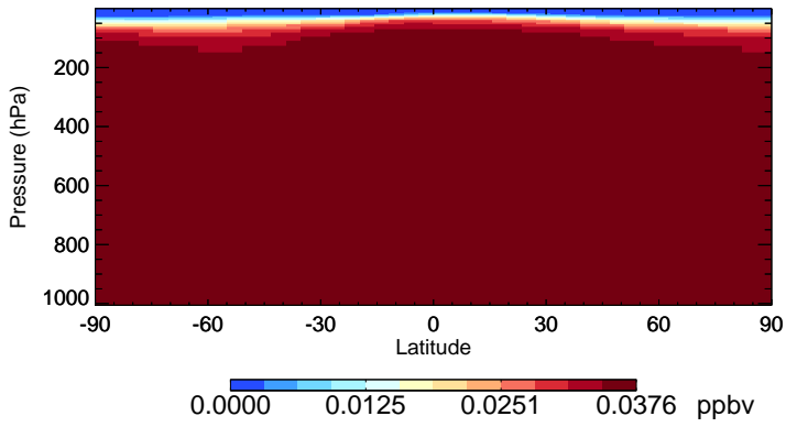
v11-02e-Run0 HCFC141b - Species Zonal Mean for Jul
