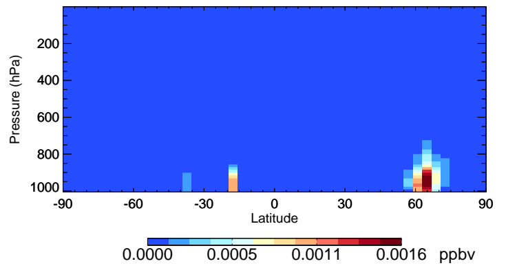
v11-02e-Run1 GLYX - Species Curtain @ -180.000 for Jul
