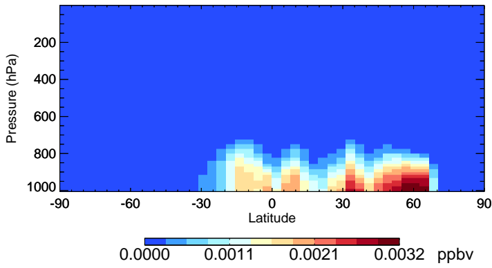
v11-02e-Run0 ISOPNB - Species Zonal Mean for Jul
