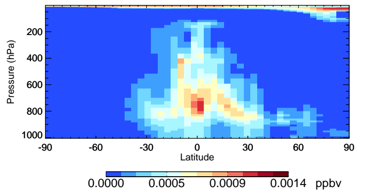
v11-02f-Run1 HBr - Species Curtain @ -180.000 for Jul
