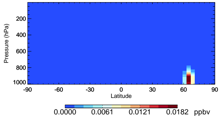
v11-02e-Run0 MACR - Species Curtain @ -180.000 for Jul
