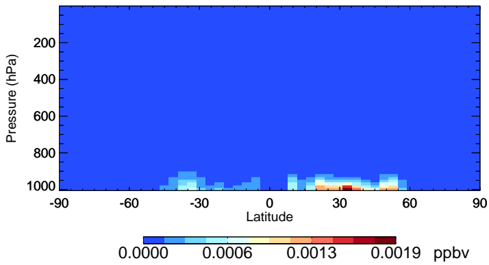
v11-02f-Run1 ClNO2 - Species Zonal Mean for Jul
