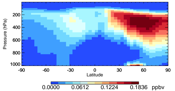
v11-02f-Run1 PAN - Species Curtain @ -180.000 for Jul
