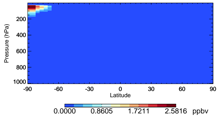
v11-02e-Run1 NIT - Species Curtain @ -180.000 for Jul
