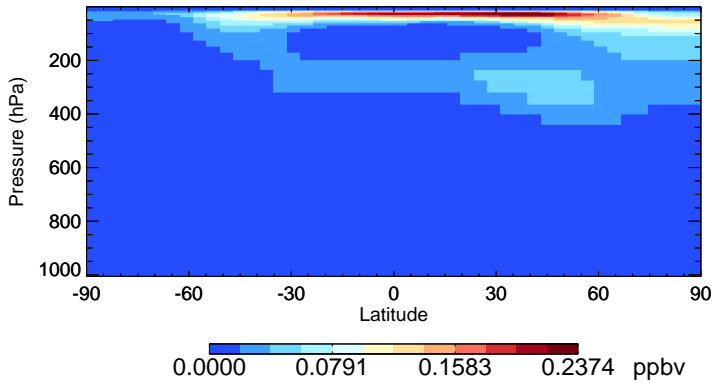
v11-02e-Run1 HNO4 - Species Zonal Mean for Jul
