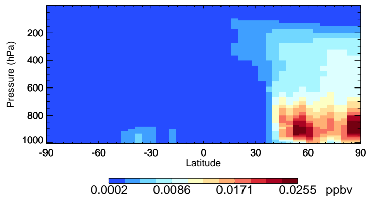
v11-02f-Run1 INDIOL - Species Curtain @ -180.000 for Jul
