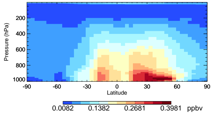
v11-02e-Run0 CH2O - Species Curtain @ -180.000 for Jul
