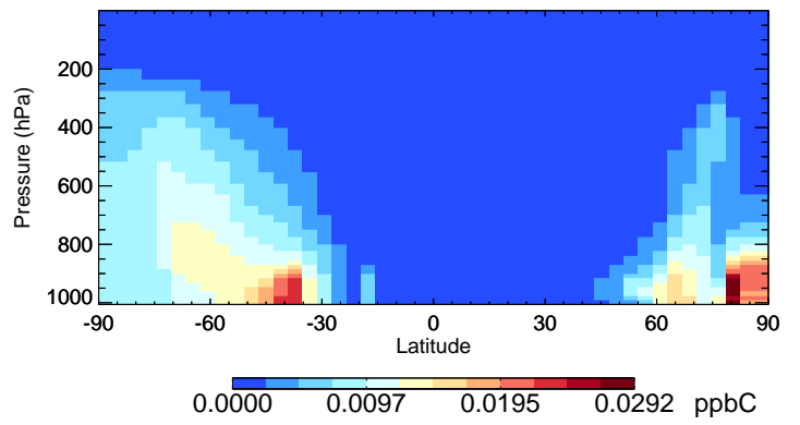
v11-02e-Run1 TOLU - Species Curtain @ -180.000 for Jul
