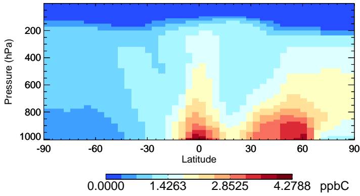
v11-02e-Run1 ACET - Species Zonal Mean for Jul
