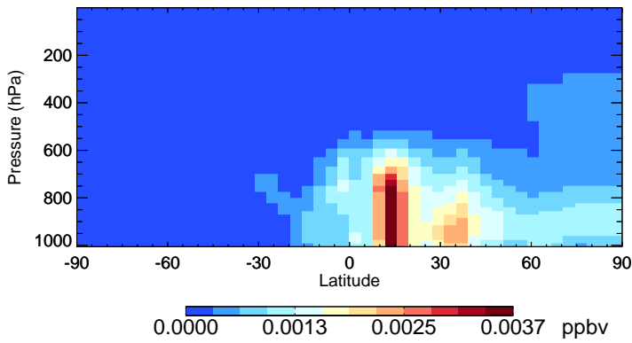
v11-02f-Run1 SOAME - Species Zonal Mean for Jul
