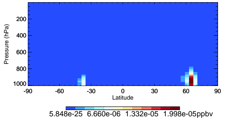
v11-02e-Run0 MACRN - Species Curtain @ -180.000 for Jul
