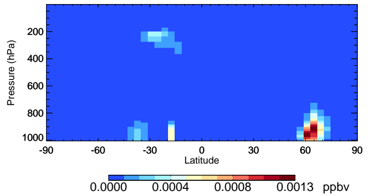
v11-02f-Run1 IEPOXB - Species Curtain @ -180.000 for Jul
