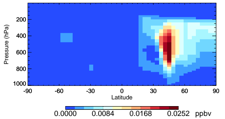
v11-02e-Run1 DST2 - Species Curtain @ -180.000 for Jul
