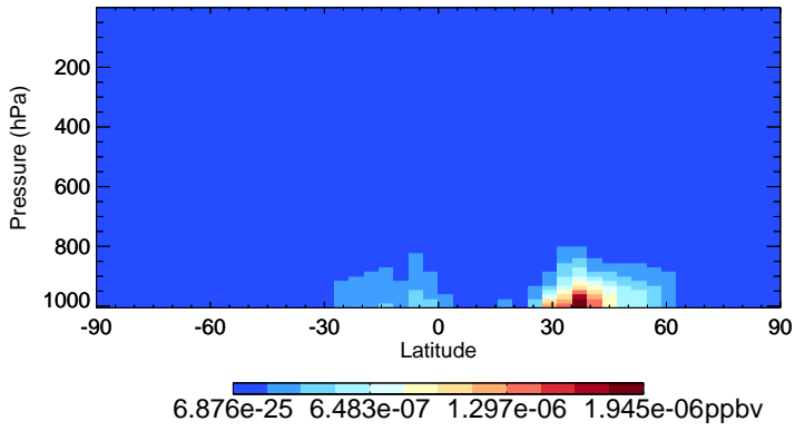
v11-02e-Run1 NPMN - Species Zonal Mean for Jul
