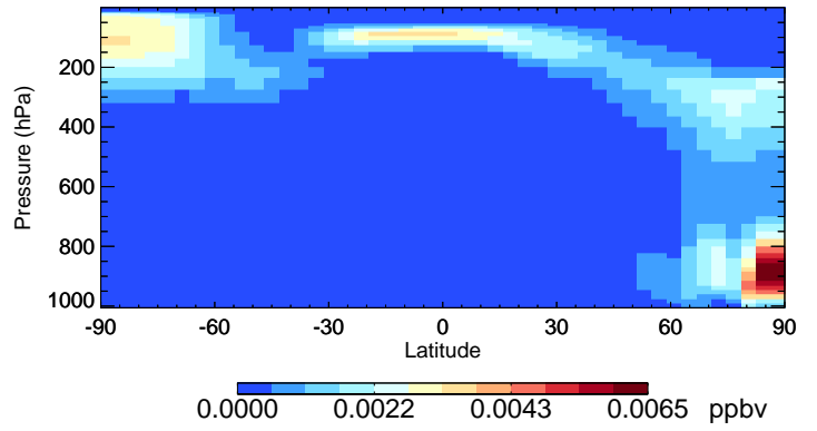
v11-02e-Run1 TSOA2 - Species Curtain @ -180.000 for Jul
