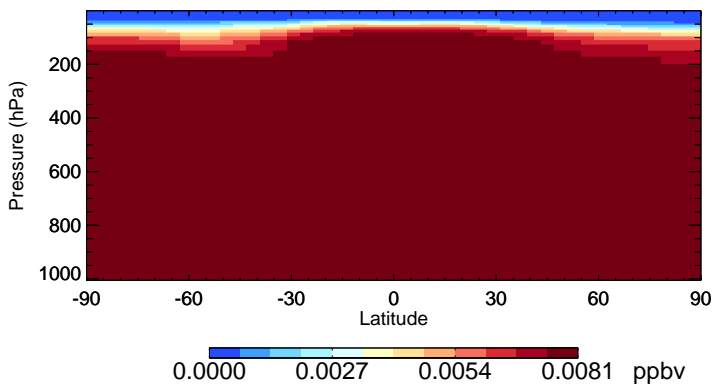
v11-02f-Run1 CH3CCI3 - Species Zonal Mean for Jul
