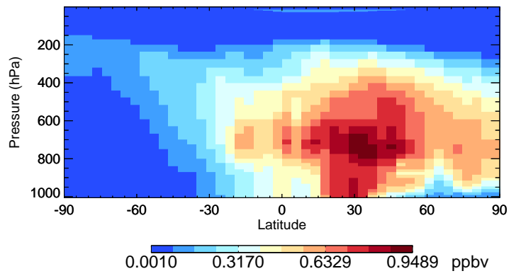
v11-02e-Run0 H2O2 - Species Curtain @ -180.000 for Jul
