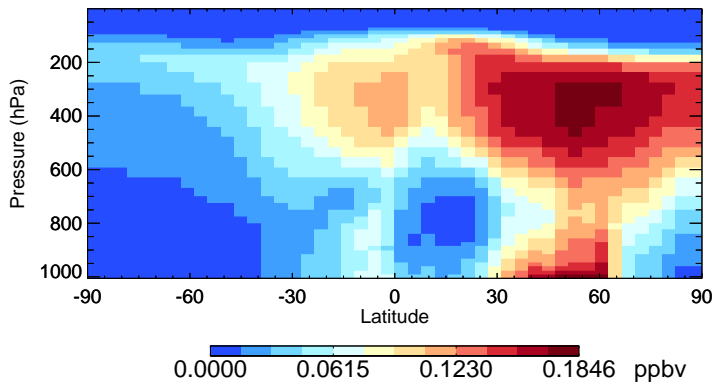
v11-02f-Run1 PAN - Species Zonal Mean for Jul
