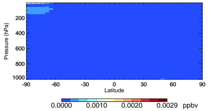
v11-02e-Run1 Br2 - Species Curtain @ -180.000 for Jul
