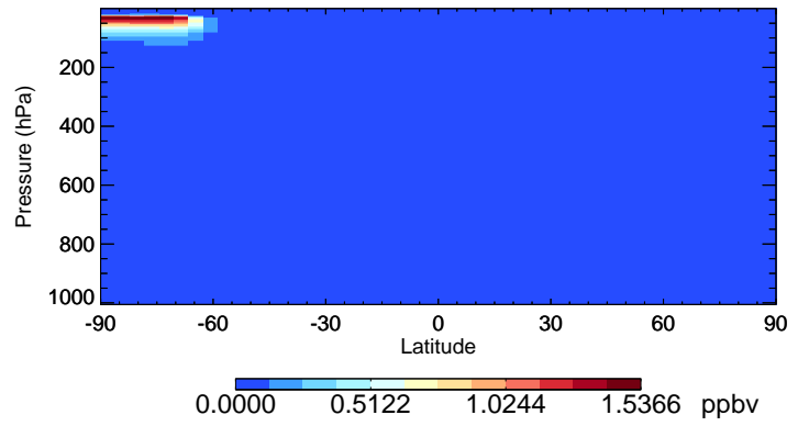
v11-02e-Run0 HOCl - Species Curtain @ -180.000 for Jul
