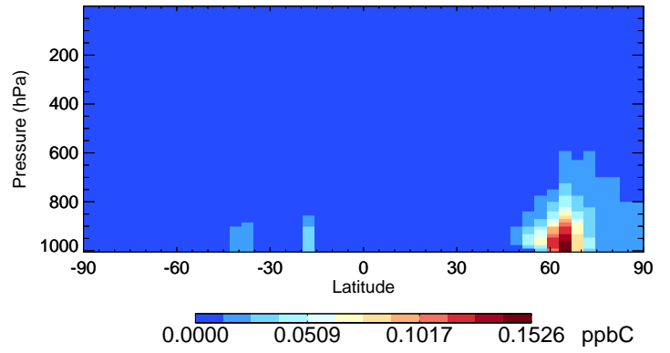
v11-02e-Run1 EOH - Species Curtain @ -180.000 for Jul
