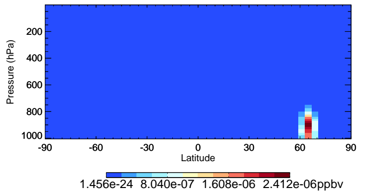
v11-02e-Run0 LVOC - Species Curtain @ -180.000 for Jul
