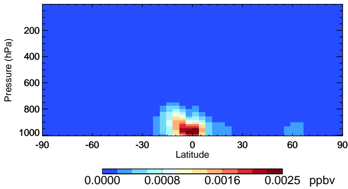
v11-02f-Run1 RIPD - Species Zonal Mean for Jul
