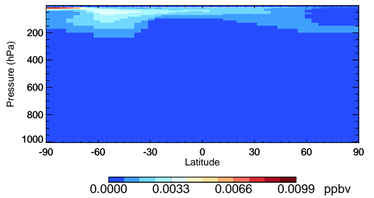
v11-02f-Run1 HOBr - Species Curtain @ -180.000 for Jul
