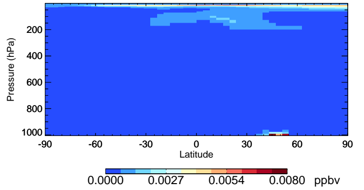
v11-02e-Run1 HNO 2 - Species Curtain @ -180.000 for Jul
