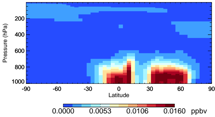
v11-02e-Run0 ISOA1 - Species Zonal Mean for Jul
