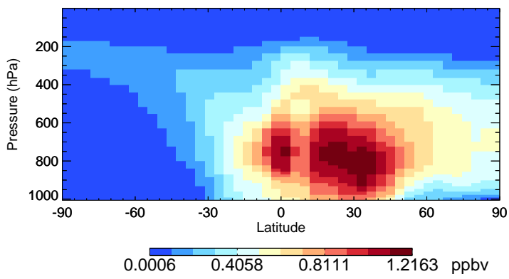
v11-02e-Run1 H2O2 - Species Zonal Mean for Jul
