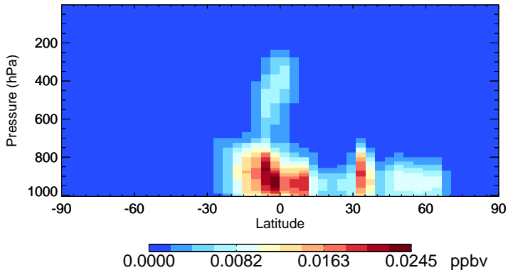
v11-02e-Run1 IEPOXB - Species Zonal Mean for Jul
