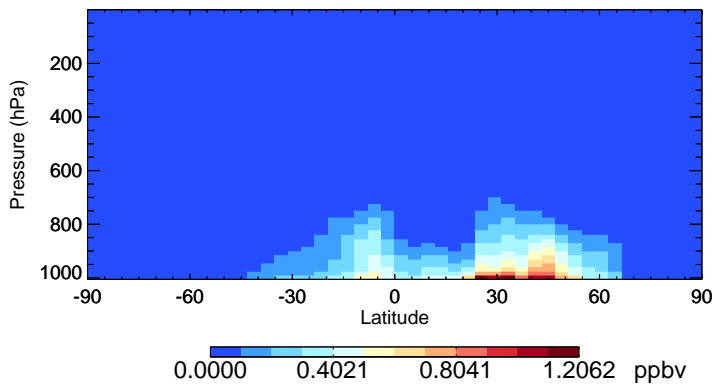
v11-02e-Run0 NH3 - Species Zonal Mean for Jul
