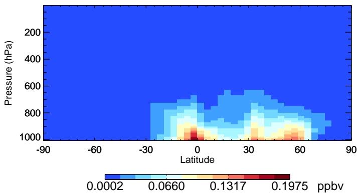
v11-02f-Run1 TSOG3 - Species Zonal Mean for Jul
