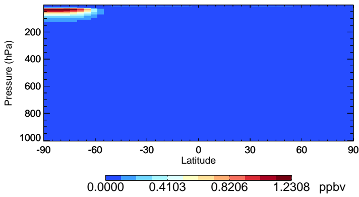
v11-02e-Run1 HOCl - Species Zonal Mean for Jul
