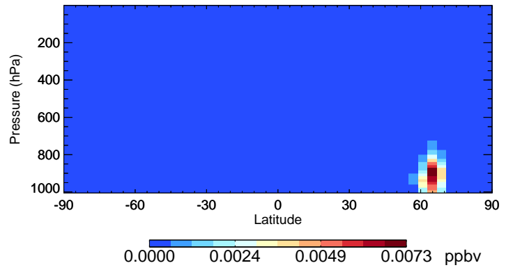
v11-02e-Run0 IEPOXA - Species Curtain @ -180.000 for Jul
