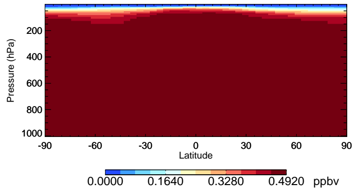
v11-02f-Run1 CFC12 - Species Curtain @ -180.000 for Jul
