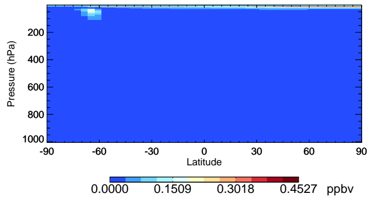
v11-02e-Run0 CIO - Species Curtain @ -180.000 for Jul
