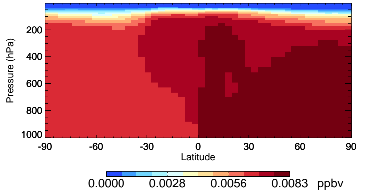
v11-02e-Run1 CH3Br - Species Curtain @ -180.000 for Jul
