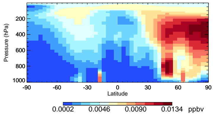
v11-02e-Run0 TSOG3 - Species Curtain @ -180.000 for Jul
