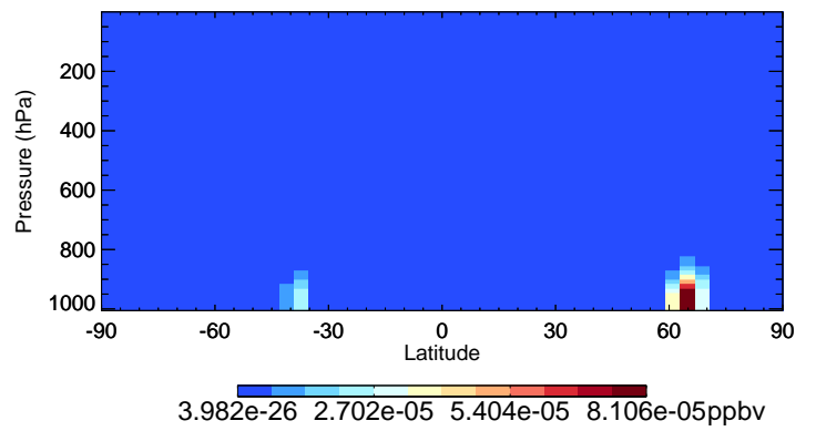
v11-02f-Run1 MOBA - Species Curtain @ -180.000 for Jul
