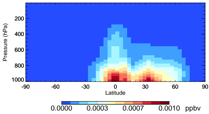
v11-02e-Run0 ACTA - Species Zonal Mean for Jul
