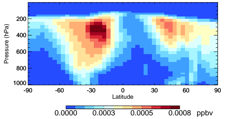
v11-02e-Run0 R4N2 - Species Curtain @ -180.000 for Jul
