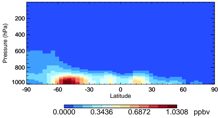
v11-02e-Run1 SALA - Species Zonal Mean for Jul
