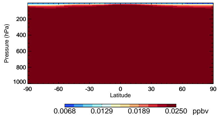
v11-02e-Run0 HCFC142b - Species Curtain @ -180.000 for Jul
