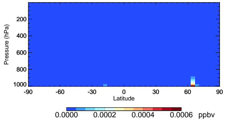
v11-02e-Run0 LIMO - Species Curtain @ -180.000 for Jul
