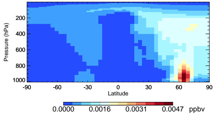
v11-02e-Run1 IONITA - Species Curtain @ -180.000 for Jul
