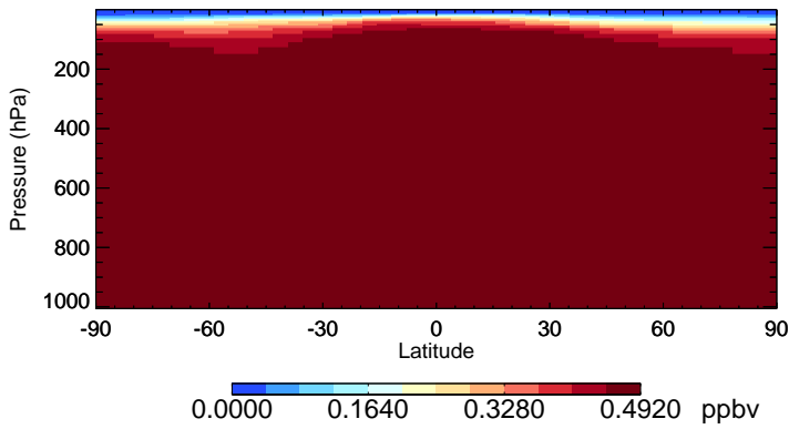
v11-02f-Run1 CFC12 - Species Zonal Mean for Jul
