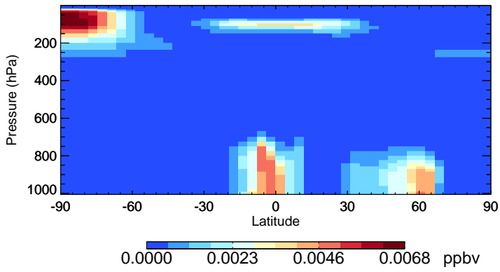
v11-02e-Run0 ISOA3 - Species Zonal Mean for Jul
