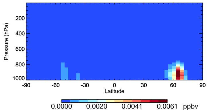
v11-02e-Run0 IPMN - Species Curtain @ -180.000 for Jul
