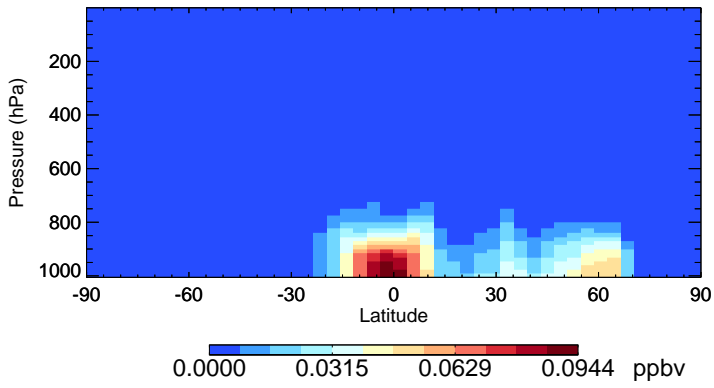
v11-02e-Run0 MACR - Species Zonal Mean for Jul
