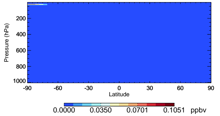
v11-02e-Run0 ClNO2 - Species Curtain @ -180.000 for Jul
