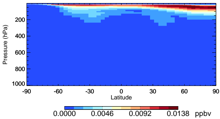
v11-02f-Run1 BrNO3 - Species Zonal Mean for Jul
