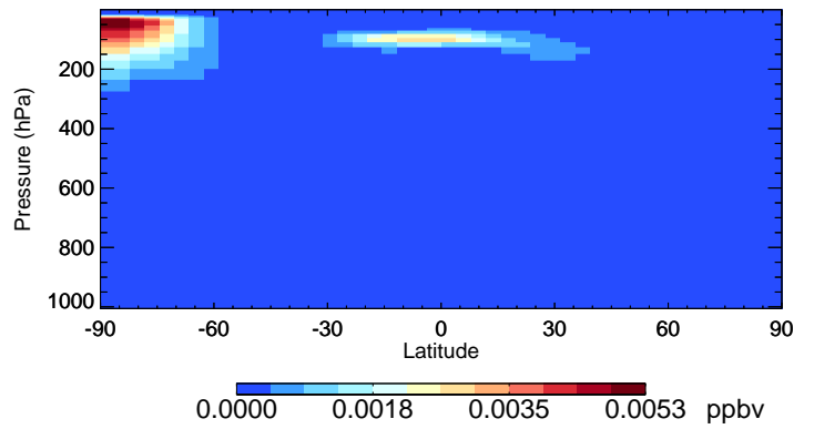
v11-02f-Run1 ISOA3 - Species Curtain @ -180.000 for Jul
