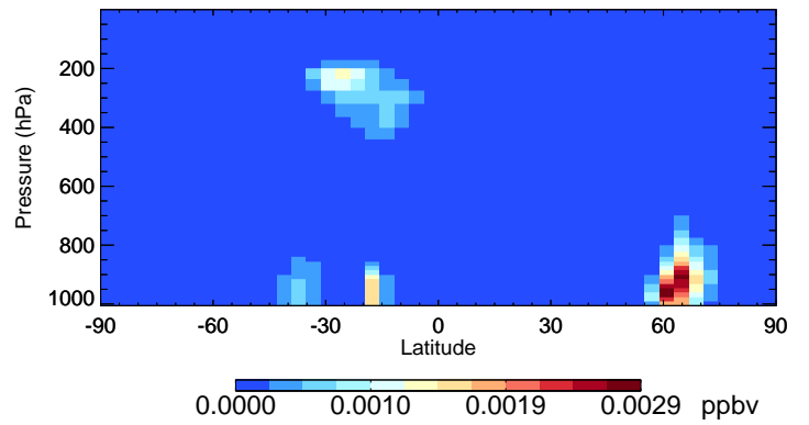
v11-02f-Run1 IEPOXA - Species Curtain @ -180.000 for Jul
