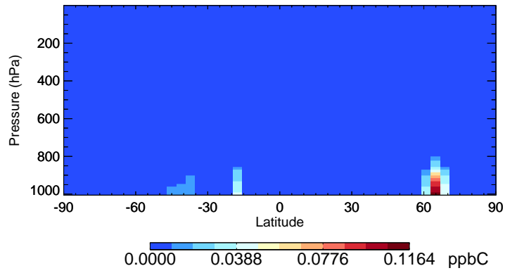
v11-02e-Run0 PRPE - Species Curtain @ -180.000 for Jul
