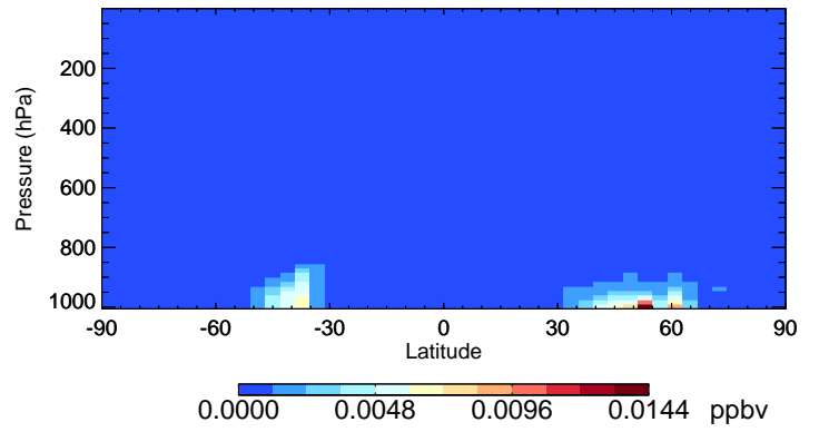
v11-02e-Run0 BCPO - Species Curtain @ -180.000 for Jul
