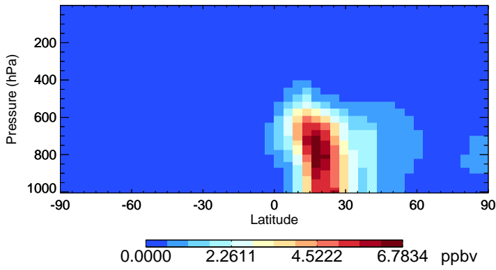
v11-02e-Run0 DST1 - Species Zonal Mean for Jul
