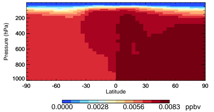
v11-02f-Run1 CH3Br - Species Curtain @ -180.000 for Jul
