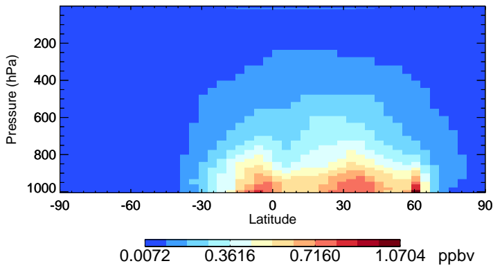
v11-02f-Run1 CH2O - Species Zonal Mean for Jul
