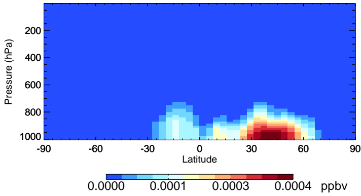
v11-02e-Run1 MACRN - Species Zonal Mean for Jul
