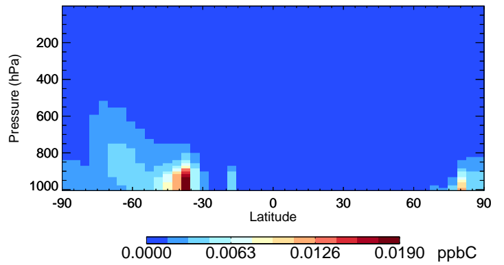
v11-02f-Run1 XYLE - Species Curtain @ -180.000 for Jul
