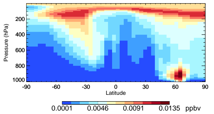
v11-02e-Run1 ISO3 - Species Curtain @ -180.000 for Jul
