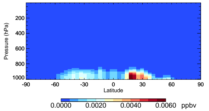
v11-02e-Run1 NITs - Species Curtain @ -180.000 for Jul
