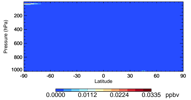
v11-02e-Run1 ClNO2 - Species Curtain @ -180.000 for Jul
