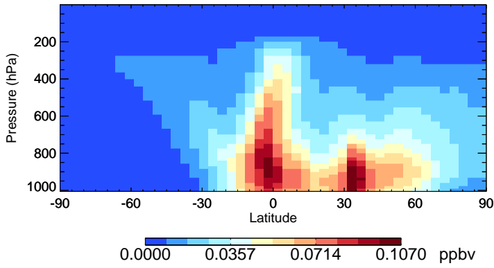
v11-02e-Run1 MAP - Species Zonal Mean for Jul
