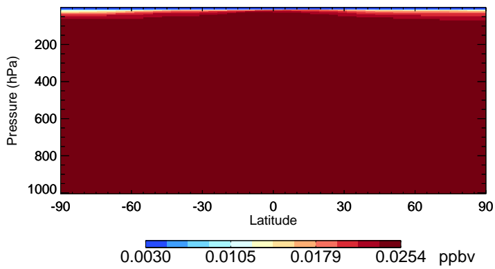
v11-02f-Run1 HCFC142b - Species Zonal Mean for Jul
