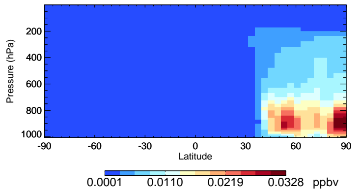
v11-02e-Run1 INDIOL - Species Curtain @ -180.000 for Jul
