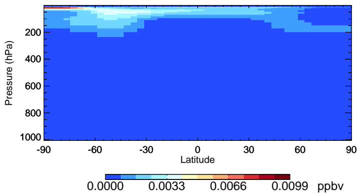
v11-02f-Run1 HOBr - Species Zonal Mean for Jul
