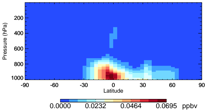
v11-02f-Run1 GLYC - Species Zonal Mean for Jul
