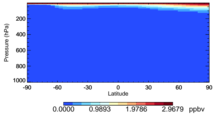
v11-02e-Run1 HCl - Species Curtain @ -180.000 for Jul
