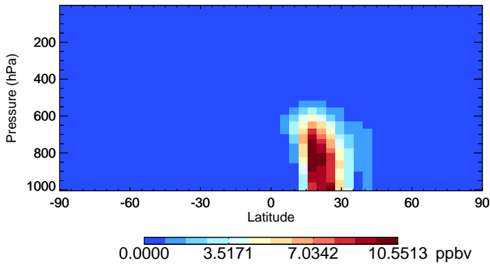
v11-02e-Run0 DST2 - Species Zonal Mean for Jul
