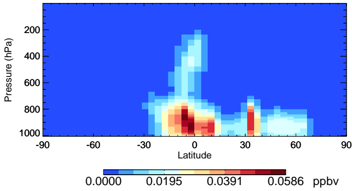
v11-02e-Run1 IEPOXA - Species Zonal Mean for Jul
