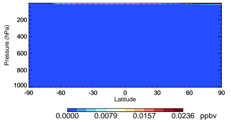
v11-02e-Run0 Br - Species Curtain @ -180.000 for Jul
