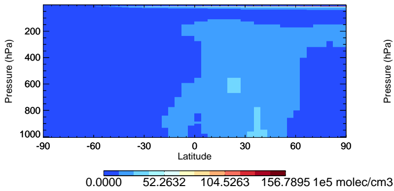
v11-02e-Run1 OH - Species Zonal Mean for Jul
