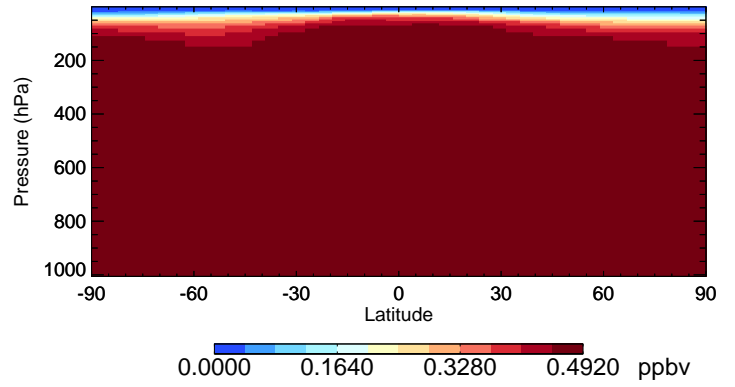
v11-02e-Run1 CFC12 - Species Curtain @ -180.000 for Jul
