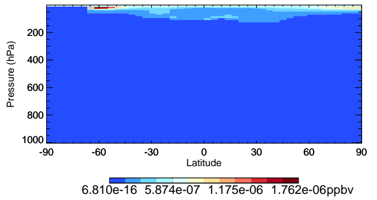
v11-02e-Run0 CIOO - Species Curtain @ -180.000 for Jul
