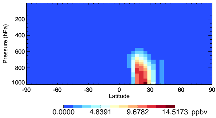
v11-02e-Run0 DST4 - Species Zonal Mean for Jul
