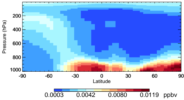
v11-02e-Run0 MSA - Species Zonal Mean for Jul
