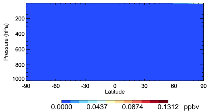
v11-02f-Run1 ACTA - Species Curtain @ -180.000 for Jul
