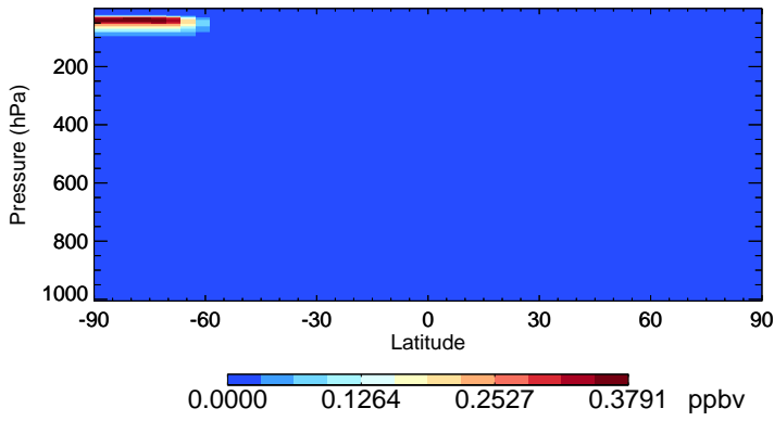
v11-02e-Run0 Cl2O2 - Species Zonal Mean for Jul
