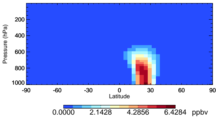
v11-02f-Run1 DST2 - Species Zonal Mean for Jul
