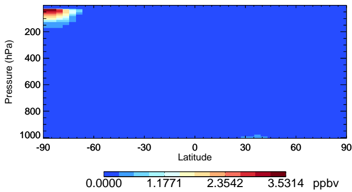
v11-02f-Run1 NIT - Species Zonal Mean for Jul
