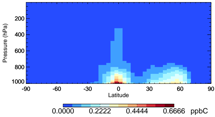
v11-02e-Run0 EOH - Species Zonal Mean for Jul
