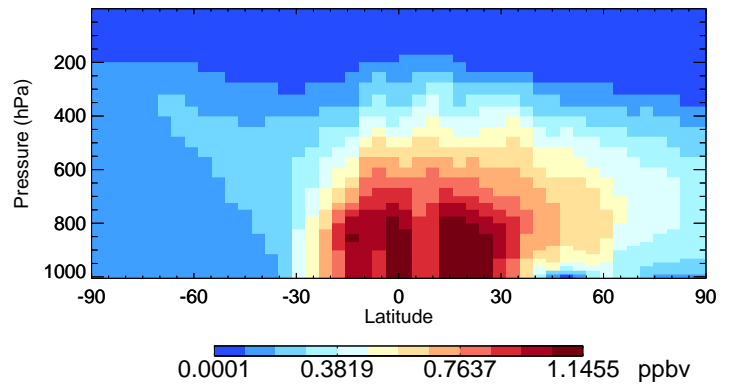
v11-02f-Run1 MP - Species Curtain @ -180.000 for Jul
