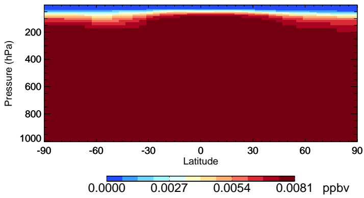
v11-02e-Run1 CH3CCI3 - Species Zonal Mean for Jul
