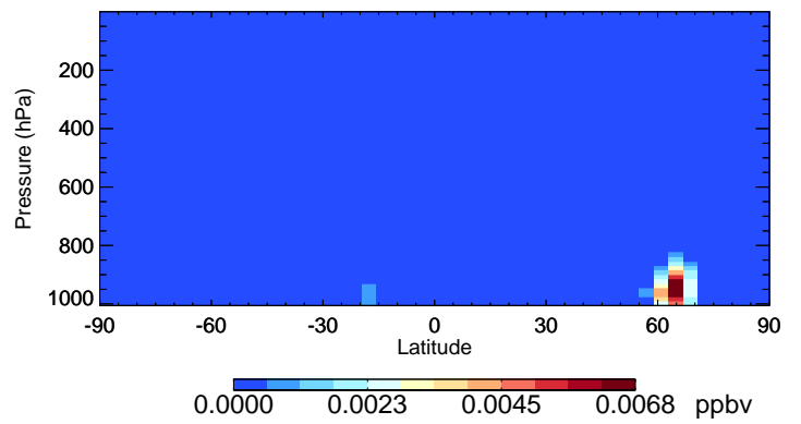
v11-02f-Run1 RIPA - Species Curtain @ -180.000 for Jul
