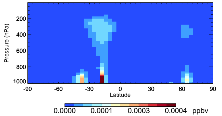
v11-02f-Run1 HONIT - Species Curtain @ -180.000 for Jul
