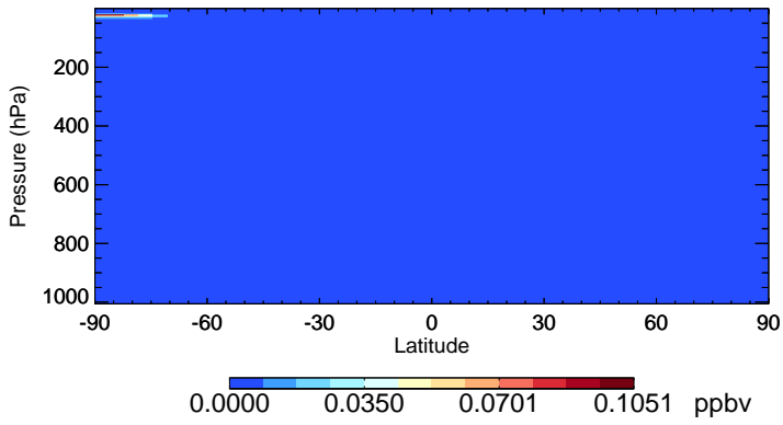
v11-02e-Run0 ClNO2 - Species Zonal Mean for Jul
