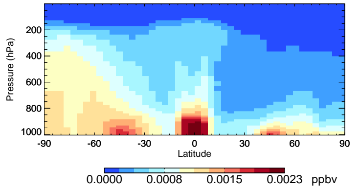
v11-02e-Run0 CHBr3 - Species Curtain @ -180.000 for Jul
