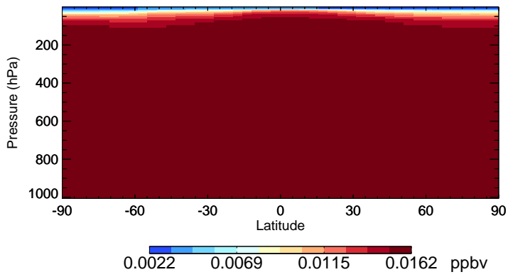
v11-02e-Run0 CFC114 - Species Zonal Mean for Jul
