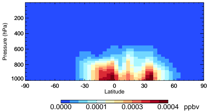
v11-02f-Run1 ISN10A - Species Zonal Mean for Jul
