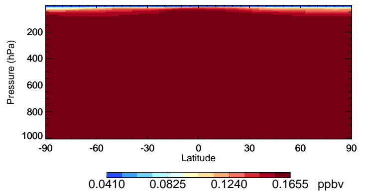
v11-02f-Run1 HCFC22 - Species Curtain @ -180.000 for Jul
