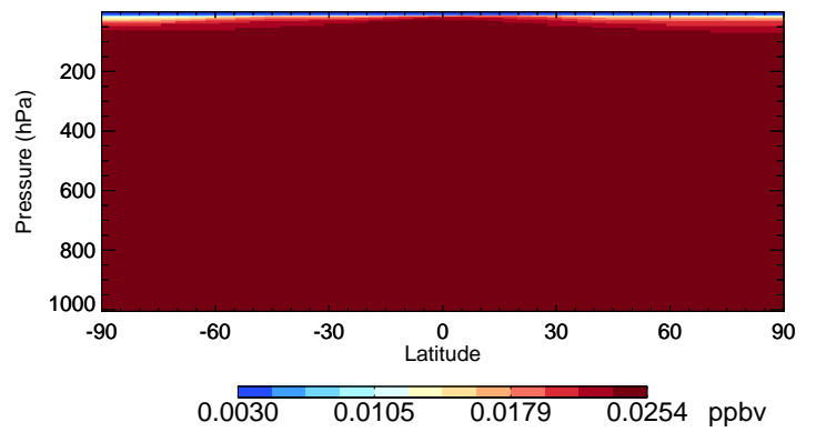
v11-02f-Run1 HCFC142b - Species Curtain @ -180.000 for Jul
