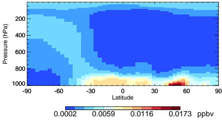
v11-02e-Run1 MSA - Species Zonal Mean for Jul
