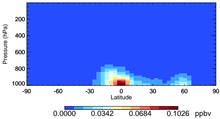
v11-02f-Run1 MACR - Species Zonal Mean for Jul
