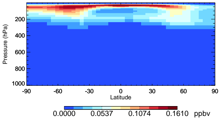
v11-02f-Run1 MPN - Species Zonal Mean for Jul
