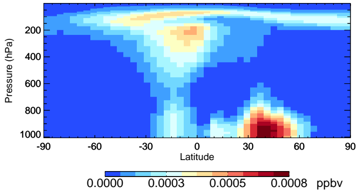
v11-02e-Run1 DHDN - Species Zonal Mean for Jul
