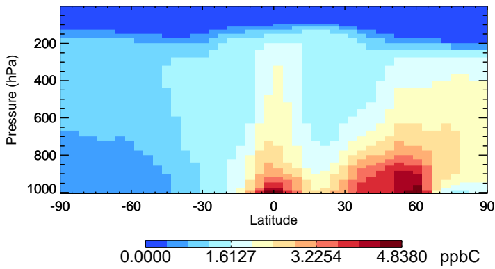
v11-02f-Run1 ACET - Species Zonal Mean for Jul
