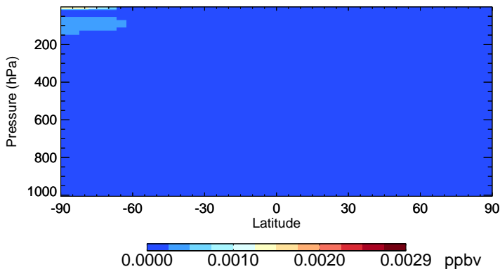
v11-02e-Run1 Br2 - Species Zonal Mean for Jul
