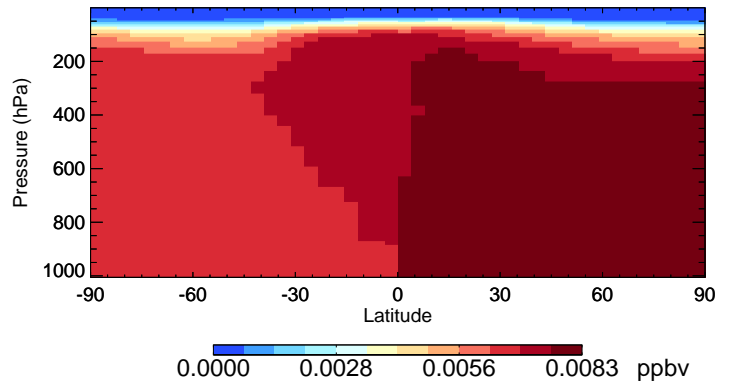
v11-02e-Run0 CH3Br - Species Curtain @ -180.000 for Jul
