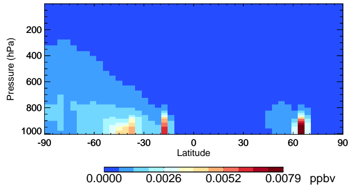
v11-02e-Run0 RCHO - Species Curtain @ -180.000 for Jul
