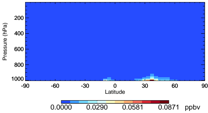
v11-02e-Run0 HNO 2 - Species Zonal Mean for Jul
