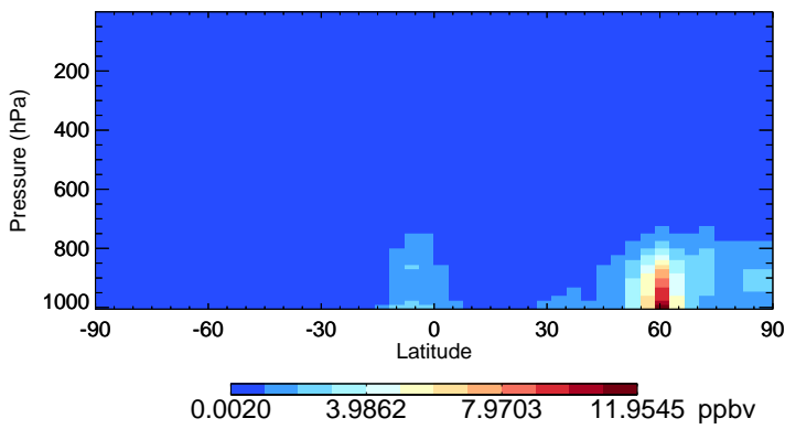
v11-02f-Run1 OCPI - Species Zonal Mean for Jul
