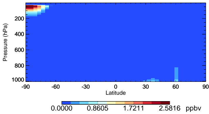
v11-02e-Run1 NIT - Species Zonal Mean for Jul
