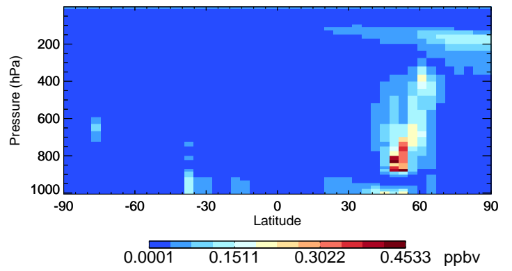
v11-02e-Run1 SO2 - Species Curtain @ -180.000 for Jul
