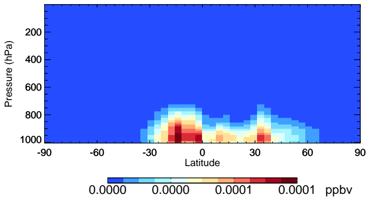
v11-02f-Run1 ETHLN - Species Zonal Mean for Jul
