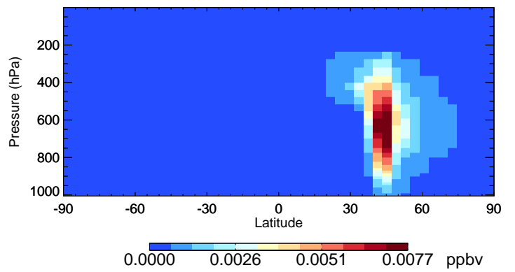
v11-02f-Run1 DST4 - Species Curtain @ -180.000 for Jul
