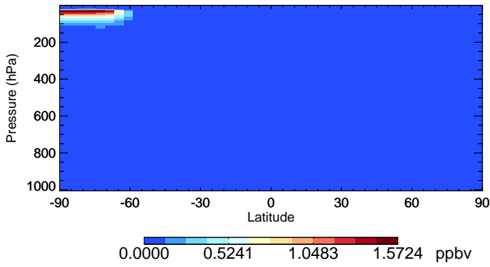
v11-02e-Run0 HOCl - Species Zonal Mean for Jul
