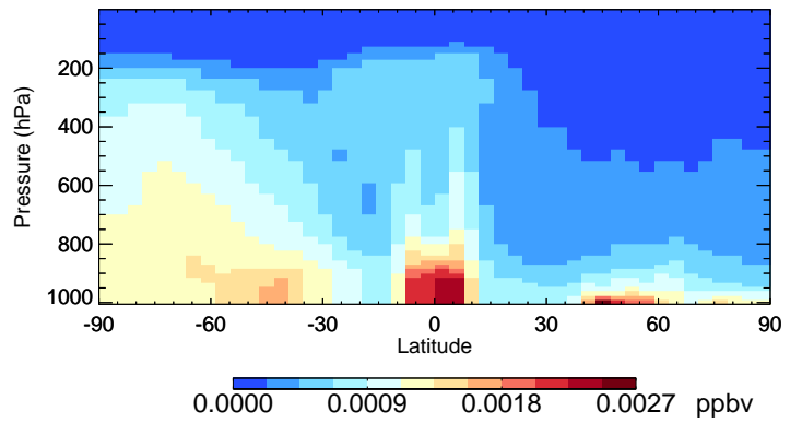
v11-02f-Run1 CHBr3 - Species Curtain @ -180.000 for Jul
