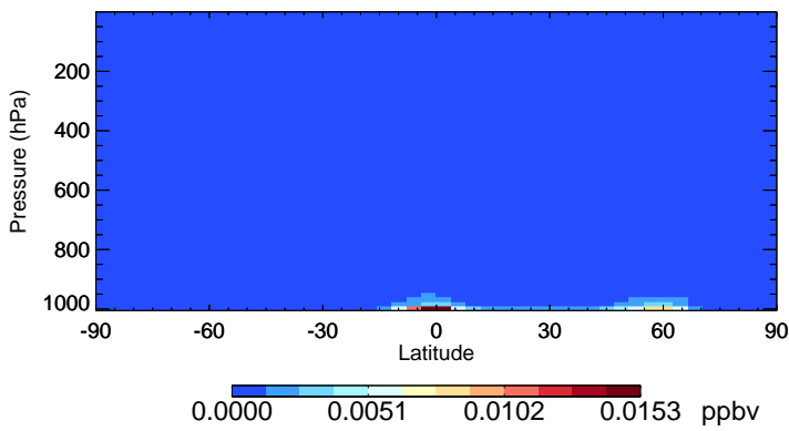
v11-02f-Run1 MTPO - Species Zonal Mean for Jul
