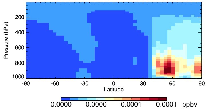
v11-02e-Run1 ISN10A - Species Curtain @ -180.000 for Jul
