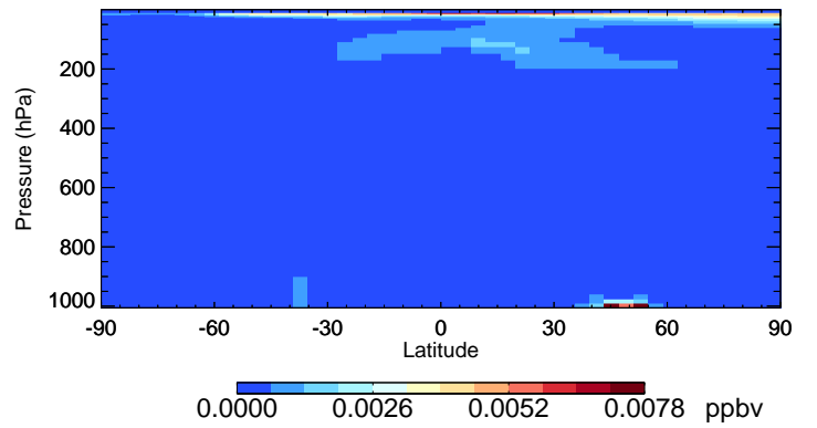
v11-02f-Run1 HNO 2 - Species Curtain @ -180.000 for Jul
