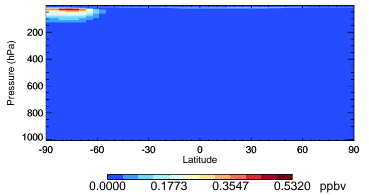
v11-02f-Run1 HOCl - Species Curtain @ -180.000 for Jul
