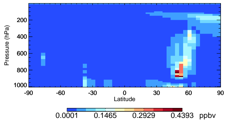
v11-02f-Run1 SO2 - Species Curtain @ -180.000 for Jul
