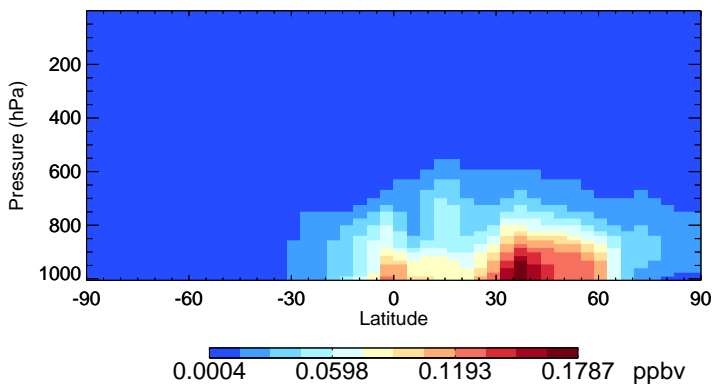
v11-02f-Run1 INDIOL - Species Zonal Mean for Jul
