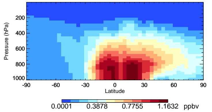
v11-02e-Run0 MP - Species Curtain @ -180.000 for Jul
