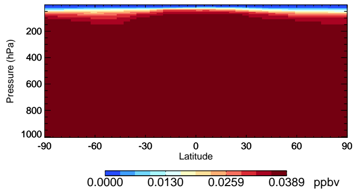
v11-02e-Run1 HCFC141b - Species Curtain @ -180.000 for Jul
