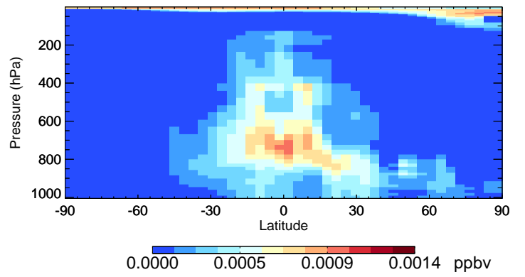
v11-02e-Run0 HBr - Species Curtain @ -180.000 for Jul
