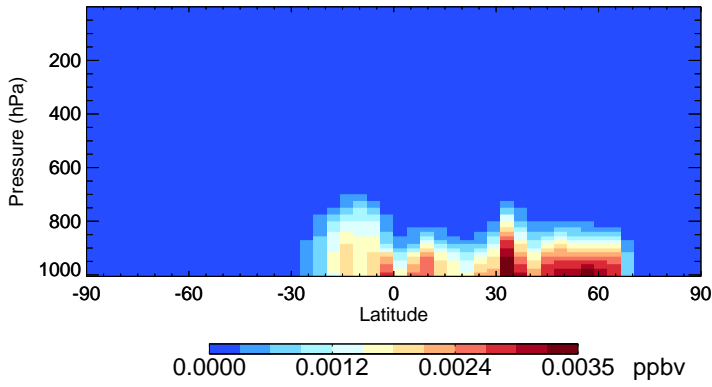
v11-02e-Run1 ISOPNB - Species Zonal Mean for Jul
