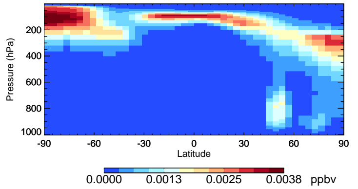
v11-02e-Run0 TSOA2 - Species Curtain @ -180.000 for Jul
