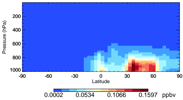
v11-02e-Run1 INDIOL - Species Zonal Mean for Jul
