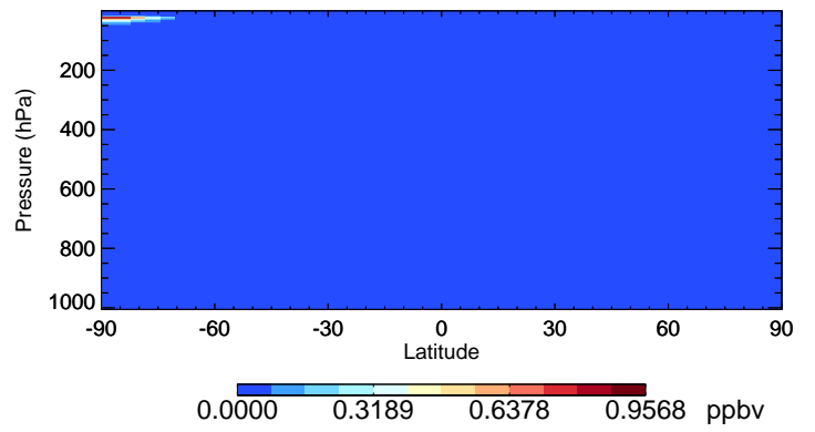
v11-02e-Run1 Cl2 - Species Curtain @ -180.000 for Jul
