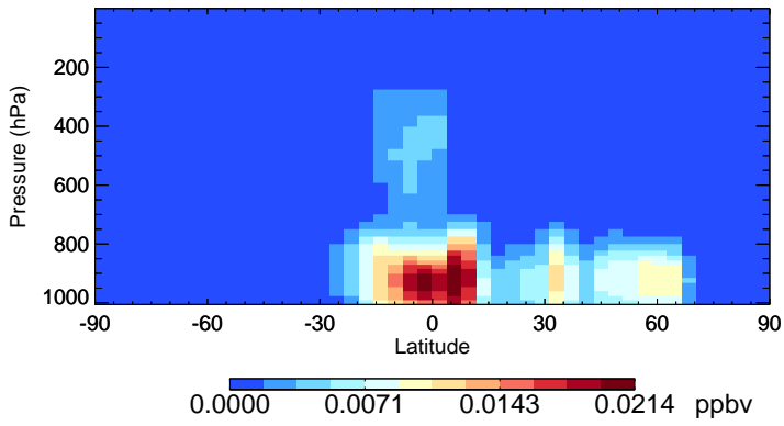
v11-02e-Run0 IEPOXB - Species Zonal Mean for Jul
