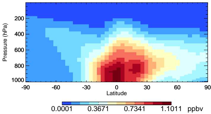
v11-02f-Run1 MP - Species Zonal Mean for Jul
