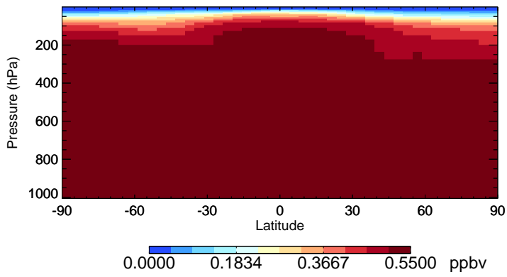
v11-02e-Run1 CH3Cl - Species Zonal Mean for Jul
