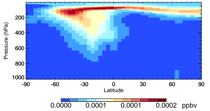
v11-02e-Run0 DHDN - Species Curtain @ -180.000 for Jul
