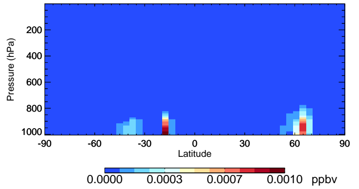
v11-02e-Run0 GLYX - Species Curtain @ -180.000 for Jul
