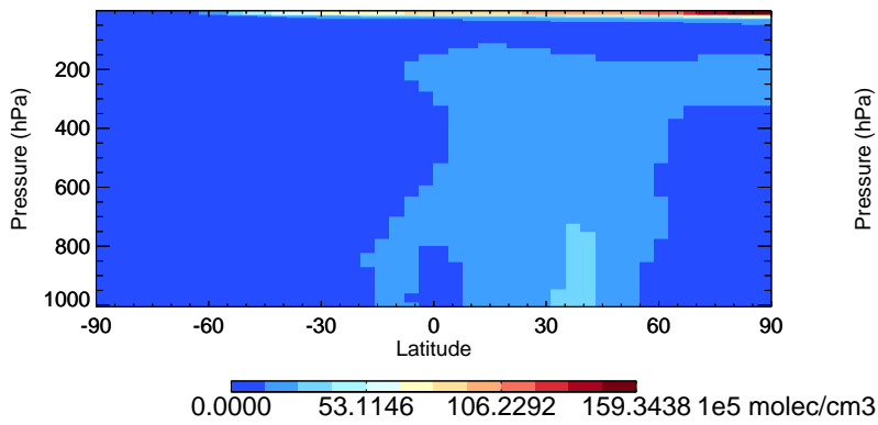
v11-02e-Run0 OH - Species Zonal Mean for Jul
