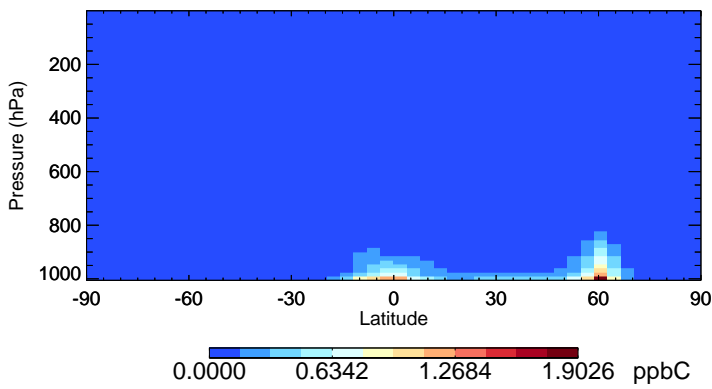
v11-02f-Run1 PRPE - Species Zonal Mean for Jul
