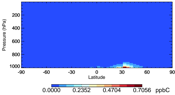
v11-02e-Run0 XYLE - Species Zonal Mean for Jul
