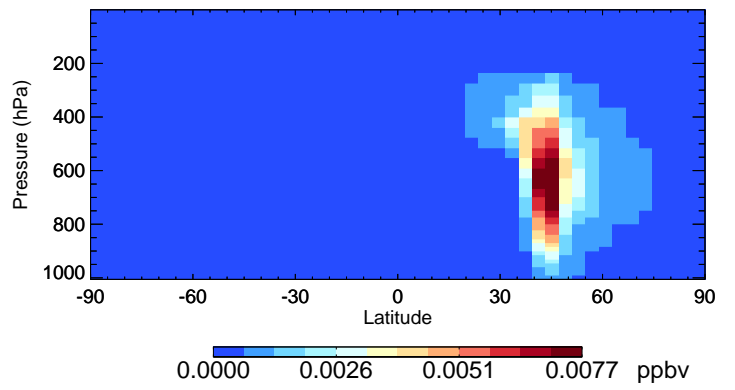
v11-02e-Run1 DST4 - Species Curtain @ -180.000 for Jul
