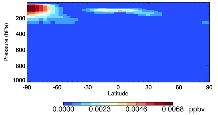
v11-02e-Run0 ISOA3 - Species Curtain @ -180.000 for Jul
