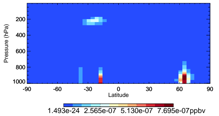
v11-02f-Run1 LVOC - Species Curtain @ -180.000 for Jul
