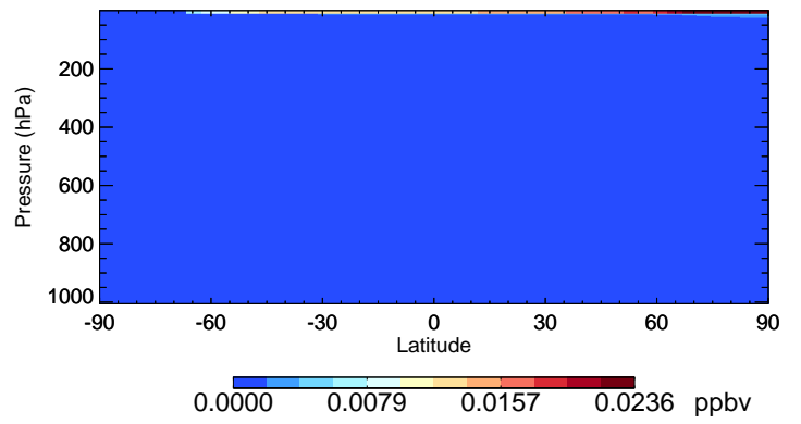
v11-02e-Run1 Br - Species Curtain @ -180.000 for Jul
