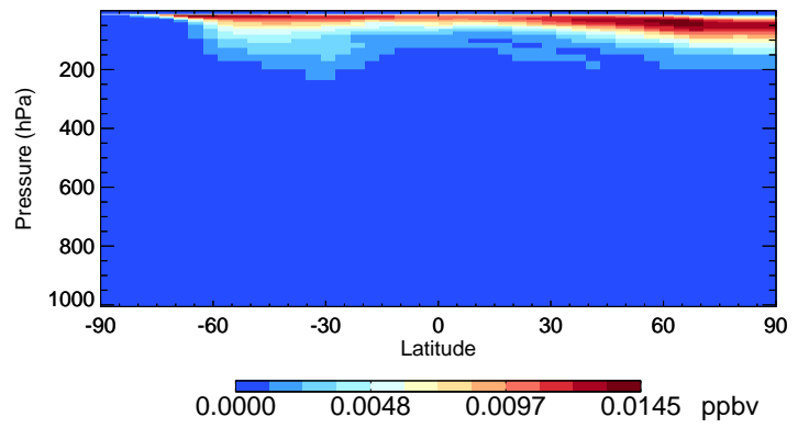
v11-02e-Run1 BrNO3 - Species Curtain @ -180.000 for Jul
