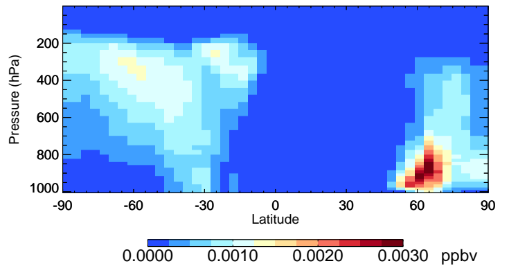
v11-02f-Run1 IMAE - Species Curtain @ -180.000 for Jul
