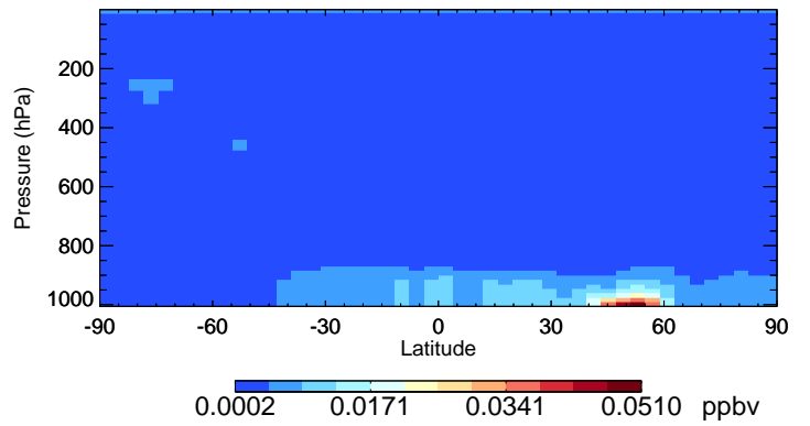
v11-02f-Run1 MSA - Species Curtain @ -180.000 for Jul
