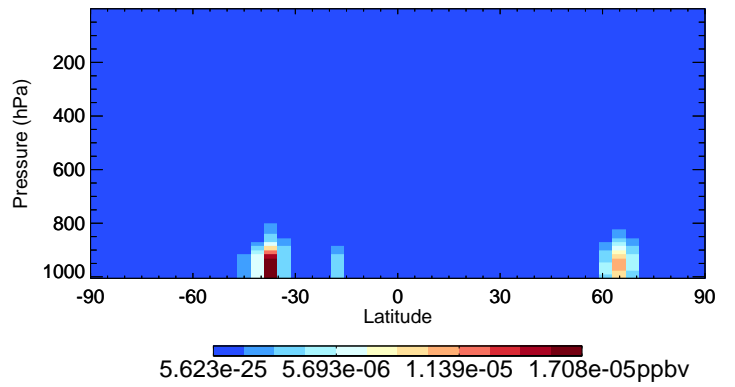
v11-02f-Run1 MACRN - Species Curtain @ -180.000 for Jul
