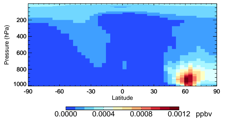
v11-02e-Run1 LVOCOA - Species Curtain @ -180.000 for Jul
