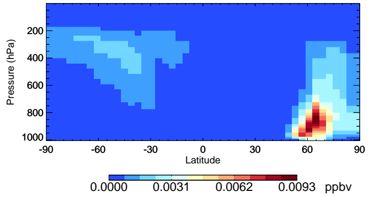
v11-02e-Run1 IMAE - Species Curtain @ -180.000 for Jul
