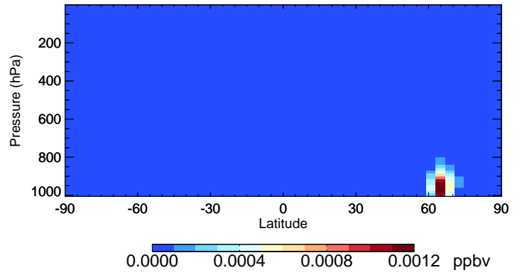
v11-02e-Run1 ISOPNB - Species Curtain @ -180.000 for Jul
