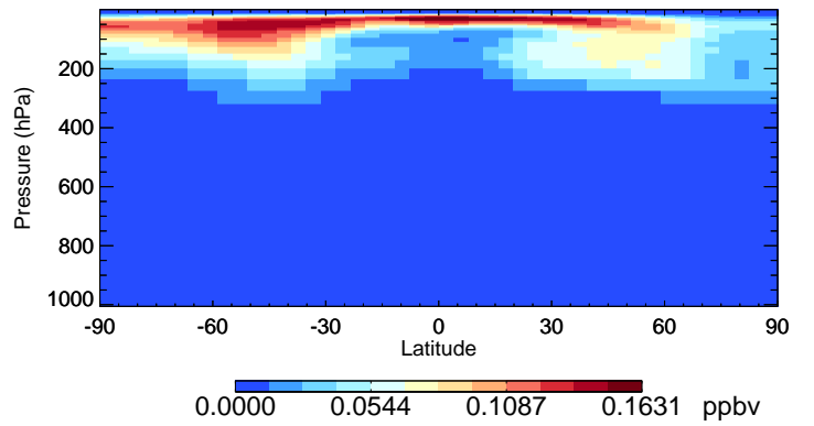
v11-02f-Run1 MPN - Species Curtain @ -180.000 for Jul
