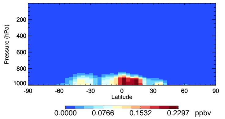
v11-02f-Run1 NH3 - Species Curtain @ -180.000 for Jul
