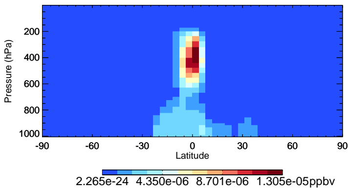
v11-02f-Run1 LVOC - Species Zonal Mean for Jul
