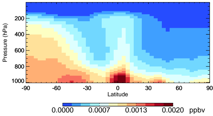
v11-02e-Run0 CHBr3 - Species Zonal Mean for Jul
