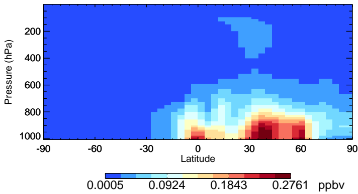
v11-02f-Run1 SOAS - Species Zonal Mean for Jul
