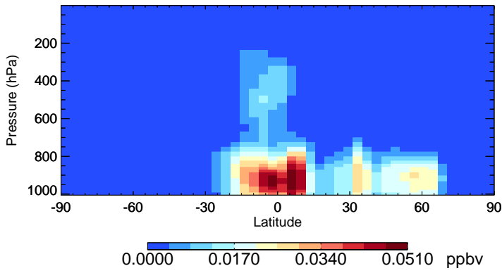
v11-02e-Run0 IEPOXA - Species Zonal Mean for Jul
