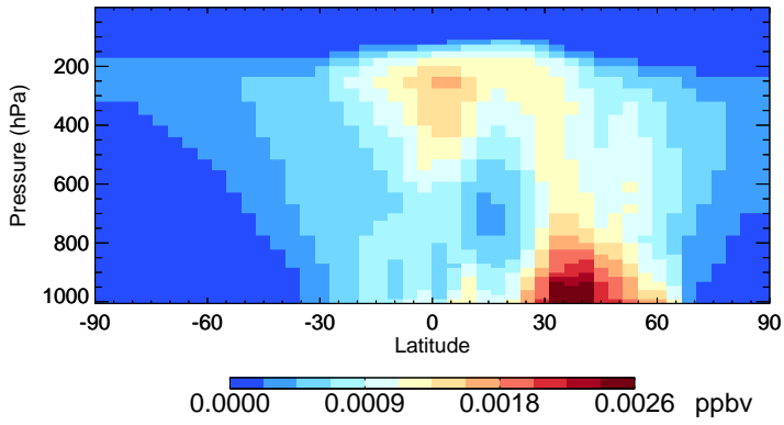
v11-02e-Run1 R4N2 - Species Zonal Mean for Jul
