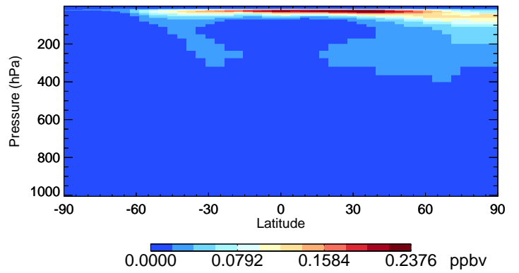
v11-02f-Run1 HNO4 - Species Curtain @ -180.000 for Jul
