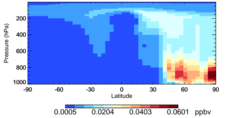
v11-02e-Run1 SOAS - Species Curtain @ -180.000 for Jul
