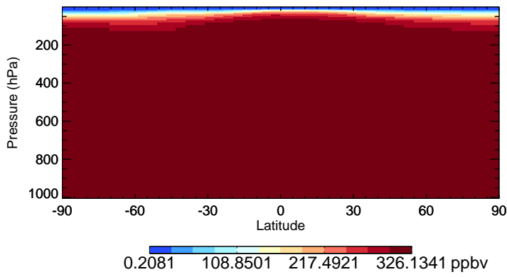
v11-02e-Run0 N2O - Species Zonal Mean for Jul
