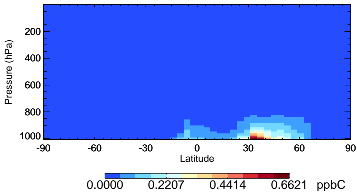
v11-02e-Run0 TOLU - Species Zonal Mean for Jul
