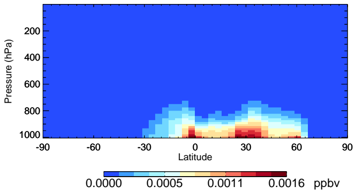
v11-02f-Run1 IONITA - Species Zonal Mean for Jul
