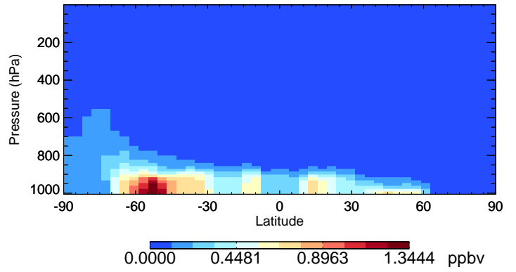
v11-02e-Run1 SALA - Species Curtain @ -180.000 for Jul
