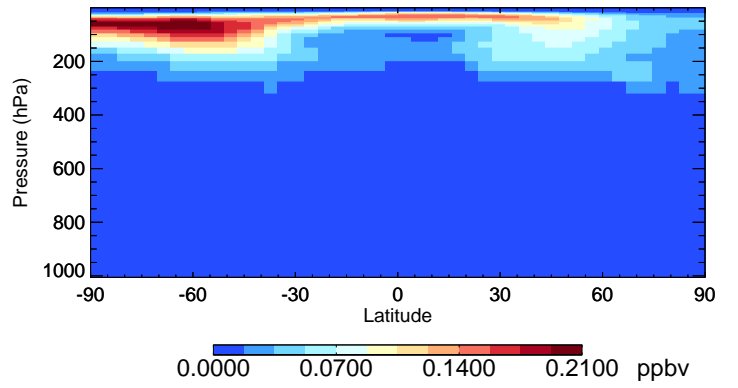
v11-02e-Run0 MPN - Species Curtain @ -180.000 for Jul
