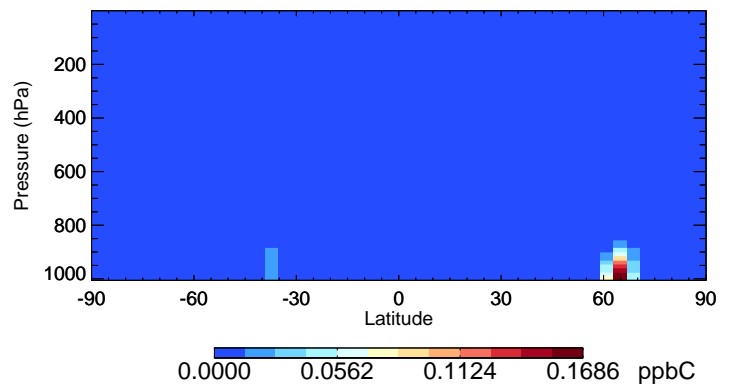
v11-02f-Run1 ISOP - Species Curtain @ -180.000 for Jul
