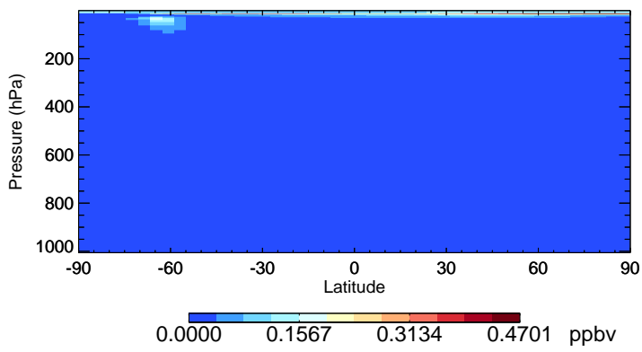
v11-02e-Run1 CIO - Species Zonal Mean for Jul
