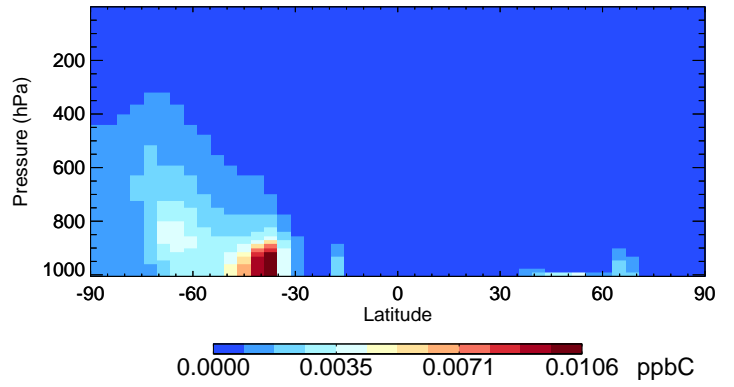
v11-02e-Run1 XYLE - Species Curtain @ -180.000 for Jul
