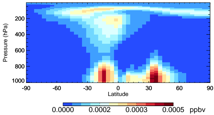
v11-02f-Run1 DHDN - Species Zonal Mean for Jul
