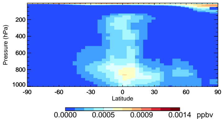
v11-02e-Run0 HBr - Species Zonal Mean for Jul
