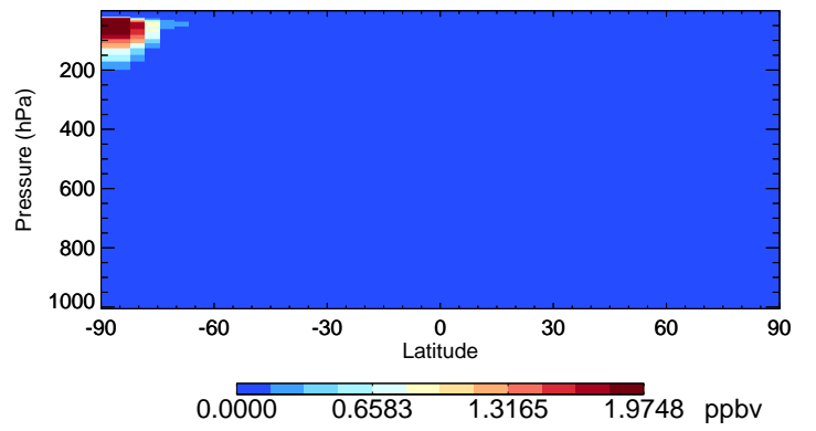
v11-02e-Run0 NIT - Species Curtain @ -180.000 for Jul
