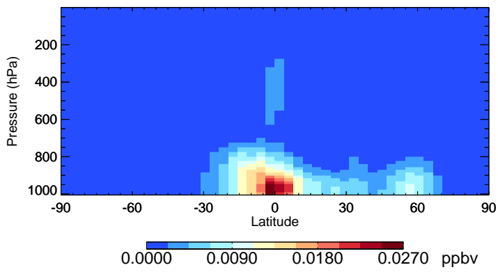
v11-02f-Run1 IPMN - Species Zonal Mean for Jul
