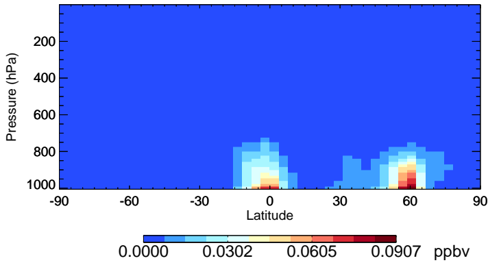
v11-02e-Run1 TSOA2 - Species Zonal Mean for Jul
