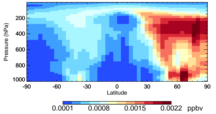
v11-02e-Run0 IONITA - Species Curtain @ -180.000 for Jul
