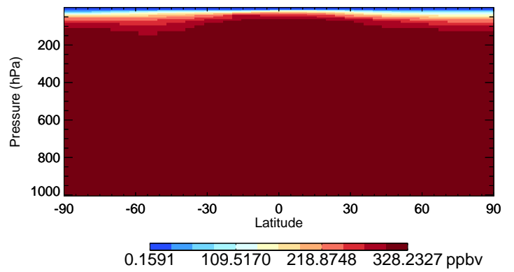
v11-02f-Run1 N2O - Species Curtain @ -180.000 for Jul
