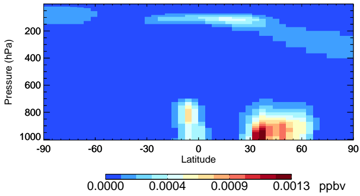
v11-02e-Run0 ASOA2 - Species Zonal Mean for Jul
