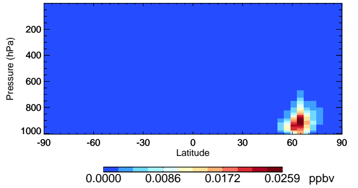
v11-02e-Run1 GLYC - Species Curtain @ -180.000 for Jul
