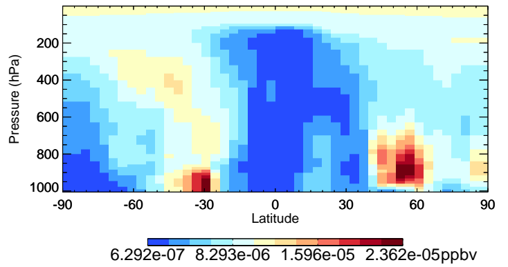
v11-02f-Run1 ISN10A - Species Curtain @ -180.000 for Jul
