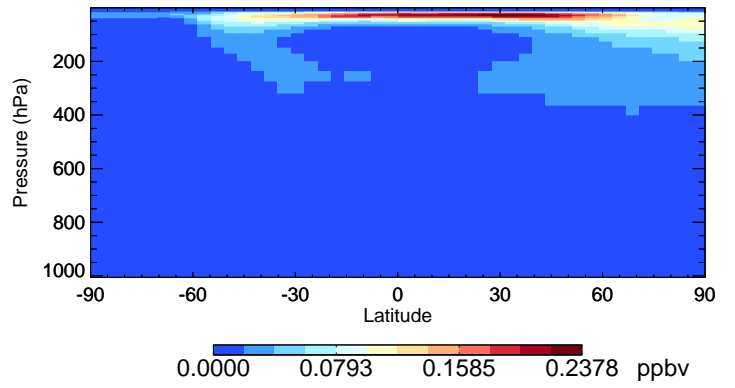
v11-02e-Run0 HNO4 - Species Curtain @ -180.000 for Jul
