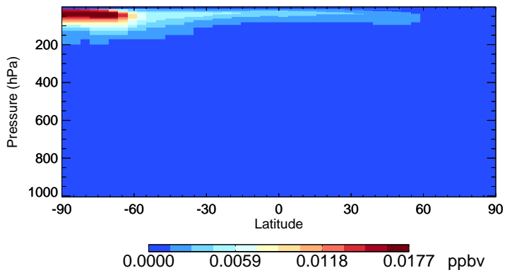
v11-02e-Run0 BrCl - Species Zonal Mean for Jul
