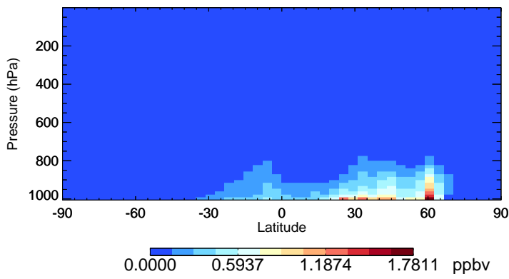
v11-02f-Run1 NH3 - Species Zonal Mean for Jul
