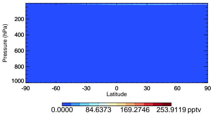
v11-02f-Run1 HO2 - Species Zonal Mean for Jul
