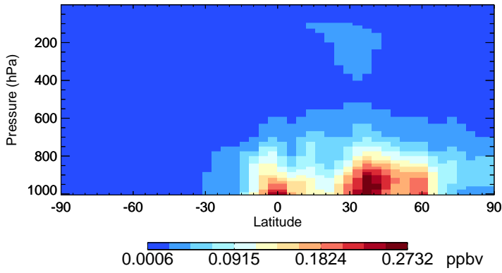
v11-02e-Run1 SOAS - Species Zonal Mean for Jul
