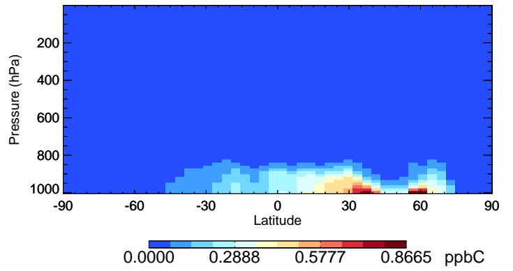
v11-02e-Run0 ALD2 - Species Curtain @ -180.000 for Jul
