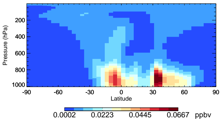
v11-02e-Run1 ISO3 - Species Zonal Mean for Jul
