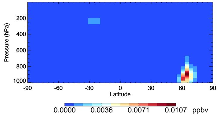
v11-02e-Run1 IEPOXA - Species Curtain @ -180.000 for Jul
