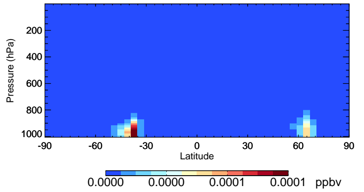
v11-02e-Run0 ISN1 - Species Curtain @ -180.000 for Jul
