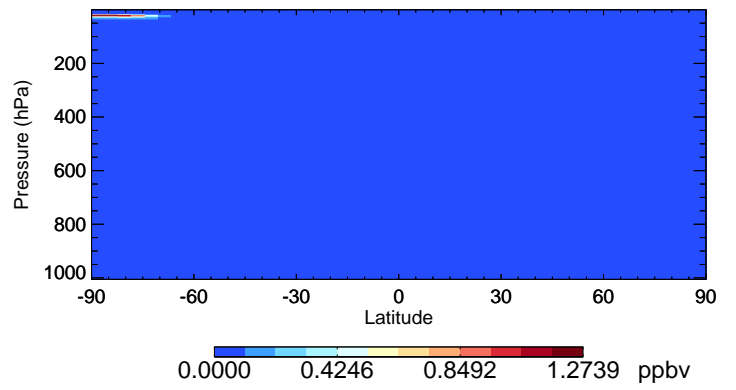
v11-02e-Run0 Cl2 - Species Curtain @ -180.000 for Jul
