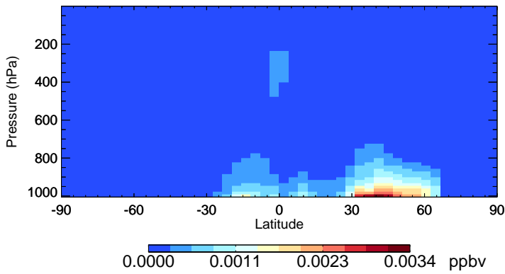
v11-02f-Run1 HONIT - Species Zonal Mean for Jul
