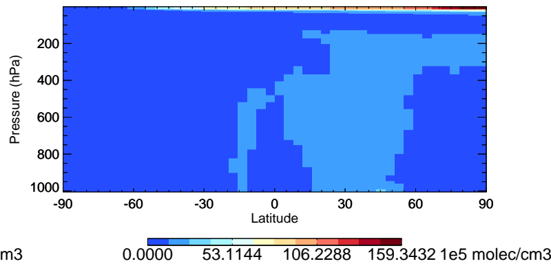
v11-02e-Run0 OH - Species Curtain @ -180.000 for Jul
