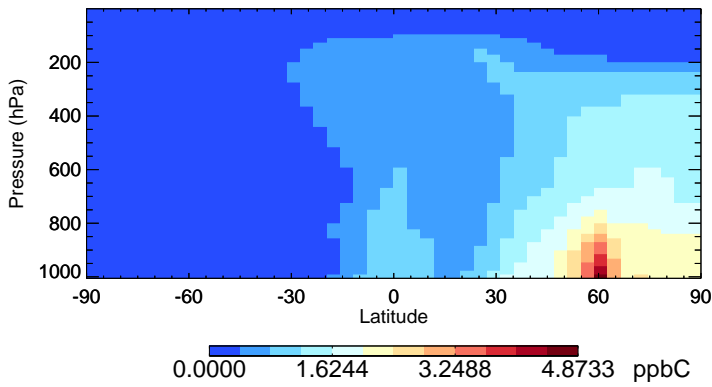
v11-02f-Run1 C2H6 - Species Zonal Mean for Jul
