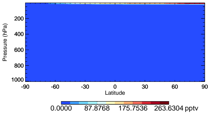
v11-02e-Run0 HO2 - Species Zonal Mean for Jul
