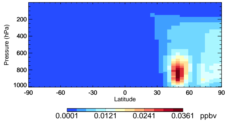
v11-02e-Run0 INDIOL - Species Curtain @ -180.000 for Jul
