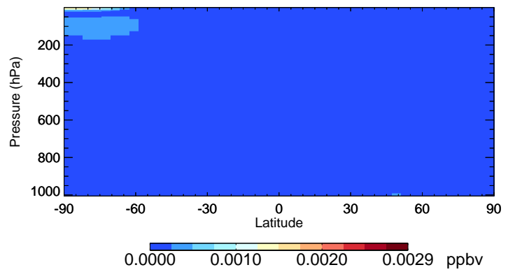
v11-02f-Run1 Br2 - Species Curtain @ -180.000 for Jul
