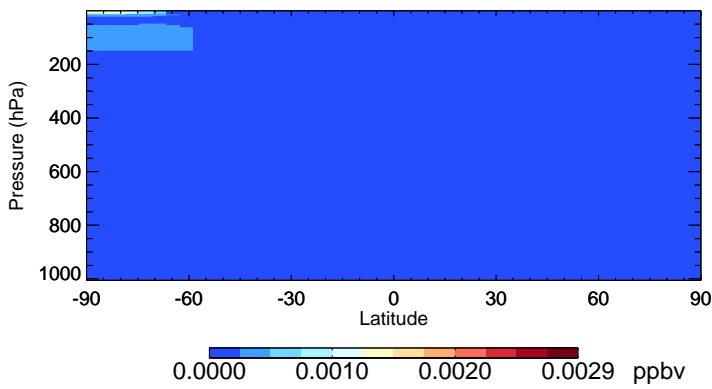
v11-02f-Run1 Br2 - Species Zonal Mean for Jul
