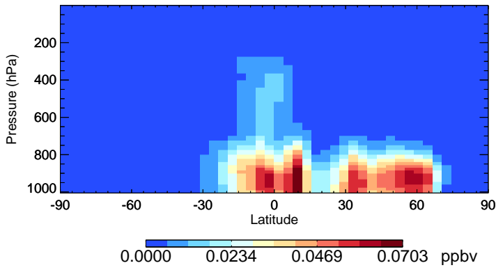
v11-02e-Run0 HAC - Species Zonal Mean for Jul
