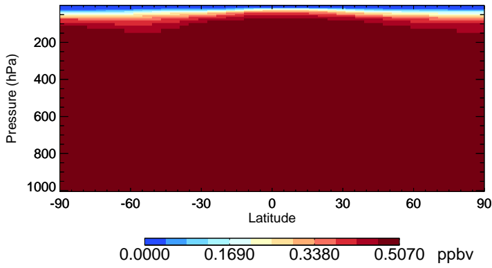
v11-02e-Run0 CFC12 - Species Zonal Mean for Jul
