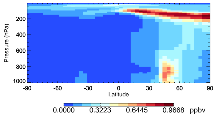
v11-02e-Run0 SO4 - Species Curtain @ -180.000 for Jul
