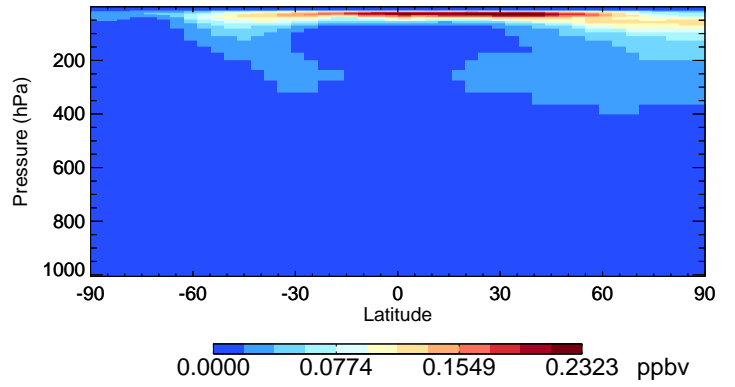
v11-02e-Run1 HNO4 - Species Curtain @ -180.000 for Jul
