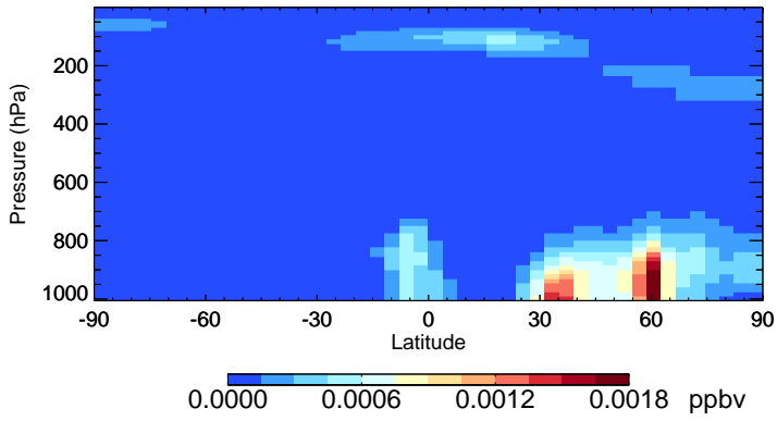
v11-02e-Run1 ASOA2 - Species Zonal Mean for Jul
