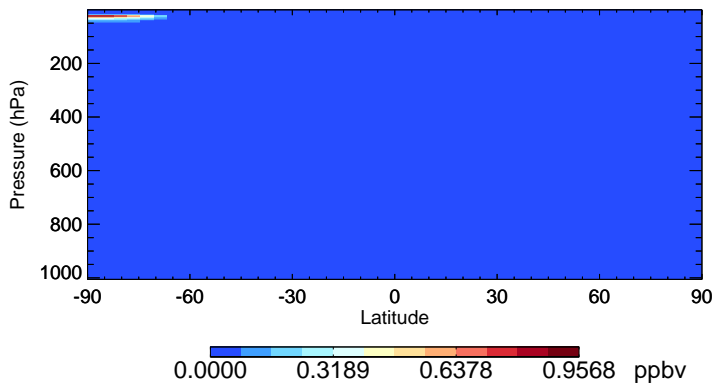
v11-02e-Run1 Cl2 - Species Zonal Mean for Jul
