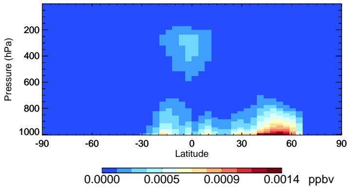
v11-02e-Run0 HONIT - Species Zonal Mean for Jul
