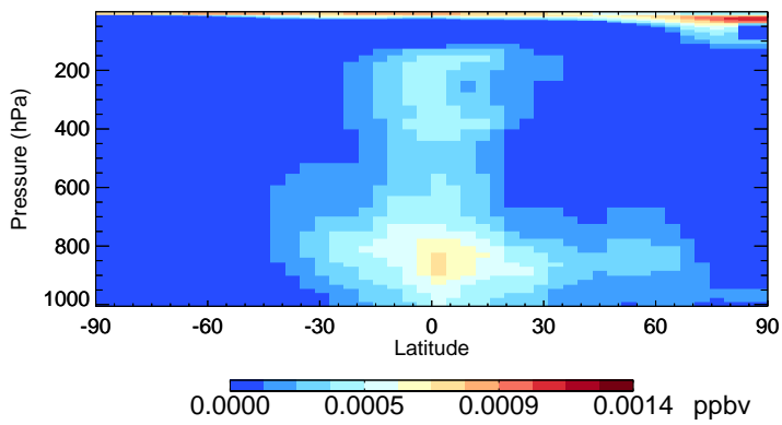
v11-02f-Run1 HBr - Species Zonal Mean for Jul
