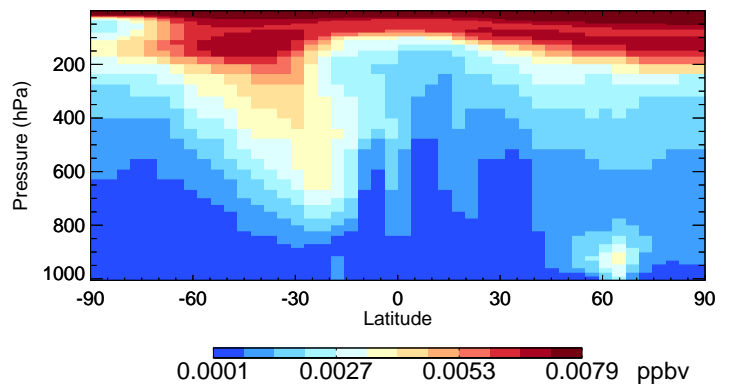
v11-02f-Run1 ISO3 - Species Curtain @ -180.000 for Jul
