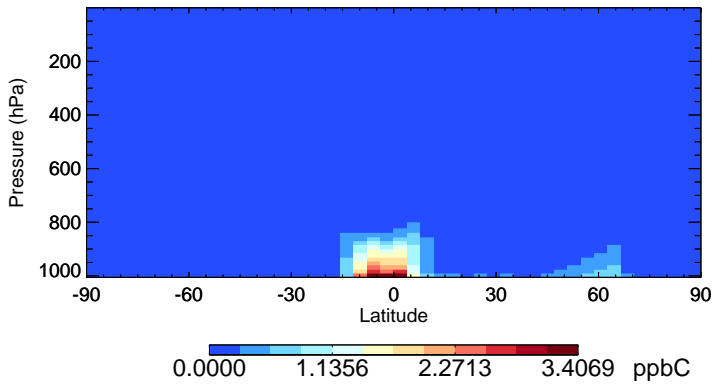
v11-02e-Run0 ISOP - Species Zonal Mean for Jul
