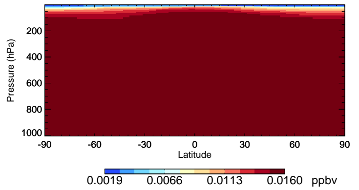
v11-02e-Run1 CFC114 - Species Curtain @ -180.000 for Jul
