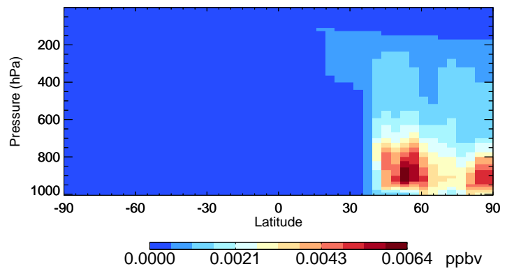
v11-02f-Run1 SOAGX - Species Curtain @ -180.000 for Jul
