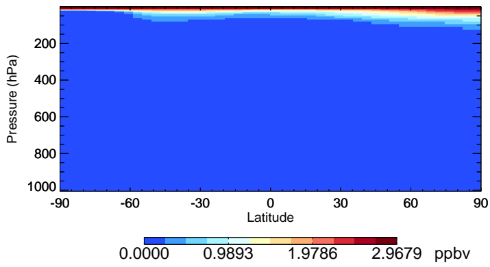
v11-02e-Run1 HCl - Species Zonal Mean for Jul
