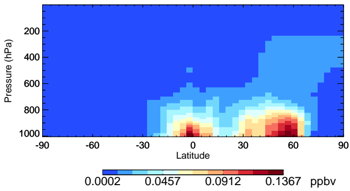
v11-02e-Run0 TSOG3 - Species Zonal Mean for Jul
