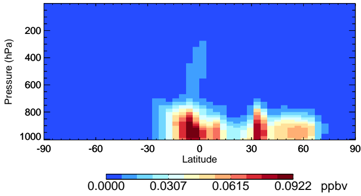
v11-02e-Run1 GLYC - Species Zonal Mean for Jul
