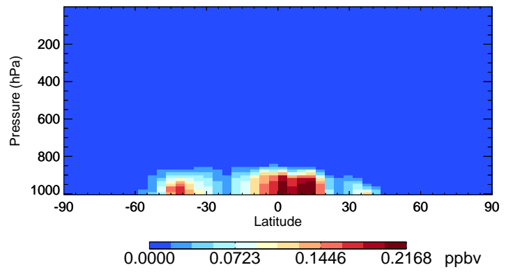
v11-02e-Run0 NH3 - Species Curtain @ -180.000 for Jul
