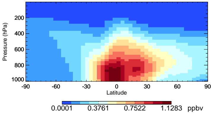
v11-02e-Run1 MP - Species Zonal Mean for Jul
