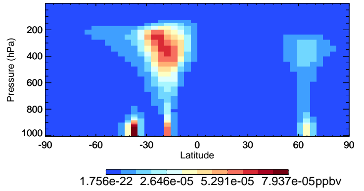
v11-02e-Run1 HONIT - Species Curtain @ -180.000 for Jul
