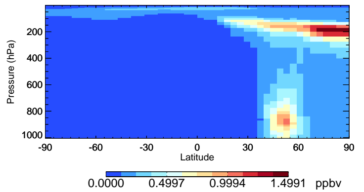
v11-02f-Run1 SO4 - Species Curtain @ -180.000 for Jul
