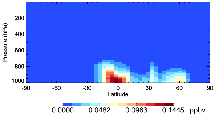
v11-02e-Run1 MACR - Species Zonal Mean for Jul
