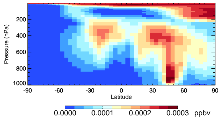
v11-02e-Run0 ASOG1 - Species Curtain @ -180.000 for Jul
