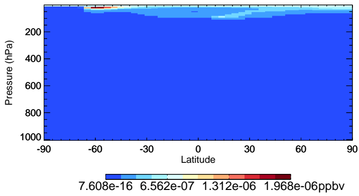
v11-02e-Run1 CIOO - Species Zonal Mean for Jul
