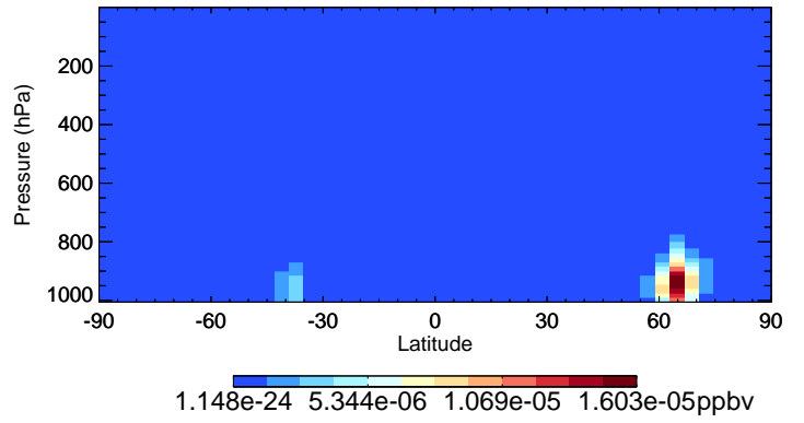
v11-02e-Run1 ETHLN - Species Curtain @ -180.000 for Jul
