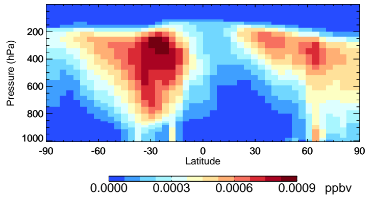
v11-02f-Run1 R4N2 - Species Curtain @ -180.000 for Jul
