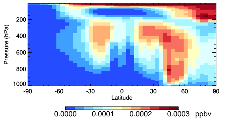
v11-02e-Run1 ASOG1 - Species Curtain @ -180.000 for Jul
