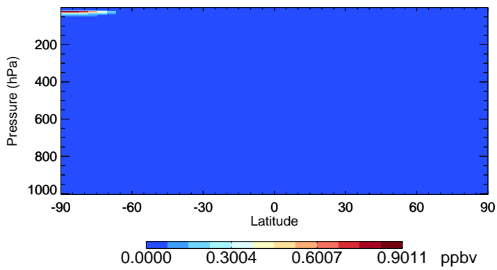
v11-02f-Run1 Cl2 - Species Zonal Mean for Jul
