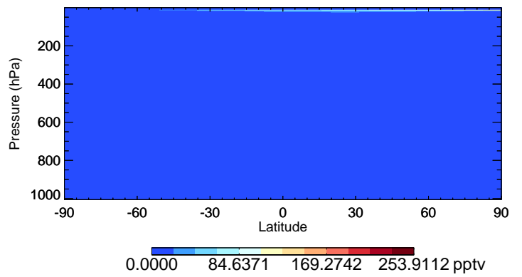
v11-02f-Run1 HO2 - Species Curtain @ -180.000 for Jul
