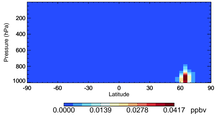
v11-02e-Run1 MACR - Species Curtain @ -180.000 for Jul
