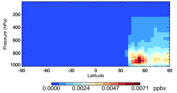
v11-02e-Run1 SOAME - Species Curtain @ -180.000 for Jul
