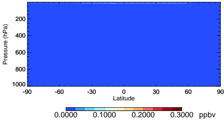
v11-02e-Run1 NO3 - Species Zonal Mean for Jul
