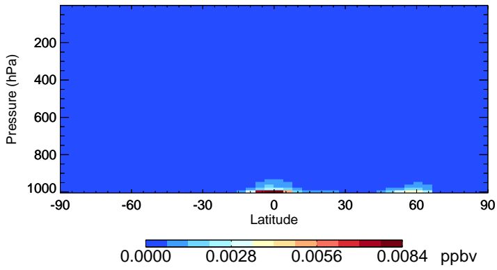
v11-02e-Run0 LIMO - Species Zonal Mean for Jul
