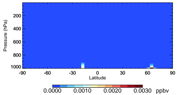
v11-02f-Run1 MTPO - Species Curtain @ -180.000 for Jul
