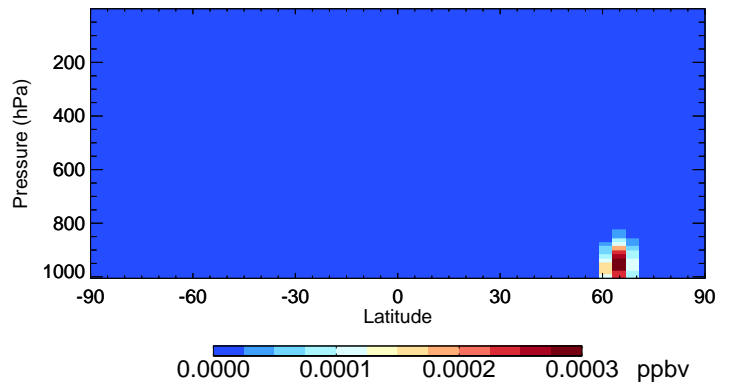
v11-02f-Run1 RIPD - Species Curtain @ -180.000 for Jul
