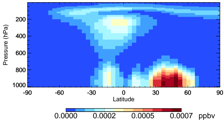
v11-02e-Run0 DHDN - Species Zonal Mean for Jul
