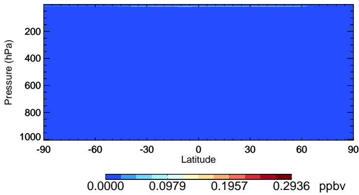
v11-02f-Run1 NO3 - Species Zonal Mean for Jul
