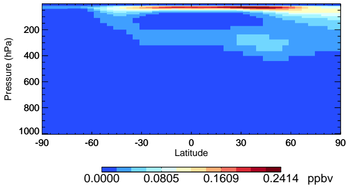
v11-02e-Run0 HNO4 - Species Zonal Mean for Jul
