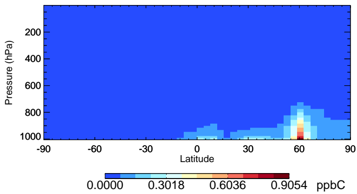
v11-02f-Run1 TOLU - Species Zonal Mean for Jul
