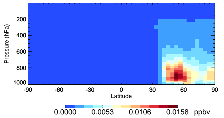
v11-02e-Run1 SOAGX - Species Curtain @ -180.000 for Jul
