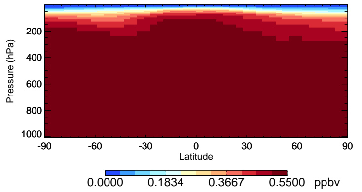
v11-02e-Run1 CH3Cl - Species Curtain @ -180.000 for Jul
