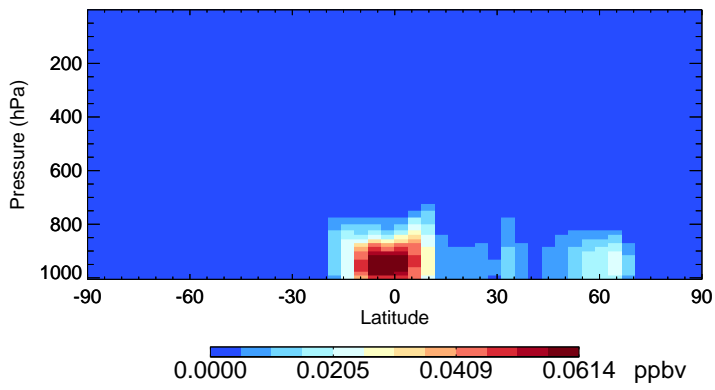
v11-02e-Run0 RIPA - Species Zonal Mean for Jul
