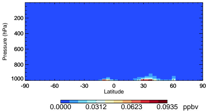
v11-02f-Run1 HNO 2 - Species Zonal Mean for Jul
