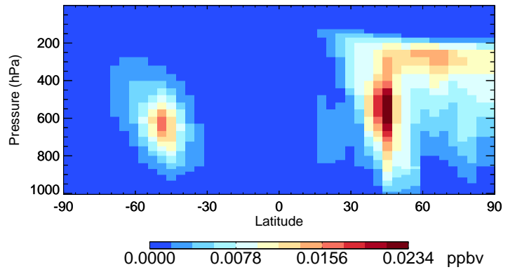
v11-02e-Run0 DST2 - Species Curtain @ -180.000 for Jul
