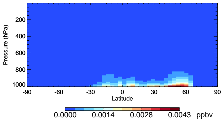
v11-02e-Run0 MONITS - Species Zonal Mean for Jul
