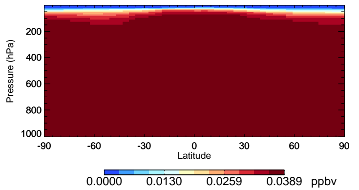
v11-02f-Run1 HCFC141b - Species Curtain @ -180.000 for Jul
