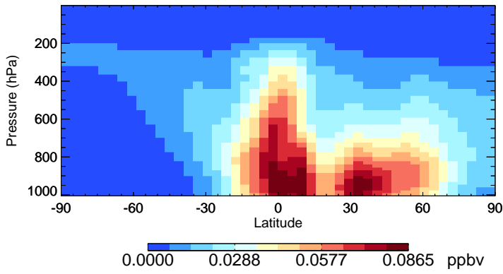
v11-02e-Run0 MAP - Species Zonal Mean for Jul
