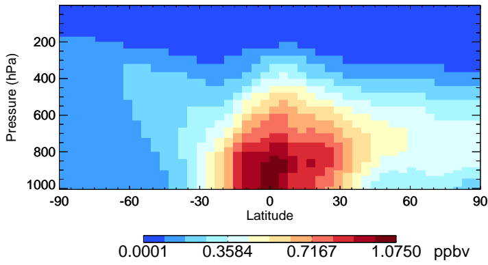
v11-02e-Run0 MP - Species Zonal Mean for Jul
