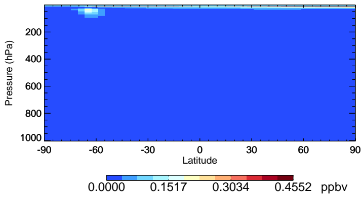
v11-02e-Run0 CIO - Species Zonal Mean for Jul
