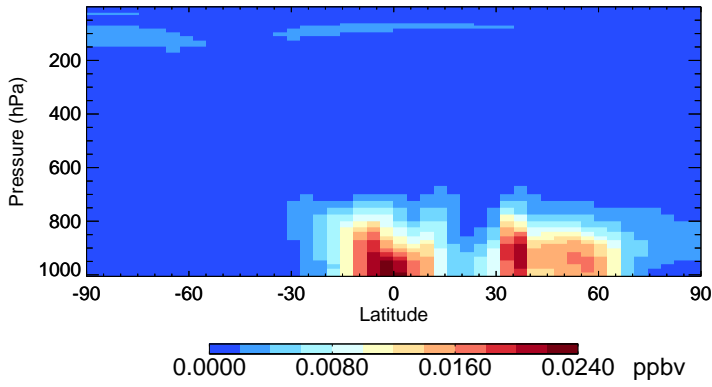
v11-02e-Run1 ISOA1 - Species Zonal Mean for Jul
