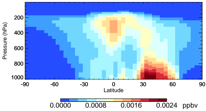
v11-02e-Run0 R4N2 - Species Zonal Mean for Jul
