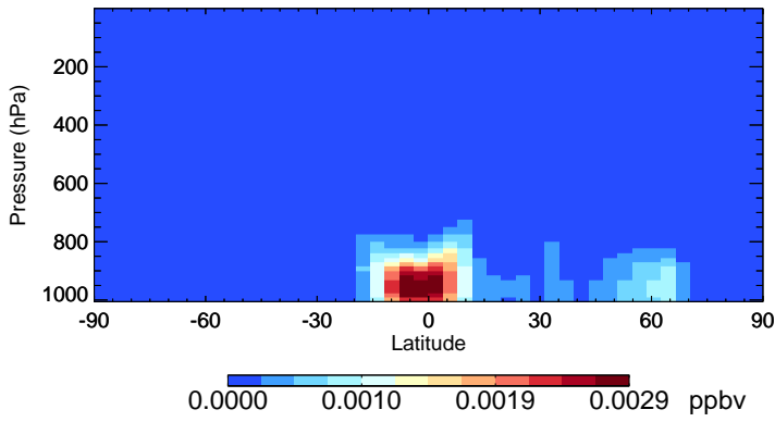
v11-02e-Run0 RIPD - Species Zonal Mean for Jul
