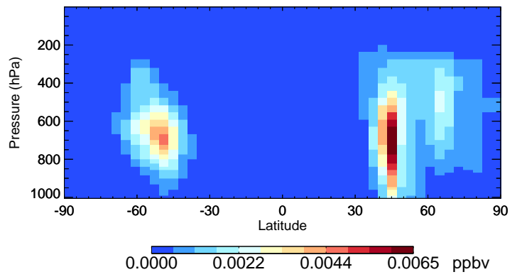
v11-02e-Run0 DST4 - Species Curtain @ -180.000 for Jul
