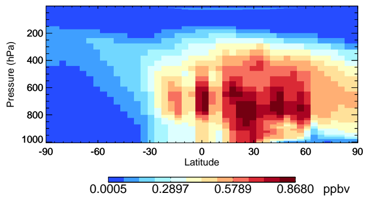
v11-02e-Run1 H2O2 - Species Curtain @ -180.000 for Jul
