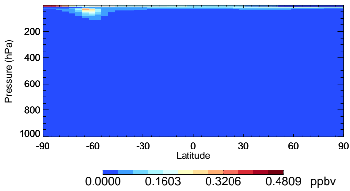
v11-02f-Run1 CIO - Species Zonal Mean for Jul
