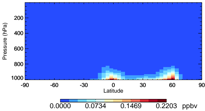
v11-02f-Run1 RCHO - Species Zonal Mean for Jul
