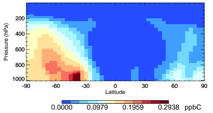
v11-02e-Run1 ALK4 - Species Curtain @ -180.000 for Jul
