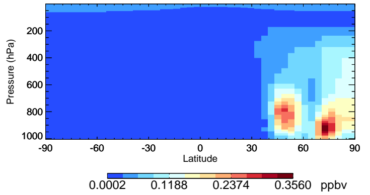
v11-02e-Run0 OCPI - Species Curtain @ -180.000 for Jul
