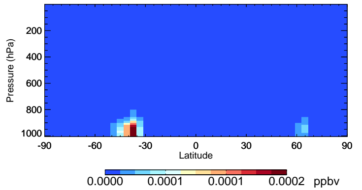
v11-02f-Run1 ISN1 - Species Curtain @ -180.000 for Jul
