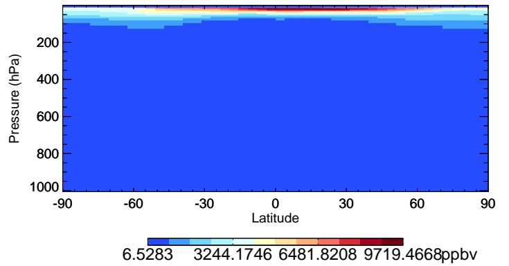
v11-02e-Run0 O3 - Species Curtain @ -180.000 for Jul
