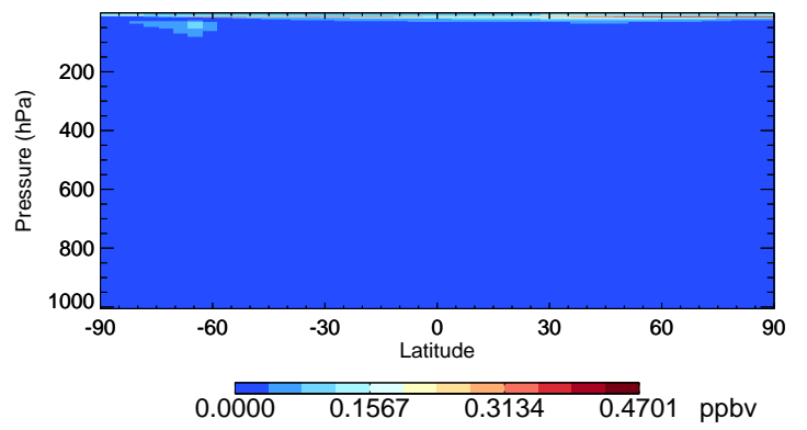
v11-02e-Run1 CIO - Species Curtain @ -180.000 for Jul
