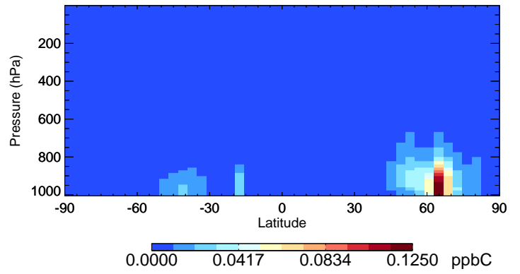
v11-02e-Run0 EOH - Species Curtain @ -180.000 for Jul
