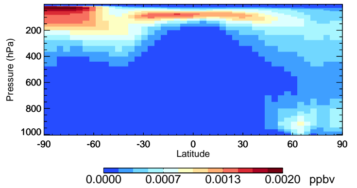
v11-02f-Run1 ISOA1 - Species Curtain @ -180.000 for Jul
