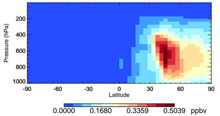
v11-02f-Run1 DST1 - Species Curtain @ -180.000 for Jul
