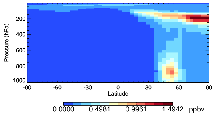
v11-02e-Run1 SO4 - Species Curtain @ -180.000 for Jul
