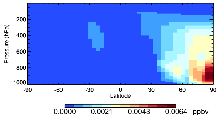
v11-02f-Run1 ASOAN - Species Curtain @ -180.000 for Jul
