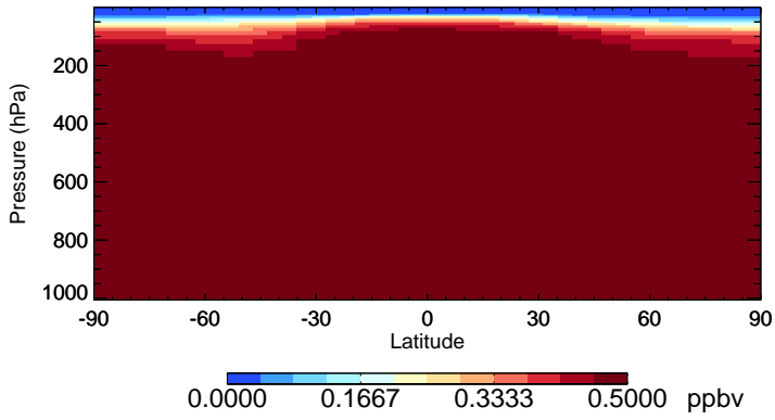
v11-02e-Run1 OCS - Species Zonal Mean for Jul
