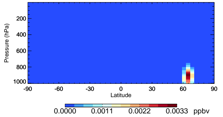
v11-02e-Run0 IEPOXB - Species Curtain @ -180.000 for Jul
