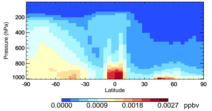
v11-02e-Run1 CHBr3 - Species Curtain @ -180.000 for Jul
