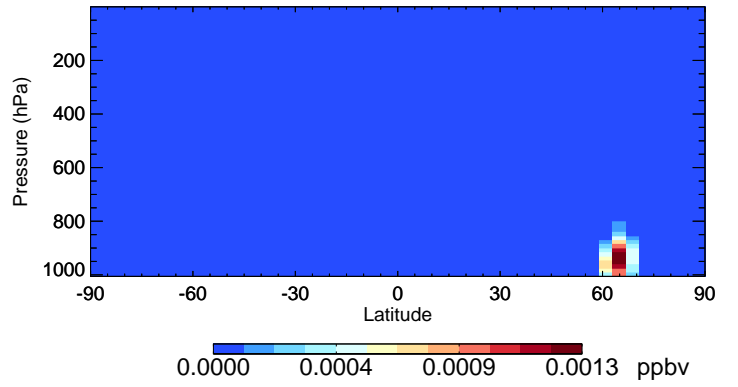
v11-02e-Run1 RIPD - Species Curtain @ -180.000 for Jul
