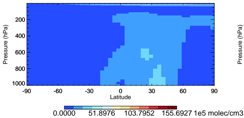
v11-02f-Run1 OH - Species Zonal Mean for Jul
