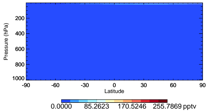
v11-02e-Run1 HO2 - Species Curtain @ -180.000 for Jul
