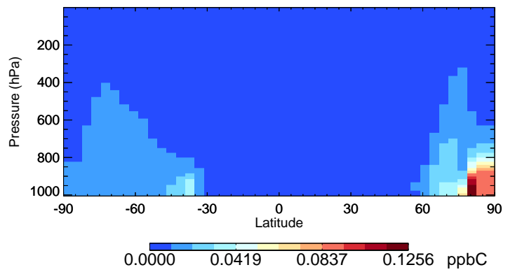
v11-02f-Run1 TOLU - Species Curtain @ -180.000 for Jul
