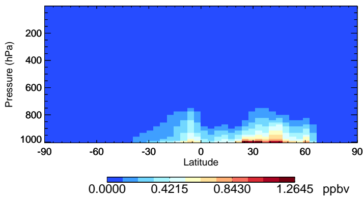
v11-02e-Run1 NH3 - Species Zonal Mean for Jul
