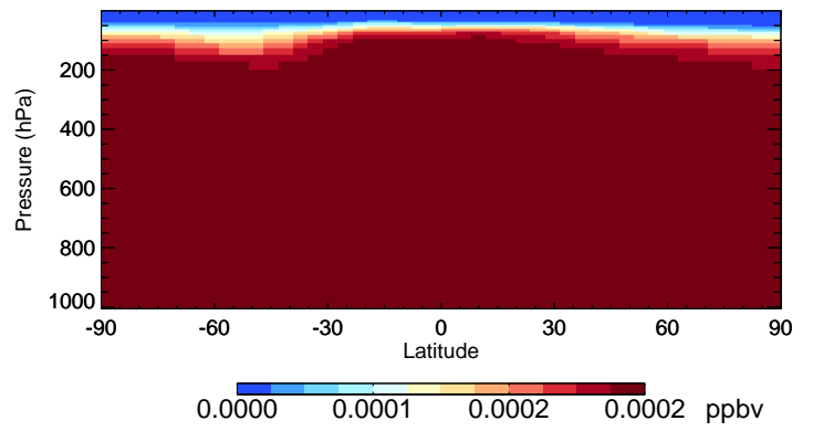
v11-02e-Run1 H2402 - Species Curtain @ -180.000 for Jul
