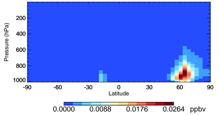
v11-02e-Run1 HAC - Species Curtain @ -180.000 for Jul
