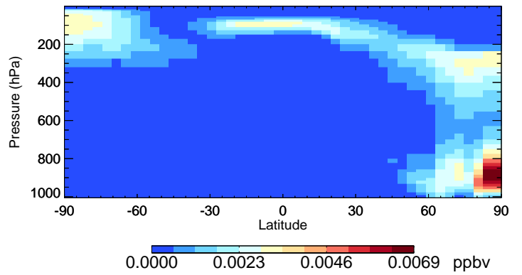
v11-02f-Run1 TSOA2 - Species Curtain @ -180.000 for Jul
