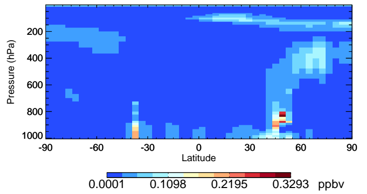
v11-02e-Run0 SO2 - Species Curtain @ -180.000 for Jul
