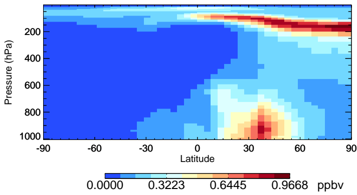
v11-02e-Run0 SO4 - Species Zonal Mean for Jul
