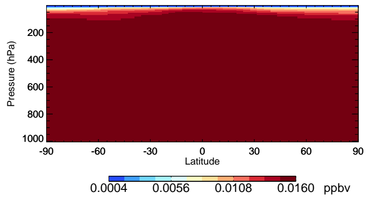
v11-02f-Run1 CFC114 - Species Curtain @ -180.000 for Jul
