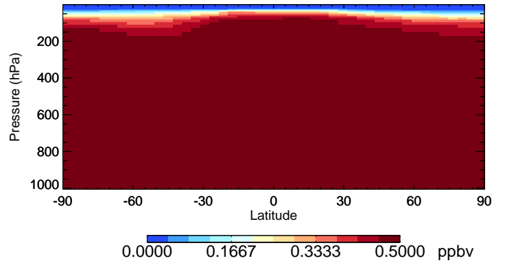
v11-02e-Run1 OCS - Species Curtain @ -180.000 for Jul
