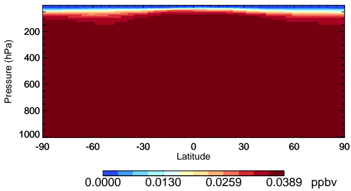
v11-02f-Run1 HCFC141b - Species Zonal Mean for Jul
