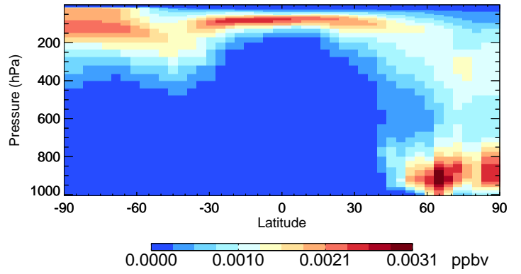
v11-02e-Run1 ISOA1 - Species Curtain @ -180.000 for Jul
