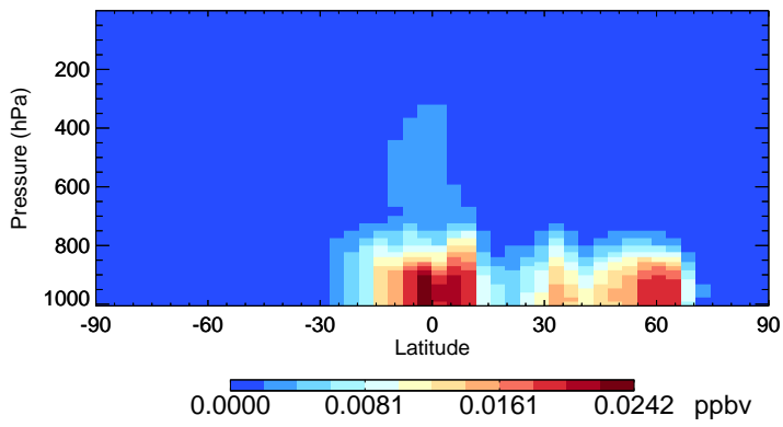
v11-02e-Run0 IPMN - Species Zonal Mean for Jul
