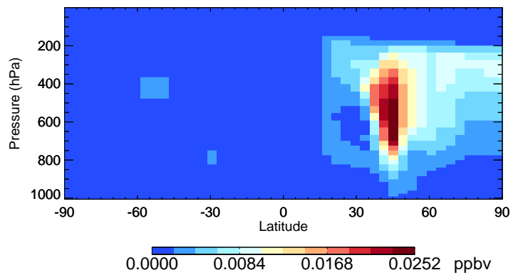
v11-02f-Run1 DST2 - Species Curtain @ -180.000 for Jul
