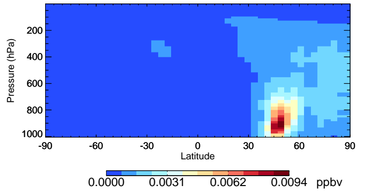
v11-02e-Run0 ASOAN - Species Curtain @ -180.000 for Jul
