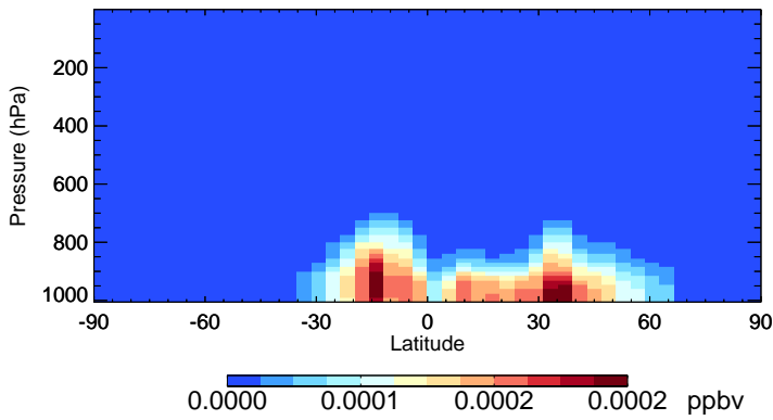
v11-02f-Run1 MACRN - Species Zonal Mean for Jul
