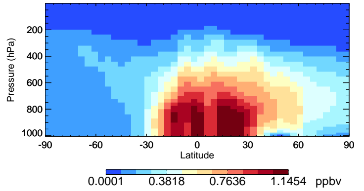
v11-02e-Run1 MP - Species Curtain @ -180.000 for Jul
