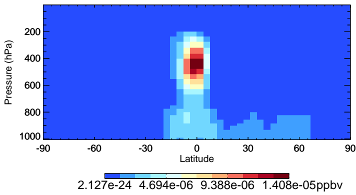
v11-02e-Run0 LVOC - Species Zonal Mean for Jul
