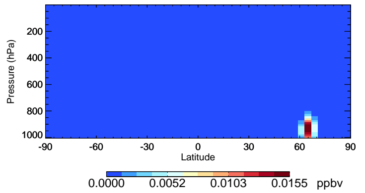
v11-02e-Run0 RIPA - Species Curtain @ -180.000 for Jul
