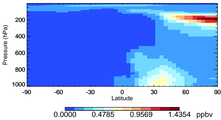
v11-02f-Run1 SO4 - Species Zonal Mean for Jul
