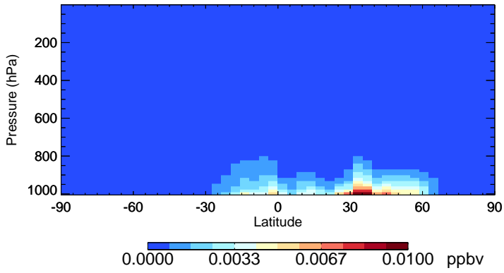
v11-02e-Run1 ISN1 - Species Zonal Mean for Jul
