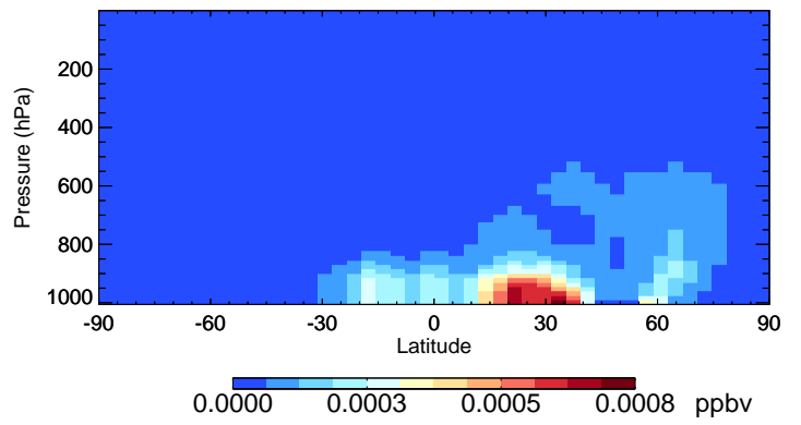
v11-02e-Run1 ACTA - Species Curtain @ -180.000 for Jul
