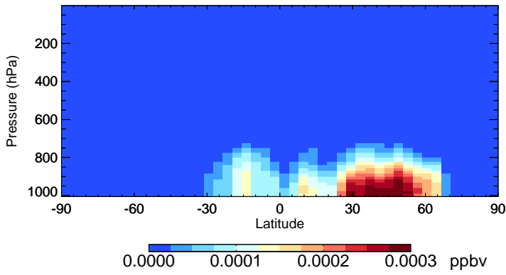
v11-02e-Run0 MACRN - Species Zonal Mean for Jul
