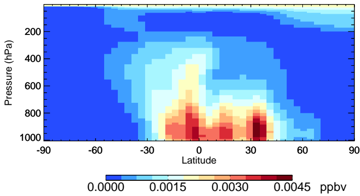
v11-02f-Run1 ISOG1 - Species Zonal Mean for Jul
