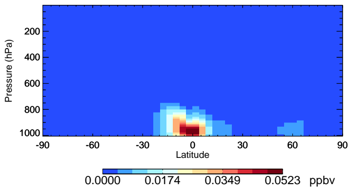
v11-02f-Run1 RIPA - Species Zonal Mean for Jul
