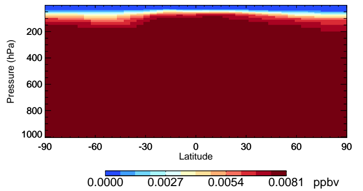
v11-02f-Run1 CH3CCI3 - Species Curtain @ -180.000 for Jul
