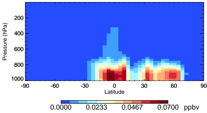
v11-02e-Run0 GLYC - Species Zonal Mean for Jul
