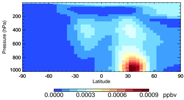
v11-02e-Run0 ASOG1 - Species Zonal Mean for Jul
