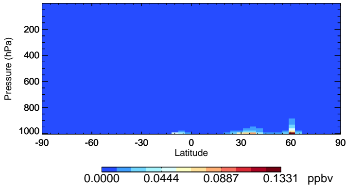
v11-02e-Run1 HNO 2 - Species Zonal Mean for Jul
