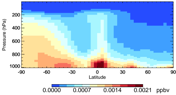
v11-02e-Run1 CHBr3 - Species Zonal Mean for Jul
