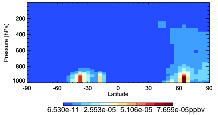
v11-02f-Run1 IONITA - Species Curtain @ -180.000 for Jul
