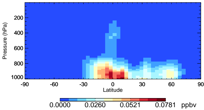
v11-02f-Run1 HAC - Species Zonal Mean for Jul
