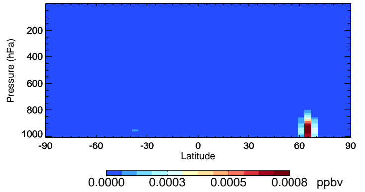
v11-02e-Run0 ISOPNB - Species Curtain @ -180.000 for Jul
