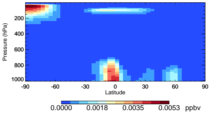
v11-02f-Run1 ISOA3 - Species Zonal Mean for Jul
