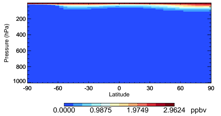
v11-02e-Run0 HCl - Species Curtain @ -180.000 for Jul
