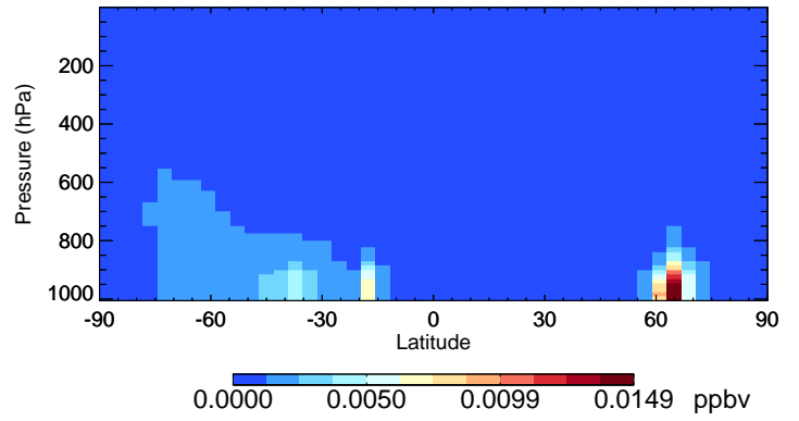
v11-02e-Run1 RCHO - Species Curtain @ -180.000 for Jul
