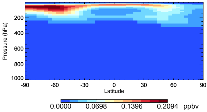
v11-02e-Run0 MPN - Species Zonal Mean for Jul
