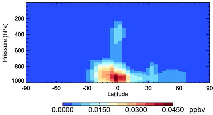
v11-02f-Run1 IEPOXA - Species Zonal Mean for Jul
