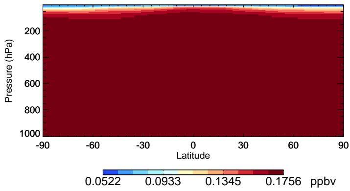
v11-02e-Run0 HCFC22 - Species Zonal Mean for Jul
