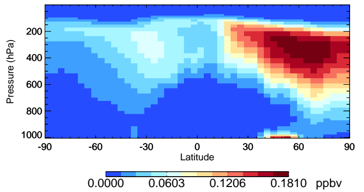
v11-02e-Run1 PAN - Species Curtain @ -180.000 for Jul
