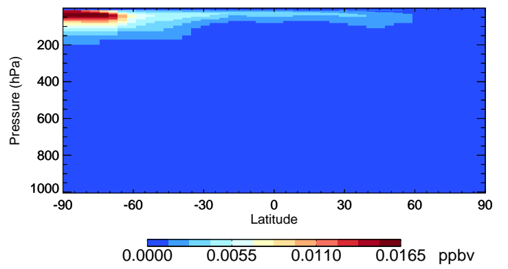
v11-02e-Run1 BrCl - Species Curtain @ -180.000 for Jul
