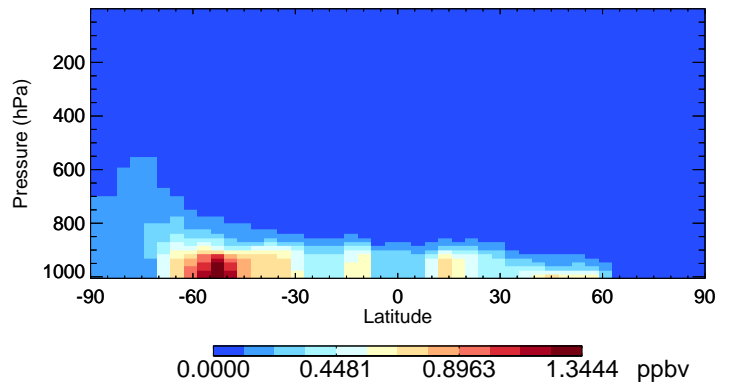
v11-02f-Run1 SALA - Species Curtain @ -180.000 for Jul
