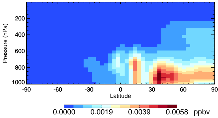
v11-02e-Run1 SOAME - Species Zonal Mean for Jul
