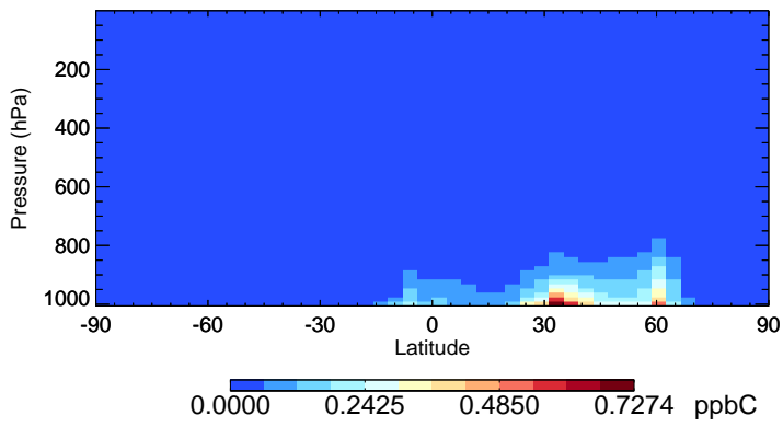
v11-02e-Run1 TOLU - Species Zonal Mean for Jul
