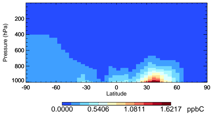
v11-02e-Run0 ALK4 - Species Zonal Mean for Jul
