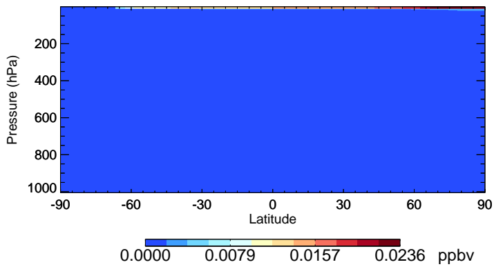
v11-02e-Run0 Br - Species Zonal Mean for Jul
