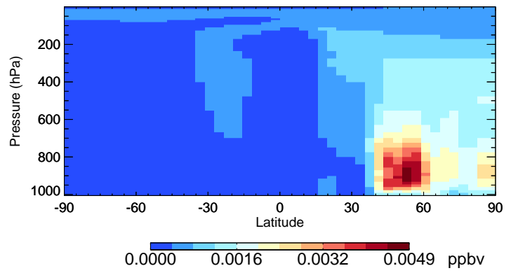
v11-02e-Run1 ASOAN - Species Curtain @ -180.000 for Jul
