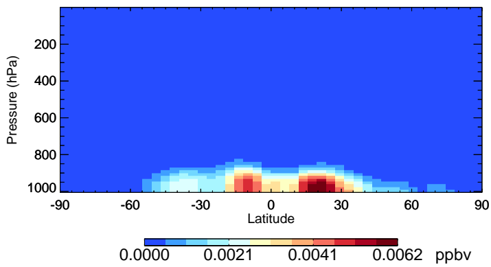
v11-02f-Run1 NITs - Species Zonal Mean for Jul
