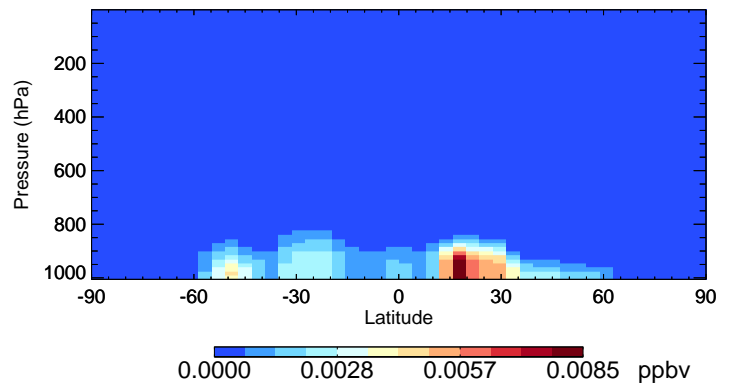
v11-02e-Run0 NITs - Species Curtain @ -180.000 for Jul
