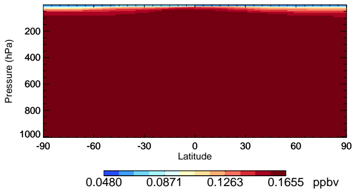
v11-02e-Run1 HCFC22 - Species Zonal Mean for Jul
