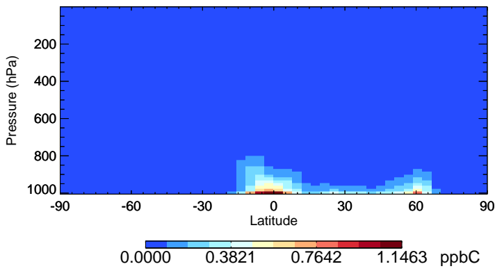
v11-02e-Run1 PRPE - Species Zonal Mean for Jul
