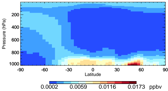
v11-02f-Run1 MSA - Species Zonal Mean for Jul
