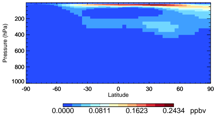
v11-02f-Run1 HNO4 - Species Zonal Mean for Jul
