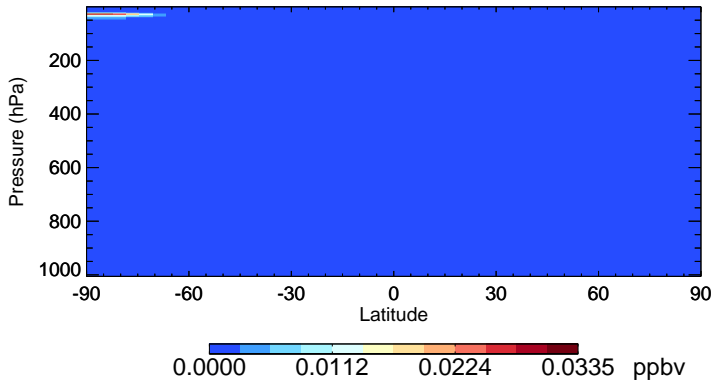
v11-02e-Run1 ClNO2 - Species Zonal Mean for Jul
