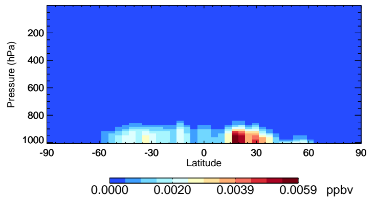
v11-02f-Run1 NITs - Species Curtain @ -180.000 for Jul
