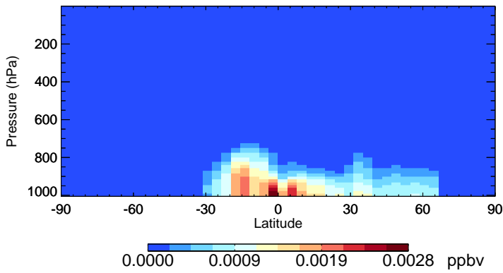
v11-02f-Run1 ISOPNB - Species Zonal Mean for Jul
