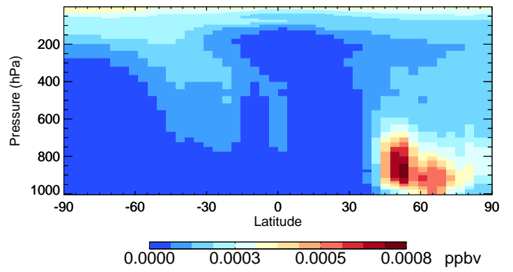
v11-02e-Run0 LVOCOA - Species Curtain @ -180.000 for Jul
