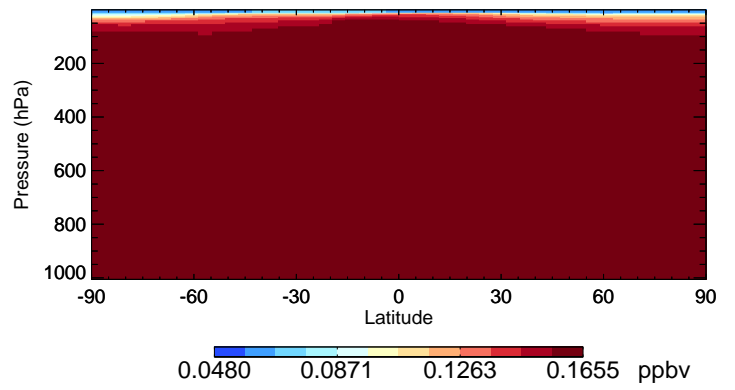
v11-02e-Run1 HCFC22 - Species Curtain @ -180.000 for Jul
