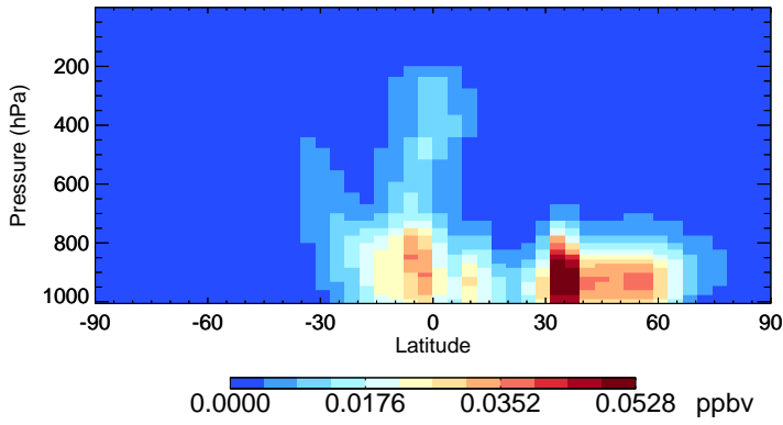
v11-02e-Run1 IMAE - Species Zonal Mean for Jul
