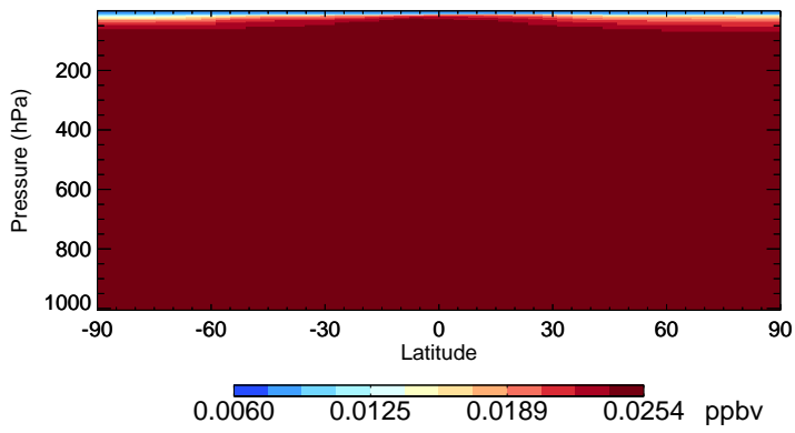
v11-02e-Run1 HCFC142b - Species Zonal Mean for Jul
