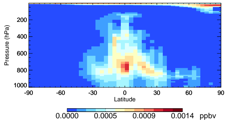
v11-02e-Run1 HBr - Species Curtain @ -180.000 for Jul
