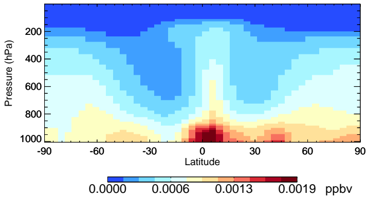
v11-02e-Run0 CHBr3 - Species Zonal Mean for Oct
