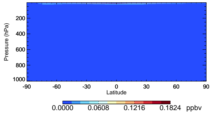
v11-02f-Run1 NO3 - Species Curtain @ -180.000 for Oct
