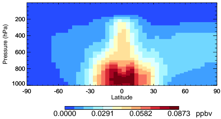
v11-02f-Run1 MAP - Species Zonal Mean for Oct
