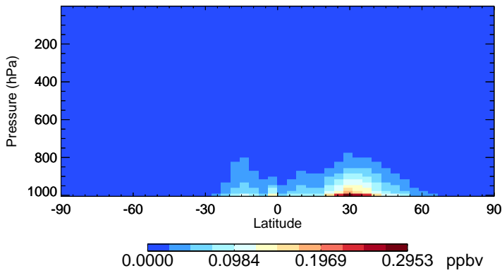
v11-02f-Run1 BCPO - Species Zonal Mean for Oct
