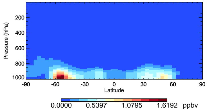
v11-02e-Run0 SALA - Species Curtain @ -180.000 for Oct
