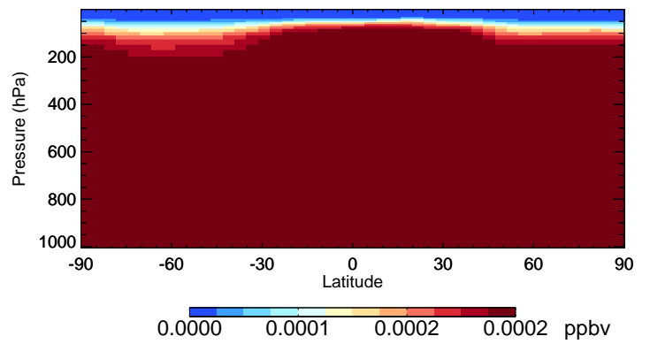
v11-02f-Run1 H2402 - Species Curtain @ -180.000 for Oct
