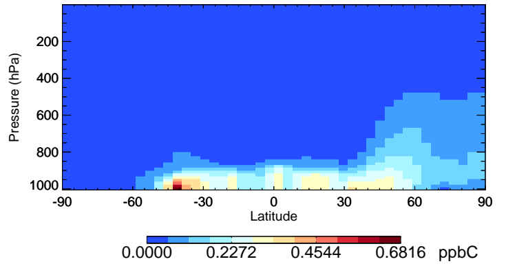
v11-02e-Run1 ALD2 - Species Curtain @ -180.000 for Oct
