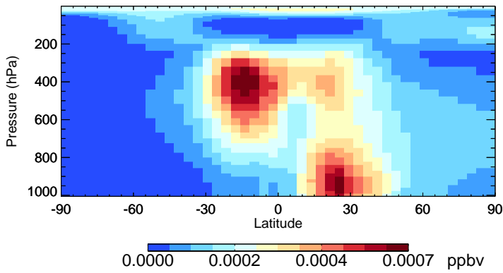
v11-02f-Run1 ASOG1 - Species Zonal Mean for Oct
