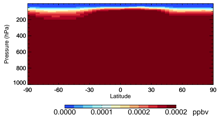
v11-02e-Run1 H2402 - Species Curtain @ -180.000 for Oct
