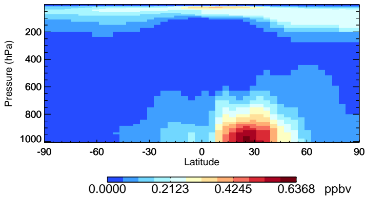
v11-02f-Run1 SO4 - Species Zonal Mean for Oct
