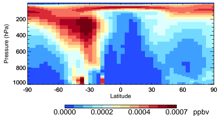
v11-02e-Run1 TSOA0 - Species Curtain @ -180.000 for Oct
