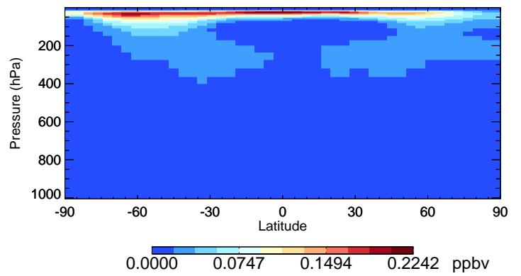
v11-02f-Run1 HNO4 - Species Curtain @ -180.000 for Oct
