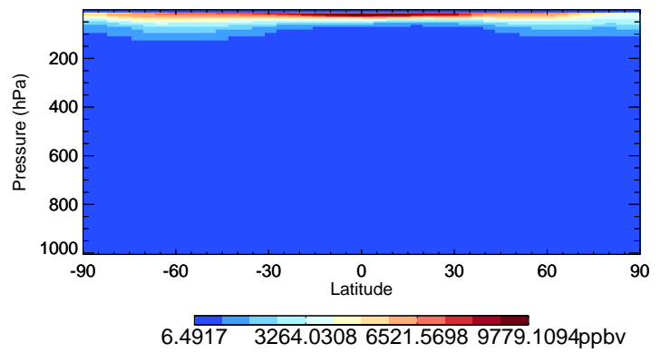
v11-02f-Run1 O3 - Species Curtain @ -180.000 for Oct
