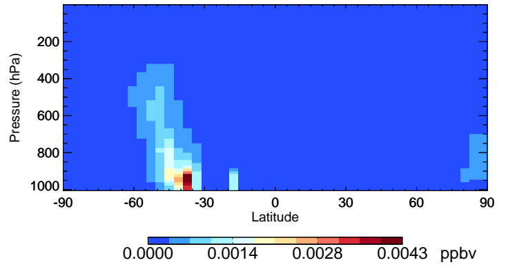
v11-02e-Run1 GLYC - Species Curtain @ -180.000 for Oct
