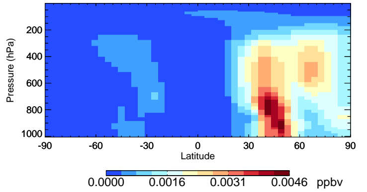
v11-02e-Run1 SOAGX - Species Curtain @ -180.000 for Oct
