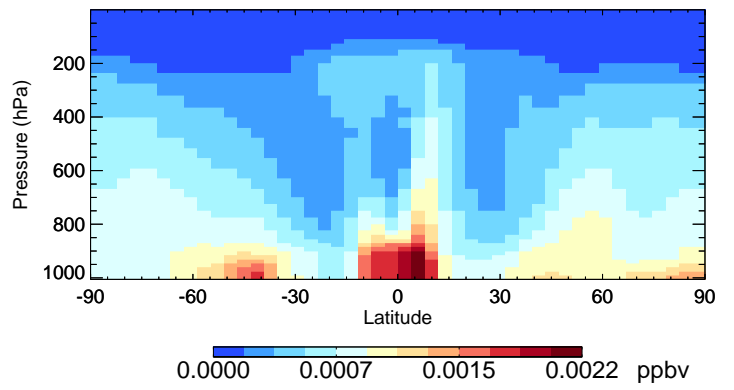
v11-02e-Run1 CHBr3 - Species Curtain @ -180.000 for Oct
