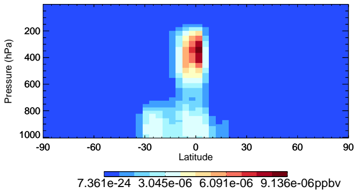
v11-02f-Run1 LVOC - Species Zonal Mean for Oct
