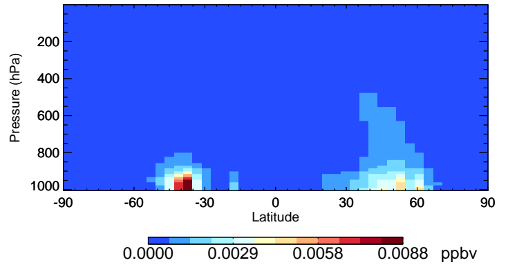
v11-02e-Run1 BCPO - Species Curtain @ -180.000 for Oct
