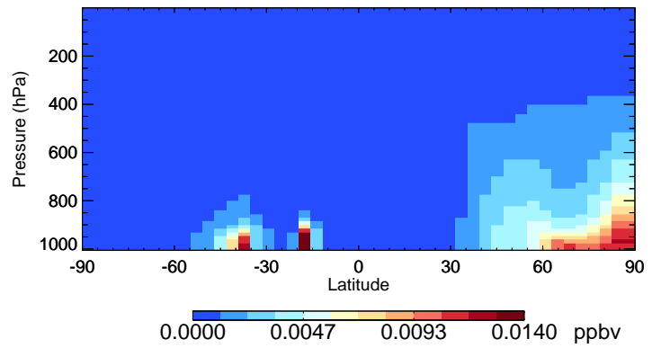
v11-02f-Run1 RCHO - Species Curtain @ -180.000 for Oct
