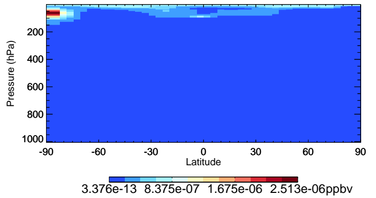
v11-02f-Run1 CIOO - Species Curtain @ -180.000 for Oct
