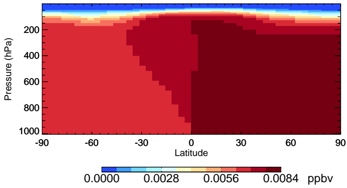
v11-02e-Run0 CH3Br - Species Zonal Mean for Oct
