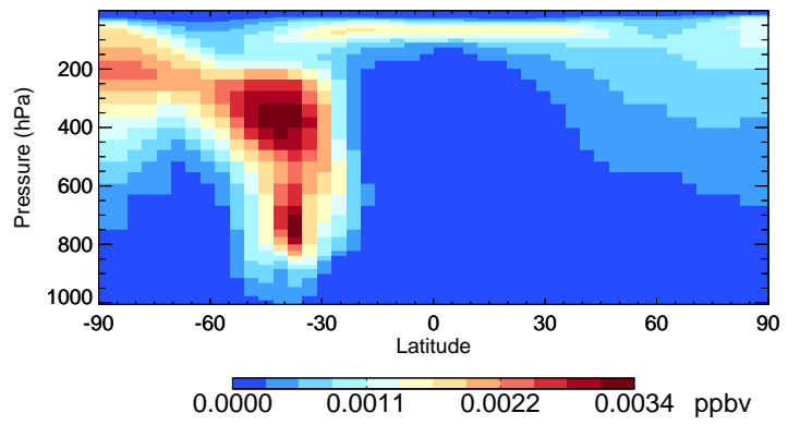
v11-02e-Run0 ISOA1 - Species Curtain @ -180.000 for Oct
