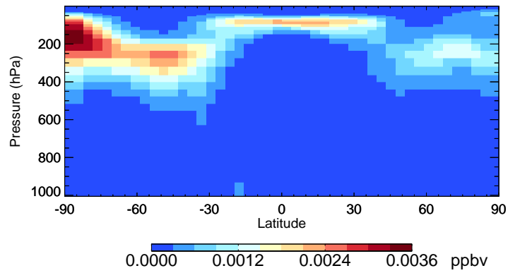
v11-02f-Run1 TSOA2 - Species Curtain @ -180.000 for Oct
