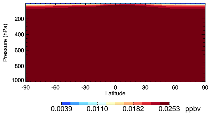
v11-02f-Run1 HCFC142b - Species Zonal Mean for Oct
