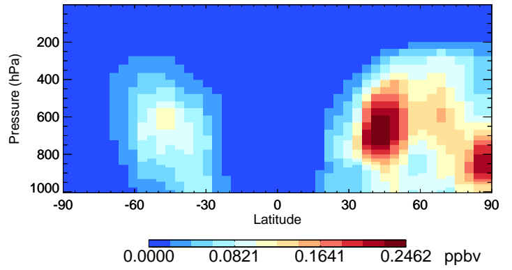
v11-02e-Run1 DST1 - Species Curtain @ -180.000 for Oct
