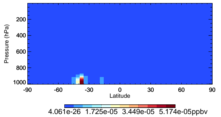
v11-02f-Run1 MOBA - Species Curtain @ -180.000 for Oct
