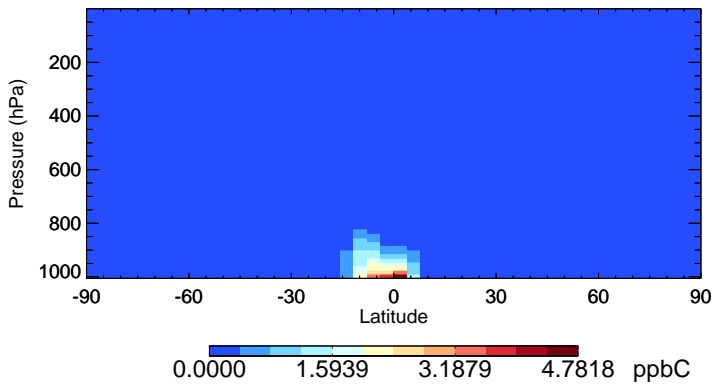
v11-02f-Run1 ISOP - Species Zonal Mean for Oct
