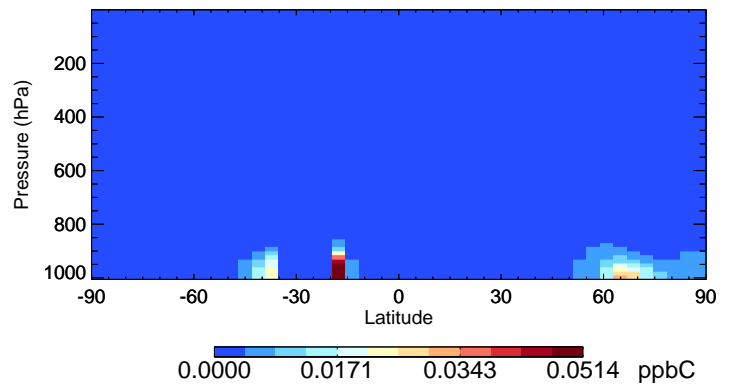
v11-02e-Run1 PRPE - Species Curtain @ -180.000 for Oct
