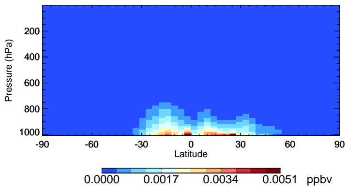
v11-02f-Run1 ISN1 - Species Zonal Mean for Oct
