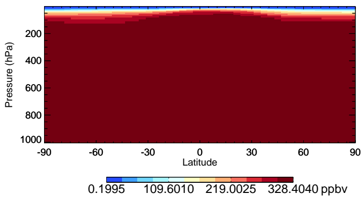
v11-02f-Run1 N2O - Species Zonal Mean for Oct
