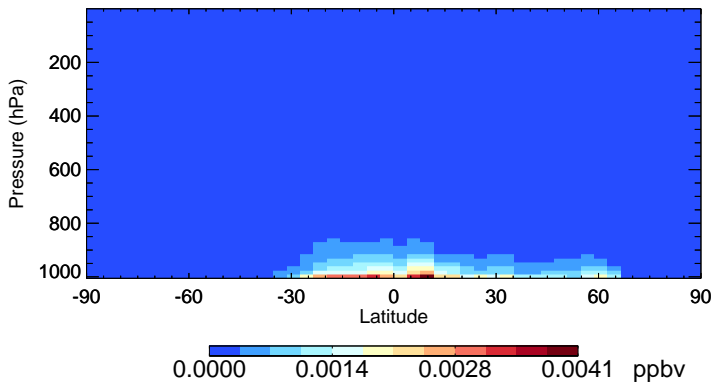
v11-02f-Run1 MONITS - Species Zonal Mean for Oct
