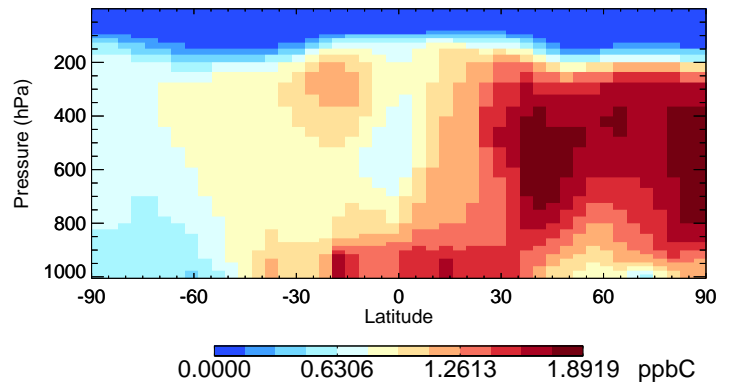
v11-02f-Run1 ACET - Species Curtain @ -180.000 for Oct
