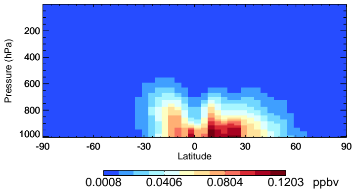
v11-02f-Run1 INDIOL - Species Zonal Mean for Oct
