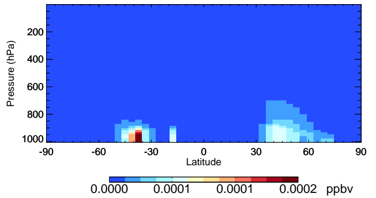
v11-02f-Run1 IONITA - Species Curtain @ -180.000 for Oct
