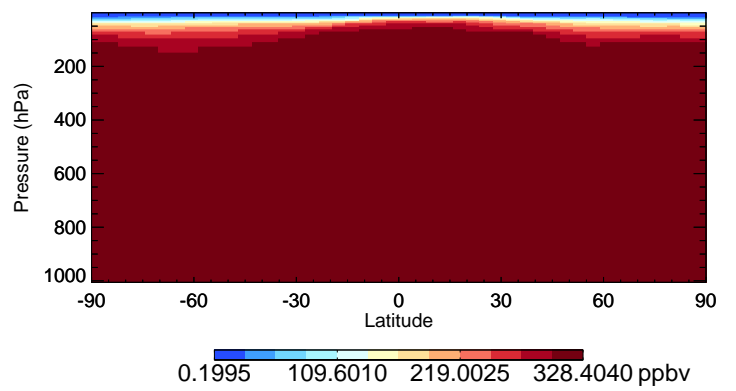
v11-02f-Run1 N2O - Species Curtain @ -180.000 for Oct
