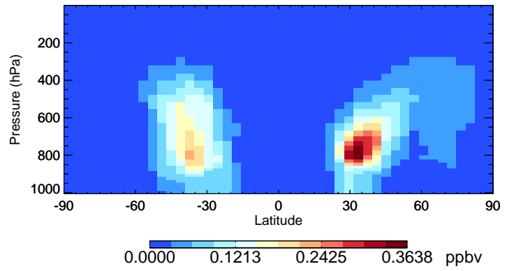
v11-02e-Run0 DST2 - Species Curtain @ -180.000 for Oct
