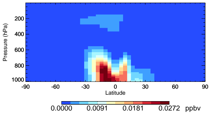
v11-02e-Run1 ISOA1 - Species Zonal Mean for Oct
