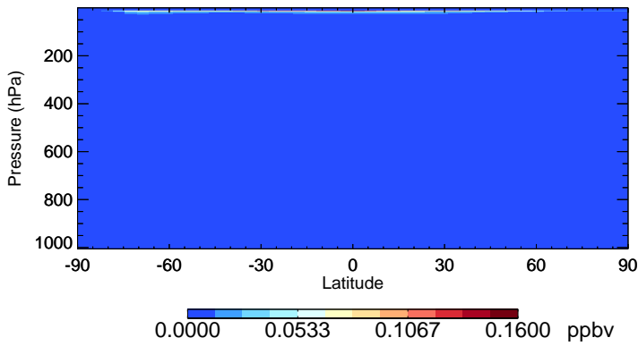
v11-02f-Run1 NO3 - Species Zonal Mean for Oct
