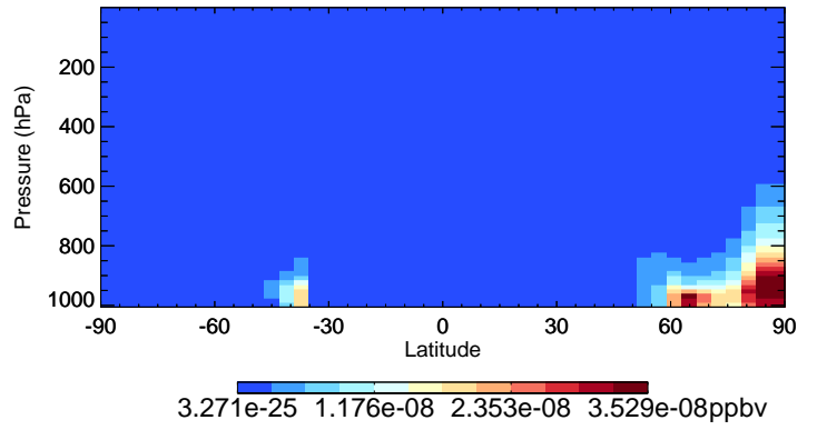
v11-02e-Run1 NPMN - Species Curtain @ -180.000 for Oct
