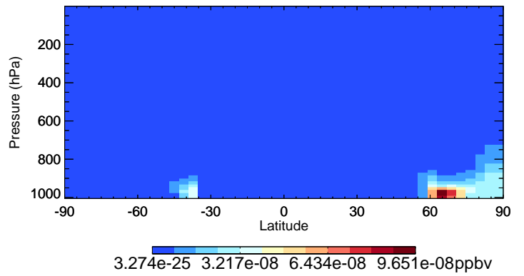
v11-02f-Run1 NPMN - Species Curtain @ -180.000 for Oct
