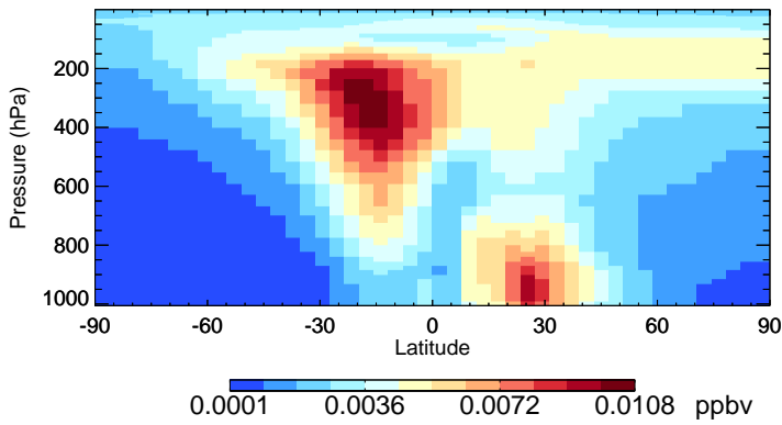
v11-02f-Run1 ASOG3 - Species Zonal Mean for Oct
