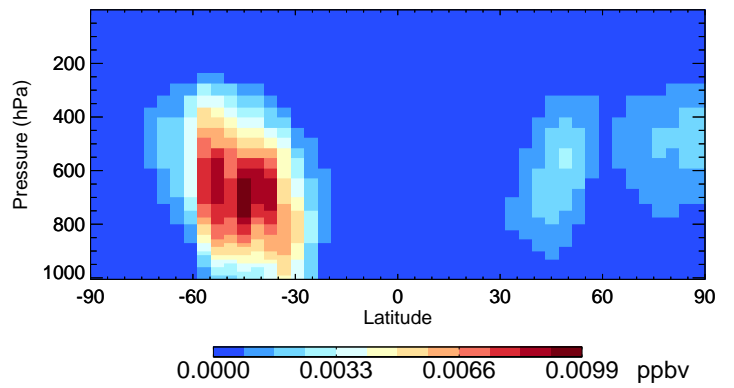
v11-02e-Run1 DST4 - Species Curtain @ -180.000 for Oct
