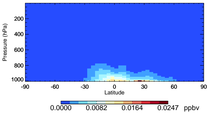
v11-02f-Run1 GLYX - Species Zonal Mean for Oct
