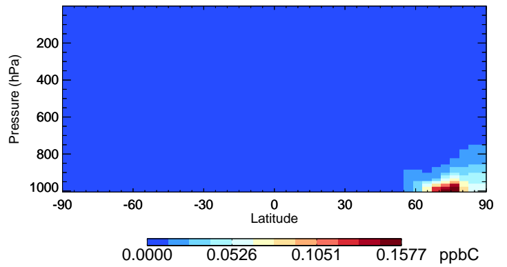
v11-02f-Run1 XYLE - Species Curtain @ -180.000 for Oct
