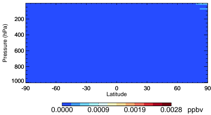
v11-02f-Run1 Br2 - Species Zonal Mean for Oct
