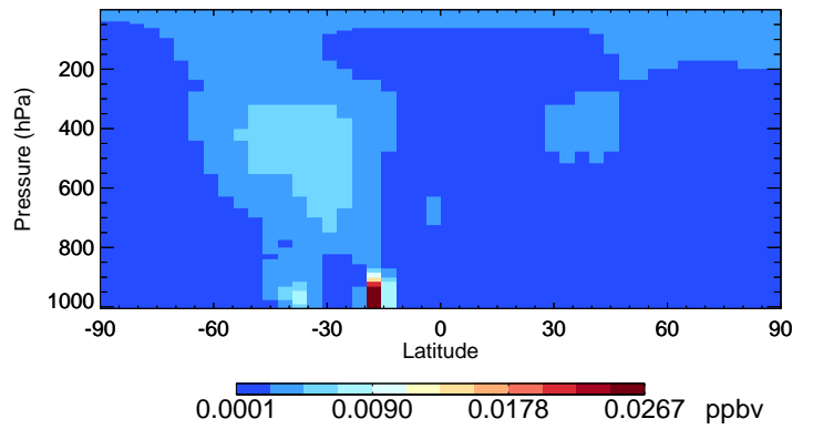
v11-02f-Run1 TSOG2 - Species Curtain @ -180.000 for Oct
