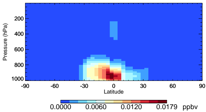
v11-02f-Run1 IEPOXB - Species Zonal Mean for Oct
