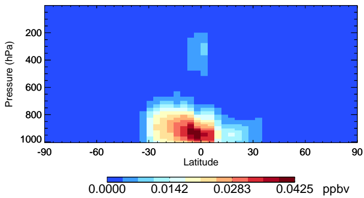
v11-02f-Run1 IEPOXA - Species Zonal Mean for Oct
