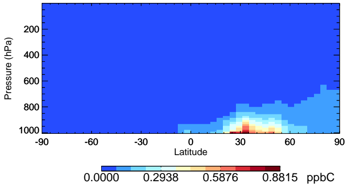
v11-02e-Run1 TOLU - Species Zonal Mean for Oct
