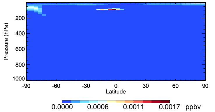
v11-02f-Run1 Cl2 - Species Curtain @ -180.000 for Oct
