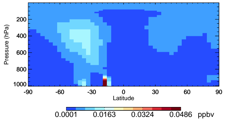
v11-02f-Run1 TSOG3 - Species Curtain @ -180.000 for Oct
