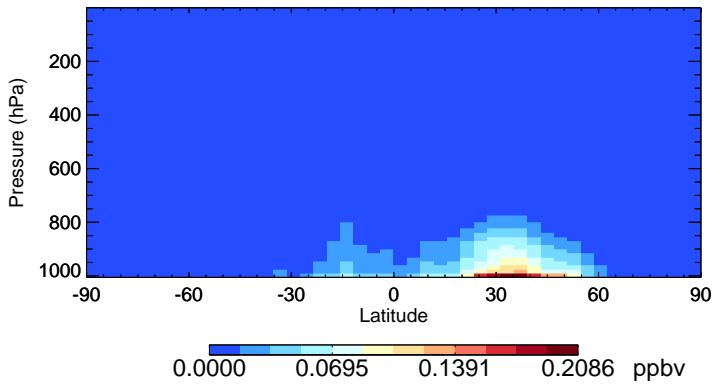
v11-02e-Run0 BCPO - Species Zonal Mean for Oct
