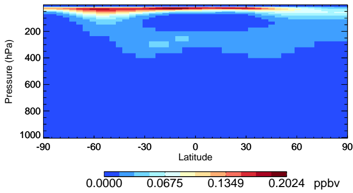
v11-02e-Run0 HNO4 - Species Zonal Mean for Oct
