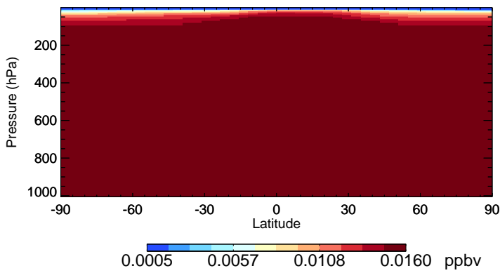
v11-02f-Run1 CFC114 - Species Zonal Mean for Oct
