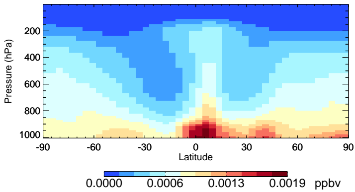
v11-02f-Run1 CHBr3 - Species Zonal Mean for Oct
