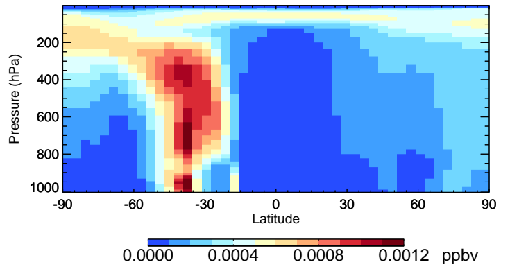
v11-02e-Run0 TSOA0 - Species Curtain @ -180.000 for Oct
