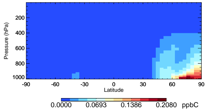
v11-02f-Run1 TOLU - Species Curtain @ -180.000 for Oct
