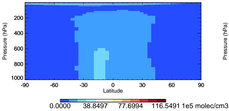
v11-02f-Run1 OH - Species Zonal Mean for Oct
