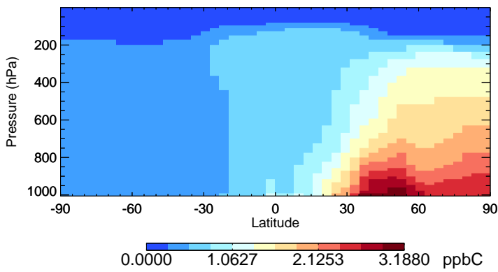
v11-02f-Run1 C2H6 - Species Zonal Mean for Oct
