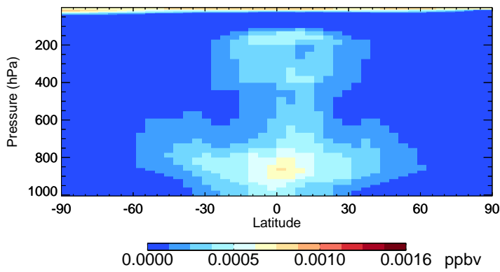
v11-02f-Run1 HBr - Species Zonal Mean for Oct
