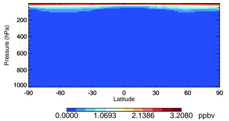
v11-02f-Run1 HCl - Species Curtain @ -180.000 for Oct
