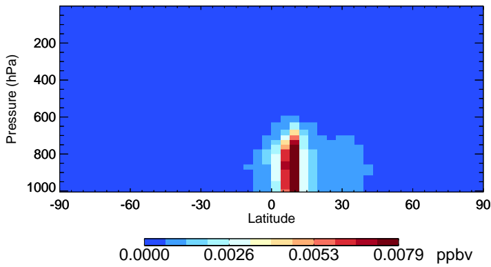
v11-02f-Run1 SOAME - Species Zonal Mean for Oct
