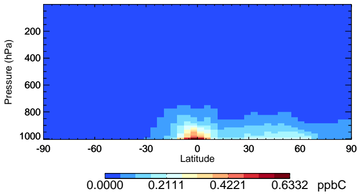
v11-02f-Run1 EOH - Species Zonal Mean for Oct
