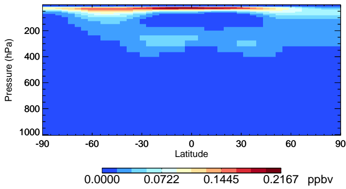
v11-02e-Run1 HNO4 - Species Zonal Mean for Oct
