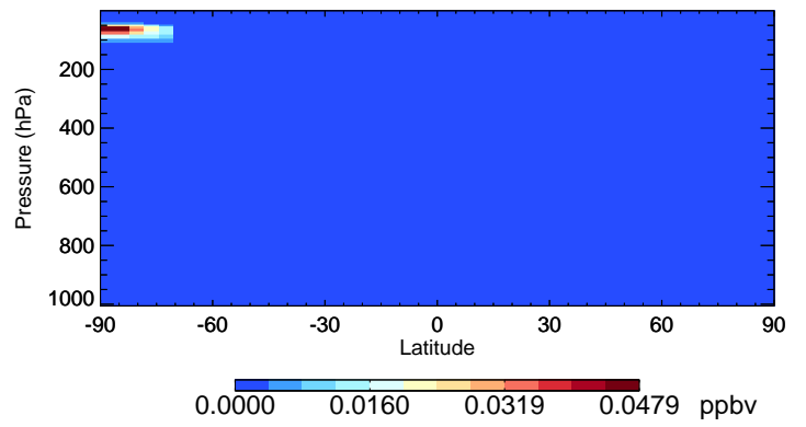
v11-02e-Run1 Cl2O2 - Species Curtain @ -180.000 for Oct
