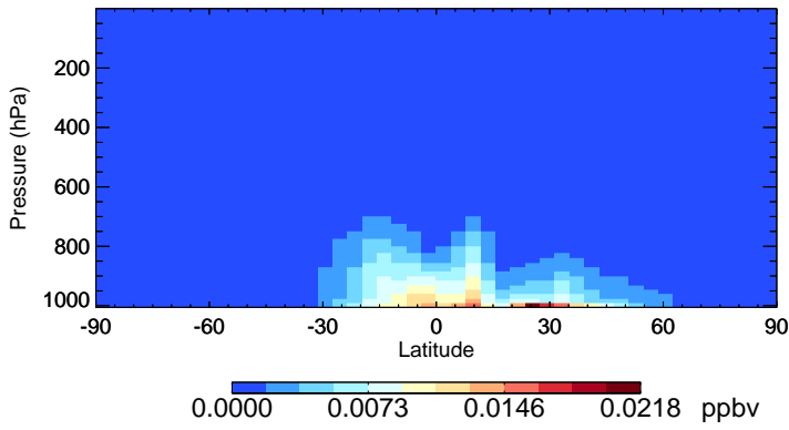
v11-02e-Run0 GLYX - Species Zonal Mean for Oct
