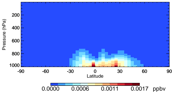
v11-02f-Run1 IONITA - Species Zonal Mean for Oct
