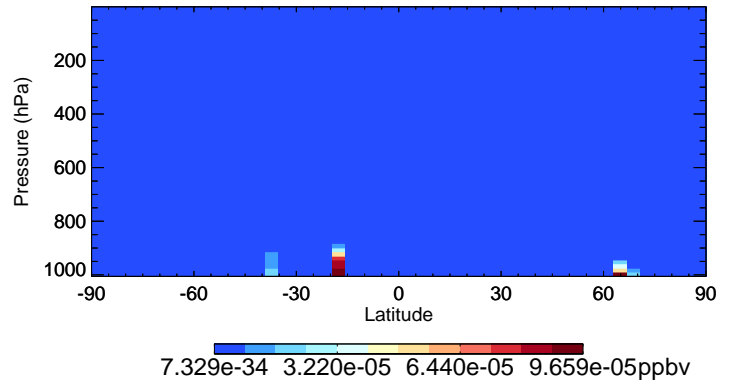
v11-02e-Run1 LIMO - Species Curtain @ -180.000 for Oct
