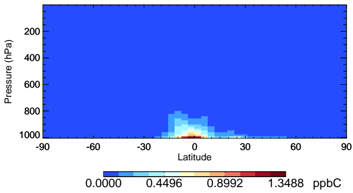
v11-02e-Run1 PRPE - Species Zonal Mean for Oct
