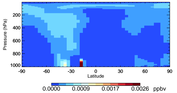
v11-02f-Run1 TSOA0 - Species Curtain @ -180.000 for Oct
