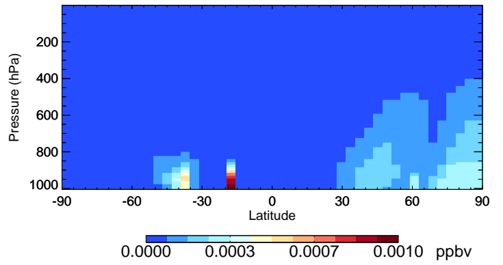
v11-02e-Run0 GLYX - Species Curtain @ -180.000 for Oct
