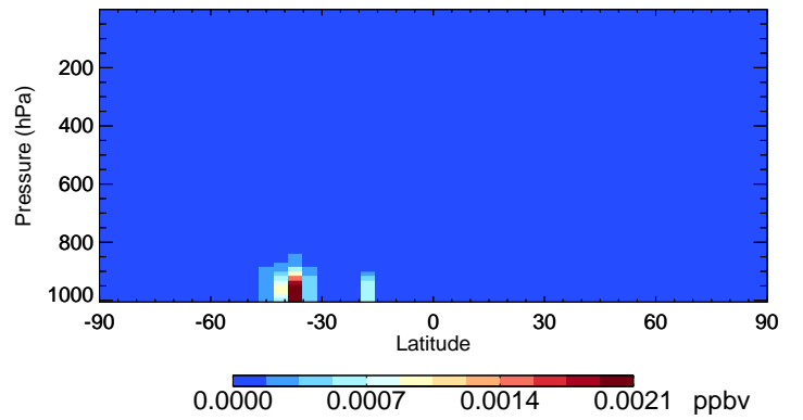
v11-02f-Run1 RIPA - Species Curtain @ -180.000 for Oct
