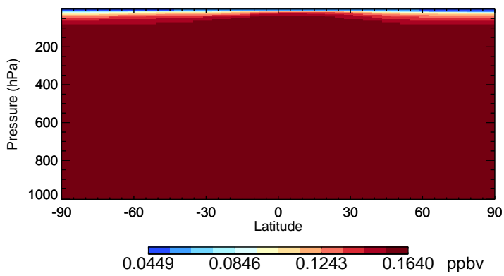
v11-02f-Run1 HCFC22 - Species Zonal Mean for Oct
