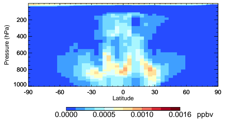
v11-02f-Run1 HBr - Species Curtain @ -180.000 for Oct
