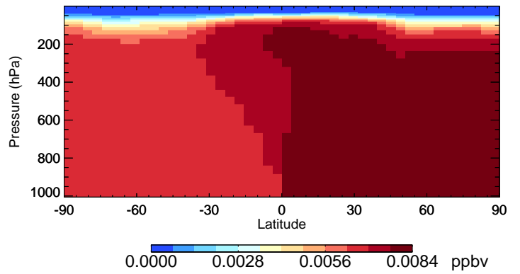
v11-02f-Run1 CH3Br - Species Curtain @ -180.000 for Oct
