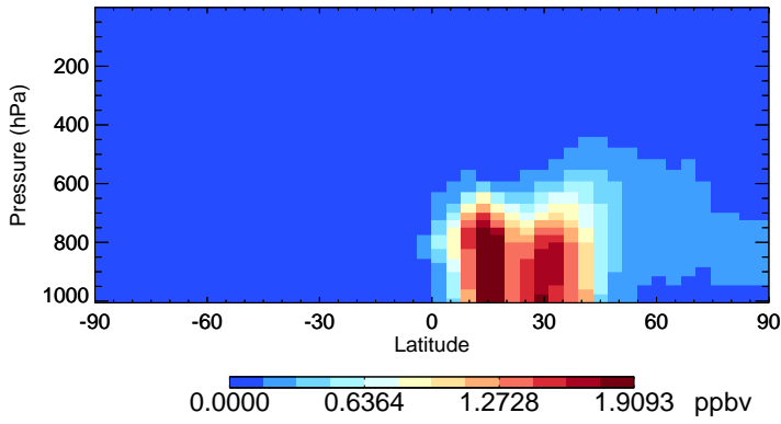
v11-02e-Run1 DST1 - Species Zonal Mean for Oct
