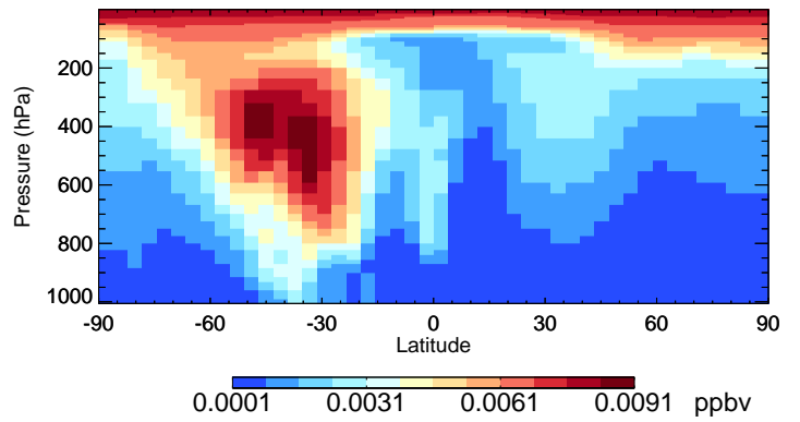
v11-02f-Run1 ISOG3 - Species Curtain @ -180.000 for Oct
