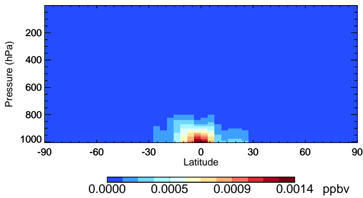
v11-02f-Run1 MOBA - Species Zonal Mean for Oct
