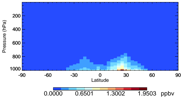
v11-02f-Run1 NH3 - Species Zonal Mean for Oct
