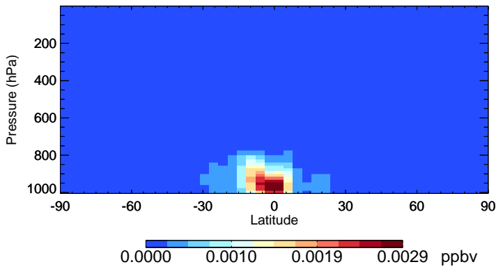
v11-02f-Run1 RIPD - Species Zonal Mean for Oct
