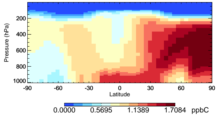
v11-02e-Run0 ACET - Species Curtain @ -180.000 for Oct
