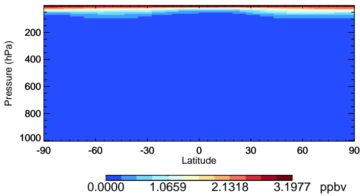
v11-02f-Run1 HCl - Species Zonal Mean for Oct
