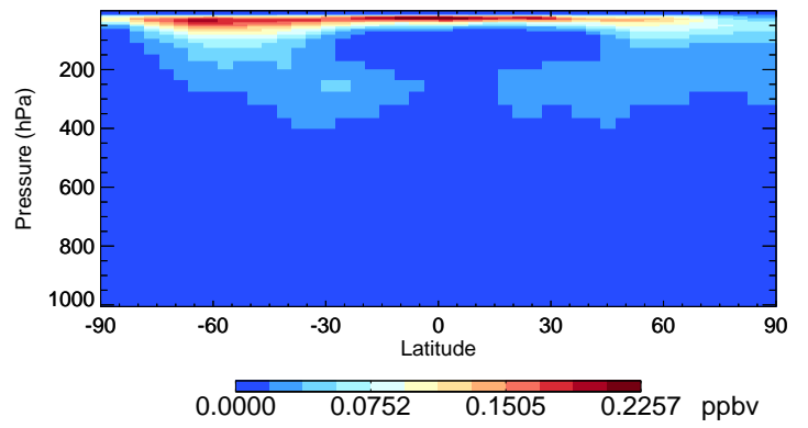
v11-02e-Run1 HNO4 - Species Curtain @ -180.000 for Oct
