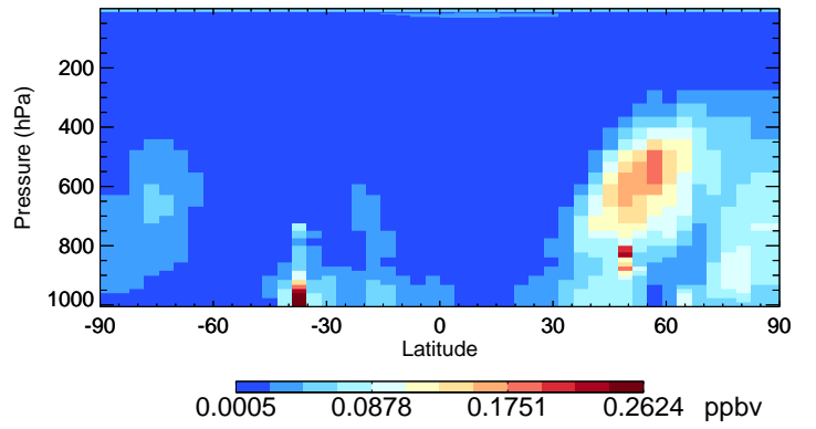
v11-02e-Run0 SO2 - Species Curtain @ -180.000 for Oct
