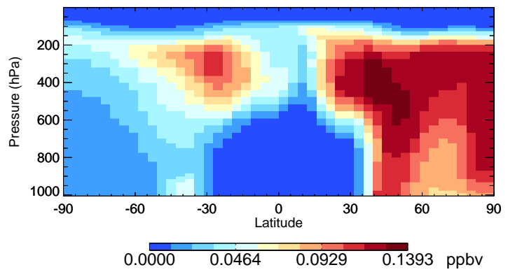
v11-02f-Run1 PAN - Species Curtain @ -180.000 for Oct
