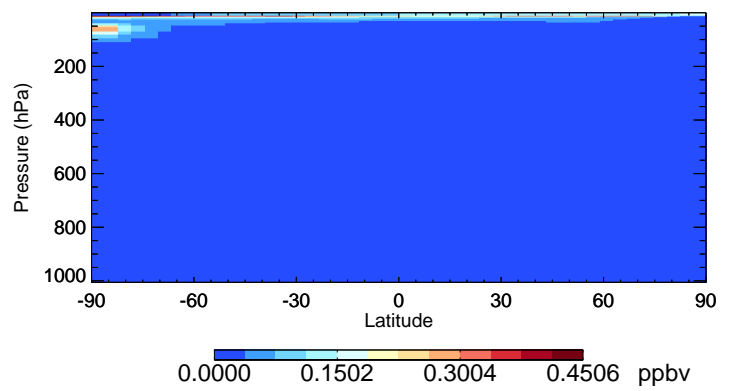
v11-02f-Run1 ClO - Species Curtain @ -180.000 for Oct
