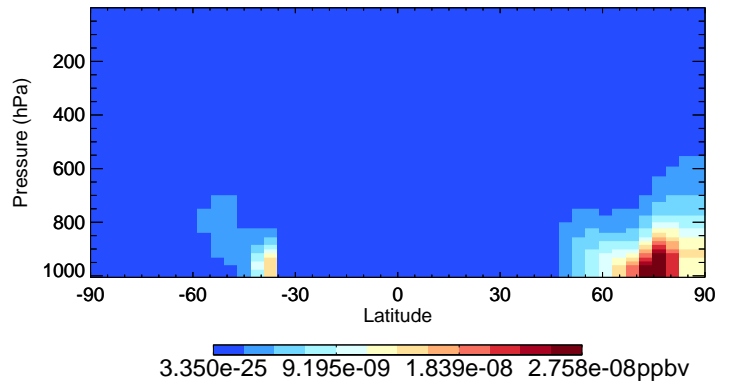
v11-02e-Run0 NPMN - Species Curtain @ -180.000 for Oct
