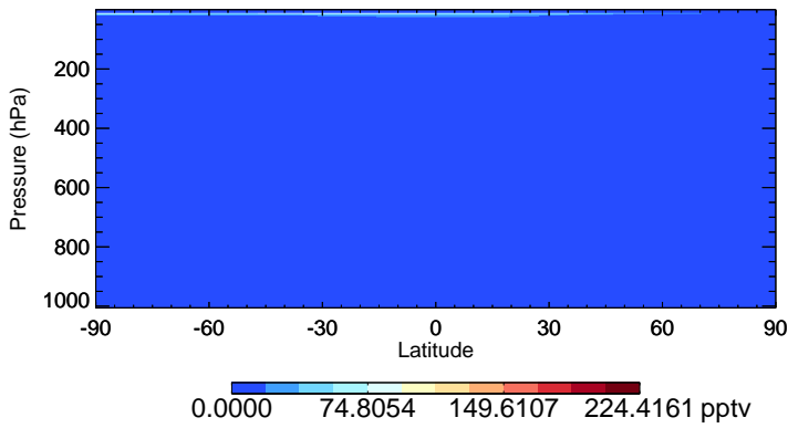
v11-02f-Run1 HO2 - Species Zonal Mean for Oct
