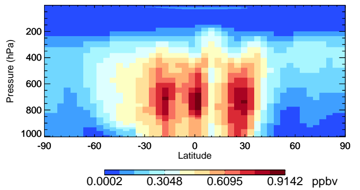
v11-02f-Run1 H2O2 - Species Curtain @ -180.000 for Oct
