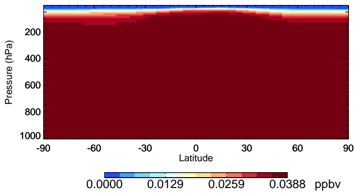
v11-02f-Run1 HCFC141b - Species Zonal Mean for Oct
