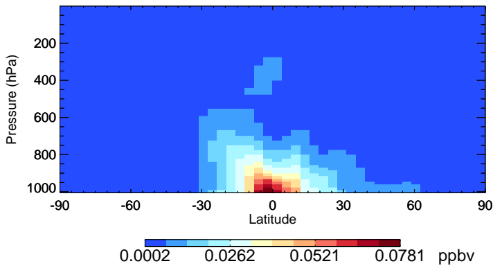
v11-02f-Run1 TSOG2 - Species Zonal Mean for Oct
