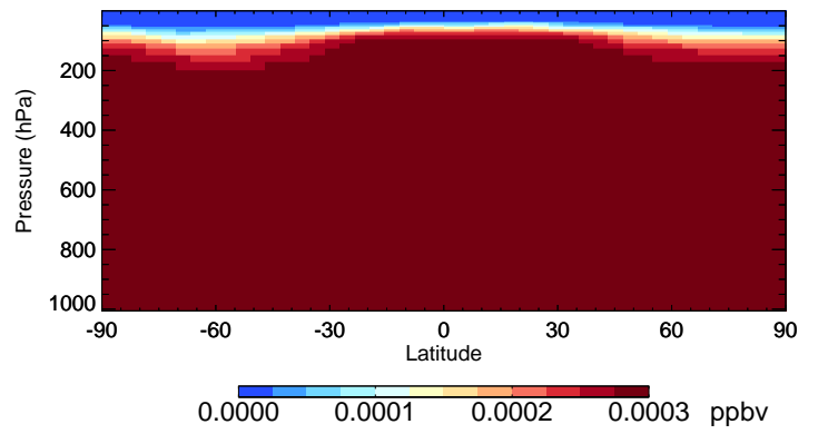
v11-02e-Run0 H2402 - Species Curtain @ -180.000 for Oct
