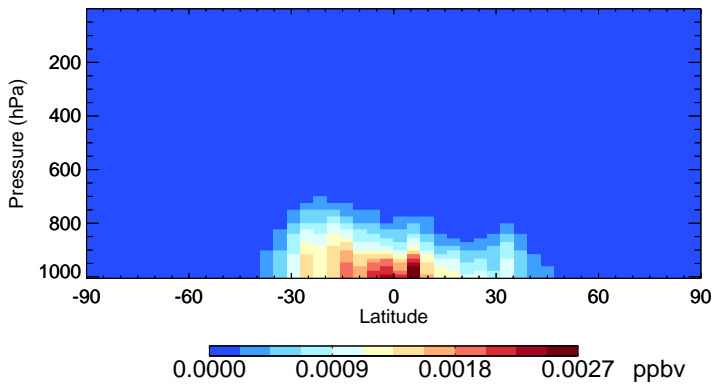
v11-02f-Run1 ISOPNB - Species Zonal Mean for Oct
