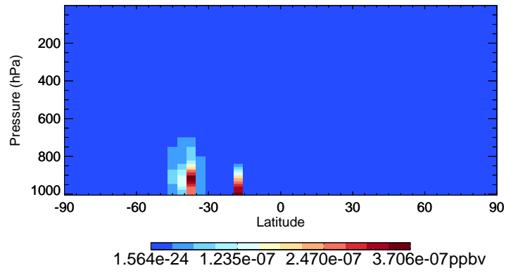
v11-02e-Run0 LVOC - Species Curtain @ -180.000 for Oct
