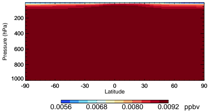
v11-02f-Run1 CFC115 - Species Zonal Mean for Oct
