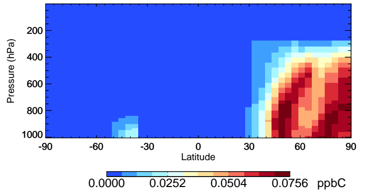
v11-02e-Run0 TOLU - Species Curtain @ -180.000 for Oct
