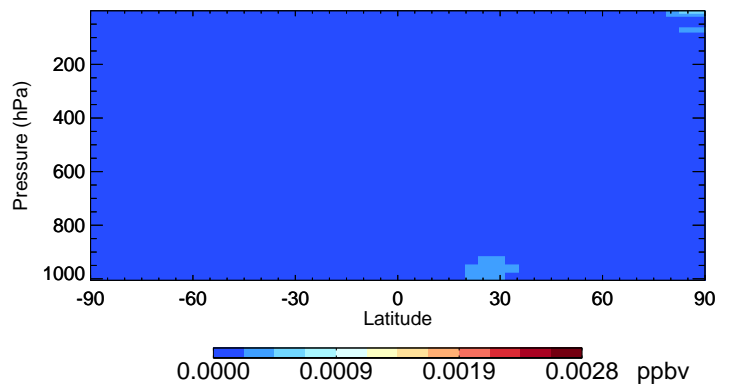
v11-02f-Run1 Br2 - Species Curtain @ -180.000 for Oct
