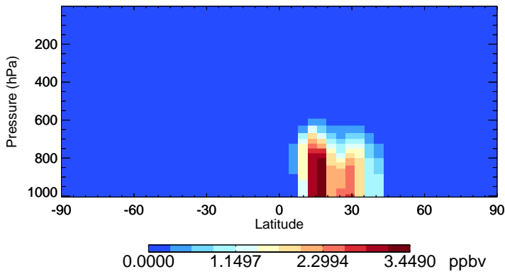
v11-02f-Run1 DST2 - Species Zonal Mean for Oct
