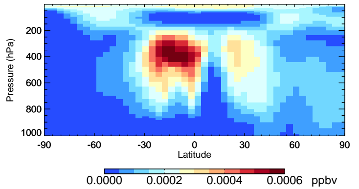
v11-02f-Run1 ASOG1 - Species Curtain @ -180.000 for Oct
