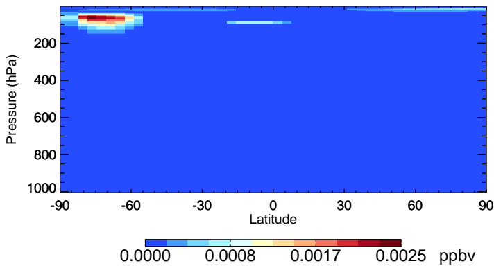
v11-02f-Run1 Cl2 - Species Zonal Mean for Oct
