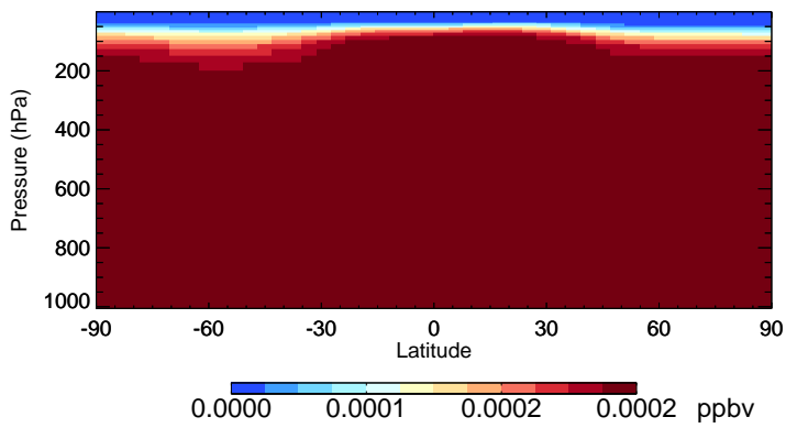
v11-02f-Run1 H2402 - Species Zonal Mean for Oct
