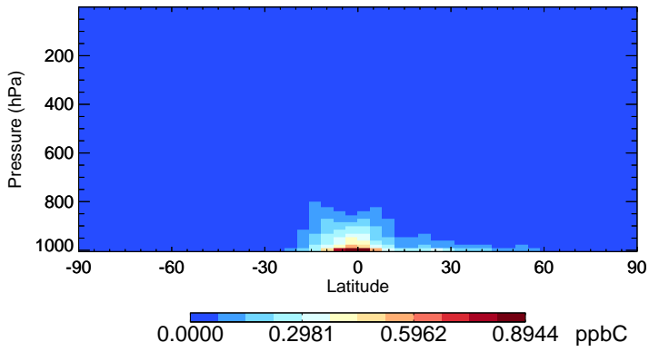
v11-02e-Run0 PRPE - Species Zonal Mean for Oct
