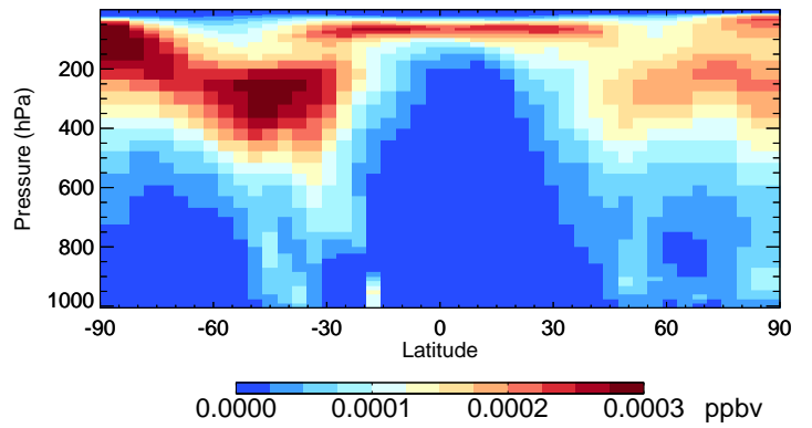
v11-02f-Run1 TSOA1 - Species Curtain @ -180.000 for Oct
