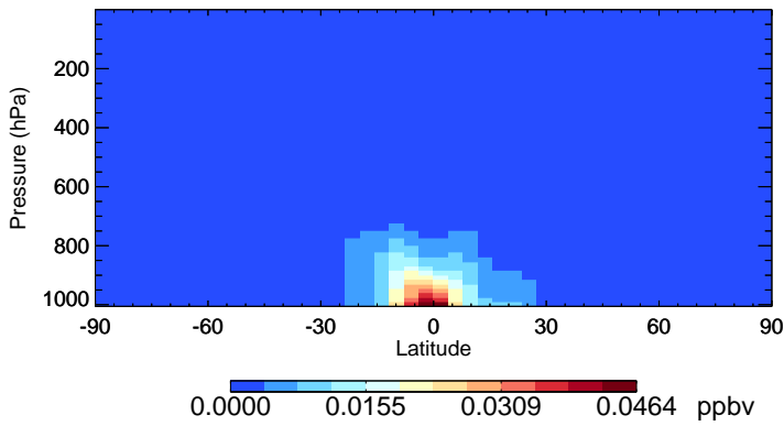
v11-02f-Run1 TSOA0 - Species Zonal Mean for Oct
