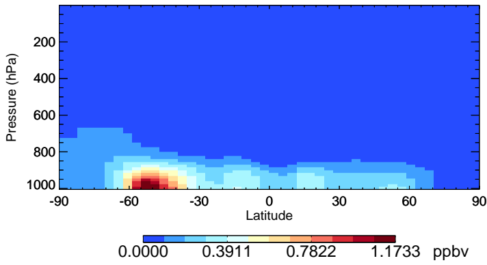
v11-02e-Run0 SALA - Species Zonal Mean for Oct
