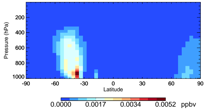
v11-02e-Run0 GLYC - Species Curtain @ -180.000 for Oct
