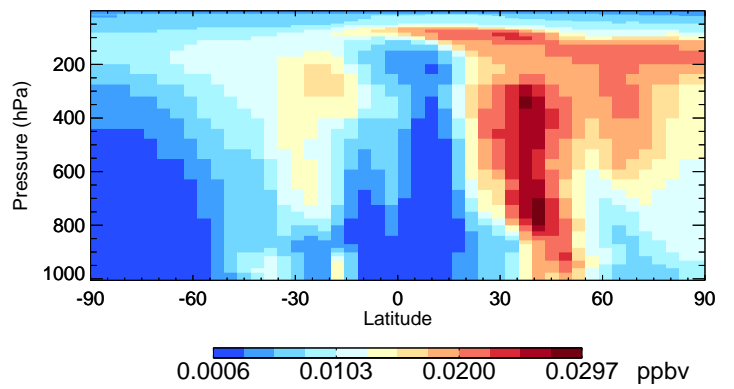
v11-02f-Run1 SOAS - Species Curtain @ -180.000 for Oct
