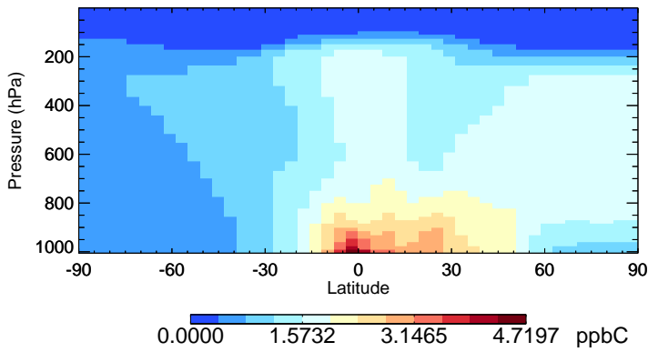
v11-02f-Run1 ACET - Species Zonal Mean for Oct
