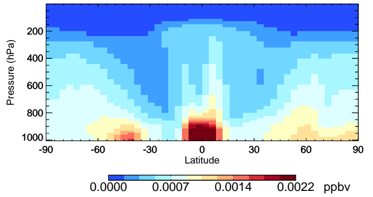
v11-02e-Run0 CHBr3 - Species Curtain @ -180.000 for Oct
