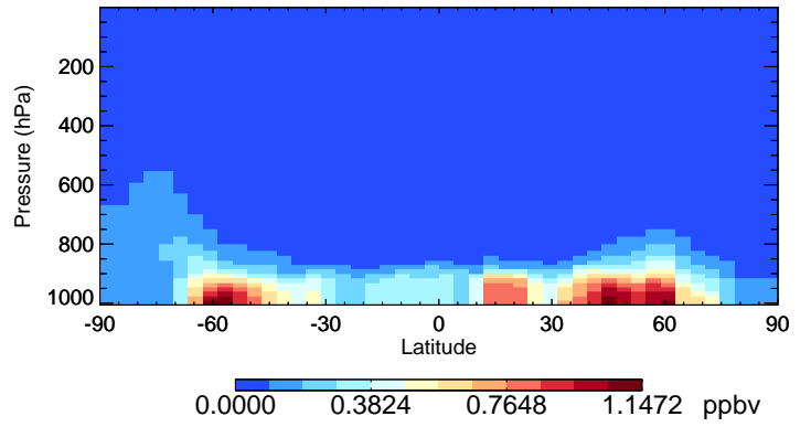
v11-02e-Run1 SALA - Species Curtain @ -180.000 for Oct
