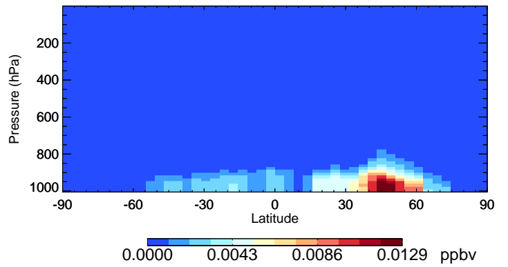
v11-02f-Run1 NITs - Species Curtain @ -180.000 for Oct
