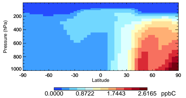
v11-02f-Run1 C2H6 - Species Curtain @ -180.000 for Oct
