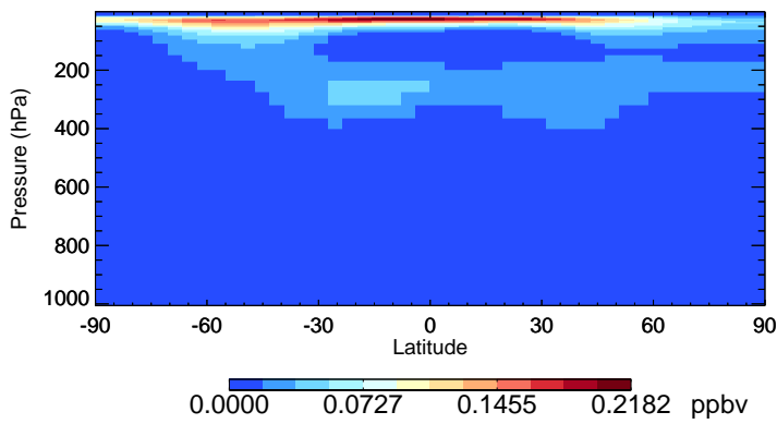
v11-02f-Run1 HNO4 - Species Zonal Mean for Oct
