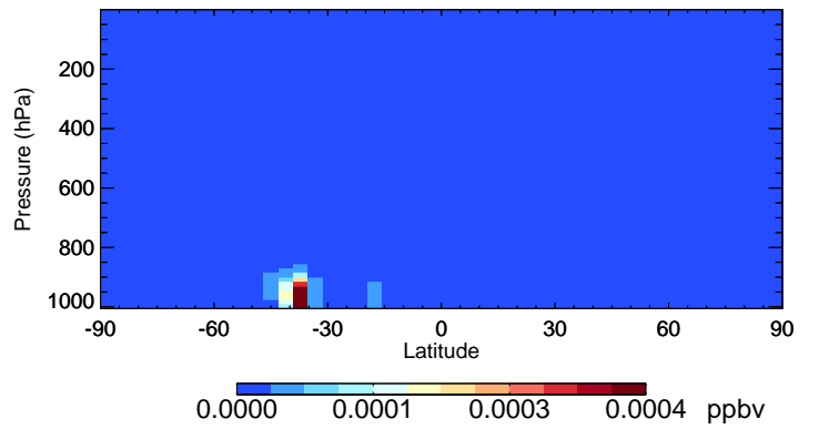
v11-02f-Run1 ISOPNB - Species Curtain @ -180.000 for Oct
