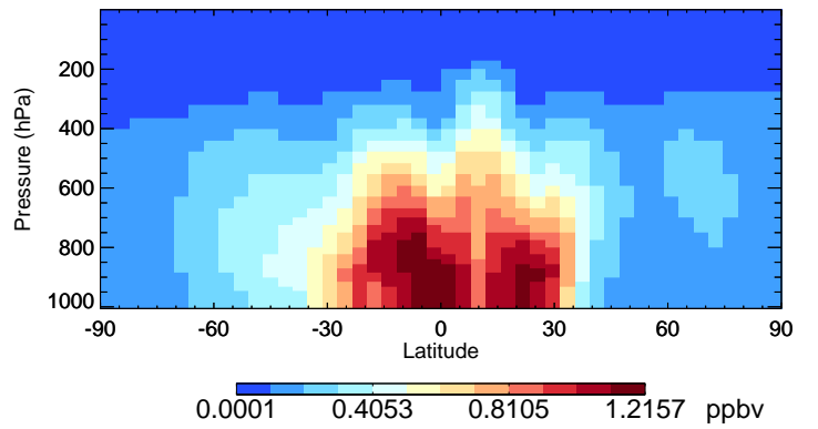
v11-02f-Run1 MP - Species Curtain @ -180.000 for Oct
