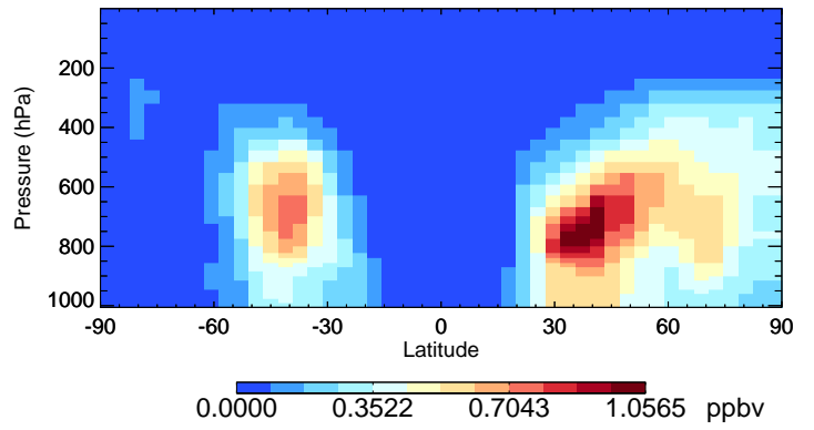
v11-02e-Run0 DST1 - Species Curtain @ -180.000 for Oct
