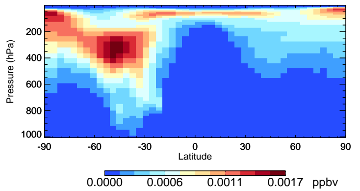
v11-02f-Run1 ISOA1 - Species Curtain @ -180.000 for Oct
