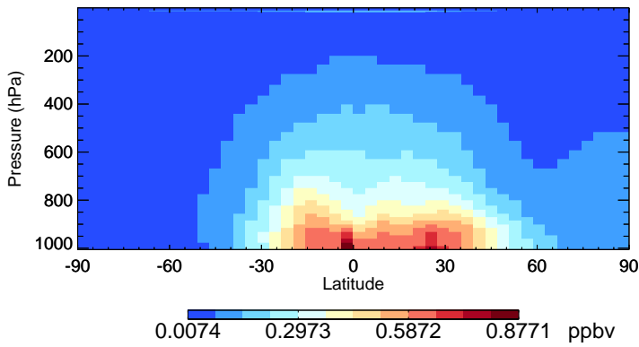
v11-02f-Run1 CH2O - Species Zonal Mean for Oct
