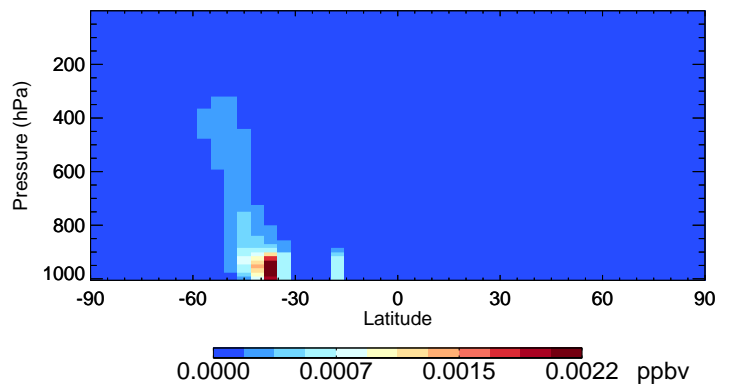
v11-02f-Run1 IEPOXB - Species Curtain @ -180.000 for Oct
