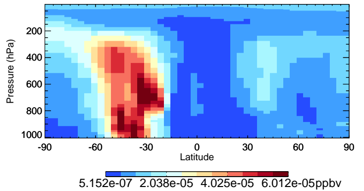
v11-02f-Run1 ISN10A - Species Curtain @ -180.000 for Oct
