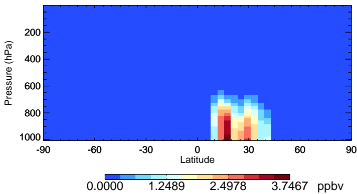
v11-02f-Run1 DST4 - Species Zonal Mean for Oct
