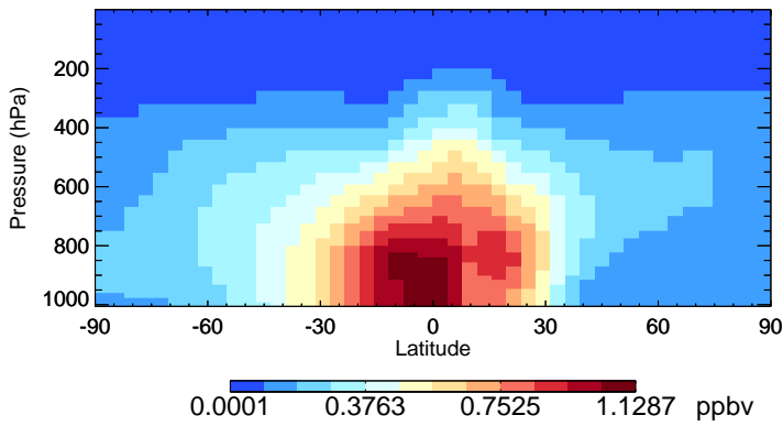
v11-02f-Run1 MP - Species Zonal Mean for Oct
