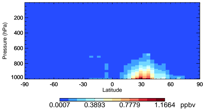
v11-02f-Run1 SO2 - Species Zonal Mean for Oct
