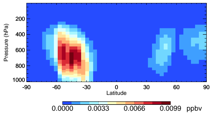
v11-02f-Run1 DST4 - Species Curtain @ -180.000 for Oct
