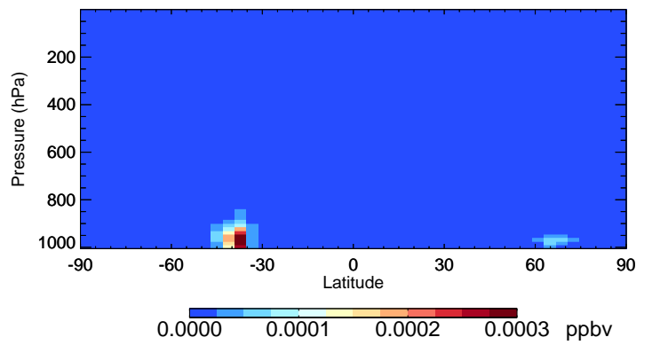
v11-02f-Run1 ISN1 - Species Curtain @ -180.000 for Oct
