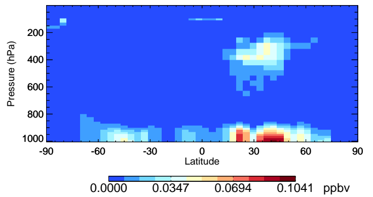
v11-02f-Run1 NIT - Species Curtain @ -180.000 for Oct
