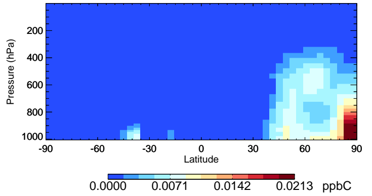
v11-02e-Run1 XYLE - Species Curtain @ -180.000 for Oct
