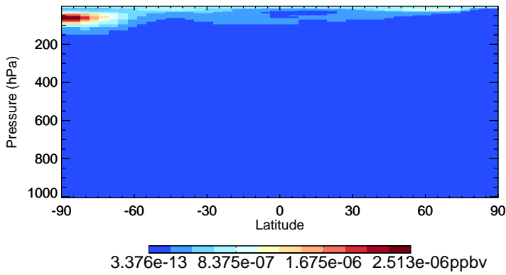
v11-02f-Run1 CIOO - Species Zonal Mean for Oct
