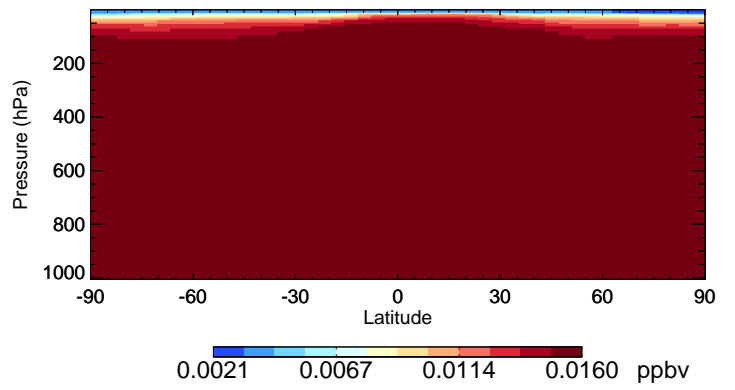
v11-02e-Run1 CFC114 - Species Curtain @ -180.000 for Oct
