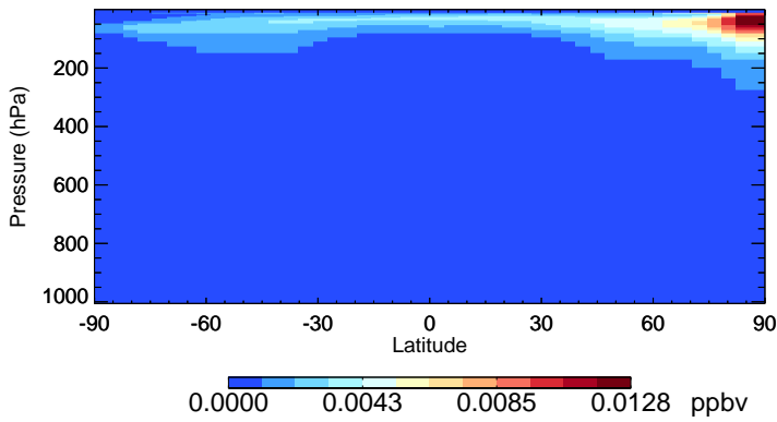
v11-02f-Run1 BrCl - Species Zonal Mean for Oct
