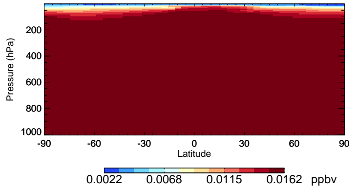
v11-02e-Run0 CFC114 - Species Curtain @ -180.000 for Oct
