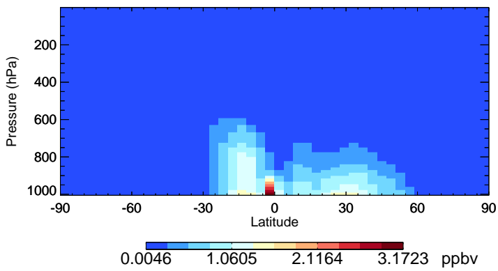
v11-02f-Run1 OCPI - Species Zonal Mean for Oct
