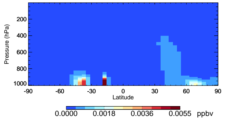
v11-02f-Run1 BCPO - Species Curtain @ -180.000 for Oct
