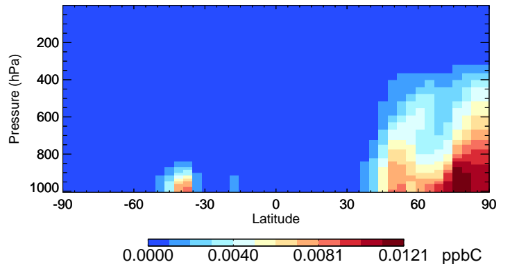
v11-02e-Run0 XYLE - Species Curtain @ -180.000 for Oct
