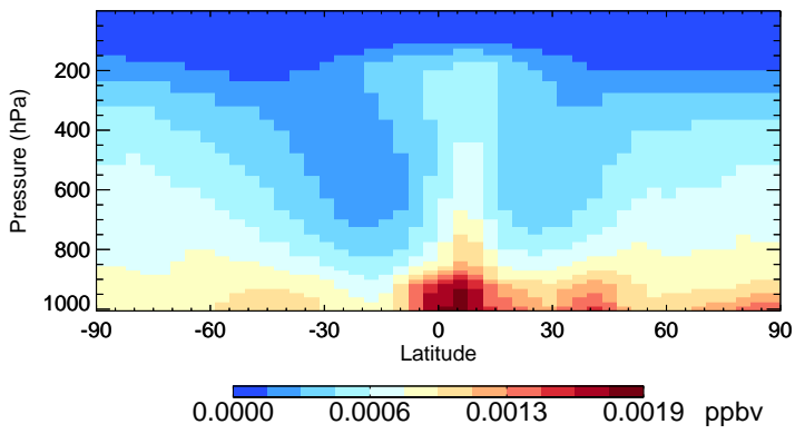
v11-02e-Run1 CHBr3 - Species Zonal Mean for Oct
