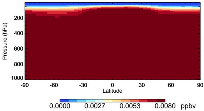
v11-02f-Run1 CH3CCI3 - Species Zonal Mean for Oct
