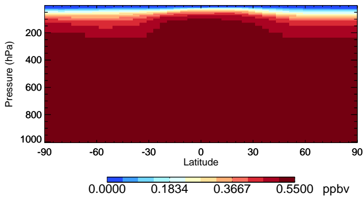
v11-02f-Run1 CH3Cl - Species Zonal Mean for Oct
