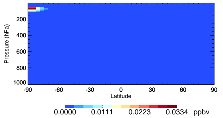
v11-02e-Run0 Cl2O2 - Species Curtain @ -180.000 for Oct
