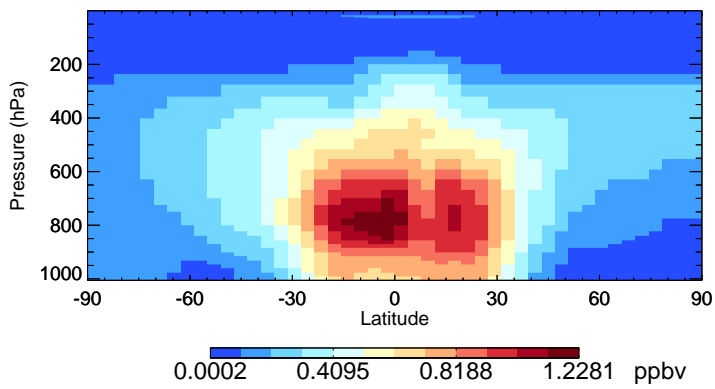
v11-02f-Run1 H2O2 - Species Zonal Mean for Oct
