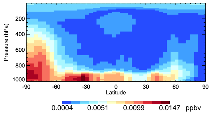
v11-02f-Run1 MSA - Species Curtain @ -180.000 for Oct
