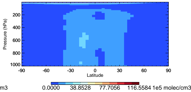
v11-02f-Run1 OH - Species Curtain @ -180.000 for Oct
