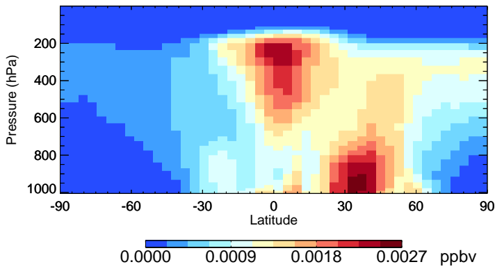
v11-02f-Run1 R4N2 - Species Zonal Mean for Oct
