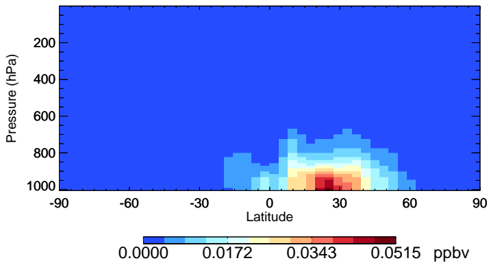
v11-02f-Run1 SOAGX - Species Zonal Mean for Oct
