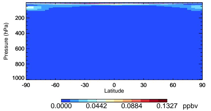
v11-02f-Run1 HOCl - Species Curtain @ -180.000 for Oct
