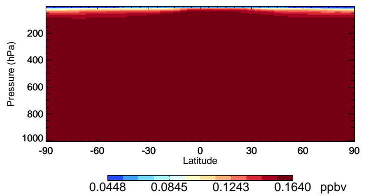
v11-02f-Run1 HCFC22 - Species Curtain @ -180.000 for Oct
