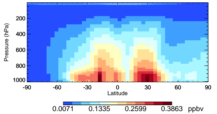
v11-02f-Run1 CH2O - Species Curtain @ -180.000 for Oct
