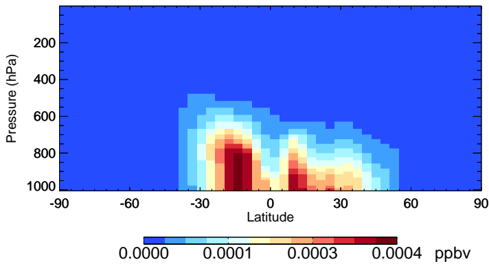
v11-02f-Run1 ISN10A - Species Zonal Mean for Oct
