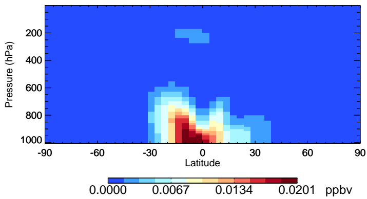
v11-02f-Run1 ISOA1 - Species Zonal Mean for Oct
