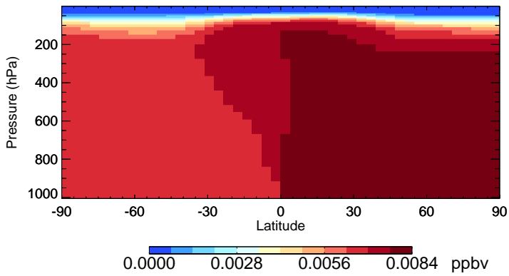
v11-02f-Run1 CH3Br - Species Zonal Mean for Oct
