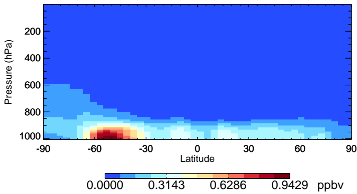
v11-02f-Run1 SALA - Species Zonal Mean for Oct
