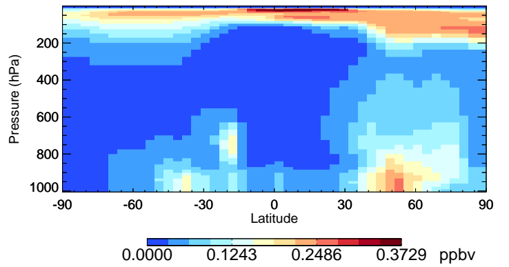
v11-02f-Run1 SO4 - Species Curtain @ -180.000 for Oct
