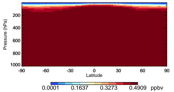
v11-02f-Run1 CFC12 - Species Curtain @ -180.000 for Oct
