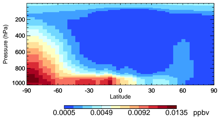
v11-02f-Run1 MSA - Species Zonal Mean for Oct
