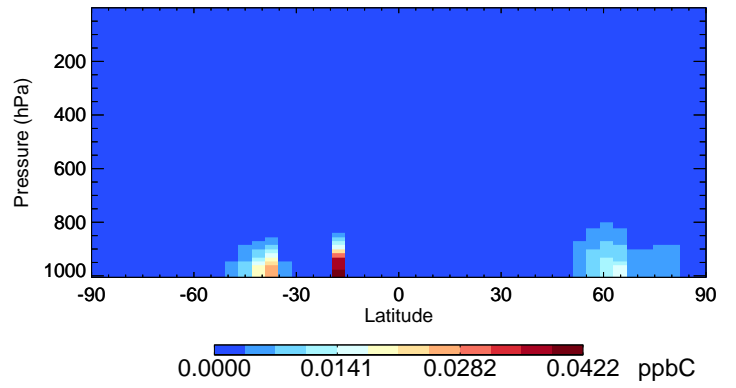
v11-02e-Run0 PRPE - Species Curtain @ -180.000 for Oct
