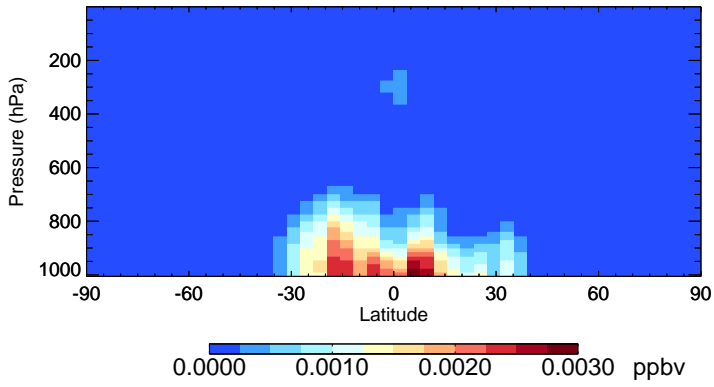
v11-02e-Run1 ISOPNB - Species Zonal Mean for Oct
