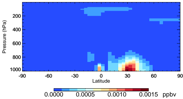
v11-02f-Run1 ASOA2 - Species Zonal Mean for Oct
