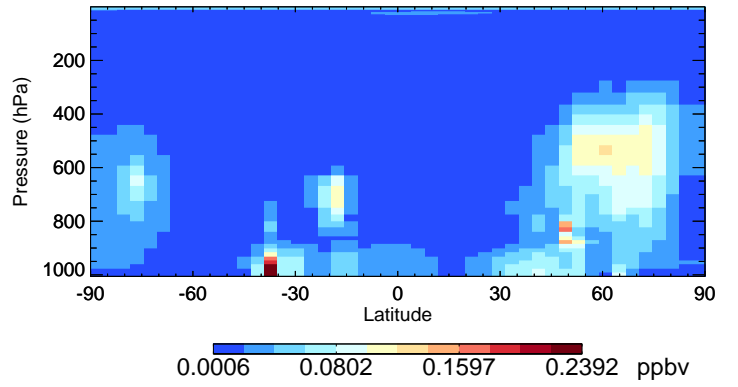
v11-02e-Run1 SO2 - Species Curtain @ -180.000 for Oct
