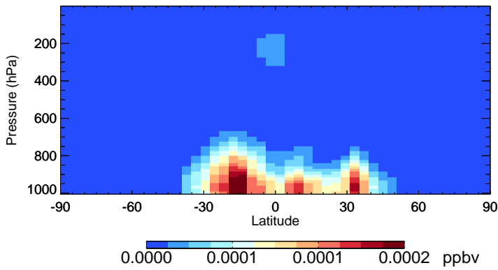
v11-02f-Run1 MACRN - Species Zonal Mean for Oct
