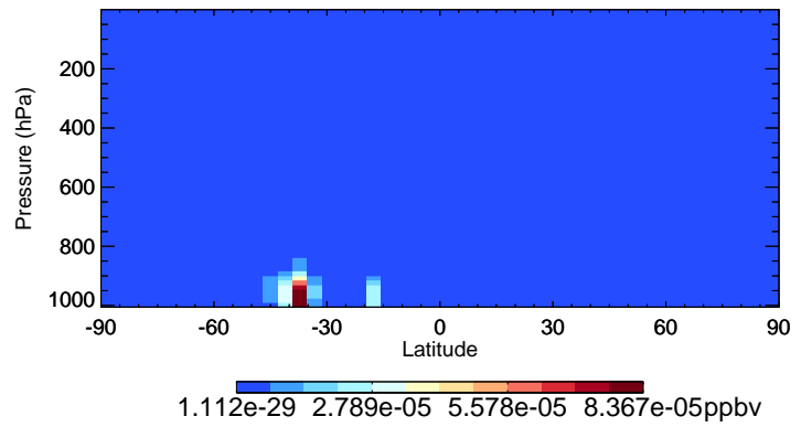
v11-02f-Run1 RIPD - Species Curtain @ -180.000 for Oct
