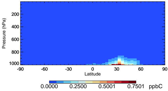
v11-02e-Run1 XYLE - Species Zonal Mean for Oct
