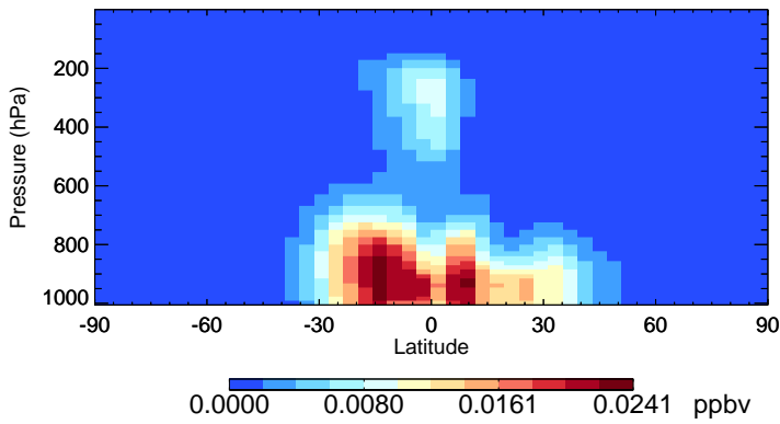
v11-02f-Run1 IMAE - Species Zonal Mean for Oct
