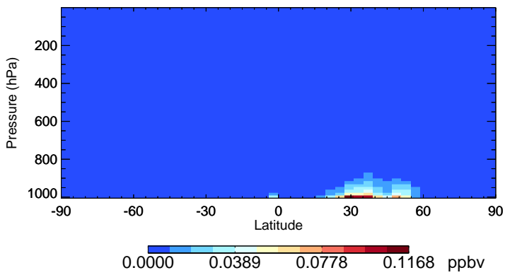
v11-02f-Run1 HNO 2 - Species Zonal Mean for Oct
