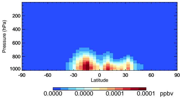
v11-02f-Run1 ETHLN - Species Zonal Mean for Oct
