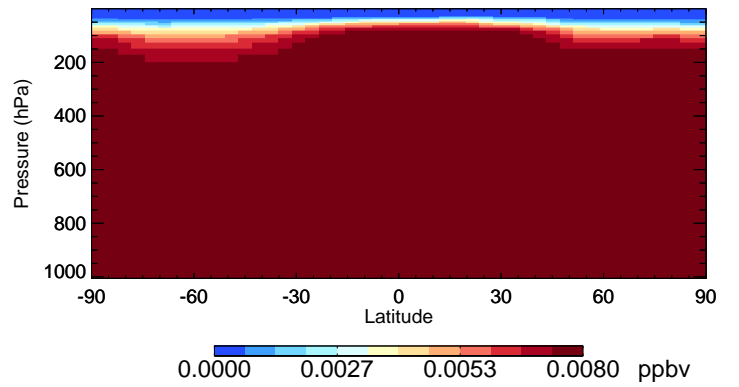
v11-02f-Run1 CH3CCI3 - Species Curtain @ -180.000 for Oct
