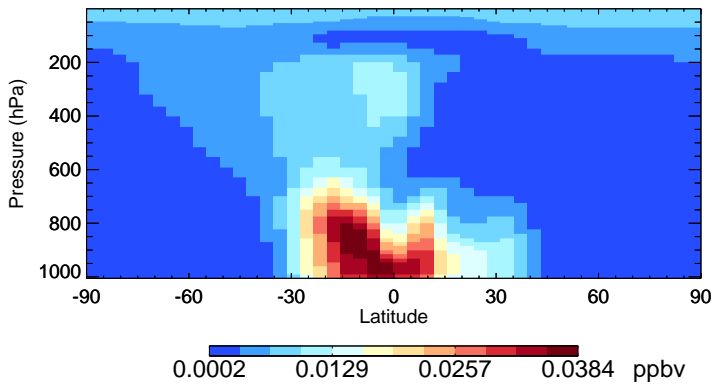
v11-02f-Run1 ISOG3 - Species Zonal Mean for Oct
