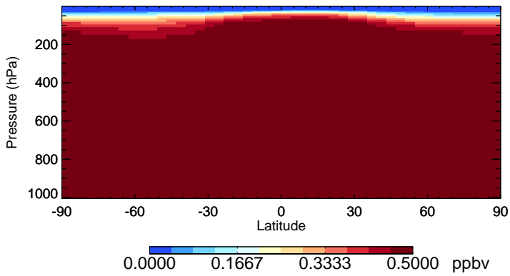
v11-02f-Run1 OCS - Species Zonal Mean for Oct
