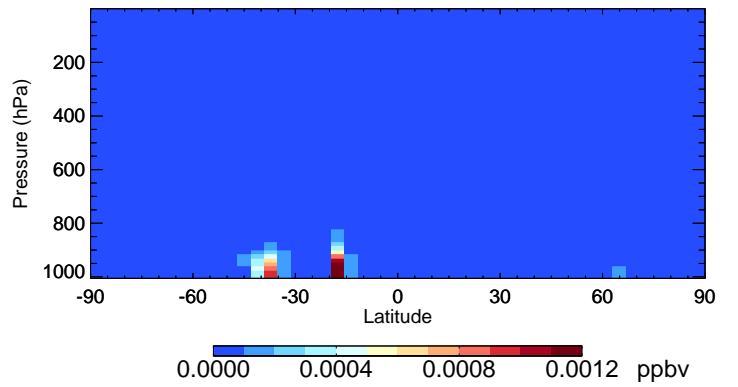
v11-02f-Run1 MONITS - Species Curtain @ -180.000 for Oct
