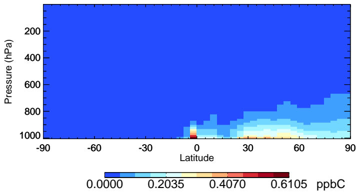
v11-02f-Run1 TOLU - Species Zonal Mean for Oct
