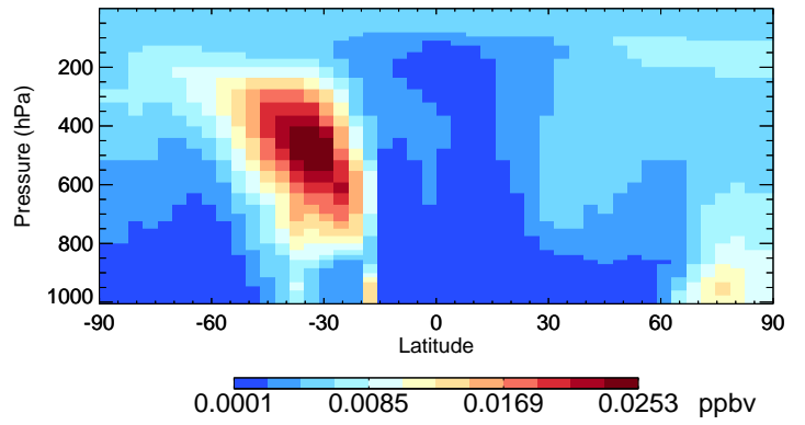
v11-02e-Run0 TSOG3 - Species Curtain @ -180.000 for Oct
