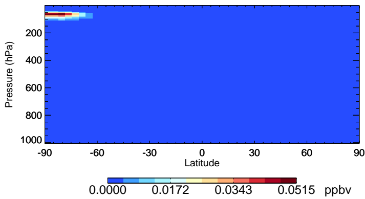
v11-02f-Run1 Cl2O2 - Species Zonal Mean for Oct
