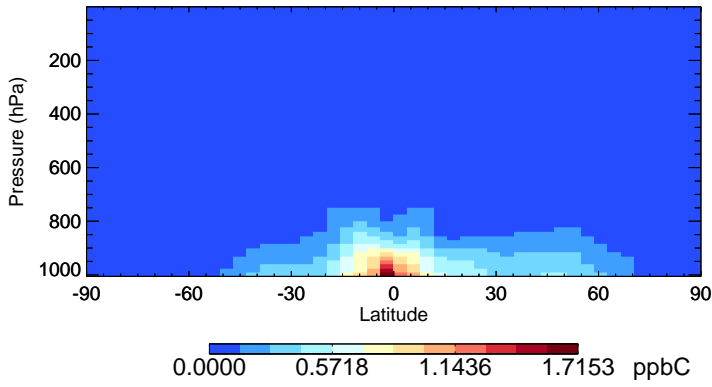
v11-02e-Run1 ALD2 - Species Zonal Mean for Oct
