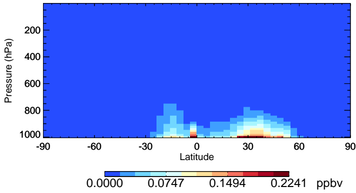
v11-02e-Run1 BCPO - Species Zonal Mean for Oct
