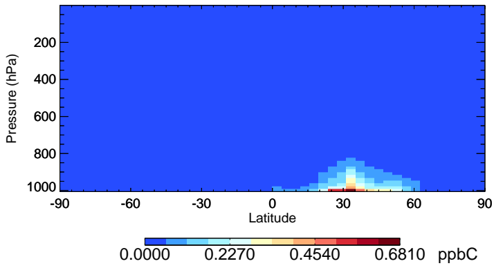
v11-02e-Run0 XYLE - Species Zonal Mean for Oct
