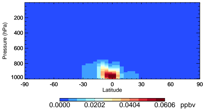
v11-02f-Run1 RIPA - Species Zonal Mean for Oct
