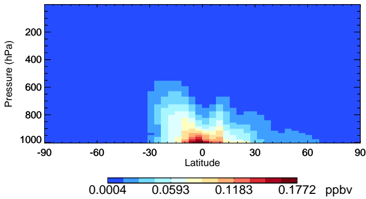
v11-02f-Run1 TSOG3 - Species Zonal Mean for Oct
