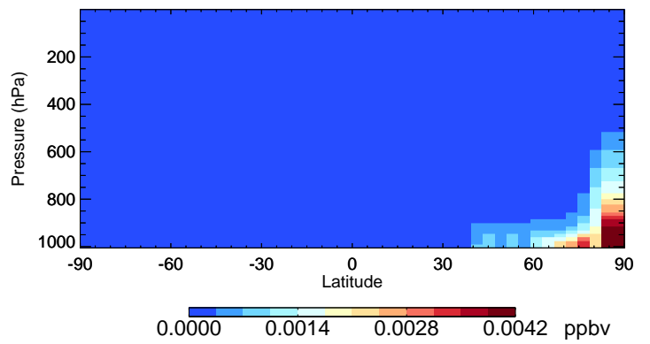
v11-02f-Run1 ClNO 2 - Species Curtain @ -180.000 for Oct
