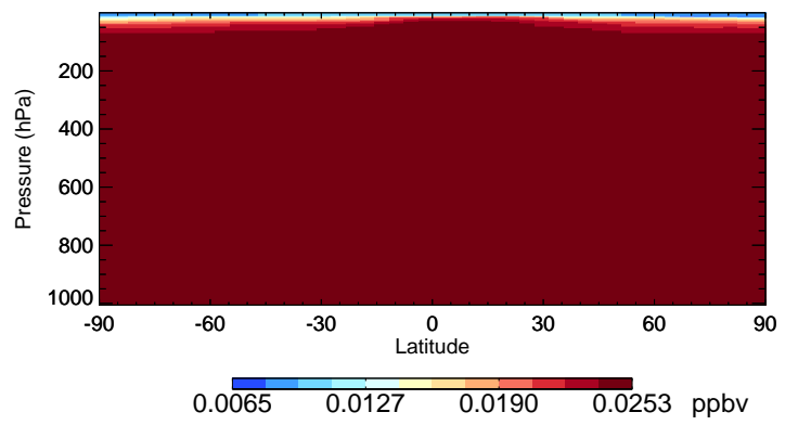
v11-02e-Run1 HCFC142b - Species Curtain @ -180.000 for Oct
