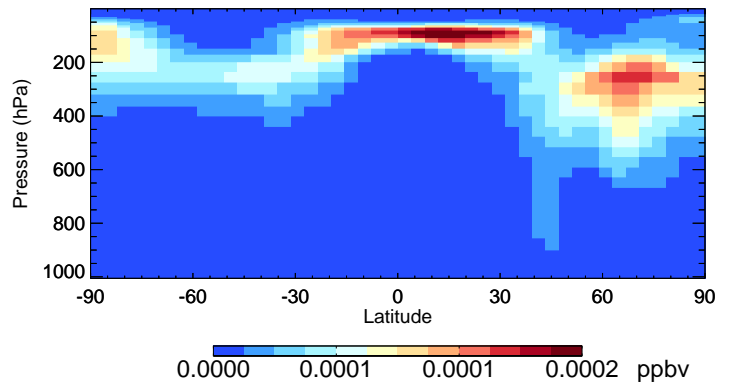
v11-02f-Run1 ASOA2 - Species Curtain @ -180.000 for Oct
