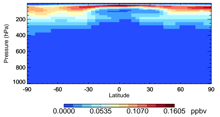
v11-02f-Run1 MPN - Species Curtain @ -180.000 for Oct
