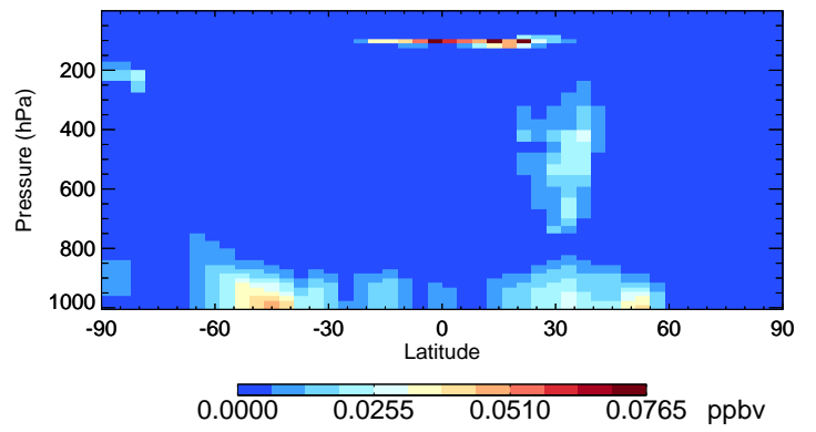
v11-02e-Run0 NIT - Species Curtain @ -180.000 for Oct
