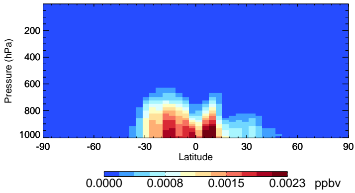
v11-02e-Run0 ISOPNB - Species Zonal Mean for Oct
