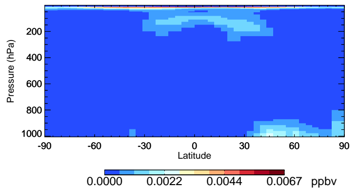
v11-02f-Run1 HNO 2 - Species Curtain @ -180.000 for Oct
