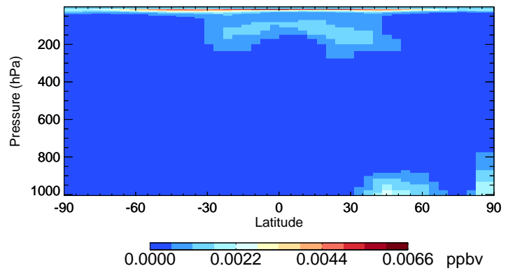
v11-02e-Run1 HNO 2 - Species Curtain @ -180.000 for Oct
