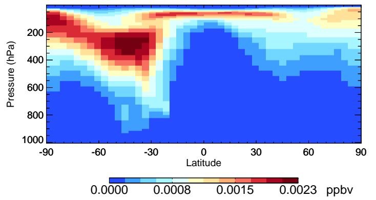
v11-02e-Run1 ISOA1 - Species Curtain @ -180.000 for Oct
