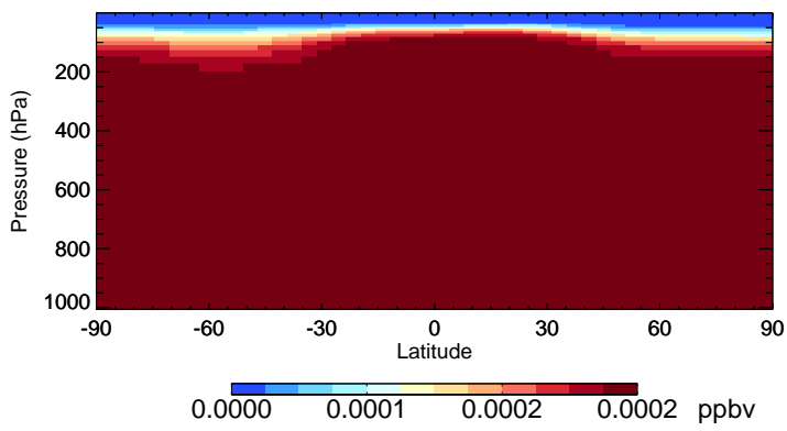
v11-02e-Run1 H2402 - Species Zonal Mean for Oct
