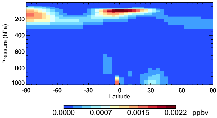
v11-02f-Run1 ASOA3 - Species Zonal Mean for Oct
