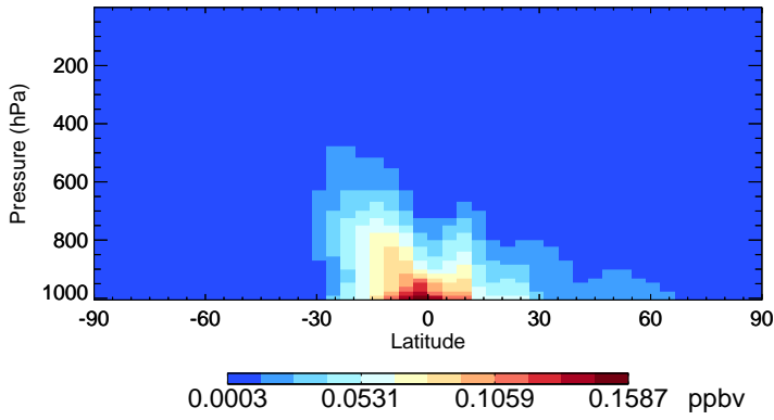
v11-02e-Run1 TSOG3 - Species Zonal Mean for Oct
