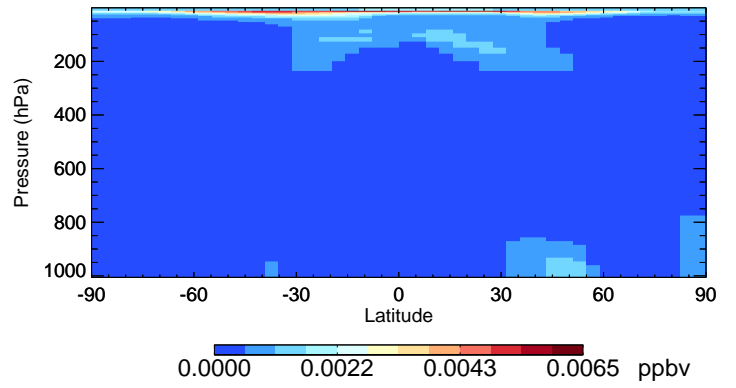
v11-02e-Run0 HNO 2 - Species Curtain @ -180.000 for Oct
