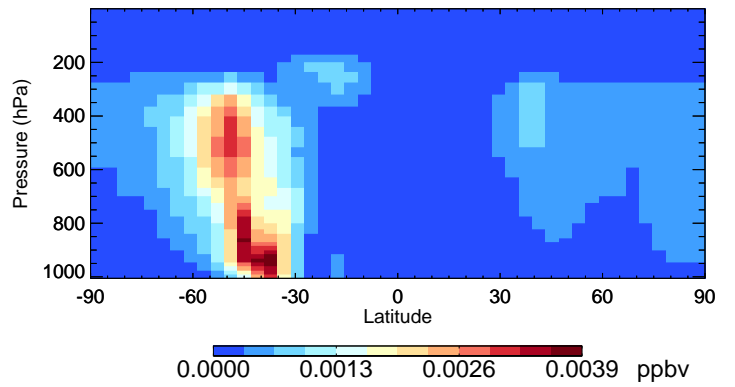
v11-02f-Run1 IMAE - Species Curtain @ -180.000 for Oct
