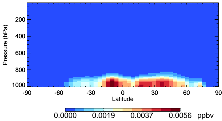
v11-02f-Run1 NITs - Species Zonal Mean for Oct
