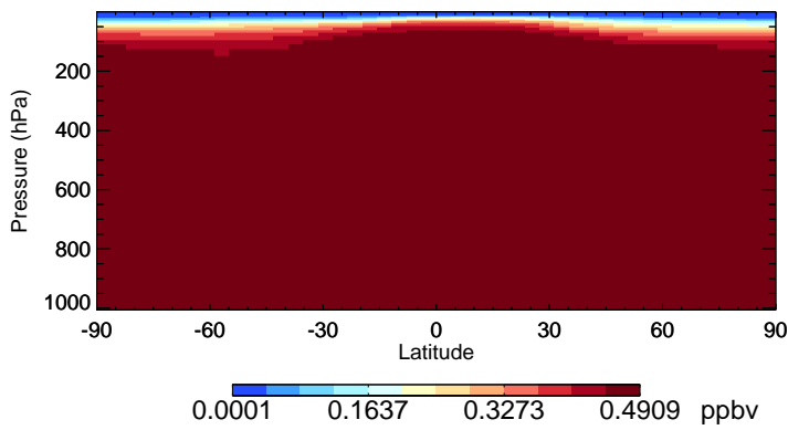
v11-02f-Run1 CFC12 - Species Zonal Mean for Oct
