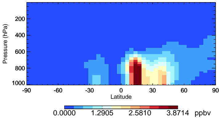
v11-02e-Run0 DST1 - Species Zonal Mean for Oct
