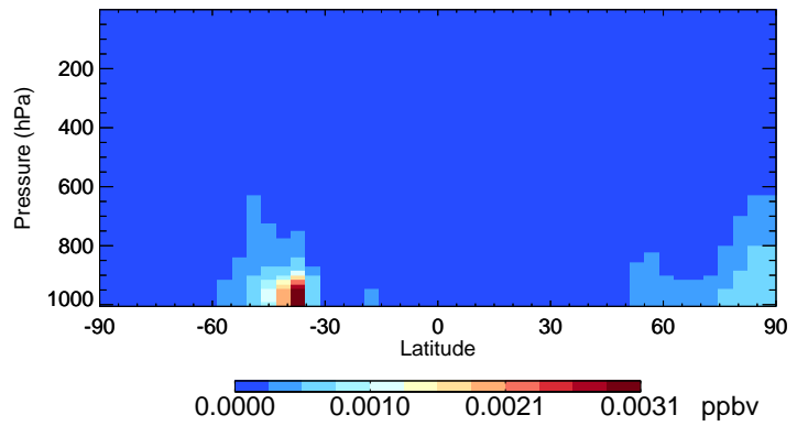
v11-02f-Run1 IPMN - Species Curtain @ -180.000 for Oct
