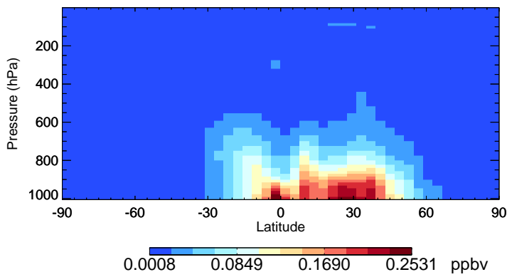
v11-02f-Run1 SOAS - Species Zonal Mean for Oct
