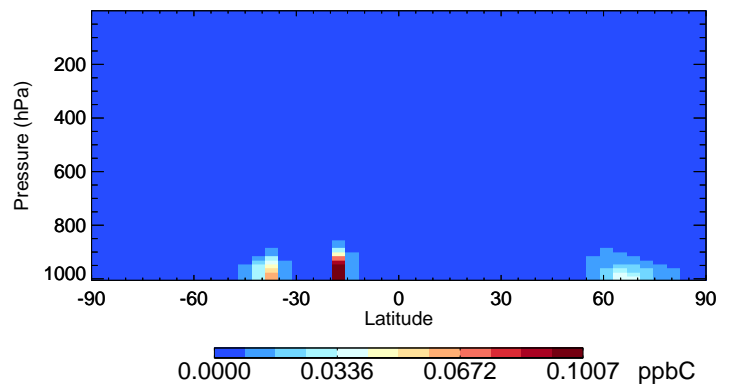
v11-02f-Run1 PRPE - Species Curtain @ -180.000 for Oct
