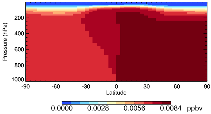
v11-02e-Run1 CH3Br - Species Zonal Mean for Oct
