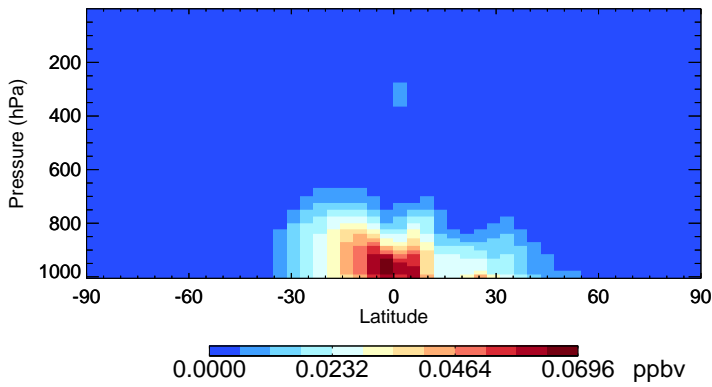
v11-02f-Run1 GLYC - Species Zonal Mean for Oct
