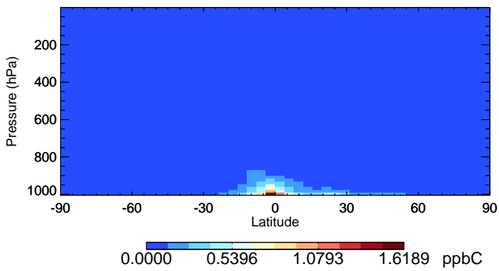
v11-02f-Run1 PRPE - Species Zonal Mean for Oct
