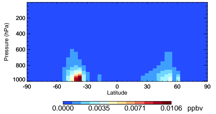
v11-02e-Run0 BCPO - Species Curtain @ -180.000 for Oct
