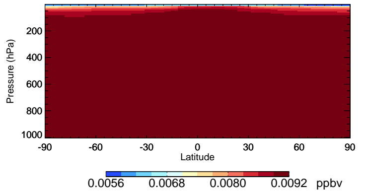
v11-02f-Run1 CFC115 - Species Curtain @ -180.000 for Oct
