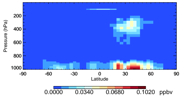
v11-02e-Run1 NIT - Species Curtain @ -180.000 for Oct
