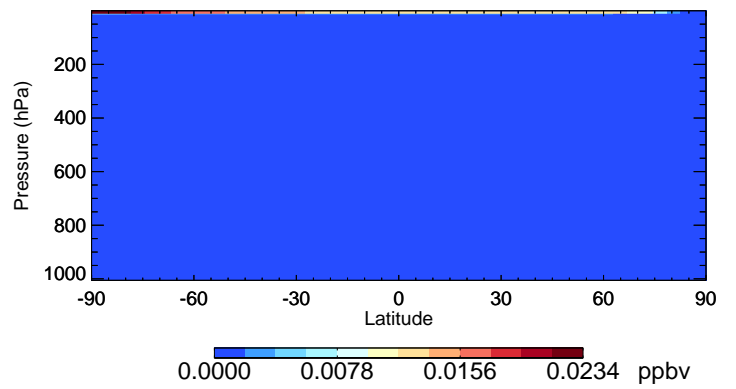
v11-02f-Run1 Br - Species Curtain @ -180.000 for Oct
