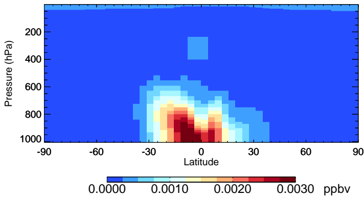
v11-02f-Run1 LVOCOA - Species Zonal Mean for Oct
