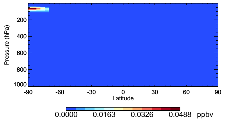
v11-02f-Run1 Cl2O2 - Species Curtain @ -180.000 for Oct
