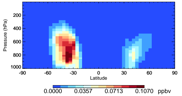
v11-02e-Run0 DST4 - Species Curtain @ -180.000 for Oct
