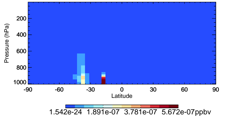
v11-02e-Run1 LVOC - Species Curtain @ -180.000 for Oct
