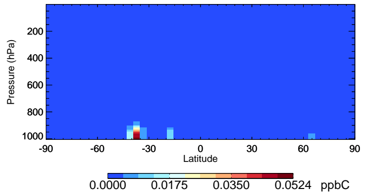
v11-02f-Run1 ISOP - Species Curtain @ -180.000 for Oct
