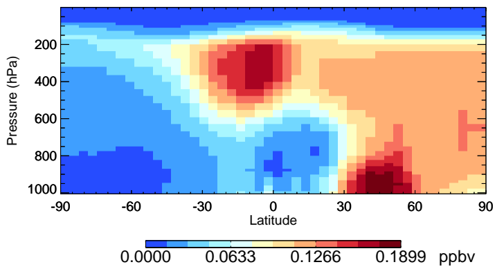
v11-02f-Run1 PAN - Species Zonal Mean for Oct
