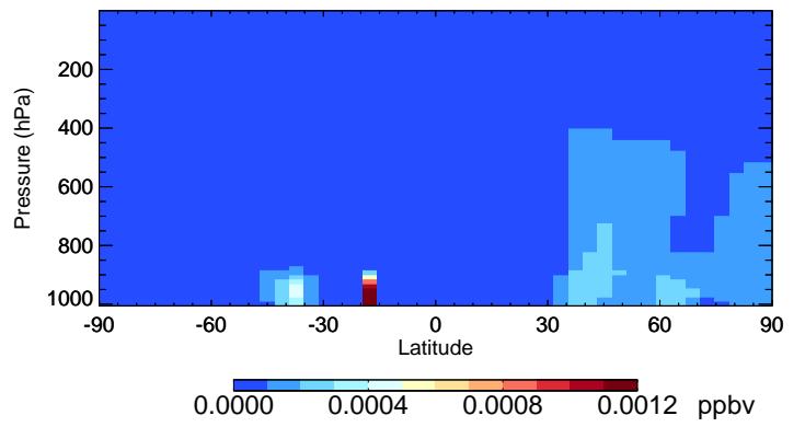
v11-02e-Run1 GLYX - Species Curtain @ -180.000 for Oct
