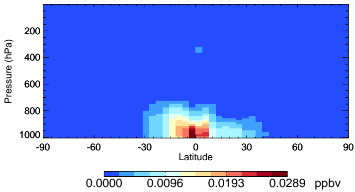
v11-02f-Run1 IPMN - Species Zonal Mean for Oct
