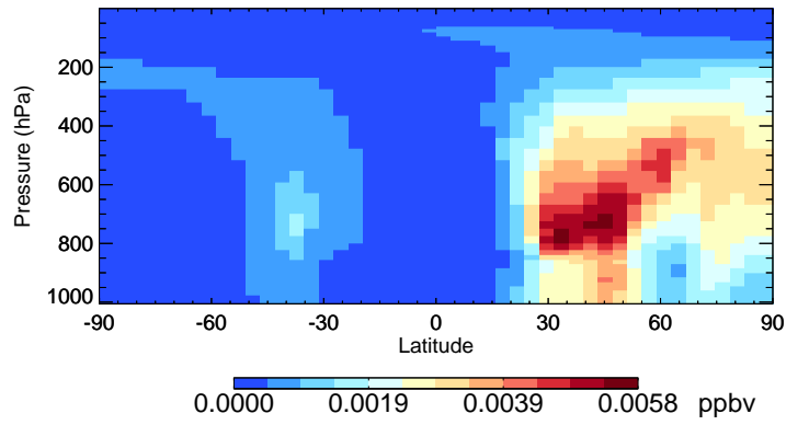
v11-02e-Run0 SOAGX - Species Curtain @ -180.000 for Oct
