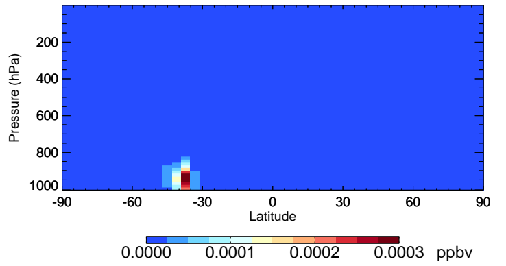
v11-02e-Run0 ISOPNB - Species Curtain @ -180.000 for Oct
