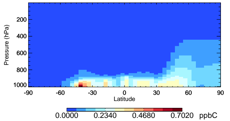
v11-02f-Run1 ALD2 - Species Curtain @ -180.000 for Oct
