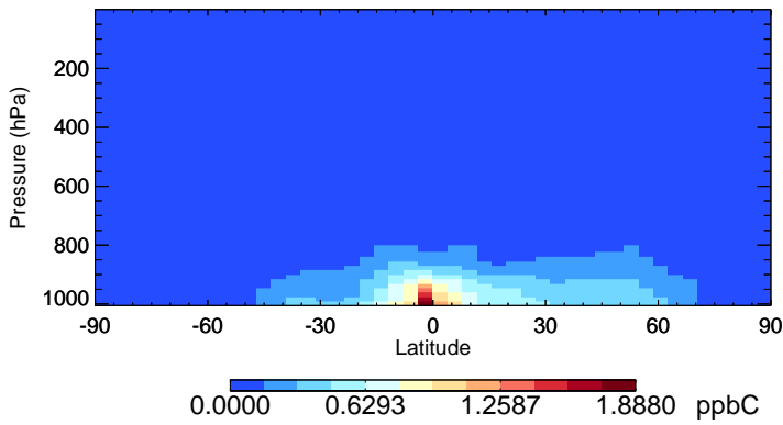
v11-02f-Run1 ALD2 - Species Zonal Mean for Oct
