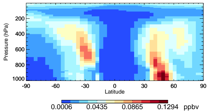
v11-02f-Run1 OCPI - Species Curtain @ -180.000 for Oct
