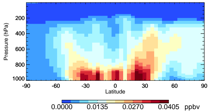
v11-02f-Run1 MAP - Species Curtain @ -180.000 for Oct
