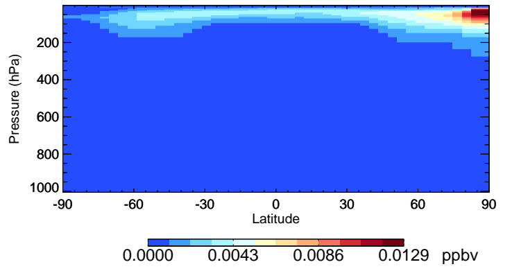
v11-02e-Run0 BrCl - Species Curtain @ -180.000 for Oct
