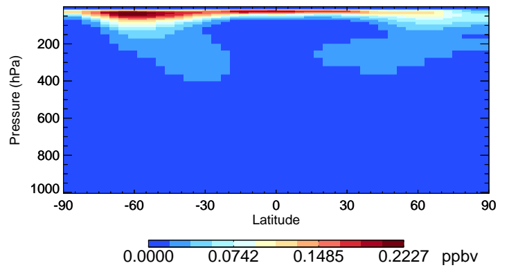
v11-02e-Run0 HNO4 - Species Curtain @ -180.000 for Oct
