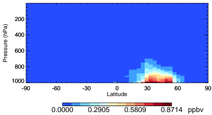
v11-02f-Run1 NIT - Species Zonal Mean for Oct
