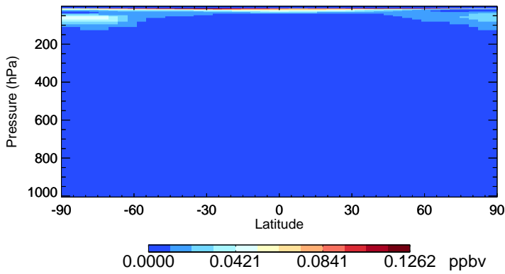
v11-02f-Run1 HOCl - Species Zonal Mean for Oct
