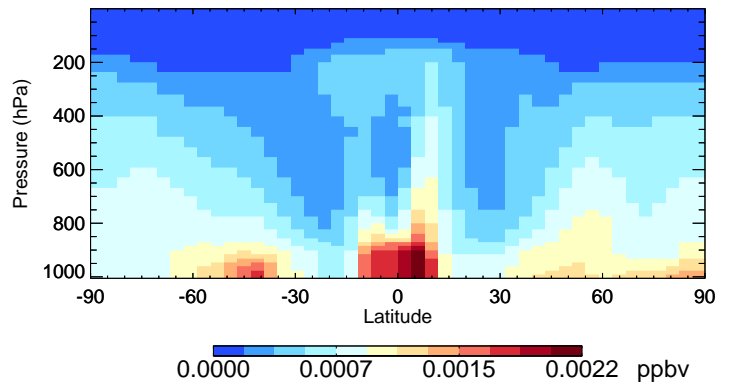
v11-02f-Run1 CHBr3 - Species Curtain @ -180.000 for Oct
