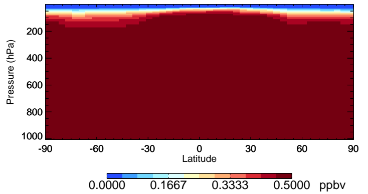
v11-02f-Run1 OCS - Species Curtain @ -180.000 for Oct
