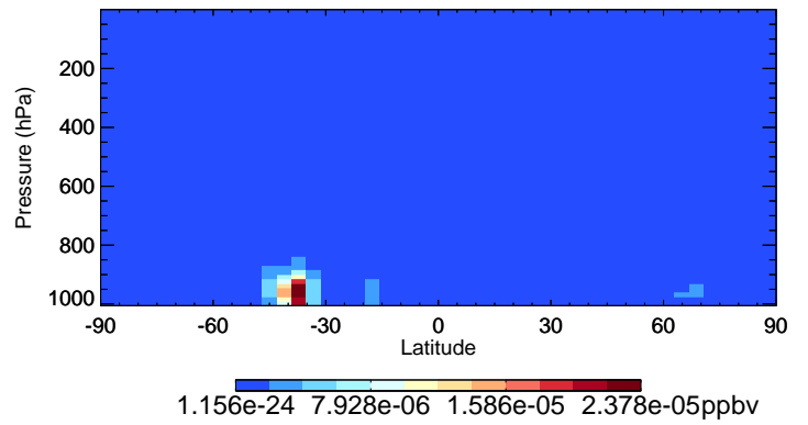
v11-02f-Run1 ETHLN - Species Curtain @ -180.000 for Oct
