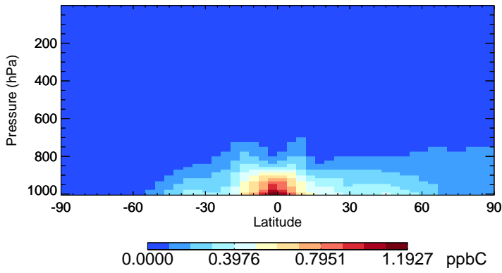
v11-02e-Run0 ALD2 - Species Zonal Mean for Oct
