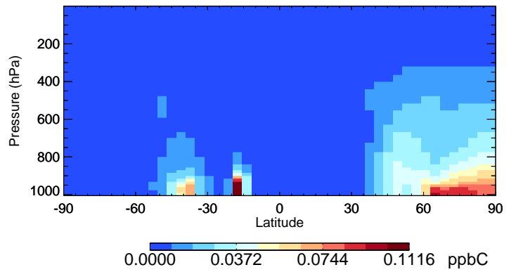
v11-02f-Run1 EOH - Species Curtain @ -180.000 for Oct
