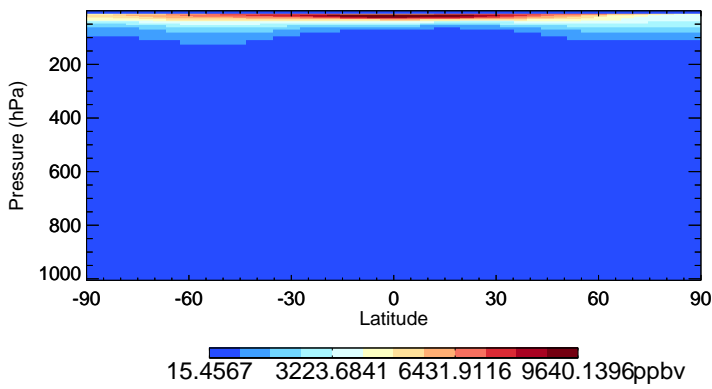
v11-02f-Run1 O3 - Species Zonal Mean for Oct
