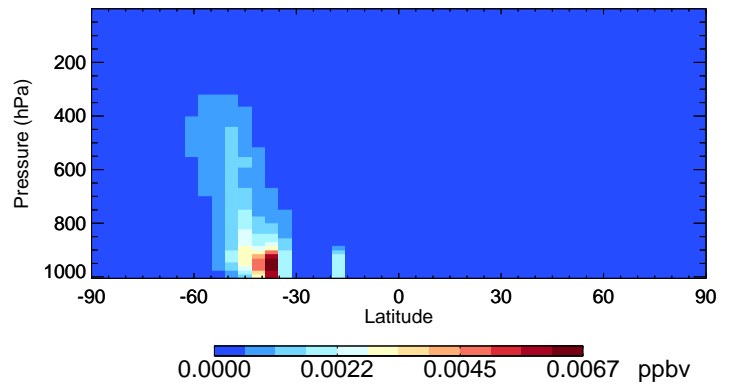
v11-02f-Run1 GLYC - Species Curtain @ -180.000 for Oct
