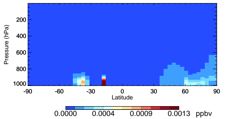
v11-02f-Run1 GLYX - Species Curtain @ -180.000 for Oct
