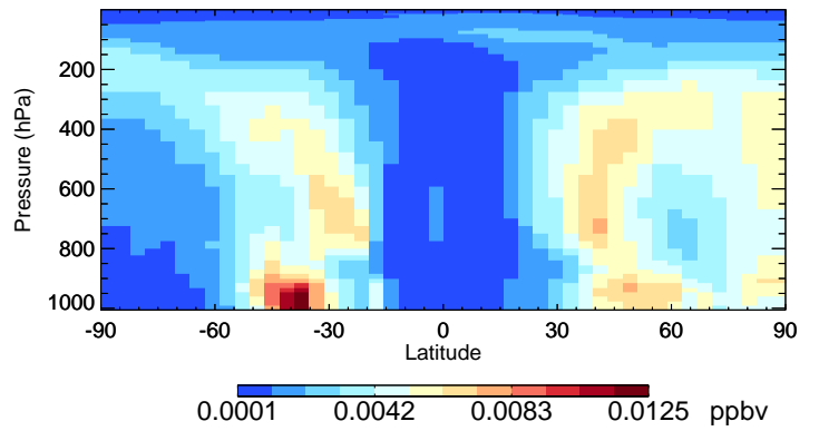
v11-02f-Run1 INDIOL - Species Curtain @ -180.000 for Oct
