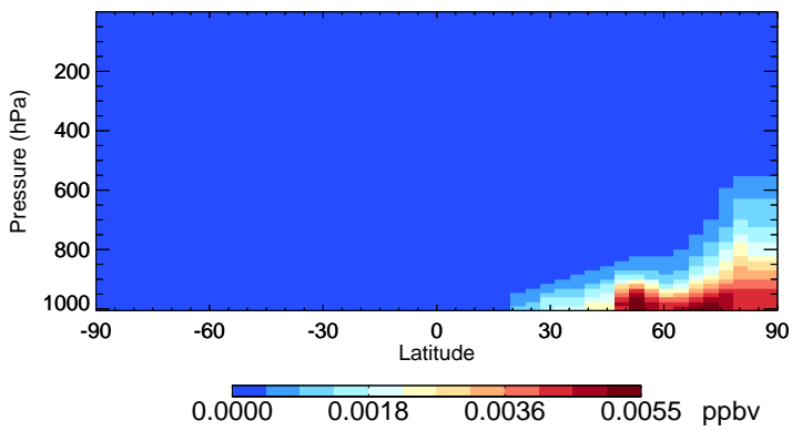
v11-02f-Run1 ClNO 2 - Species Zonal Mean for Oct
