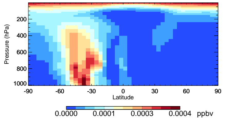
v11-02f-Run1 LVOCOA - Species Curtain @ -180.000 for Oct
