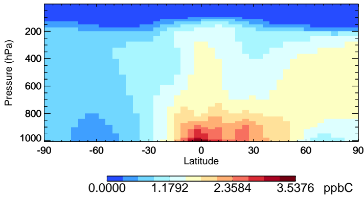
v11-02e-Run0 ACET - Species Zonal Mean for Oct
