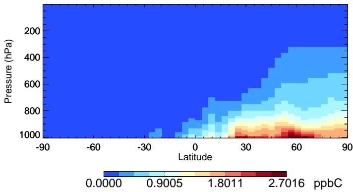
v11-02f-Run1 ALK4 - Species Zonal Mean for Oct
