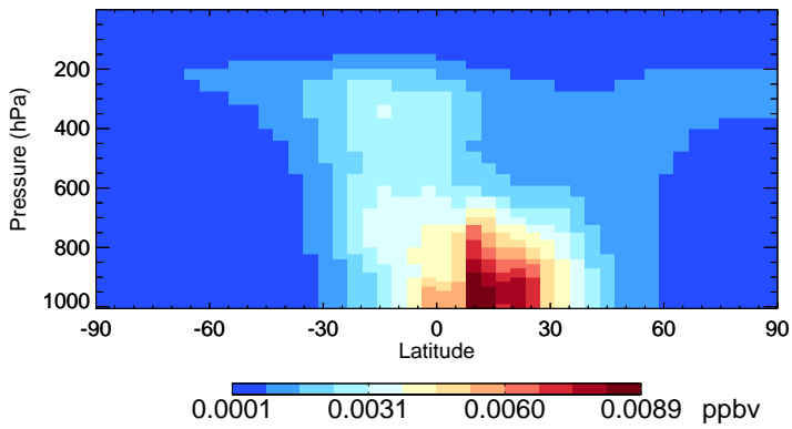
v11-02f-Run1 ASOAN - Species Zonal Mean for Oct
