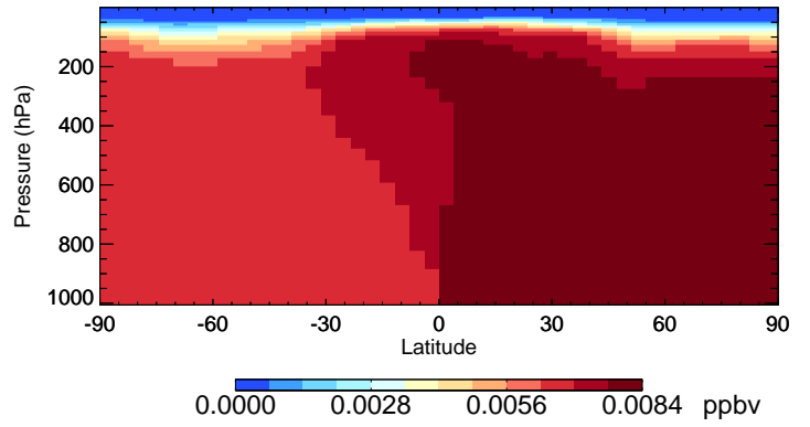
v11-02e-Run1 CH3Br - Species Curtain @ -180.000 for Oct
