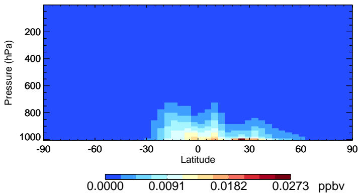
v11-02e-Run1 GLYX - Species Zonal Mean for Oct
