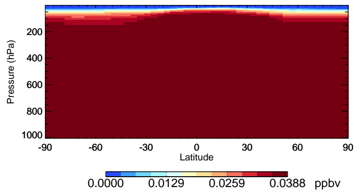
v11-02f-Run1 HCFC141b - Species Curtain @ -180.000 for Oct
