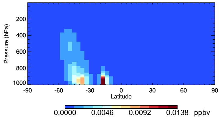
v11-02f-Run1 HAC - Species Curtain @ -180.000 for Oct
