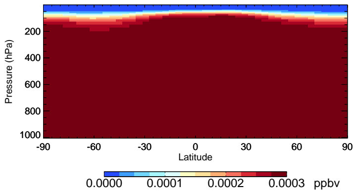
v11-02e-Run0 H2402 - Species Zonal Mean for Oct
