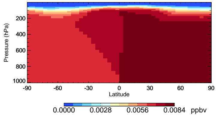
v11-02e-Run0 CH3Br - Species Curtain @ -180.000 for Oct
