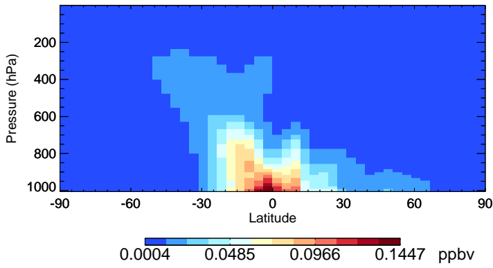
v11-02e-Run0 TSOG3 - Species Zonal Mean for Oct
