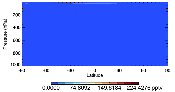
v11-02f-Run1 HO2 - Species Curtain @ -180.000 for Oct
