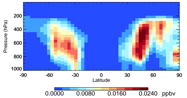
v11-02f-Run1 DST2 - Species Curtain @ -180.000 for Oct
