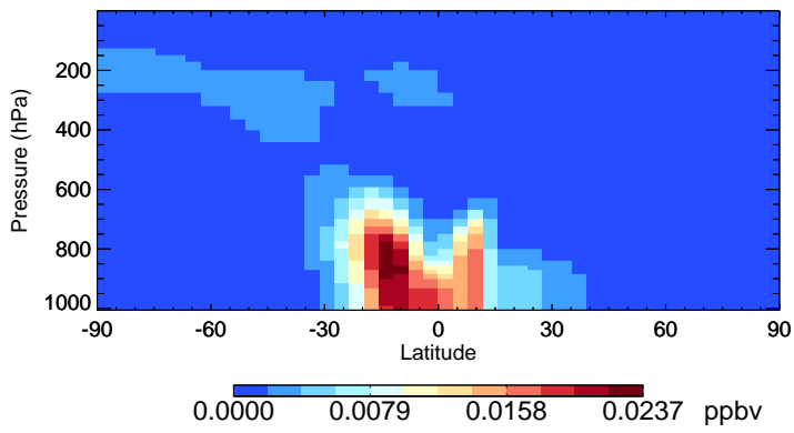
v11-02e-Run0 ISOA1 - Species Zonal Mean for Oct
