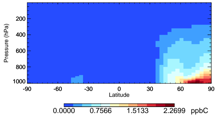
v11-02f-Run1 ALK4 - Species Curtain @ -180.000 for Oct
