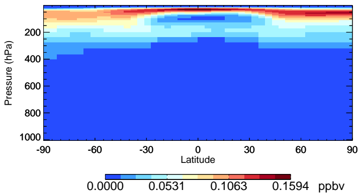
v11-02f-Run1 MPN - Species Zonal Mean for Oct
