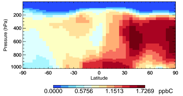
v11-02e-Run1 ACET - Species Curtain @ -180.000 for Oct
