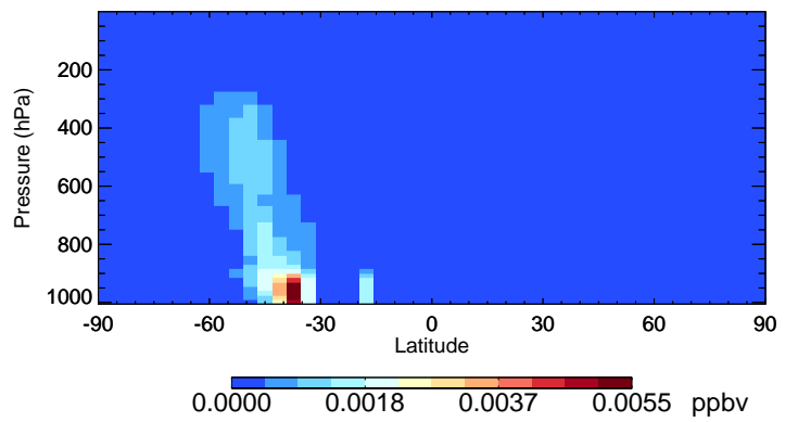
v11-02f-Run1 IEPOXA - Species Curtain @ -180.000 for Oct
