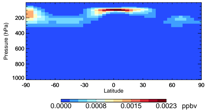
v11-02f-Run1 ASOA3 - Species Curtain @ -180.000 for Oct
