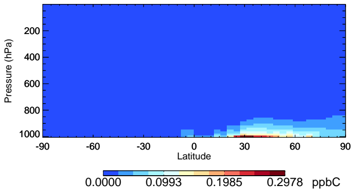
v11-02f-Run1 XYLE - Species Zonal Mean for Oct
