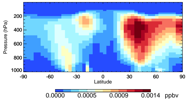
v11-02f-Run1 R4N2 - Species Curtain @ -180.000 for Oct
