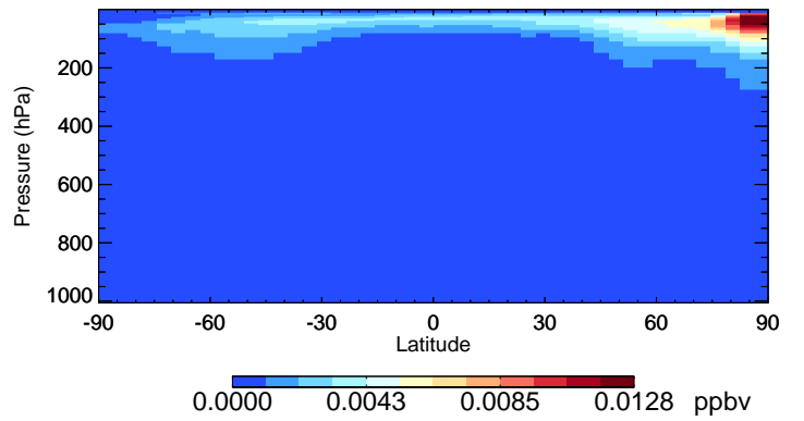
v11-02f-Run1 BrCl - Species Curtain @ -180.000 for Oct
