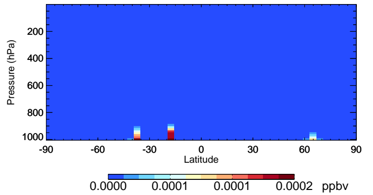
v11-02f-Run1 LIMO - Species Curtain @ -180.000 for Oct
