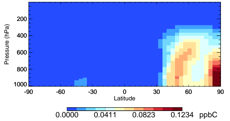
v11-02e-Run1 TOLU - Species Curtain @ -180.000 for Oct
