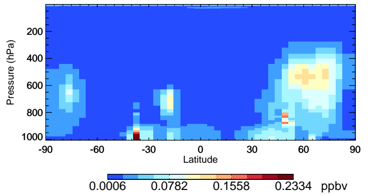
v11-02f-Run1 SO2 - Species Curtain @ -180.000 for Oct
