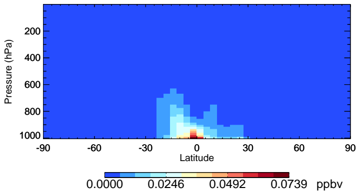
v11-02f-Run1 TSOA2 - Species Zonal Mean for Oct
