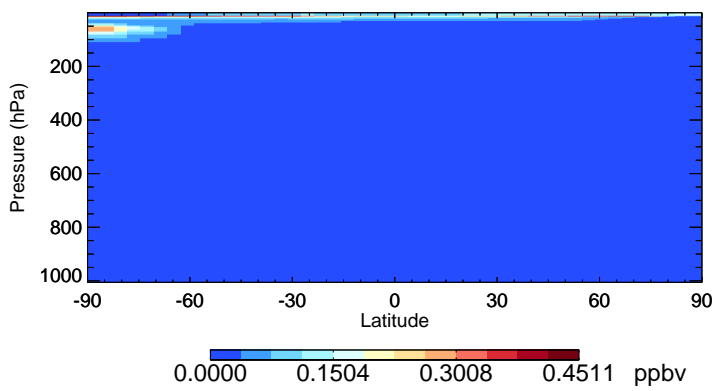
v11-02f-Run1 ClO - Species Zonal Mean for Oct
