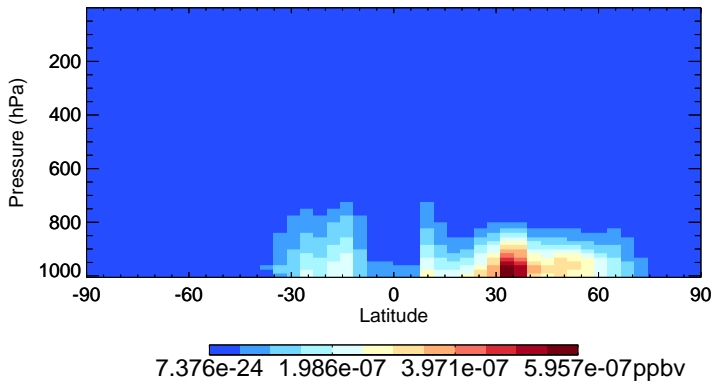
v11-02e-Run0 NPMN - Species Zonal Mean for Oct
