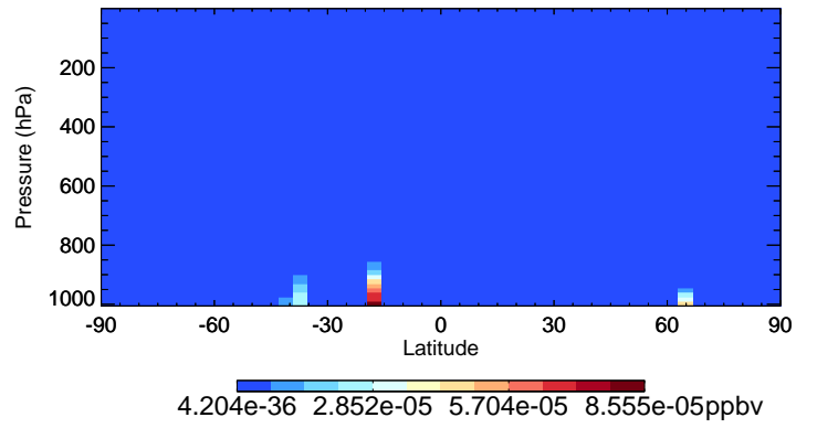
v11-02e-Run0 LIMO - Species Curtain @ -180.000 for Oct
