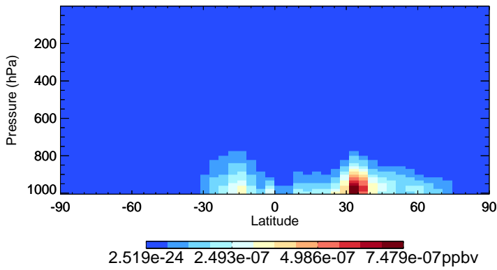
v11-02f-Run1 NPMN - Species Zonal Mean for Oct
