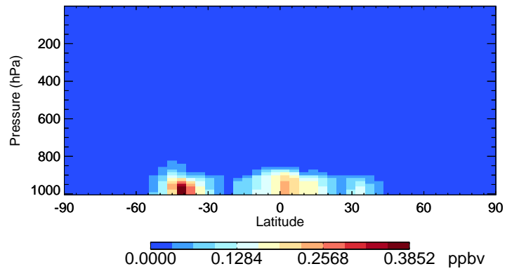
v11-02f-Run1 NH3 - Species Curtain @ -180.000 for Oct
