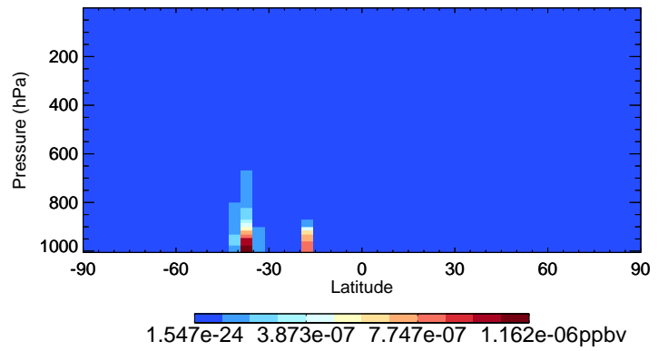
v11-02f-Run1 LVOC - Species Curtain @ -180.000 for Oct
