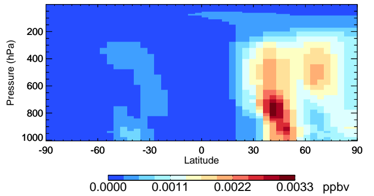
v11-02f-Run1 SOAGX - Species Curtain @ -180.000 for Oct
