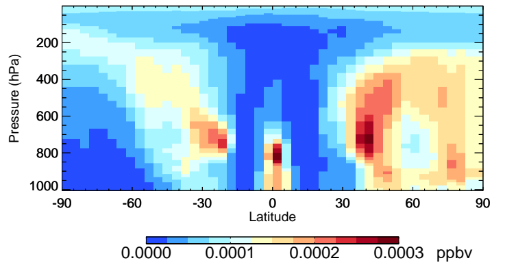
v11-02f-Run1 SOAME - Species Curtain @ -180.000 for Oct
