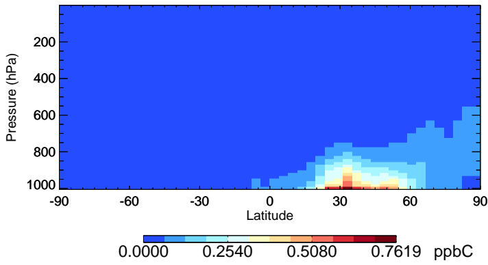
v11-02e-Run0 TOLU - Species Zonal Mean for Oct
