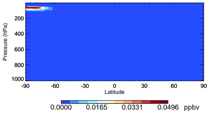
v11-02e-Run1 Cl2O2 - Species Zonal Mean for Oct
