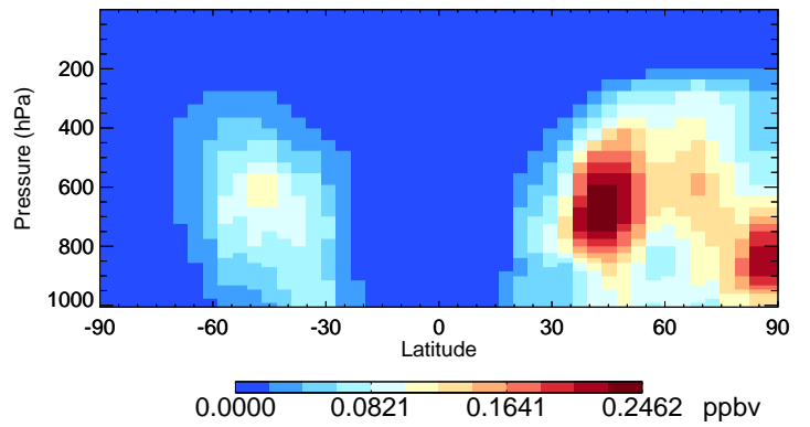
v11-02f-Run1 DST1 - Species Curtain @ -180.000 for Oct
