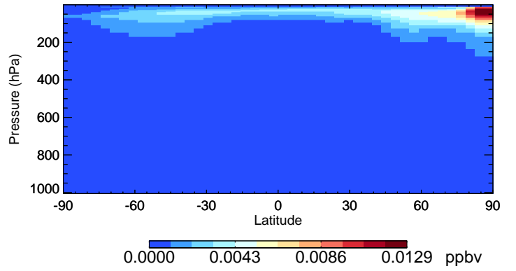
v11-02e-Run1 BrCl - Species Curtain @ -180.000 for Oct
