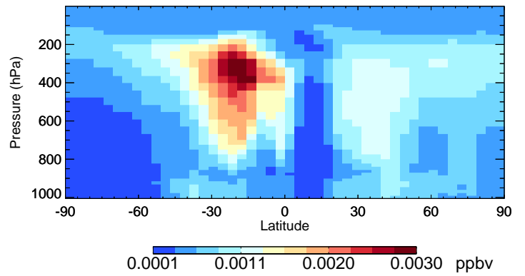
v11-02f-Run1 ASOAN - Species Curtain @ -180.000 for Oct
