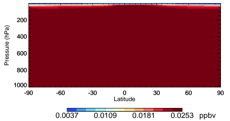
v11-02f-Run1 HCFC142b - Species Curtain @ -180.000 for Oct
