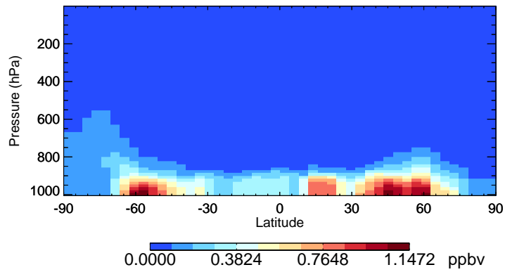
v11-02f-Run1 SALA - Species Curtain @ -180.000 for Oct
