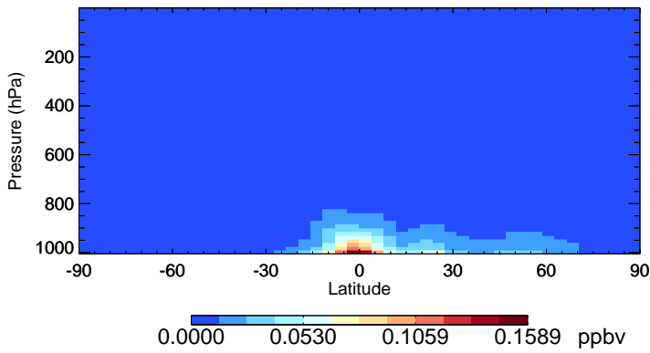
v11-02f-Run1 RCHO - Species Zonal Mean for Oct
