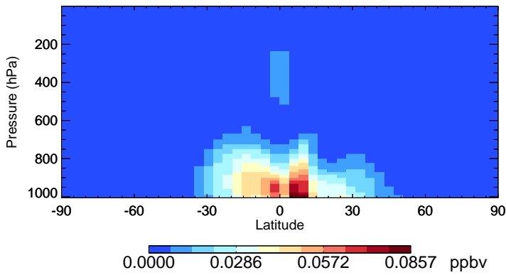
v11-02f-Run1 HAC - Species Zonal Mean for Oct
