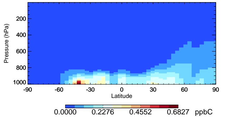
v11-02e-Run0 ALD2 - Species Curtain @ -180.000 for Oct
