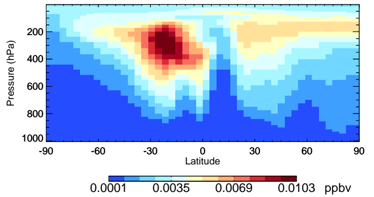
v11-02f-Run1 ASOG3 - Species Curtain @ -180.000 for Oct
