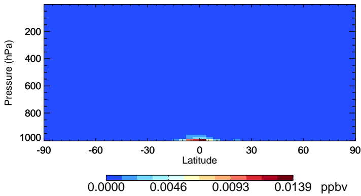
v11-02f-Run1 LIMO - Species Zonal Mean for Oct
