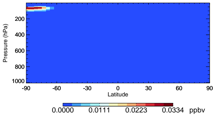
v11-02e-Run0 Cl2O2 - Species Zonal Mean for Oct
