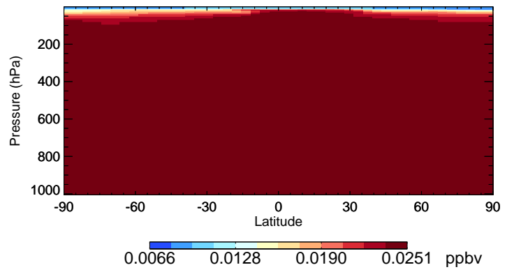
v11-02e-Run0 HCFC142b - Species Curtain @ -180.000 for Oct
