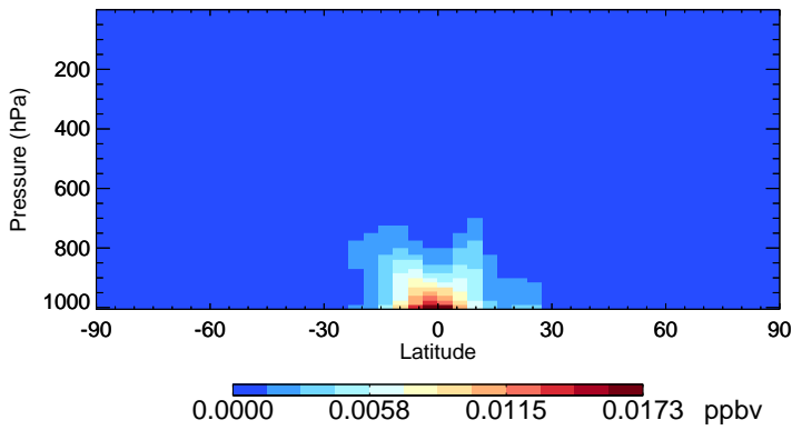
v11-02f-Run1 TSOA1 - Species Zonal Mean for Oct
