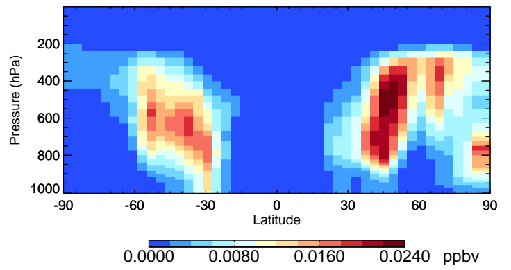
v11-02e-Run1 DST2 - Species Curtain @ -180.000 for Oct
