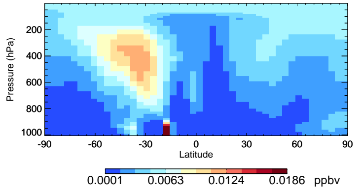
v11-02e-Run1 TSOG3 - Species Curtain @ -180.000 for Oct
