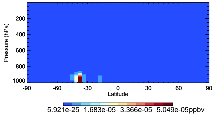
v11-02f-Run1 MACRN - Species Curtain @ -180.000 for Oct
