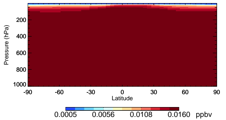
v11-02f-Run1 CFC114 - Species Curtain @ -180.000 for Oct
