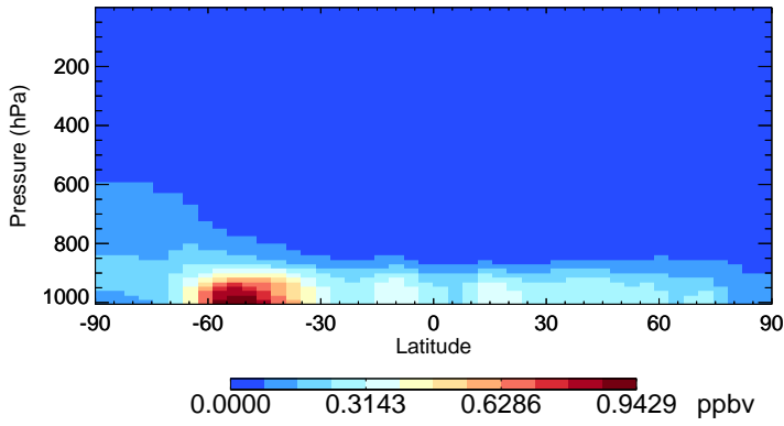
v11-02e-Run1 SALA - Species Zonal Mean for Oct
