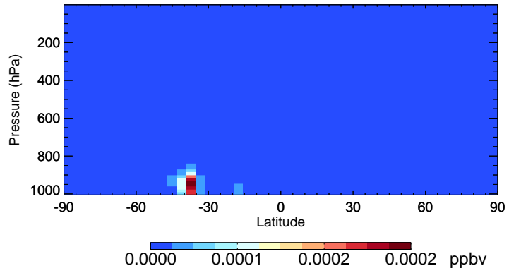
v11-02e-Run1 ISOPNB - Species Curtain @ -180.000 for Oct
