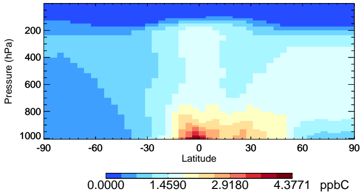
v11-02e-Run1 ACET - Species Zonal Mean for Oct
