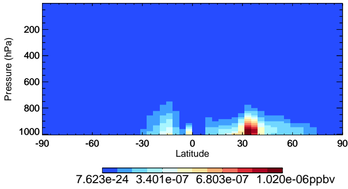
v11-02e-Run1 NPMN - Species Zonal Mean for Oct
