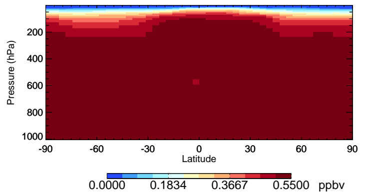
v11-02f-Run1 CH3Cl - Species Curtain @ -180.000 for Oct
